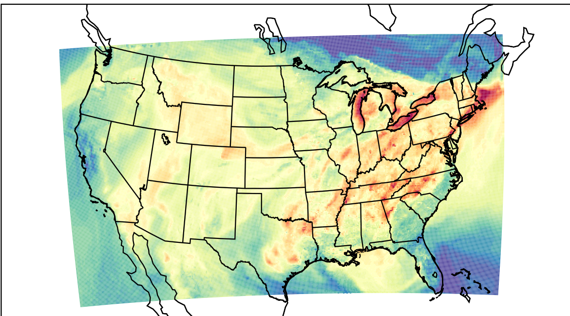
WRF (2022-09-18_23:00:00)
