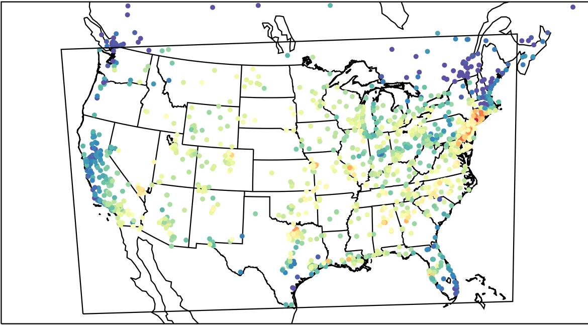
AirNOW (2022-09-19_18:00:00)
