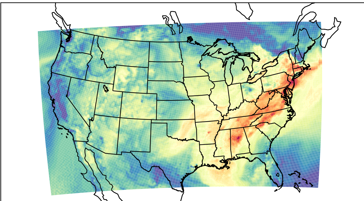
WRF (2022-09-19_16:00:00)
