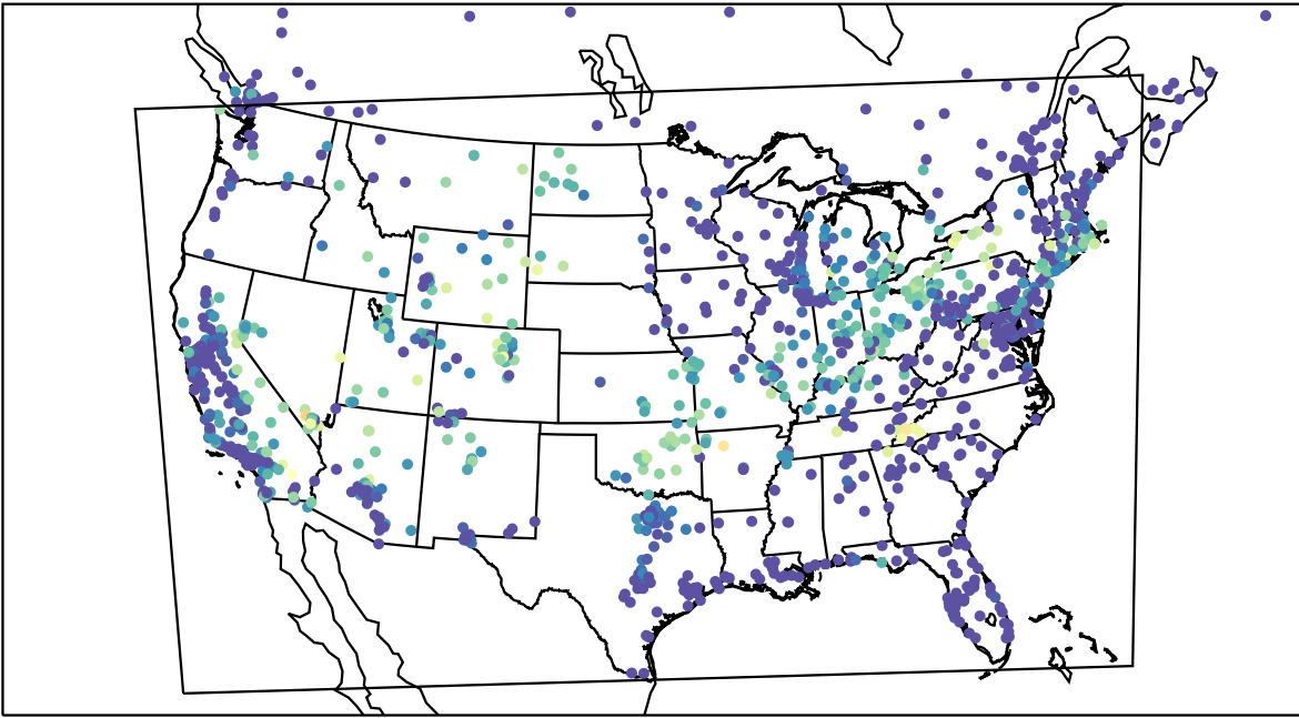
AirNOW (2022-09-19_08:00:00)
