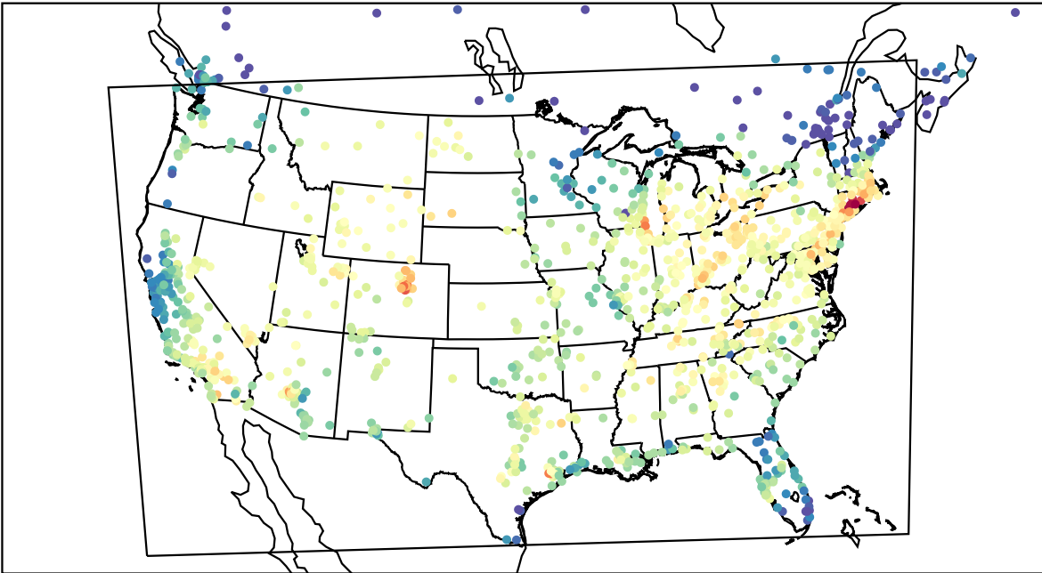
AirNOW (2022-09-18_20:00:00)
