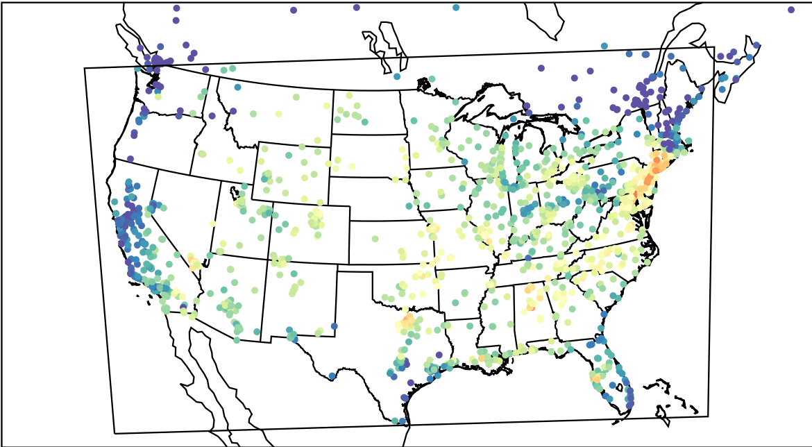
AirNOW (2022-09-19_17:00:00)
