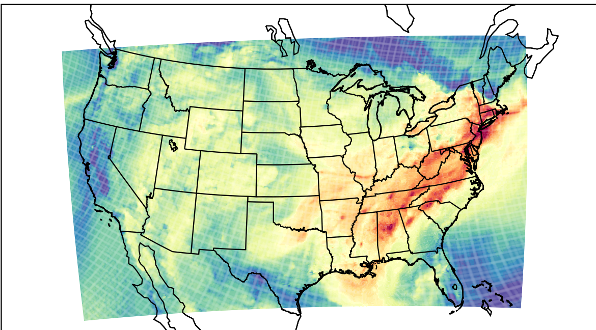
WRF (2022-09-19_17:00:00)
