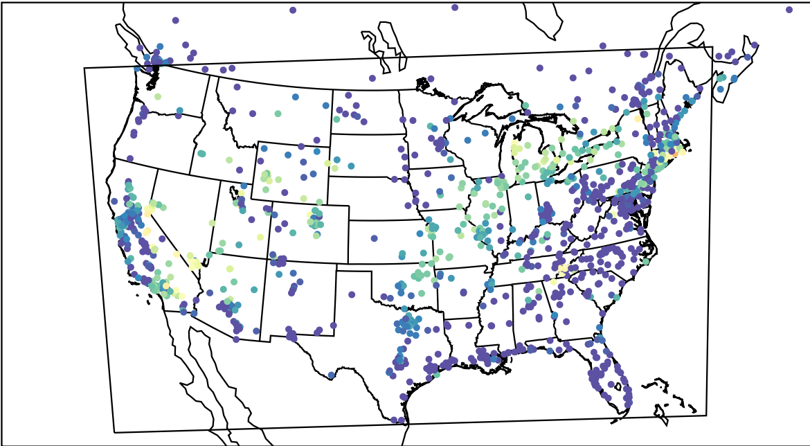
AirNOW (2022-09-18_10:00:00)
