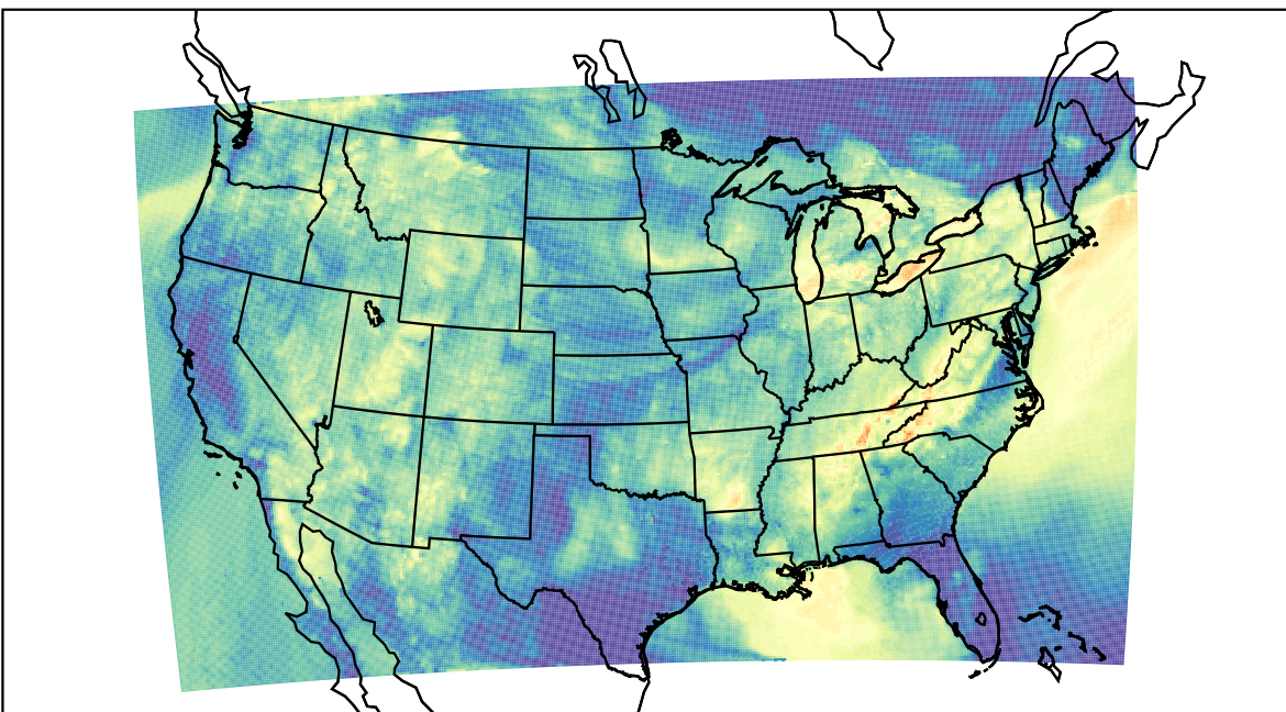
WRF (2022-09-19_08:00:00)
