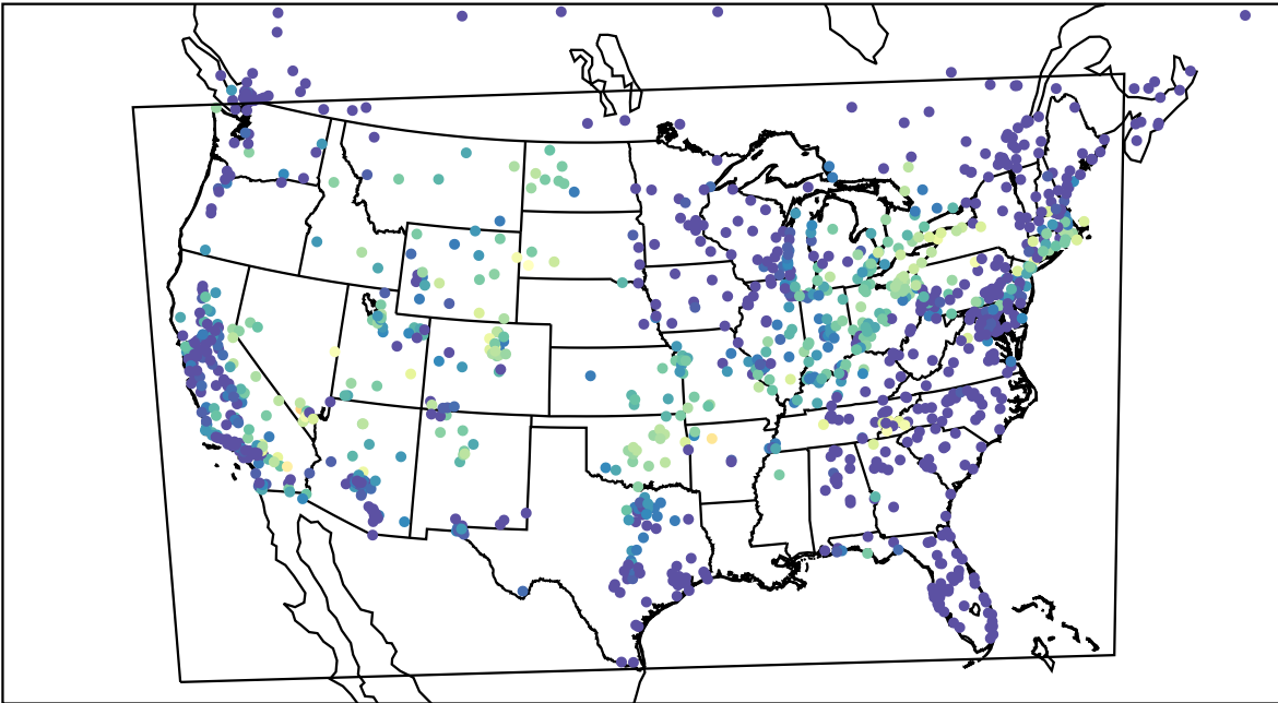
AirNOW (2022-09-19_07:00:00)
