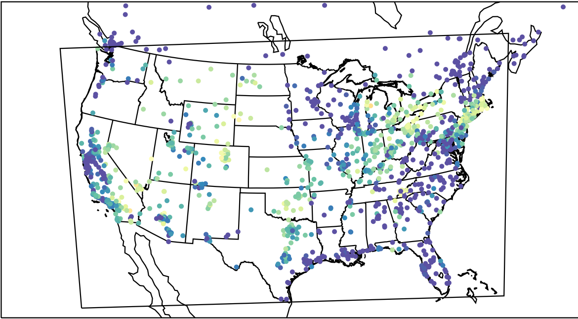
AirNOW (2022-09-19_04:00:00)
