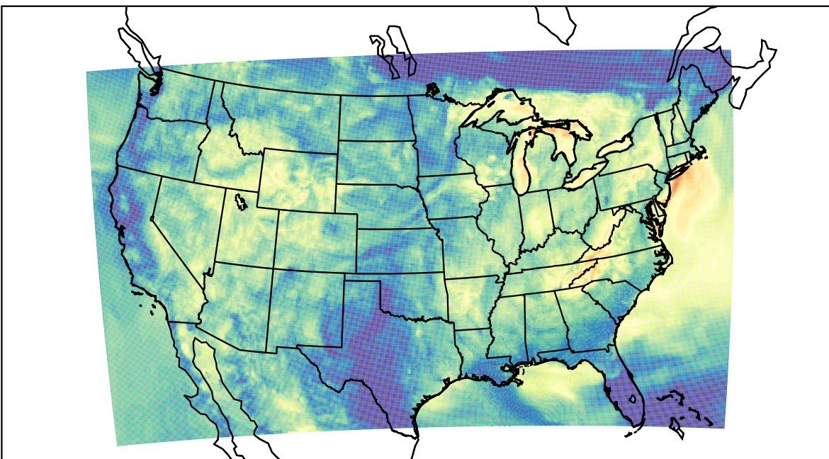
WRF (2022-09-18_08:00:00)
