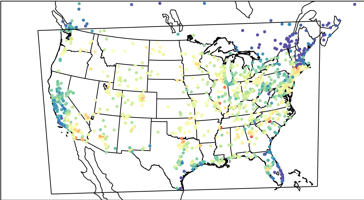
AirNOW (2022-09-19_21:00:00)
