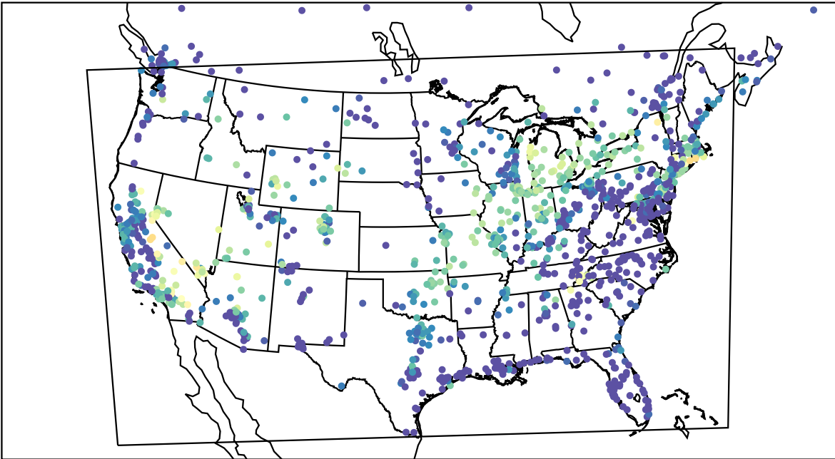
AirNOW (2022-09-18_09:00:00)
