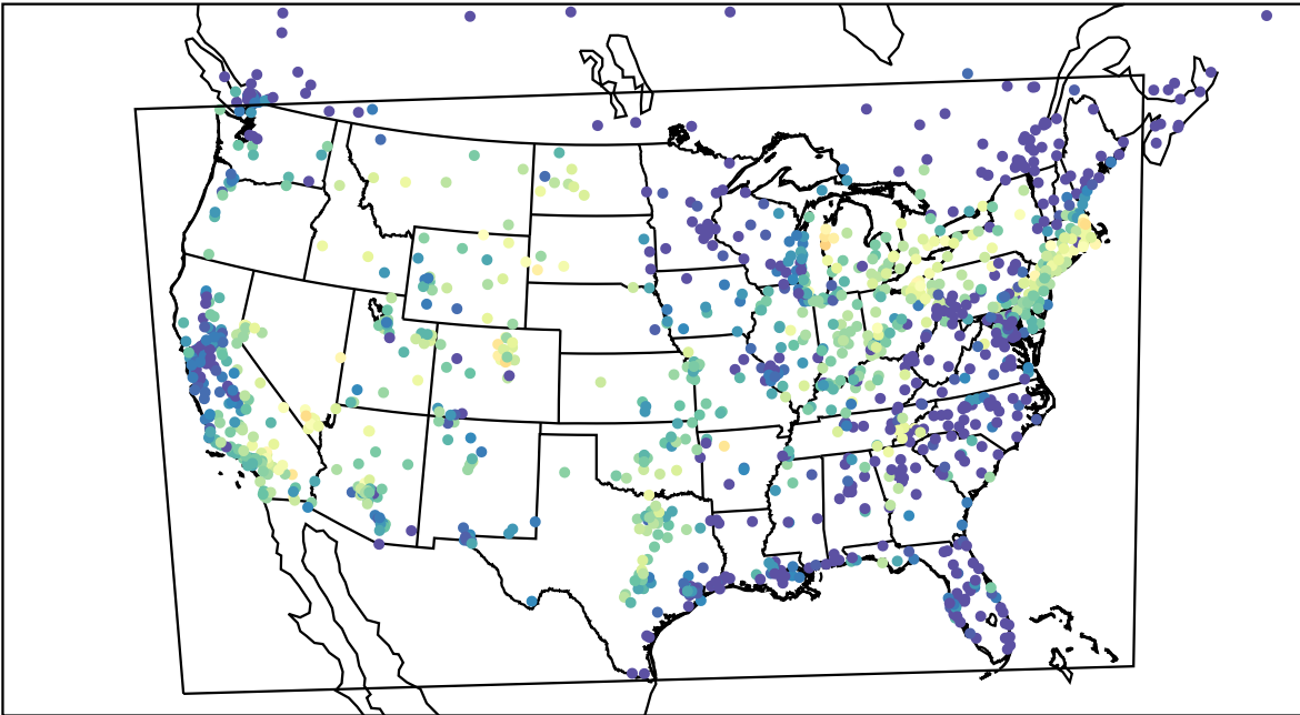
AirNOW (2022-09-19_02:00:00)
