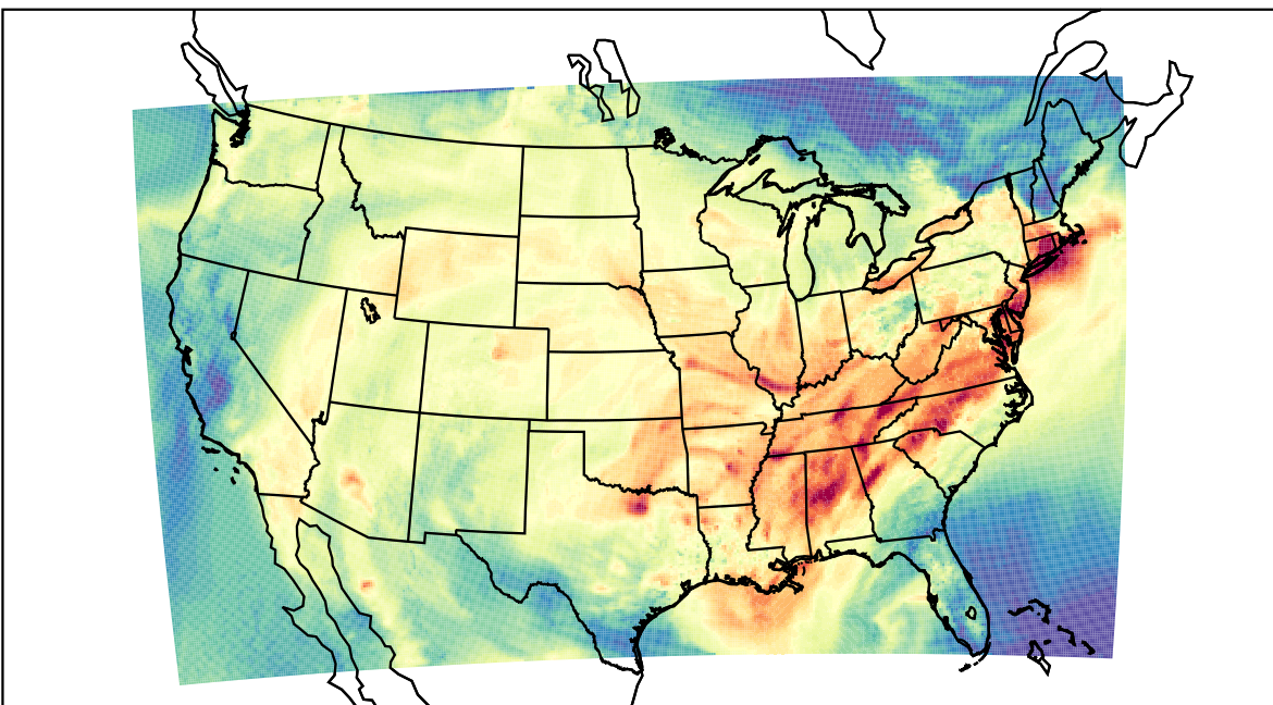
WRF (2022-09-19_21:00:00)
