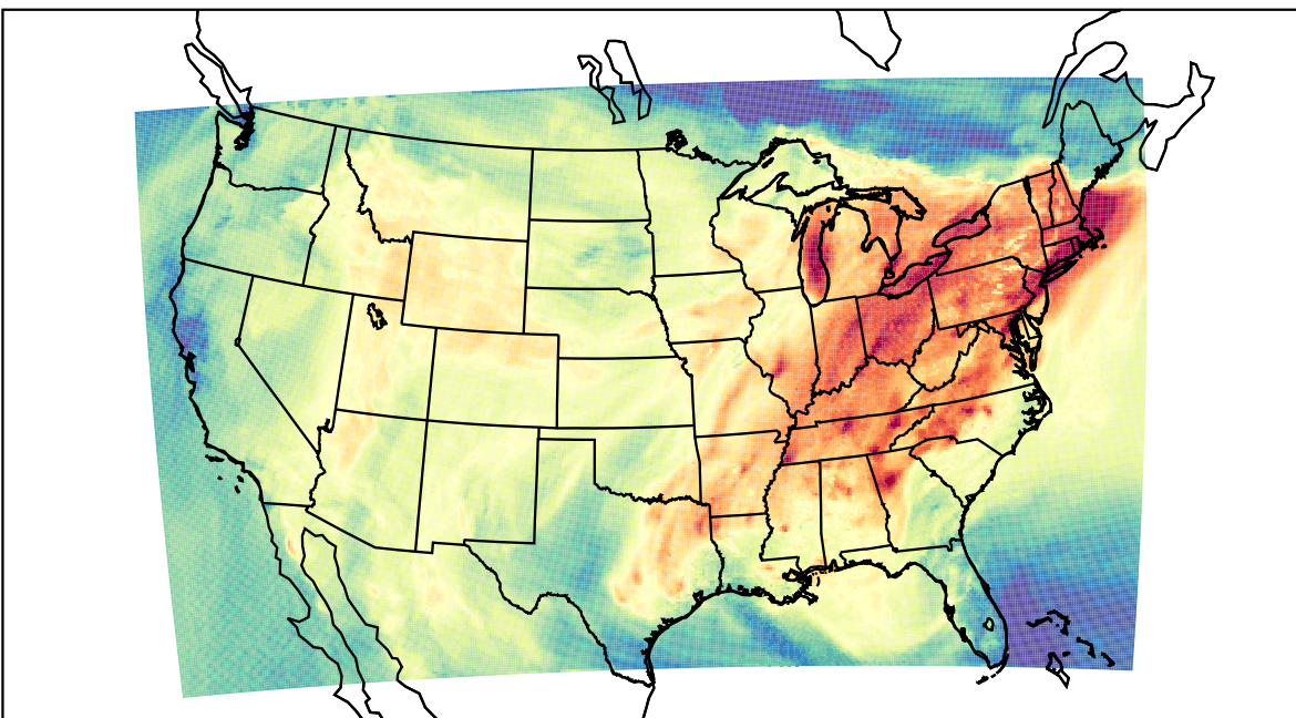
WRF (2022-09-18_19:00:00)
