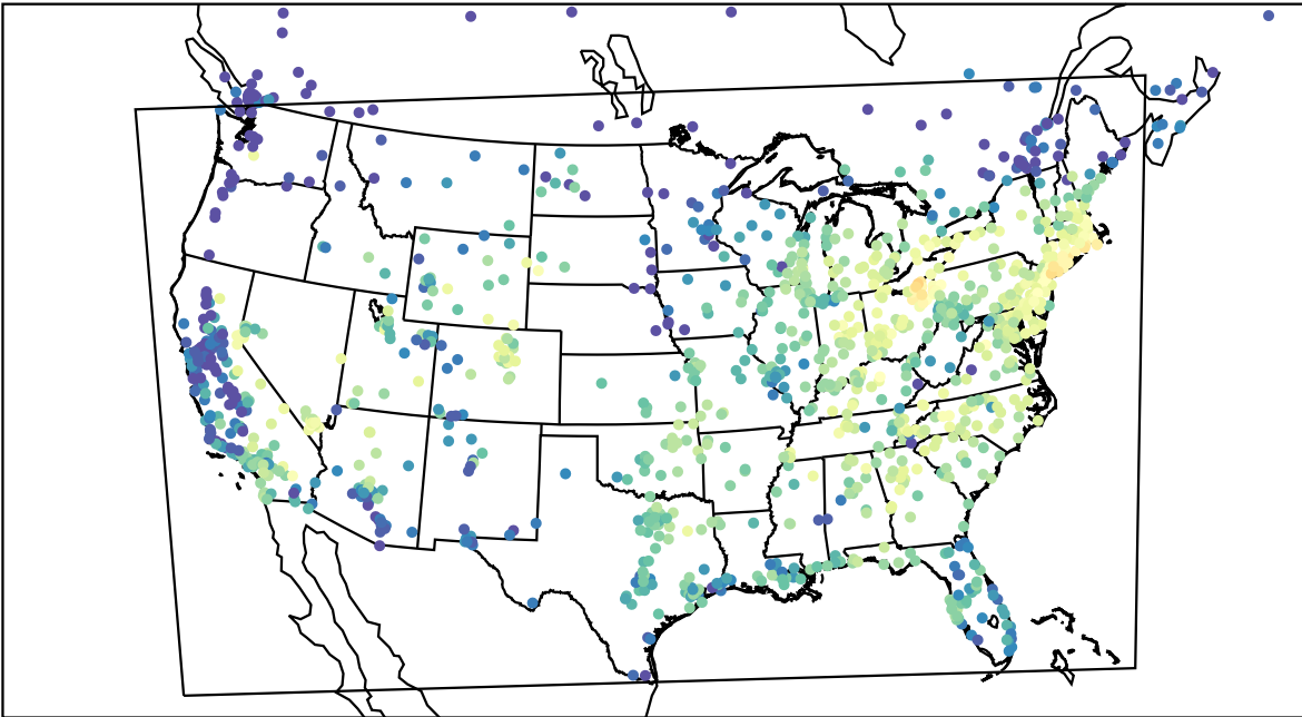
AirNOW (2022-09-18_15:00:00)
