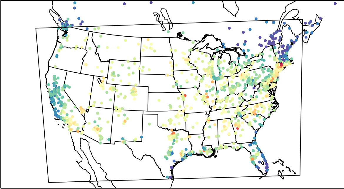
AirNOW (2022-09-19_20:00:00)
