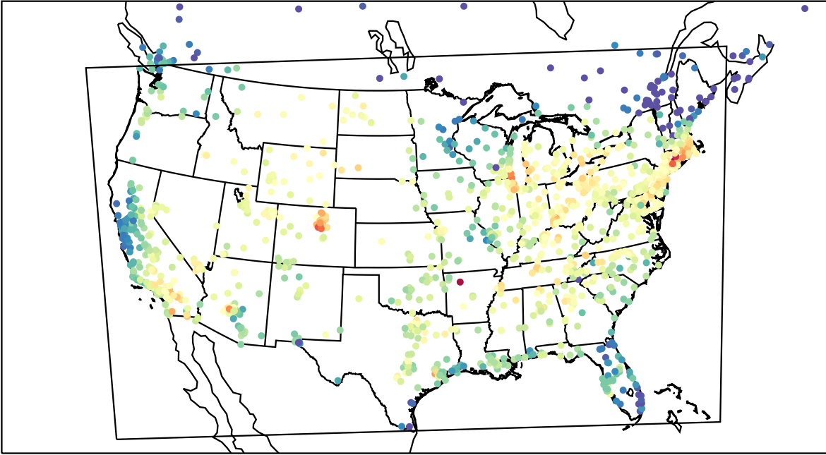
AirNOW (2022-09-18_21:00:00)
