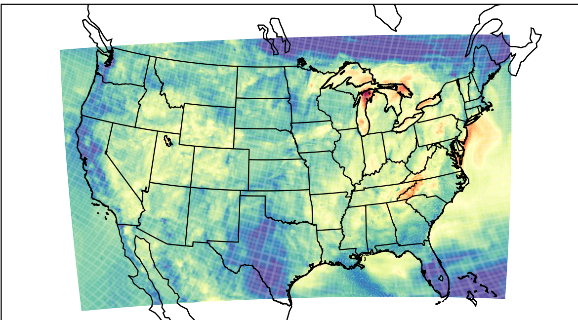
WRF (2022-09-18_05:00:00)
