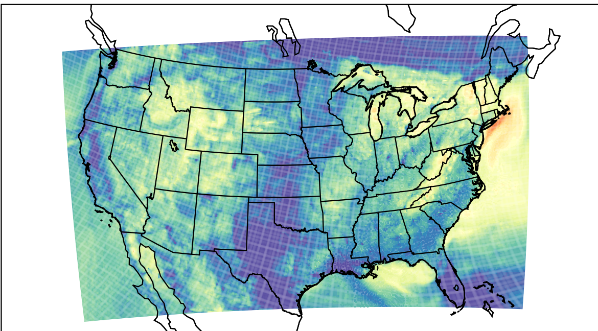
WRF (2022-09-18_13:00:00)
