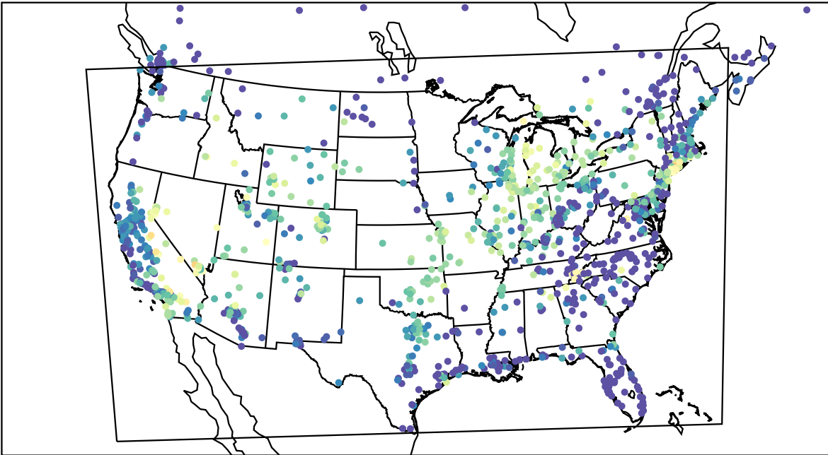
AirNOW (2022-09-18_06:00:00)
