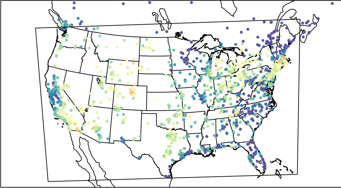
AirNOW (2022-09-19_00:00:00)
