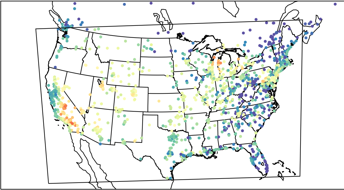
AirNOW (2022-09-18_00:00:00)
