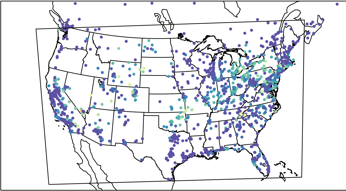
AirNOW (2022-09-19_13:00:00)
