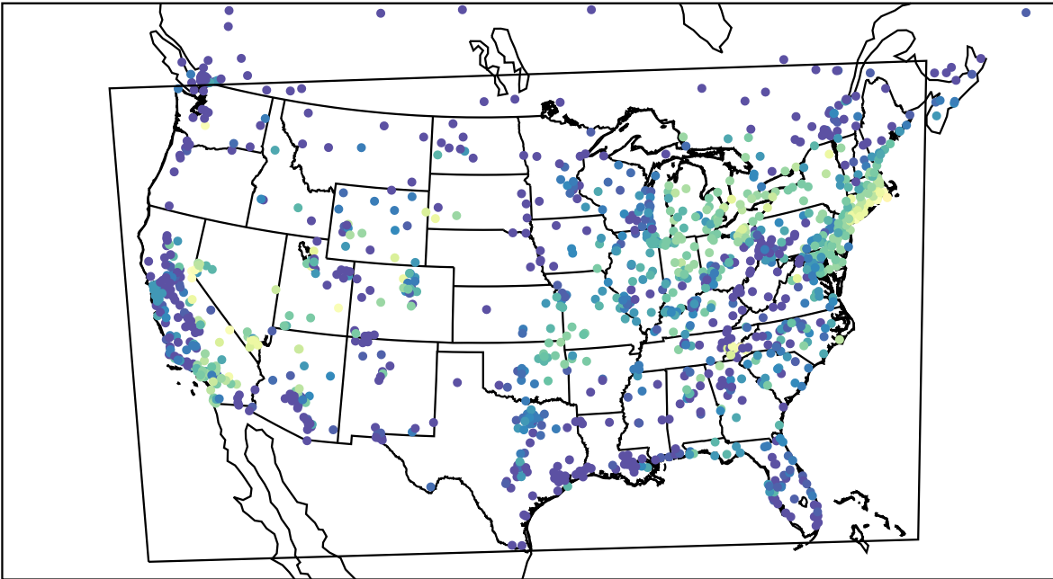
AirNOW (2022-09-18_13:00:00)
