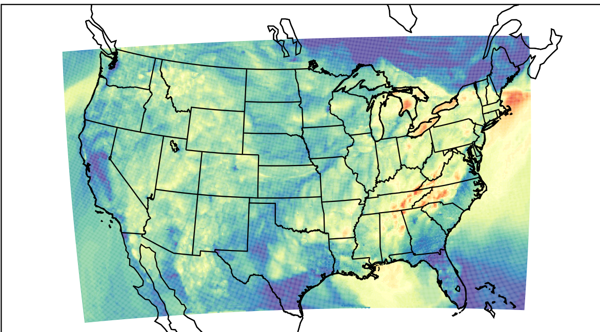
WRF (2022-09-19_04:00:00)
