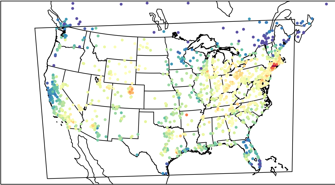
AirNOW (2022-09-18_19:00:00)
