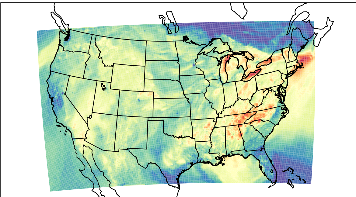
WRF (2022-09-19_01:00:00)
