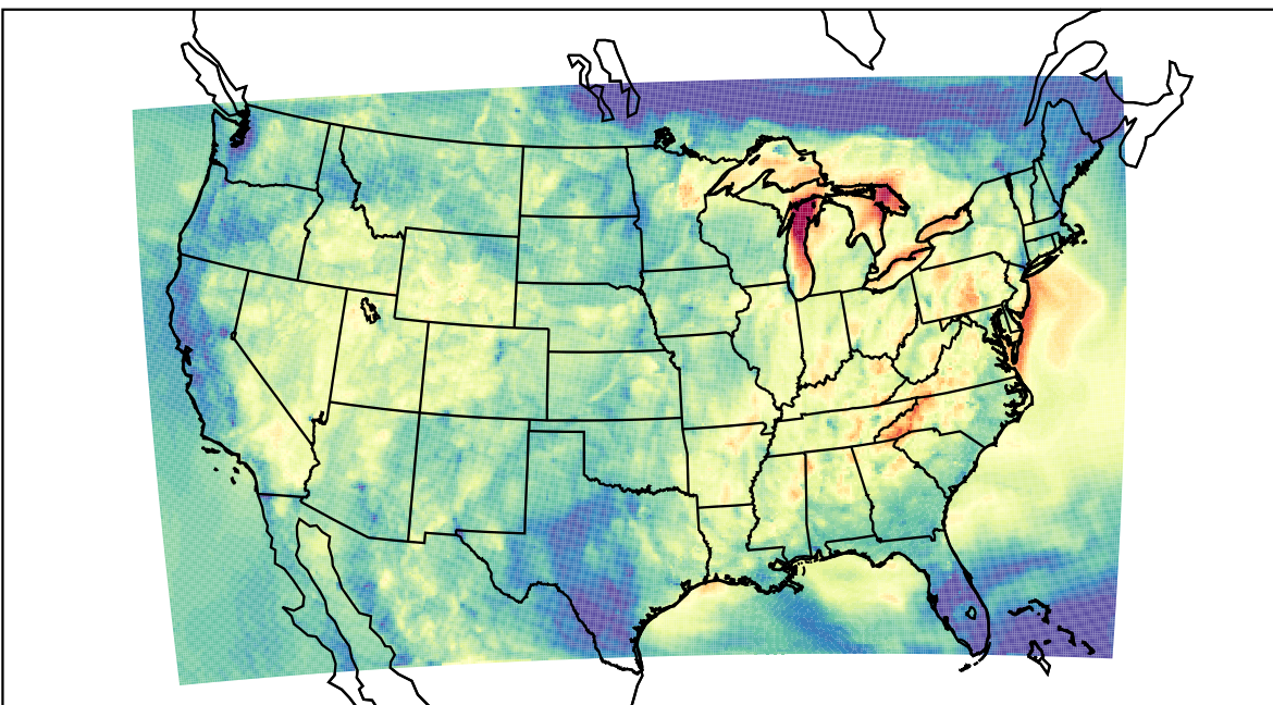
WRF (2022-09-18_03:00:00)
