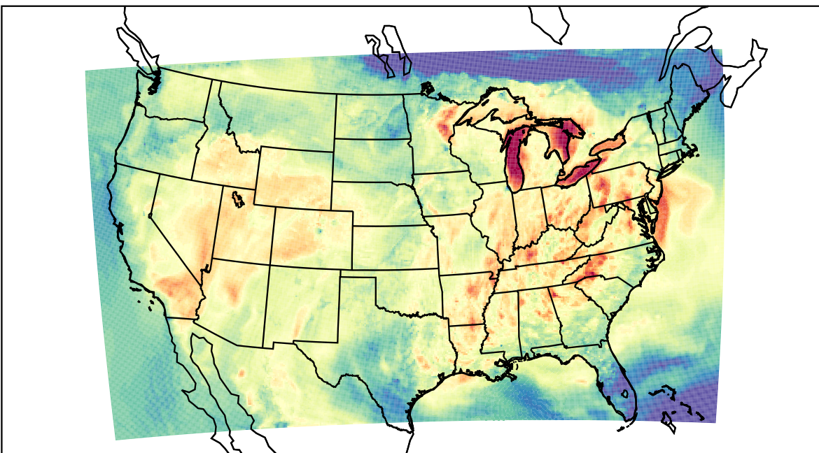
WRF (2022-09-18_00:00:00)
