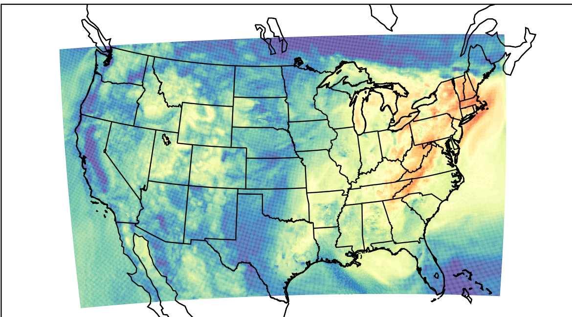
WRF (2022-09-18_15:00:00)
