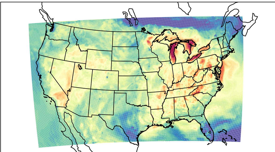
WRF (2022-09-18_01:00:00)
