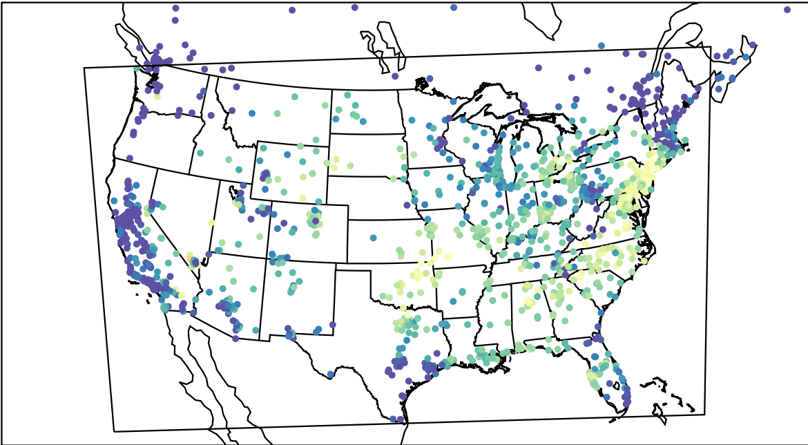
AirNOW (2022-09-19_15:00:00)
