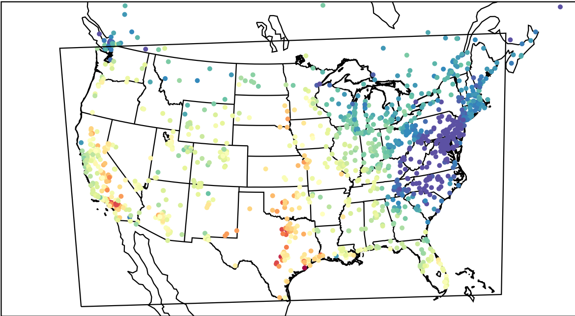
AirNOW (2022-10-02_21:00:00)
