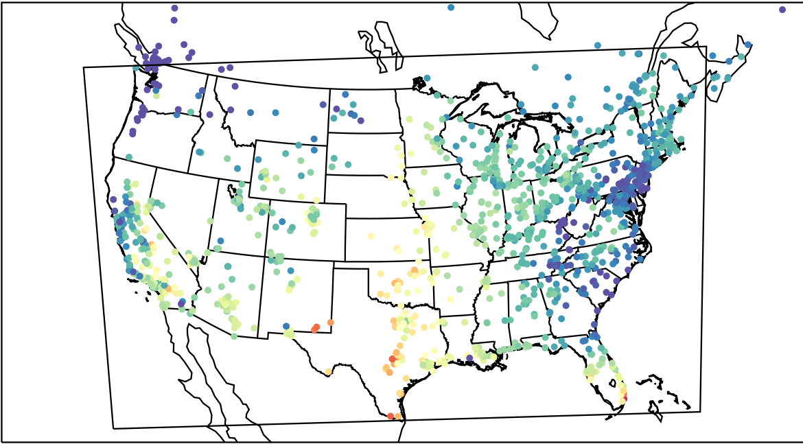
AirNOW (2022-10-03_17:00:00)
