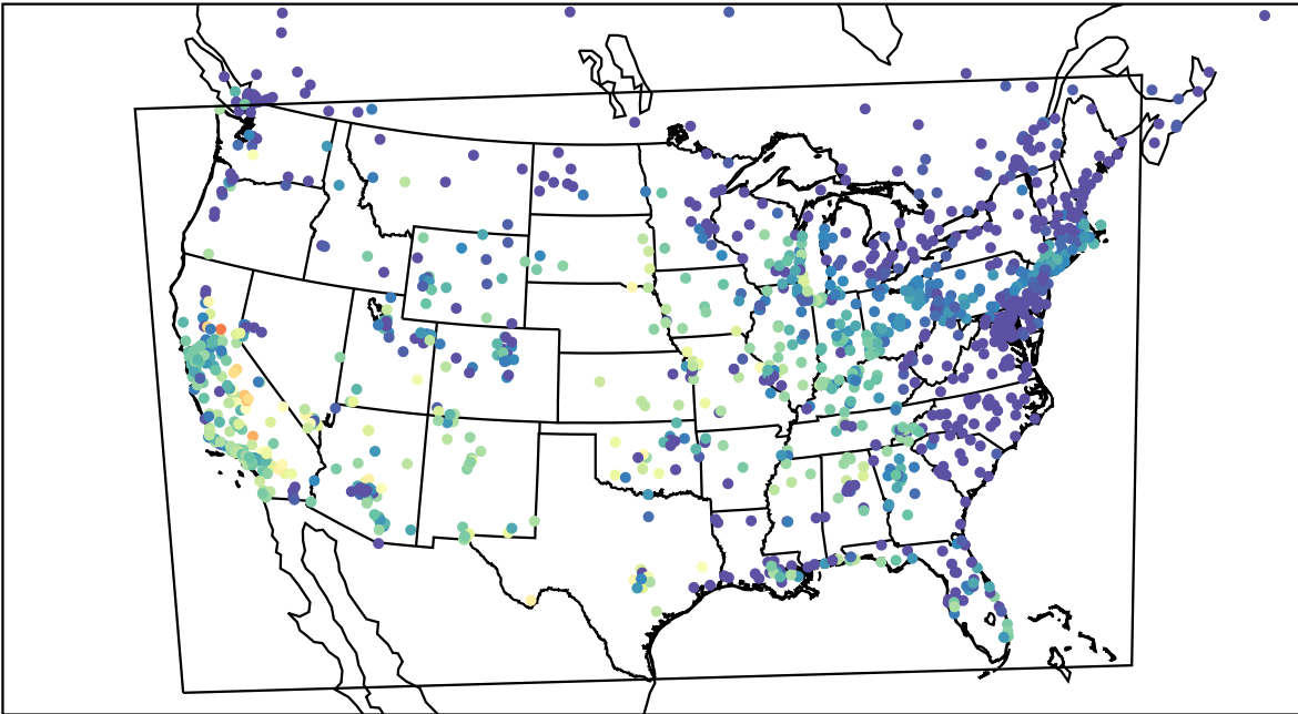
AirNOW (2022-10-02_04:00:00)
