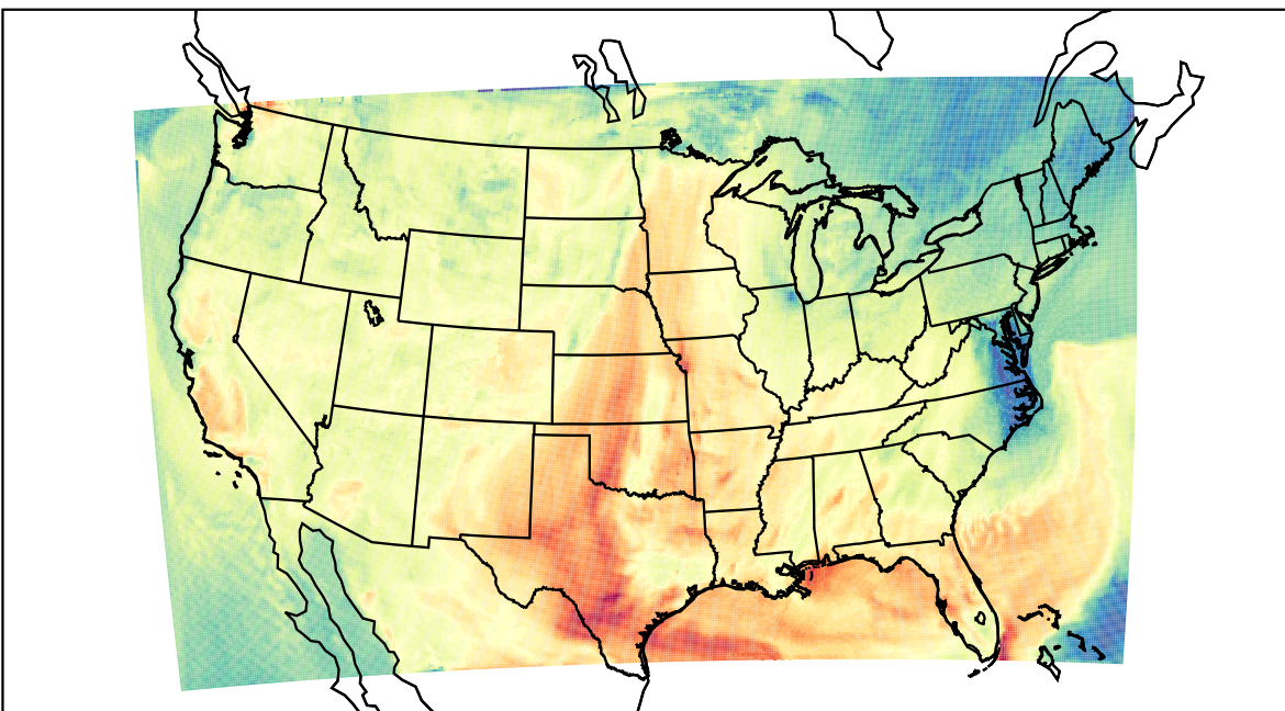
WRF (2022-10-03_20:00:00)
