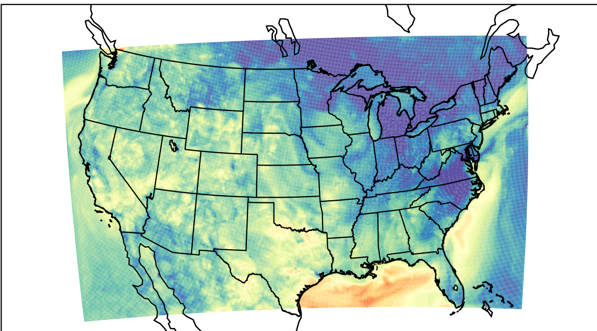
WRF (2022-10-02_07:00:00)
