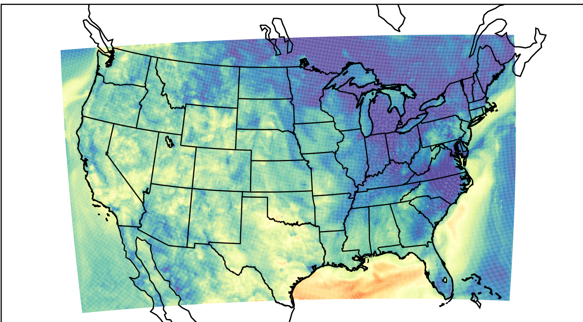
WRF (2022-10-02_09:00:00)
