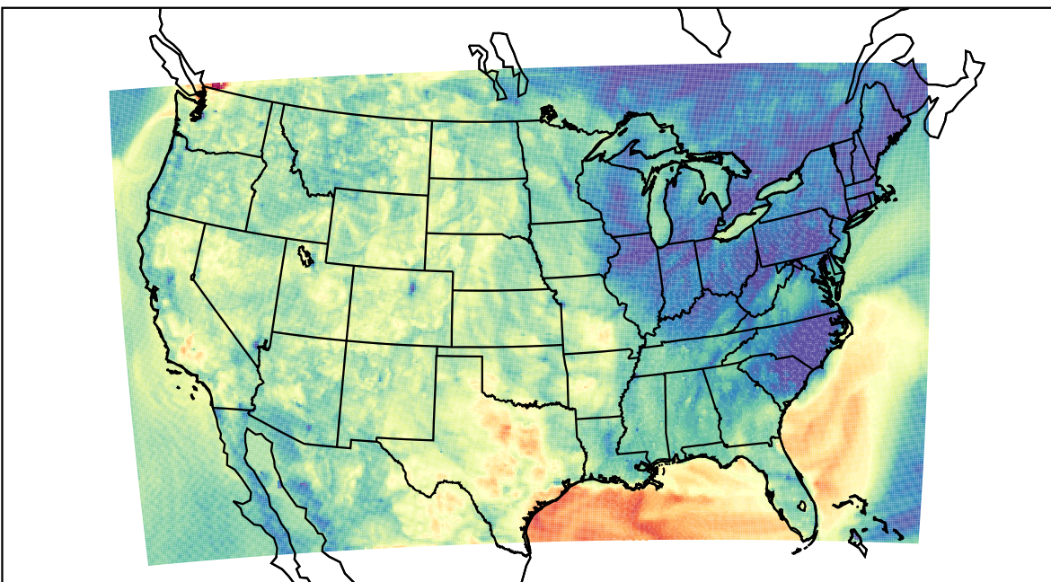
WRF (2022-10-03_04:00:00)
