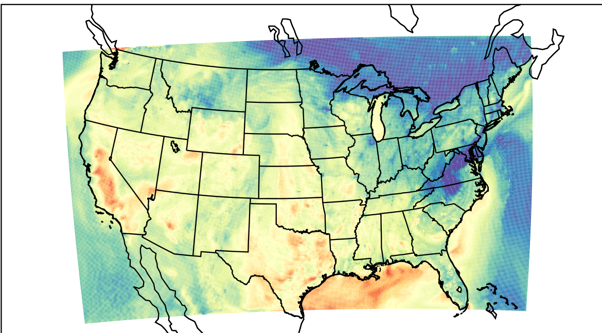
WRF (2022-10-02_00:00:00)
