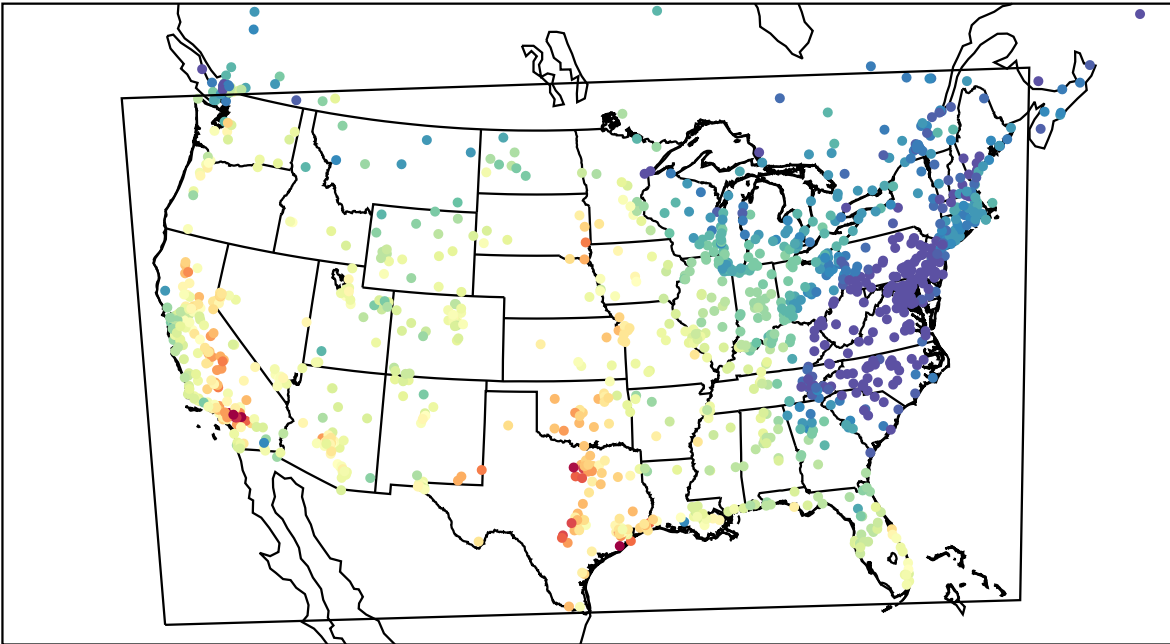
AirNOW (2022-10-02_22:00:00)
