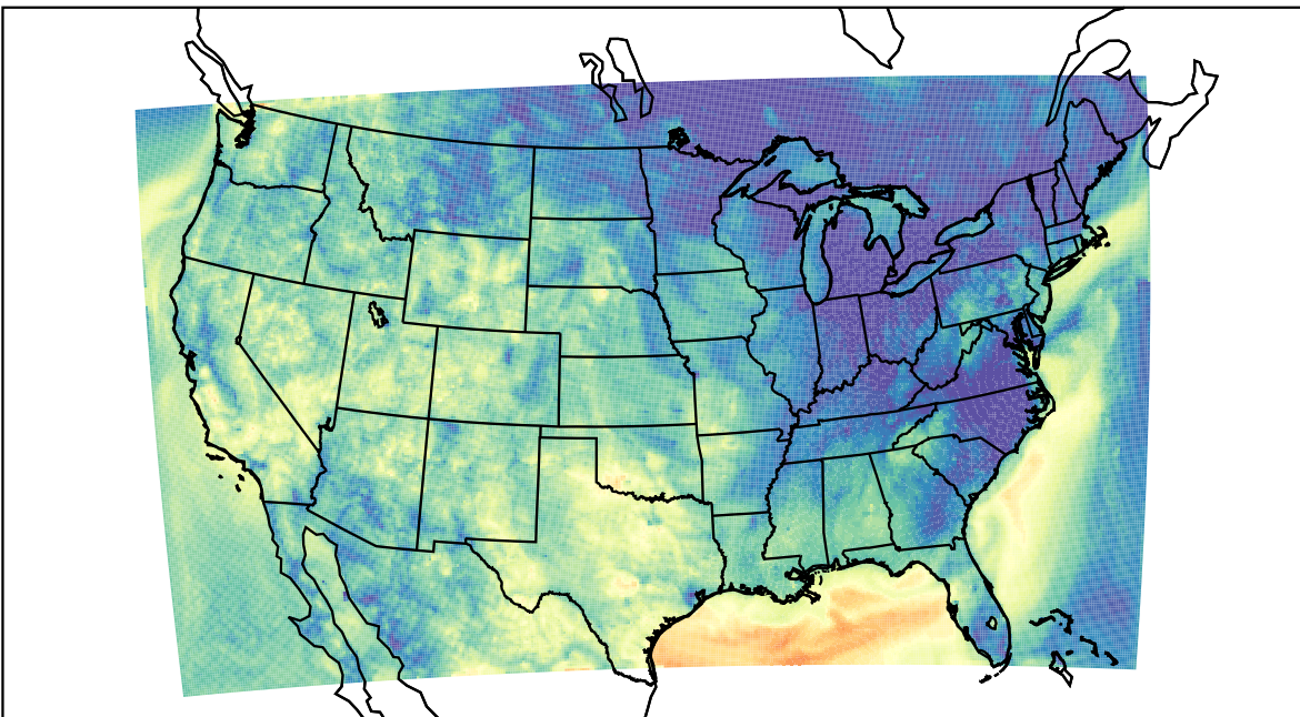
WRF (2022-10-02_10:00:00)
