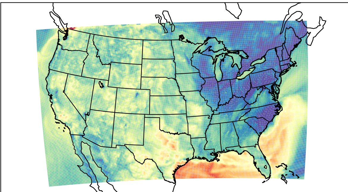
WRF (2022-10-03_05:00:00)
