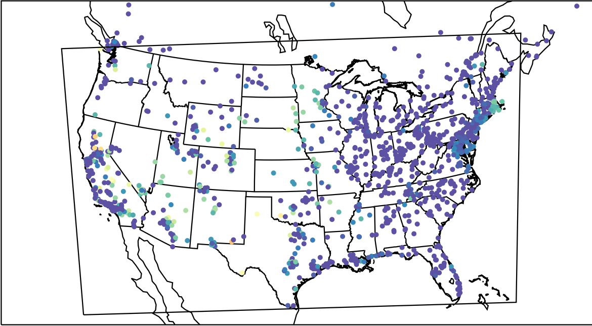
AirNOW (2022-10-03_11:00:00)
