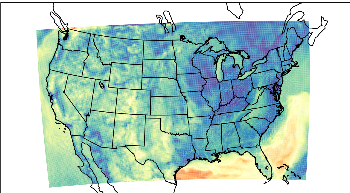
WRF (2022-10-03_14:00:00)
