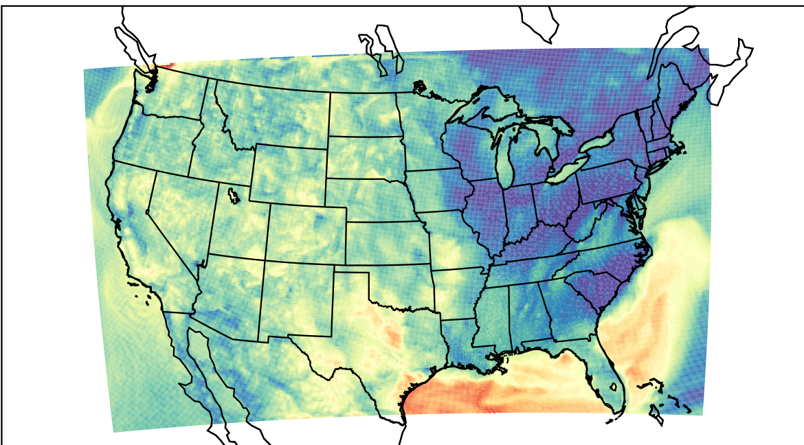
WRF (2022-10-03_07:00:00)
