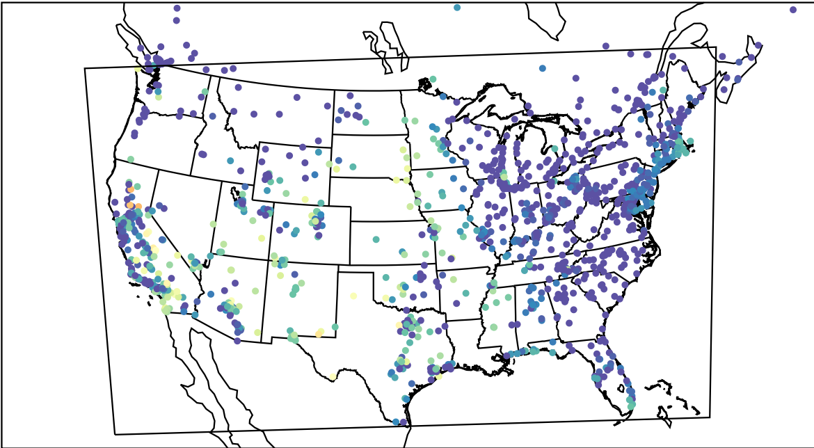
AirNOW (2022-10-03_07:00:00)
