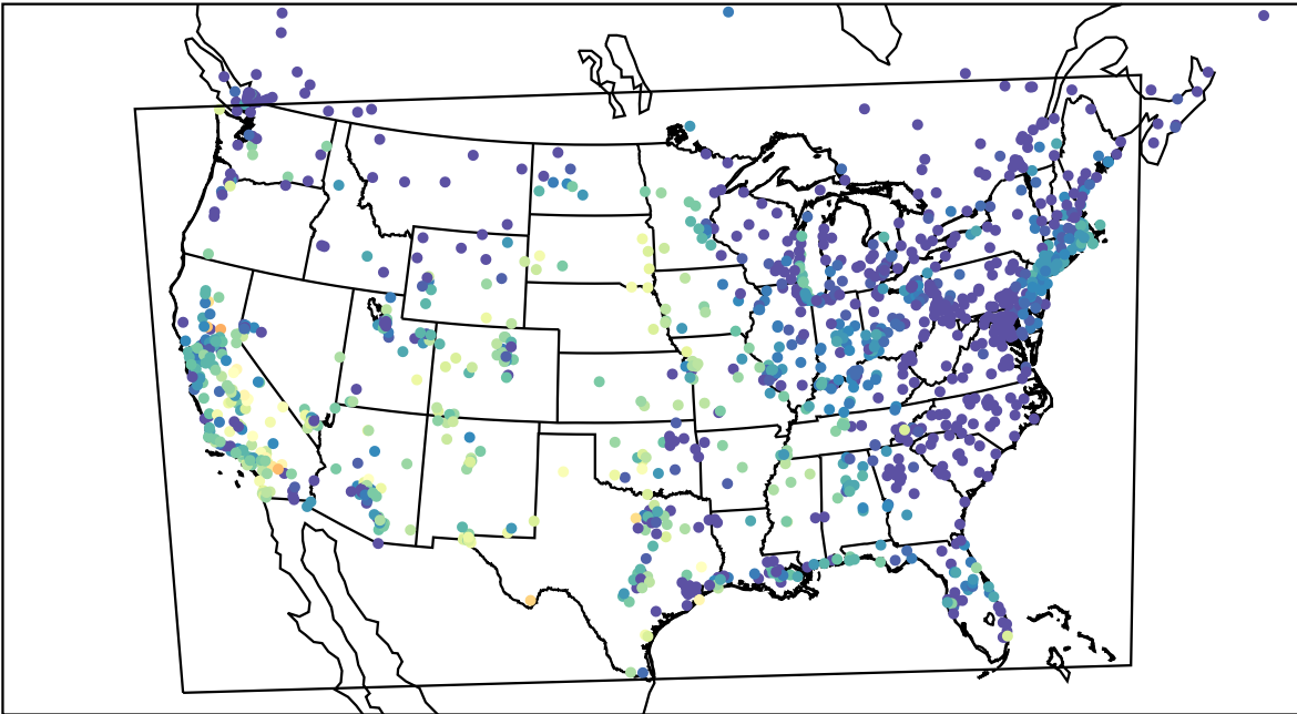
AirNOW (2022-10-03_04:00:00)
