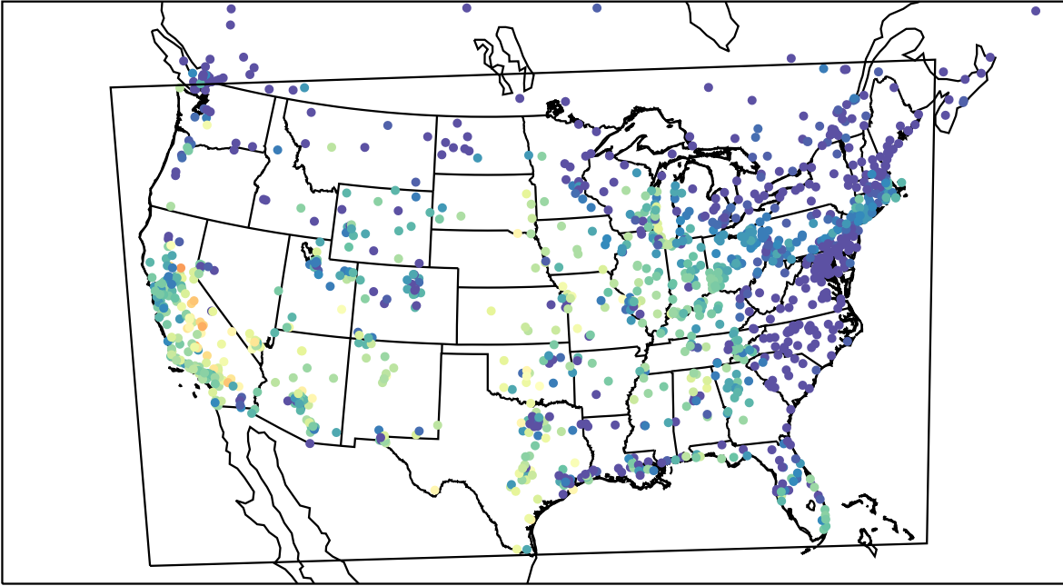
AirNOW (2022-10-02_03:00:00)
