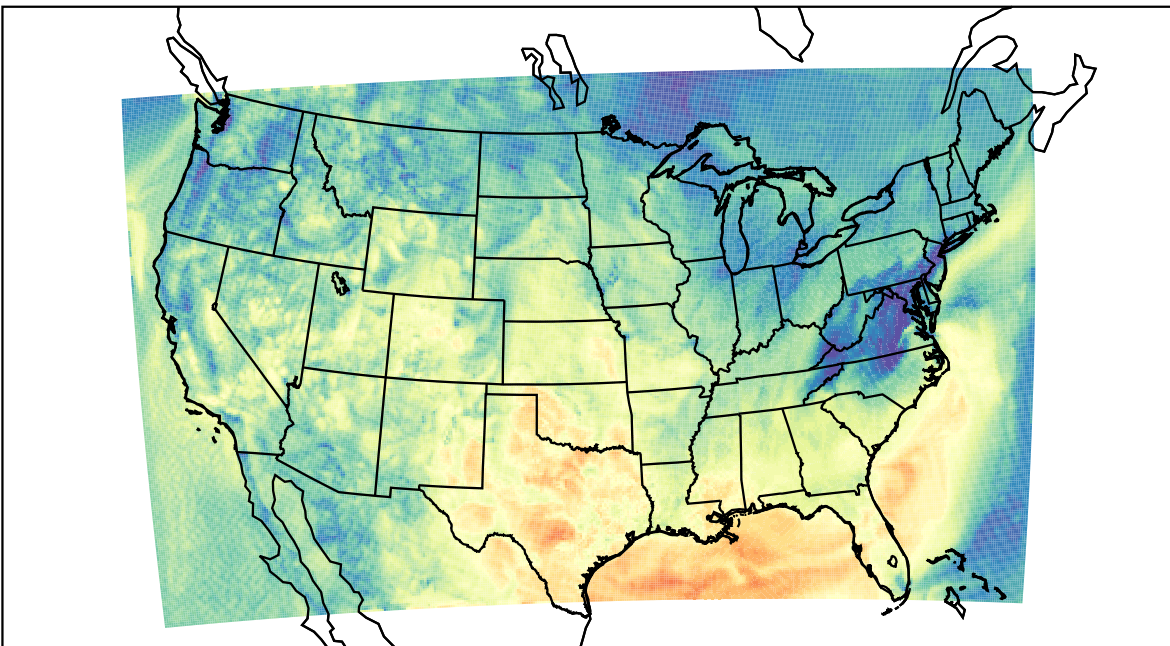
WRF (2022-10-02_16:00:00)
