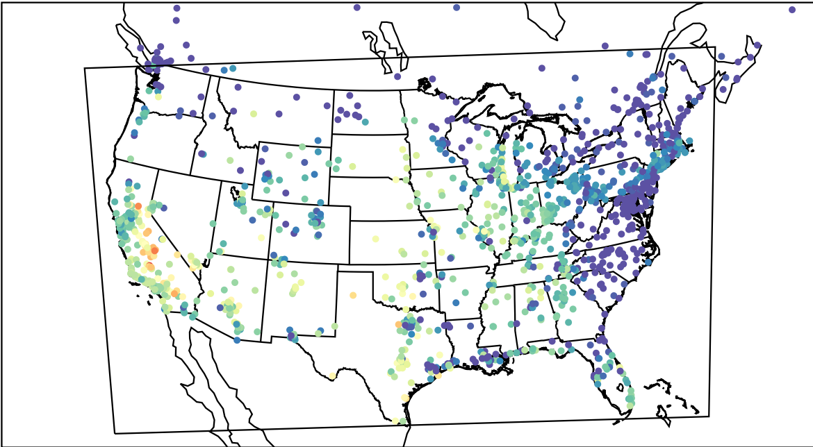
AirNOW (2022-10-02_02:00:00)
