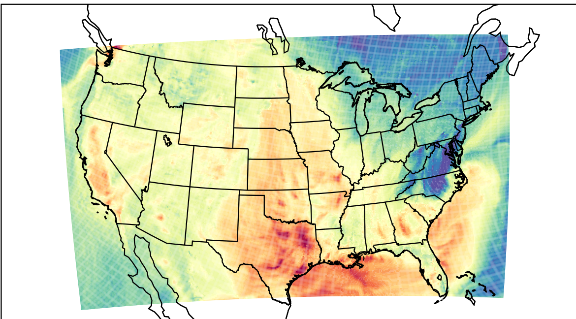
WRF (2022-10-02_22:00:00)
