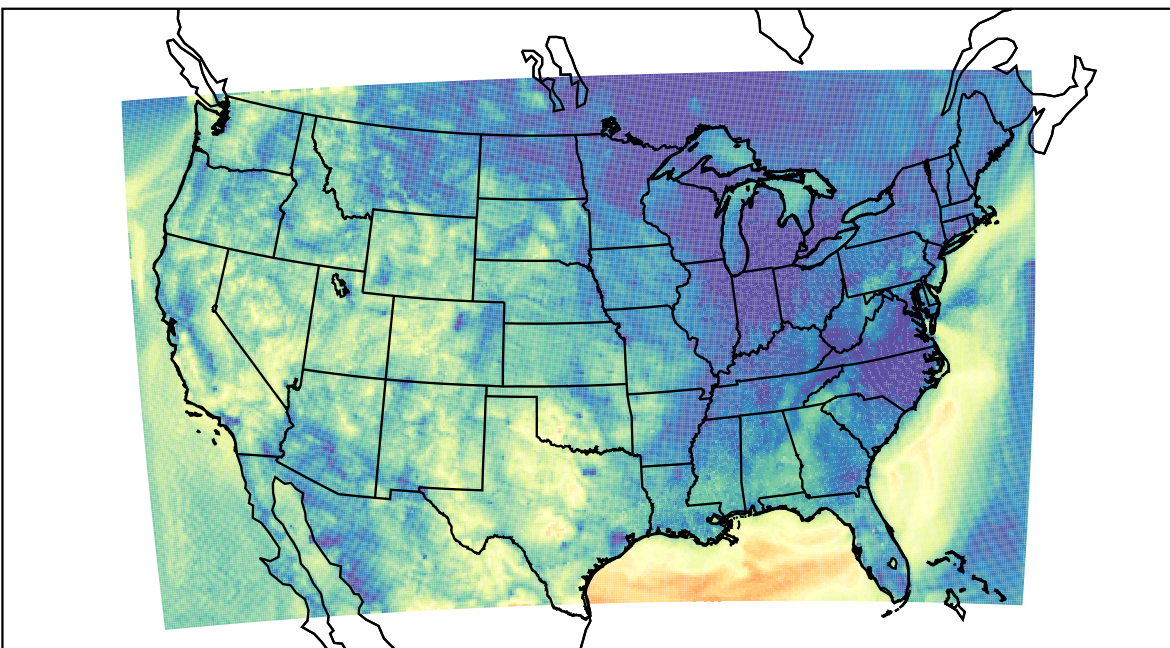
WRF (2022-10-02_13:00:00)
