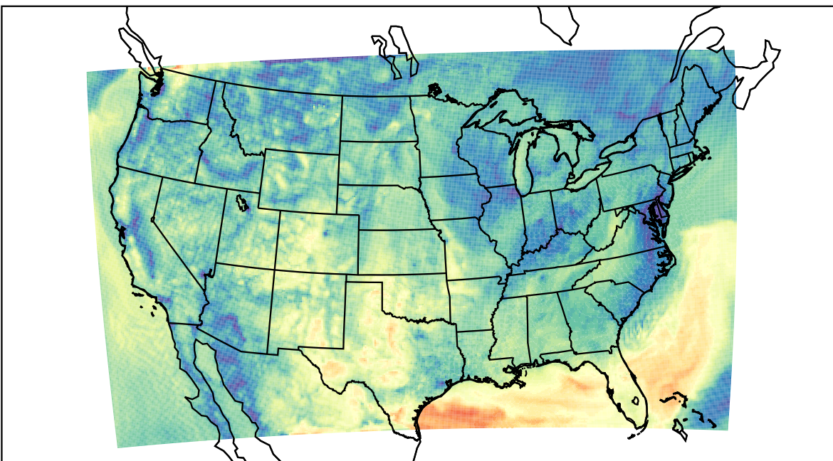
WRF (2022-10-03_15:00:00)
