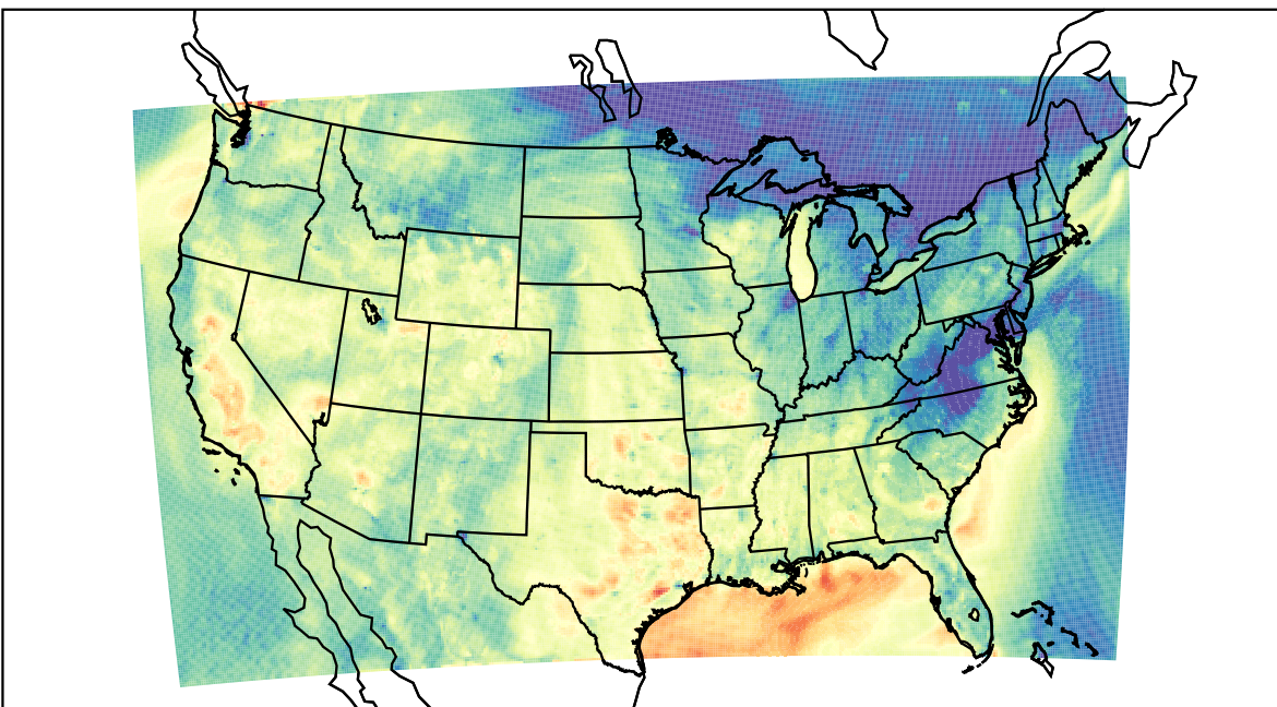
WRF (2022-10-02_01:00:00)
