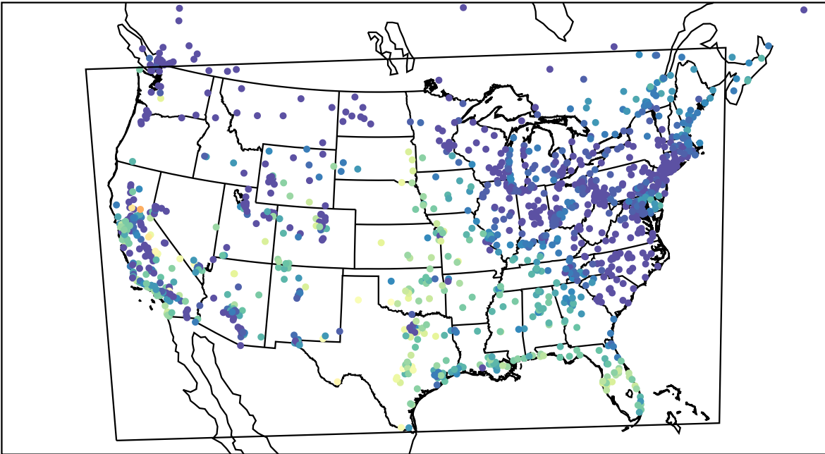
AirNOW (2022-10-02_14:00:00)
