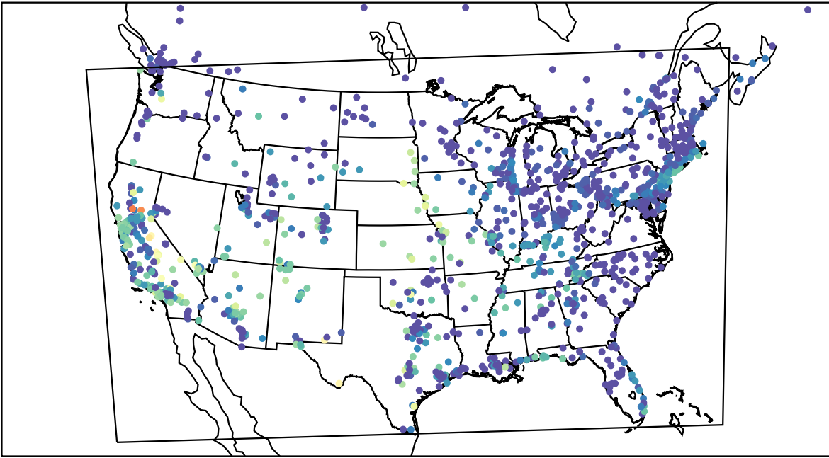
AirNOW (2022-10-02_09:00:00)
