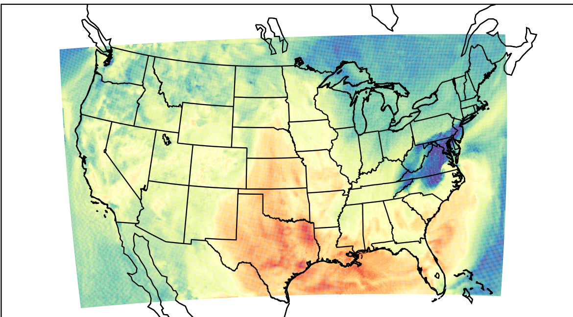
WRF (2022-10-02_18:00:00)
