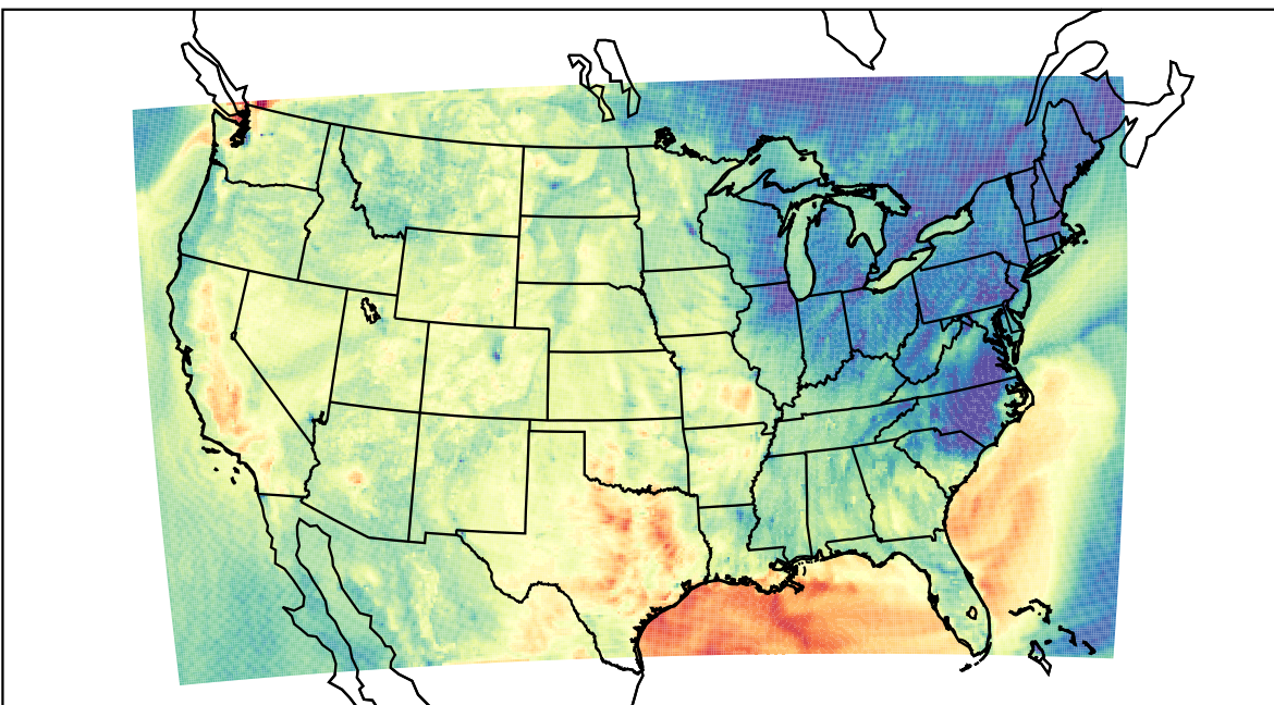
WRF (2022-10-03_01:00:00)
