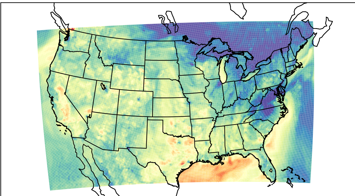
WRF (2022-10-02_02:00:00)
