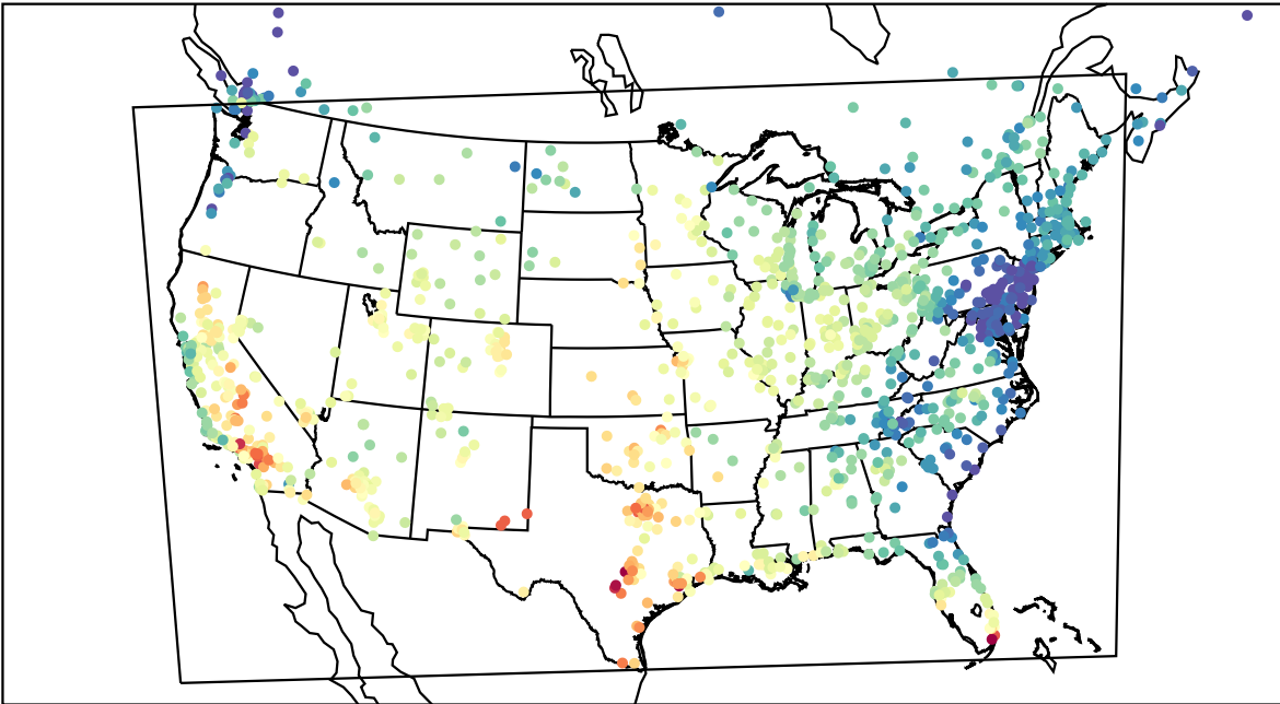
AirNOW (2022-10-03_20:00:00)
