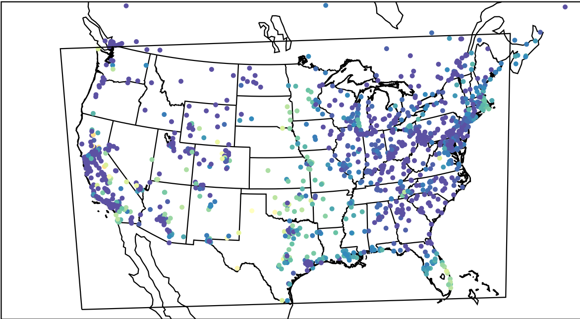
AirNOW (2022-10-03_14:00:00)
