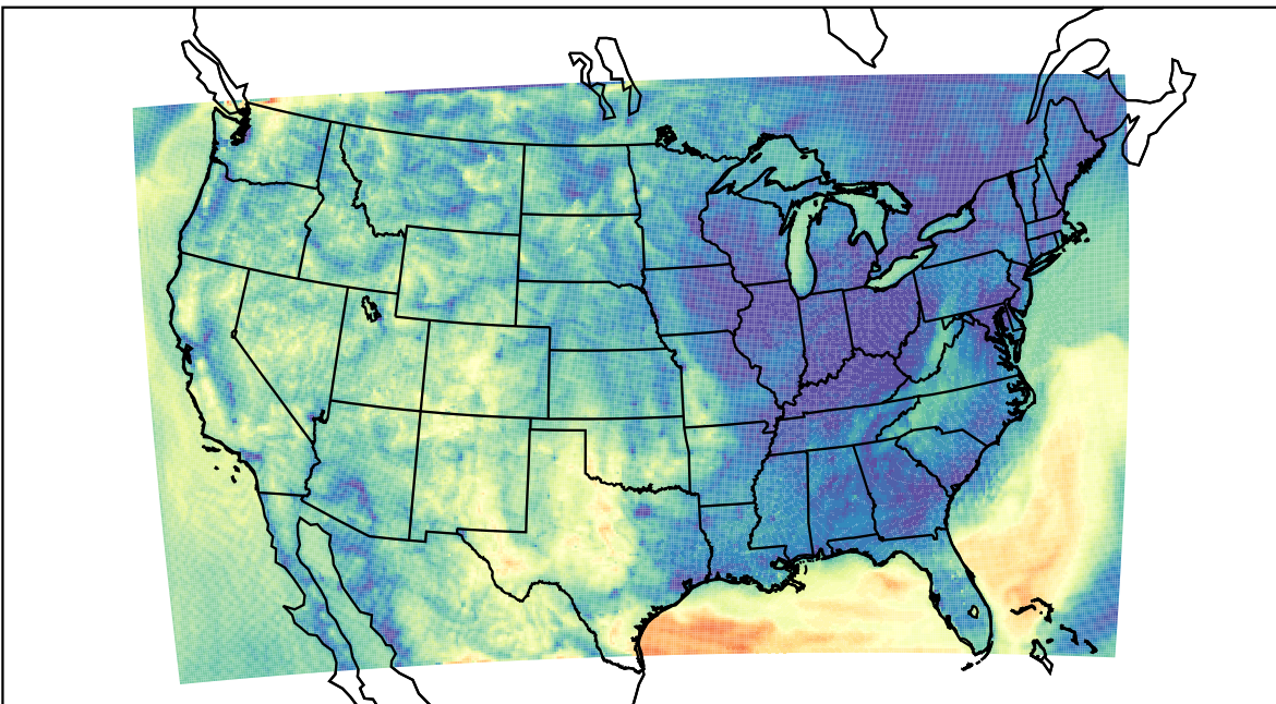
WRF (2022-10-03_13:00:00)
