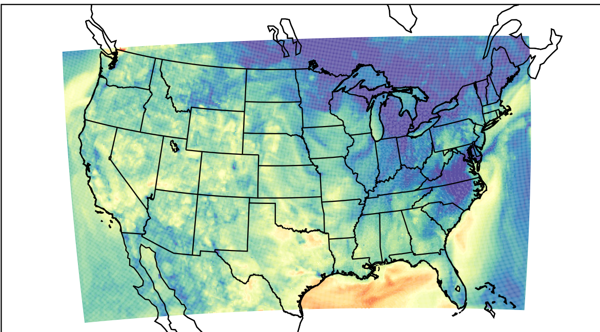
WRF (2022-10-02_06:00:00)
