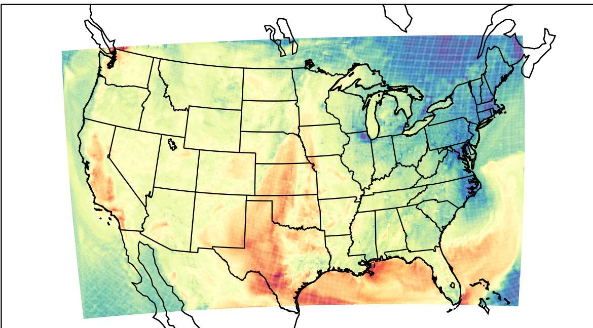
WRF (2022-10-03_23:00:00)
