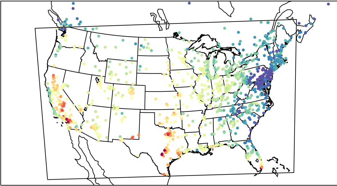
AirNOW (2022-10-03_21:00:00)
