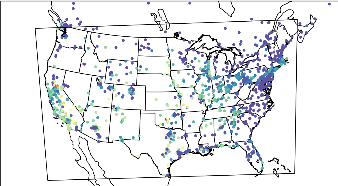
AirNOW (2022-10-02_05:00:00)
