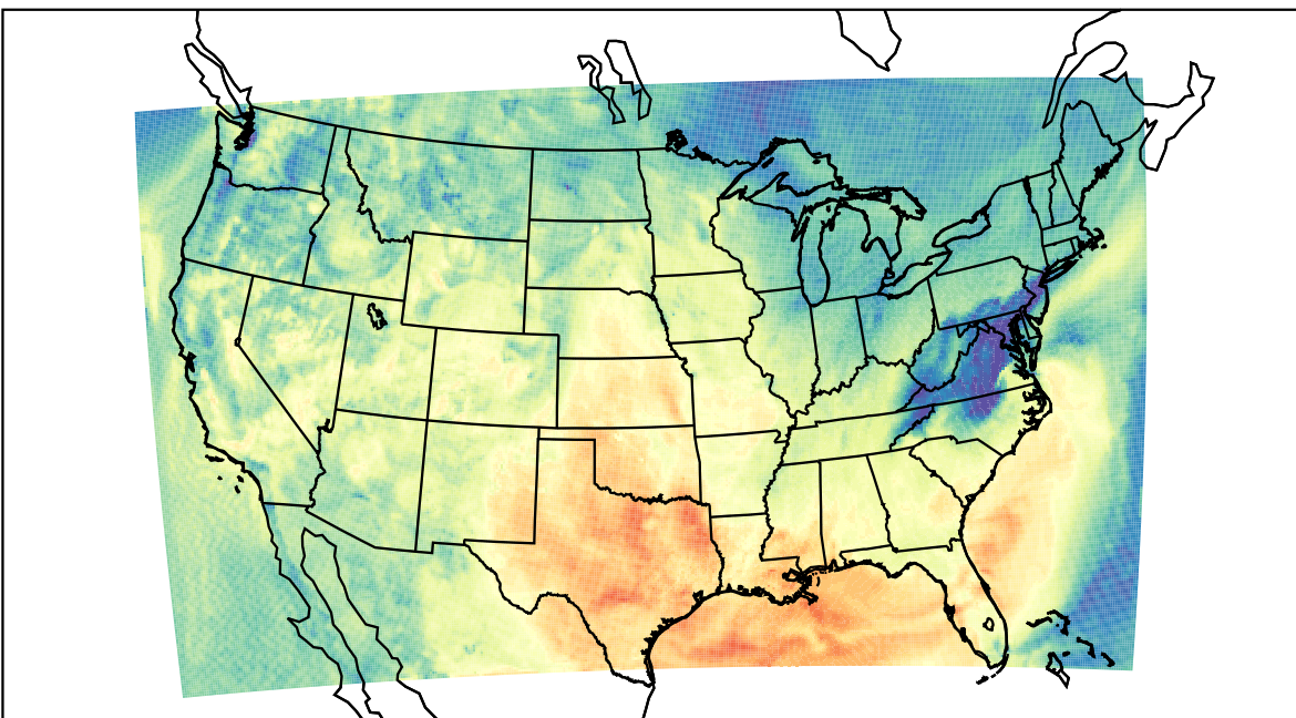
WRF (2022-10-02_17:00:00)
