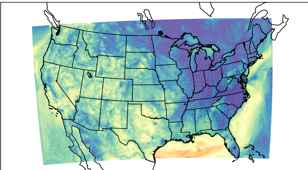
WRF (2022-10-02_12:00:00)
