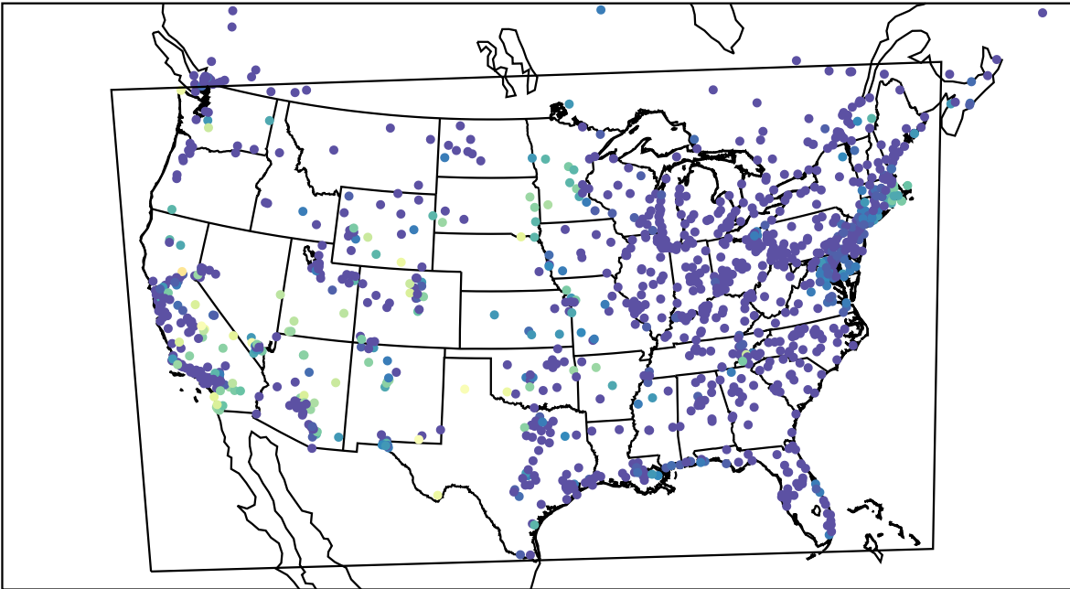
AirNOW (2022-10-03_12:00:00)
