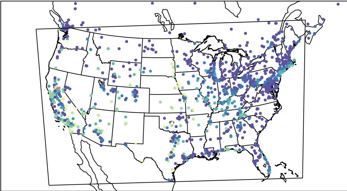
AirNOW (2022-10-02_08:00:00)
