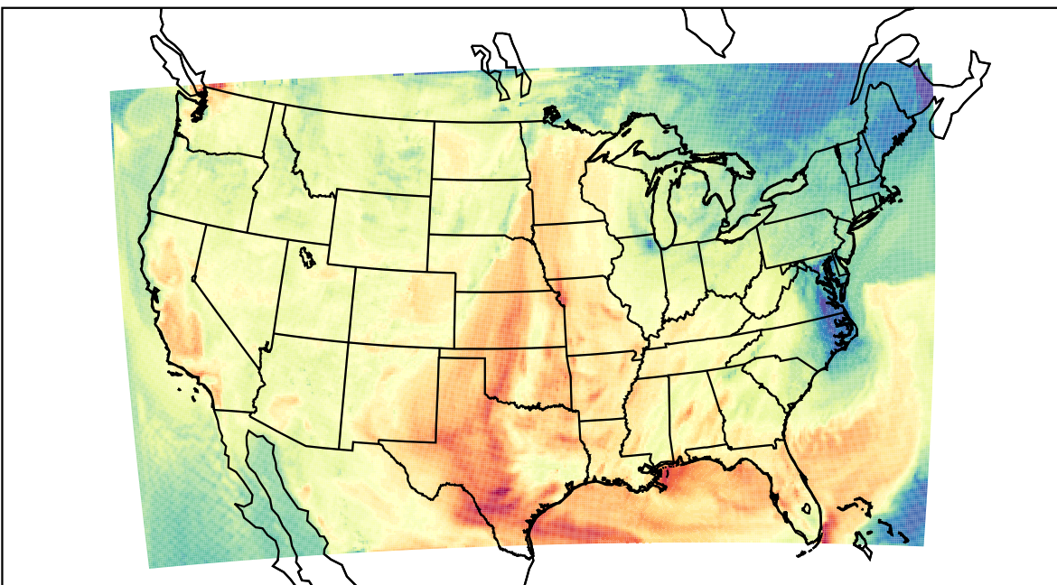
WRF (2022-10-03_21:00:00)
