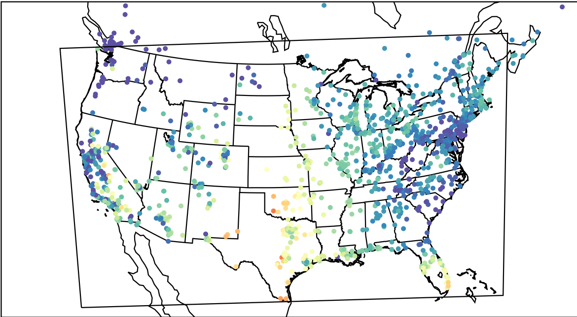
AirNOW (2022-10-03_16:00:00)
