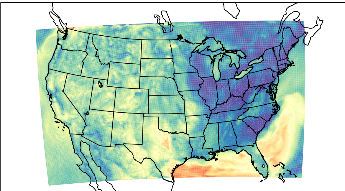
WRF (2022-10-03_09:00:00)
