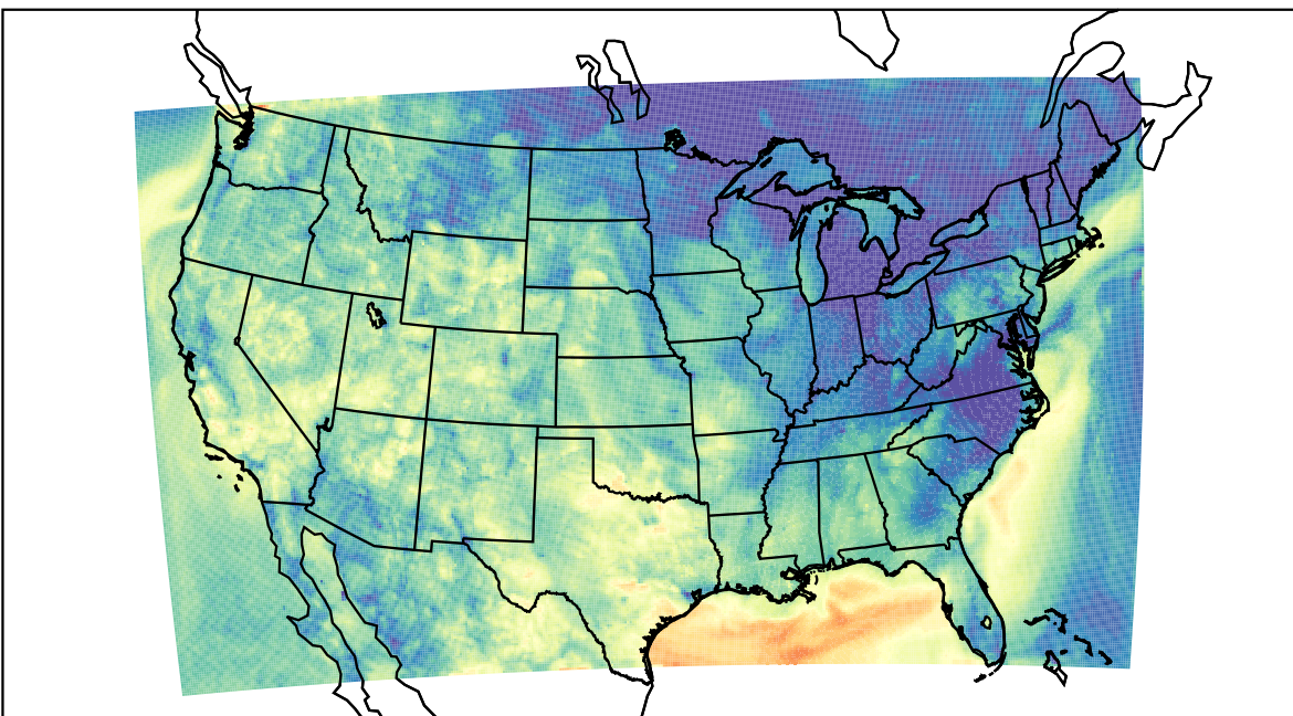
WRF (2022-10-02_08:00:00)
