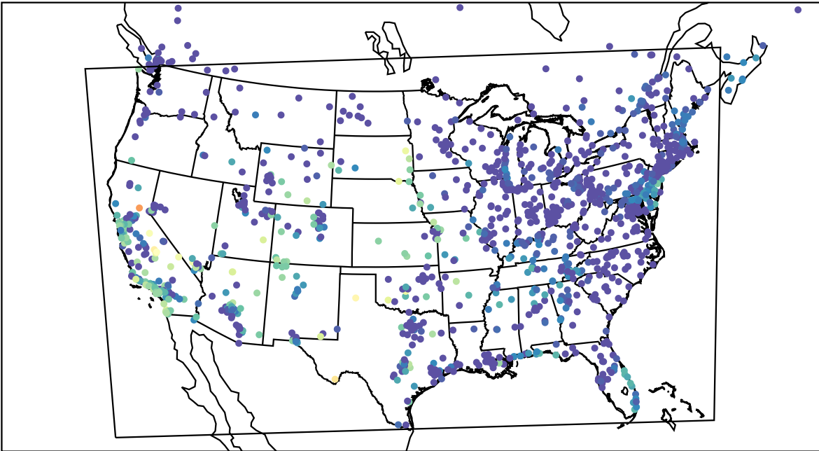
AirNOW (2022-10-02_12:00:00)
