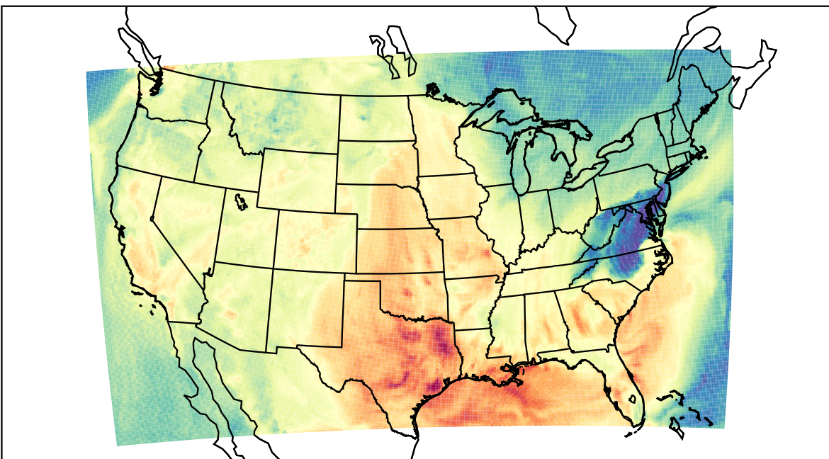
WRF (2022-10-02_20:00:00)
