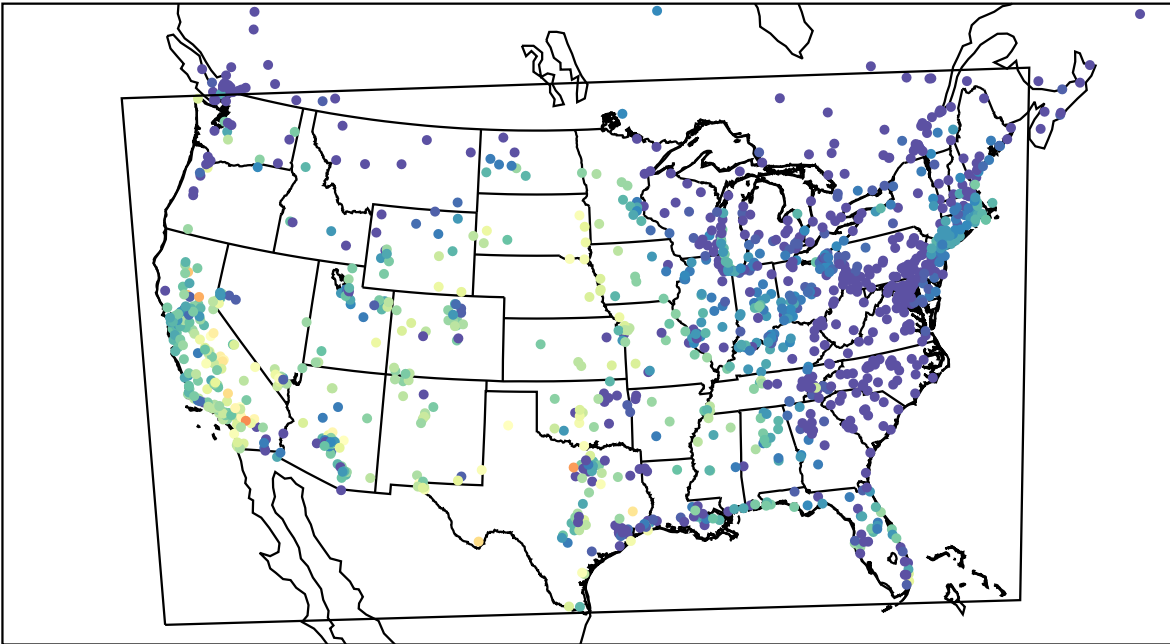
AirNOW (2022-10-03_03:00:00)
