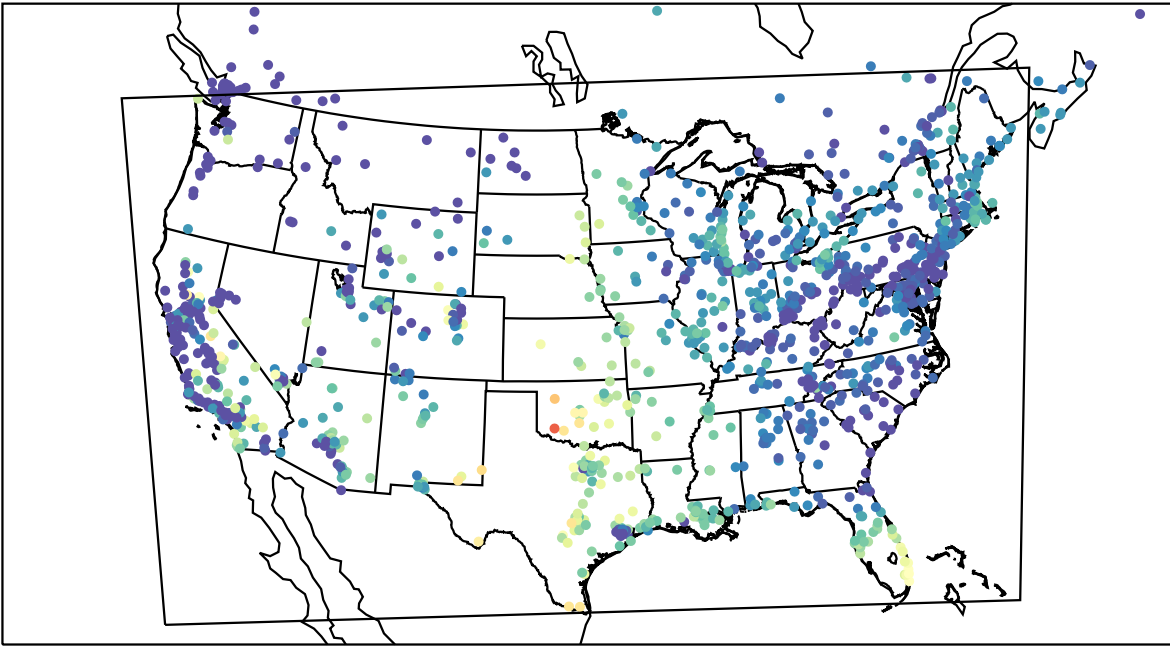
AirNOW (2022-10-03_15:00:00)
