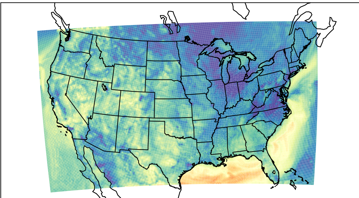
WRF (2022-10-02_14:00:00)
