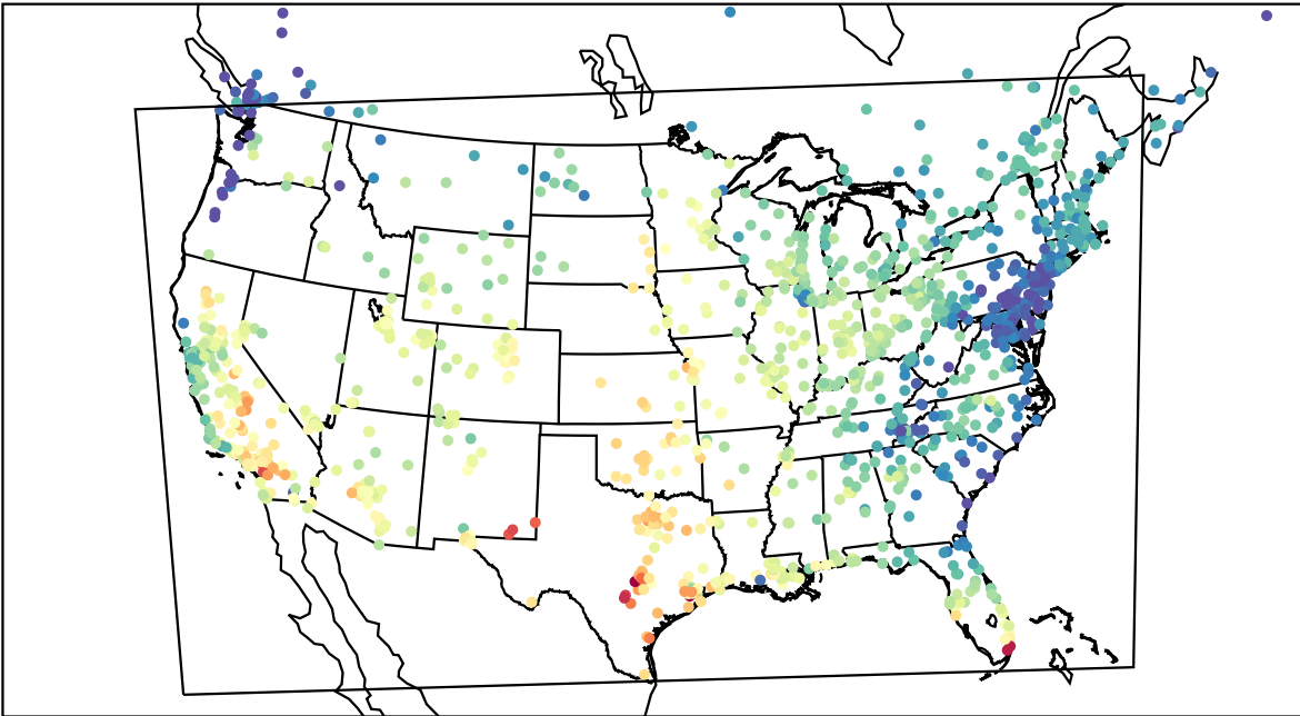
AirNOW (2022-10-03_19:00:00)
