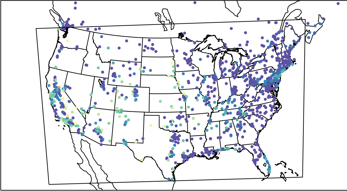
AirNOW (2022-10-02_10:00:00)
