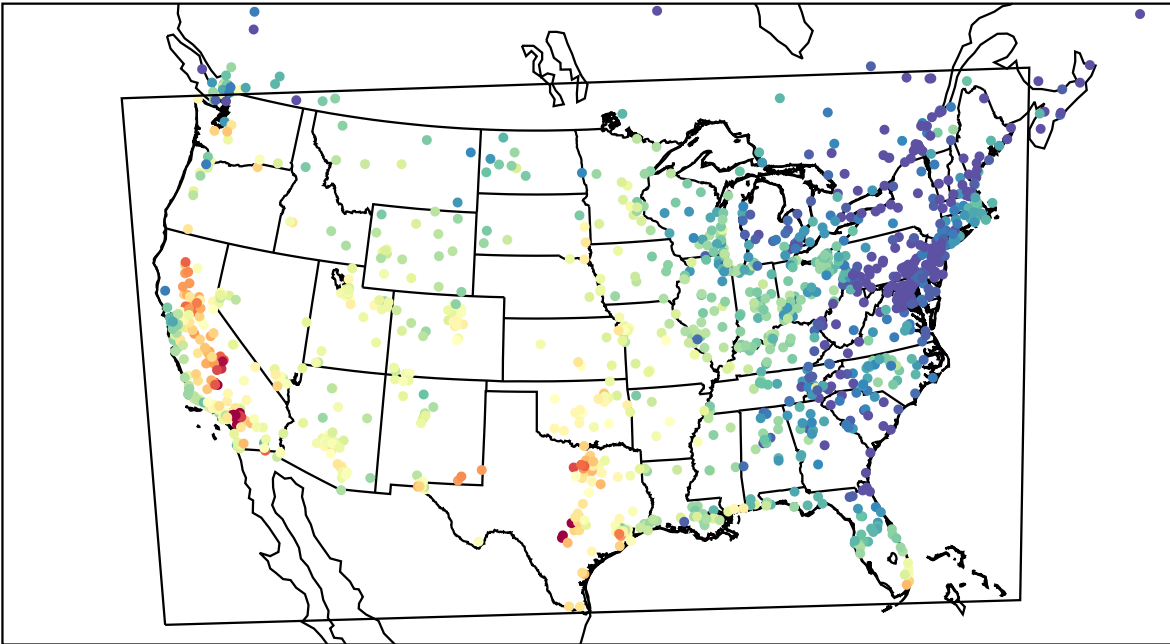
AirNOW (2022-10-03_23:00:00)
