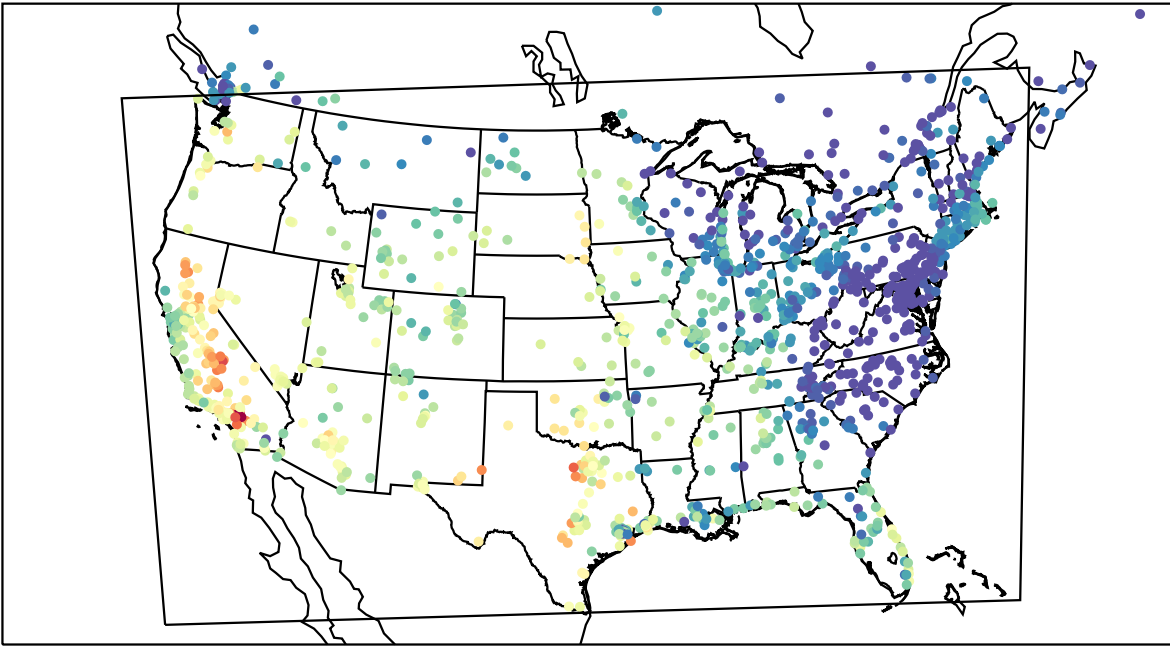
AirNOW (2022-10-03_00:00:00)
