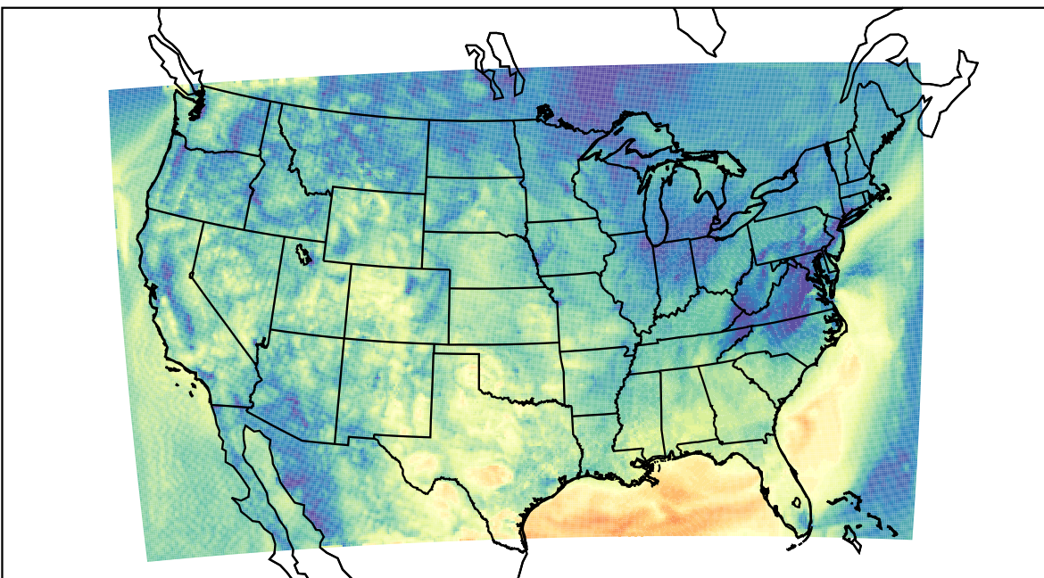
WRF (2022-10-02_15:00:00)
