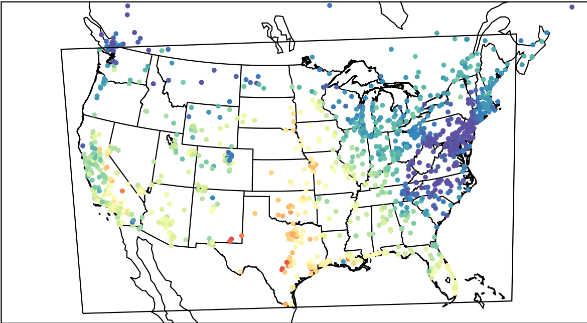
AirNOW (2022-10-02_18:00:00)
