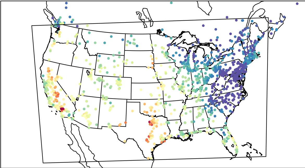
AirNOW (2022-10-02_23:00:00)
