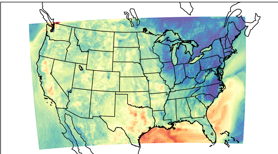
WRF (2022-10-03_02:00:00)
