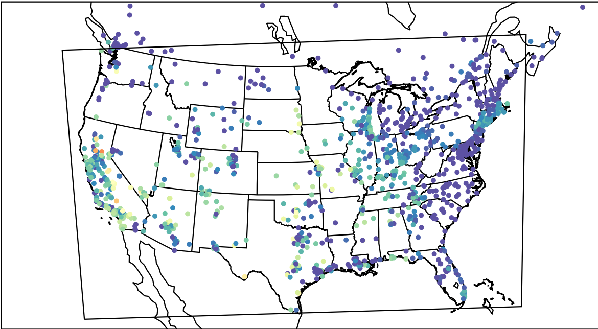
AirNOW (2022-10-02_06:00:00)
