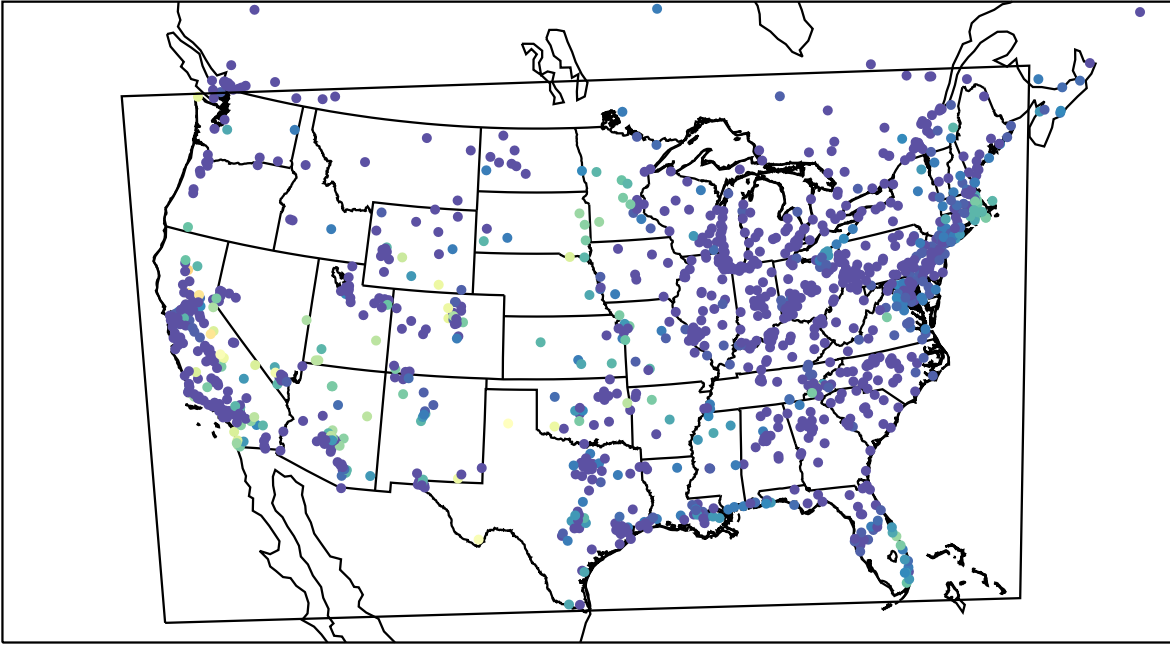
AirNOW (2022-10-03_13:00:00)
