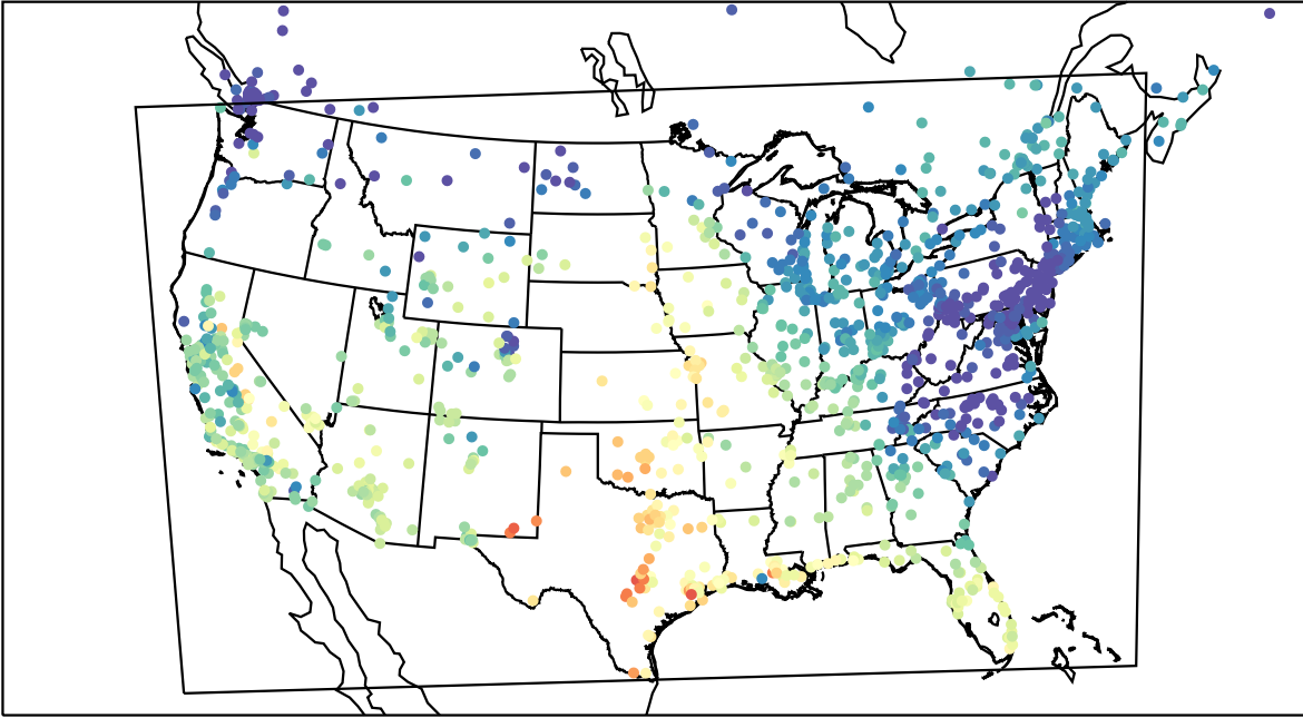
AirNOW (2022-10-02_17:00:00)
