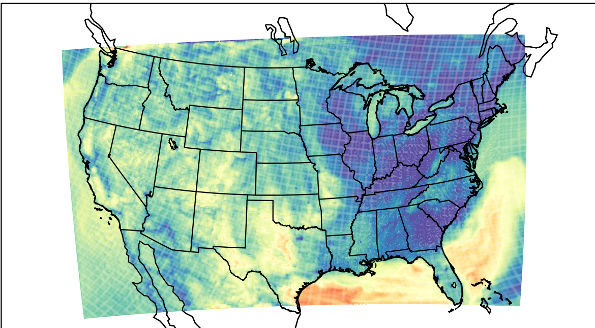
WRF (2022-10-03_11:00:00)
