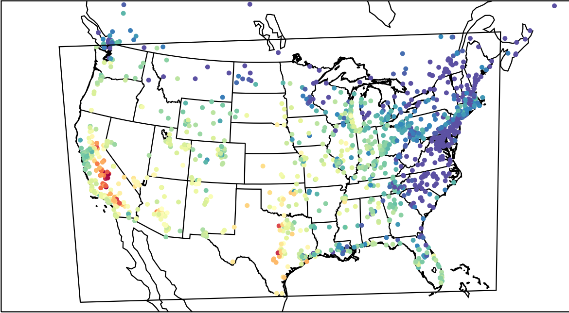
AirNOW (2022-10-02_00:00:00)
