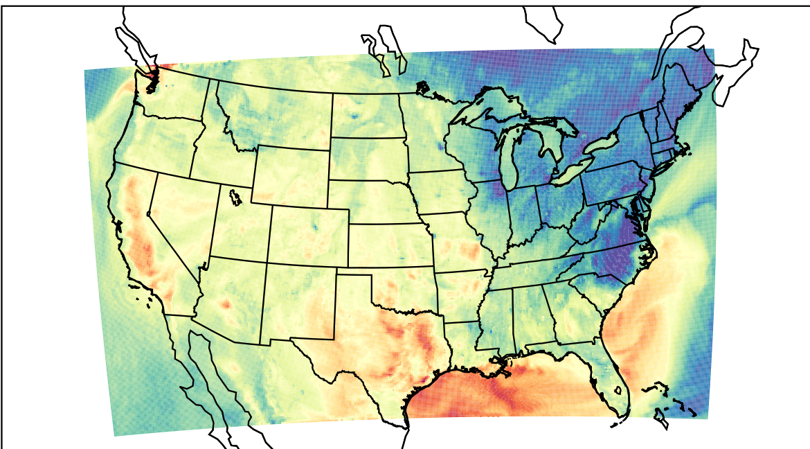
WRF (2022-10-03_00:00:00)
