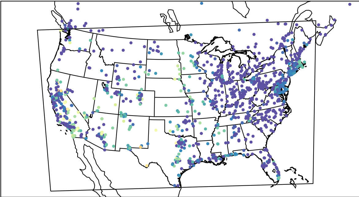
AirNOW (2022-10-03_09:00:00)
