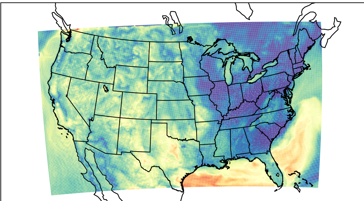
WRF (2022-10-03_10:00:00)
