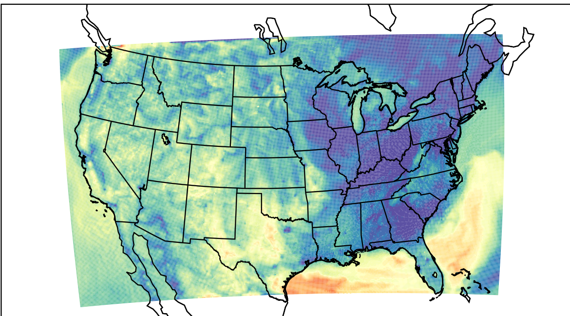
WRF (2022-10-03_12:00:00)
