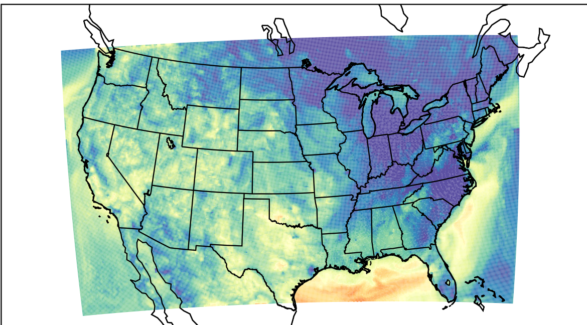
WRF (2022-10-02_11:00:00)
