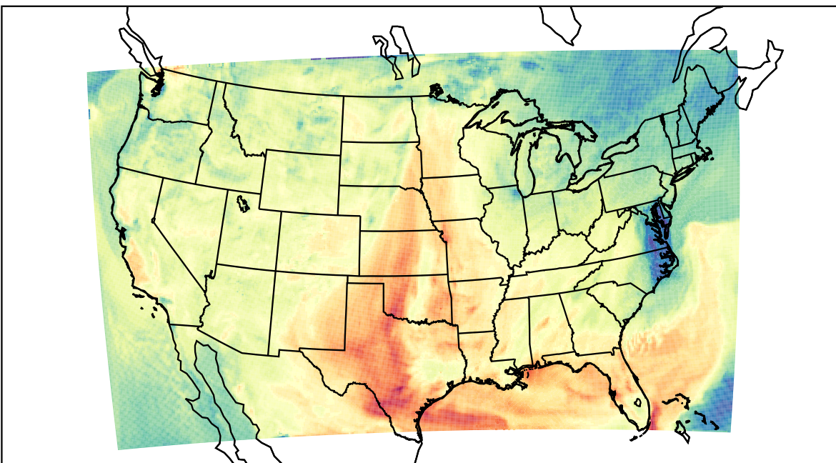
WRF (2022-10-03_19:00:00)
