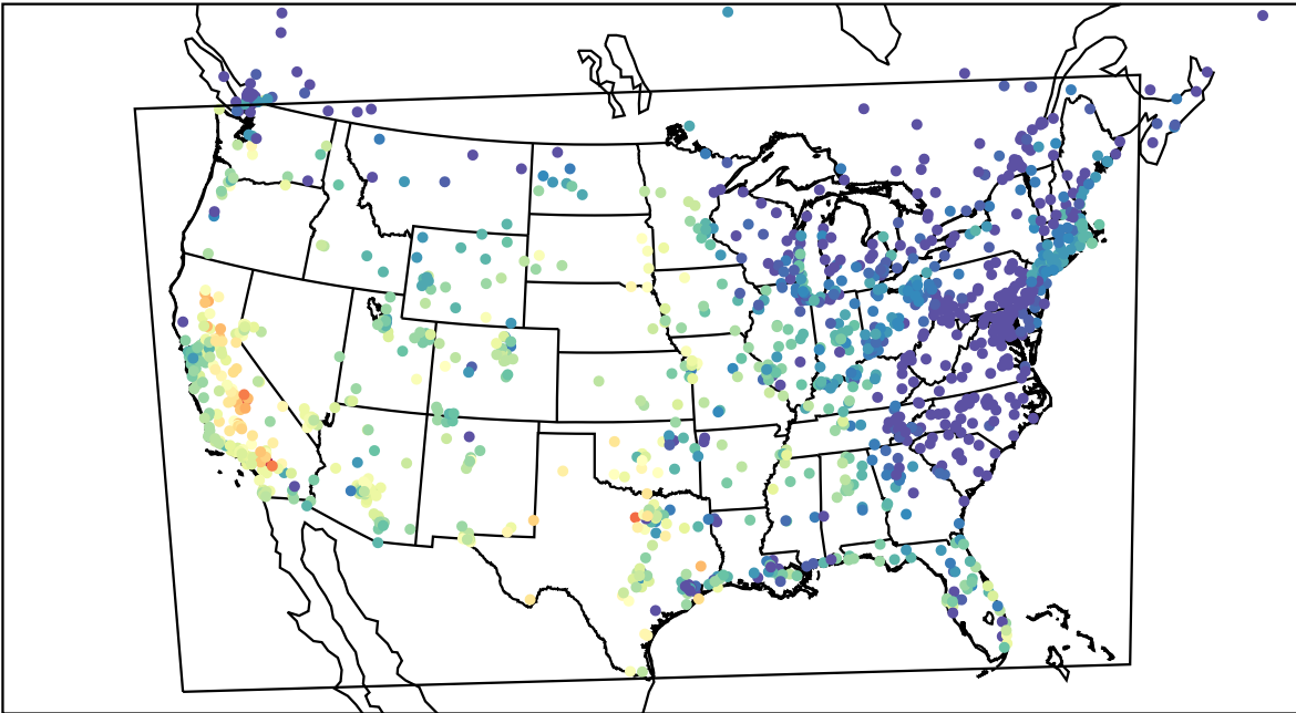
AirNOW (2022-10-03_01:00:00)
