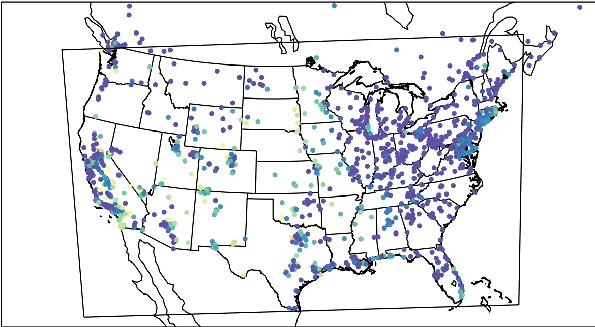
AirNOW (2022-10-03_08:00:00)
