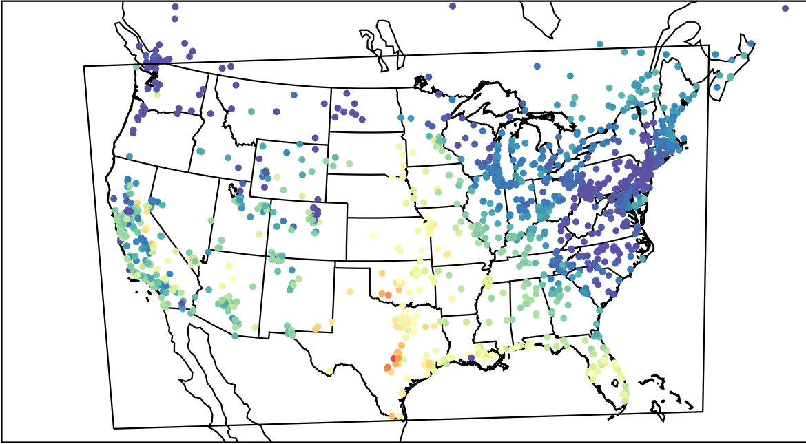
AirNOW (2022-10-02_16:00:00)
