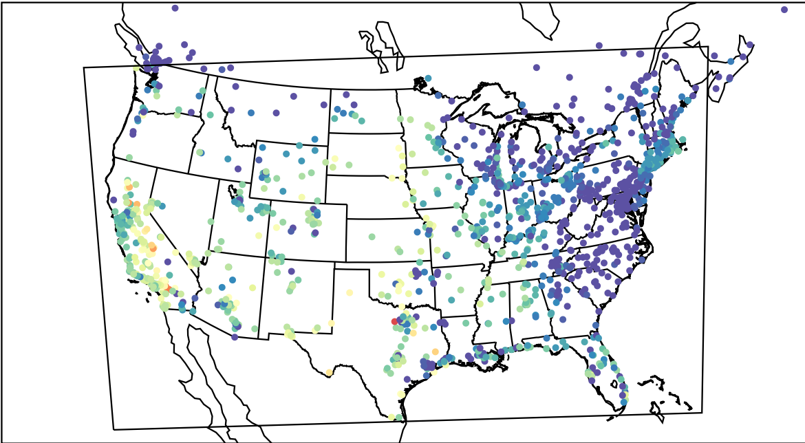
AirNOW (2022-10-03_02:00:00)
