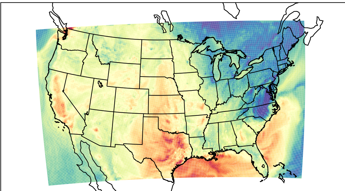
WRF (2022-10-02_23:00:00)
