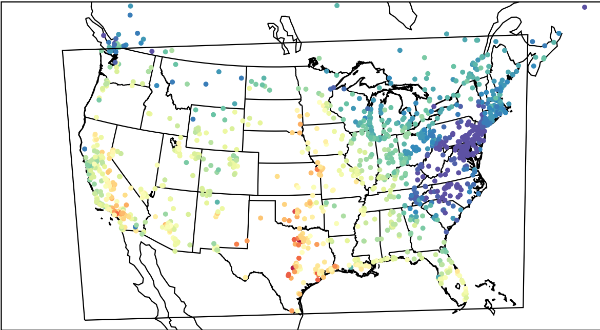
AirNOW (2022-10-02_20:00:00)
