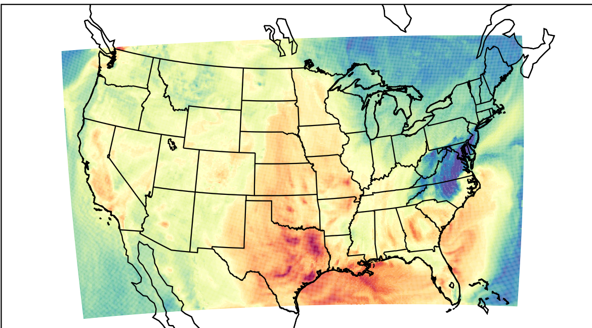
WRF (2022-10-02_21:00:00)
