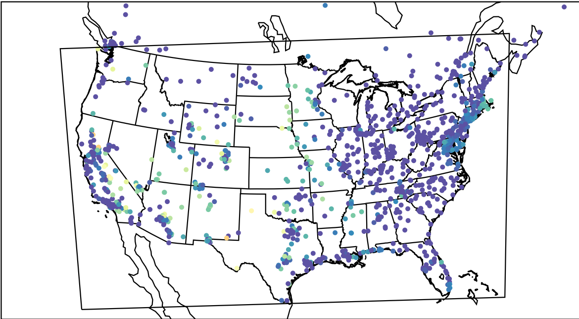
AirNOW (2022-10-03_10:00:00)
