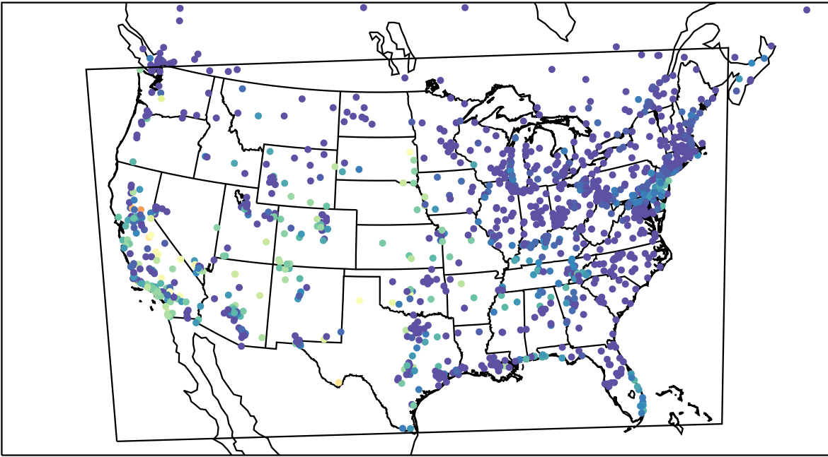
AirNOW (2022-10-02_11:00:00)
