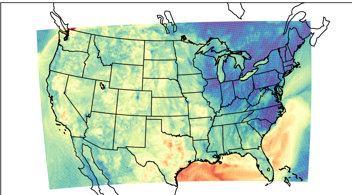
WRF (2022-10-03_03:00:00)
