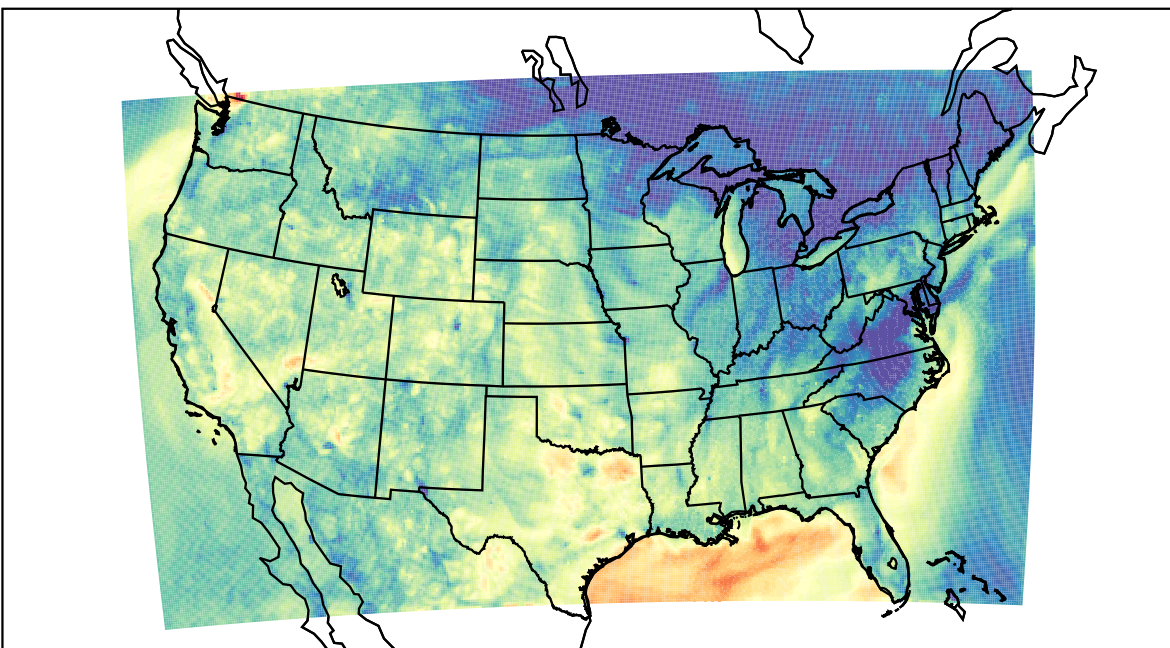
WRF (2022-10-02_04:00:00)
