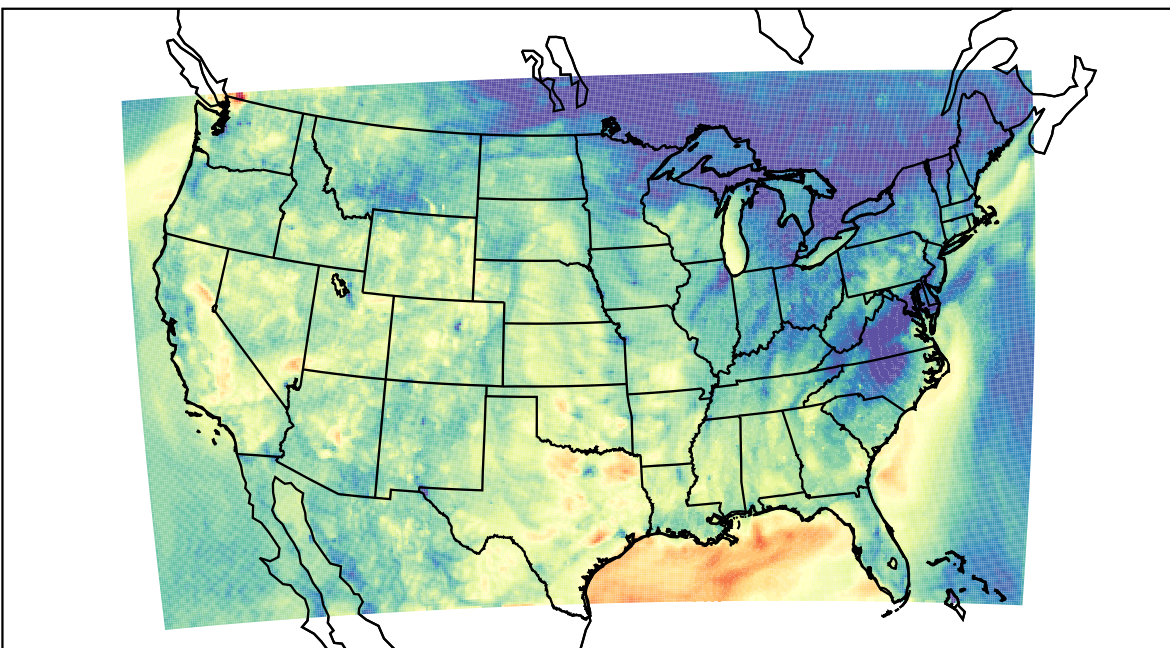
WRF (2022-10-02_03:00:00)
