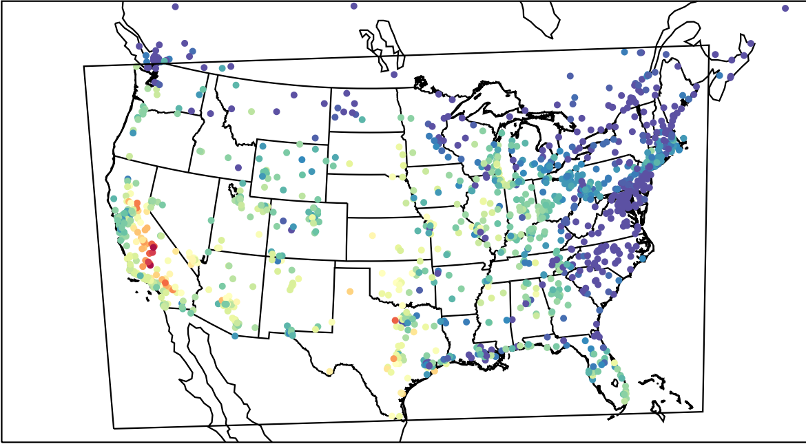
AirNOW (2022-10-02_01:00:00)
