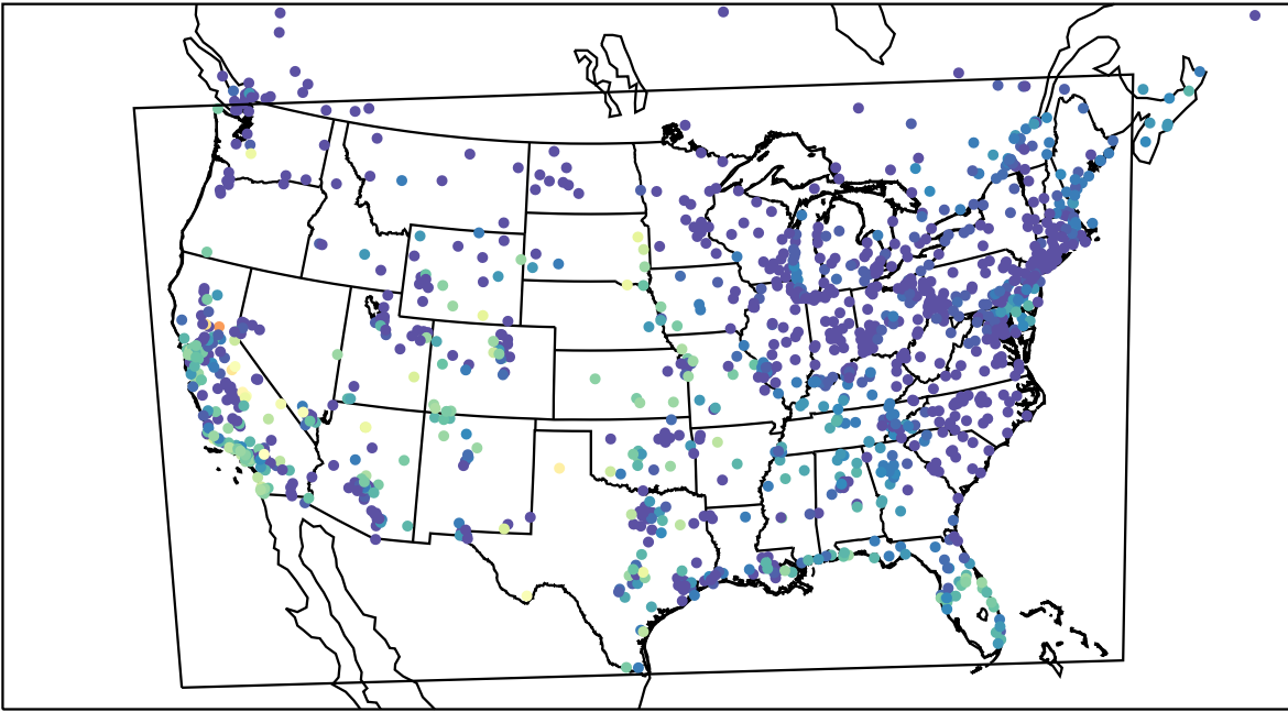
AirNOW (2022-10-02_13:00:00)
