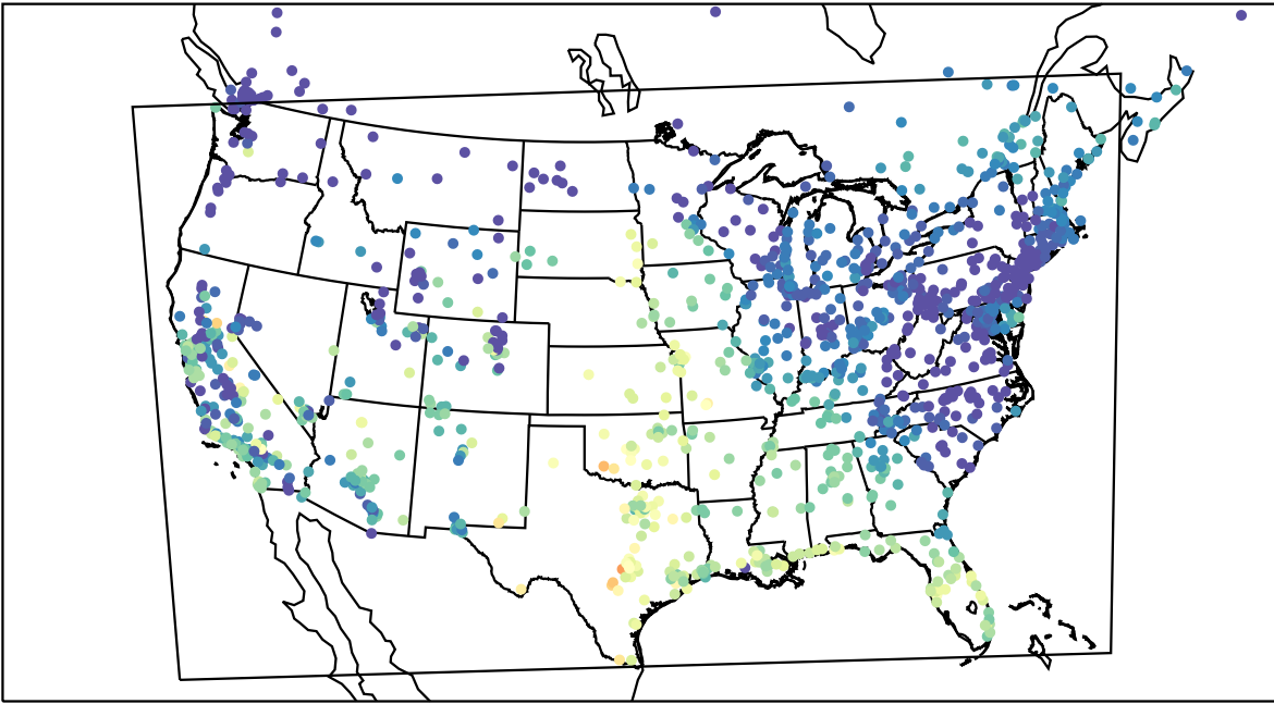
AirNOW (2022-10-02_15:00:00)
