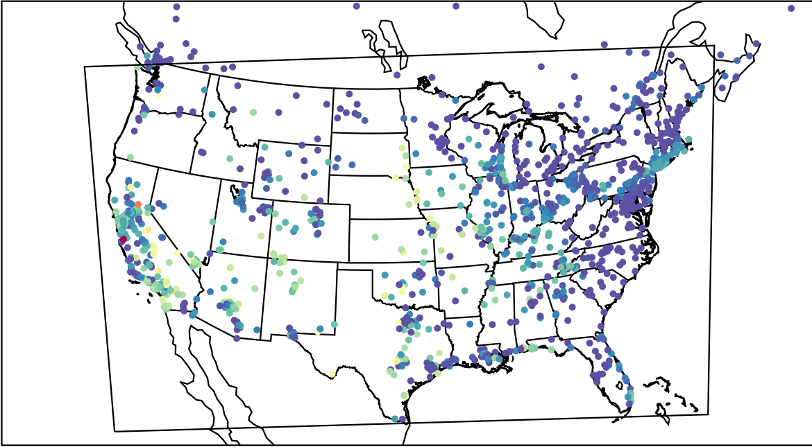
AirNOW (2022-10-02_07:00:00)
