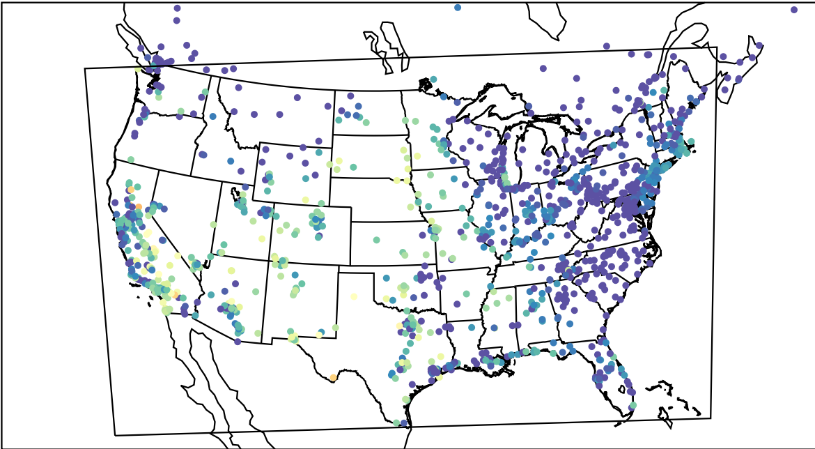
AirNOW (2022-10-03_05:00:00)
