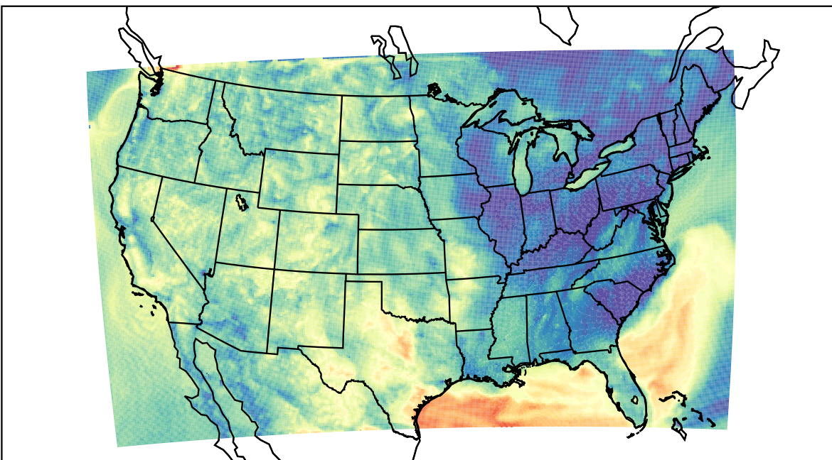
WRF (2022-10-03_08:00:00)
