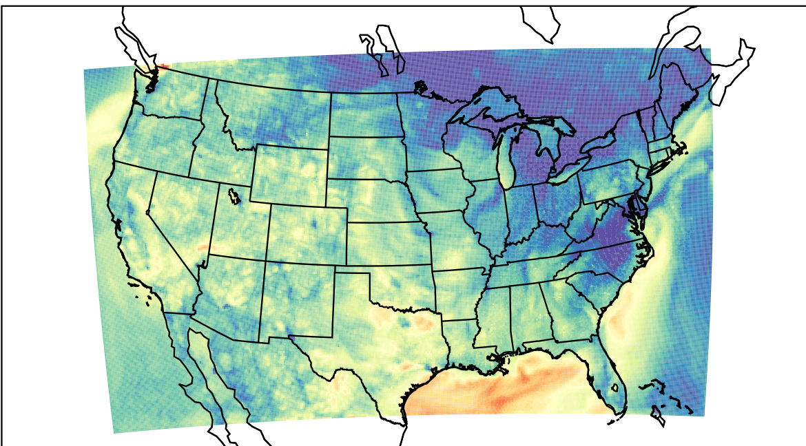
WRF (2022-10-02_05:00:00)
