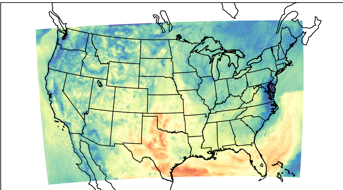
WRF (2022-10-03_16:00:00)
