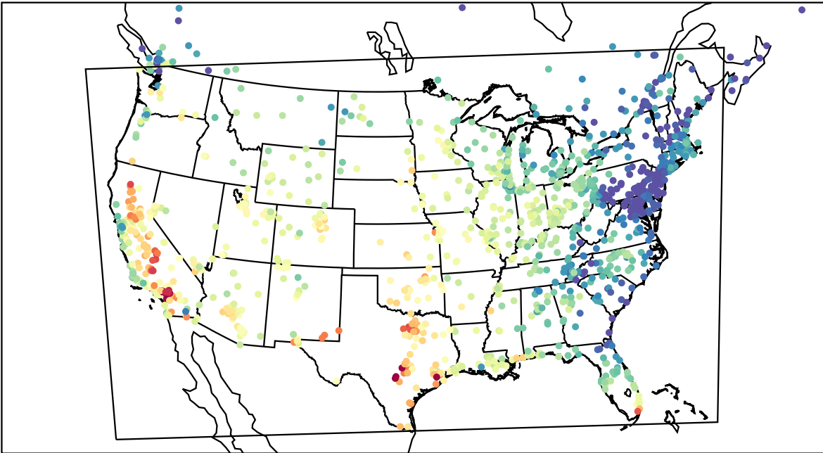
AirNOW (2022-10-03_22:00:00)
