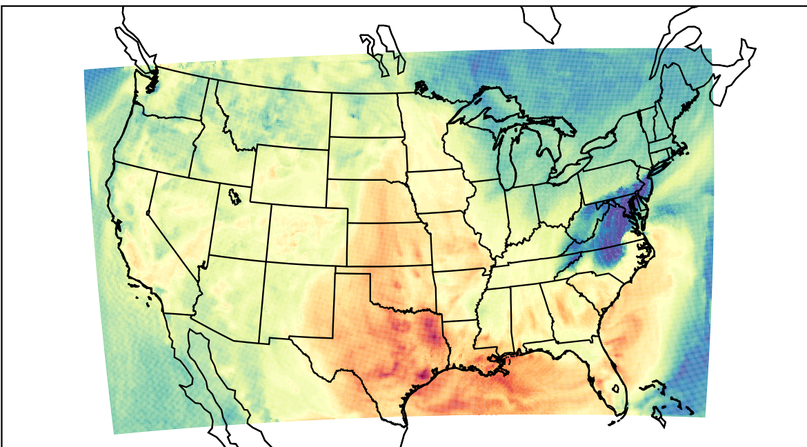
WRF (2022-10-02_19:00:00)
