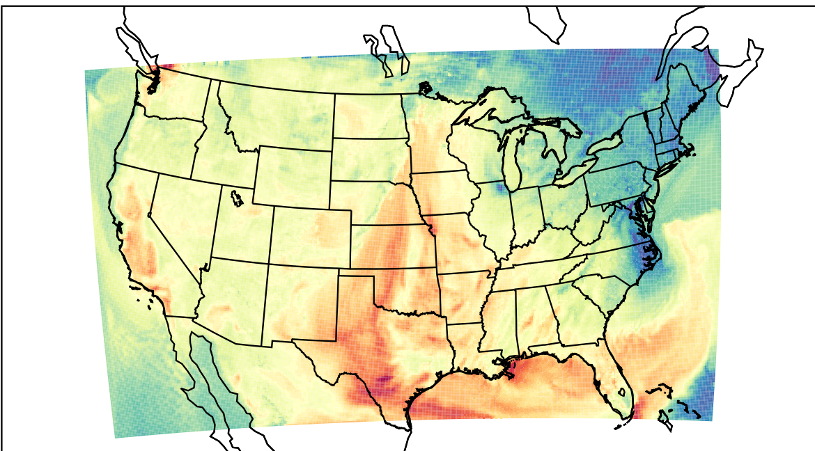
WRF (2022-10-03_22:00:00)
