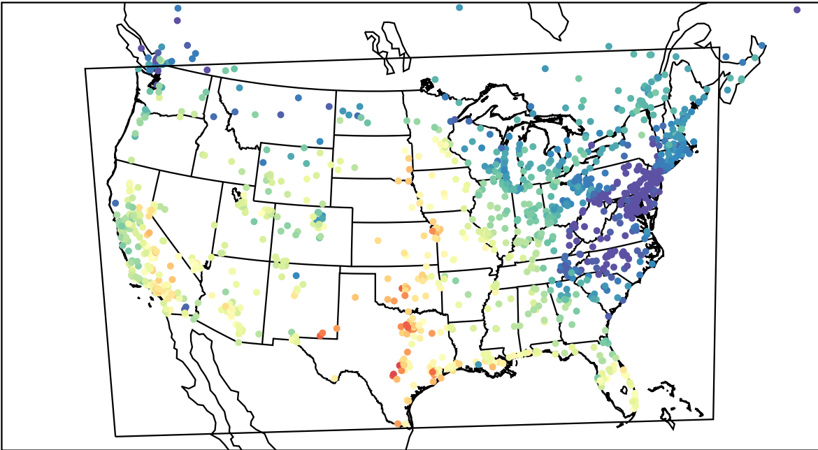
AirNOW (2022-10-02_19:00:00)
