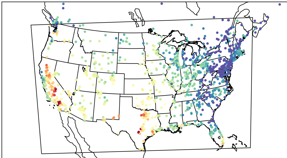
AirNOW (2022-10-03_23:00:00)
