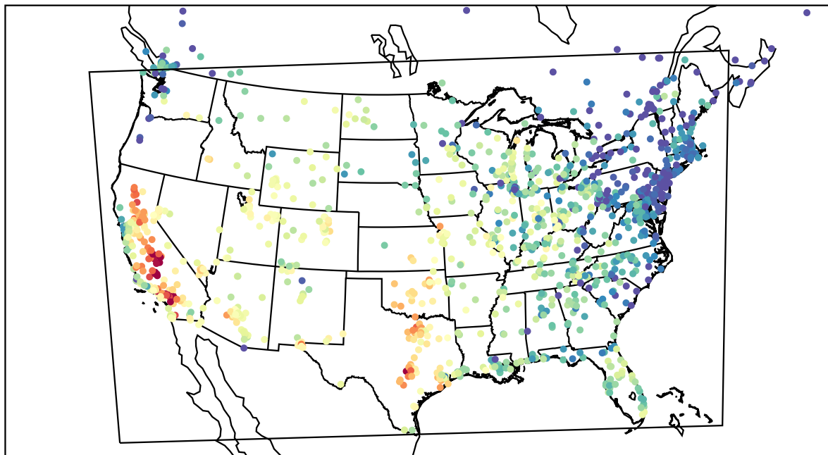
AirNOW (2022-10-04_23:00:00)
