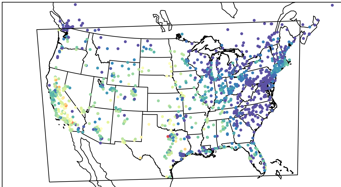
AirNOW (2022-10-03_02:00:00)
