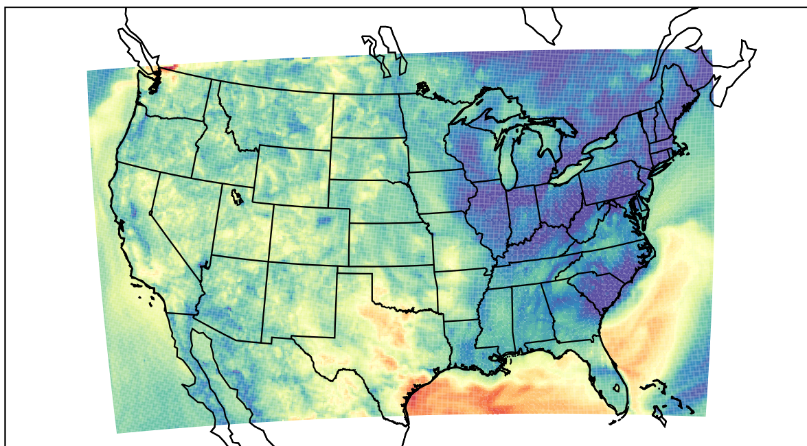
WRF (2022-10-03_07:00:00)
