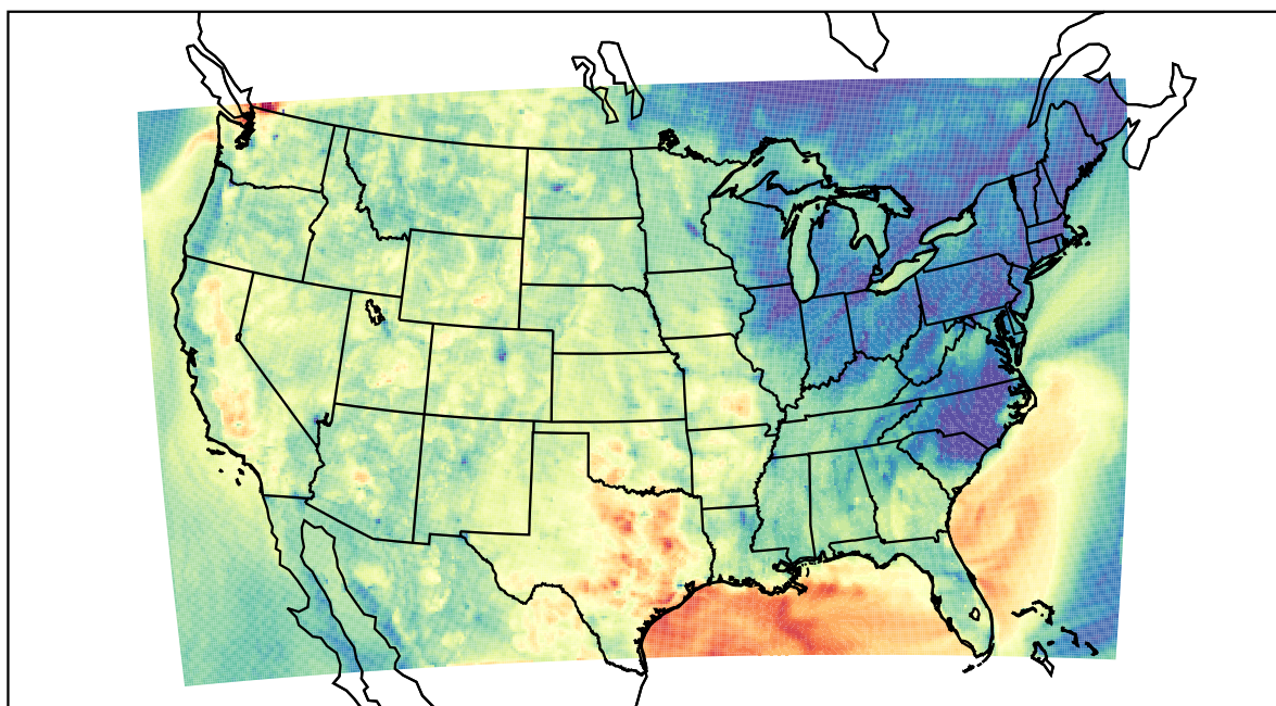
WRF (2022-10-03_02:00:00)
