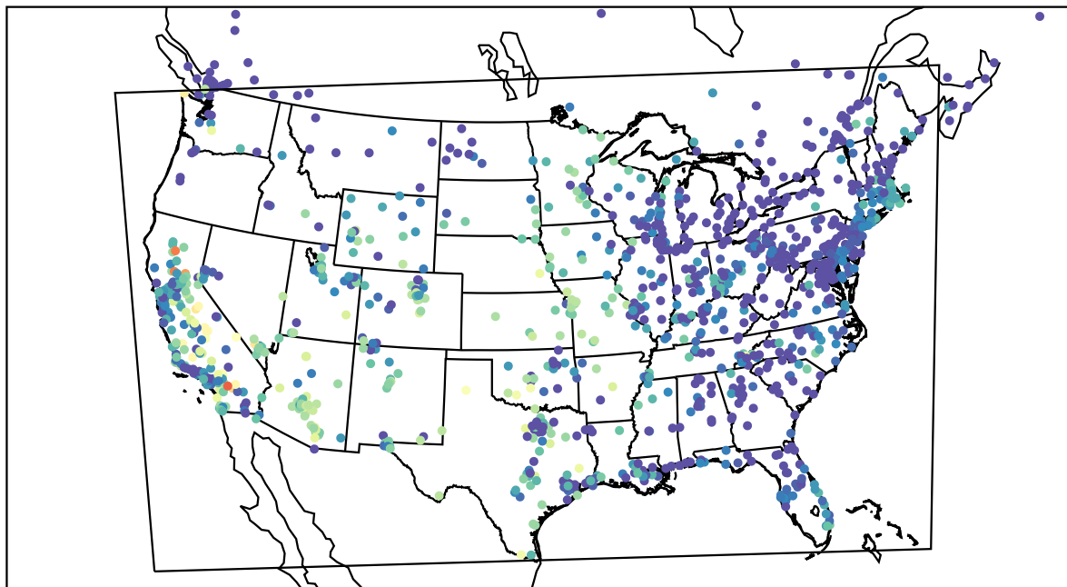
AirNOW (2022-10-04_04:00:00)
