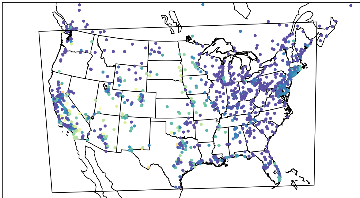
AirNOW (2022-10-03_08:00:00)
