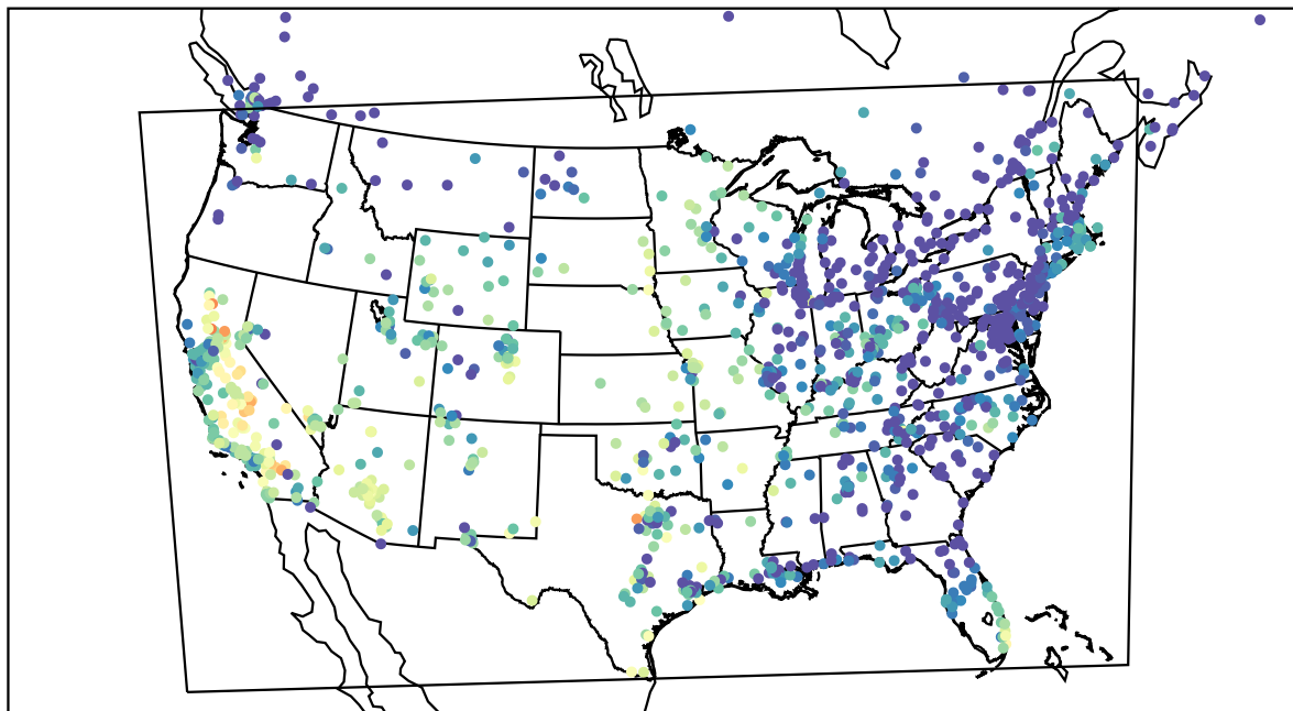
AirNOW (2022-10-04_02:00:00)
