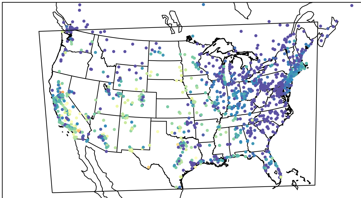
AirNOW (2022-10-03_04:00:00)
