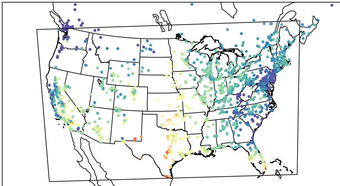
AirNOW (2022-10-03_17:00:00)
