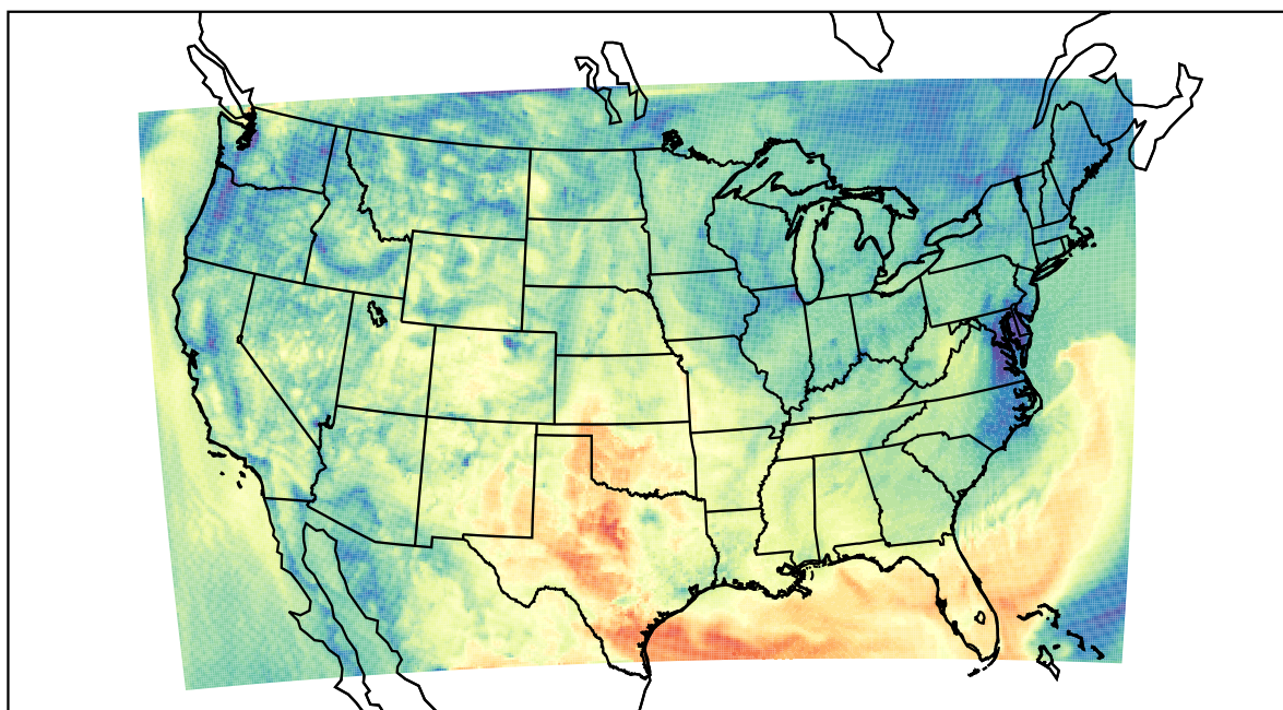
WRF (2022-10-03_16:00:00)
