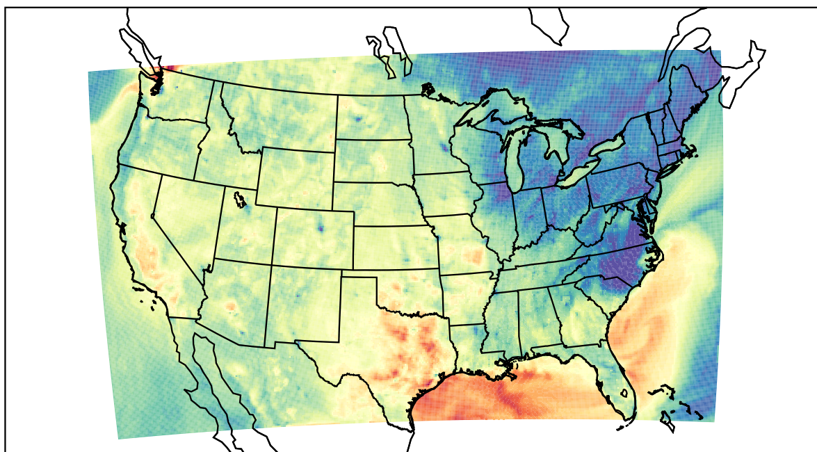
WRF (2022-10-03_01:00:00)
