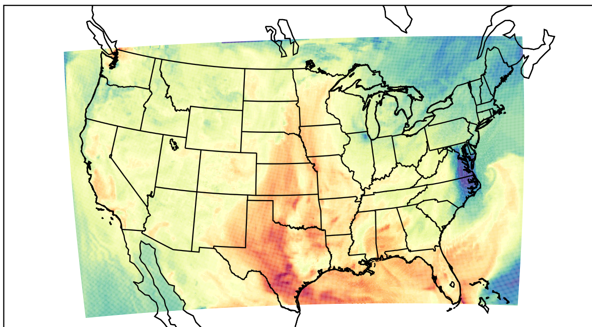
WRF (2022-10-03_20:00:00)
