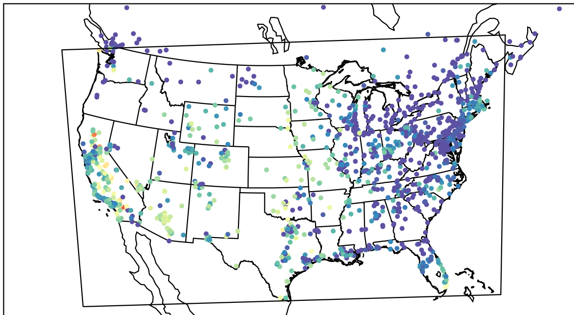
AirNOW (2022-10-04_03:00:00)
