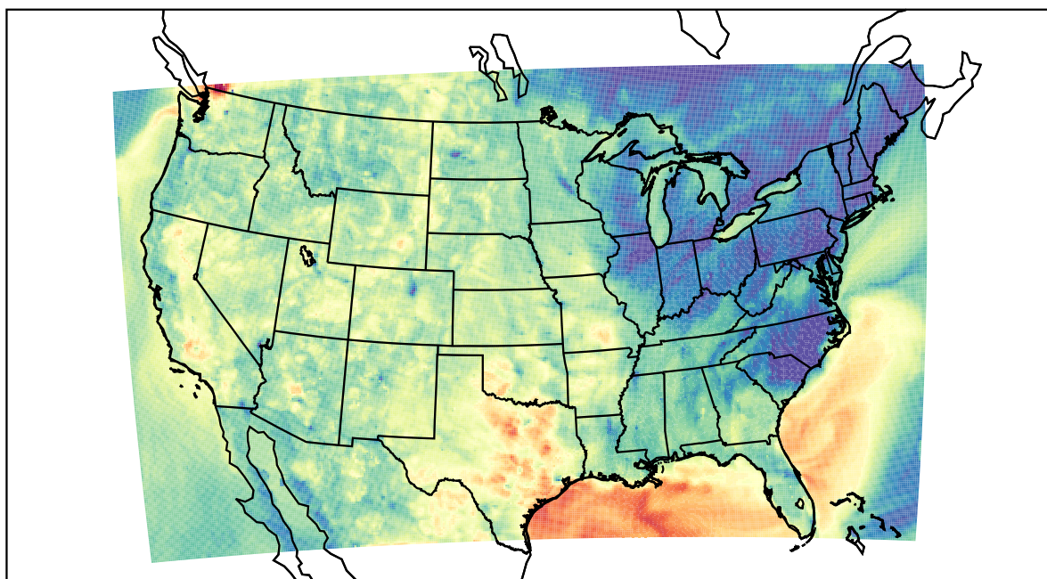
WRF (2022-10-03_03:00:00)
