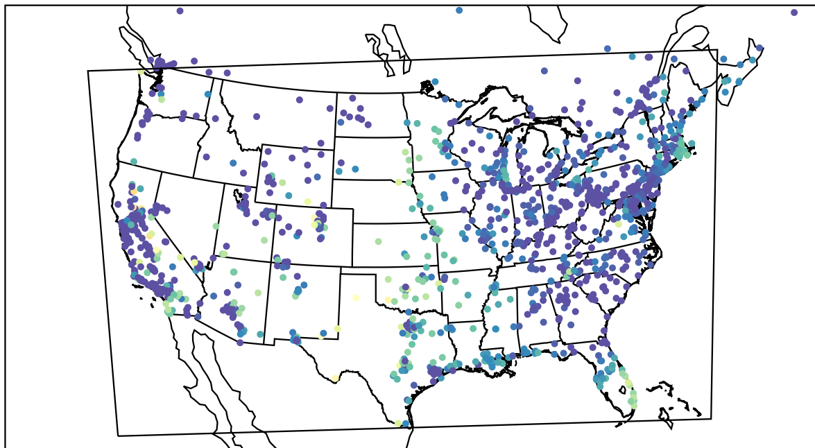
AirNOW (2022-10-03_14:00:00)
