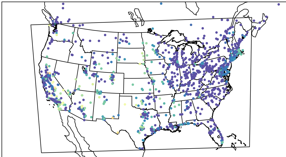
AirNOW (2022-10-03_09:00:00)
