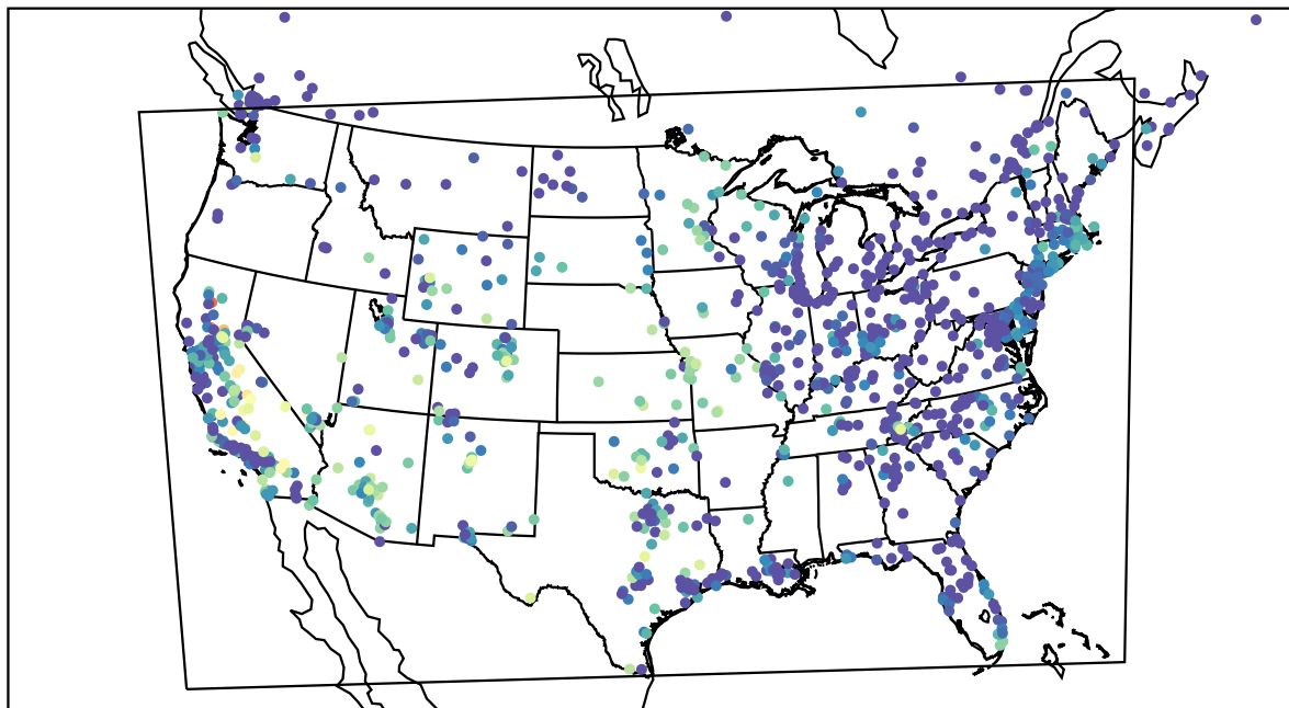
AirNOW (2022-10-04_06:00:00)
