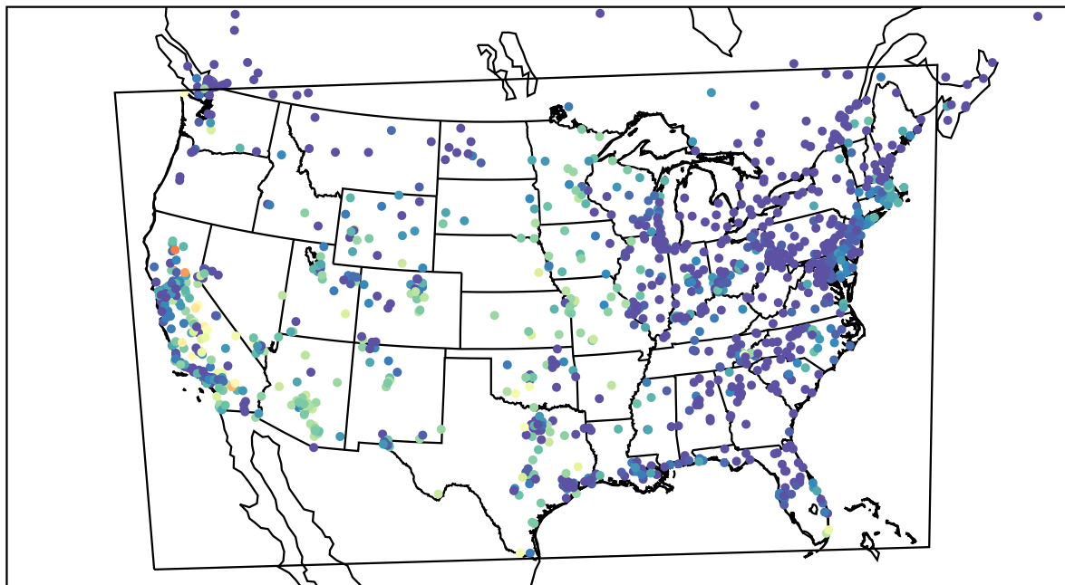
AirNOW (2022-10-04_05:00:00)
