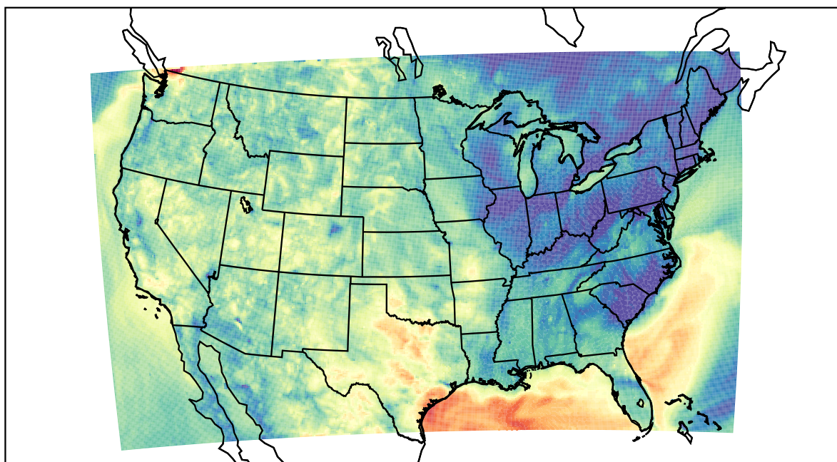
WRF (2022-10-03_06:00:00)
