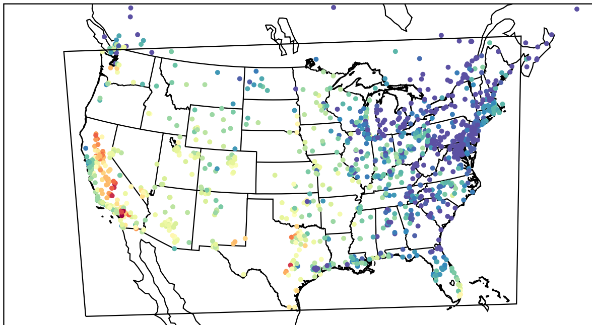
AirNOW (2022-10-04_00:00:00)
