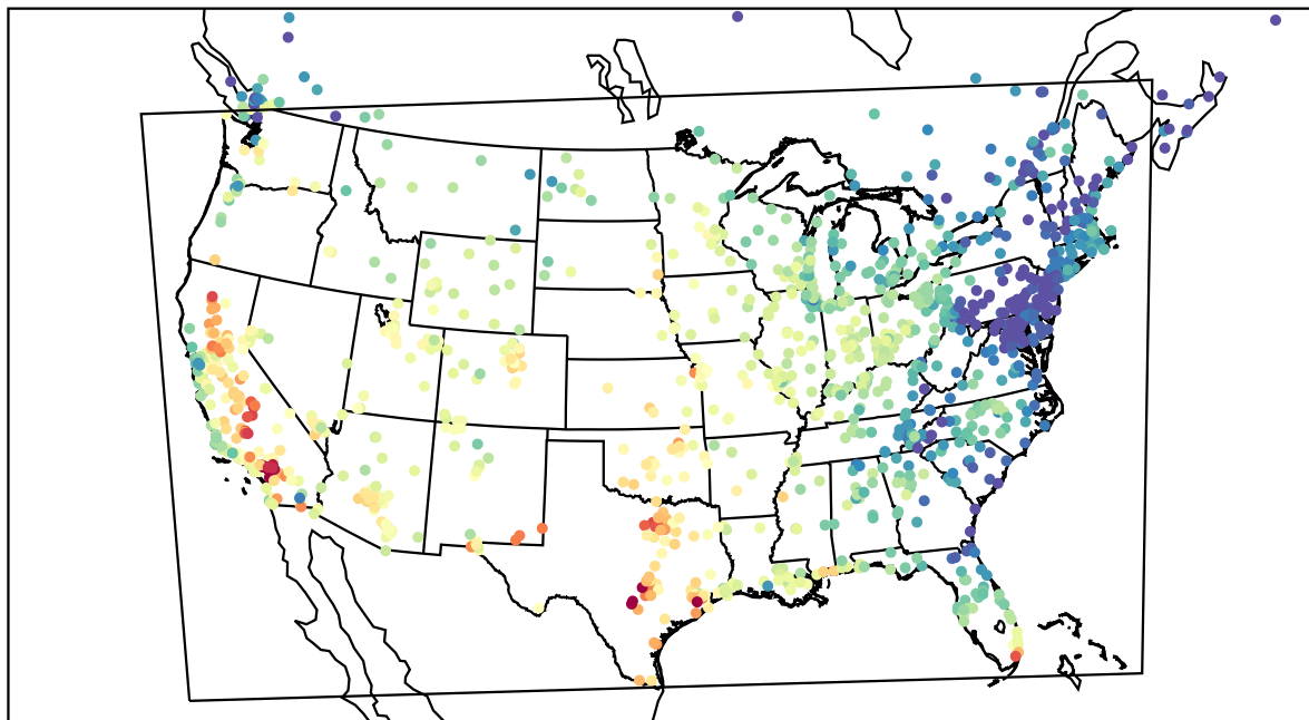
AirNOW (2022-10-03_22:00:00)
