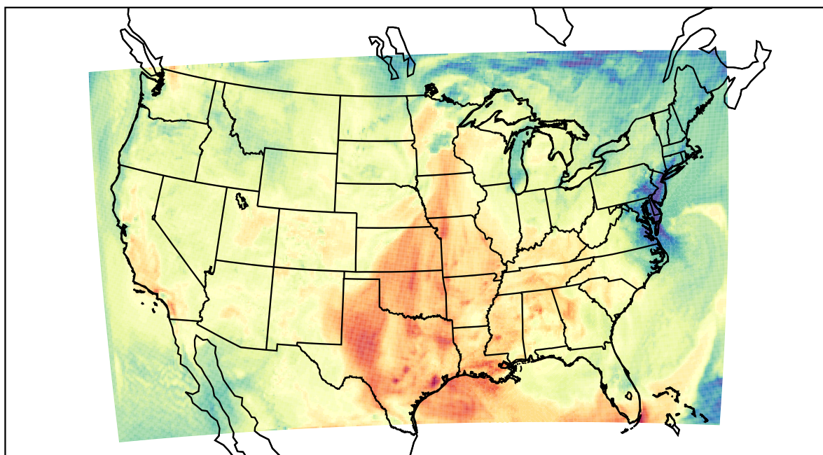
WRF (2022-10-04_20:00:00)
