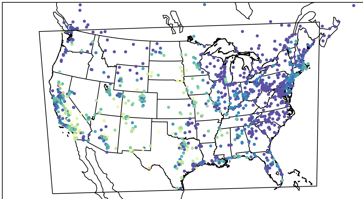
AirNOW (2022-10-03_05:00:00)
