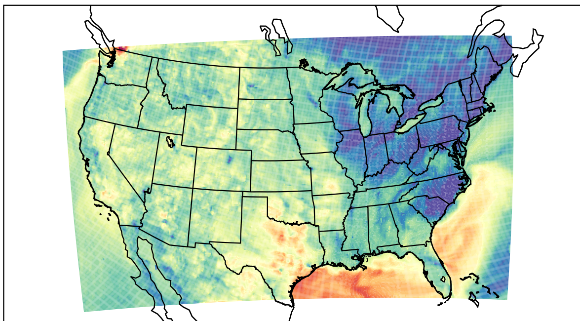
WRF (2022-10-03_04:00:00)
