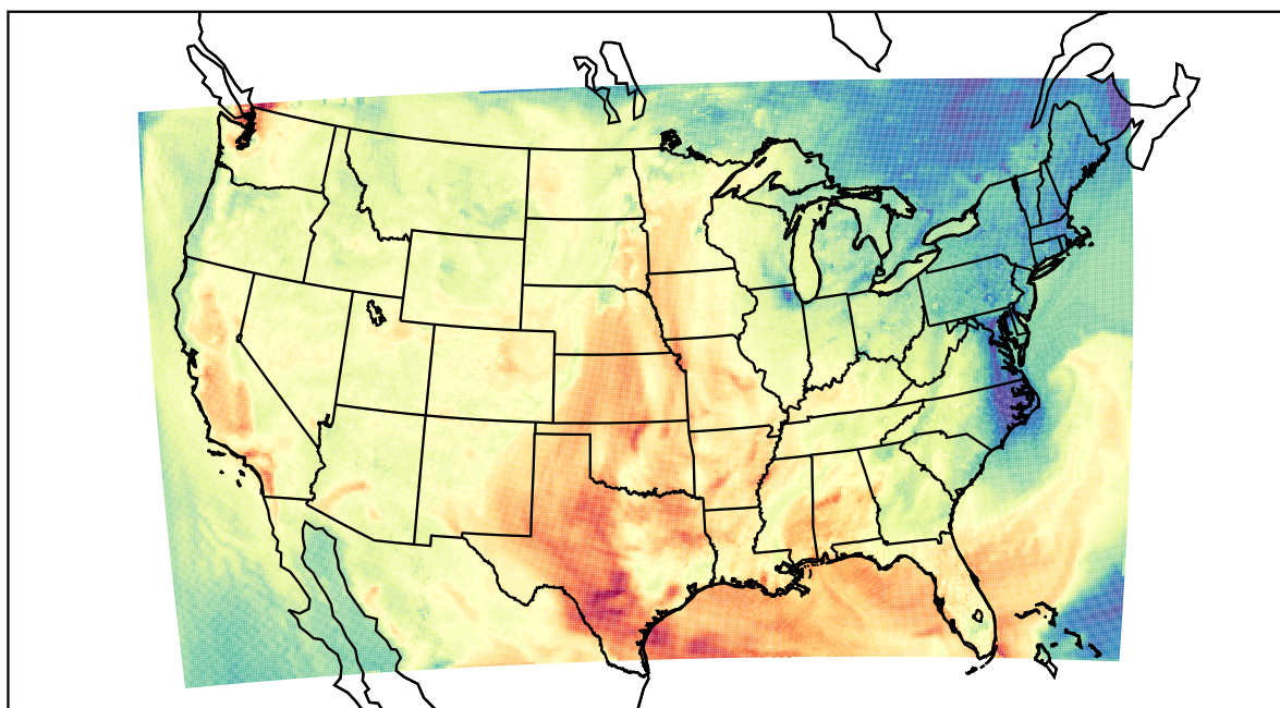
WRF (2022-10-03_22:00:00)
