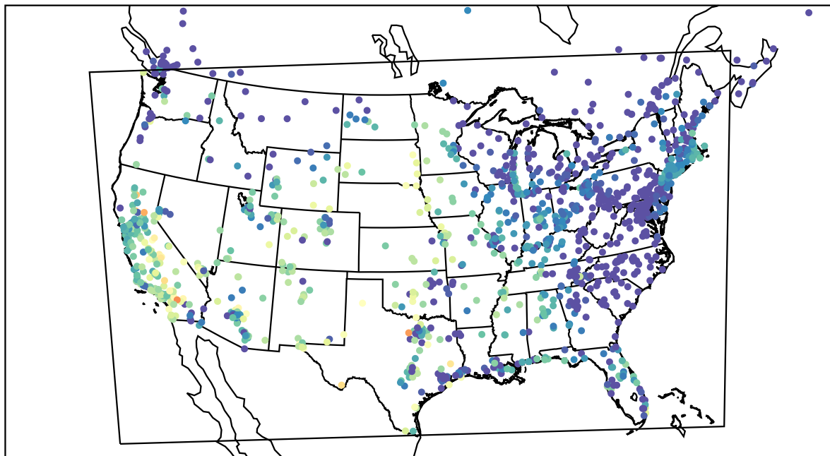
AirNOW (2022-10-03_03:00:00)
