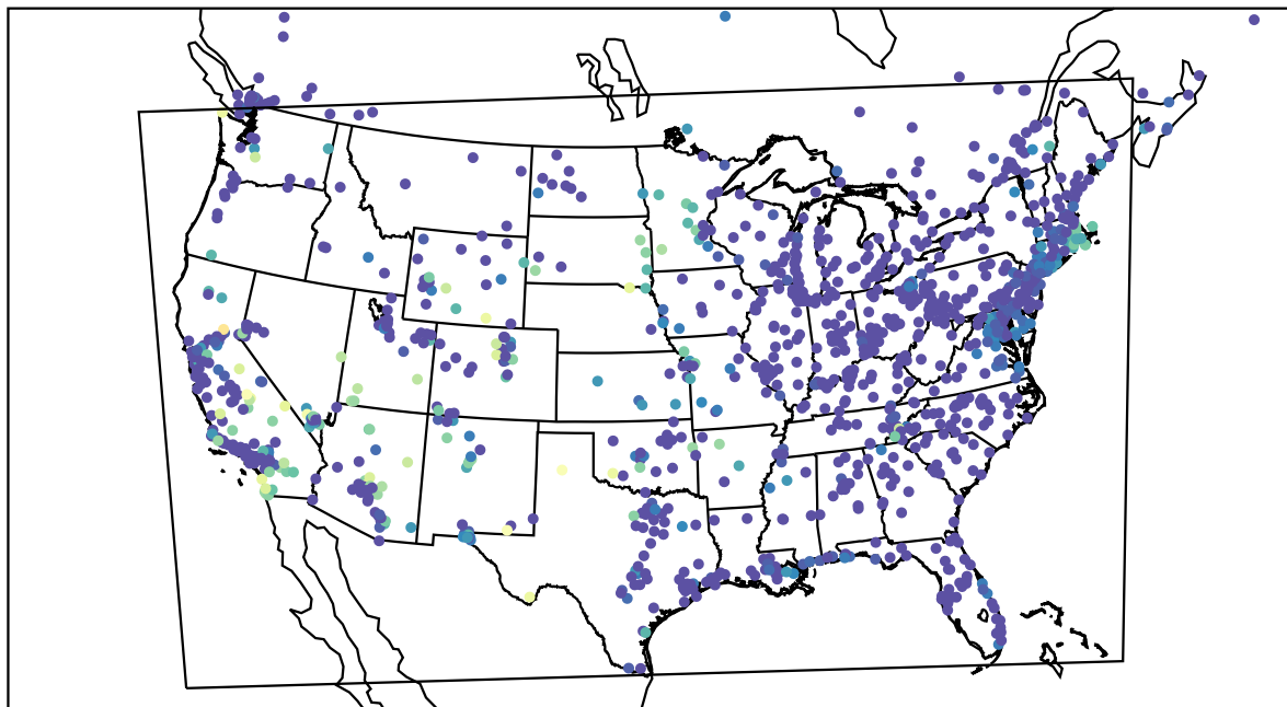
AirNOW (2022-10-03_12:00:00)
