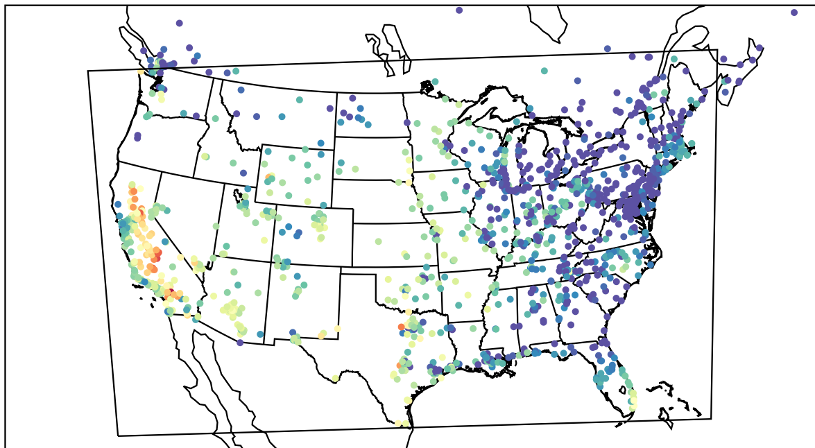
AirNOW (2022-10-04_01:00:00)
