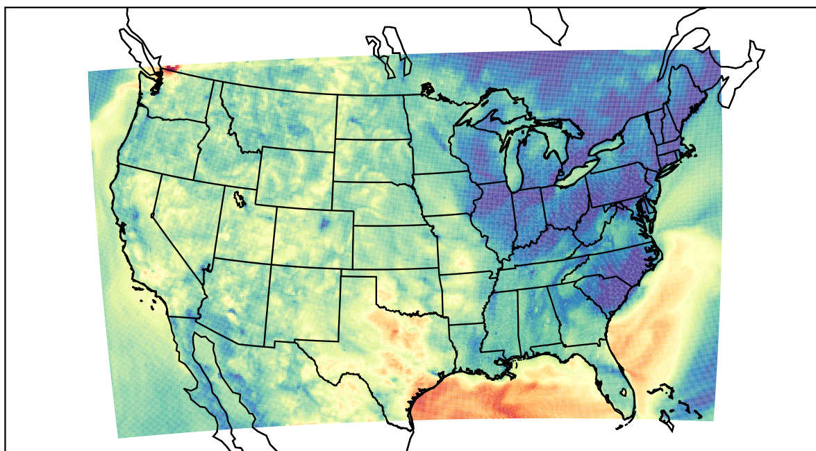
WRF (2022-10-03_05:00:00)
