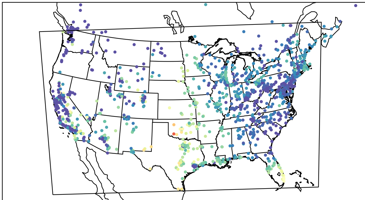
AirNOW (2022-10-03_15:00:00)
