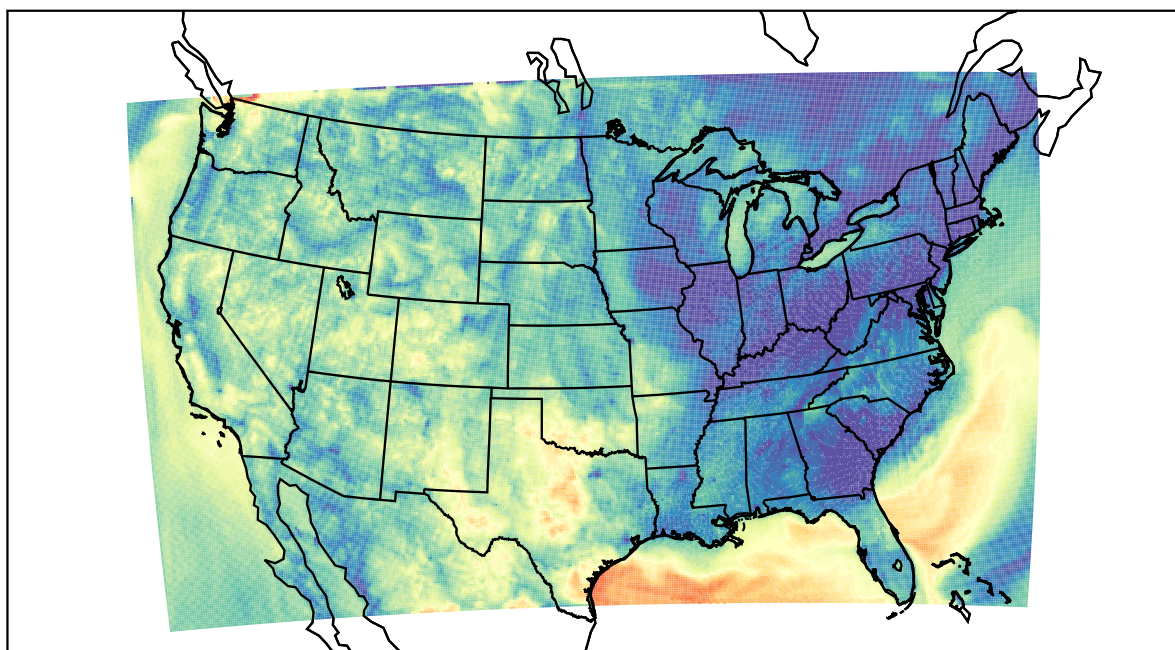
WRF (2022-10-03_11:00:00)
