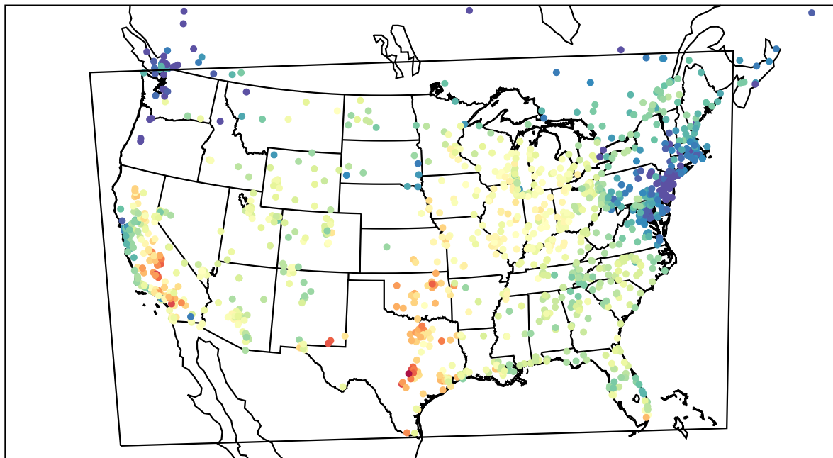
AirNOW (2022-10-04_19:00:00)
