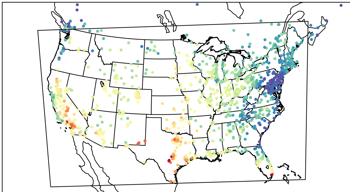
AirNOW (2022-10-03_20:00:00)
