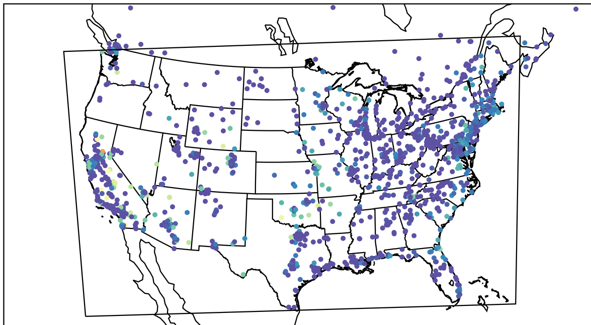
AirNOW (2022-10-04_13:00:00)
