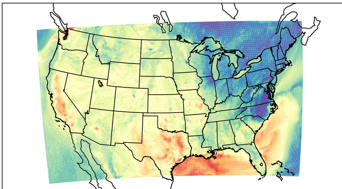
WRF (2022-10-03_00:00:00)
