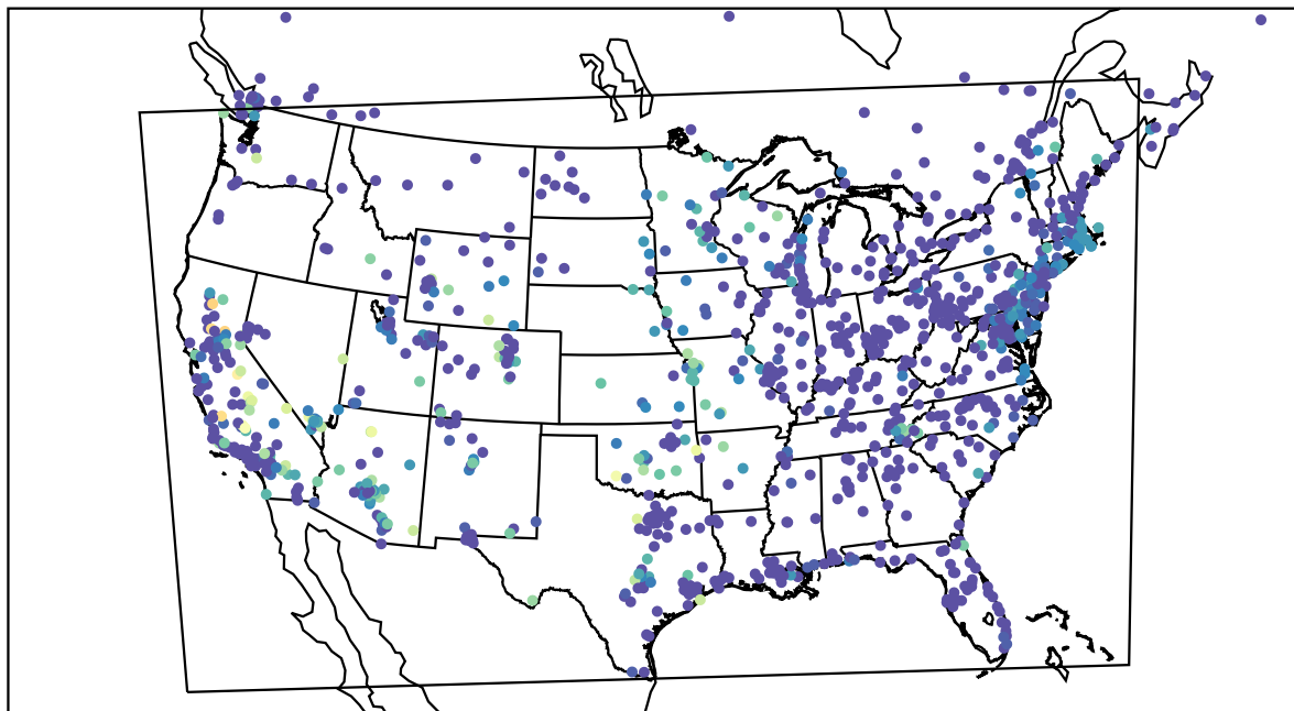
AirNOW (2022-10-04_11:00:00)
