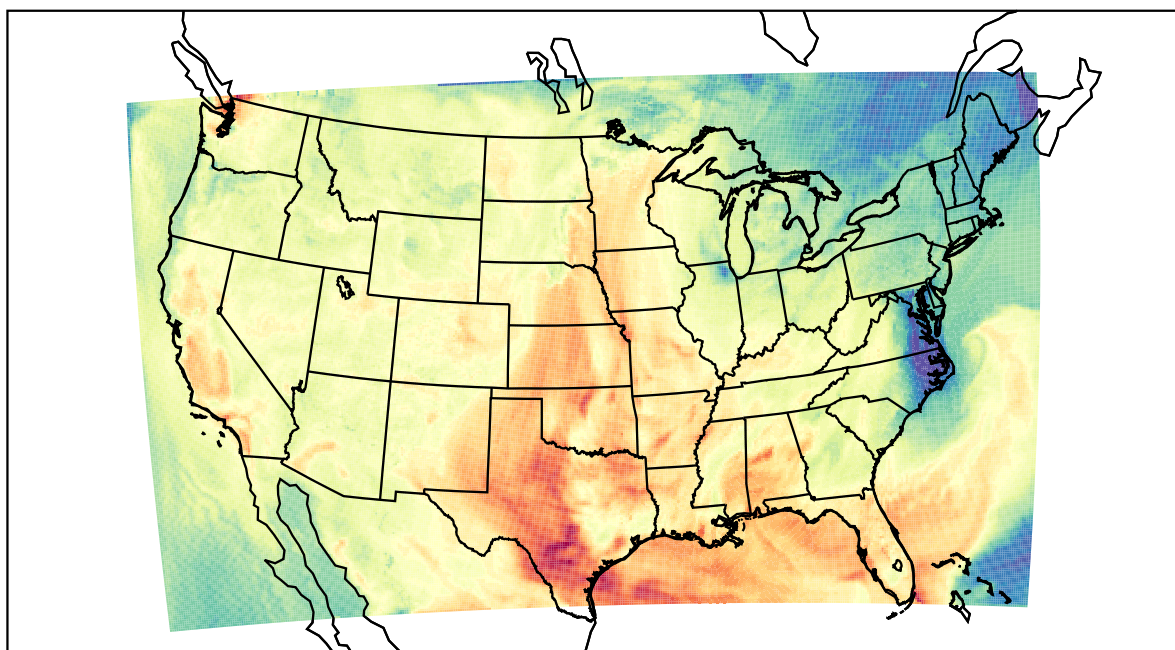
WRF (2022-10-03_21:00:00)
