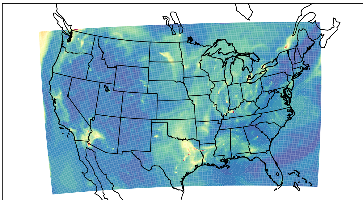
WRF 2022-10-05_16:00:00
