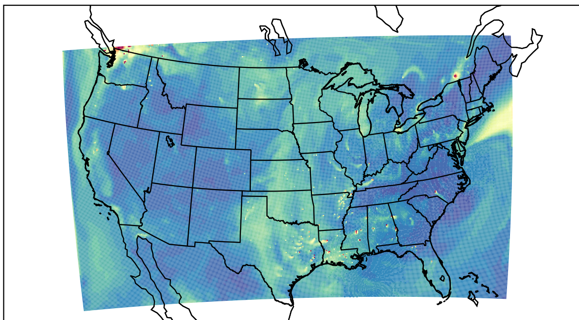
WRF 2022-10-04_21:00:00
