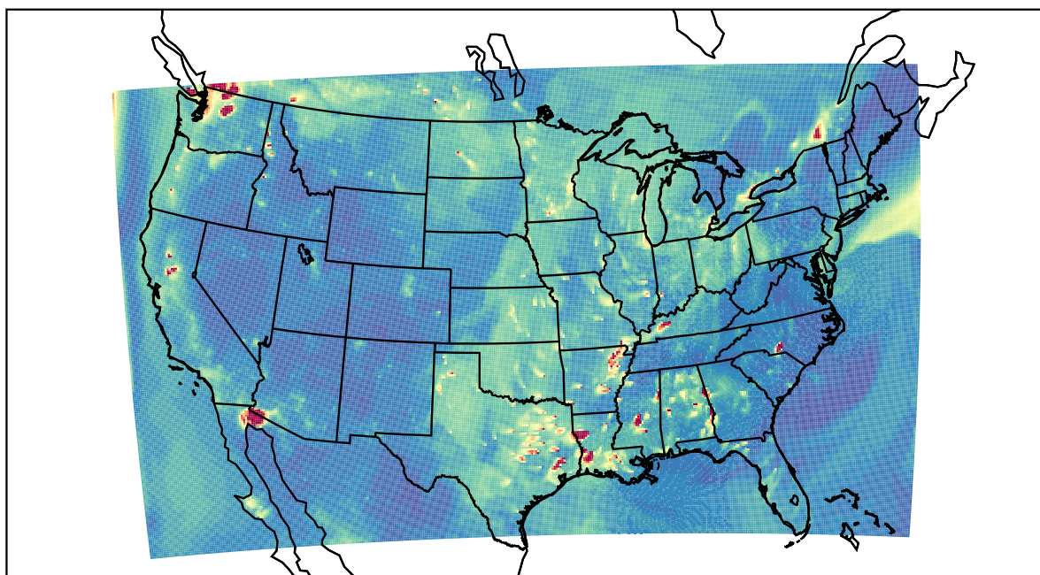
WRF 2022-10-05_02:00:00
