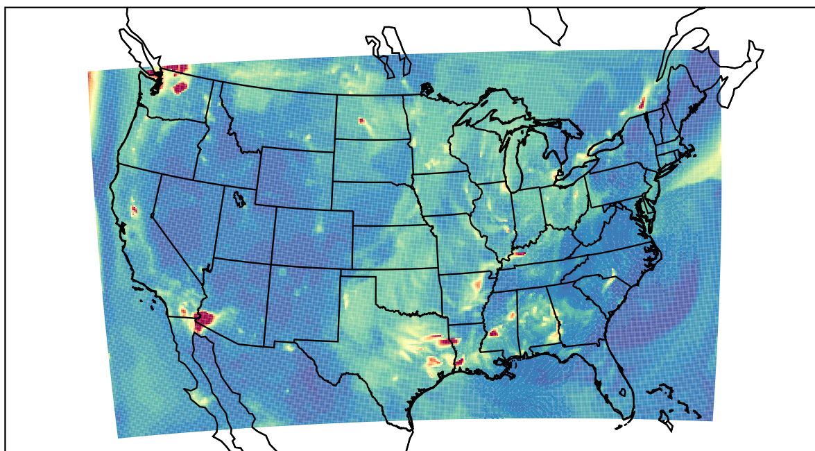
WRF 2022-10-05_05:00:00
