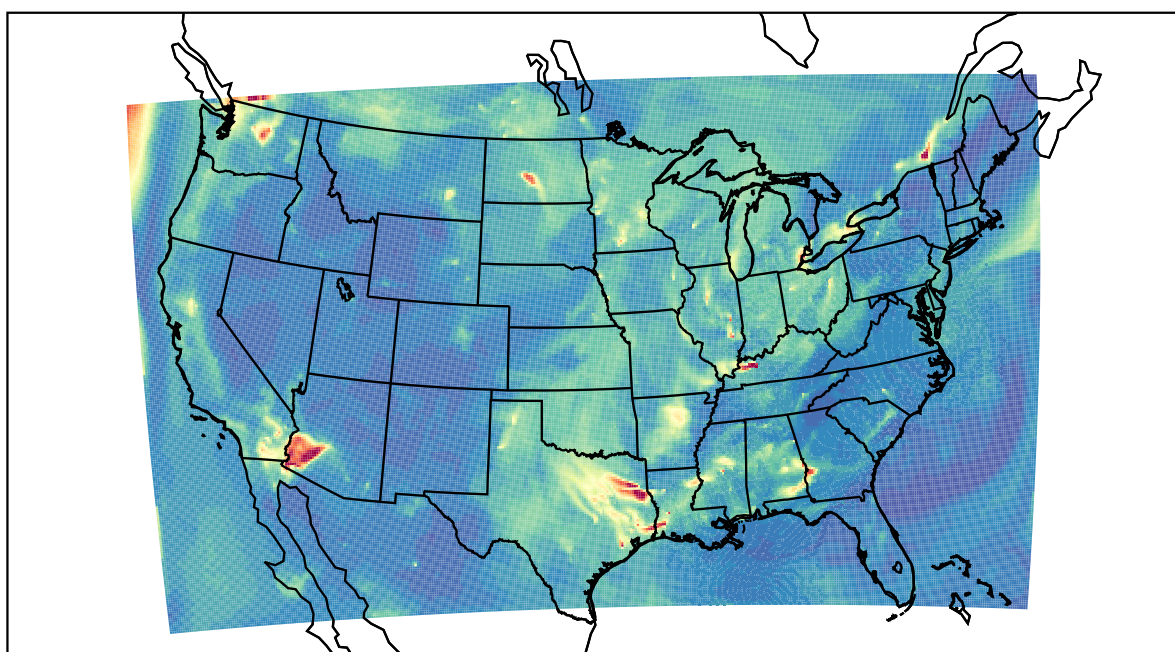
WRF 2022-10-05_09:00:00
