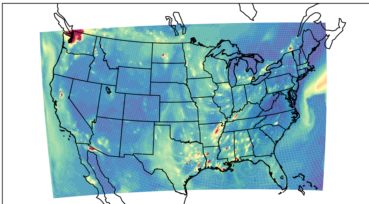
WRF 2022-10-04_03:00:00
