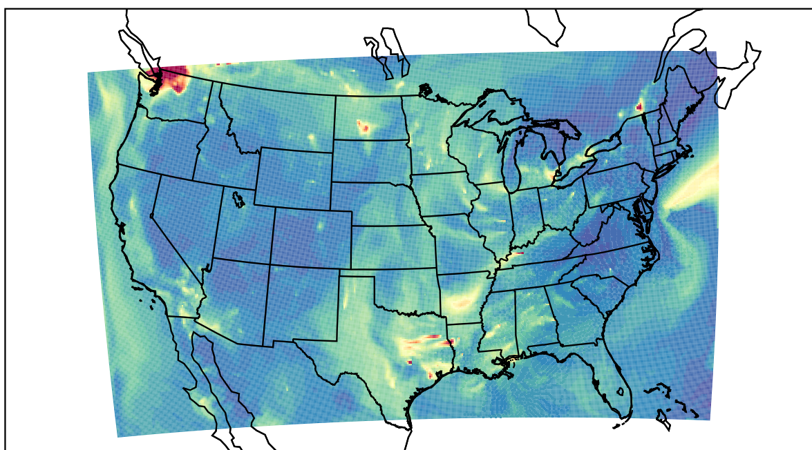
WRF 2022-10-04_08:00:00
