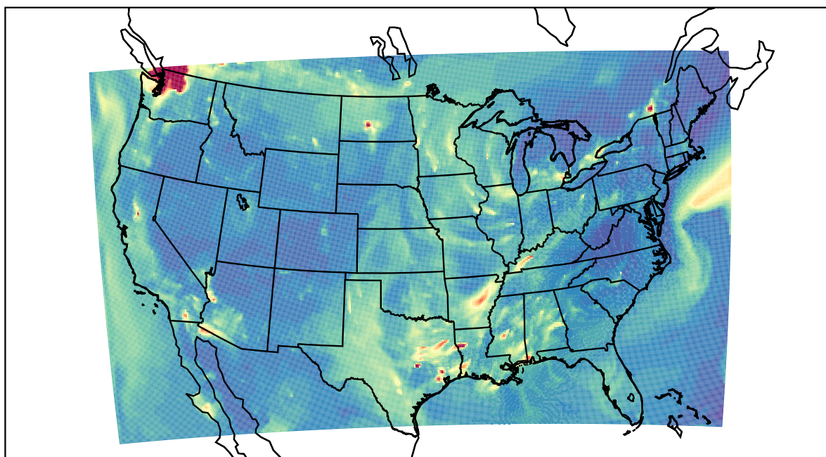
WRF 2022-10-04_05:00:00
