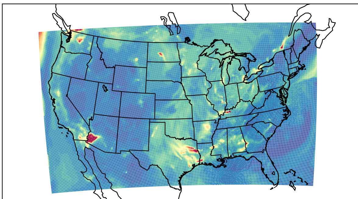
WRF 2022-10-05_08:00:00
