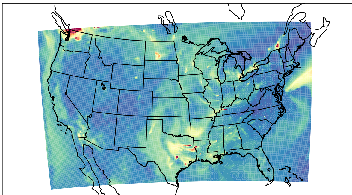
WRF 2022-10-04_11:00:00
