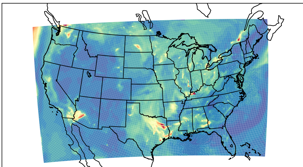
WRF 2022-10-05_11:00:00
