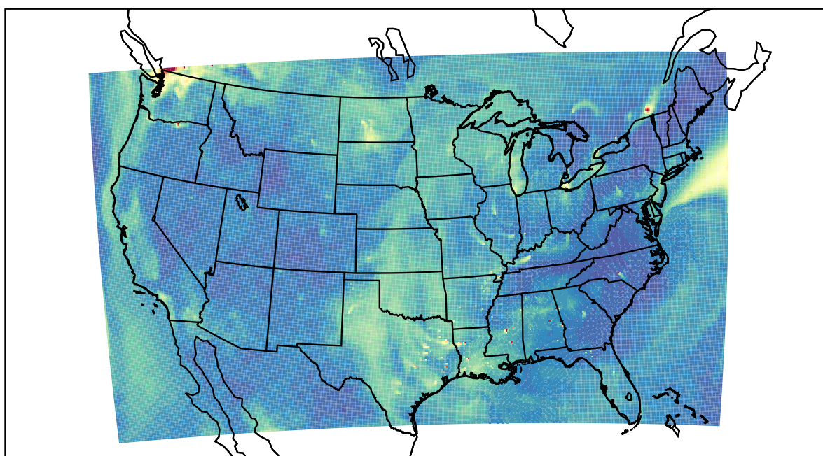
WRF 2022-10-04_19:00:00
