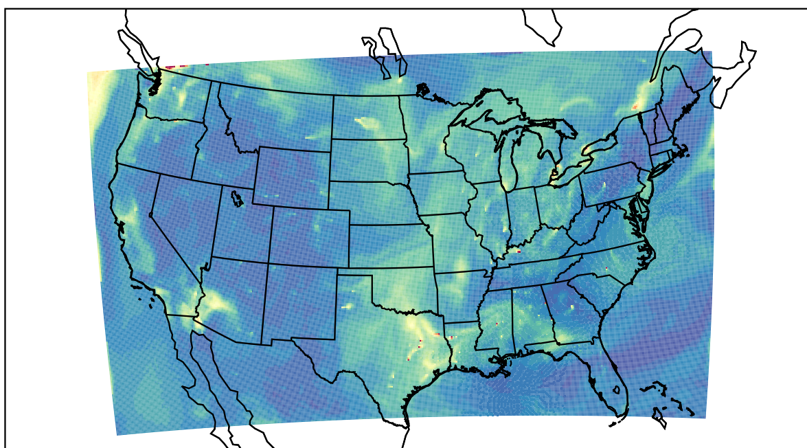
WRF 2022-10-05_17:00:00
