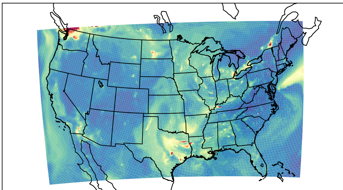
WRF 2022-10-04_12:00:00
