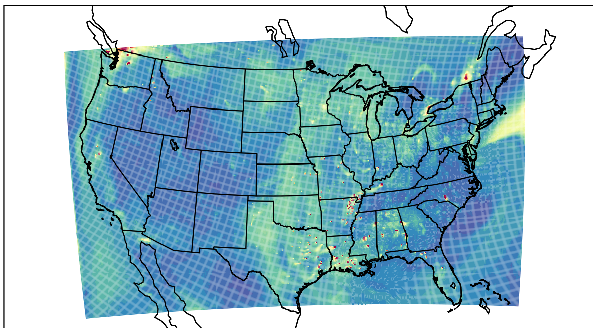
WRF 2022-10-04_23:00:00
