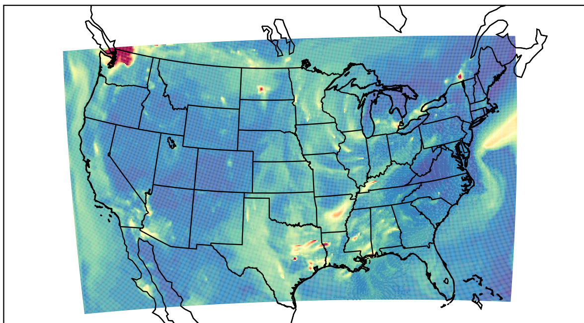
WRF 2022-10-04_06:00:00
