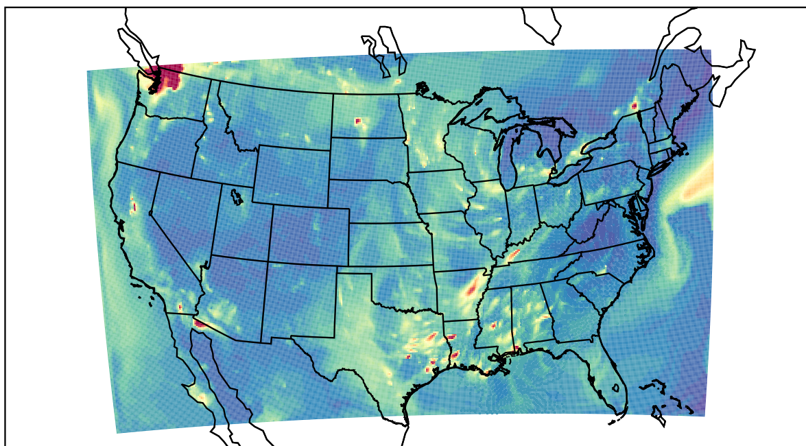
WRF 2022-10-04_04:00:00
