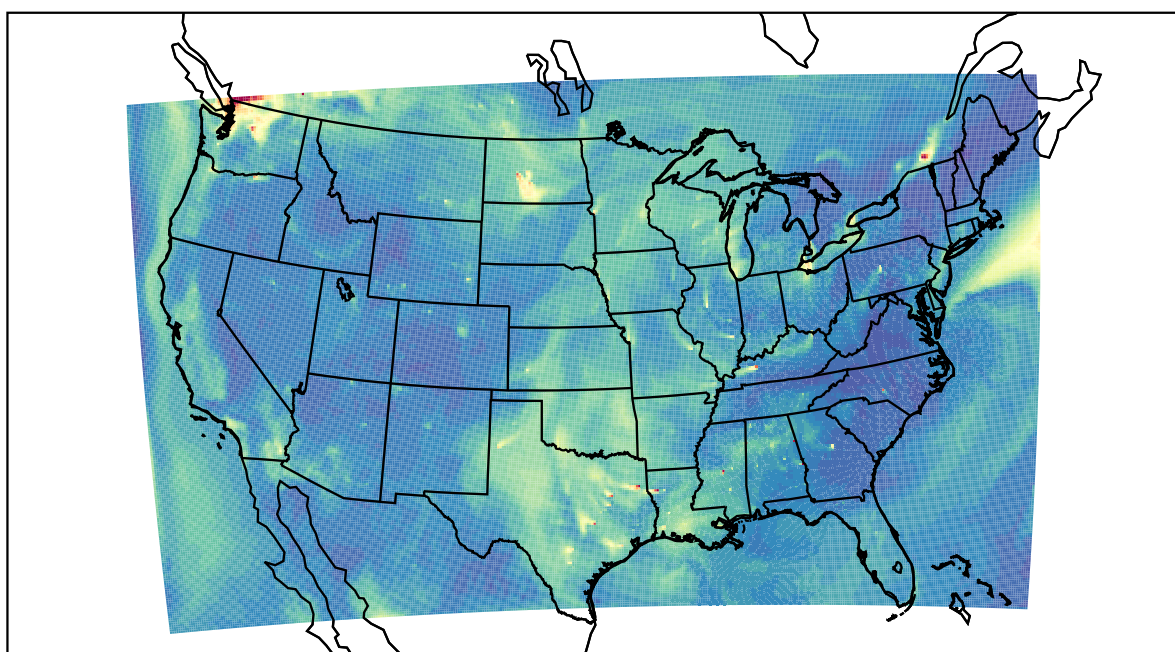
WRF 2022-10-04_17:00:00
