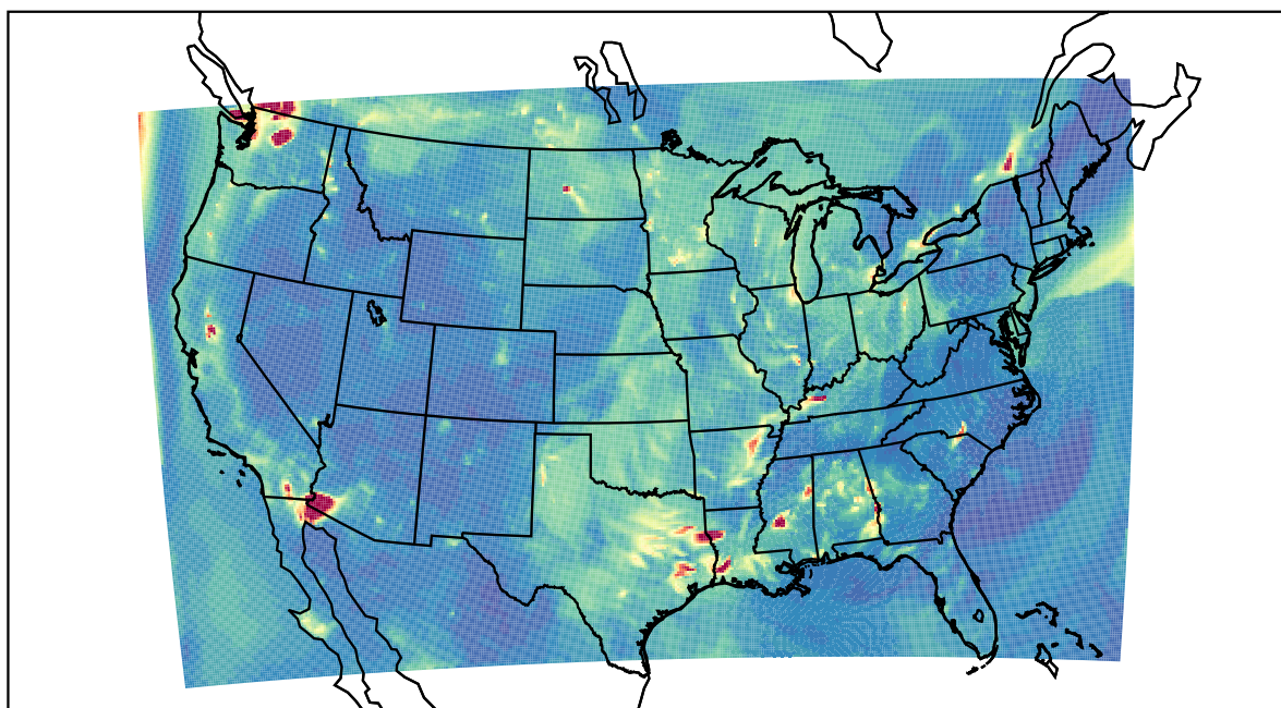
WRF 2022-10-05_04:00:00
