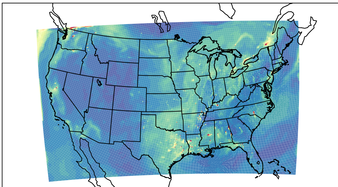
WRF 2022-10-05_22:00:00
