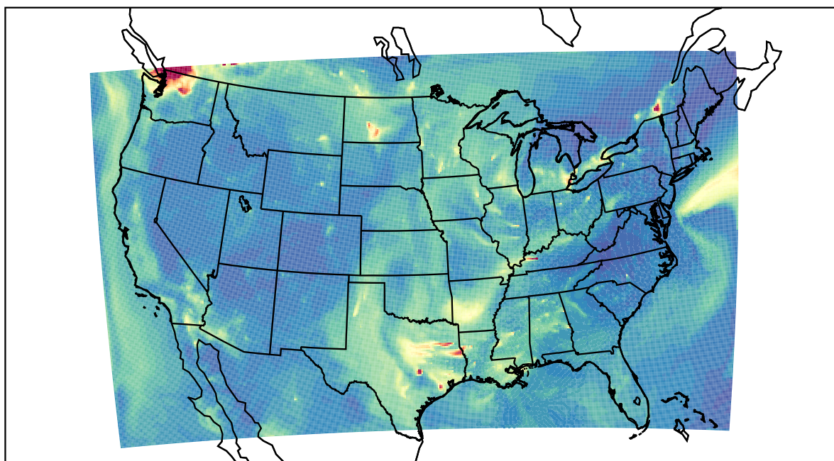
WRF 2022-10-04_10:00:00
