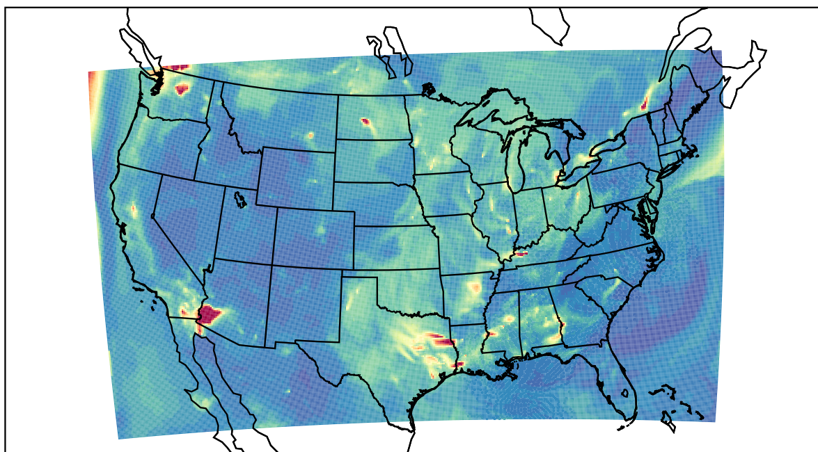
WRF 2022-10-05_07:00:00
