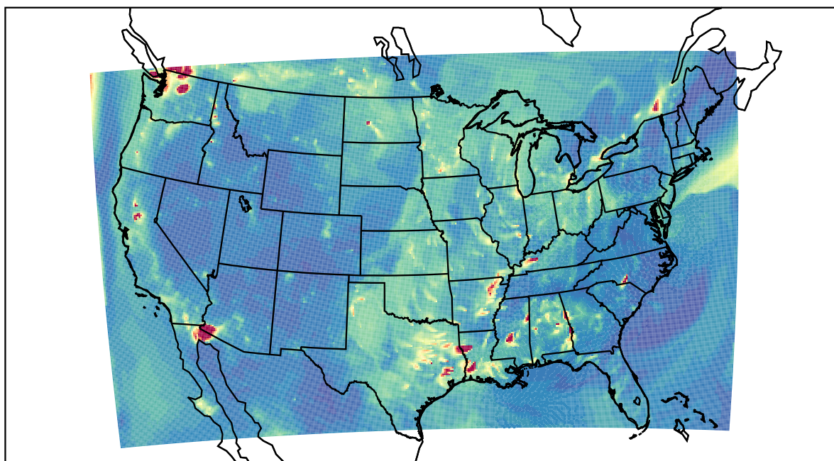
WRF 2022-10-05_03:00:00
