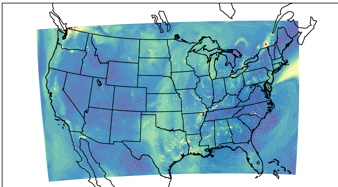
WRF 2022-10-04_22:00:00
