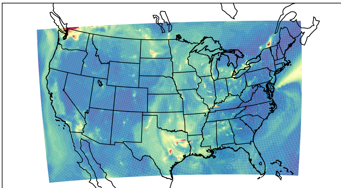
WRF 2022-10-04_14:00:00
