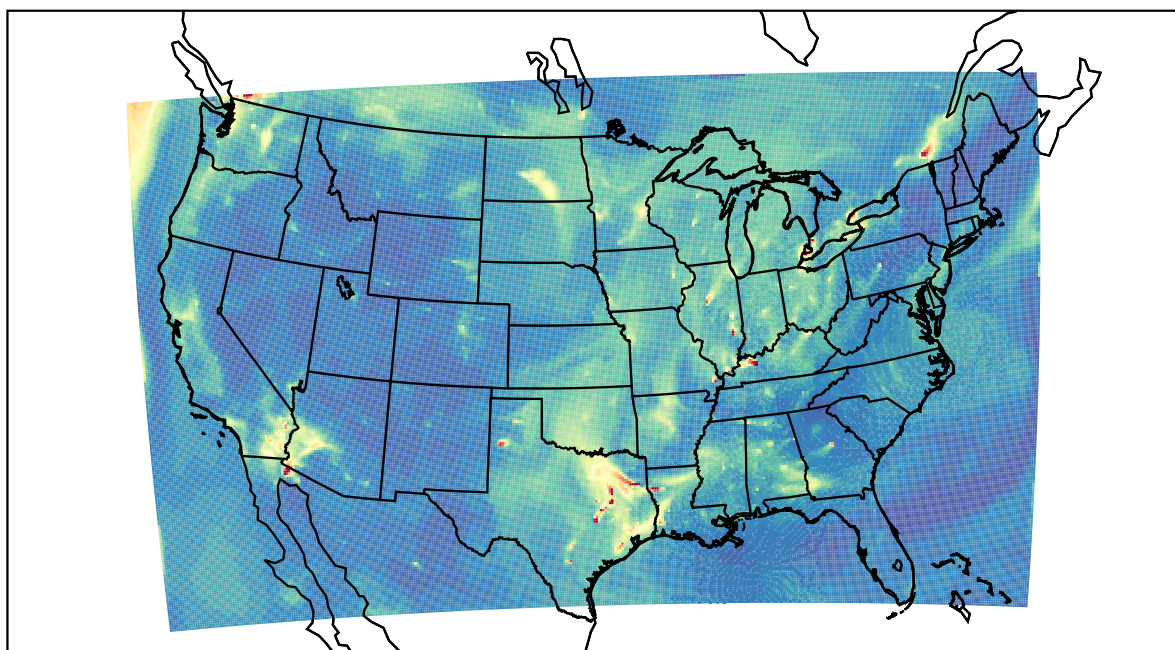
WRF 2022-10-05_15:00:00
