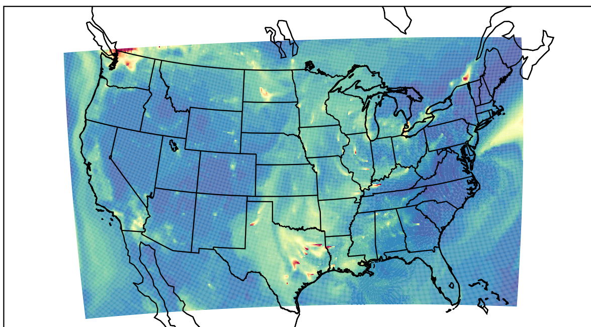
WRF 2022-10-04_15:00:00
