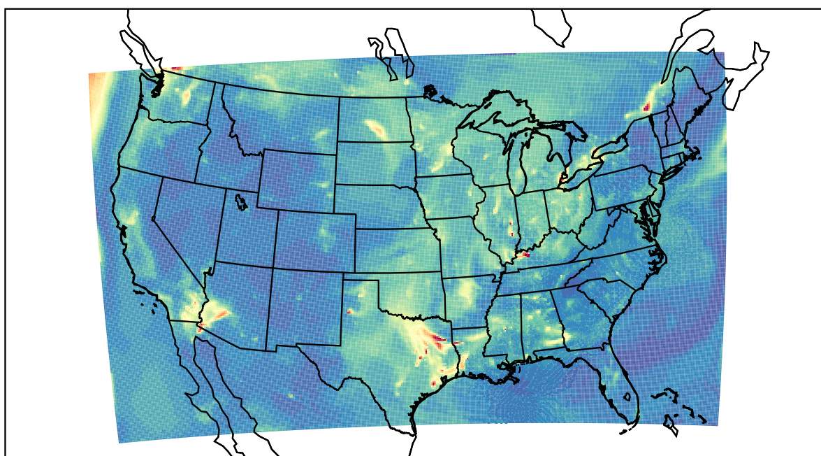
WRF 2022-10-05_13:00:00
