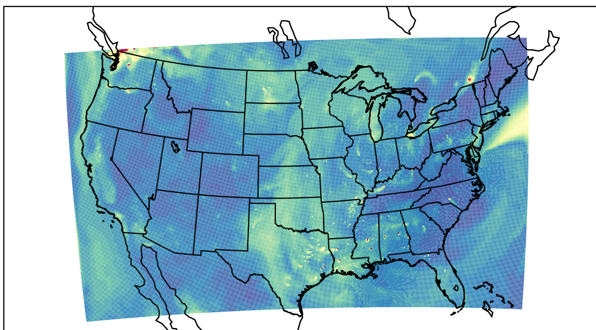
WRF 2022-10-04_20:00:00
