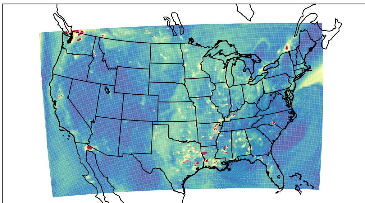
WRF 2022-10-05_01:00:00
