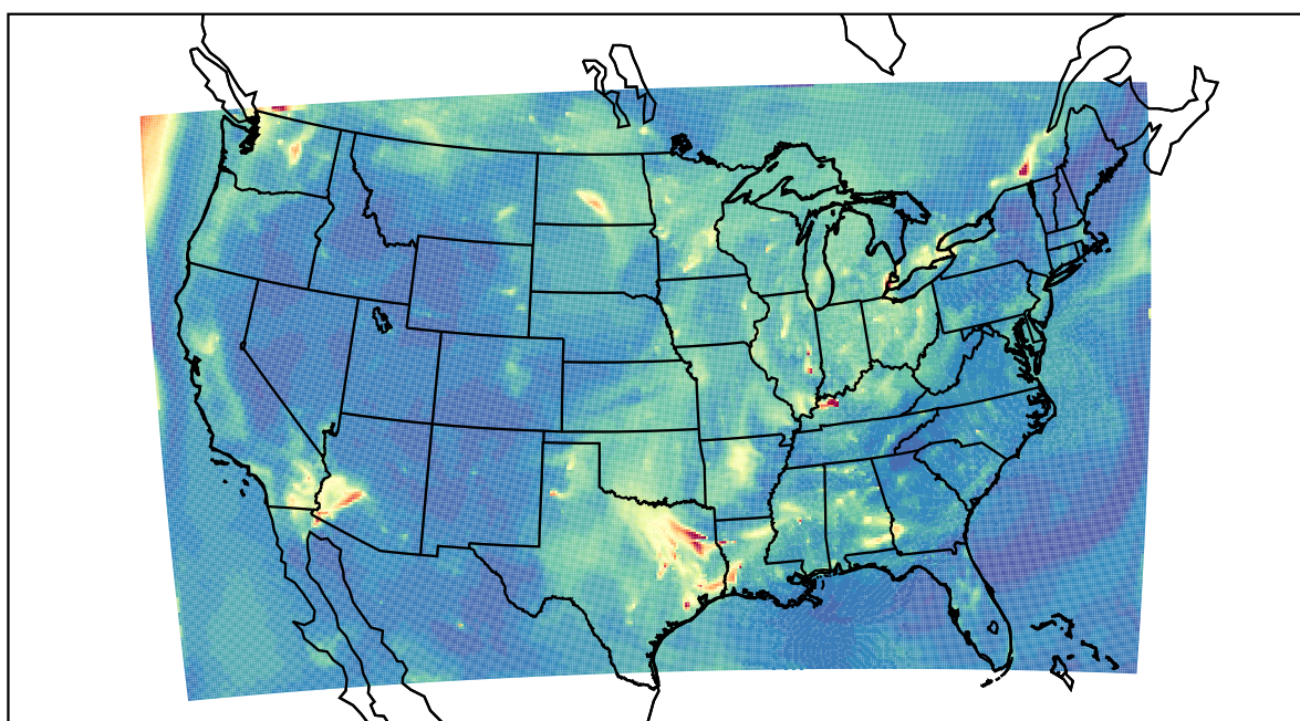
WRF 2022-10-05_12:00:00
