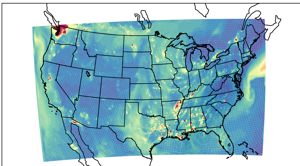
WRF 2022-10-04_02:00:00
