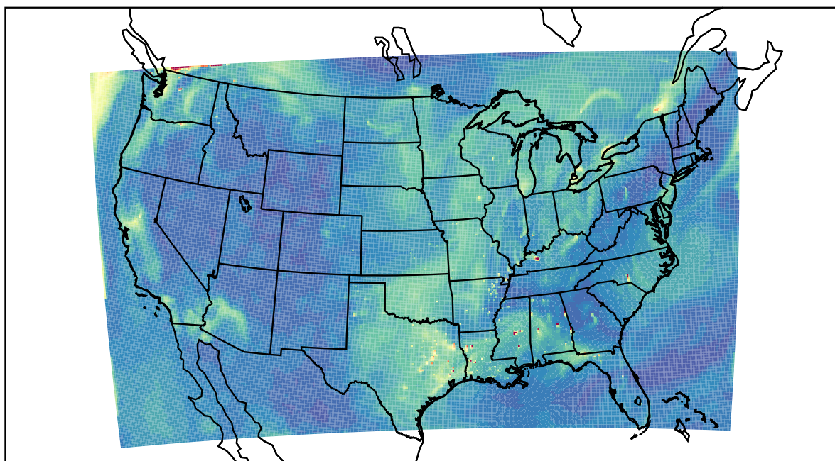
WRF 2022-10-05_20:00:00
