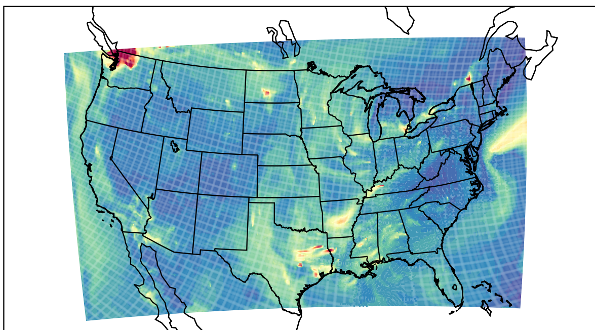
WRF 2022-10-04_07:00:00
