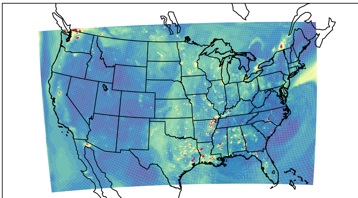
WRF 2022-10-05_00:00:00
