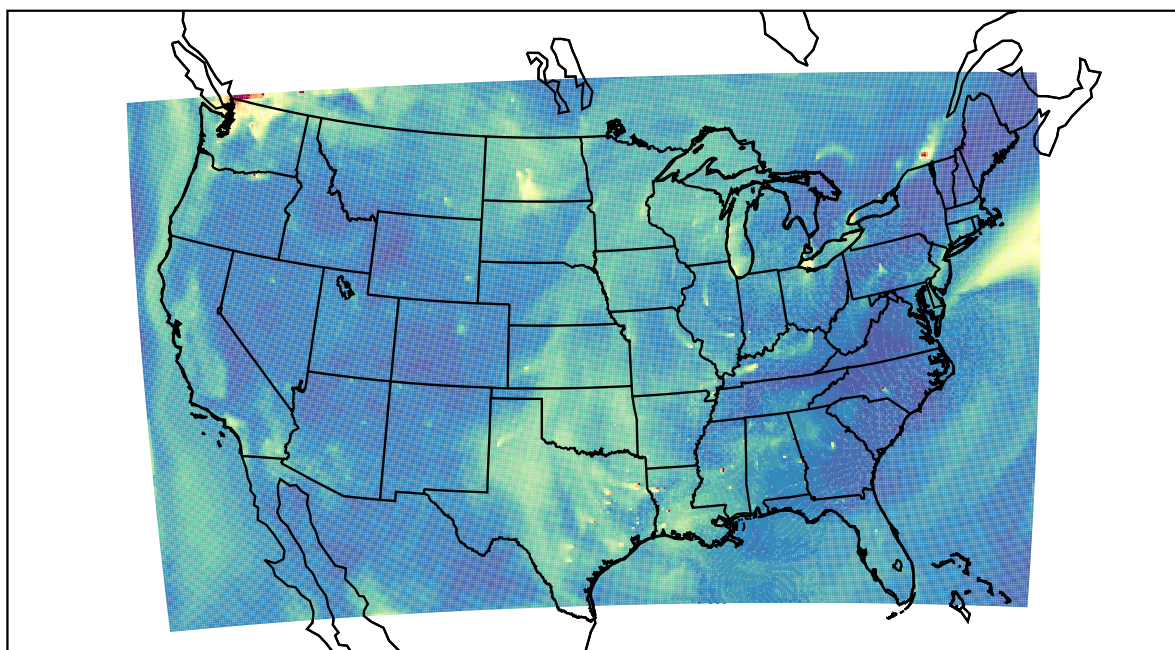
WRF 2022-10-04_18:00:00
