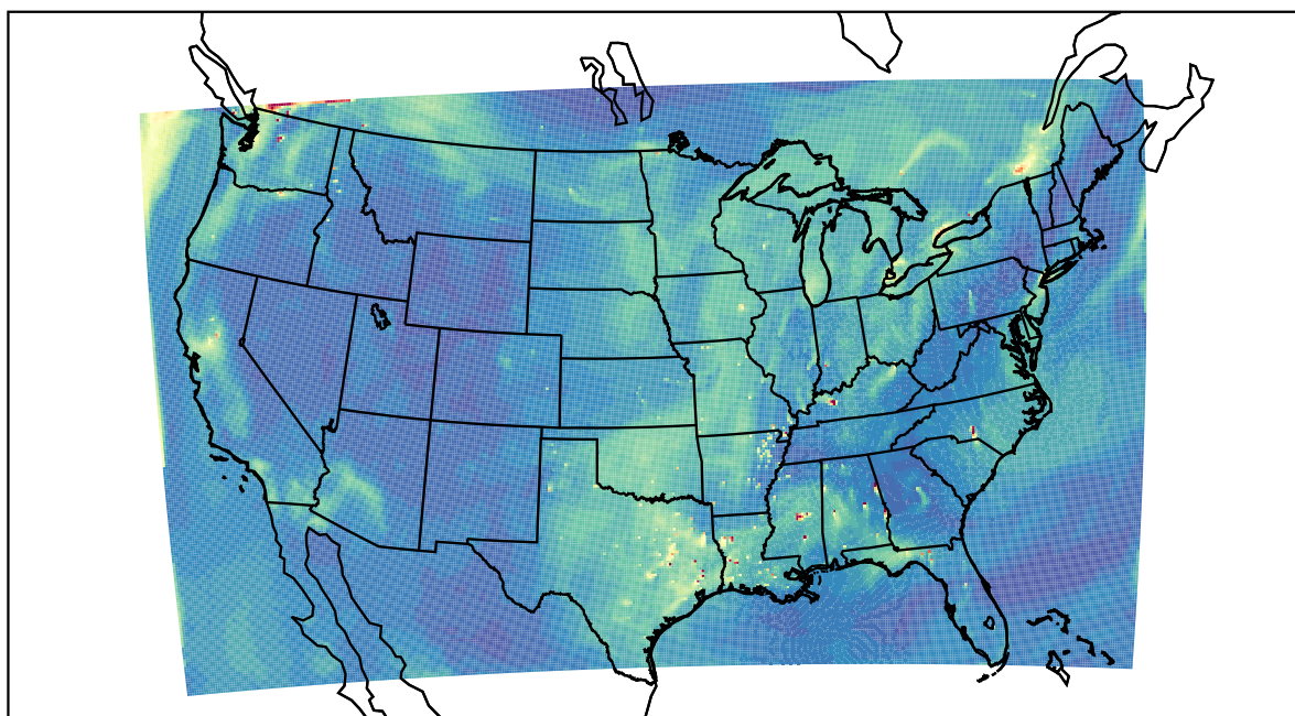
WRF 2022-10-05_21:00:00
