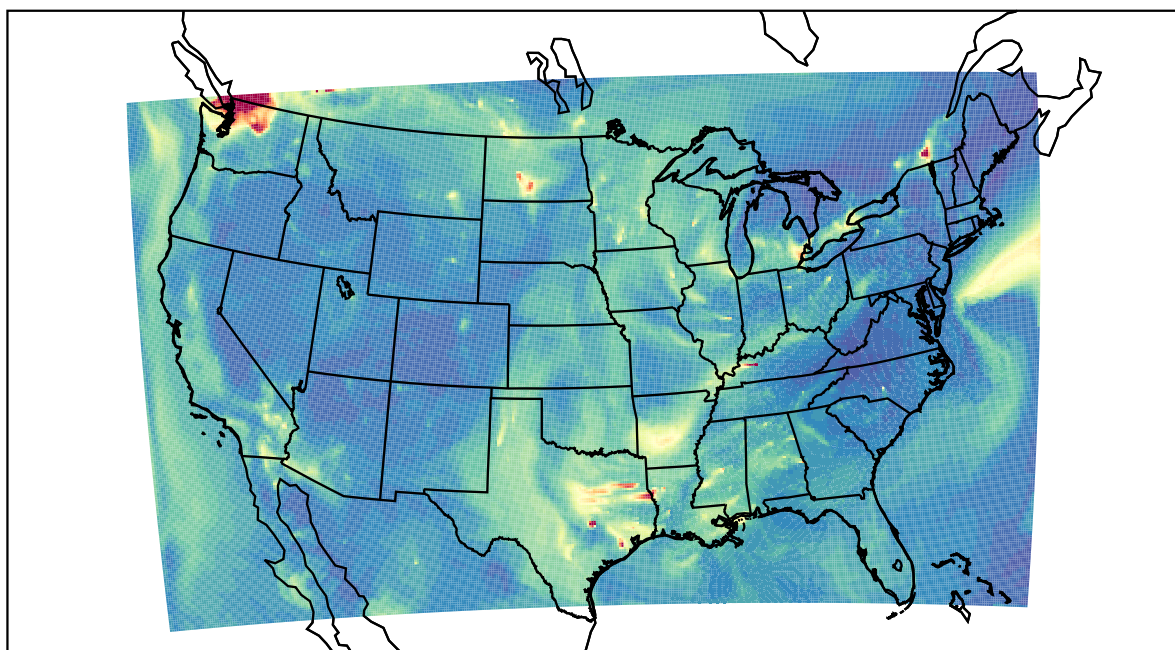
WRF 2022-10-04_09:00:00
