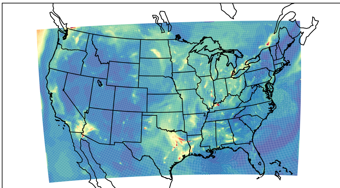
WRF 2022-10-05_14:00:00
