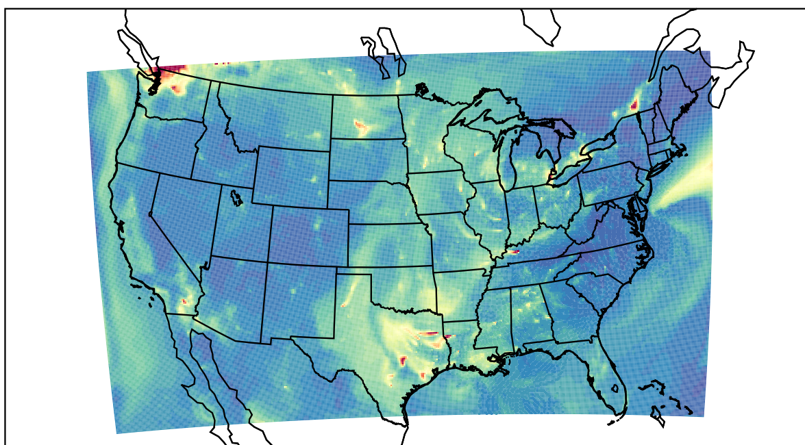
WRF 2022-10-04_13:00:00
