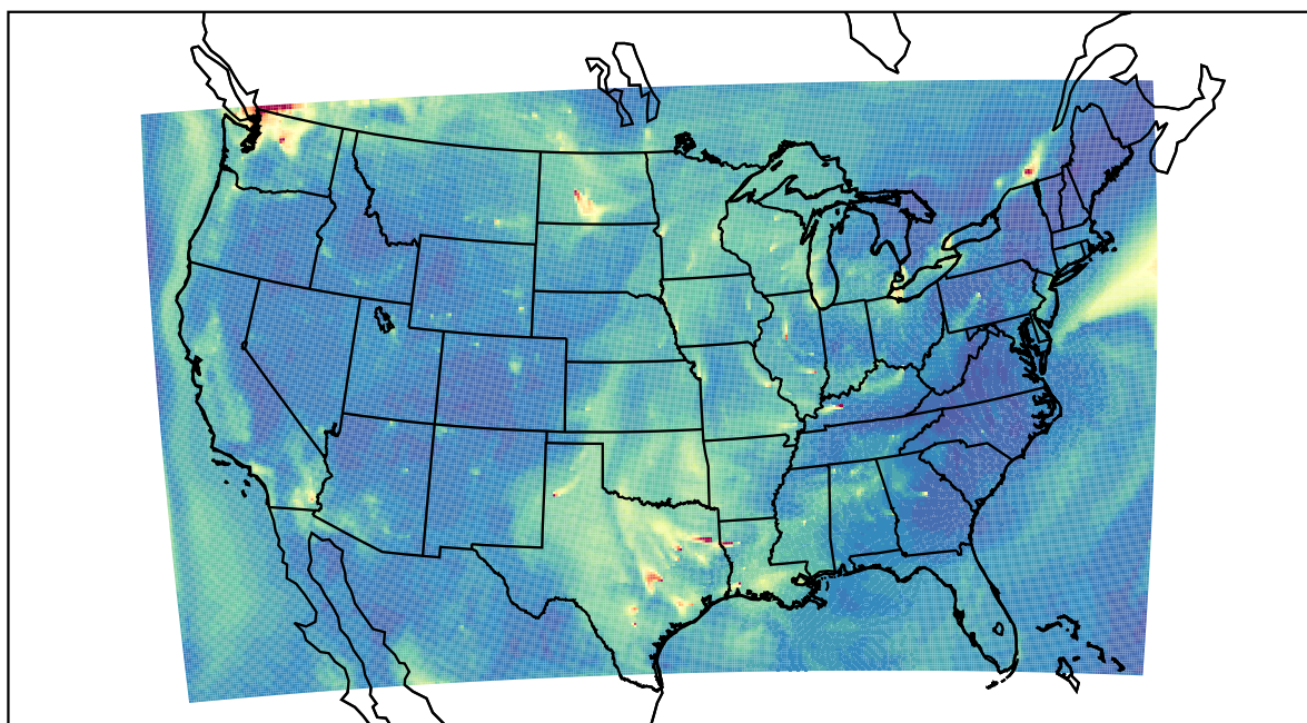
WRF 2022-10-04_16:00:00
