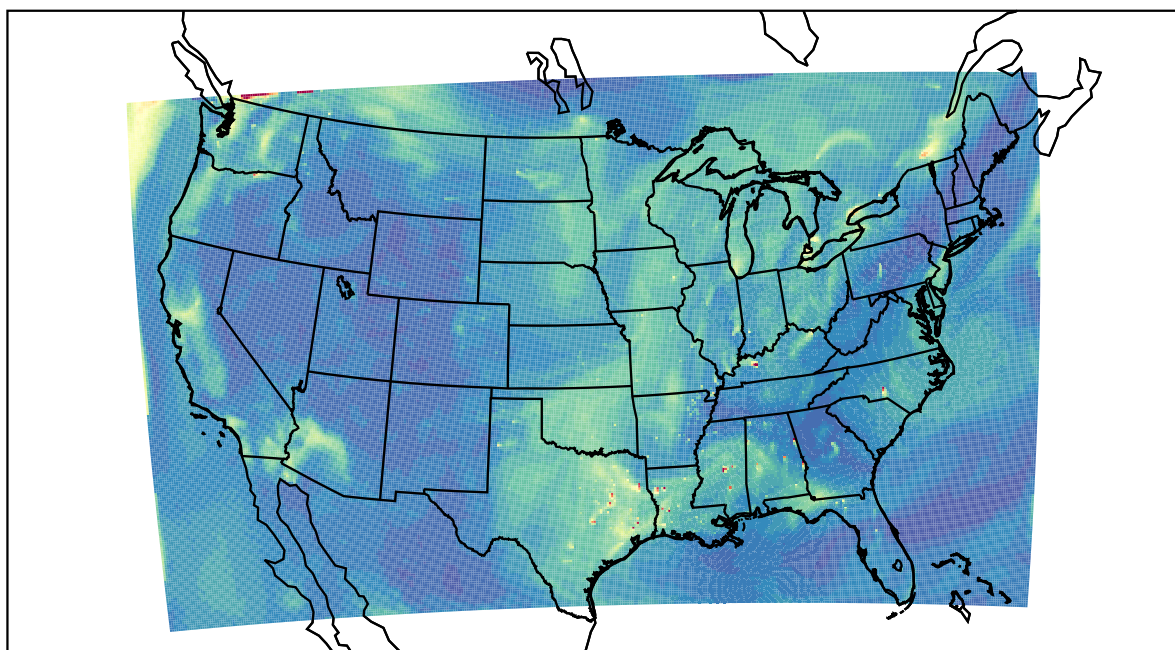
WRF 2022-10-05_19:00:00
