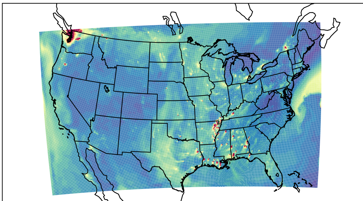
WRF 2022-10-04_00:00:00
