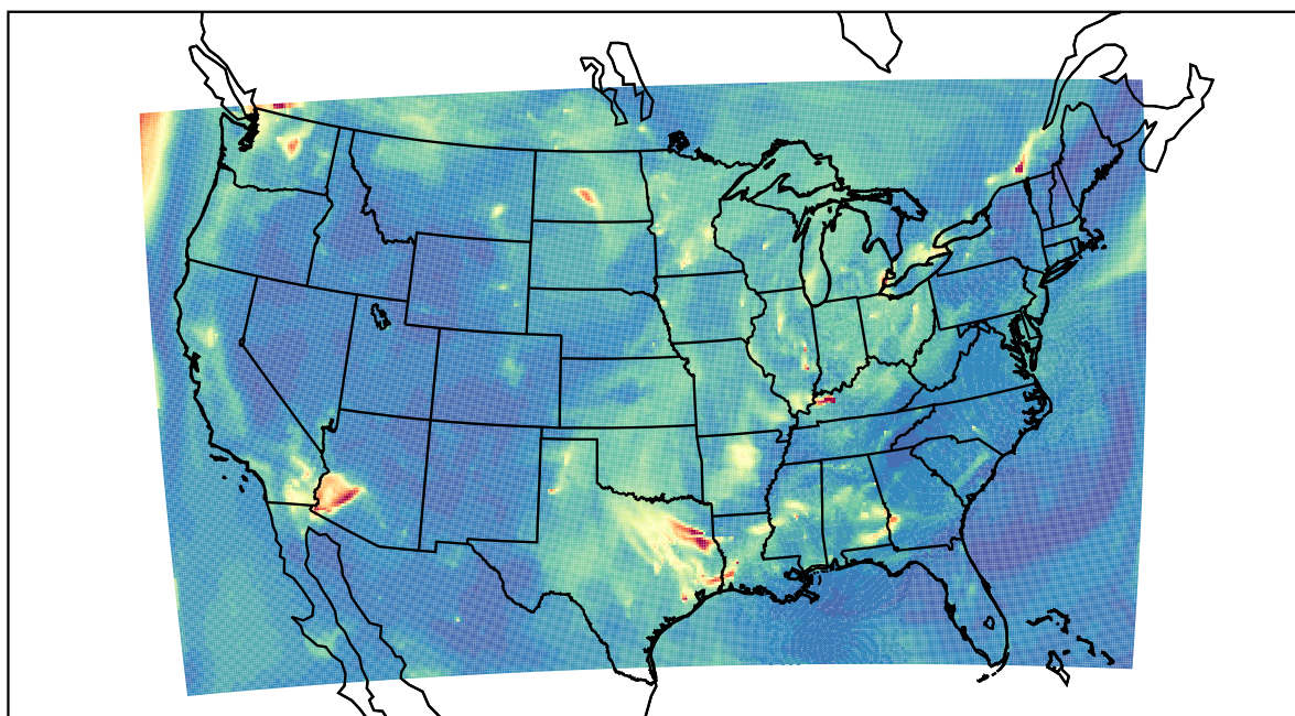
WRF 2022-10-05_10:00:00
