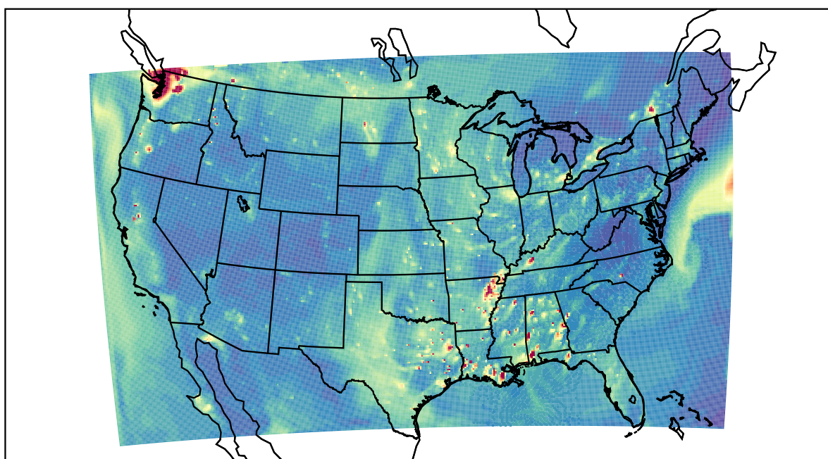
WRF 2022-10-04_01:00:00
