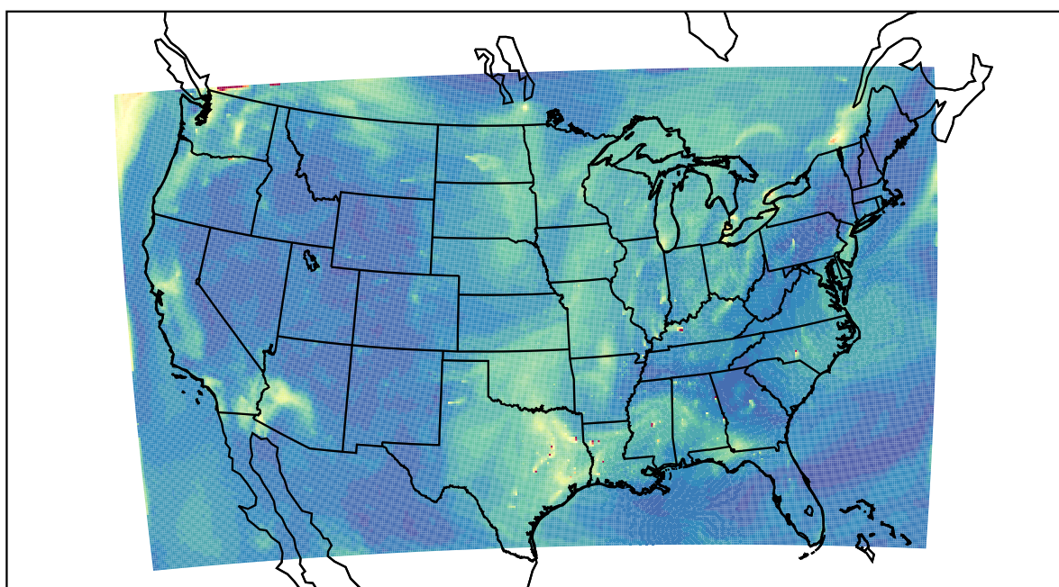
WRF 2022-10-05_18:00:00
