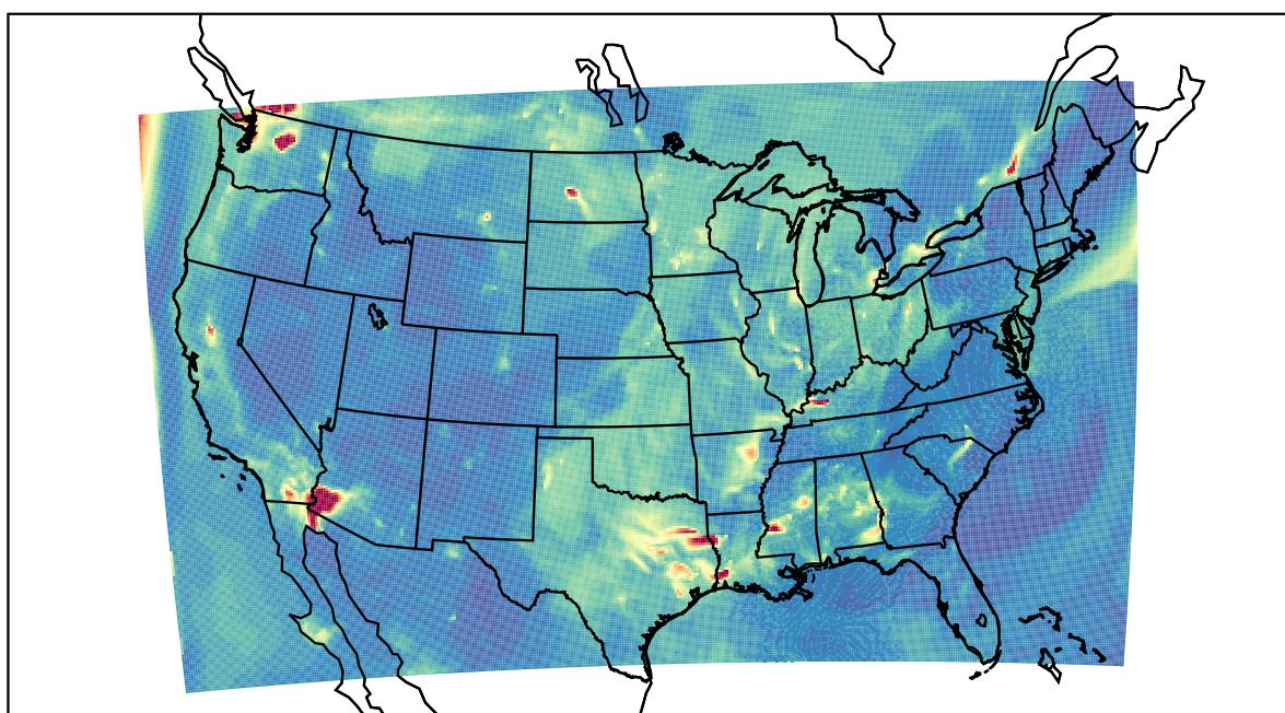
WRF 2022-10-05_06:00:00
