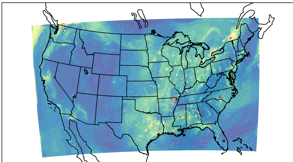
WRF 2022-10-05_23:00:00
