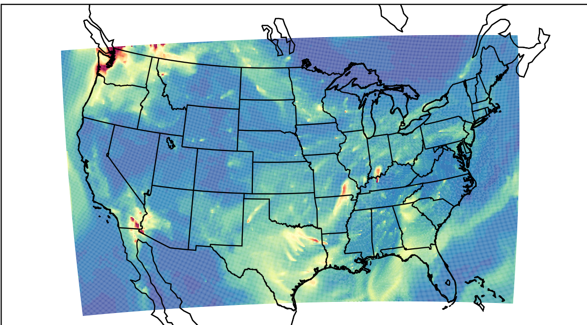
WRF 2022-10-09_14:00:00
