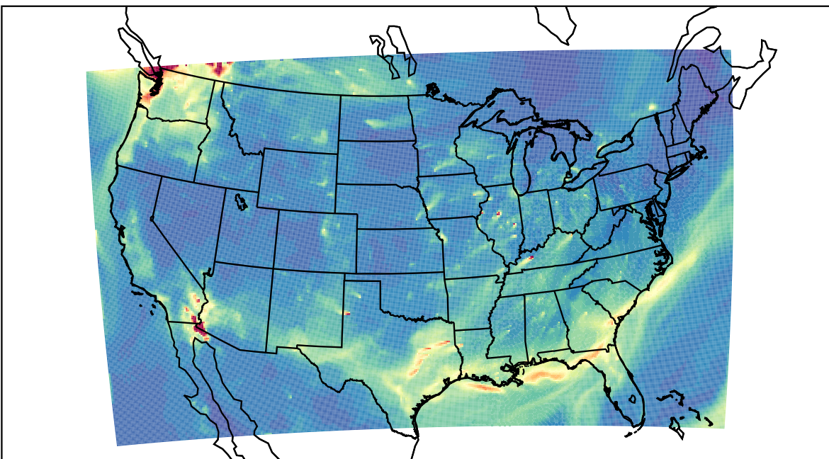
WRF 2022-10-08_14:00:00
