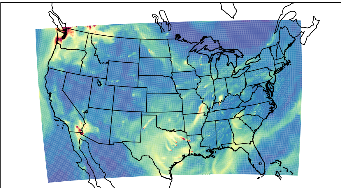
WRF 2022-10-09_15:00:00
