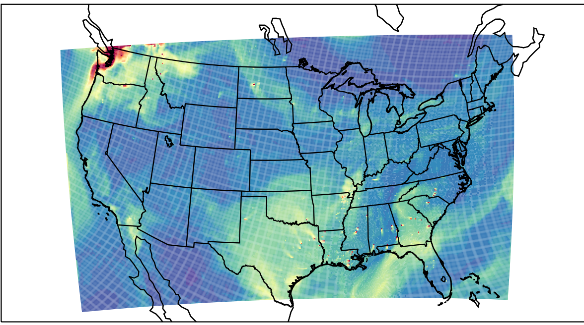
WRF 2022-10-09_19:00:00
