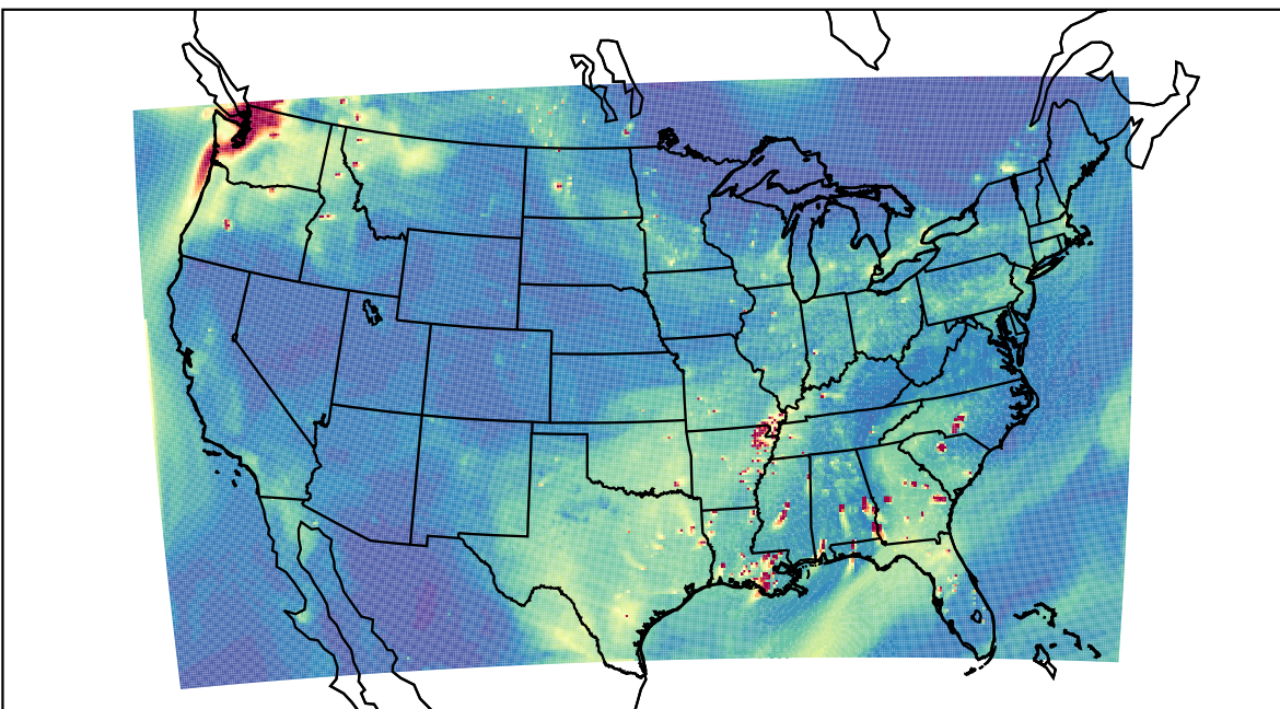
WRF 2022-10-09_23:00:00
