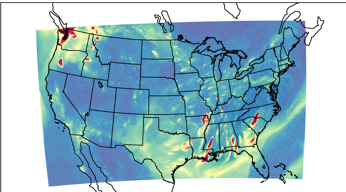
WRF 2022-10-09_03:00:00
