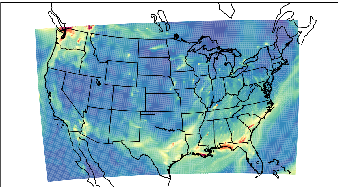
WRF 2022-10-08_10:00:00
