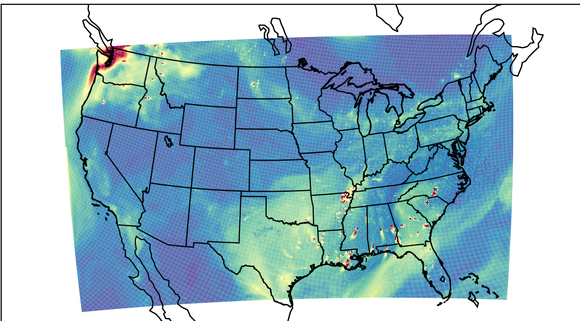
WRF 2022-10-09_22:00:00
