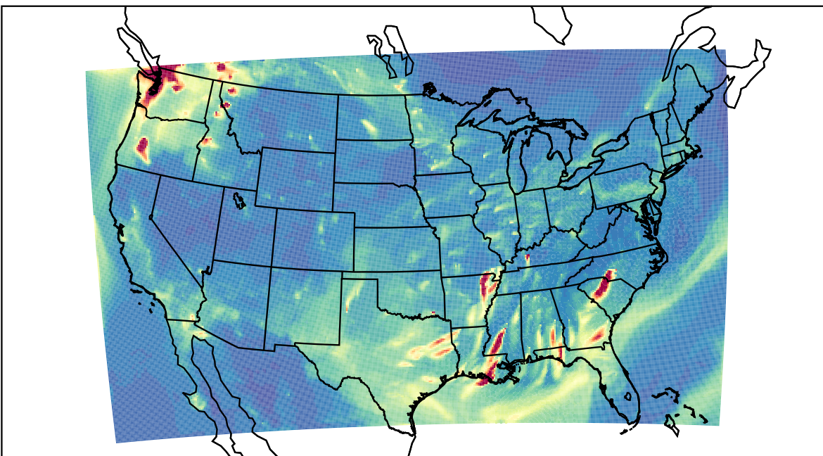
WRF 2022-10-09_04:00:00
