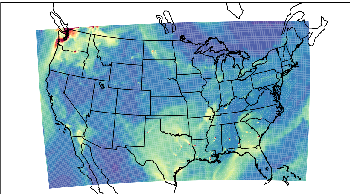
WRF 2022-10-09_18:00:00
