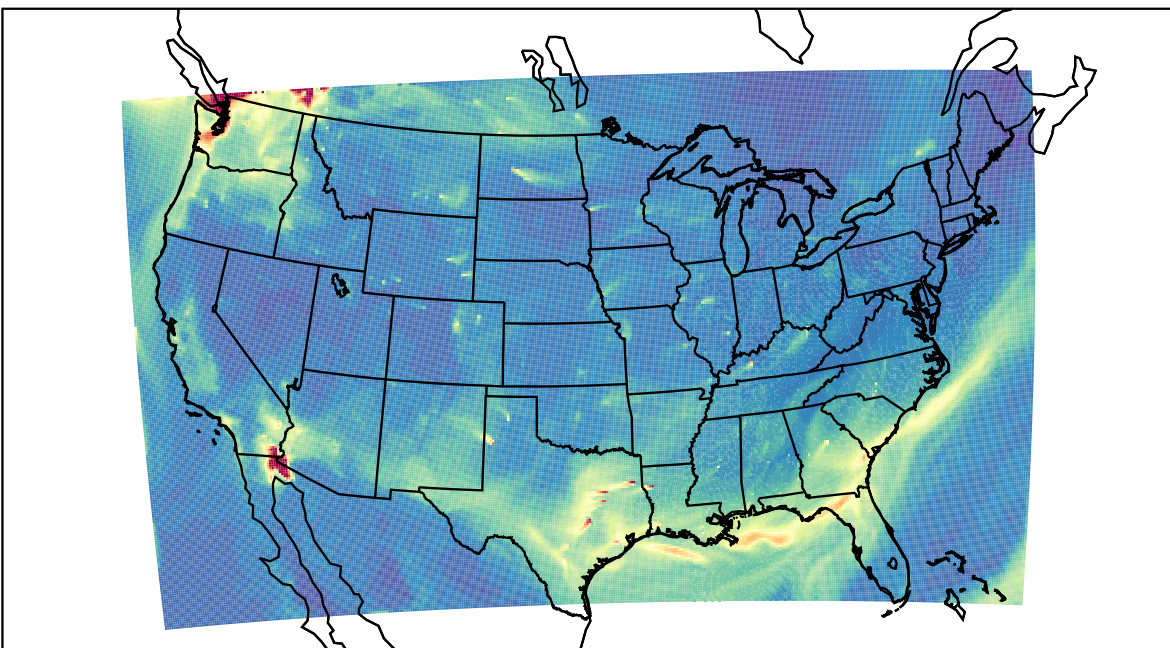
WRF 2022-10-08_16:00:00
