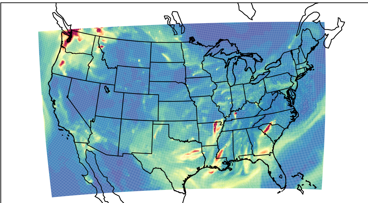
WRF 2022-10-09_06:00:00
