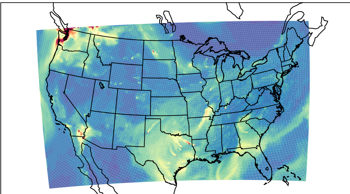
WRF 2022-10-09_16:00:00
