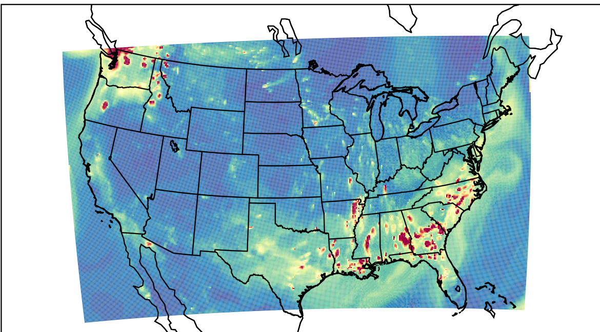
WRF 2022-10-08_02:00:00
