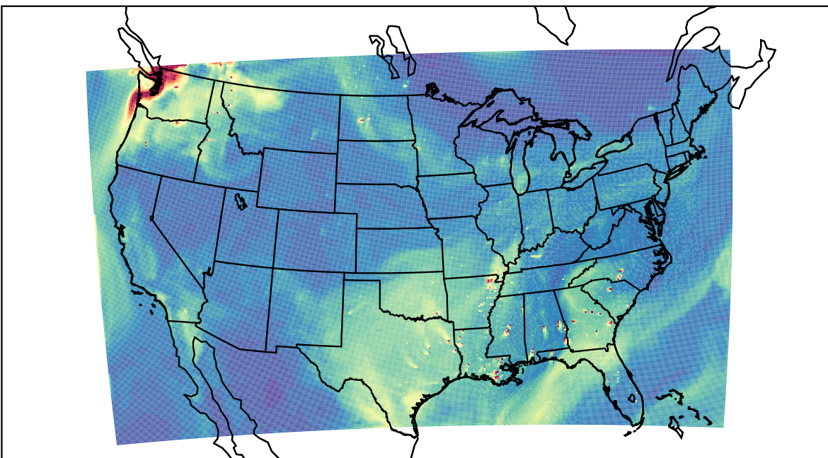
WRF 2022-10-09_20:00:00
