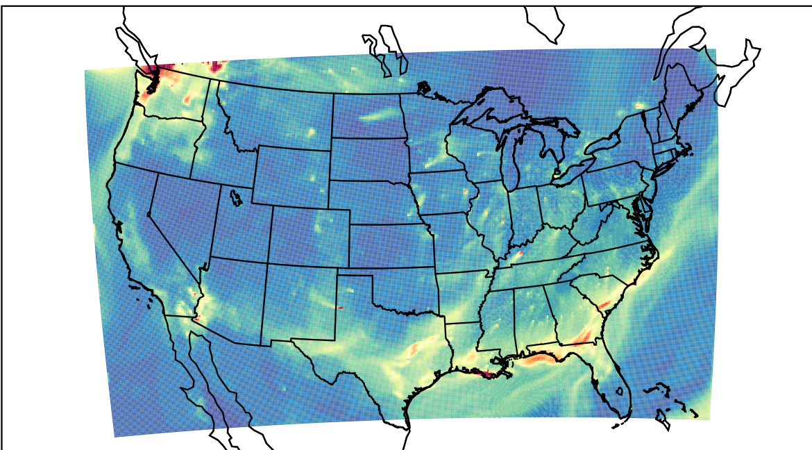
WRF 2022-10-08_11:00:00
