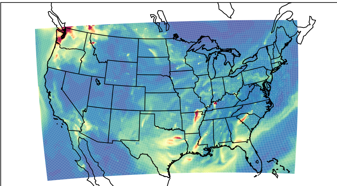
WRF 2022-10-09_08:00:00
