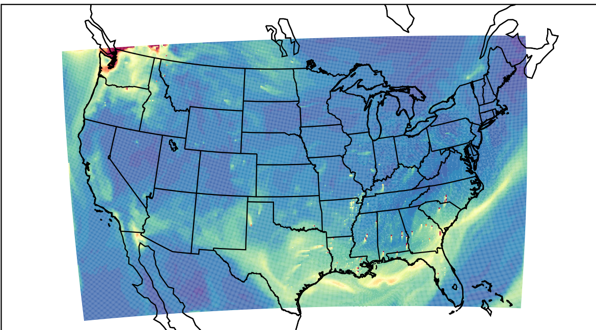
WRF 2022-10-08_19:00:00
