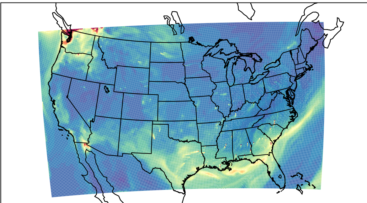
WRF 2022-10-08_18:00:00
