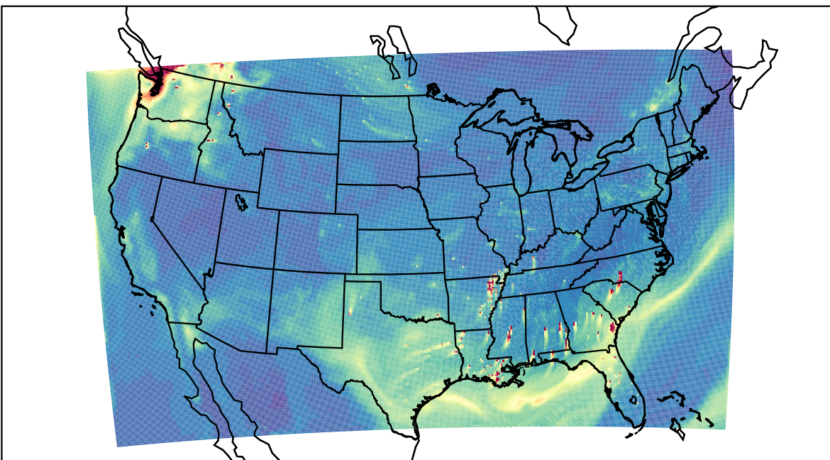
WRF 2022-10-08_22:00:00
