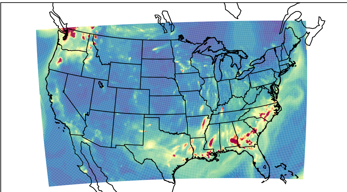
WRF 2022-10-08_04:00:00
