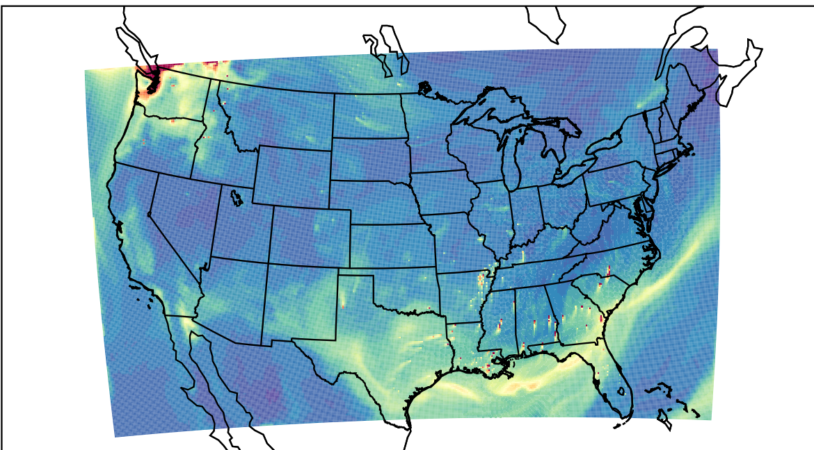
WRF 2022-10-08_20:00:00
