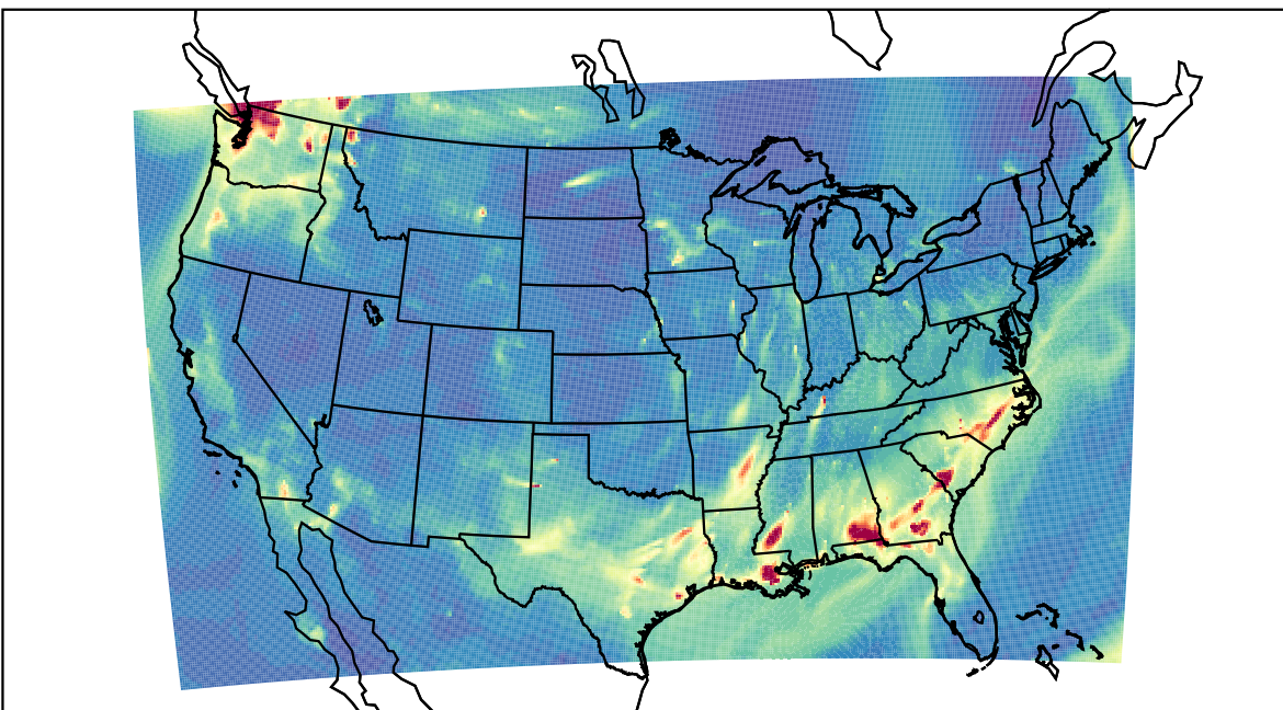
WRF 2022-10-08_06:00:00
