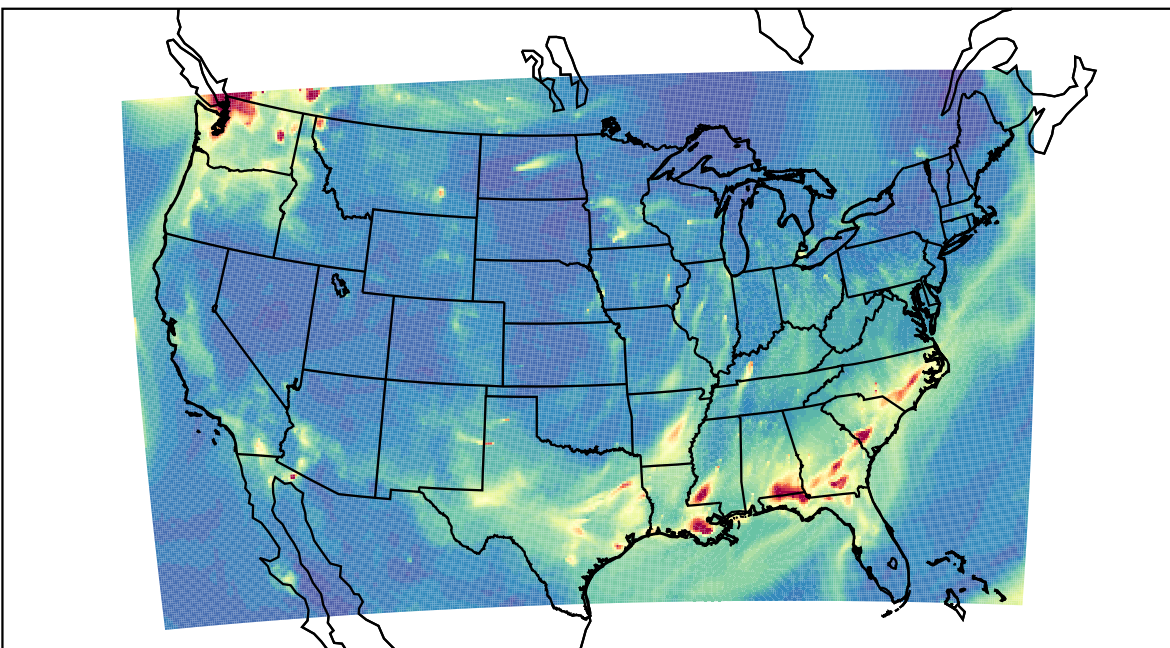
WRF 2022-10-08_07:00:00
