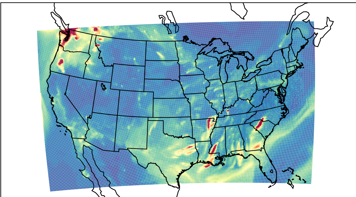
WRF 2022-10-09_05:00:00
