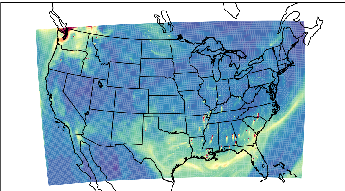
WRF 2022-10-08_21:00:00
