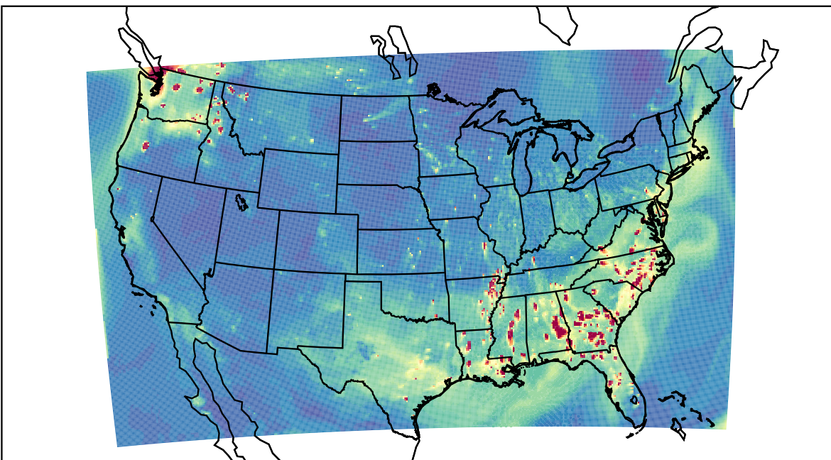
WRF 2022-10-08_00:00:00
