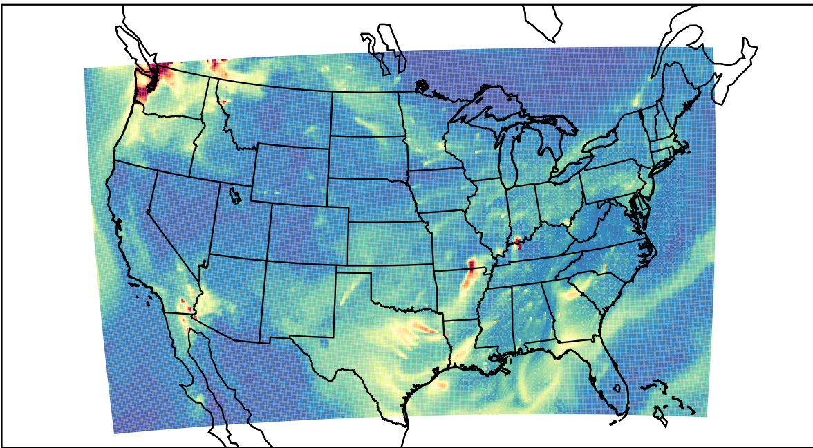
WRF 2022-10-09_11:00:00
