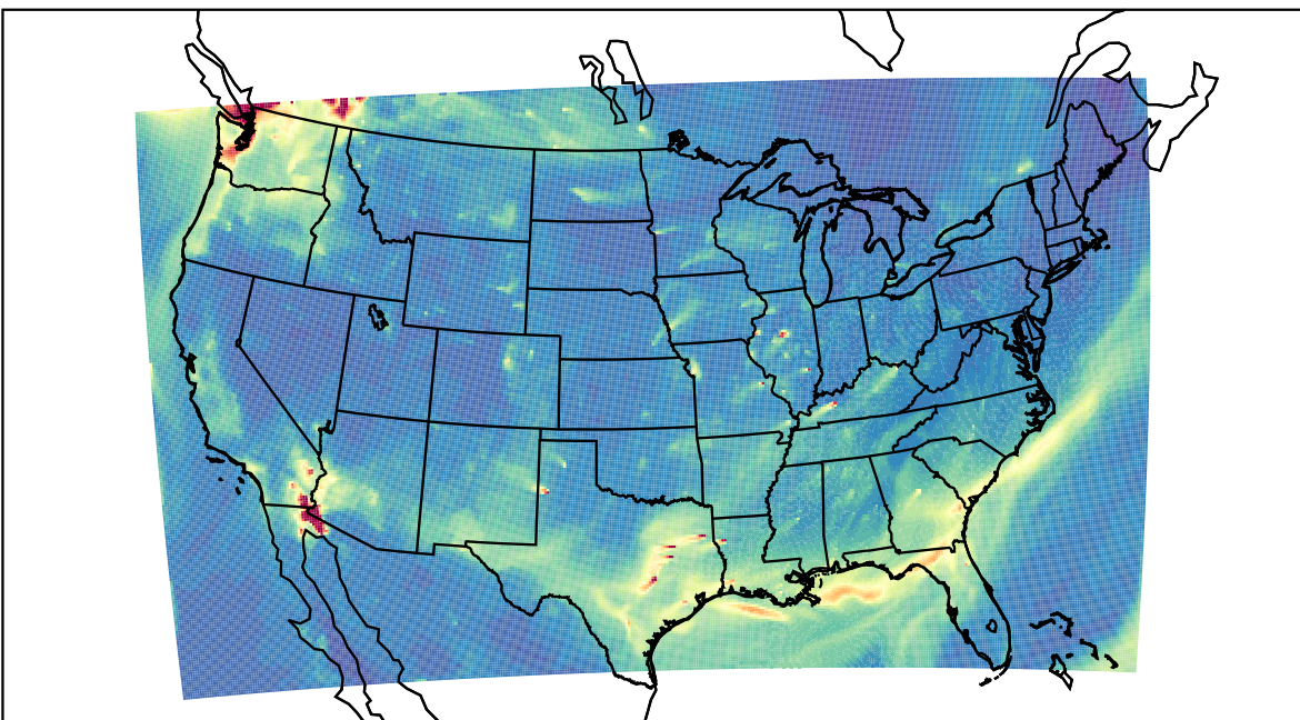
WRF 2022-10-08_15:00:00
