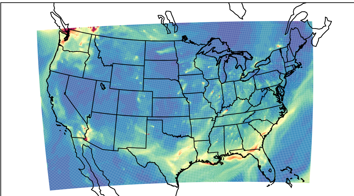
WRF 2022-10-08_12:00:00
