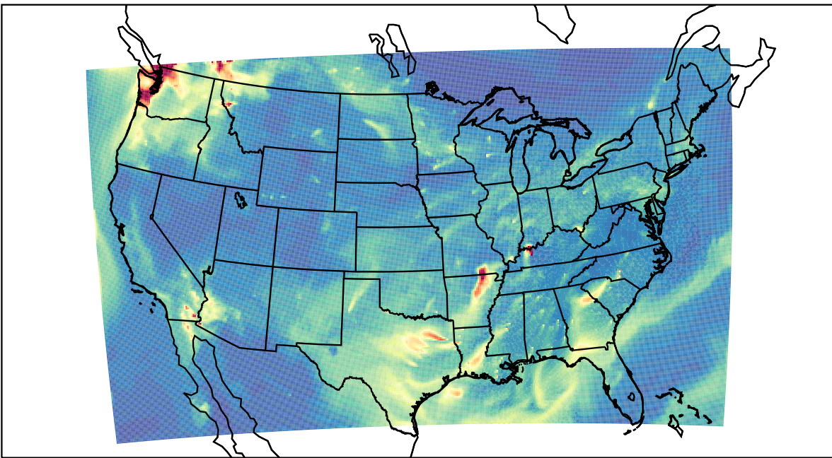
WRF 2022-10-09_10:00:00
