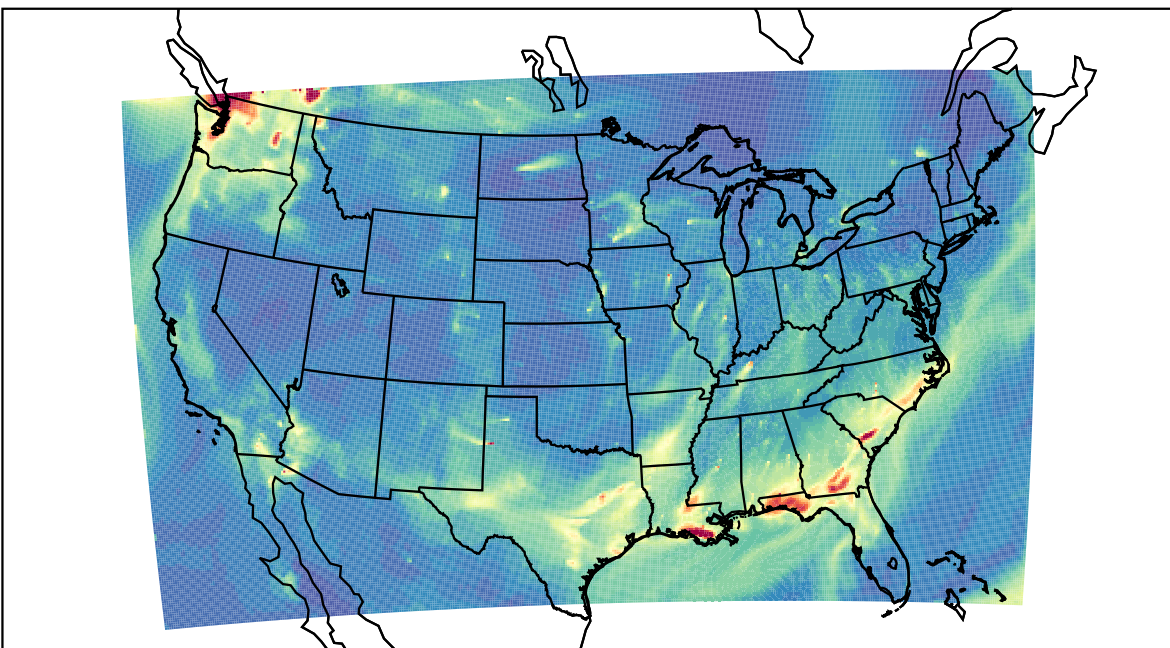
WRF 2022-10-08_09:00:00
