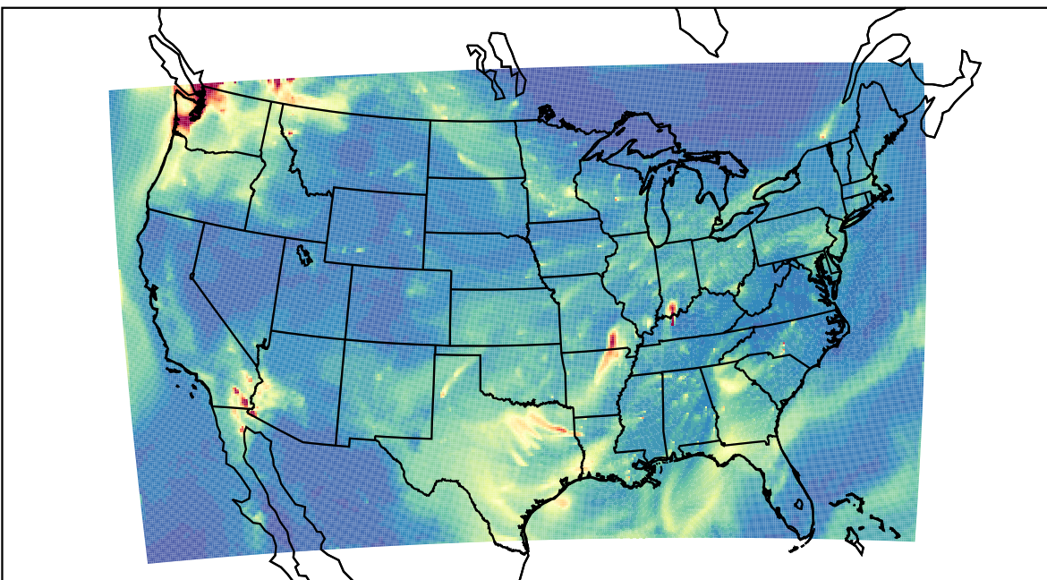
WRF 2022-10-09_13:00:00
