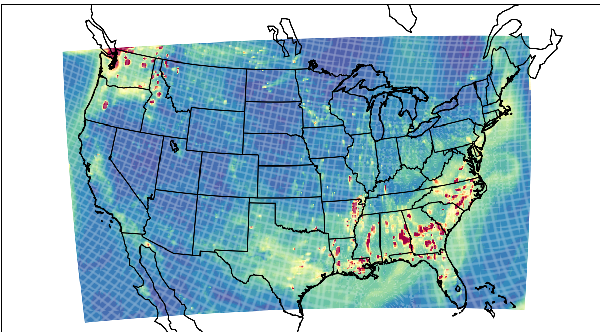
WRF 2022-10-08_01:00:00
