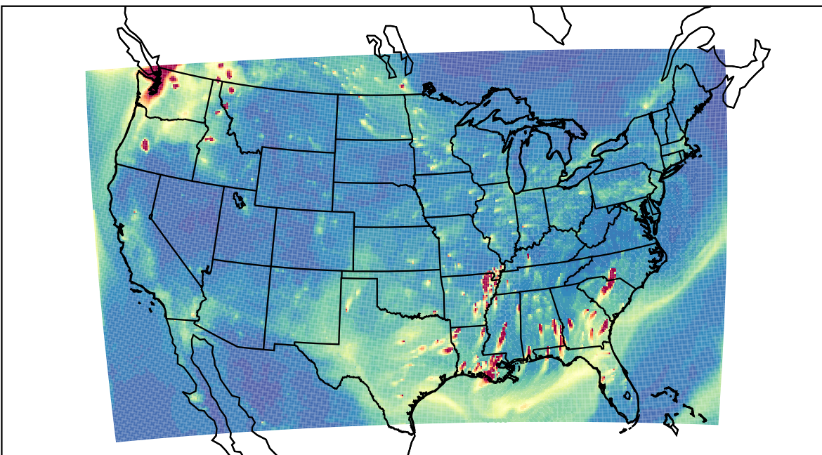
WRF 2022-10-09_01:00:00
