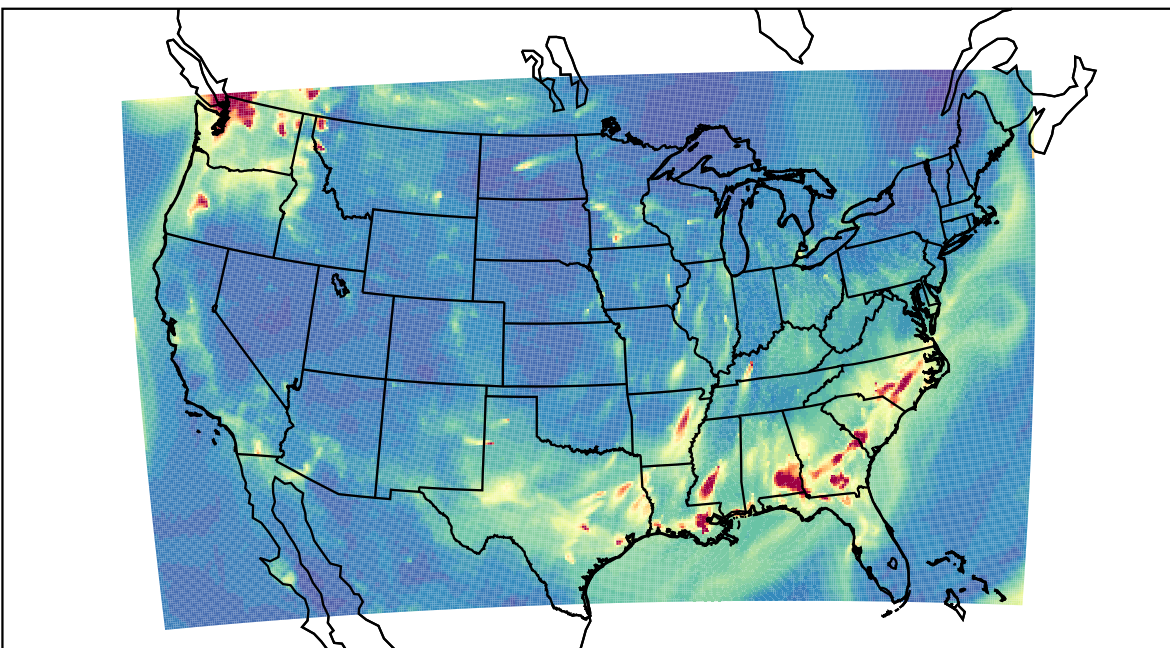
WRF 2022-10-08_05:00:00
