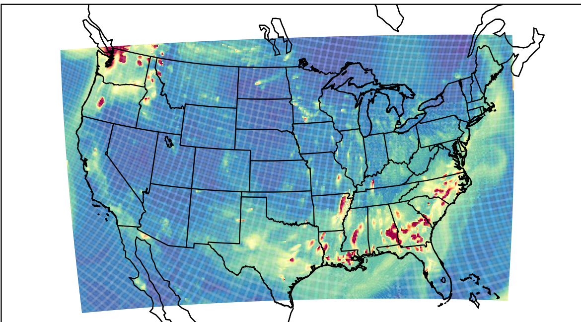
WRF 2022-10-08_03:00:00
