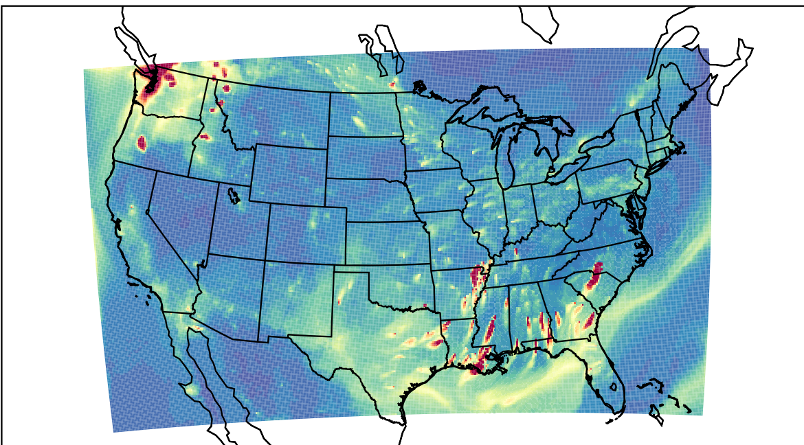
WRF 2022-10-09_02:00:00
