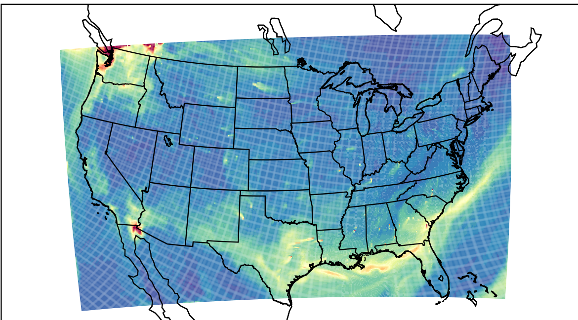
WRF 2022-10-08_17:00:00
