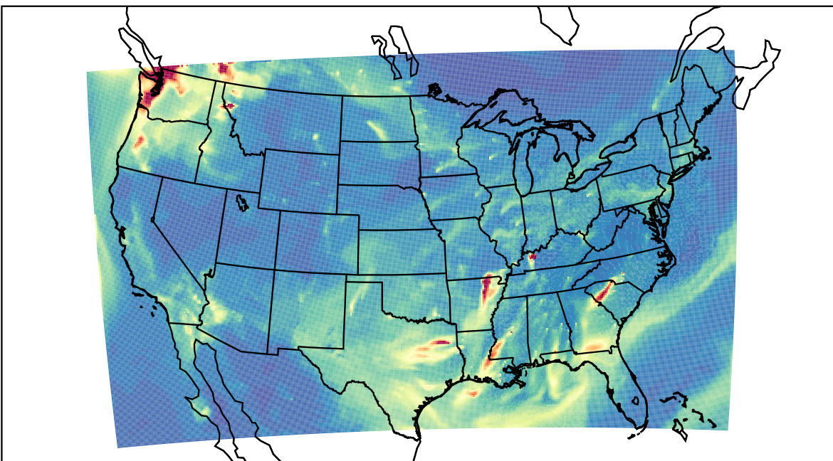
WRF 2022-10-09_07:00:00
