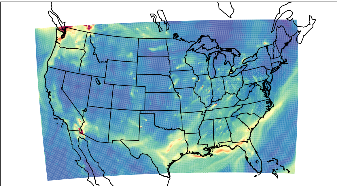
WRF 2022-10-08_13:00:00
