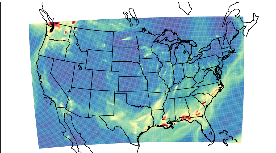
WRF 2022-10-08_08:00:00
