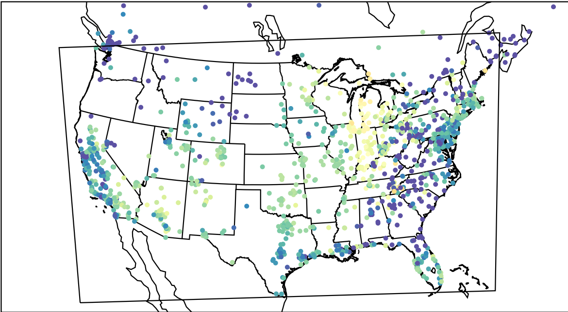
AirNOW (2022-10-24_03:00:00)
