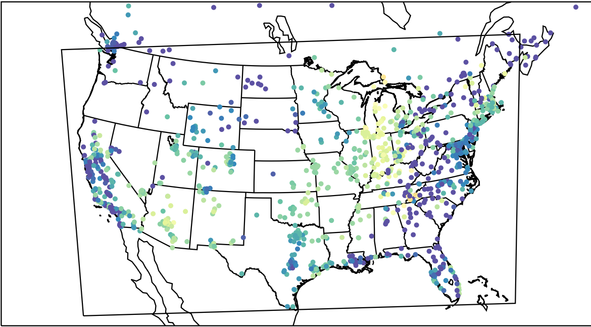
AirNOW (2022-10-24_06:00:00)
