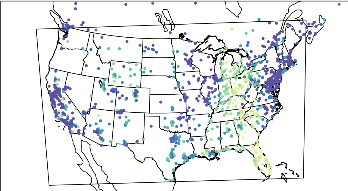
AirNOW (2022-10-25_15:00:00)
