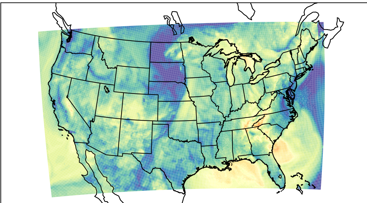
WRF (2022-10-24_06:00:00)
