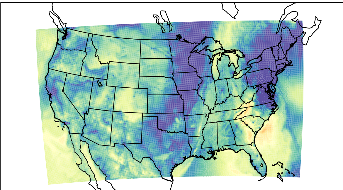
WRF (2022-10-25_12:00:00)
