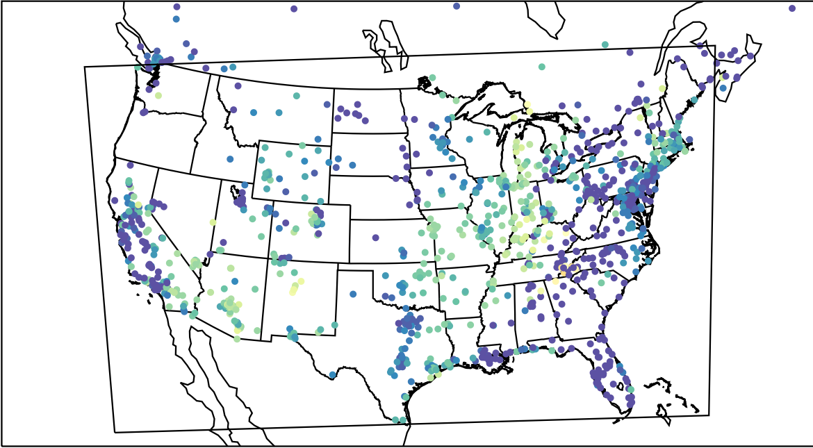
AirNOW (2022-10-24_10:00:00)
