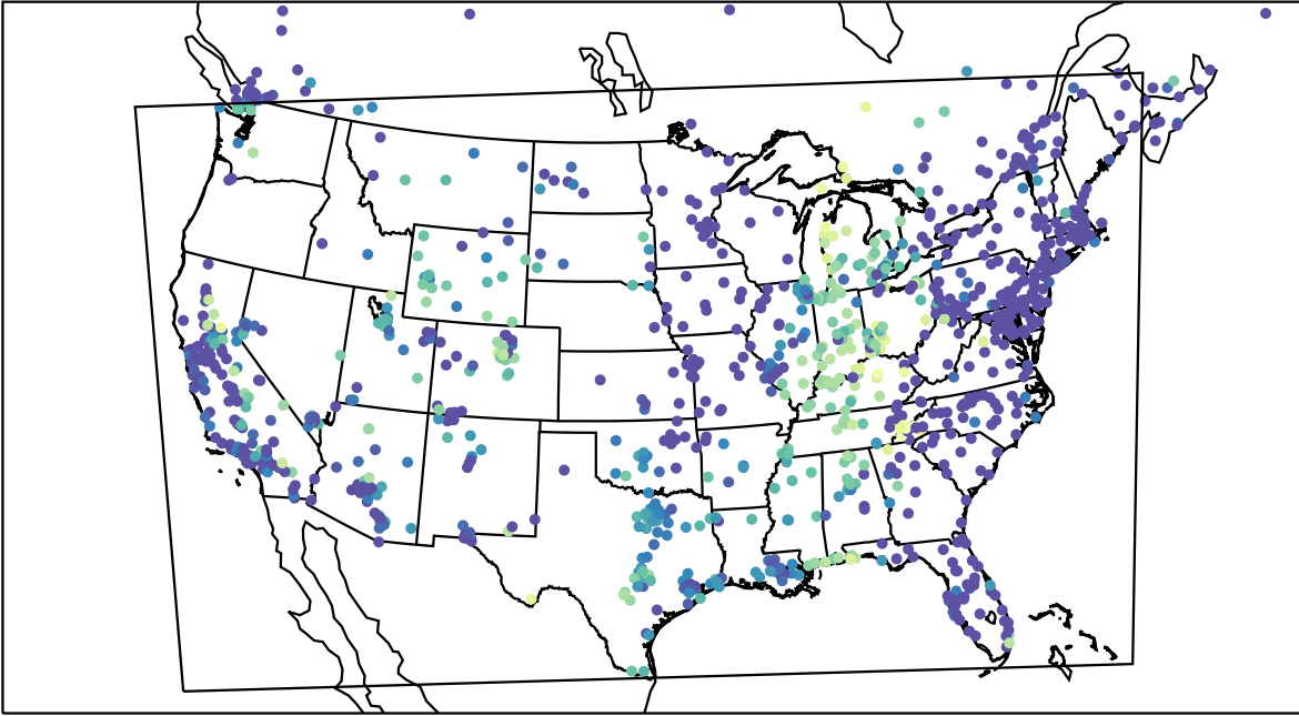
AirNOW (2022-10-25_10:00:00)
