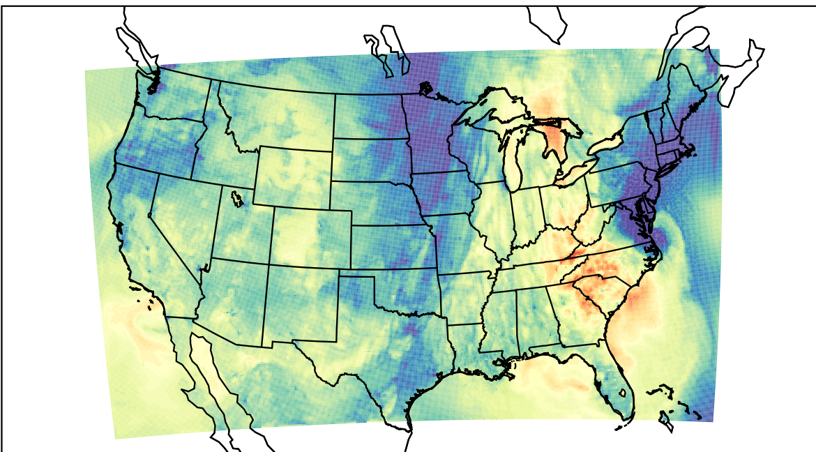
WRF (2022-10-25_01:00:00)
