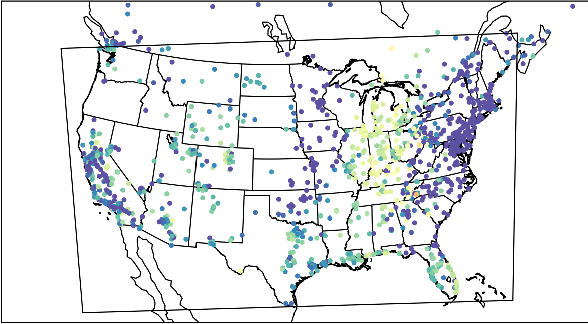
AirNOW (2022-10-25_03:00:00)
