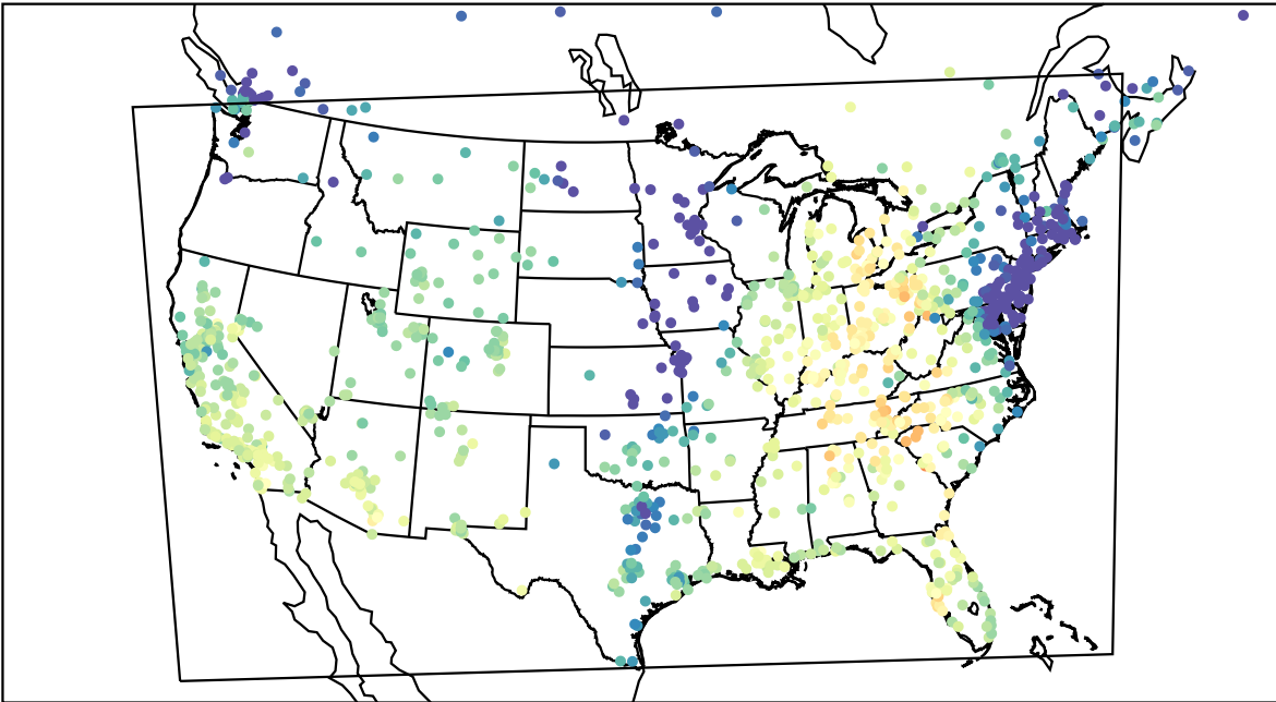
AirNOW (2022-10-24_21:00:00)
