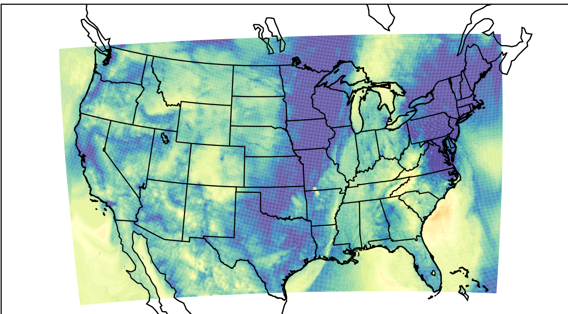
WRF (2022-10-25_13:00:00)
