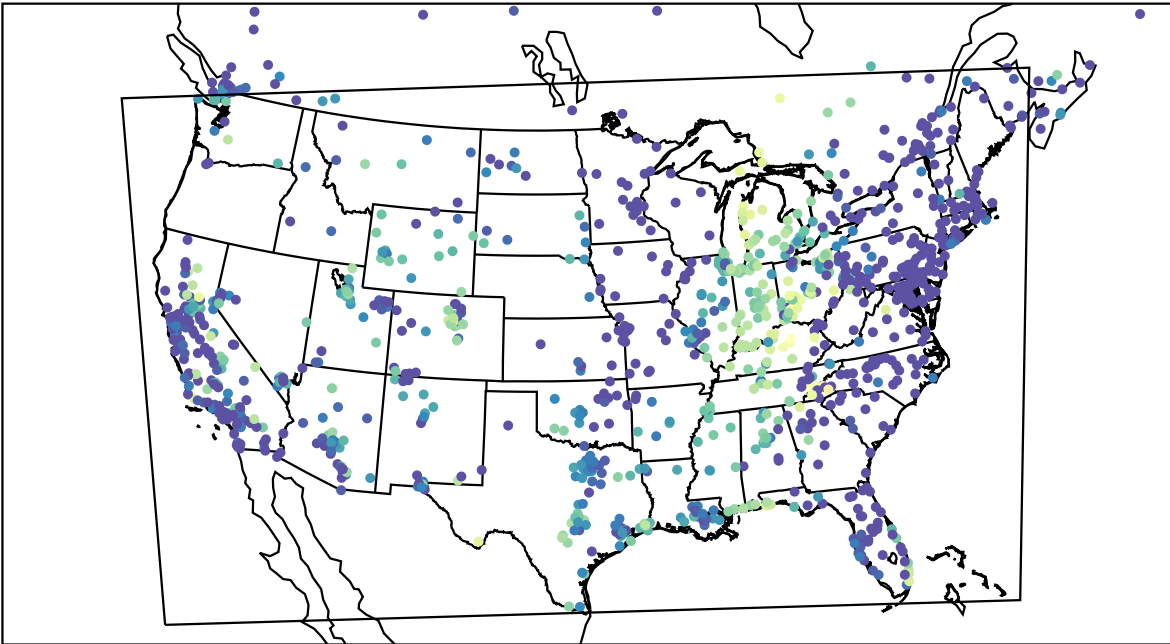
AirNOW (2022-10-25_09:00:00)
