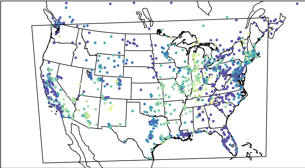
AirNOW (2022-10-24_09:00:00)
