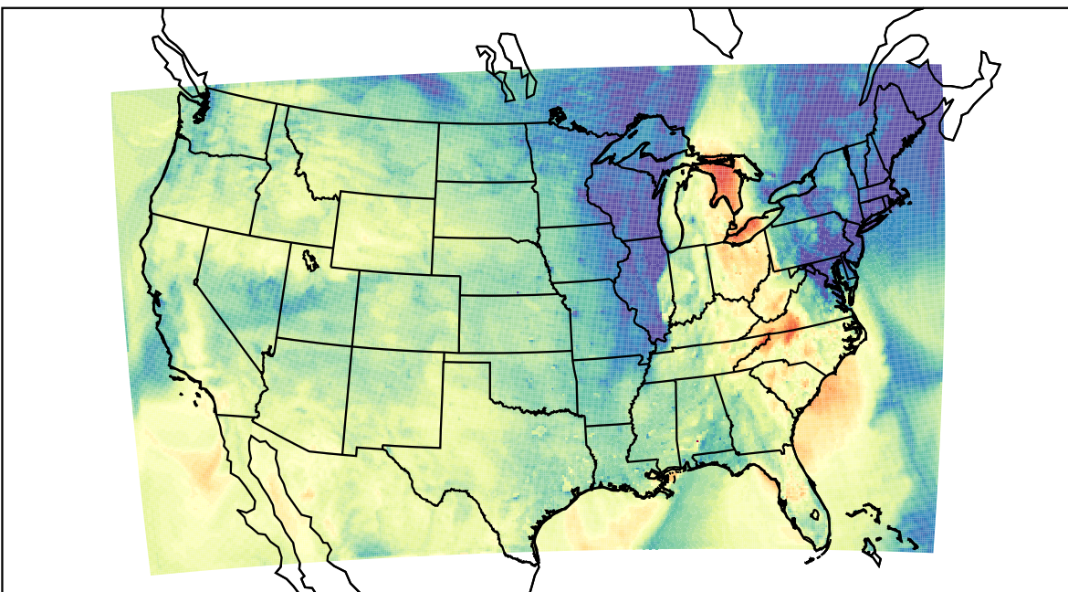
WRF (2022-10-25_23:00:00)
