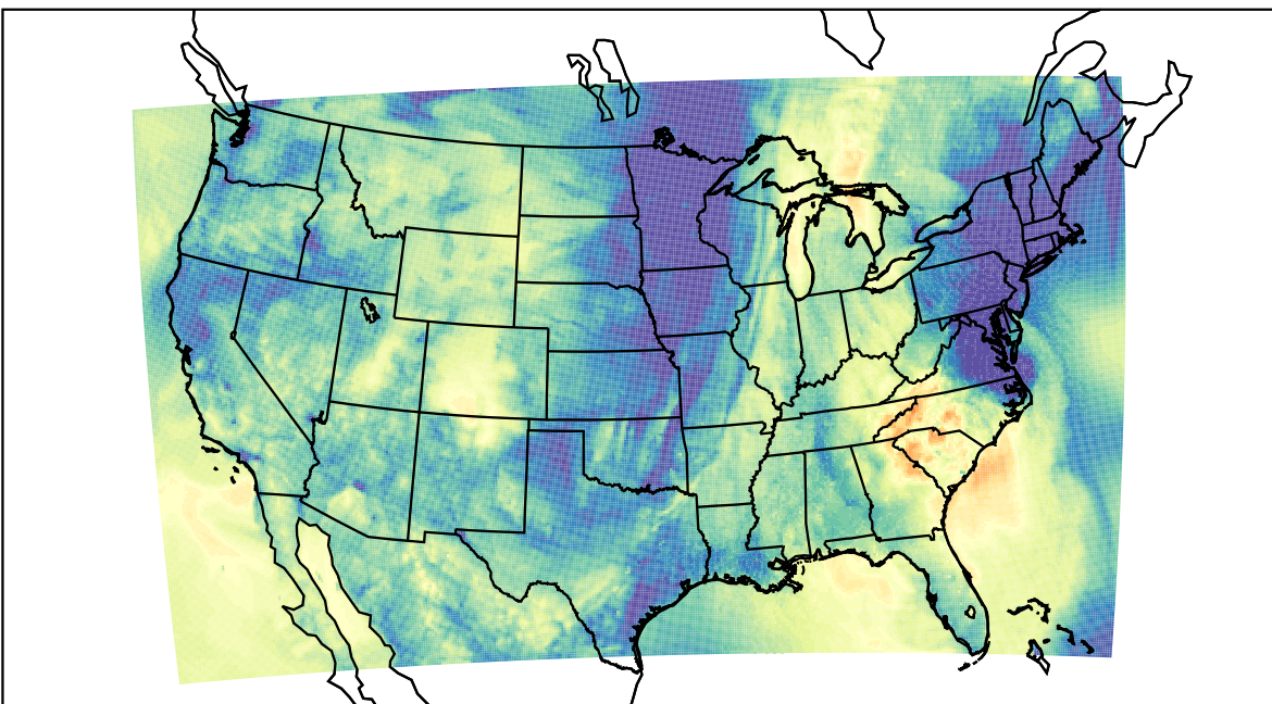
WRF (2022-10-25_06:00:00)
