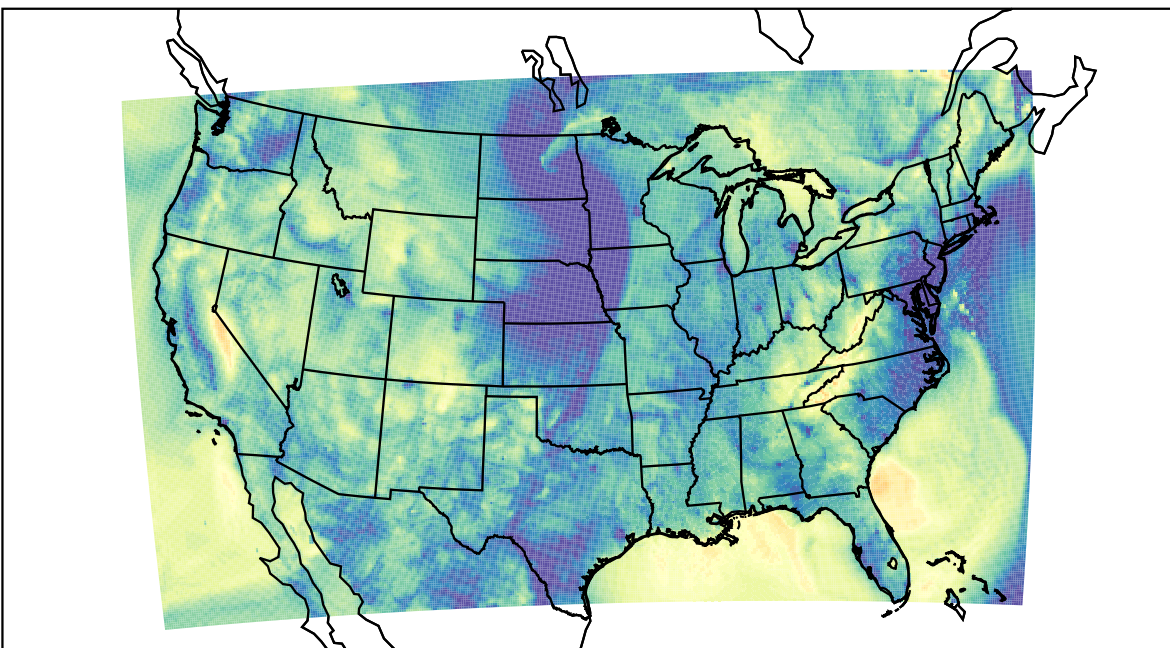
WRF (2022-10-24_12:00:00)
