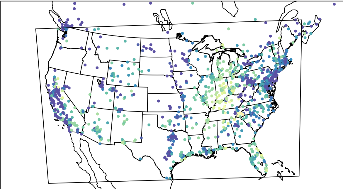
AirNOW (2022-10-24_14:00:00)
