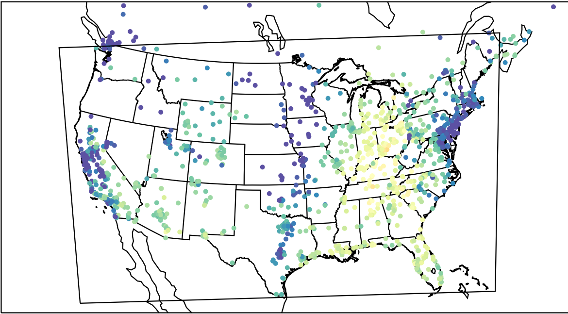
AirNOW (2022-10-24_16:00:00)
