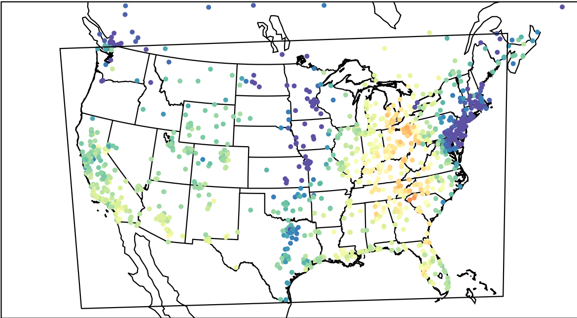
AirNOW (2022-10-24_20:00:00)
