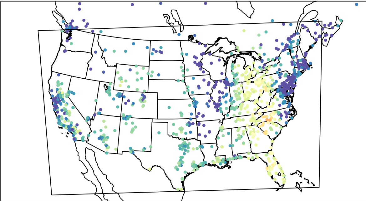
AirNOW (2022-10-25_17:00:00)
