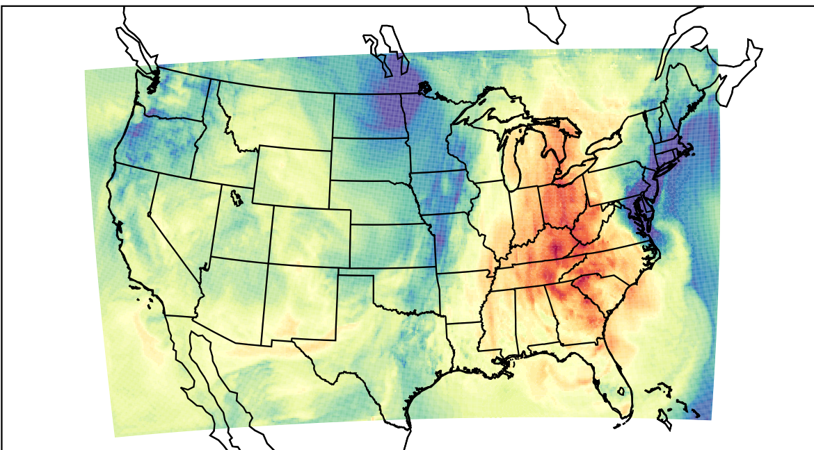
WRF (2022-10-24_20:00:00)
