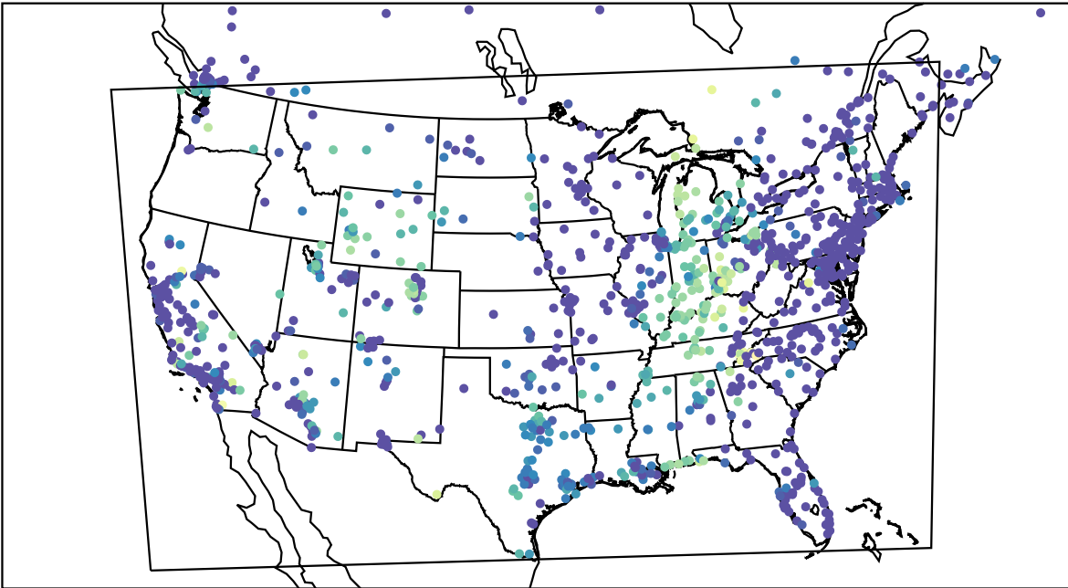
AirNOW (2022-10-25_12:00:00)
