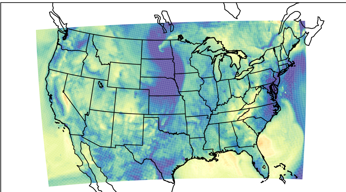
WRF (2022-10-24_11:00:00)
