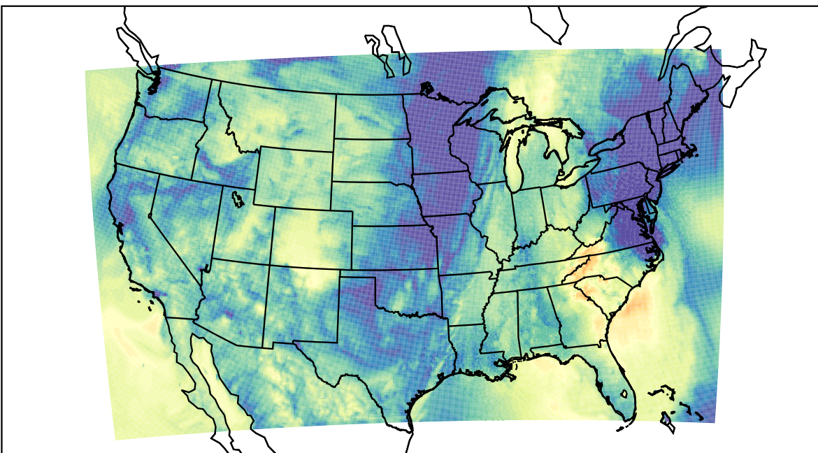
WRF (2022-10-25_09:00:00)
