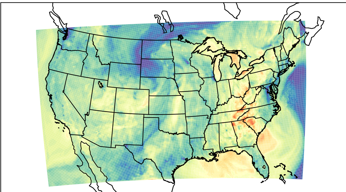
WRF (2022-10-24_01:00:00)
