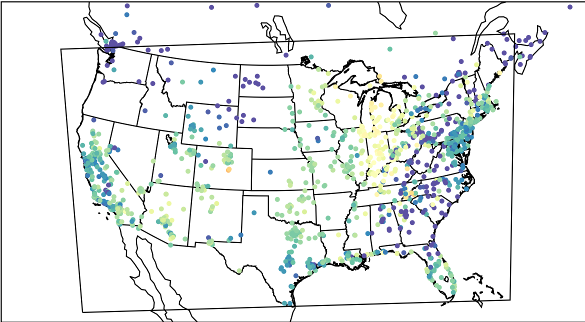
AirNOW (2022-10-24_02:00:00)
