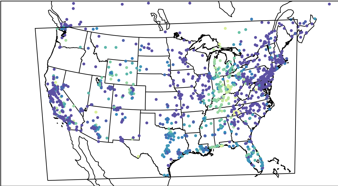
AirNOW (2022-10-25_13:00:00)
