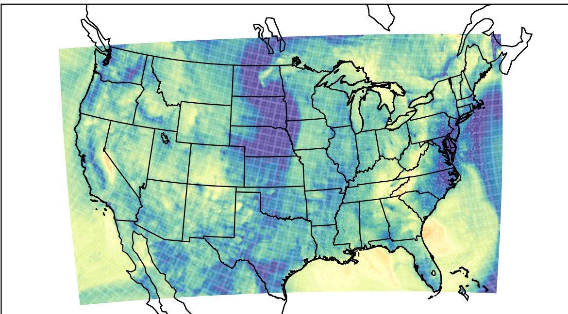
WRF (2022-10-24_10:00:00)
