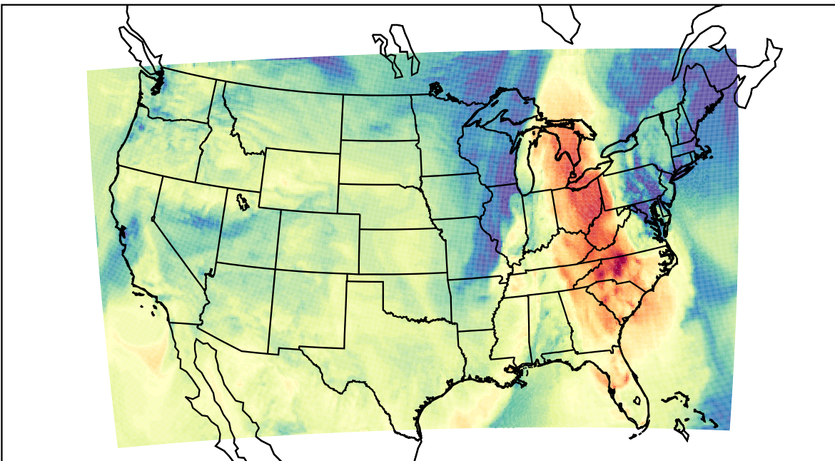
WRF (2022-10-25_20:00:00)
