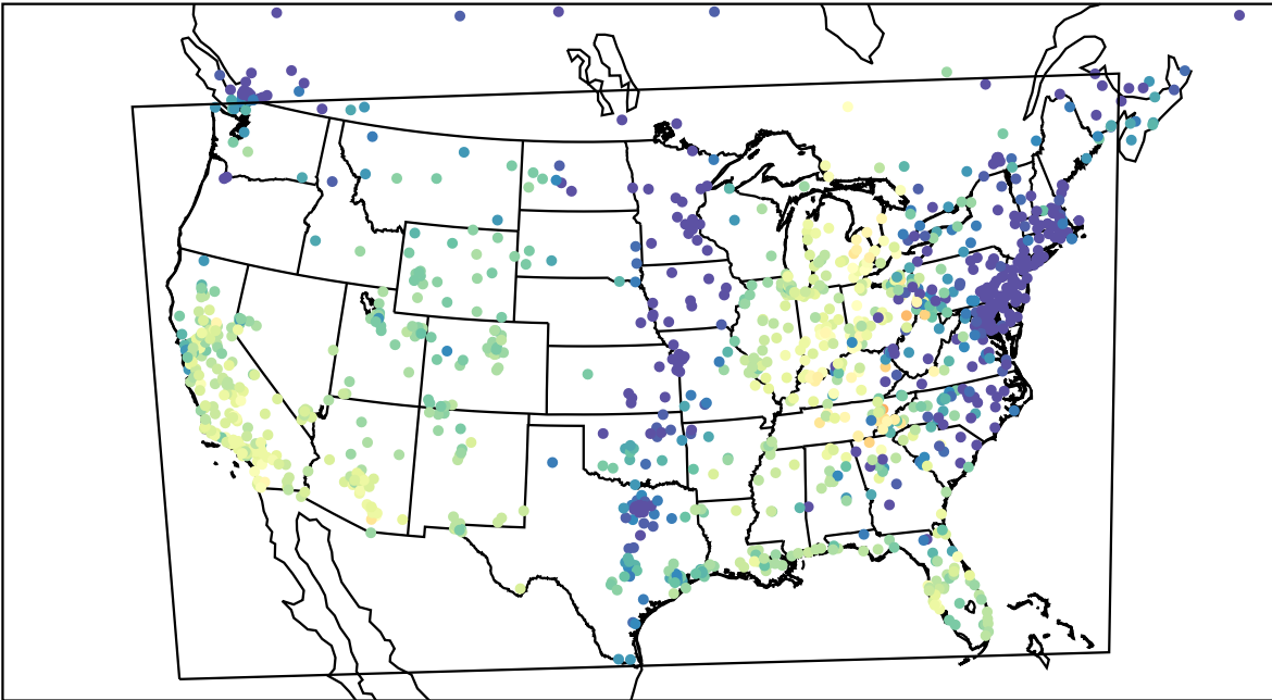
AirNOW (2022-10-24_23:00:00)
