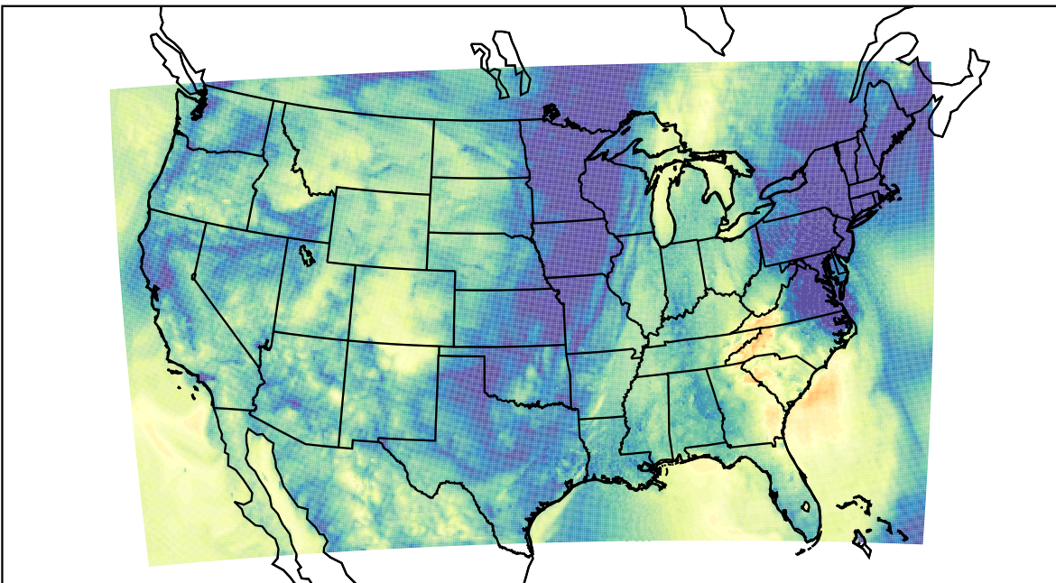
WRF (2022-10-25_10:00:00)
