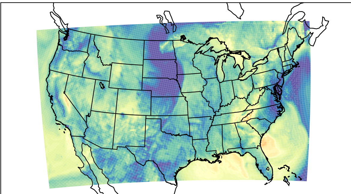
WRF (2022-10-24_09:00:00)
