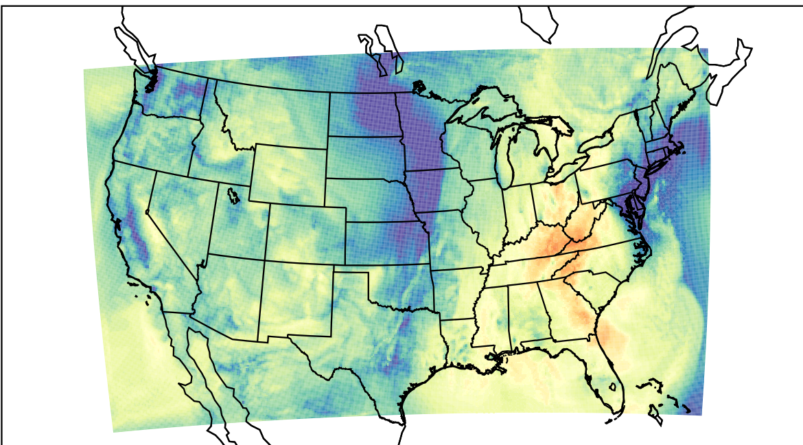
WRF (2022-10-24_16:00:00)
