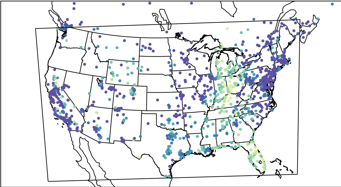
AirNOW (2022-10-25_14:00:00)
