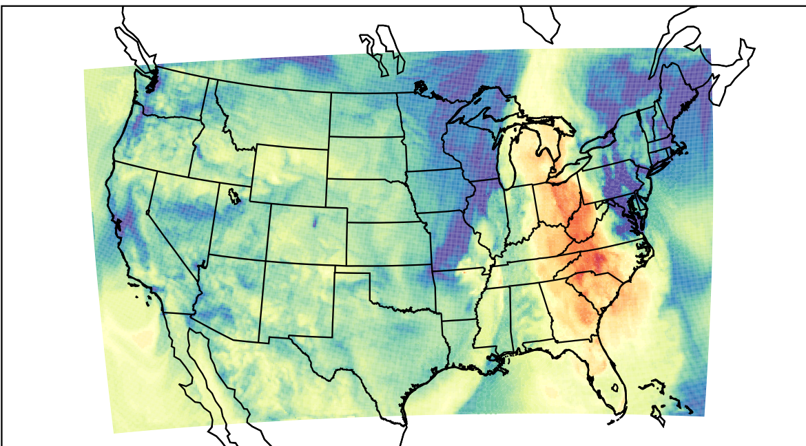
WRF (2022-10-25_17:00:00)
