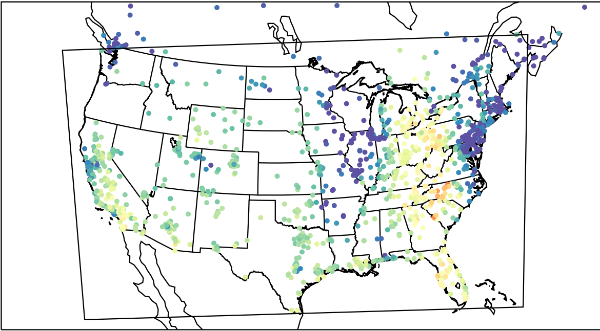
AirNOW (2022-10-25_19:00:00)
