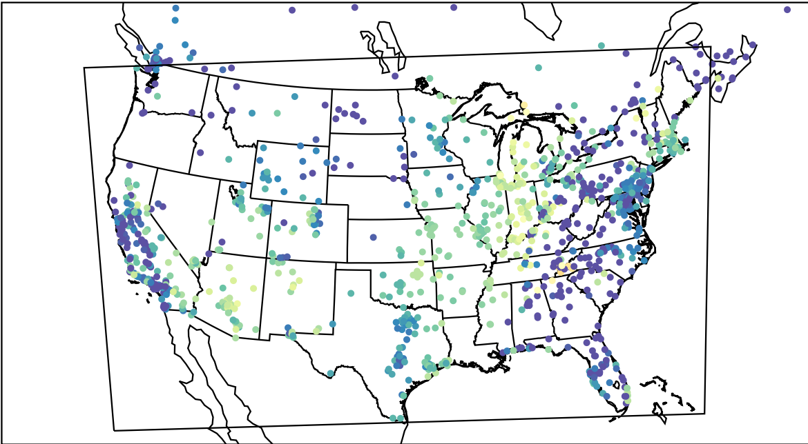
AirNOW (2022-10-24_07:00:00)
