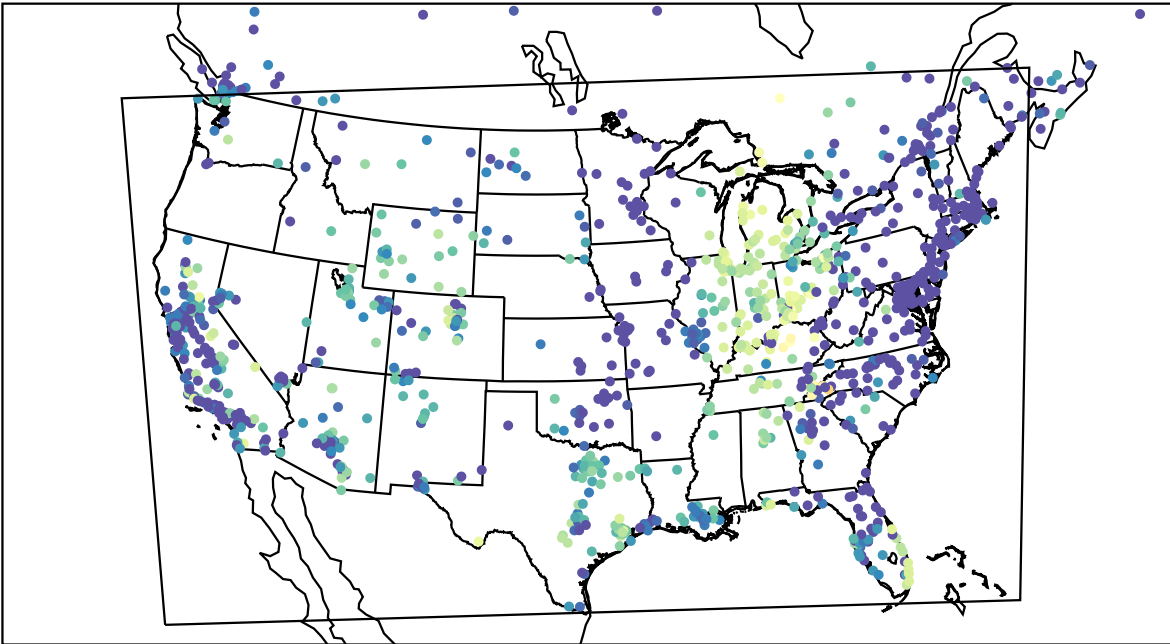
AirNOW (2022-10-25_06:00:00)
