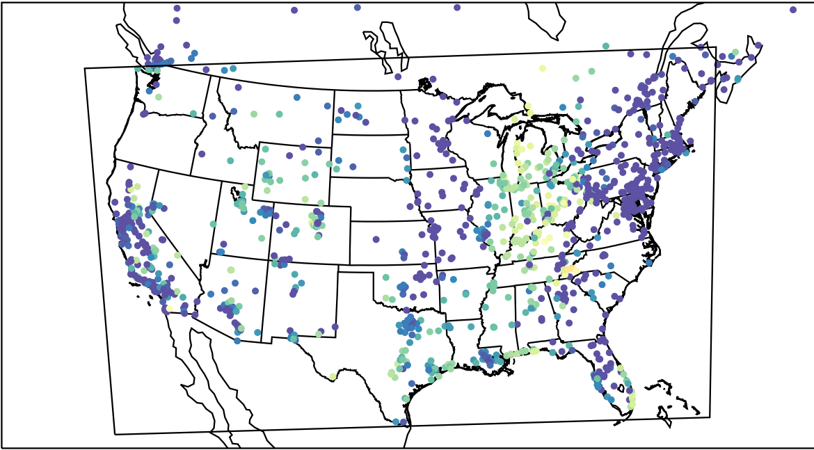
AirNOW (2022-10-25_08:00:00)
