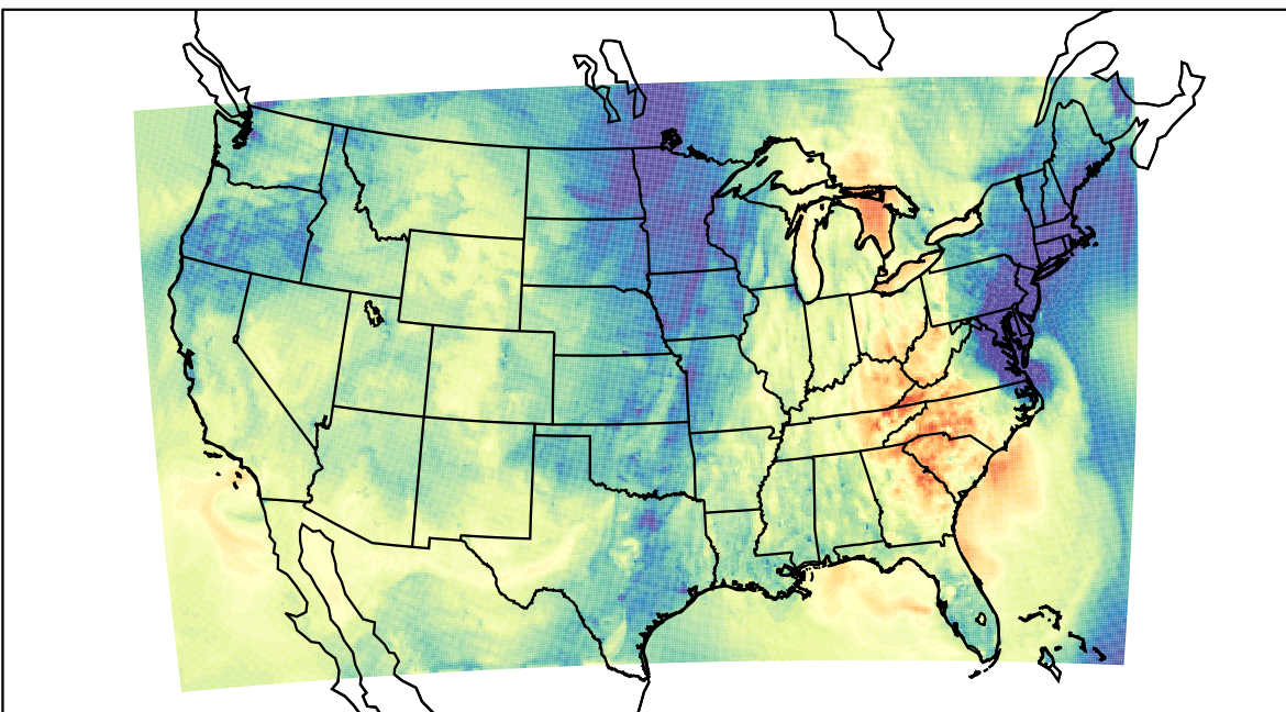
WRF (2022-10-25_00:00:00)
