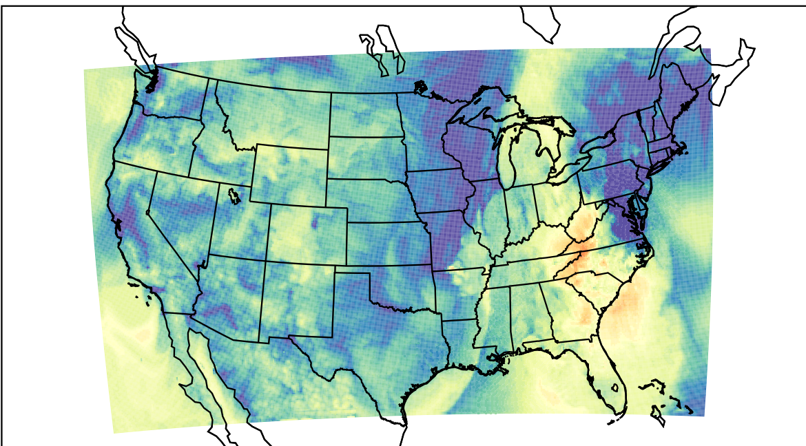
WRF (2022-10-25_15:00:00)
