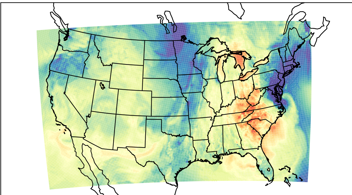
WRF (2022-10-24_23:00:00)
