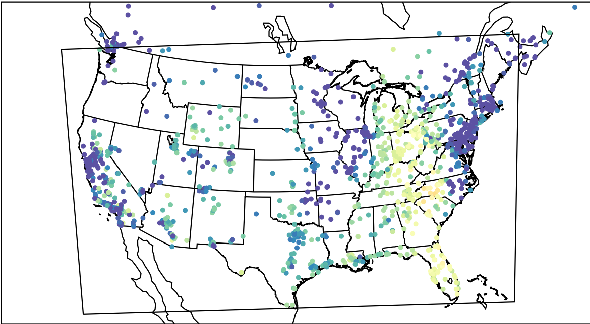
AirNOW (2022-10-25_16:00:00)
