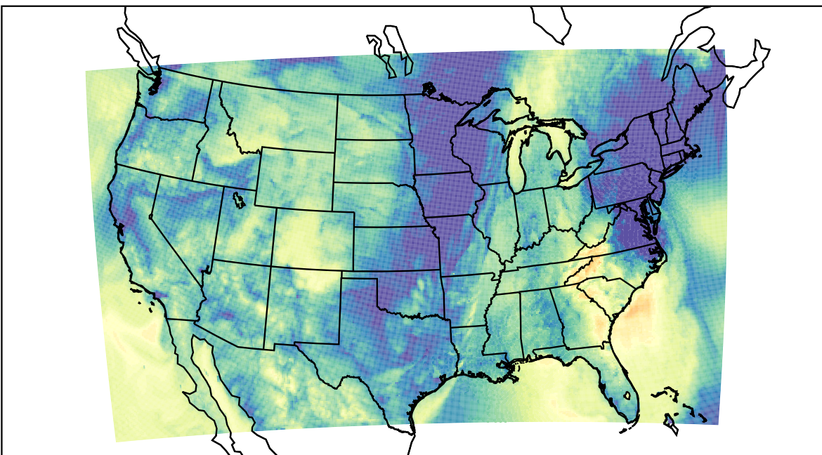
WRF (2022-10-25_11:00:00)
