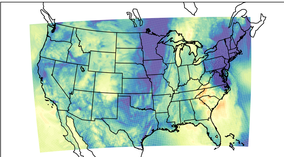
WRF (2022-10-25_08:00:00)
