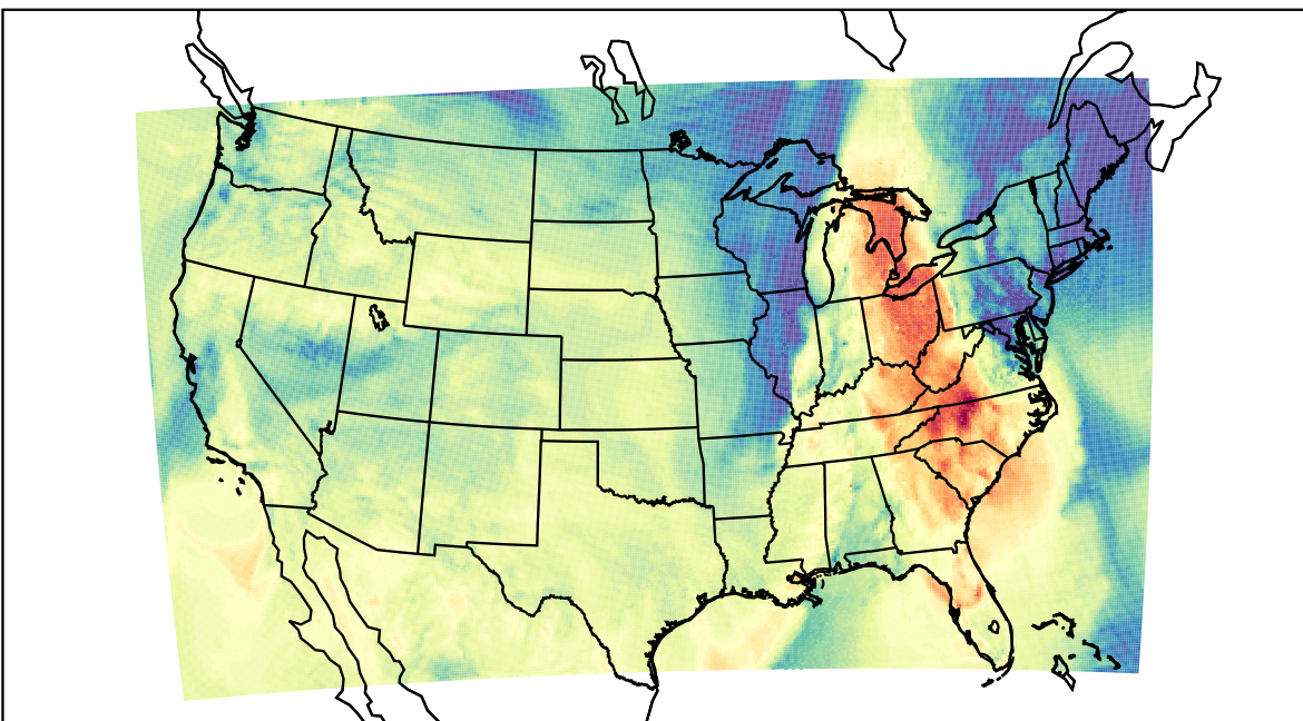
WRF (2022-10-25_21:00:00)
