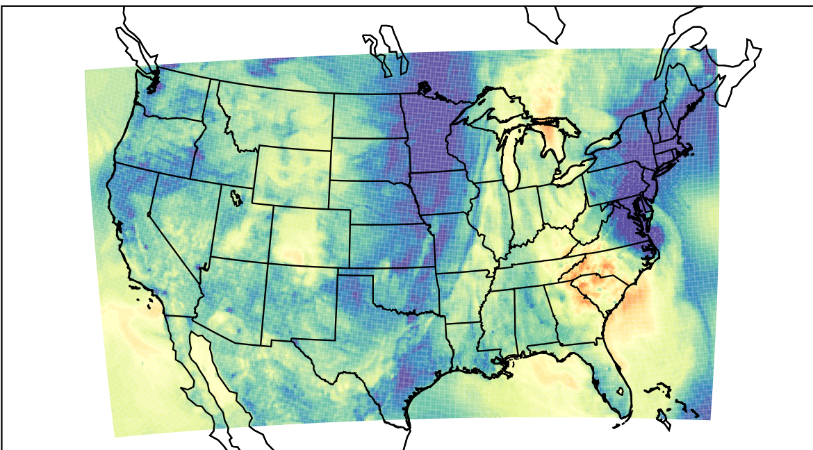
WRF (2022-10-25_04:00:00)
