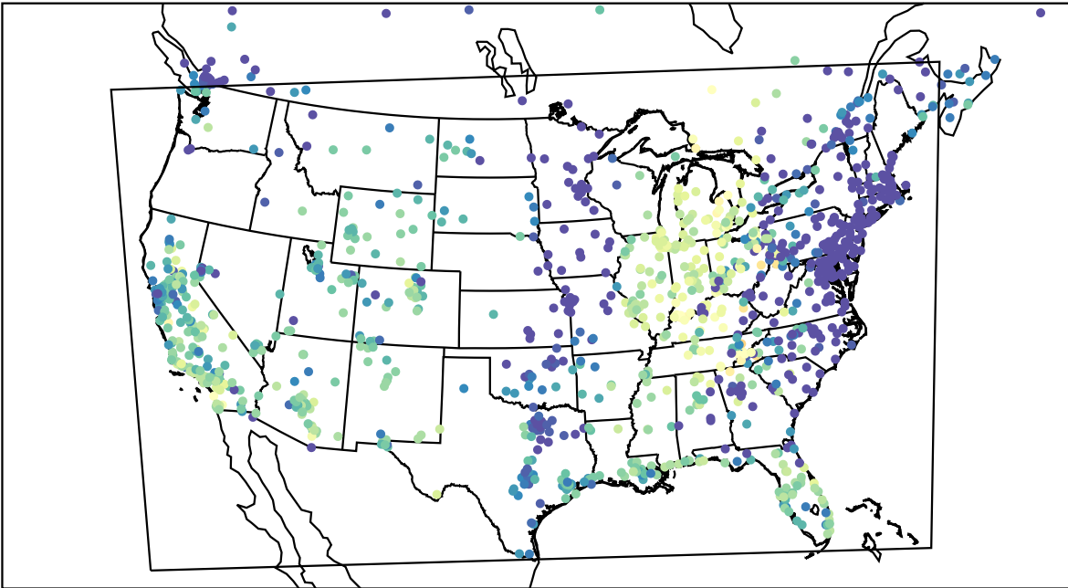
AirNOW (2022-10-25_01:00:00)
