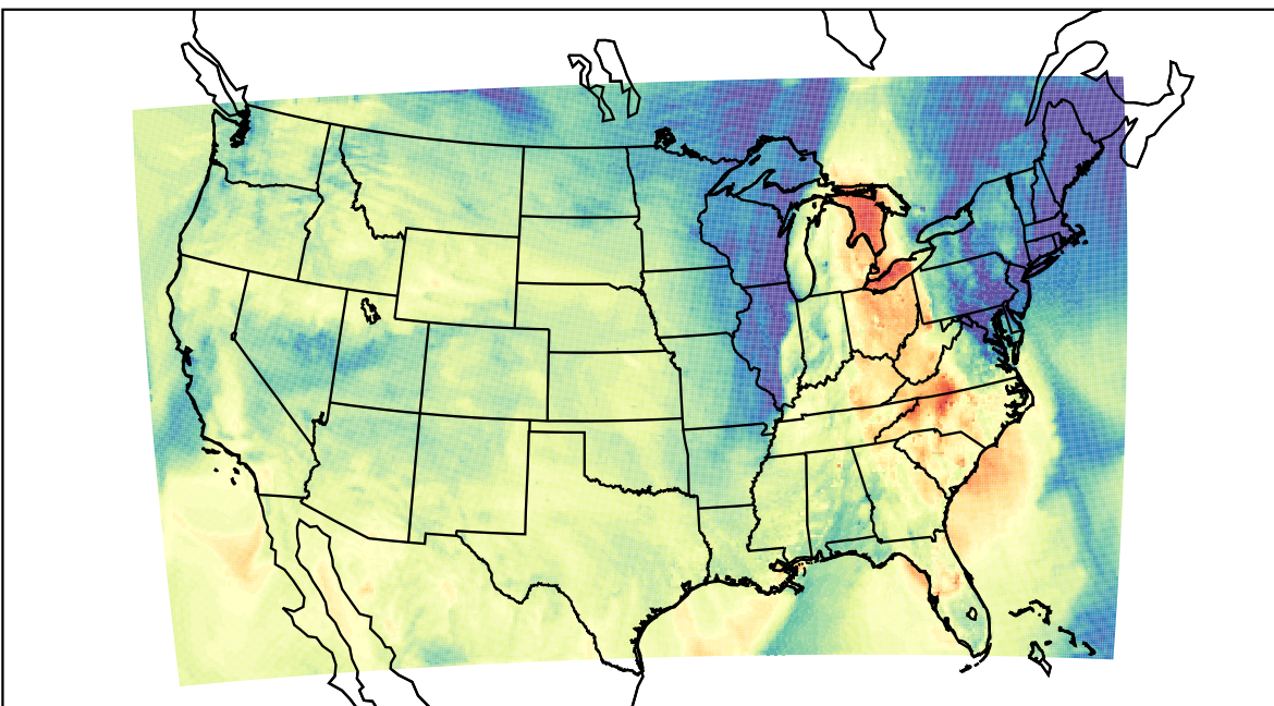
WRF (2022-10-25_22:00:00)
