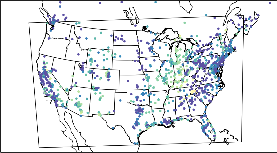
AirNOW (2022-10-24_13:00:00)
