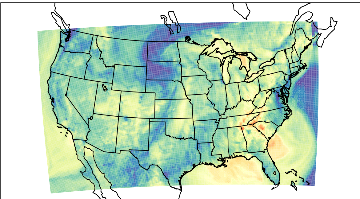
WRF (2022-10-24_03:00:00)
