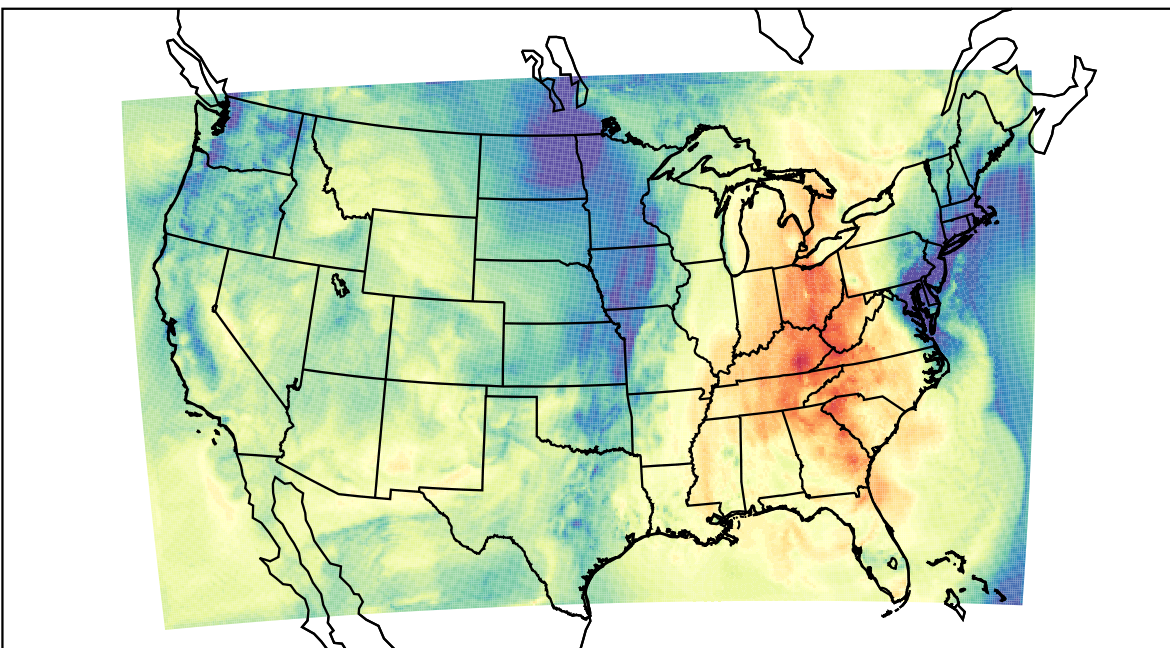
WRF (2022-10-24_18:00:00)
