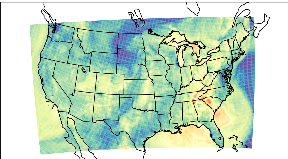
WRF (2022-10-24_02:00:00)
