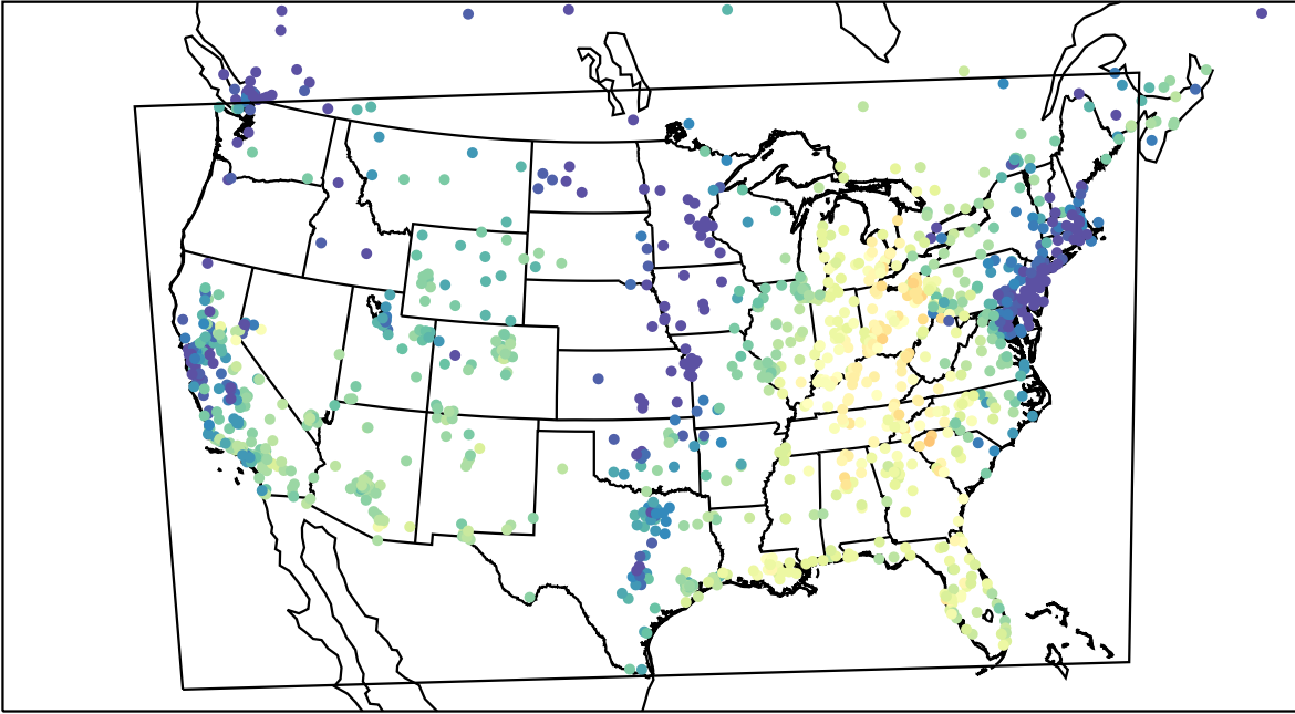
AirNOW (2022-10-24_17:00:00)
