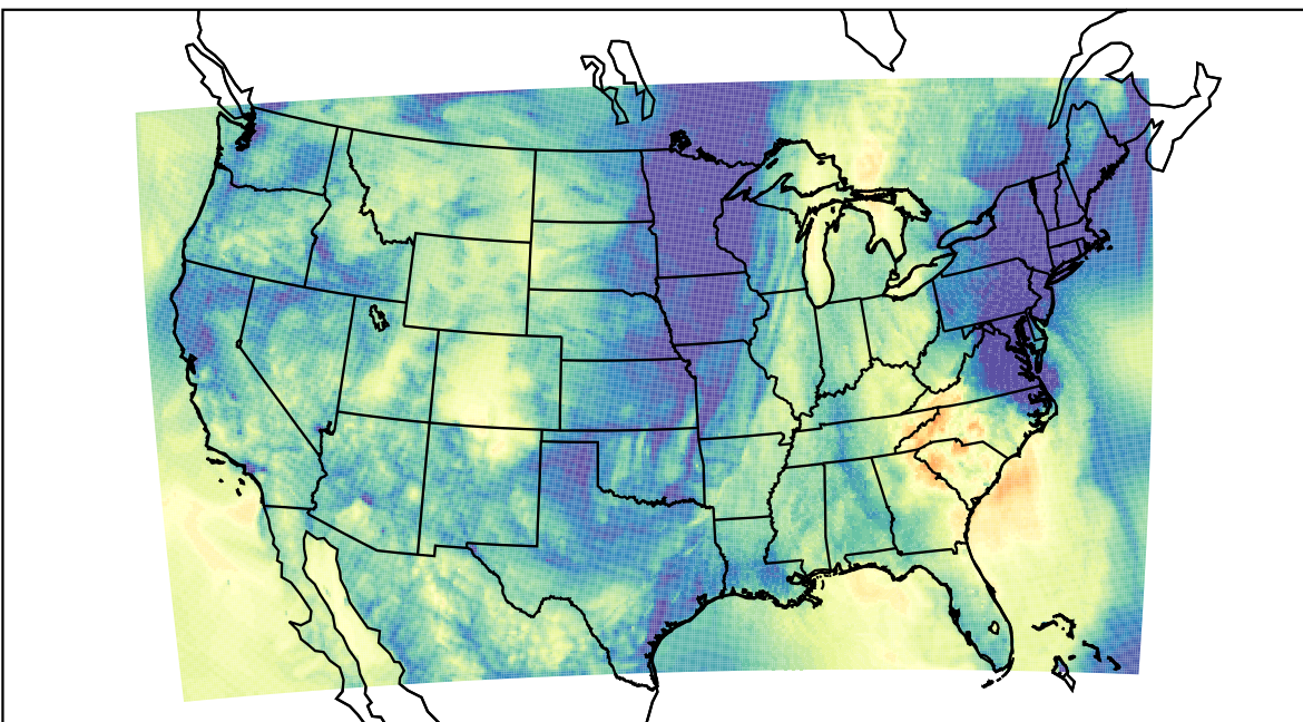
WRF (2022-10-25_07:00:00)
