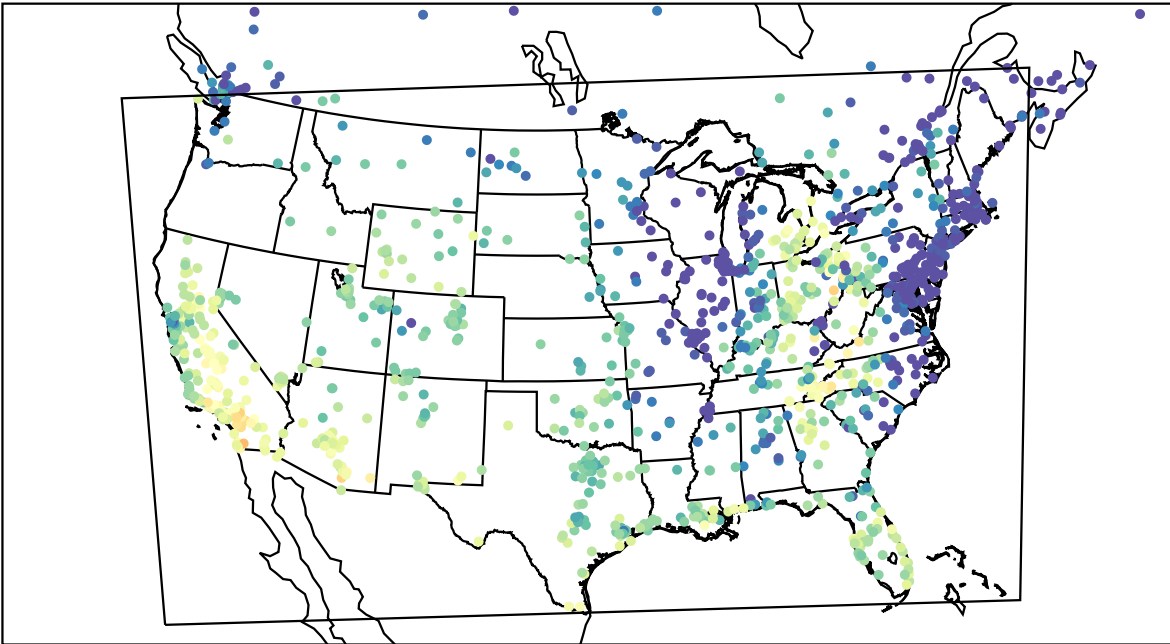
AirNOW (2022-10-25_23:00:00)
