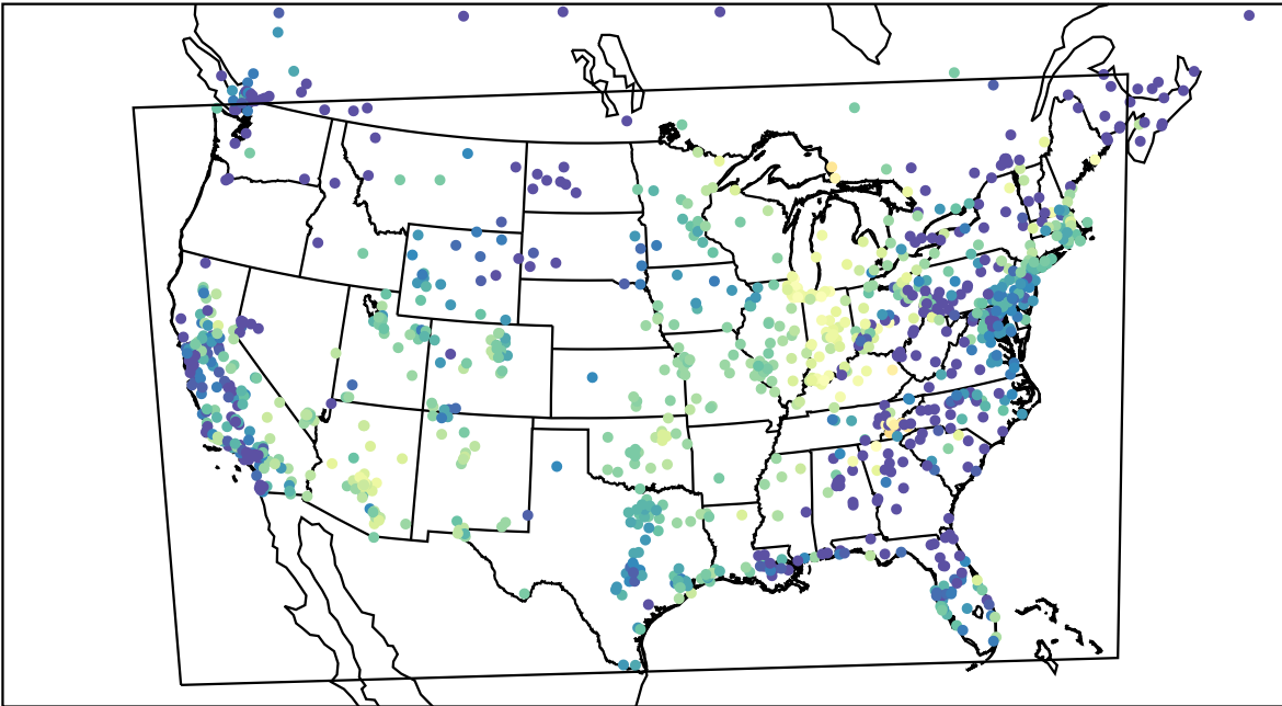
AirNOW (2022-10-24_05:00:00)
