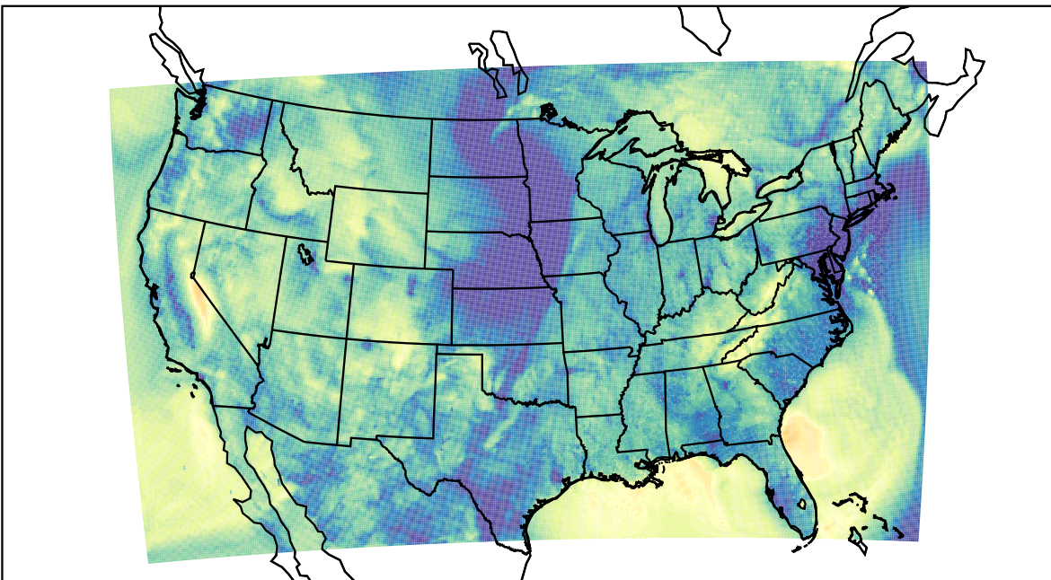
WRF (2022-10-24_13:00:00)
