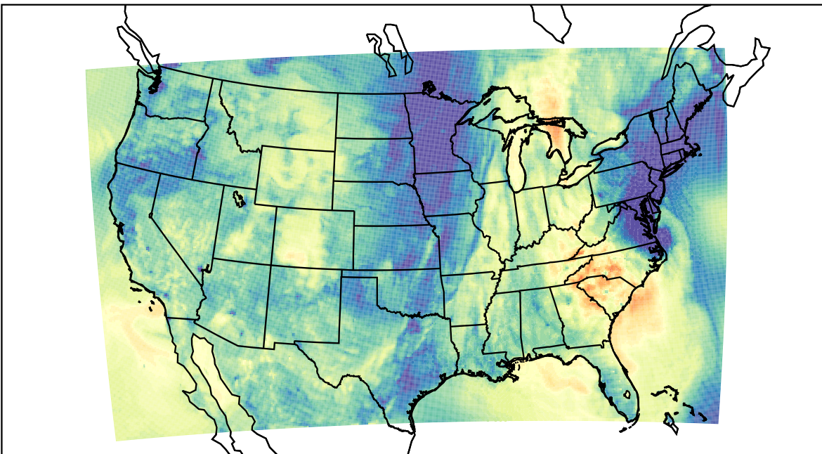
WRF (2022-10-25_03:00:00)
