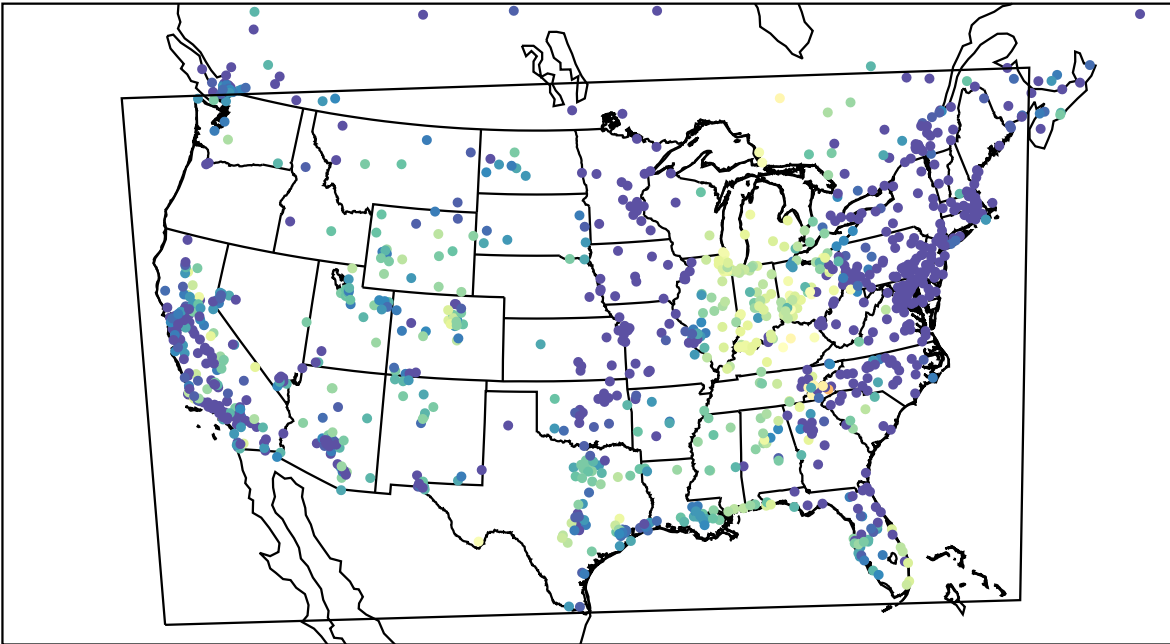
AirNOW (2022-10-25_05:00:00)
