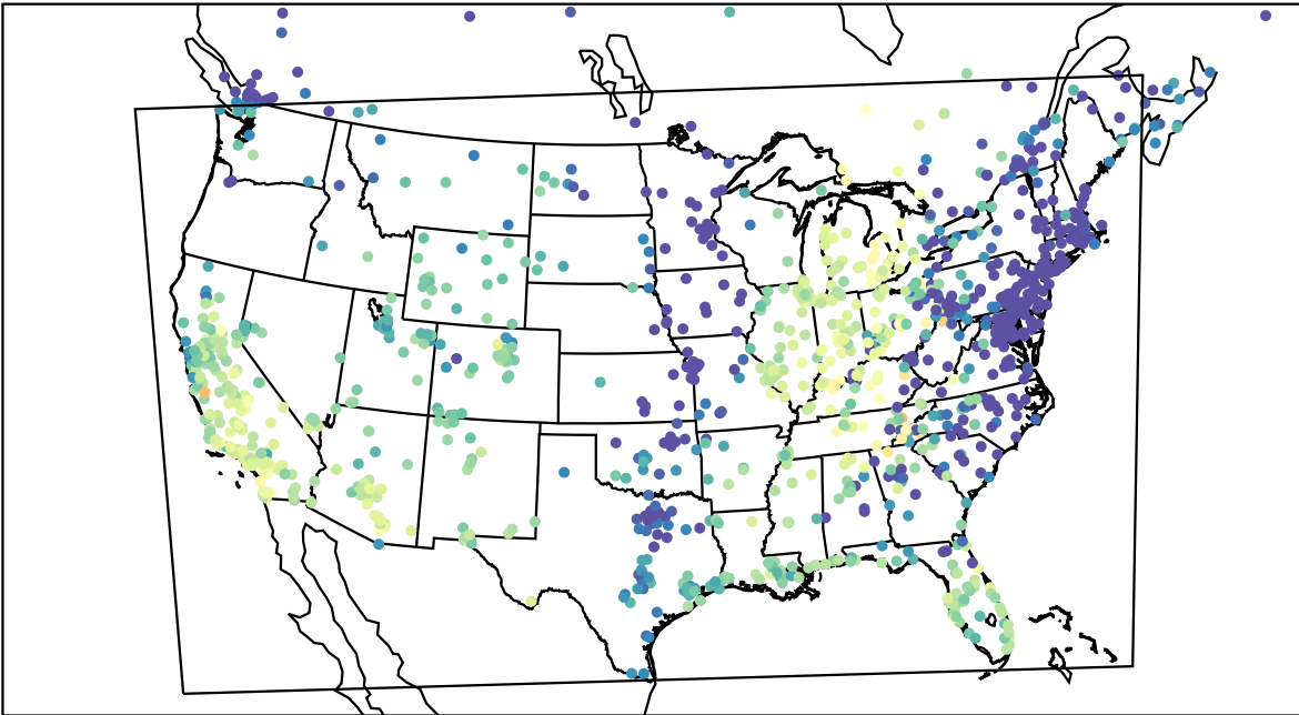
AirNOW (2022-10-25_00:00:00)
