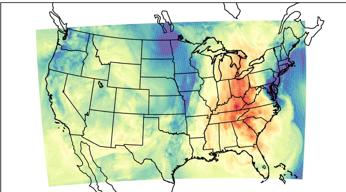
WRF (2022-10-24_19:00:00)
