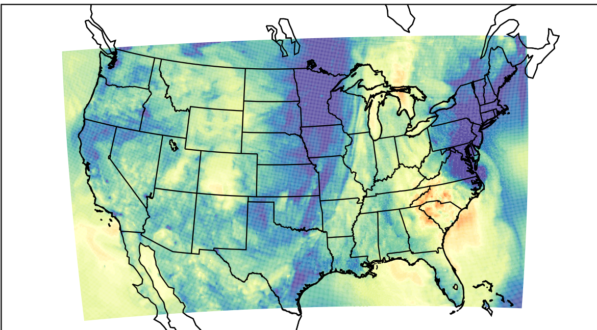
WRF (2022-10-25_05:00:00)
