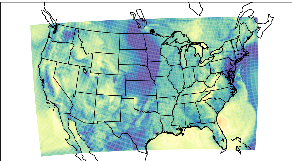
WRF (2022-10-24_14:00:00)
