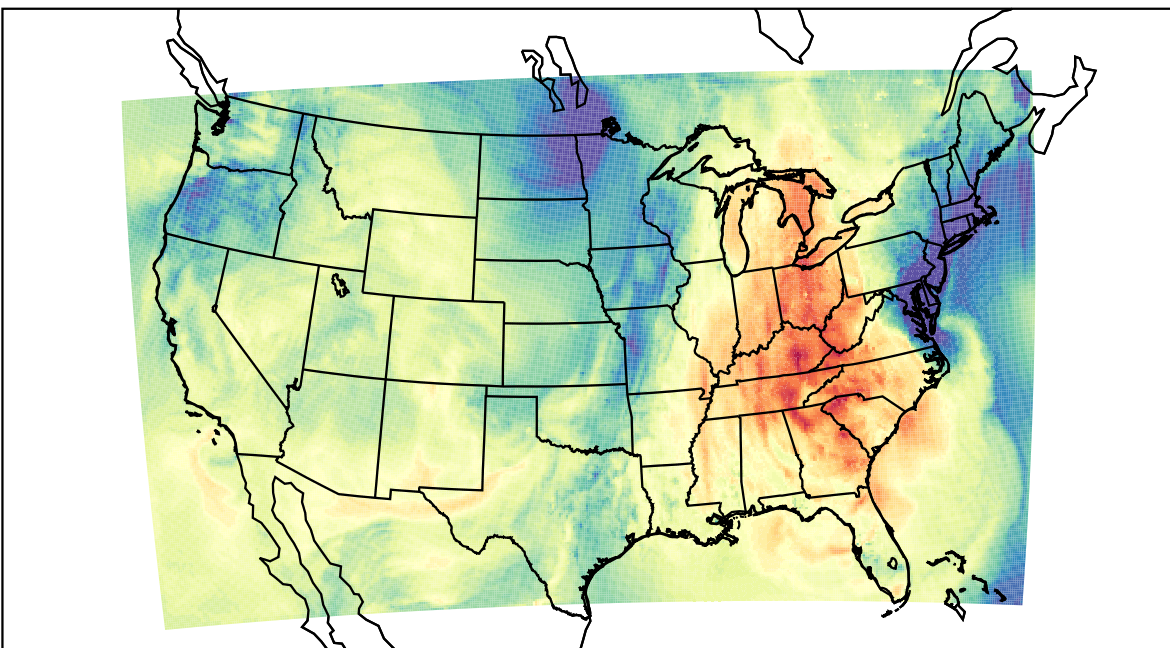
WRF (2022-10-24_21:00:00)
