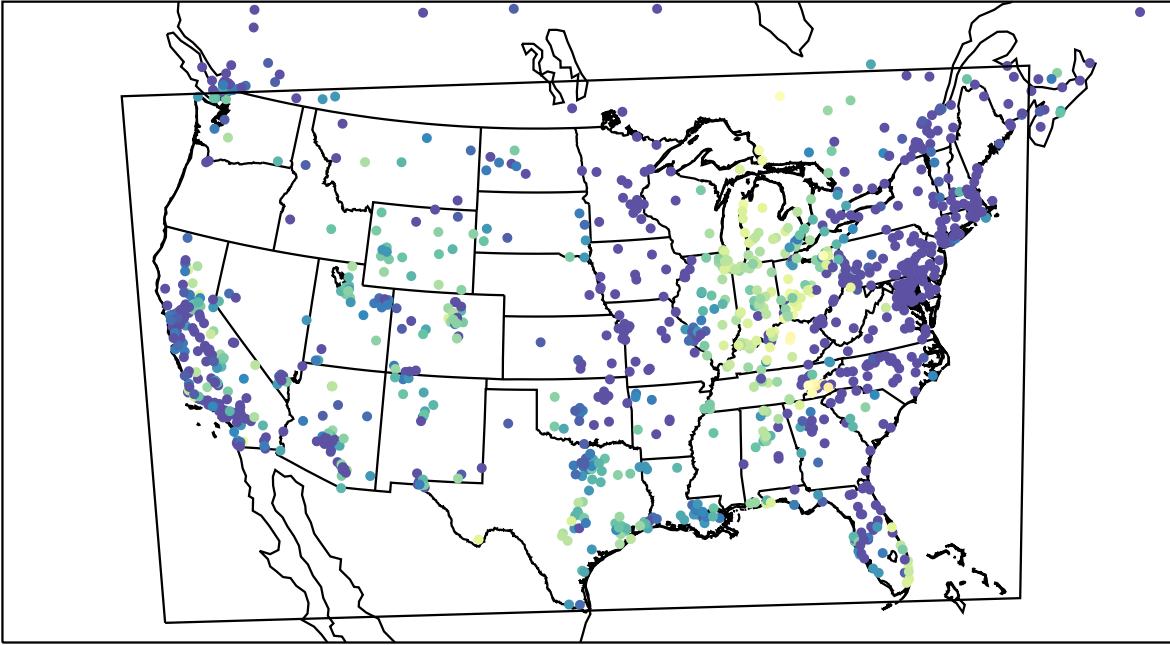
AirNOW (2022-10-25_07:00:00)
