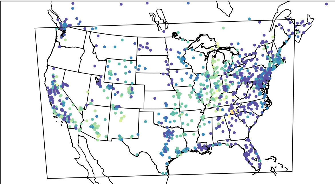
AirNOW (2022-10-24_11:00:00)
