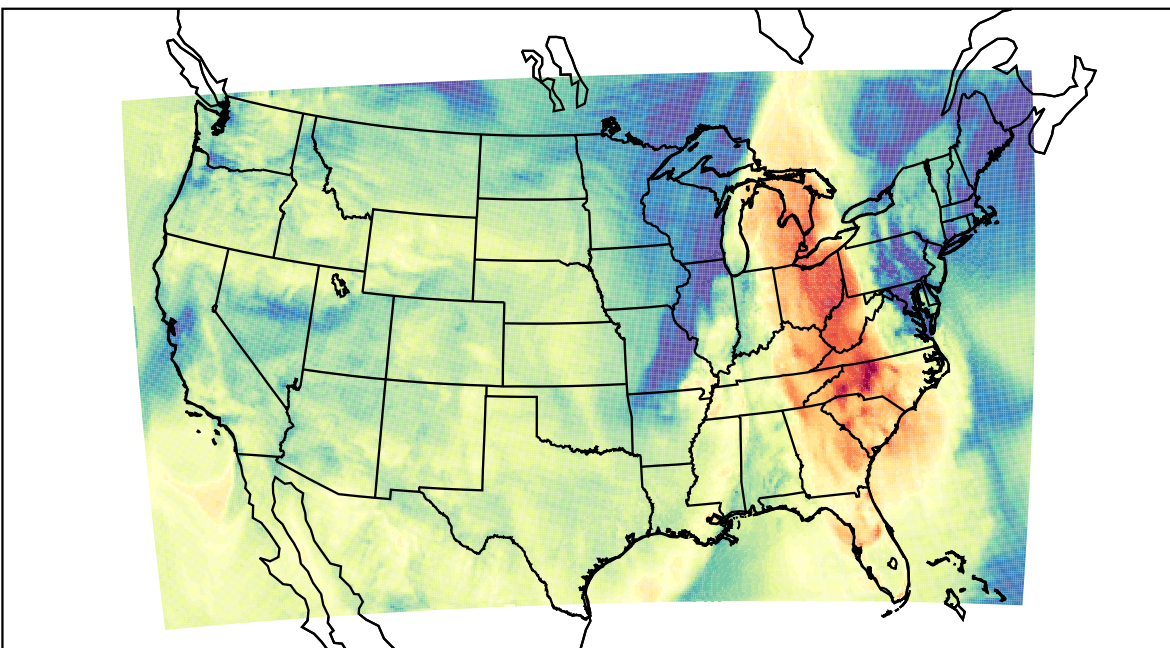
WRF (2022-10-25_19:00:00)
