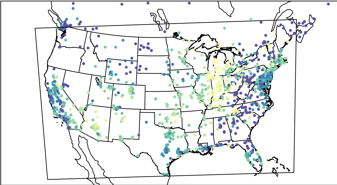
AirNOW (2022-10-24_04:00:00)
