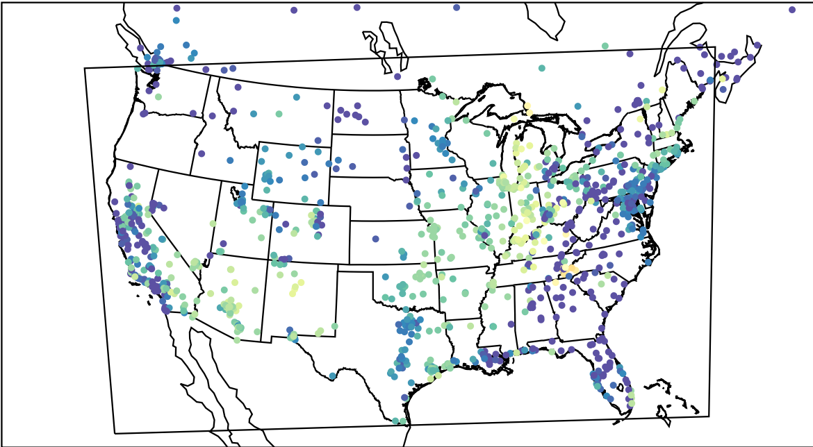
AirNOW (2022-10-24_08:00:00)
