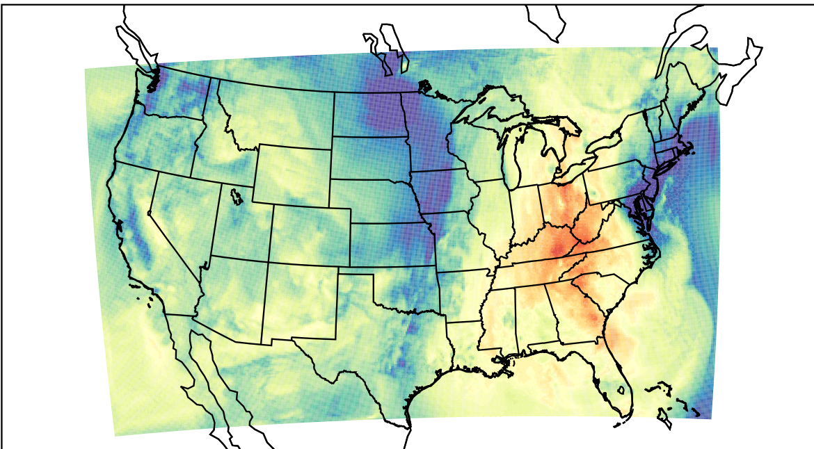
WRF (2022-10-24_17:00:00)
