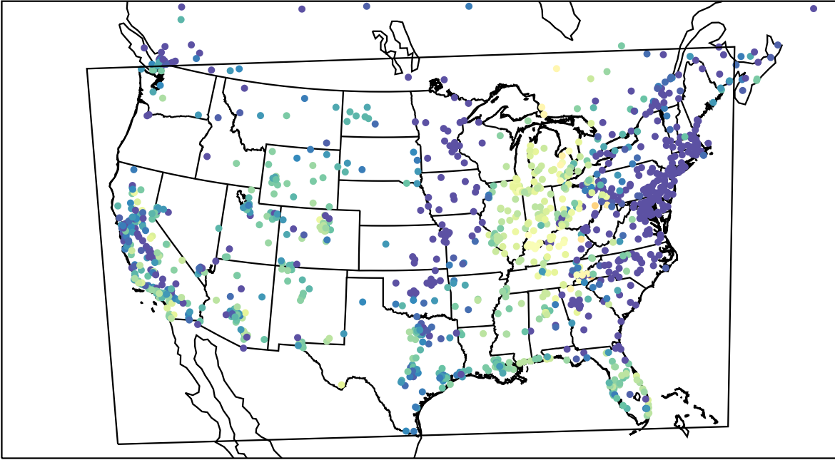
AirNOW (2022-10-25_02:00:00)
