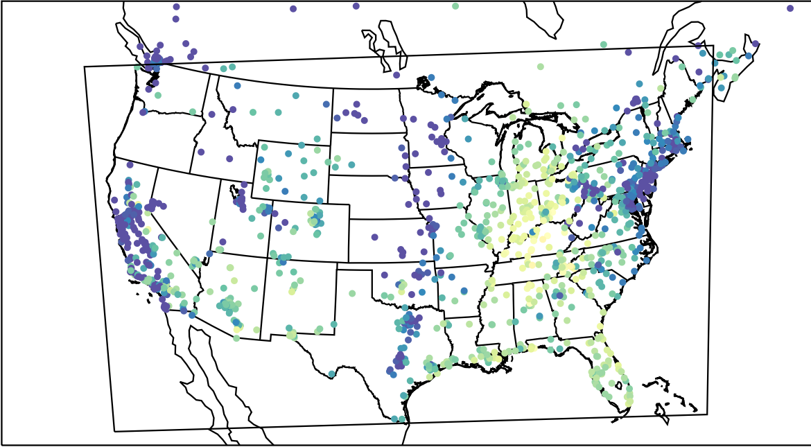
AirNOW (2022-10-24_15:00:00)
