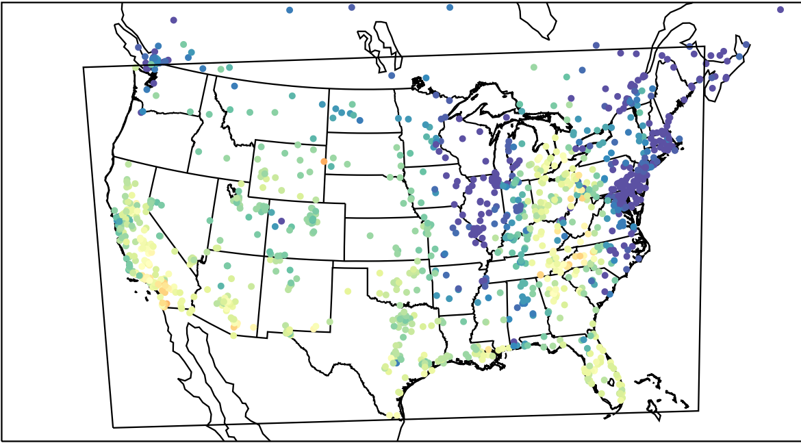
AirNOW (2022-10-25_22:00:00)
