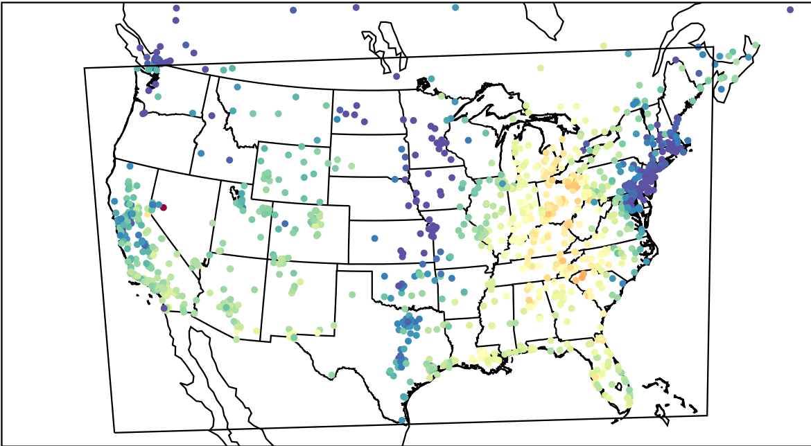
AirNOW (2022-10-24_18:00:00)
