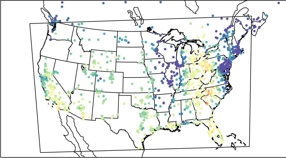
AirNOW (2022-10-25_20:00:00)
