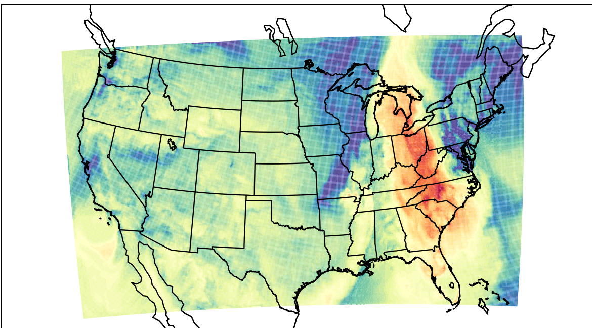
WRF (2022-10-25_18:00:00)
