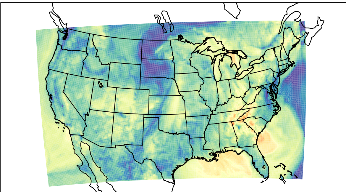
WRF (2022-10-24_04:00:00)
