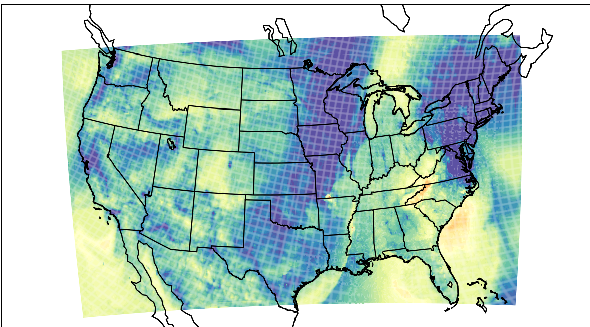
WRF (2022-10-25_14:00:00)
