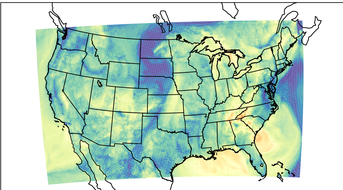
WRF (2022-10-24_05:00:00)
