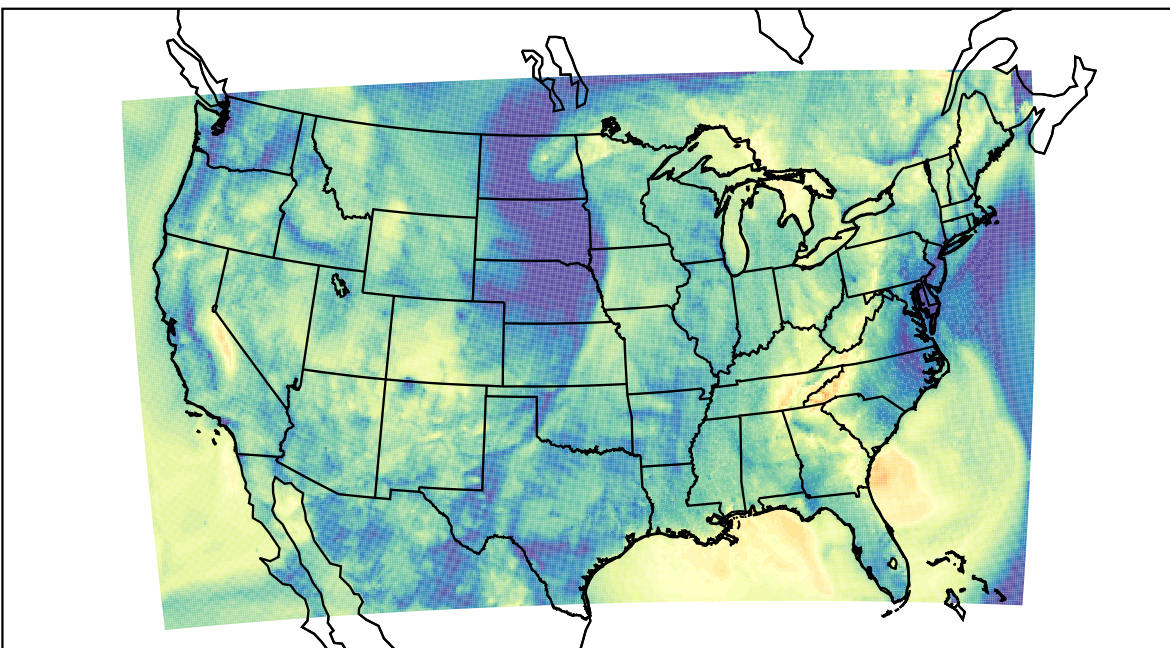
WRF (2022-10-24_08:00:00)
