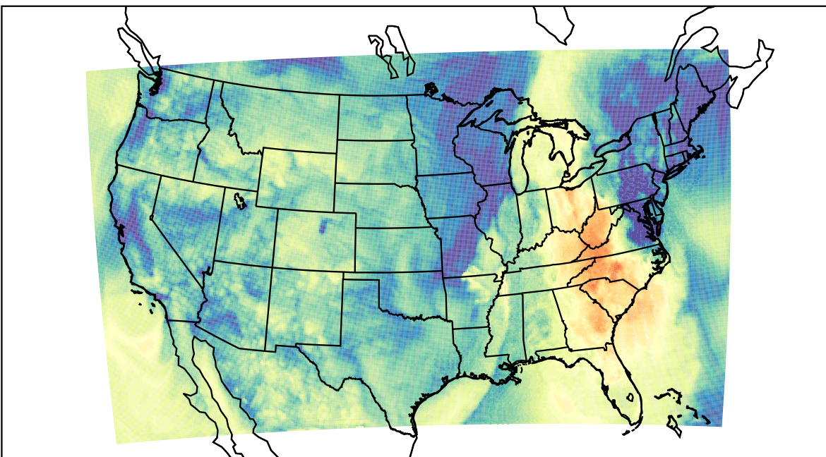
WRF (2022-10-25_16:00:00)
