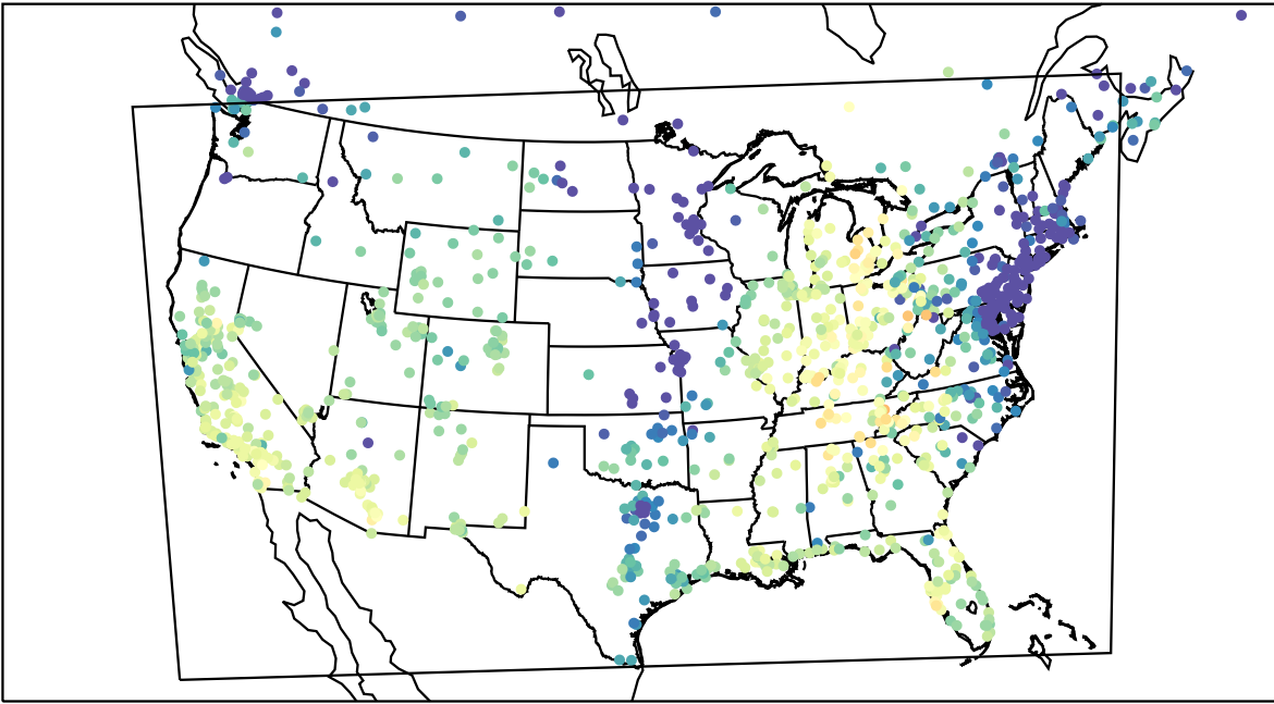
AirNOW (2022-10-24_22:00:00)
