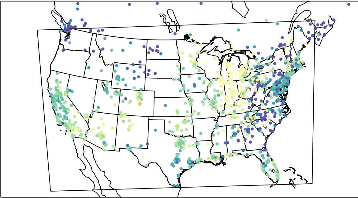
AirNOW (2022-10-24_01:00:00)
