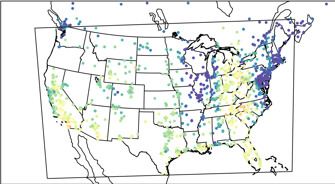
AirNOW (2022-10-25_21:00:00)
