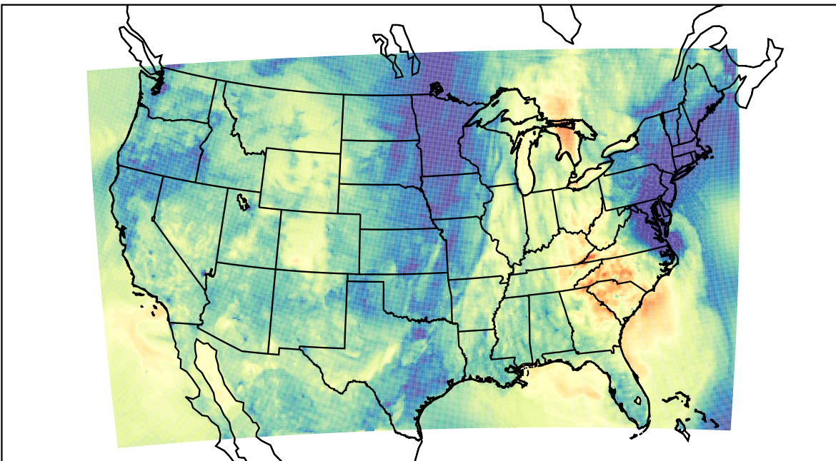
WRF (2022-10-25_02:00:00)
