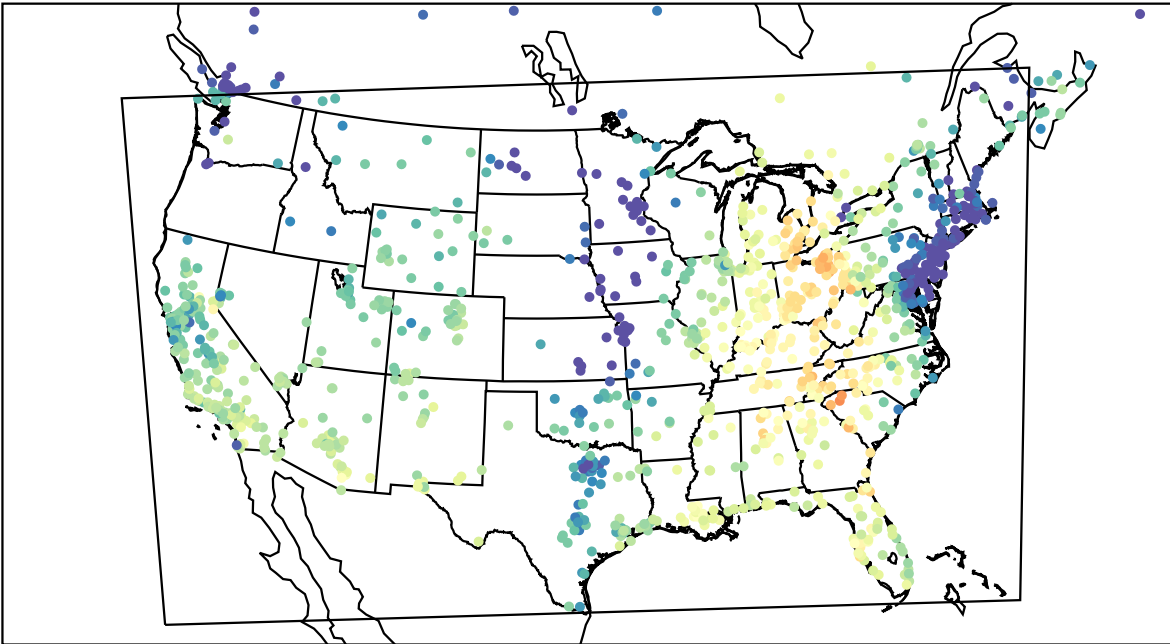
AirNOW (2022-10-24_19:00:00)
