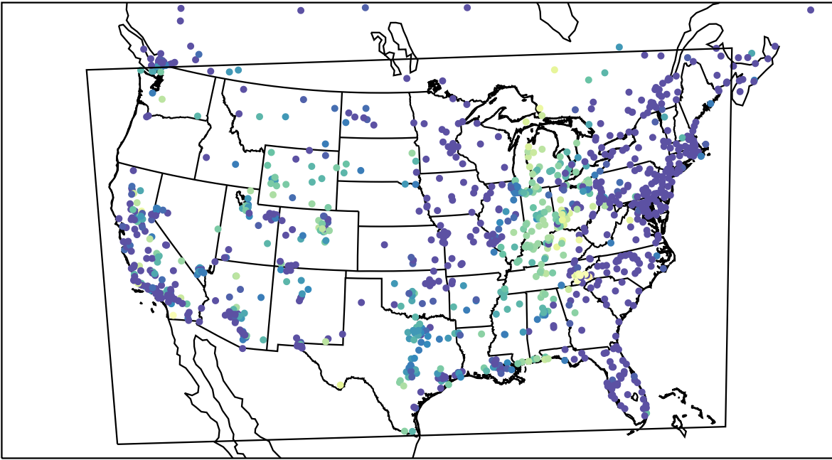
AirNOW (2022-10-25_11:00:00)
