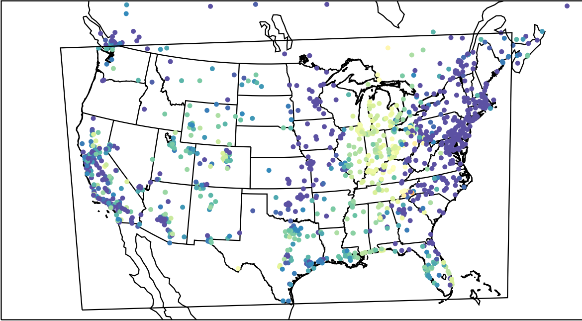
AirNOW (2022-10-25_04:00:00)
