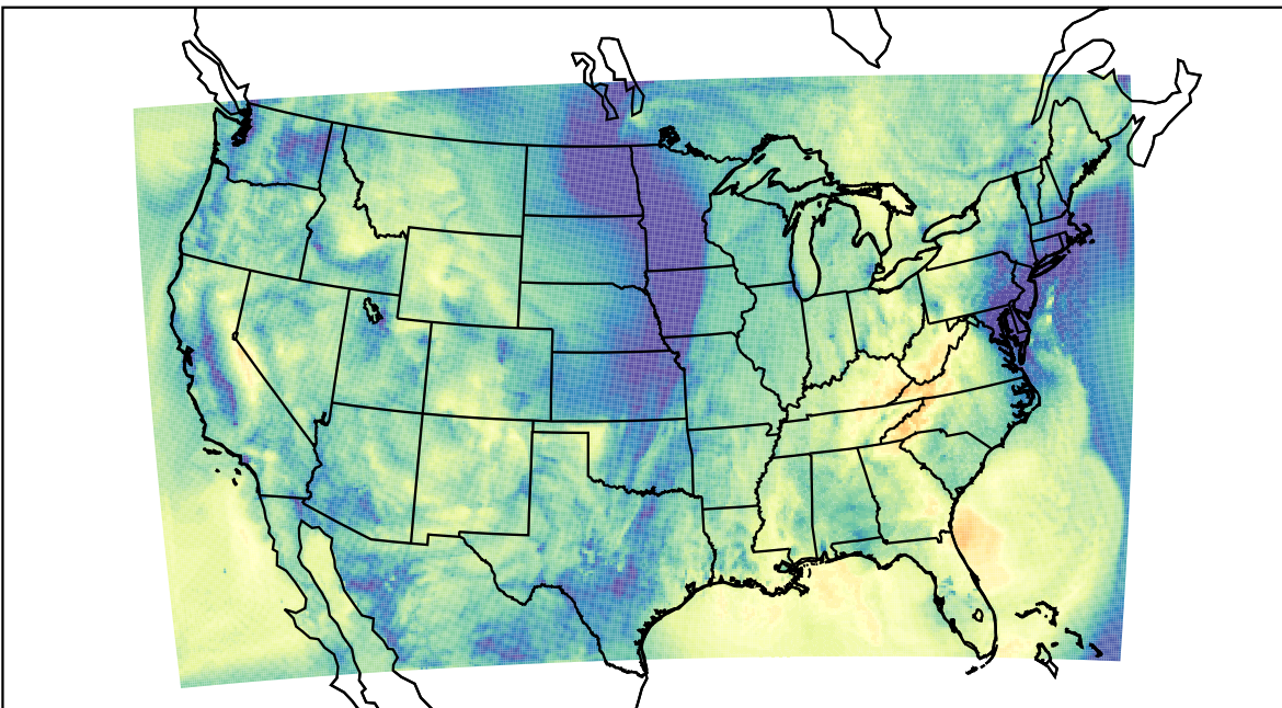
WRF (2022-10-24_15:00:00)
