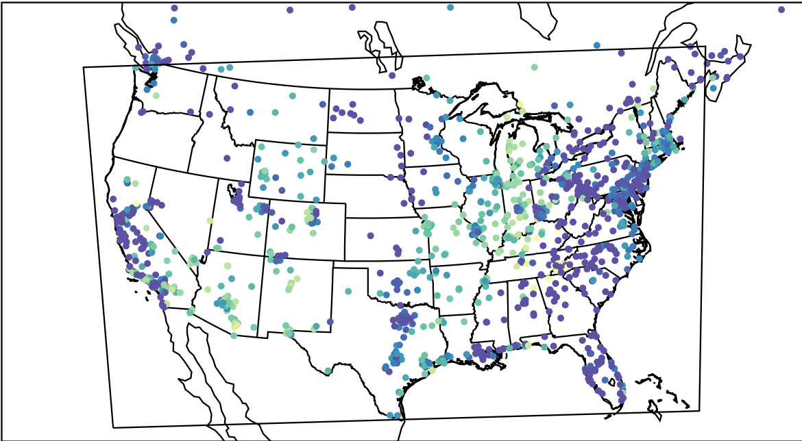
AirNOW (2022-10-24_12:00:00)
