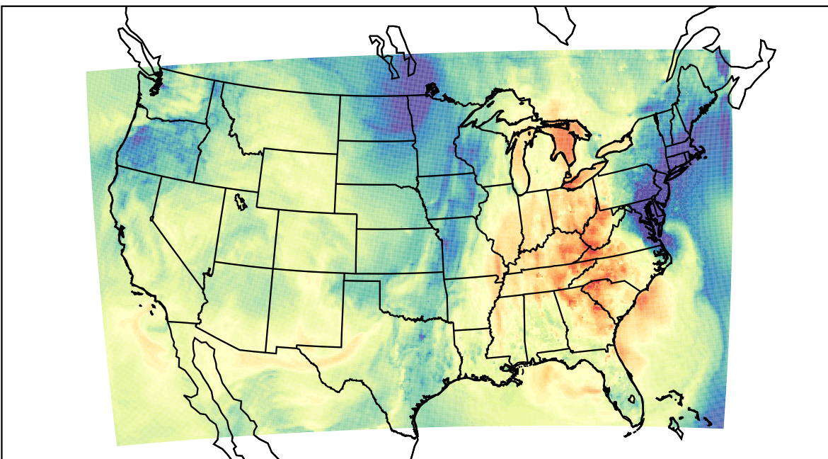
WRF (2022-10-24_22:00:00)
