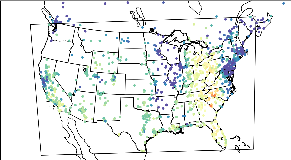
AirNOW (2022-10-25_18:00:00)
