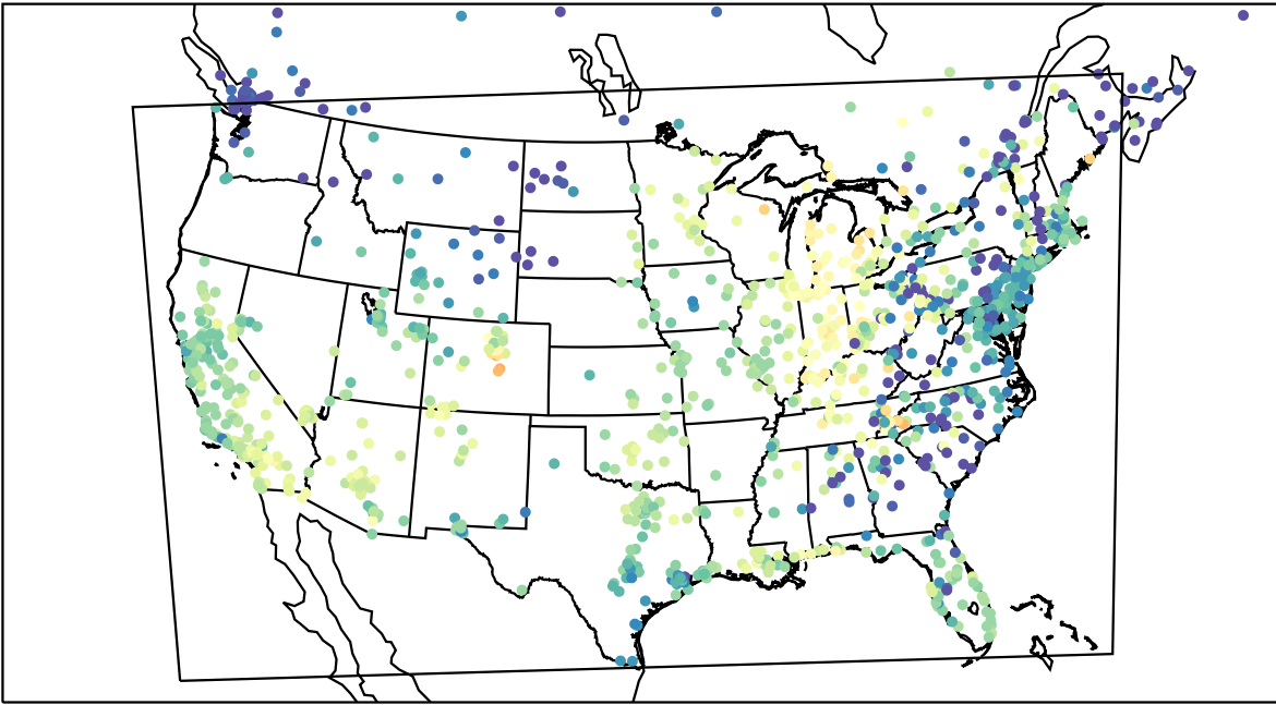
AirNOW (2022-10-24_00:00:00)
