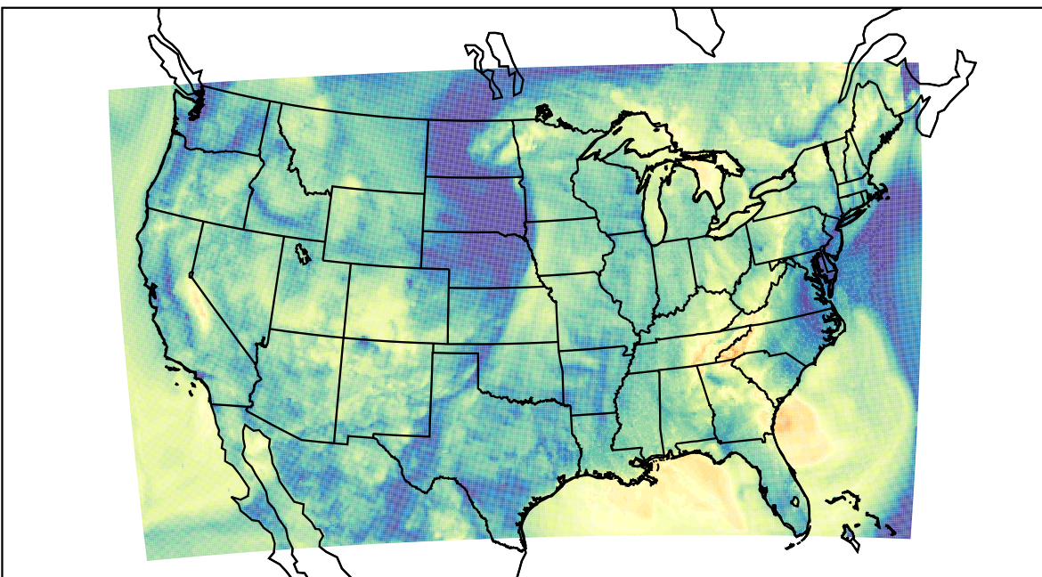
WRF (2022-10-24_07:00:00)
