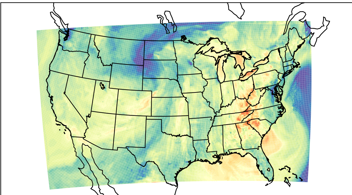
WRF (2022-10-24_00:00:00)
