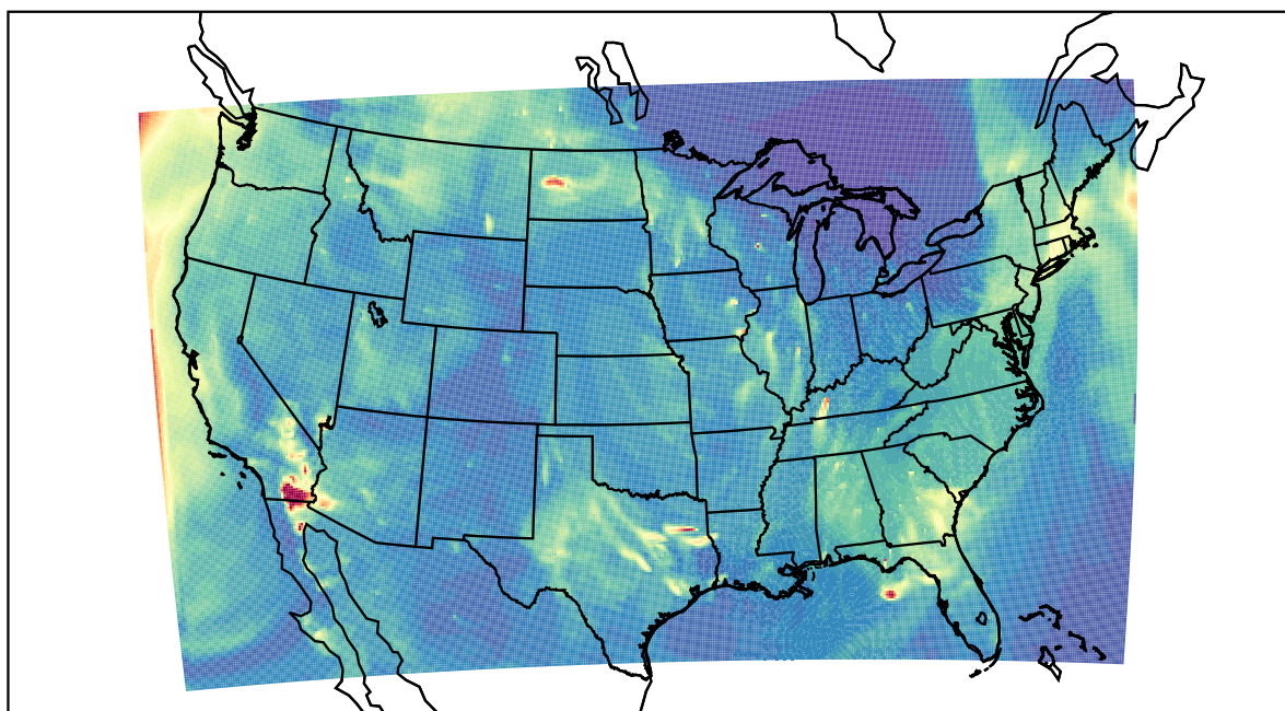
WRF 2022-10-27_06:00:00
