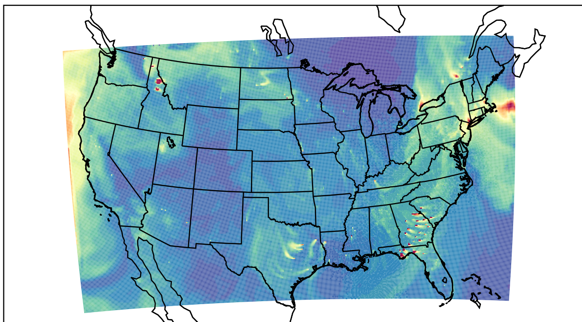
WRF 2022-10-26_22:00:00
