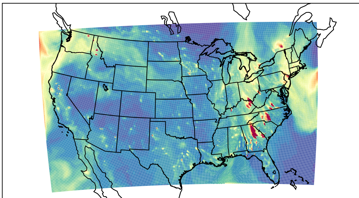
WRF 2022-10-26_01:00:00
