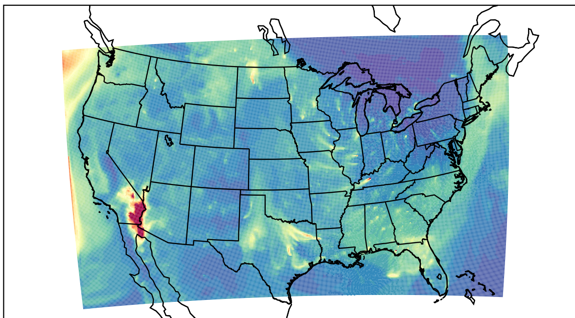
WRF 2022-10-27_13:00:00
