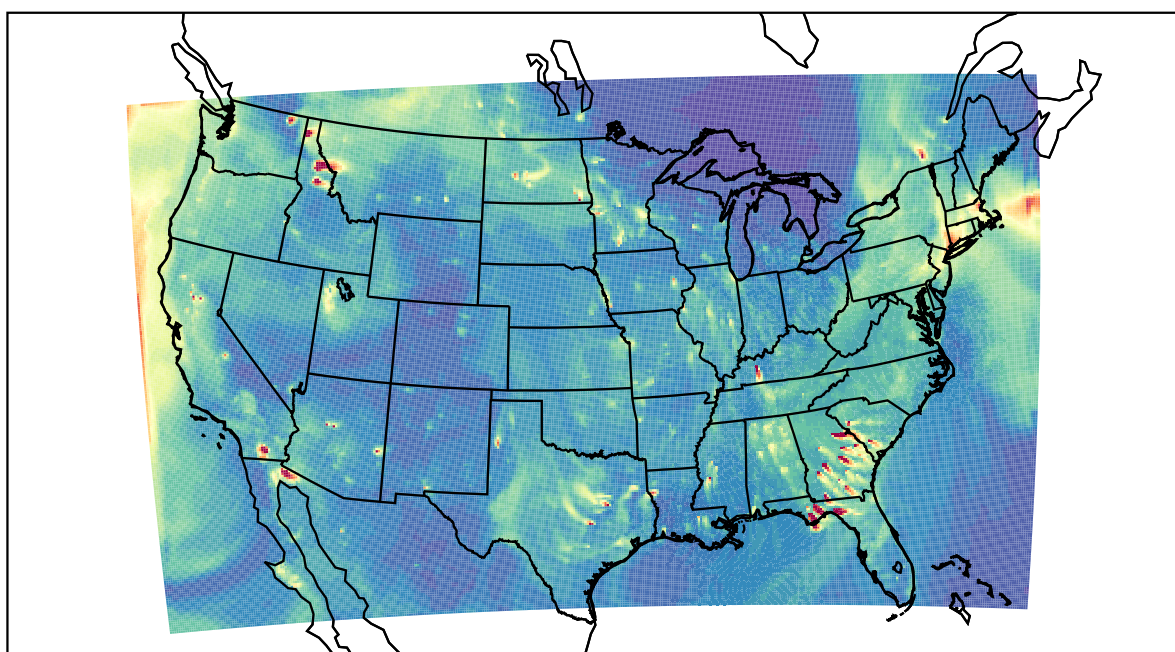
WRF 2022-10-27_01:00:00
