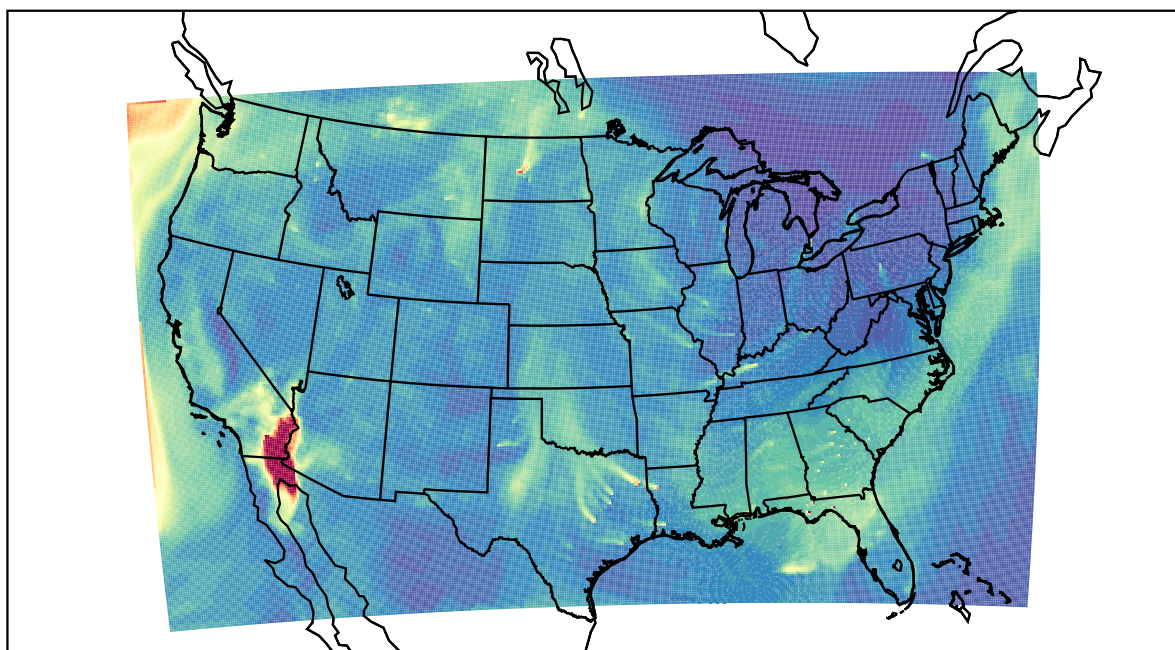
WRF 2022-10-27_17:00:00
