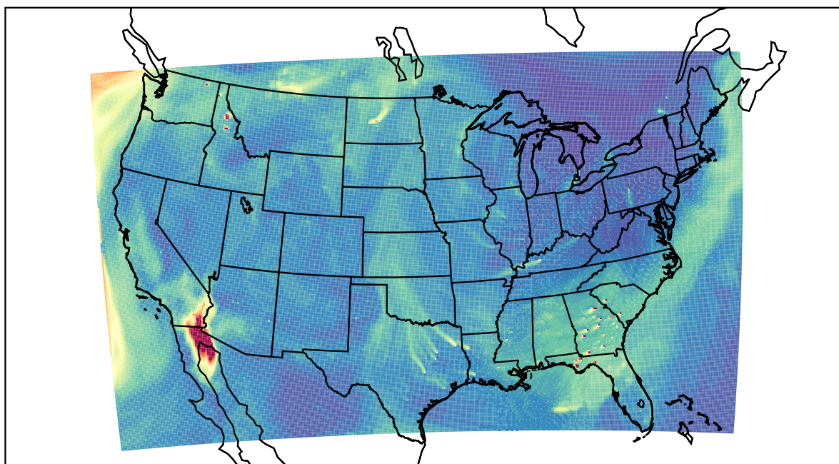
WRF 2022-10-27_20:00:00
