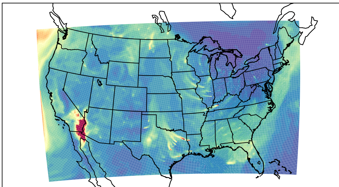
WRF 2022-10-27_15:00:00
