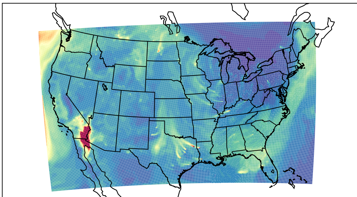
WRF 2022-10-27_16:00:00
