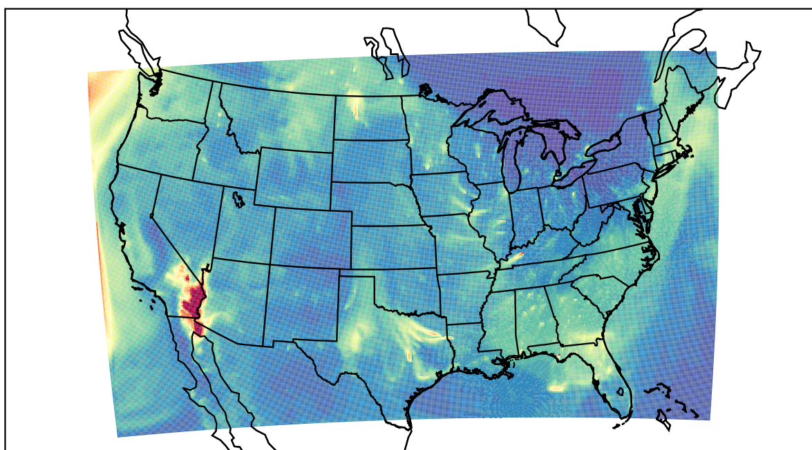
WRF 2022-10-27_12:00:00
