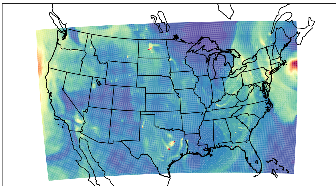
WRF 2022-10-26_17:00:00
