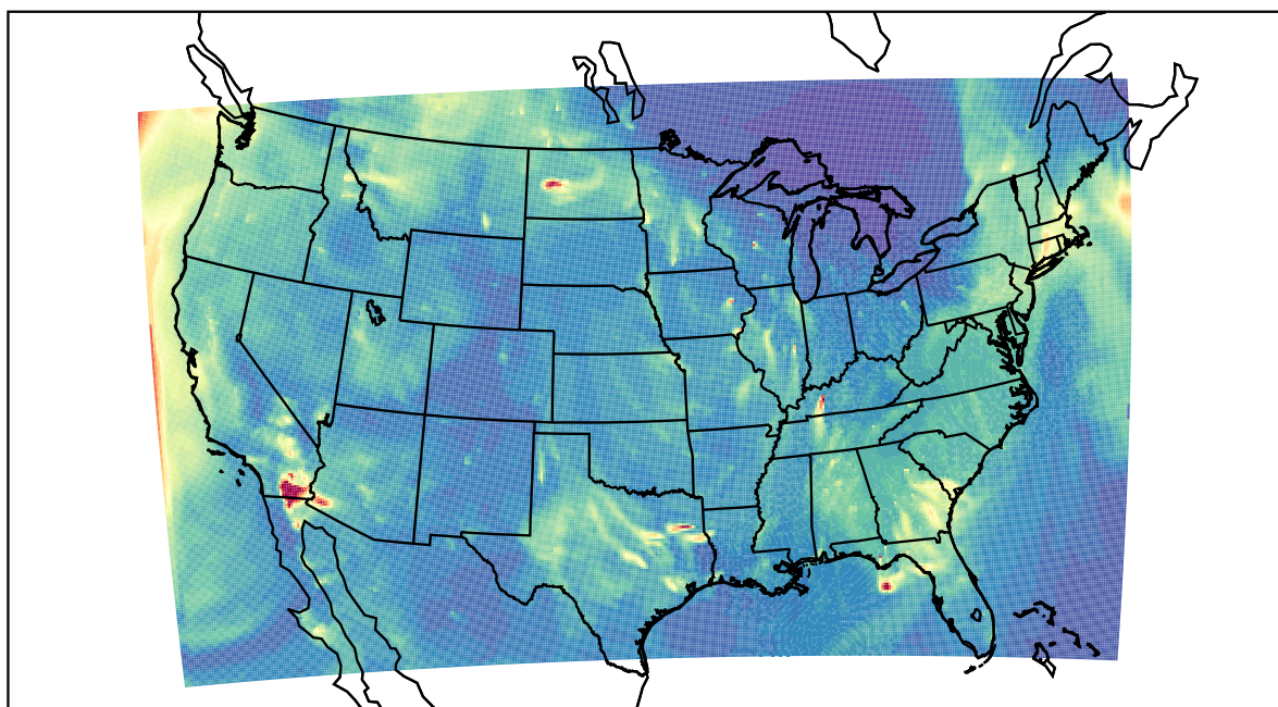
WRF 2022-10-27_05:00:00
