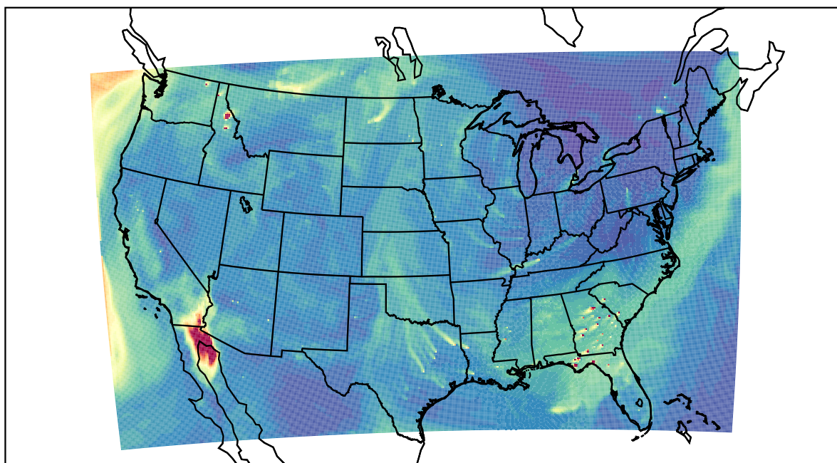
WRF 2022-10-27_21:00:00
