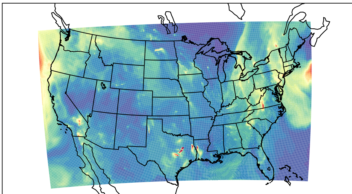
WRF 2022-10-26_10:00:00
