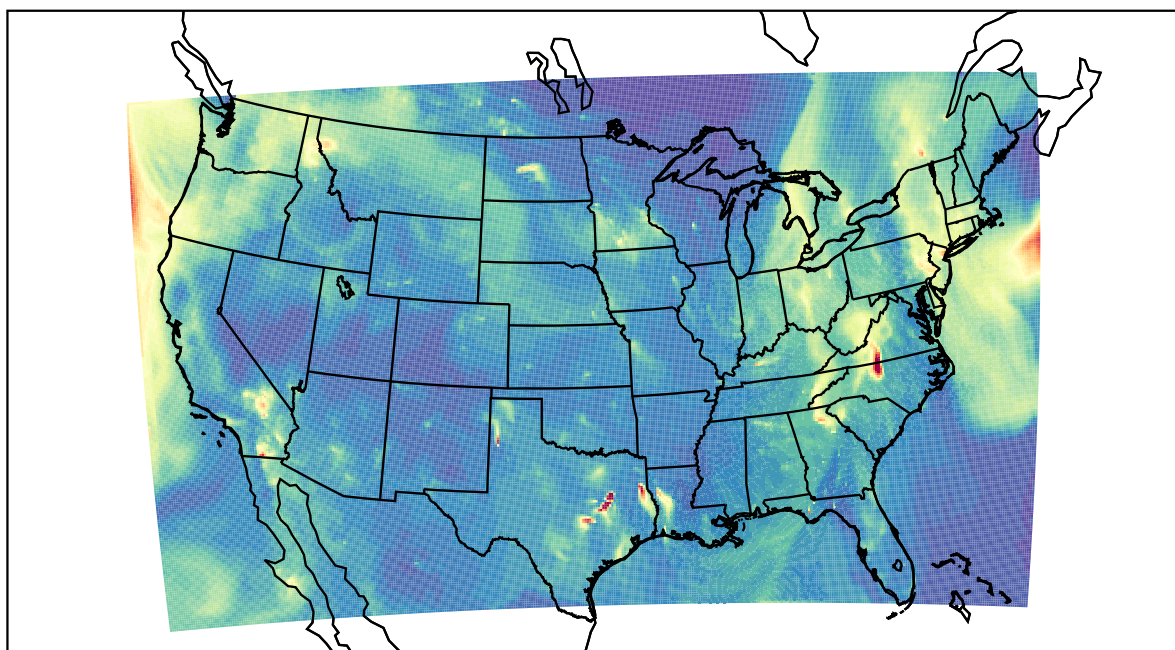
WRF 2022-10-26_08:00:00
