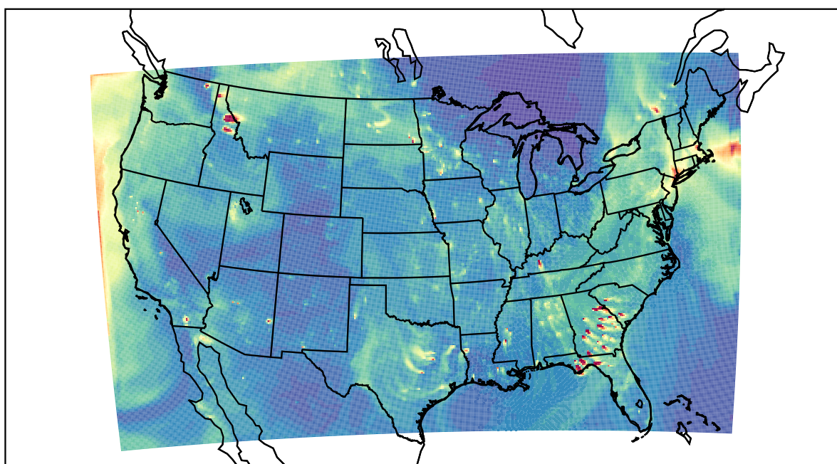
WRF 2022-10-27_00:00:00
