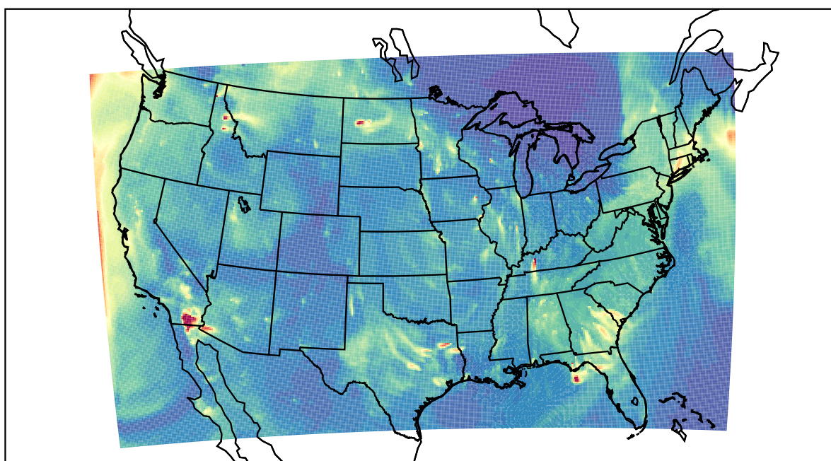
WRF 2022-10-27_04:00:00
