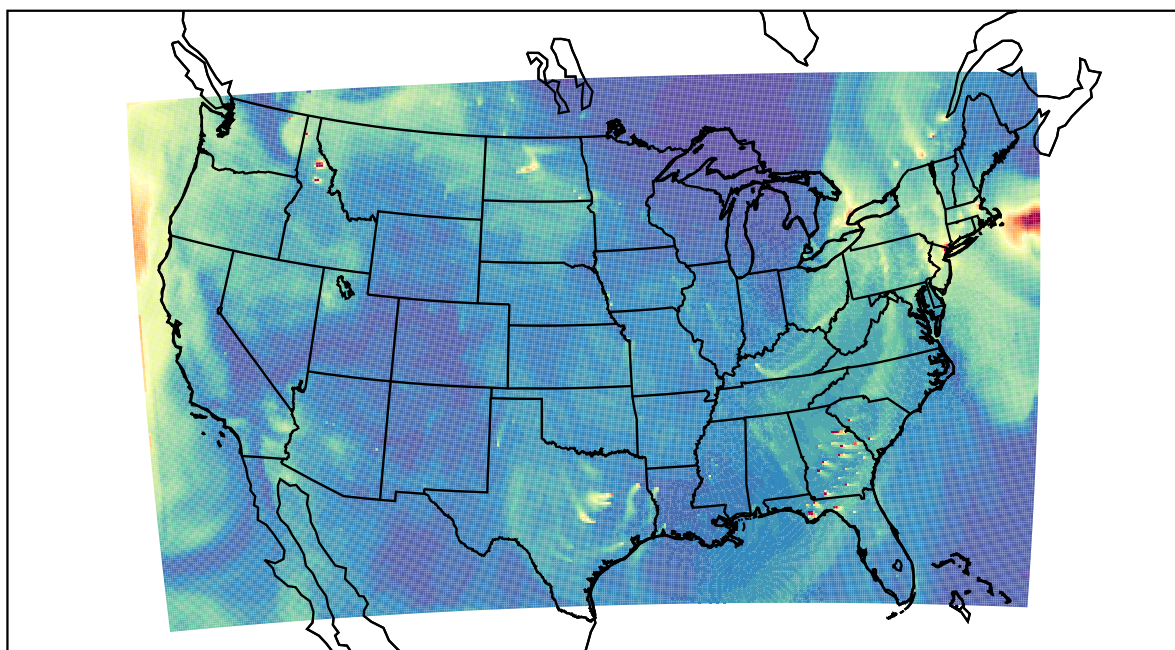
WRF 2022-10-26_20:00:00
