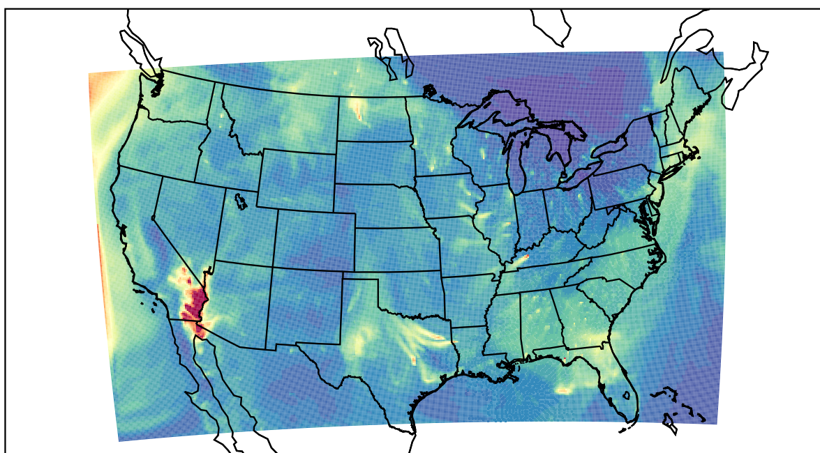
WRF 2022-10-27_11:00:00
