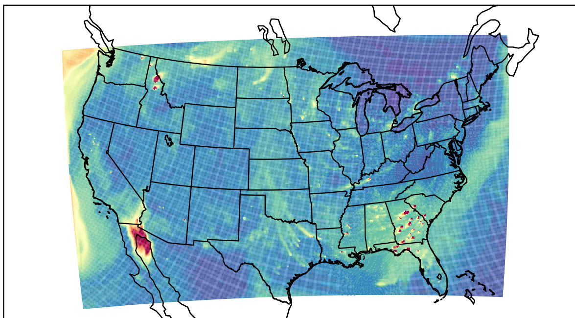
WRF 2022-10-27_23:00:00
