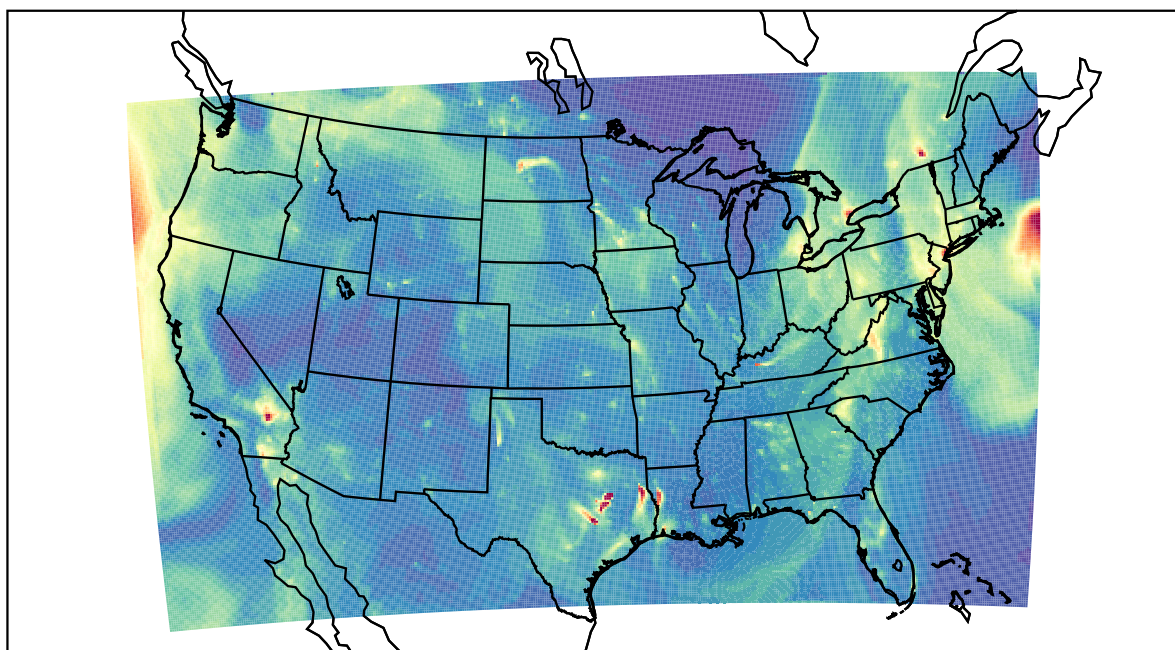
WRF 2022-10-26_13:00:00
