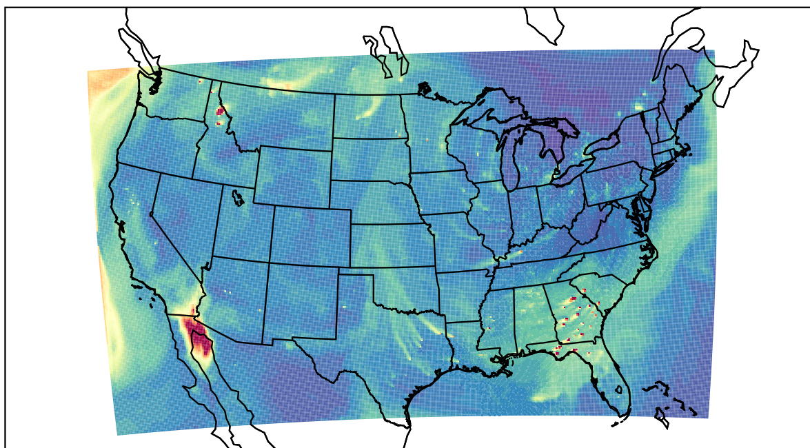
WRF 2022-10-27_22:00:00
