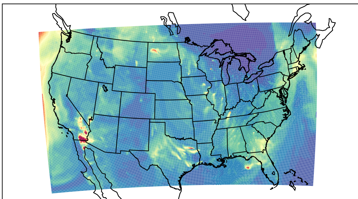
WRF 2022-10-27_07:00:00
