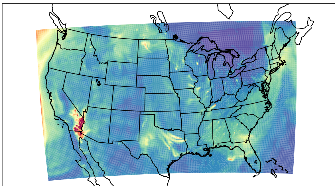
WRF 2022-10-27_10:00:00
