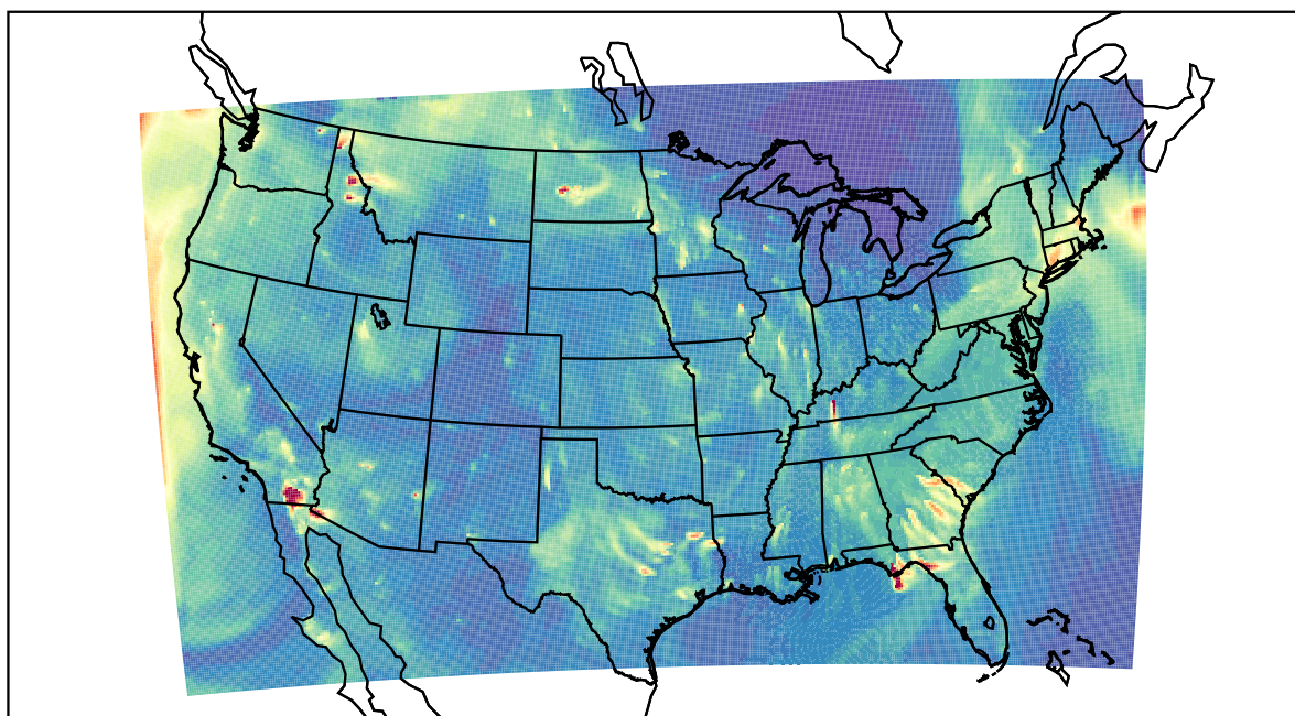
WRF 2022-10-27_03:00:00
