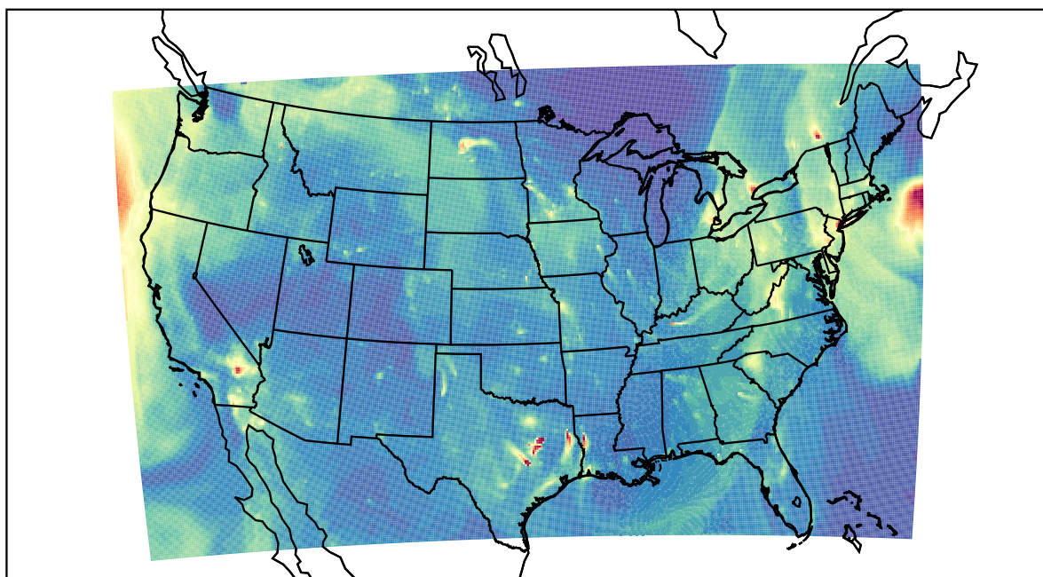
WRF 2022-10-26_14:00:00
