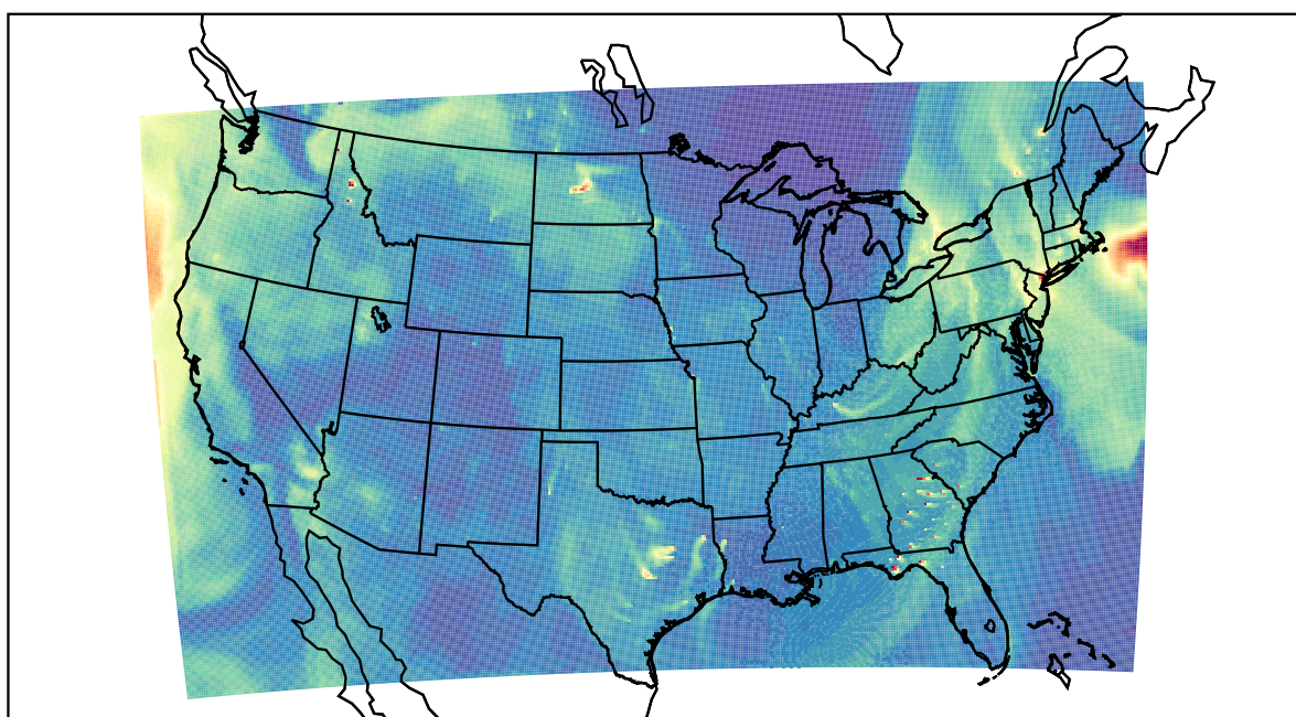
WRF 2022-10-26_19:00:00
