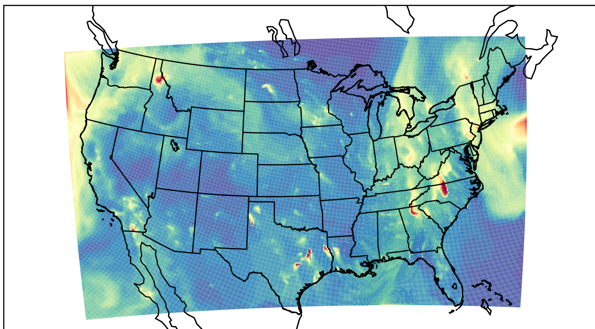
WRF 2022-10-26_06:00:00
