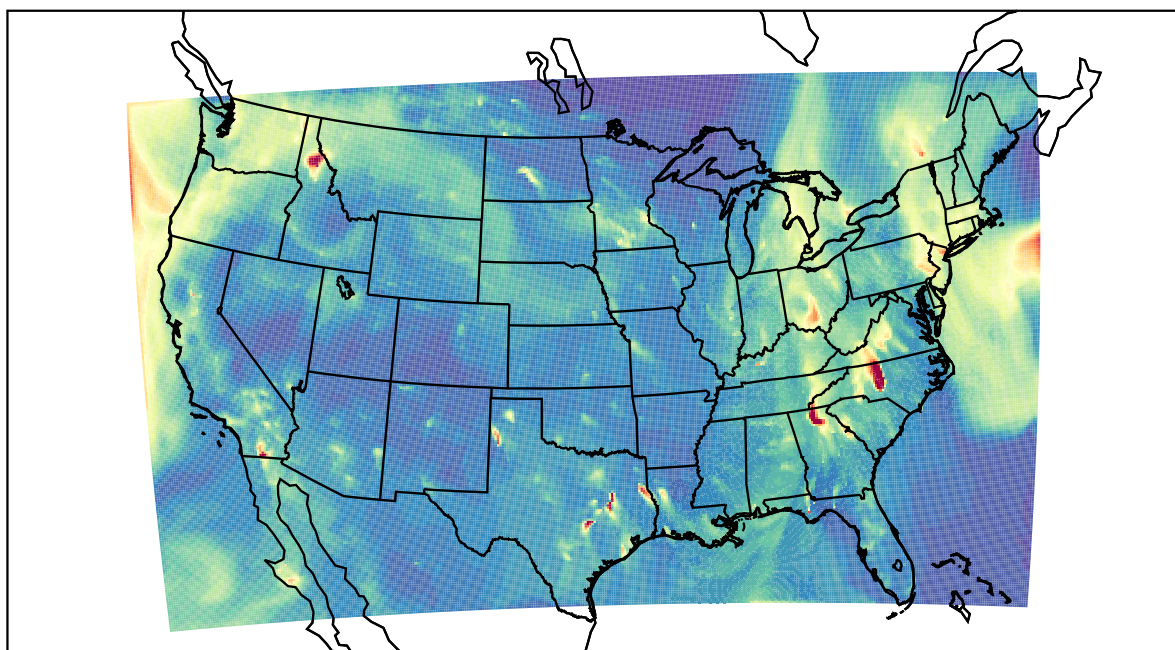
WRF 2022-10-26_05:00:00
