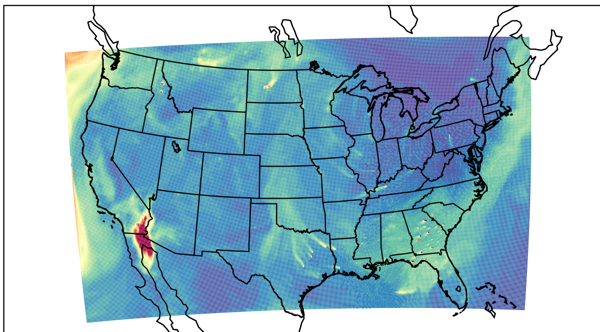
WRF 2022-10-27_19:00:00
