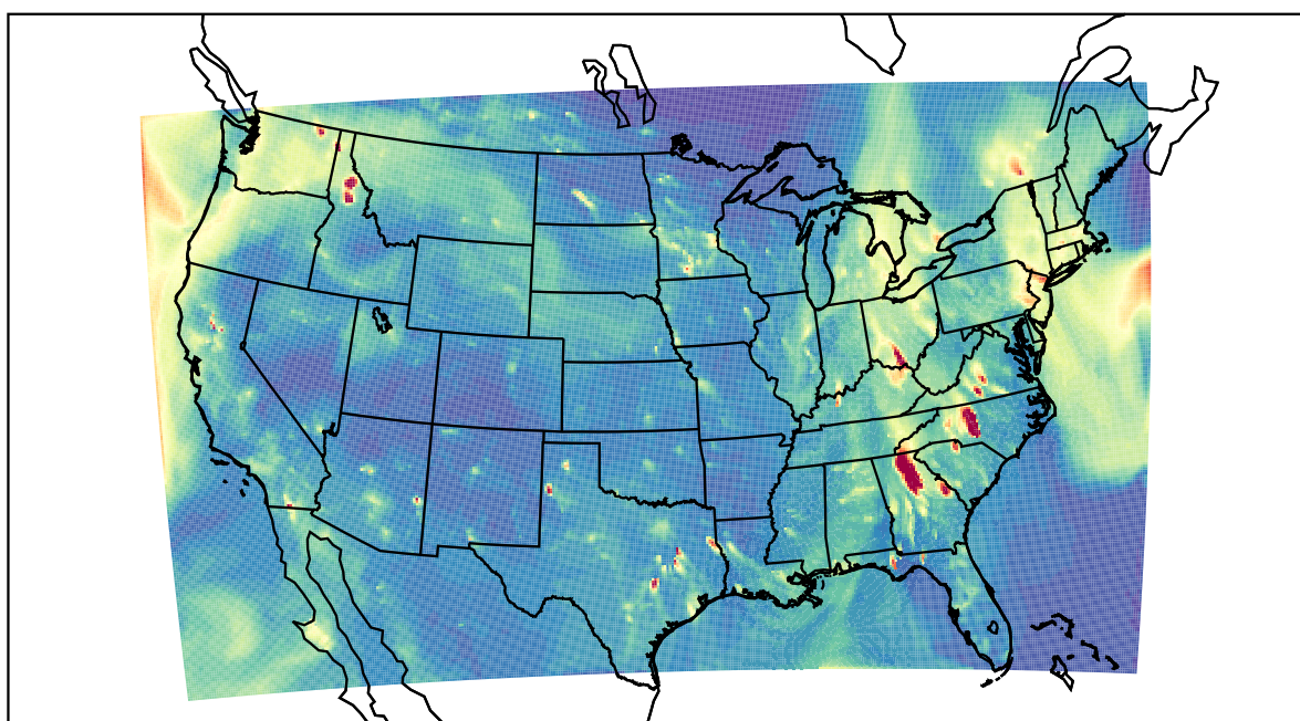
WRF 2022-10-26_03:00:00
