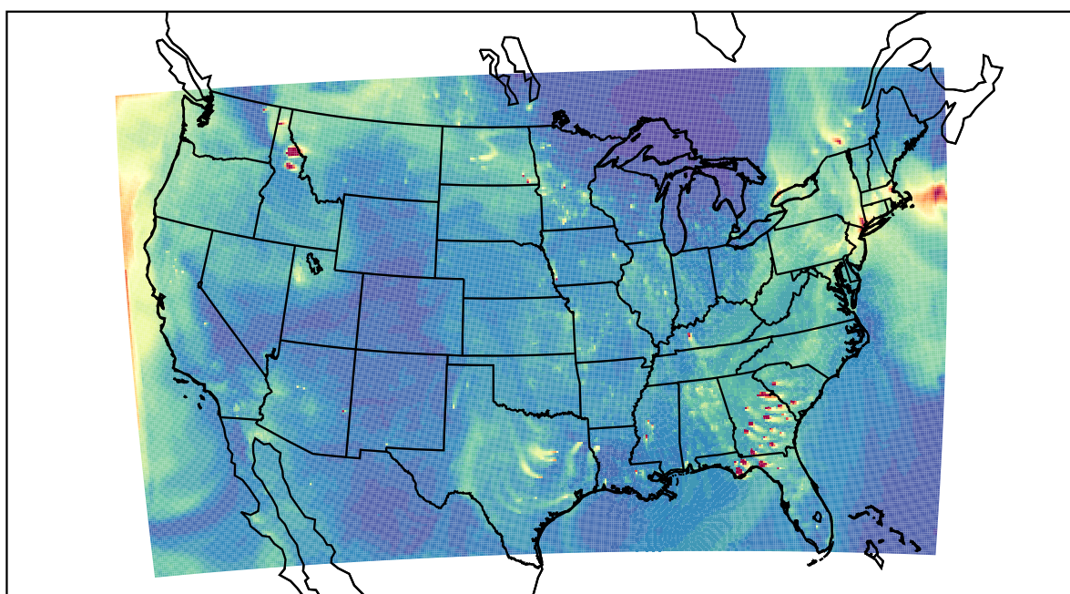
WRF 2022-10-26_23:00:00
