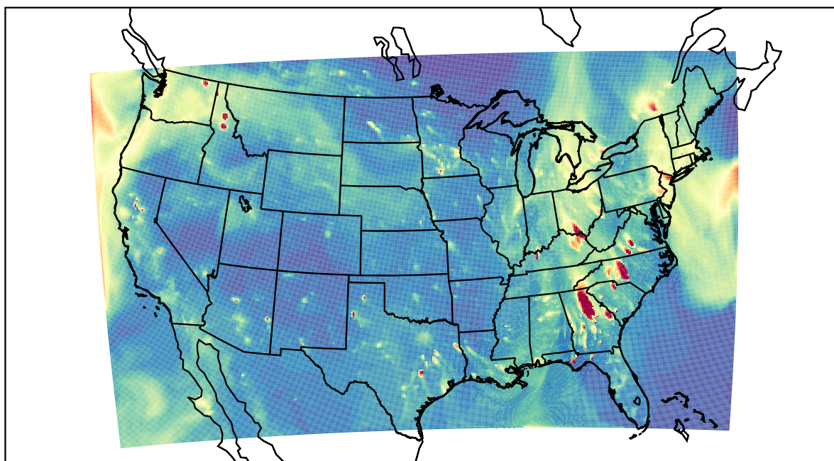
WRF 2022-10-26_02:00:00
