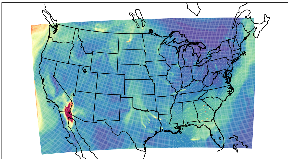
WRF 2022-10-27_18:00:00
