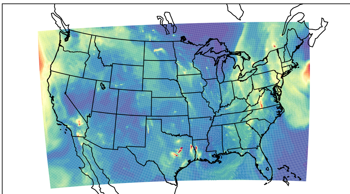
WRF 2022-10-26_11:00:00
