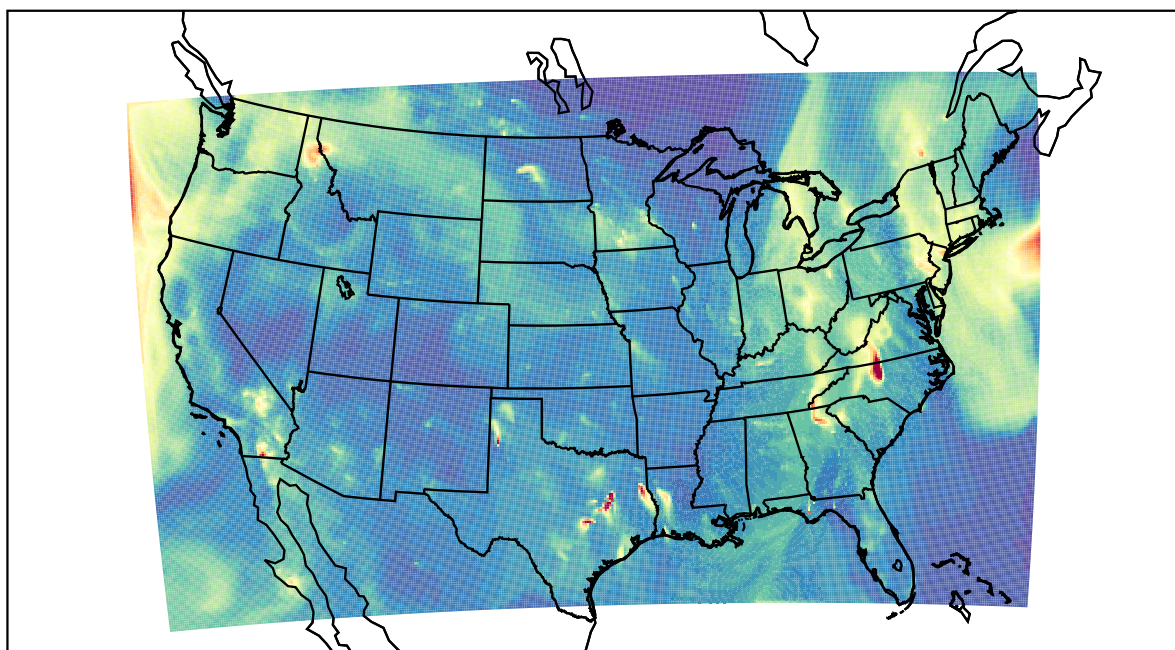
WRF 2022-10-26_07:00:00
