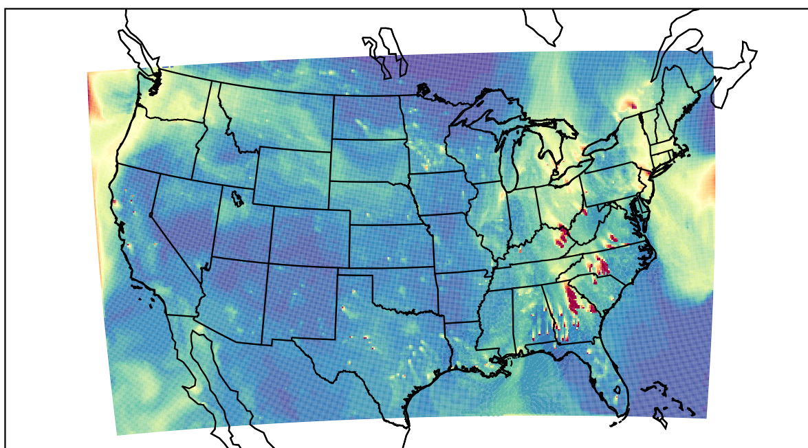
WRF 2022-10-26_00:00:00
