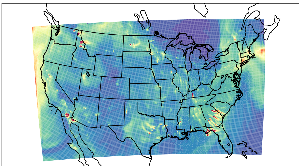
WRF 2022-10-27_02:00:00
