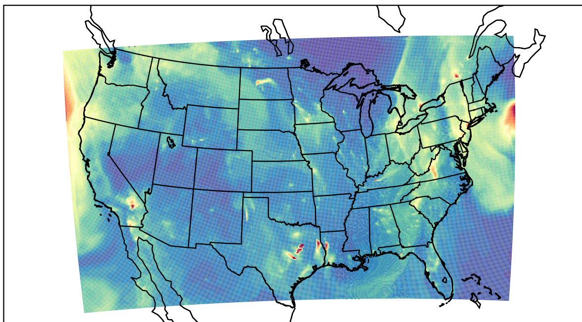
WRF 2022-10-26_12:00:00
