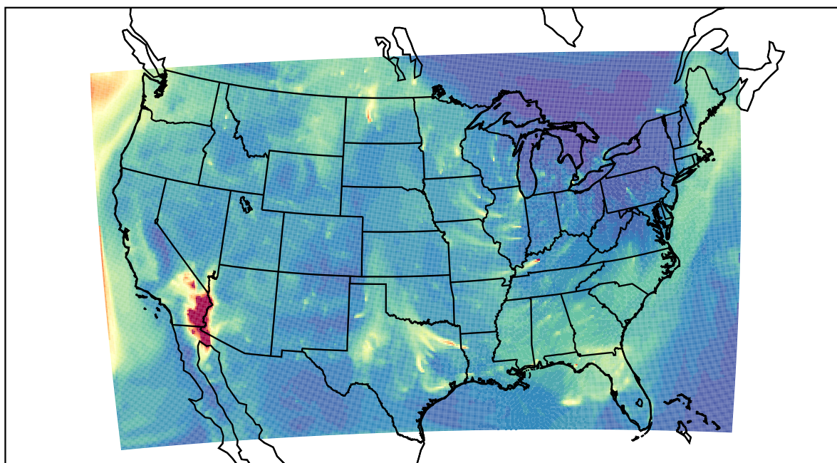
WRF 2022-10-27_14:00:00
