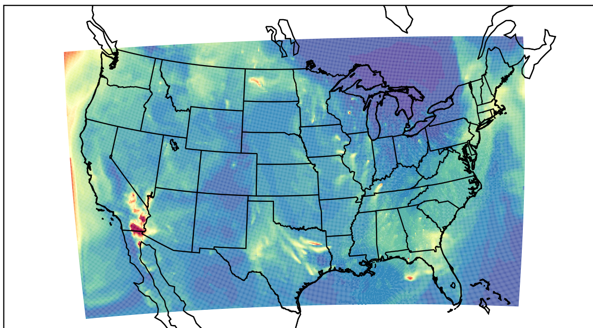
WRF 2022-10-27_08:00:00
