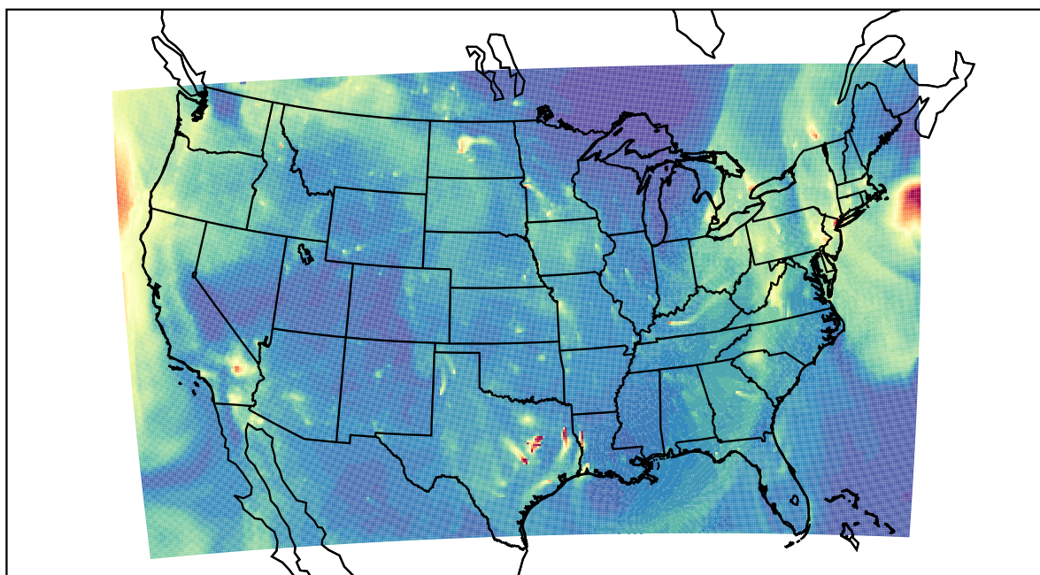
WRF 2022-10-26_15:00:00
