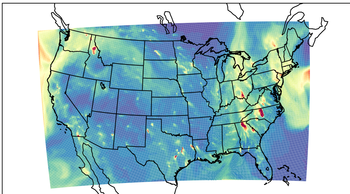
WRF 2022-10-26_04:00:00
