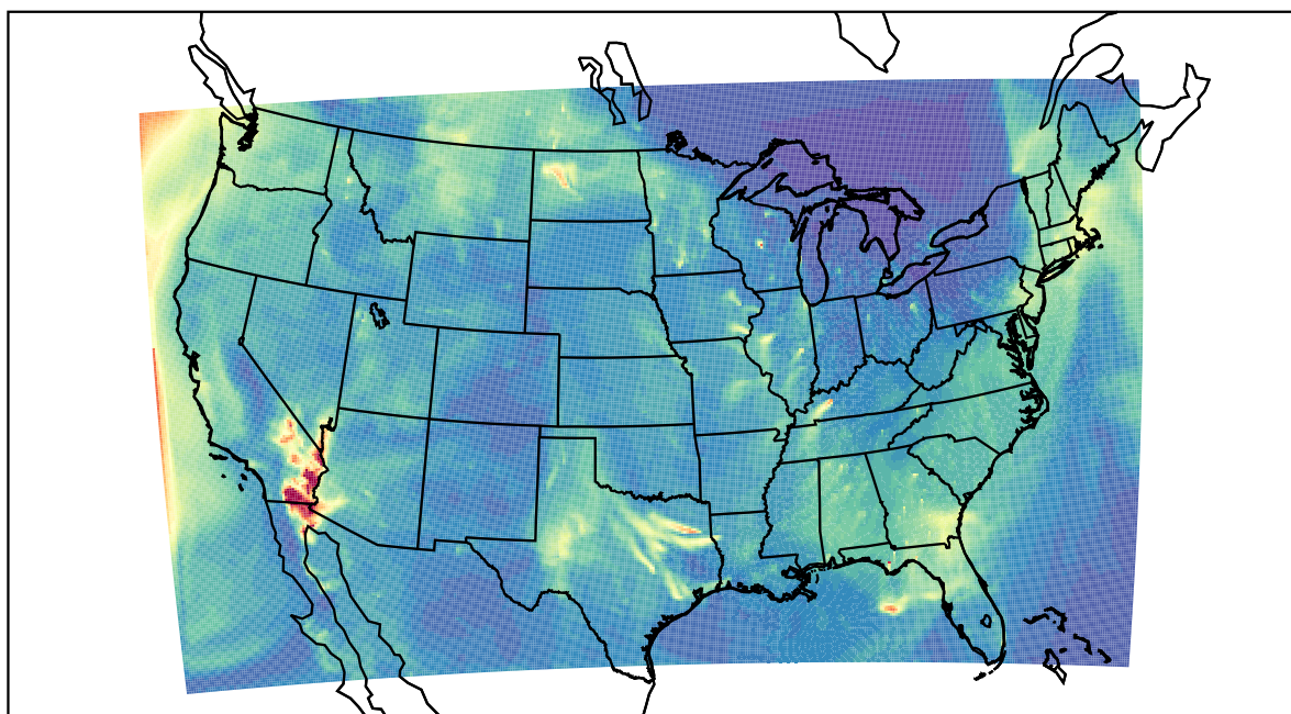
WRF 2022-10-27_09:00:00
