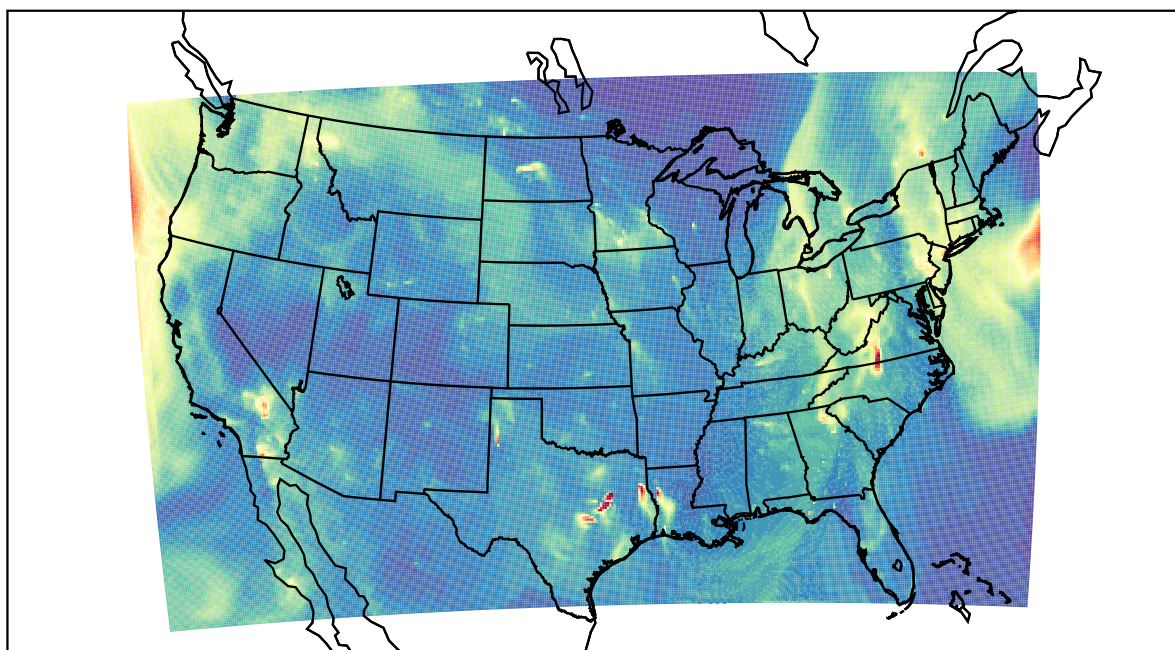
WRF 2022-10-26_09:00:00
