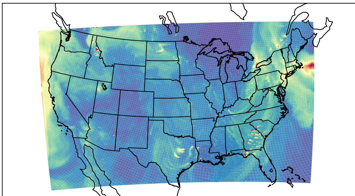
WRF 2022-10-26_21:00:00
