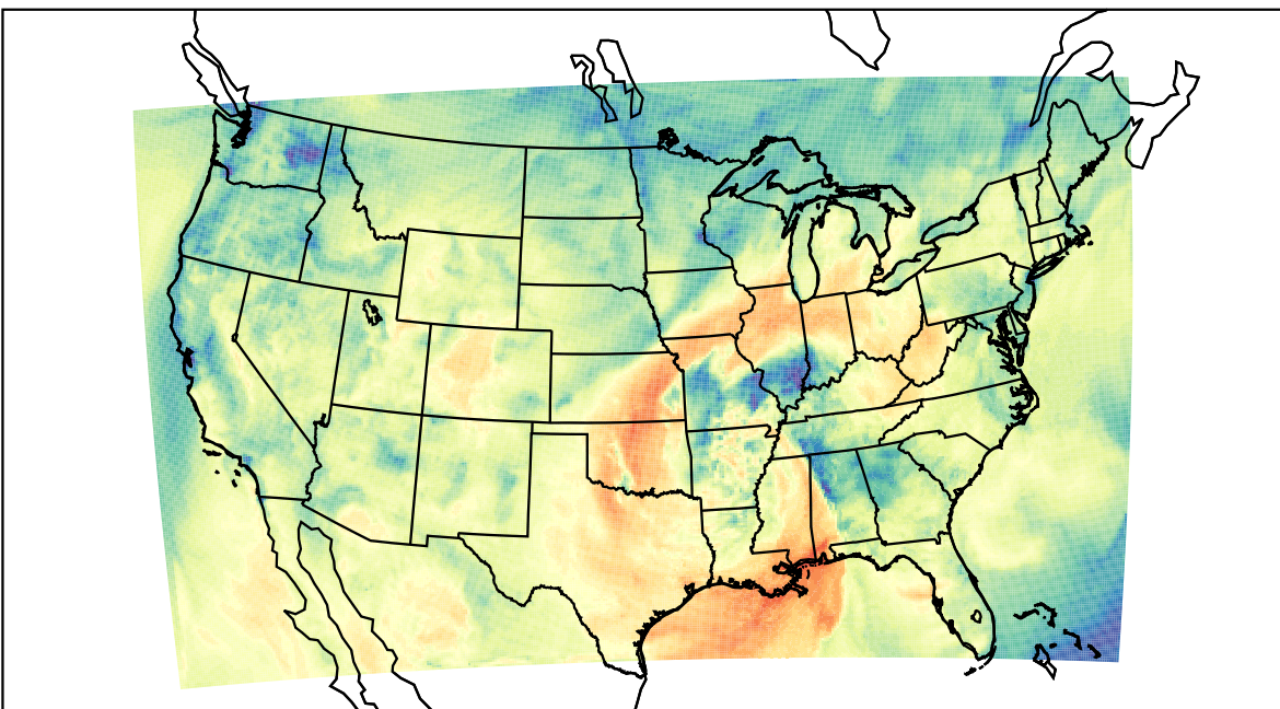
WRF (2022-10-30_19:00:00)
