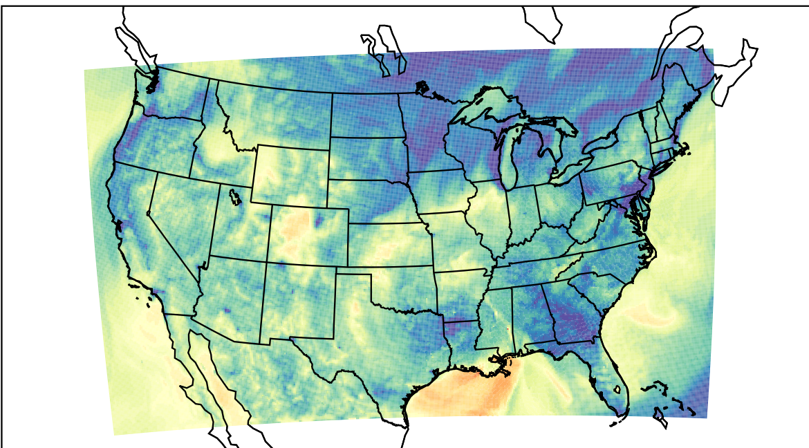
WRF (2022-10-30_07:00:00)
