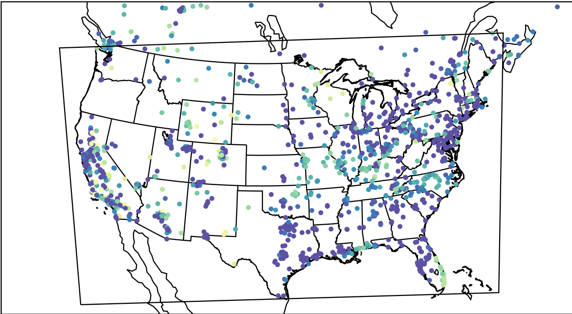
AirNOW (2022-10-30_07:00:00)
