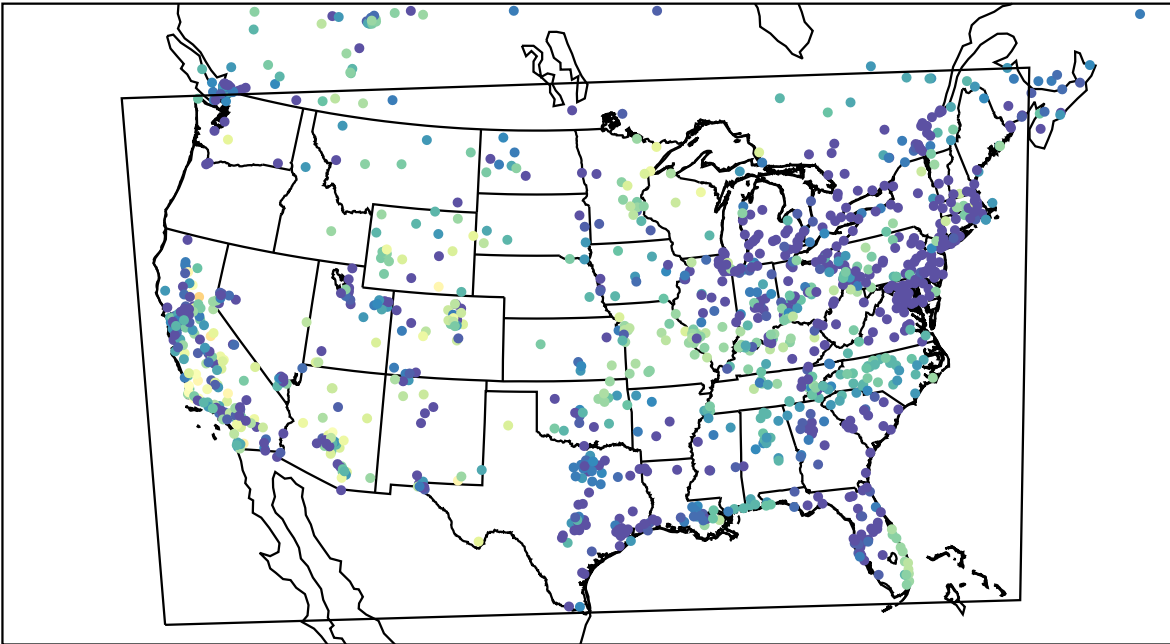
AirNOW (2022-10-30_03:00:00)
