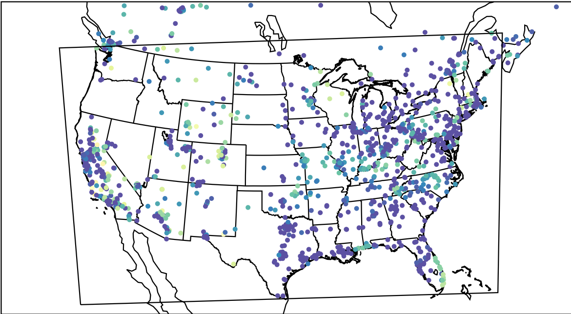
AirNOW (2022-10-30_09:00:00)
