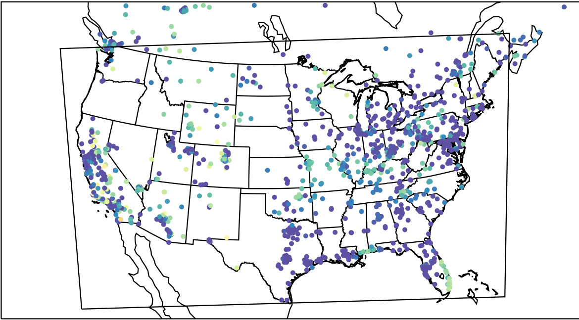
AirNOW (2022-10-30_08:00:00)
