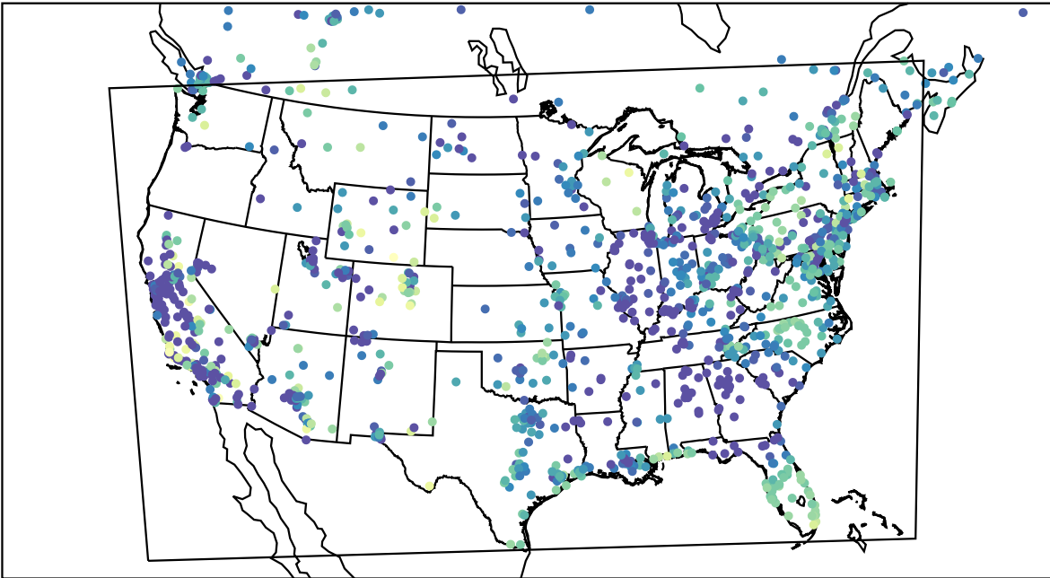
AirNOW (2022-10-30_15:00:00)
