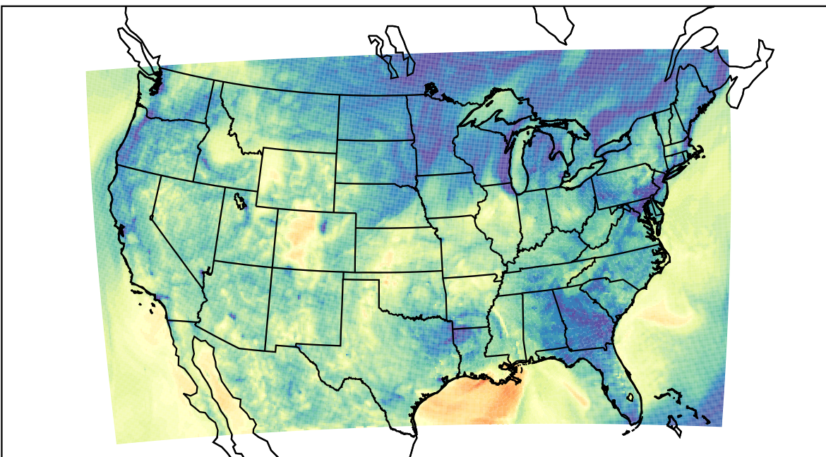
WRF (2022-10-30_05:00:00)
