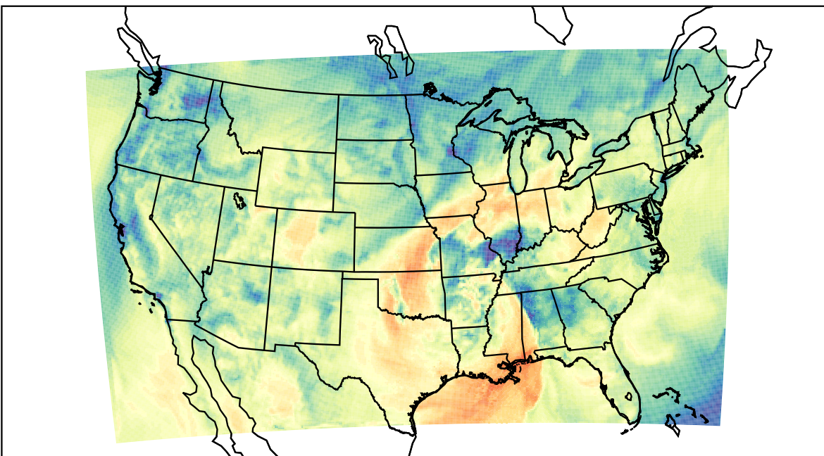
WRF (2022-10-30_18:00:00)
