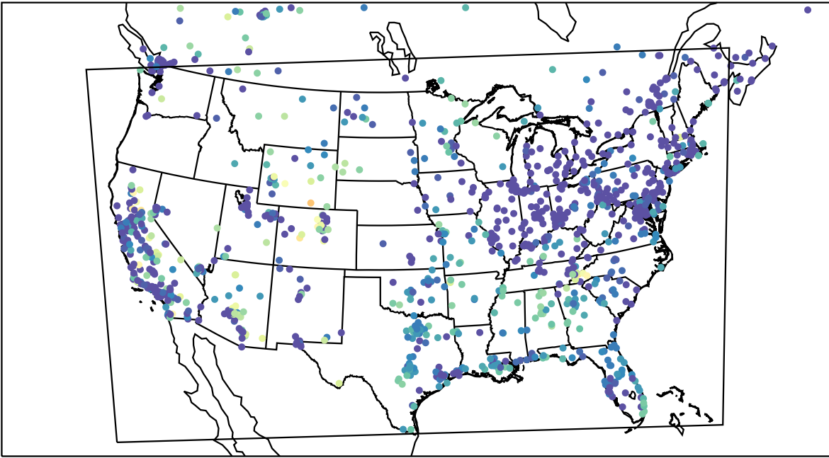
AirNOW (2022-10-29_08:00:00)
