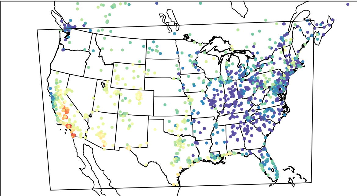
AirNOW (2022-10-30_23:00:00)
