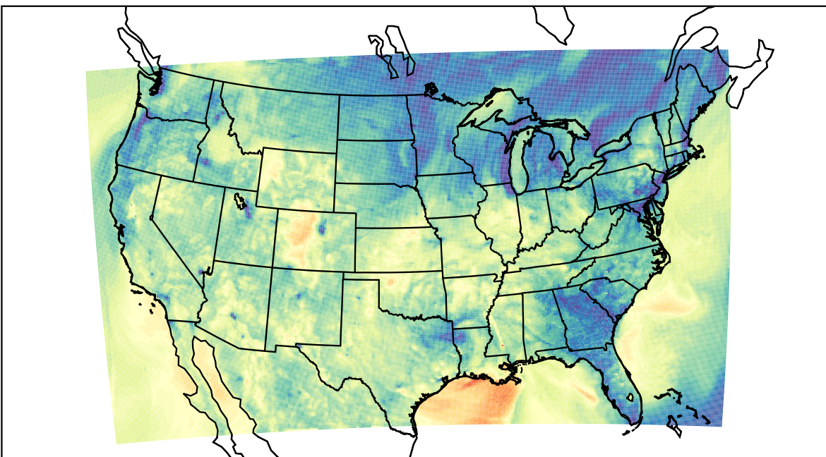
WRF (2022-10-30_02:00:00)
