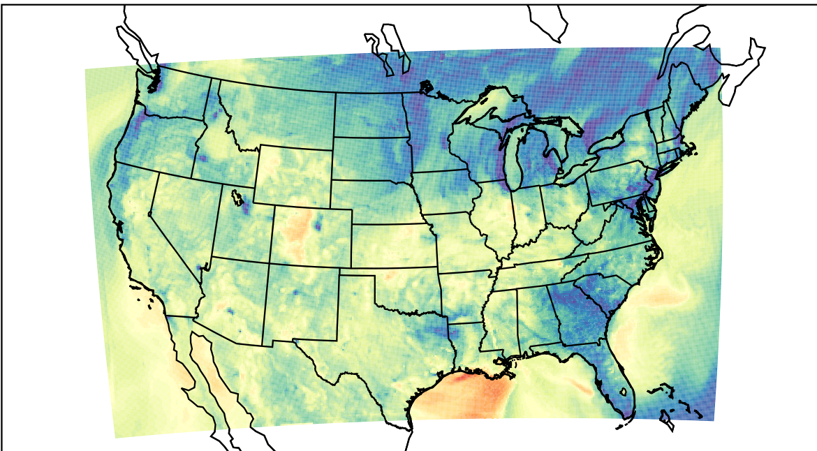
WRF (2022-10-30_01:00:00)
