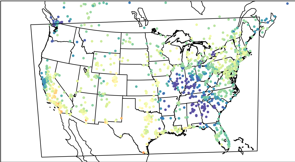
AirNOW (2022-10-30_19:00:00)
