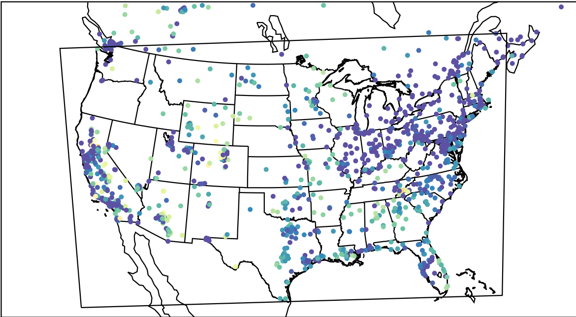
AirNOW (2022-10-29_05:00:00)
