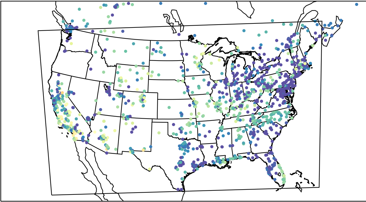
AirNOW (2022-10-30_02:00:00)
