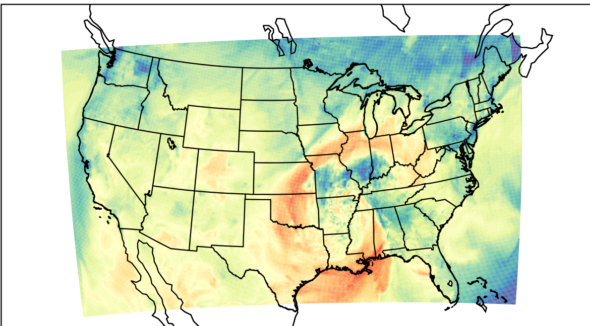
WRF (2022-10-30_21:00:00)
