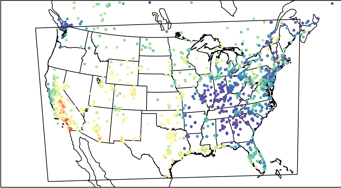
AirNOW (2022-10-30_22:00:00)
