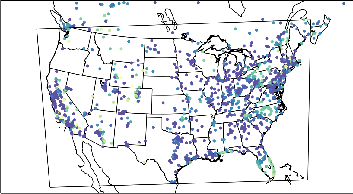
AirNOW (2022-10-30_14:00:00)
