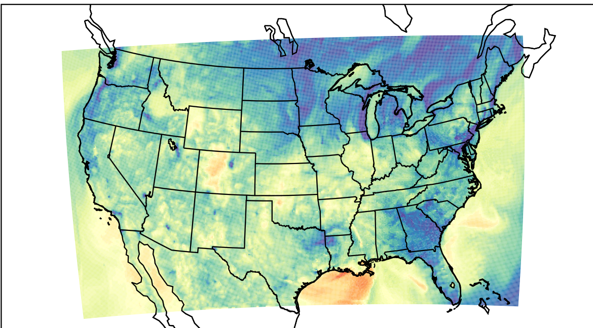
WRF (2022-10-30_03:00:00)
