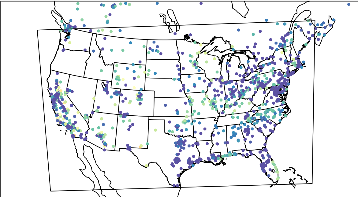
AirNOW (2022-10-30_05:00:00)
