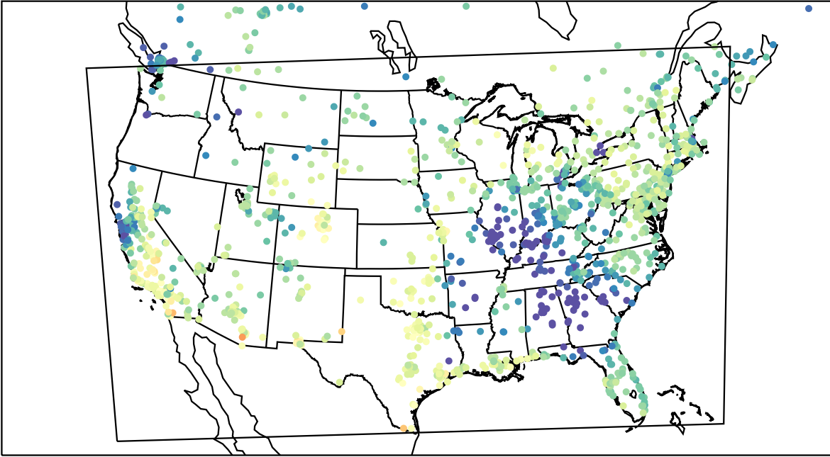
AirNOW (2022-10-30_18:00:00)
