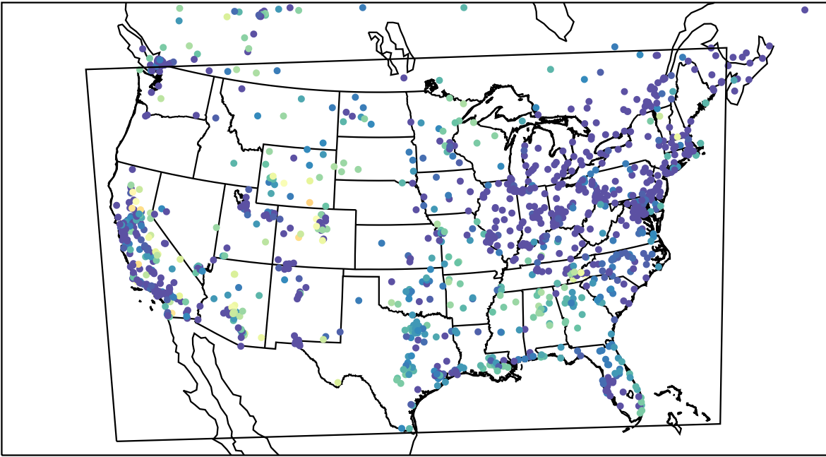
AirNOW (2022-10-29_07:00:00)
