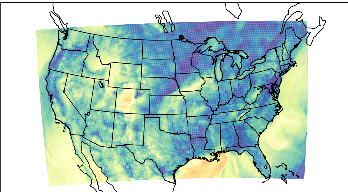
WRF (2022-10-30_13:00:00)
