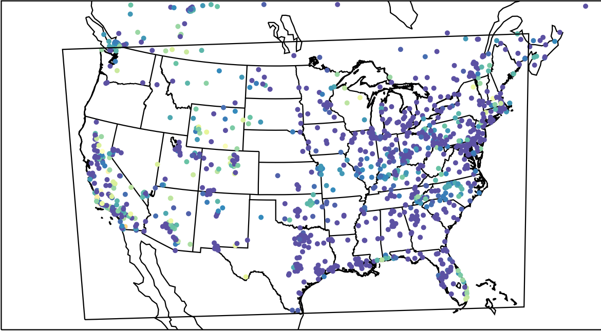
AirNOW (2022-10-30_11:00:00)
