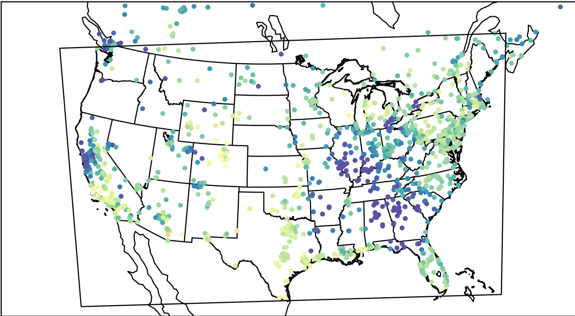
AirNOW (2022-10-30_17:00:00)
