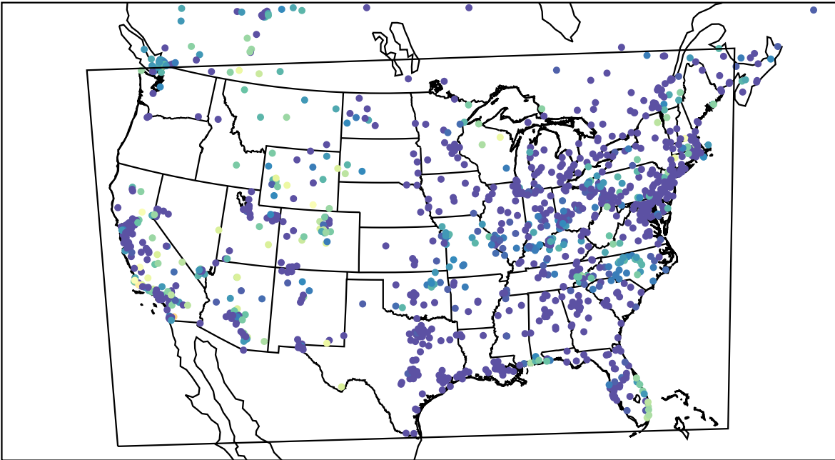
AirNOW (2022-10-30_12:00:00)
