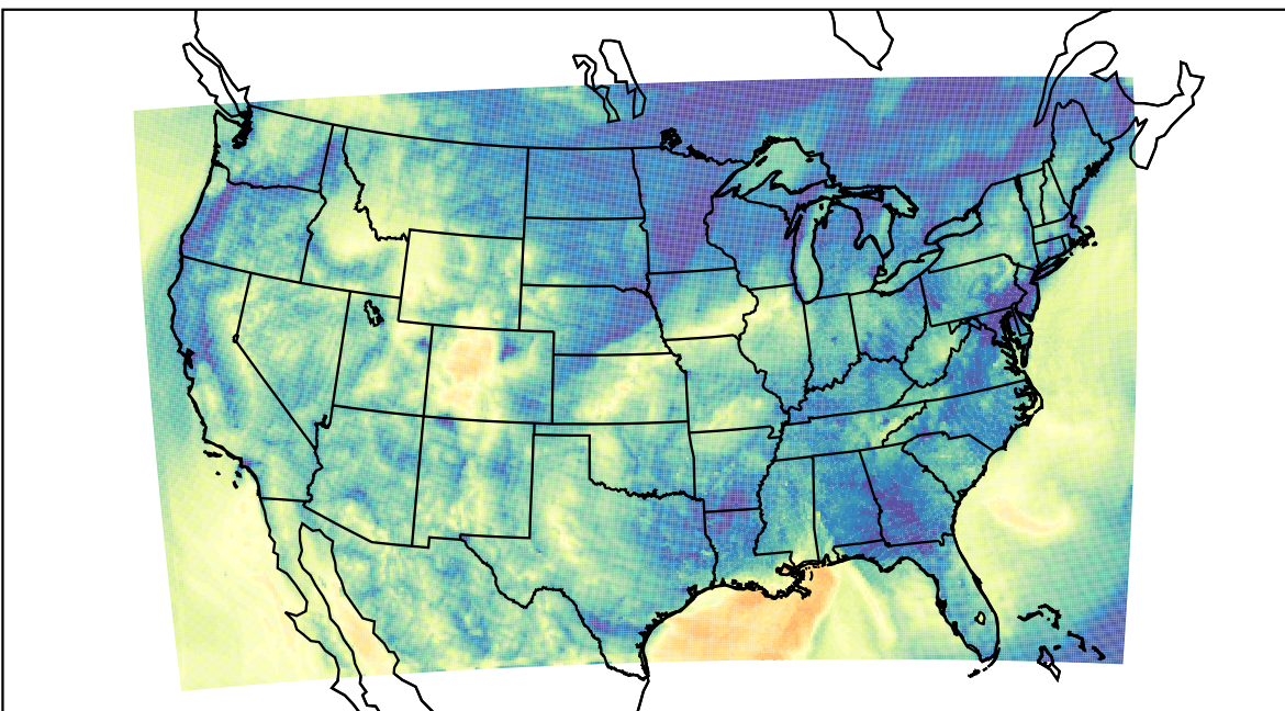
WRF (2022-10-30_10:00:00)
