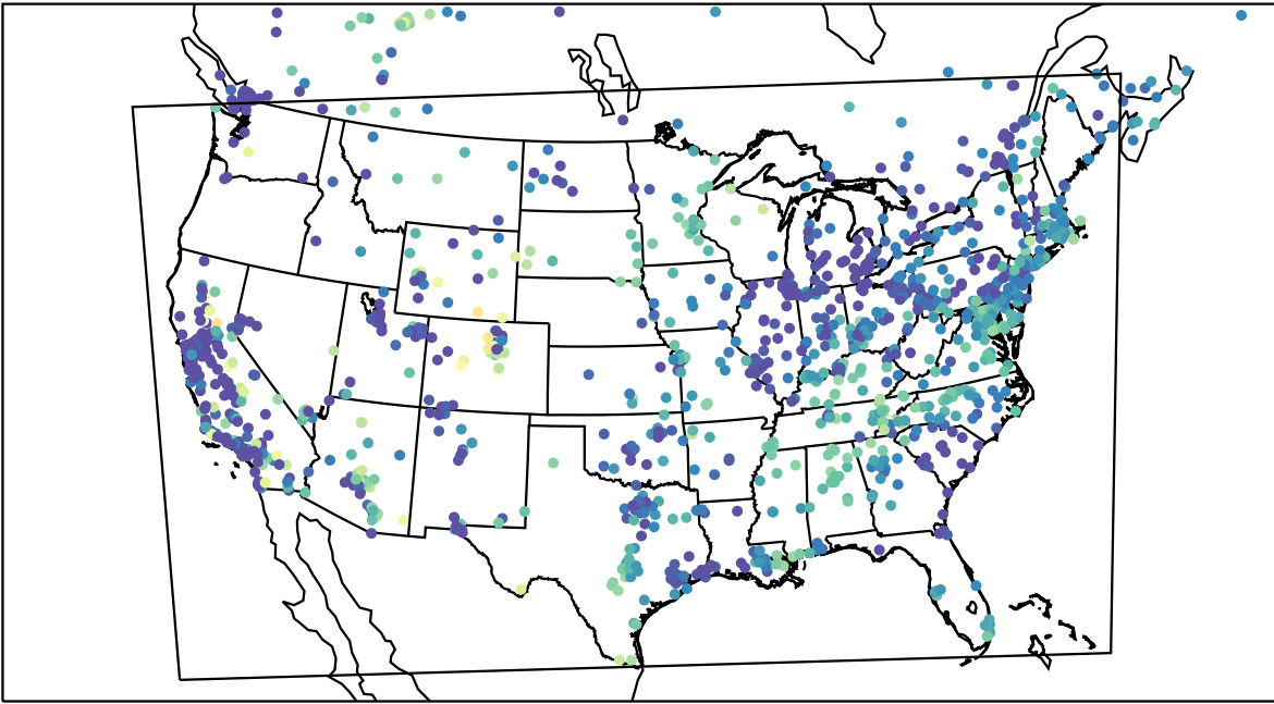
AirNOW (2022-10-29_15:00:00)
