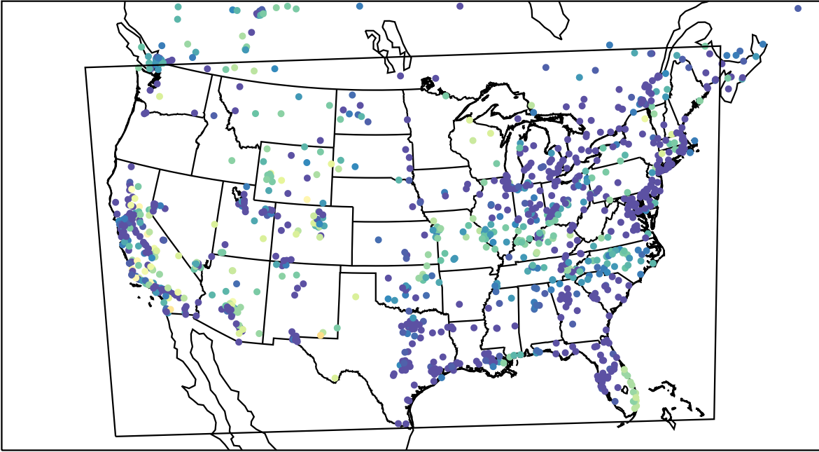
AirNOW (2022-10-30_06:00:00)
