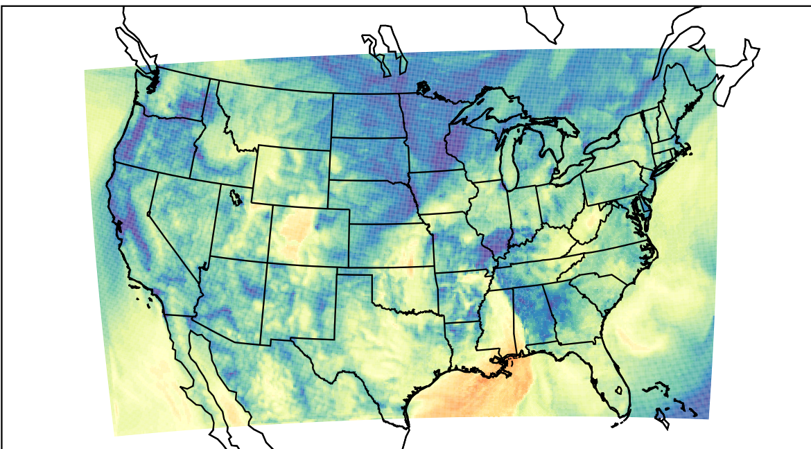
WRF (2022-10-30_16:00:00)
