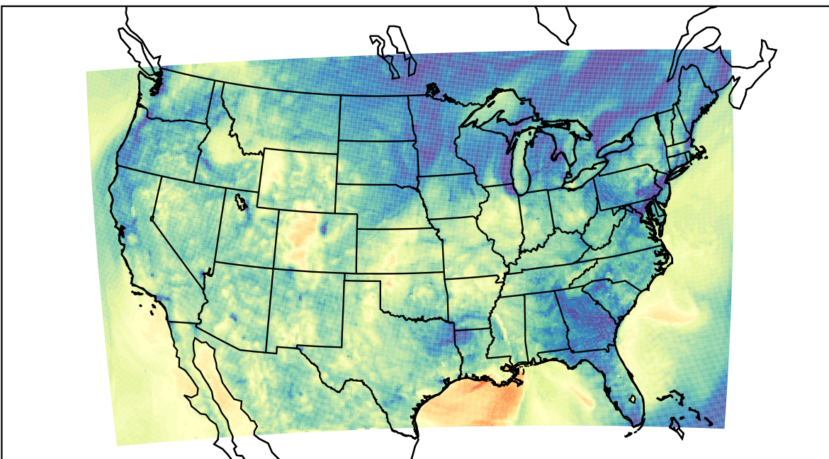
WRF (2022-10-30_04:00:00)
