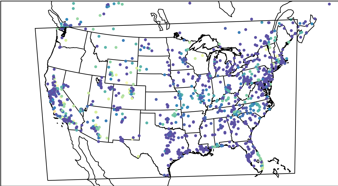
AirNOW (2022-10-30_10:00:00)
