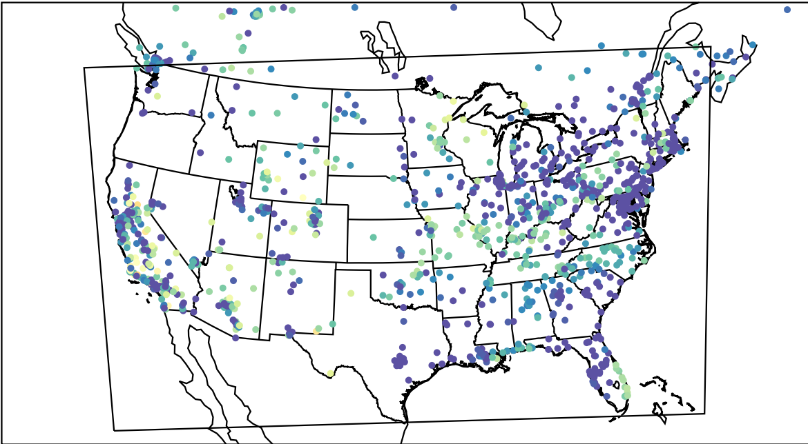
AirNOW (2022-10-30_04:00:00)
