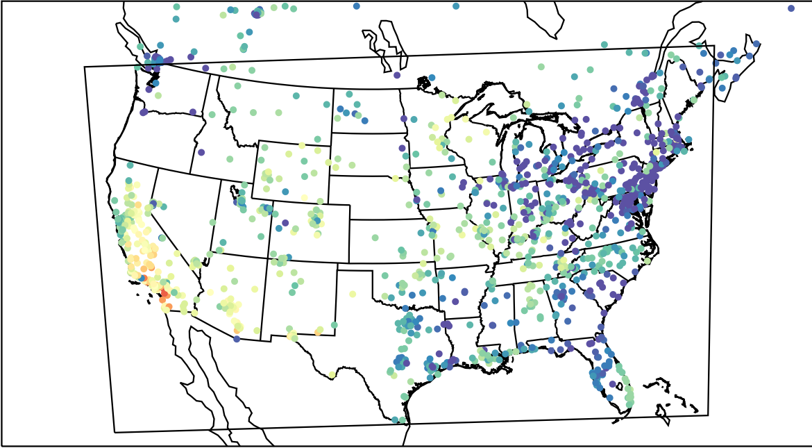
AirNOW (2022-10-30_00:00:00)
