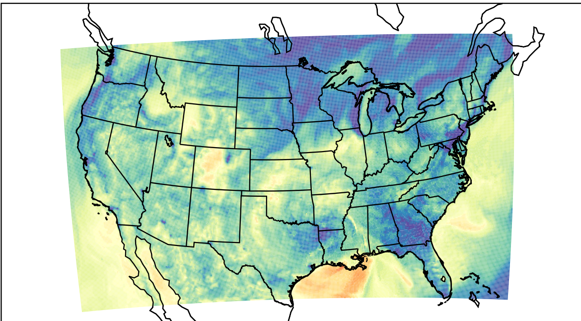
WRF (2022-10-30_06:00:00)
