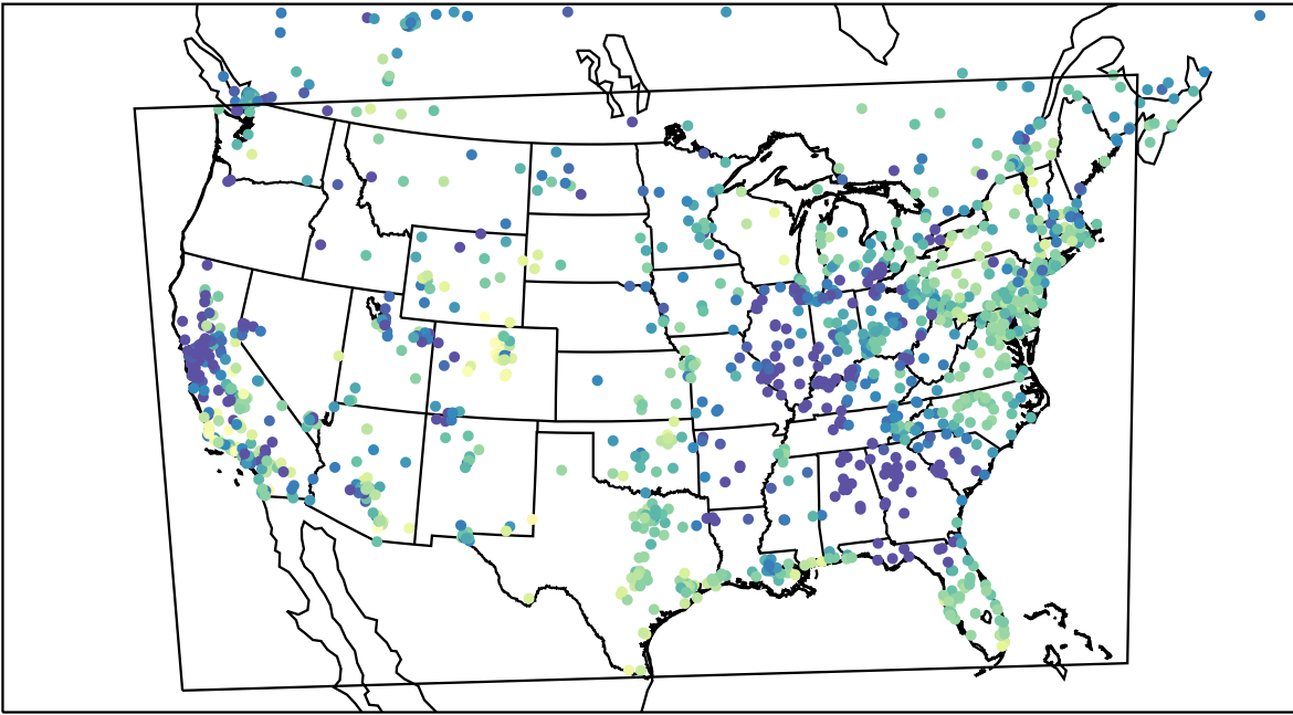
AirNOW (2022-10-30_16:00:00)
