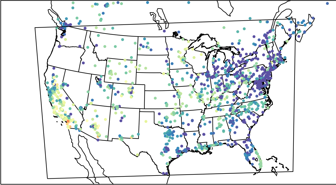
AirNOW (2022-10-30_01:00:00)
