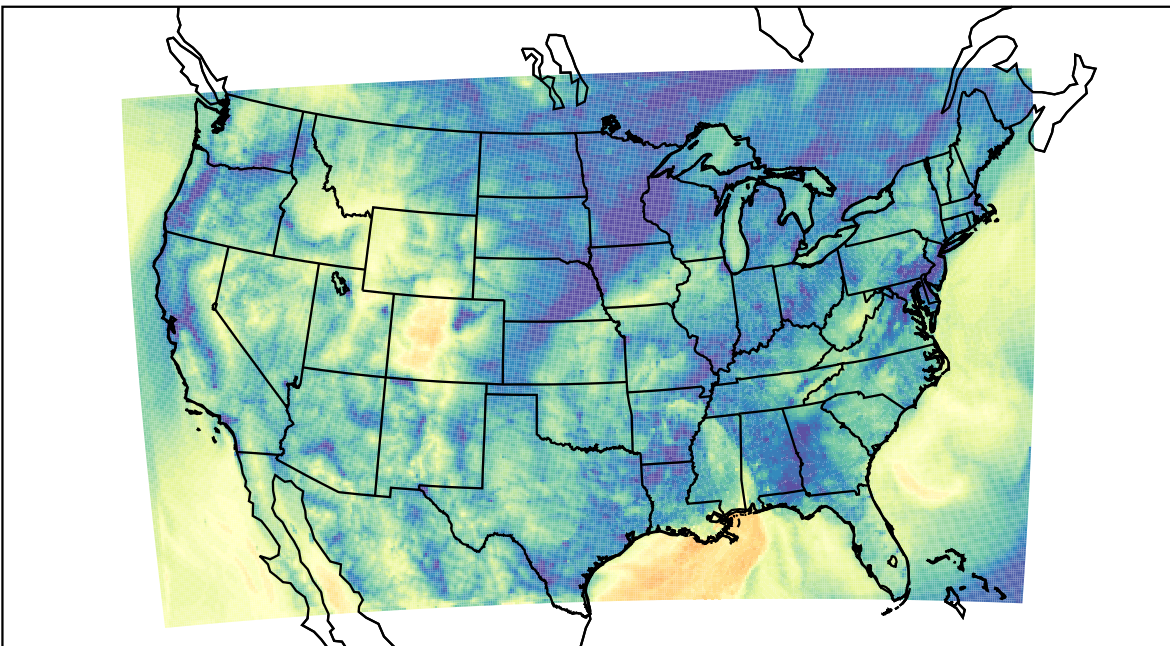
WRF (2022-10-30_14:00:00)
