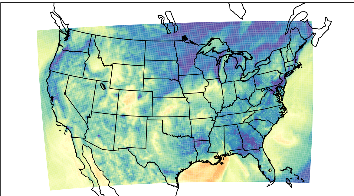
WRF (2022-10-30_08:00:00)
