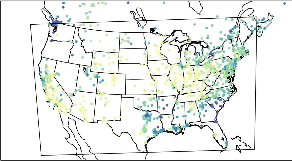
AirNOW (2022-10-29_19:00:00)
