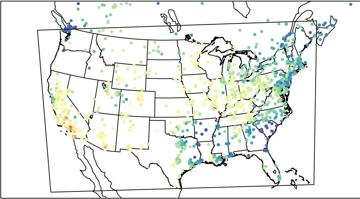
AirNOW (2022-10-29_21:00:00)
