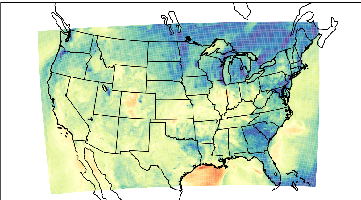
WRF (2022-10-30_00:00:00)
