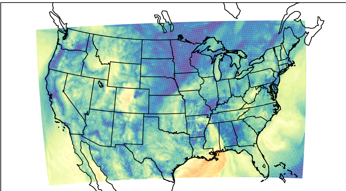
WRF (2022-10-30_15:00:00)
