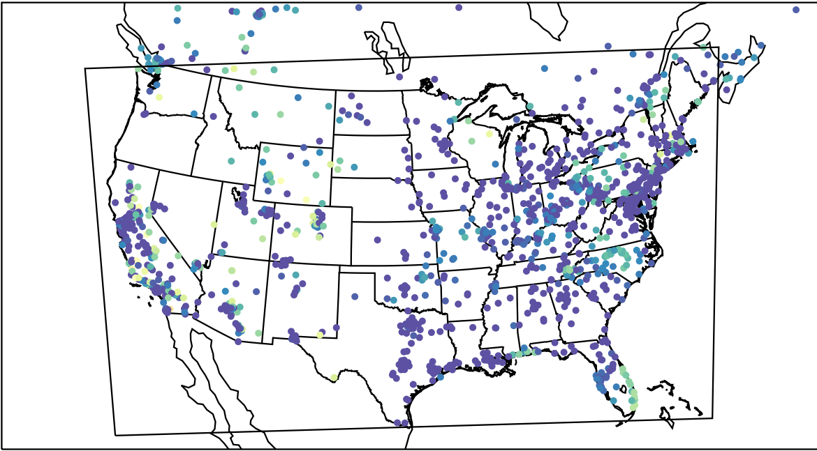
AirNOW (2022-10-30_13:00:00)
