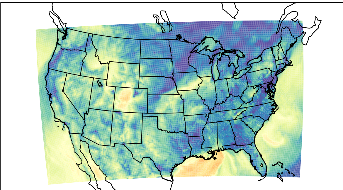
WRF (2022-10-30_12:00:00)
