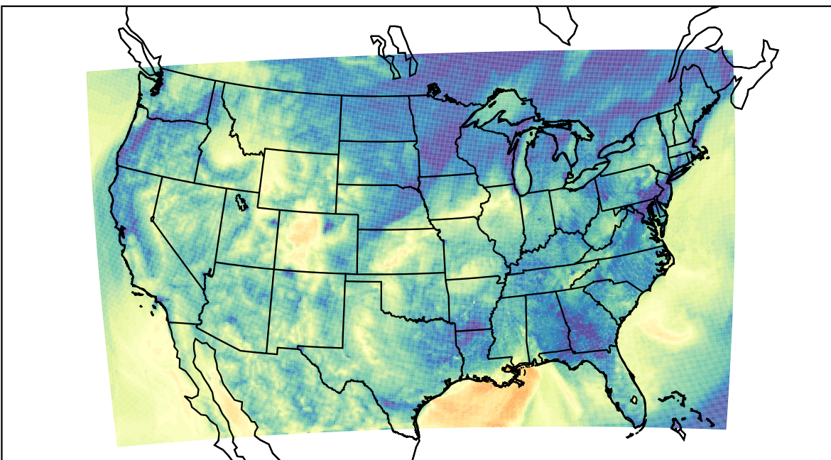
WRF (2022-10-30_09:00:00)
