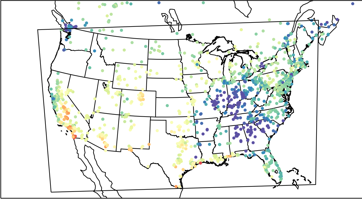
AirNOW (2022-10-30_21:00:00)
