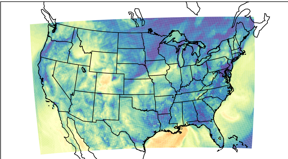
WRF (2022-10-30_11:00:00)
