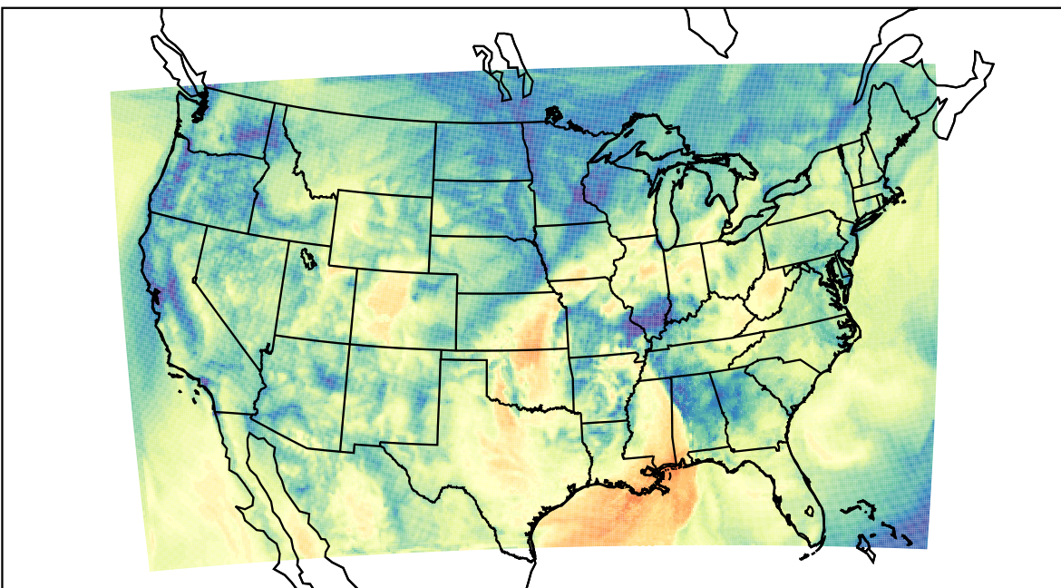
WRF (2022-10-30_17:00:00)
