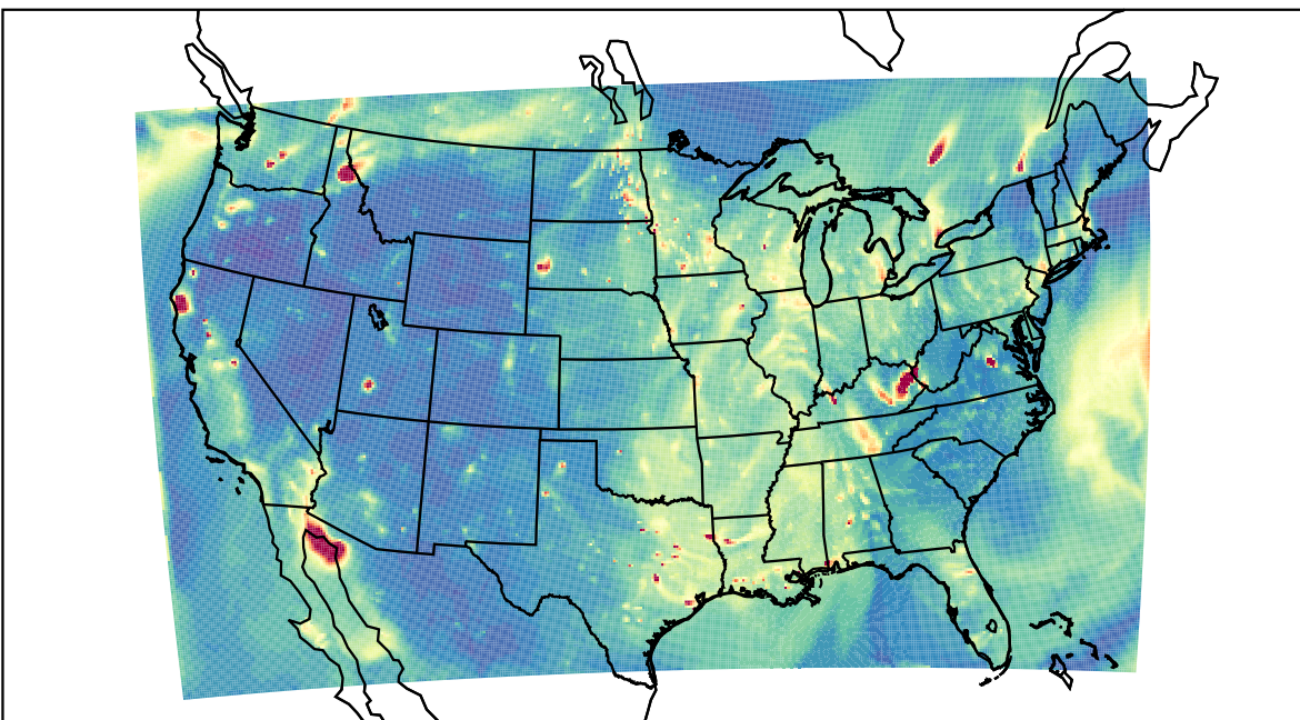
WRF 2022-10-31_02:00:00
