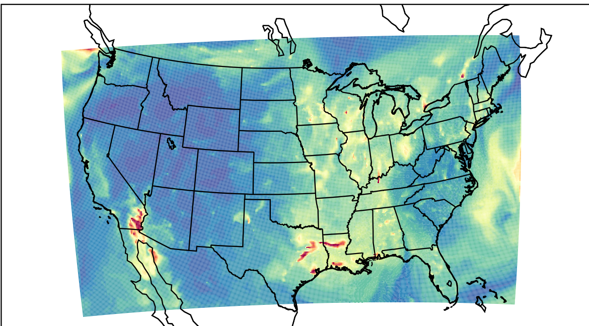
WRF 2022-10-31_12:00:00
