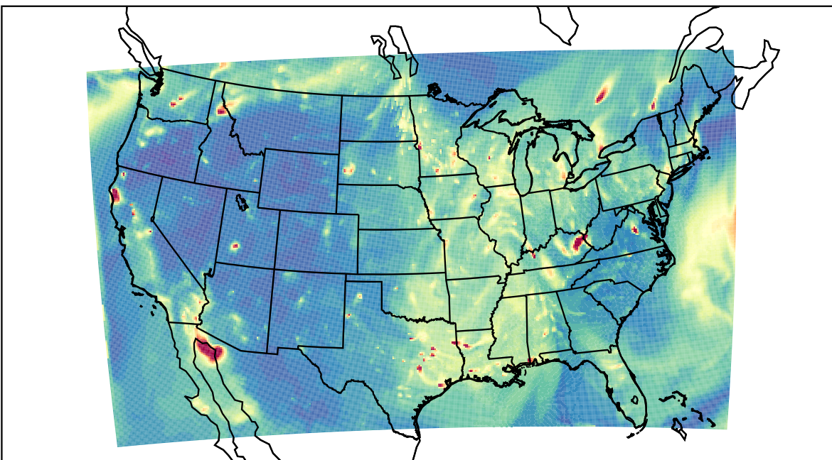
WRF 2022-10-31_03:00:00
