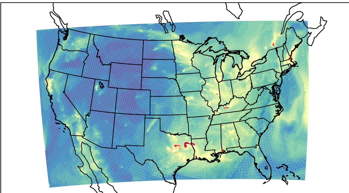
WRF 2022-11-01_09:00:00
