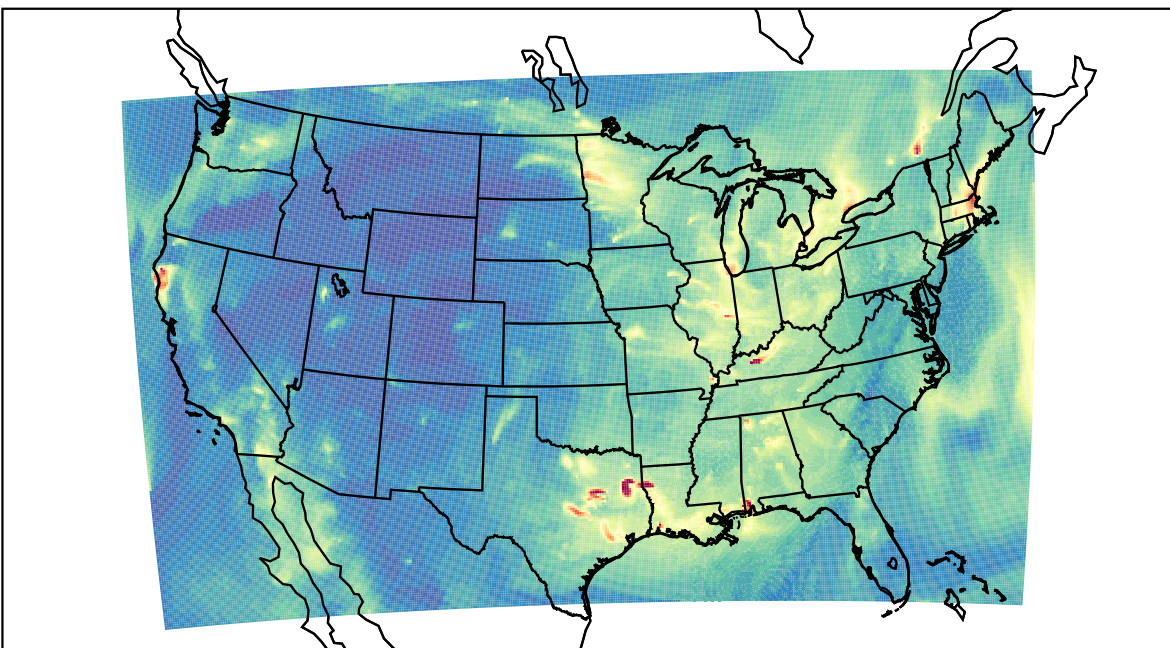
WRF 2022-11-01_07:00:00
