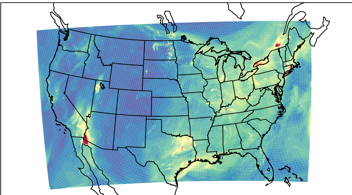
WRF 2022-11-01_21:00:00
