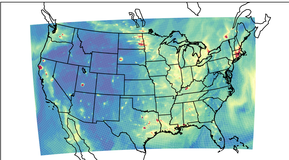
WRF 2022-11-01_02:00:00
