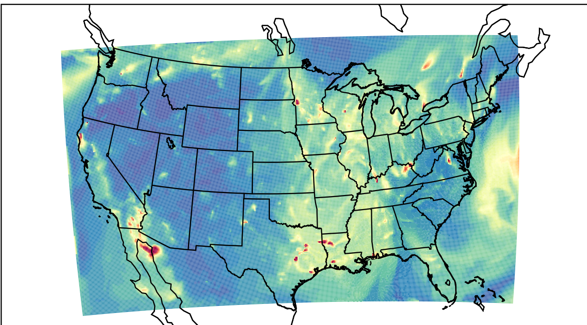
WRF 2022-10-31_05:00:00
