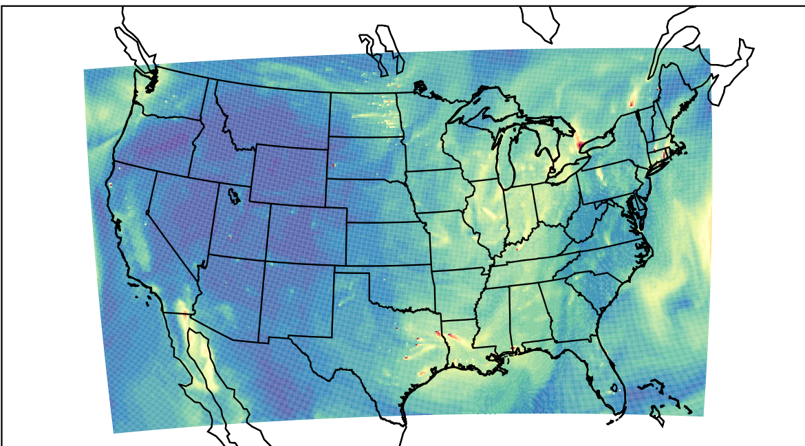
WRF 2022-10-31_20:00:00
