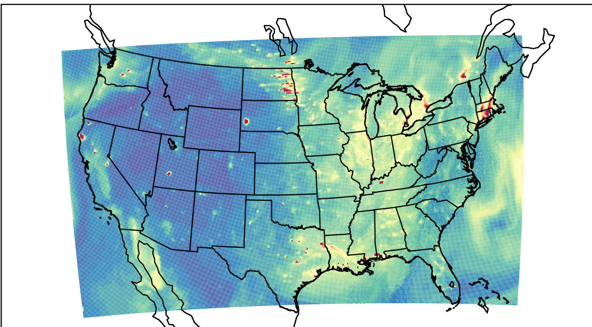
WRF 2022-11-01_00:00:00
