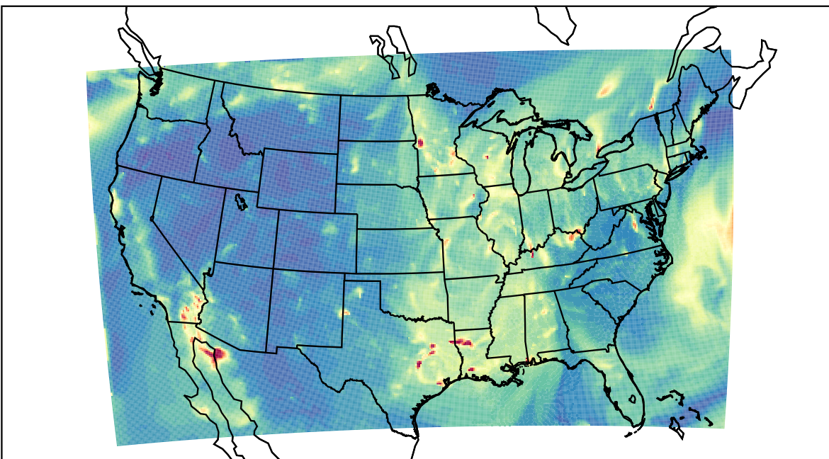
WRF 2022-10-31_06:00:00
