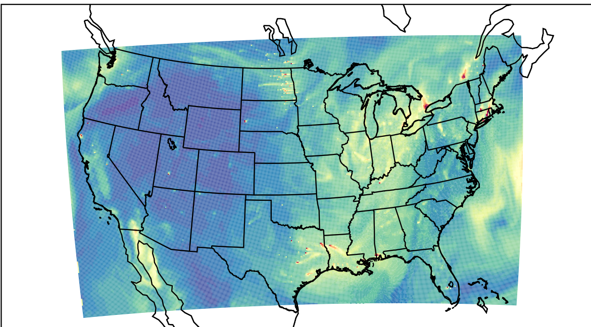
WRF 2022-10-31_21:00:00
