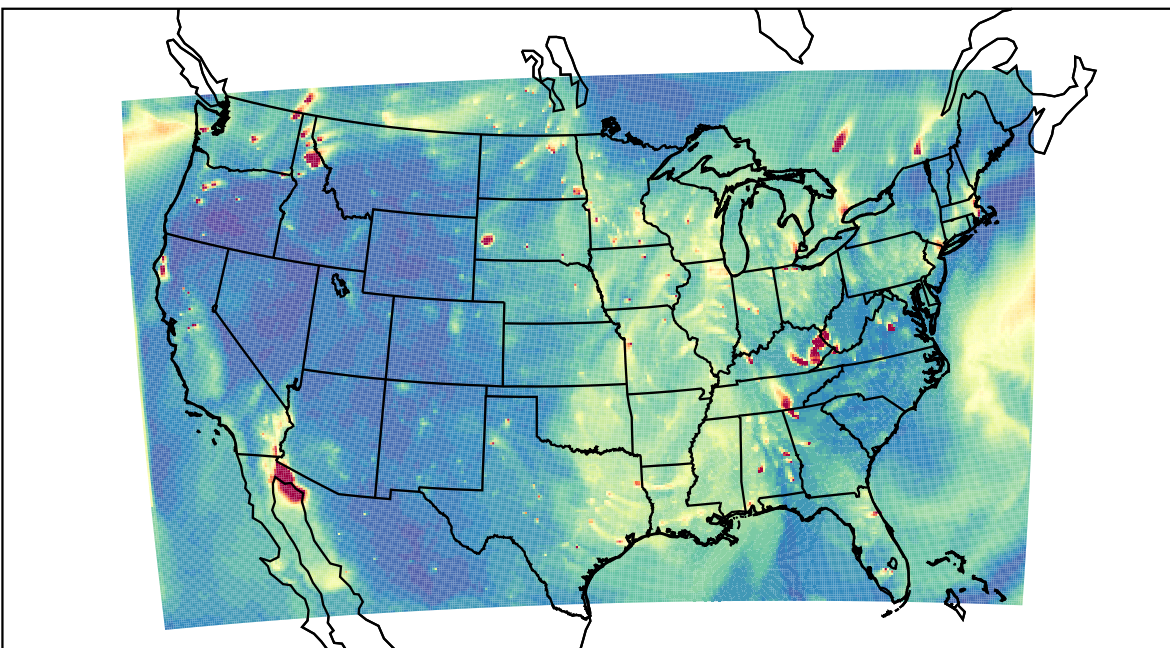
WRF 2022-10-31_00:00:00
