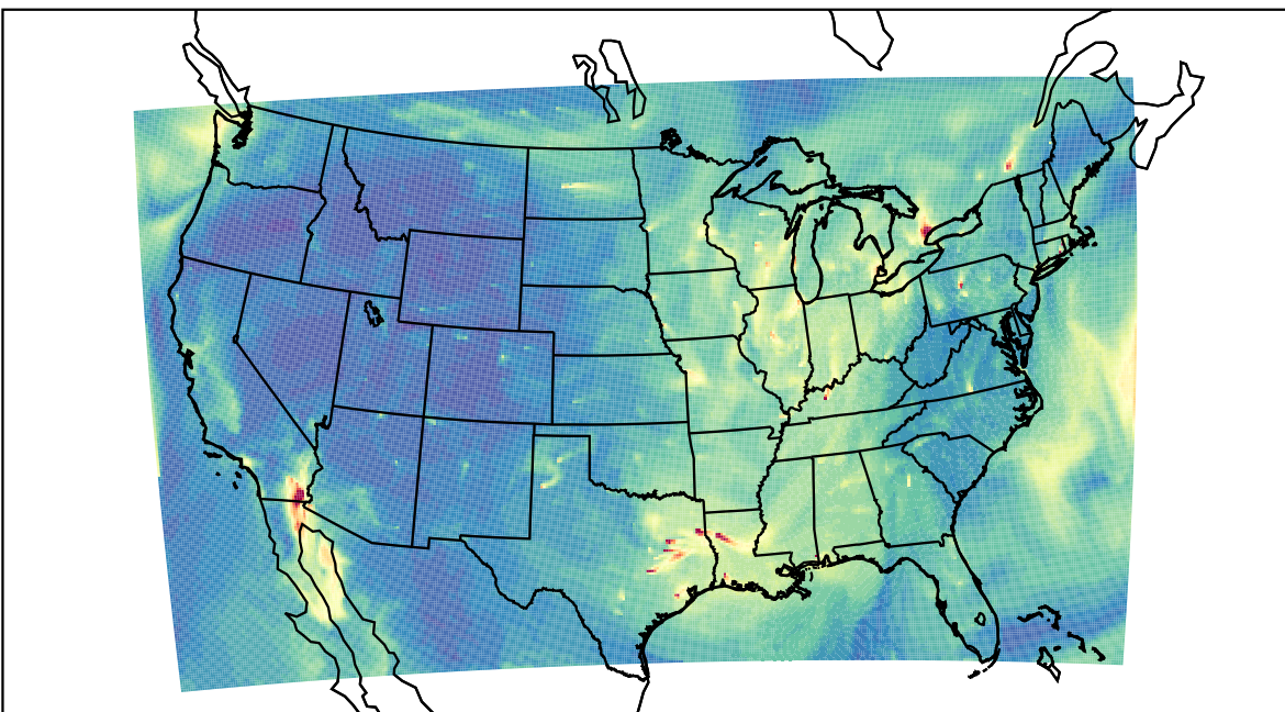
WRF 2022-10-31_17:00:00
