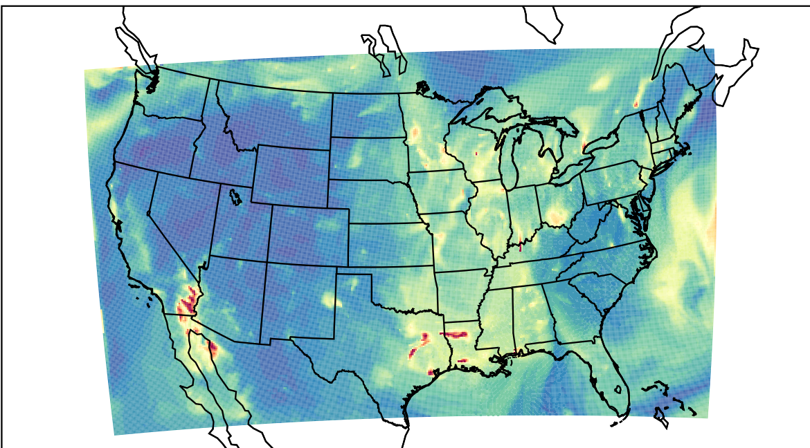
WRF 2022-10-31_09:00:00
