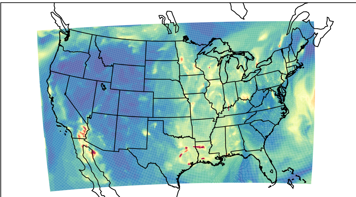
WRF 2022-10-31_08:00:00
