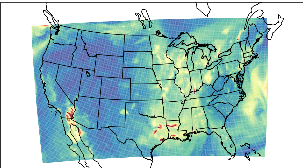
WRF 2022-10-31_11:00:00
