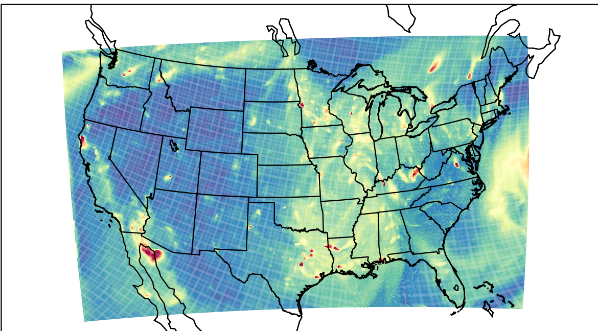
WRF 2022-10-31_04:00:00
