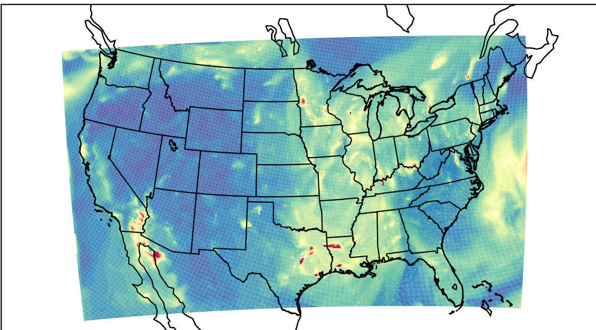
WRF 2022-10-31_07:00:00
