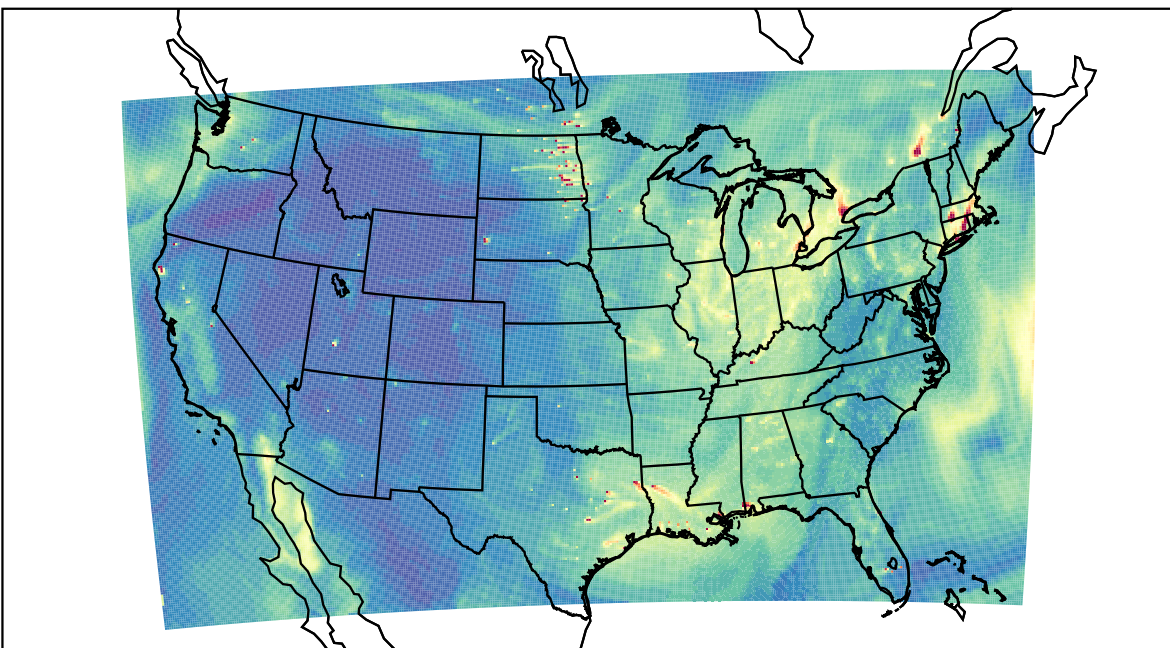
WRF 2022-10-31_22:00:00
