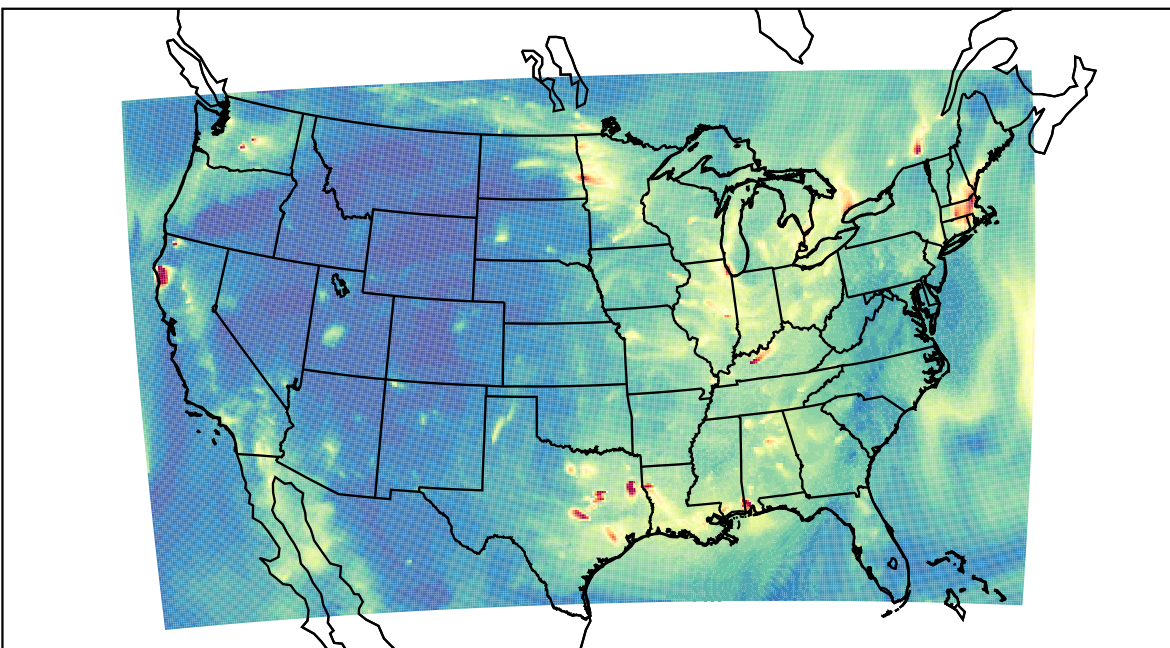
WRF 2022-11-01_05:00:00
