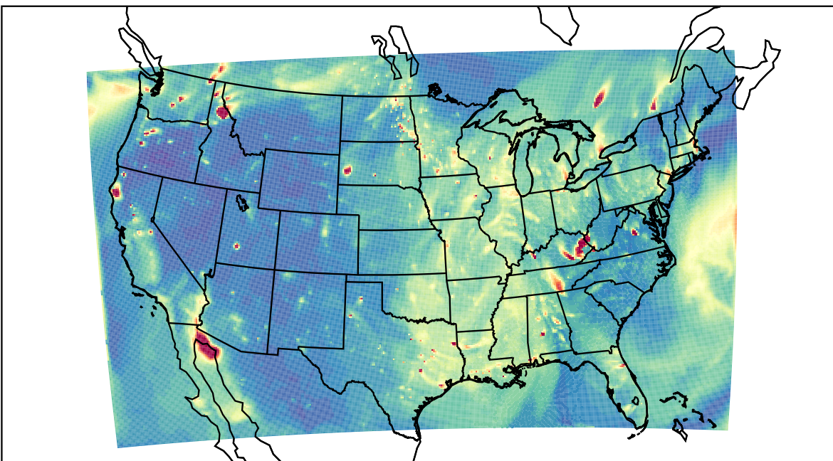
WRF 2022-10-31_01:00:00
