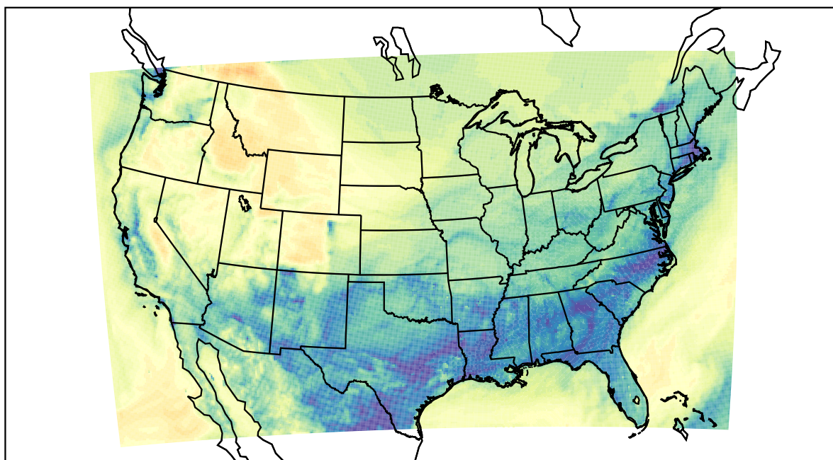
WRF (2022-11-19_07:00:00)
