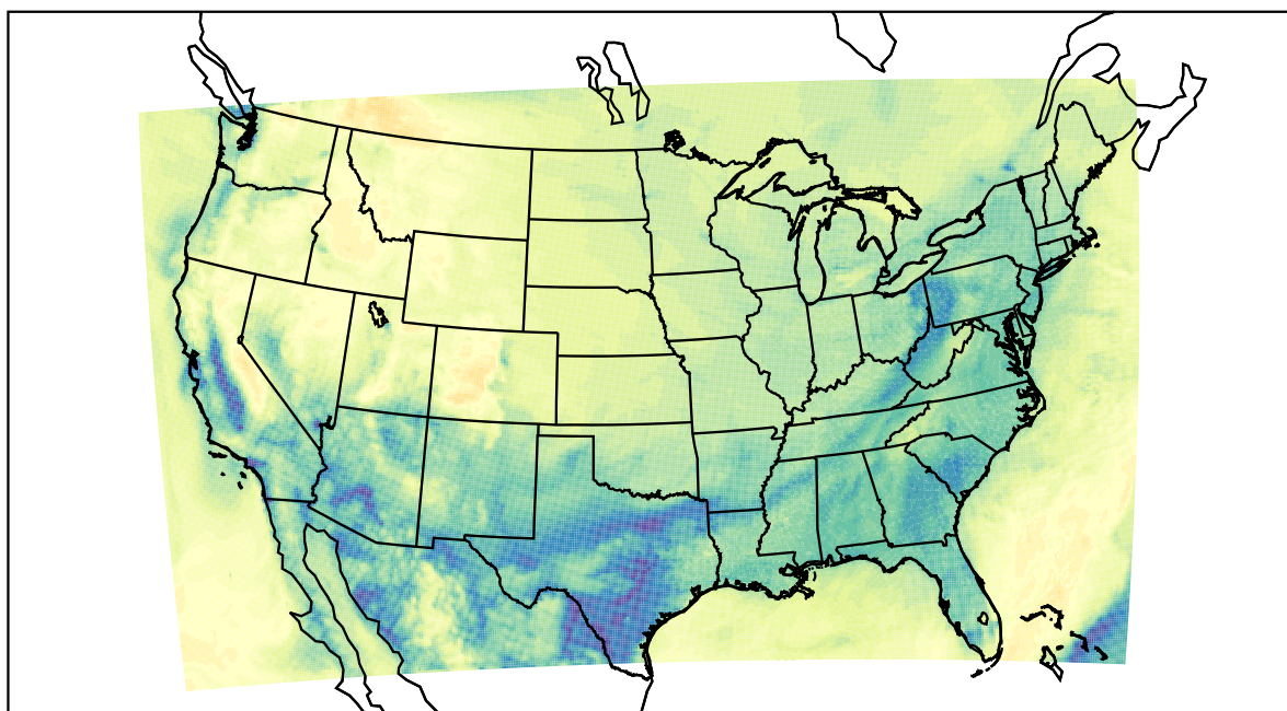
WRF (2022-11-18_16:00:00)
