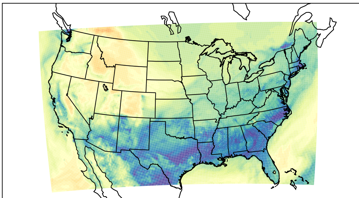
WRF (2022-11-19_09:00:00)
