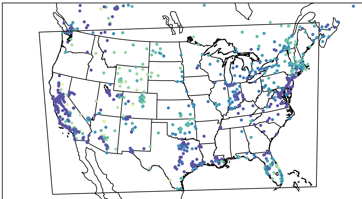
AirNOW (2022-11-18_06:00:00)
