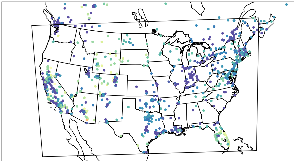
AirNOW (2022-11-19_02:00:00)
