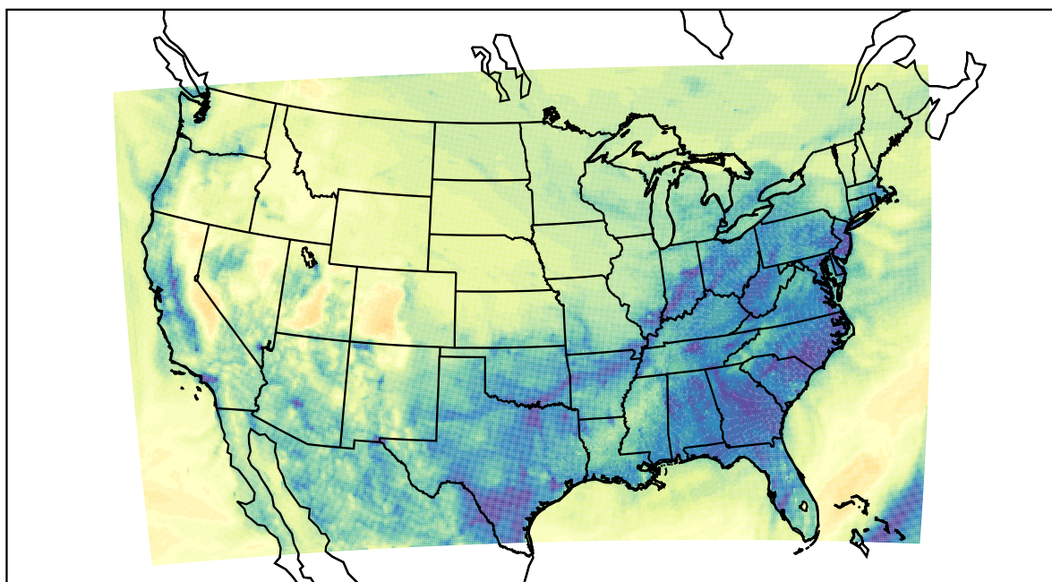
WRF (2022-11-18_07:00:00)
