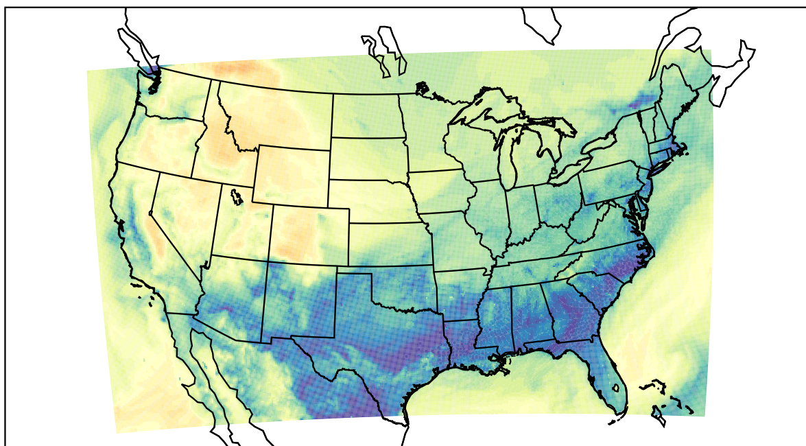
WRF (2022-11-19_11:00:00)
