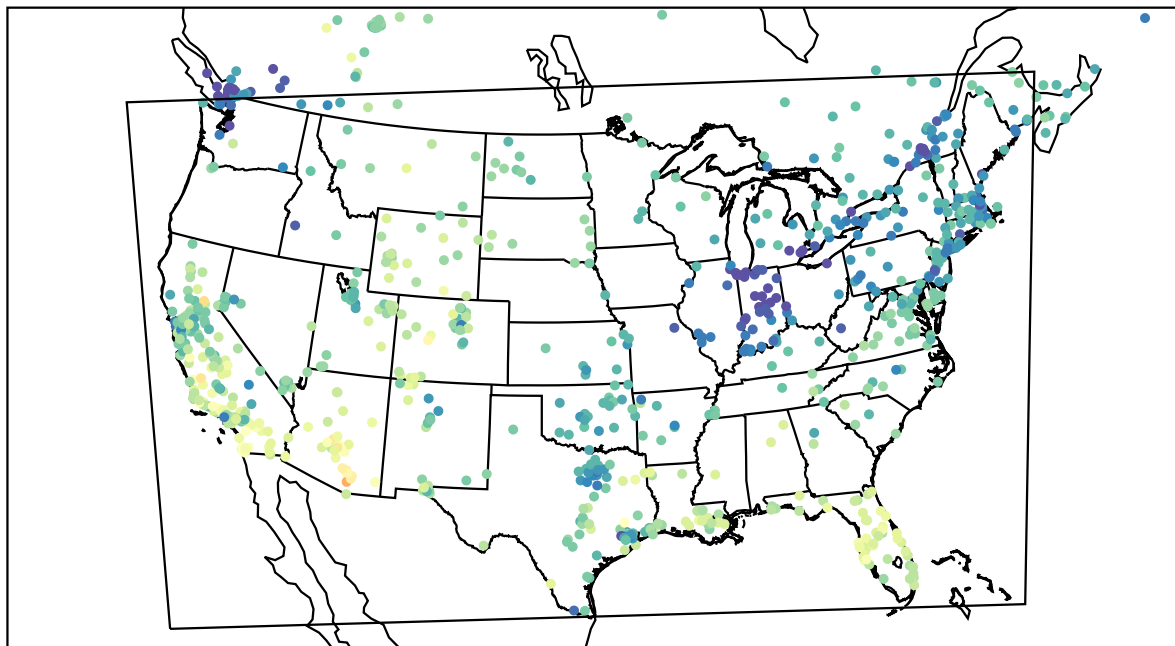
AirNOW (2022-11-18_21:00:00)
