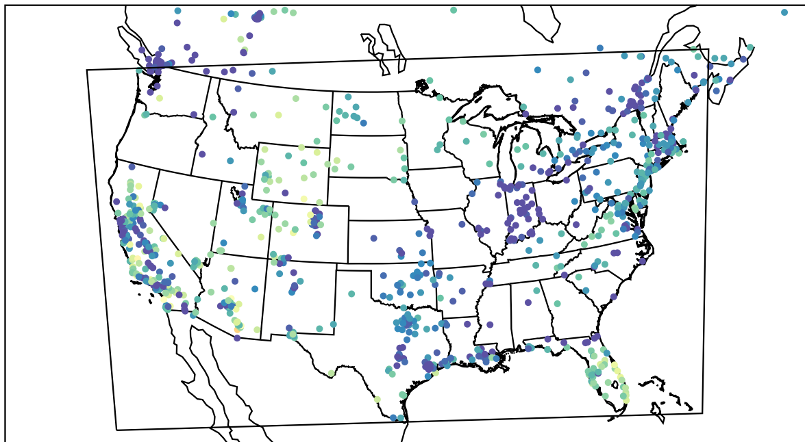
AirNOW (2022-11-19_01:00:00)
