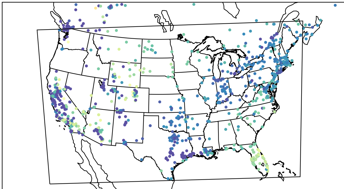
AirNOW (2022-11-19_15:00:00)
