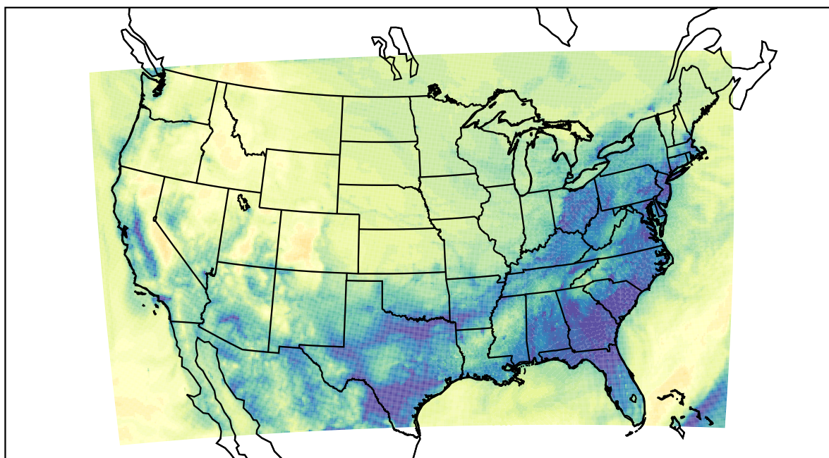
WRF (2022-11-18_12:00:00)
