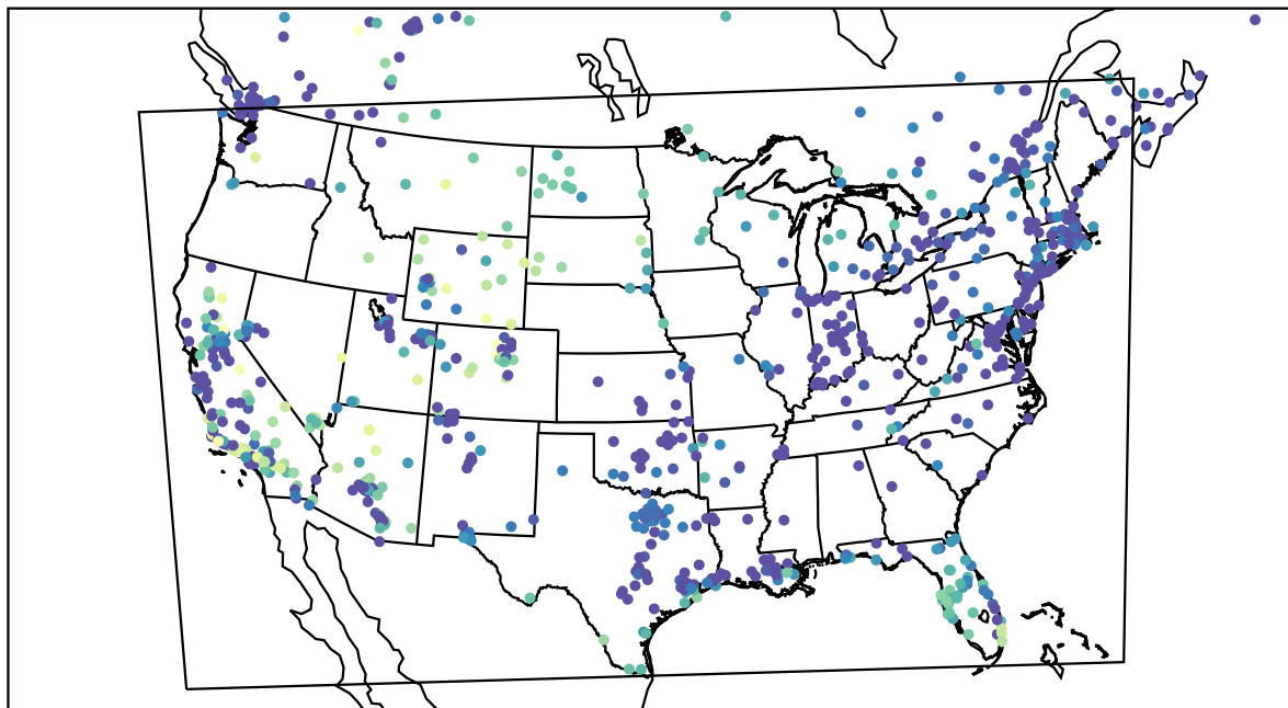
AirNOW (2022-11-19_11:00:00)
