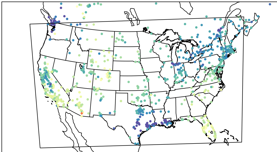
AirNOW (2022-11-19_19:00:00)
