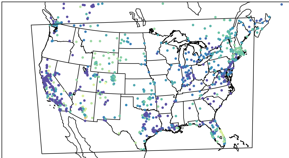
AirNOW (2022-11-18_02:00:00)
