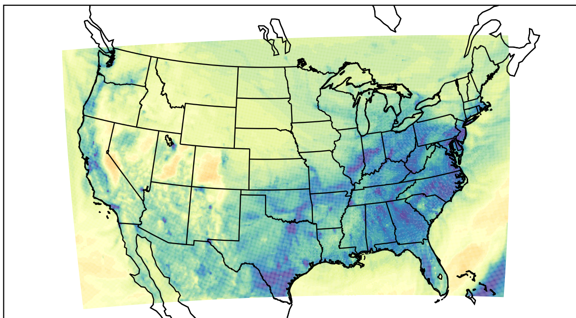
WRF (2022-11-18_04:00:00)
