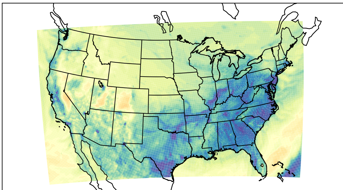
WRF (2022-11-18_05:00:00)
