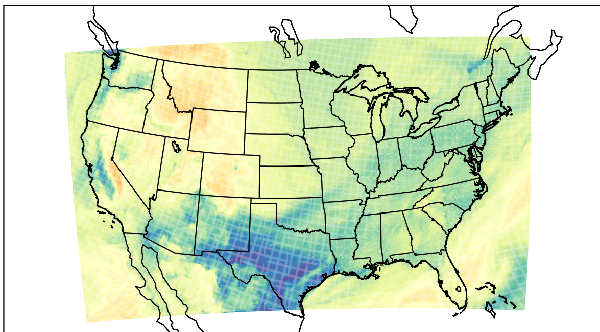
WRF (2022-11-19_18:00:00)
