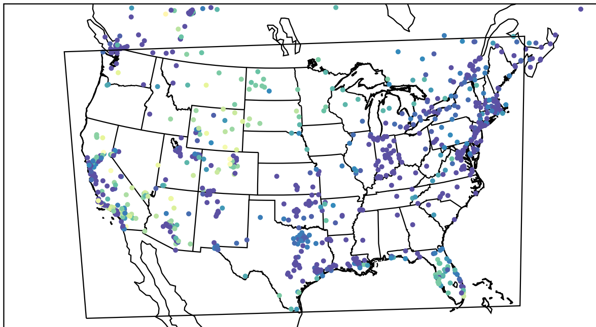
AirNOW (2022-11-19_12:00:00)
