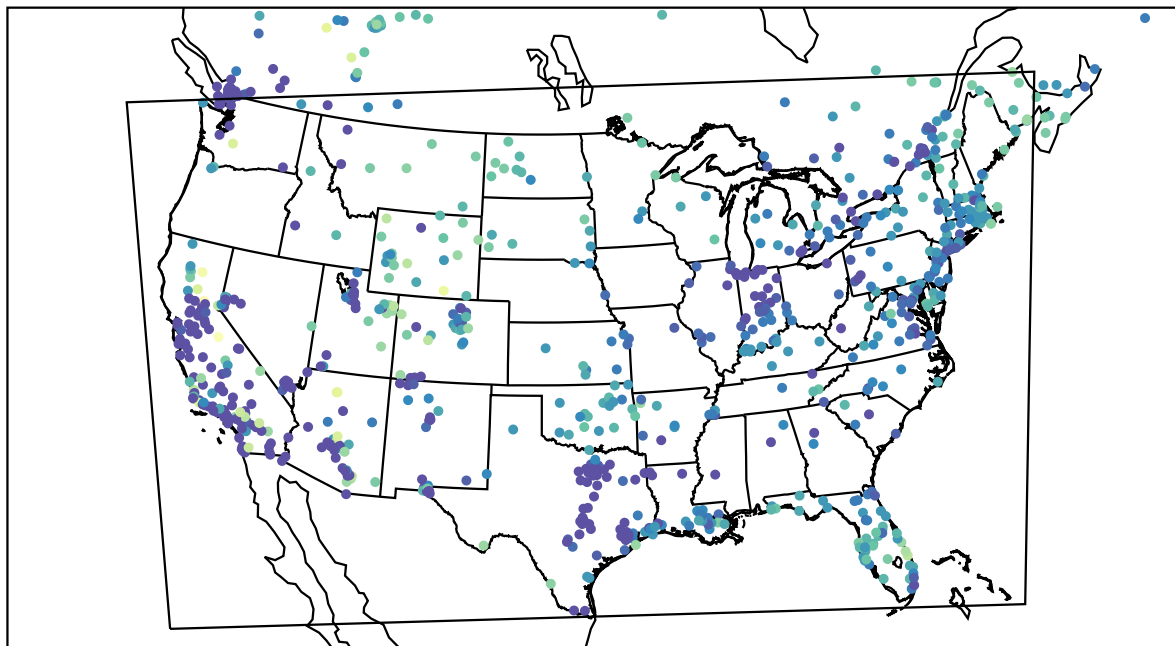
AirNOW (2022-11-18_14:00:00)
