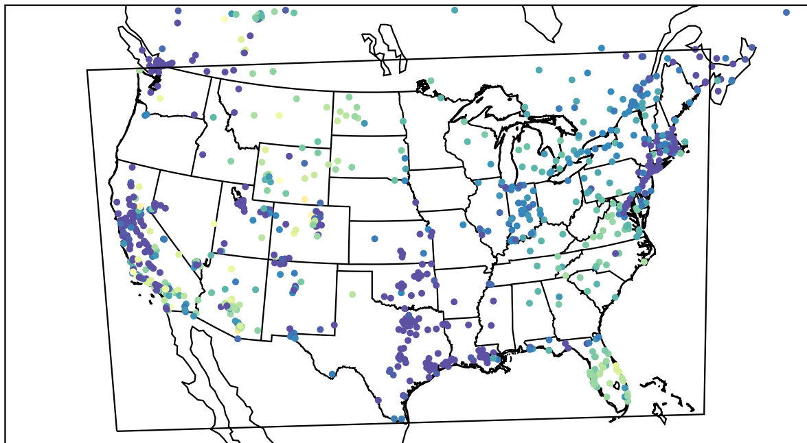
AirNOW (2022-11-20_06:00:00)
