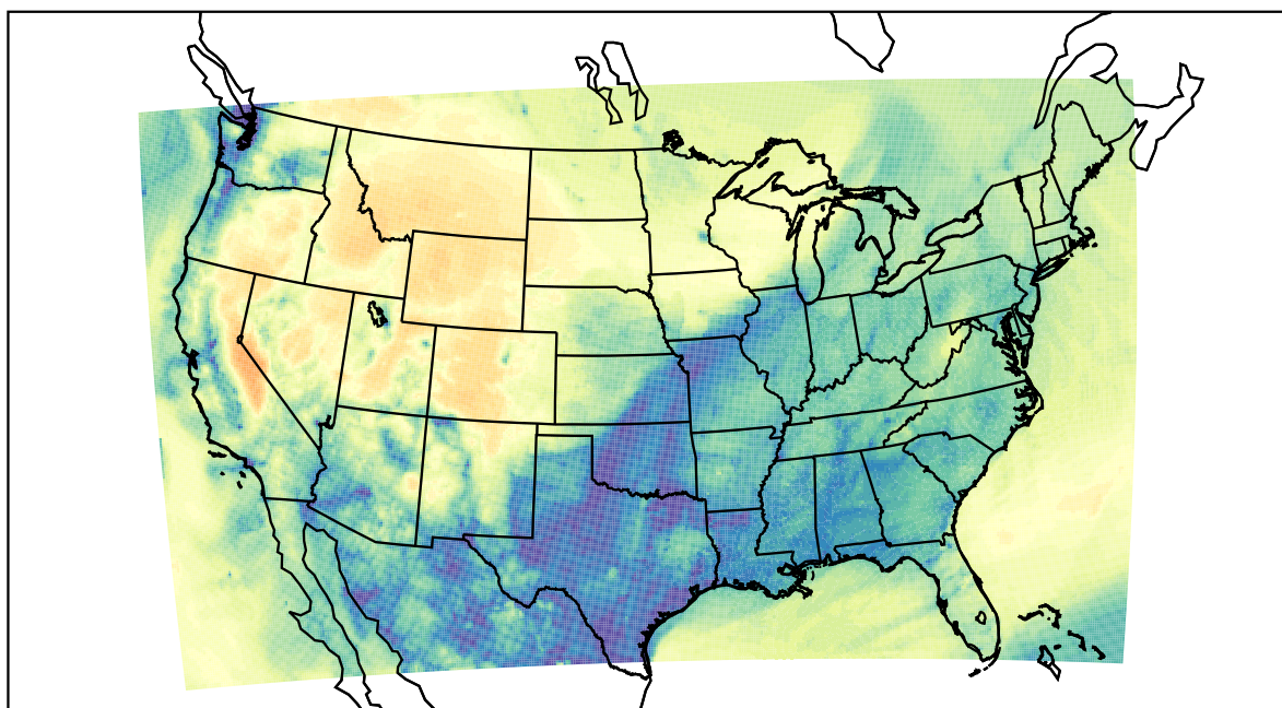
WRF (2022-11-21_15:00:00)
