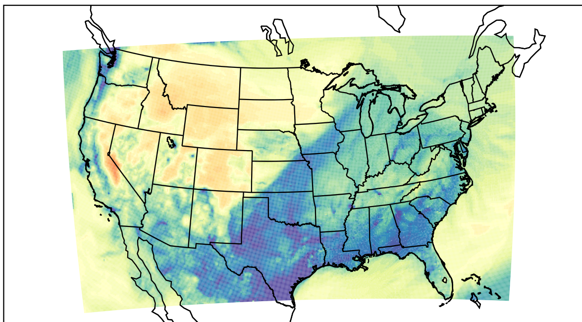
WRF (2022-11-21_07:00:00)
