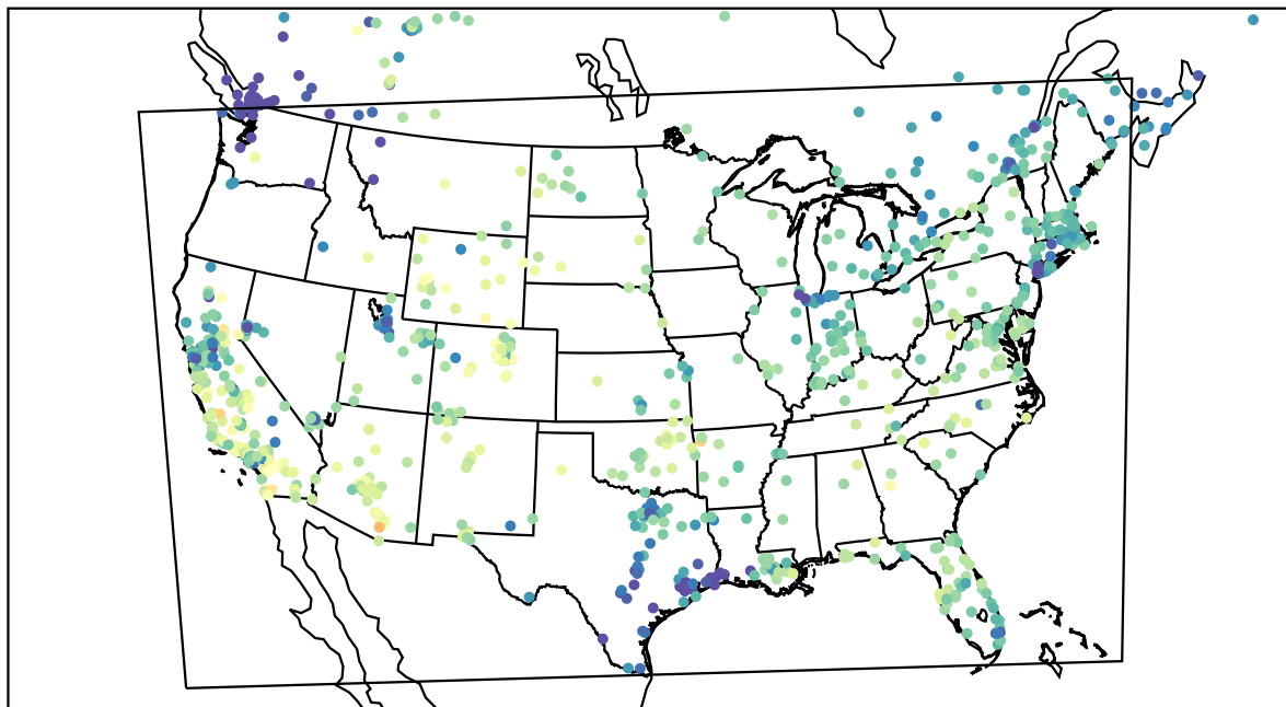
AirNOW (2022-11-21_20:00:00)
