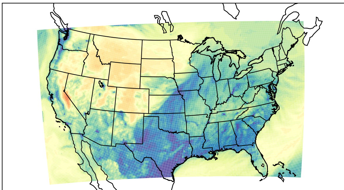
WRF (2022-11-21_04:00:00)
