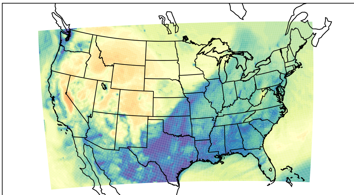
WRF (2022-11-21_14:00:00)
