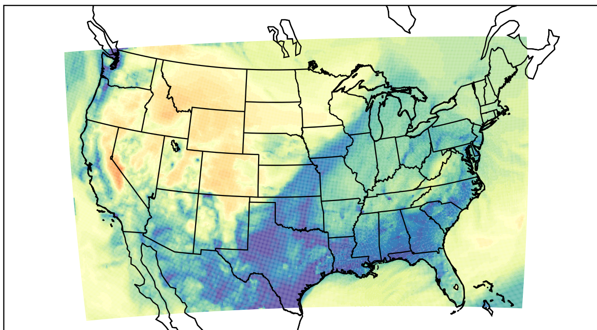
WRF (2022-11-21_10:00:00)
