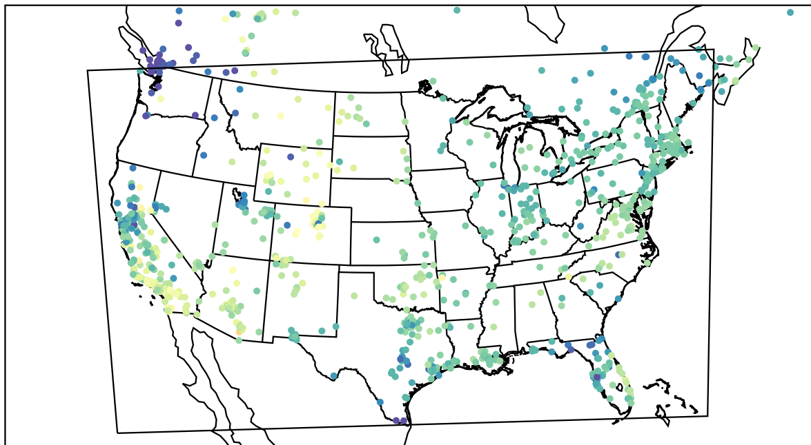
AirNOW (2022-11-20_19:00:00)
