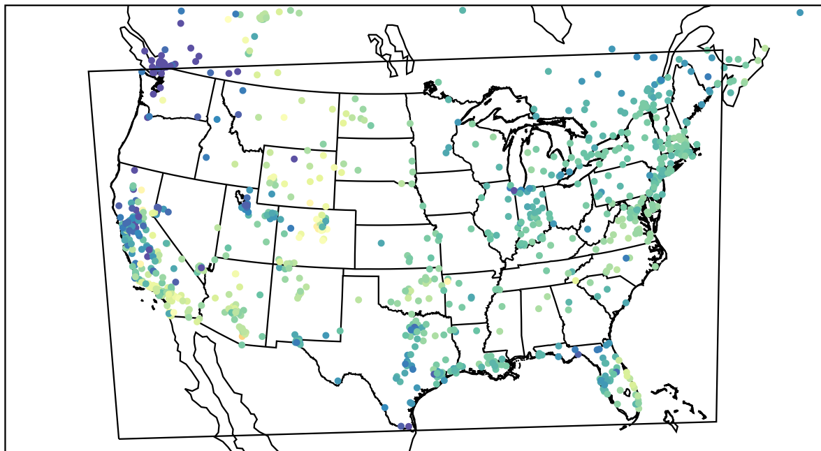
AirNOW (2022-11-20_18:00:00)
