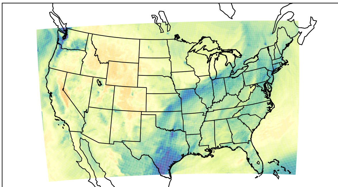
WRF (2022-11-21_20:00:00)
