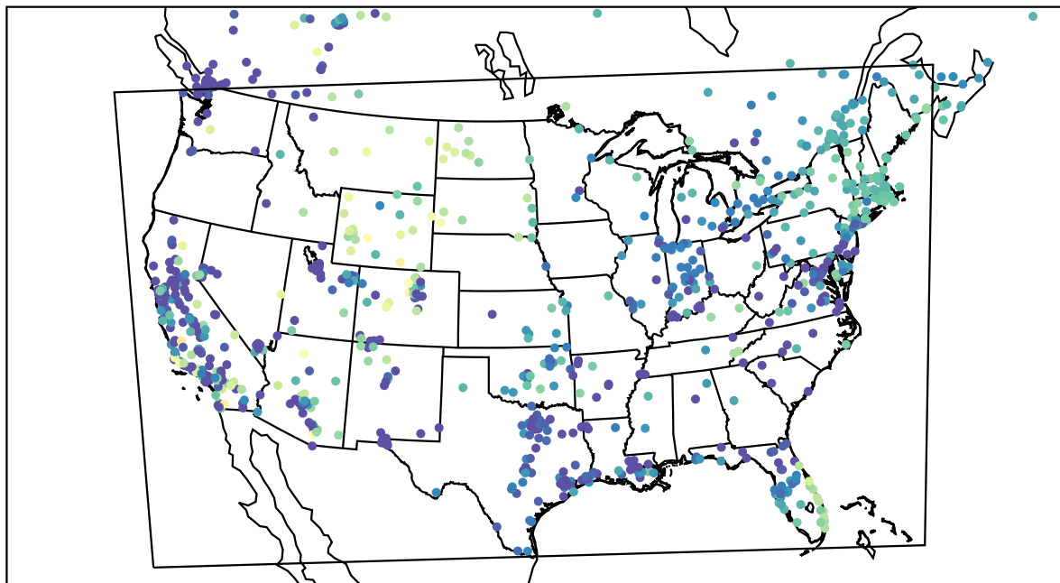
AirNOW (2022-11-21_03:00:00)
