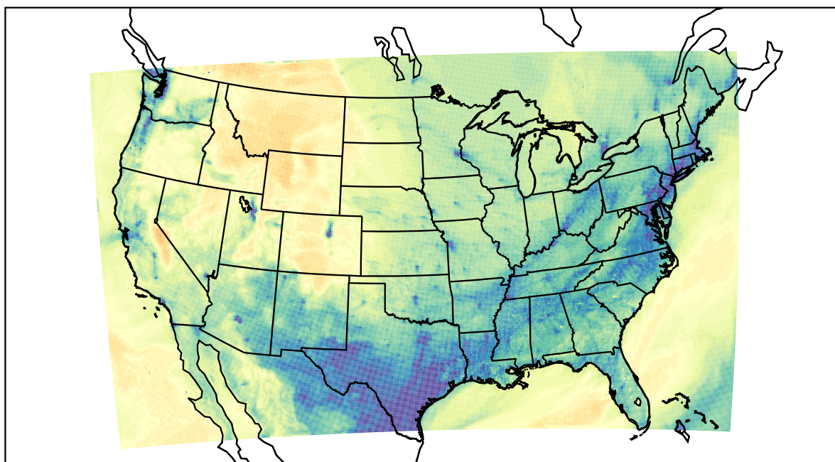
WRF (2022-11-20_01:00:00)
