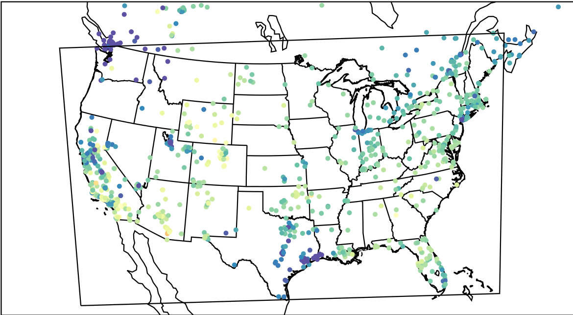
AirNOW (2022-11-21_19:00:00)
