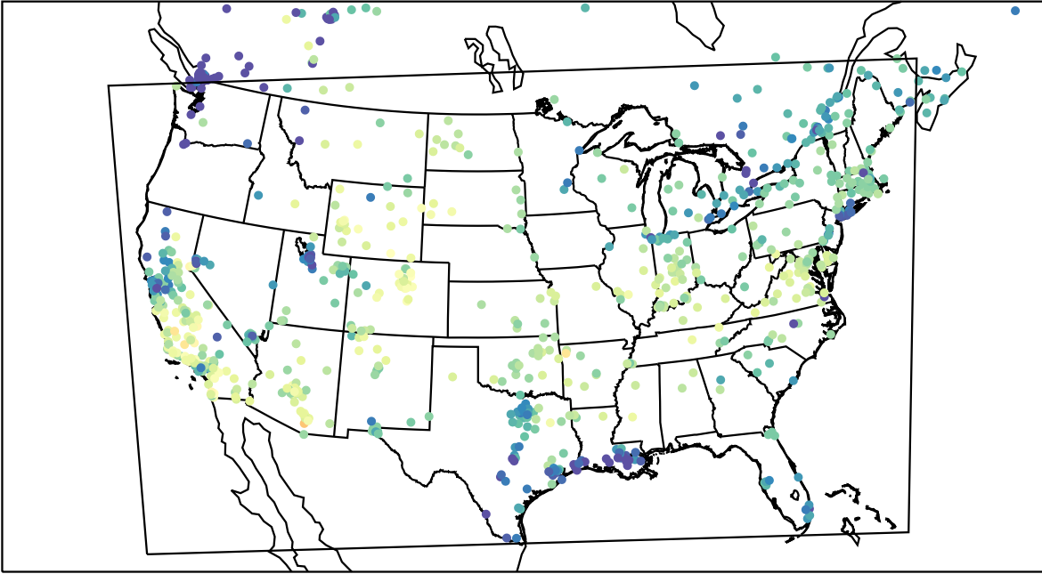
AirNOW (2022-11-22_20:00:00)
