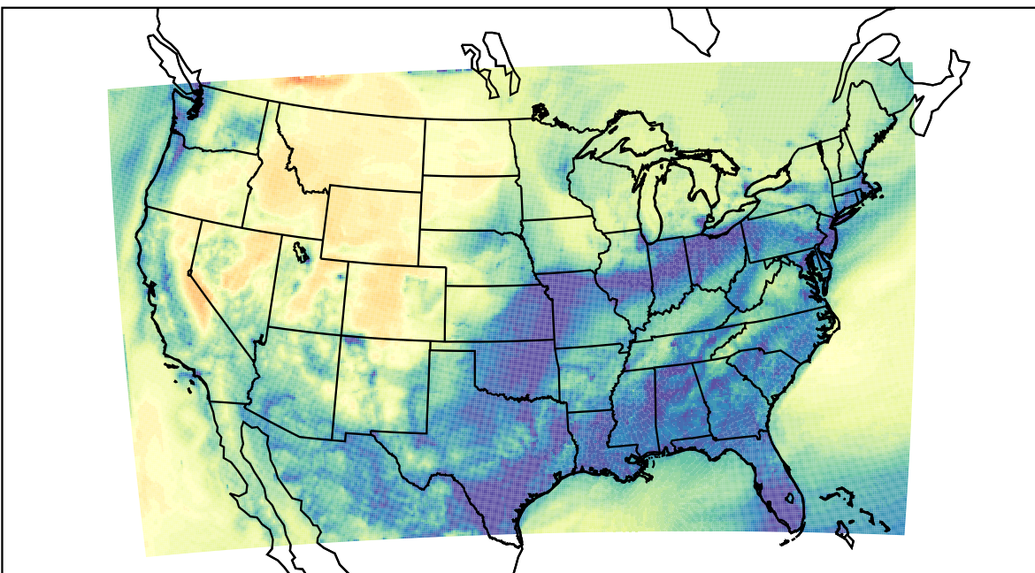
WRF (2022-11-22_12:00:00)
