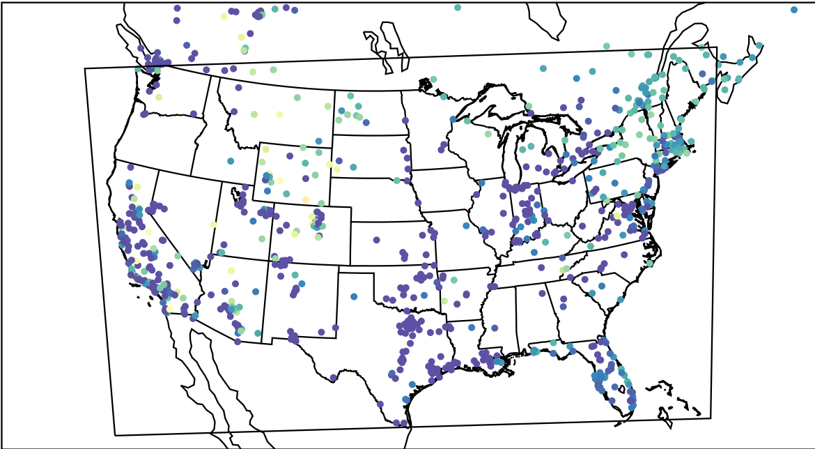
AirNOW (2022-11-22_14:00:00)
