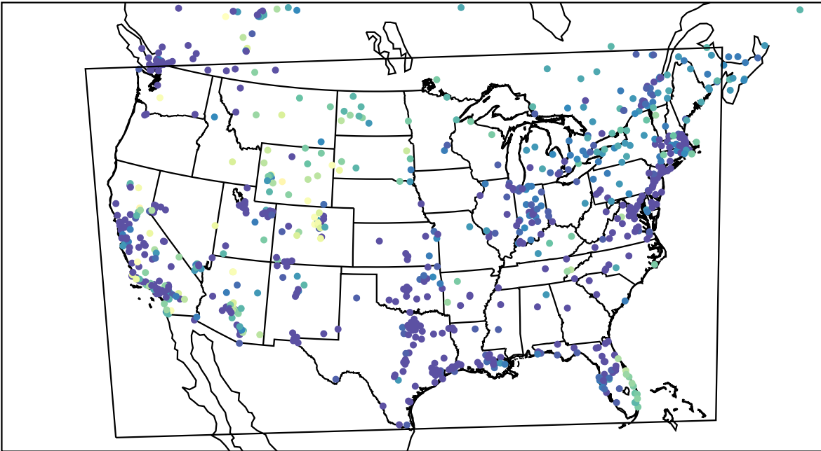
AirNOW (2022-11-21_12:00:00)
