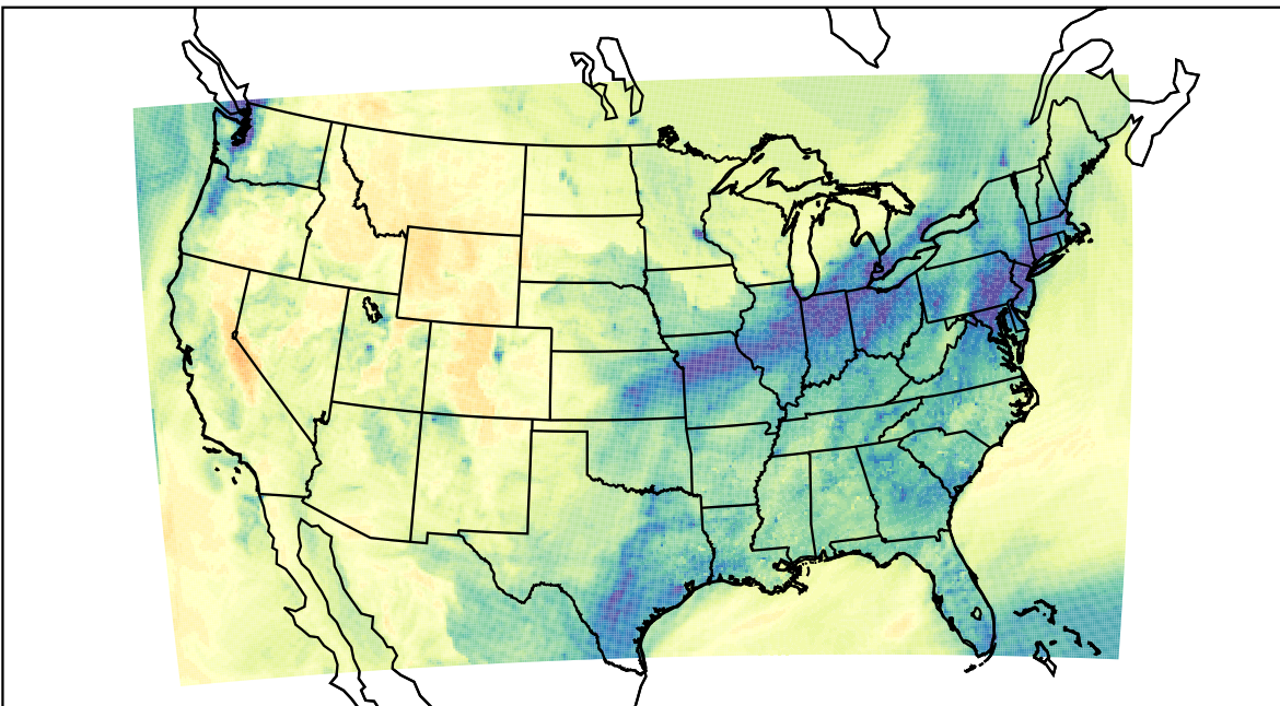
WRF (2022-11-21_22:00:00)
