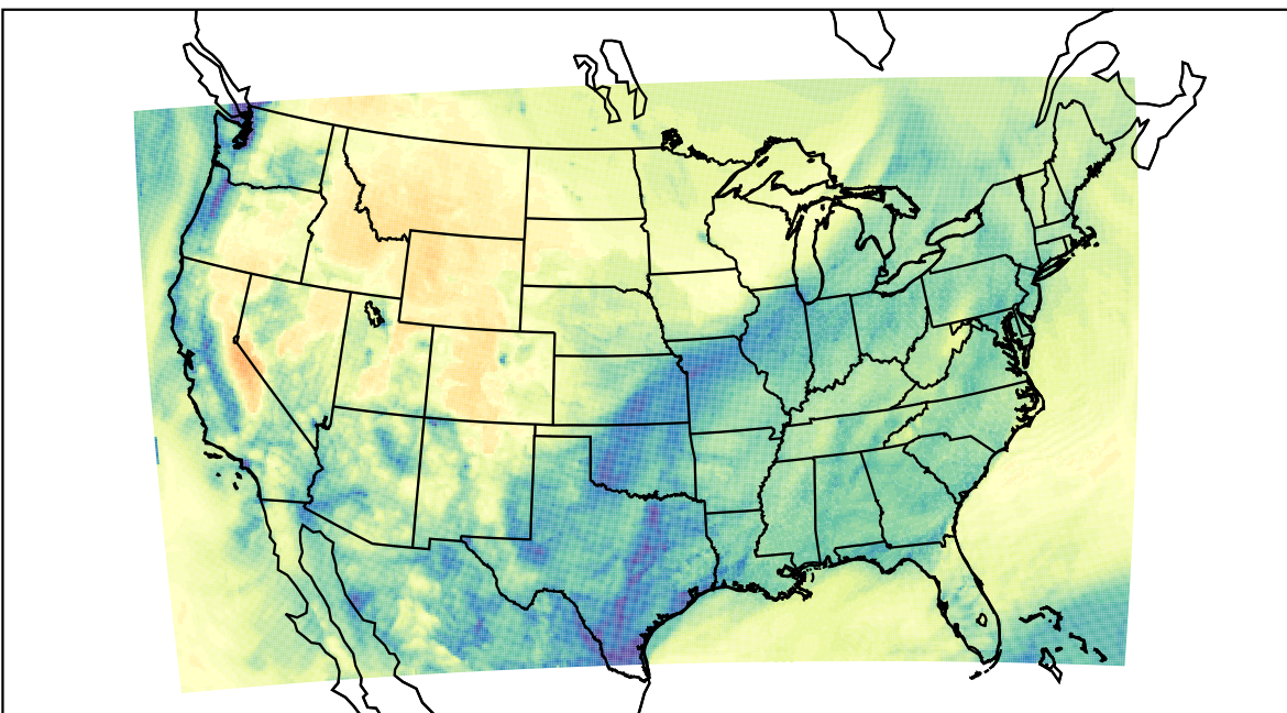
WRF (2022-11-21_17:00:00)
