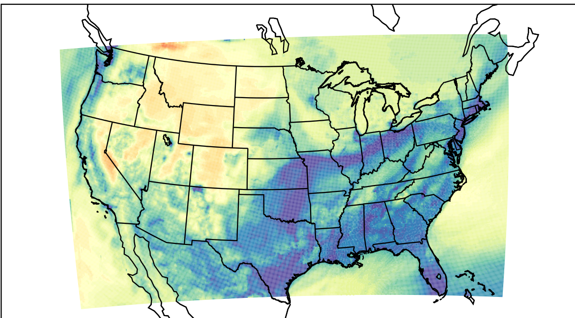
WRF (2022-11-22_09:00:00)
