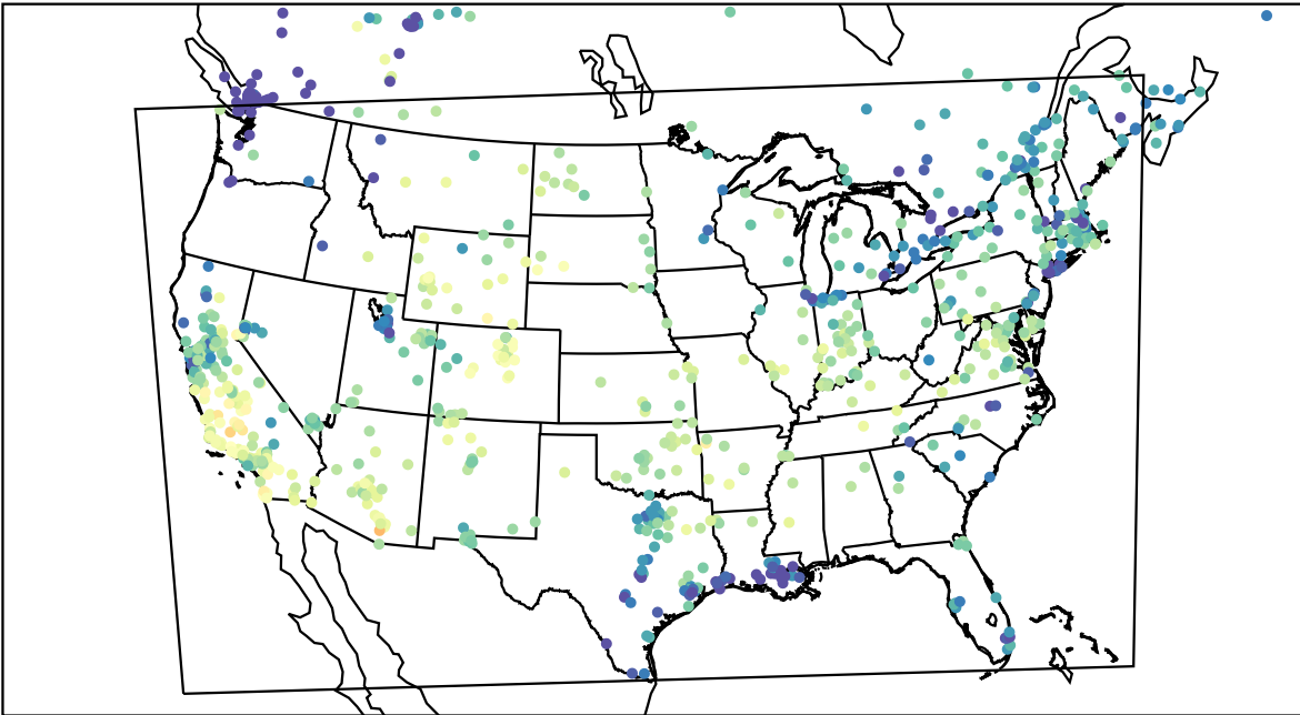
AirNOW (2022-11-22_21:00:00)
