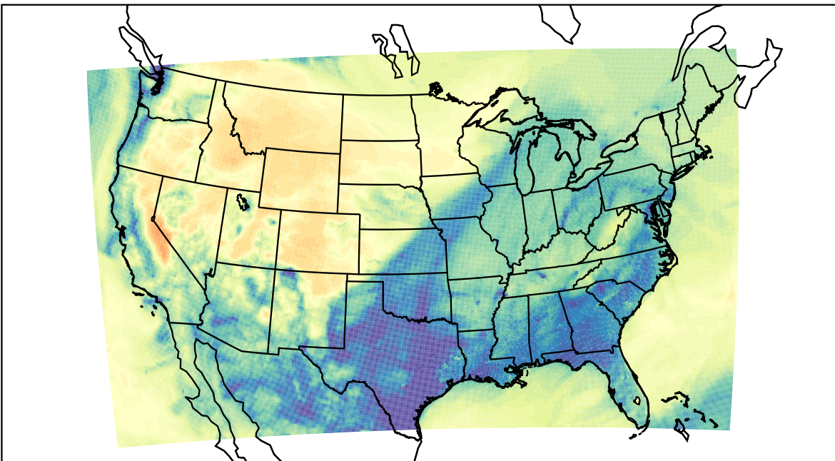
WRF (2022-11-21_10:00:00)
