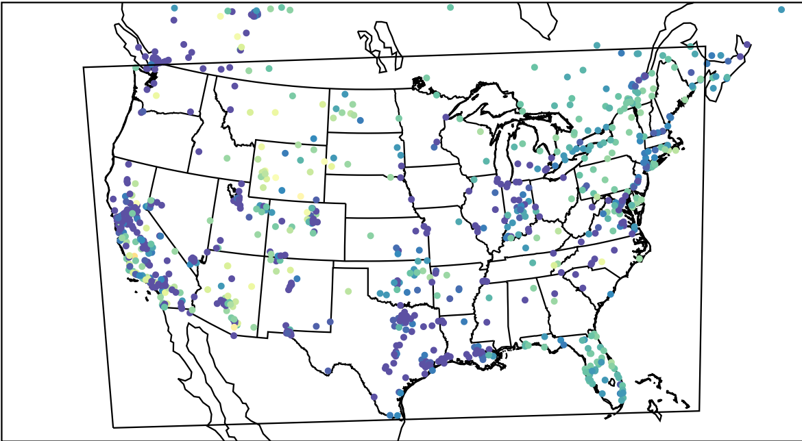
AirNOW (2022-11-22_01:00:00)
