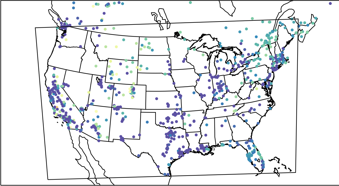
AirNOW (2022-11-22_09:00:00)
