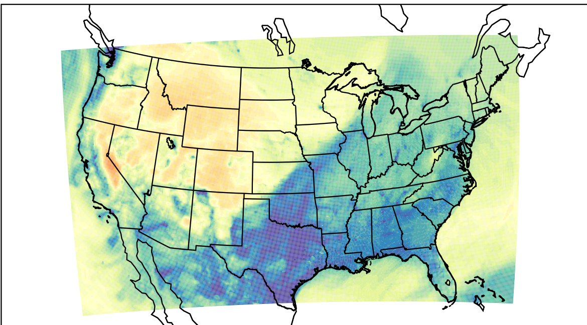
WRF (2022-11-21_14:00:00)
