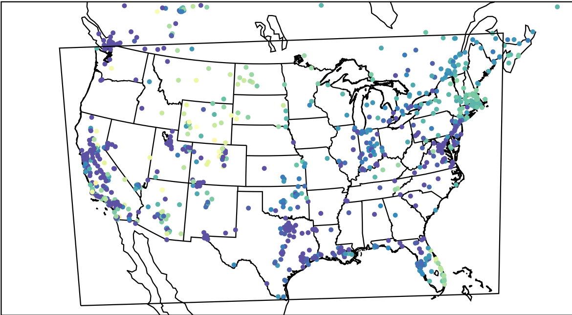
AirNOW (2022-11-21_06:00:00)
