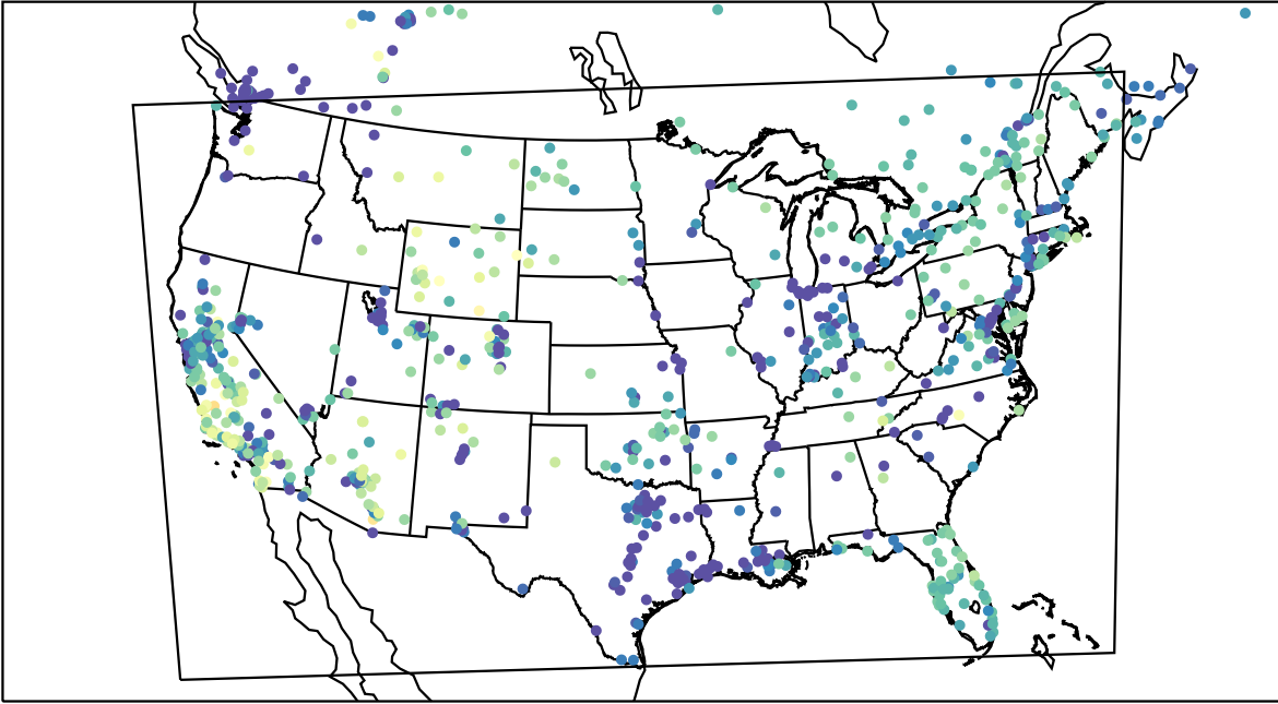
AirNOW (2022-11-22_00:00:00)
