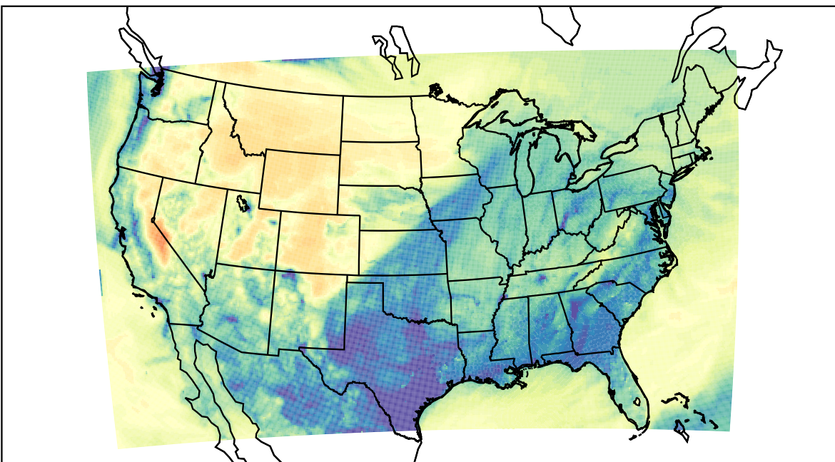
WRF (2022-11-21_06:00:00)
