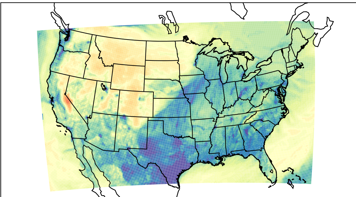
WRF (2022-11-21_03:00:00)
