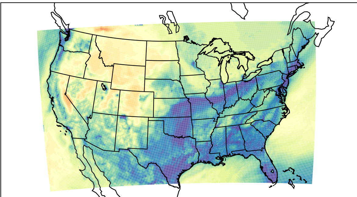
WRF (2022-11-22_07:00:00)
