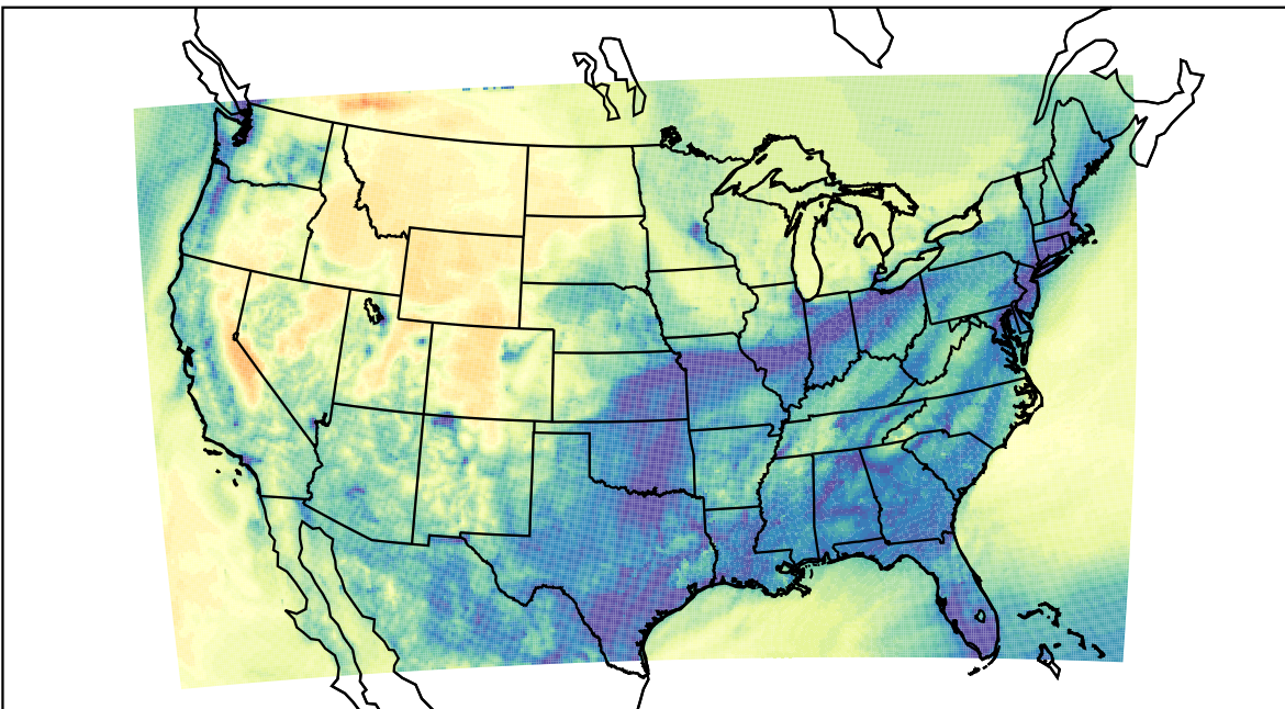
WRF (2022-11-22_06:00:00)
