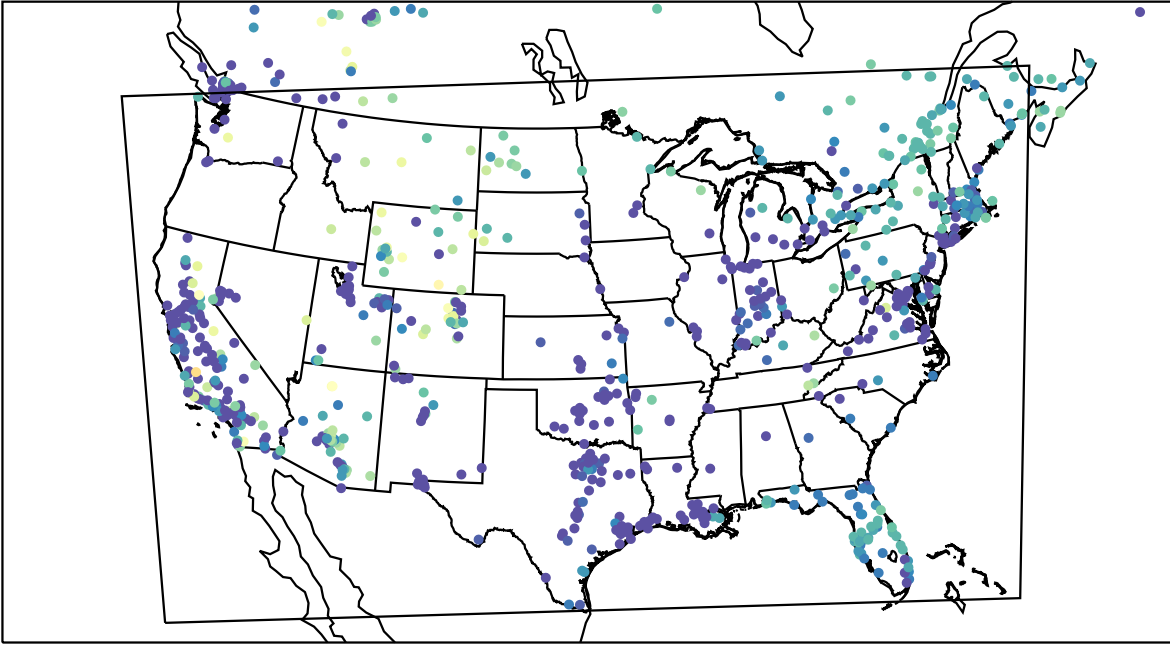
AirNOW (2022-11-22_08:00:00)
