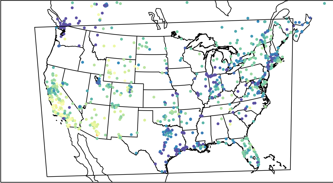
AirNOW (2022-11-21_23:00:00)
