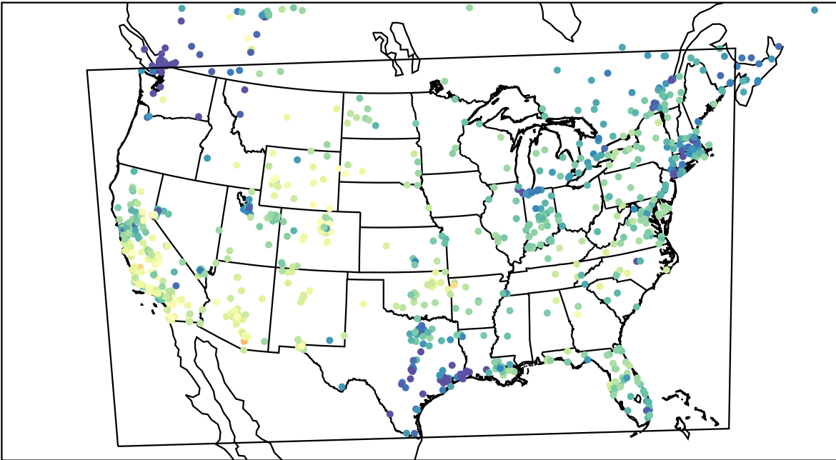
AirNOW (2022-11-21_21:00:00)
