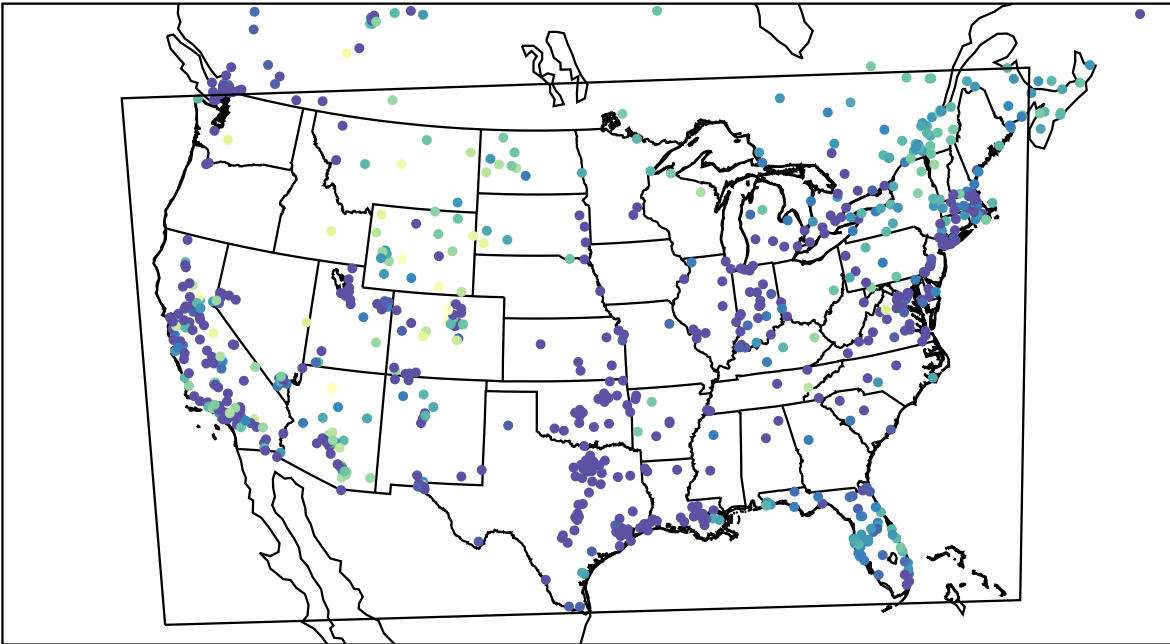
AirNOW (2022-11-22_10:00:00)
