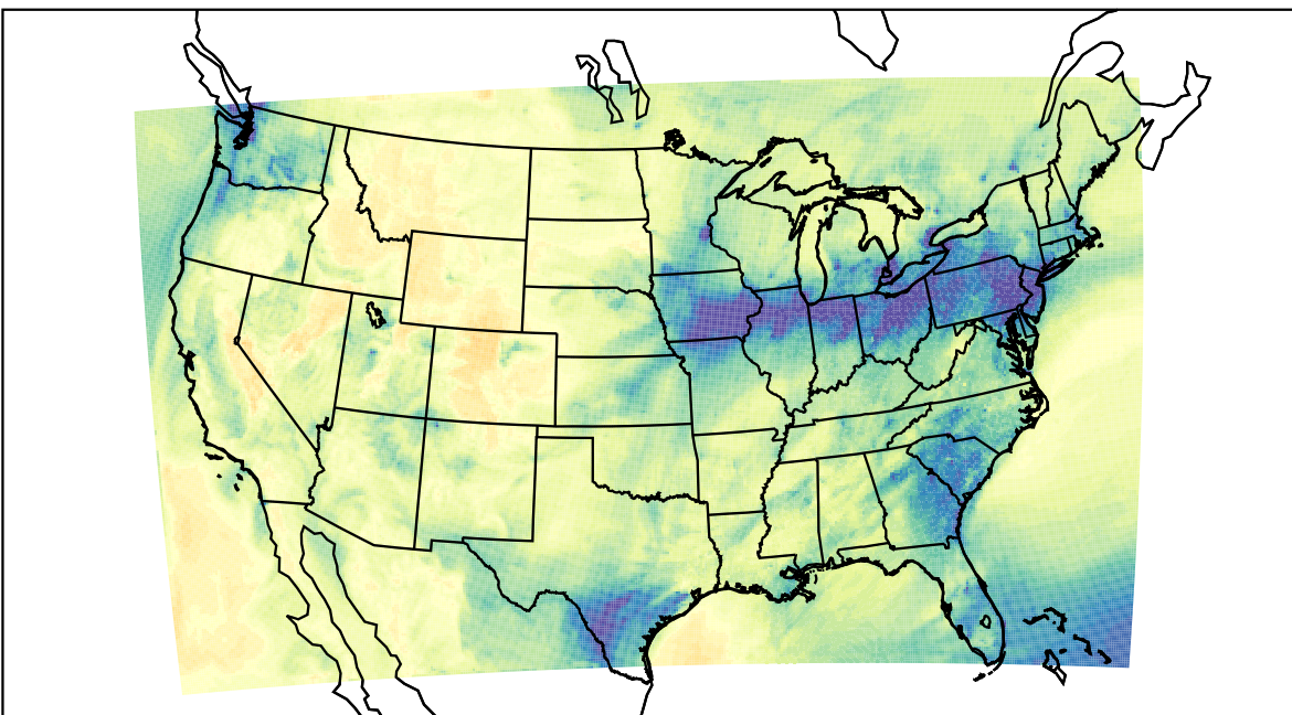
WRF (2022-11-22_21:00:00)
