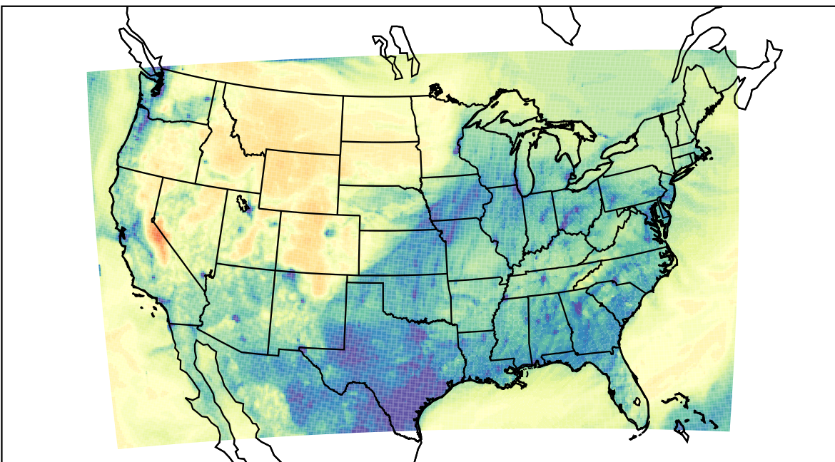
WRF (2022-11-21_02:00:00)
