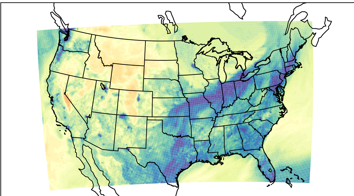
WRF (2022-11-22_01:00:00)
