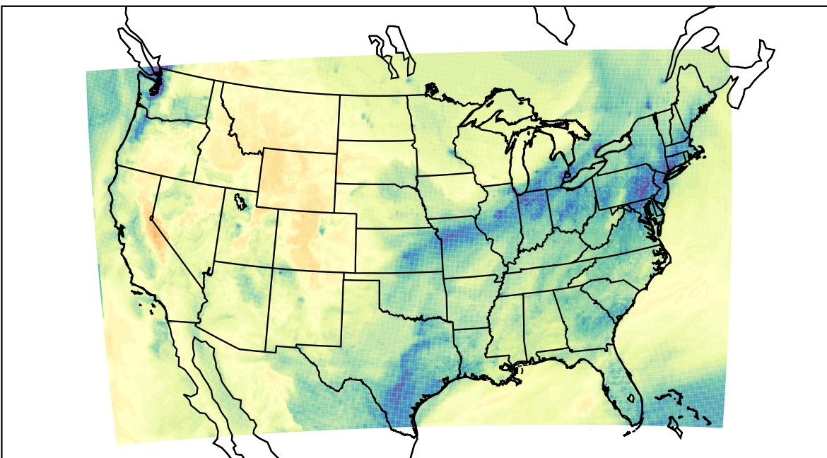
WRF (2022-11-21_21:00:00)
