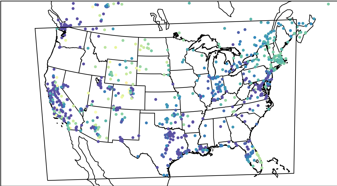
AirNOW (2022-11-21_05:00:00)
