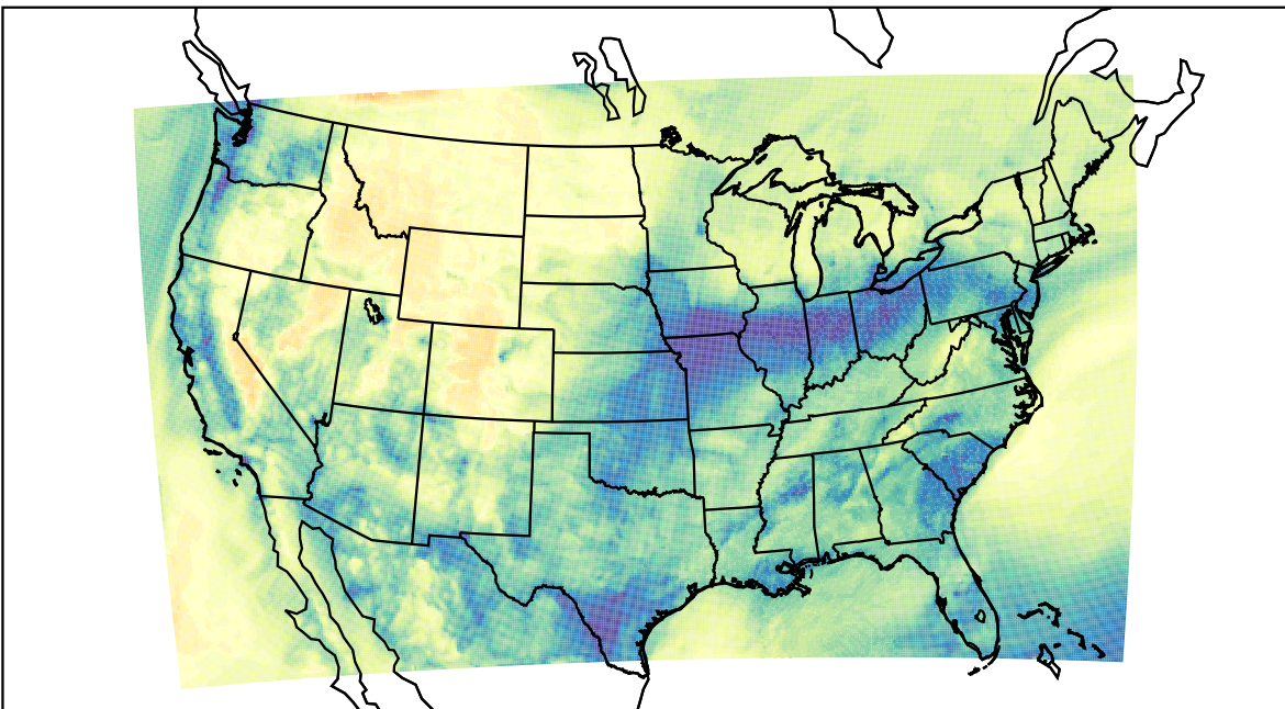
WRF (2022-11-22_17:00:00)
