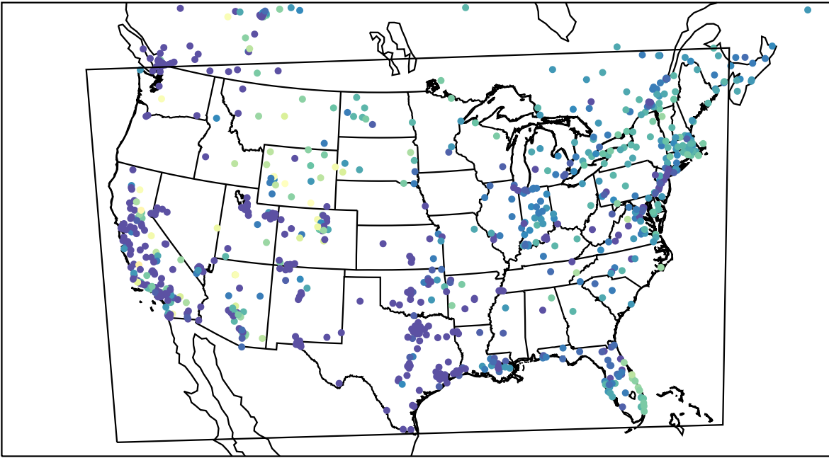
AirNOW (2022-11-21_14:00:00)
