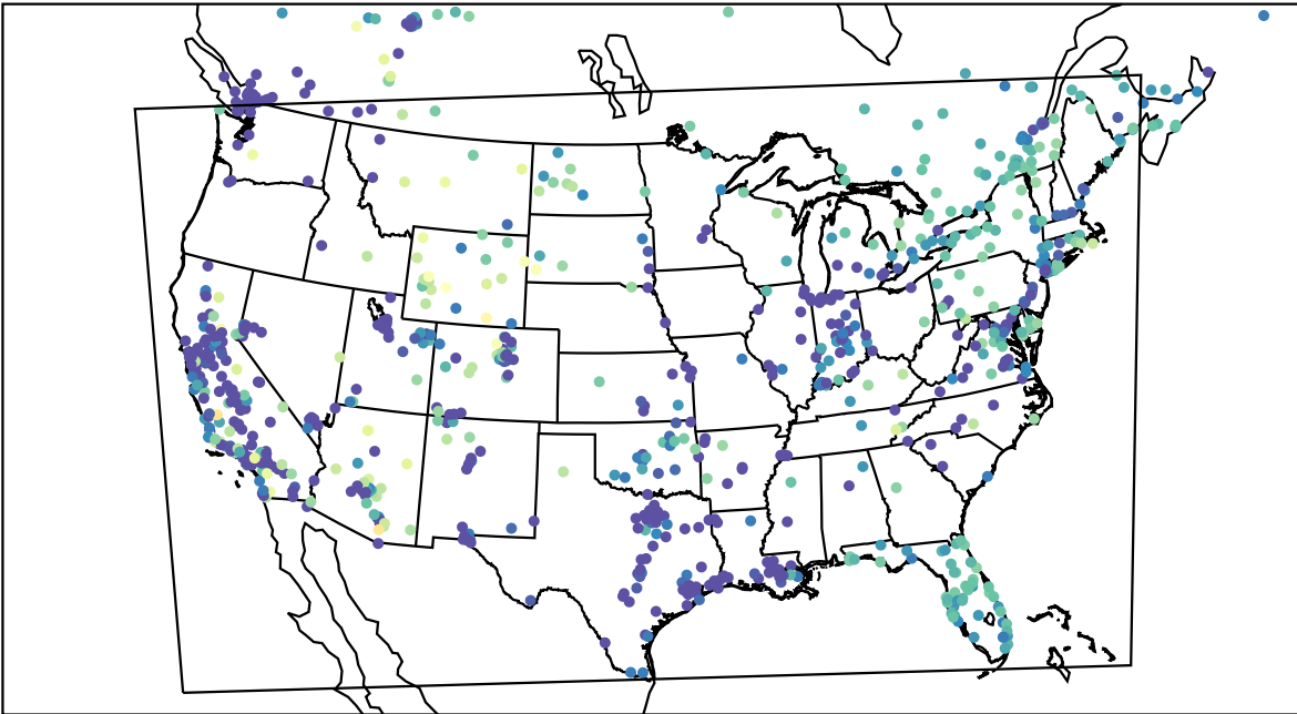
AirNOW (2022-11-22_02:00:00)
