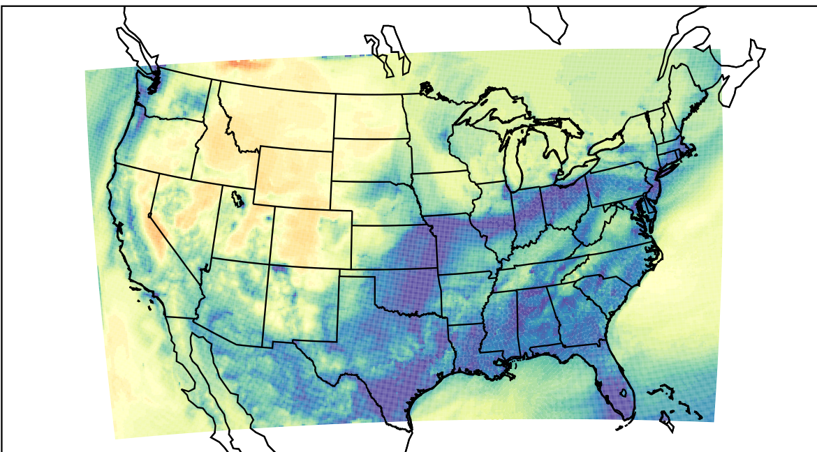
WRF (2022-11-22_11:00:00)
