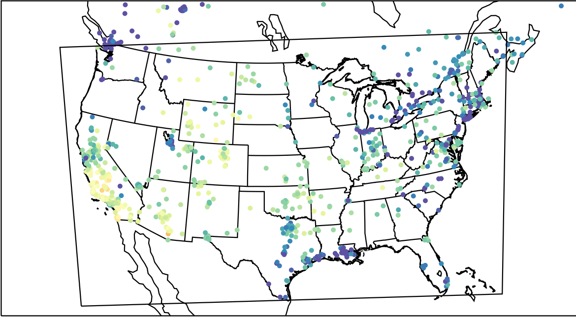
AirNOW (2022-11-22_22:00:00)
