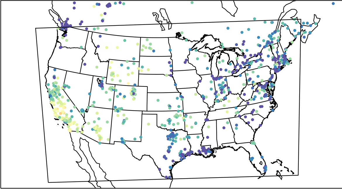
AirNOW (2022-11-22_23:00:00)
