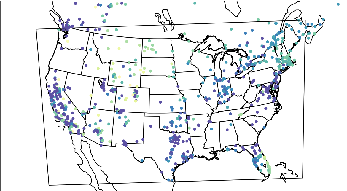
AirNOW (2022-11-21_07:00:00)
