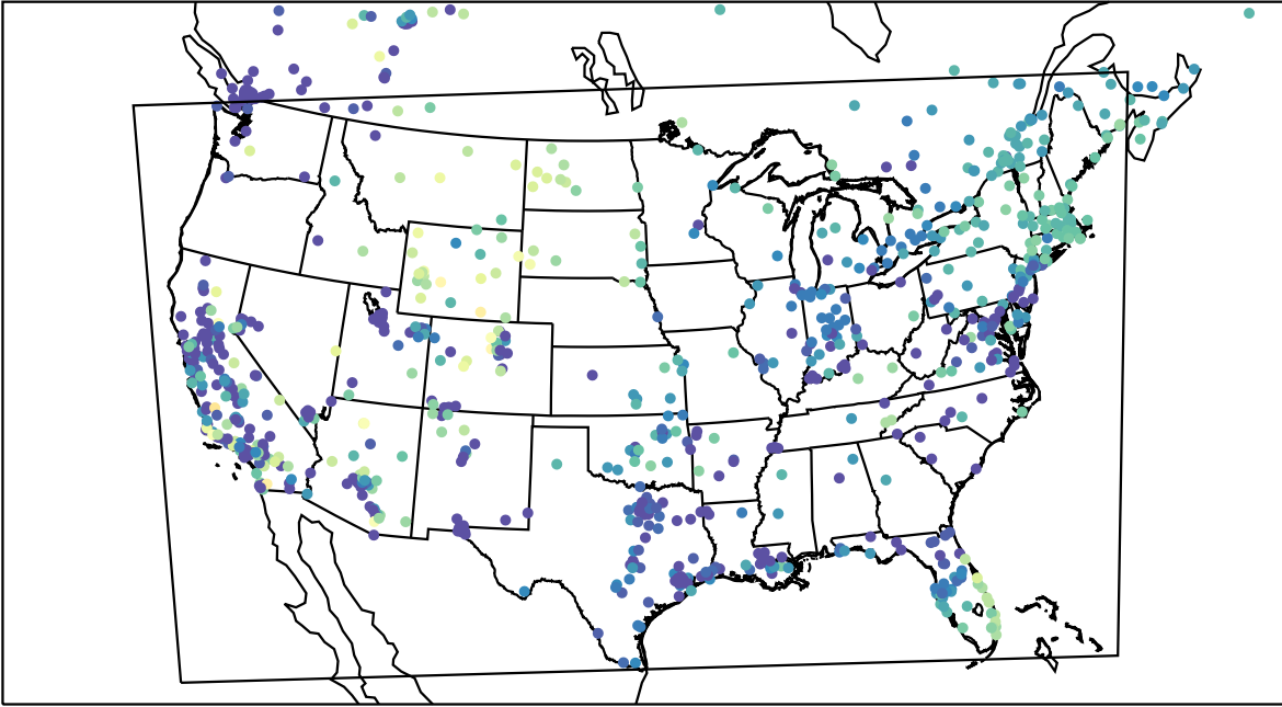
AirNOW (2022-11-21_03:00:00)
