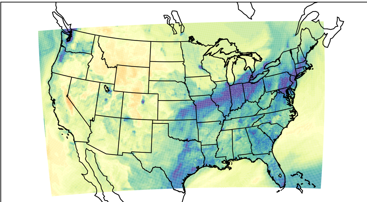
WRF (2022-11-21_23:00:00)
