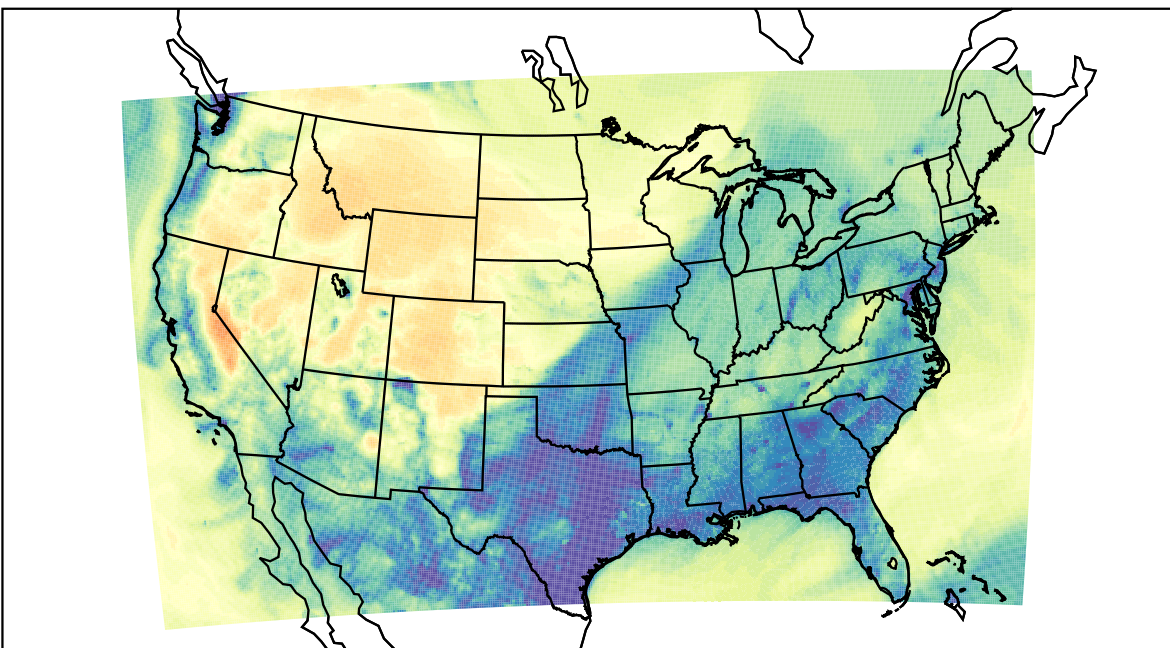
WRF (2022-11-21_12:00:00)
