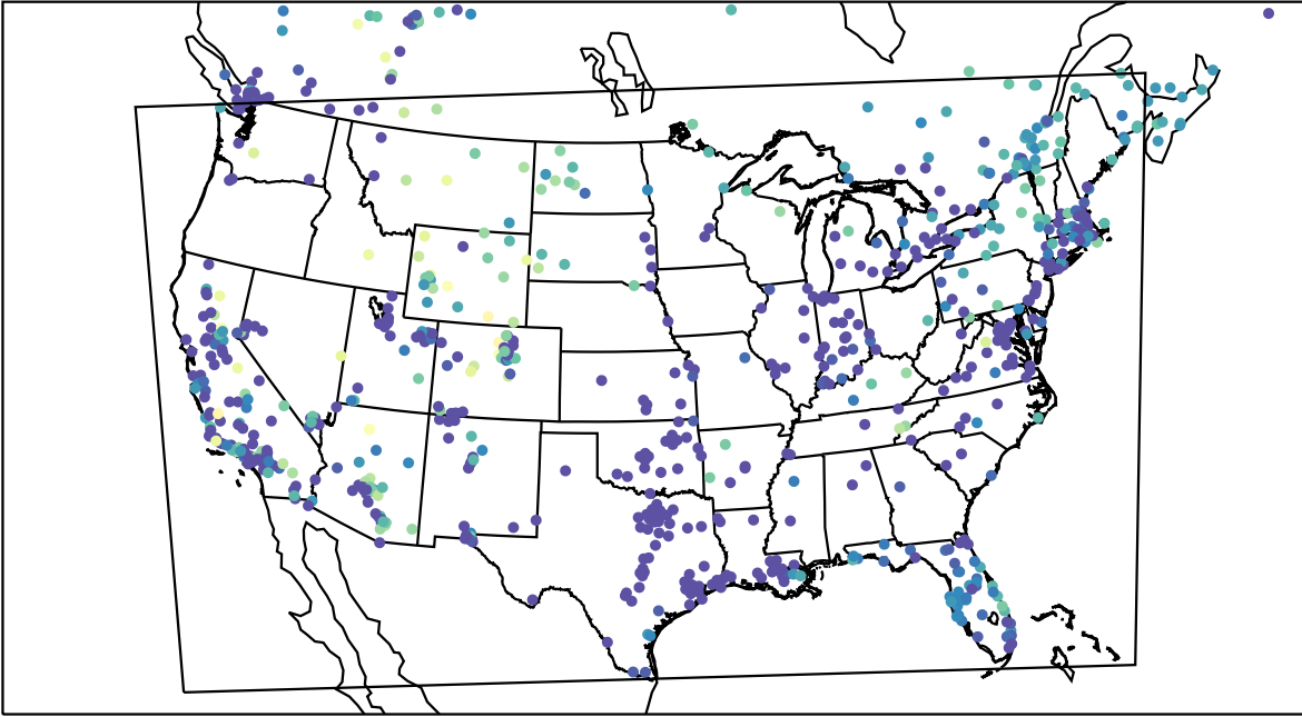
AirNOW (2022-11-22_11:00:00)
