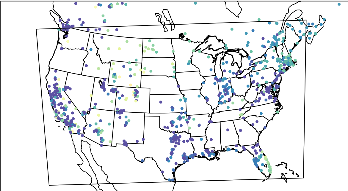
AirNOW (2022-11-21_08:00:00)
