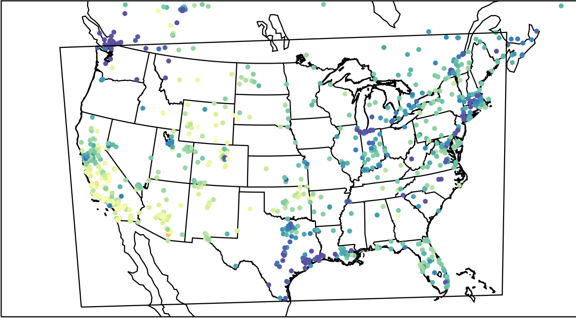
AirNOW (2022-11-21_22:00:00)
