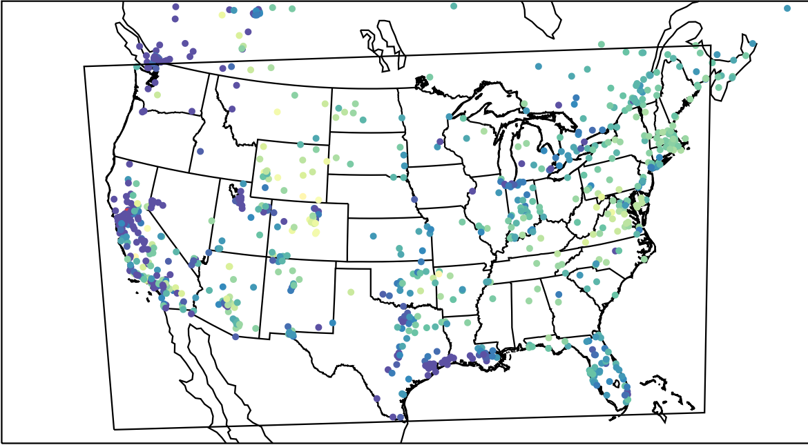
AirNOW (2022-11-22_17:00:00)
