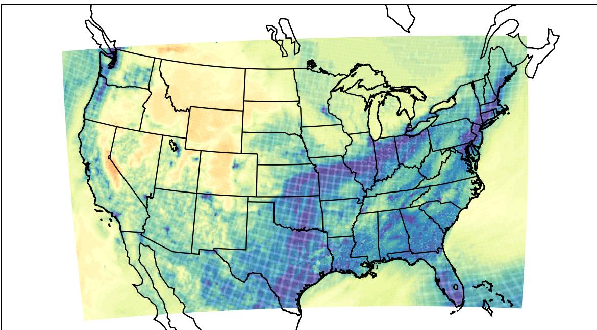
WRF (2022-11-22_04:00:00)
