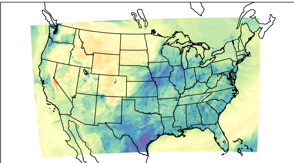
WRF (2022-11-21_00:00:00)
