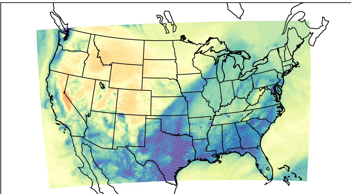
WRF (2022-11-21_11:00:00)
