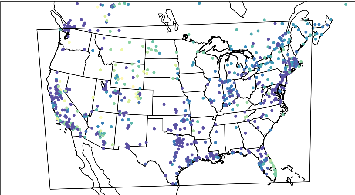
AirNOW (2022-11-21_11:00:00)
