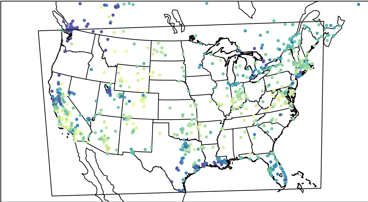
AirNOW (2022-11-22_19:00:00)
