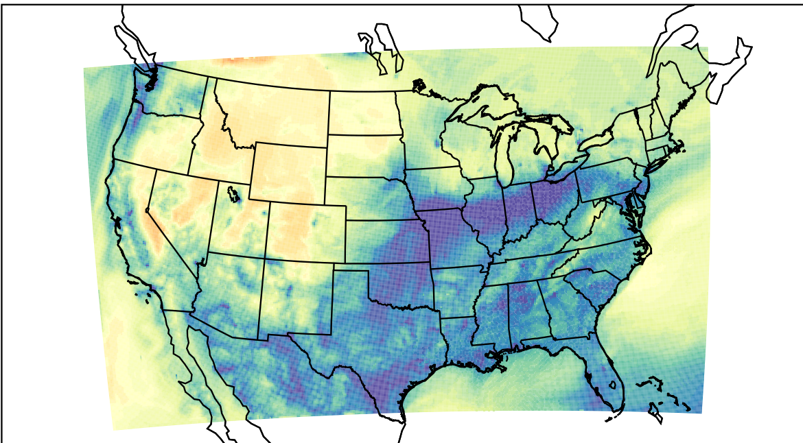
WRF (2022-11-22_15:00:00)
