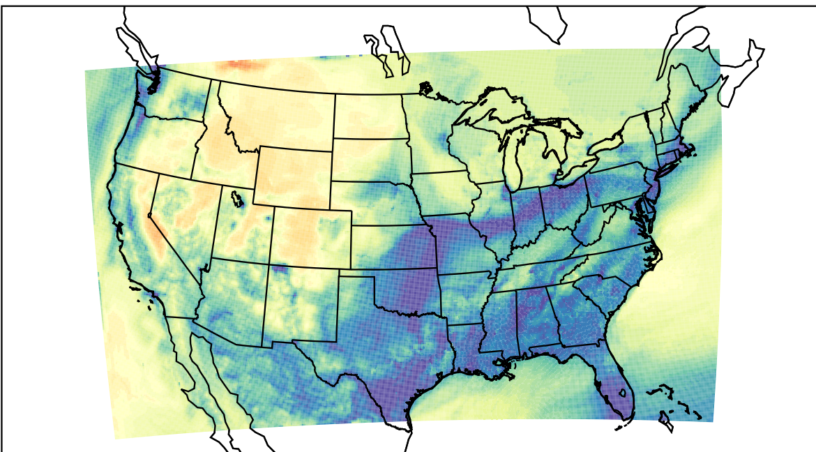
WRF (2022-11-22_10:00:00)
