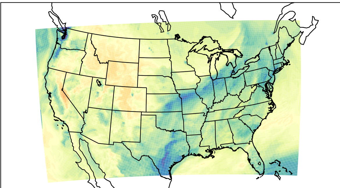
WRF (2022-11-21_20:00:00)
