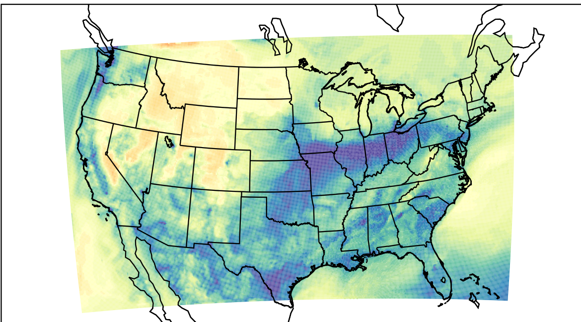
WRF (2022-11-22_16:00:00)
