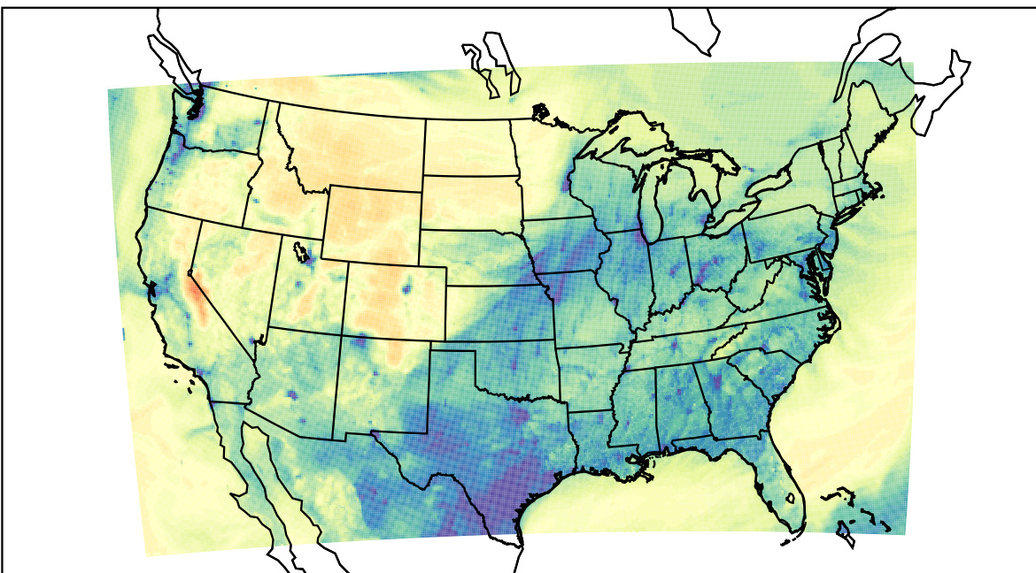
WRF (2022-11-21_01:00:00)
