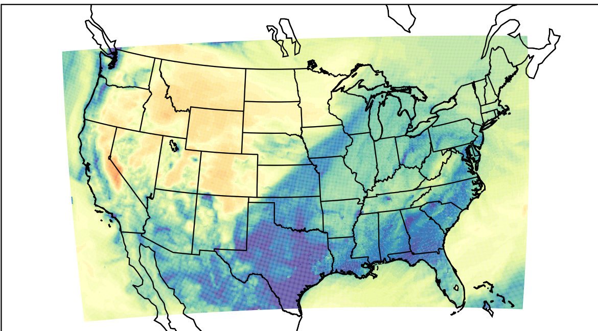
WRF (2022-11-21_08:00:00)
