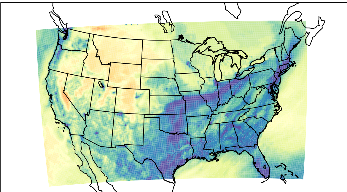
WRF (2022-11-22_05:00:00)
