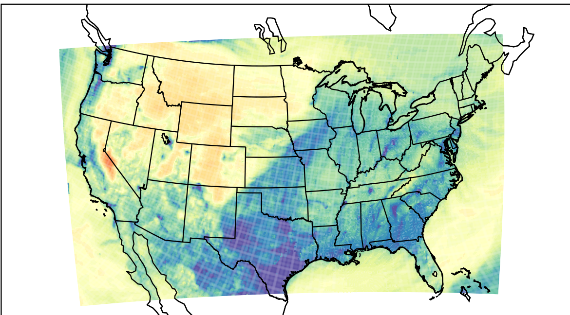
WRF (2022-11-21_04:00:00)
