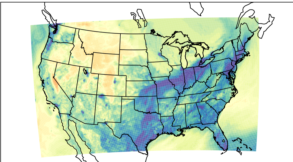
WRF (2022-11-22_02:00:00)
