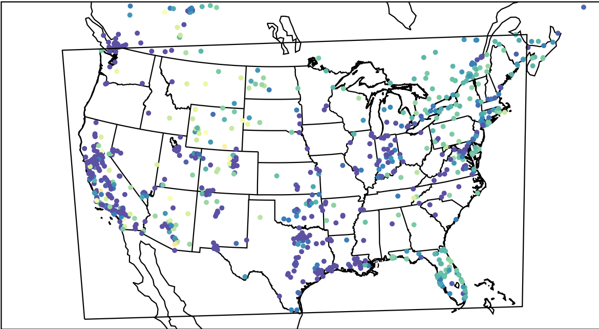
AirNOW (2022-11-22_03:00:00)
