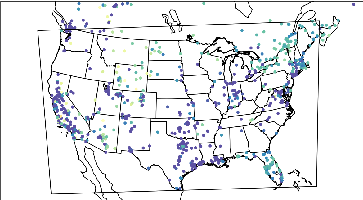
AirNOW (2022-11-22_07:00:00)
