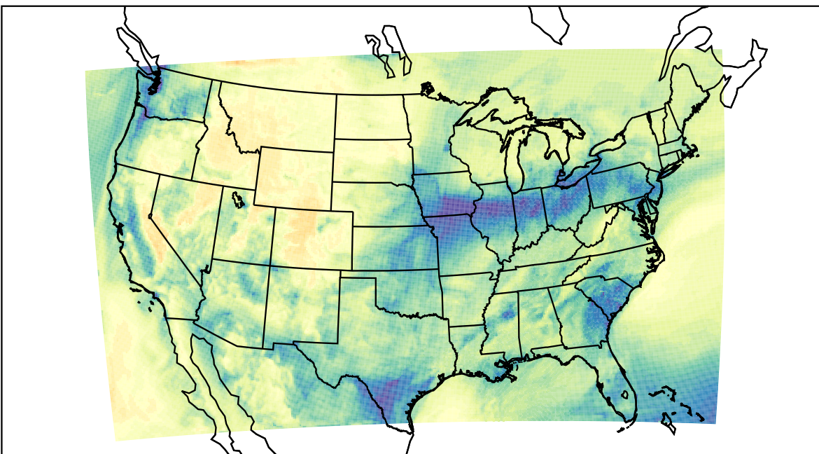
WRF (2022-11-22_18:00:00)
