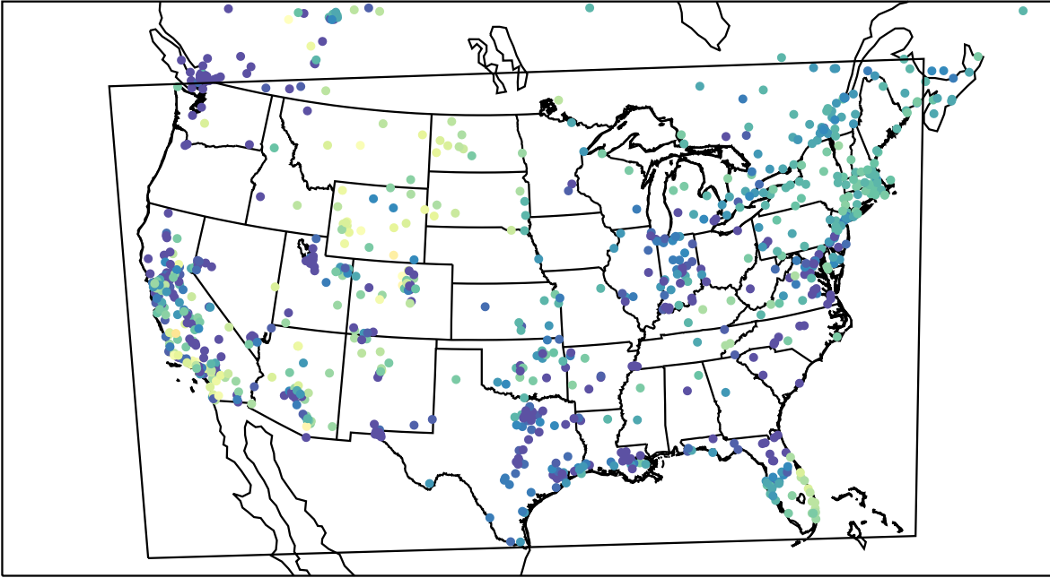
AirNOW (2022-11-21_01:00:00)
