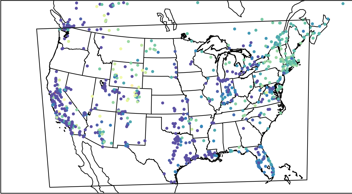
AirNOW (2022-11-22_15:00:00)
