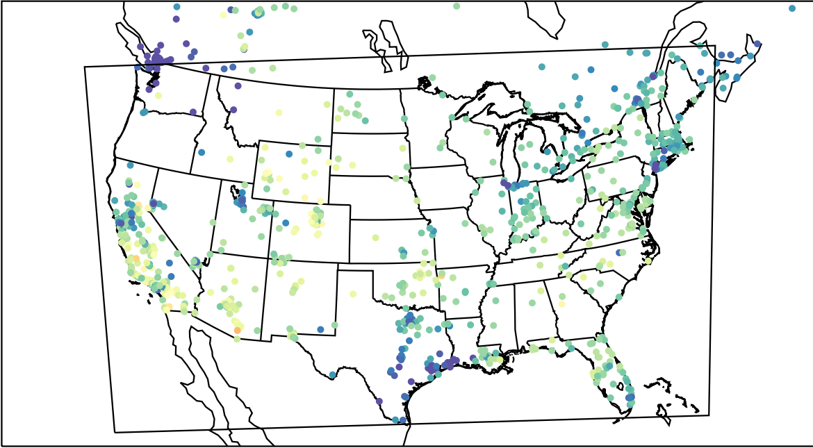
AirNOW (2022-11-21_20:00:00)
