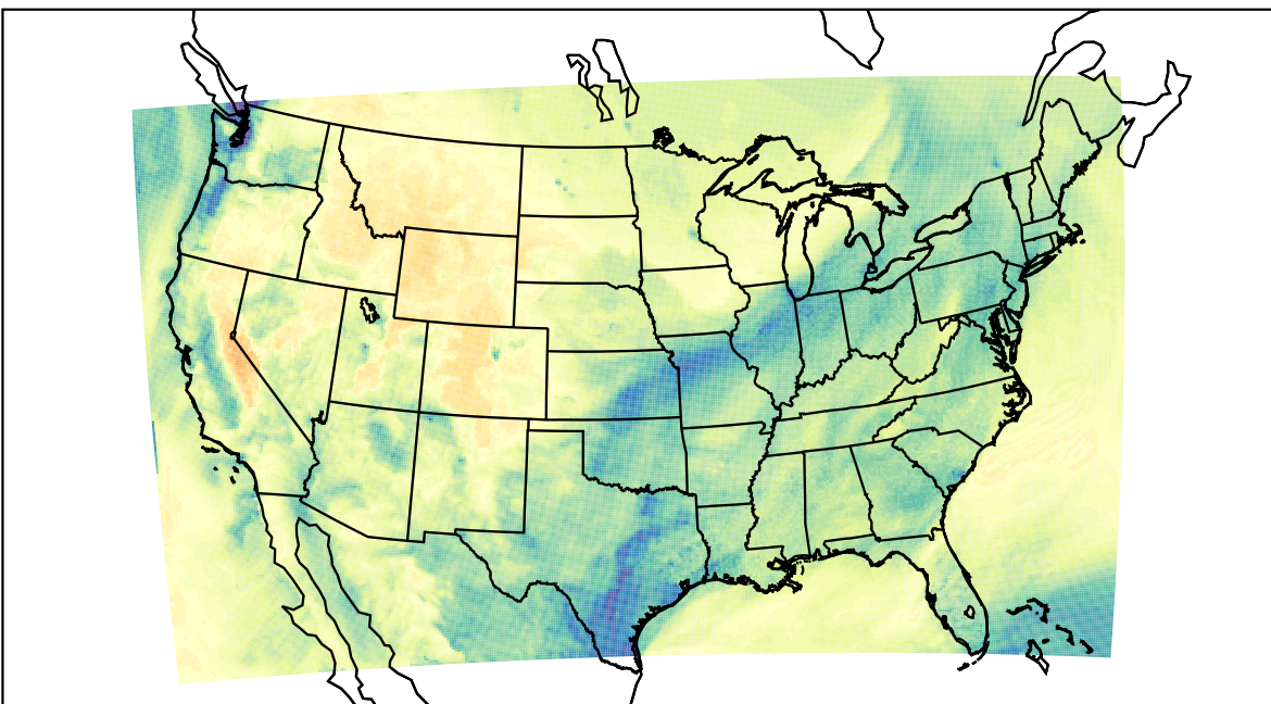
WRF (2022-11-21_19:00:00)
