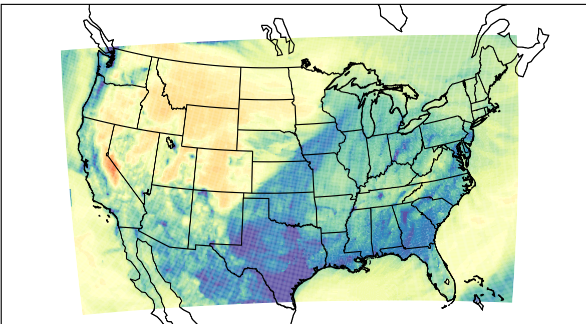
WRF (2022-11-21_05:00:00)
