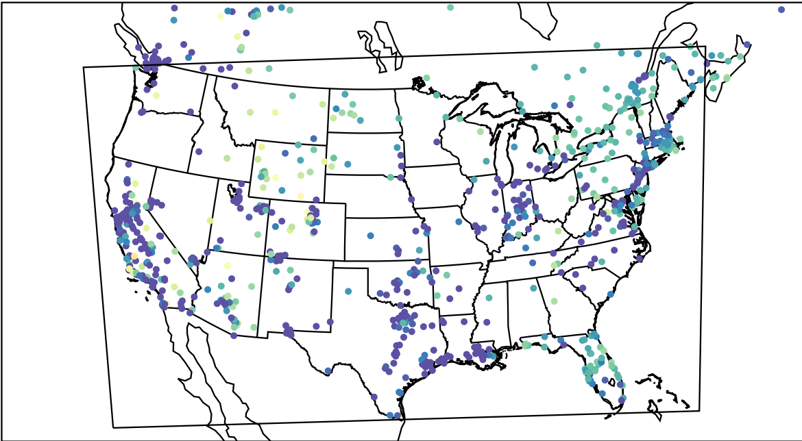
AirNOW (2022-11-22_05:00:00)
