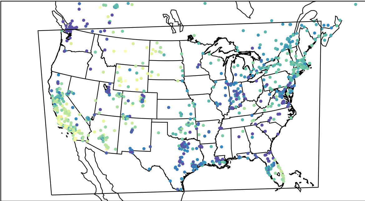
AirNOW (2022-11-21_00:00:00)
