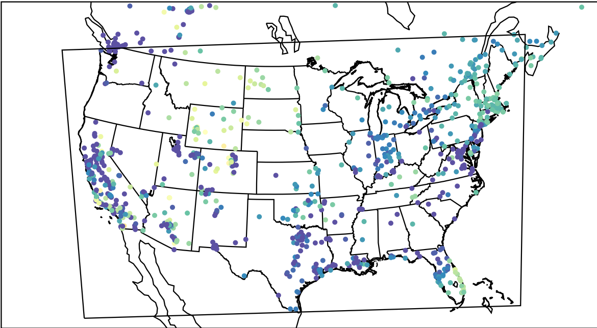
AirNOW (2022-11-21_04:00:00)
