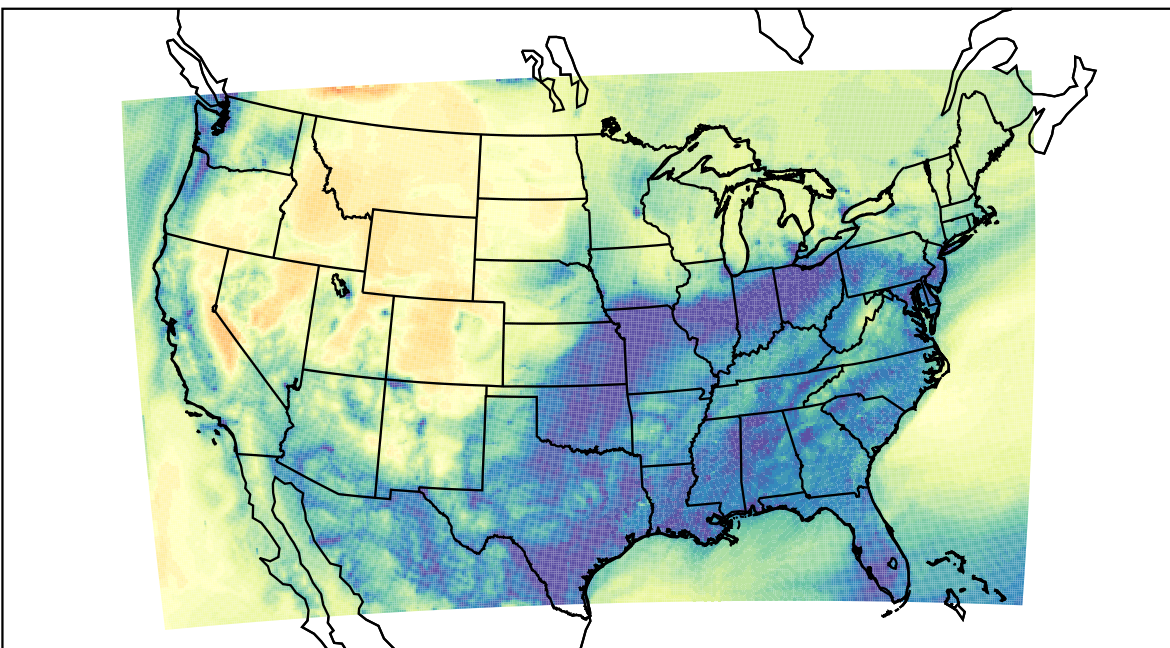
WRF (2022-11-22_14:00:00)
