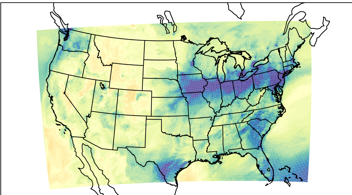
WRF (2022-11-22_22:00:00)
