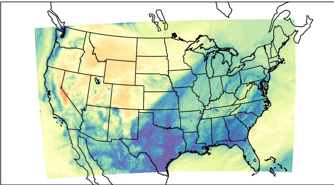
WRF (2022-11-21_09:00:00)
