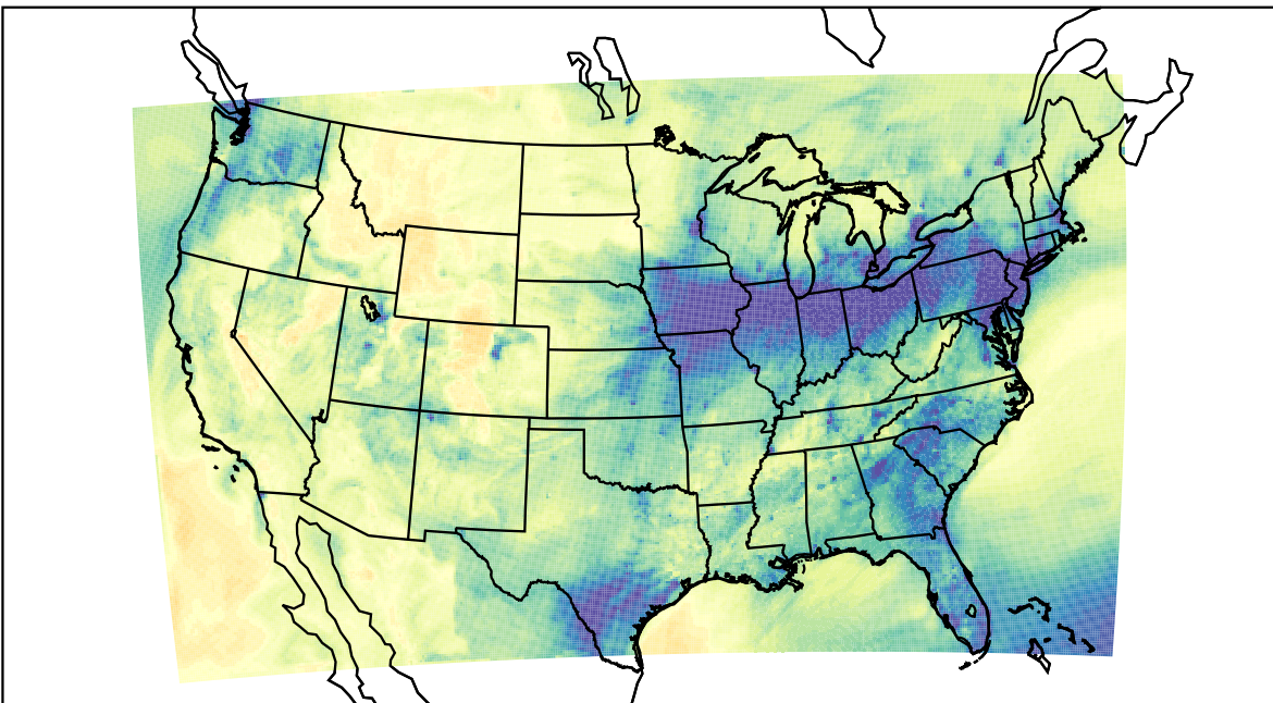
WRF (2022-11-22_23:00:00)
