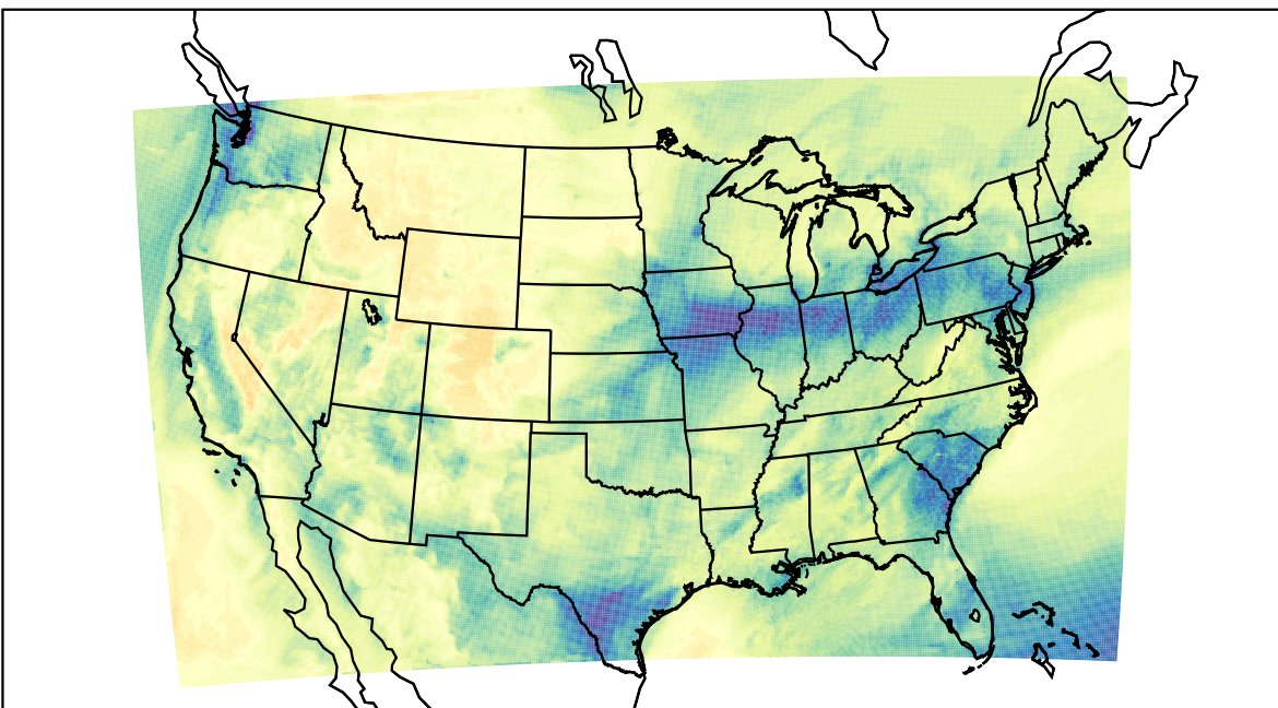
WRF (2022-11-22_19:00:00)
