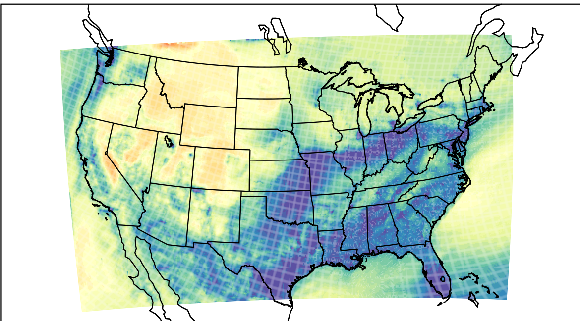
WRF (2022-11-22_13:00:00)
