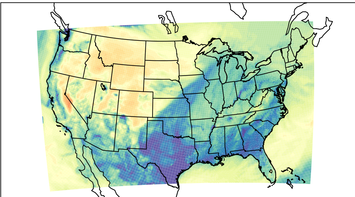
WRF (2022-11-21_07:00:00)
