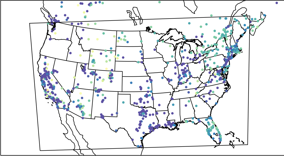
AirNOW (2022-11-22_06:00:00)
