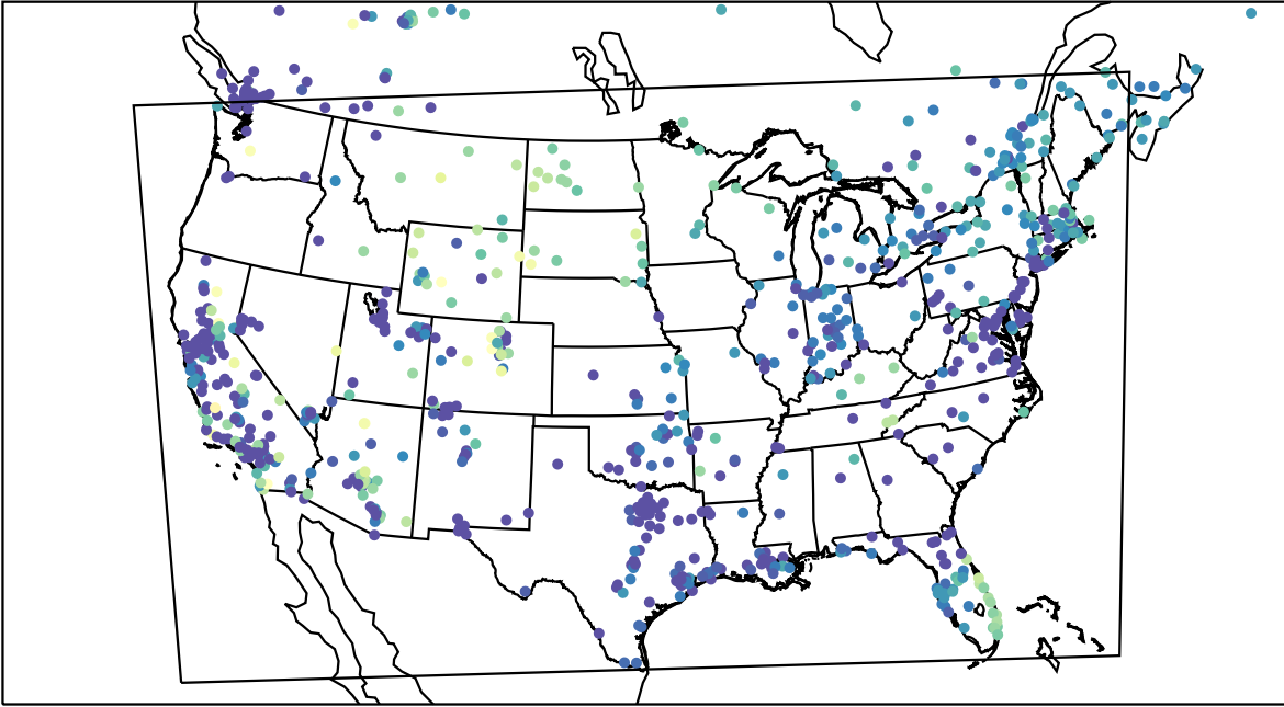
AirNOW (2022-11-21_09:00:00)
