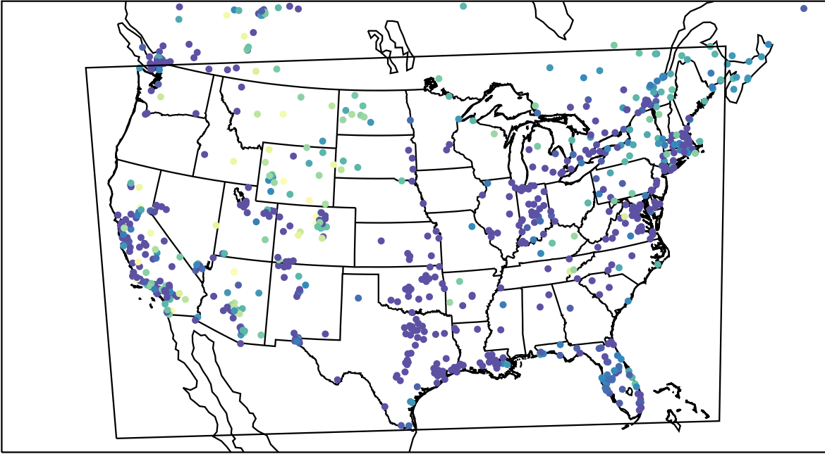
AirNOW (2022-11-22_12:00:00)
