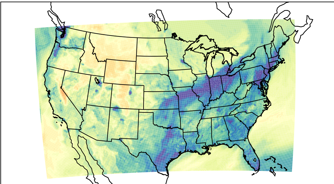
WRF (2022-11-22_00:00:00)
