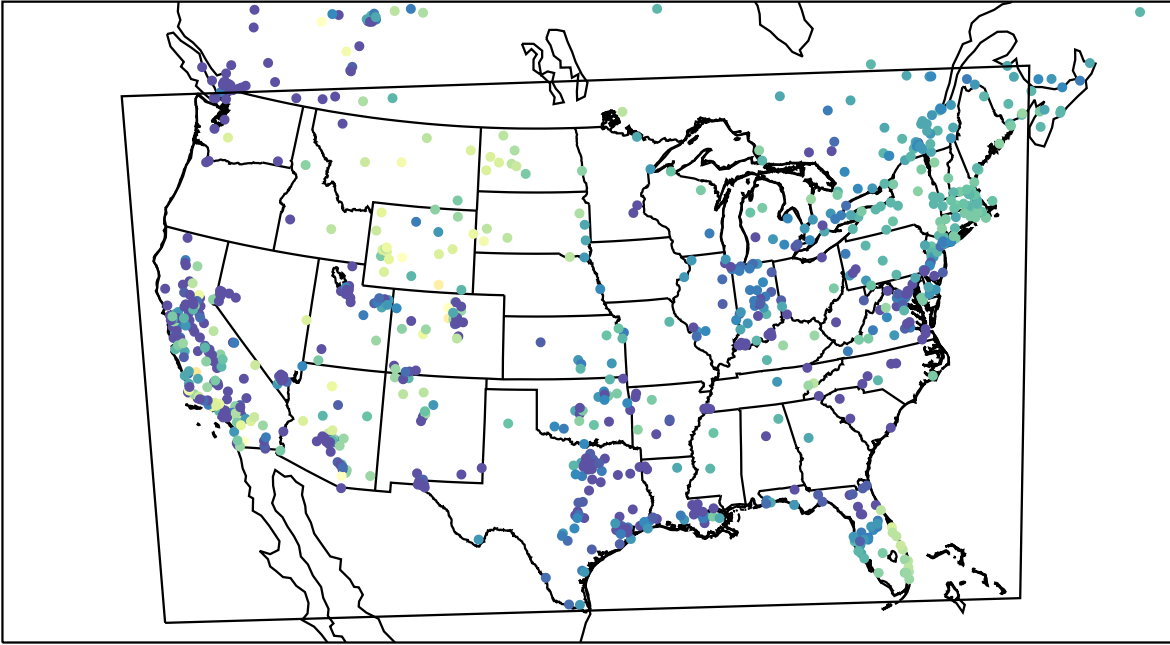
AirNOW (2022-11-21_02:00:00)
