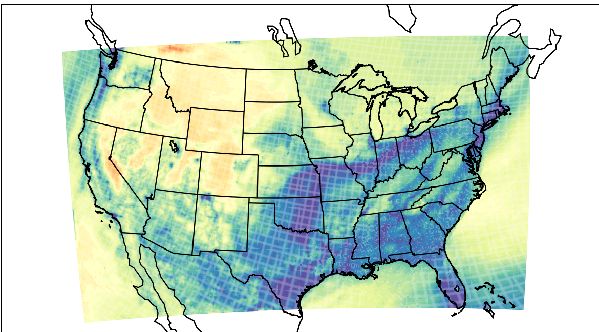
WRF (2022-11-22_08:00:00)
