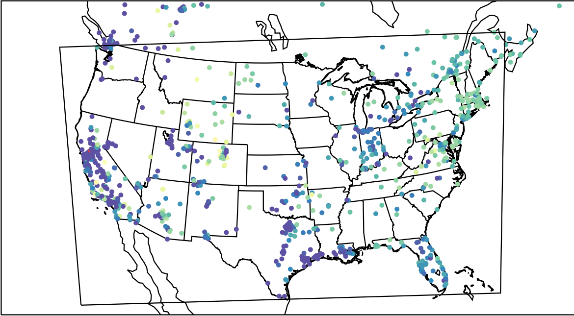
AirNOW (2022-11-22_16:00:00)
