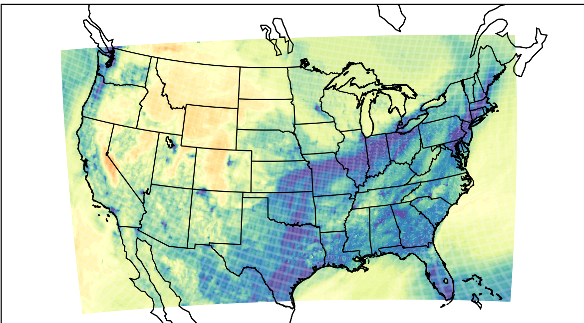
WRF (2022-11-22_03:00:00)
