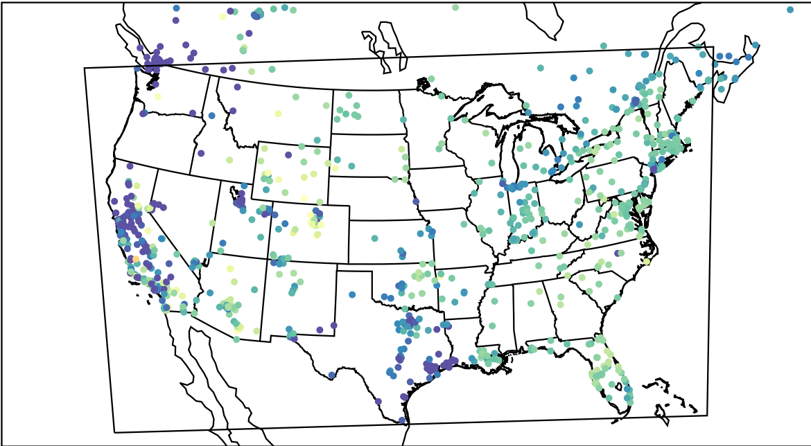
AirNOW (2022-11-21_17:00:00)
