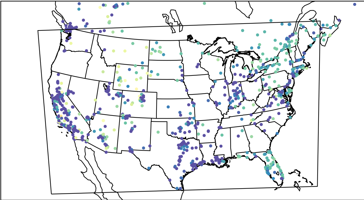
AirNOW (2022-11-22_04:00:00)
