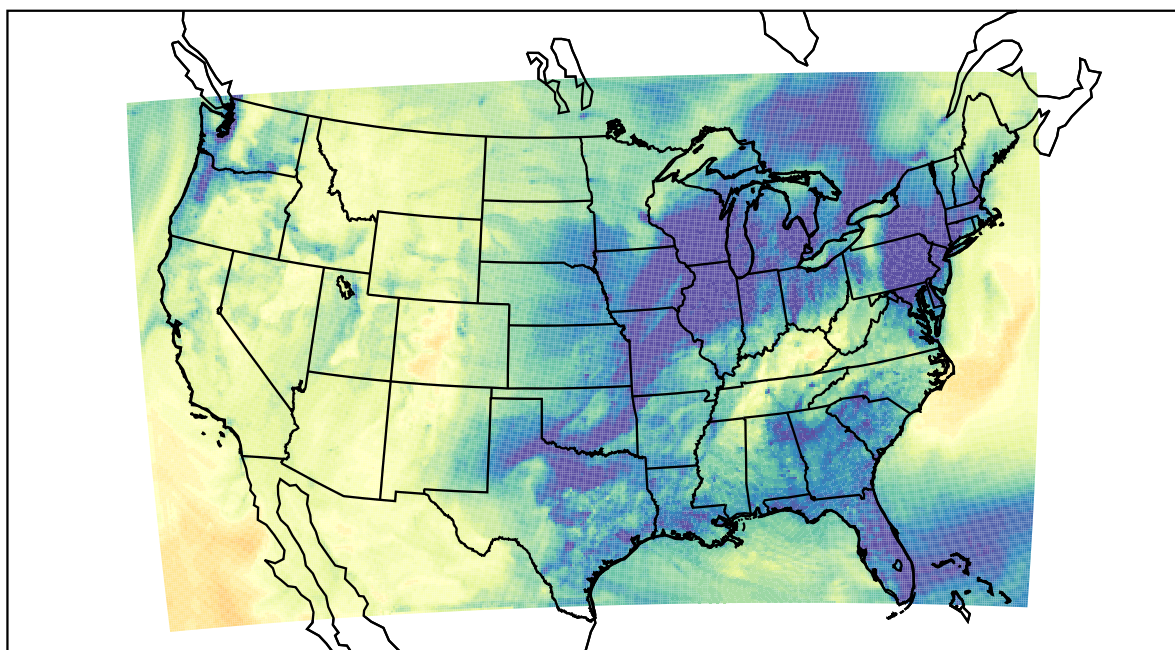
WRF (2022-11-24_23:00:00)
