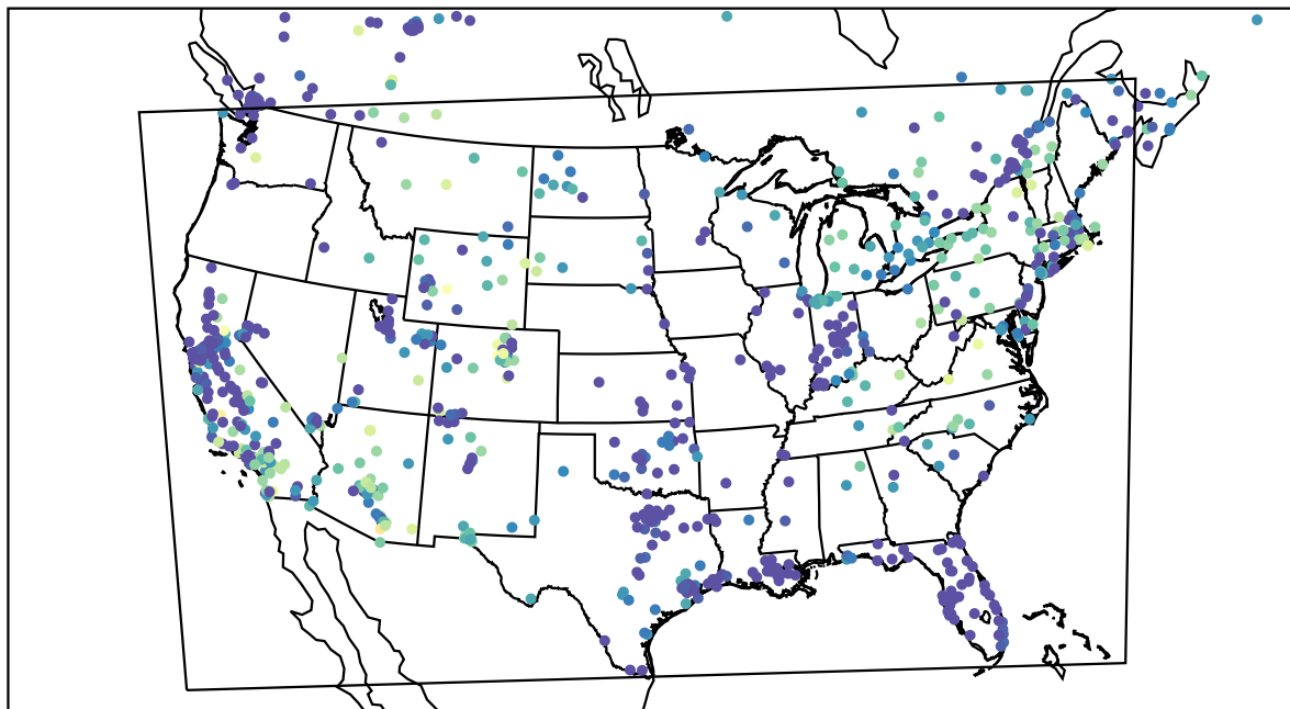
AirNOW (2022-11-25_09:00:00)
