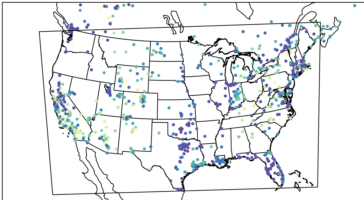
AirNOW (2022-11-25_02:00:00)
