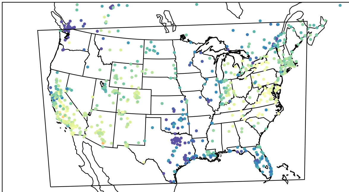
AirNOW (2022-11-24_19:00:00)
