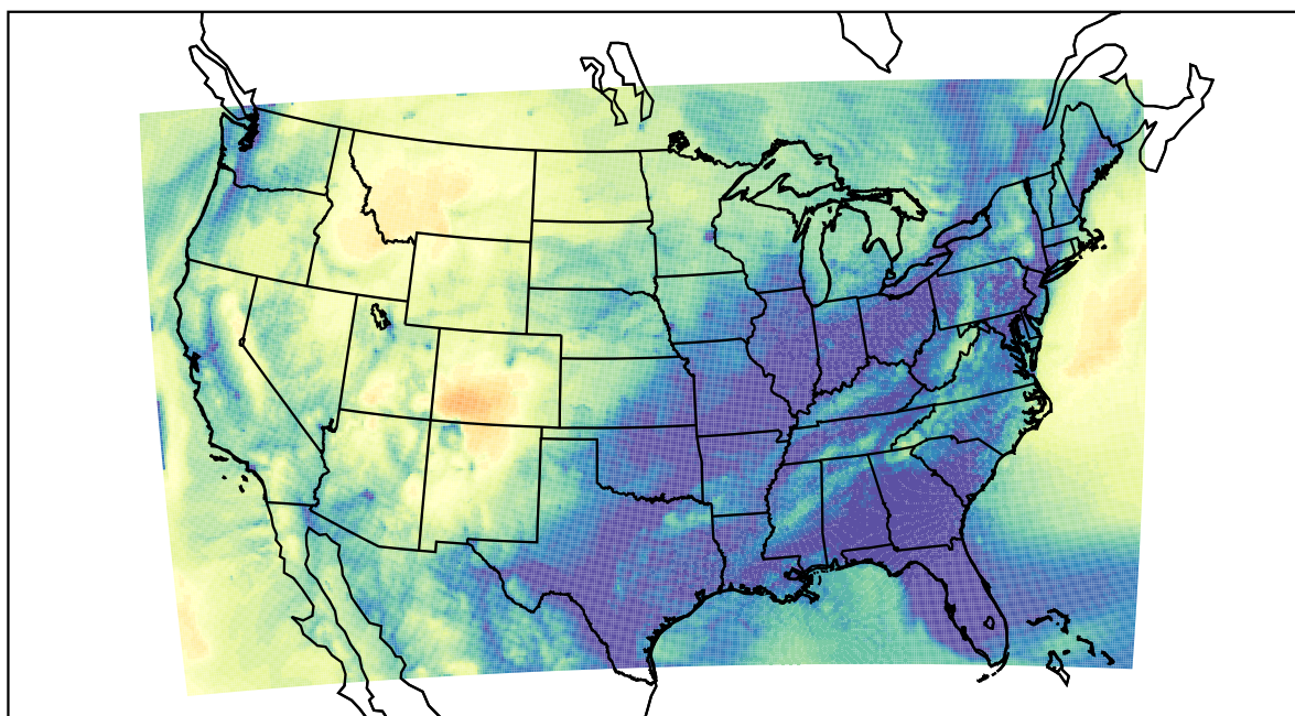
WRF (2022-11-25_14:00:00)
