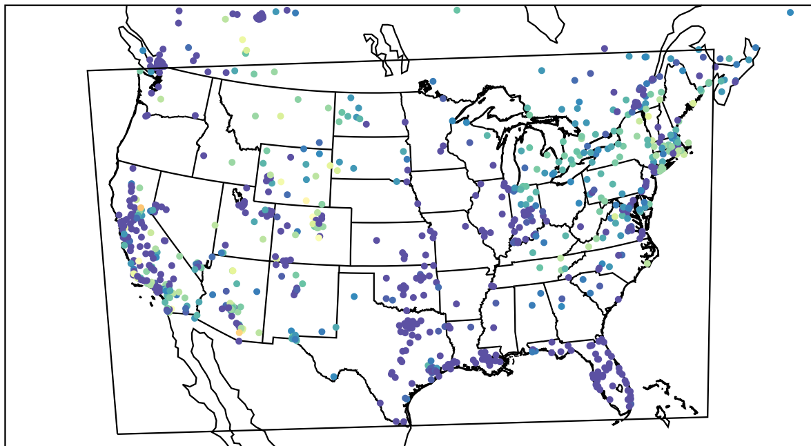
AirNOW (2022-11-25_13:00:00)
