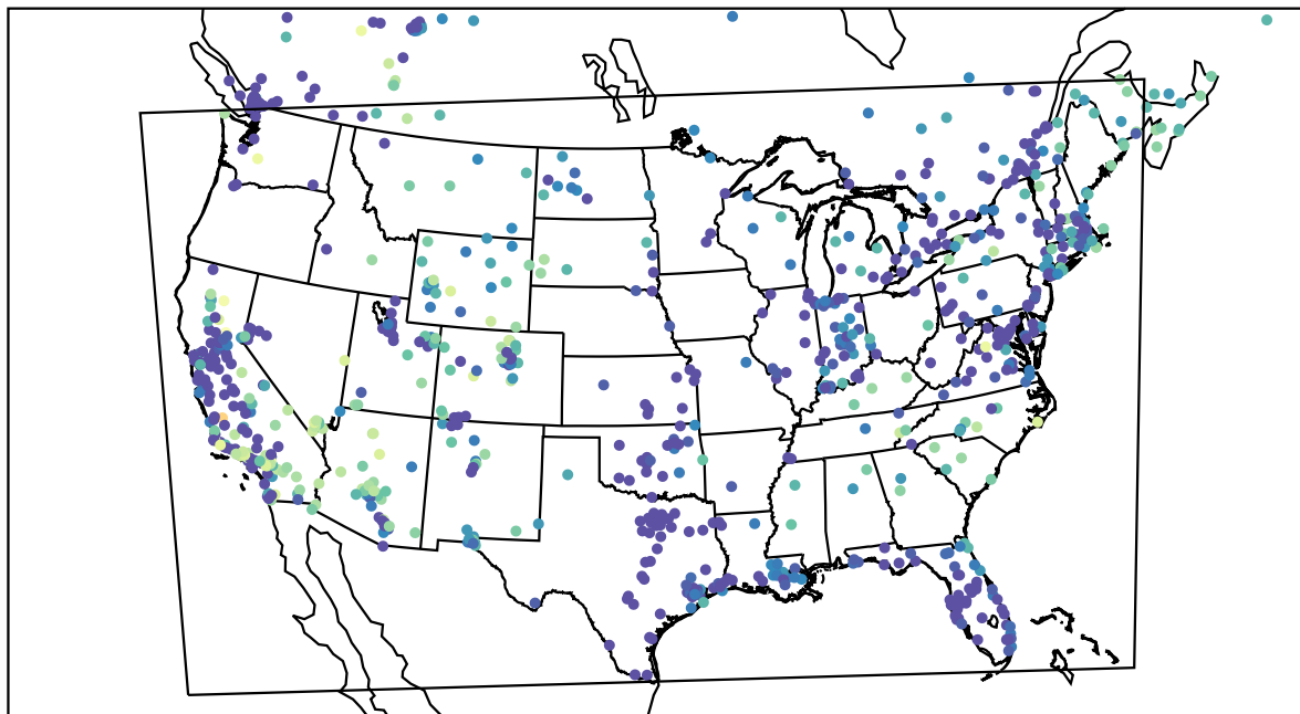
AirNOW (2022-11-24_14:00:00)
