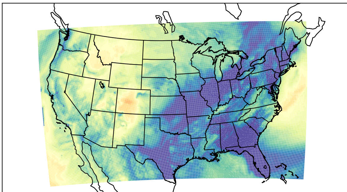
WRF (2022-11-25_09:00:00)
