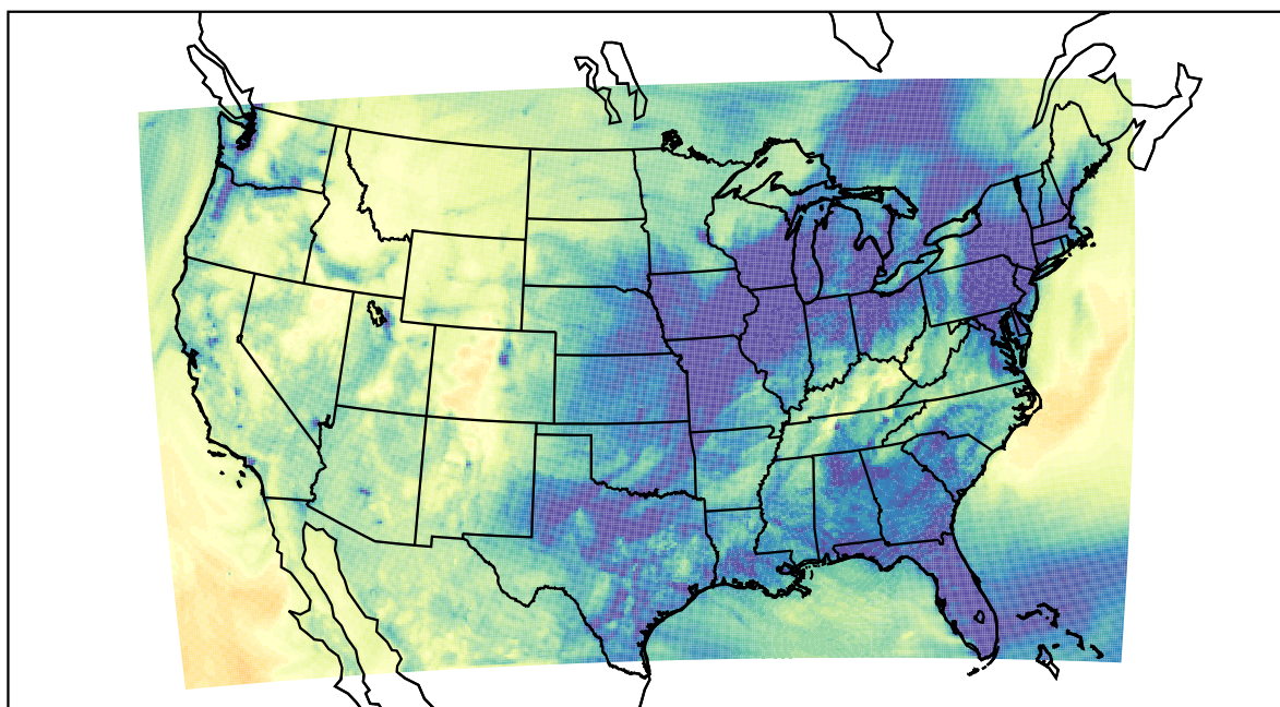
WRF (2022-11-25_01:00:00)
