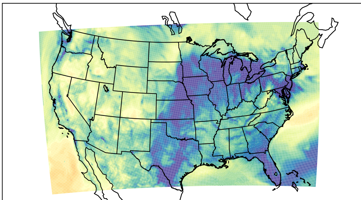
WRF (2022-11-24_05:00:00)
