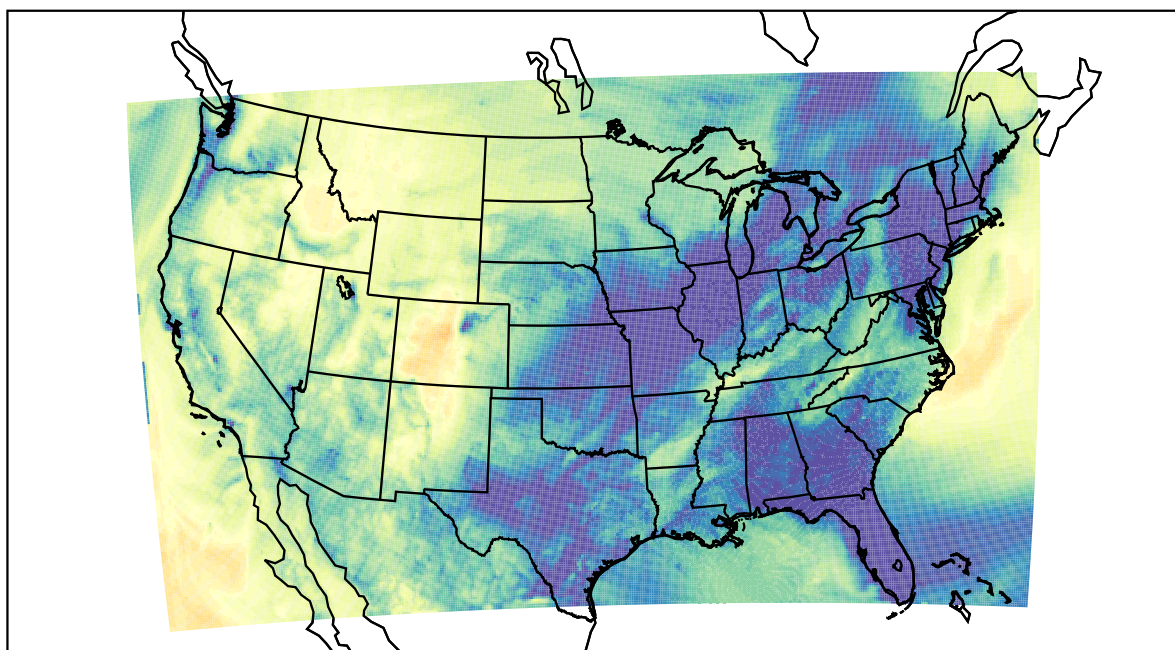
WRF (2022-11-25_05:00:00)
