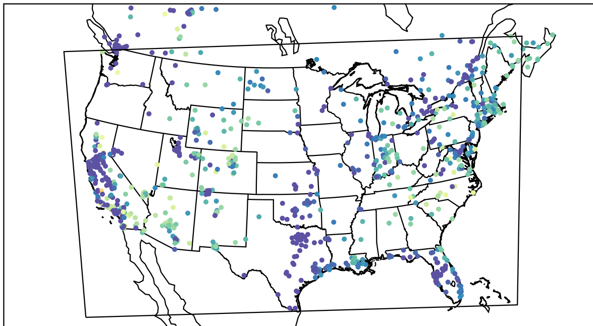
AirNOW (2022-11-24_15:00:00)
