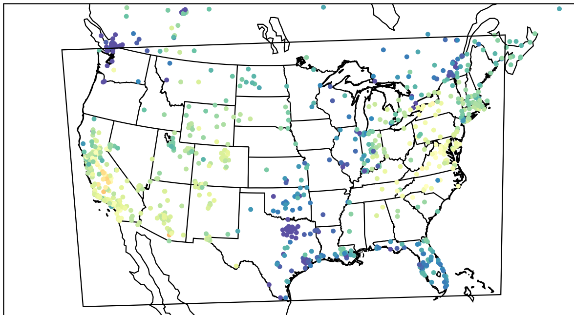
AirNOW (2022-11-24_20:00:00)
