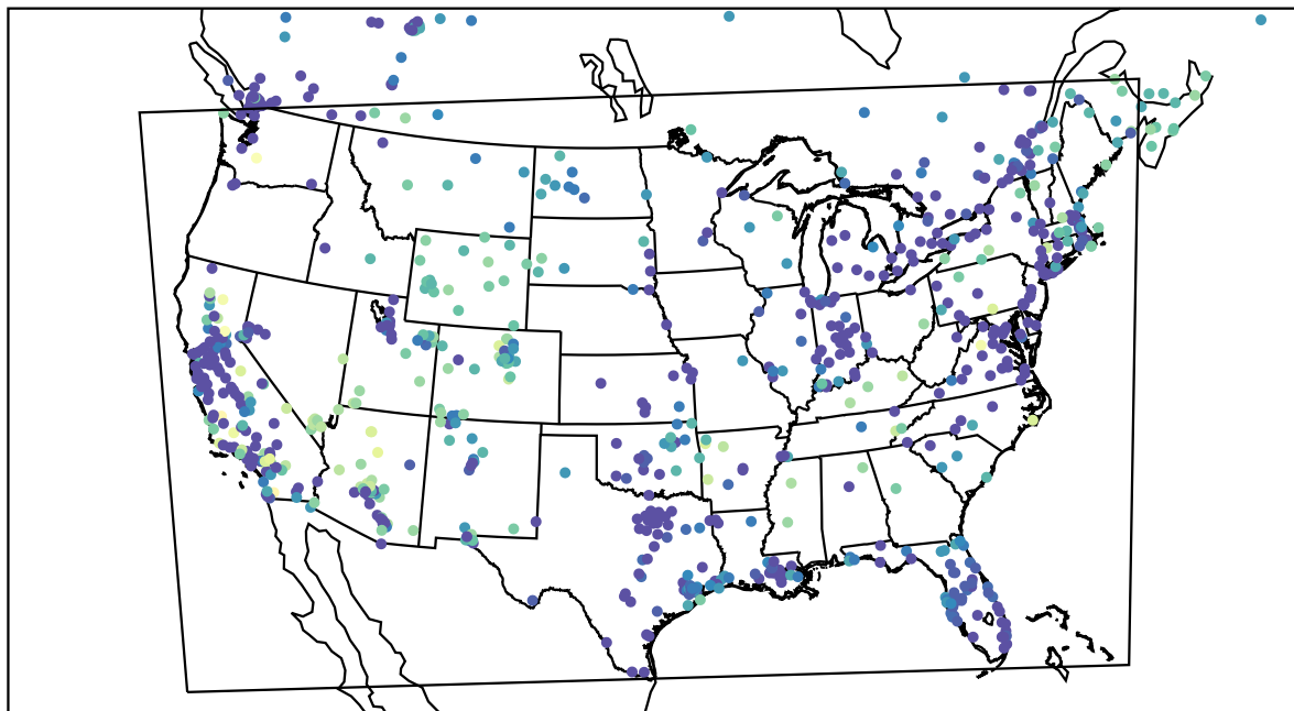
AirNOW (2022-11-24_09:00:00)
