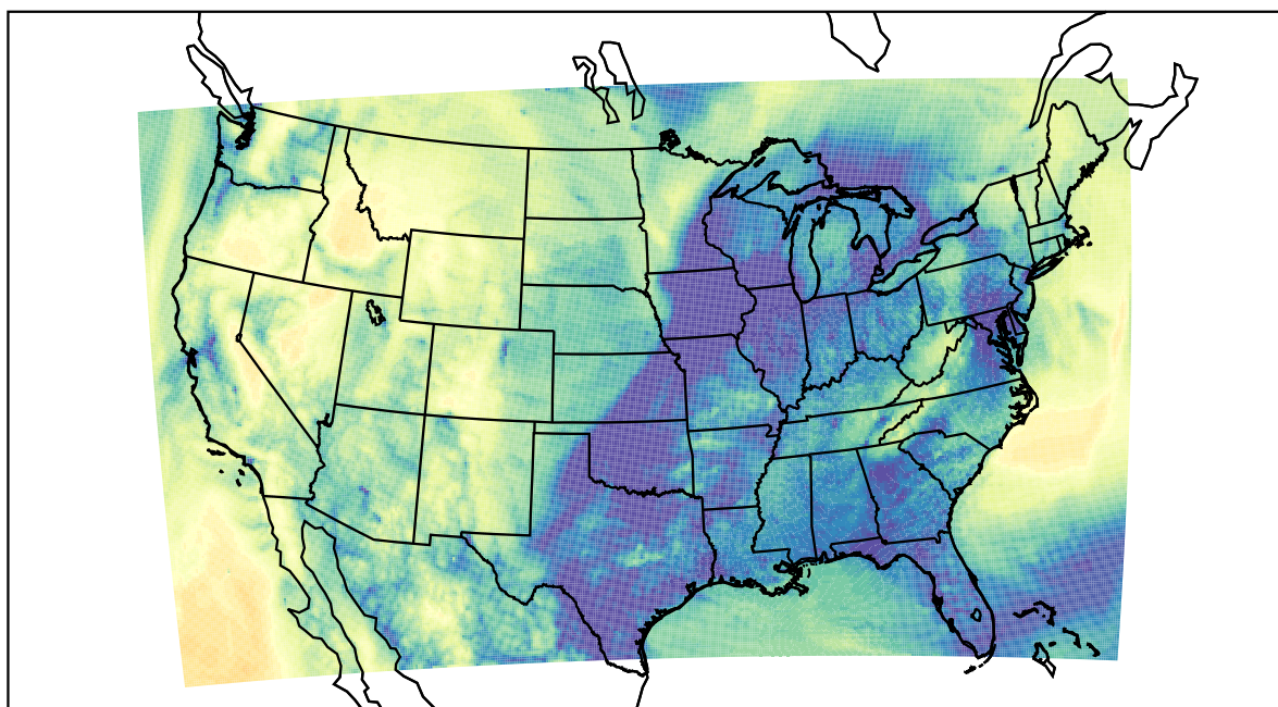
WRF (2022-11-24_15:00:00)
