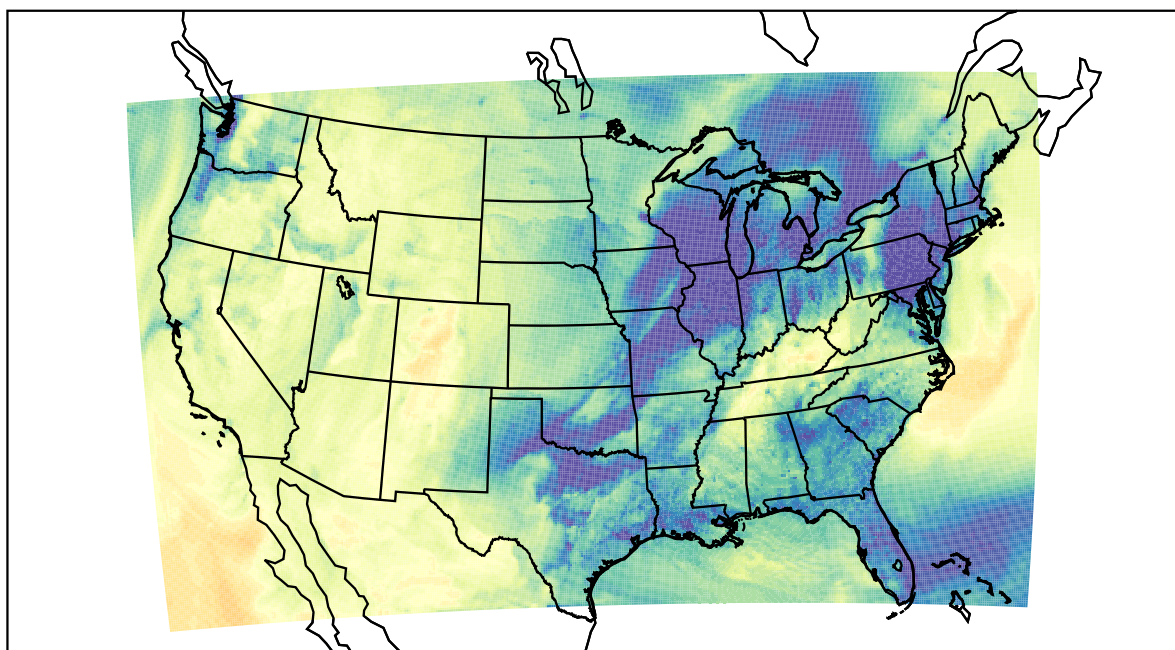
WRF (2022-11-24_22:00:00)
