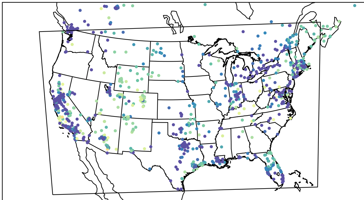
AirNOW (2022-11-24_02:00:00)
