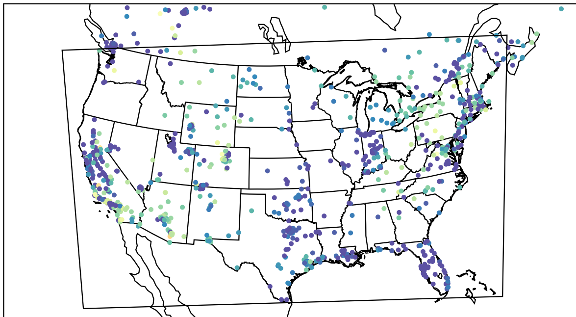
AirNOW (2022-11-25_06:00:00)
