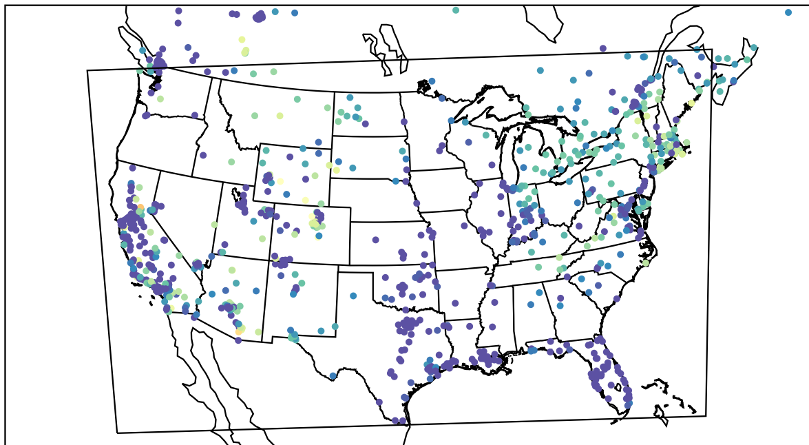
AirNOW (2022-11-25_14:00:00)
