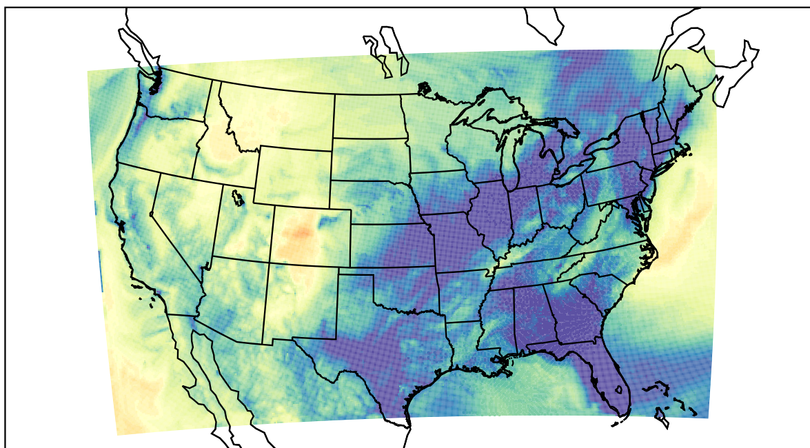
WRF (2022-11-25_07:00:00)
