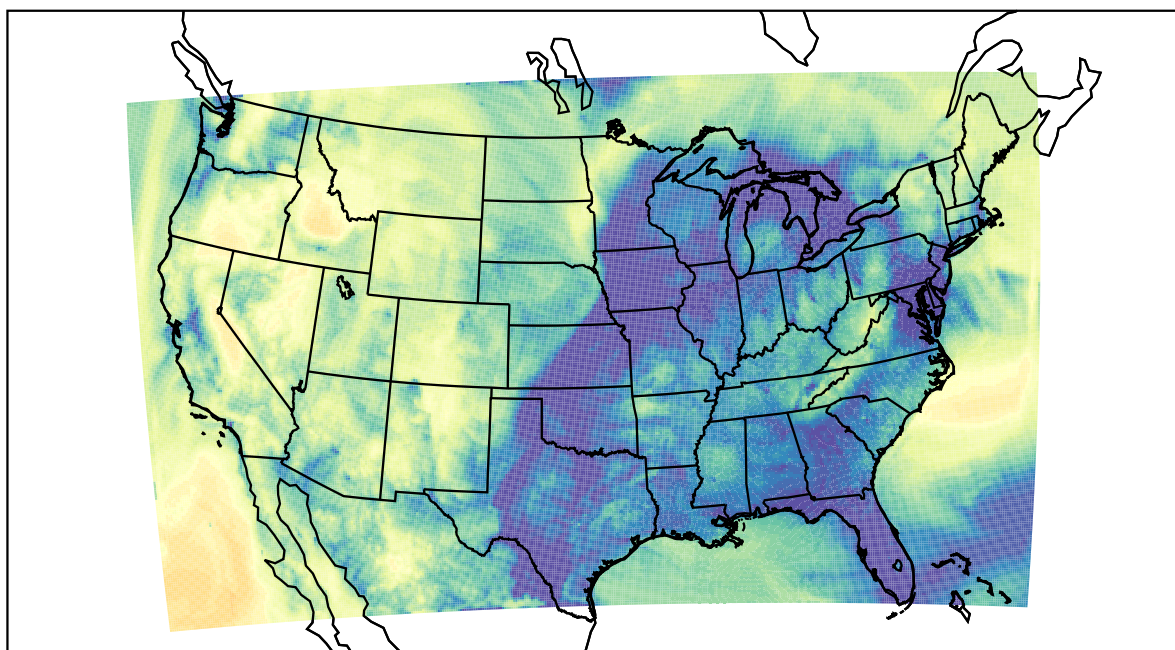
WRF (2022-11-24_11:00:00)
