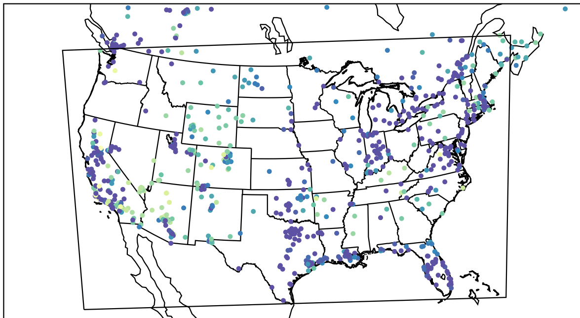
AirNOW (2022-11-24_11:00:00)
