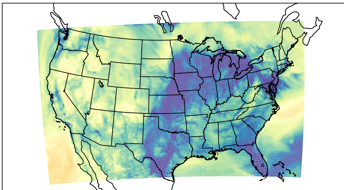
WRF (2022-11-24_06:00:00)
