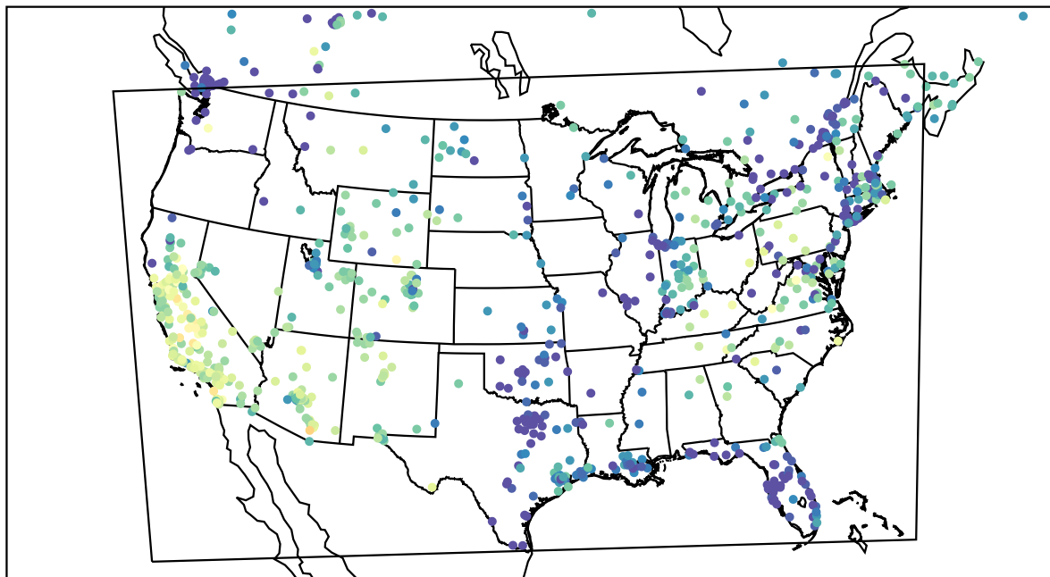
AirNOW (2022-11-25_00:00:00)
