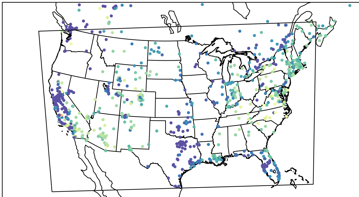
AirNOW (2022-11-24_16:00:00)
