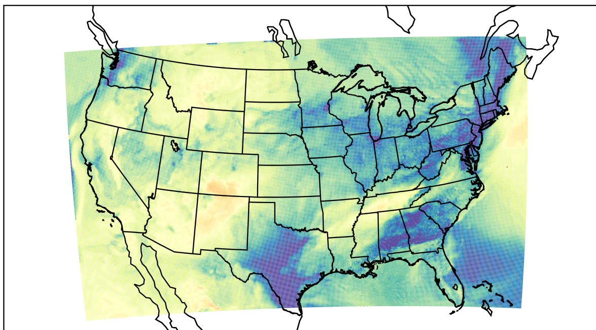
WRF (2022-11-25_21:00:00)
