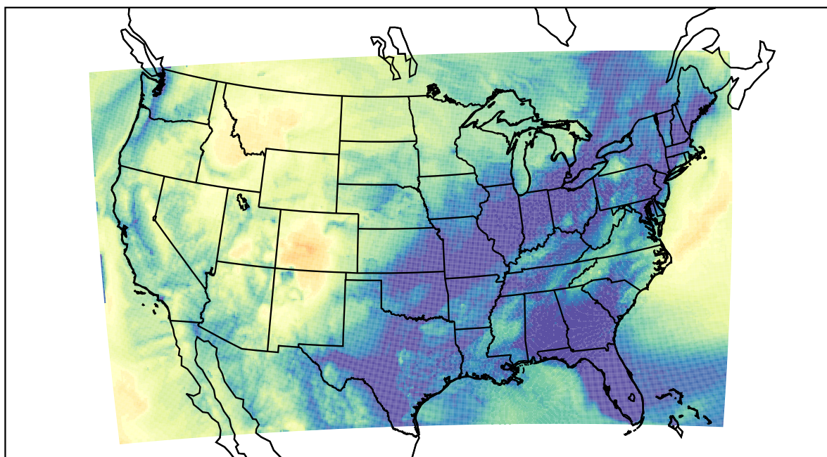
WRF (2022-11-25_11:00:00)
