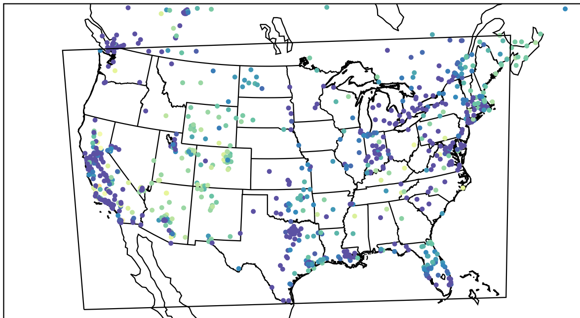
AirNOW (2022-11-24_04:00:00)
