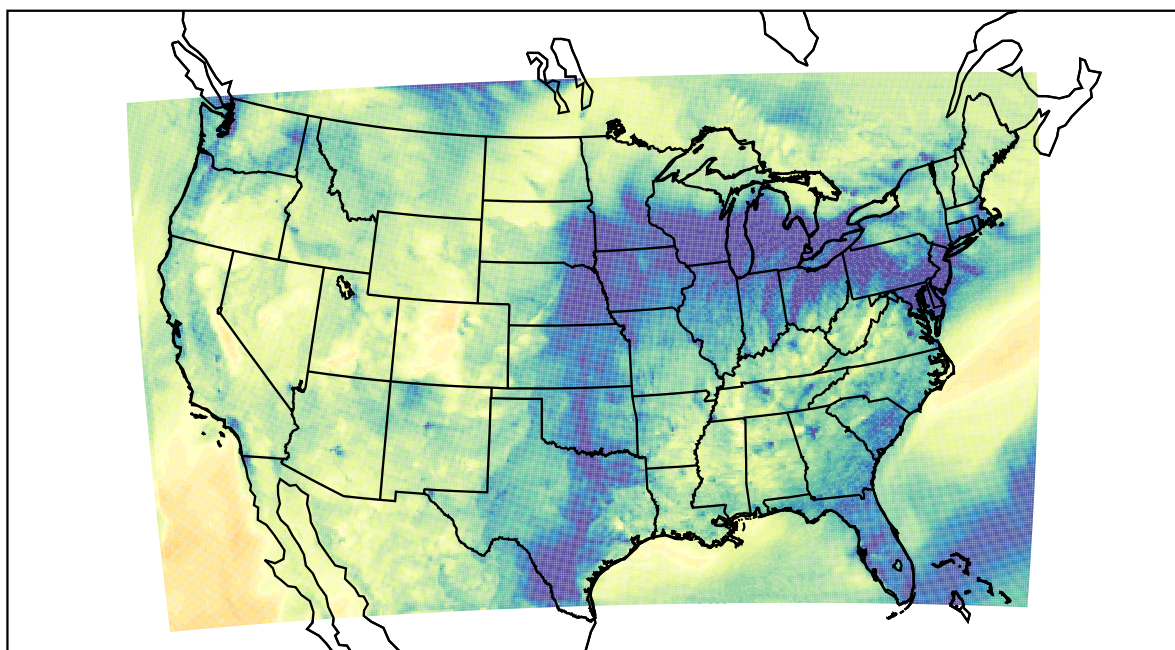
WRF (2022-11-24_00:00:00)
