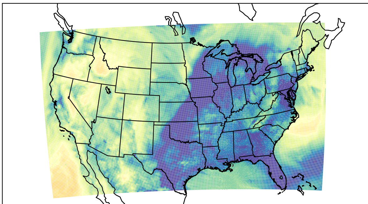
WRF (2022-11-24_13:00:00)
