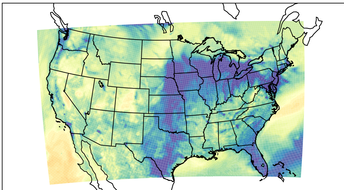
WRF (2022-11-24_02:00:00)
