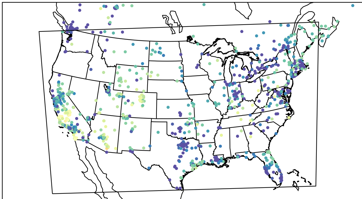
AirNOW (2022-11-24_00:00:00)
