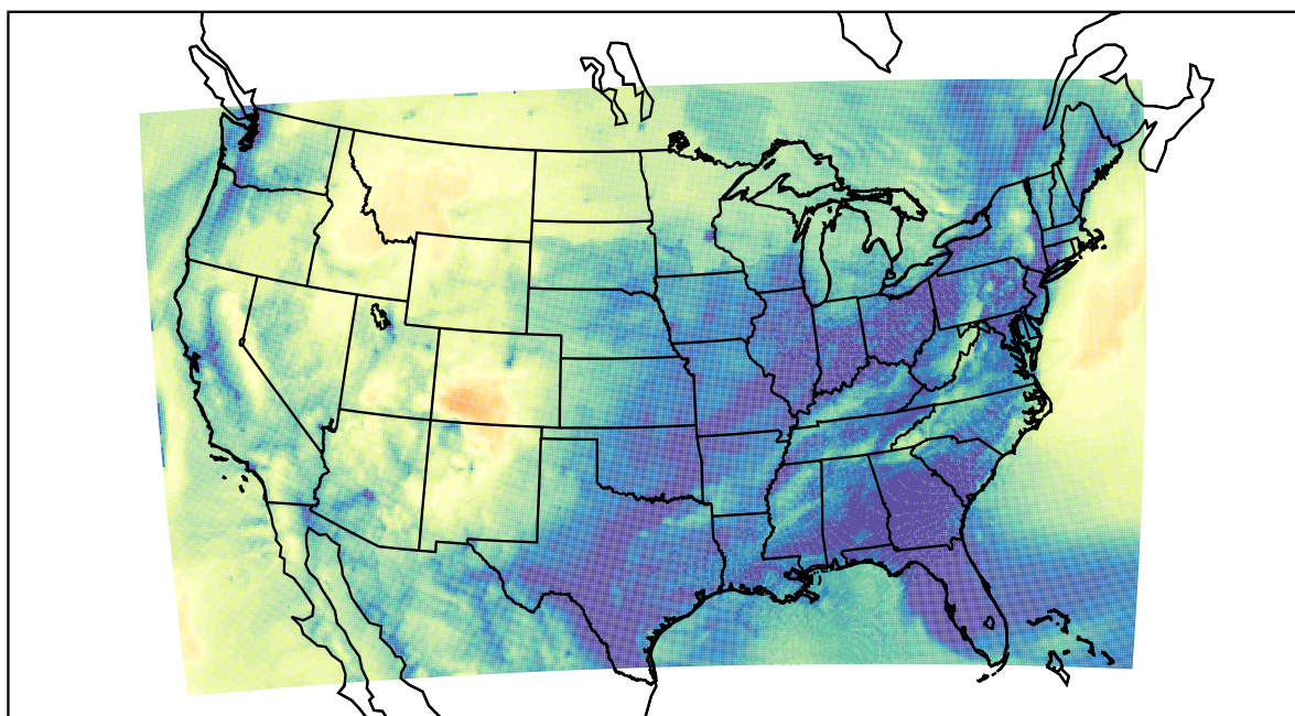
WRF (2022-11-25_15:00:00)
