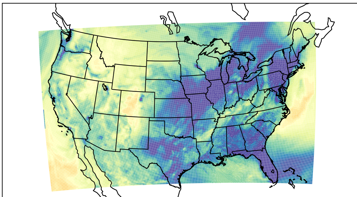
WRF (2022-11-25_03:00:00)
