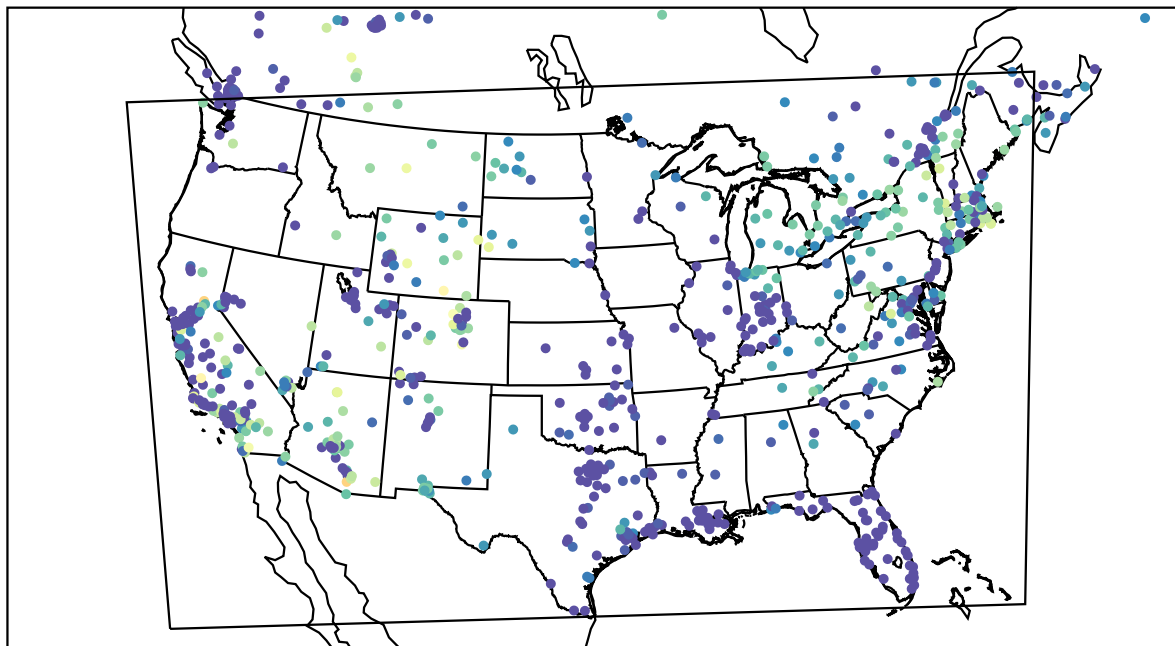
AirNOW (2022-11-25_12:00:00)
