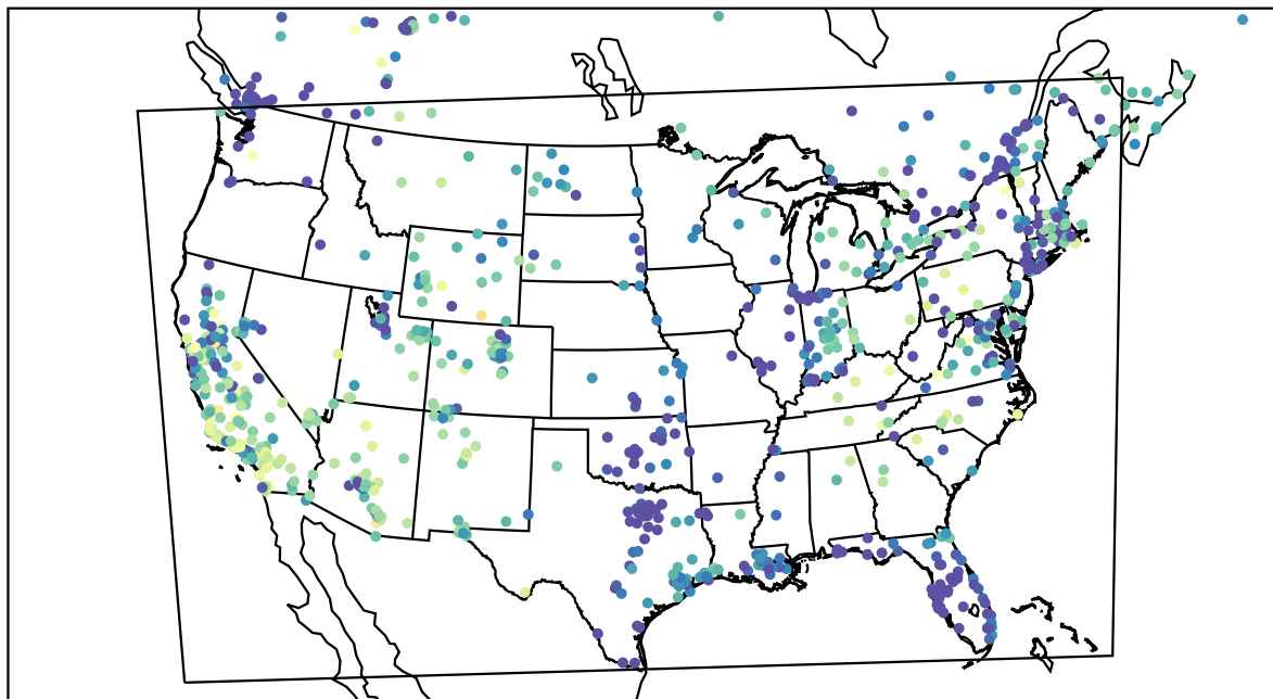
AirNOW (2022-11-25_01:00:00)
