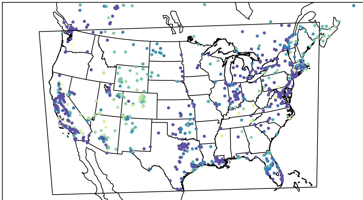
AirNOW (2022-11-24_06:00:00)
