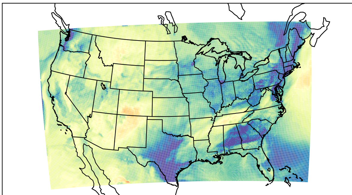
WRF (2022-11-25_20:00:00)
