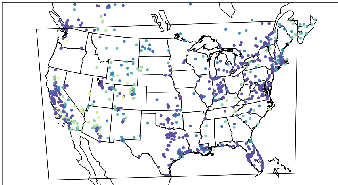
AirNOW (2022-11-24_13:00:00)
