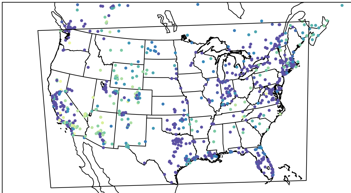
AirNOW (2022-11-24_12:00:00)
