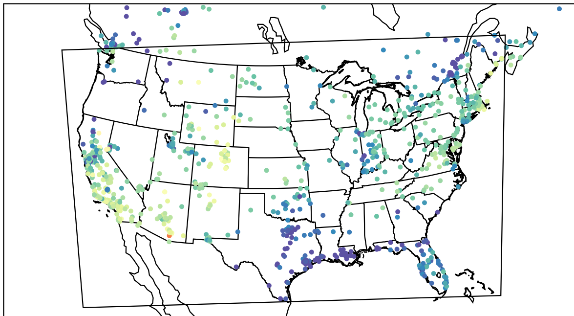
AirNOW (2022-11-25_19:00:00)
