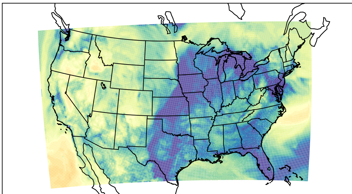
WRF (2022-11-24_08:00:00)
