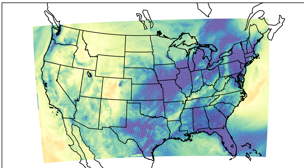
WRF (2022-11-25_04:00:00)
