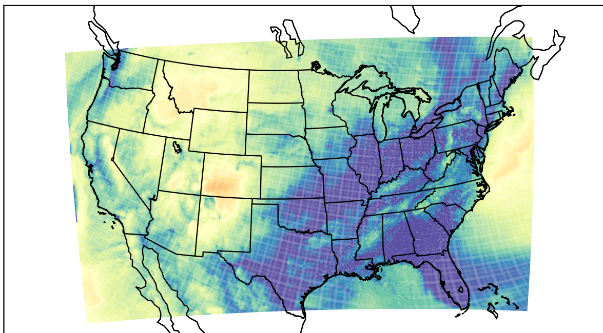
WRF (2022-11-25_13:00:00)
