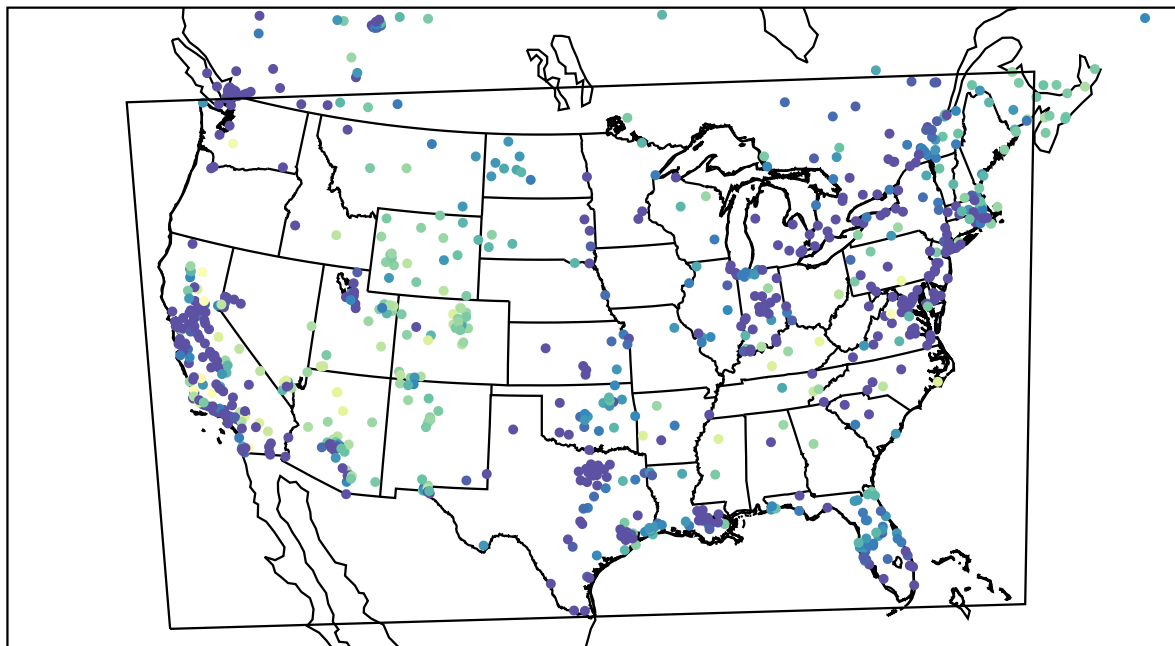
AirNOW (2022-11-24_05:00:00)
