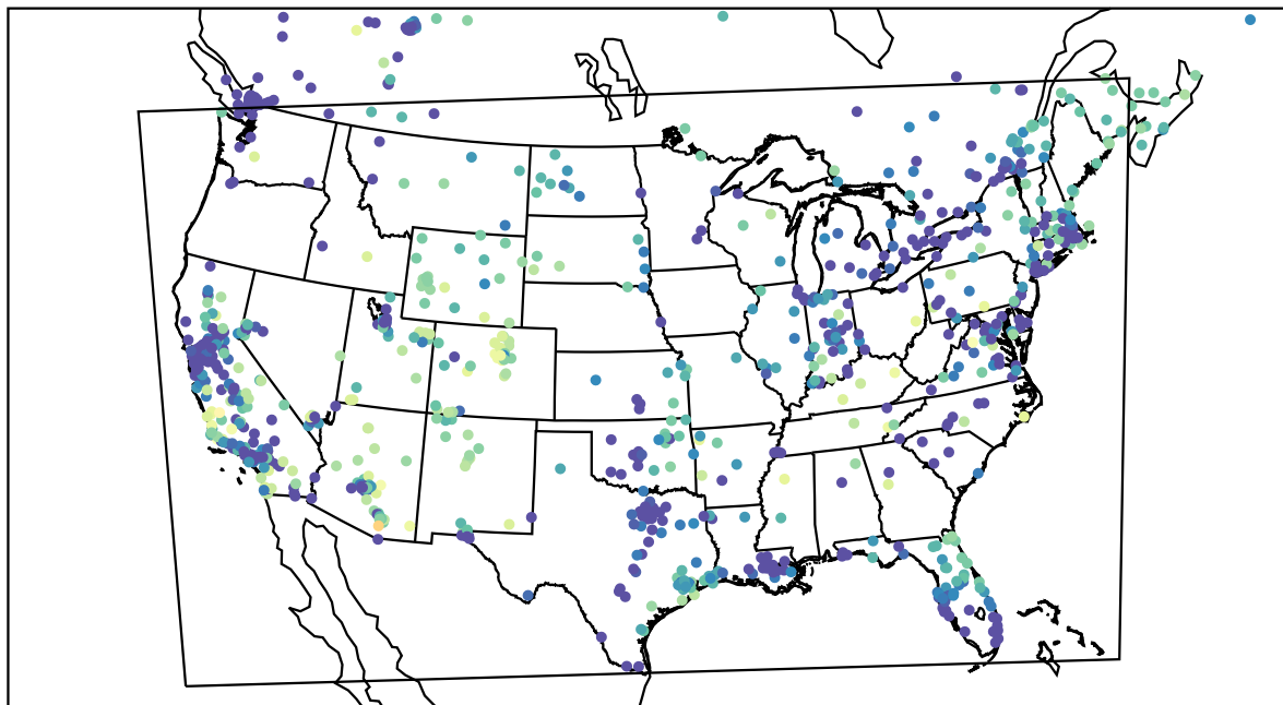
AirNOW (2022-11-24_01:00:00)
