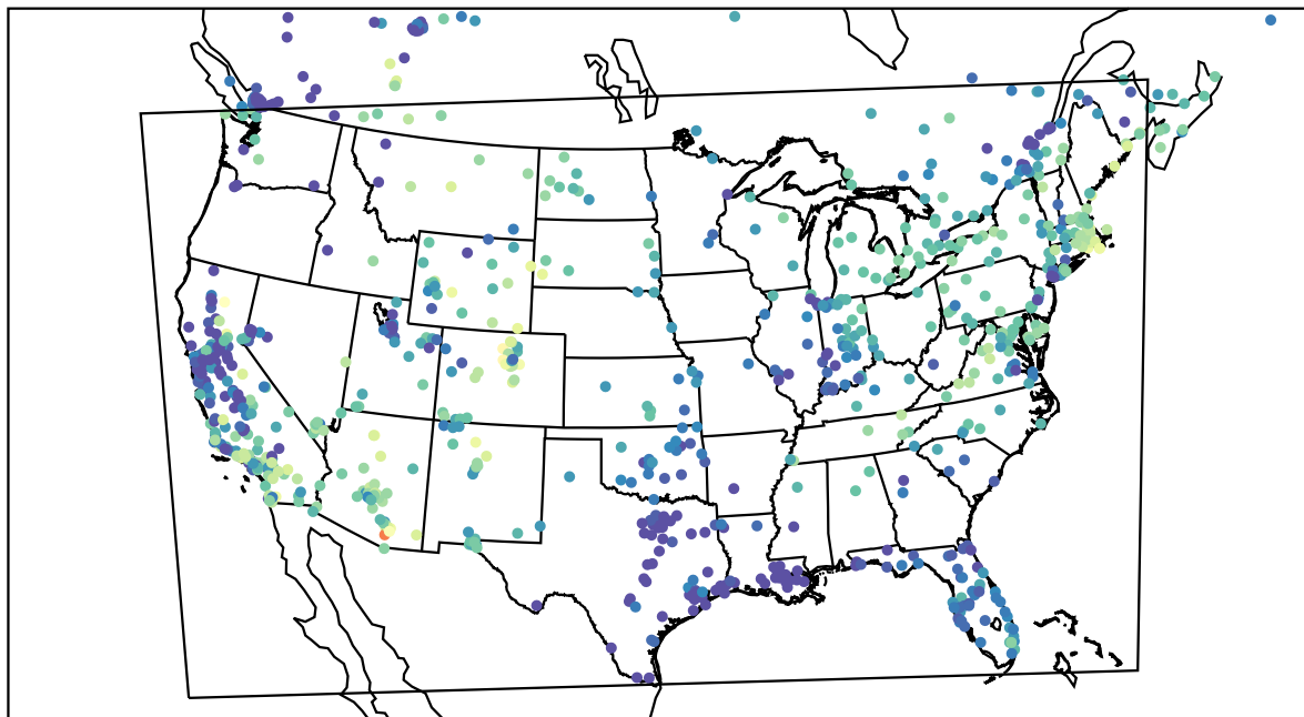
AirNOW (2022-11-25_17:00:00)
