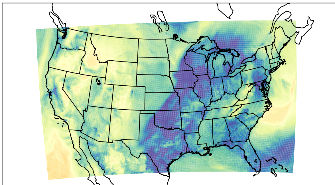
WRF (2022-11-24_16:00:00)
