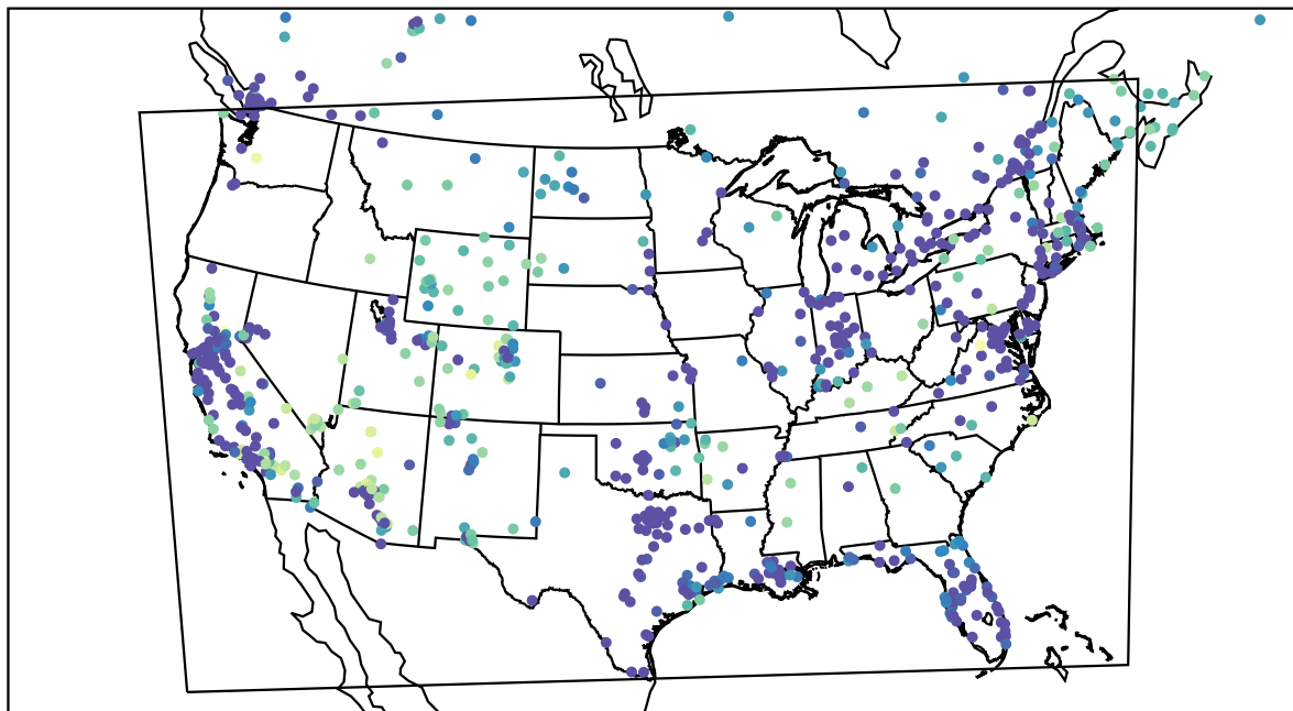
AirNOW (2022-11-24_10:00:00)
