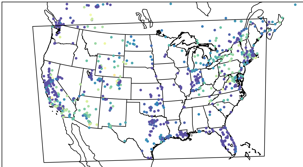
AirNOW (2022-11-25_08:00:00)
