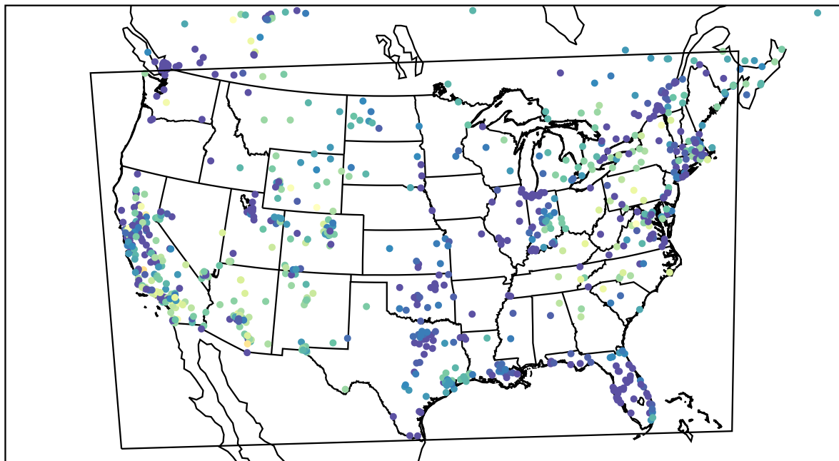
AirNOW (2022-11-25_03:00:00)
