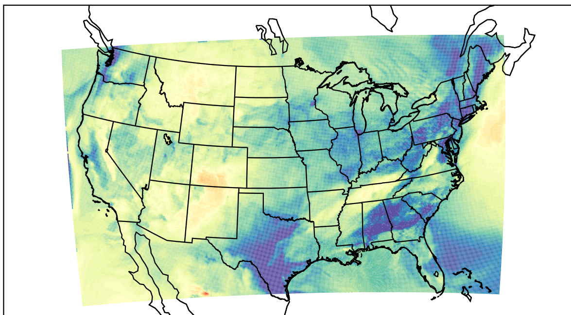
WRF (2022-11-25_19:00:00)
