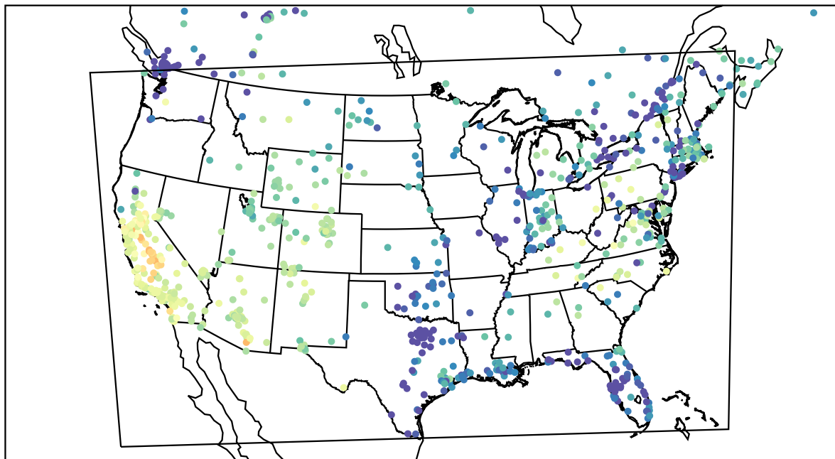
AirNOW (2022-11-24_23:00:00)
