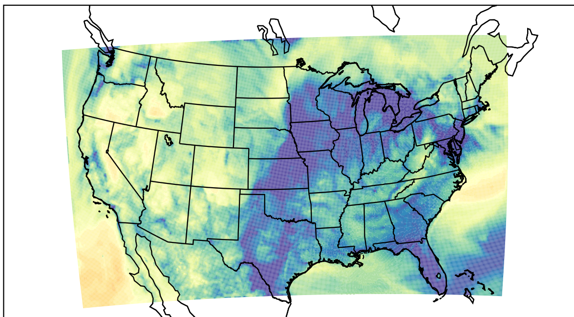
WRF (2022-11-24_07:00:00)
