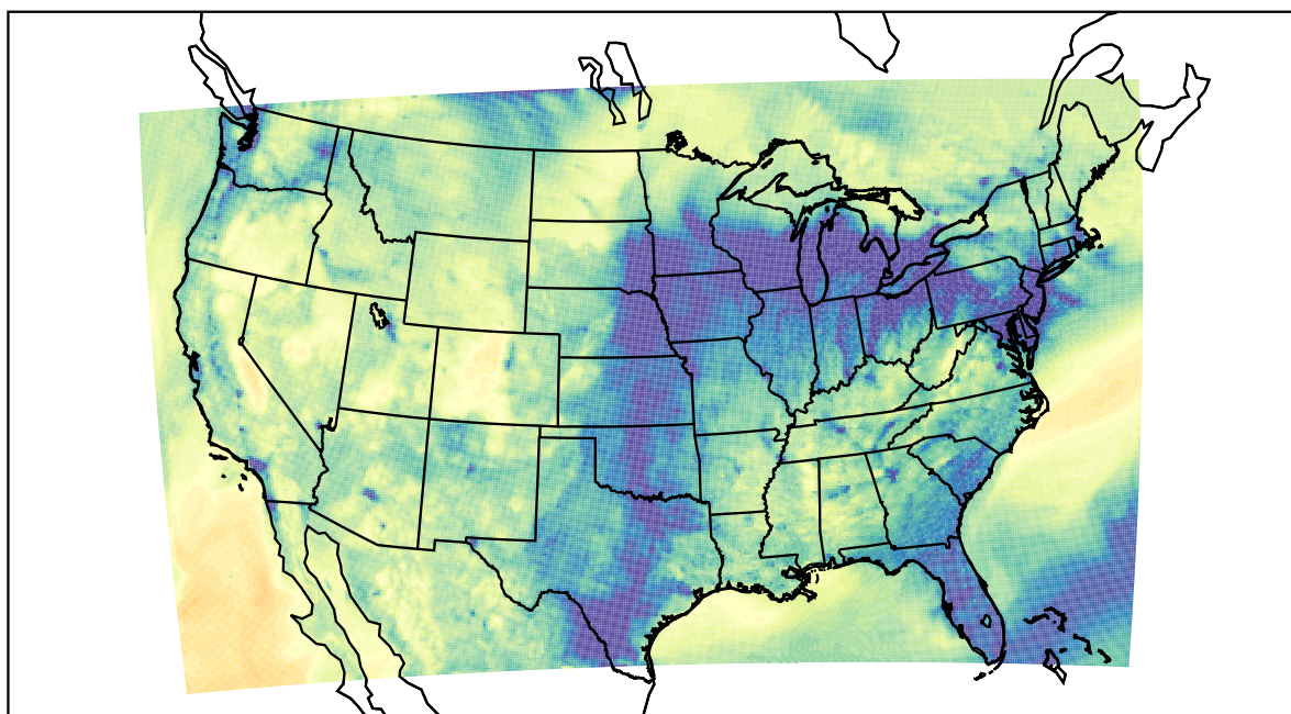
WRF (2022-11-24_01:00:00)
