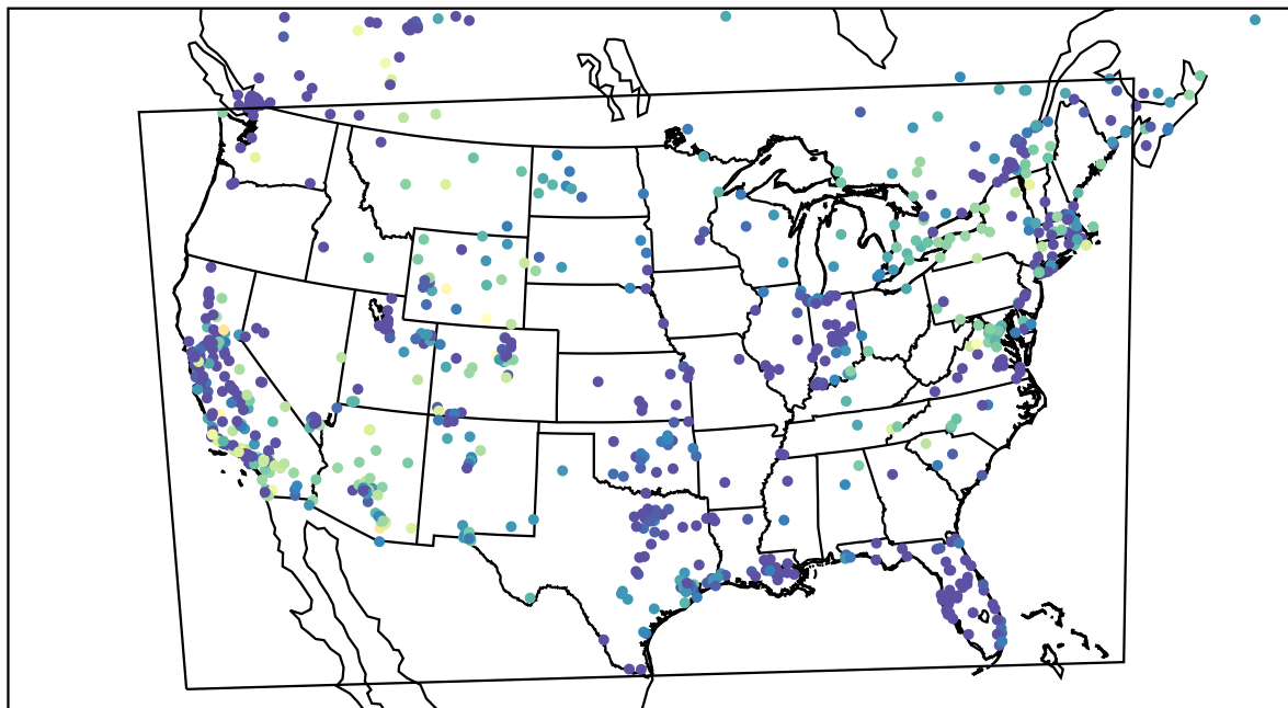
AirNOW (2022-11-25_07:00:00)
