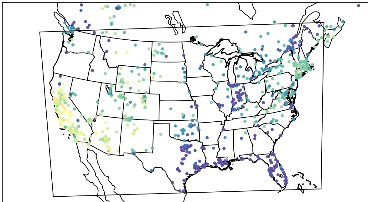
AirNOW (2022-11-25_23:00:00)
