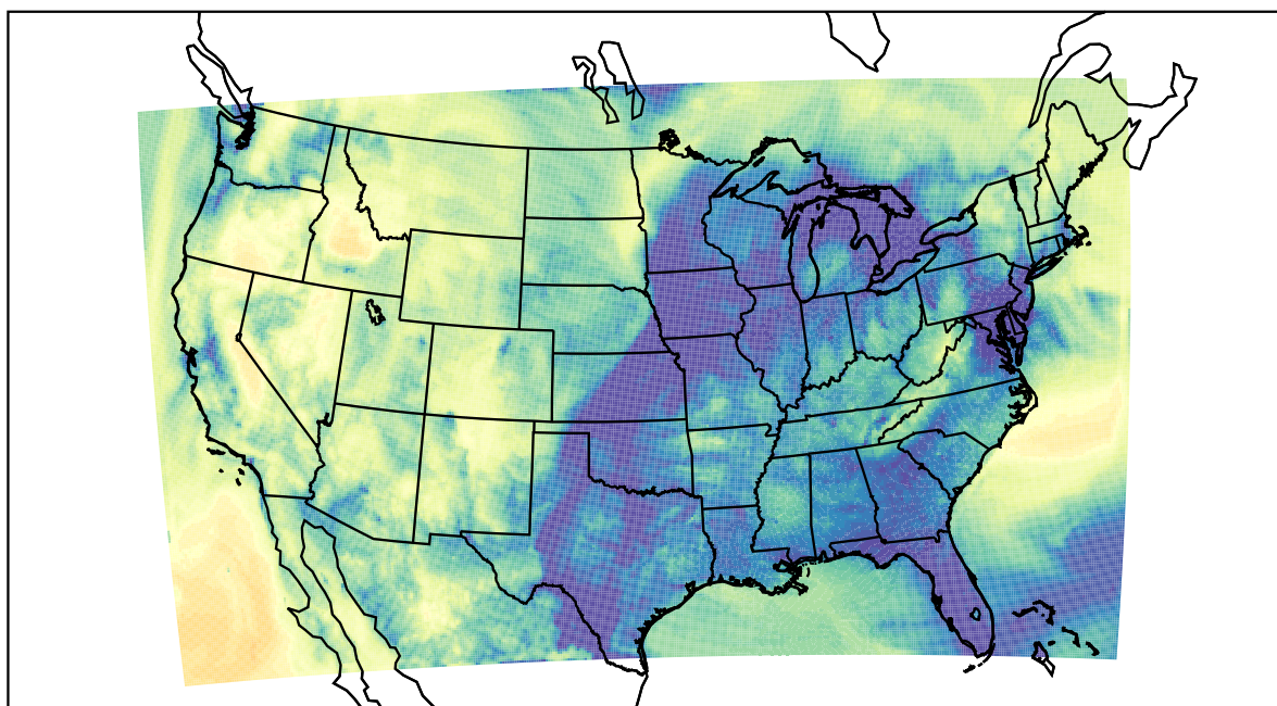
WRF (2022-11-24_10:00:00)
