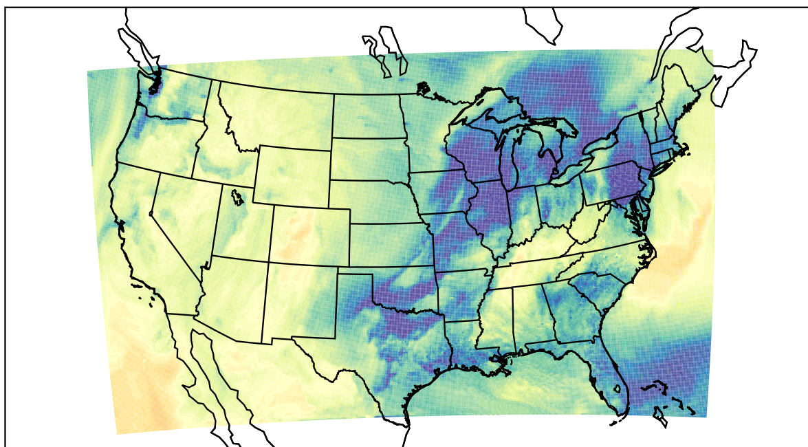
WRF (2022-11-24_21:00:00)
