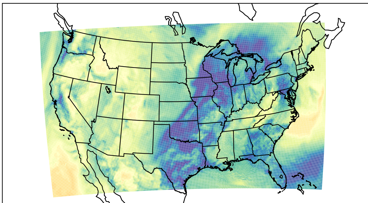
WRF (2022-11-24_17:00:00)
