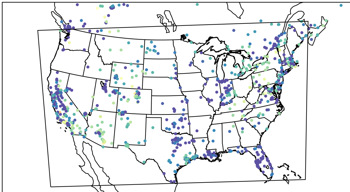
AirNOW (2022-11-25_05:00:00)
