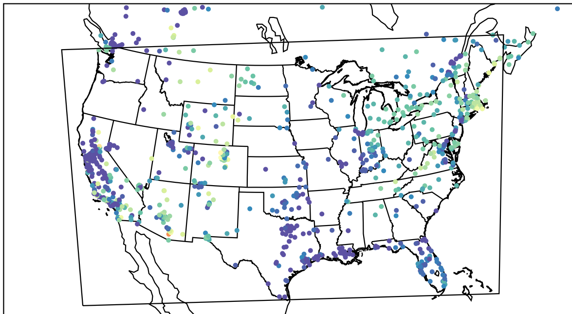
AirNOW (2022-11-25_16:00:00)
