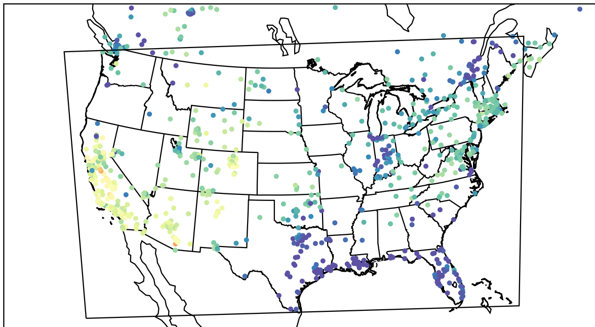
AirNOW (2022-11-25_22:00:00)
