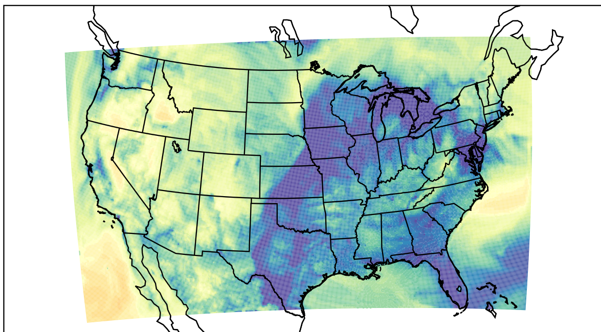
WRF (2022-11-24_09:00:00)
