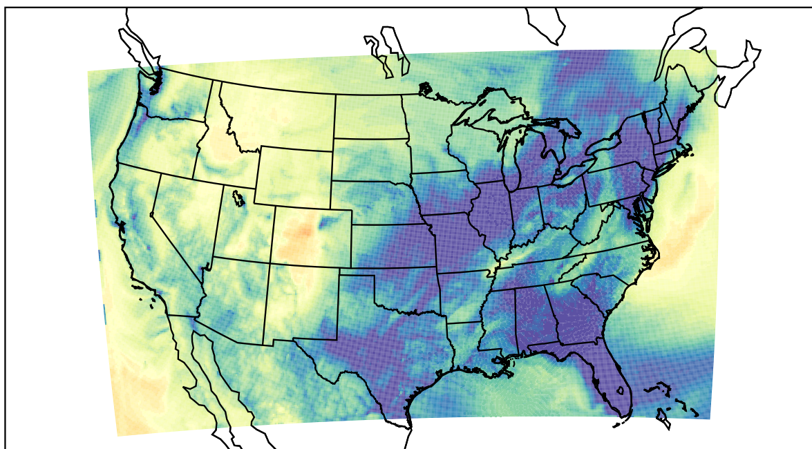
WRF (2022-11-25_06:00:00)
