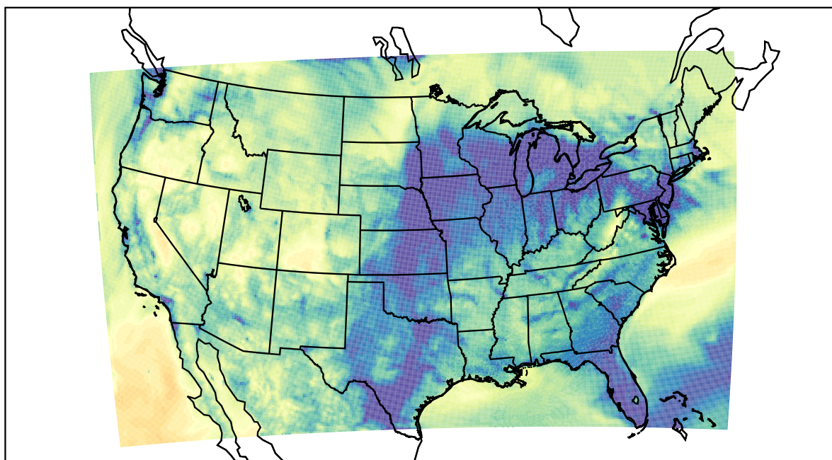
WRF (2022-11-24_04:00:00)
