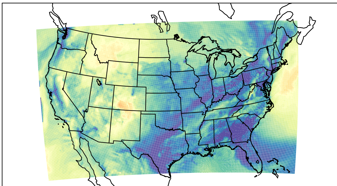
WRF (2022-11-25_16:00:00)
