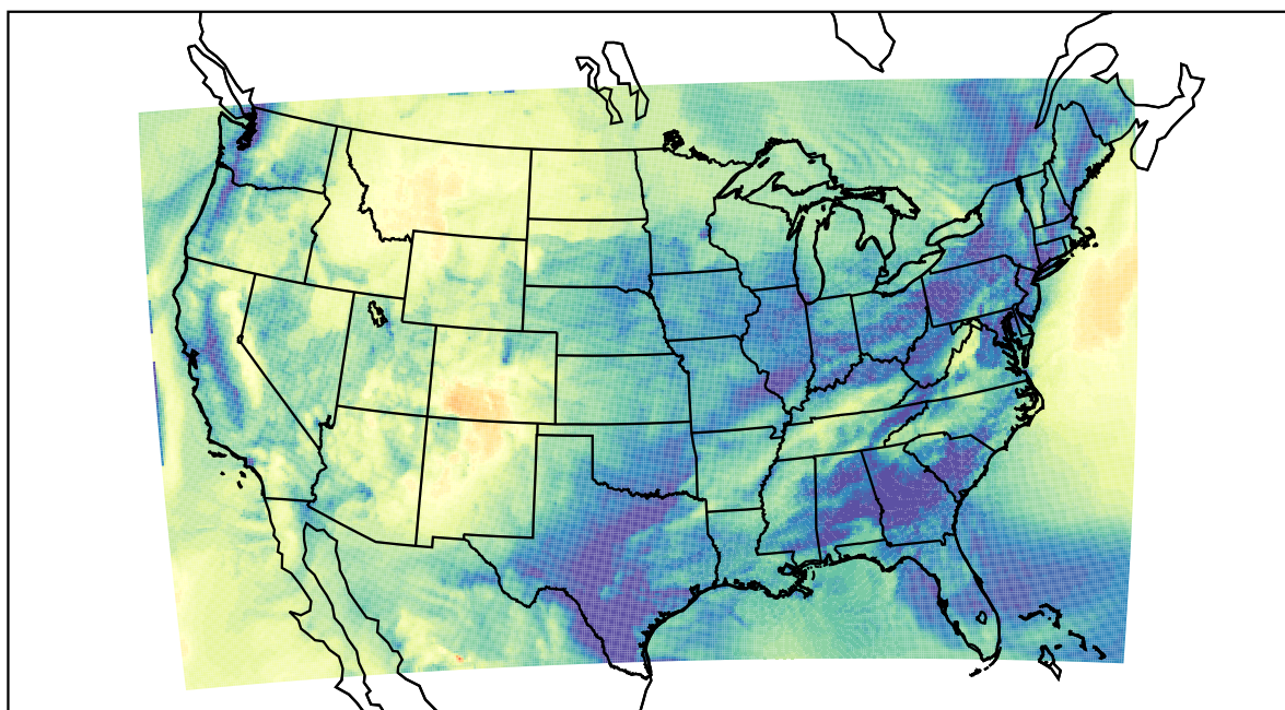
WRF (2022-11-25_17:00:00)
