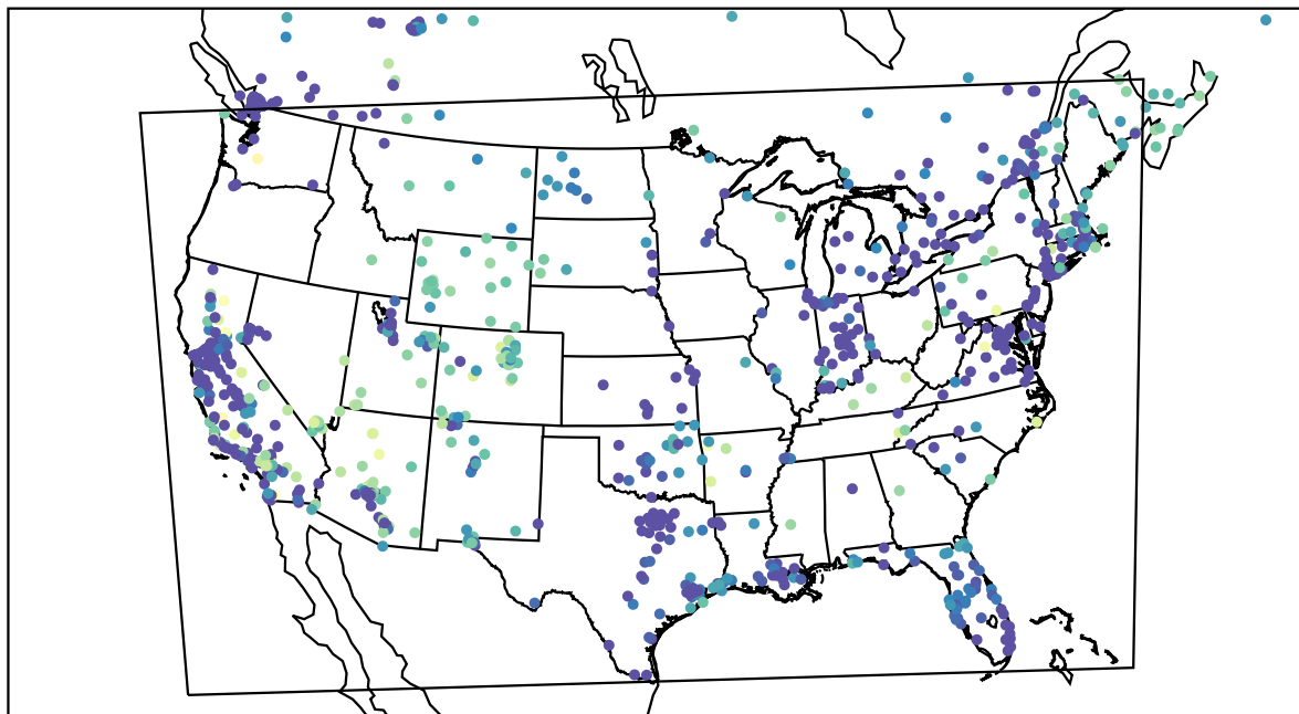
AirNOW (2022-11-24_08:00:00)
