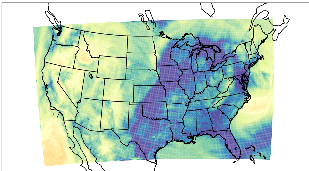
WRF (2022-11-24_12:00:00)
