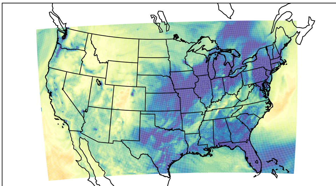
WRF (2022-11-25_02:00:00)
