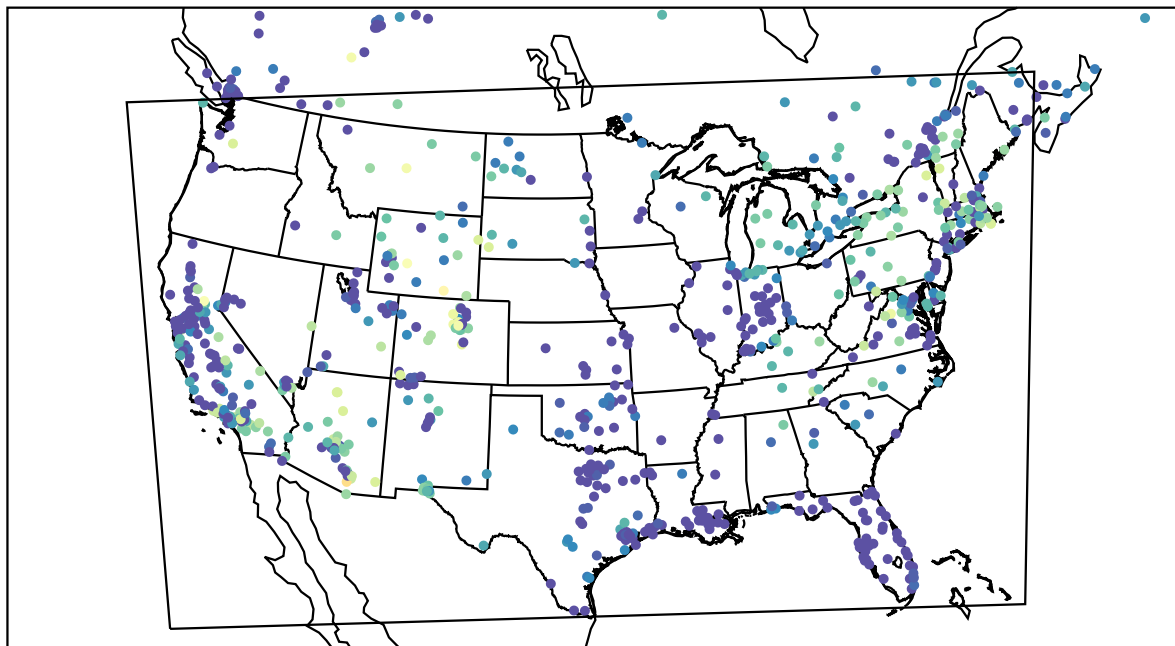
AirNOW (2022-11-25_10:00:00)
