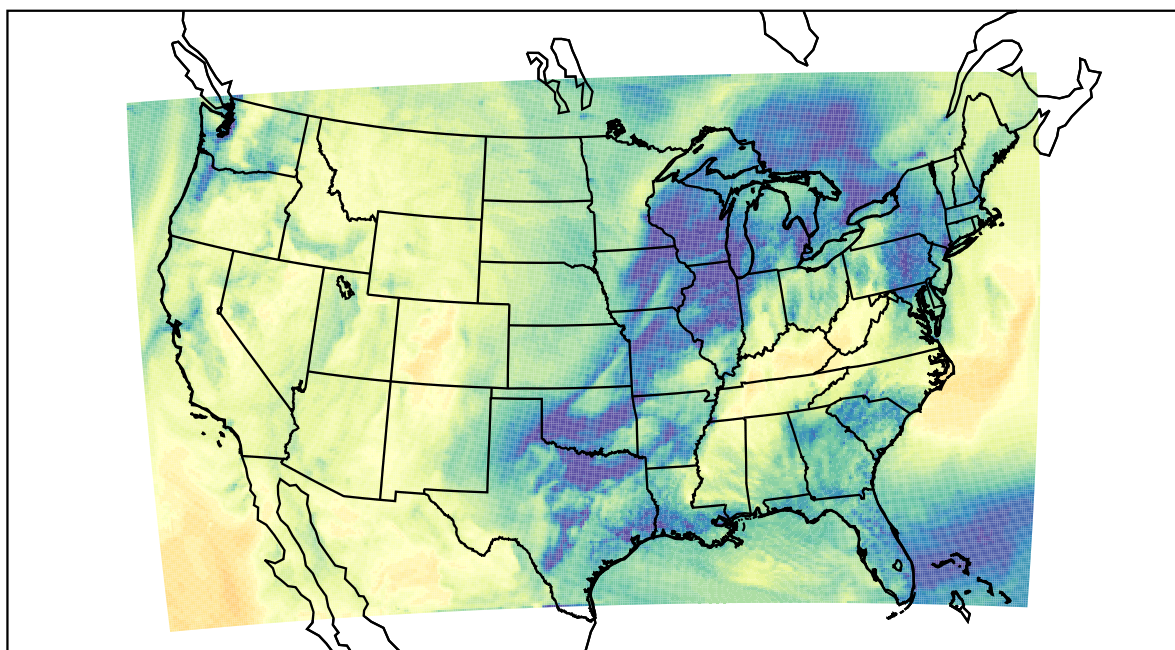
WRF (2022-11-24_20:00:00)
