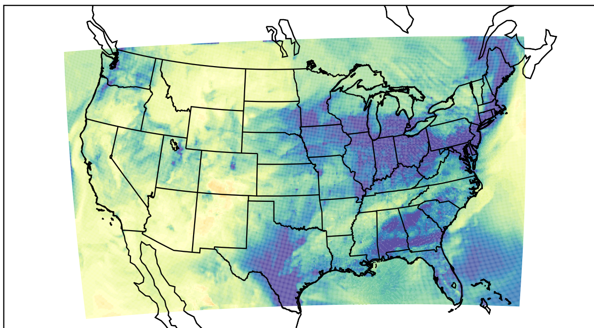
WRF (2022-11-25_23:00:00)
