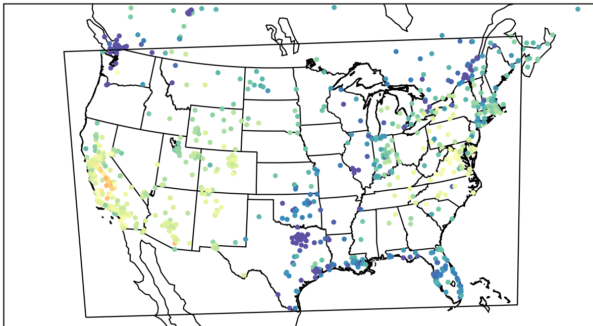
AirNOW (2022-11-24_21:00:00)
