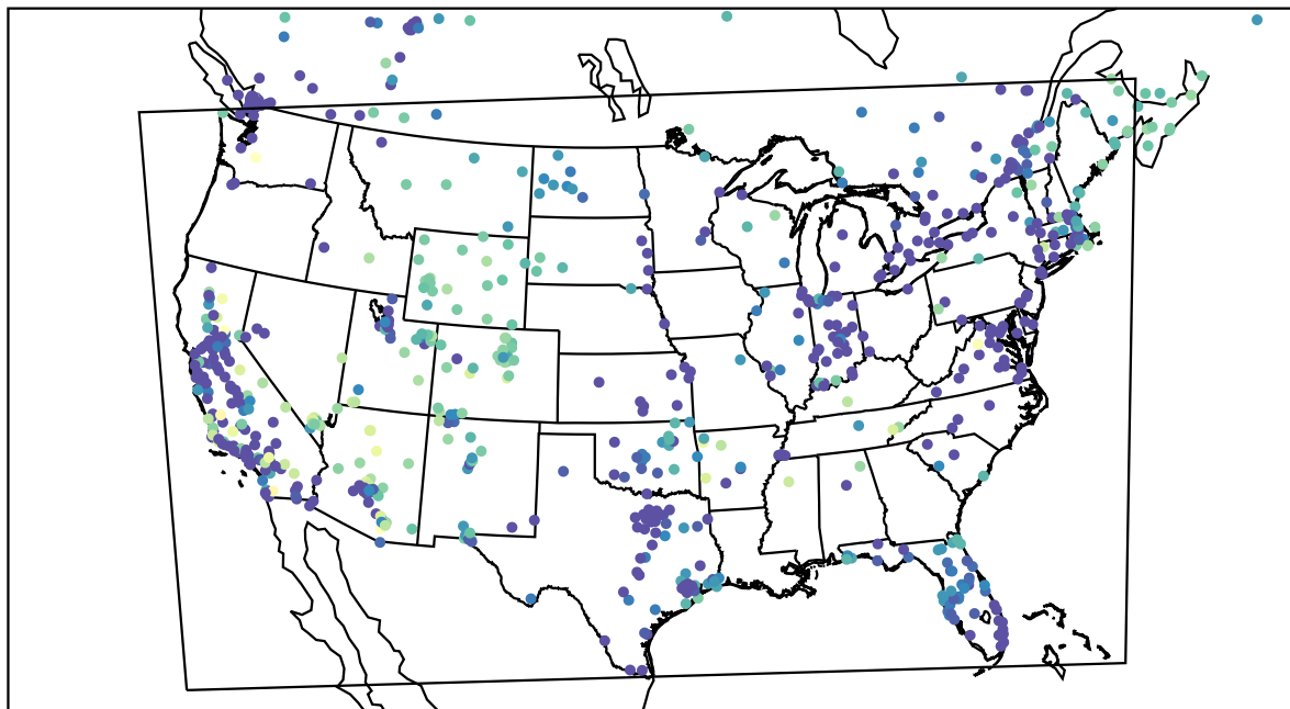
AirNOW (2022-11-24_07:00:00)
