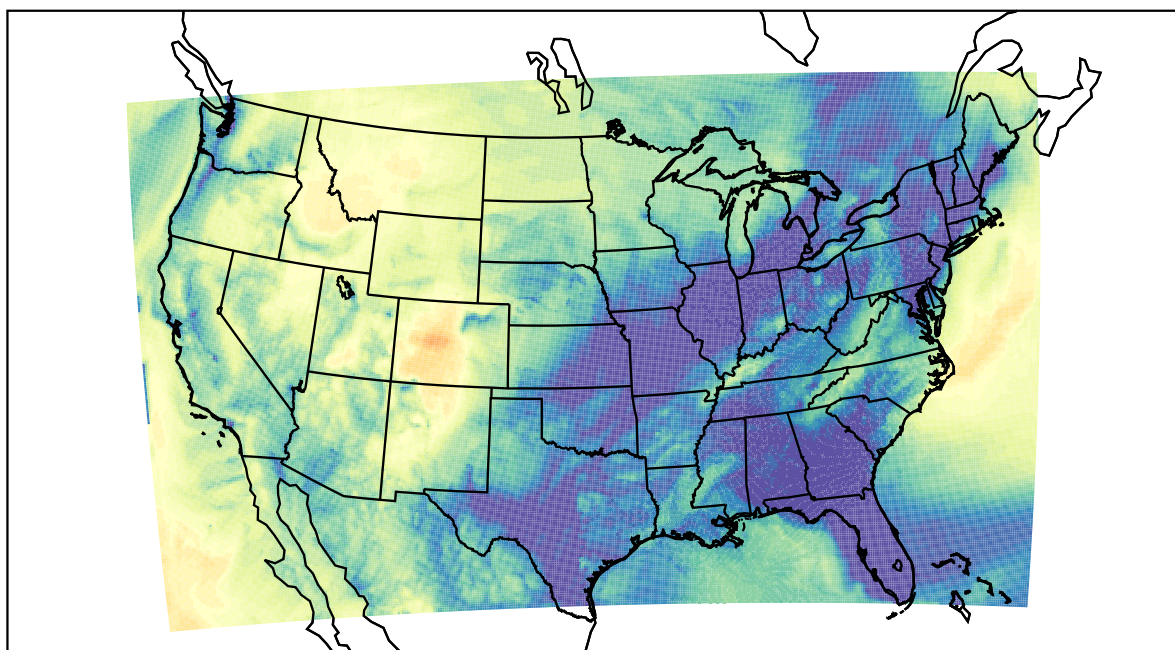
WRF (2022-11-25_08:00:00)
