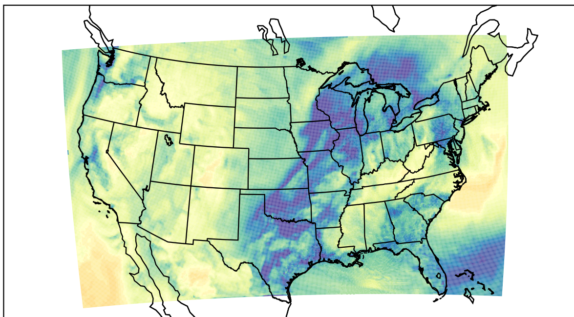
WRF (2022-11-24_18:00:00)
