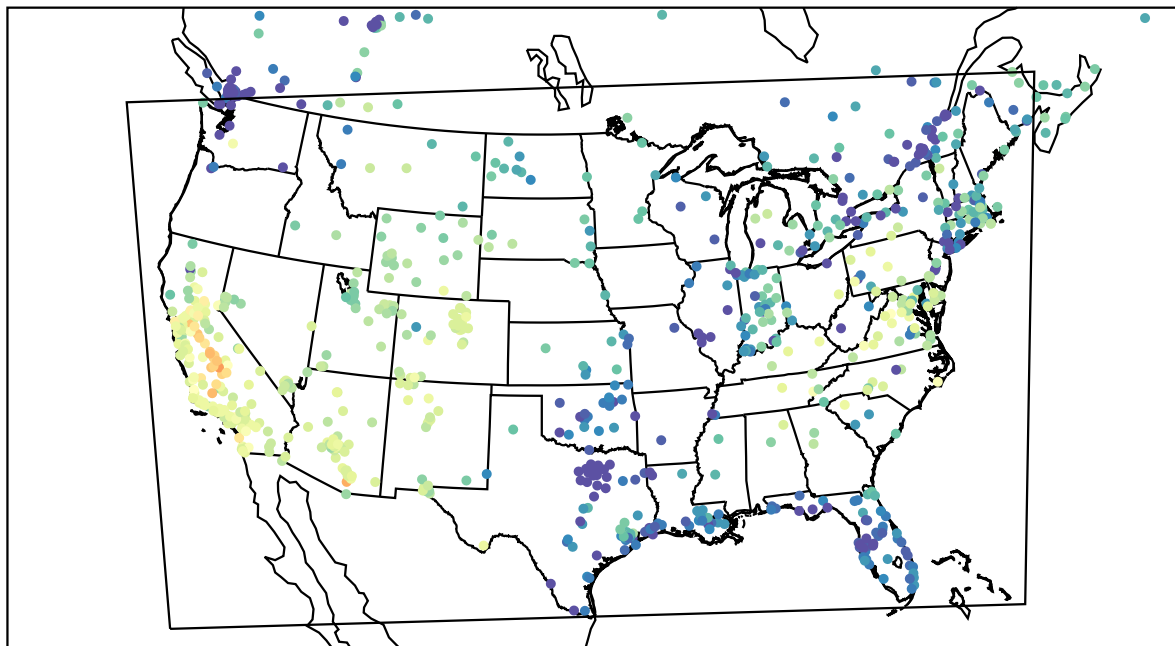
AirNOW (2022-11-24_22:00:00)
