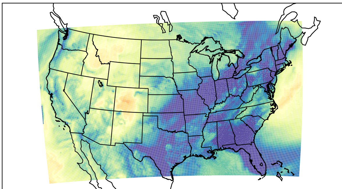
WRF (2022-11-25_10:00:00)
