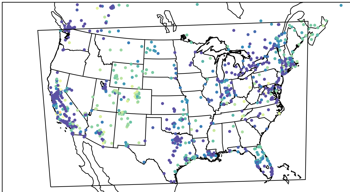
AirNOW (2022-11-24_03:00:00)
