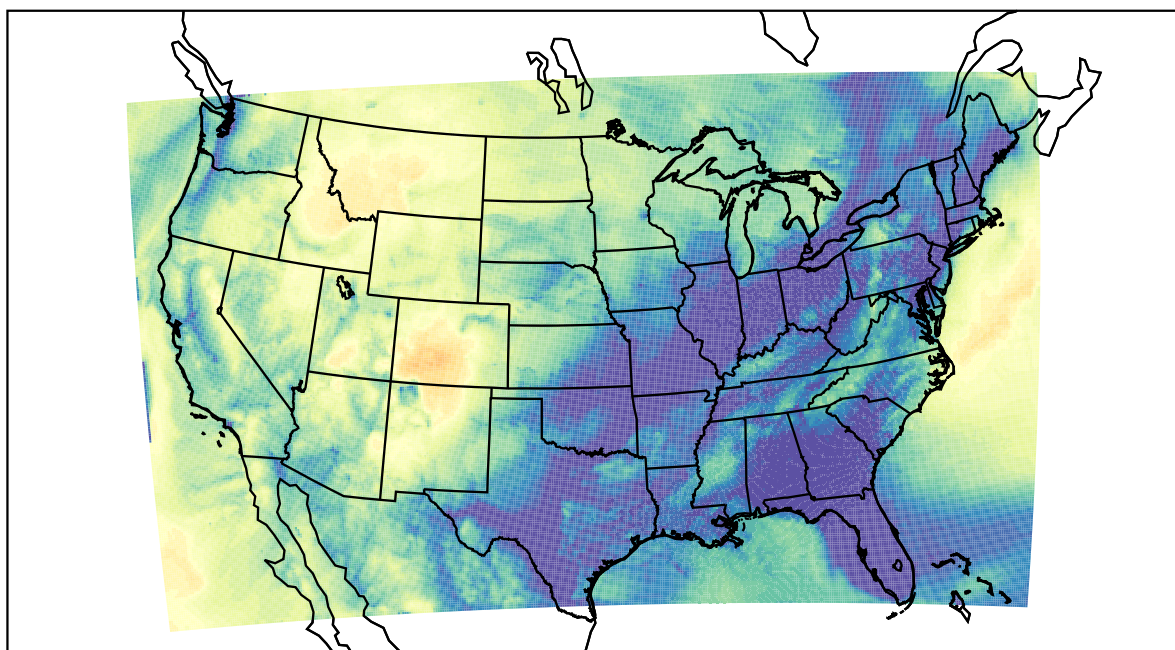
WRF (2022-11-25_12:00:00)
