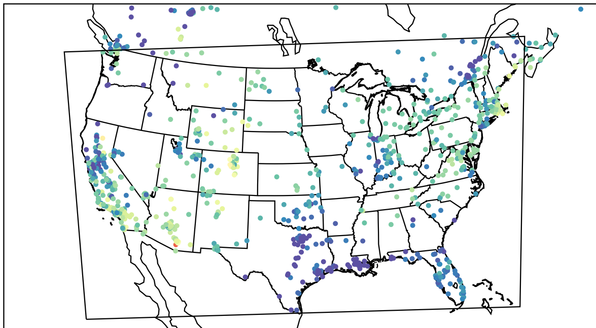
AirNOW (2022-11-25_18:00:00)
