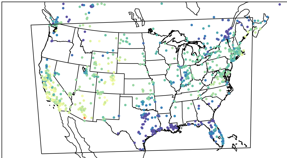
AirNOW (2022-11-25_20:00:00)
