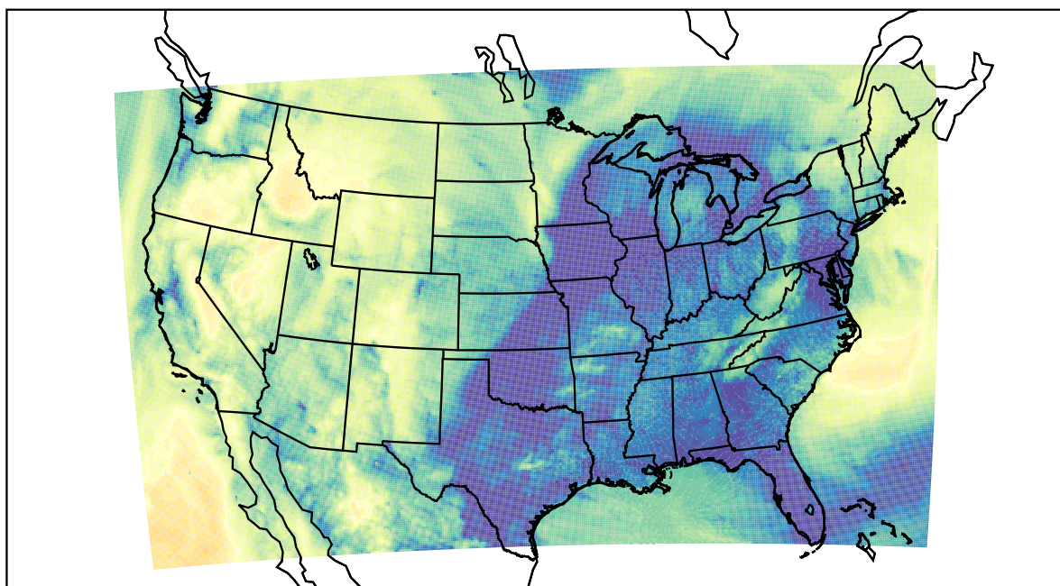
WRF (2022-11-24_14:00:00)
