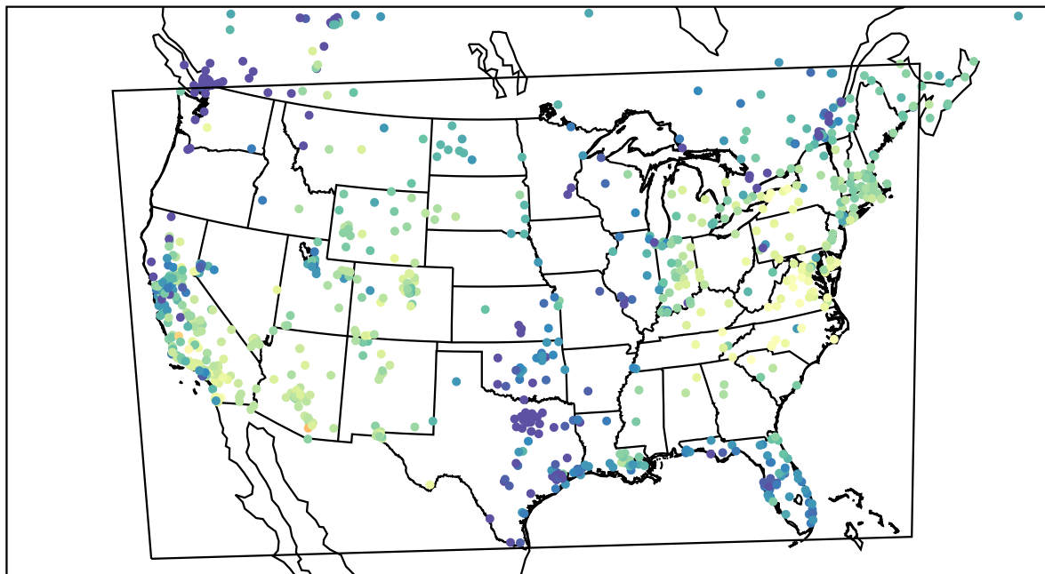
AirNOW (2022-11-24_18:00:00)
