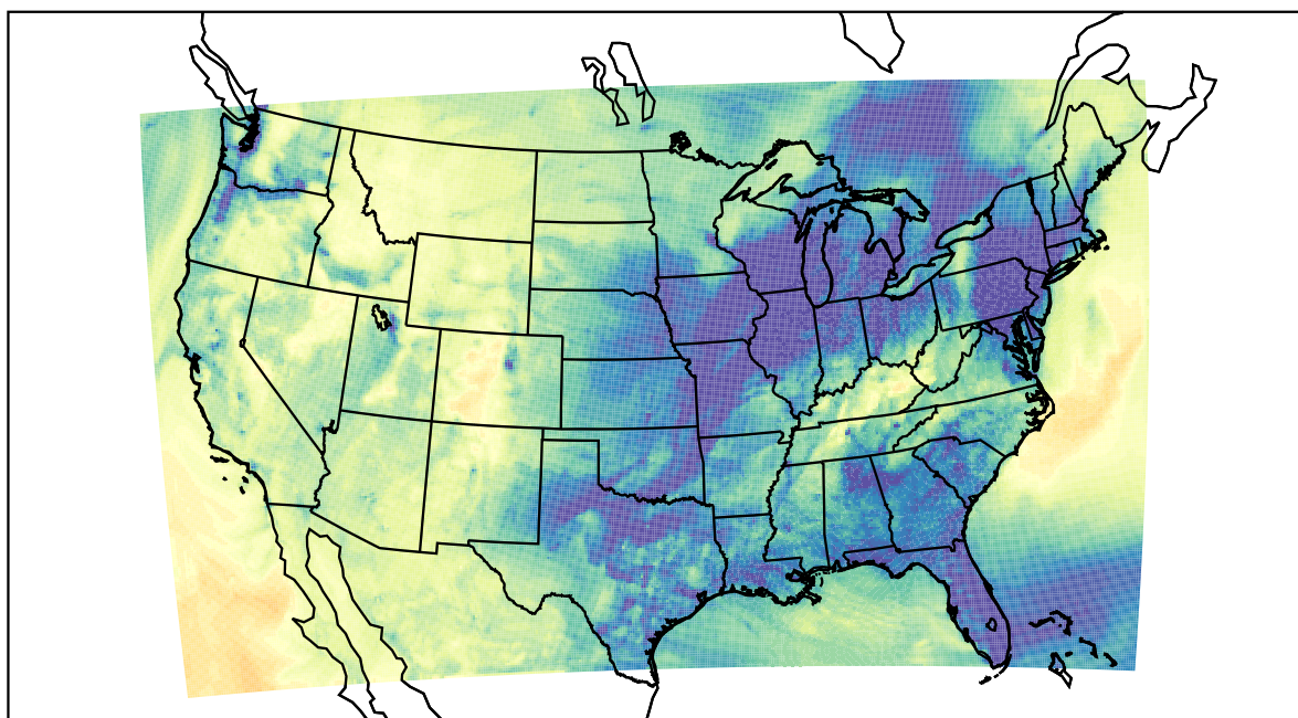
WRF (2022-11-25_00:00:00)
