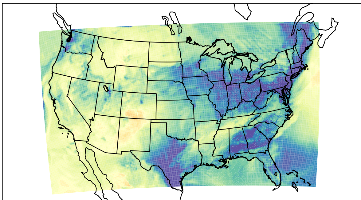
WRF (2022-11-25_22:00:00)
