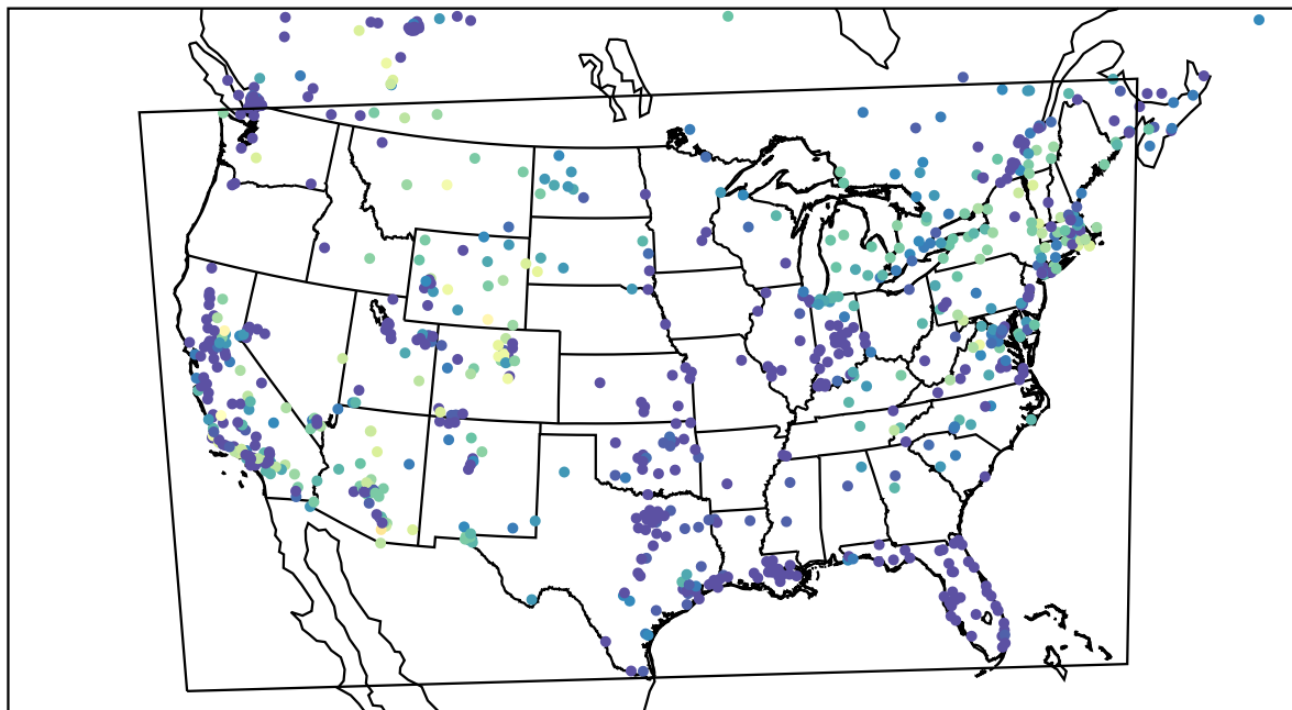
AirNOW (2022-11-25_11:00:00)
