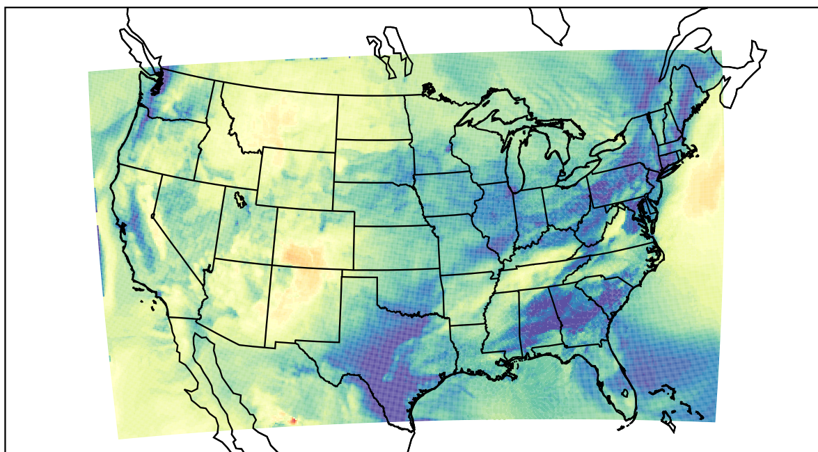
WRF (2022-11-25_18:00:00)
