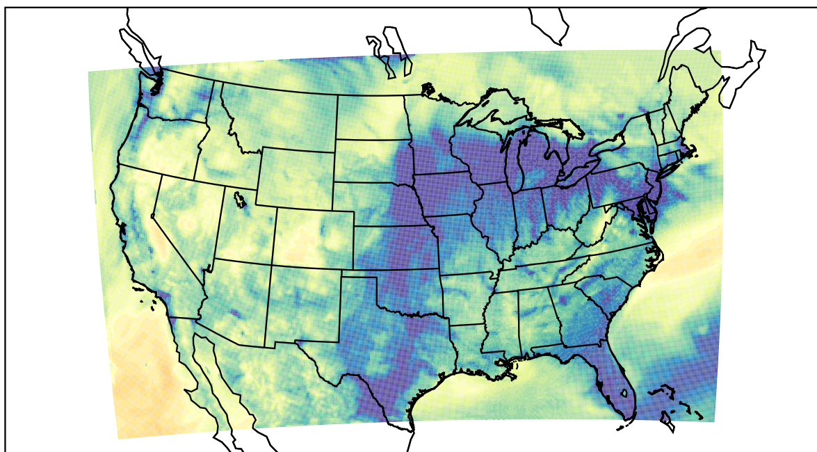
WRF (2022-11-24_03:00:00)
