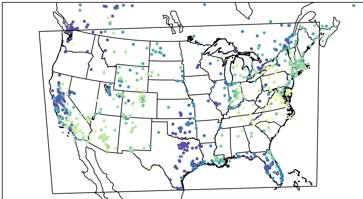
AirNOW (2022-11-24_17:00:00)
