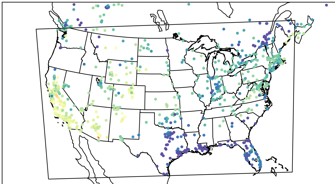
AirNOW (2022-11-25_21:00:00)
