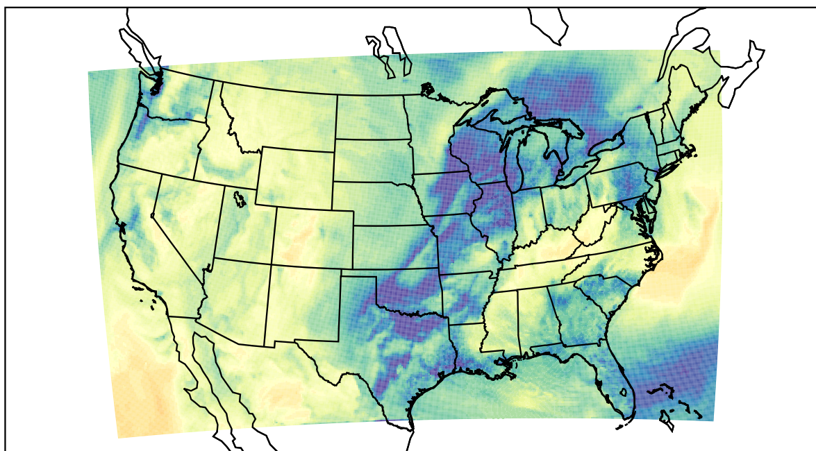
WRF (2022-11-24_19:00:00)
