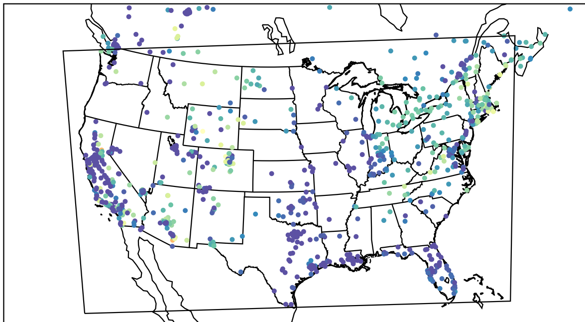
AirNOW (2022-11-25_15:00:00)
