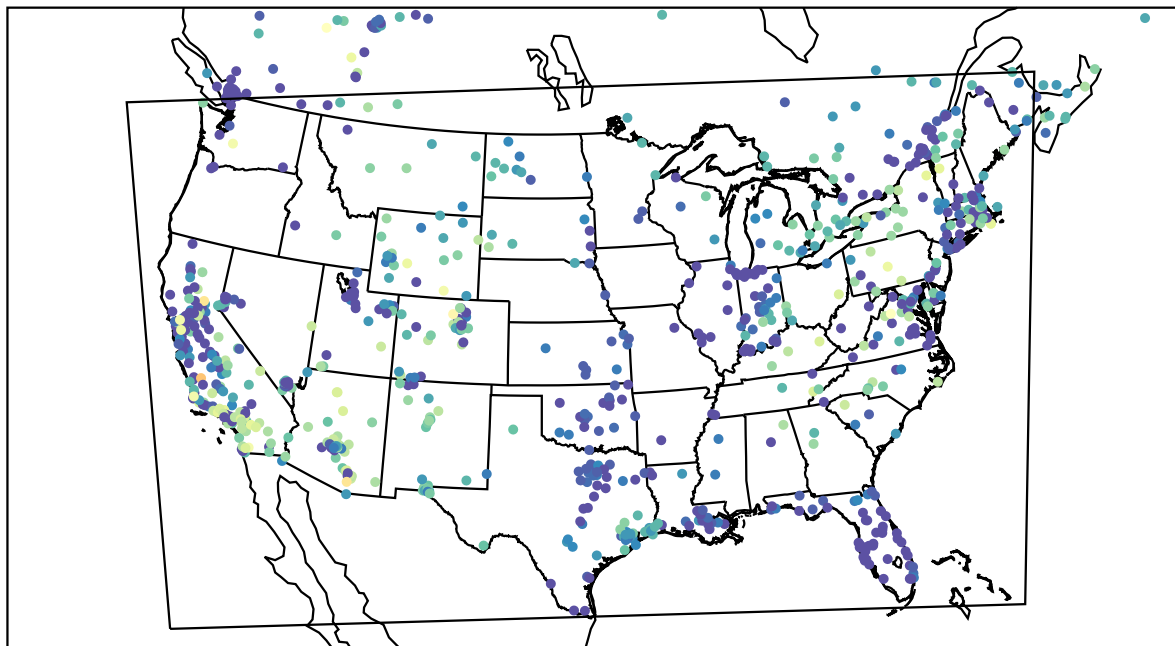
AirNOW (2022-11-25_04:00:00)
