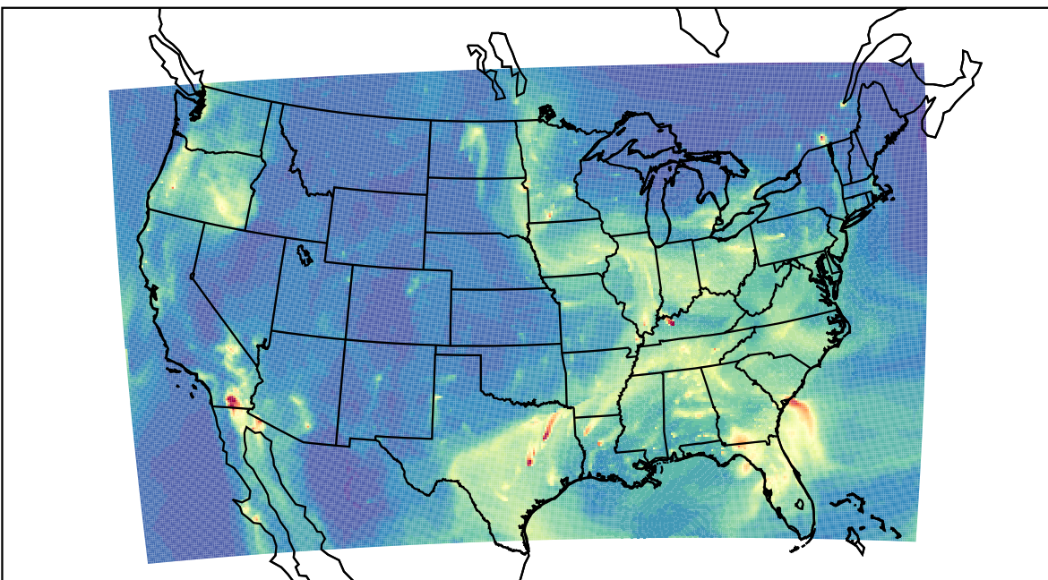
WRF 2022-12-09_14:00:00
