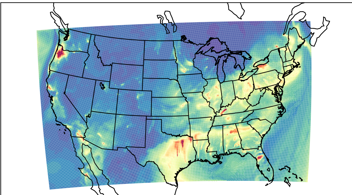
WRF 2022-12-08_07:00:00
