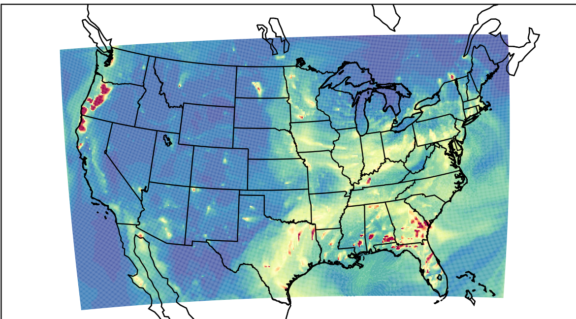
WRF 2022-12-09_02:00:00
