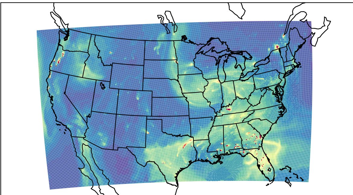
WRF 2022-12-09_21:00:00
