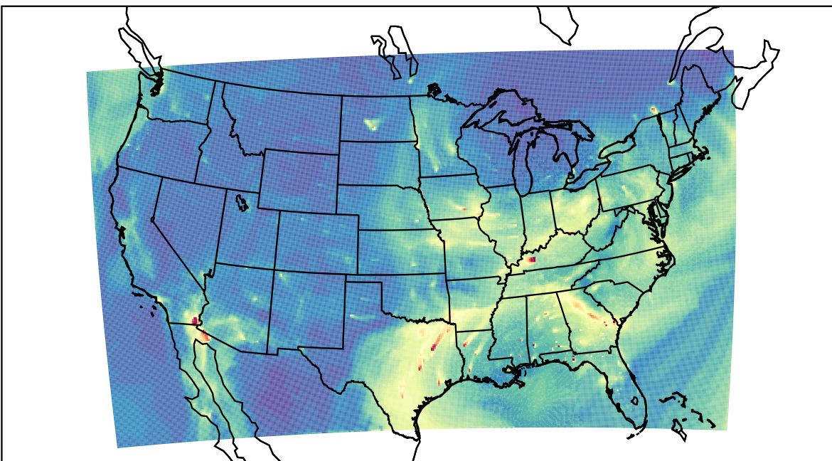
WRF 2022-12-08_17:00:00
