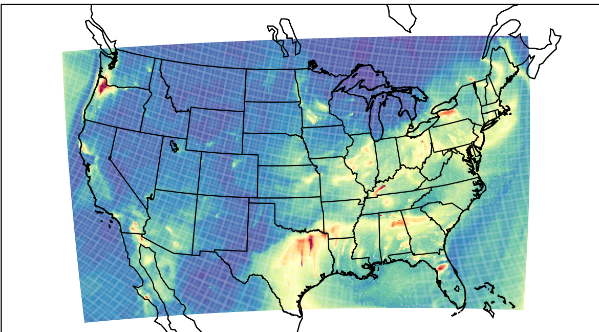
WRF 2022-12-08_08:00:00
