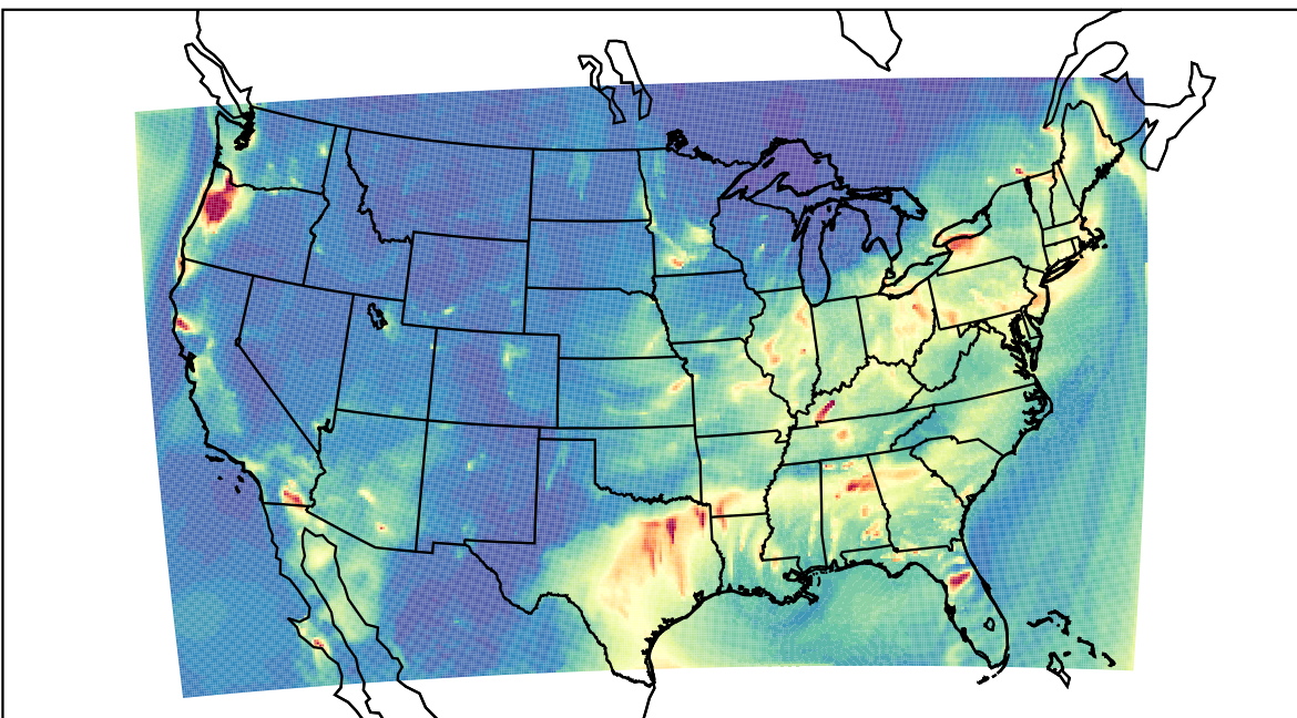
WRF 2022-12-08_06:00:00
