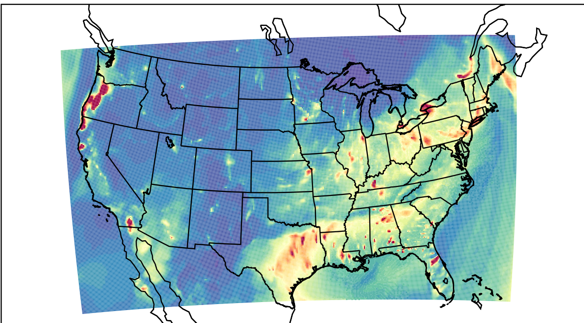
WRF 2022-12-08_03:00:00
