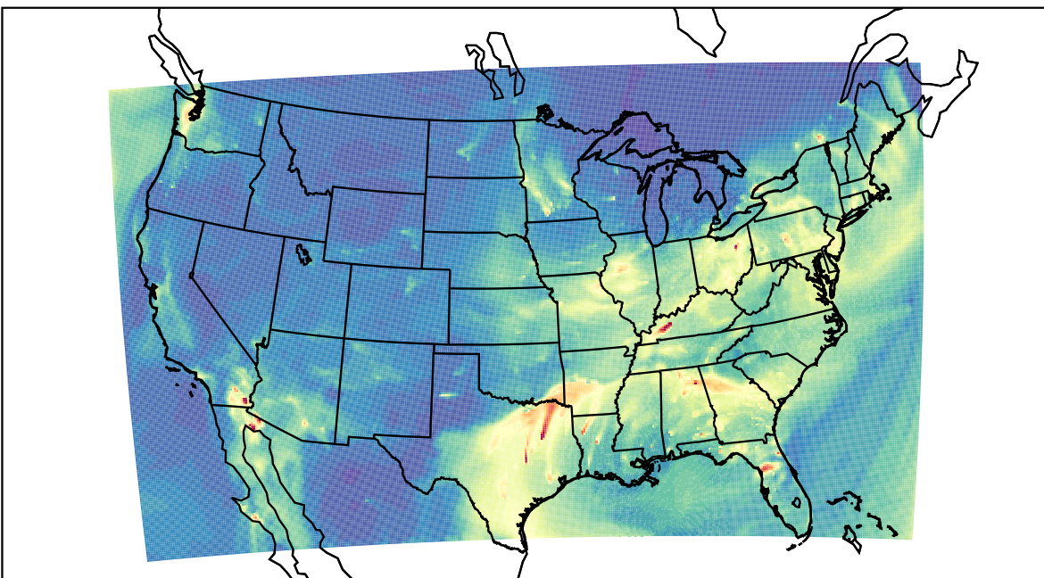
WRF 2022-12-08_12:00:00
