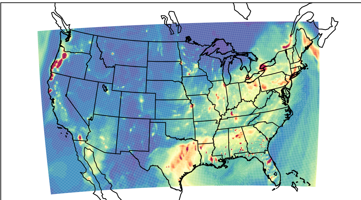
WRF 2022-12-08_02:00:00
