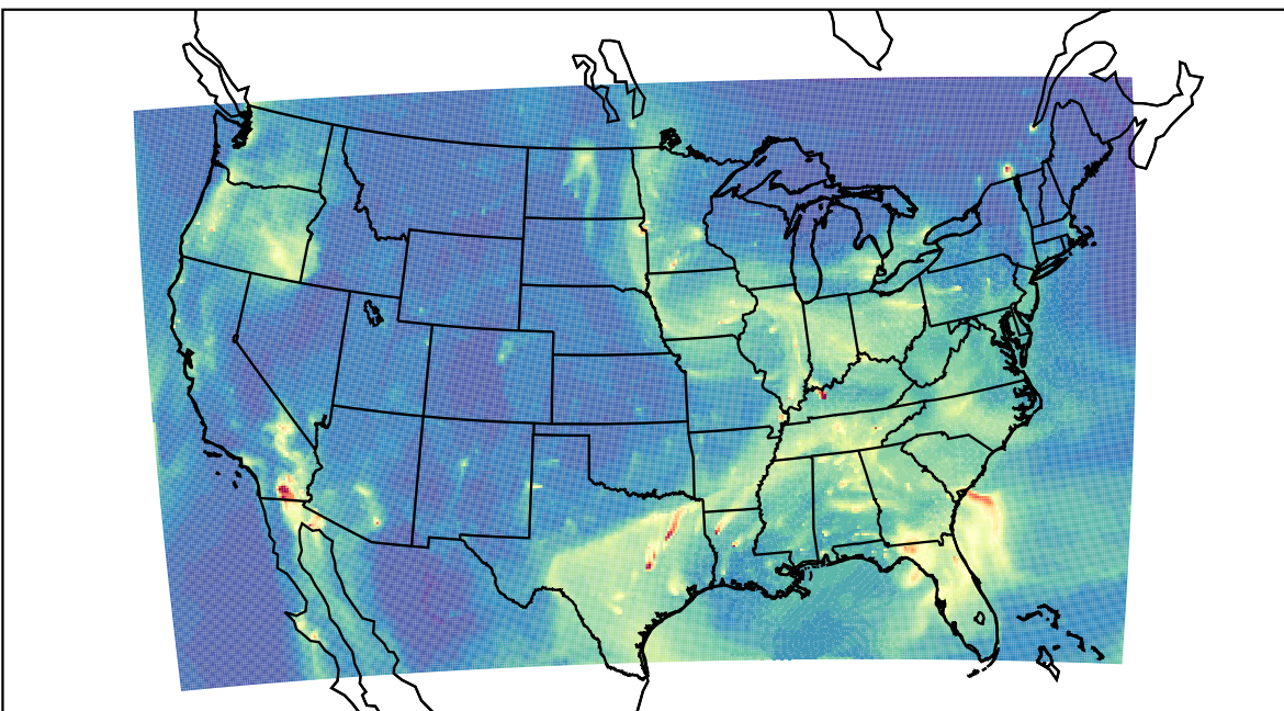
WRF 2022-12-09_15:00:00
