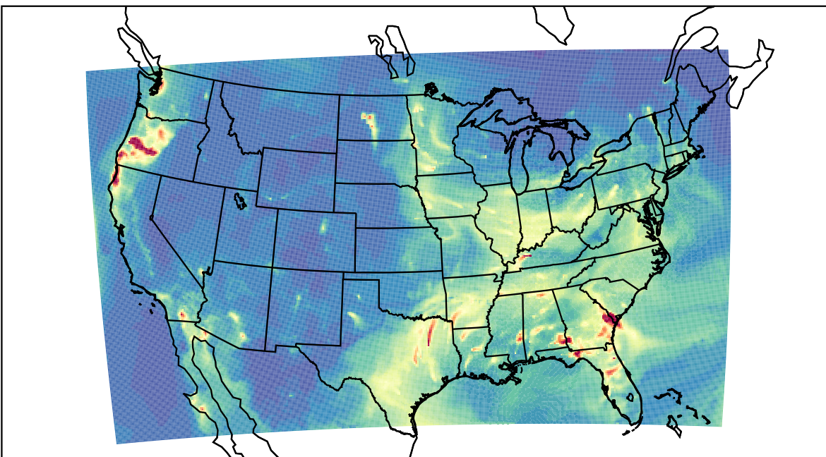
WRF 2022-12-09_06:00:00
