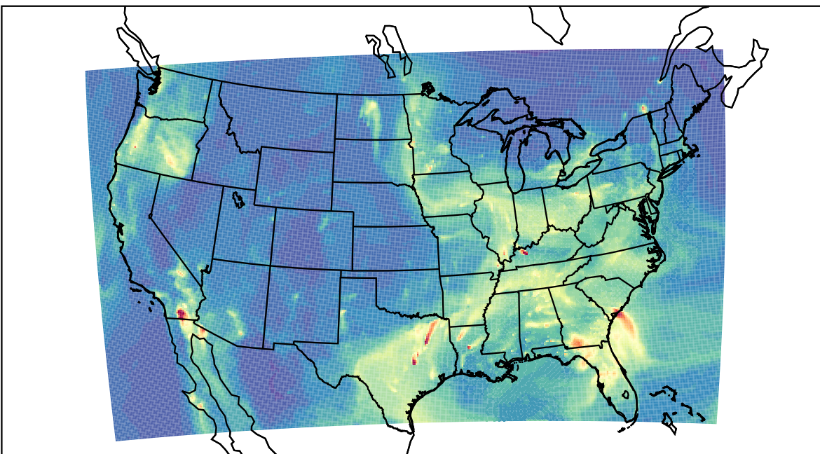
WRF 2022-12-09_13:00:00
