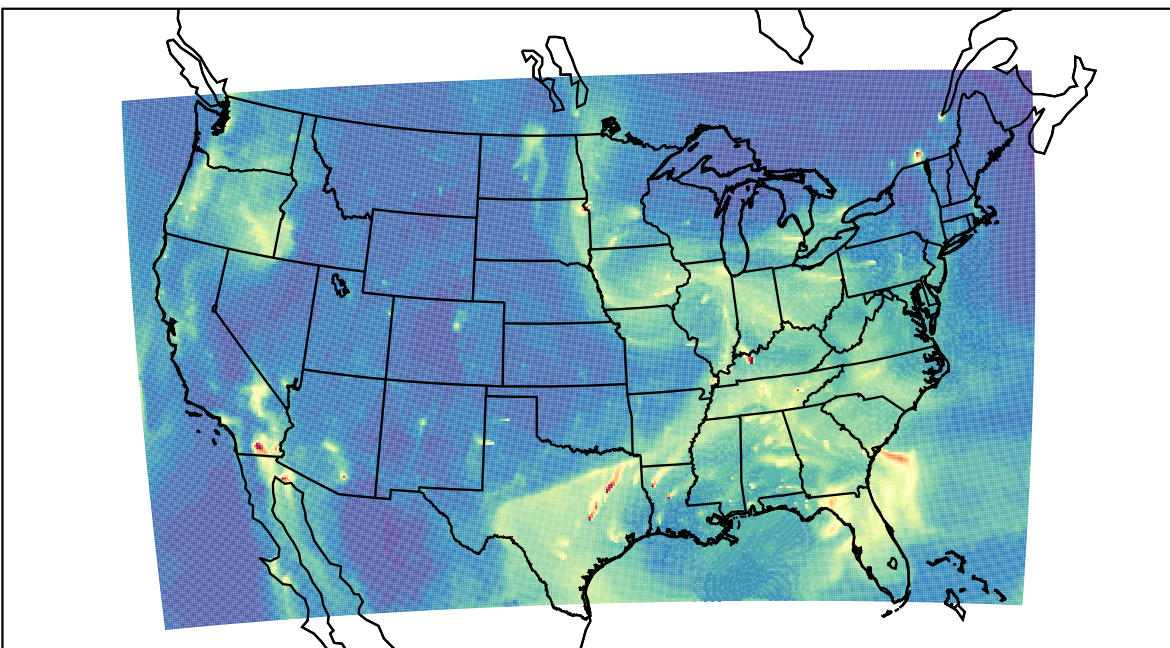
WRF 2022-12-09_16:00:00
