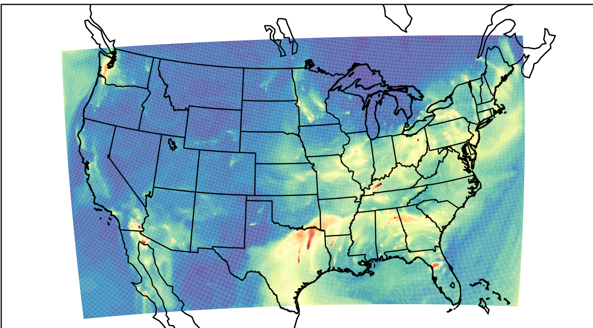
WRF 2022-12-08_11:00:00
