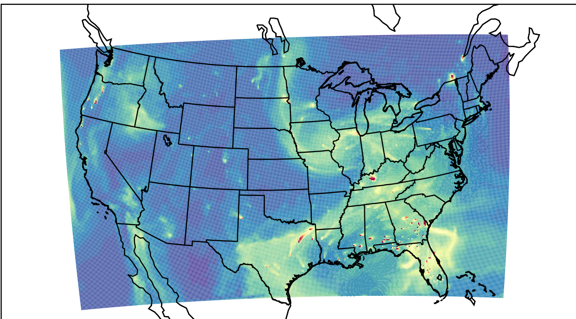
WRF 2022-12-09_20:00:00
