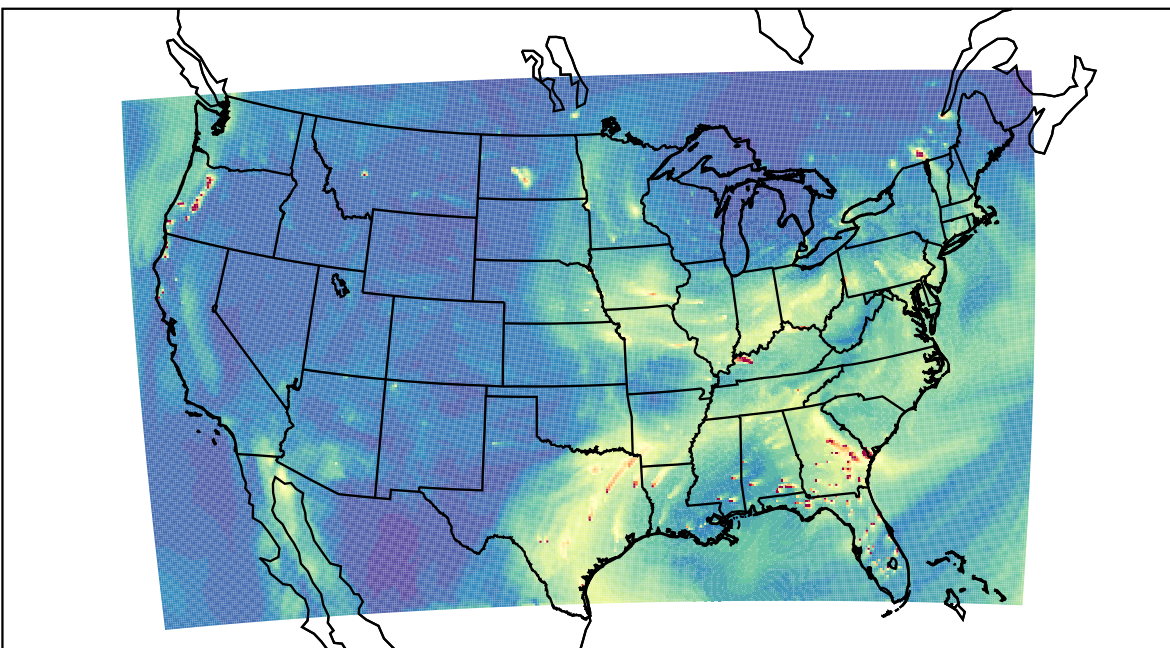
WRF 2022-12-08_21:00:00
