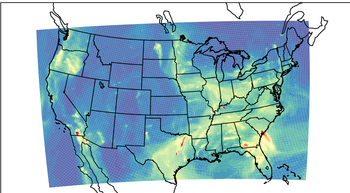
WRF 2022-12-09_12:00:00
