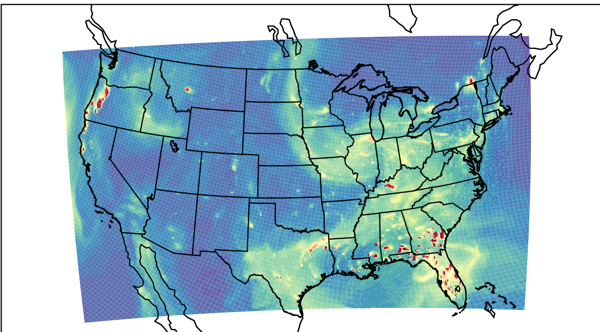
WRF 2022-12-09_23:00:00
