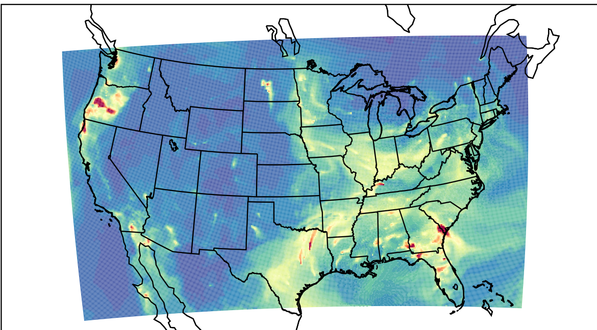
WRF 2022-12-09_07:00:00
