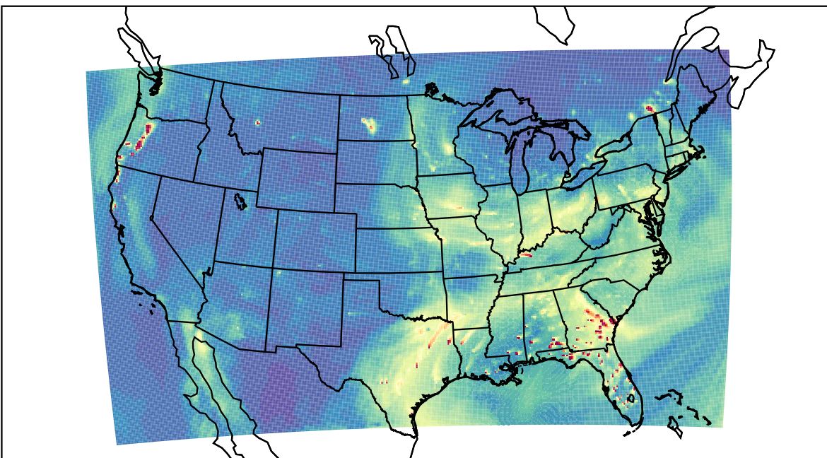
WRF 2022-12-08_22:00:00
