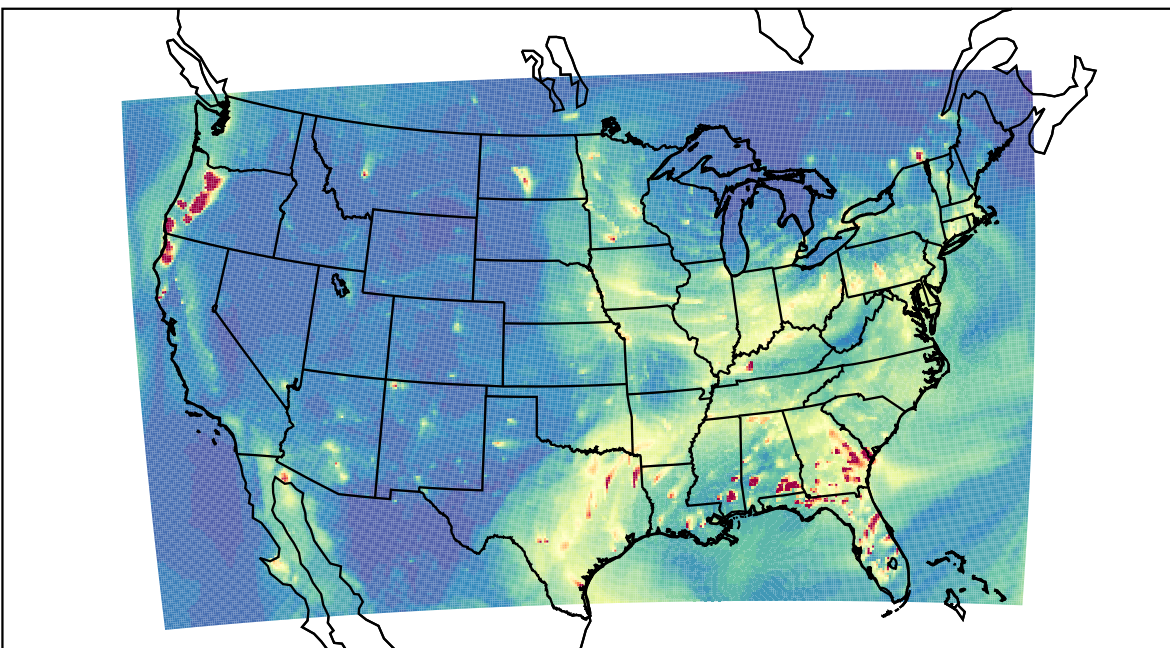
WRF 2022-12-09_01:00:00
