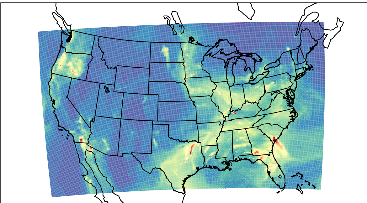
WRF 2022-12-09_11:00:00
