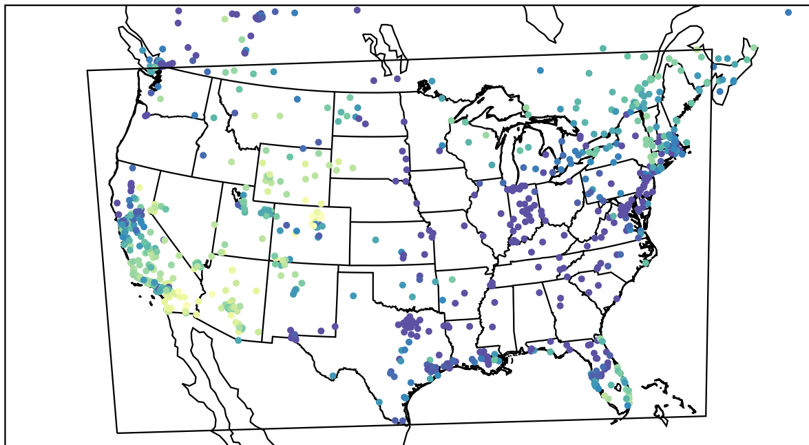
AirNOW (2022-12-09_23:00:00)
