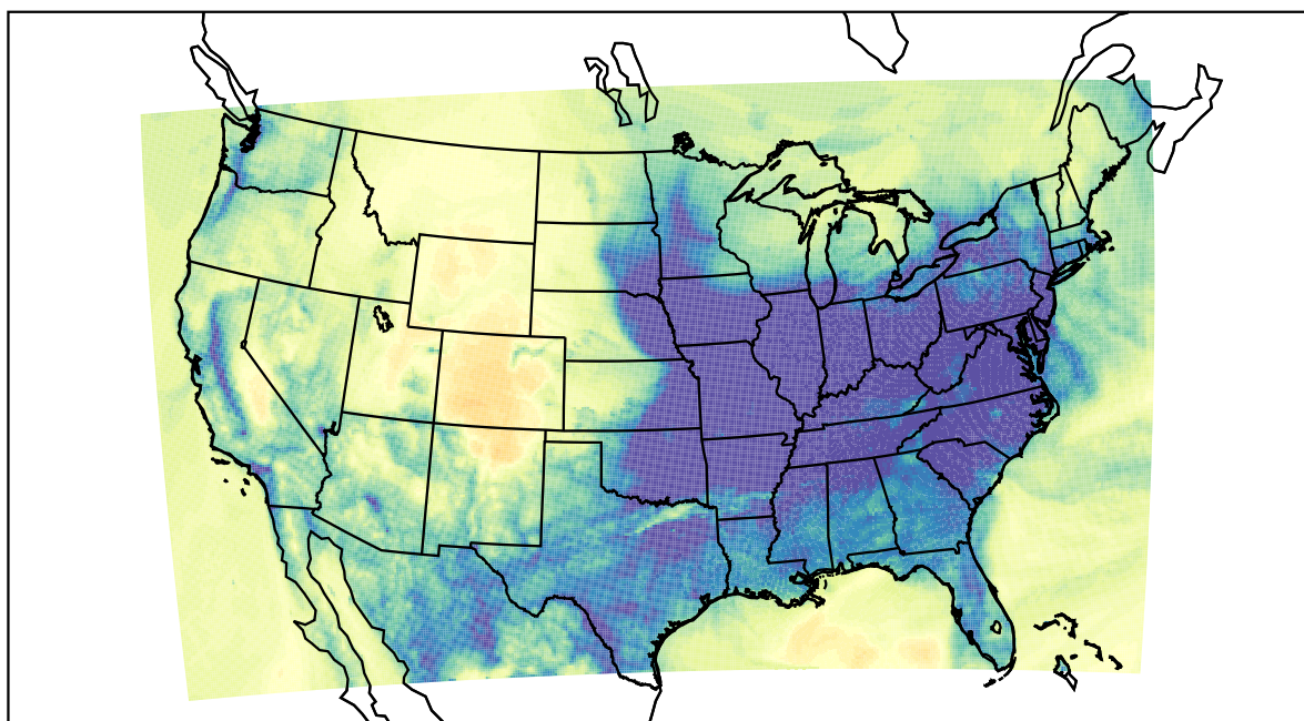
WRF (2022-12-09_09:00:00)
