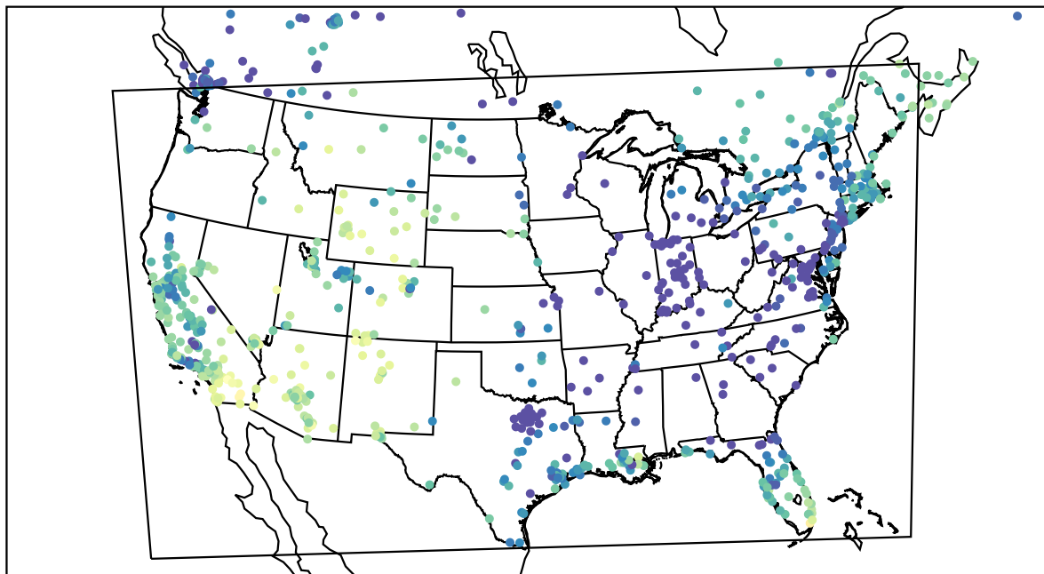
AirNOW (2022-12-10_22:00:00)
