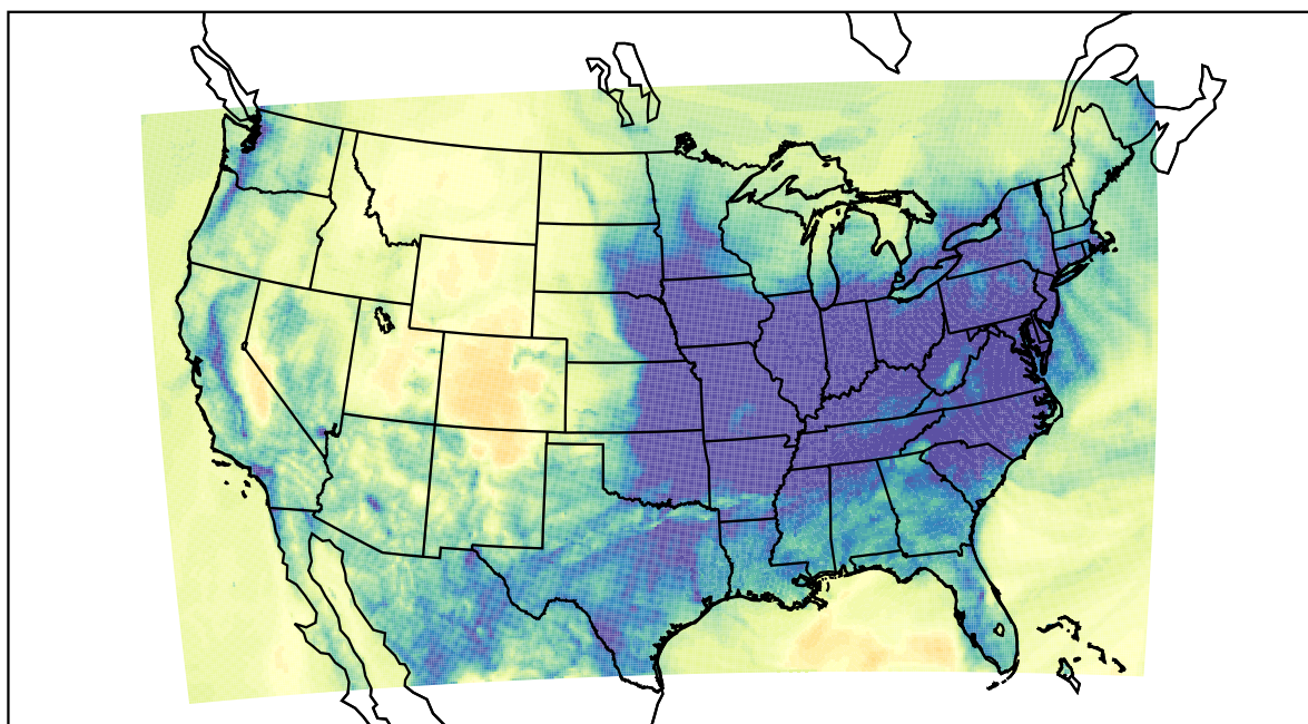
WRF (2022-12-09_06:00:00)
