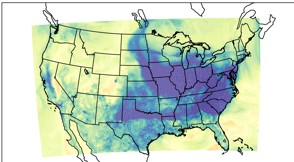
WRF (2022-12-10_03:00:00)
