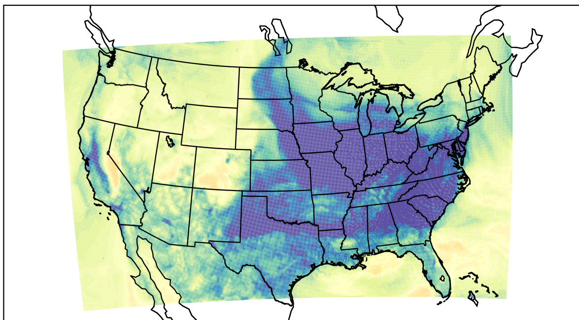
WRF (2022-12-10_05:00:00)
