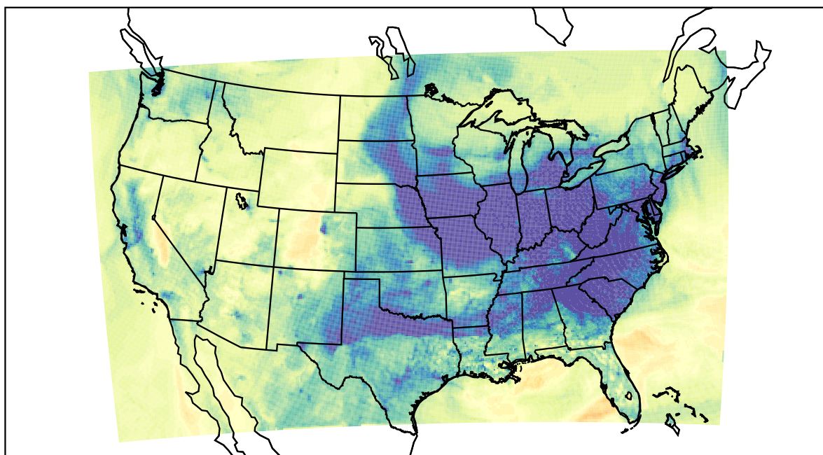
WRF (2022-12-10_00:00:00)
