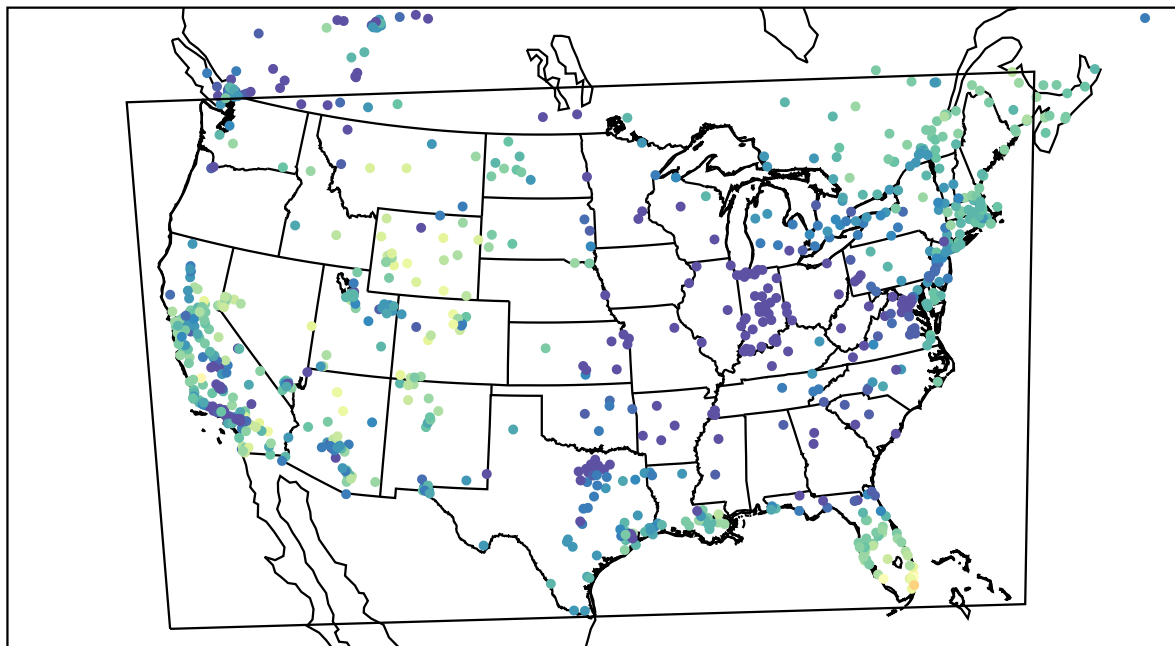
AirNOW (2022-12-10_18:00:00)
