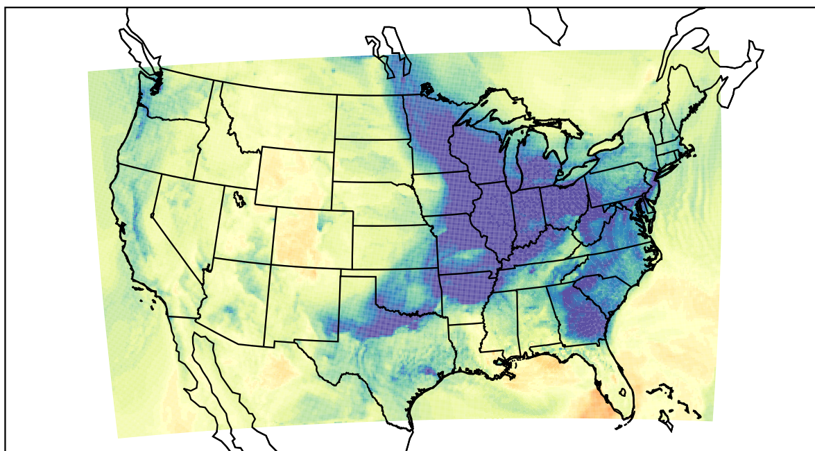
WRF (2022-12-10_21:00:00)
