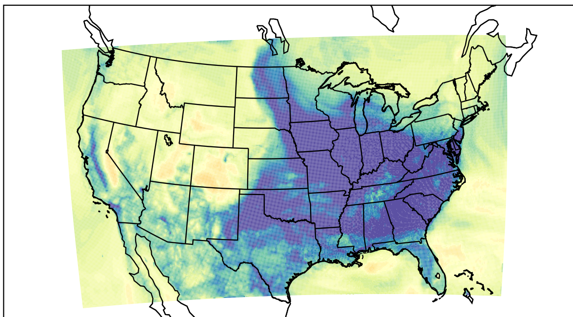
WRF (2022-12-10_09:00:00)
