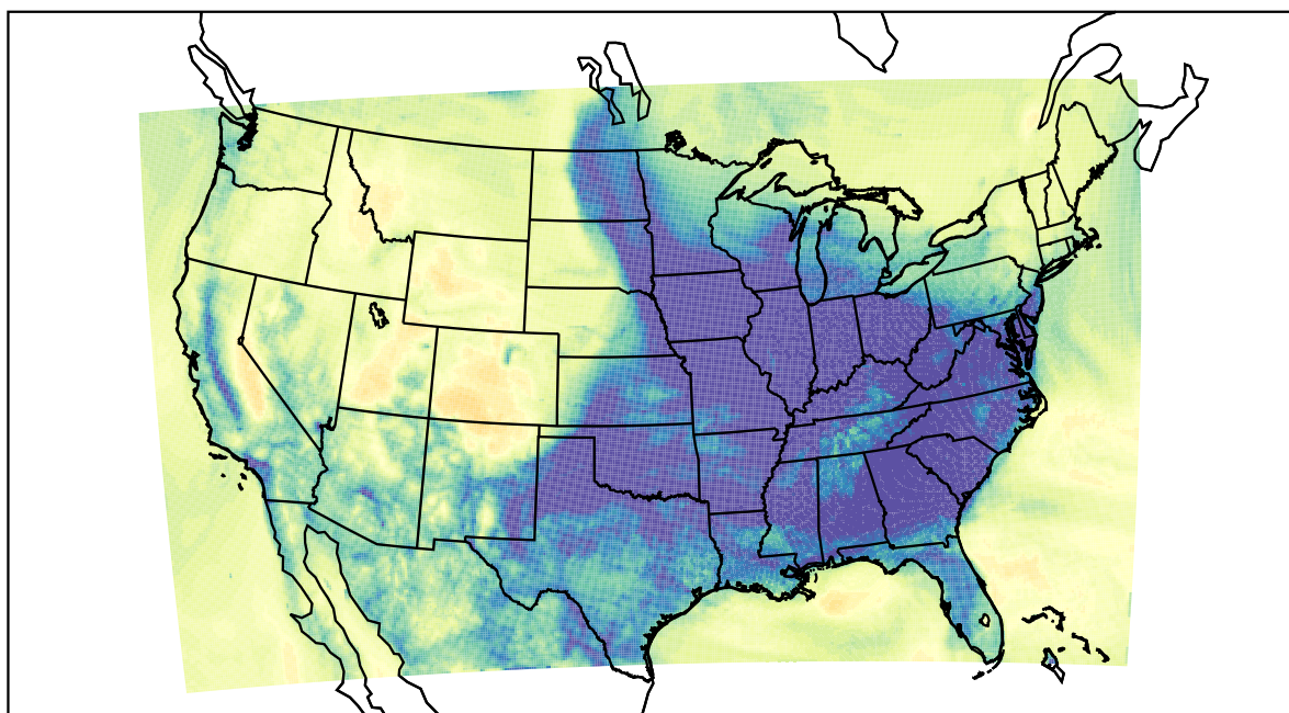
WRF (2022-12-10_10:00:00)
