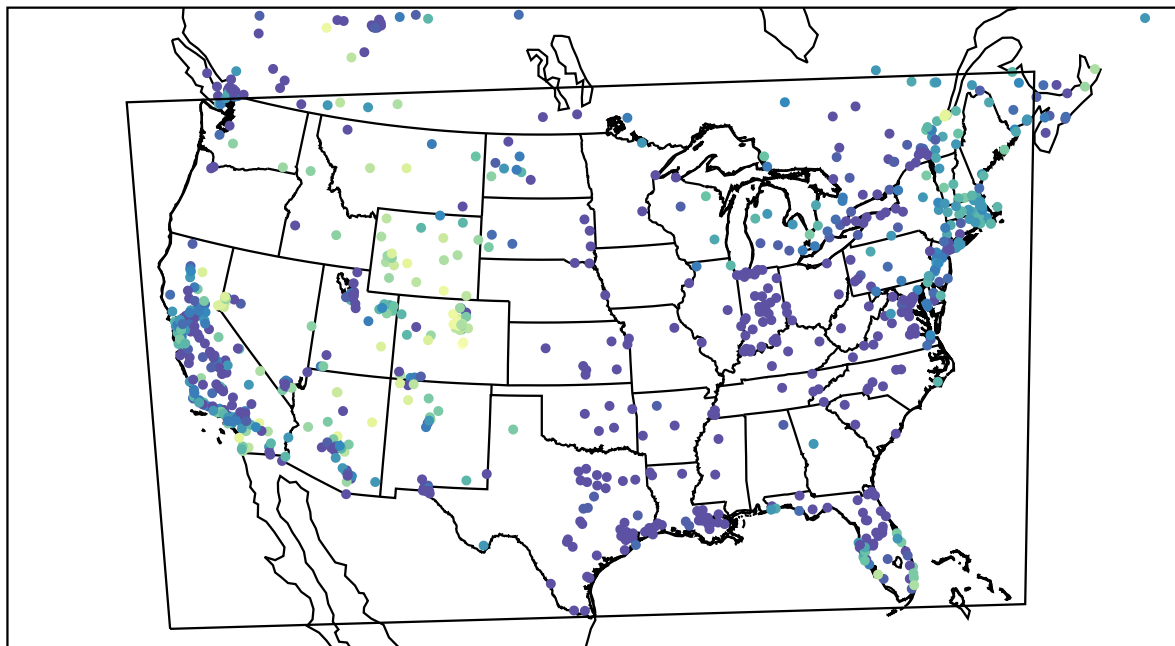
AirNOW (2022-12-09_01:00:00)
