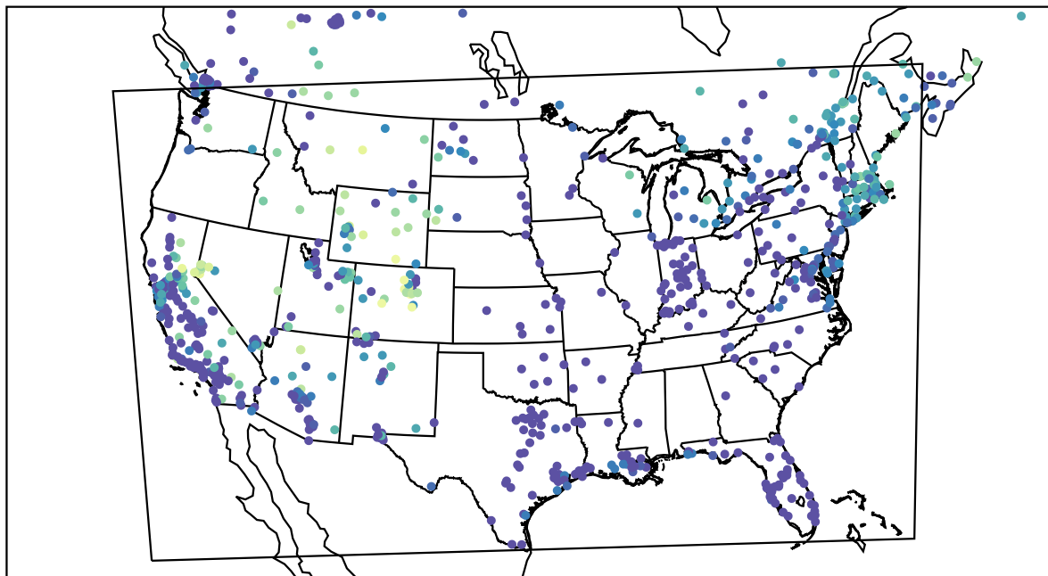
AirNOW (2022-12-09_08:00:00)
