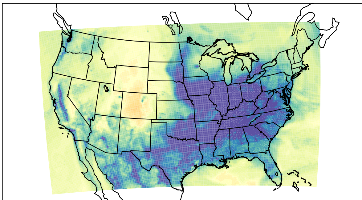
WRF (2022-12-09_15:00:00)
