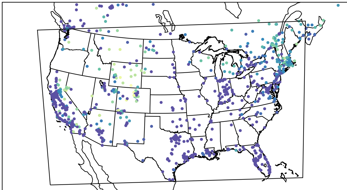
AirNOW (2022-12-09_13:00:00)
