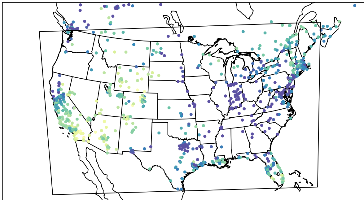
AirNOW (2022-12-09_22:00:00)
