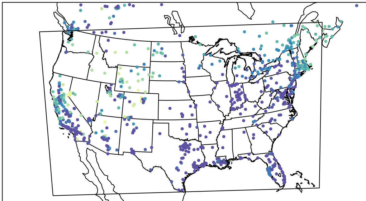
AirNOW (2022-12-10_13:00:00)
