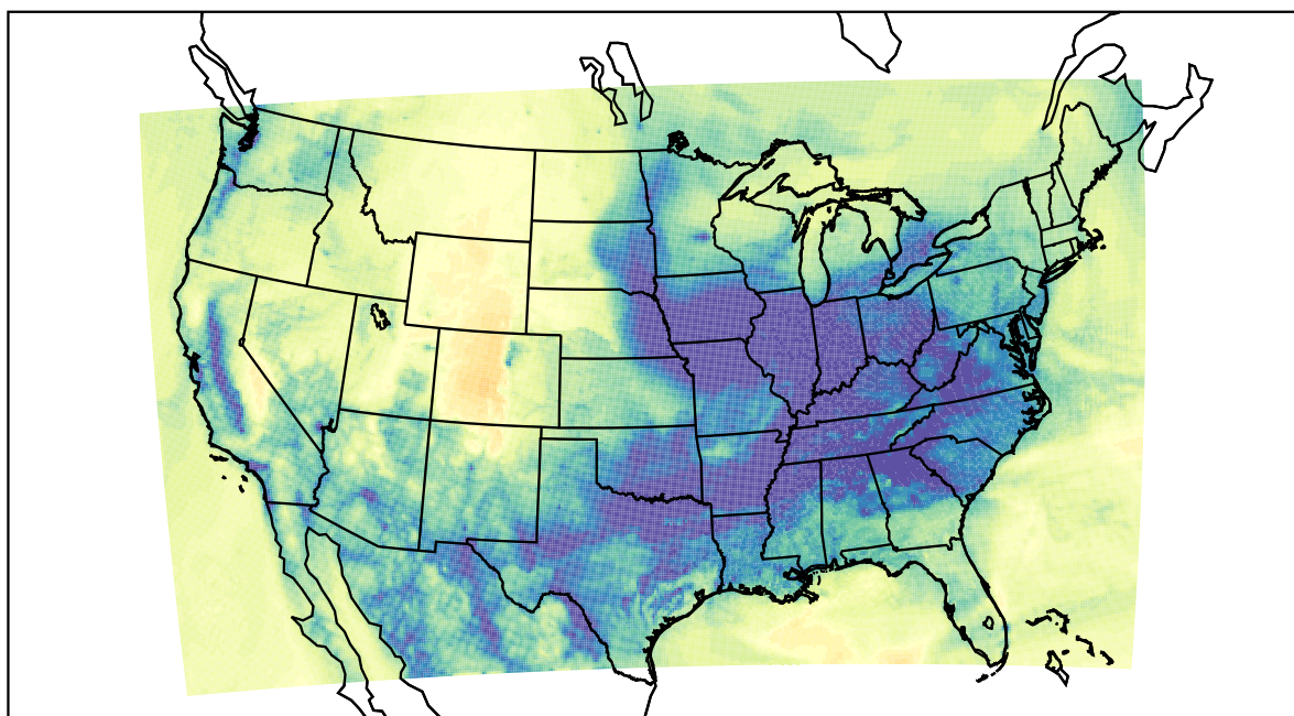
WRF (2022-12-09_16:00:00)
