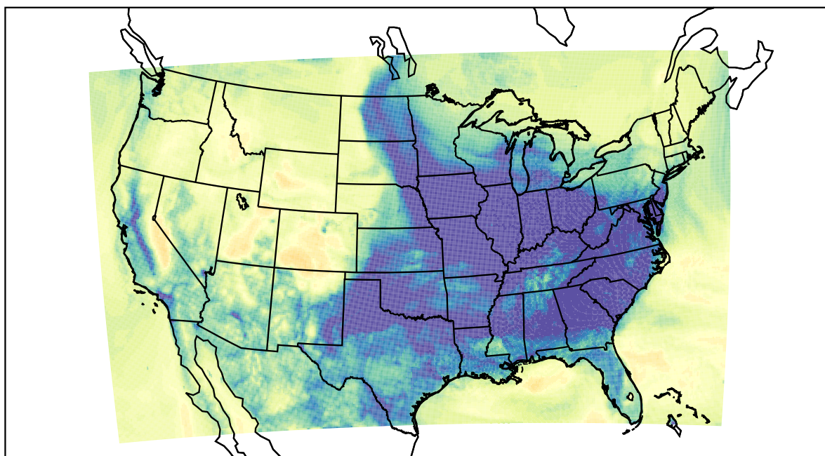
WRF (2022-12-10_08:00:00)
