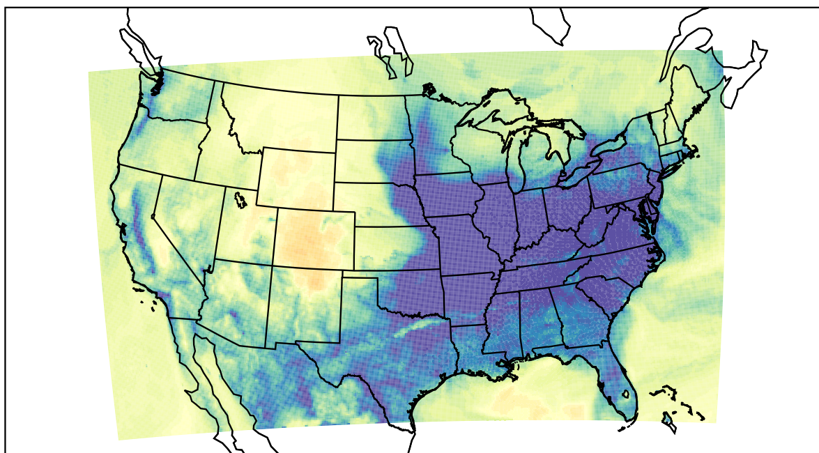
WRF (2022-12-09_11:00:00)
