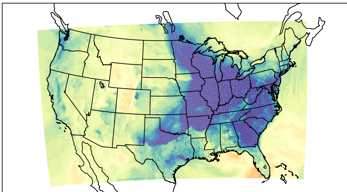
WRF (2022-12-10_23:00:00)
