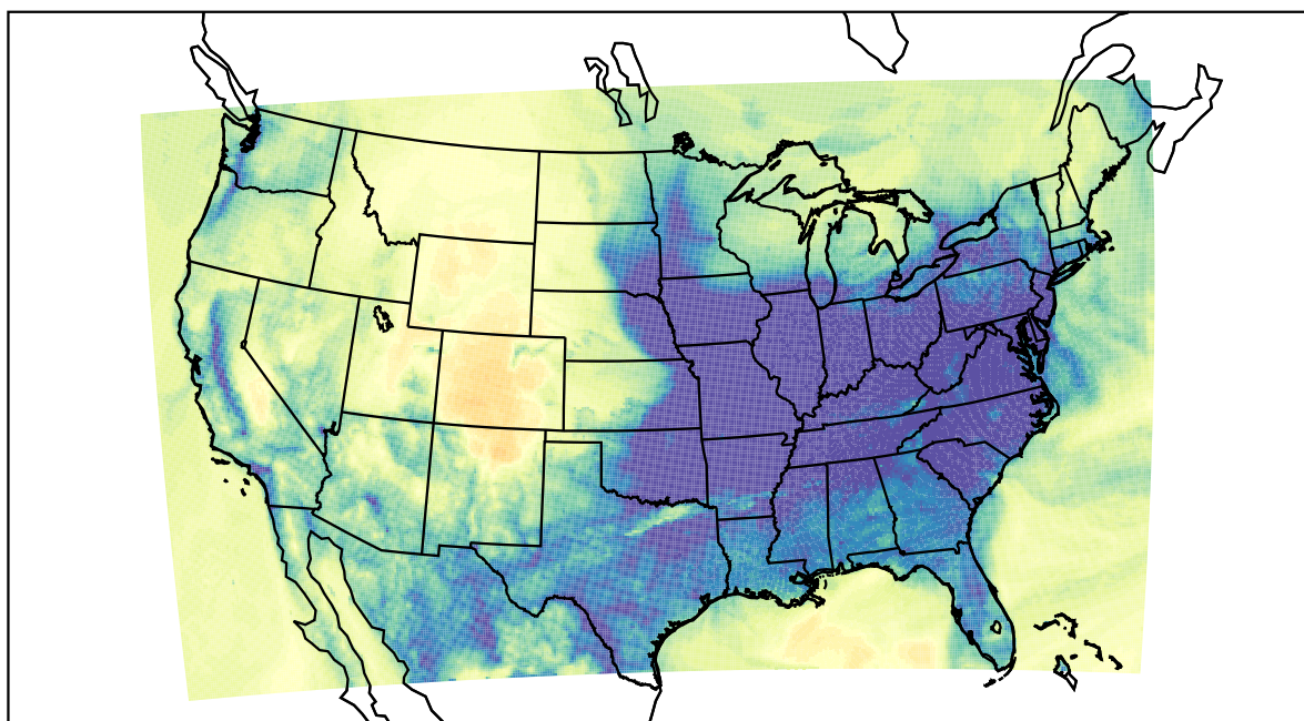
WRF (2022-12-09_10:00:00)
