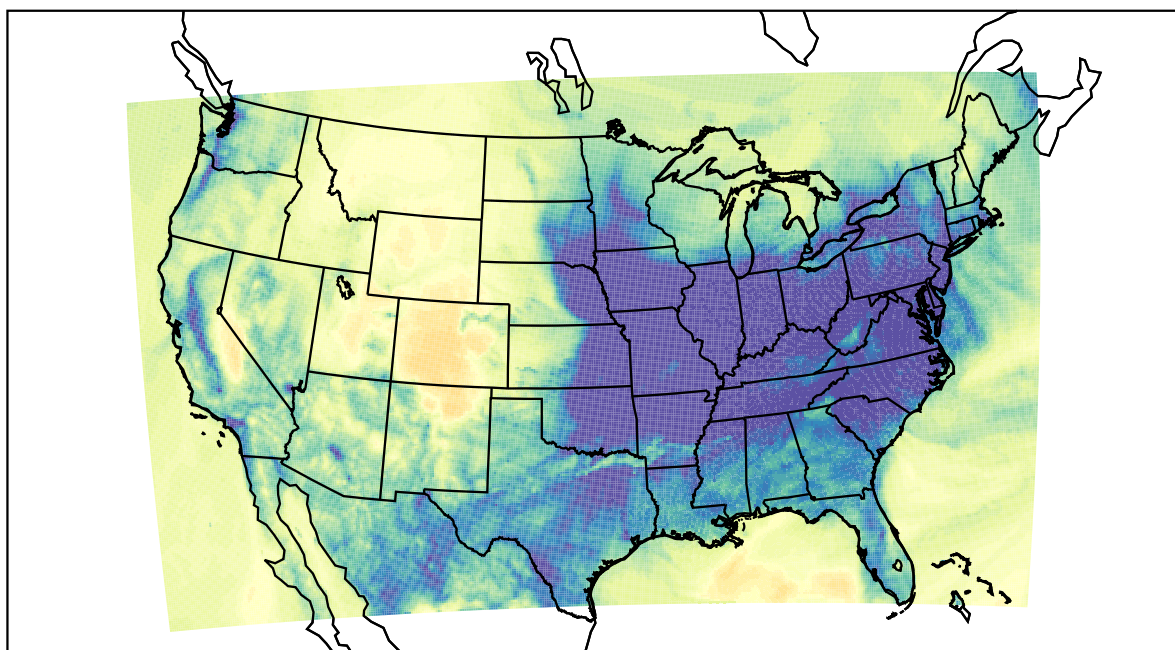
WRF (2022-12-09_07:00:00)
