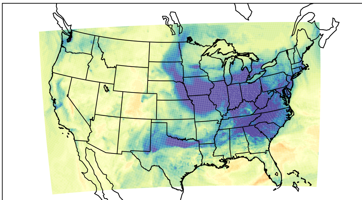
WRF (2022-12-09_22:00:00)
