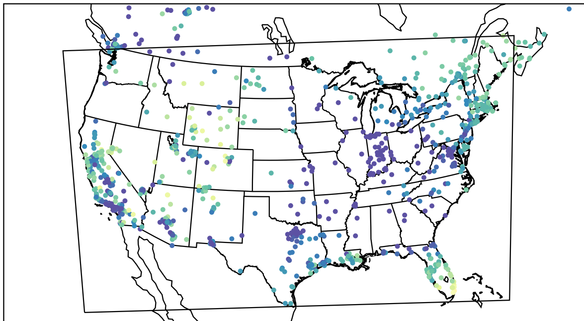
AirNOW (2022-12-10_17:00:00)
