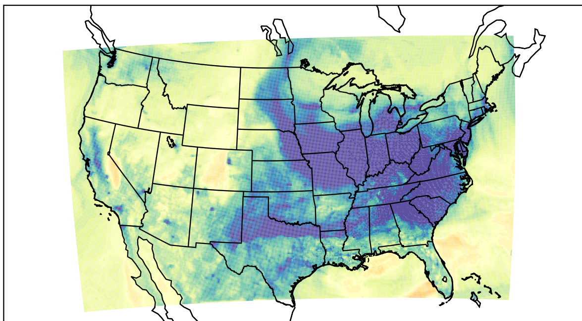
WRF (2022-12-10_01:00:00)
