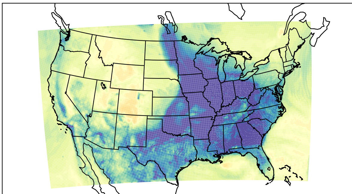
WRF (2022-12-10_15:00:00)
