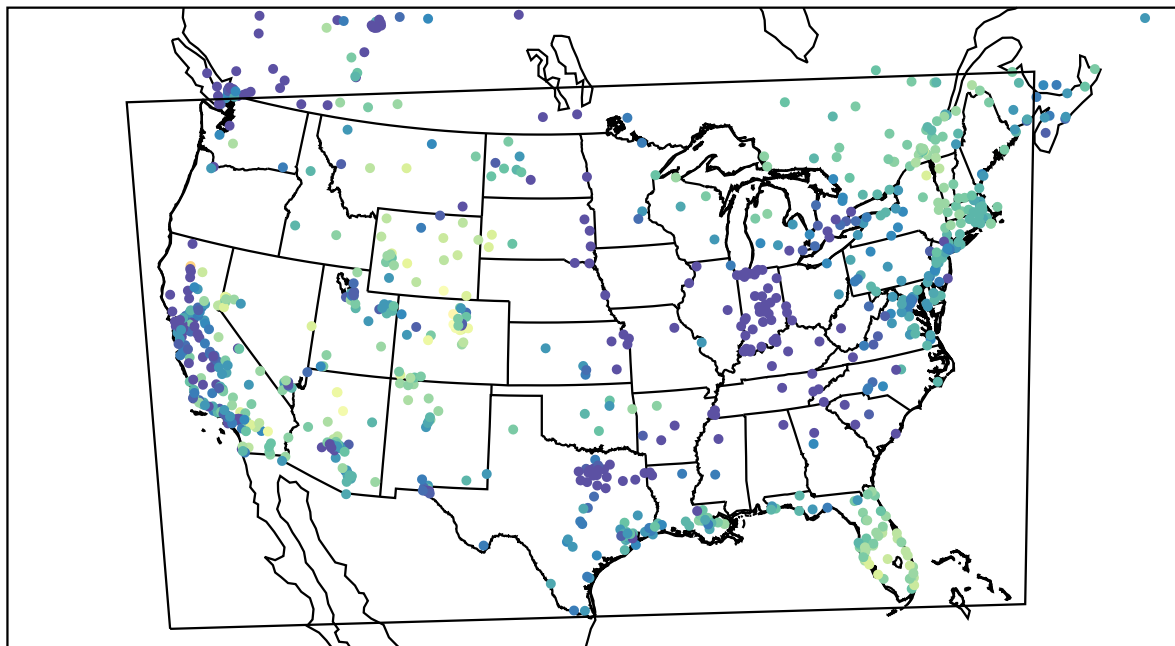
AirNOW (2022-12-09_18:00:00)
