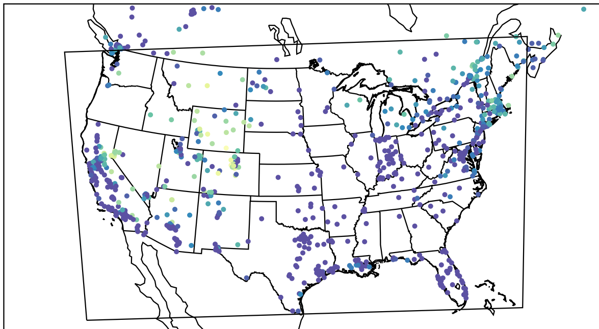
AirNOW (2022-12-09_10:00:00)
