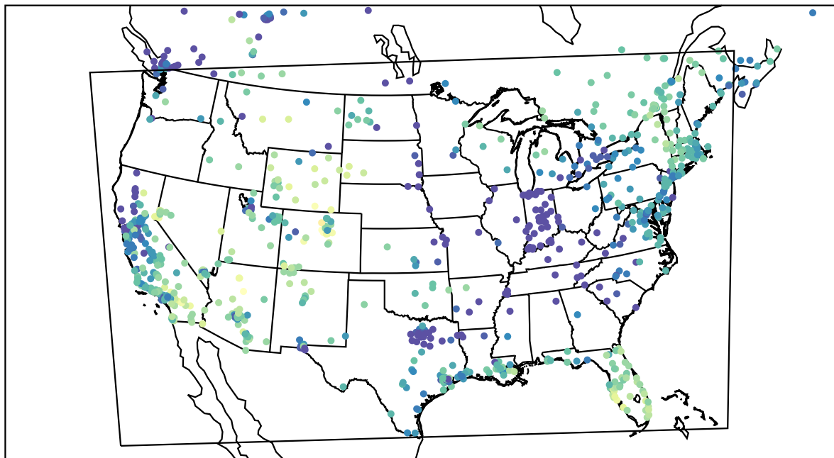
AirNOW (2022-12-09_19:00:00)
