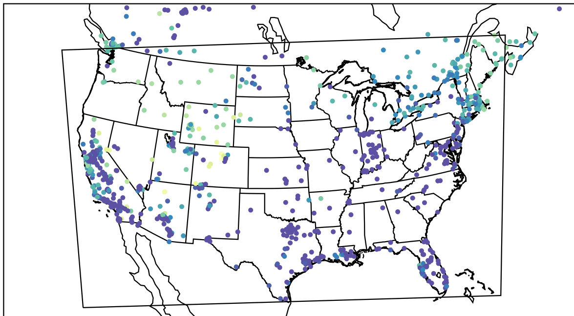
AirNOW (2022-12-10_07:00:00)
