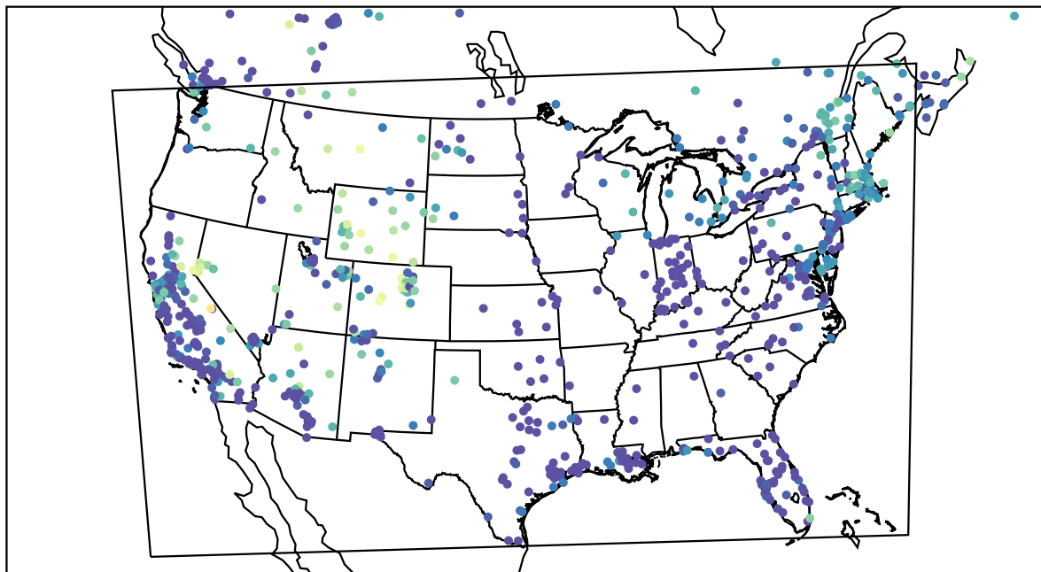
AirNOW (2022-12-09_05:00:00)
