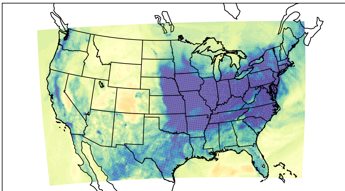
WRF (2022-12-09_03:00:00)
