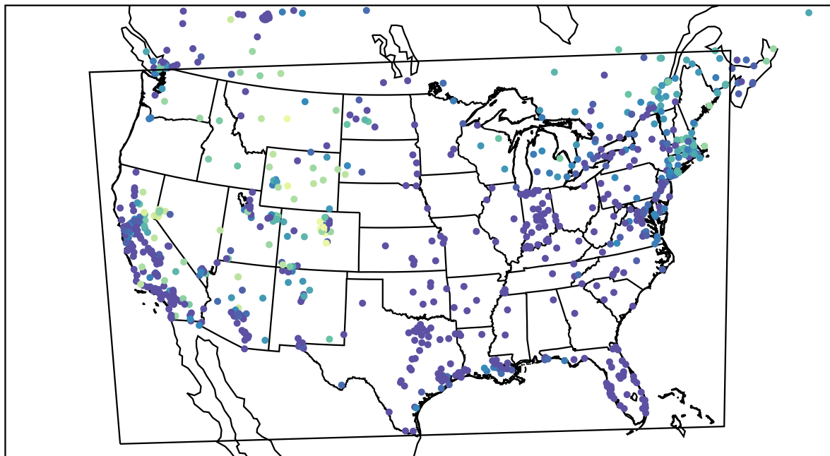
AirNOW (2022-12-09_09:00:00)
