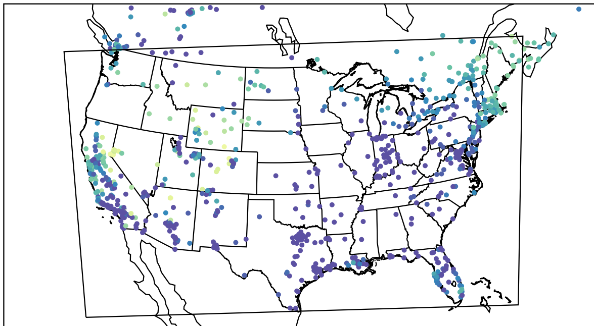
AirNOW (2022-12-10_14:00:00)
