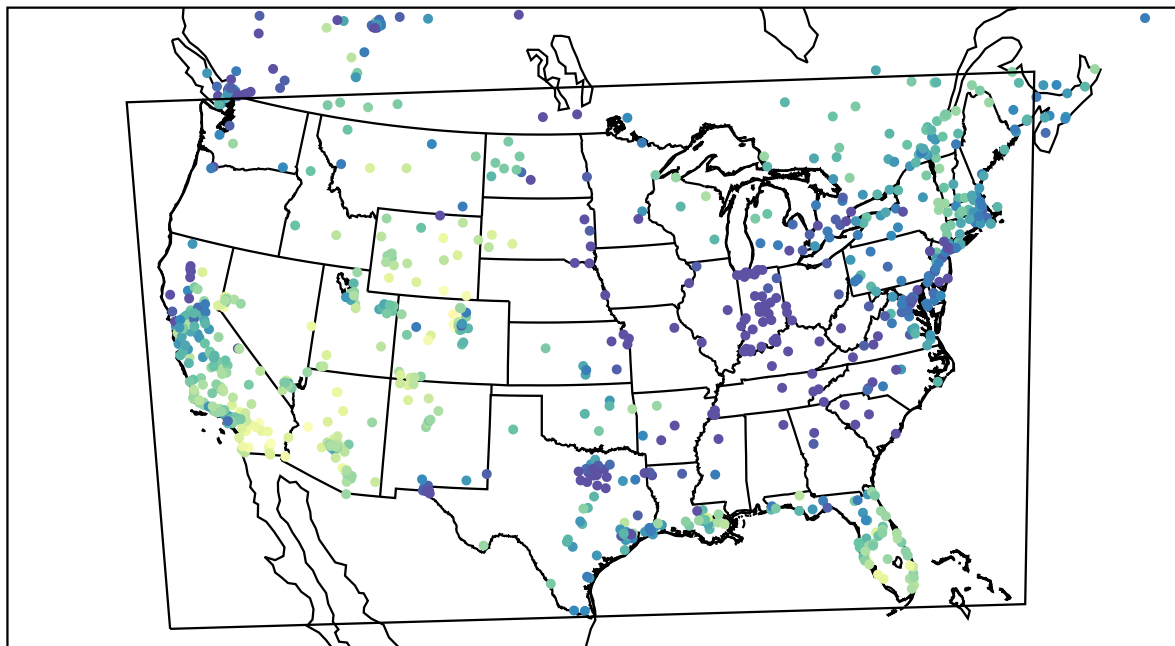
AirNOW (2022-12-09_21:00:00)
