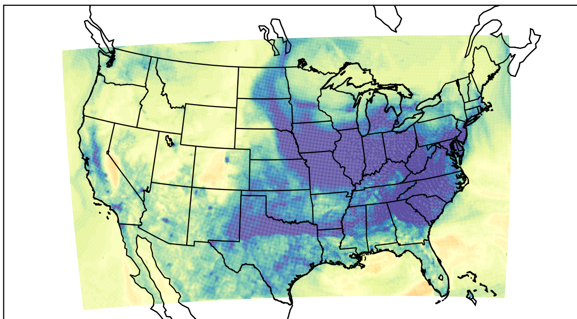
WRF (2022-12-10_02:00:00)
