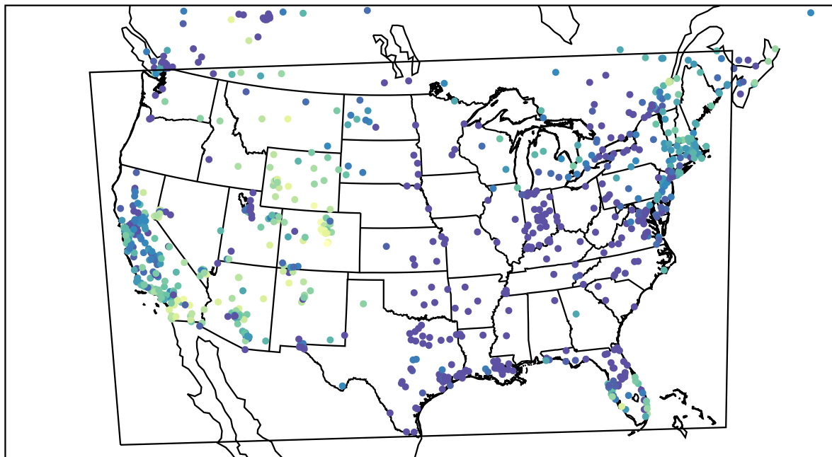
AirNOW (2022-12-09_00:00:00)
