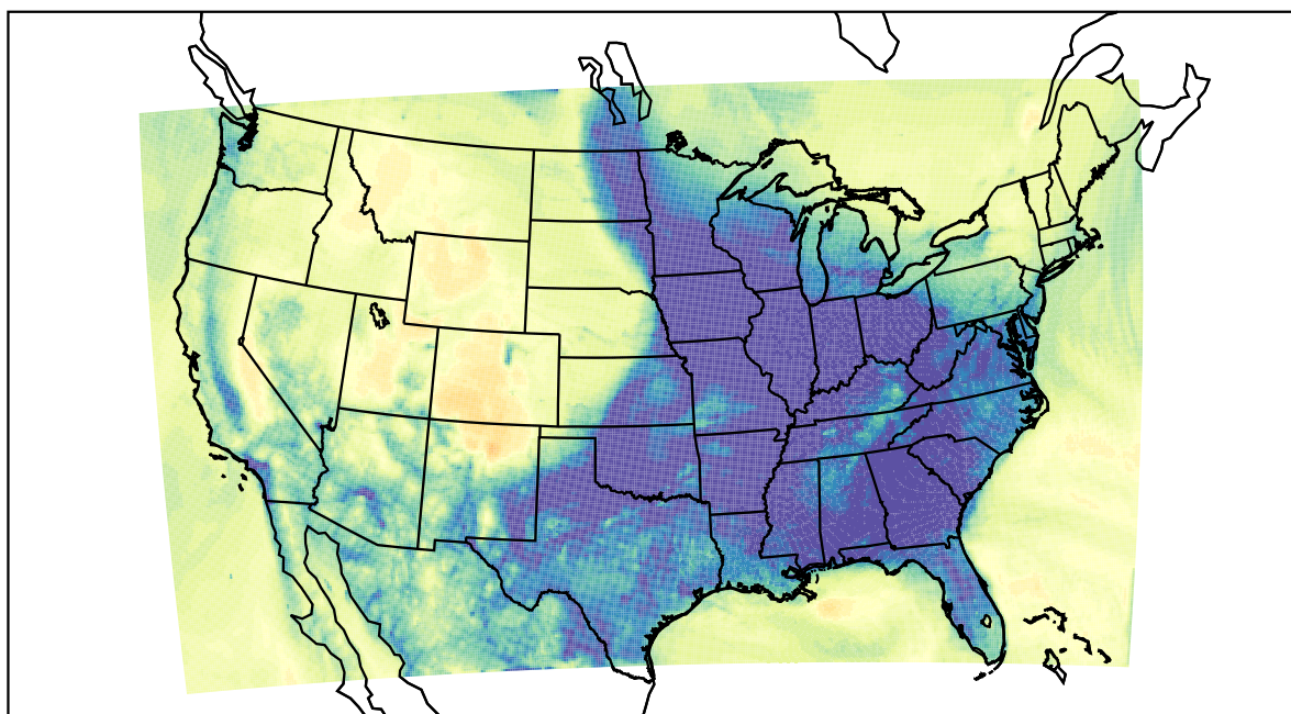
WRF (2022-12-10_14:00:00)
