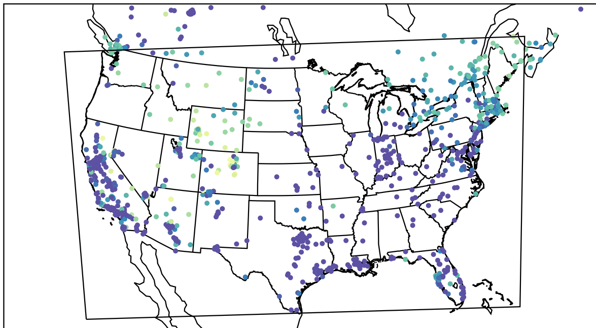
AirNOW (2022-12-10_04:00:00)
