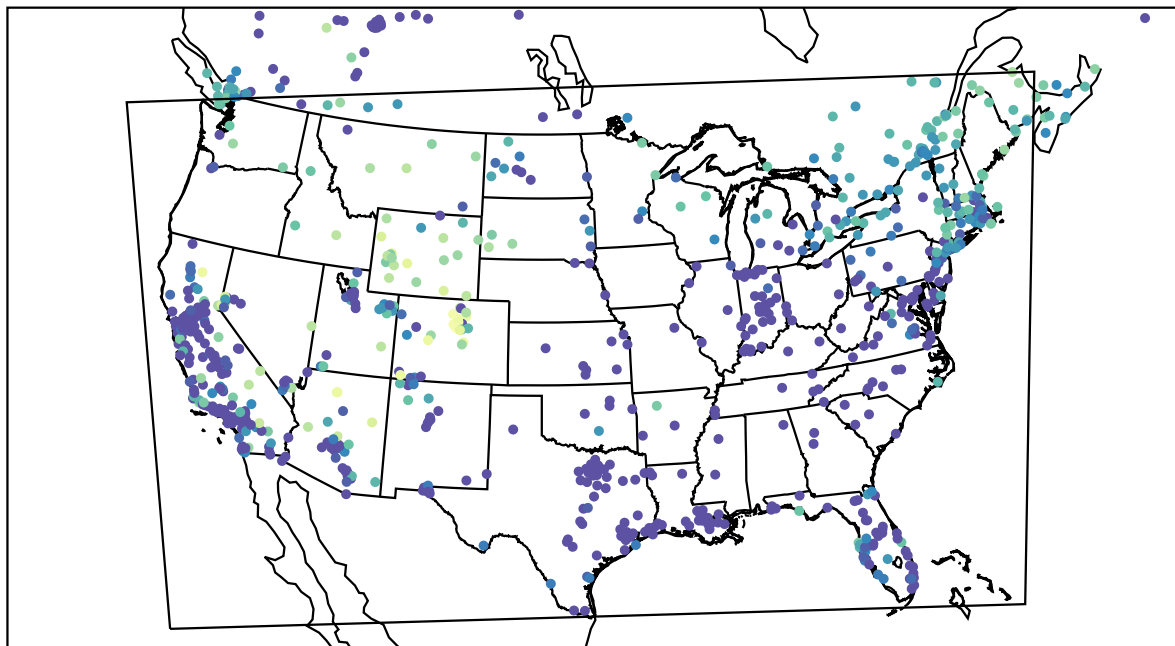
AirNOW (2022-12-10_03:00:00)
