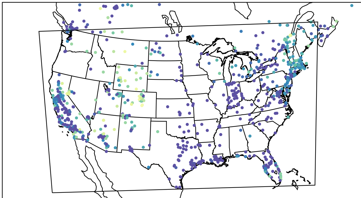
AirNOW (2022-12-09_02:00:00)
