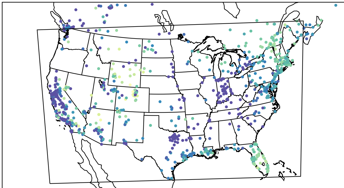
AirNOW (2022-12-09_17:00:00)
