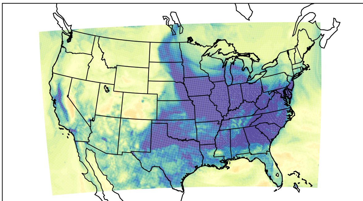
WRF (2022-12-10_06:00:00)
