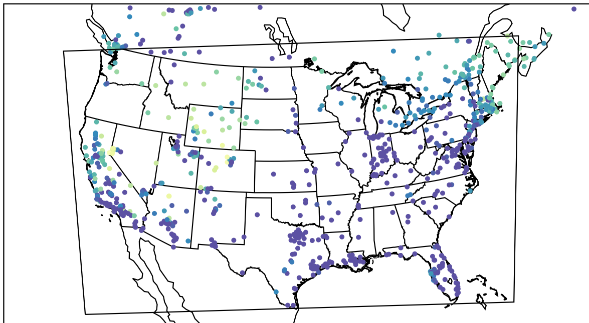
AirNOW (2022-12-10_11:00:00)
