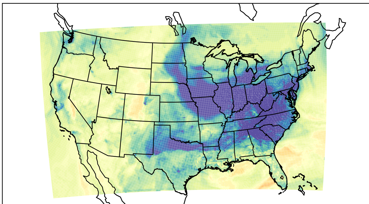
WRF (2022-12-09_23:00:00)
