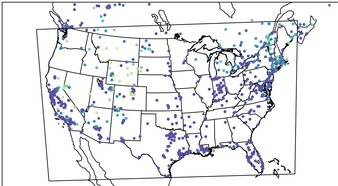
AirNOW (2022-12-09_12:00:00)
