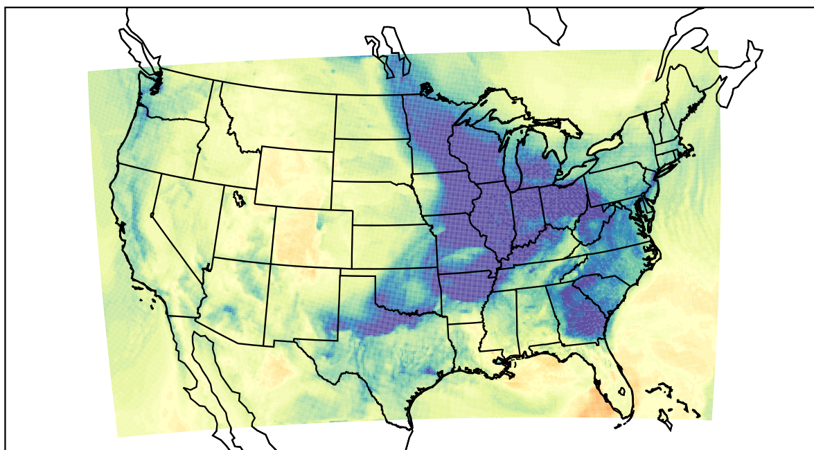
WRF (2022-12-10_20:00:00)
