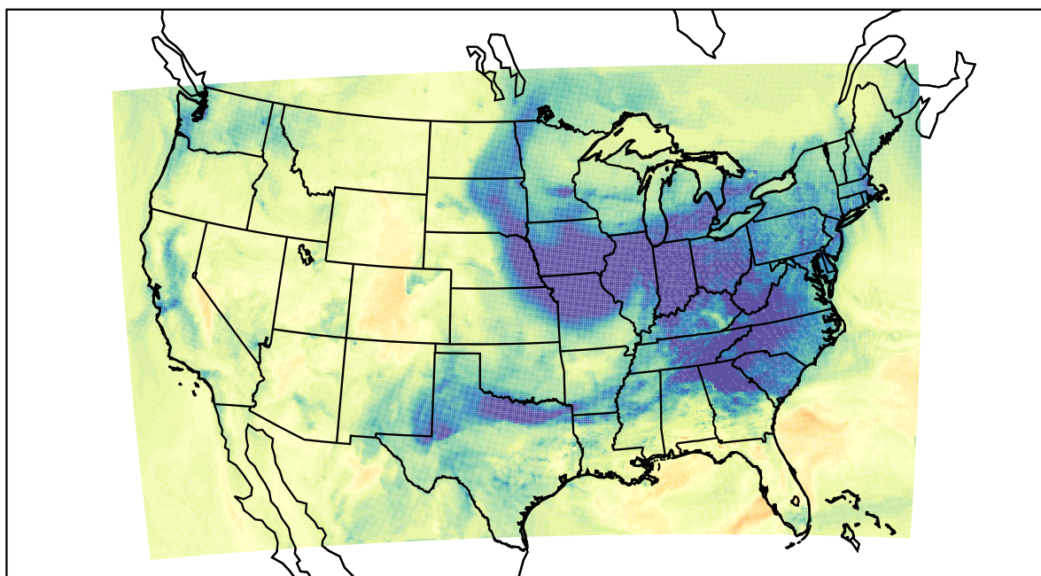
WRF (2022-12-09_21:00:00)
