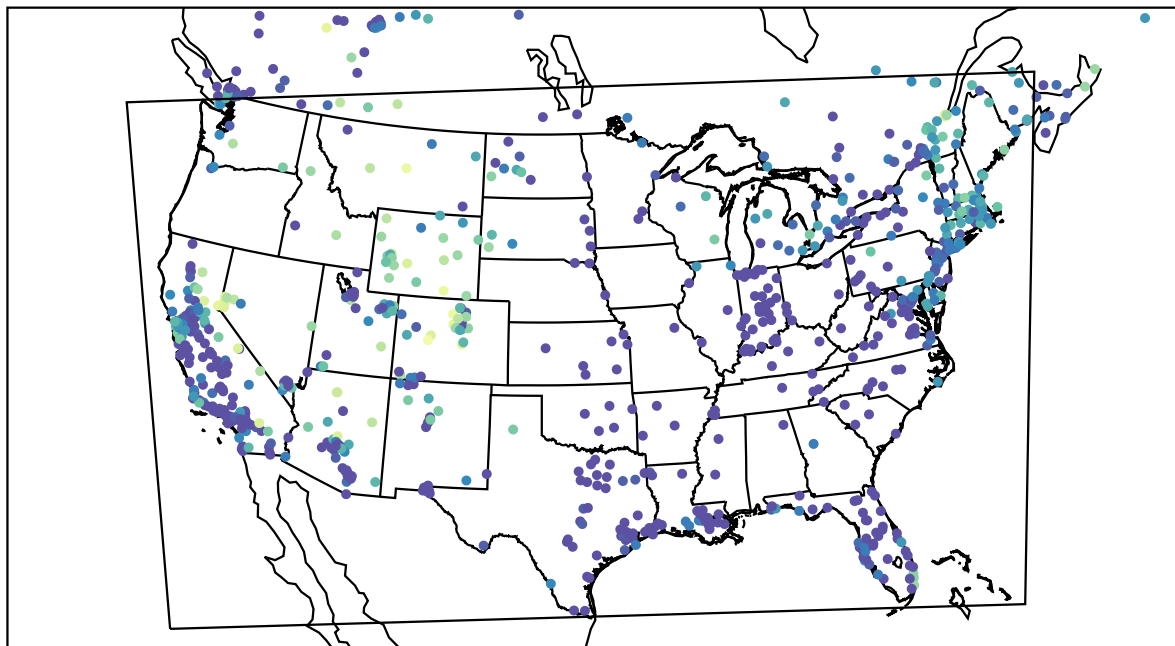
AirNOW (2022-12-09_04:00:00)
