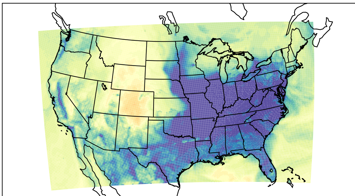
WRF (2022-12-09_13:00:00)
