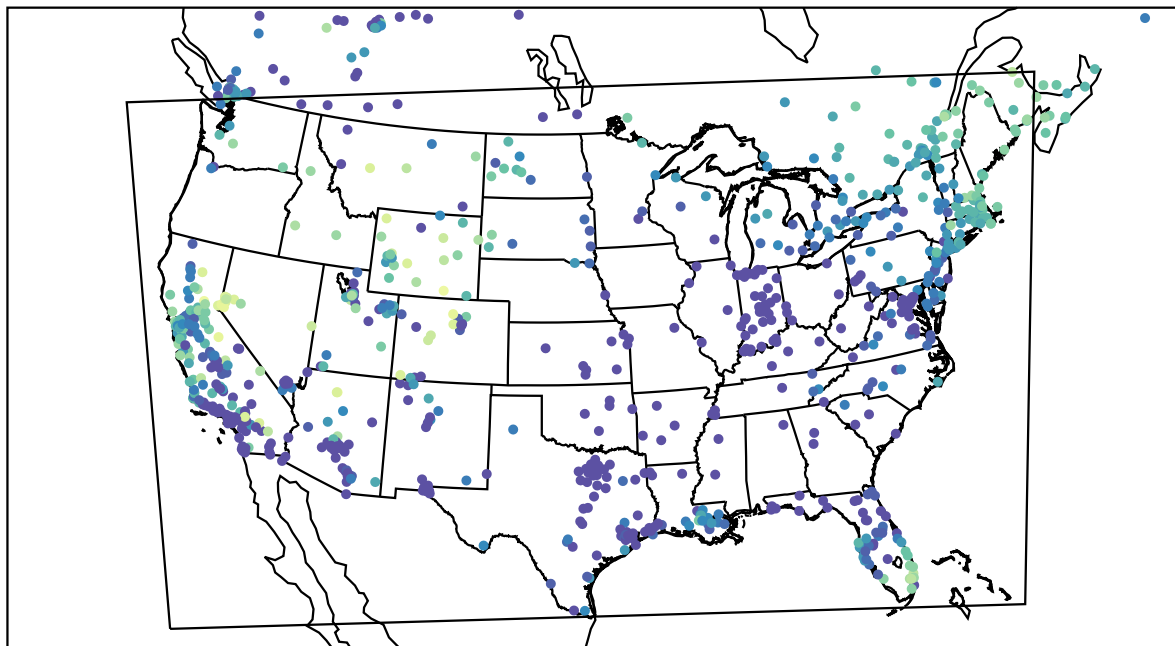
AirNOW (2022-12-10_15:00:00)
