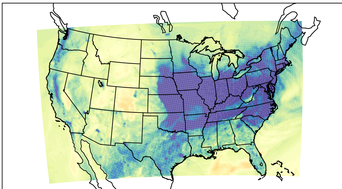
WRF (2022-12-09_01:00:00)
