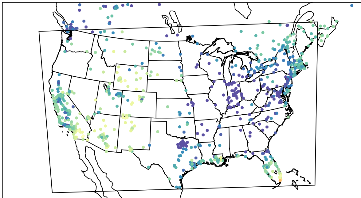
AirNOW (2022-12-10_21:00:00)
