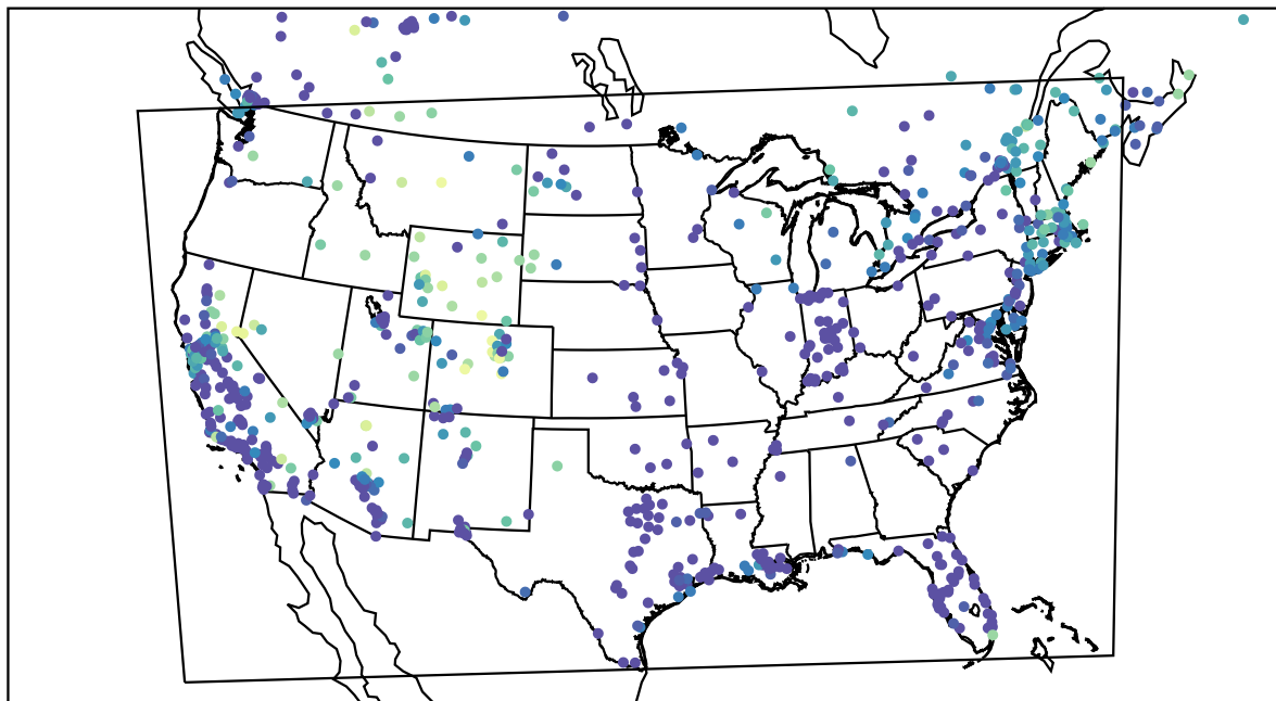
AirNOW (2022-12-09_07:00:00)
