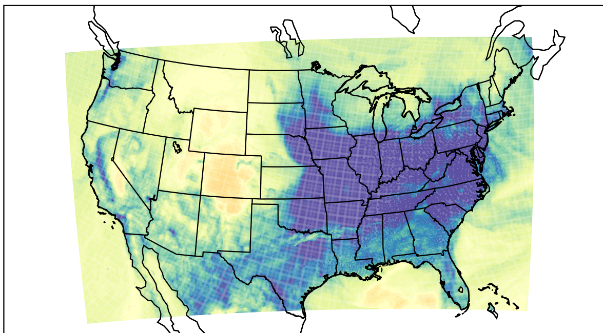
WRF (2022-12-09_08:00:00)
