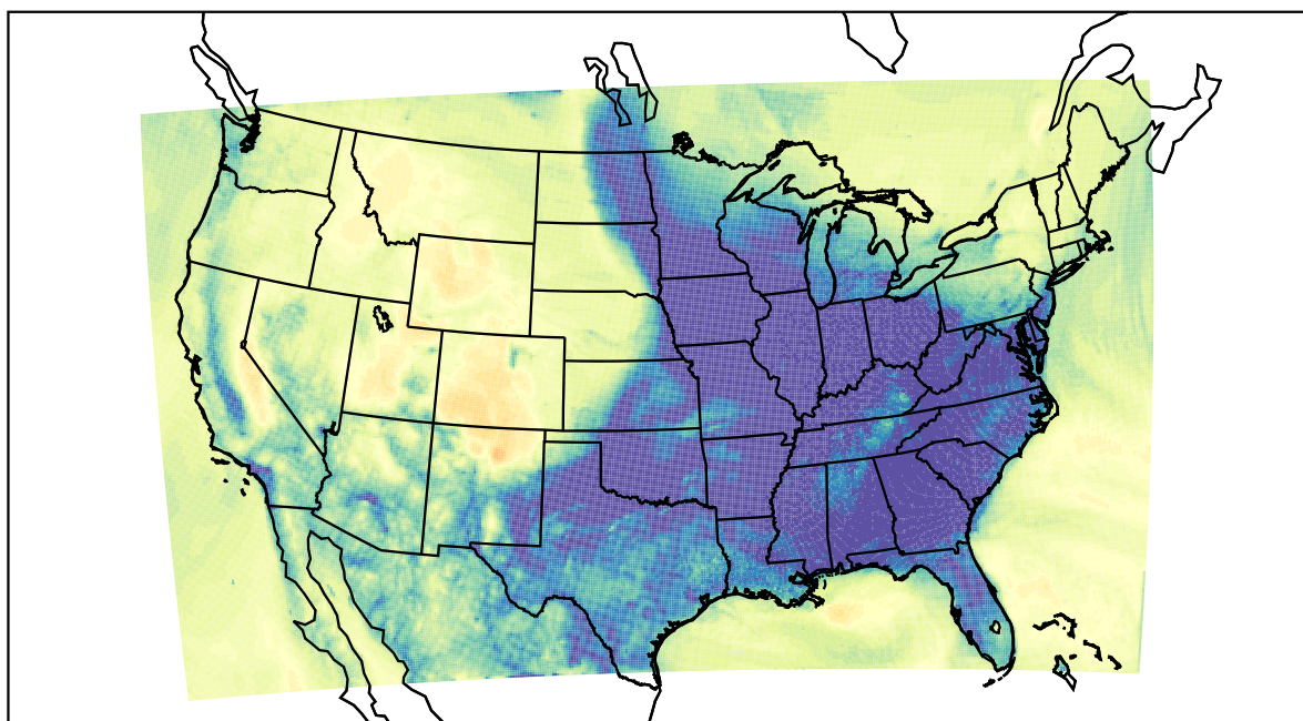
WRF (2022-12-10_13:00:00)
