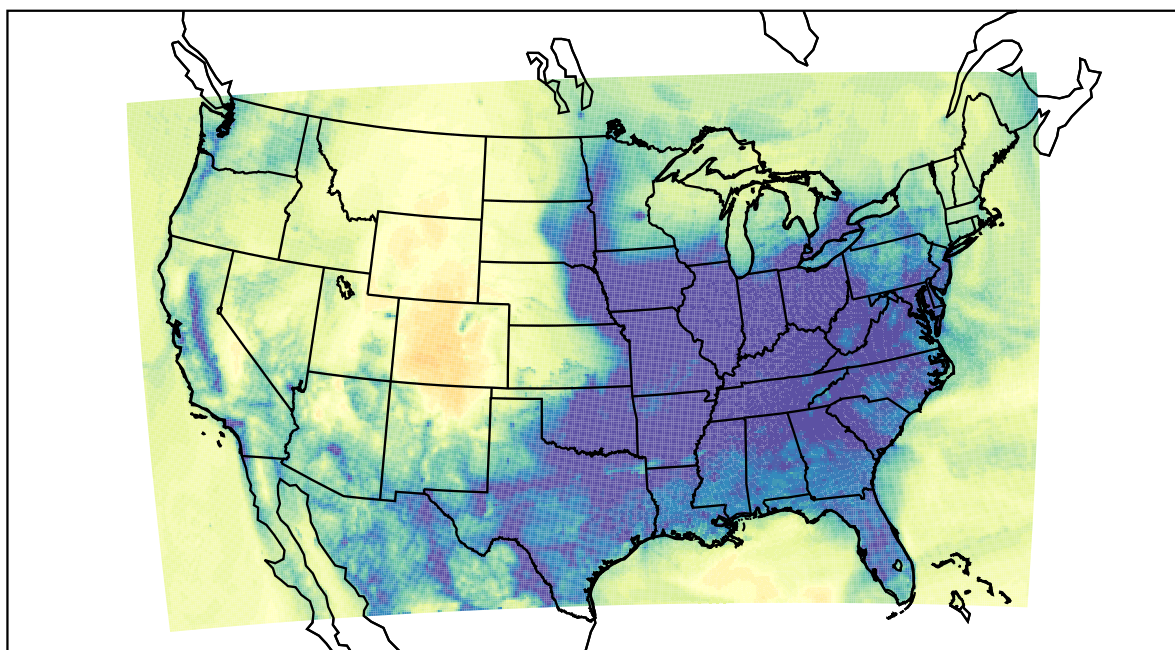
WRF (2022-12-09_14:00:00)
