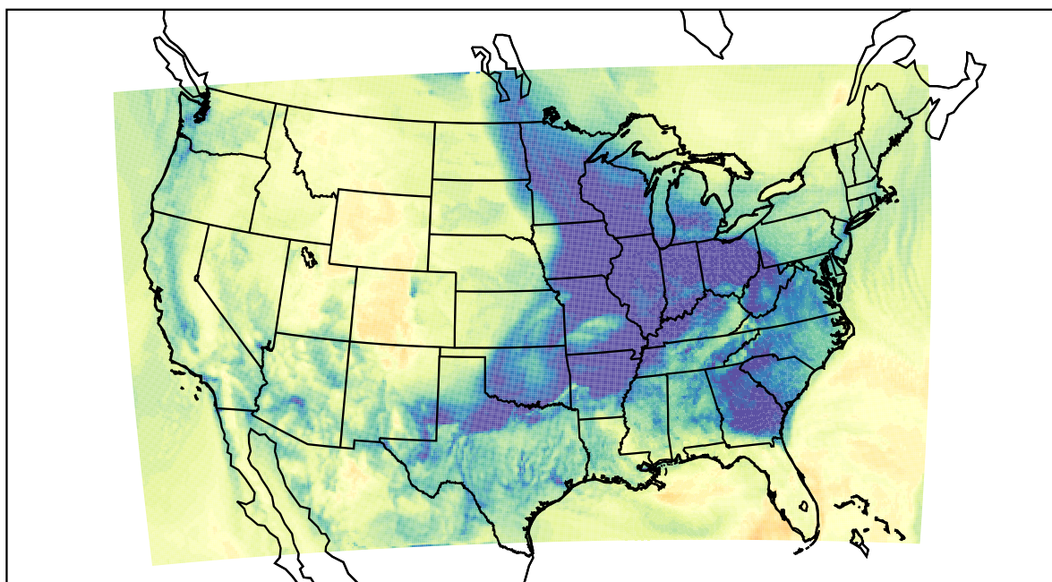
WRF (2022-12-10_18:00:00)
