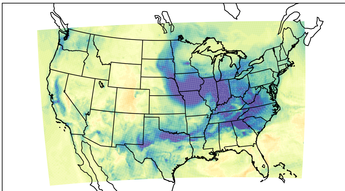
WRF (2022-12-09_19:00:00)
