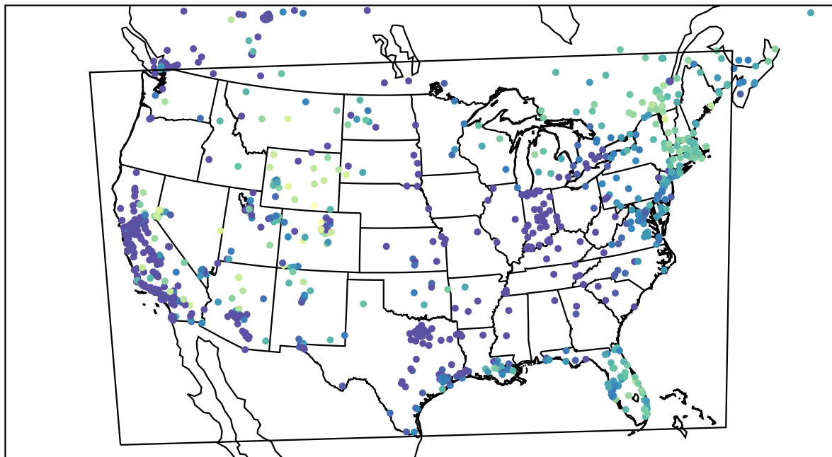
AirNOW (2022-12-09_16:00:00)
