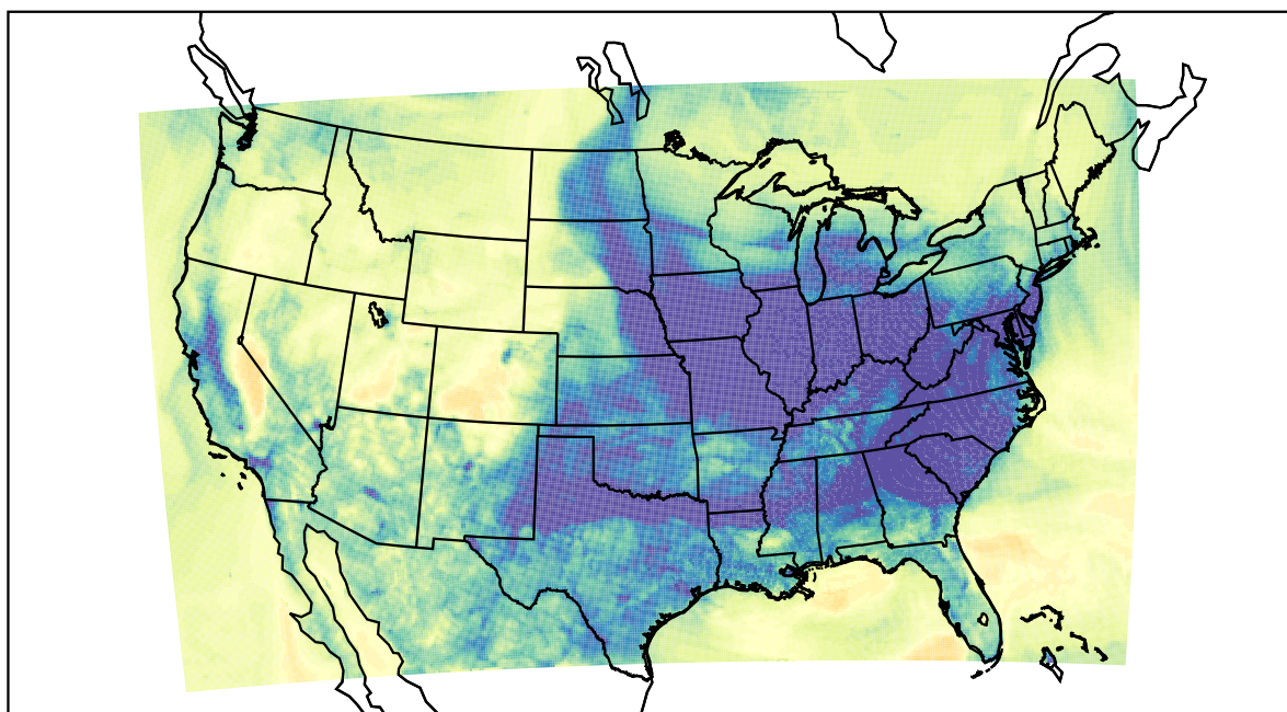
WRF (2022-12-10_04:00:00)
