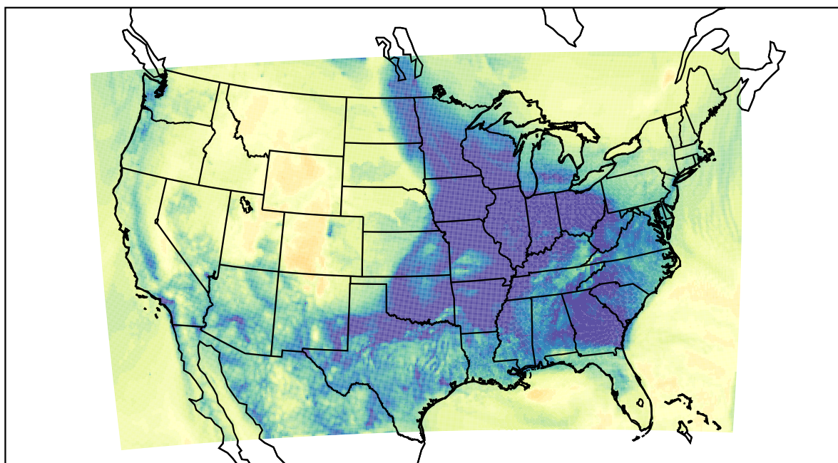
WRF (2022-12-10_16:00:00)
