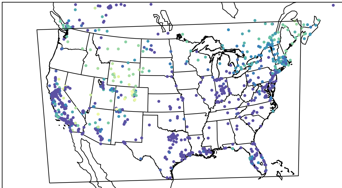
AirNOW (2022-12-10_05:00:00)
