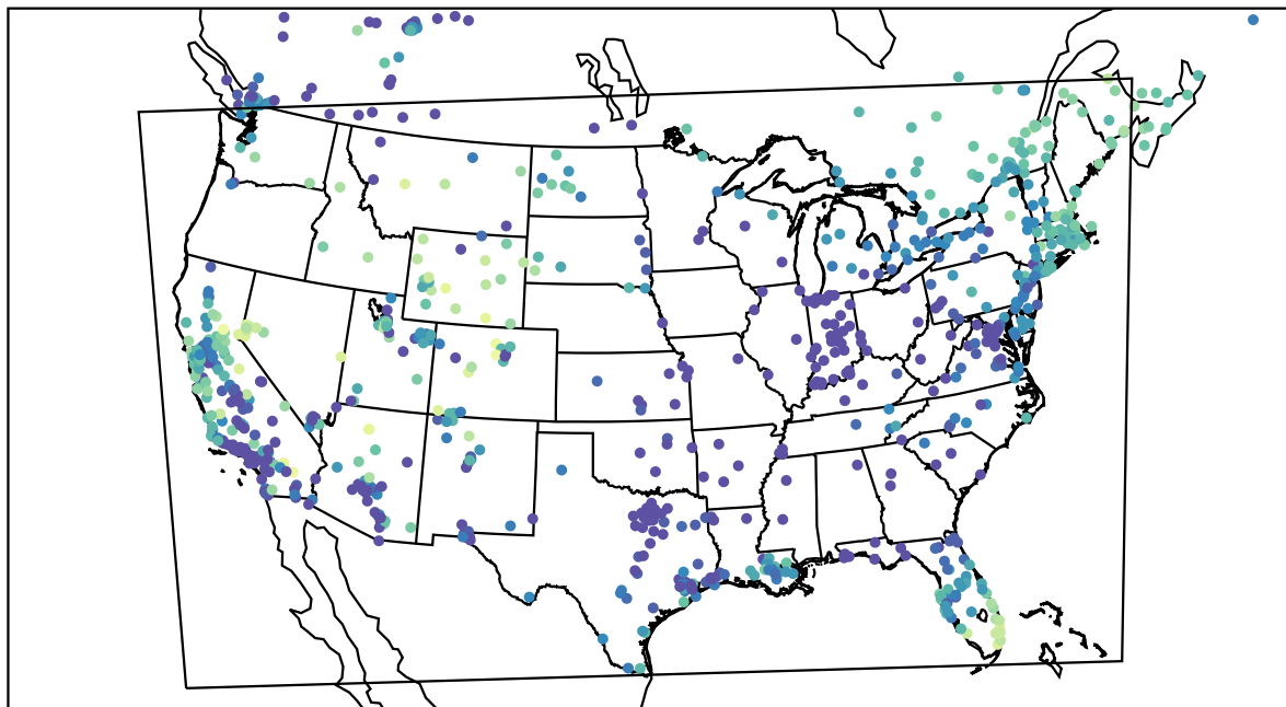
AirNOW (2022-12-10_16:00:00)
