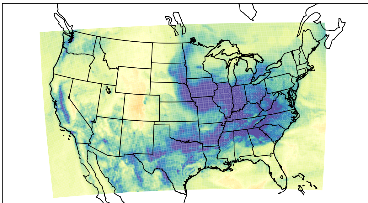
WRF (2022-12-09_17:00:00)
