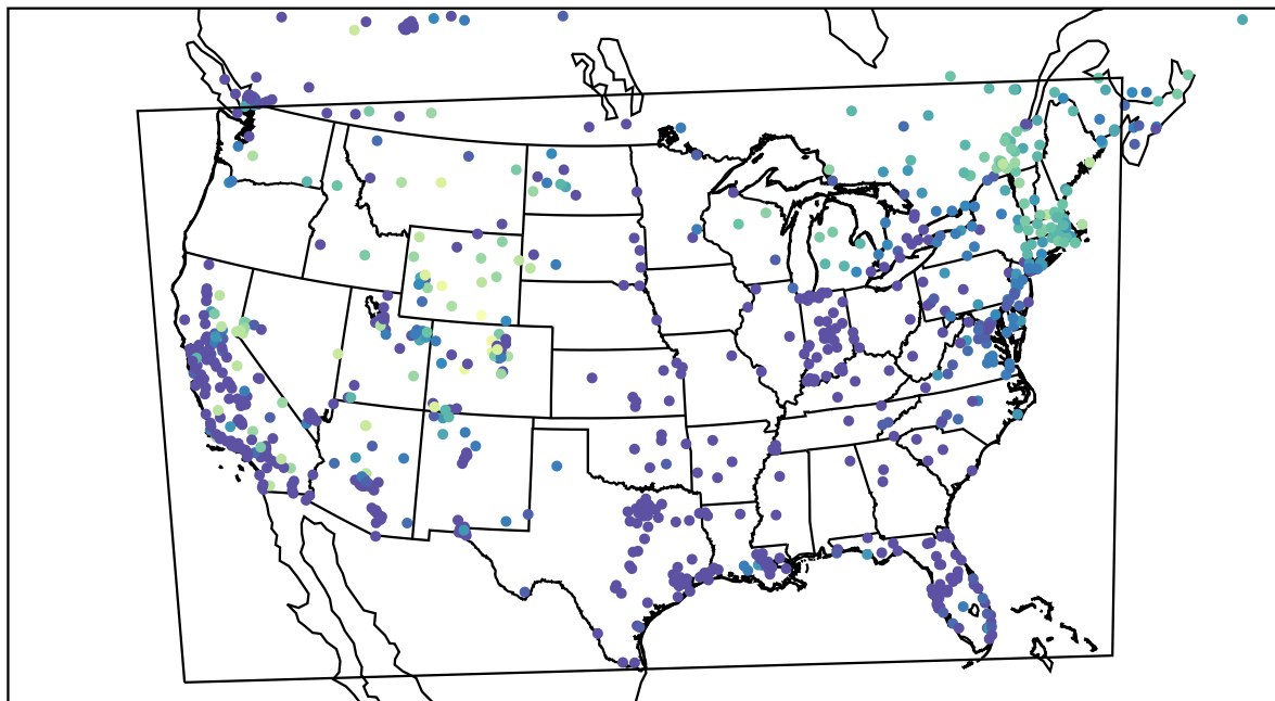
AirNOW (2022-12-09_14:00:00)
