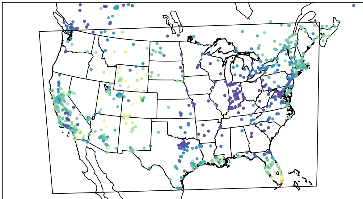
AirNOW (2022-12-10_19:00:00)
