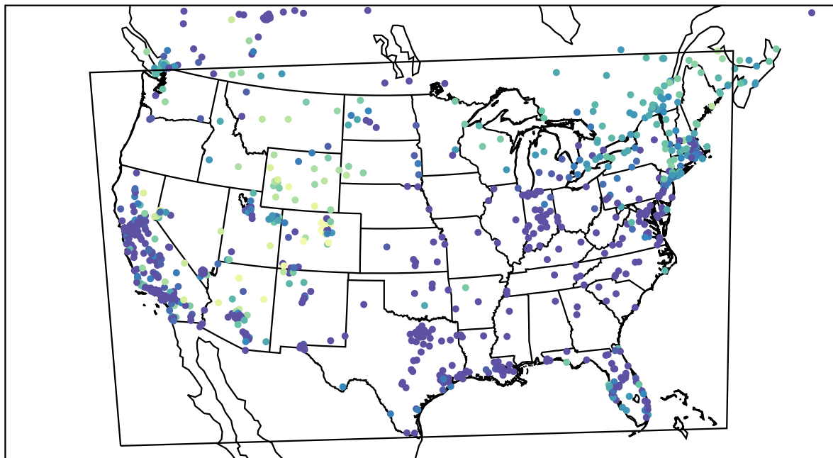
AirNOW (2022-12-10_02:00:00)
