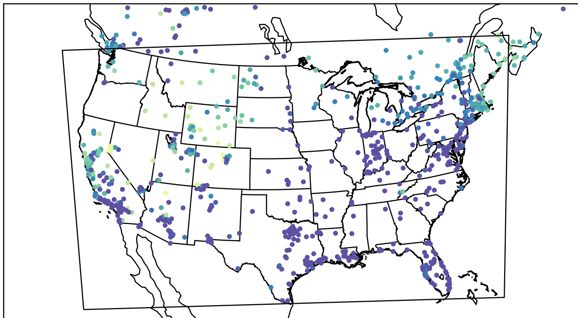
AirNOW (2022-12-10_12:00:00)
