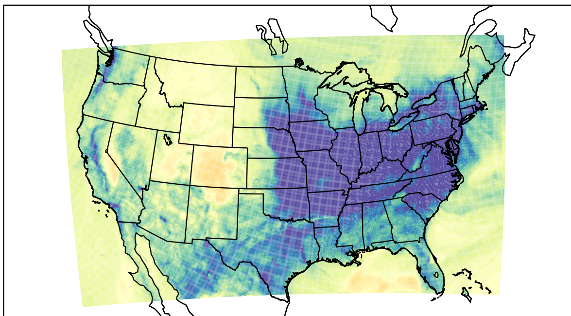
WRF (2022-12-09_05:00:00)
