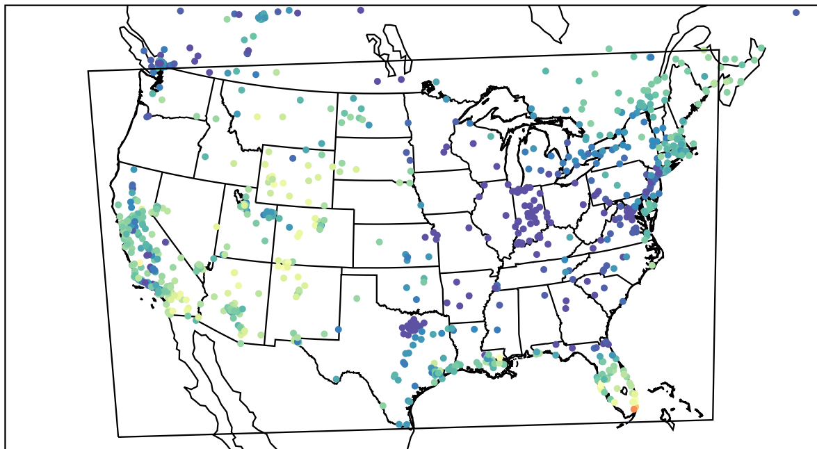
AirNOW (2022-12-10_20:00:00)
