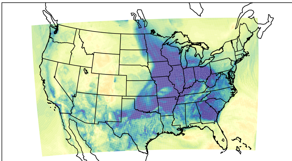
WRF (2022-12-10_17:00:00)
