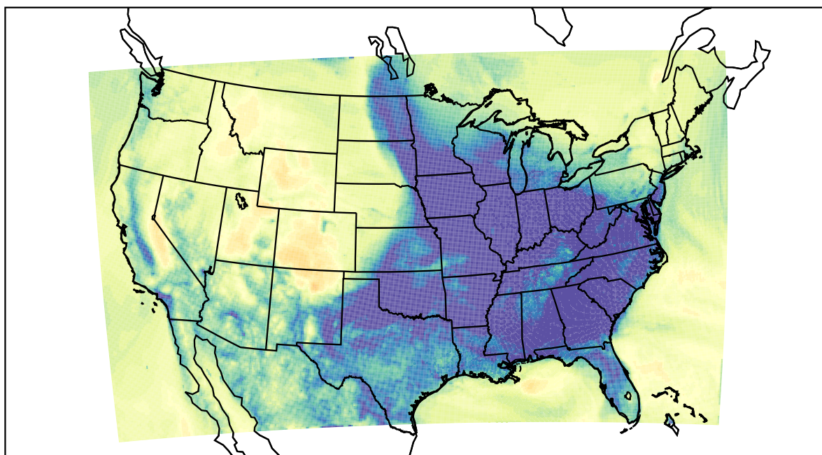
WRF (2022-12-10_12:00:00)
