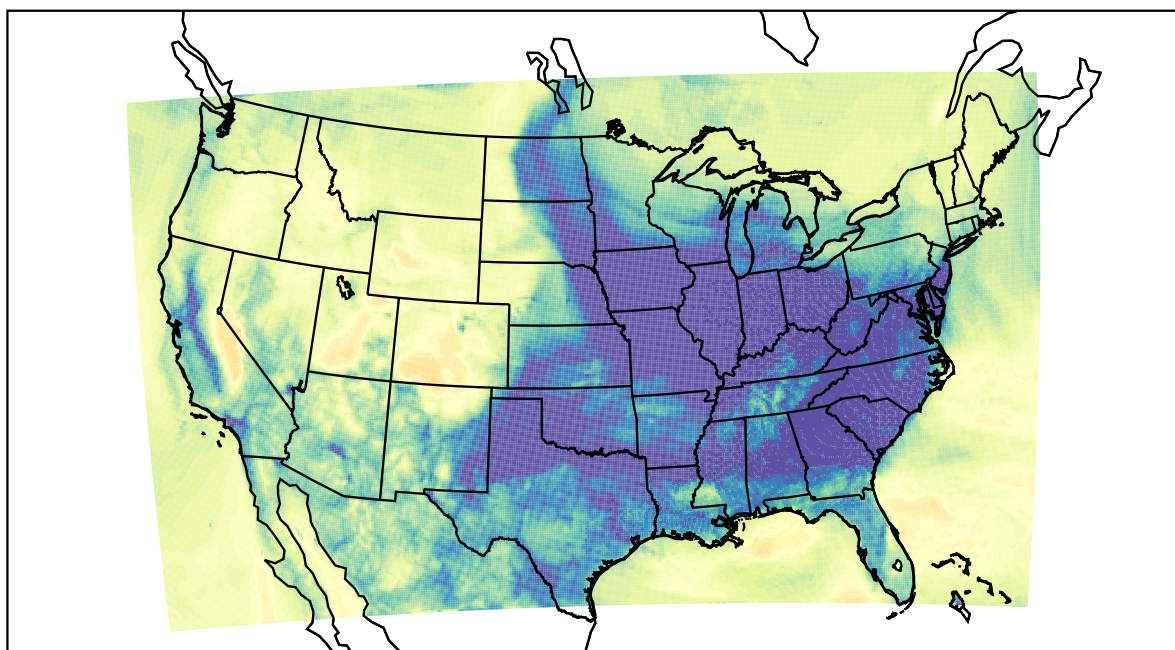
WRF (2022-12-10_07:00:00)
