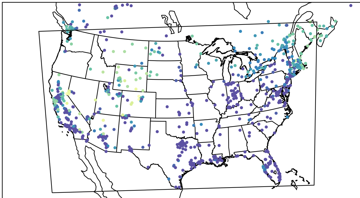
AirNOW (2022-12-10_10:00:00)
