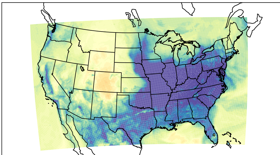
WRF (2022-12-09_12:00:00)
