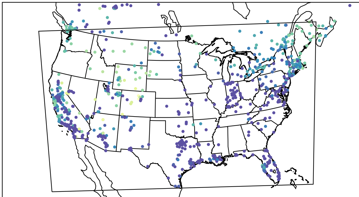
AirNOW (2022-12-10_08:00:00)
