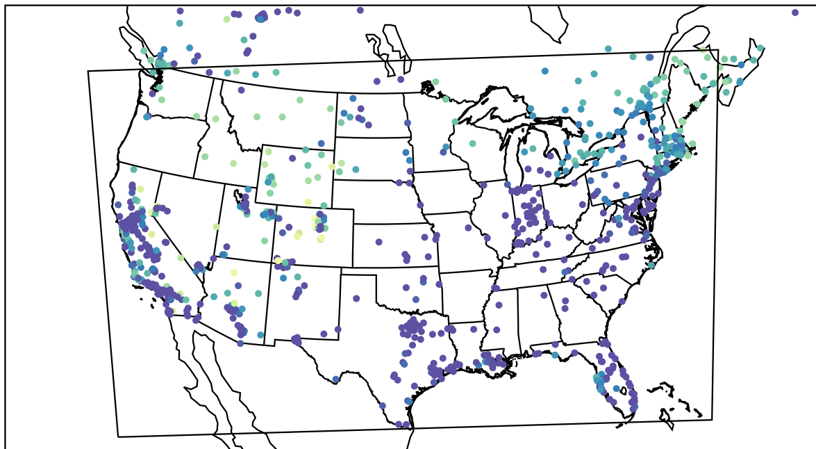
AirNOW (2022-12-10_06:00:00)
