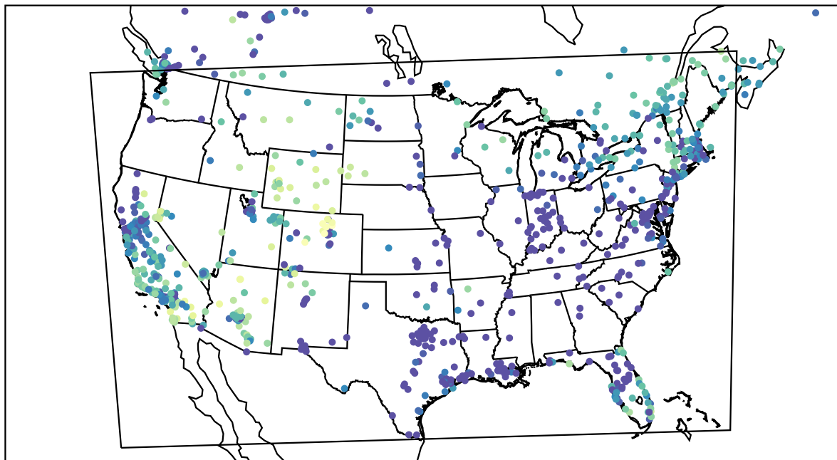
AirNOW (2022-12-10_00:00:00)
