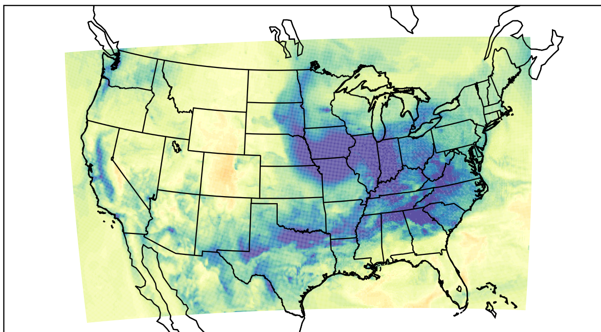
WRF (2022-12-09_18:00:00)
