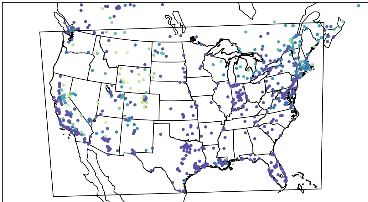
AirNOW (2022-12-09_11:00:00)
