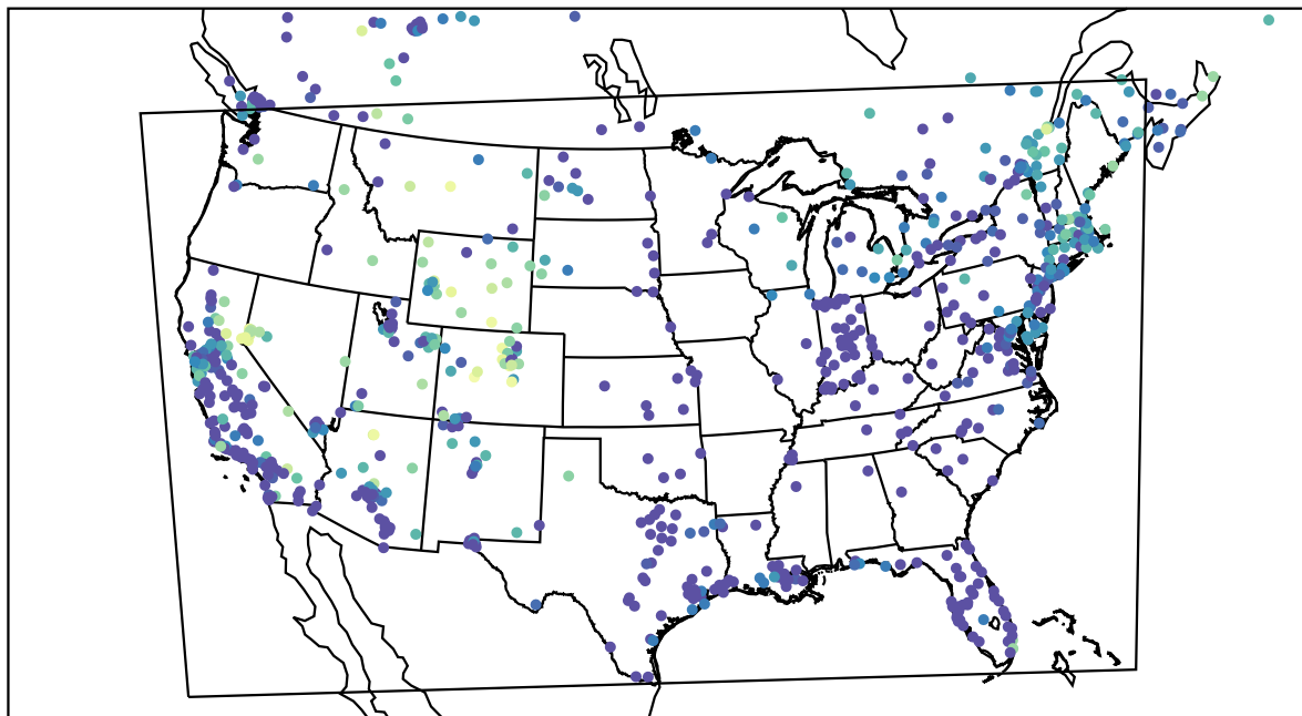
AirNOW (2022-12-09_06:00:00)
