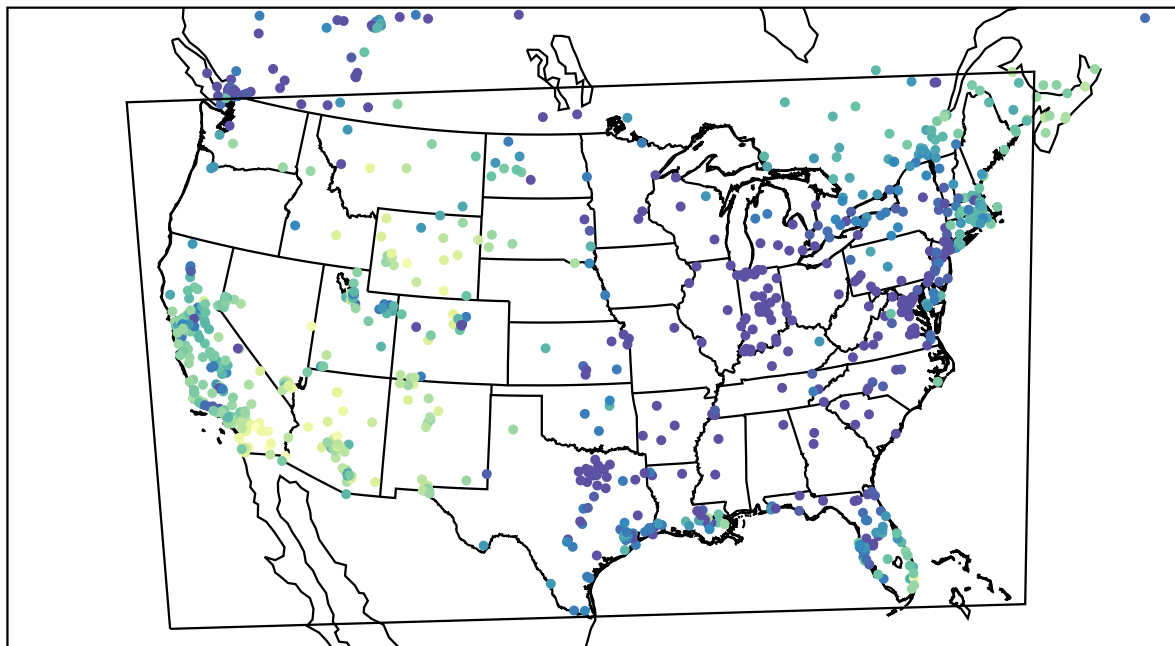
AirNOW (2022-12-10_23:00:00)
