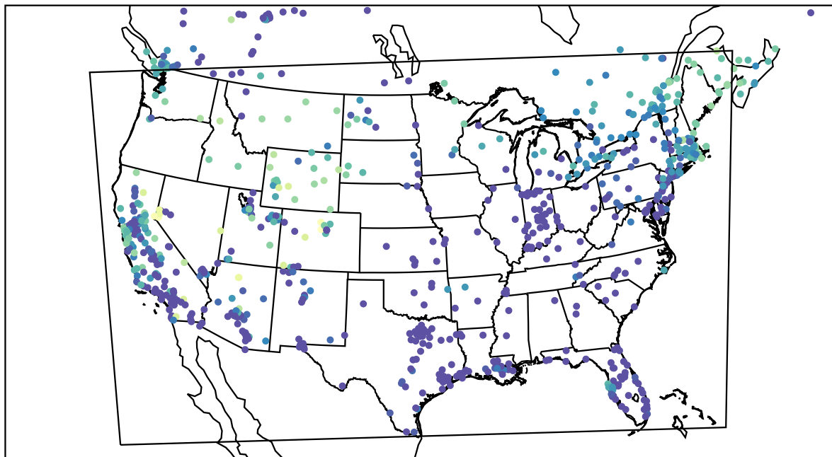
AirNOW (2022-12-10_09:00:00)
