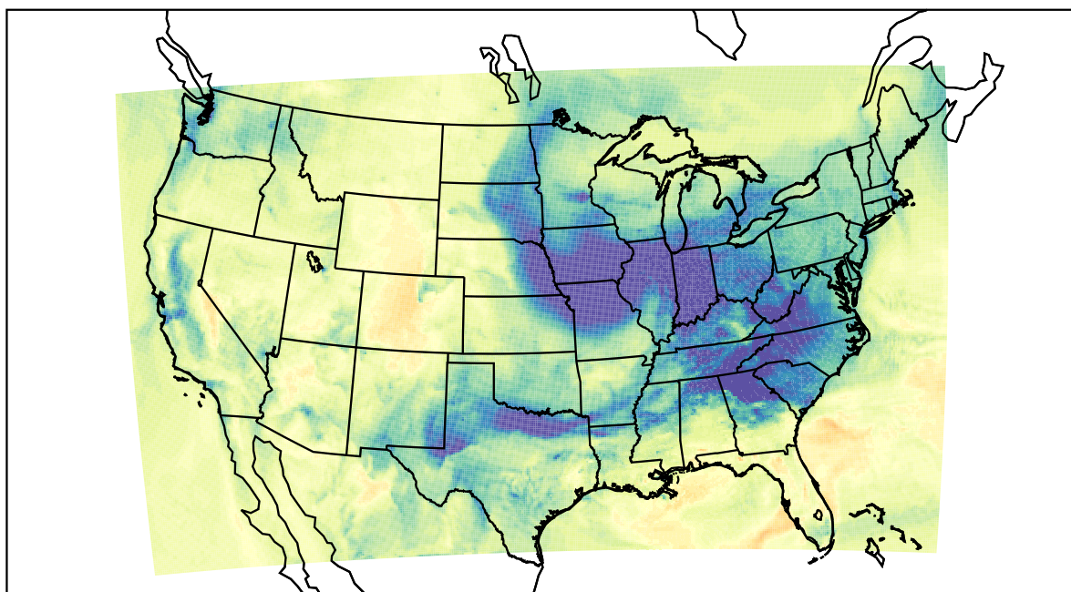
WRF (2022-12-09_20:00:00)
