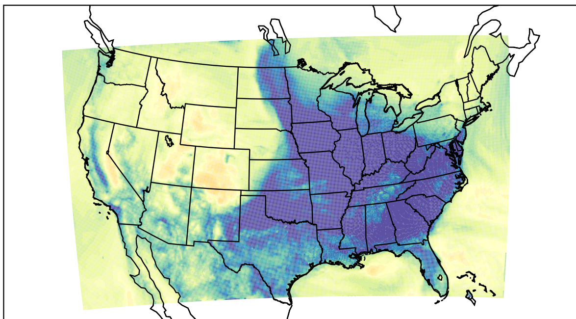
WRF (2022-12-10_11:00:00)
