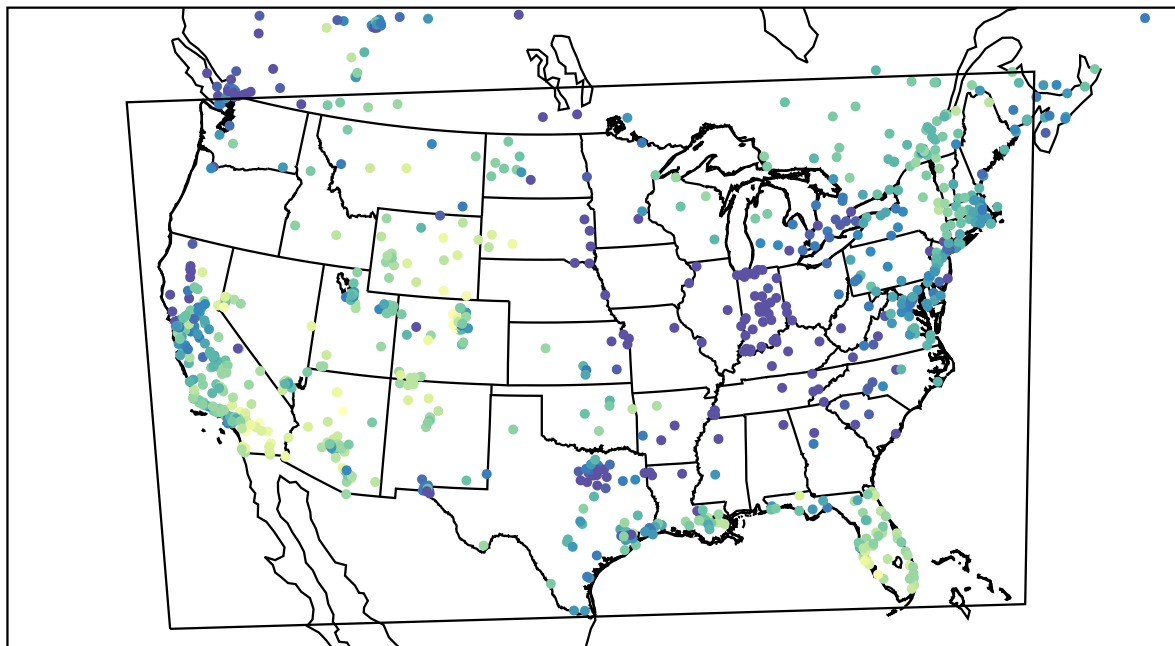
AirNOW (2022-12-09_20:00:00)
