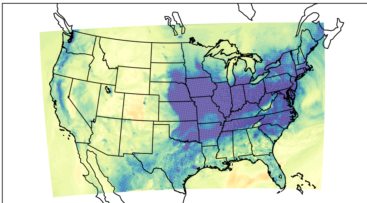
WRF (2022-12-09_00:00:00)
