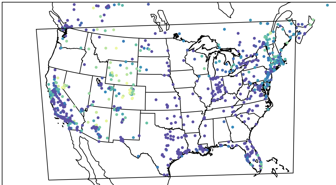
AirNOW (2022-12-09_03:00:00)
