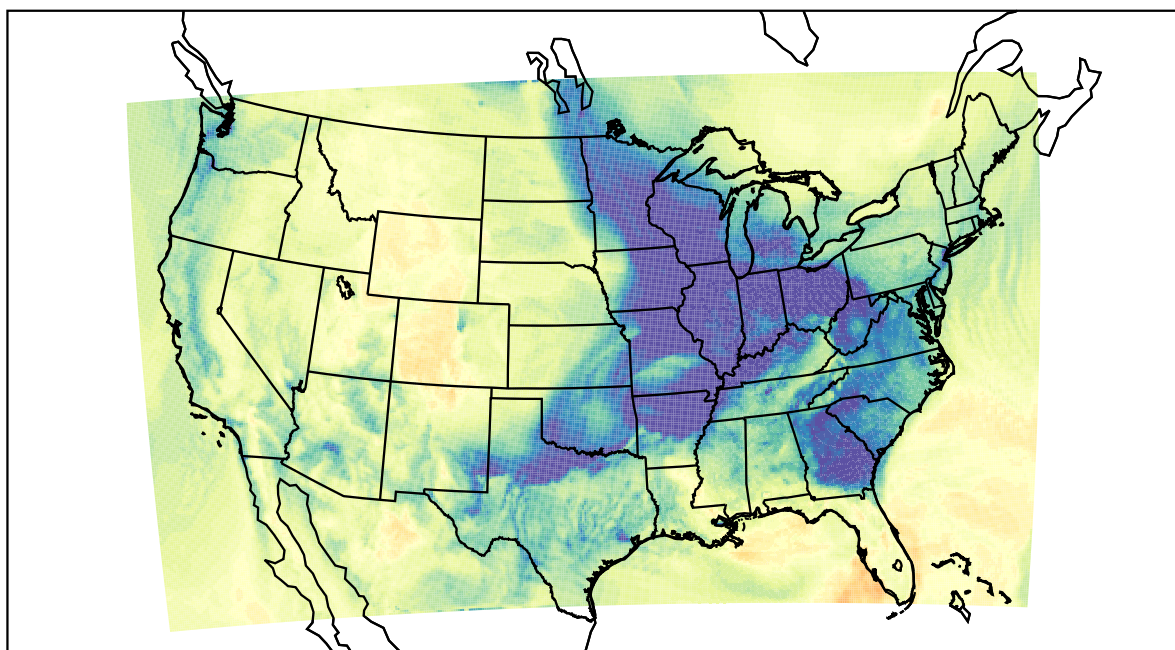
WRF (2022-12-10_19:00:00)
