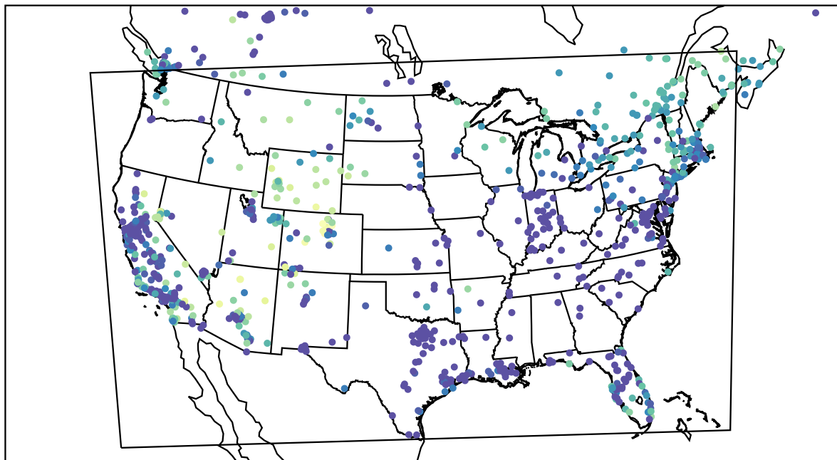
AirNOW (2022-12-10_01:00:00)
