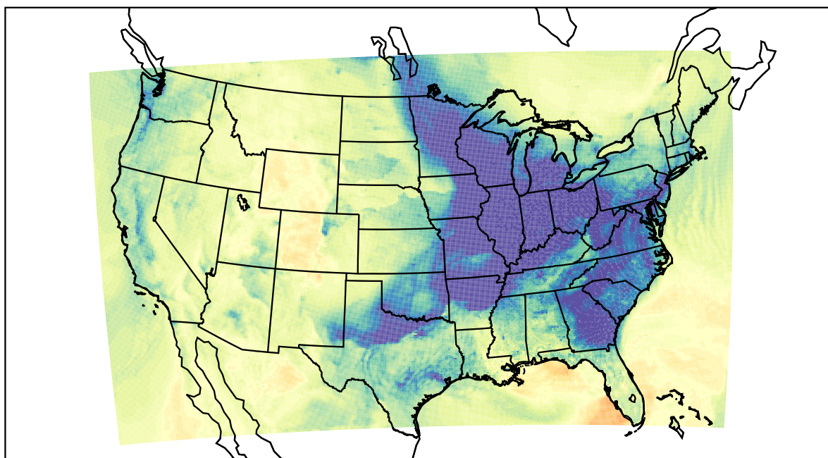
WRF (2022-12-10_22:00:00)
