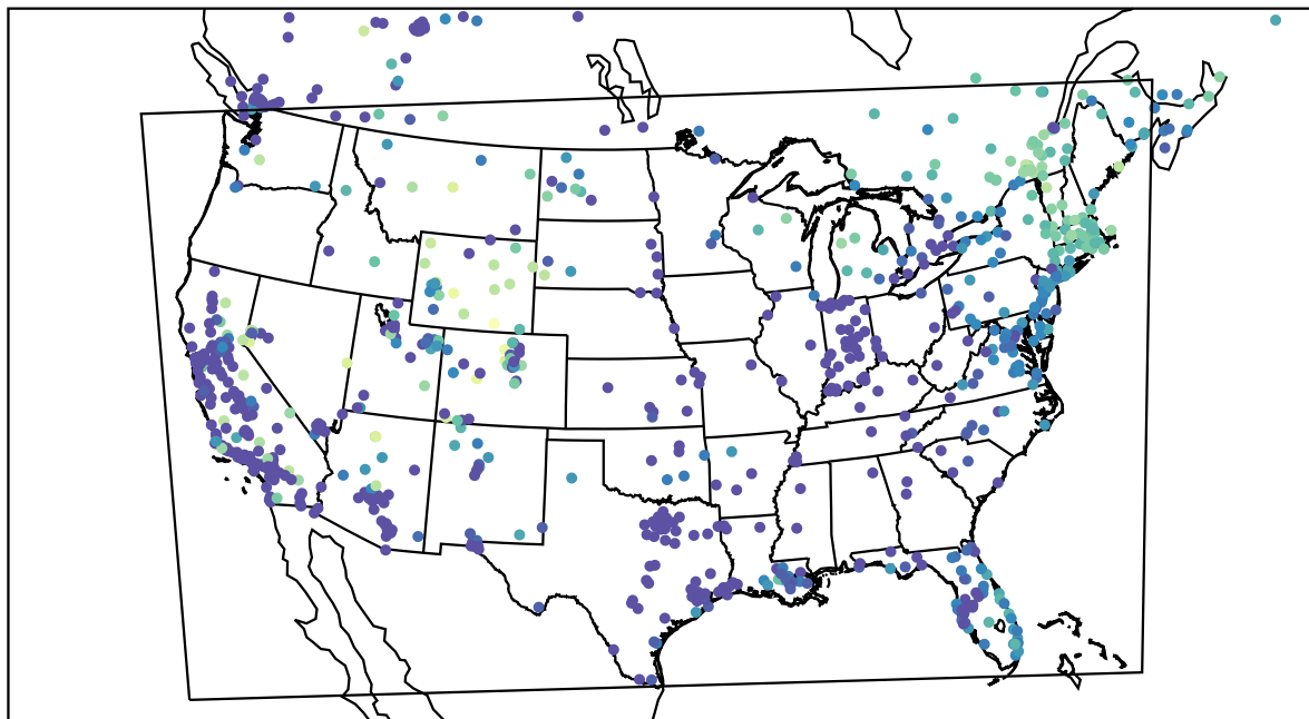
AirNOW (2022-12-09_15:00:00)
