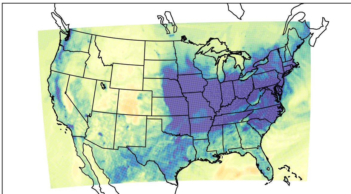
WRF (2022-12-09_02:00:00)
