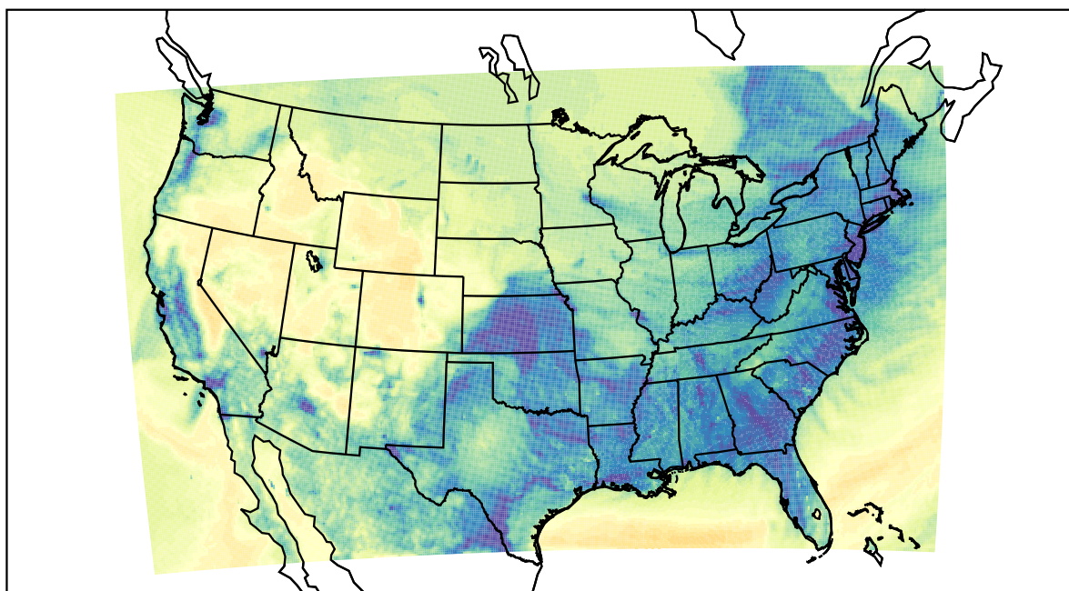
WRF (2022-12-19_04:00:00)
