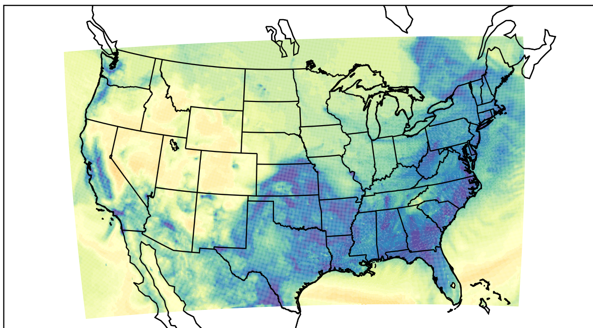
WRF (2022-12-19_08:00:00)
