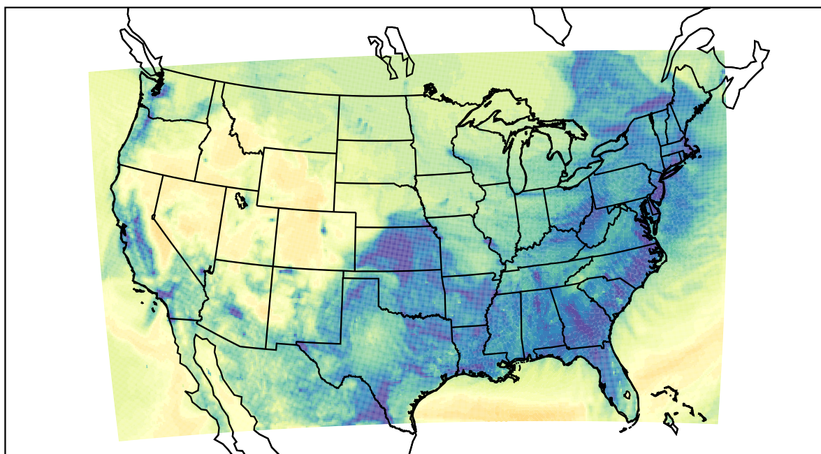
WRF (2022-12-19_05:00:00)
