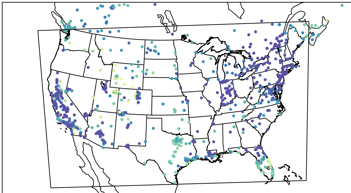
AirNOW (2022-12-19_02:00:00)
