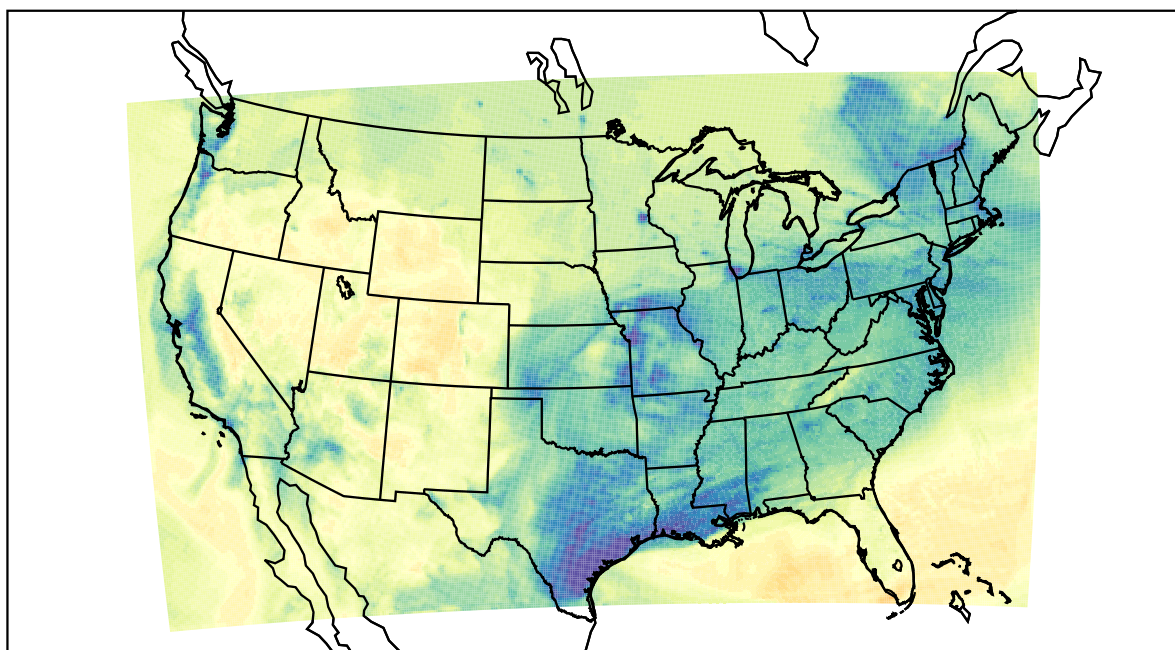
WRF (2022-12-19_20:00:00)
