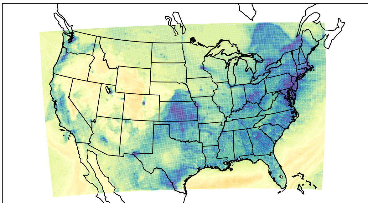
WRF (2022-12-19_00:00:00)
