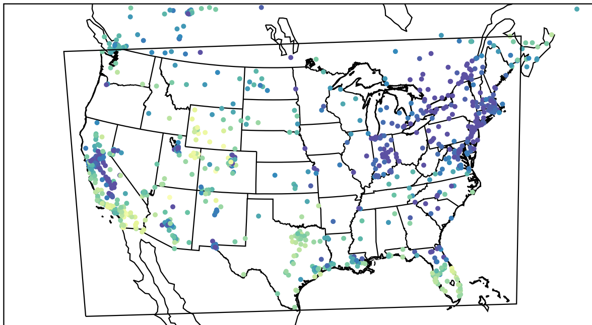
AirNOW (2022-12-18_23:00:00)
