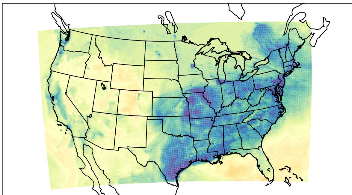
WRF (2022-12-19_22:00:00)
