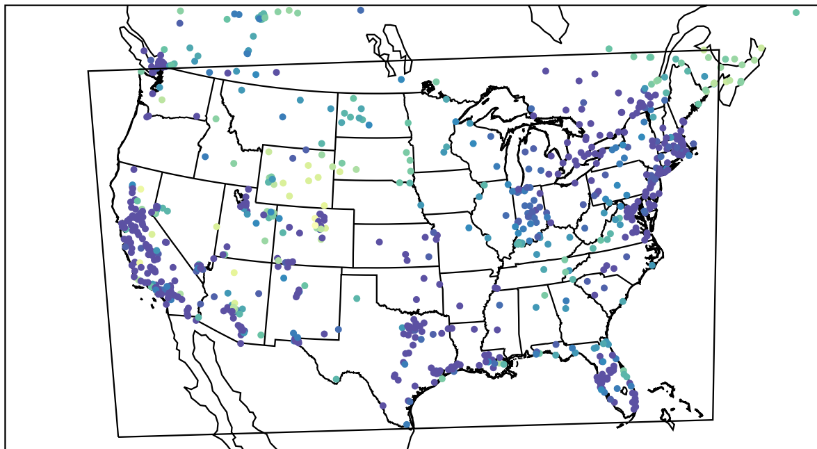
AirNOW (2022-12-18_09:00:00)
