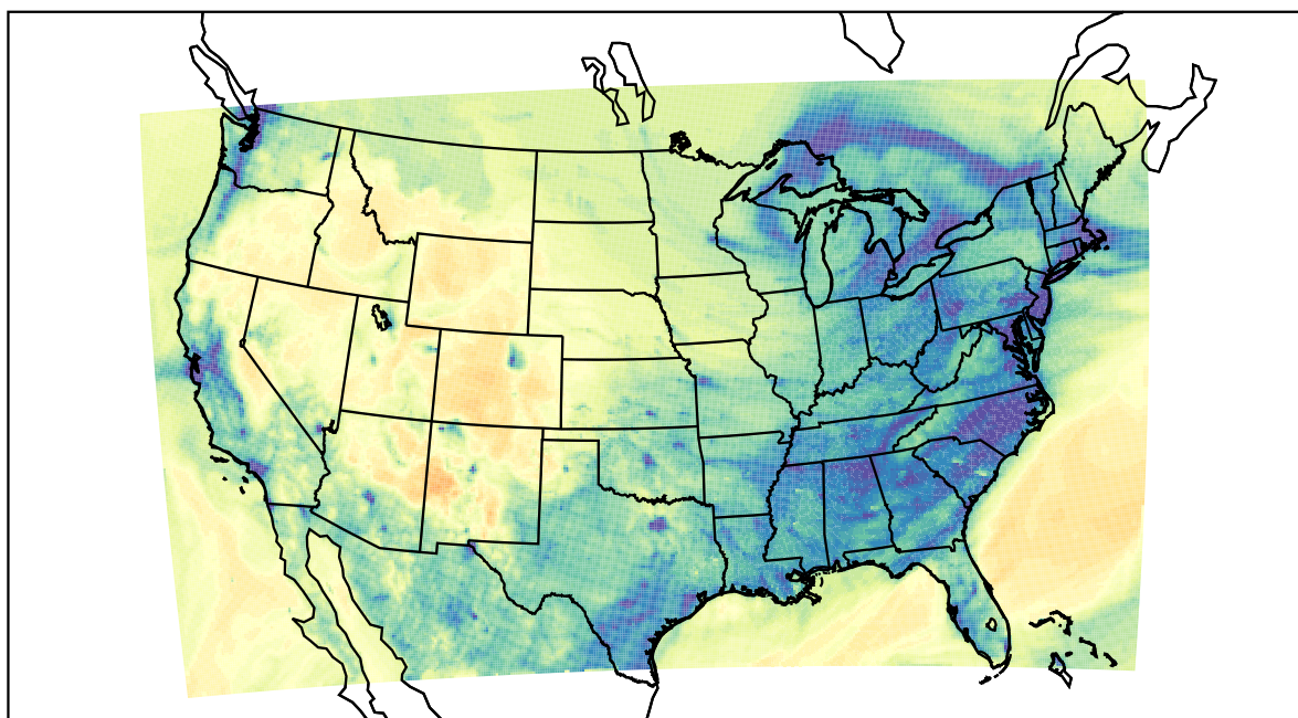
WRF (2022-12-18_03:00:00)
