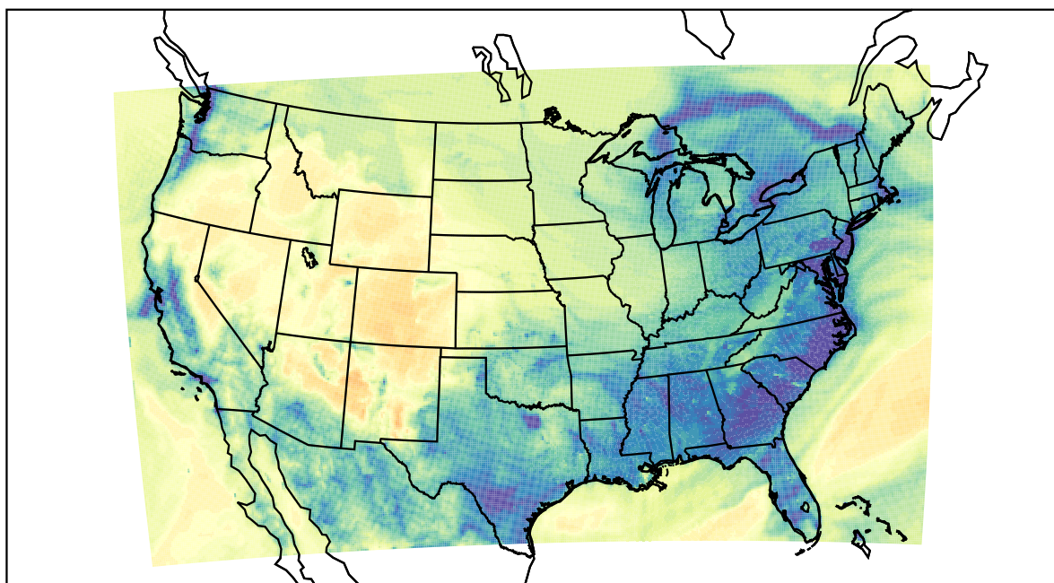
WRF (2022-12-18_09:00:00)
