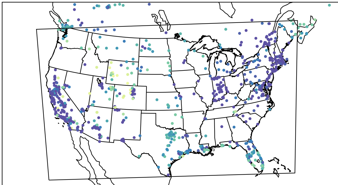
AirNOW (2022-12-19_08:00:00)
