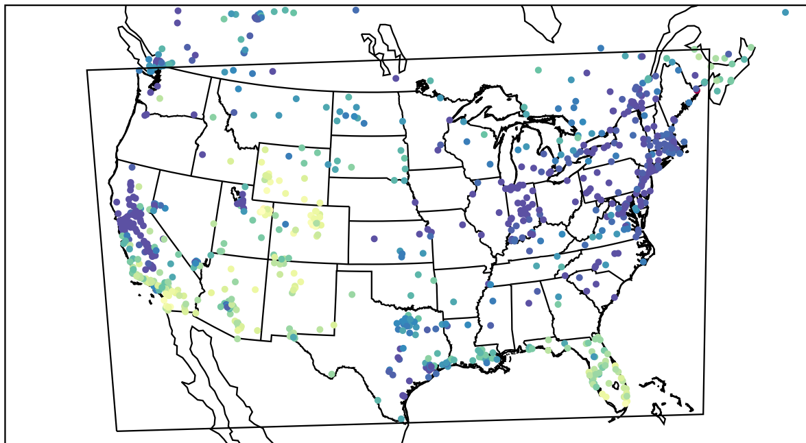
AirNOW (2022-12-19_22:00:00)
