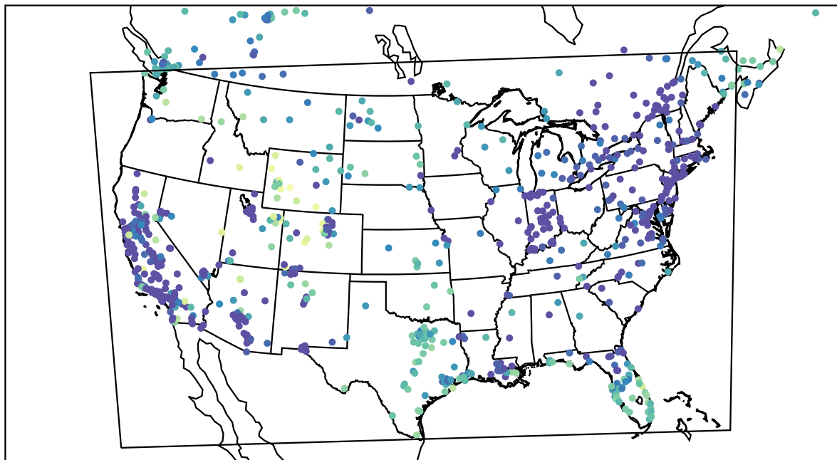
AirNOW (2022-12-19_04:00:00)
