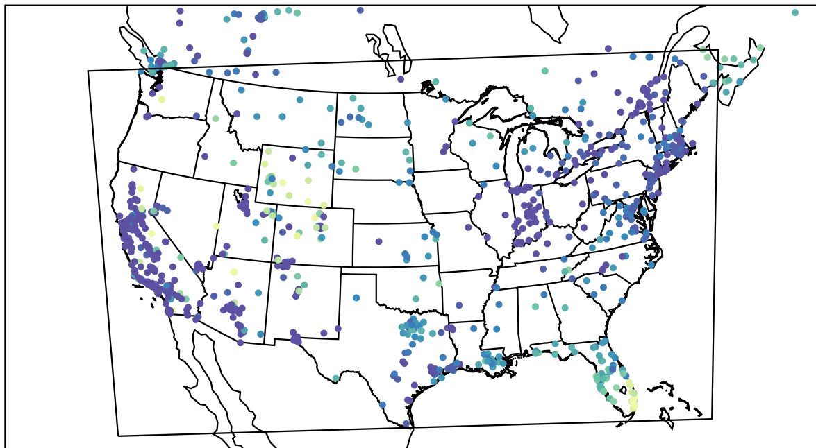
AirNOW (2022-12-19_15:00:00)
