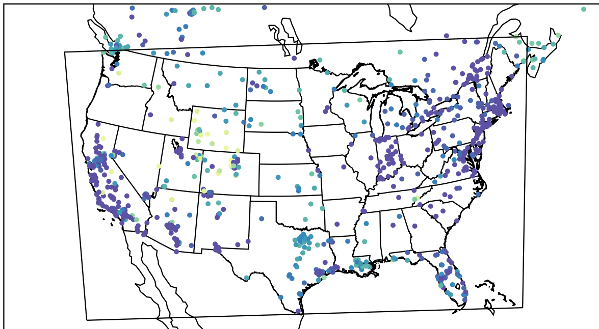
AirNOW (2022-12-19_11:00:00)
