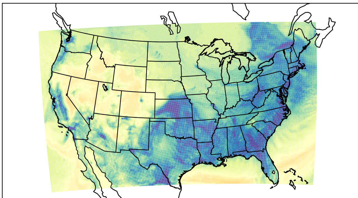
WRF (2022-12-19_06:00:00)
