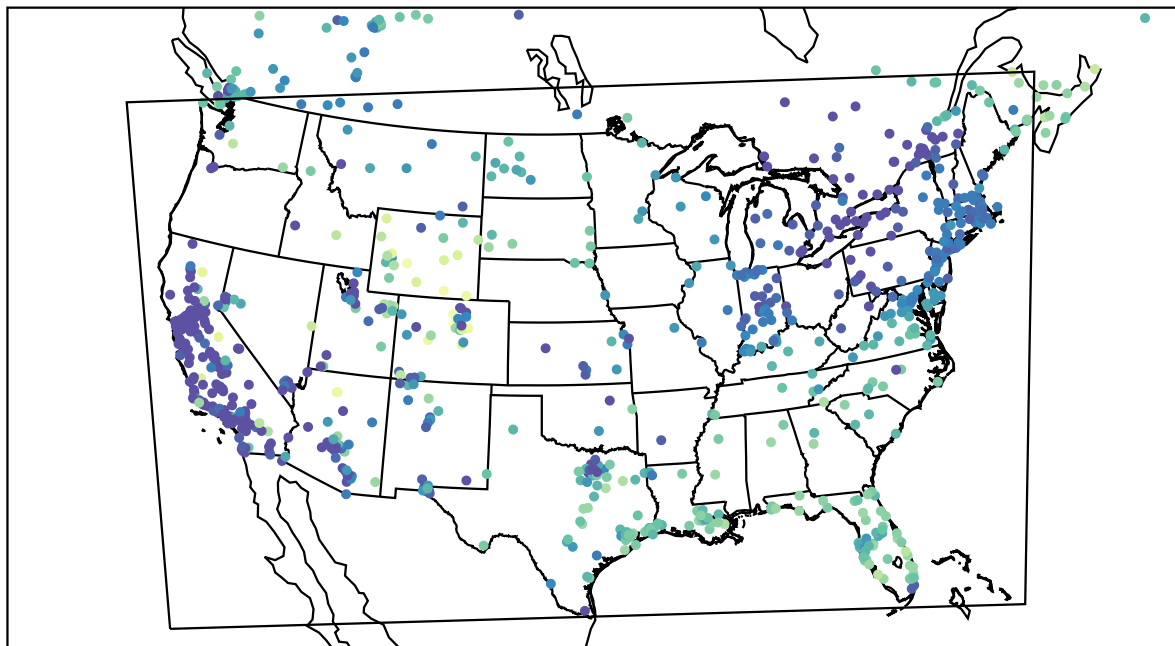
AirNOW (2022-12-18_16:00:00)
