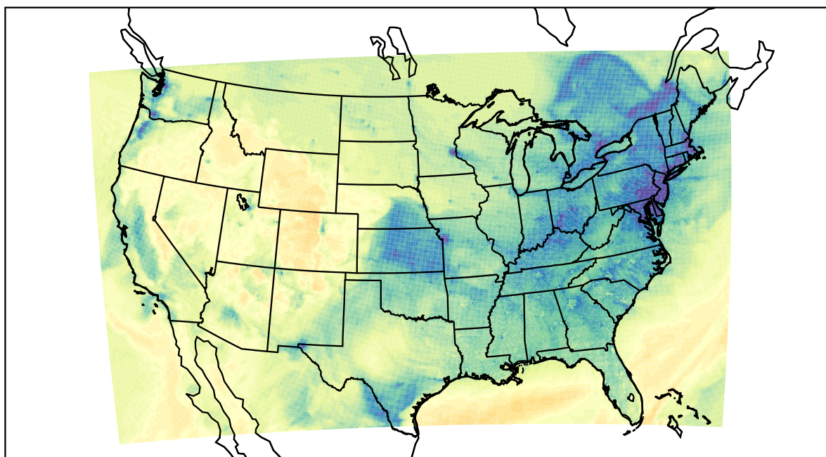
WRF (2022-12-18_22:00:00)
