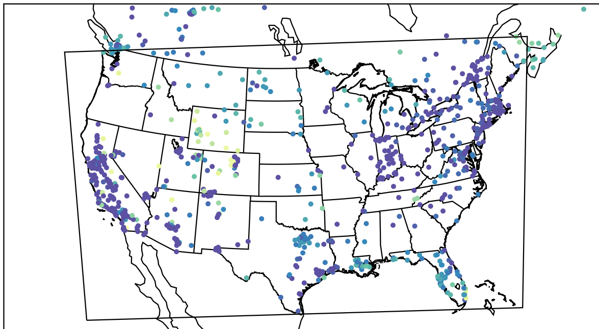
AirNOW (2022-12-19_14:00:00)
