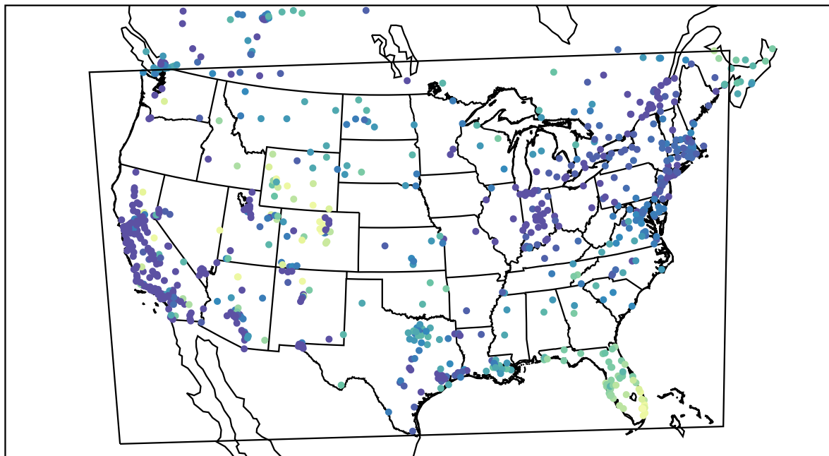
AirNOW (2022-12-19_16:00:00)
