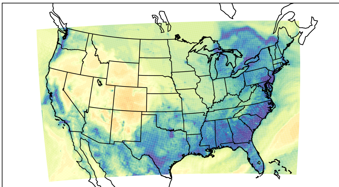
WRF (2022-12-18_13:00:00)
