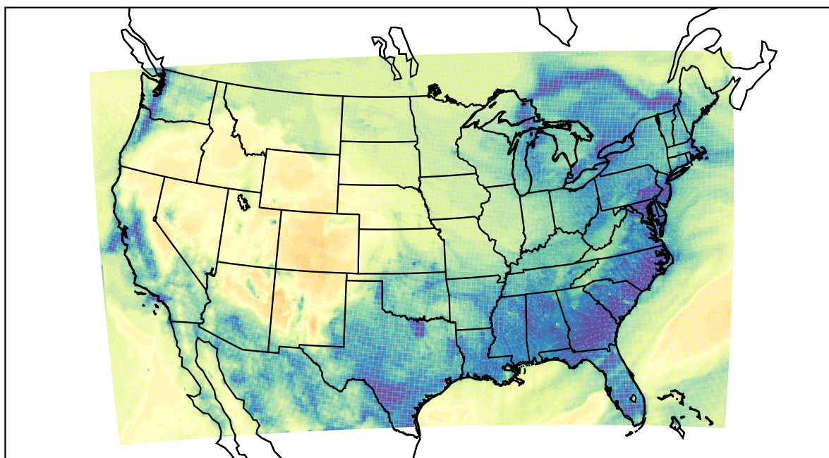
WRF (2022-12-18_11:00:00)
