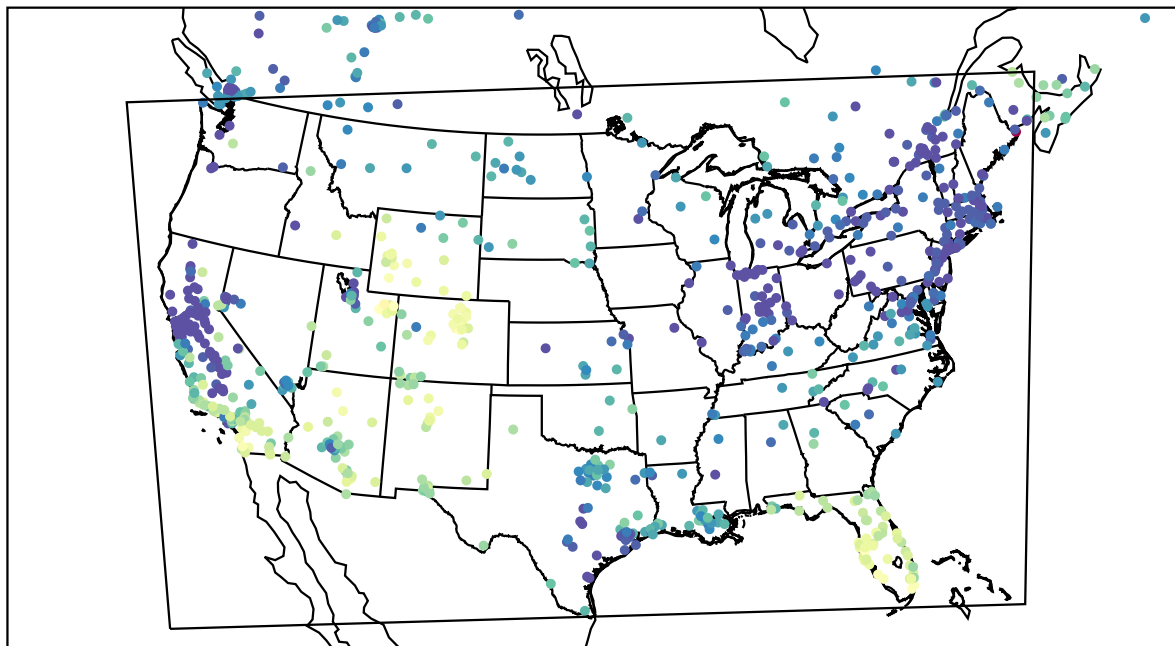
AirNOW (2022-12-19_21:00:00)
