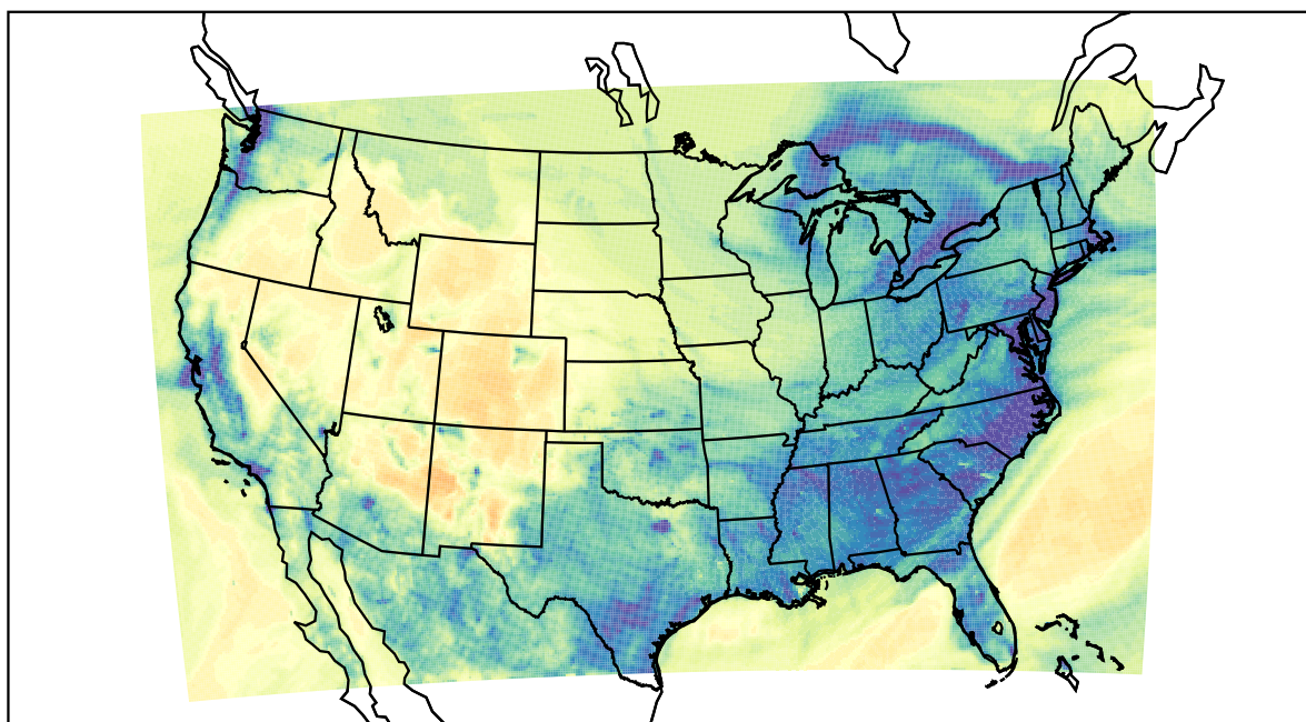
WRF (2022-12-18_06:00:00)
