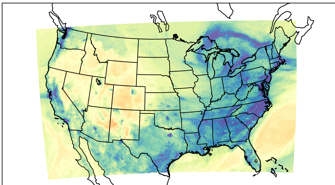
WRF (2022-12-18_04:00:00)
