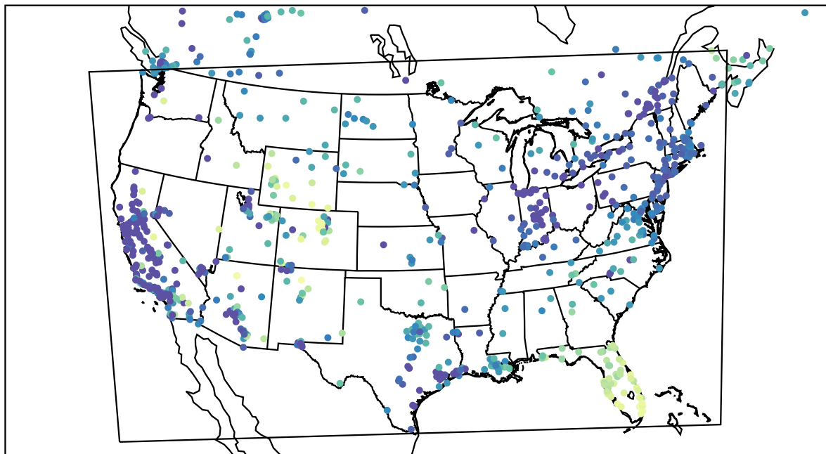
AirNOW (2022-12-19_17:00:00)
