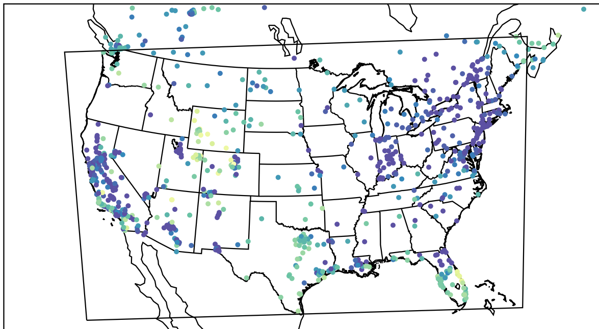
AirNOW (2022-12-19_01:00:00)
