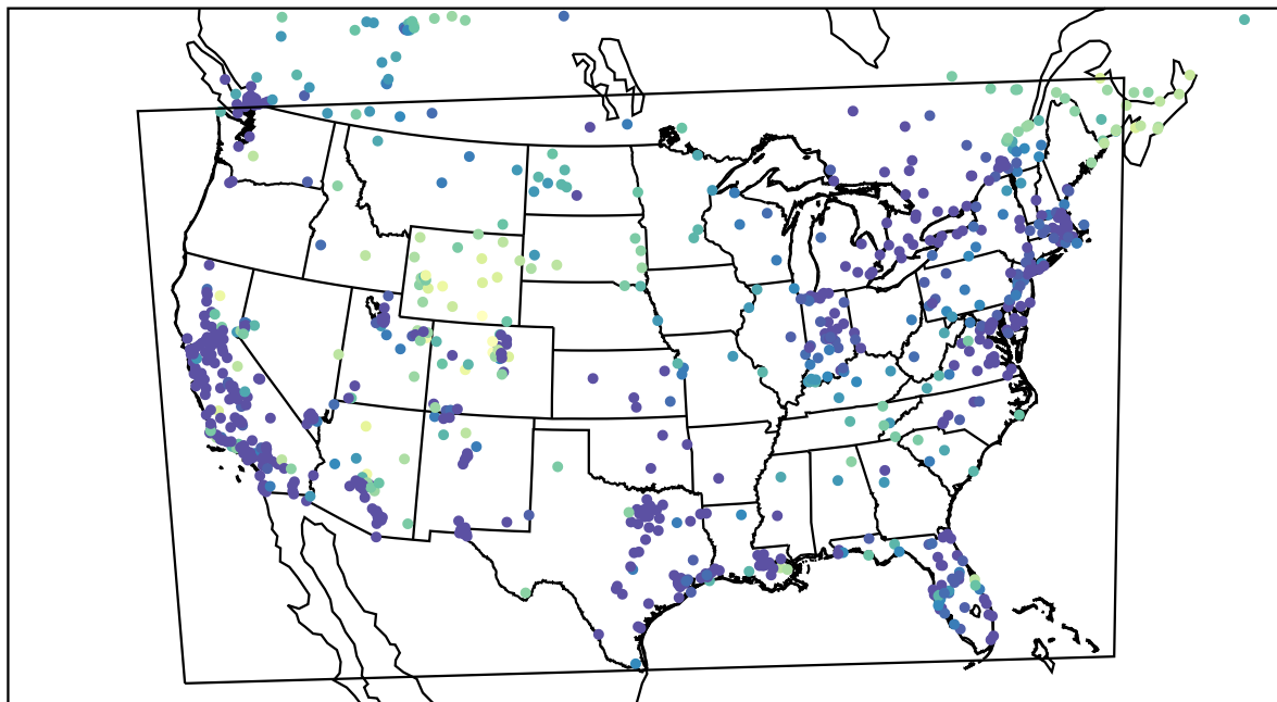
AirNOW (2022-12-18_05:00:00)
