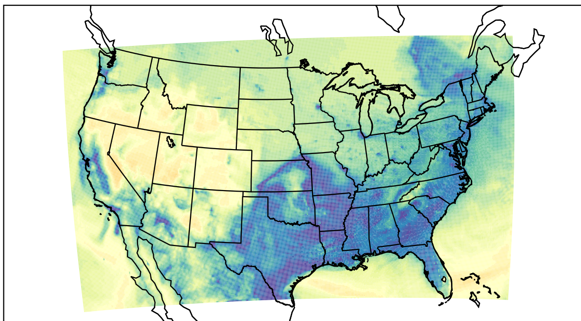
WRF (2022-12-19_14:00:00)
