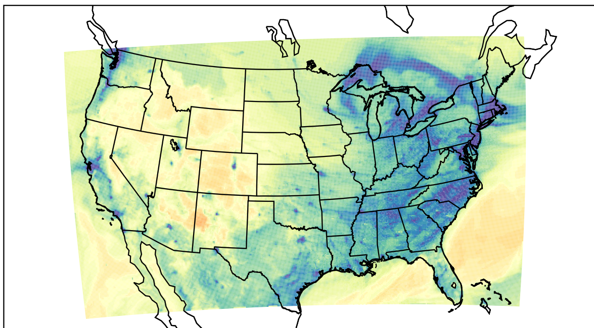
WRF (2022-12-18_01:00:00)
