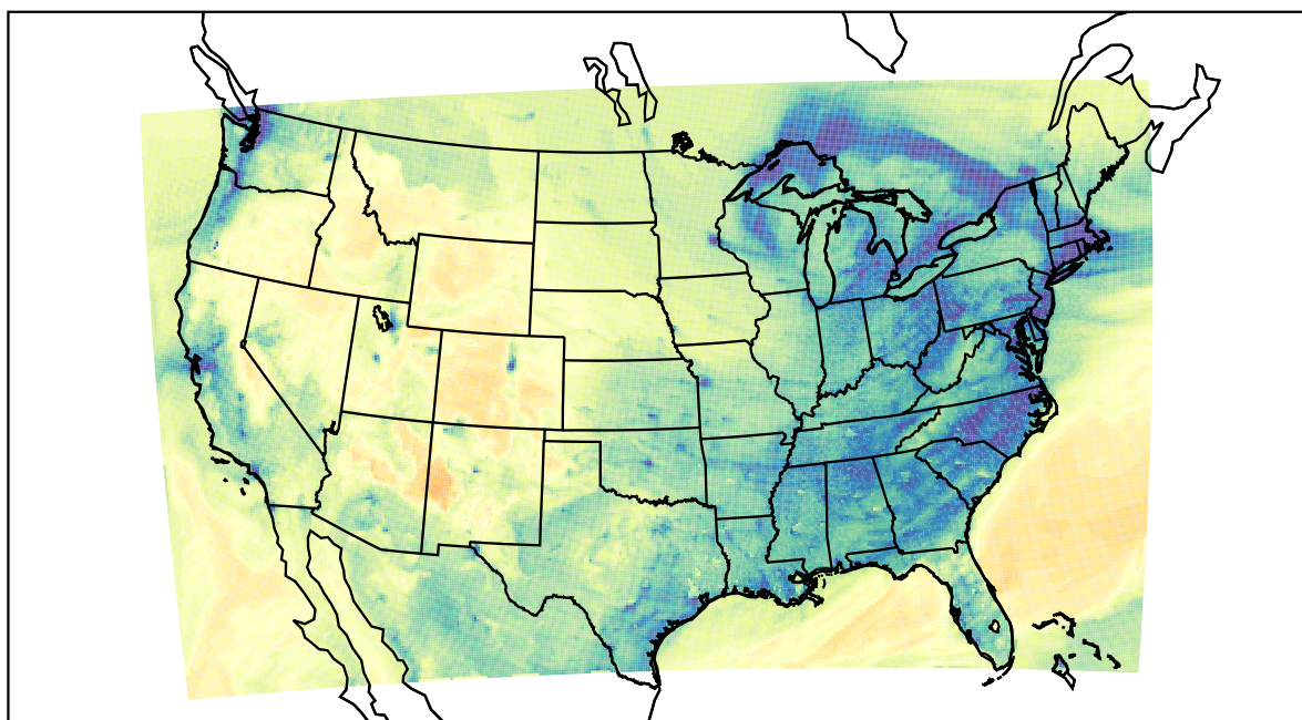
WRF (2022-12-18_00:00:00)
