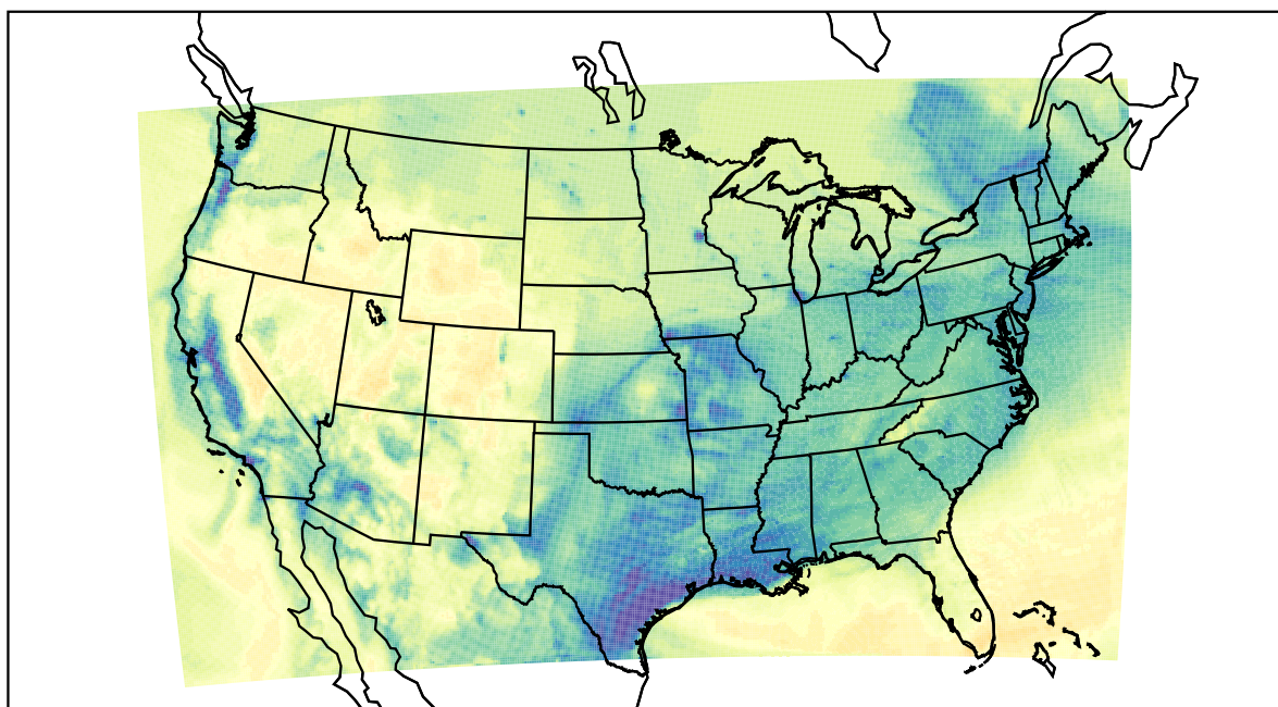
WRF (2022-12-19_18:00:00)
