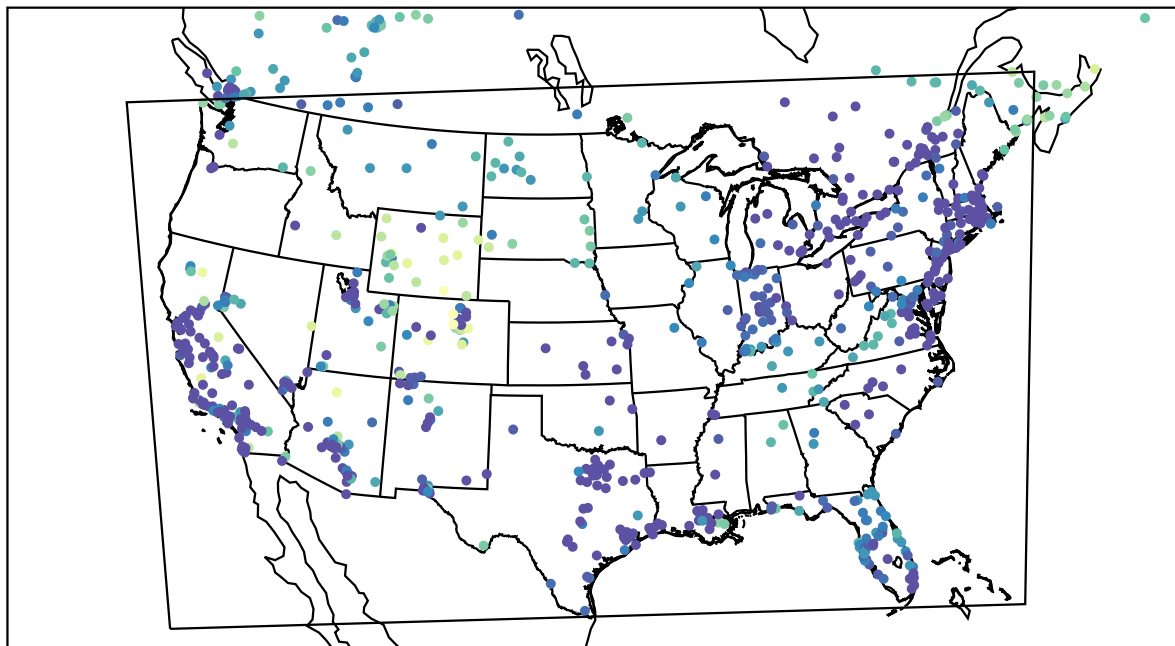
AirNOW (2022-12-18_12:00:00)
