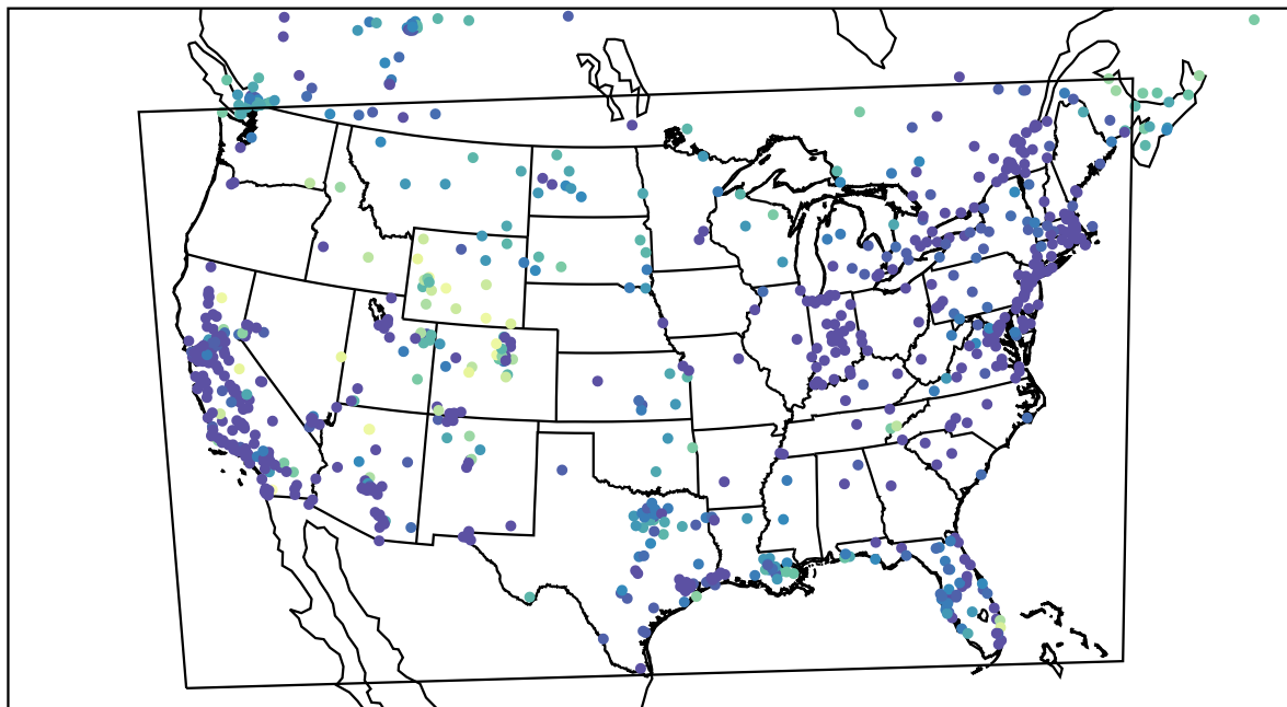
AirNOW (2022-12-19_13:00:00)
