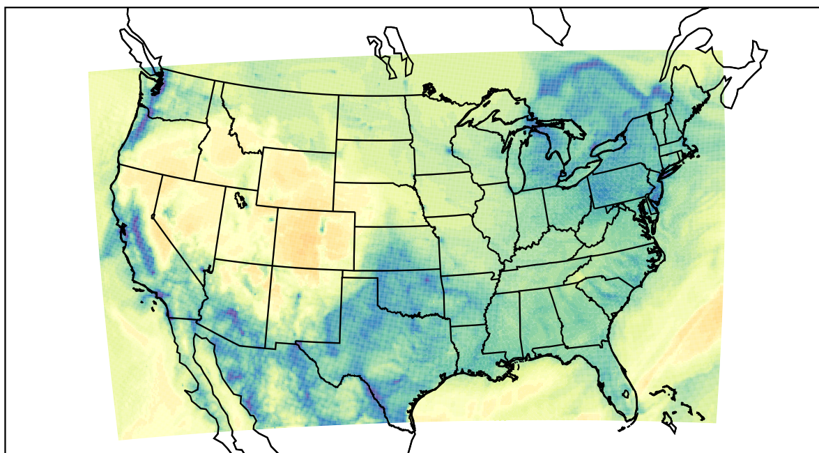
WRF (2022-12-18_16:00:00)
