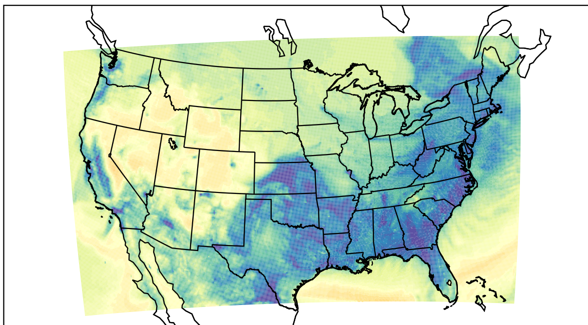
WRF (2022-12-19_07:00:00)
