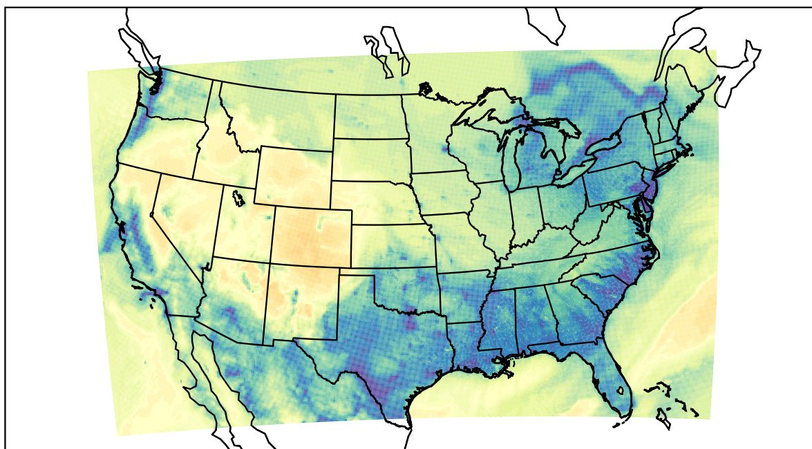
WRF (2022-12-18_14:00:00)
