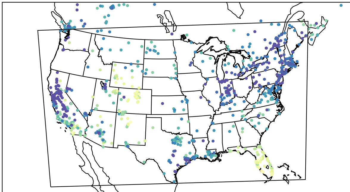
AirNOW (2022-12-19_19:00:00)
