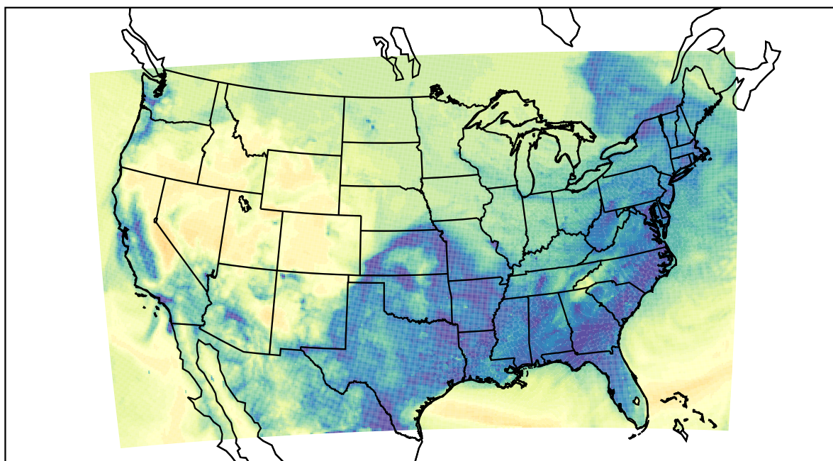
WRF (2022-12-19_11:00:00)
