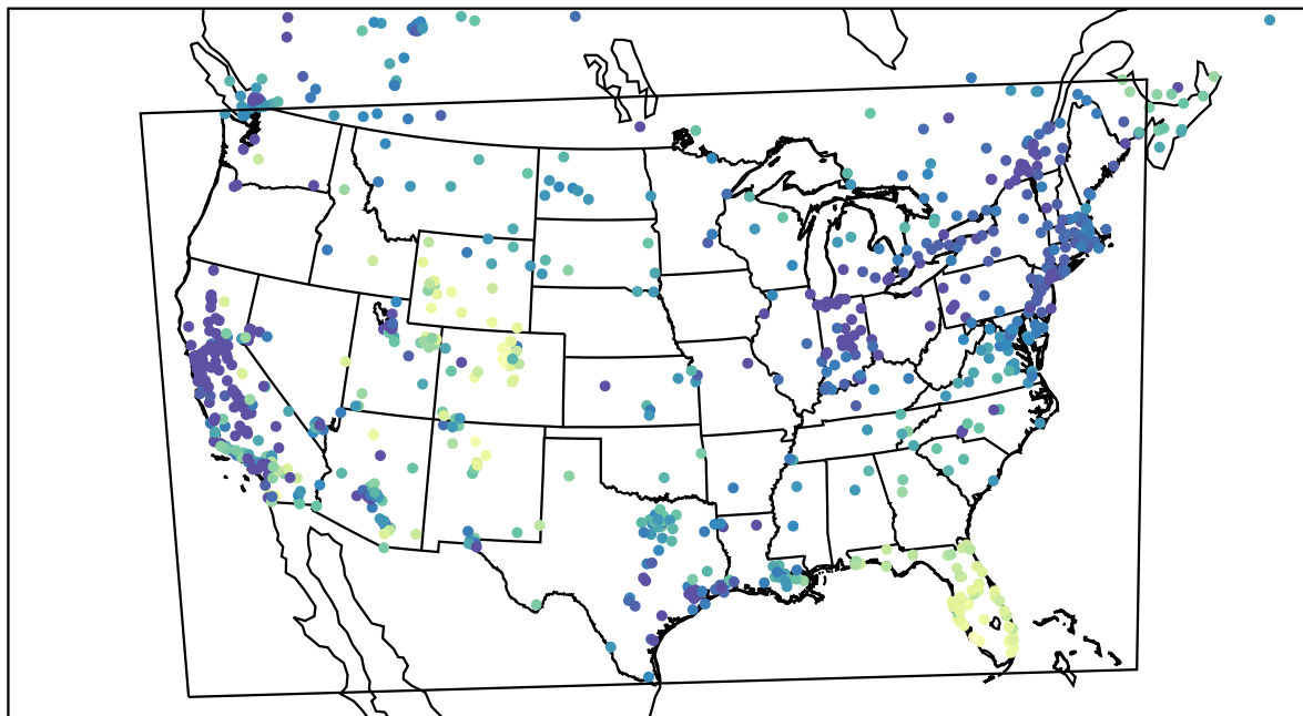
AirNOW (2022-12-19_18:00:00)
