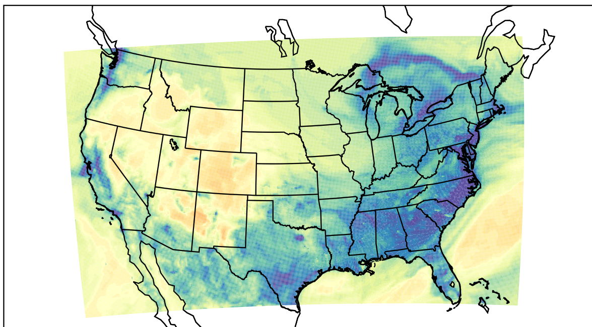
WRF (2022-12-18_07:00:00)
