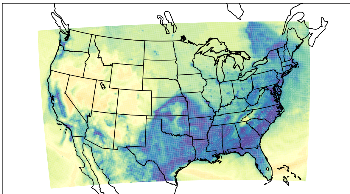
WRF (2022-12-19_13:00:00)
