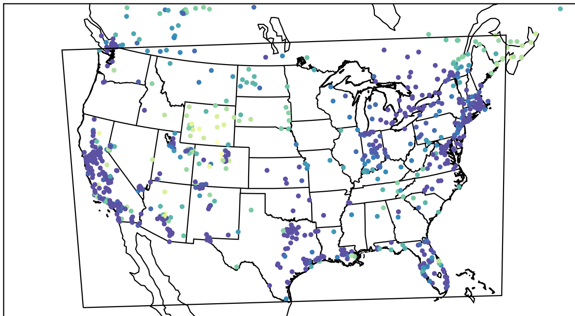
AirNOW (2022-12-18_06:00:00)
