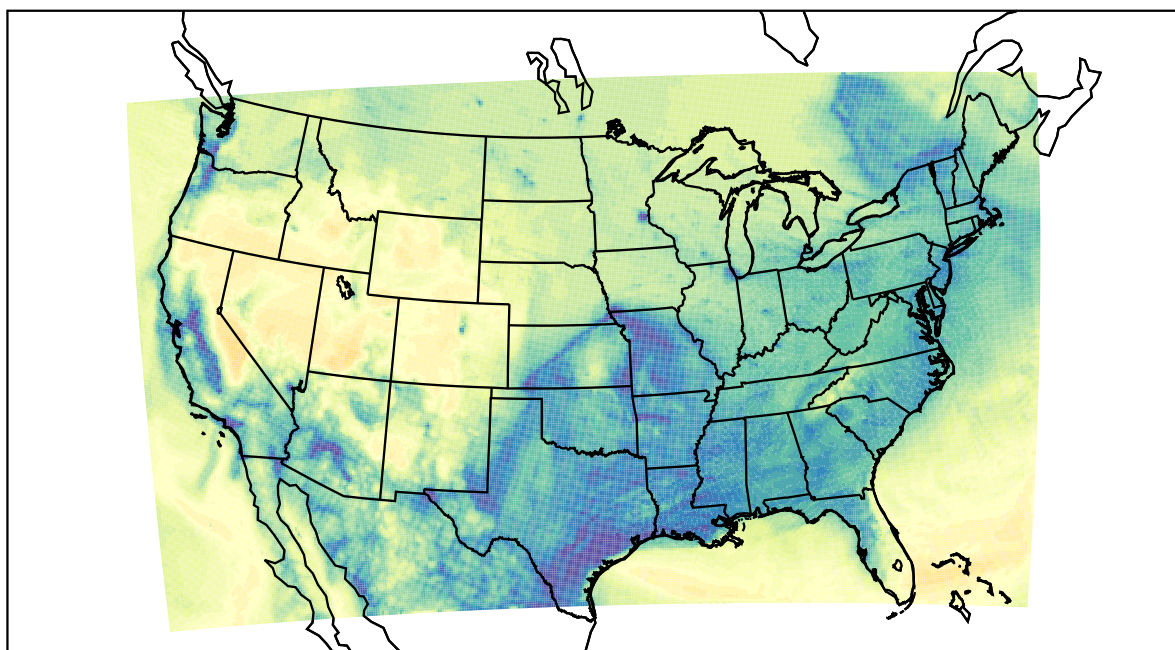
WRF (2022-12-19_16:00:00)
