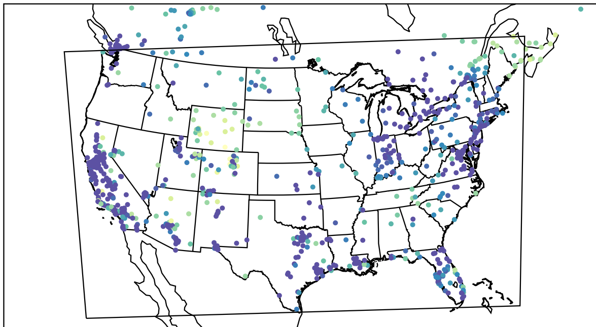
AirNOW (2022-12-18_03:00:00)
