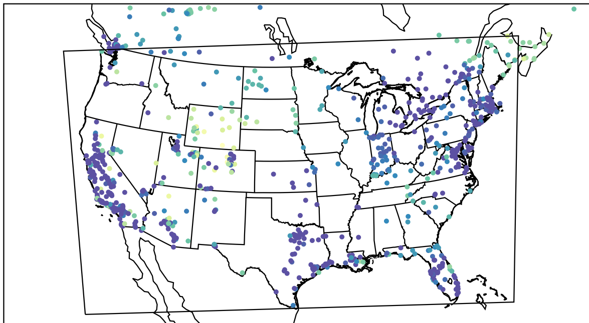
AirNOW (2022-12-18_08:00:00)
