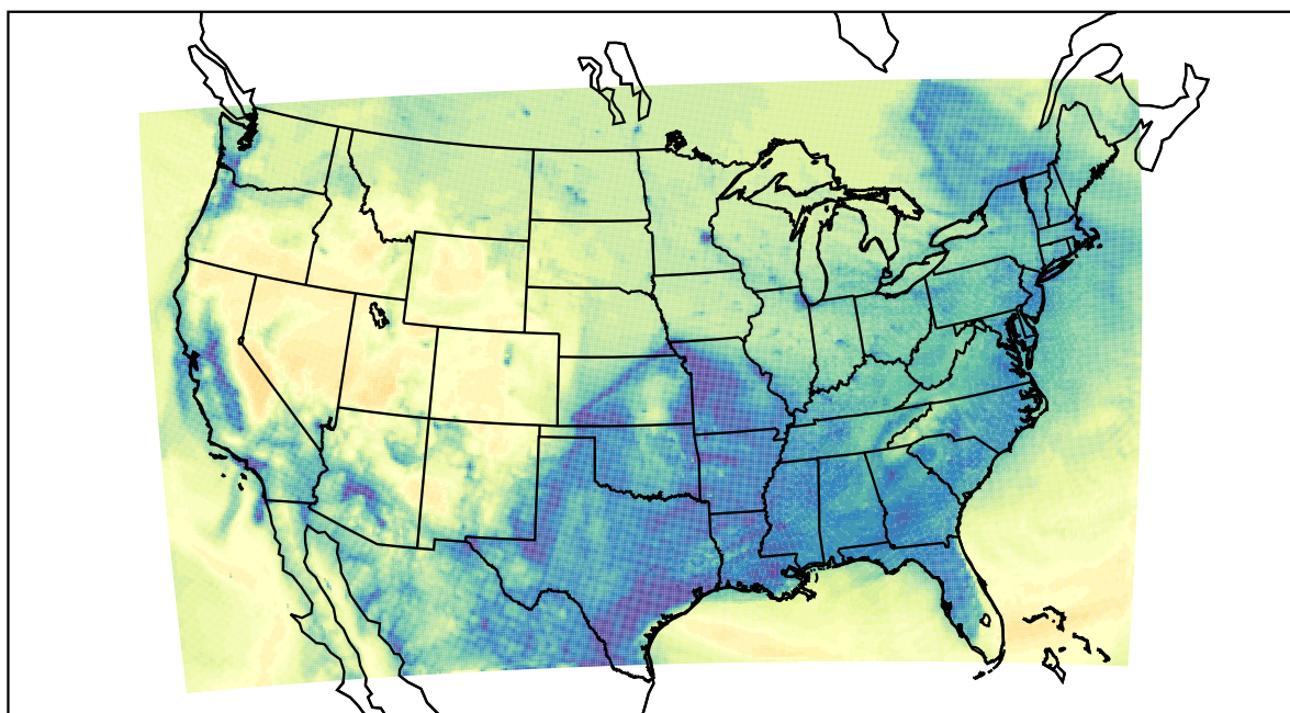
WRF (2022-12-19_15:00:00)
