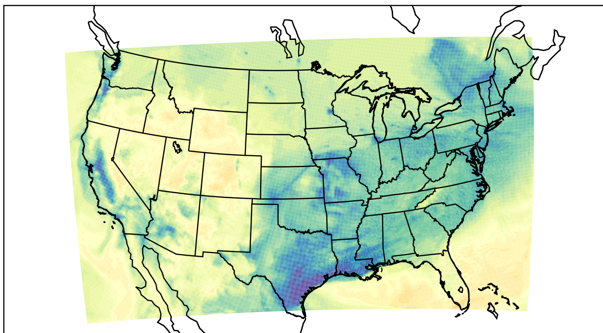
WRF (2022-12-19_19:00:00)
