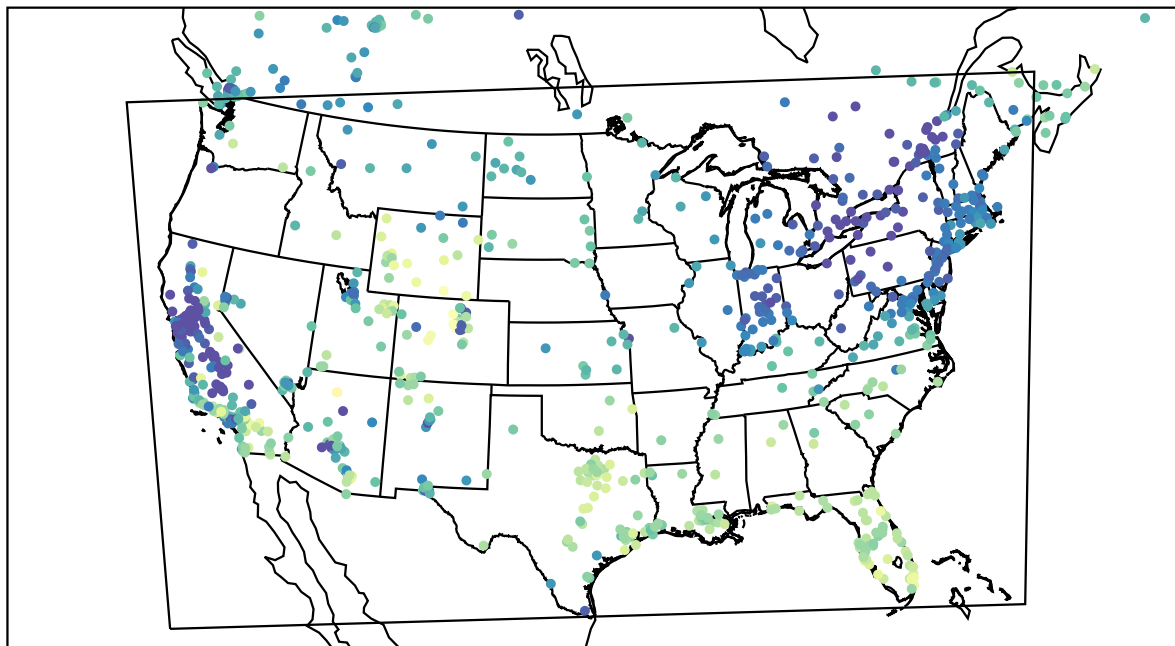
AirNOW (2022-12-18_19:00:00)
