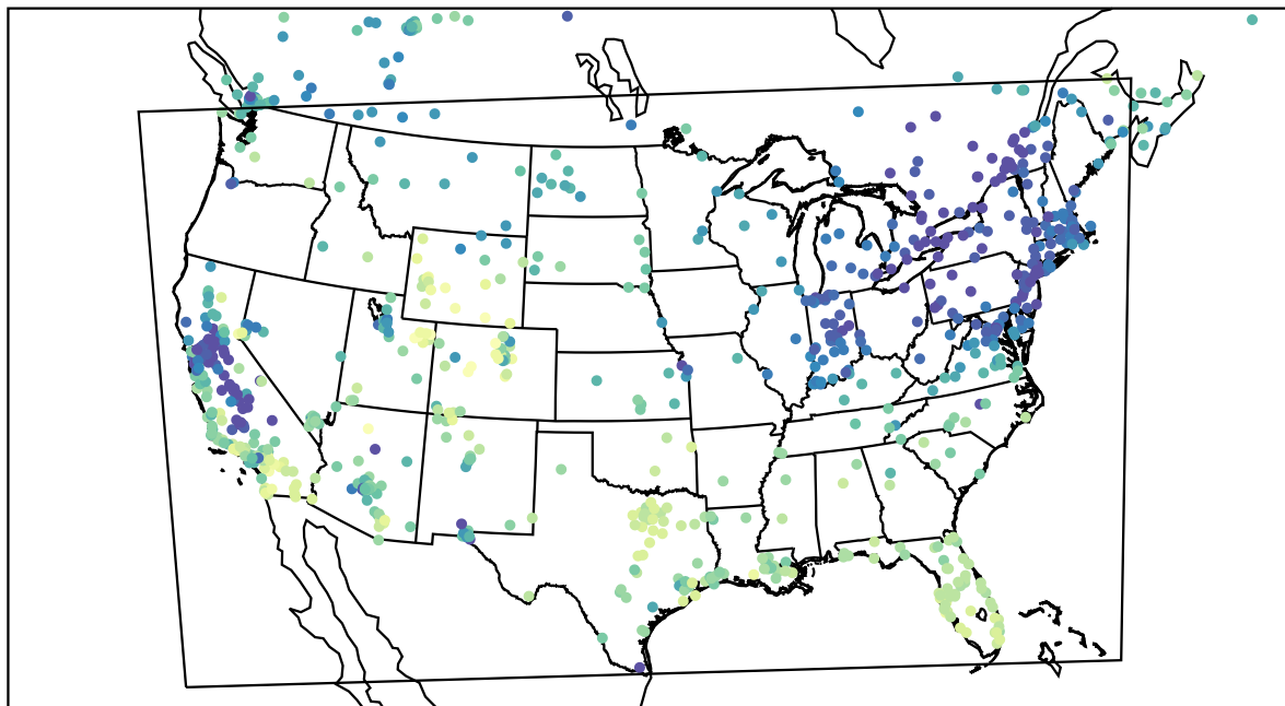
AirNOW (2022-12-18_21:00:00)
