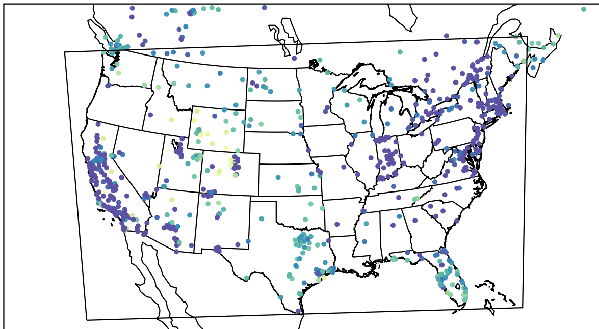
AirNOW (2022-12-19_07:00:00)
