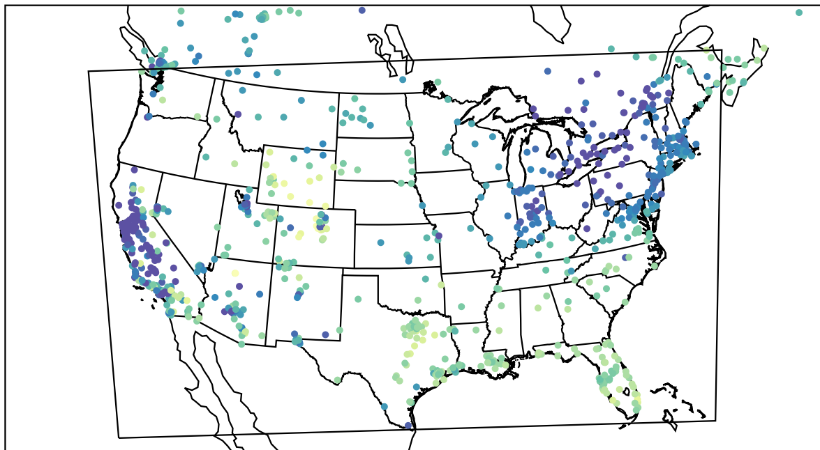
AirNOW (2022-12-18_18:00:00)
