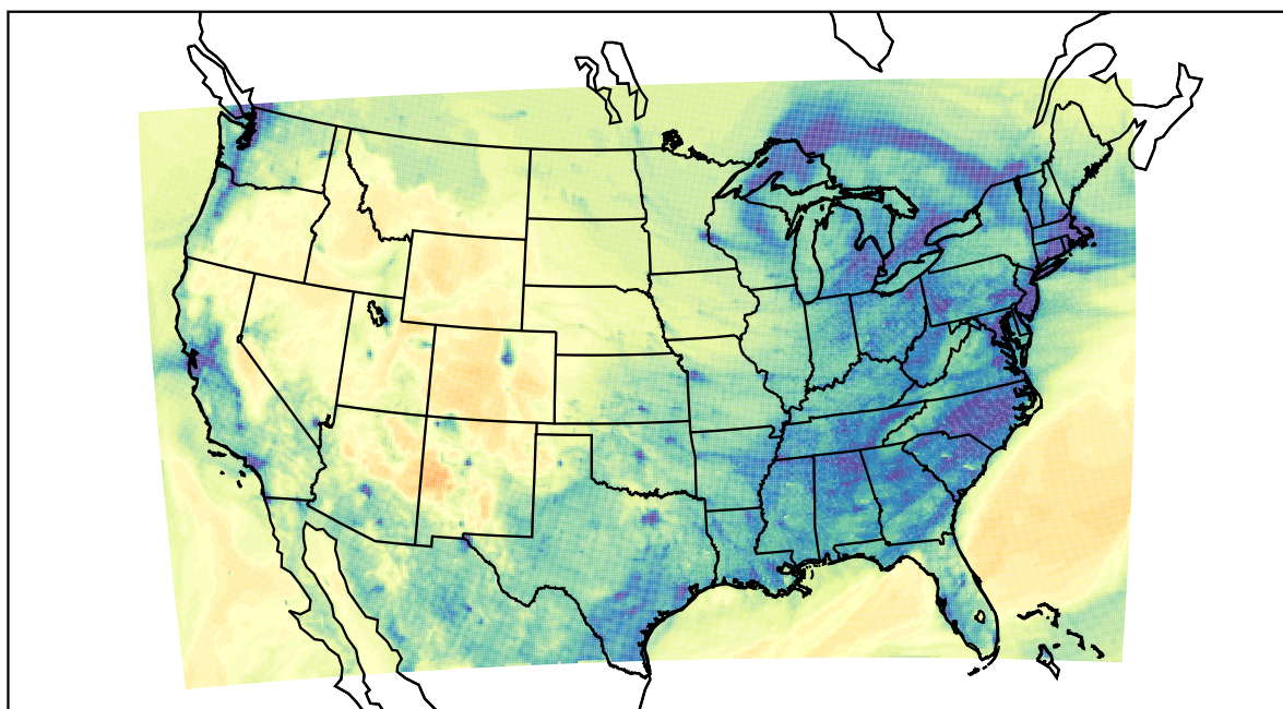
WRF (2022-12-18_02:00:00)
