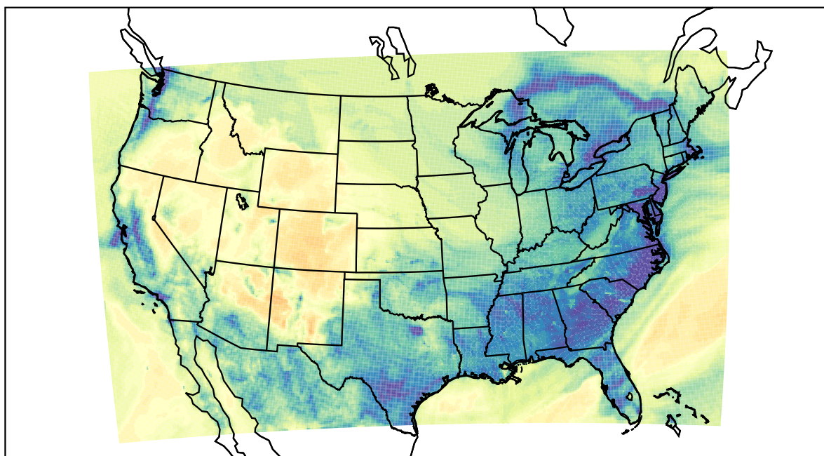
WRF (2022-12-18_08:00:00)
