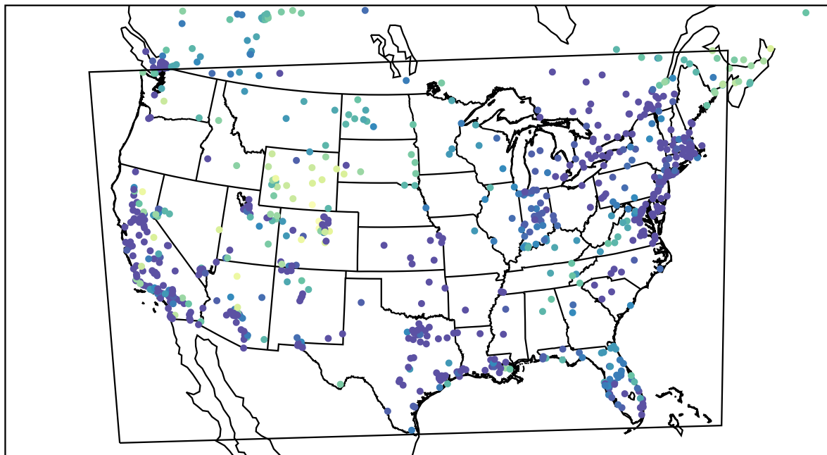
AirNOW (2022-12-18_11:00:00)
