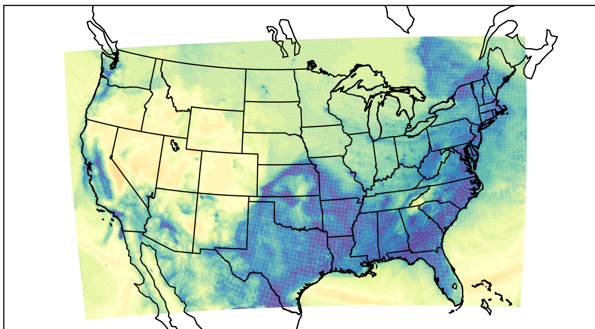
WRF (2022-12-19_12:00:00)
