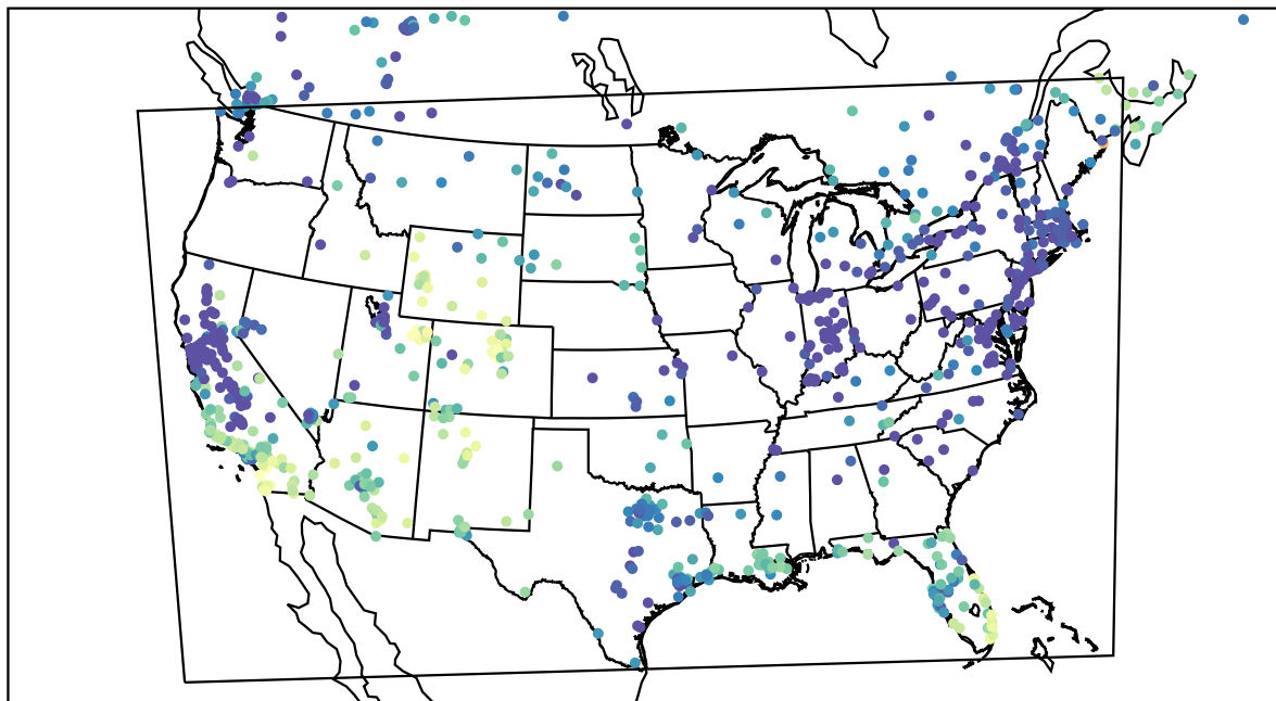
AirNOW (2022-12-19_23:00:00)
