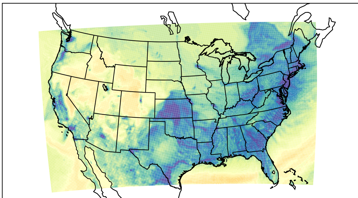
WRF (2022-12-19_03:00:00)
