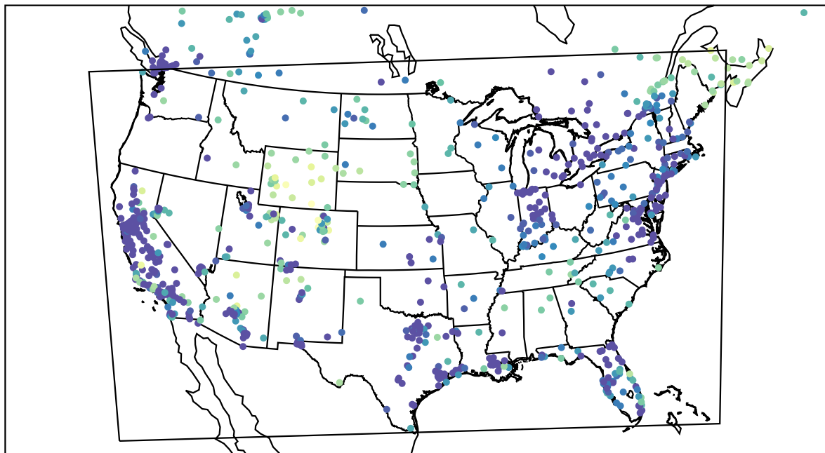
AirNOW (2022-12-18_02:00:00)
