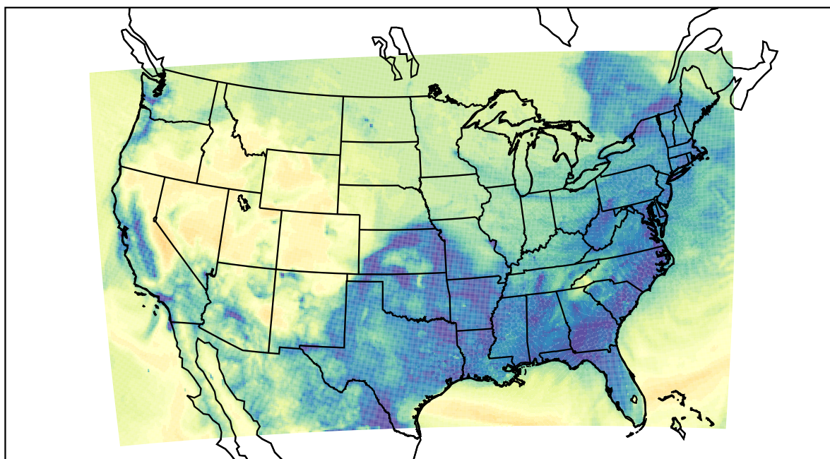
WRF (2022-12-19_10:00:00)
