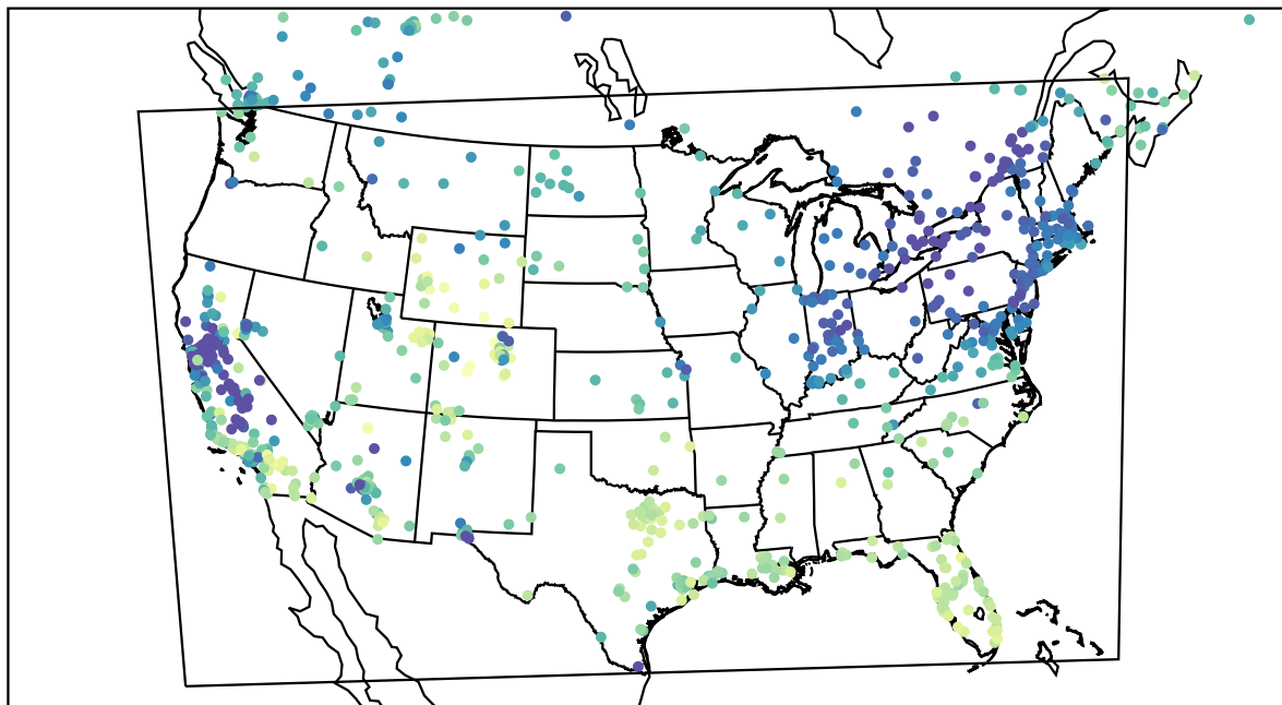
AirNOW (2022-12-18_20:00:00)
