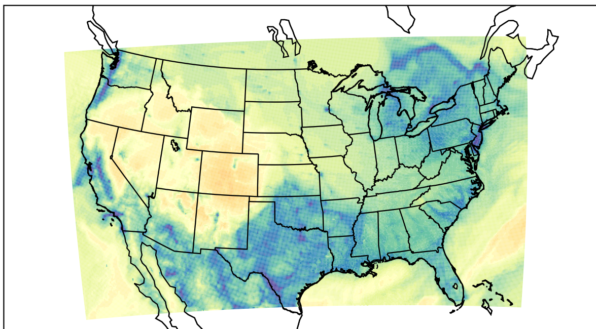
WRF (2022-12-18_15:00:00)
