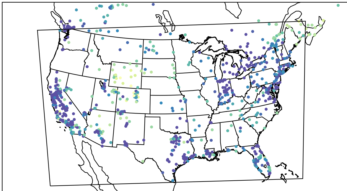
AirNOW (2022-12-18_01:00:00)
