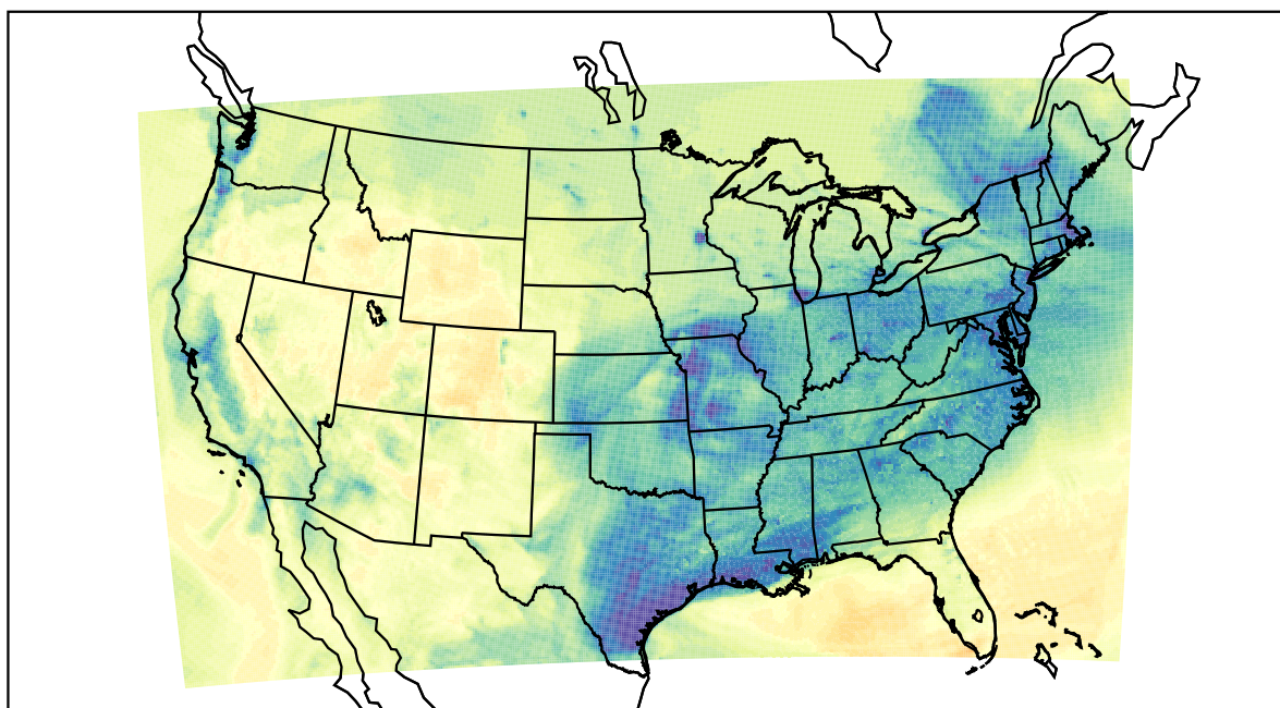
WRF (2022-12-19_21:00:00)
