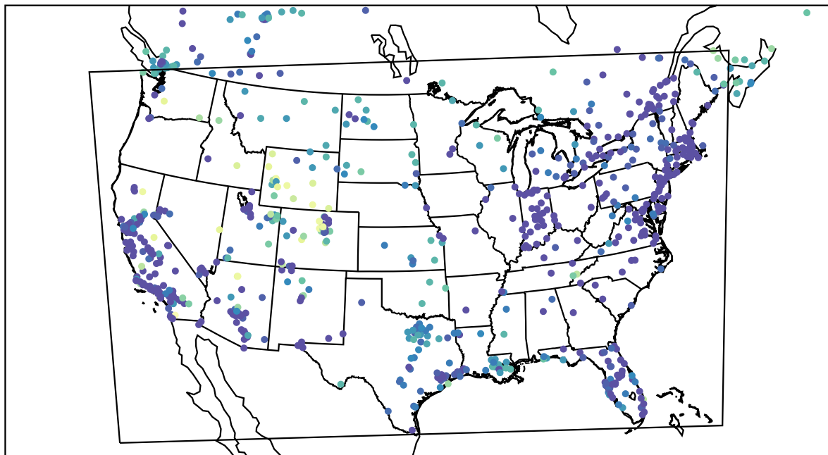
AirNOW (2022-12-19_12:00:00)
