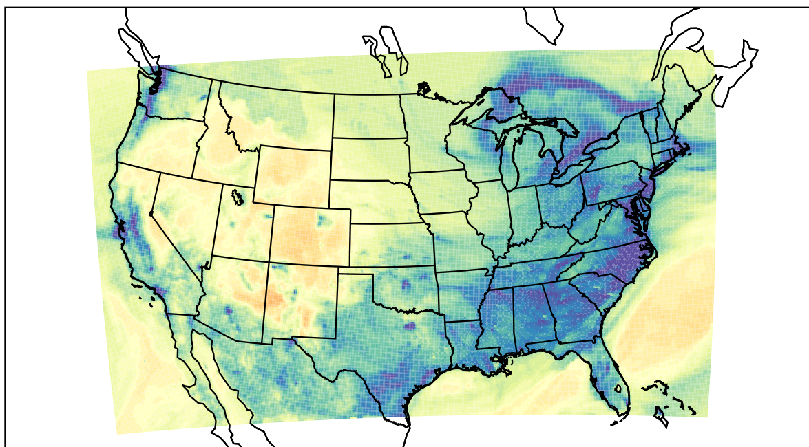
WRF (2022-12-18_05:00:00)
