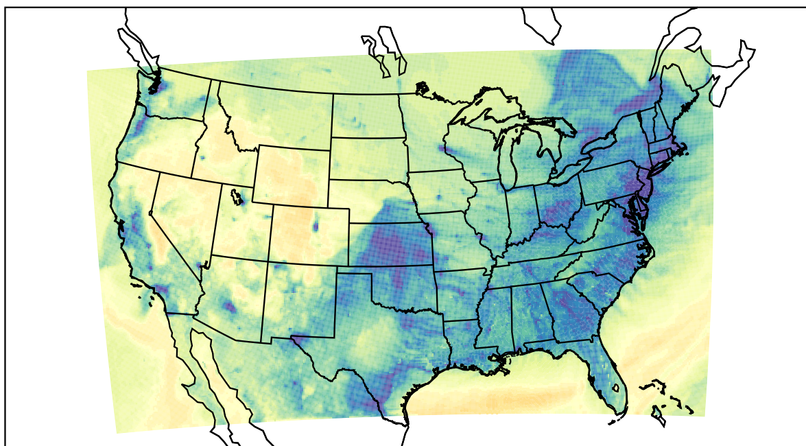
WRF (2022-12-19_01:00:00)
