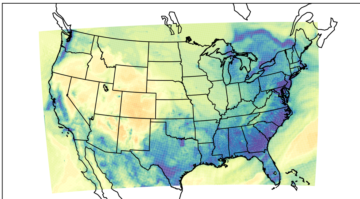
WRF (2022-12-18_12:00:00)
