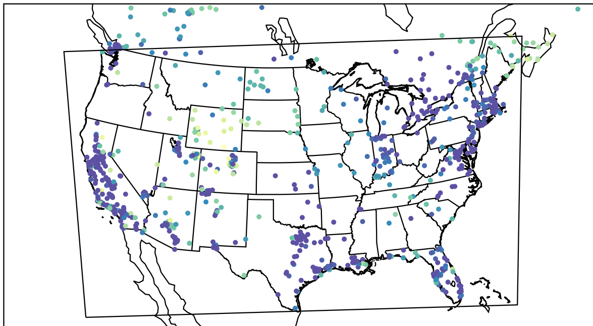
AirNOW (2022-12-18_07:00:00)
