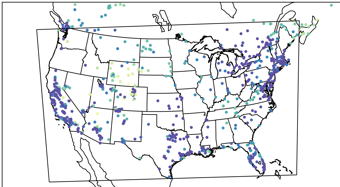
AirNOW (2022-12-18_10:00:00)
