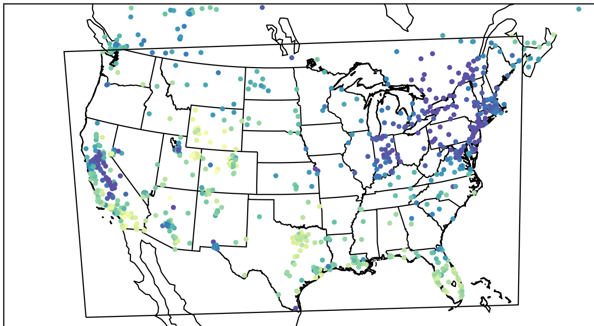
AirNOW (2022-12-18_22:00:00)
