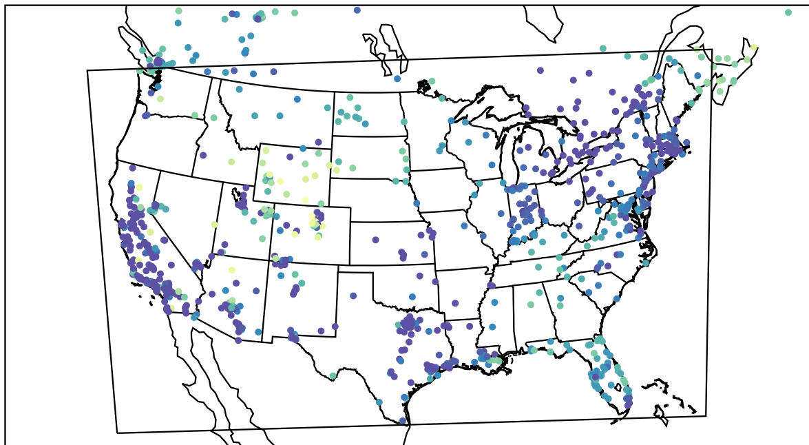
AirNOW (2022-12-18_14:00:00)
