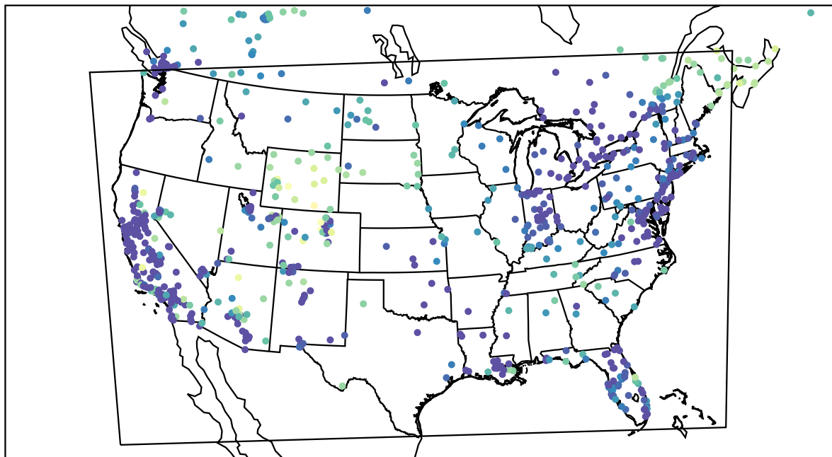
AirNOW (2022-12-18_04:00:00)
