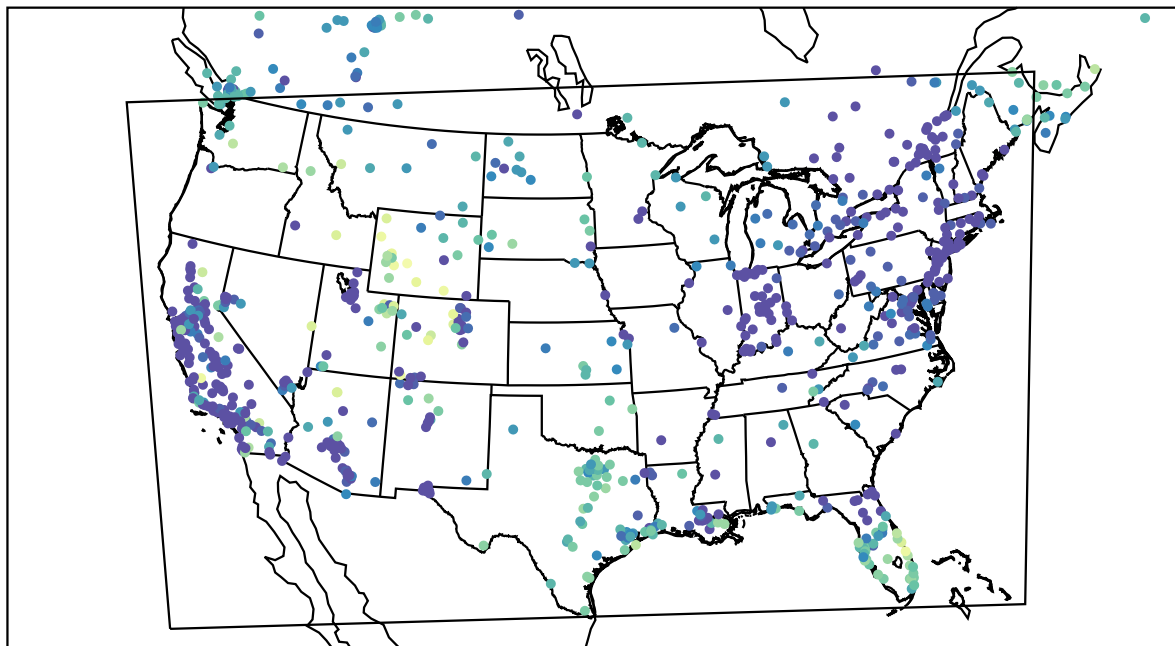
AirNOW (2022-12-19_03:00:00)
