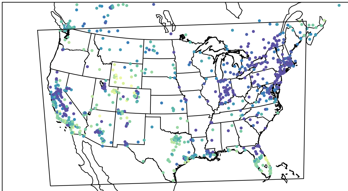
AirNOW (2022-12-19_00:00:00)
