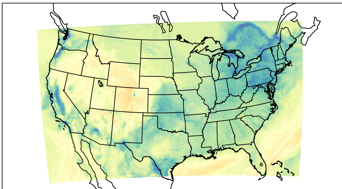
WRF (2022-12-18_19:00:00)
