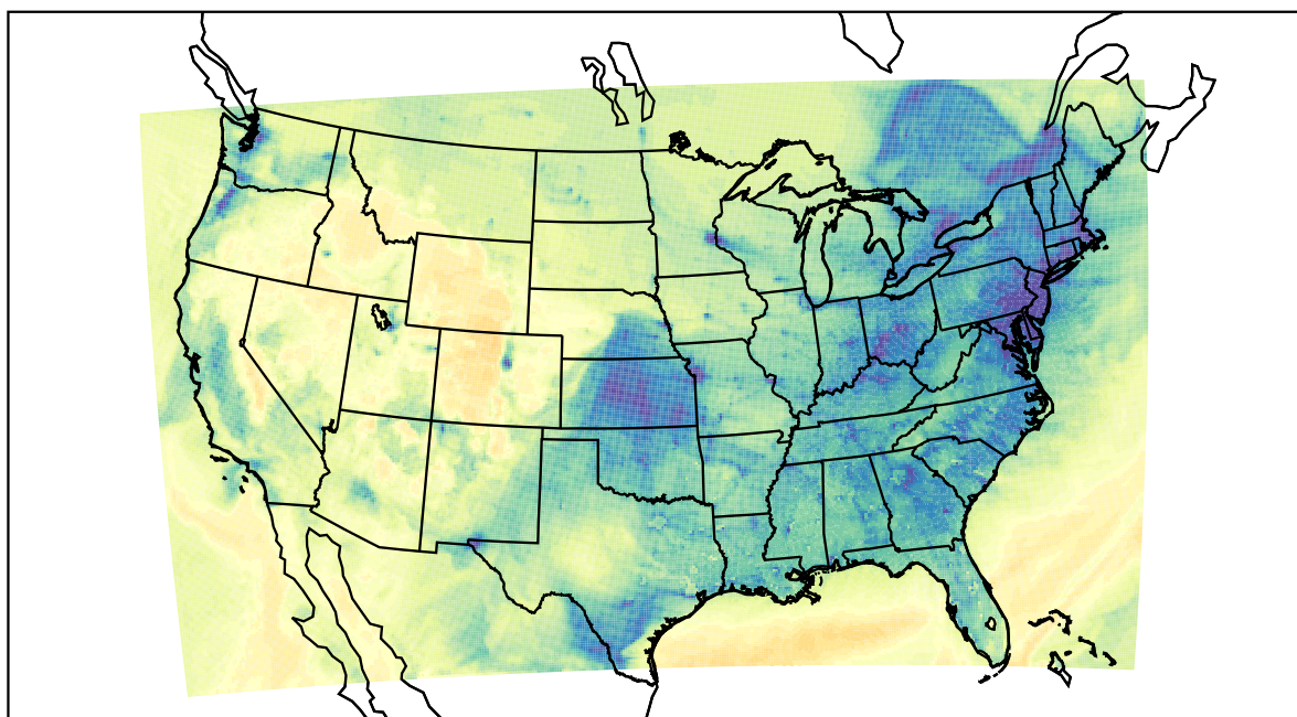
WRF (2022-12-18_23:00:00)
