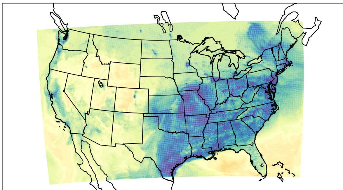
WRF (2022-12-19_23:00:00)
