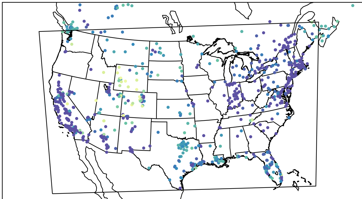
AirNOW (2022-12-19_10:00:00)
