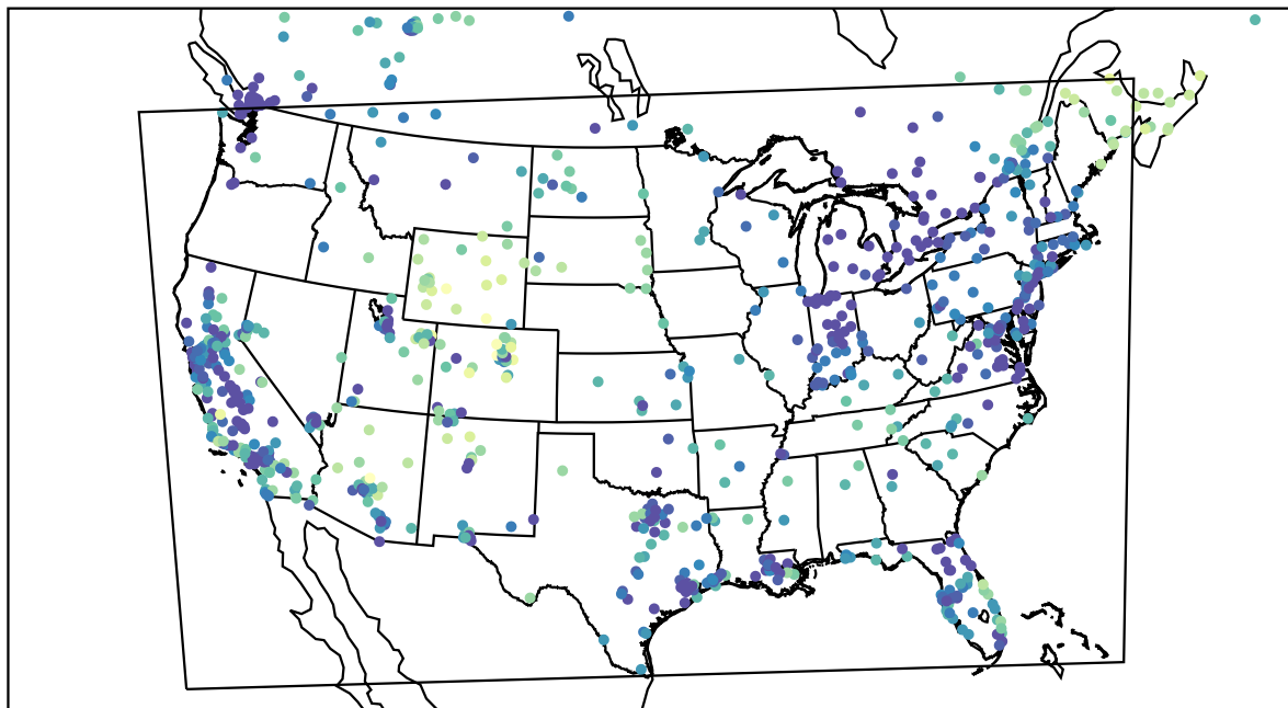
AirNOW (2022-12-18_00:00:00)
