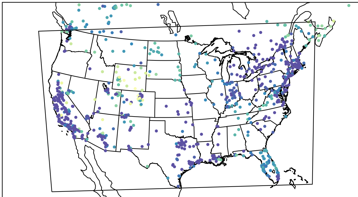
AirNOW (2022-12-18_13:00:00)
