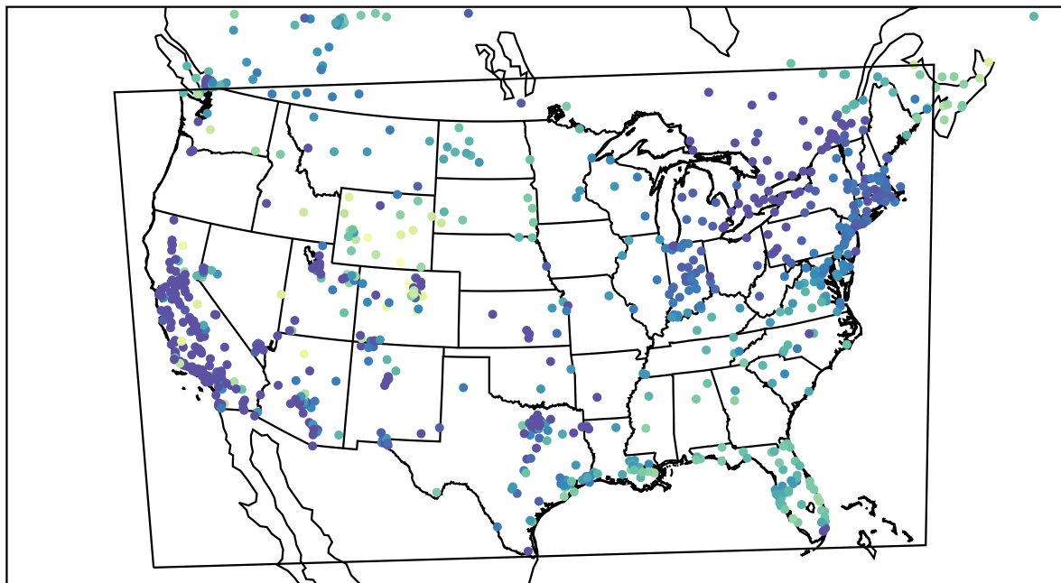
AirNOW (2022-12-18_15:00:00)
