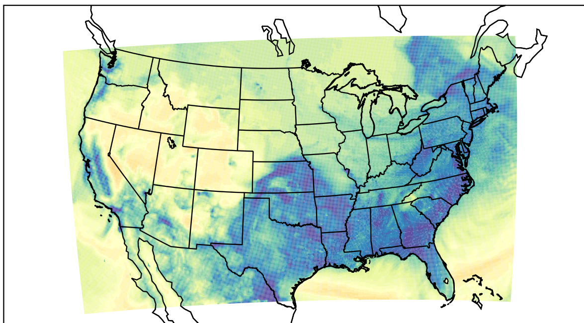
WRF (2022-12-19_09:00:00)
