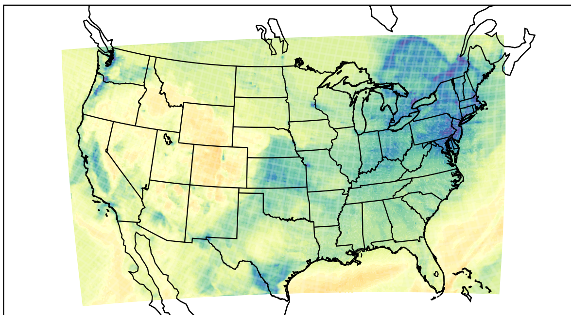
WRF (2022-12-18_21:00:00)
