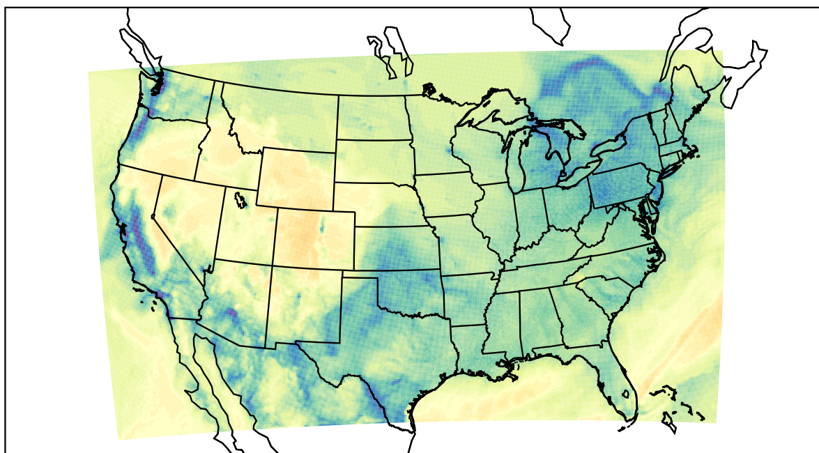
WRF (2022-12-18_17:00:00)
