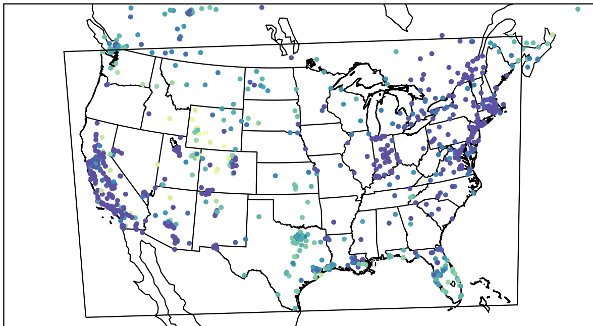
AirNOW (2022-12-19_05:00:00)
