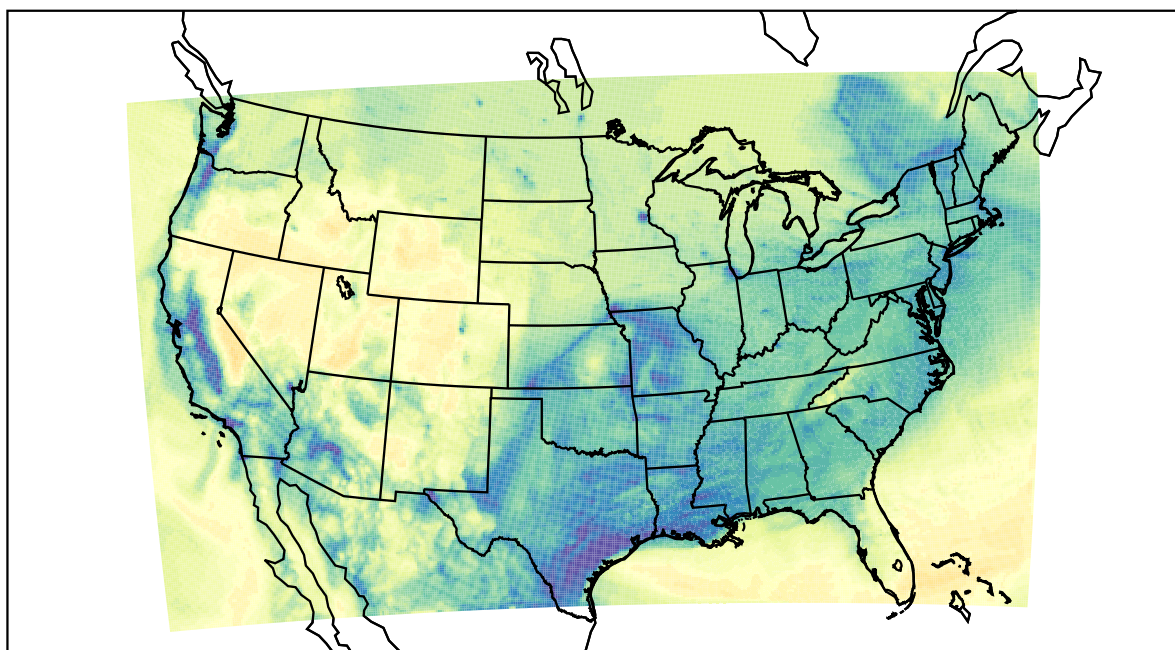
WRF (2022-12-19_17:00:00)
