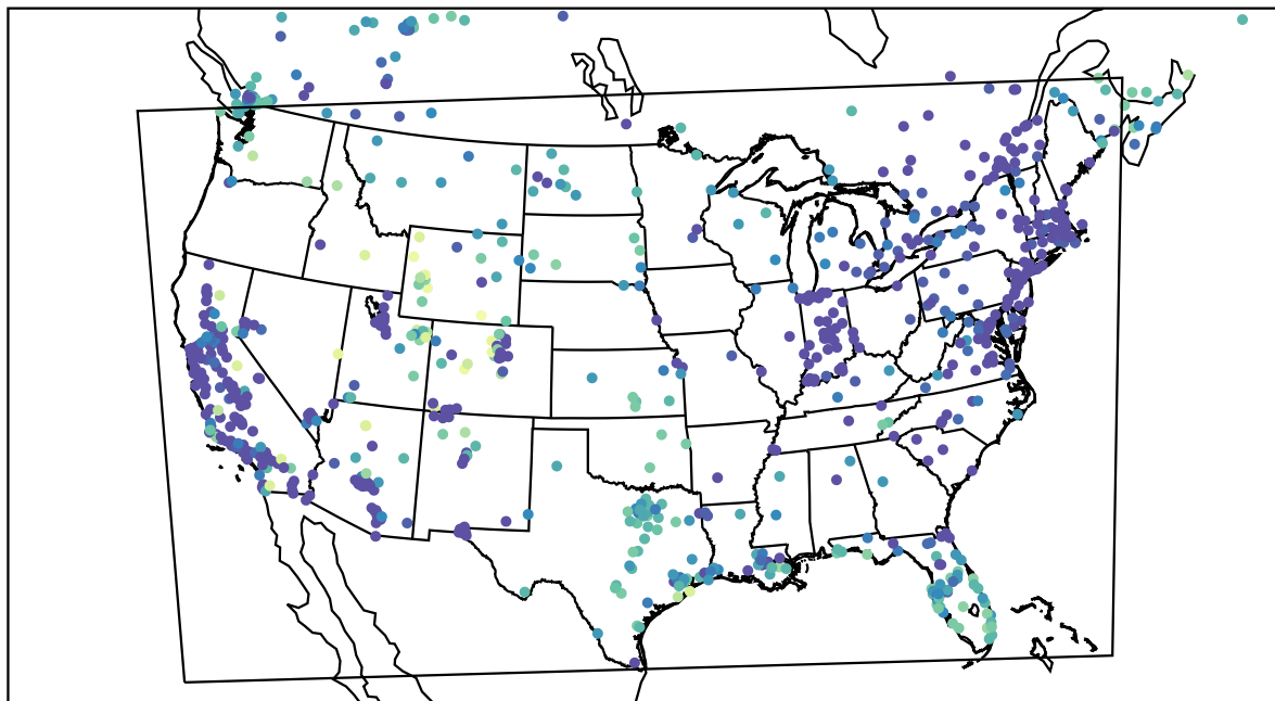
AirNOW (2022-12-19_06:00:00)
