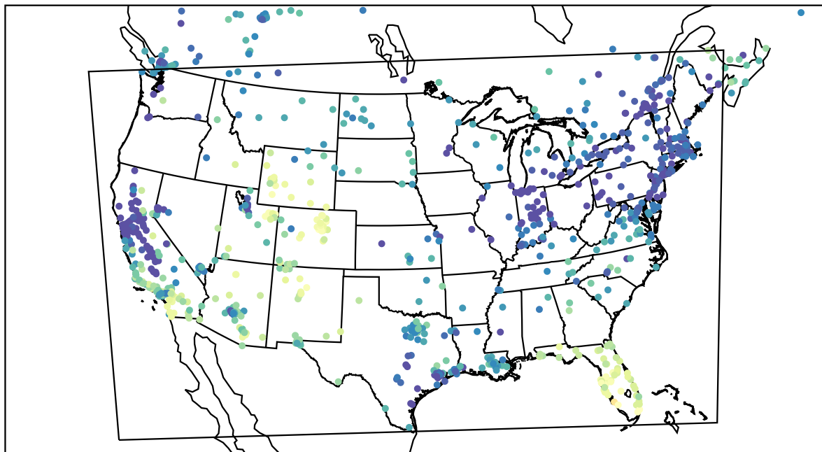
AirNOW (2022-12-19_20:00:00)
