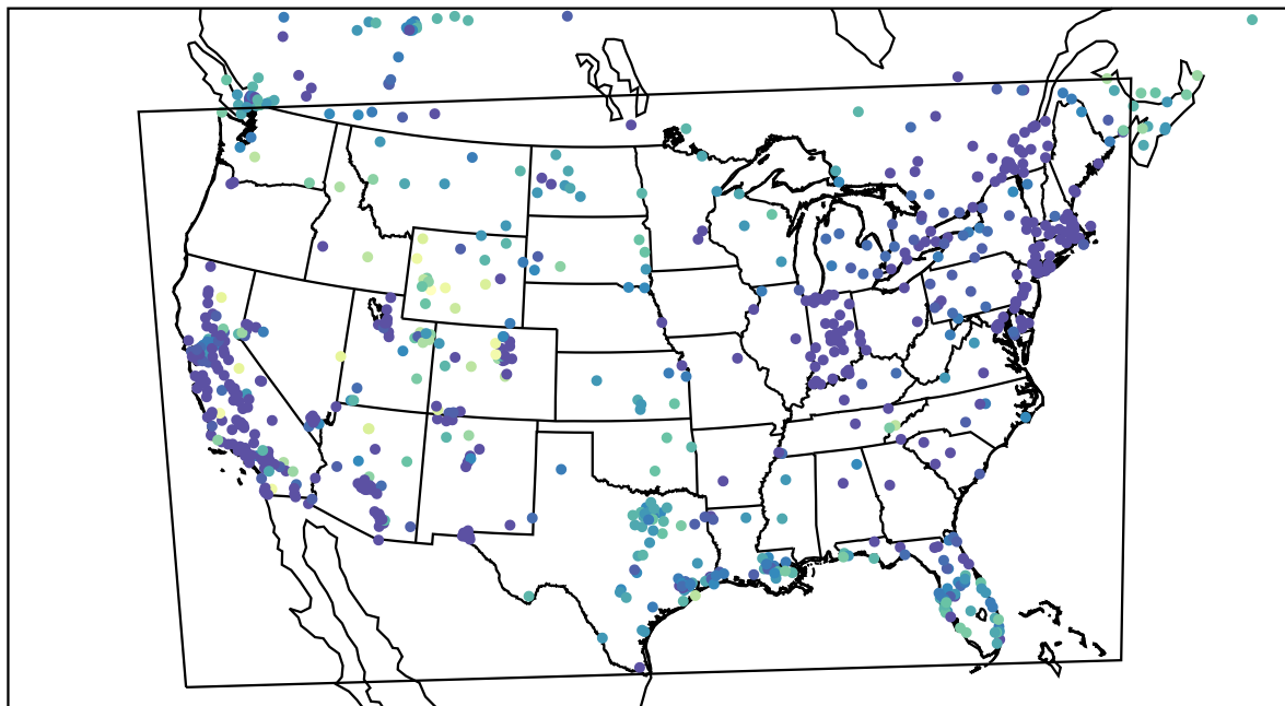
AirNOW (2022-12-19_09:00:00)
