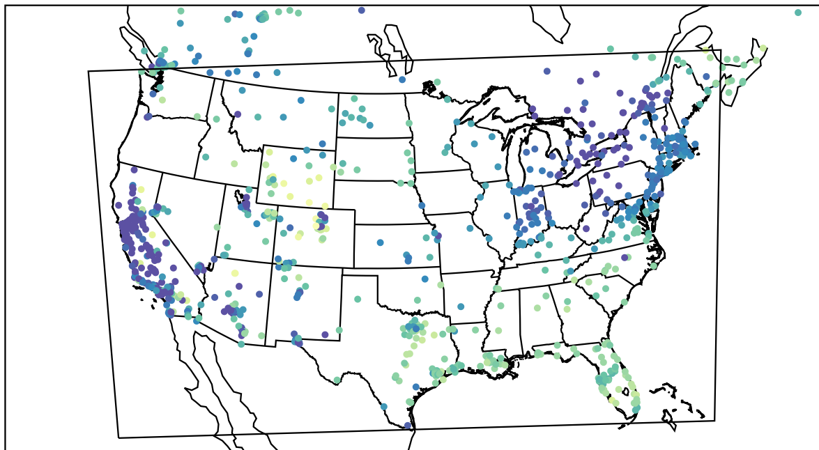
AirNOW (2022-12-18_17:00:00)
