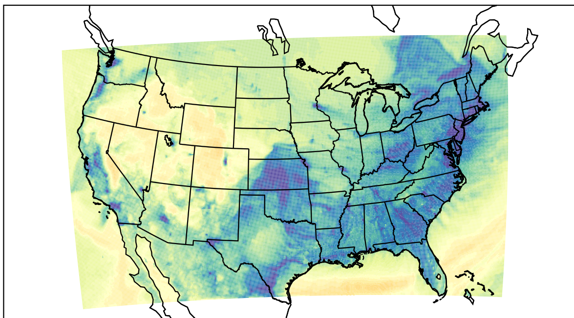
WRF (2022-12-19_02:00:00)
