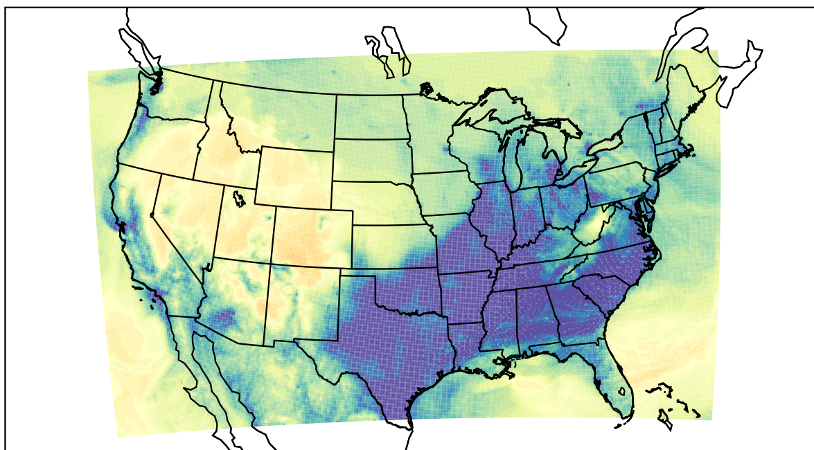
WRF (2022-12-20_13:00:00)
