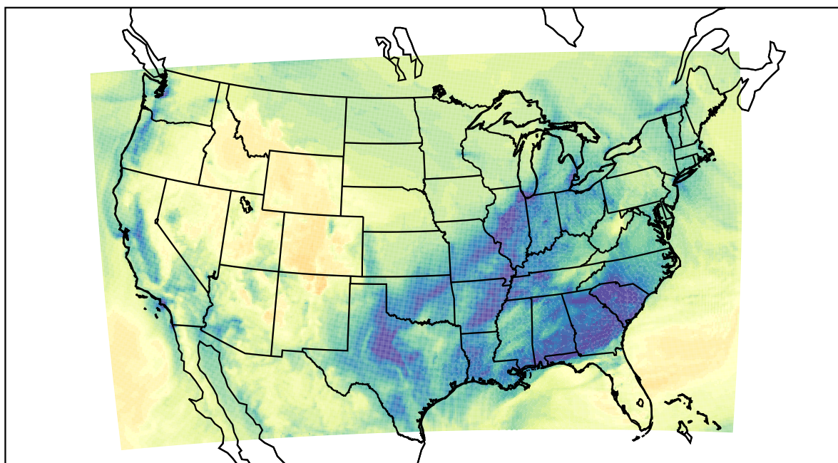
WRF (2022-12-20_19:00:00)
