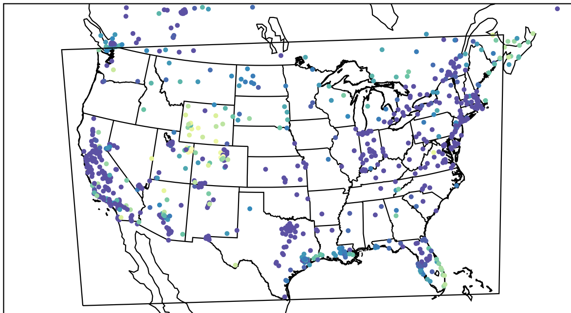
AirNOW (2022-12-21_05:00:00)
