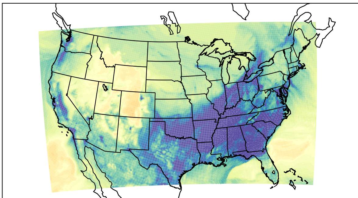
WRF (2022-12-21_04:00:00)
