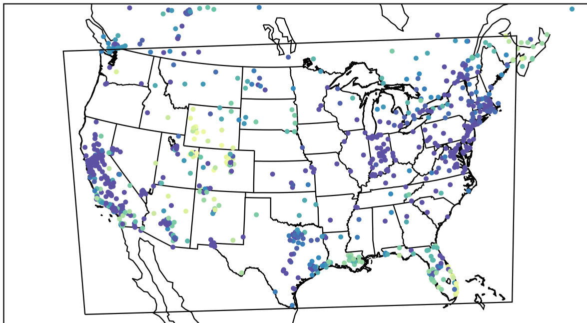
AirNOW (2022-12-20_01:00:00)
