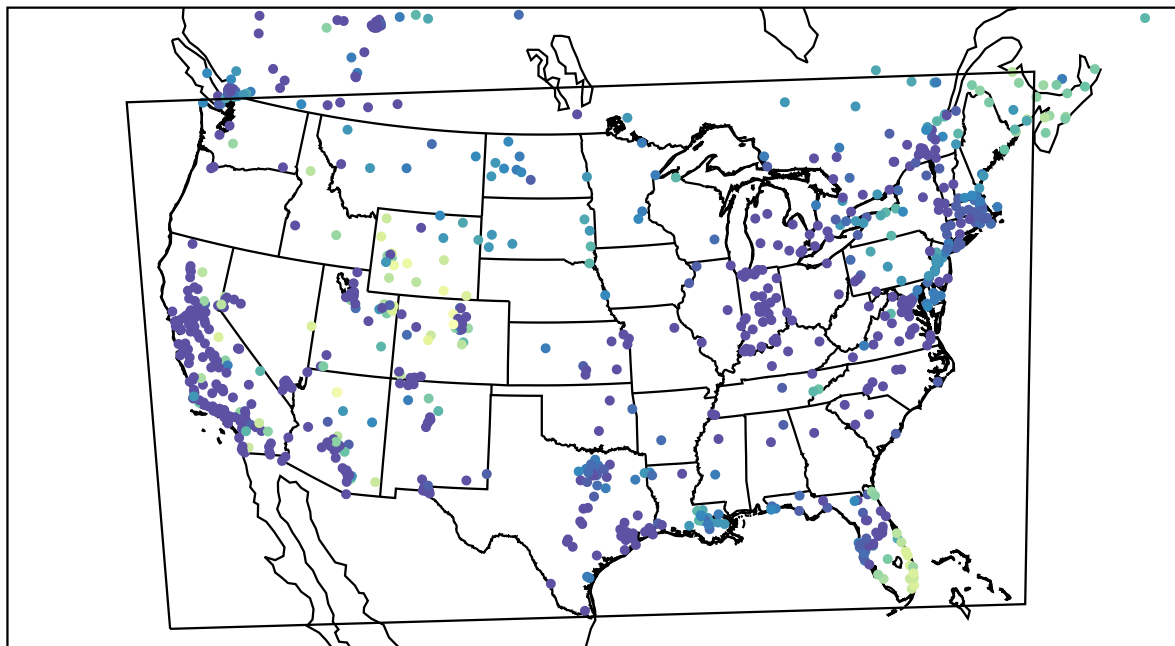
AirNOW (2022-12-20_15:00:00)
