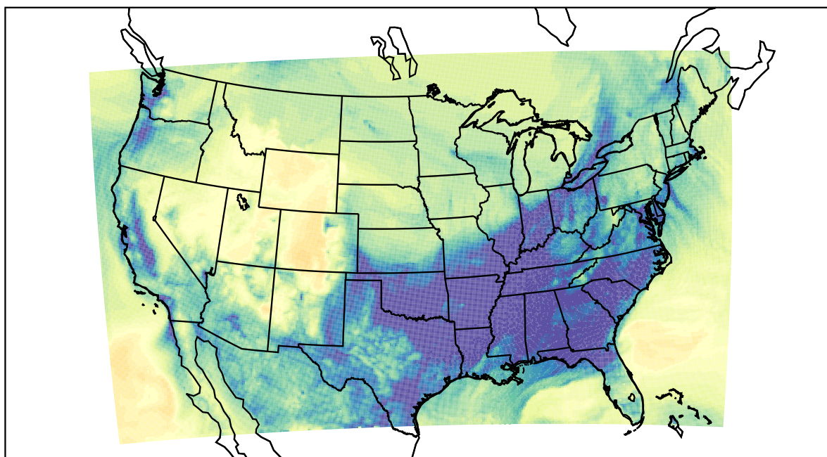
WRF (2022-12-21_07:00:00)
