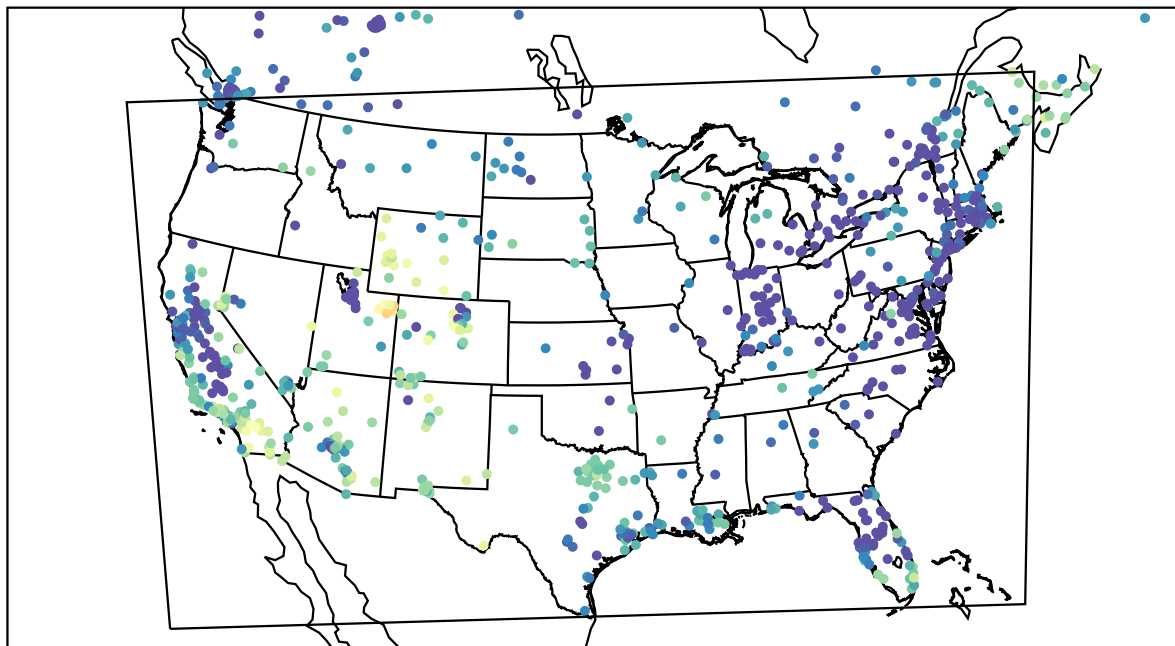
AirNOW (2022-12-20_22:00:00)
