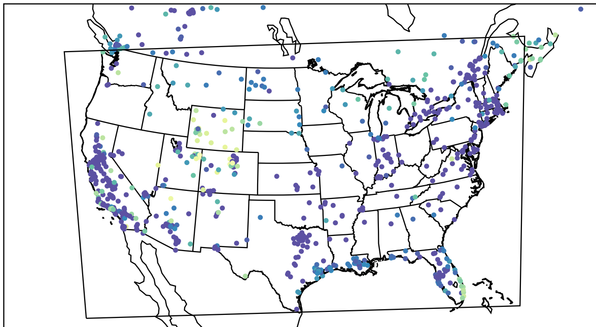
AirNOW (2022-12-21_07:00:00)
