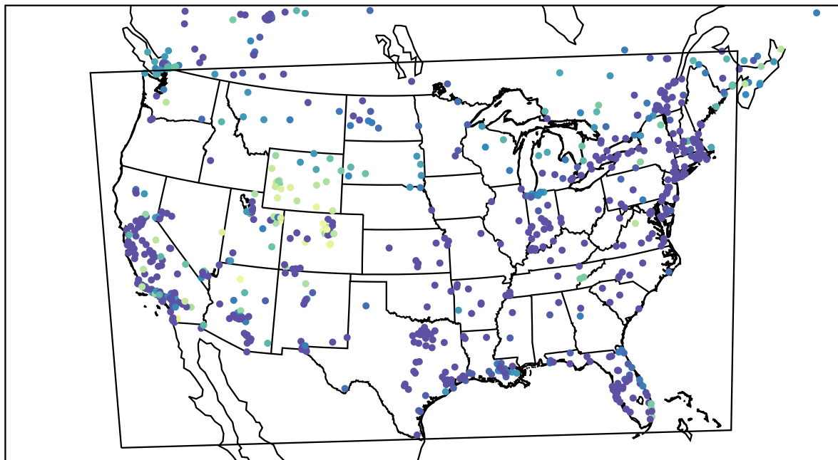
AirNOW (2022-12-21_12:00:00)
