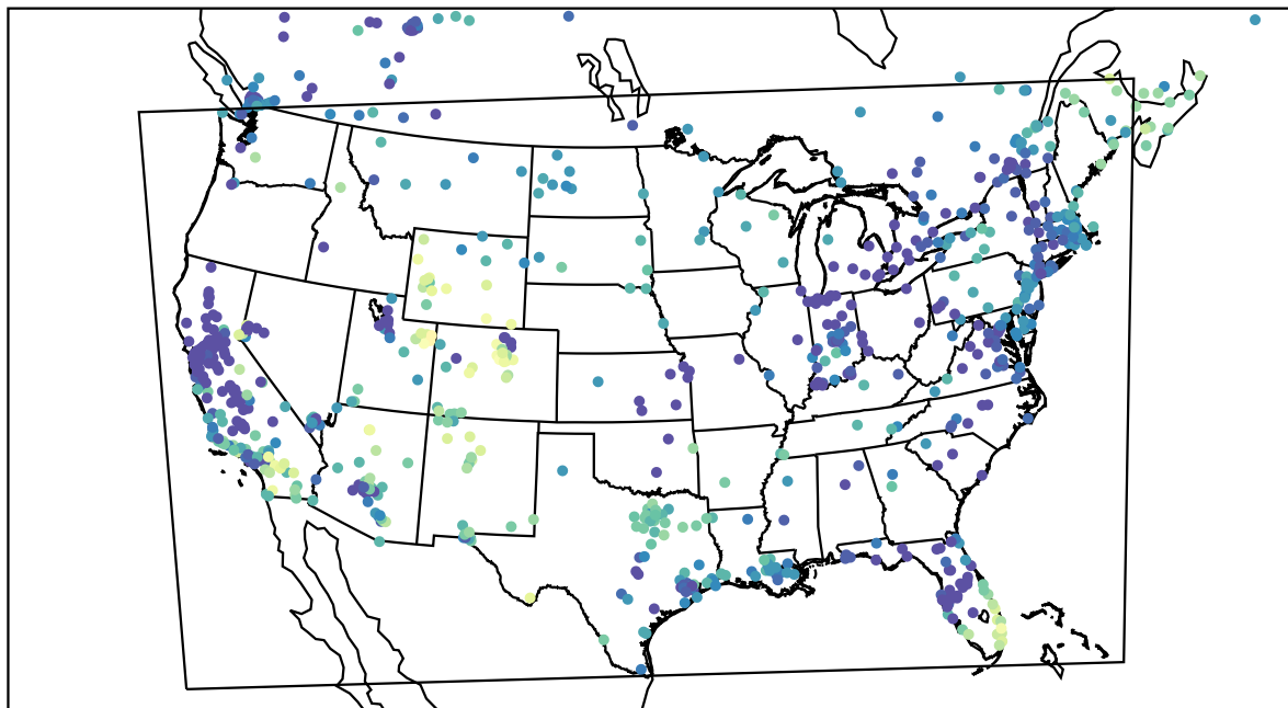
AirNOW (2022-12-20_19:00:00)
