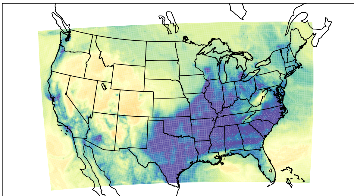
WRF (2022-12-20_11:00:00)
