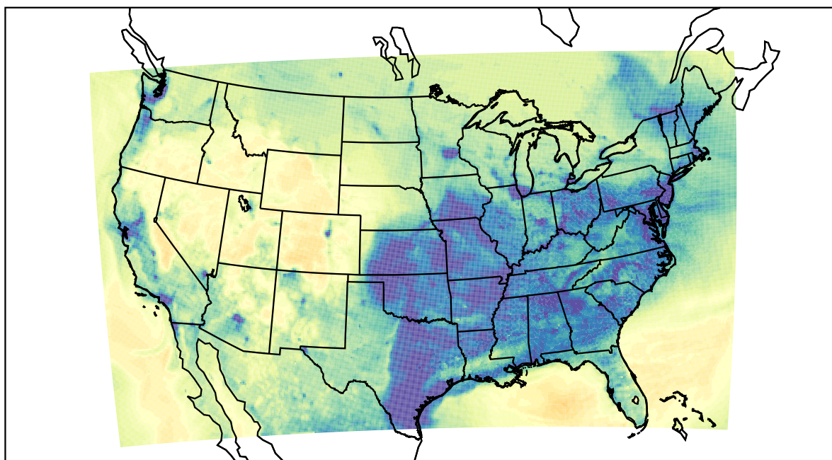
WRF (2022-12-20_01:00:00)
