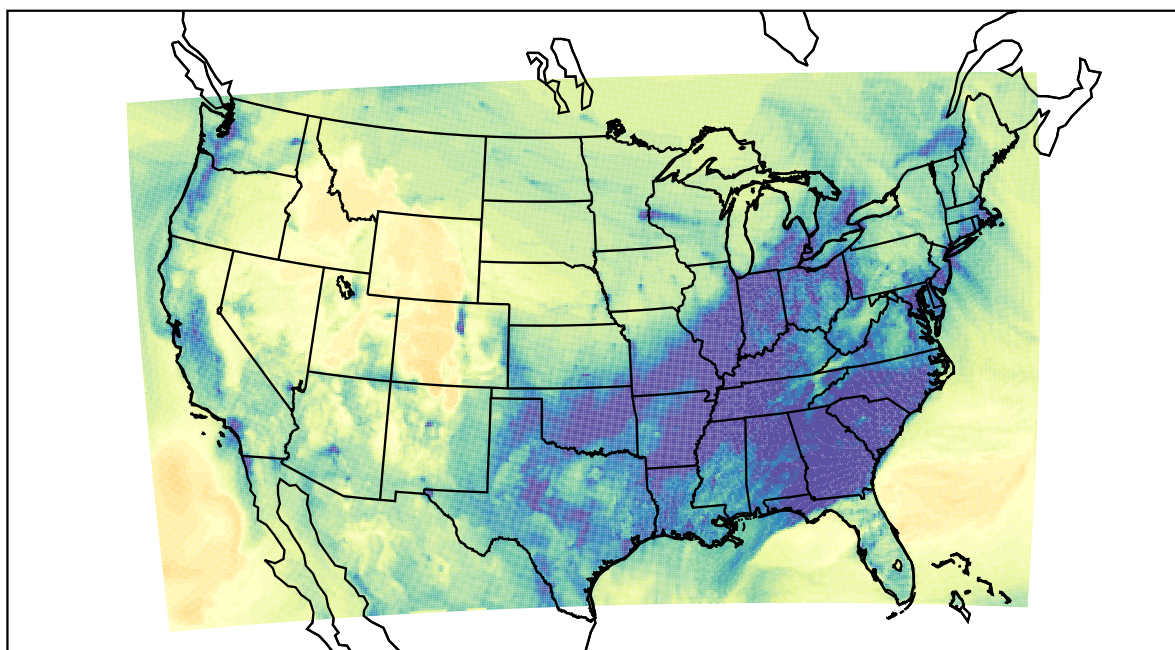
WRF (2022-12-21_00:00:00)
