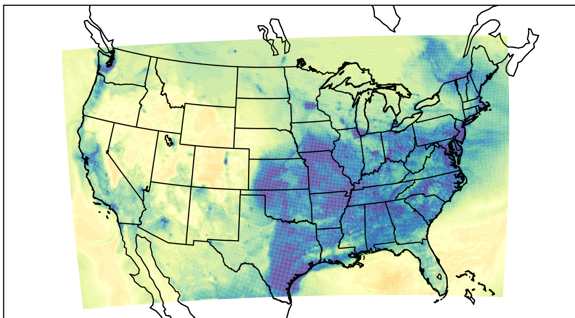
WRF (2022-12-20_00:00:00)
