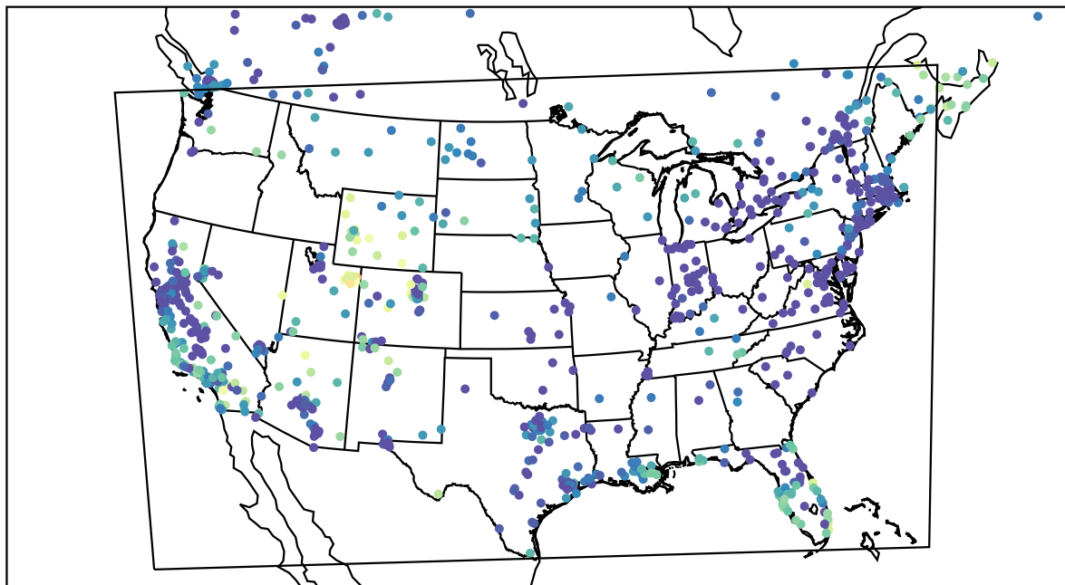
AirNOW (2022-12-21_00:00:00)
