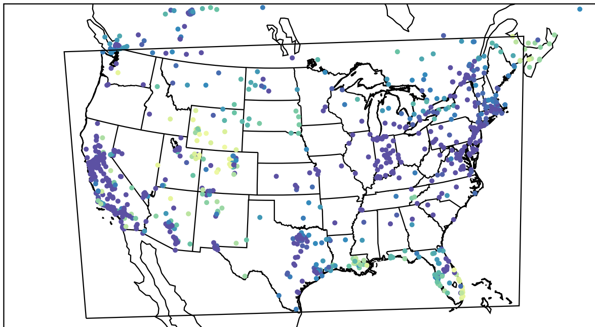
AirNOW (2022-12-20_03:00:00)
