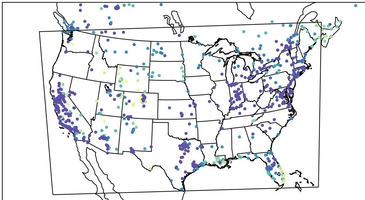
AirNOW (2022-12-20_08:00:00)
