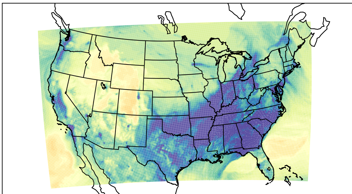
WRF (2022-12-21_02:00:00)
