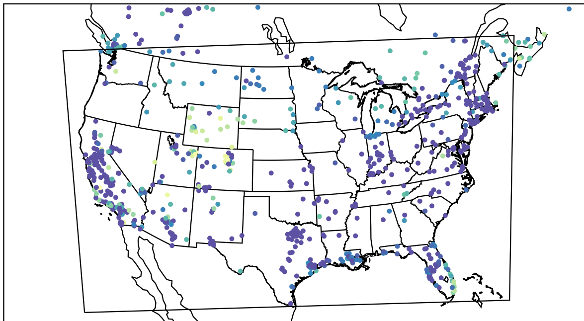
AirNOW (2022-12-21_09:00:00)
