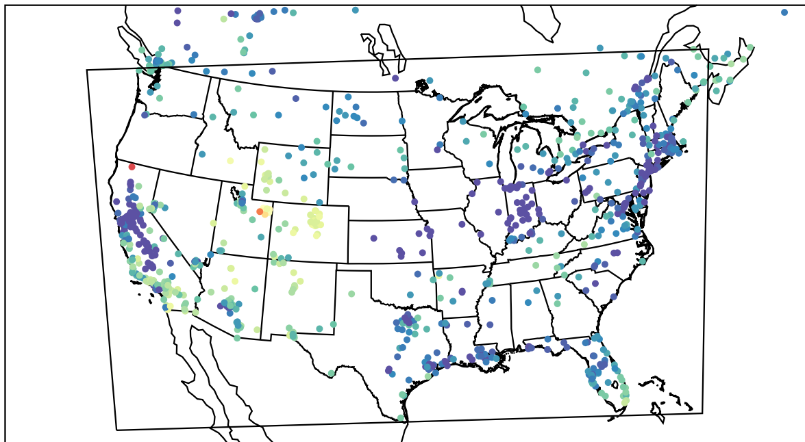
AirNOW (2022-12-21_20:00:00)
