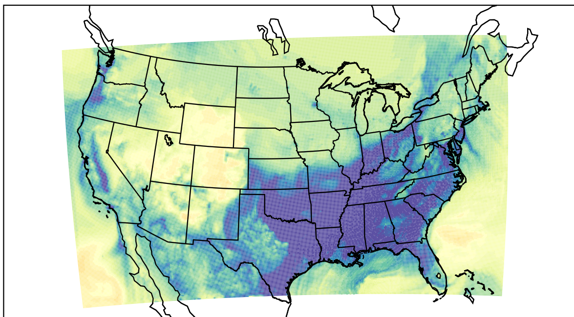
WRF (2022-12-21_12:00:00)
