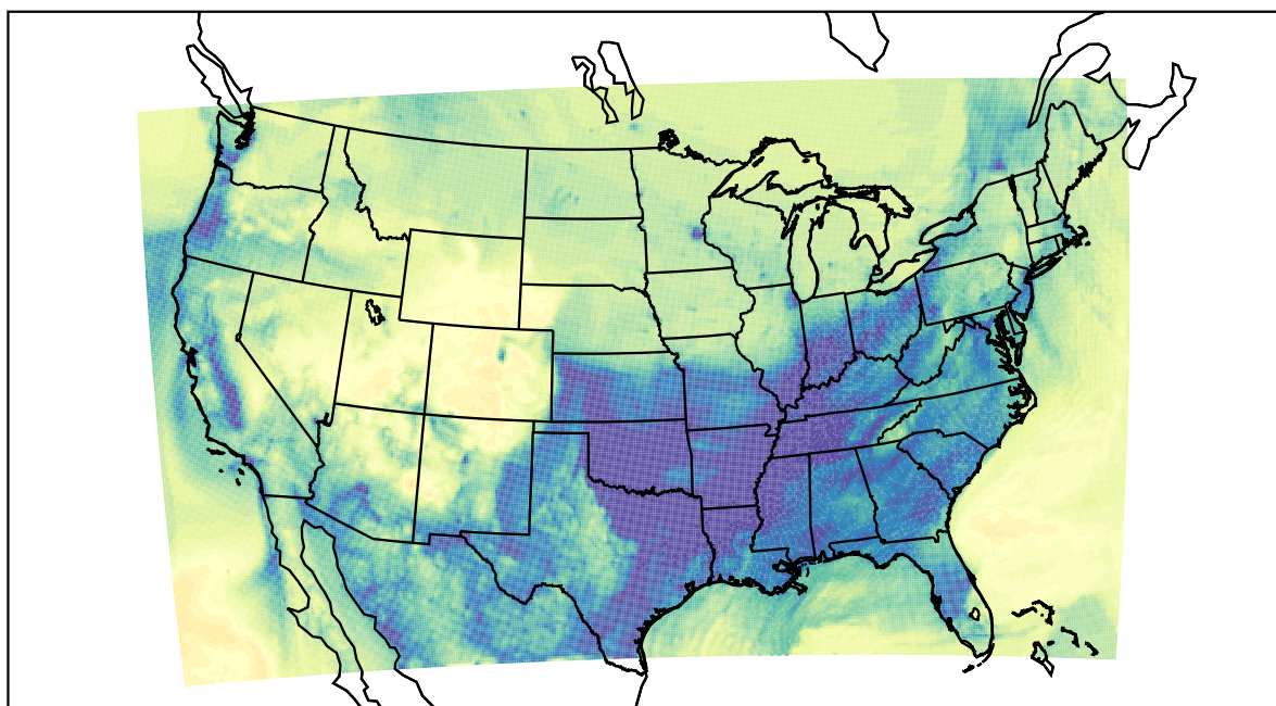
WRF (2022-12-21_15:00:00)
