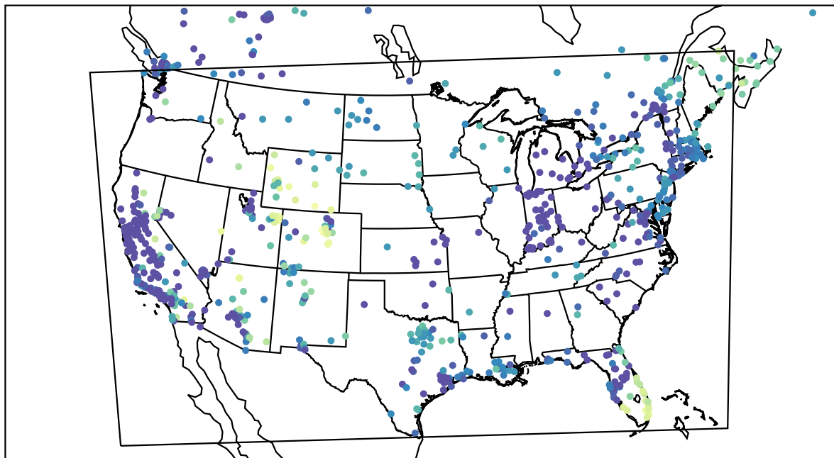
AirNOW (2022-12-20_17:00:00)
