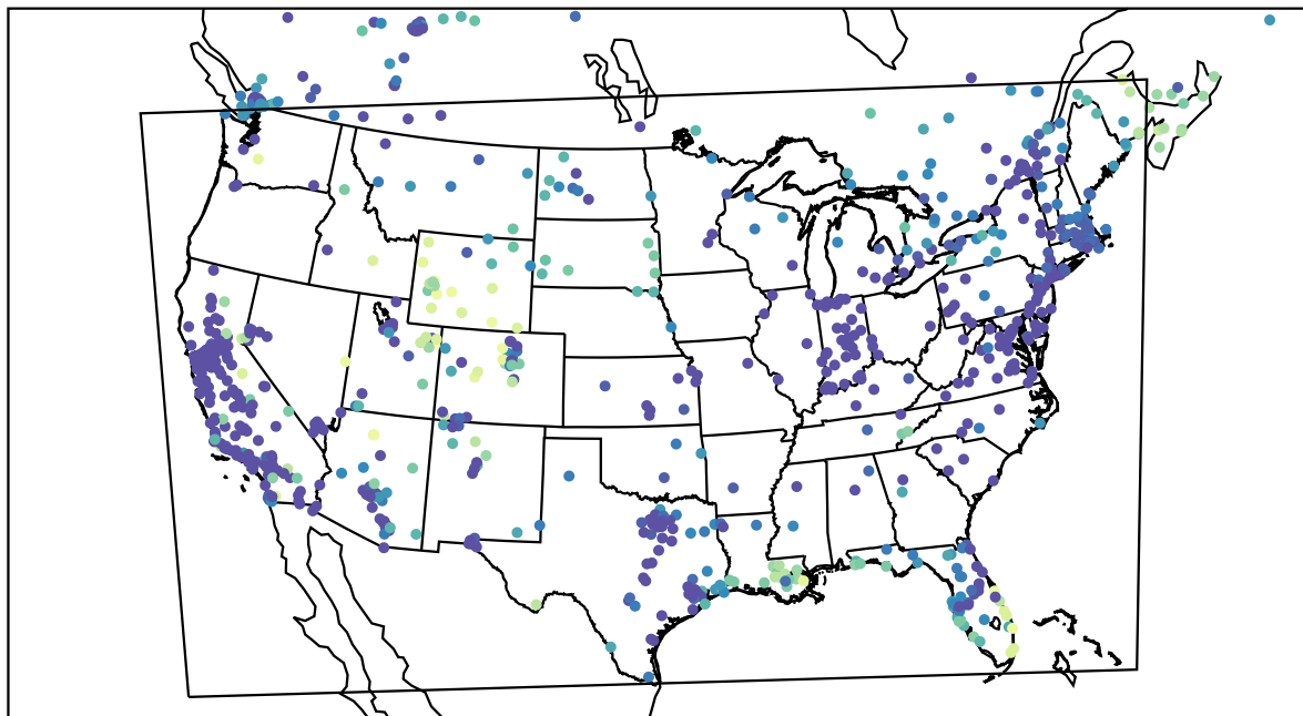
AirNOW (2022-12-20_05:00:00)
