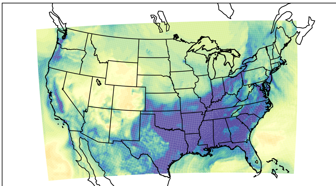
WRF (2022-12-21_11:00:00)
