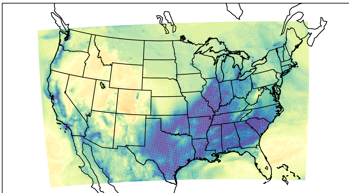
WRF (2022-12-20_16:00:00)
