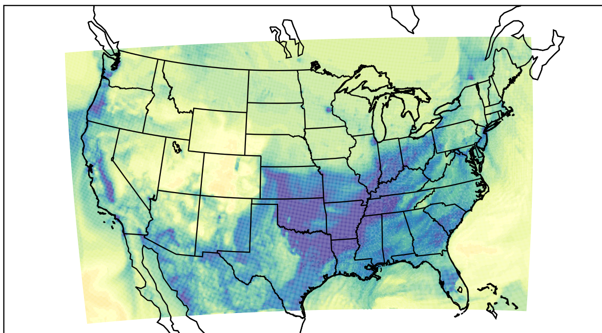
WRF (2022-12-21_16:00:00)
