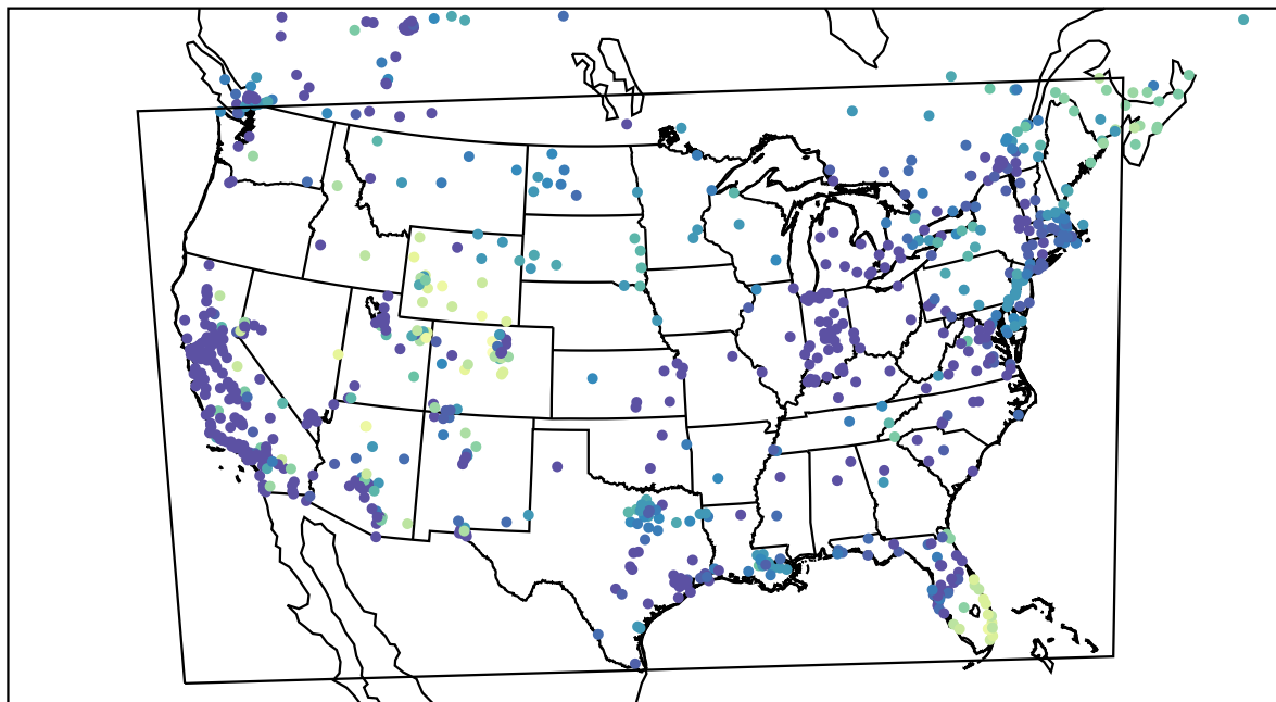
AirNOW (2022-12-20_16:00:00)
