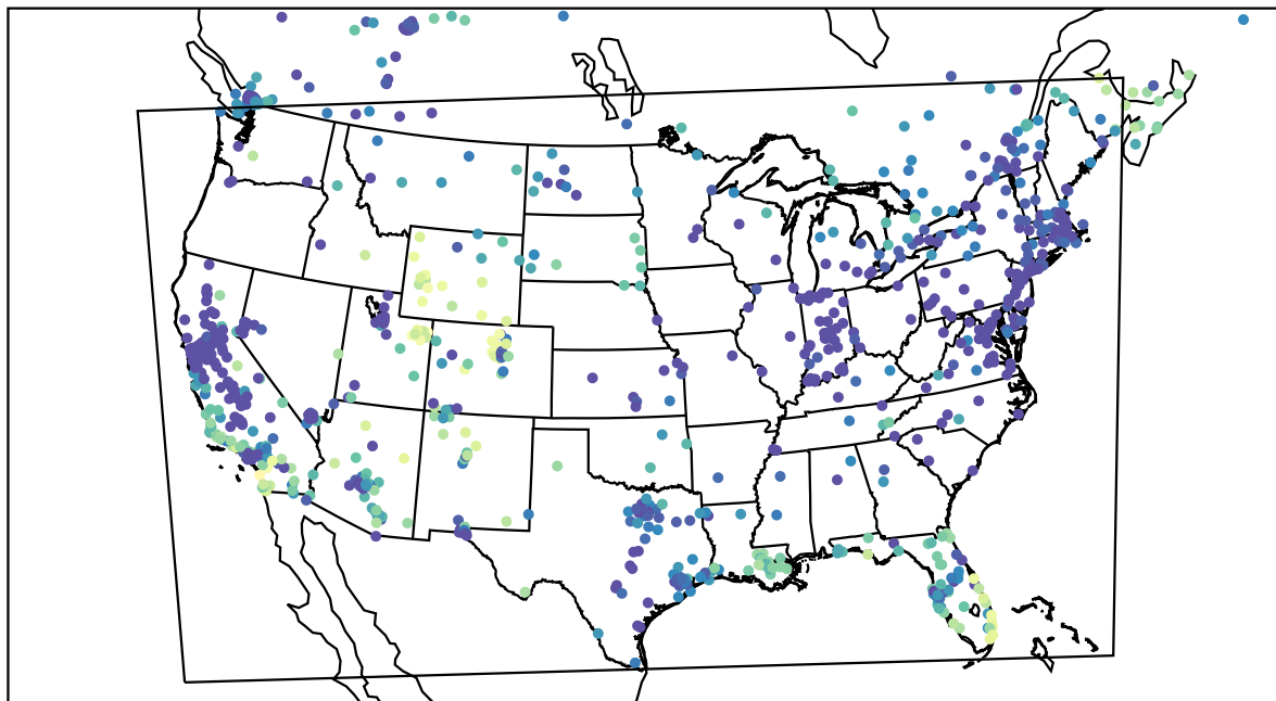
AirNOW (2022-12-20_00:00:00)
