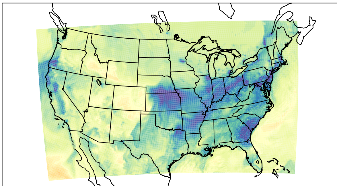
WRF (2022-12-21_21:00:00)
