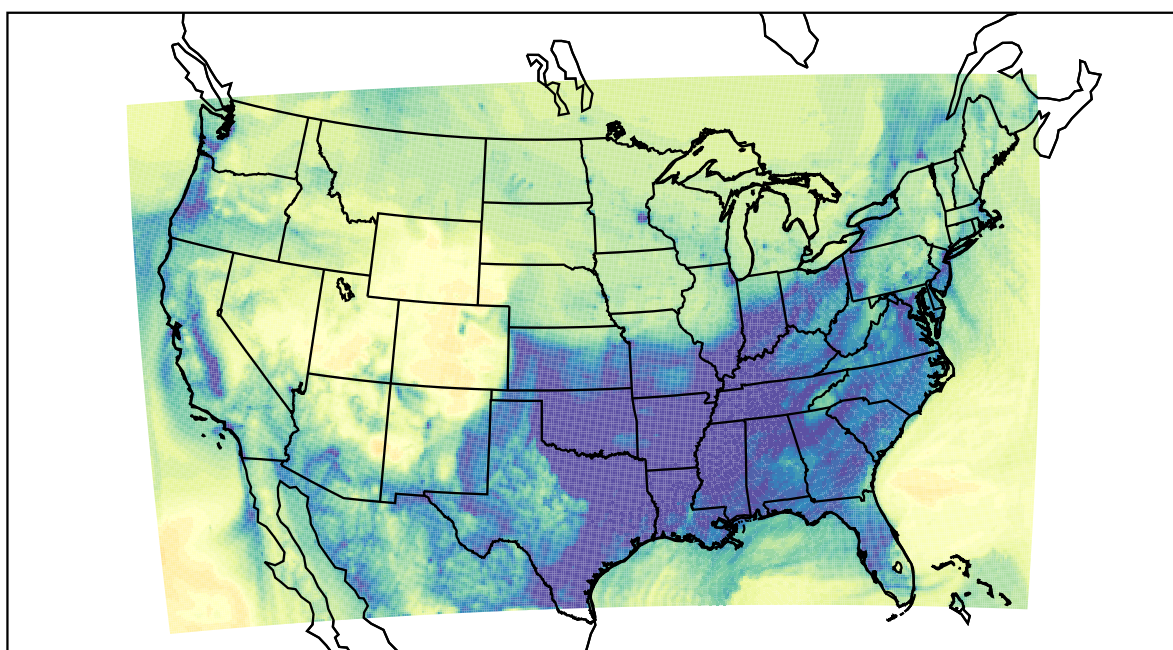
WRF (2022-12-21_14:00:00)
