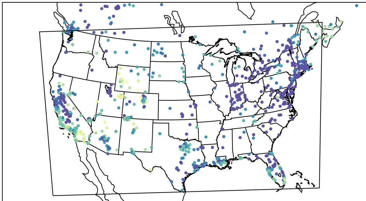
AirNOW (2022-12-20_23:00:00)
