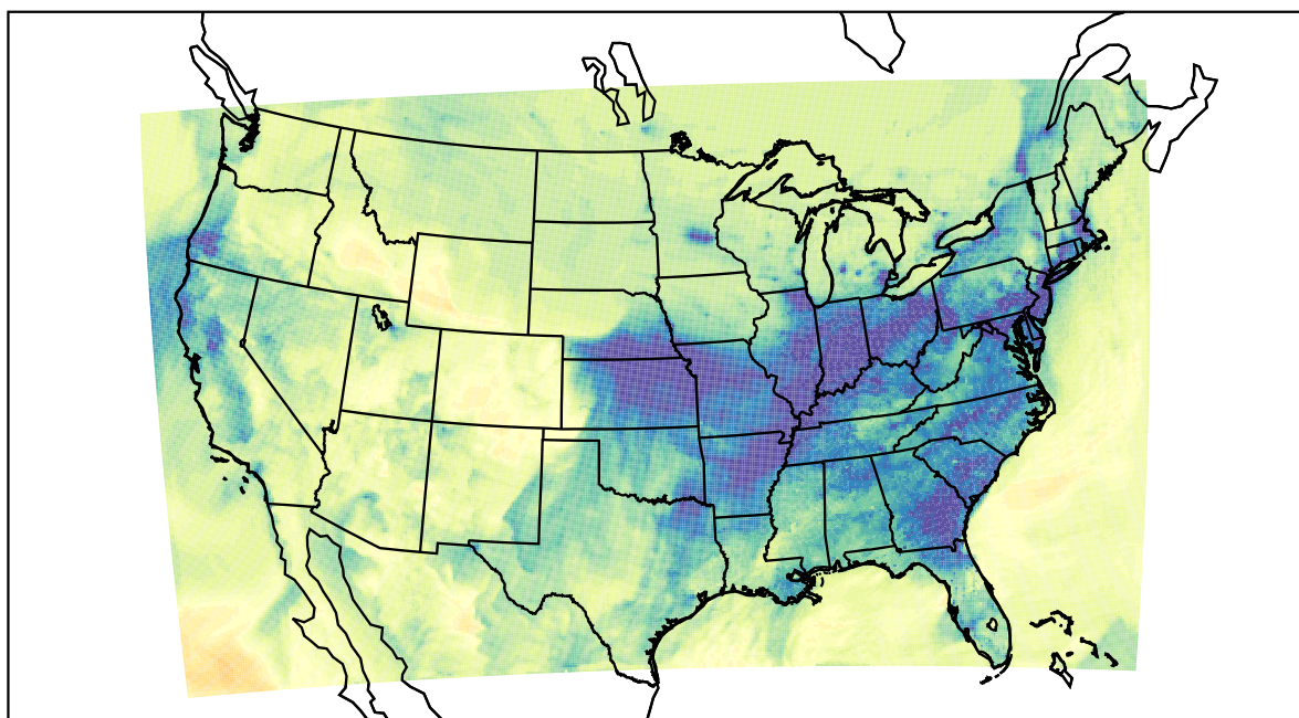
WRF (2022-12-21_22:00:00)
