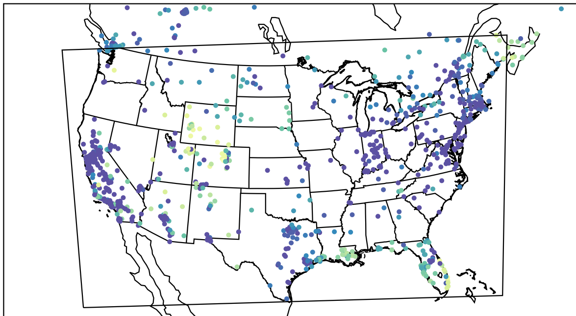
AirNOW (2022-12-20_02:00:00)
