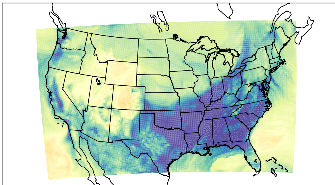
WRF (2022-12-21_08:00:00)
