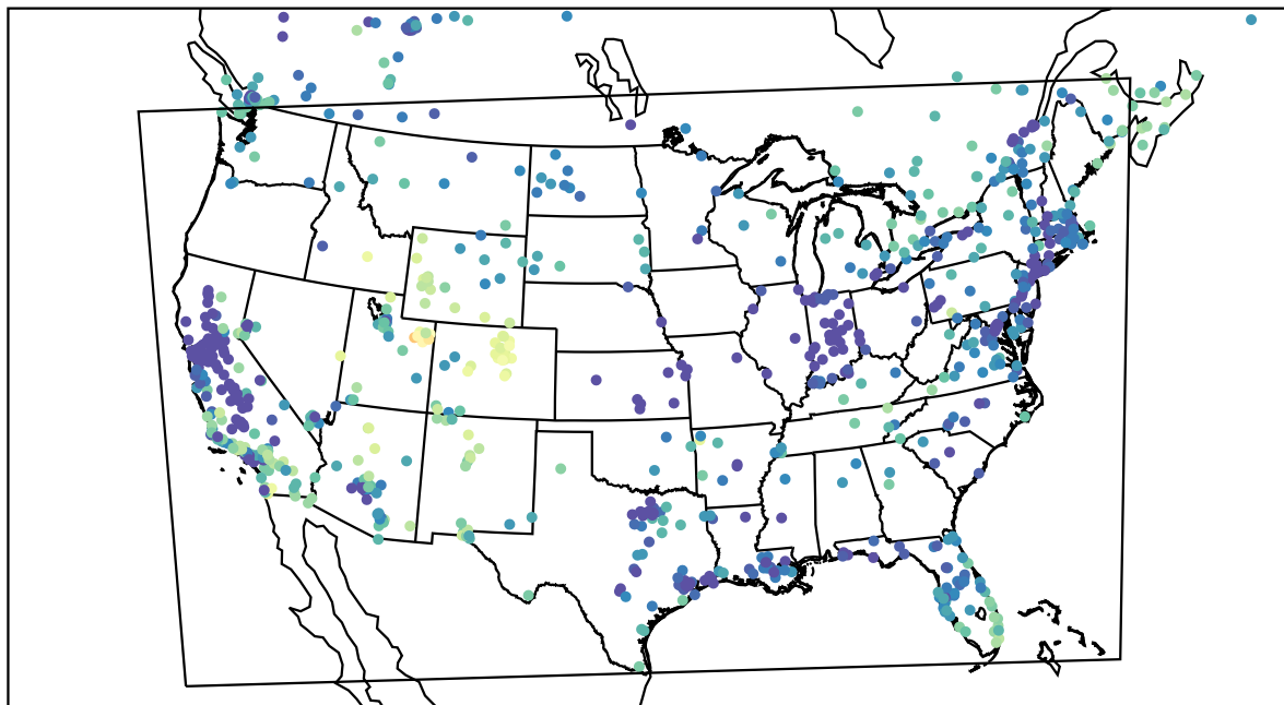
AirNOW (2022-12-21_19:00:00)
