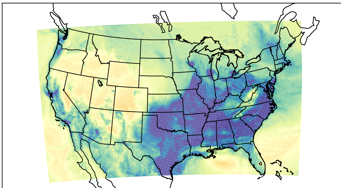
WRF (2022-12-20_07:00:00)
