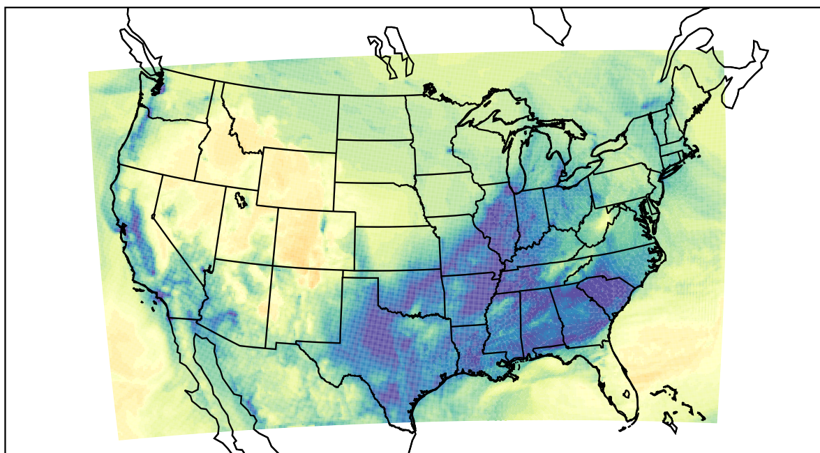
WRF (2022-12-20_17:00:00)
