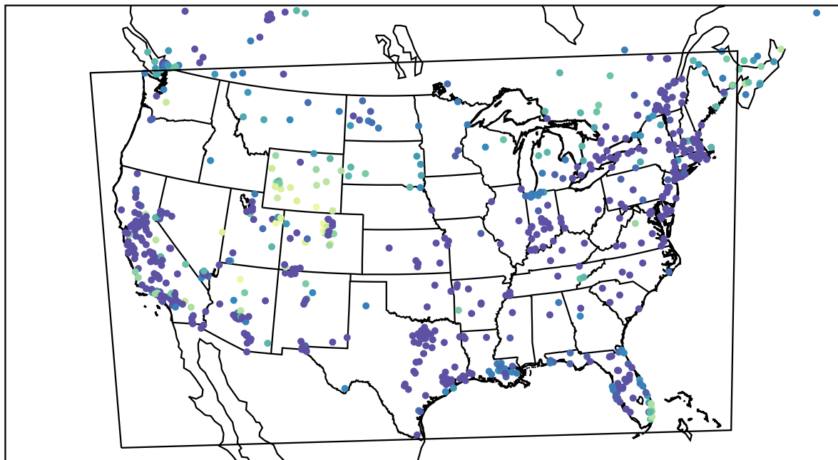
AirNOW (2022-12-21_10:00:00)
