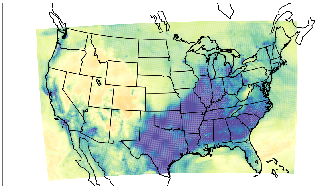
WRF (2022-12-20_14:00:00)
