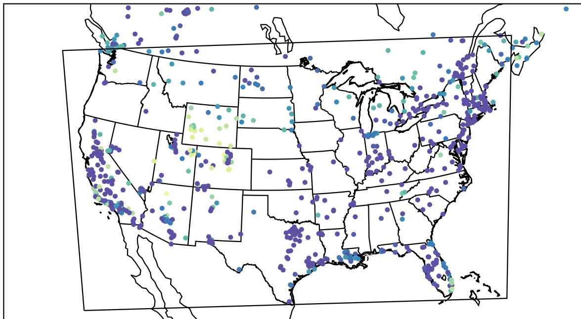
AirNOW (2022-12-21_11:00:00)
