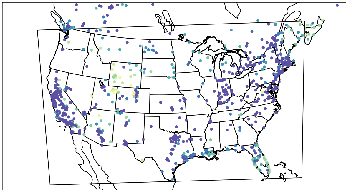
AirNOW (2022-12-21_02:00:00)
