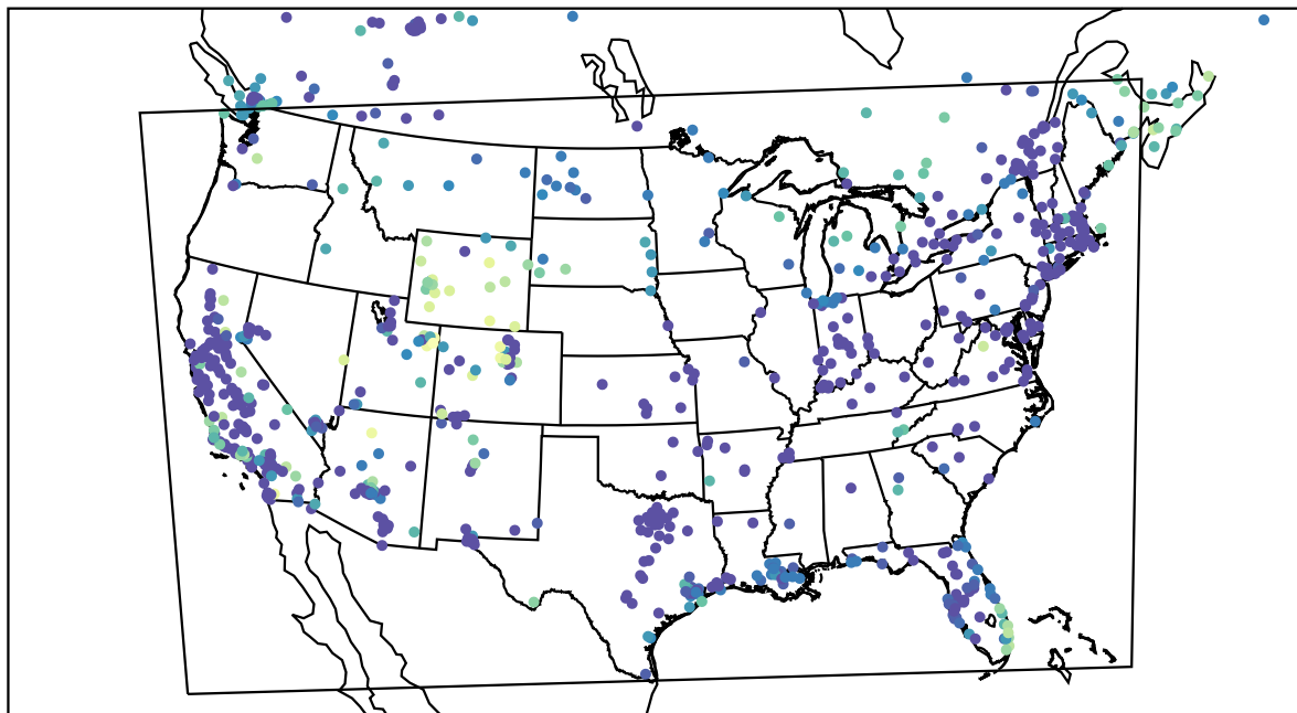
AirNOW (2022-12-21_08:00:00)
