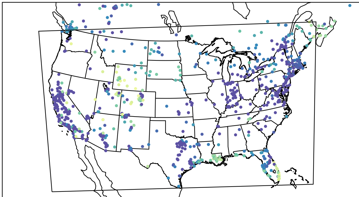
AirNOW (2022-12-20_06:00:00)
