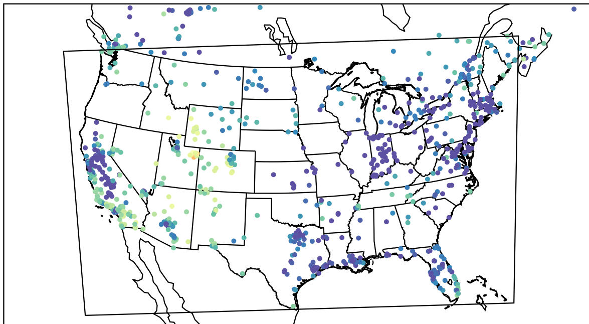
AirNOW (2022-12-21_23:00:00)
