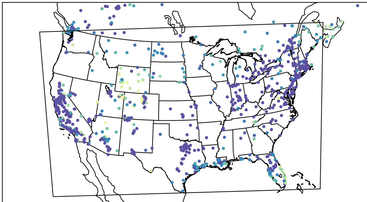
AirNOW (2022-12-21_04:00:00)
