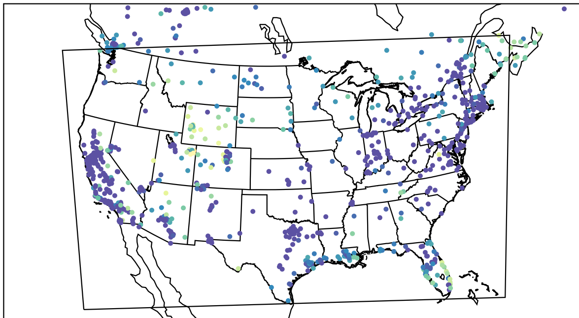
AirNOW (2022-12-21_03:00:00)
