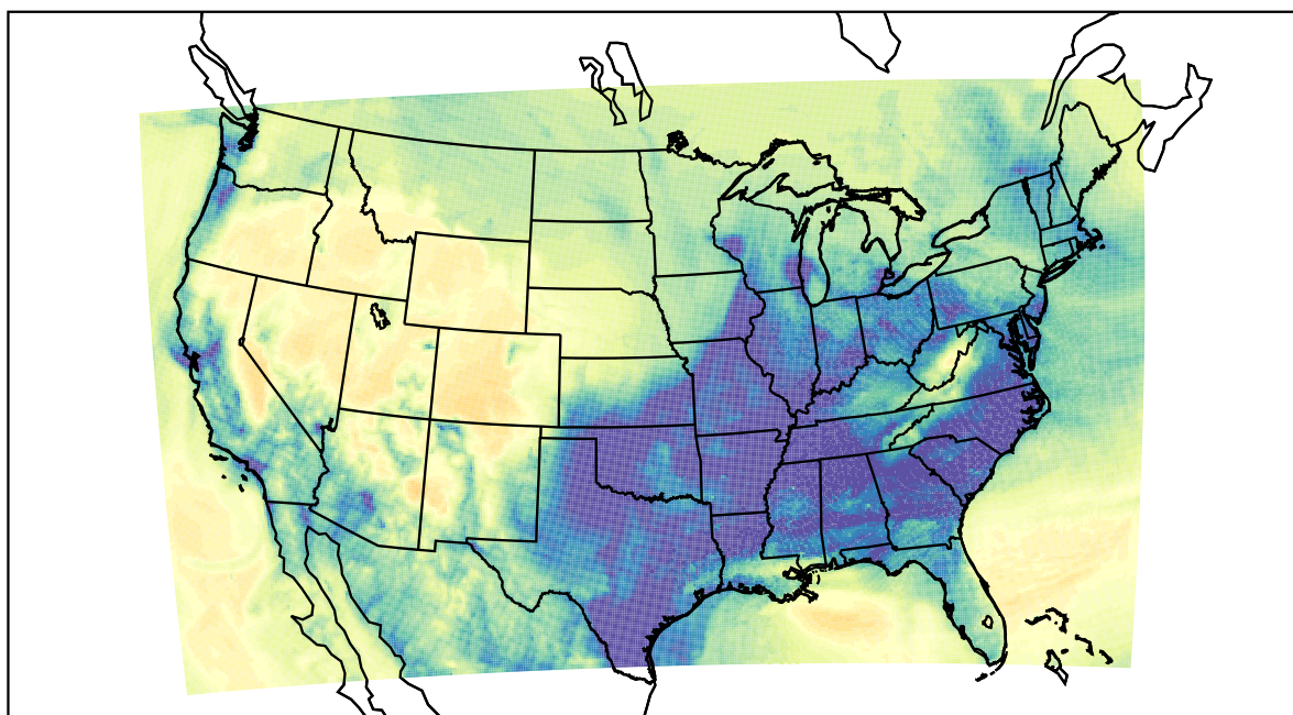
WRF (2022-12-20_08:00:00)
