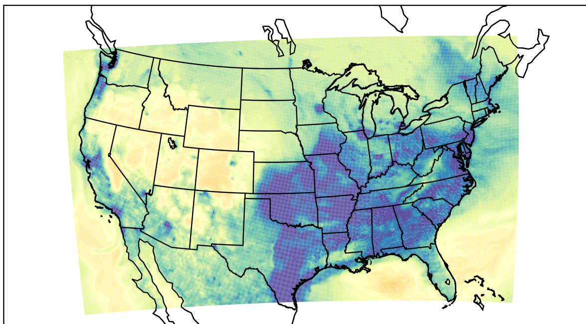
WRF (2022-12-20_03:00:00)
