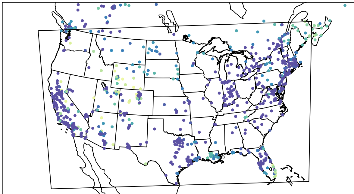
AirNOW (2022-12-20_13:00:00)
