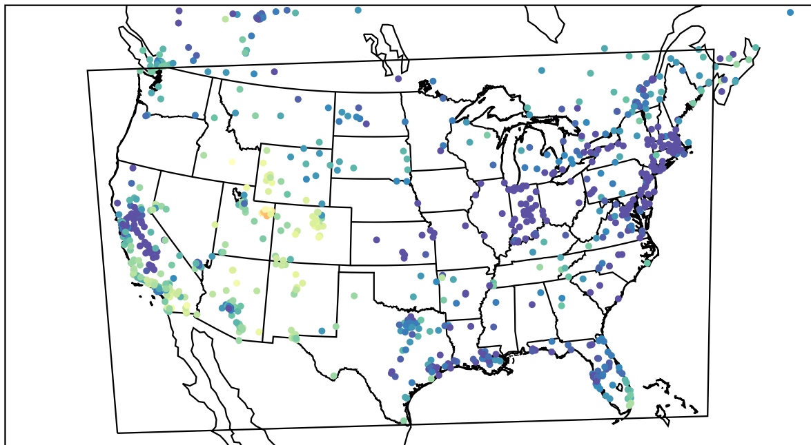
AirNOW (2022-12-21_22:00:00)
