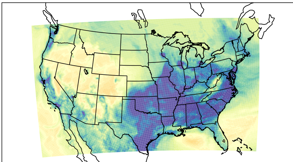
WRF (2022-12-20_06:00:00)
