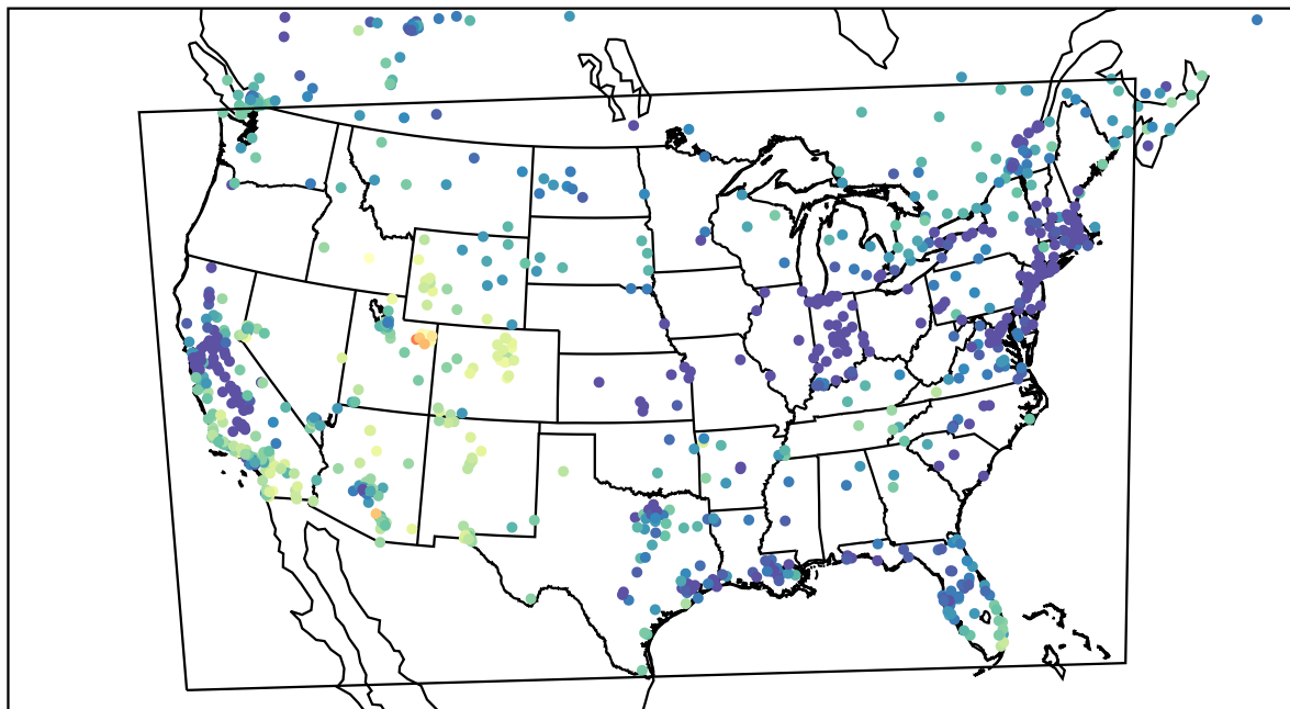
AirNOW (2022-12-21_21:00:00)
