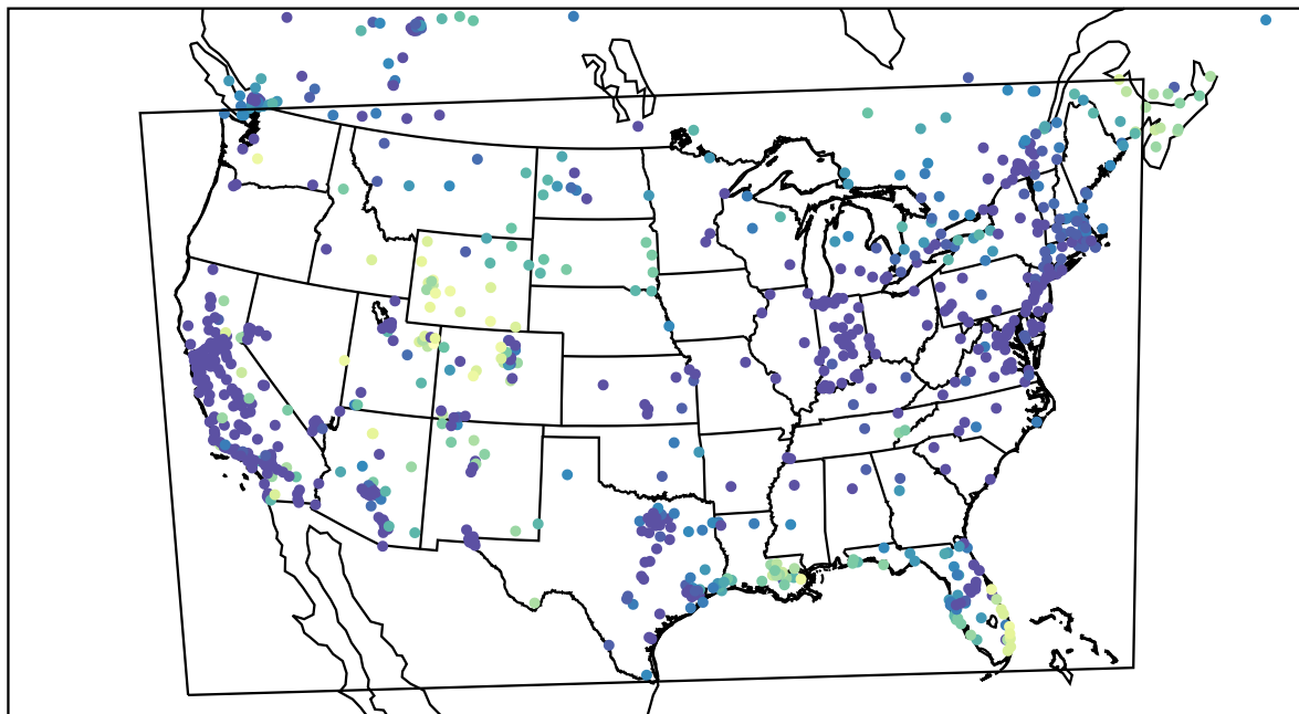
AirNOW (2022-12-20_04:00:00)
