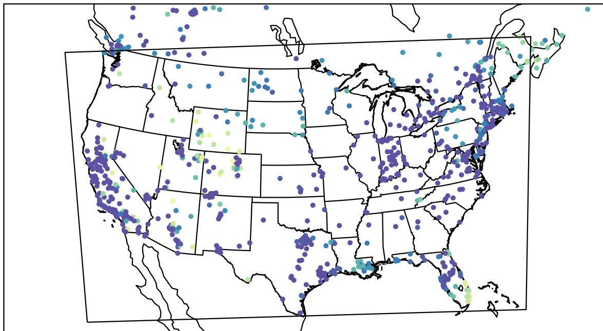
AirNOW (2022-12-20_14:00:00)
