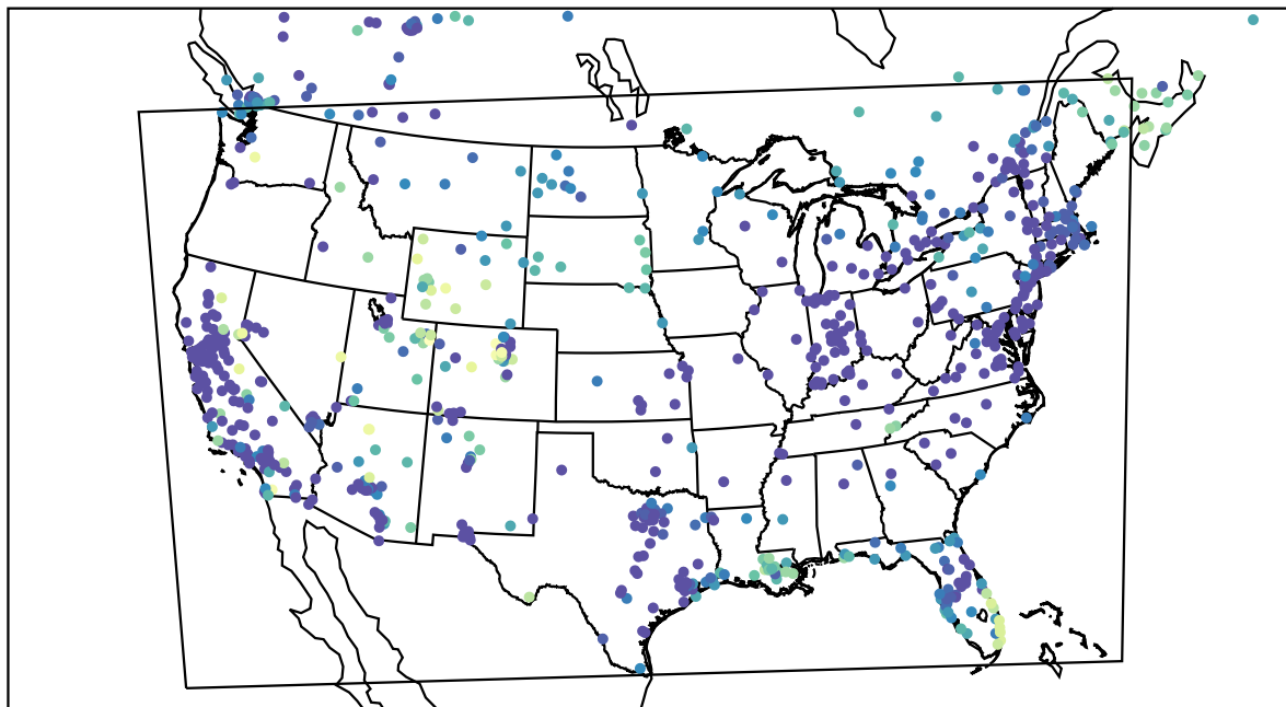
AirNOW (2022-12-20_09:00:00)
