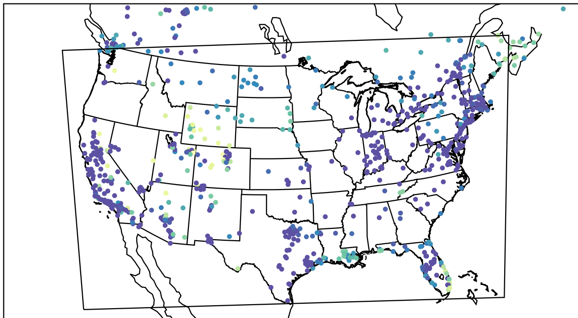
AirNOW (2022-12-20_11:00:00)
