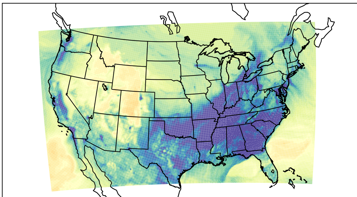
WRF (2022-12-21_03:00:00)
