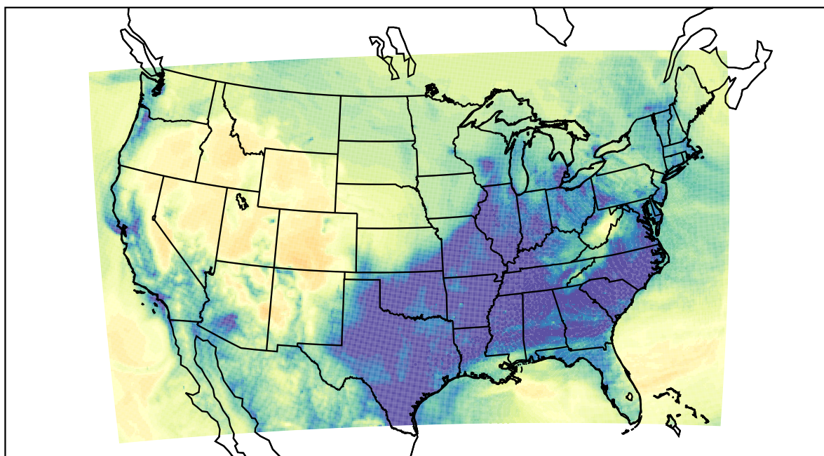
WRF (2022-12-20_12:00:00)
