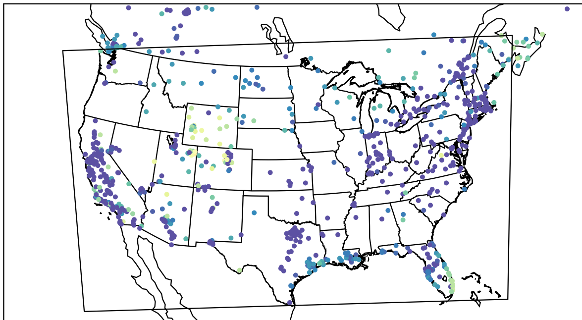
AirNOW (2022-12-21_06:00:00)
