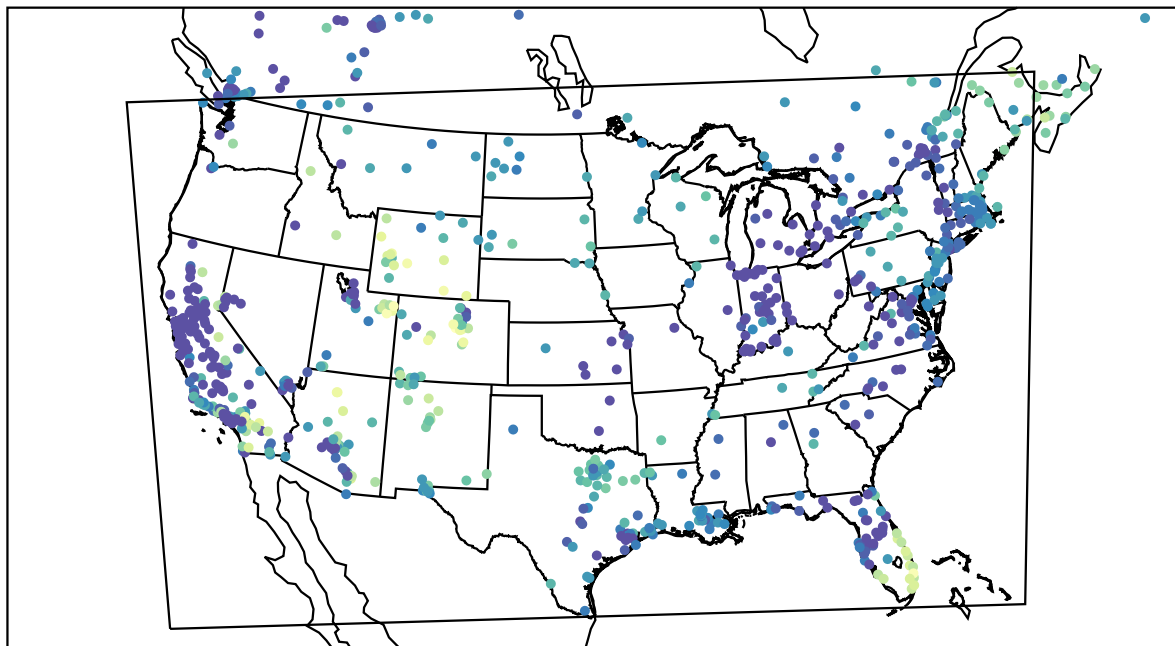
AirNOW (2022-12-20_18:00:00)
