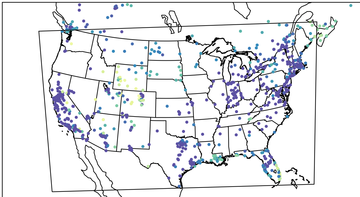
AirNOW (2022-12-20_10:00:00)
