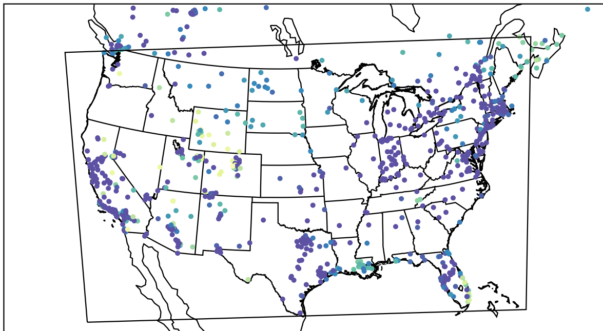
AirNOW (2022-12-20_12:00:00)
