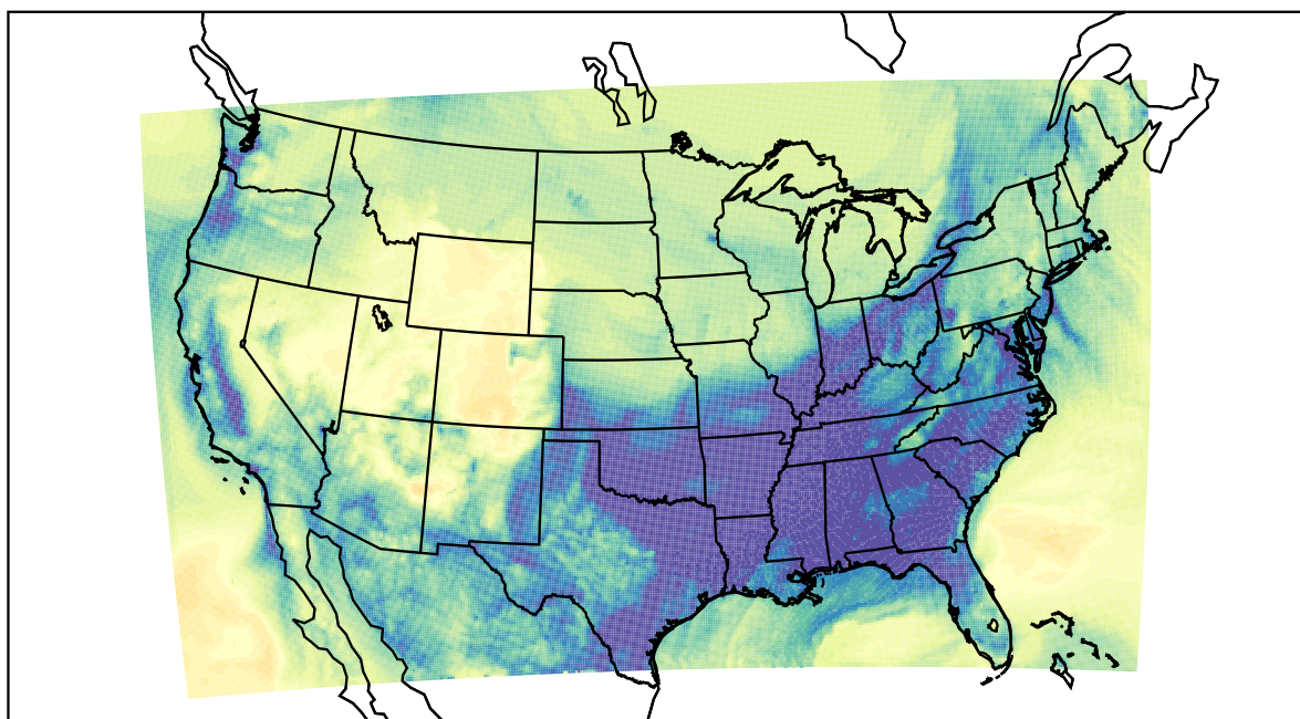
WRF (2022-12-21_10:00:00)
