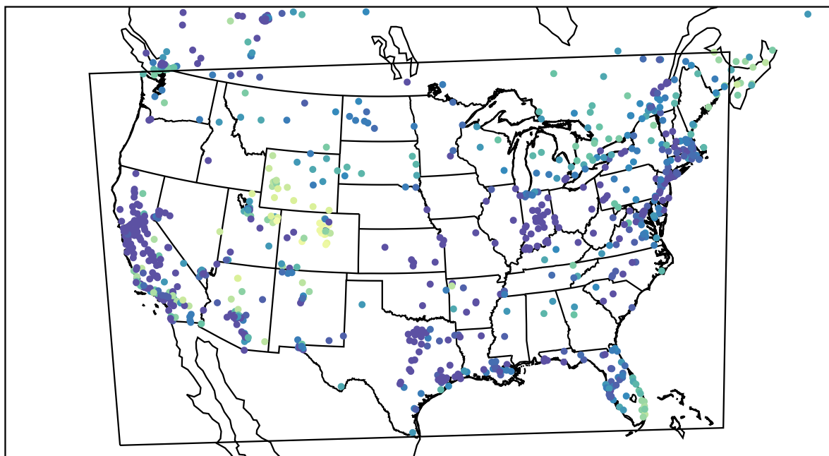
AirNOW (2022-12-21_17:00:00)
