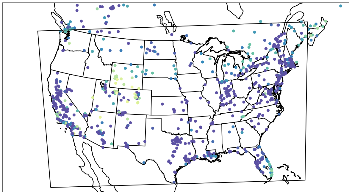
AirNOW (2022-12-21_14:00:00)
