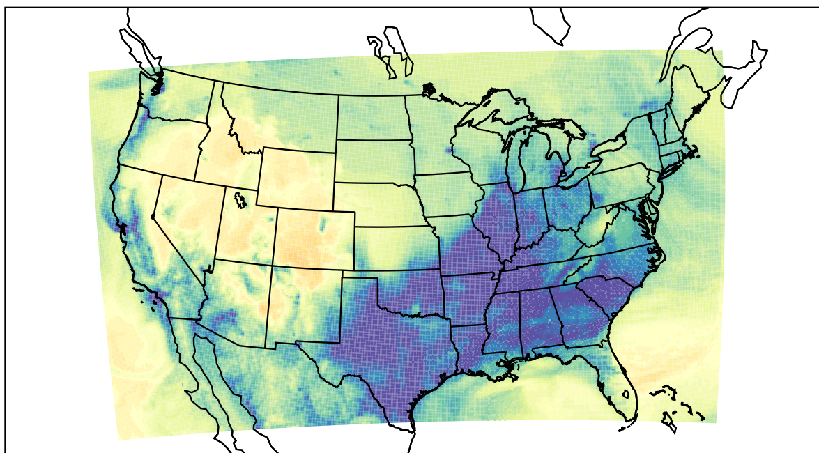
WRF (2022-12-20_15:00:00)
