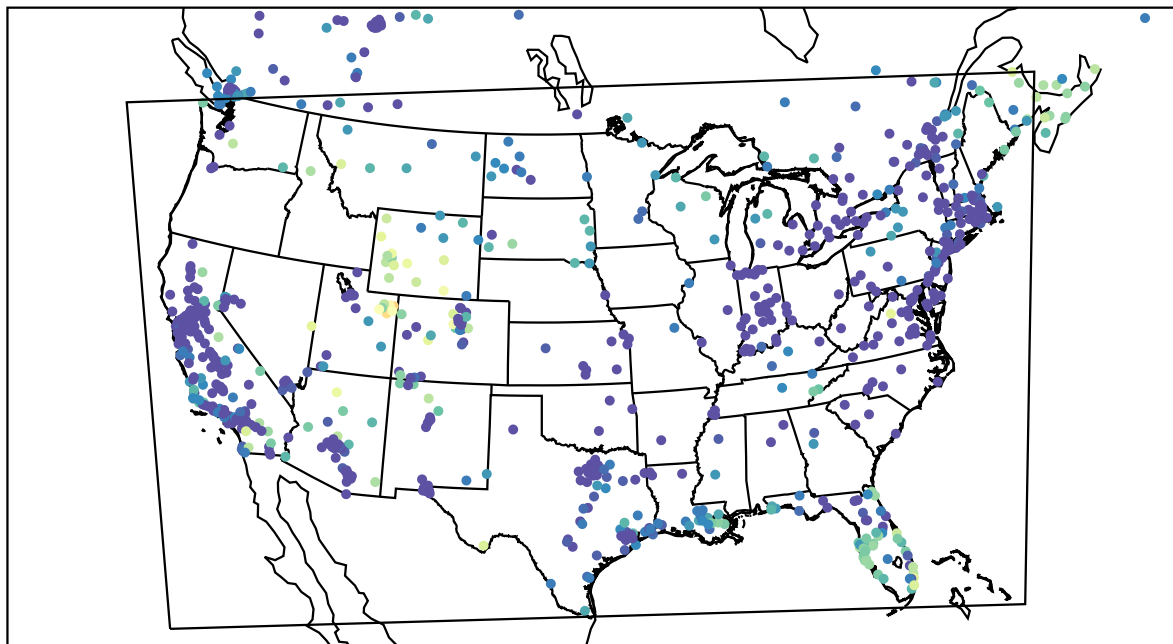
AirNOW (2022-12-21_01:00:00)
