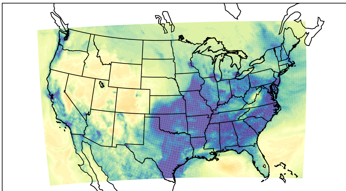
WRF (2022-12-20_05:00:00)
