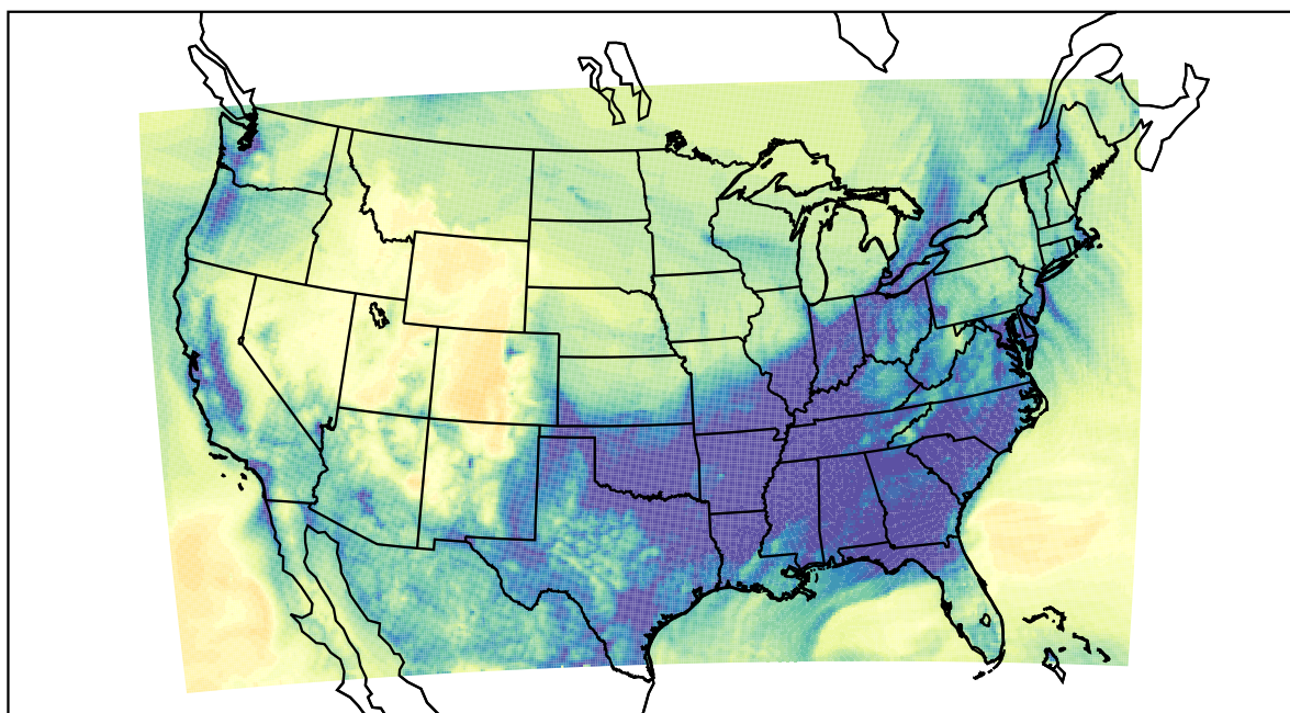
WRF (2022-12-21_06:00:00)
