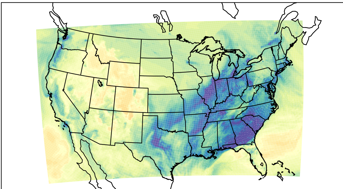
WRF (2022-12-20_21:00:00)
