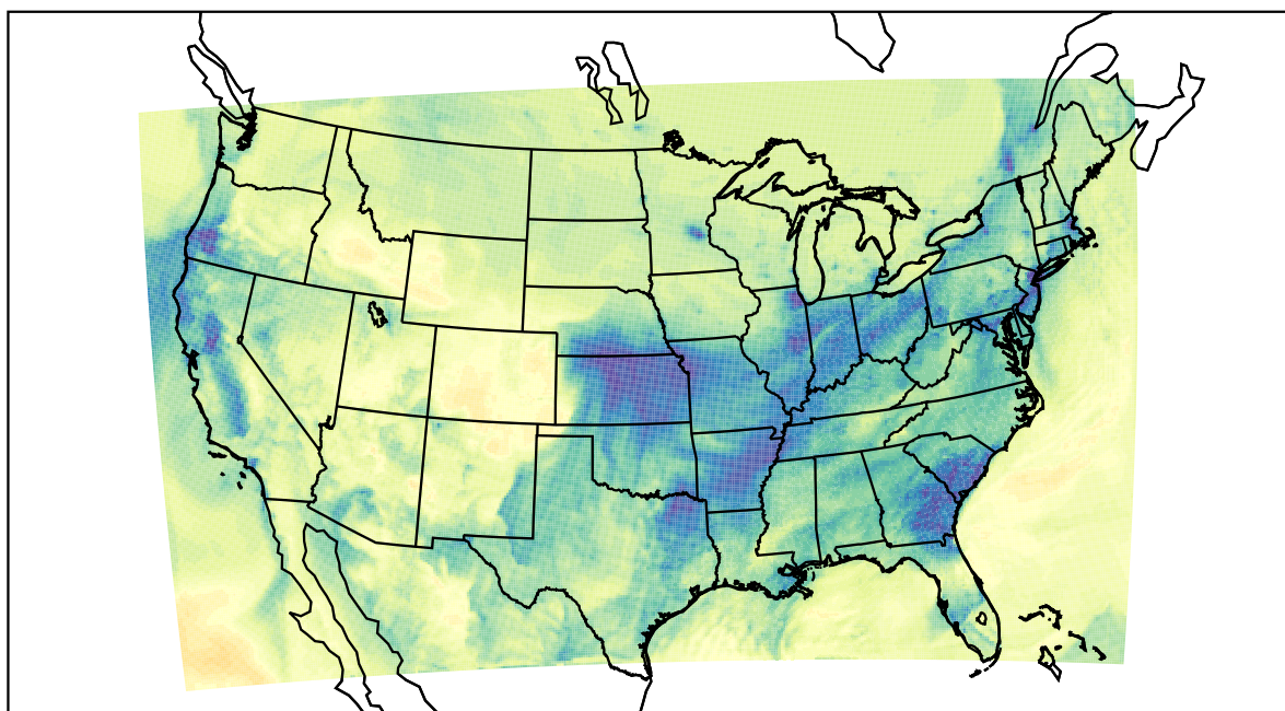
WRF (2022-12-21_20:00:00)
