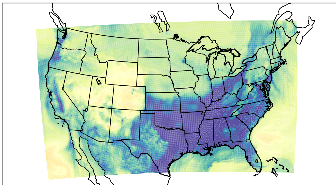
WRF (2022-12-21_13:00:00)
