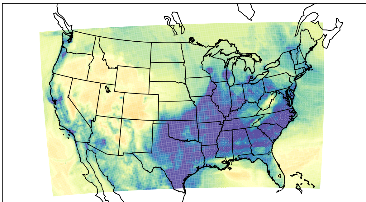
WRF (2022-12-20_09:00:00)
