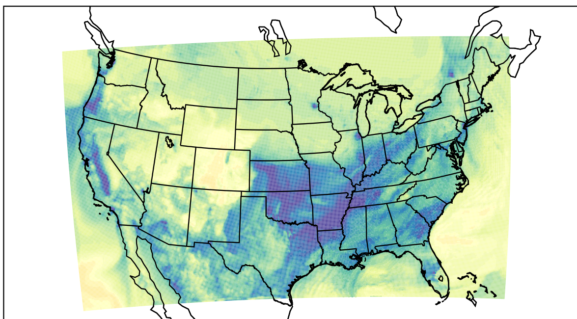
WRF (2022-12-21_17:00:00)
