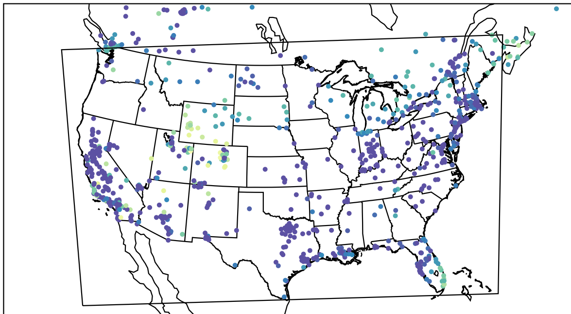
AirNOW (2022-12-21_15:00:00)
