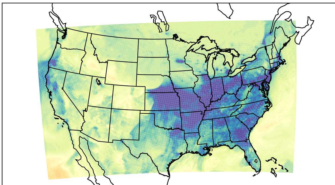
WRF (2022-12-21_23:00:00)
