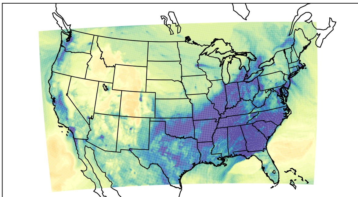
WRF (2022-12-21_01:00:00)
