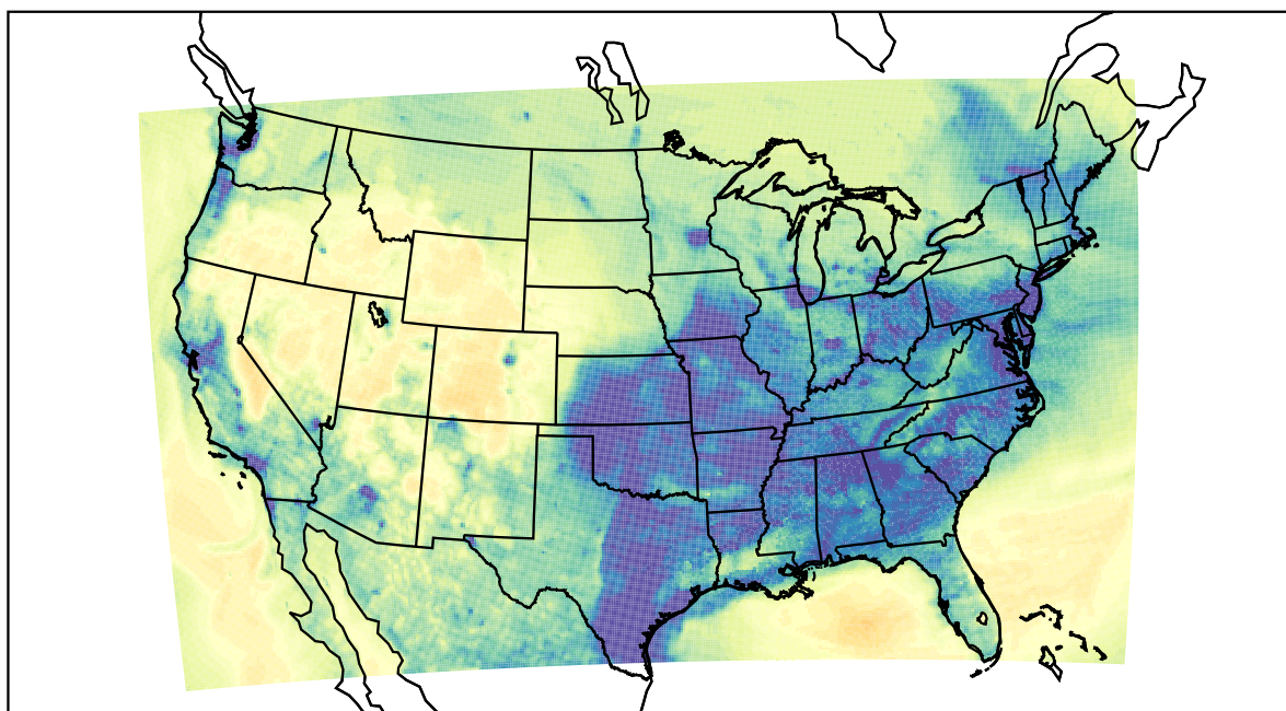
WRF (2022-12-20_02:00:00)
