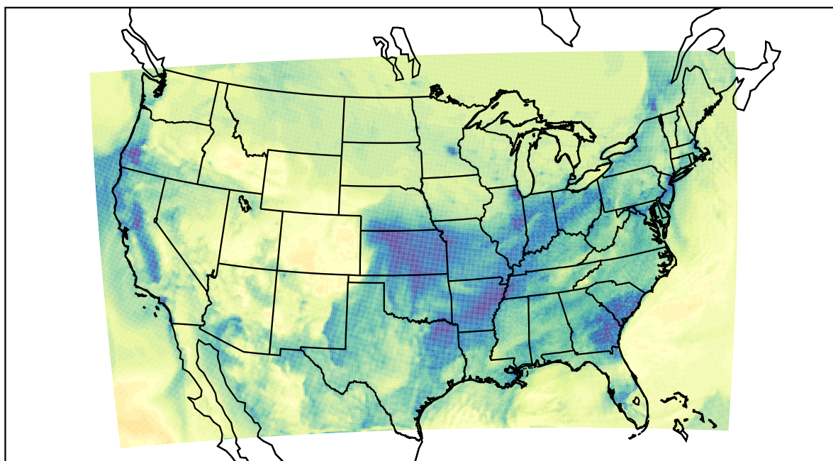
WRF (2022-12-21_19:00:00)
