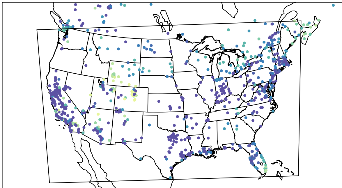
AirNOW (2022-12-21_16:00:00)
