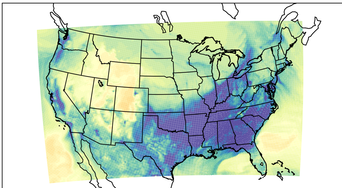
WRF (2022-12-21_05:00:00)
