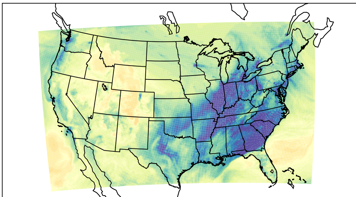
WRF (2022-12-20_22:00:00)
