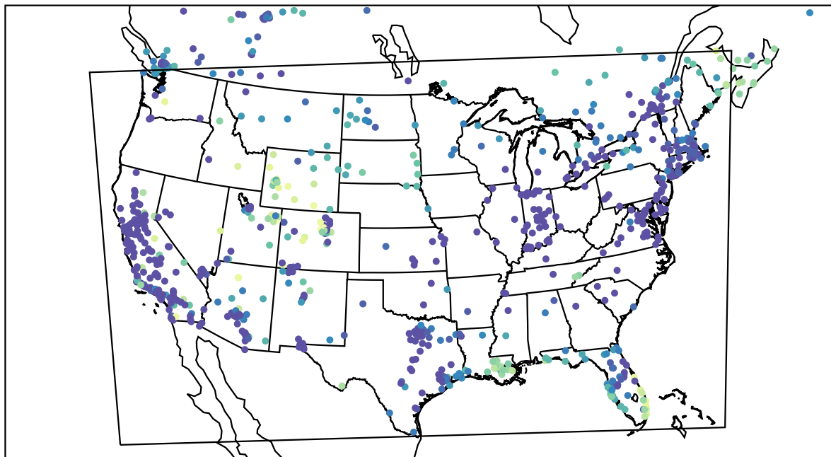
AirNOW (2022-12-20_07:00:00)
