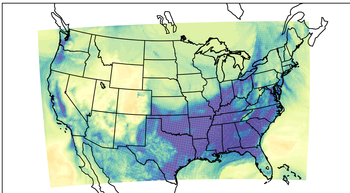
WRF (2022-12-21_09:00:00)
