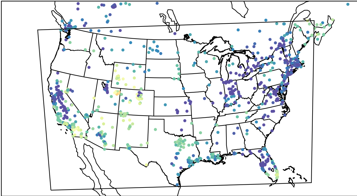
AirNOW (2022-12-20_21:00:00)
