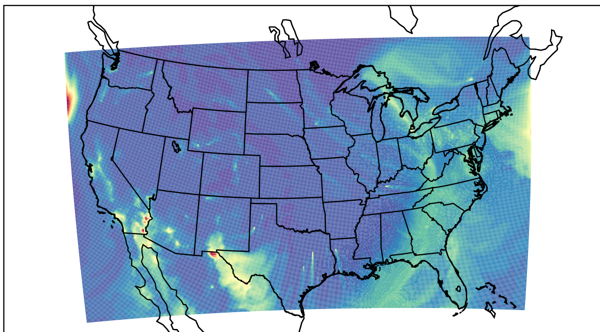
WRF 2022-12-23_08:00:00
