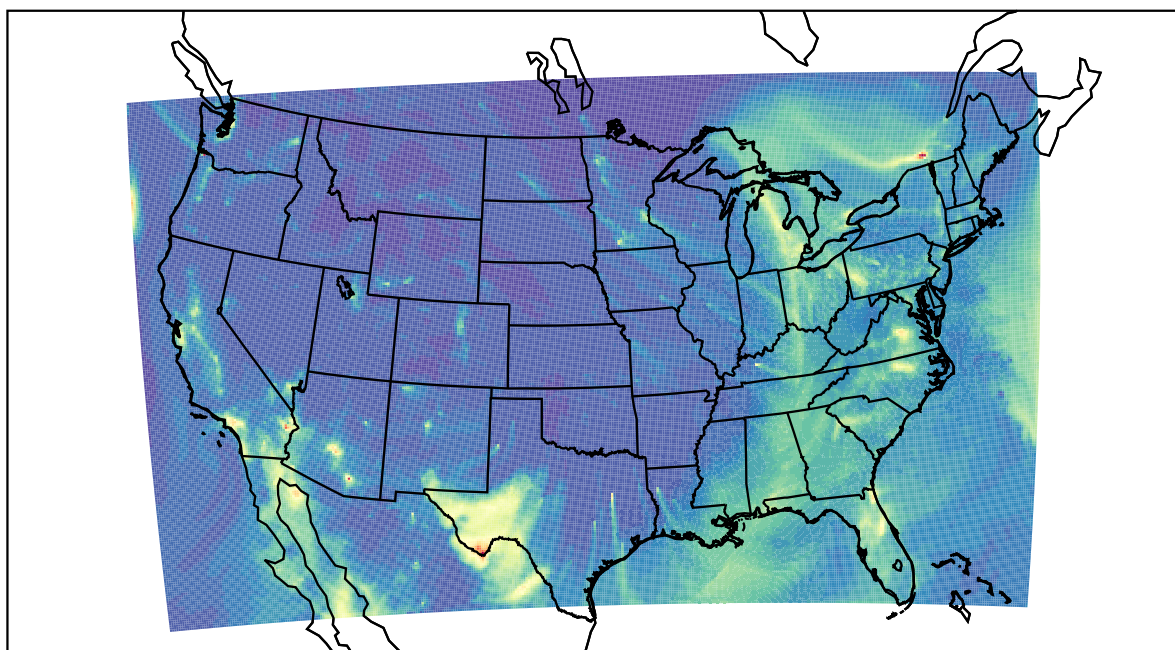
WRF 2022-12-23_04:00:00
