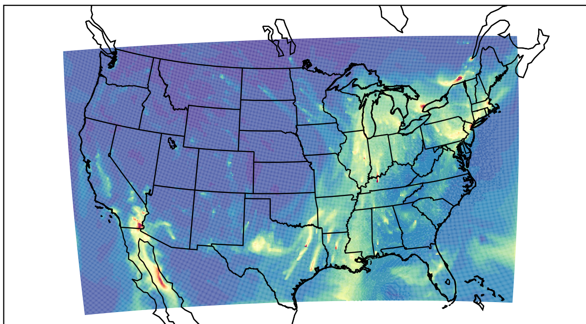
WRF 2022-12-22_15:00:00
