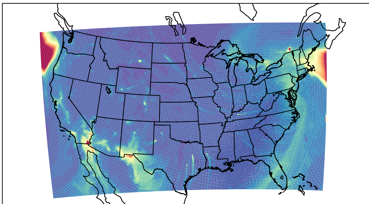
WRF 2022-12-23_15:00:00
