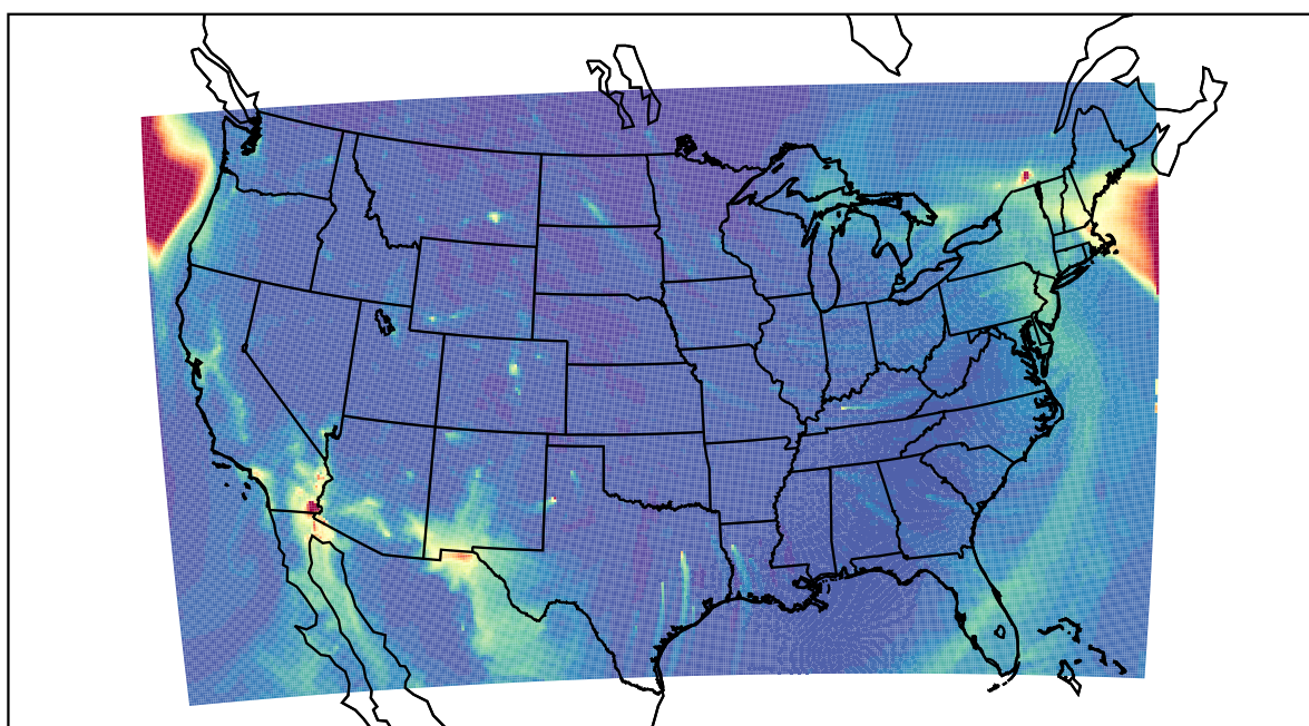
WRF 2022-12-23_16:00:00
