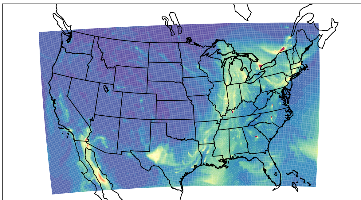
WRF 2022-12-22_19:00:00
