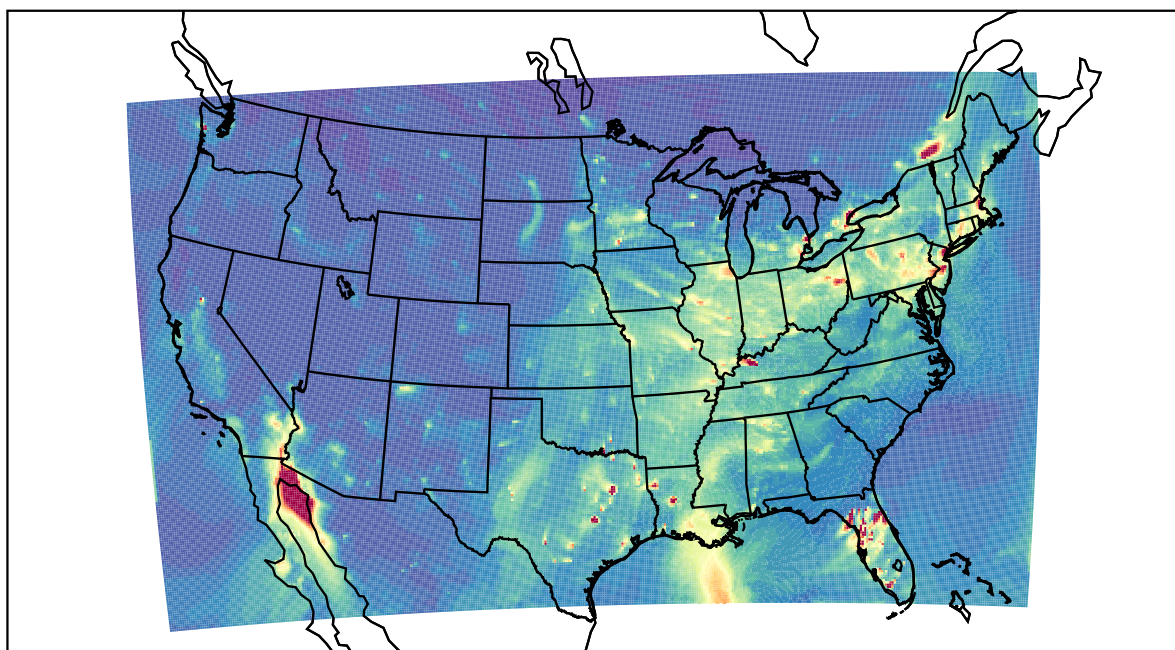
WRF 2022-12-22_00:00:00
