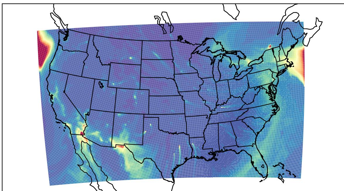
WRF 2022-12-23_14:00:00
