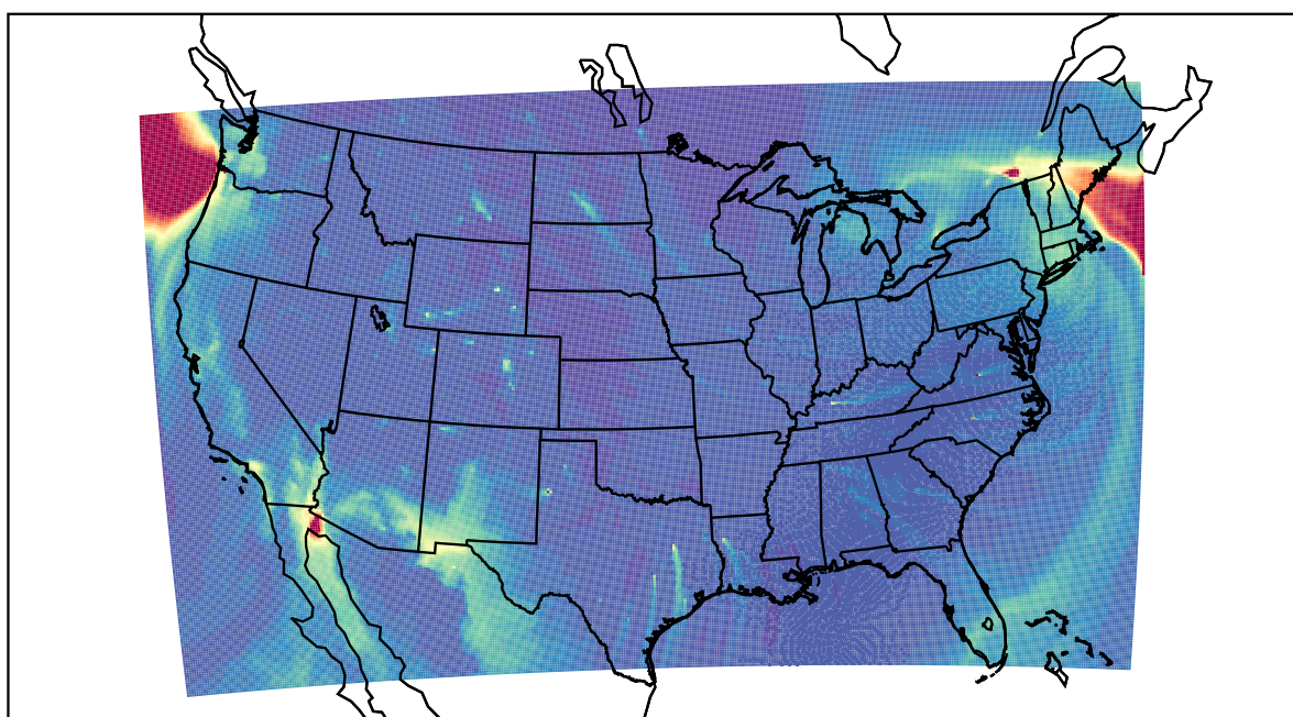
WRF 2022-12-23_20:00:00
