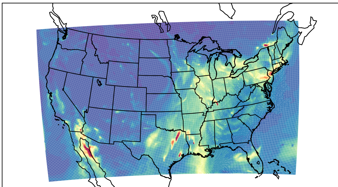
WRF 2022-12-22_08:00:00
