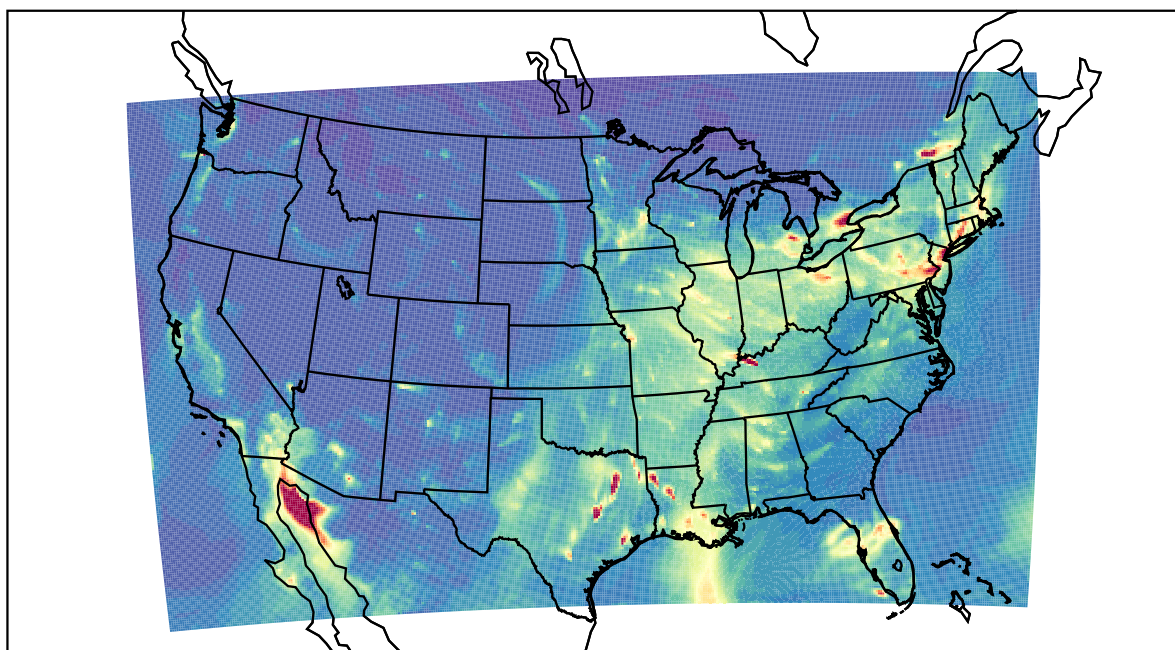
WRF 2022-12-22_04:00:00
