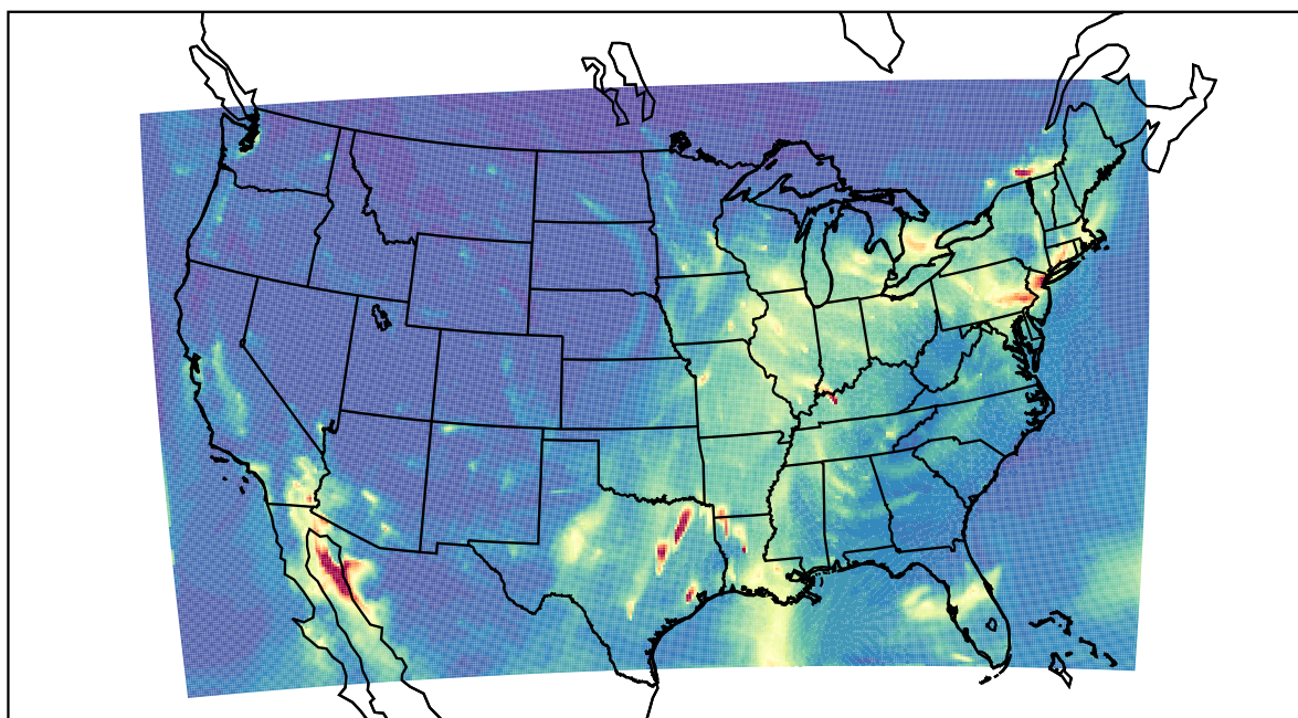
WRF 2022-12-22_07:00:00
