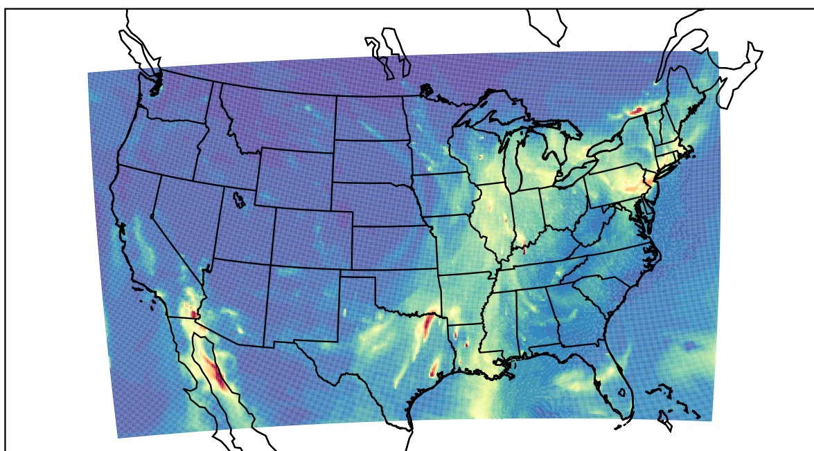
WRF 2022-12-22_11:00:00
