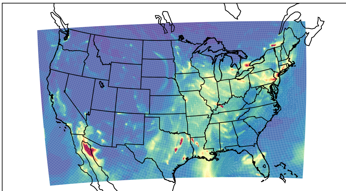
WRF 2022-12-22_05:00:00
