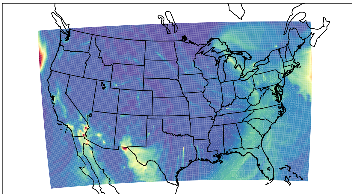
WRF 2022-12-23_09:00:00
