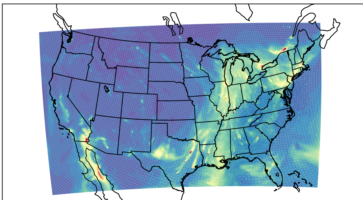
WRF 2022-12-22_16:00:00
