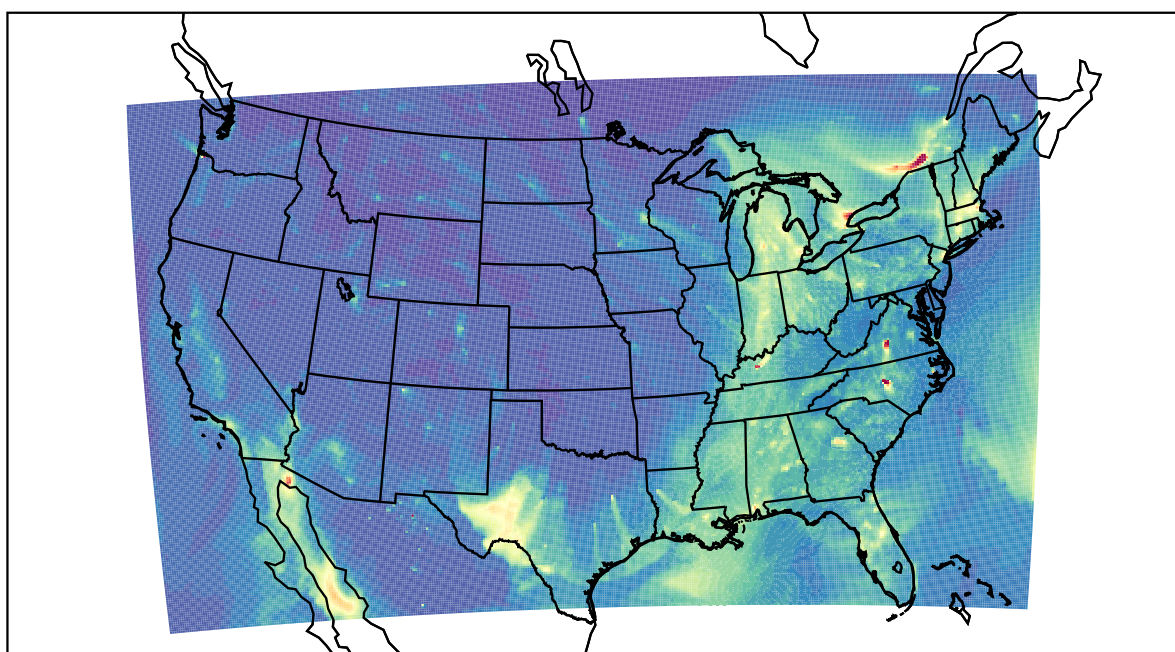
WRF 2022-12-22_23:00:00
