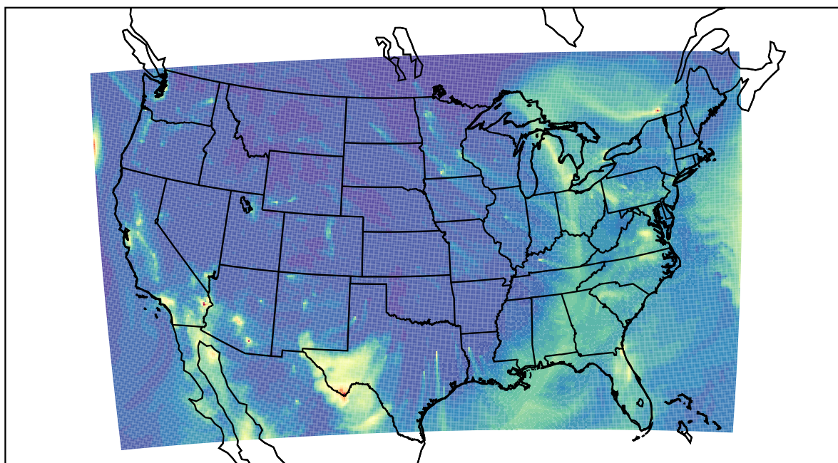
WRF 2022-12-23_05:00:00
