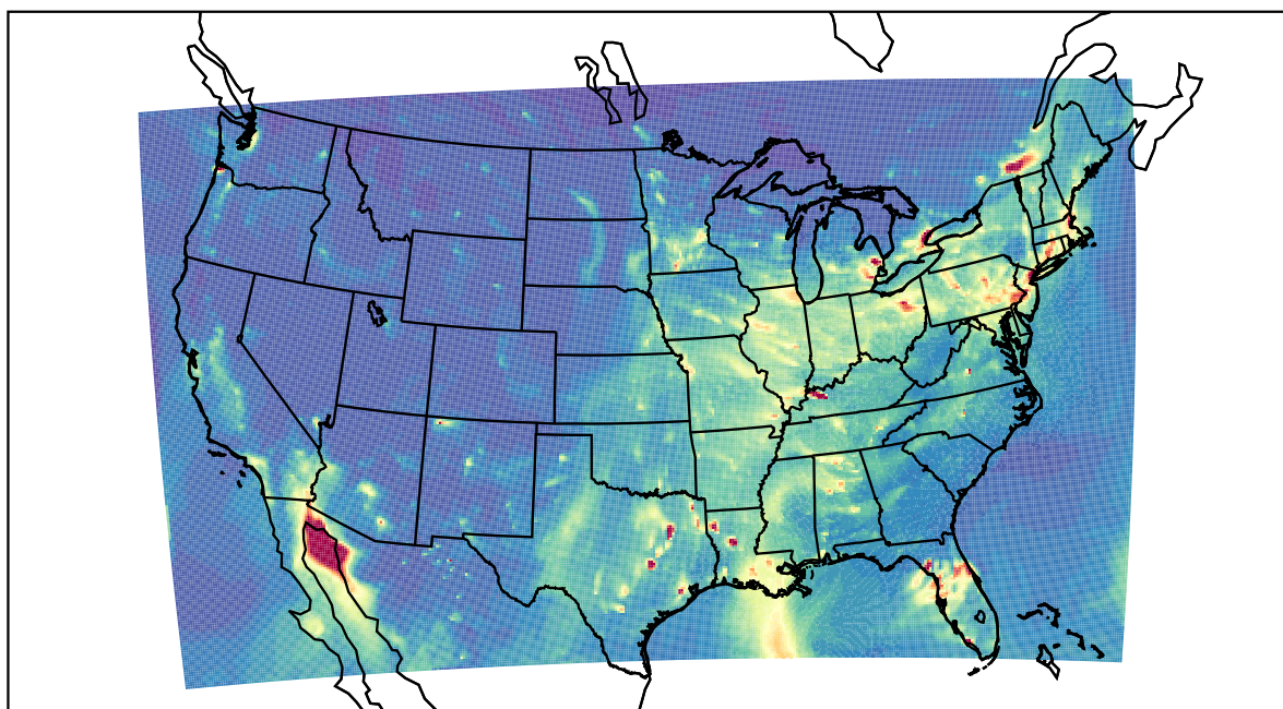
WRF 2022-12-22_02:00:00
