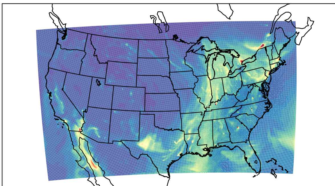
WRF 2022-12-22_18:00:00
