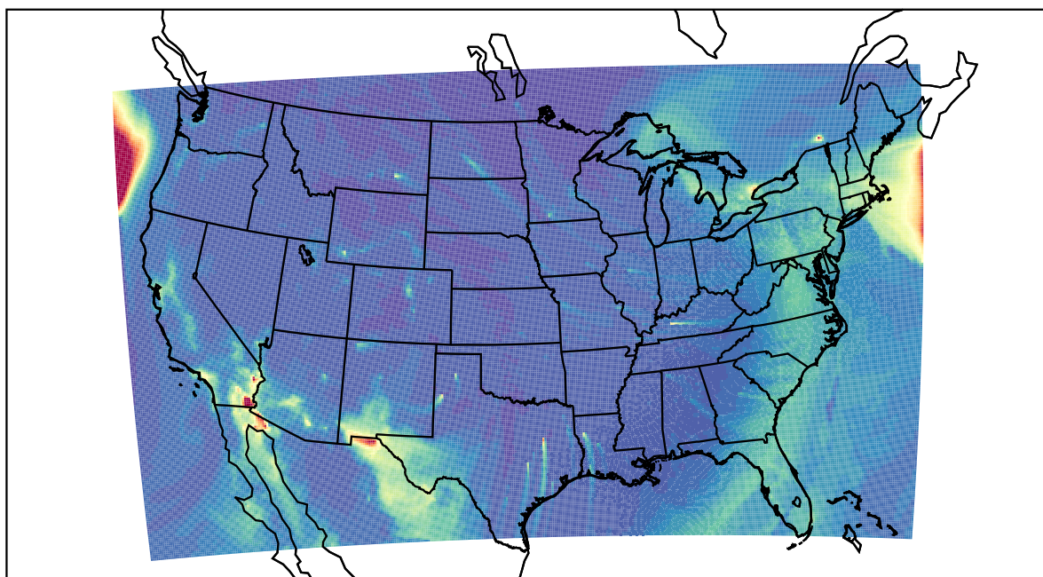
WRF 2022-12-23_12:00:00
