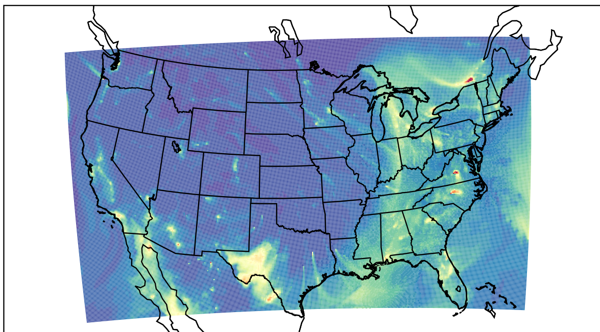
WRF 2022-12-23_02:00:00
