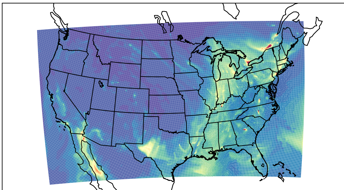
WRF 2022-12-22_20:00:00
