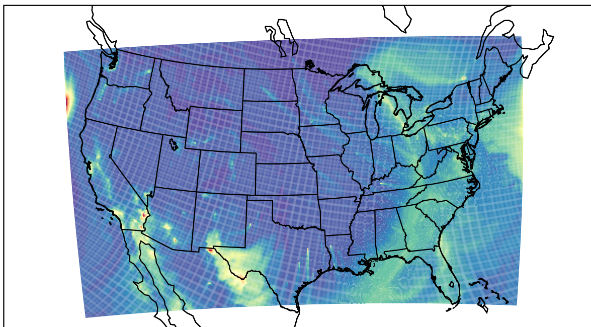
WRF 2022-12-23_07:00:00
