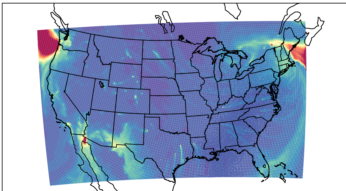
WRF 2022-12-23_21:00:00
