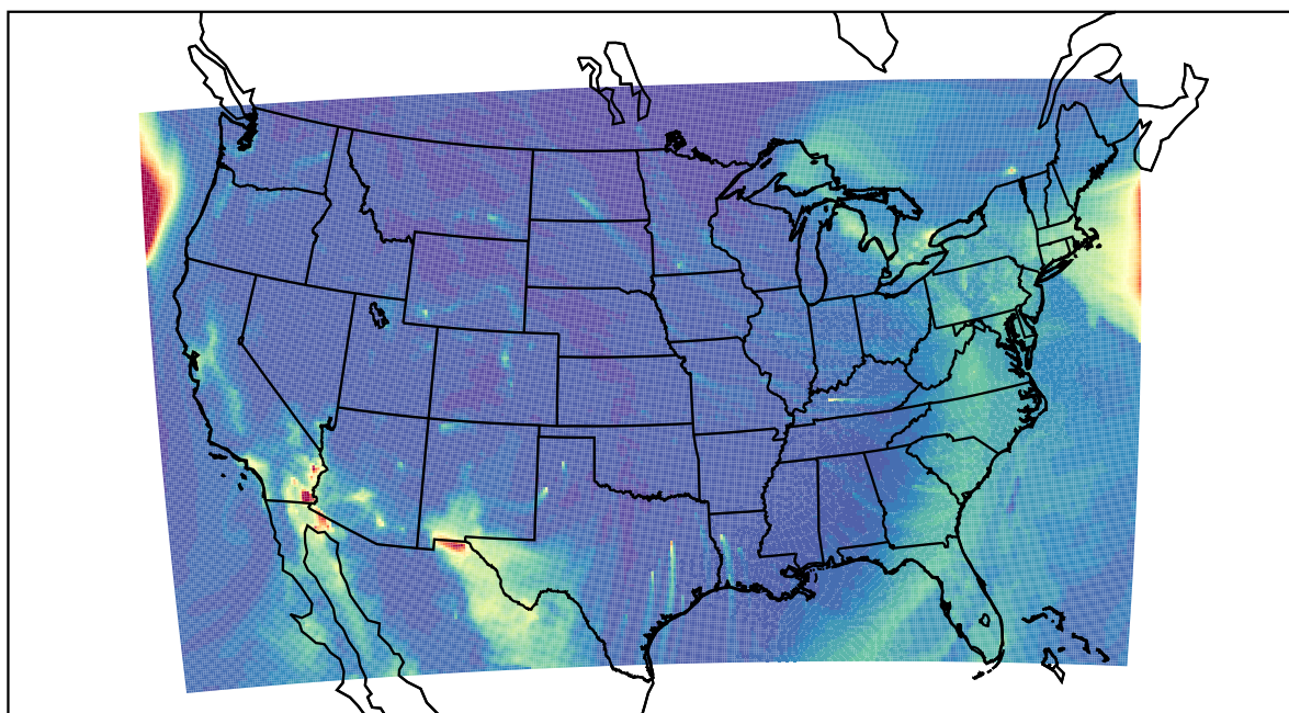
WRF 2022-12-23_11:00:00
