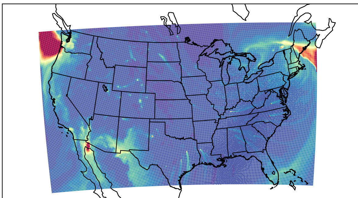
WRF 2022-12-23_22:00:00
