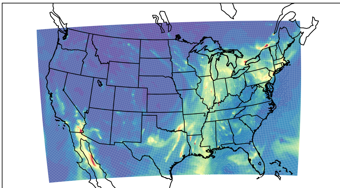
WRF 2022-12-22_14:00:00
