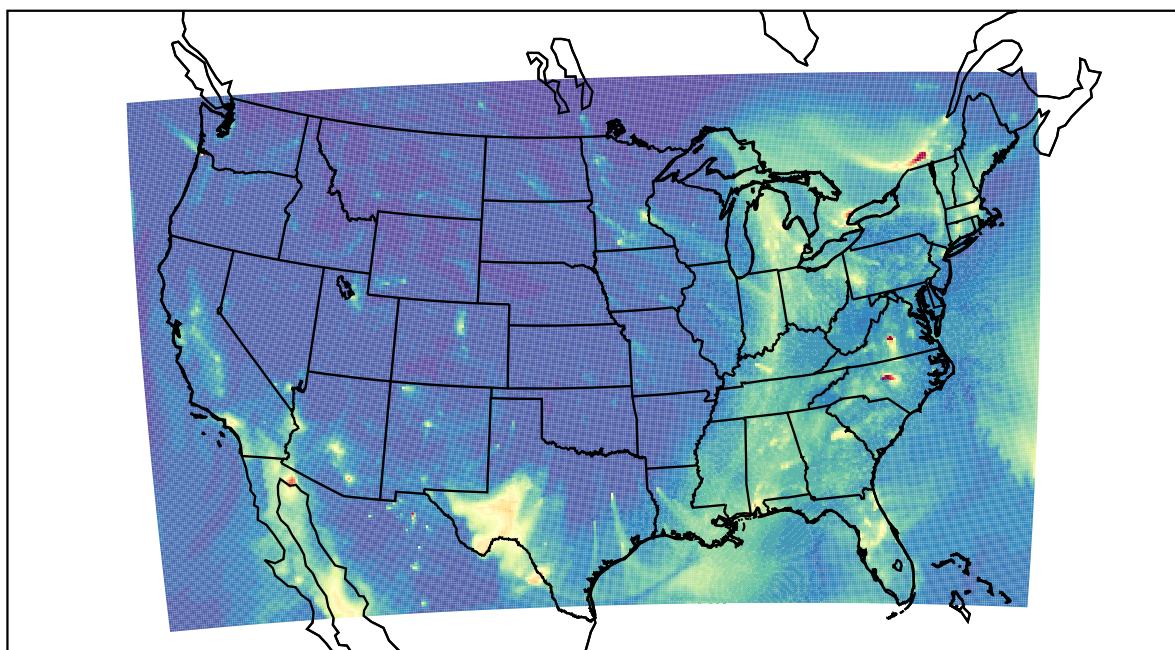
WRF 2022-12-23_01:00:00
