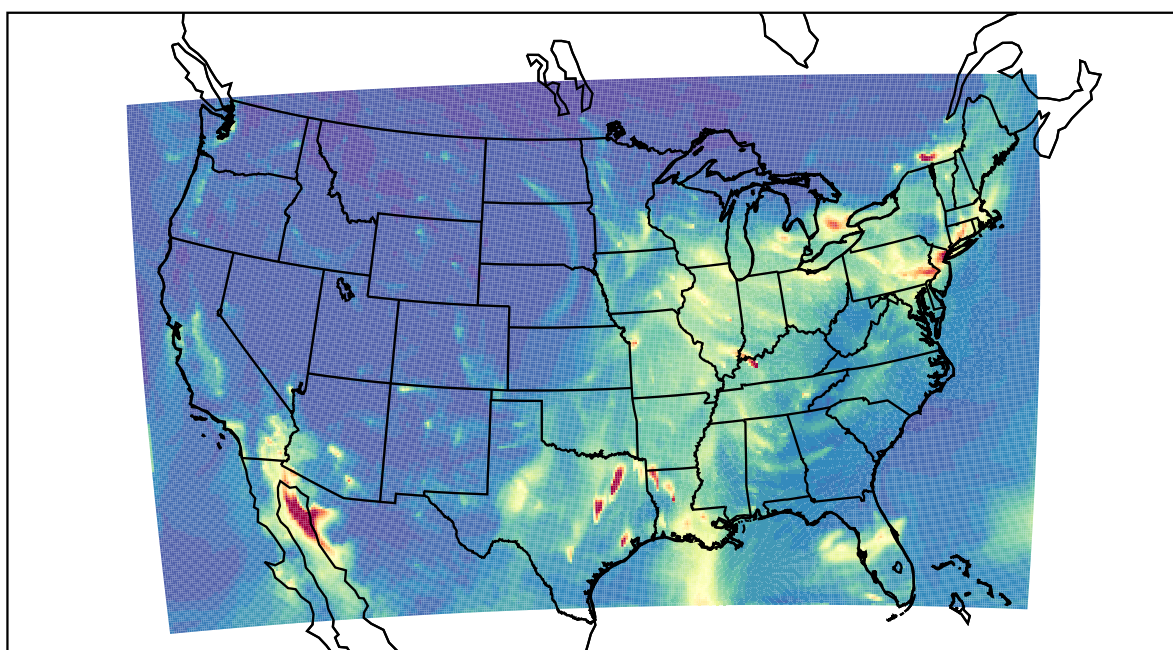
WRF 2022-12-22_06:00:00
