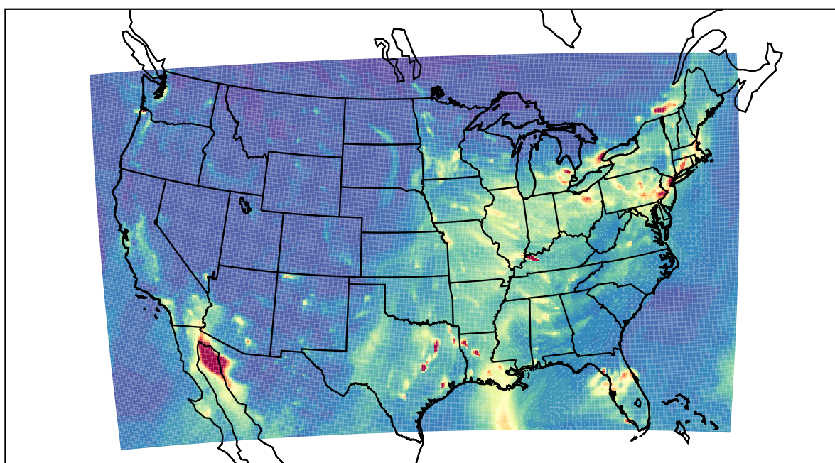
WRF 2022-12-22_03:00:00
