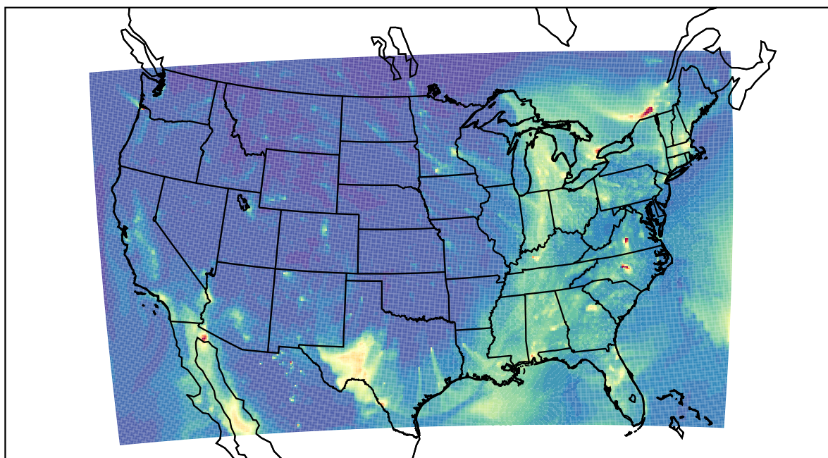
WRF 2022-12-23_00:00:00
