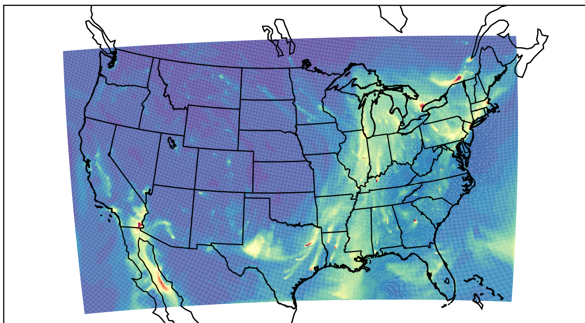
WRF 2022-12-22_17:00:00
