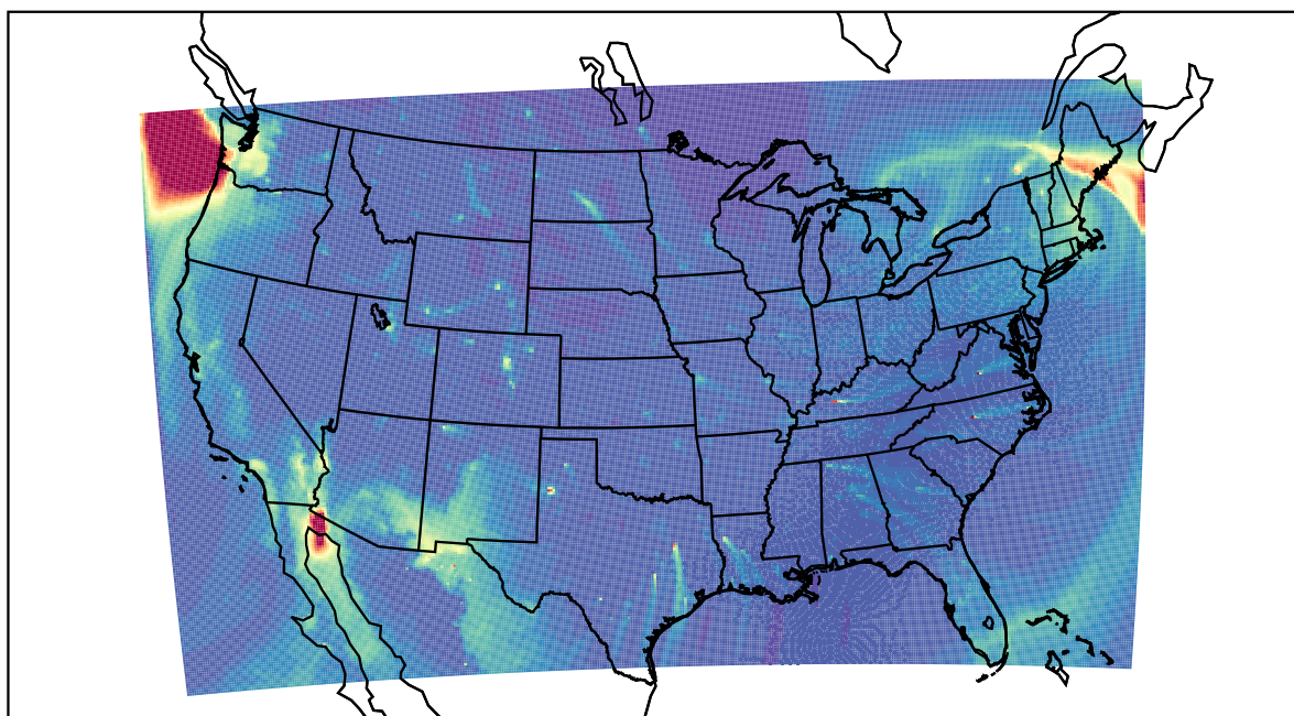
WRF 2022-12-23_23:00:00
