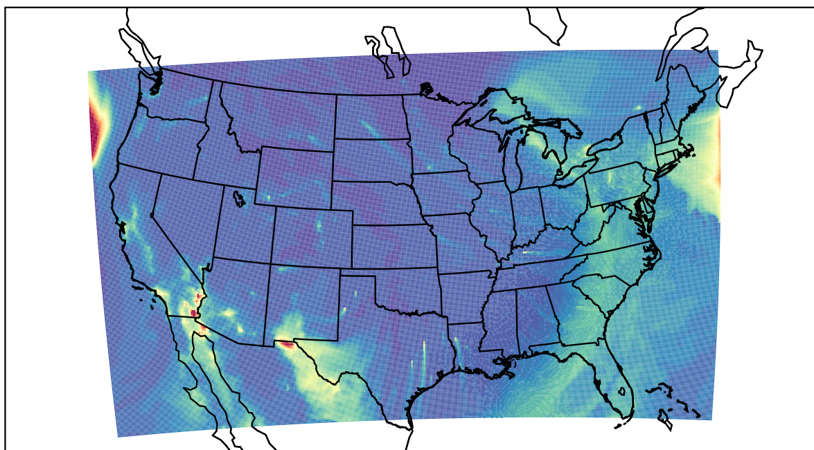
WRF 2022-12-23_10:00:00
