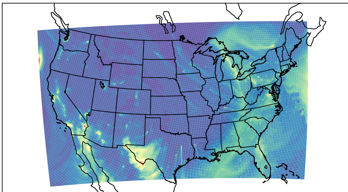
WRF 2022-12-23_06:00:00
