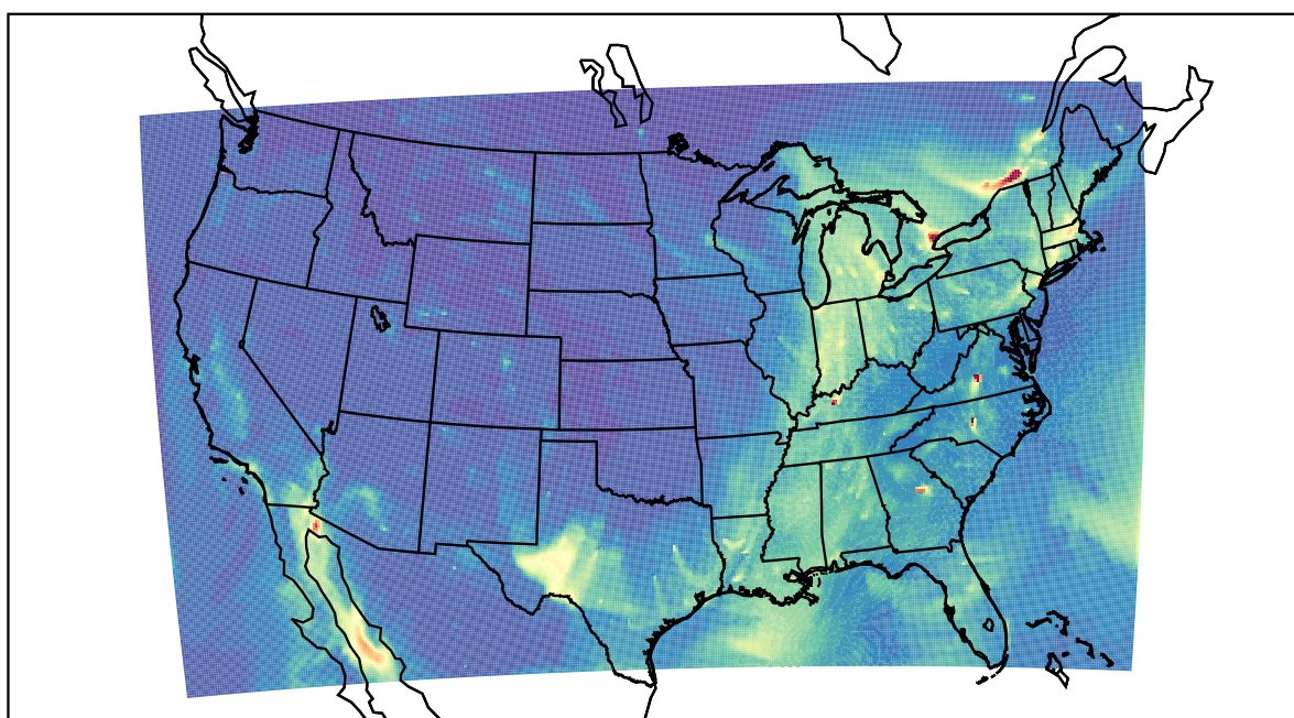
WRF 2022-12-22_21:00:00
