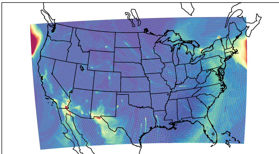
WRF 2022-12-23_13:00:00
