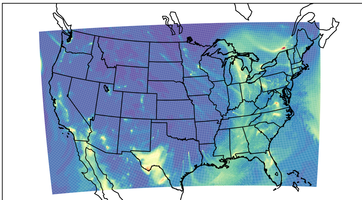
WRF 2022-12-23_03:00:00
