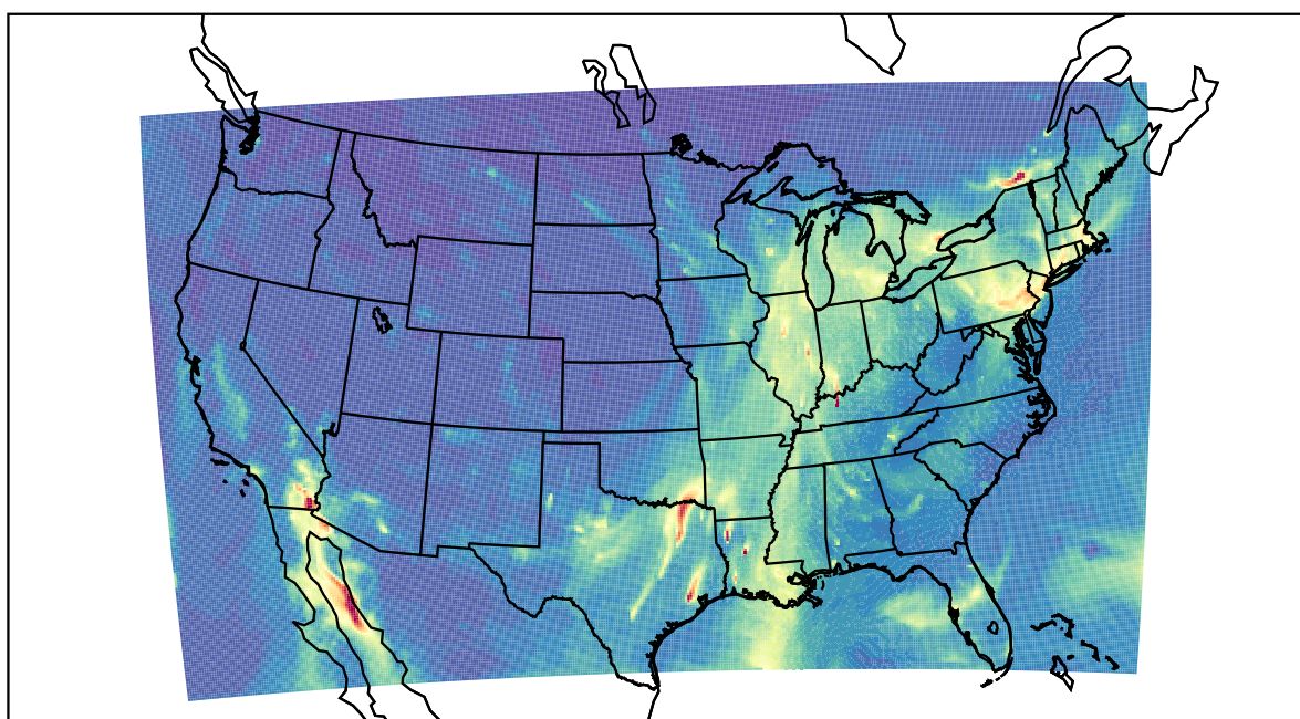
WRF 2022-12-22_12:00:00
