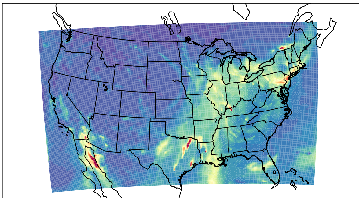
WRF 2022-12-22_09:00:00
