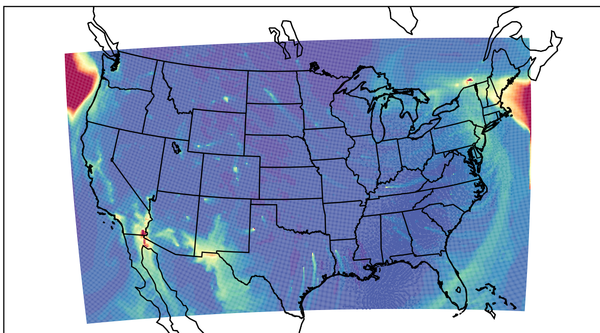
WRF 2022-12-23_17:00:00
