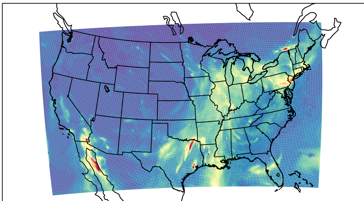
WRF 2022-12-22_10:00:00
