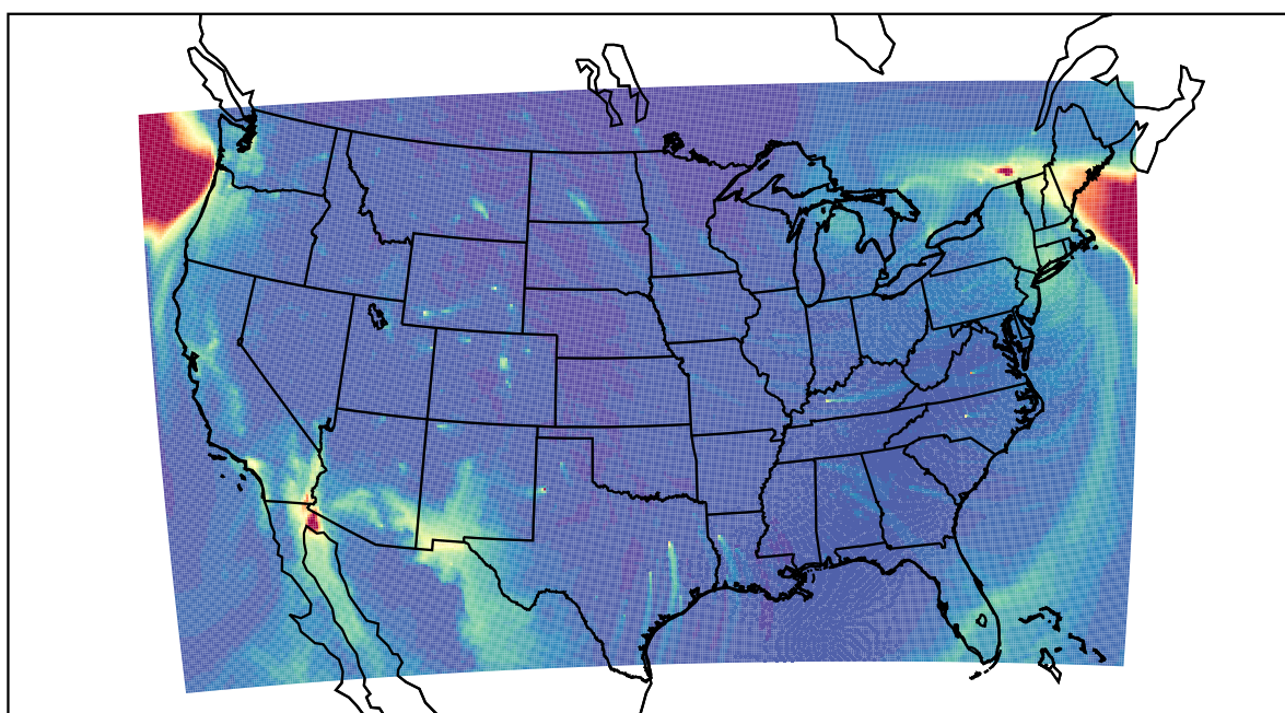
WRF 2022-12-23_19:00:00
