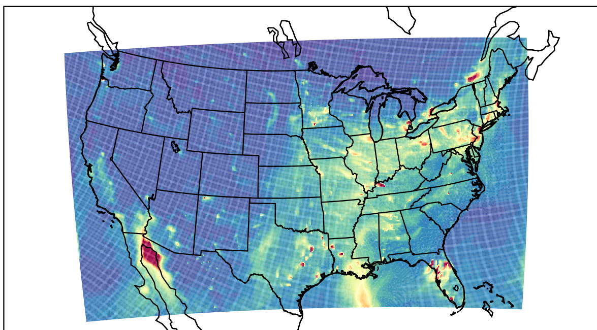
WRF 2022-12-22_01:00:00
