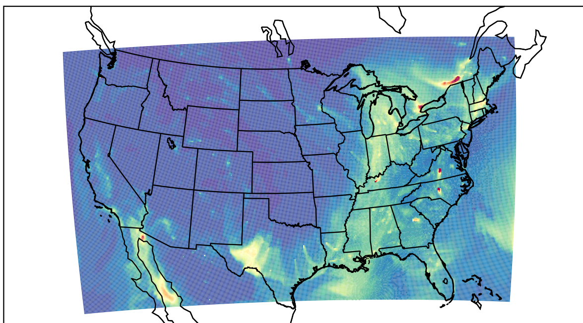
WRF 2022-12-22_22:00:00
