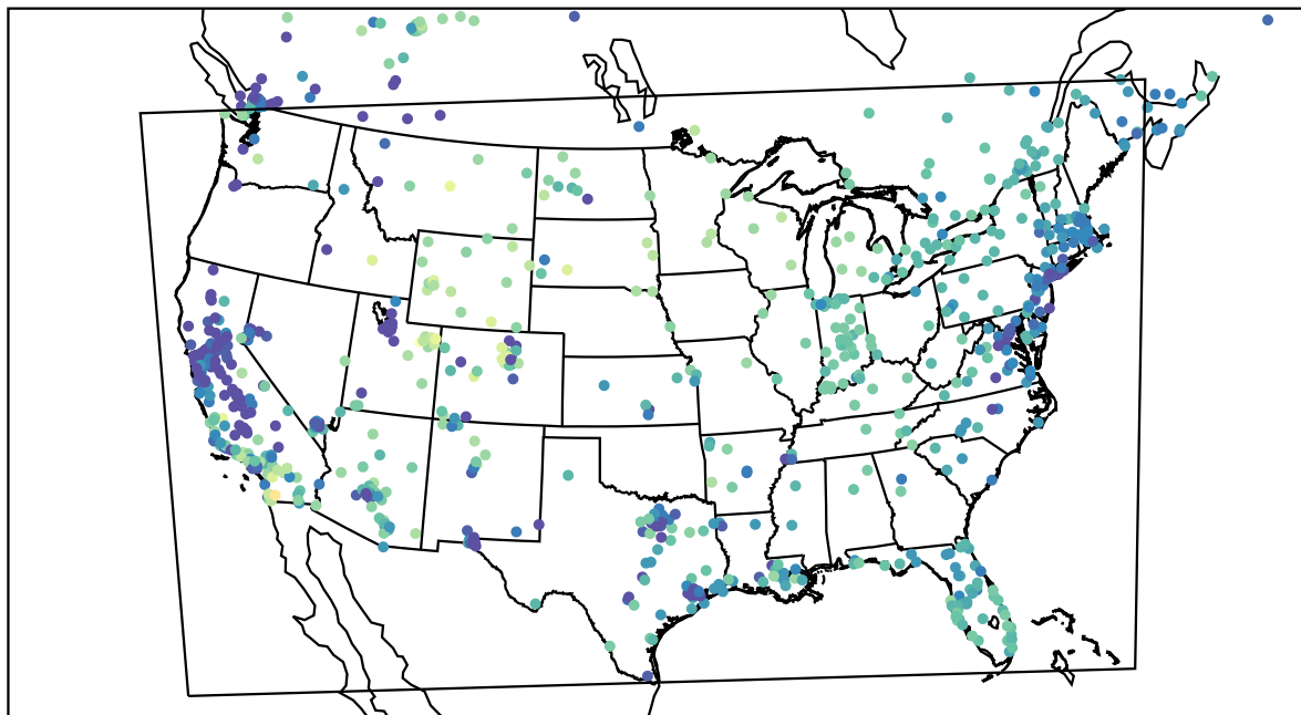
AirNOW (2022-12-25_00:00:00)
