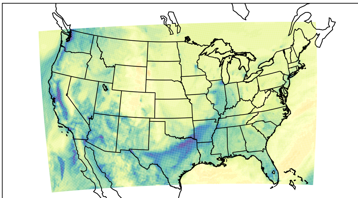
WRF (2022-12-26_17:00:00)
