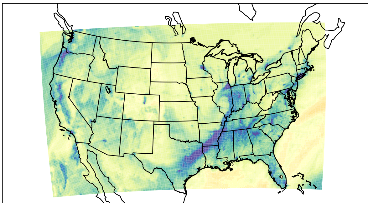
WRF (2022-12-26_23:00:00)
