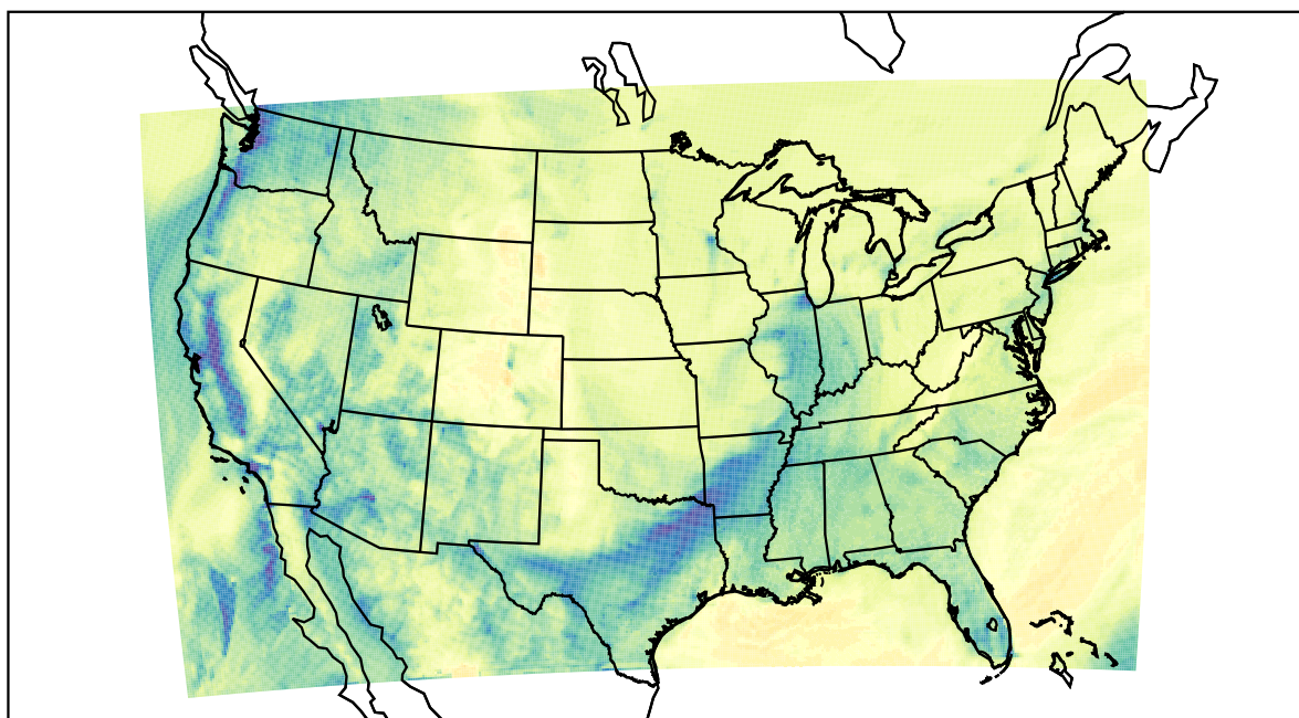
WRF (2022-12-26_18:00:00)
