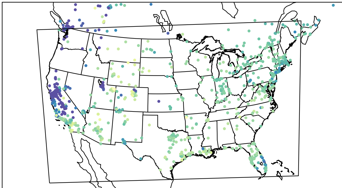
AirNOW (2022-12-25_19:00:00)
