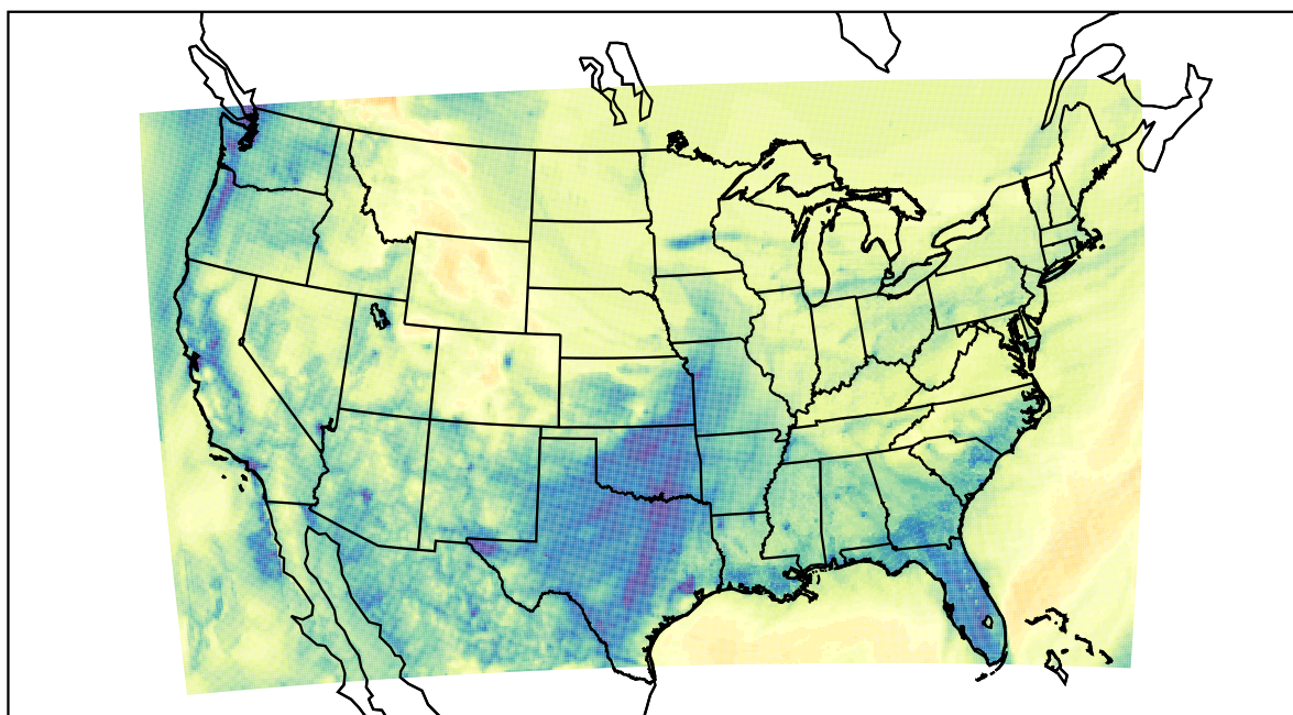
WRF (2022-12-26_06:00:00)
