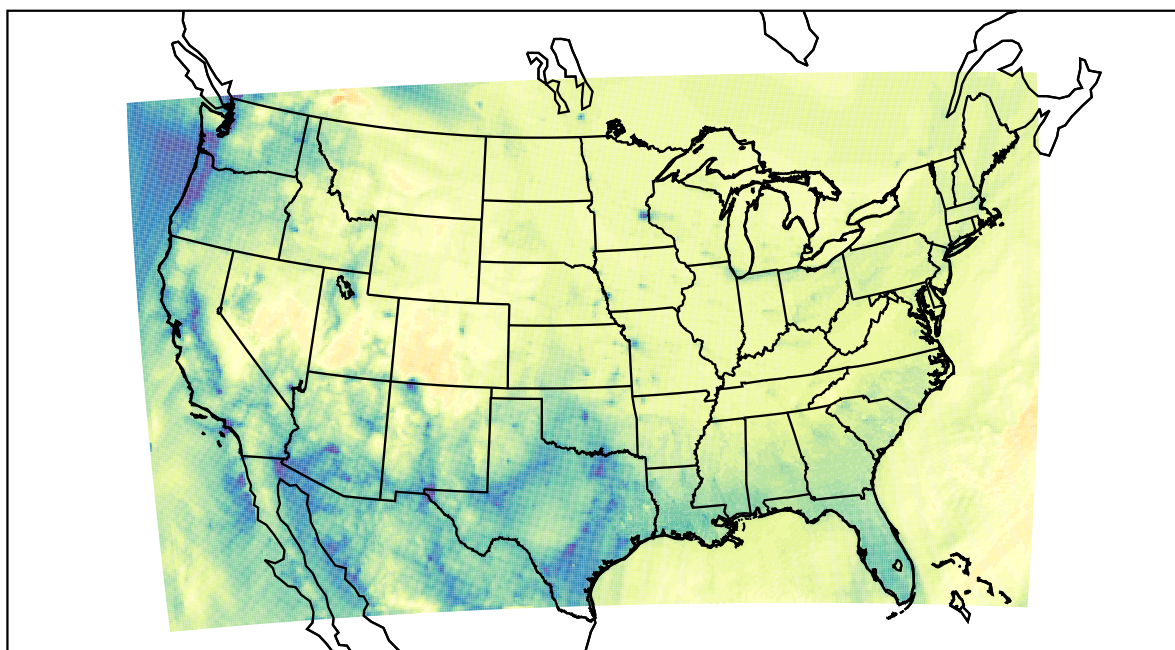
WRF (2022-12-25_15:00:00)
