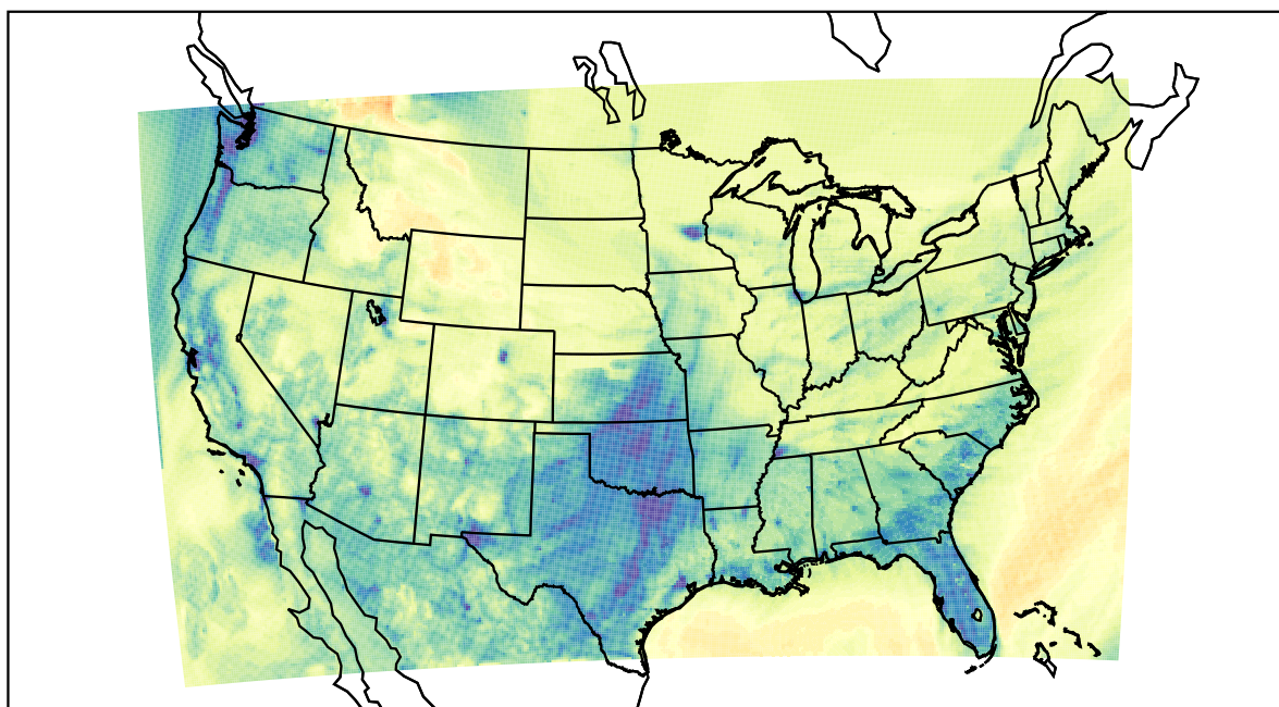
WRF (2022-12-26_03:00:00)
