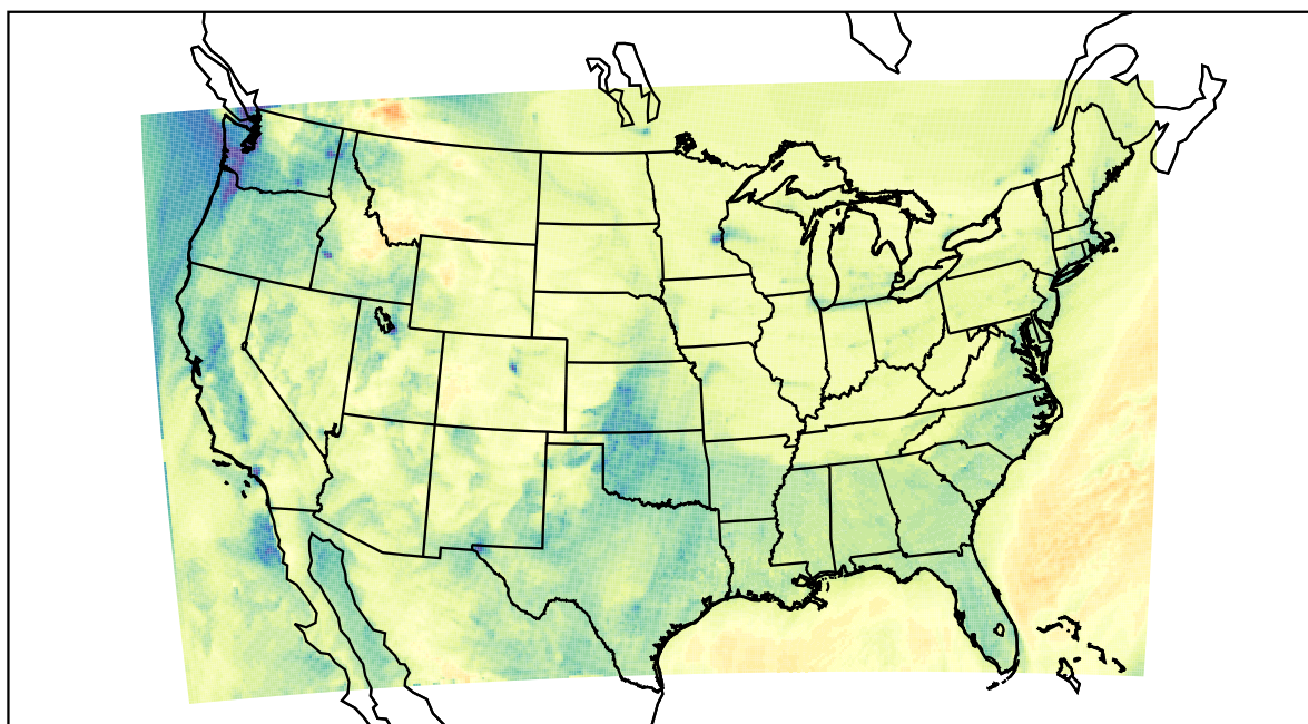
WRF (2022-12-25_21:00:00)
