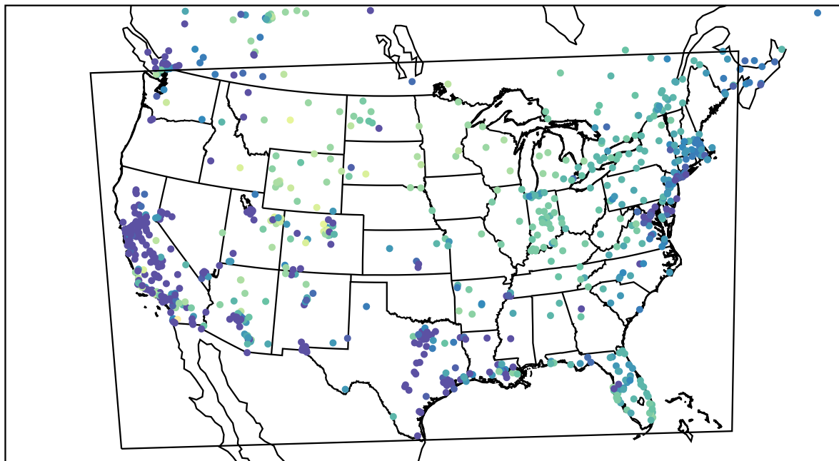
AirNOW (2022-12-25_02:00:00)
