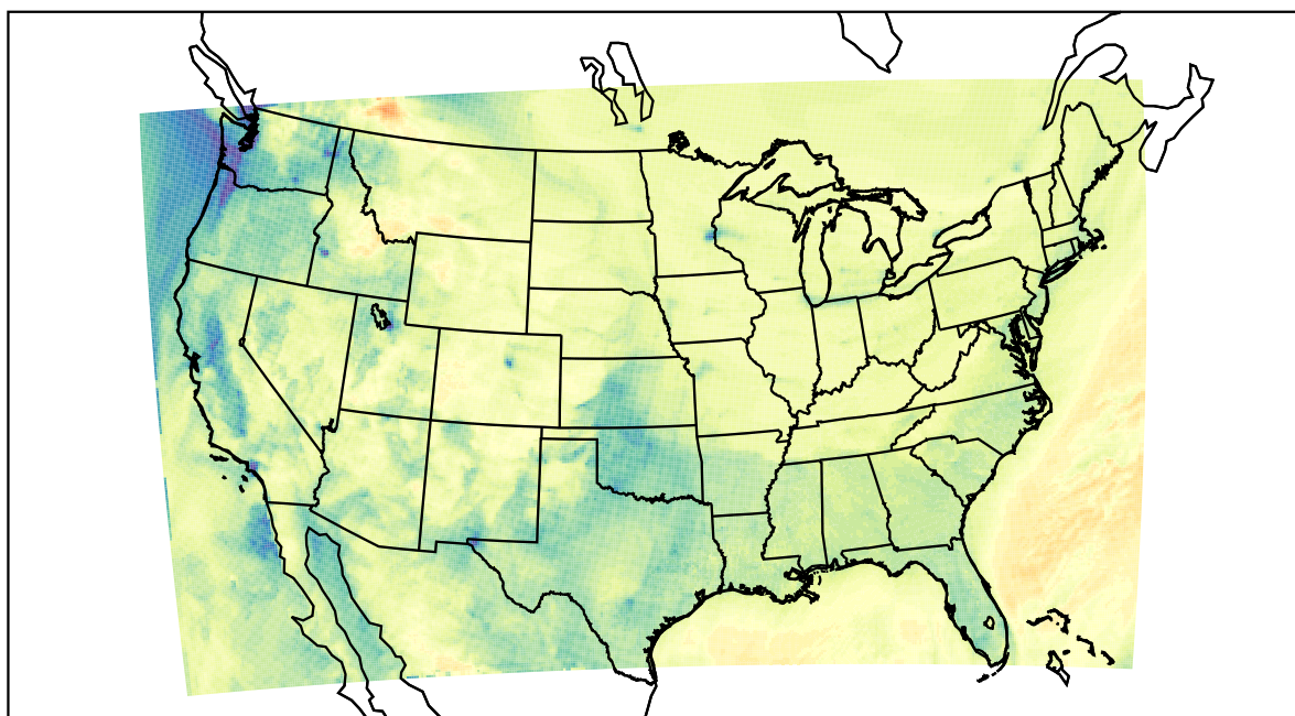
WRF (2022-12-25_20:00:00)
