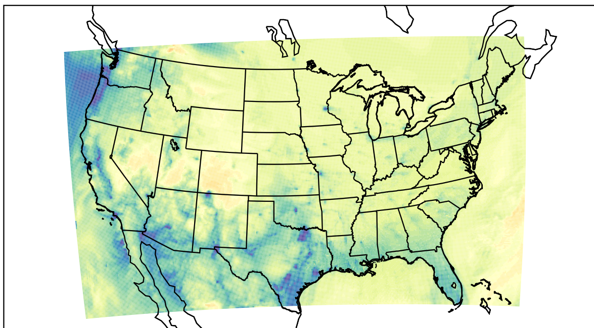
WRF (2022-12-25_14:00:00)
