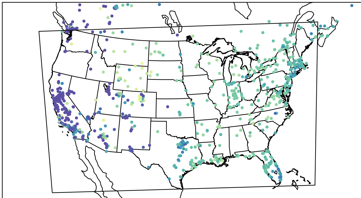
AirNOW (2022-12-25_16:00:00)
