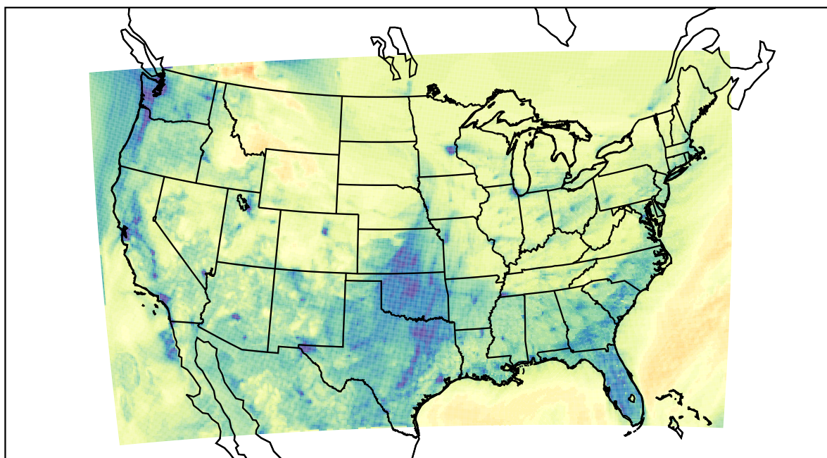
WRF (2022-12-26_01:00:00)
