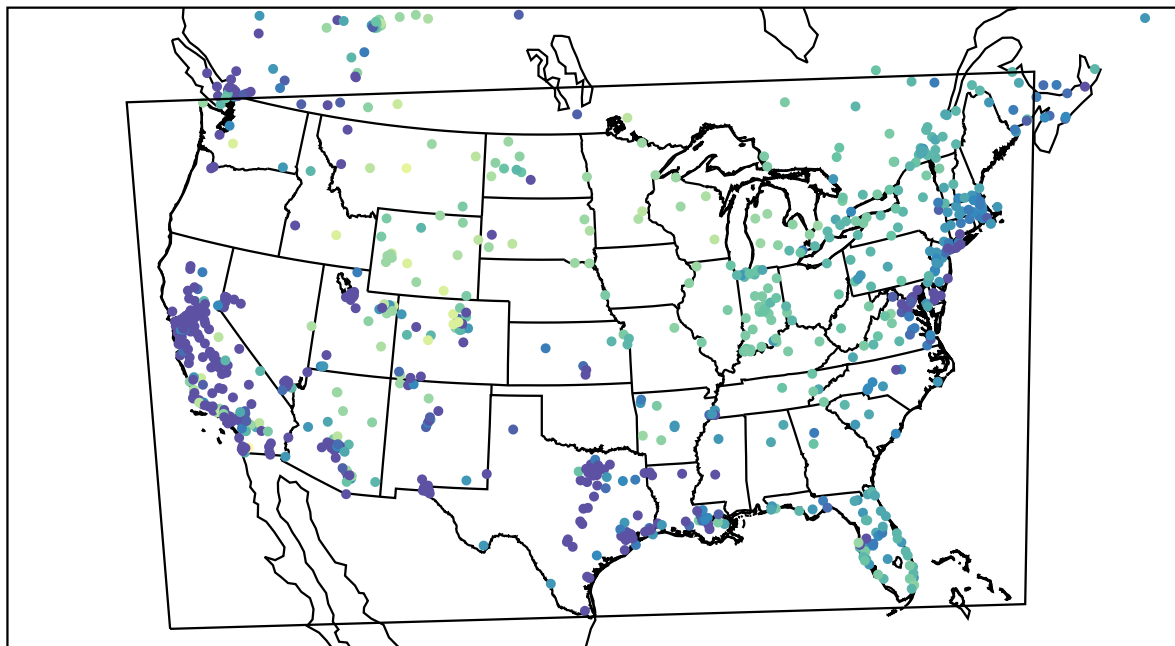
AirNOW (2022-12-25_03:00:00)
