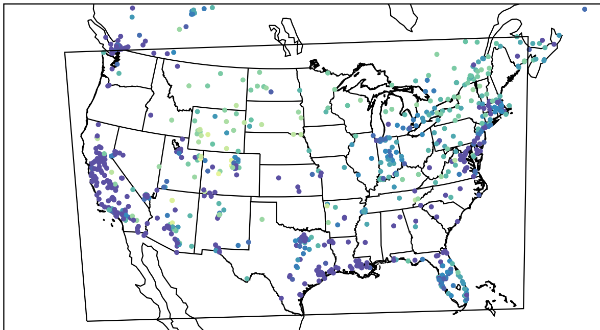
AirNOW (2022-12-26_10:00:00)
