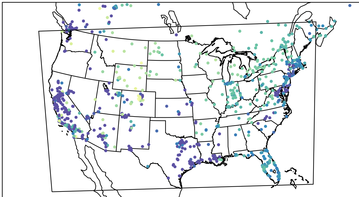
AirNOW (2022-12-25_13:00:00)
