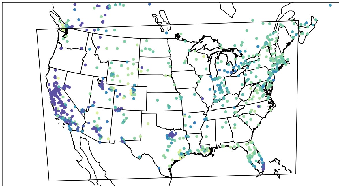
AirNOW (2022-12-26_17:00:00)
