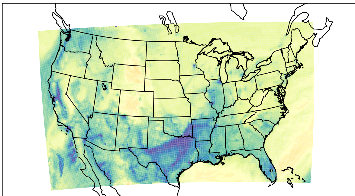
WRF (2022-12-26_15:00:00)
