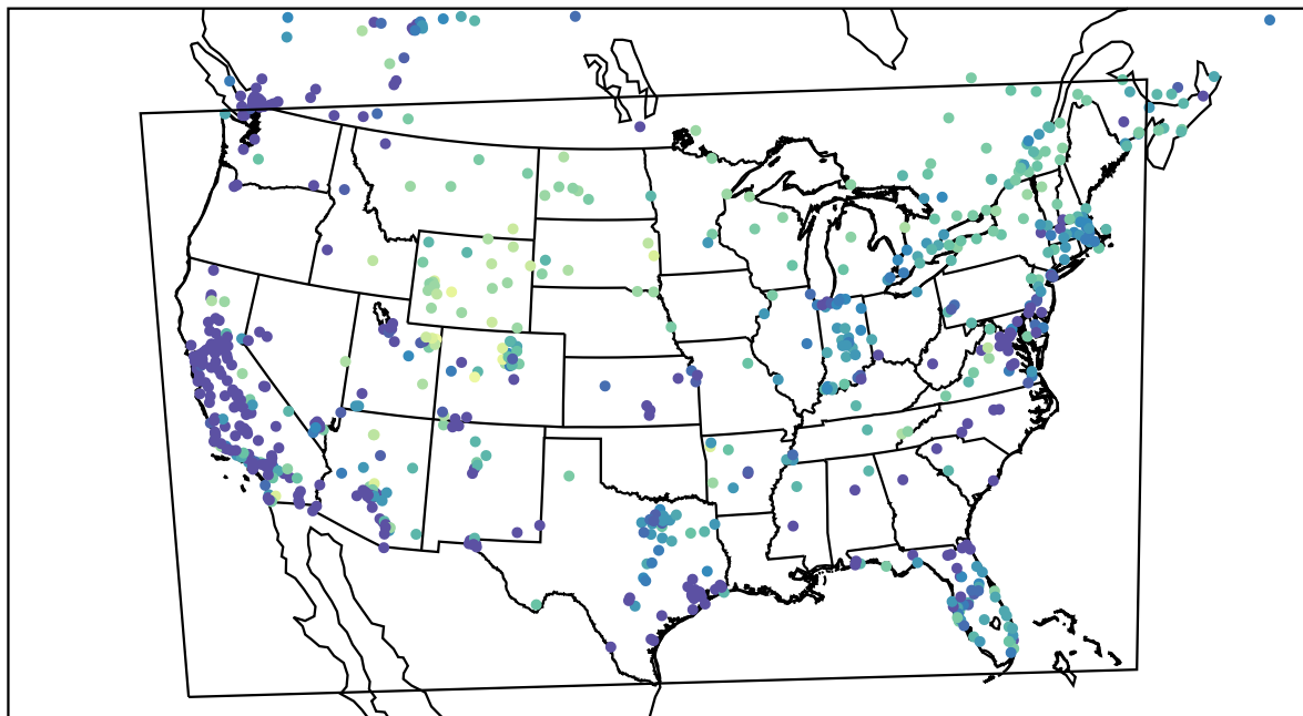
AirNOW (2022-12-26_07:00:00)
