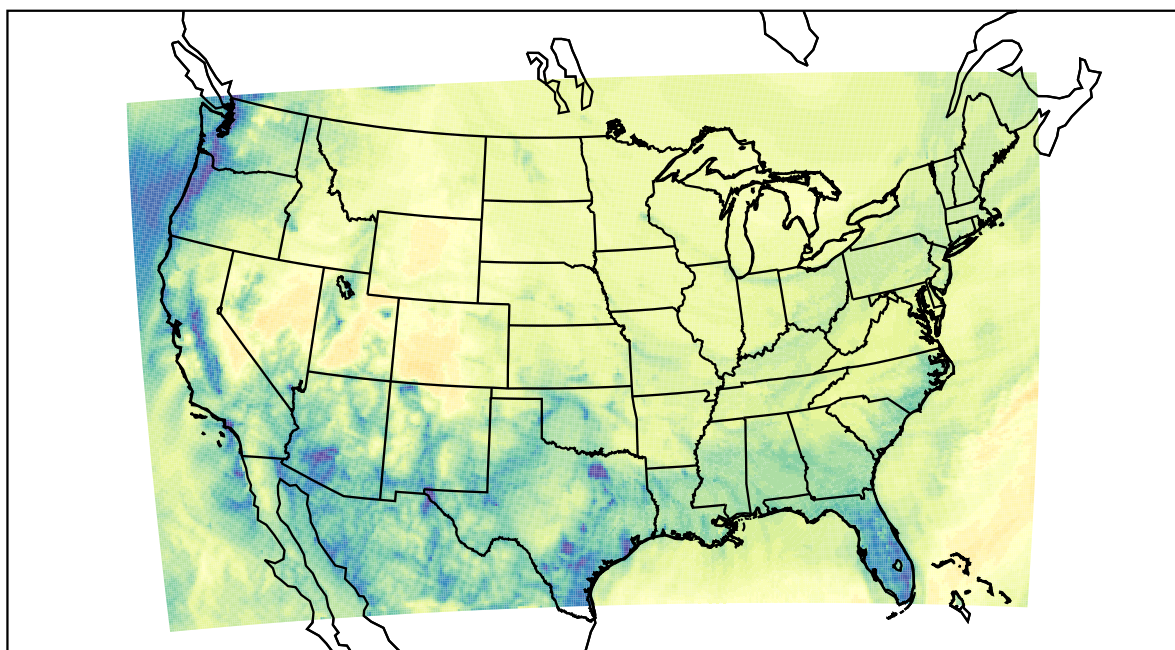
WRF (2022-12-25_08:00:00)
