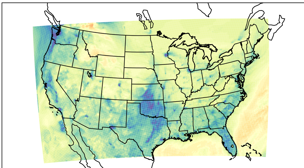
WRF (2022-12-26_00:00:00)
