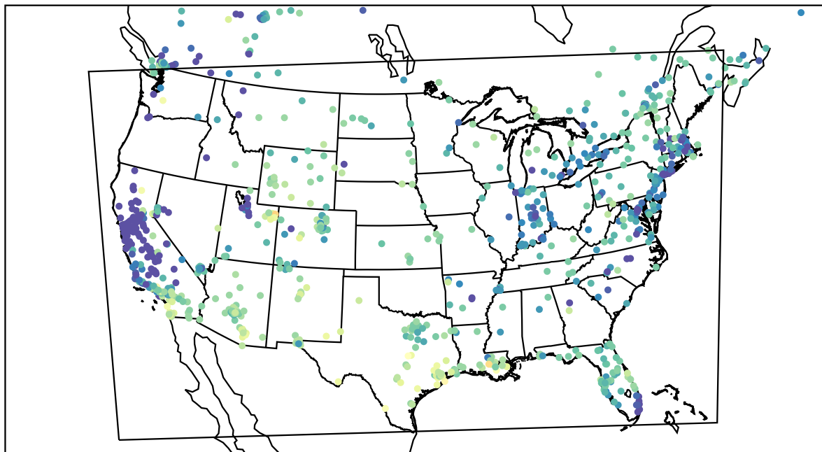
AirNOW (2022-12-26_22:00:00)
