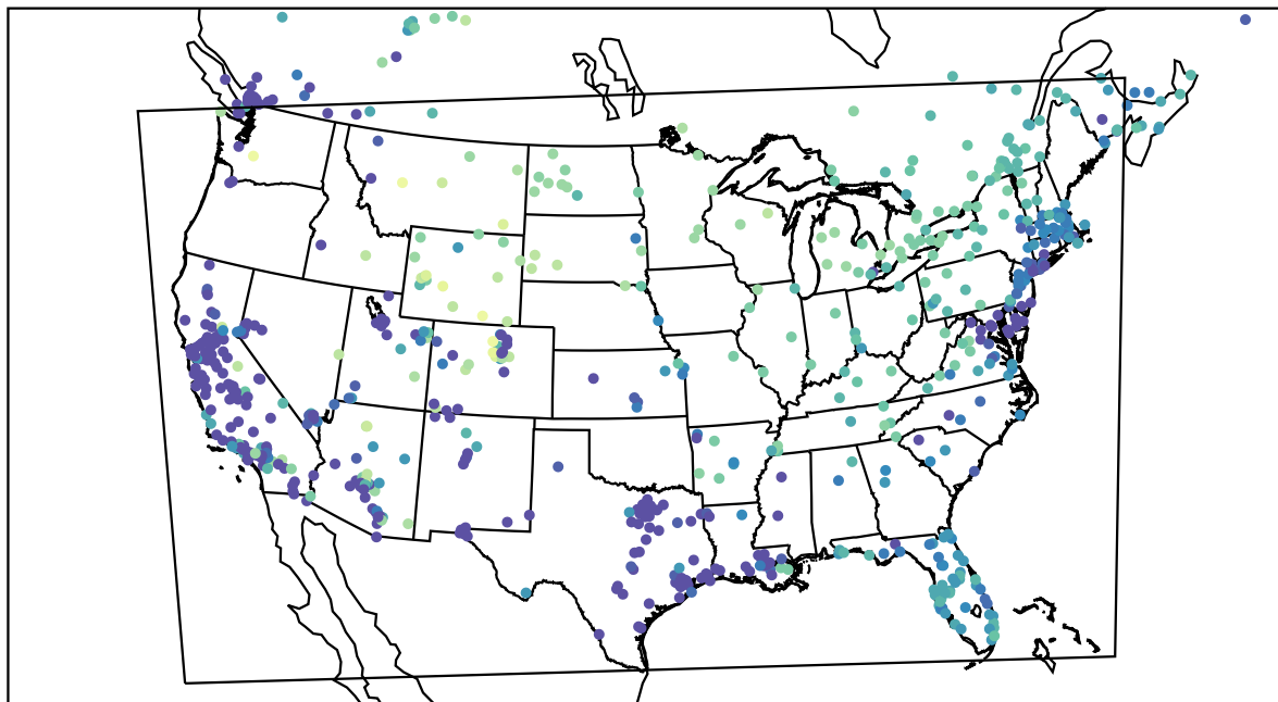
AirNOW (2022-12-25_10:00:00)
