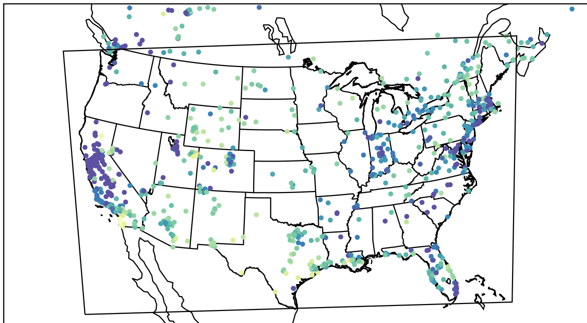
AirNOW (2022-12-26_23:00:00)
