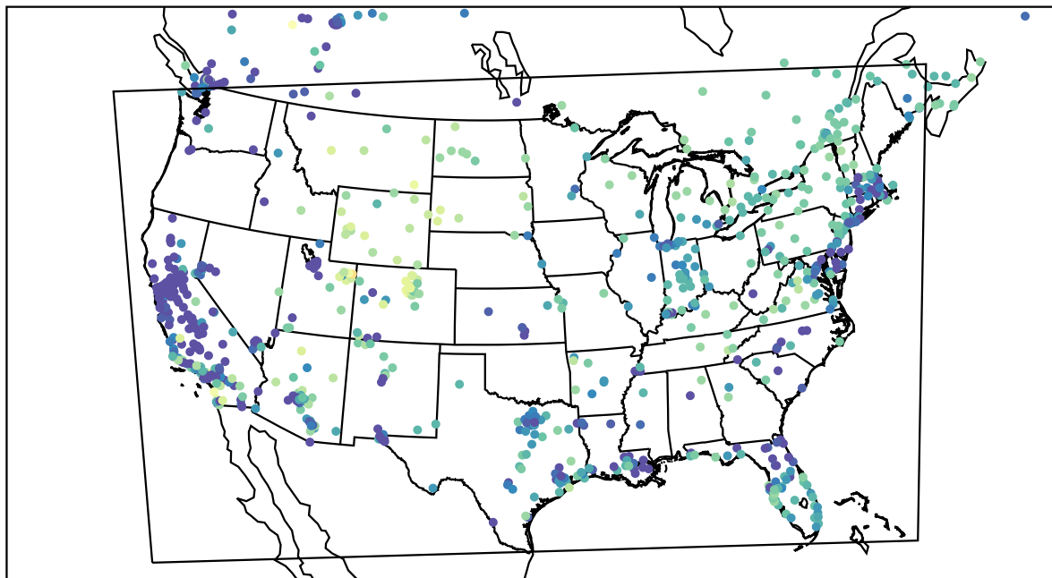
AirNOW (2022-12-26_01:00:00)
