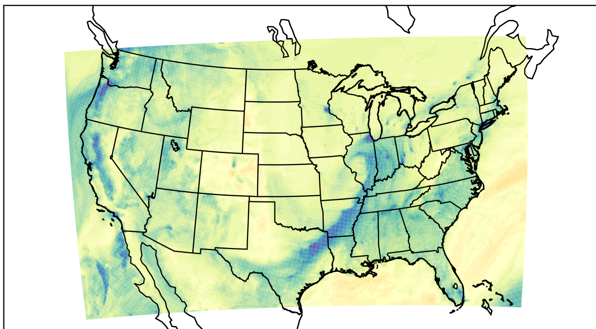
WRF (2022-12-26_21:00:00)
