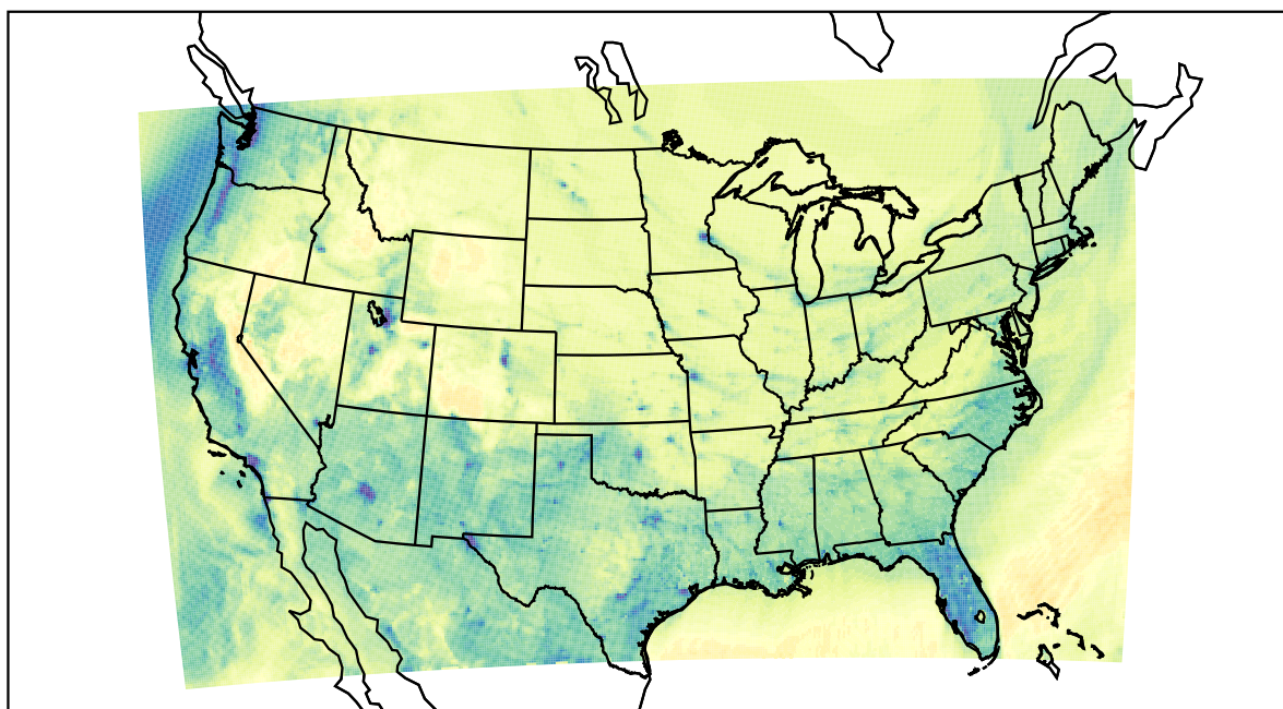
WRF (2022-12-25_00:00:00)
