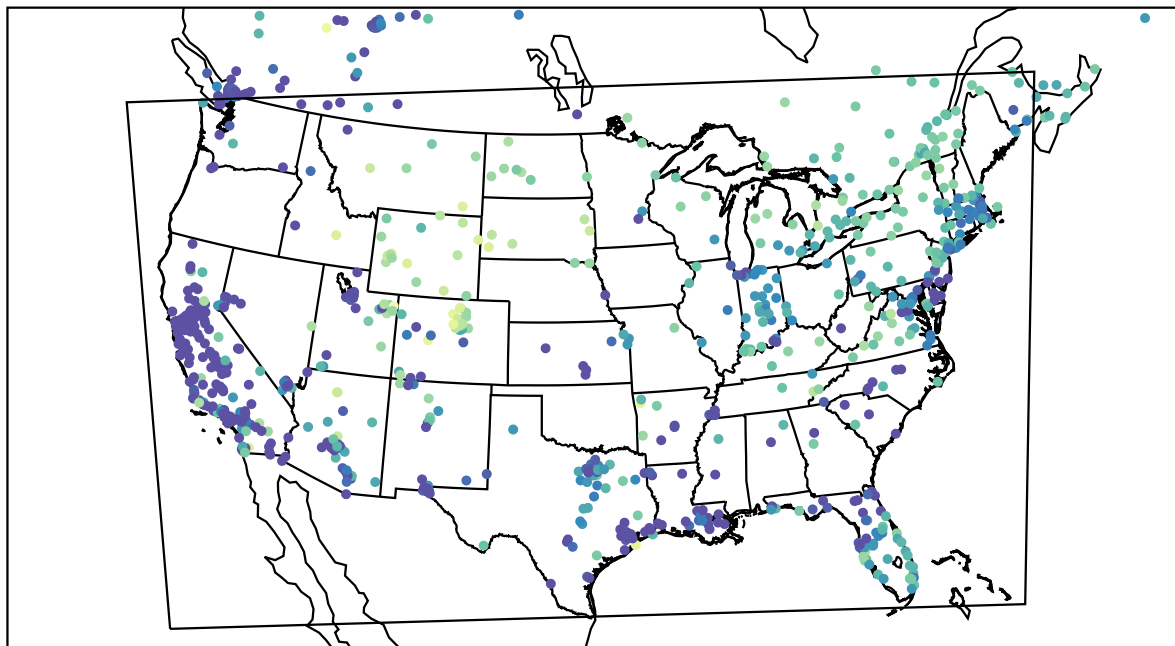
AirNOW (2022-12-26_04:00:00)
