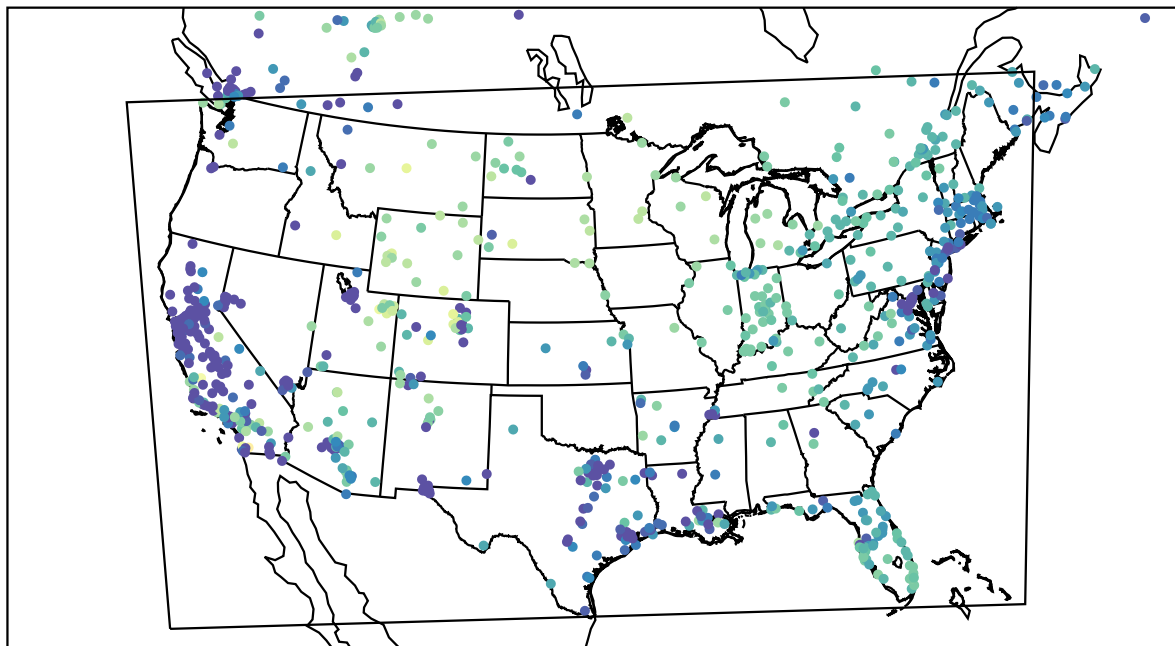
AirNOW (2022-12-25_01:00:00)
