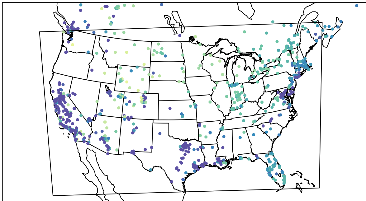
AirNOW (2022-12-25_07:00:00)
