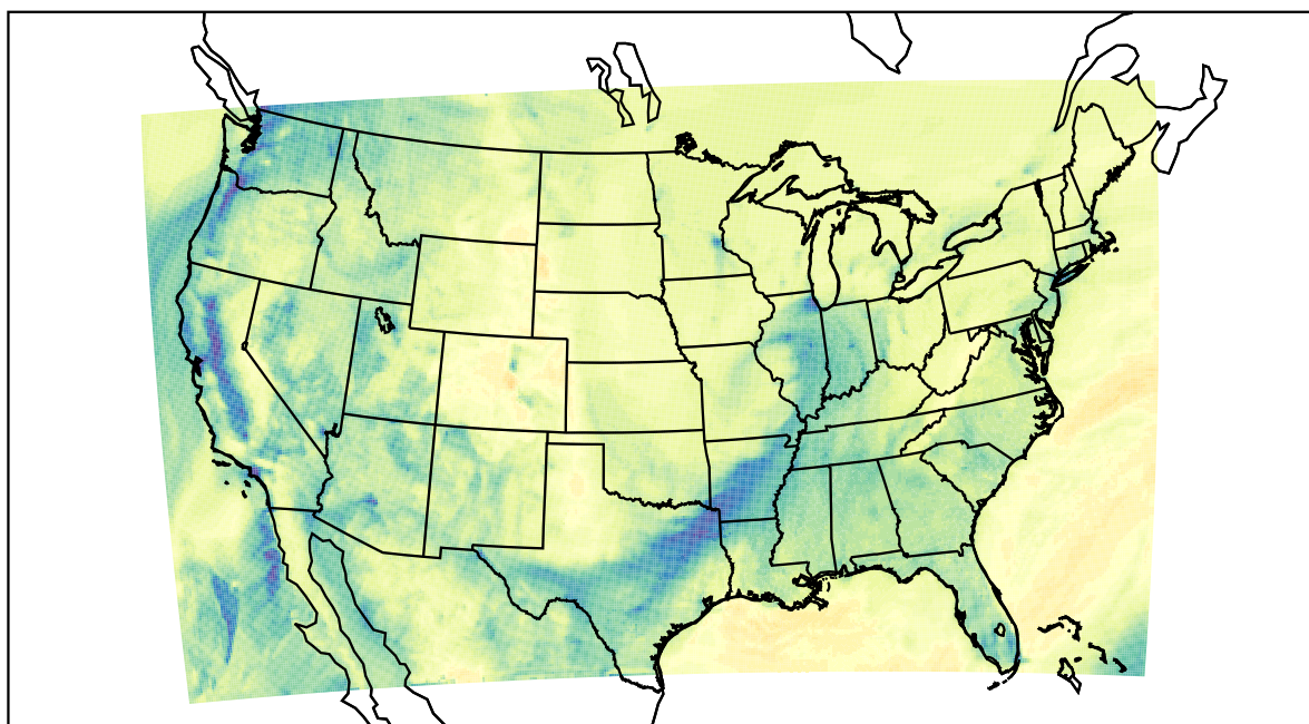
WRF (2022-12-26_19:00:00)
