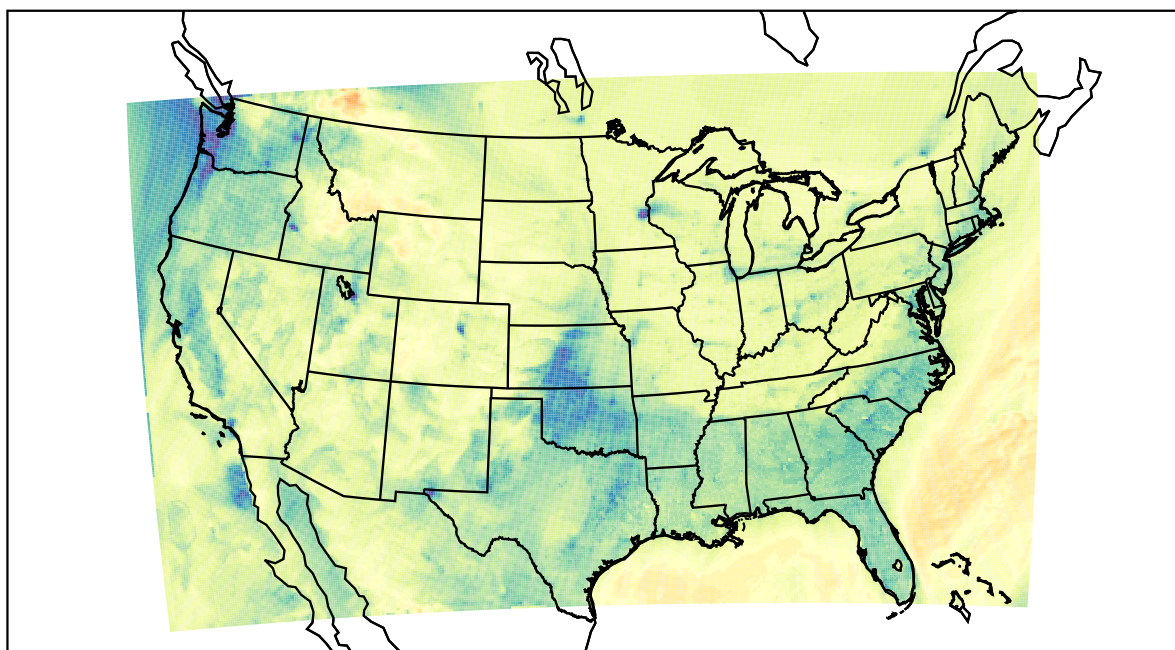
WRF (2022-12-25_22:00:00)
