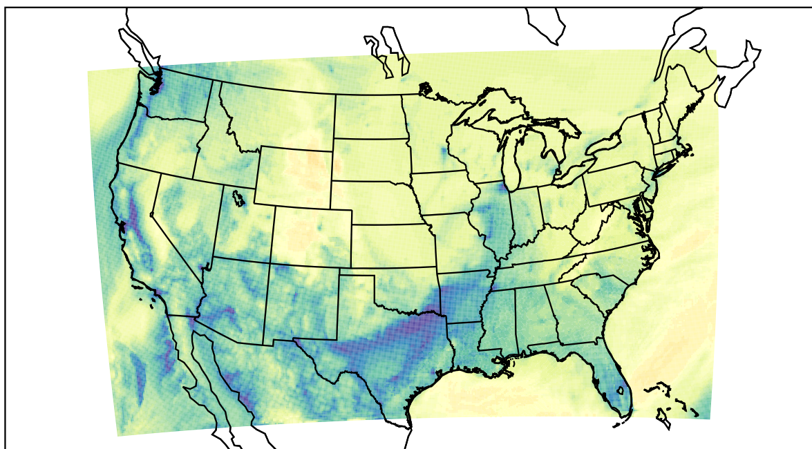
WRF (2022-12-26_16:00:00)
