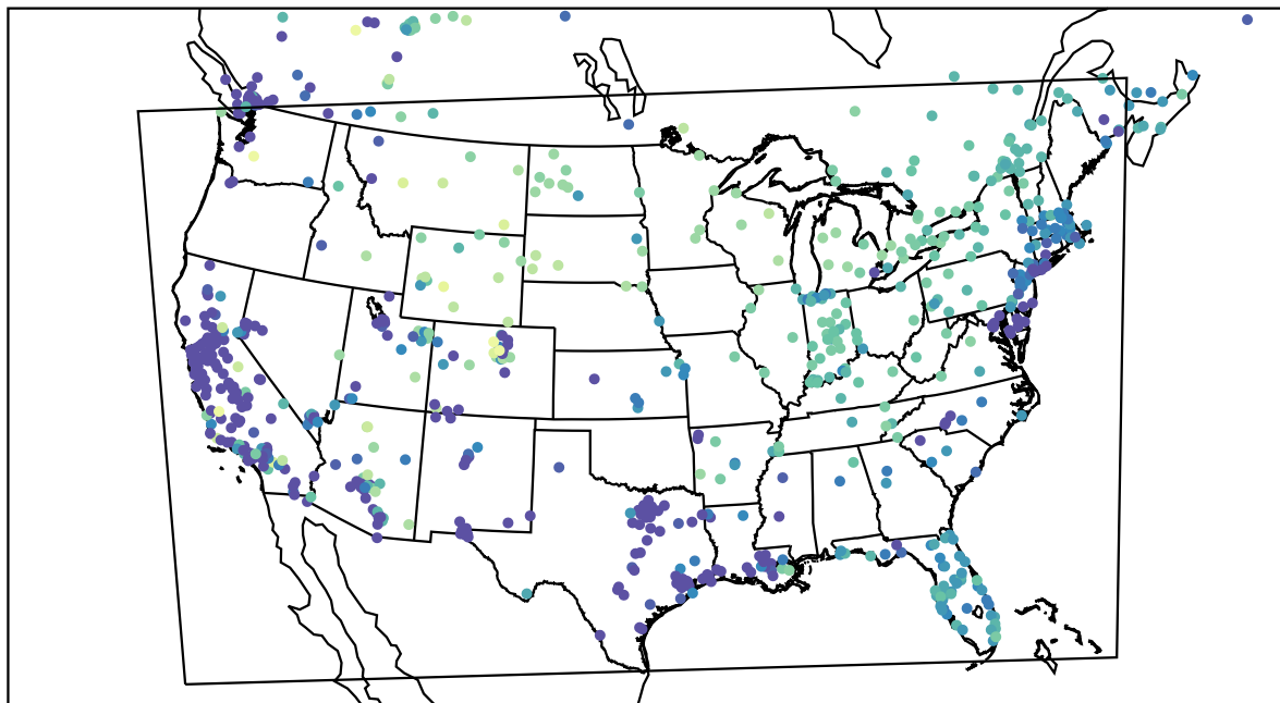
AirNOW (2022-12-25_09:00:00)
