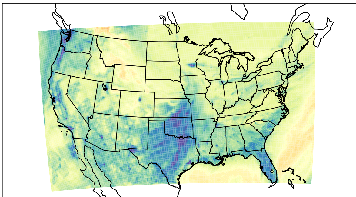
WRF (2022-12-26_04:00:00)
