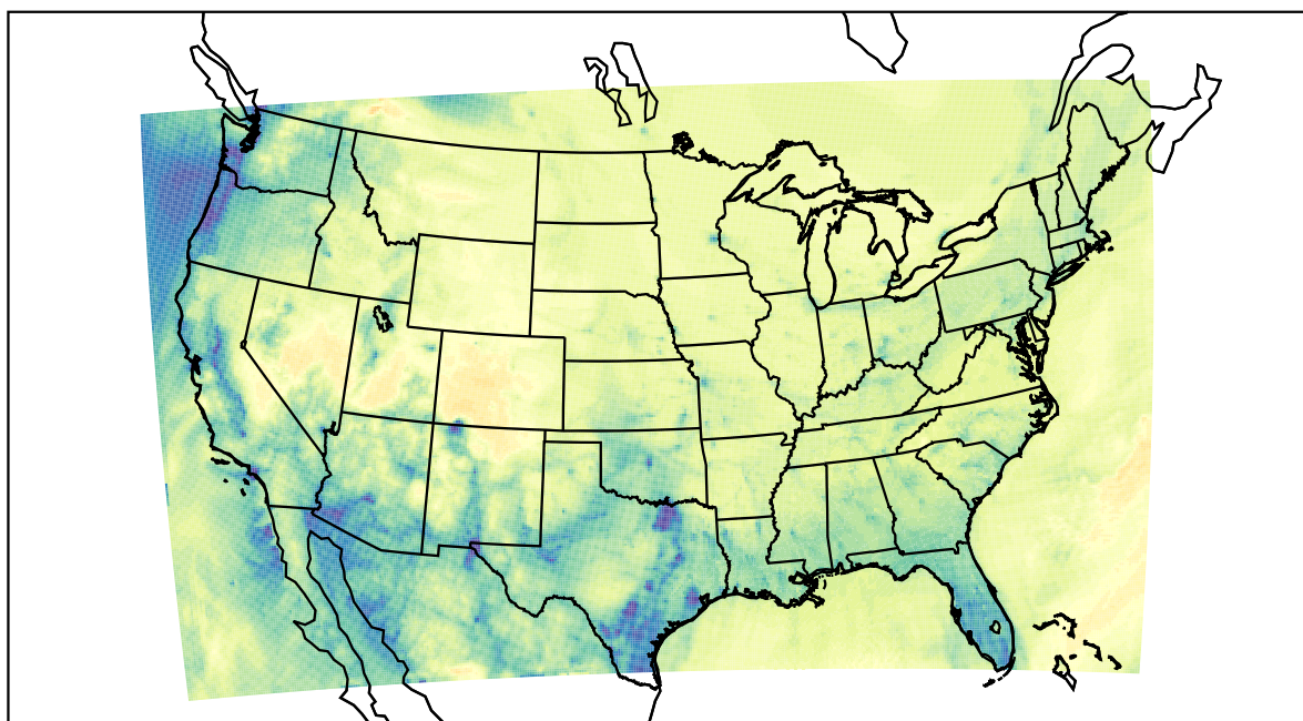
WRF (2022-12-25_13:00:00)
