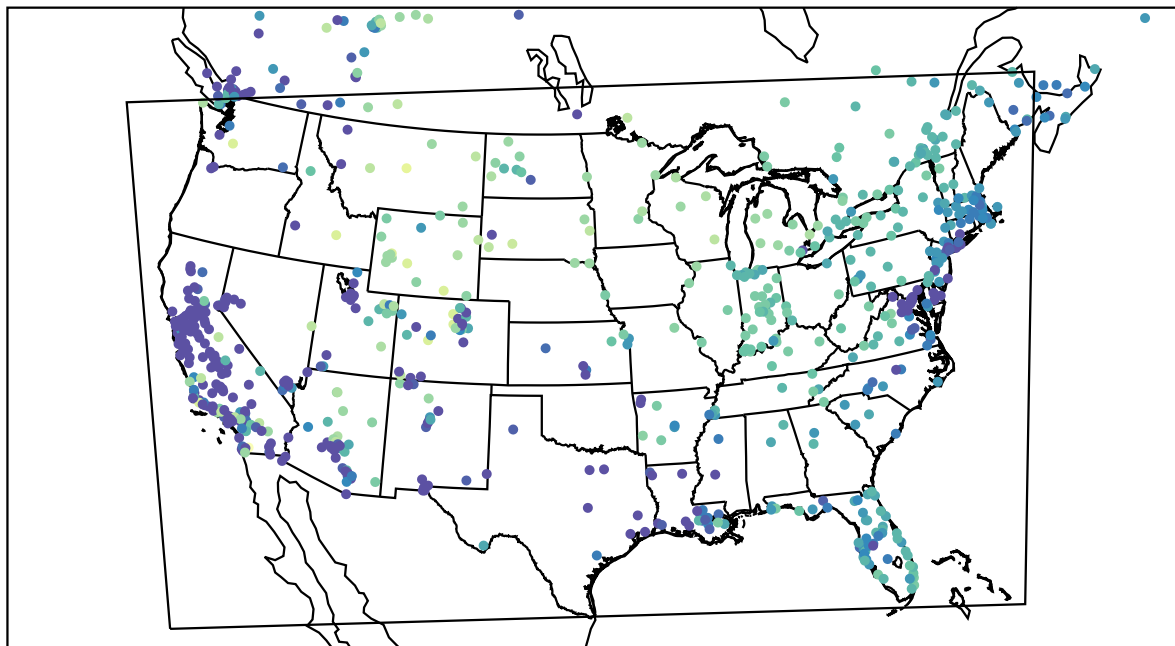
AirNOW (2022-12-25_04:00:00)
