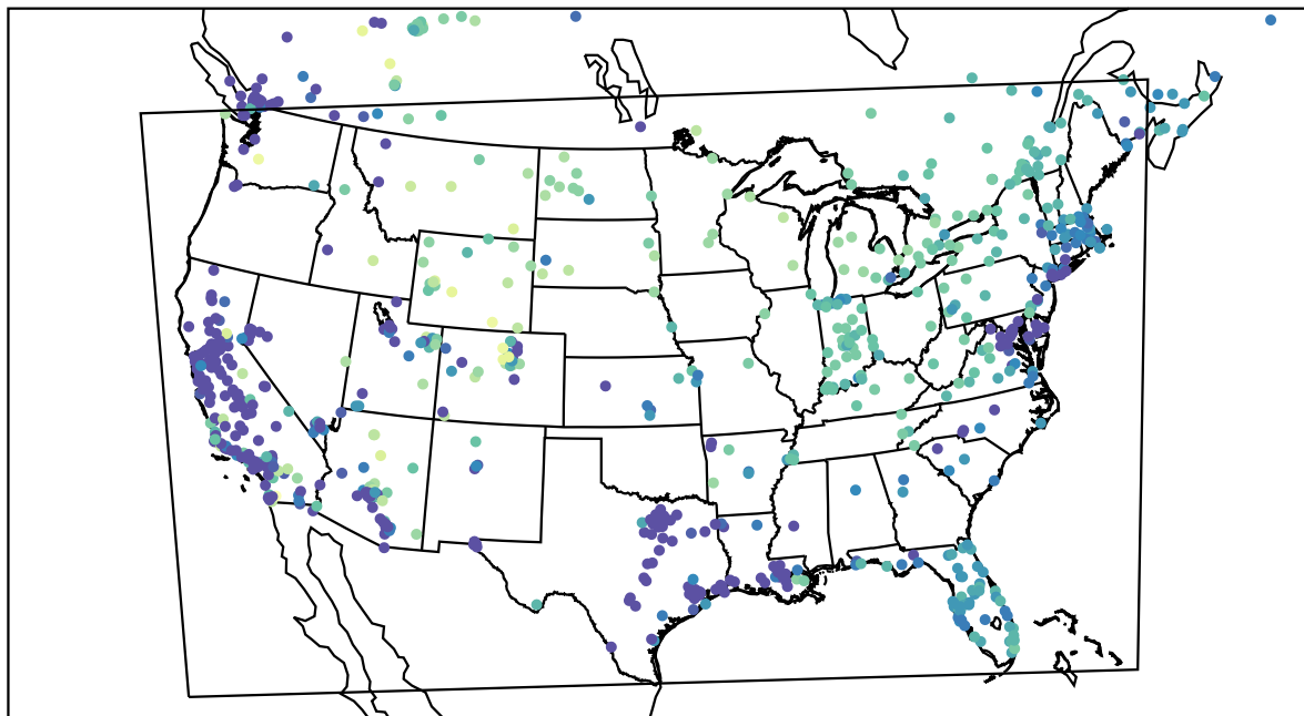
AirNOW (2022-12-25_08:00:00)
