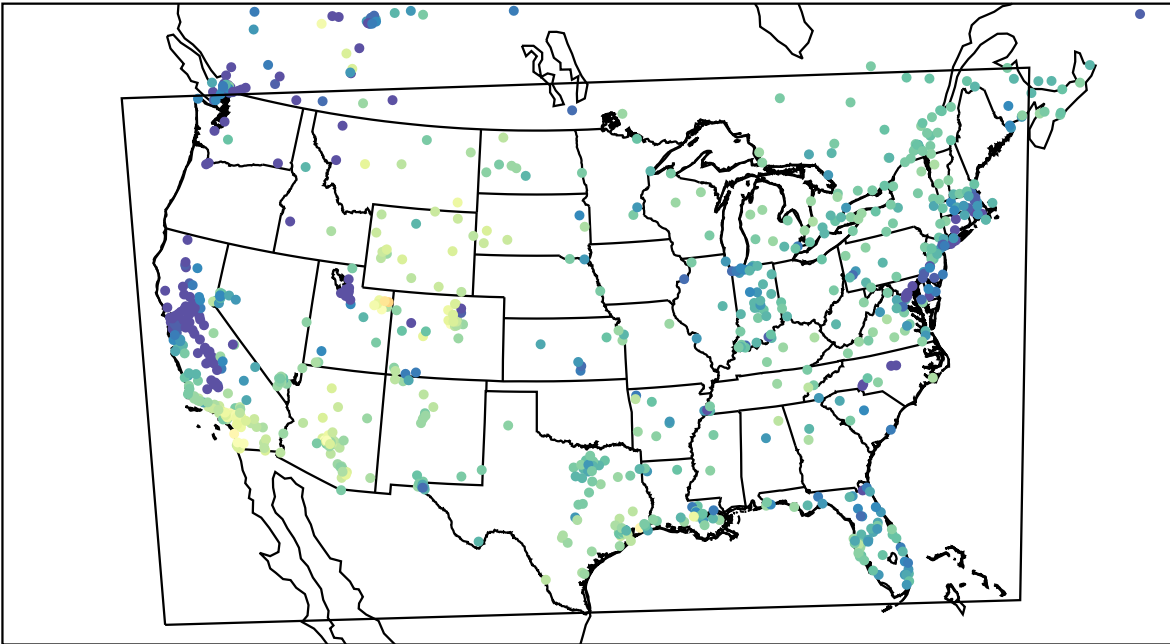
AirNOW (2022-12-25_23:00:00)
