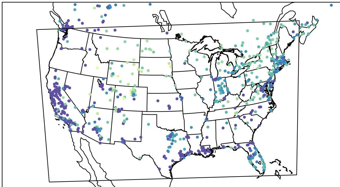
AirNOW (2022-12-26_06:00:00)
