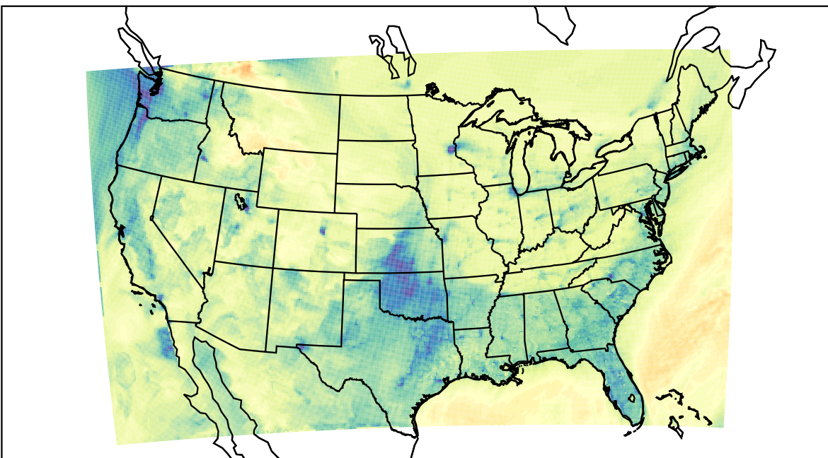
WRF (2022-12-25_23:00:00)
