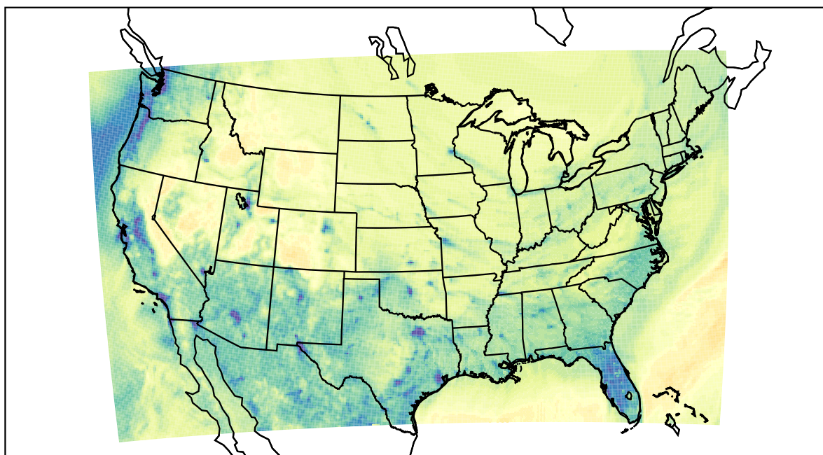
WRF (2022-12-25_02:00:00)
