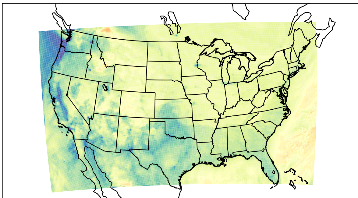
WRF (2022-12-25_18:00:00)
