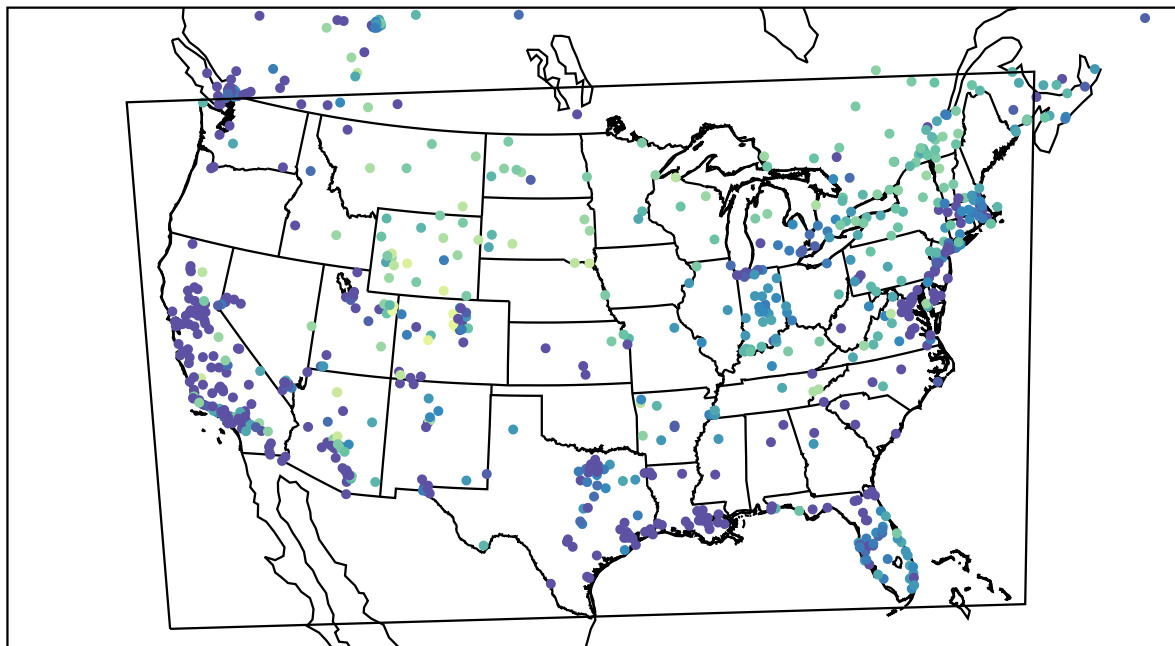
AirNOW (2022-12-26_11:00:00)
