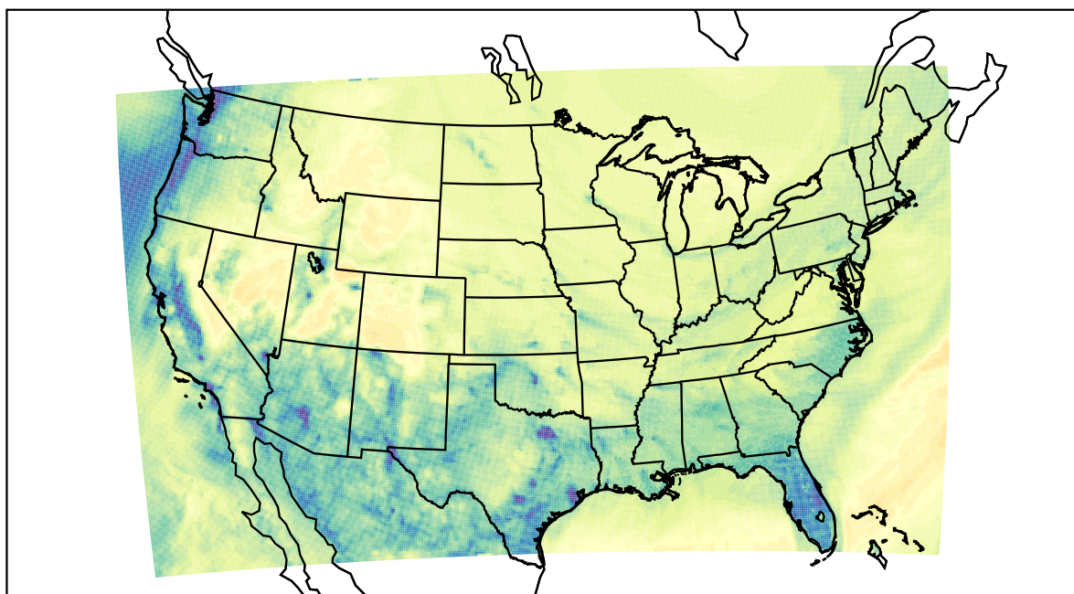
WRF (2022-12-25_05:00:00)
