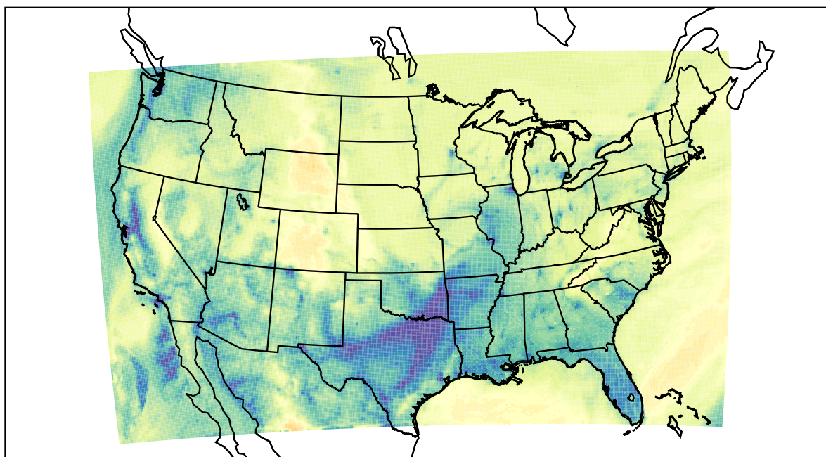
WRF (2022-12-26_14:00:00)
