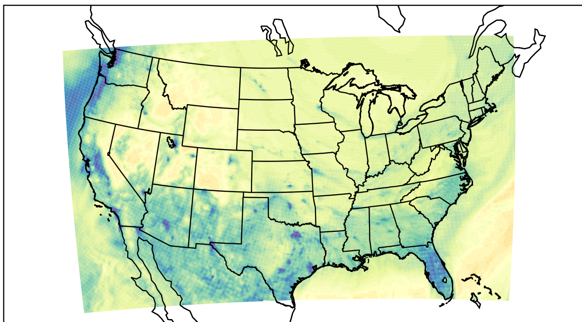
WRF (2022-12-25_03:00:00)
