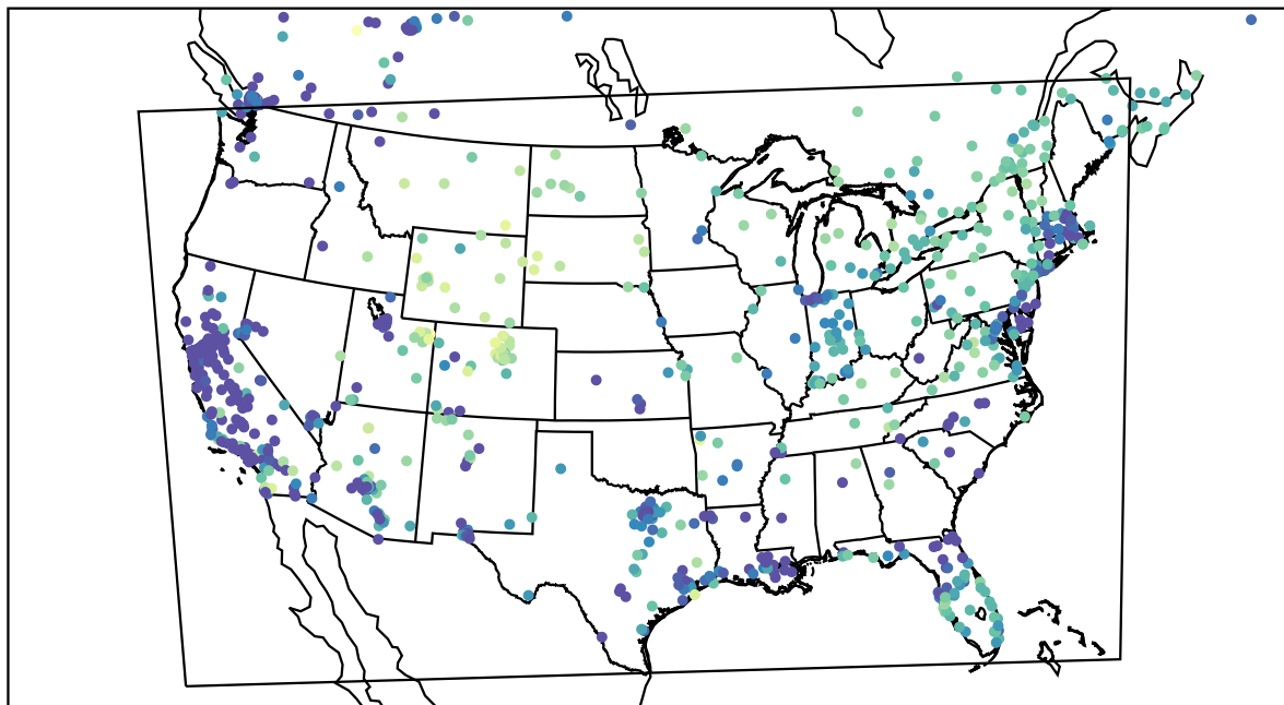
AirNOW (2022-12-26_02:00:00)
