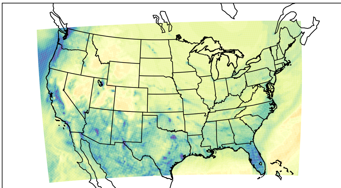
WRF (2022-12-25_04:00:00)
