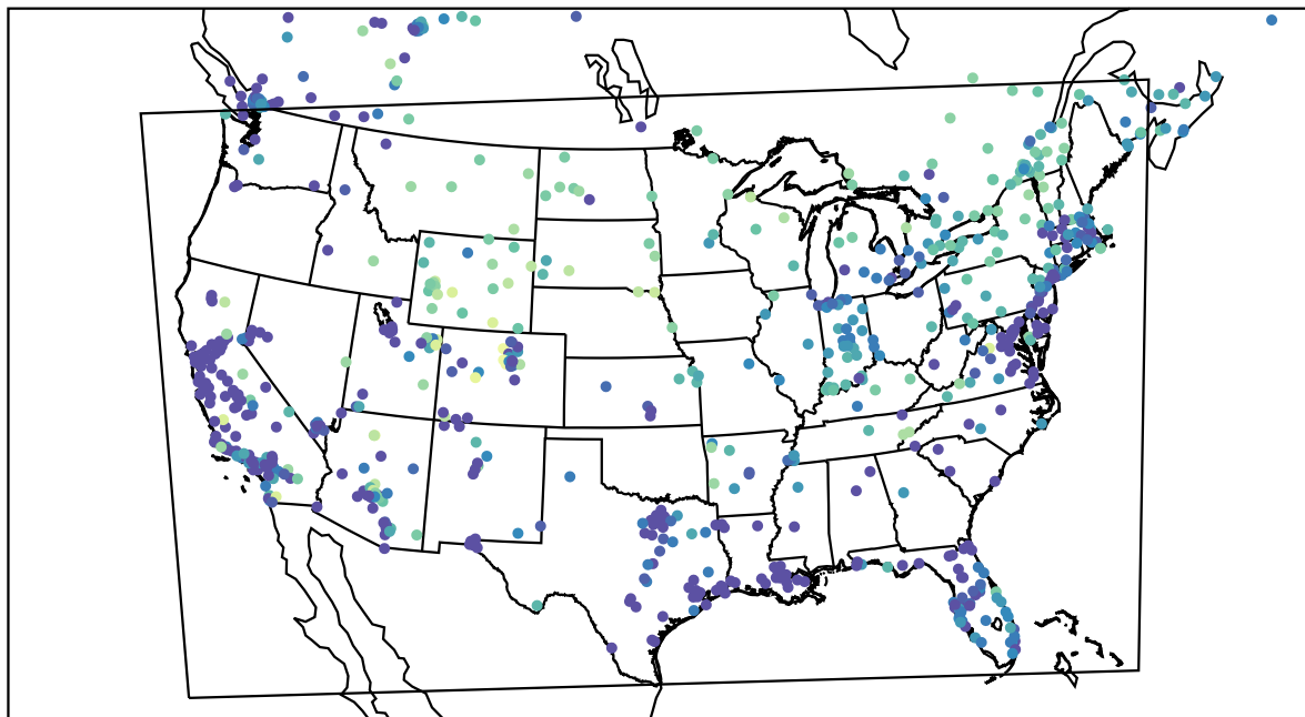
AirNOW (2022-12-26_12:00:00)
