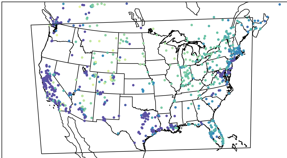
AirNOW (2022-12-25_06:00:00)
