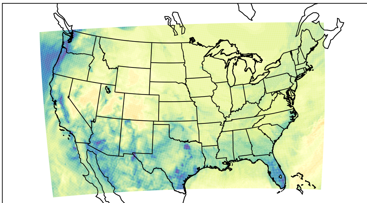
WRF (2022-12-25_09:00:00)
