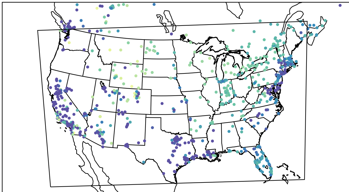
AirNOW (2022-12-25_11:00:00)
