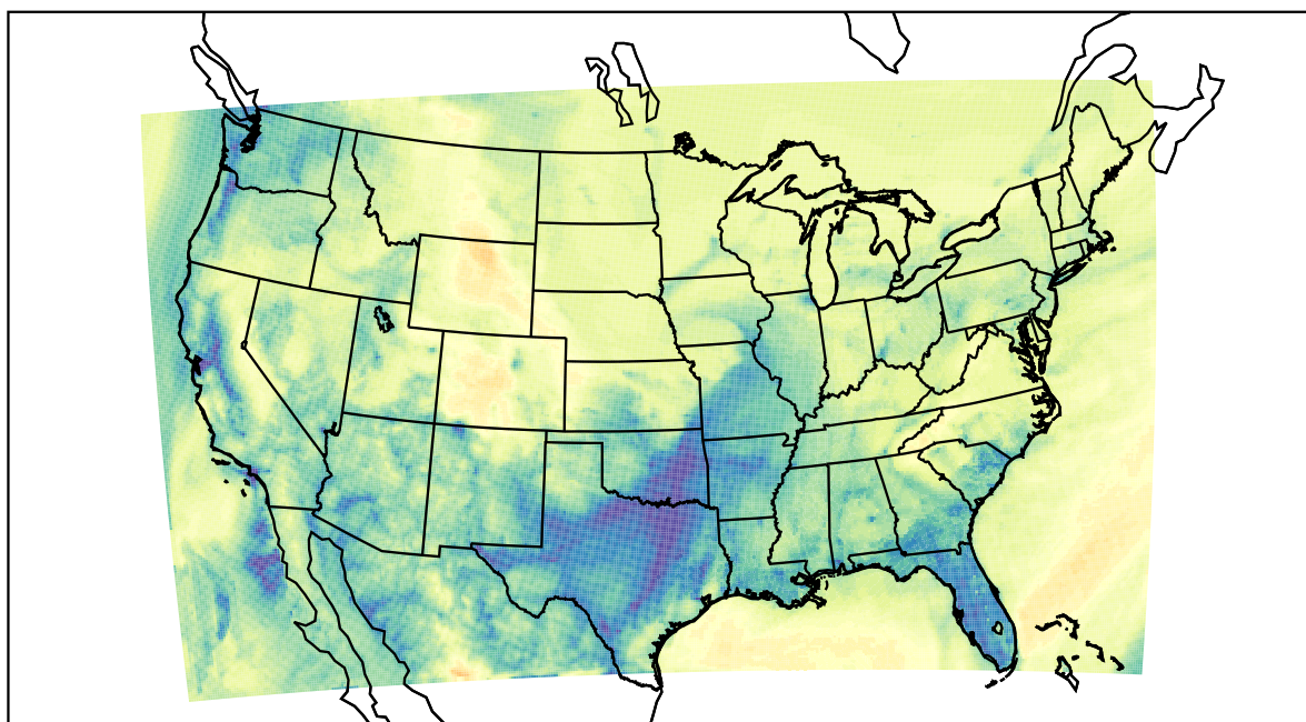
WRF (2022-12-26_11:00:00)
