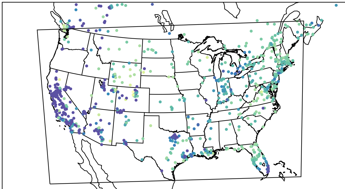
AirNOW (2022-12-26_16:00:00)
