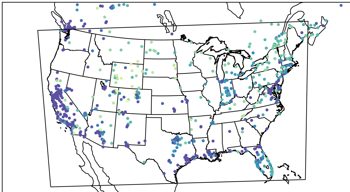
AirNOW (2022-12-26_08:00:00)
