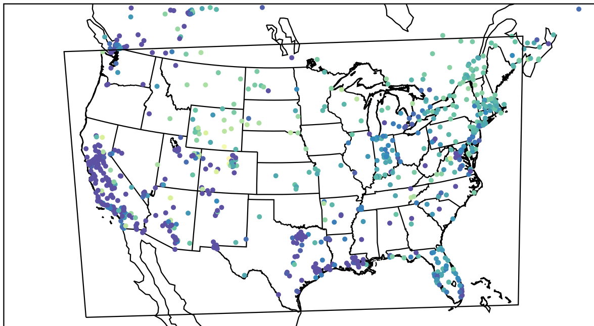
AirNOW (2022-12-26_14:00:00)
