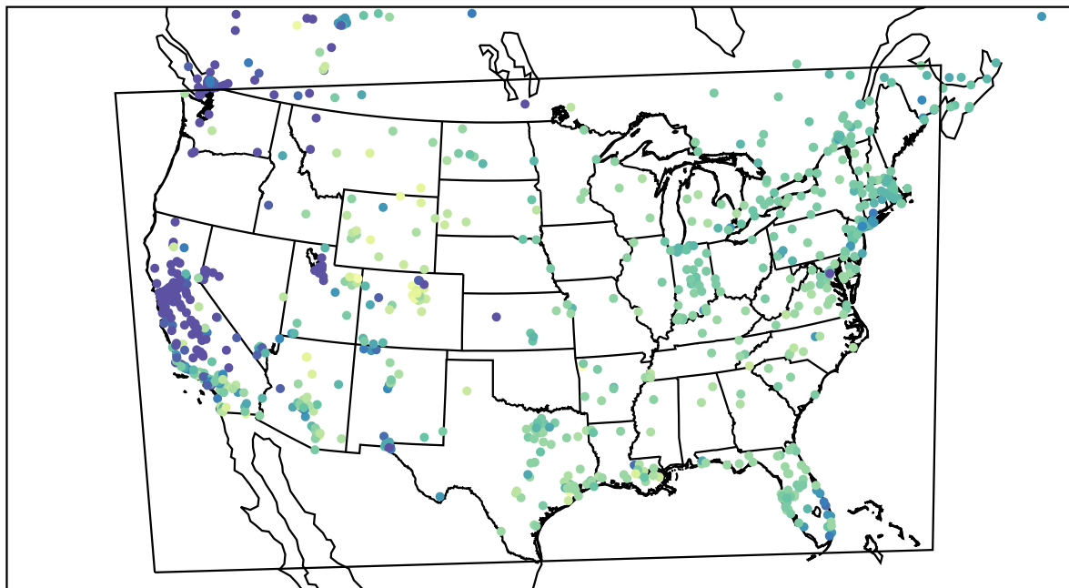
AirNOW (2022-12-25_18:00:00)
