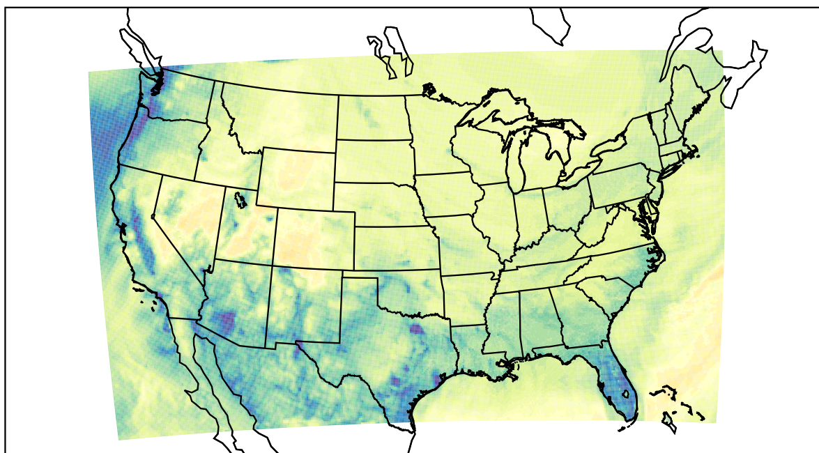
WRF (2022-12-25_07:00:00)
