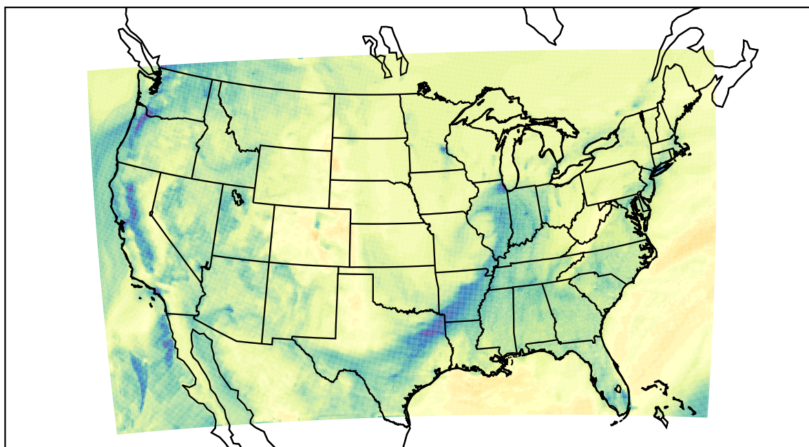
WRF (2022-12-26_20:00:00)
