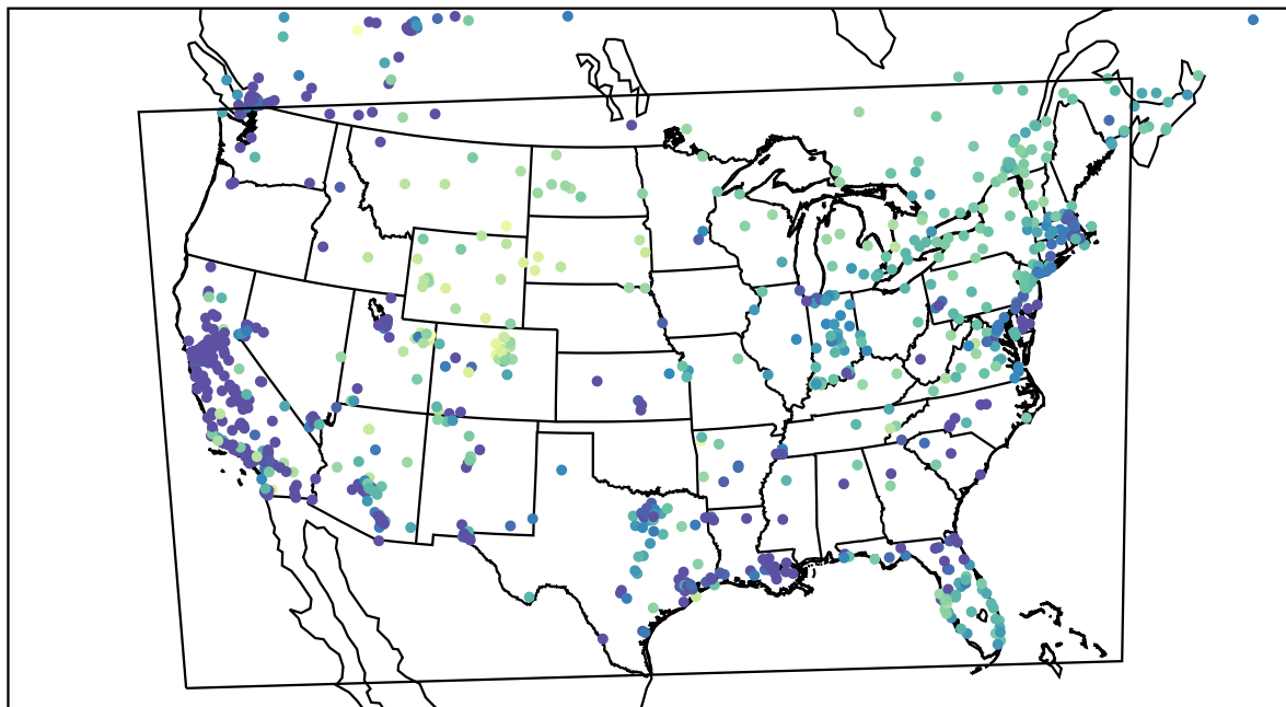
AirNOW (2022-12-26_03:00:00)
