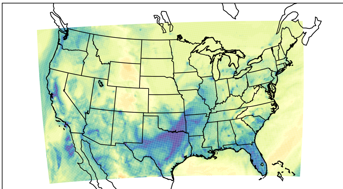
WRF (2022-12-26_13:00:00)
