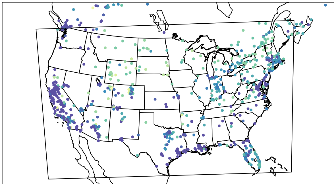
AirNOW (2022-12-26_09:00:00)
