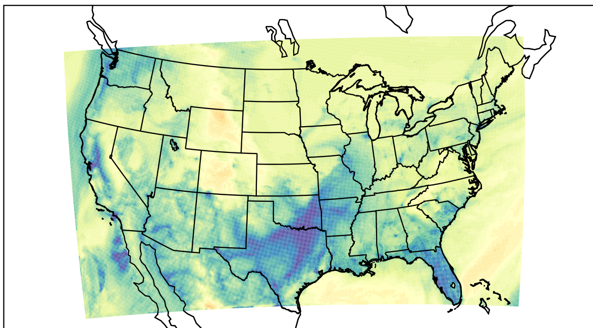
WRF (2022-12-26_12:00:00)
