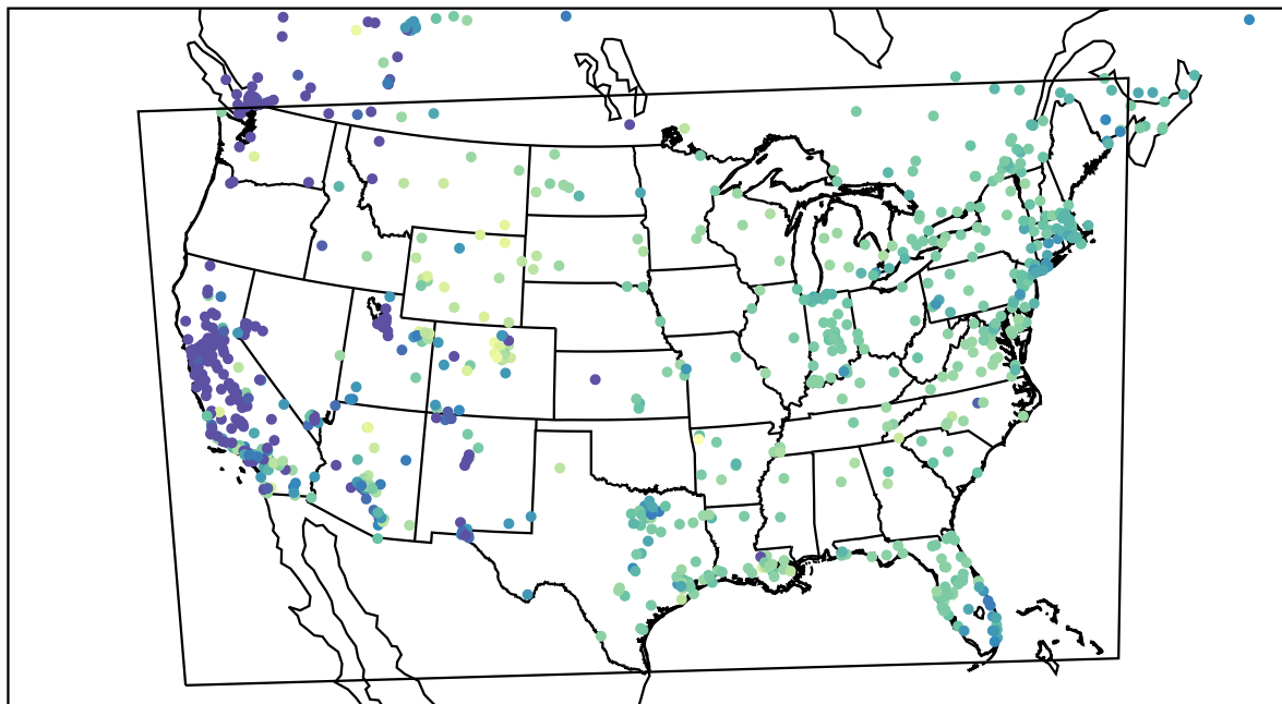
AirNOW (2022-12-25_17:00:00)
