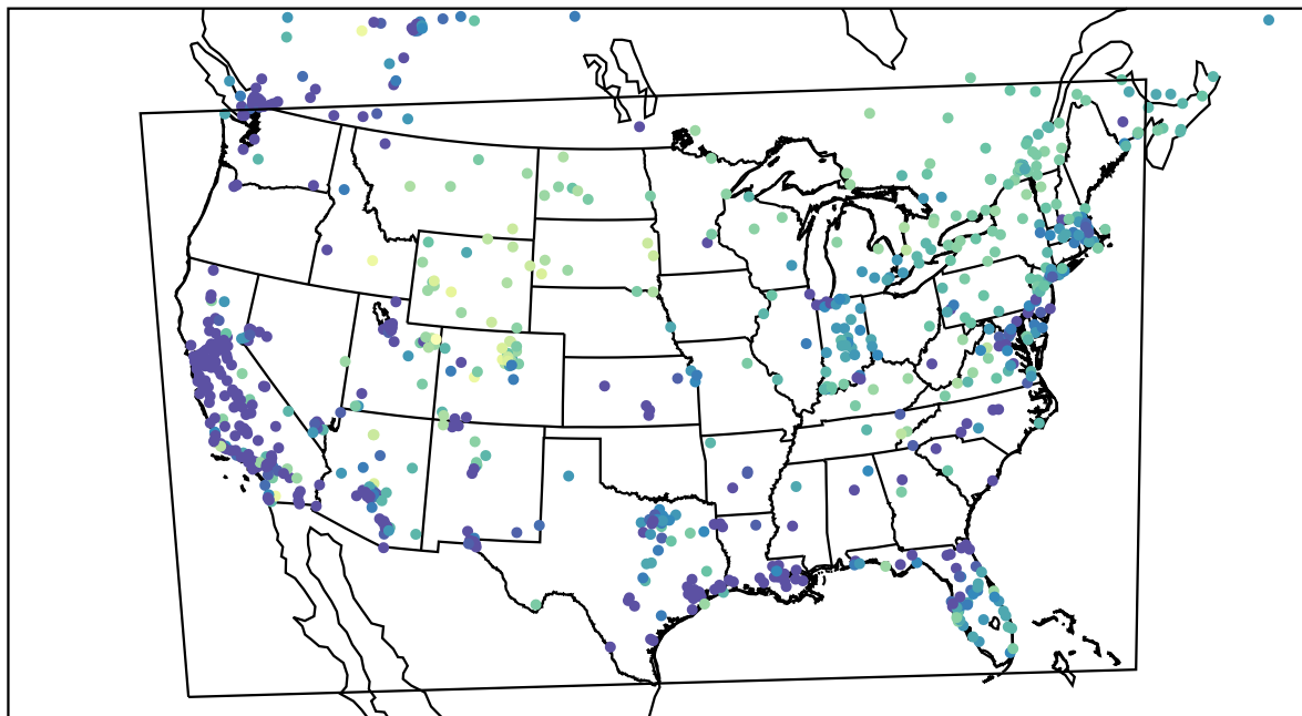
AirNOW (2022-12-26_05:00:00)
