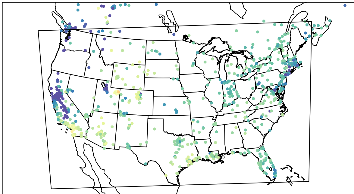
AirNOW (2022-12-25_22:00:00)
