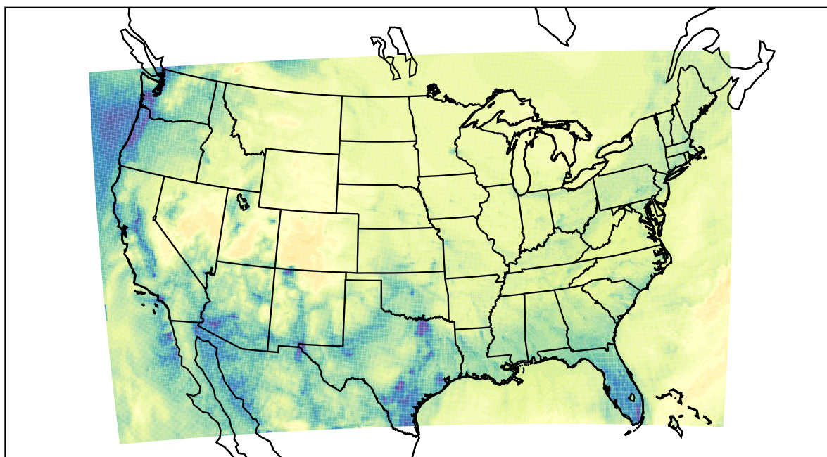
WRF (2022-12-25_12:00:00)
