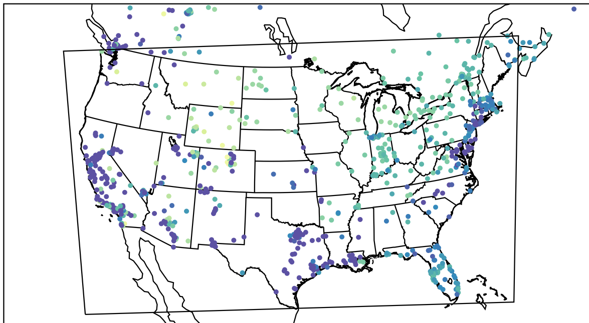
AirNOW (2022-12-25_12:00:00)
