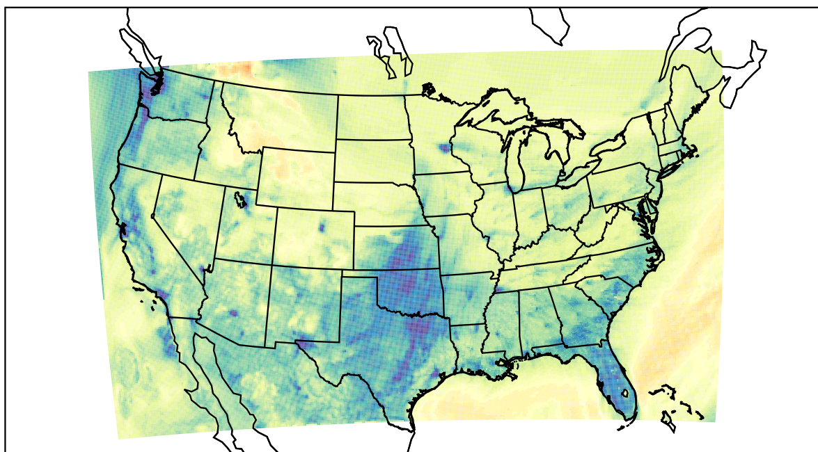
WRF (2022-12-26_02:00:00)
