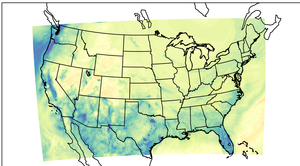
WRF (2022-12-25_06:00:00)
