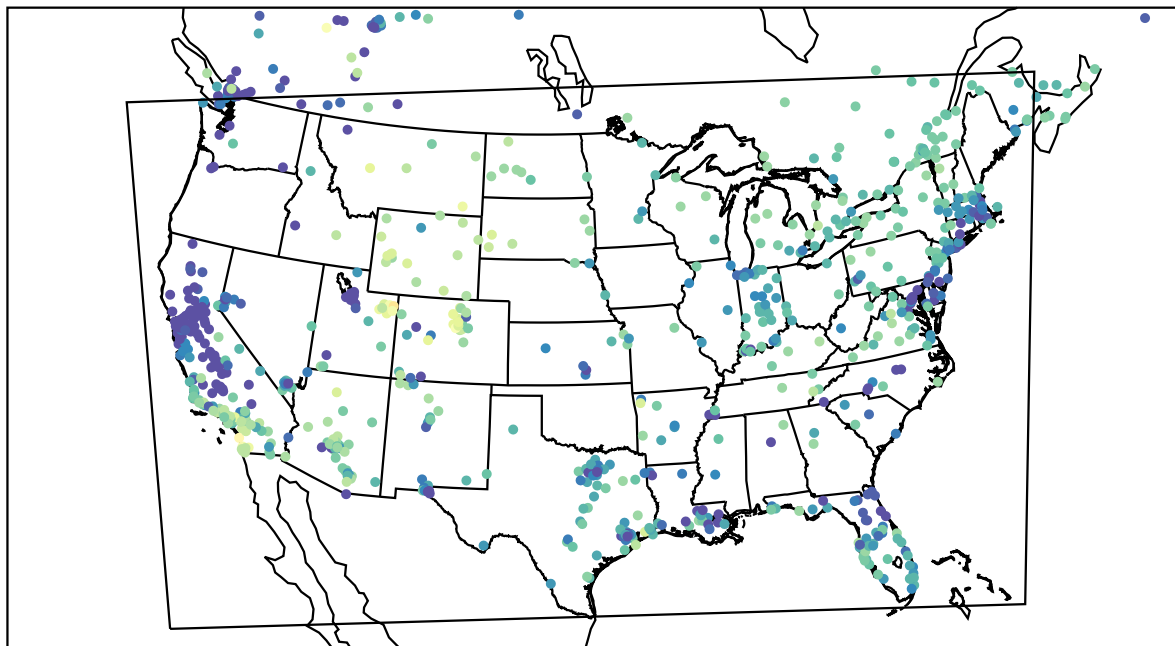
AirNOW (2022-12-26_00:00:00)
