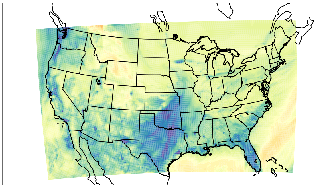
WRF (2022-12-26_05:00:00)
