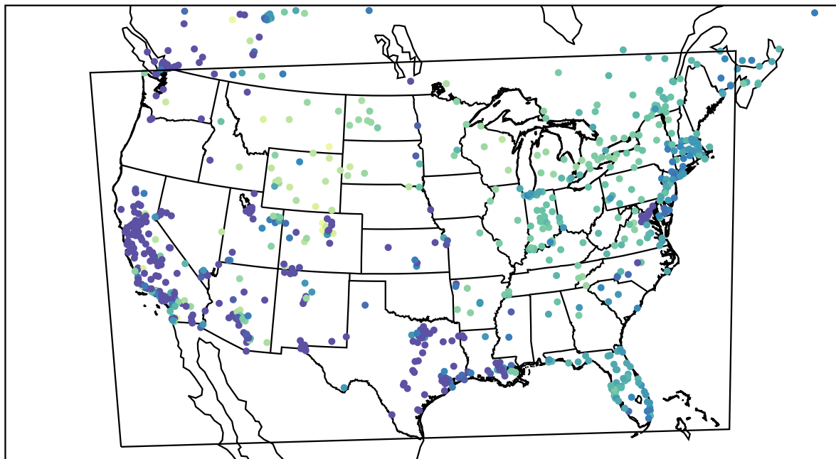
AirNOW (2022-12-25_14:00:00)
