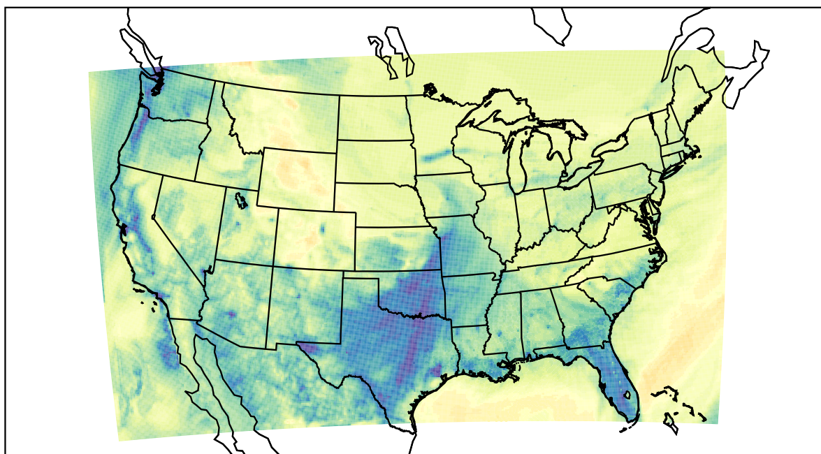
WRF (2022-12-26_07:00:00)
