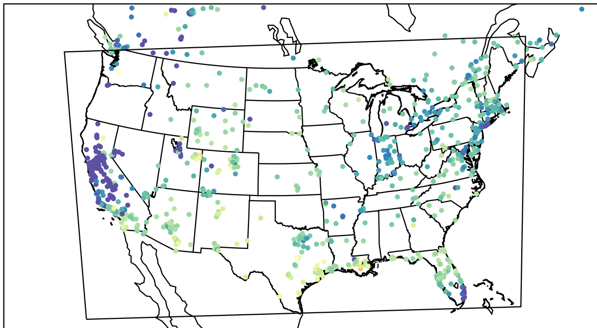
AirNOW (2022-12-26_21:00:00)
