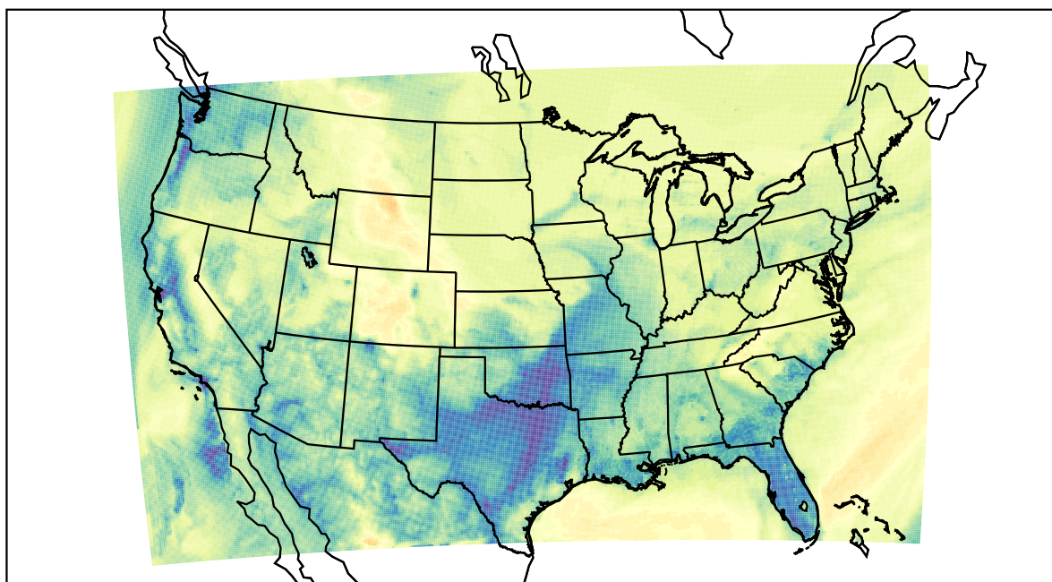
WRF (2022-12-26_10:00:00)
