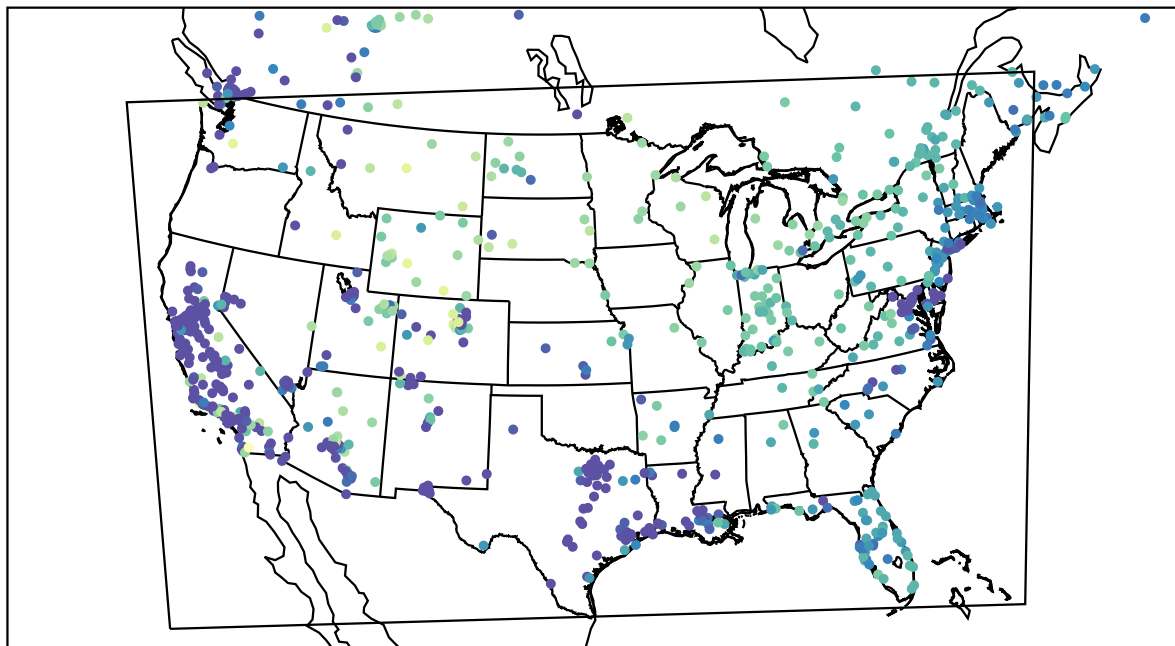
AirNOW (2022-12-25_05:00:00)
