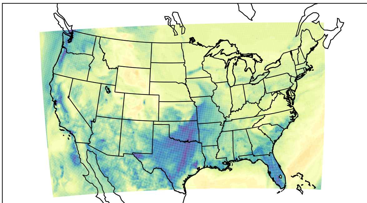
WRF (2022-12-26_08:00:00)
