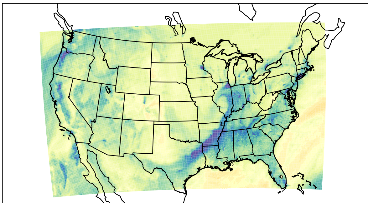
WRF (2022-12-26_22:00:00)
