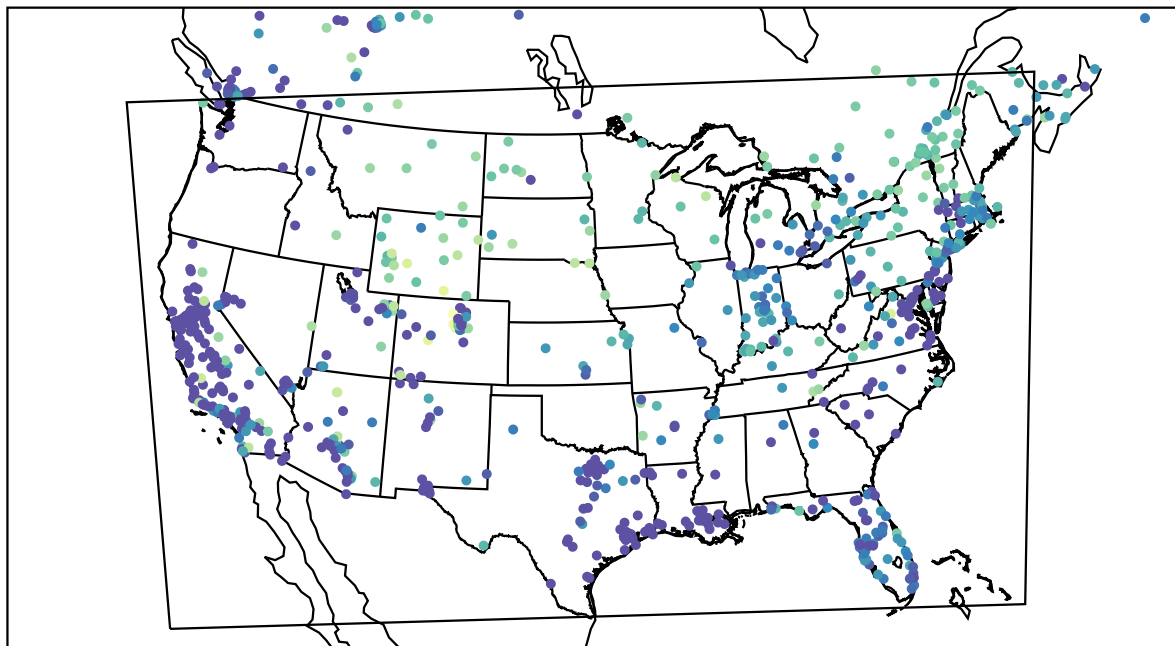
AirNOW (2022-12-26_13:00:00)
