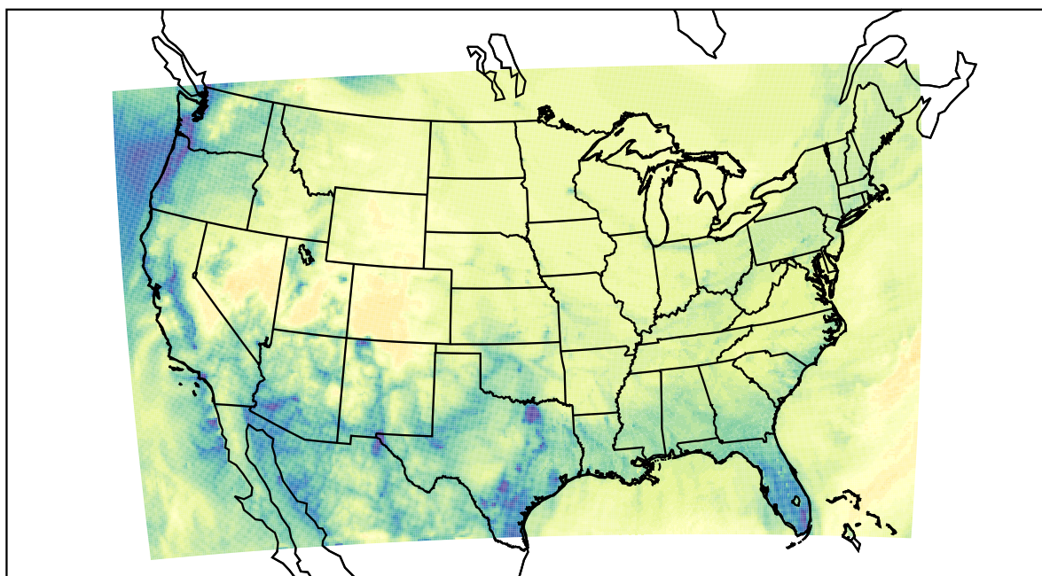
WRF (2022-12-25_11:00:00)
