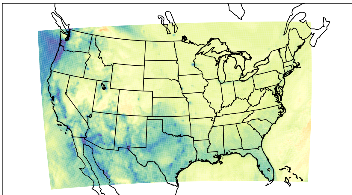
WRF (2022-12-25_16:00:00)
