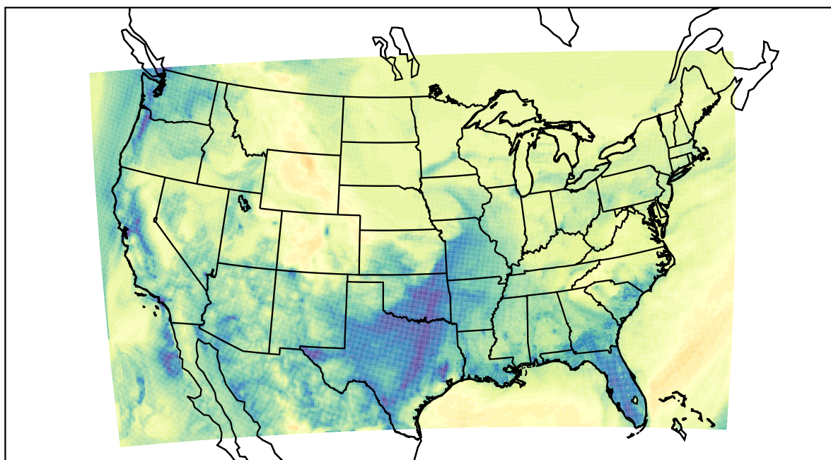
WRF (2022-12-26_09:00:00)
