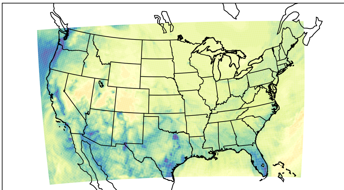
WRF (2022-12-25_10:00:00)
