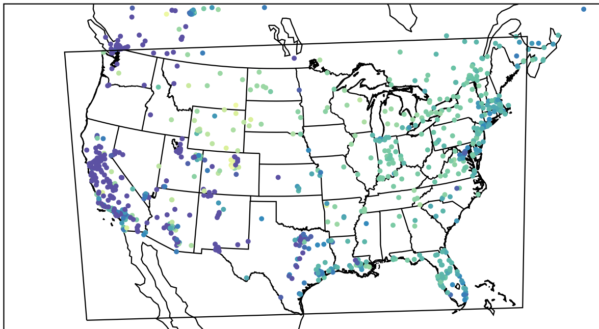
AirNOW (2022-12-25_15:00:00)
