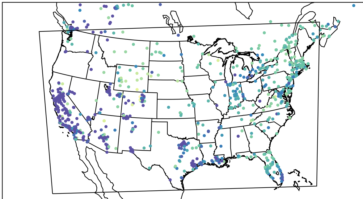
AirNOW (2022-12-26_15:00:00)
