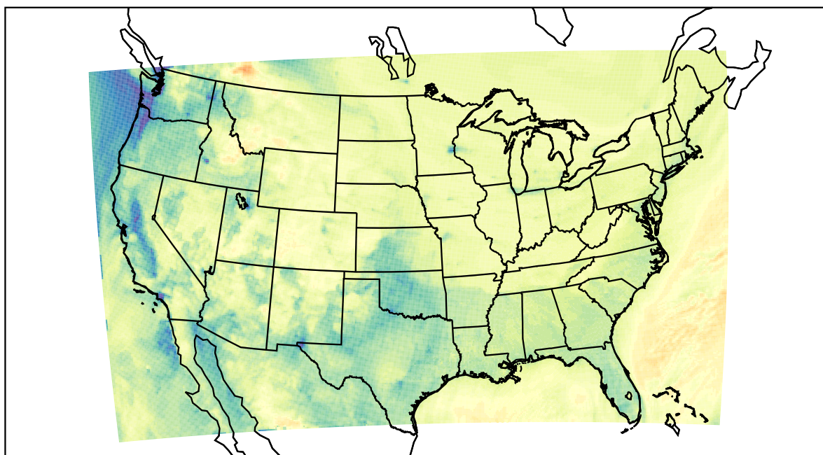
WRF (2022-12-25_19:00:00)
