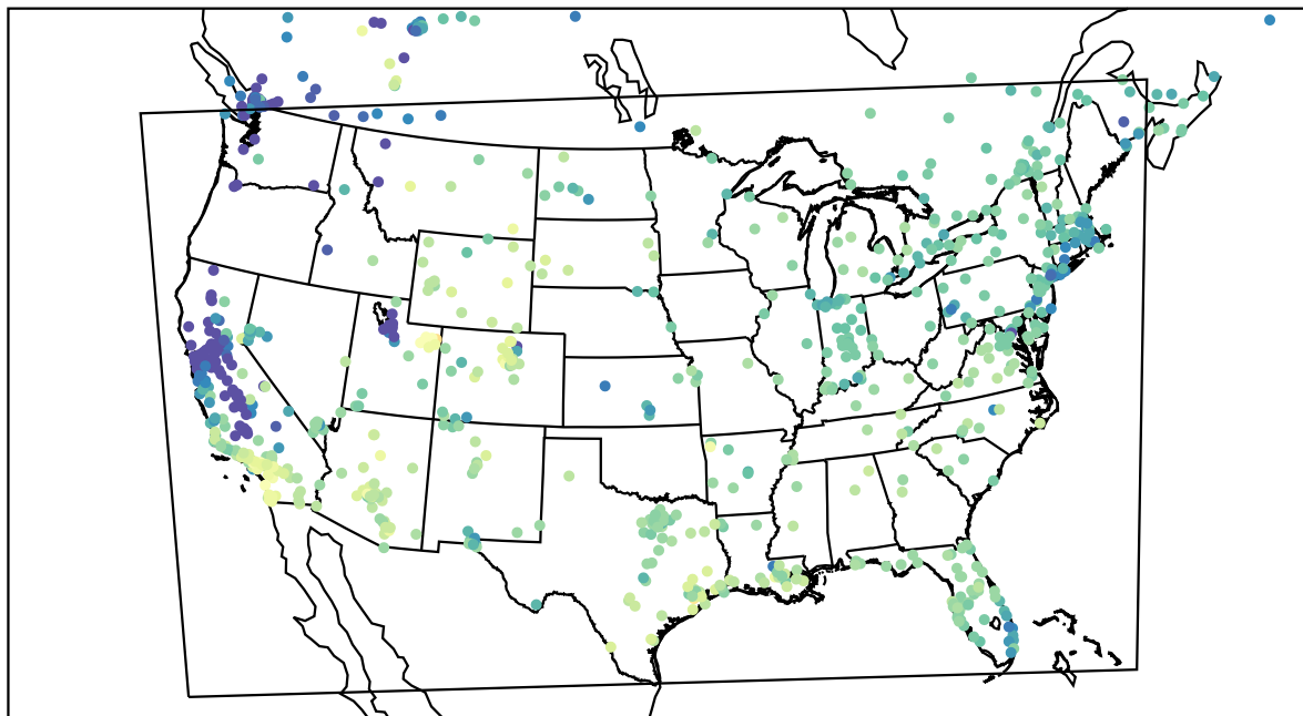
AirNOW (2022-12-25_21:00:00)
