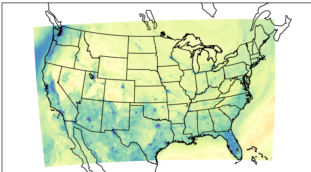
WRF (2022-12-25_01:00:00)
