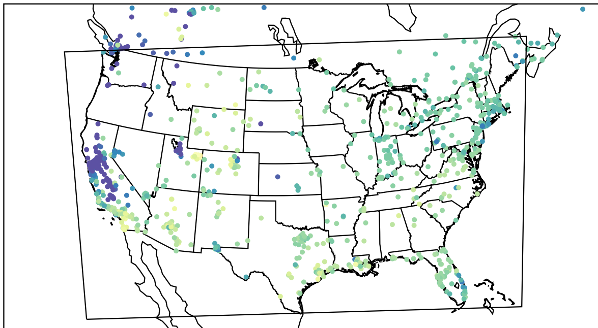
AirNOW (2022-12-25_20:00:00)
