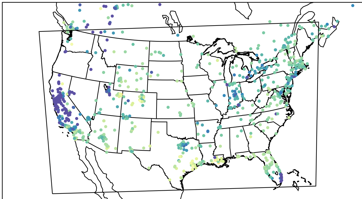
AirNOW (2022-12-26_20:00:00)
