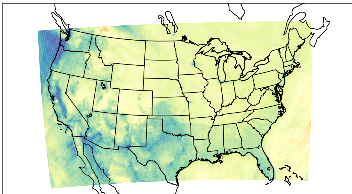
WRF (2022-12-25_17:00:00)
