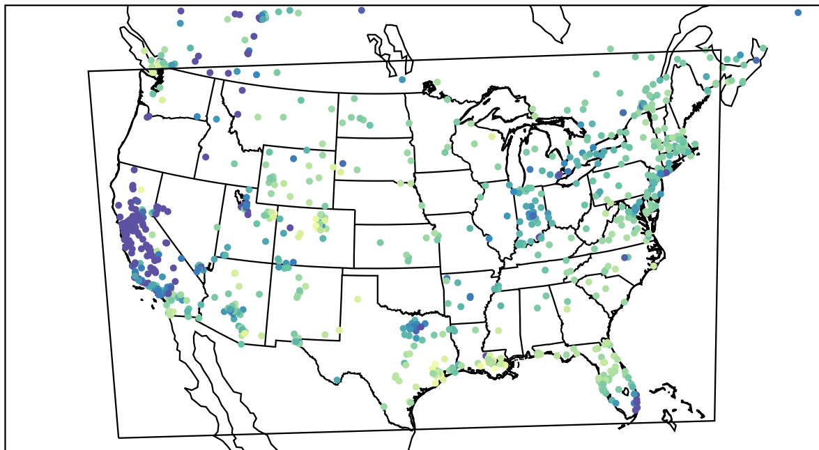
AirNOW (2022-12-26_19:00:00)
