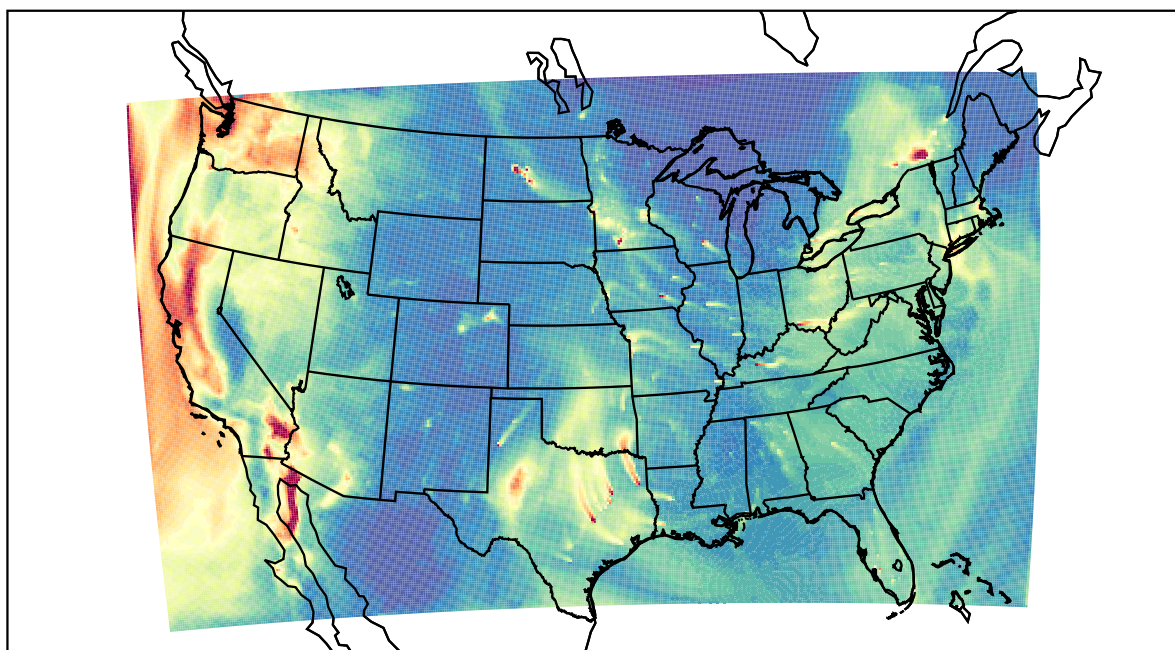
WRF 2023-01-06_17:00:00
