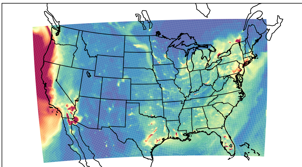
WRF 2023-01-06_00:00:00
