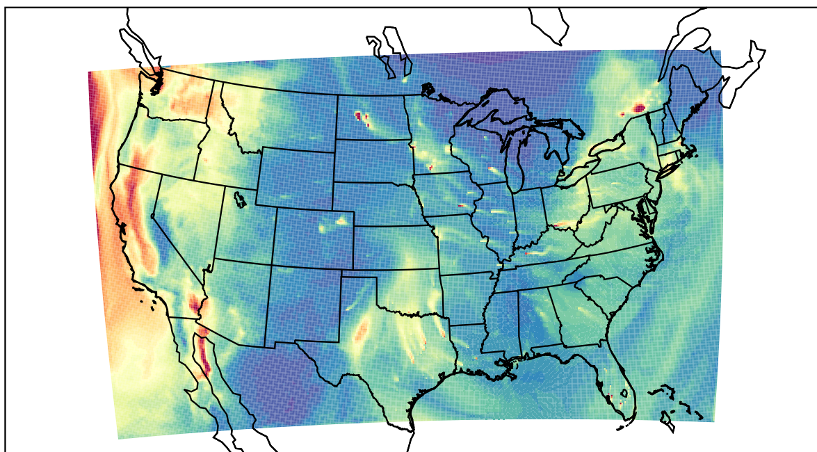
WRF 2023-01-06_19:00:00
