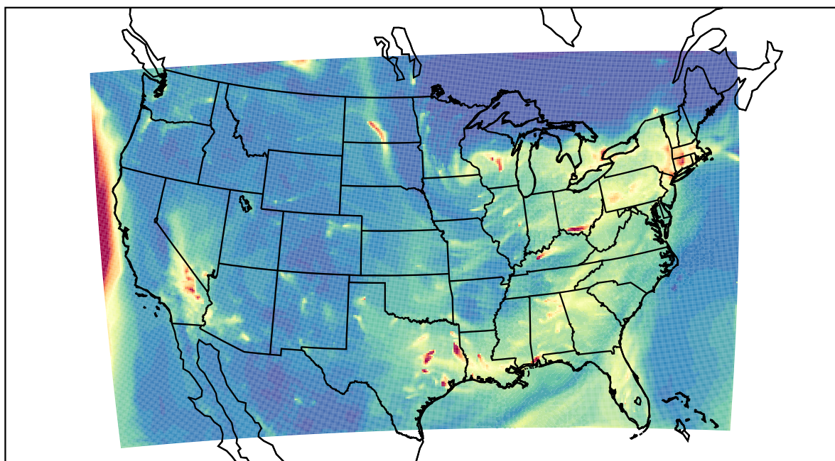
WRF 2023-01-05_06:00:00
