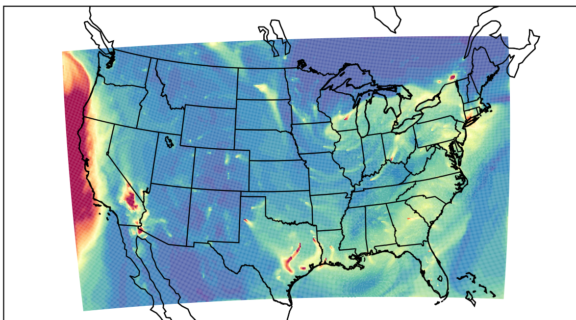
WRF 2023-01-05_17:00:00
