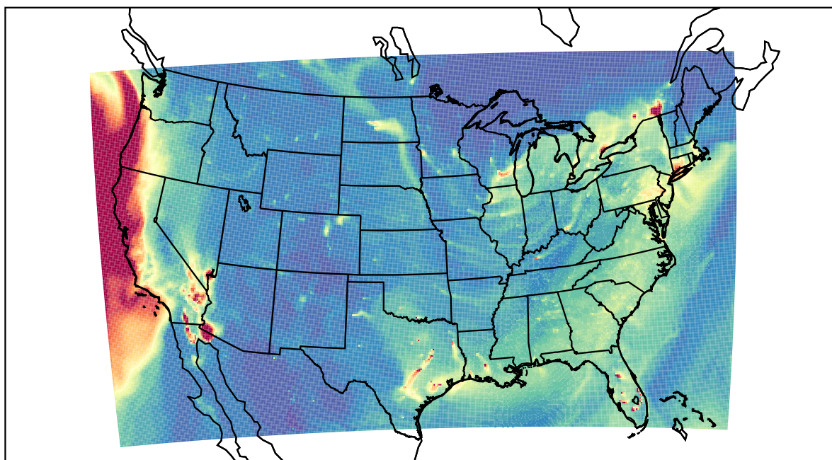
WRF 2023-01-05_22:00:00
