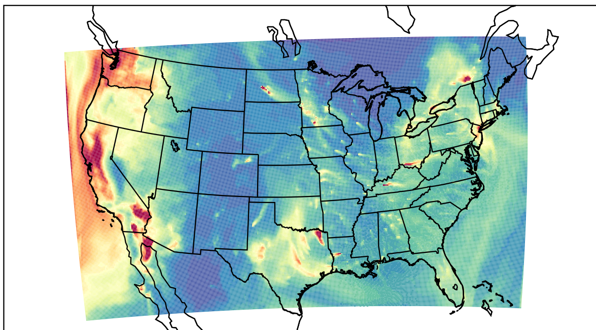
WRF 2023-01-06_14:00:00
