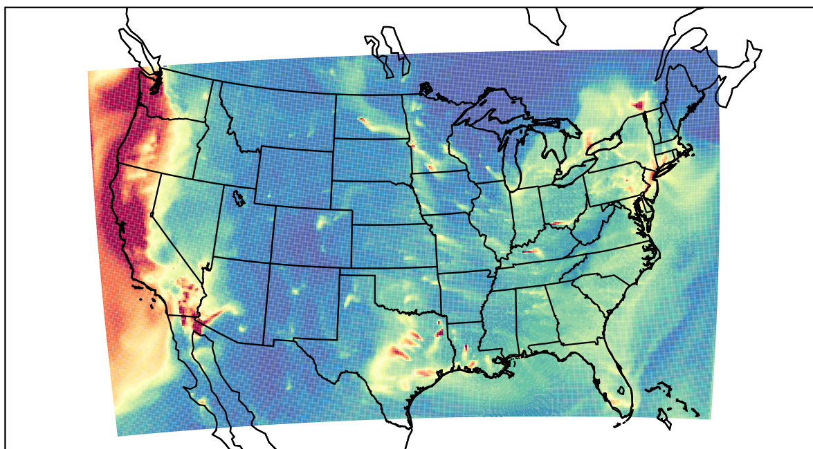
WRF 2023-01-06_06:00:00
