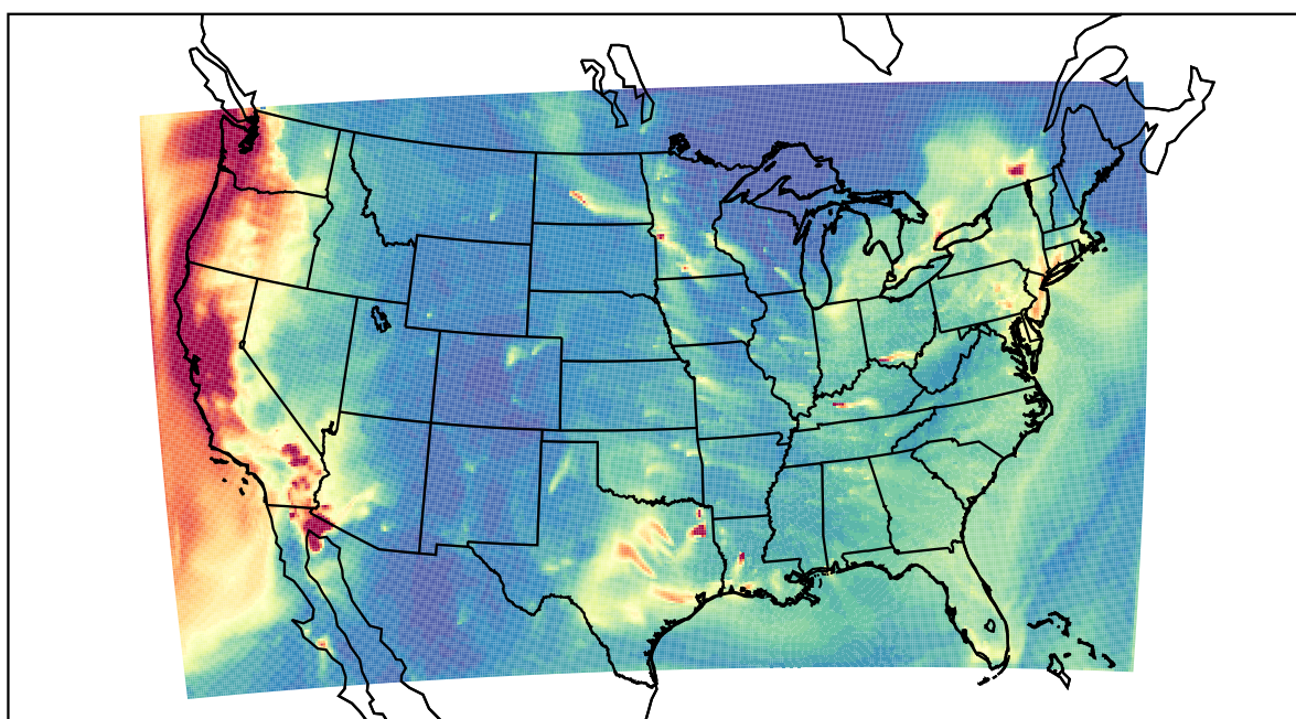
WRF 2023-01-06_08:00:00
