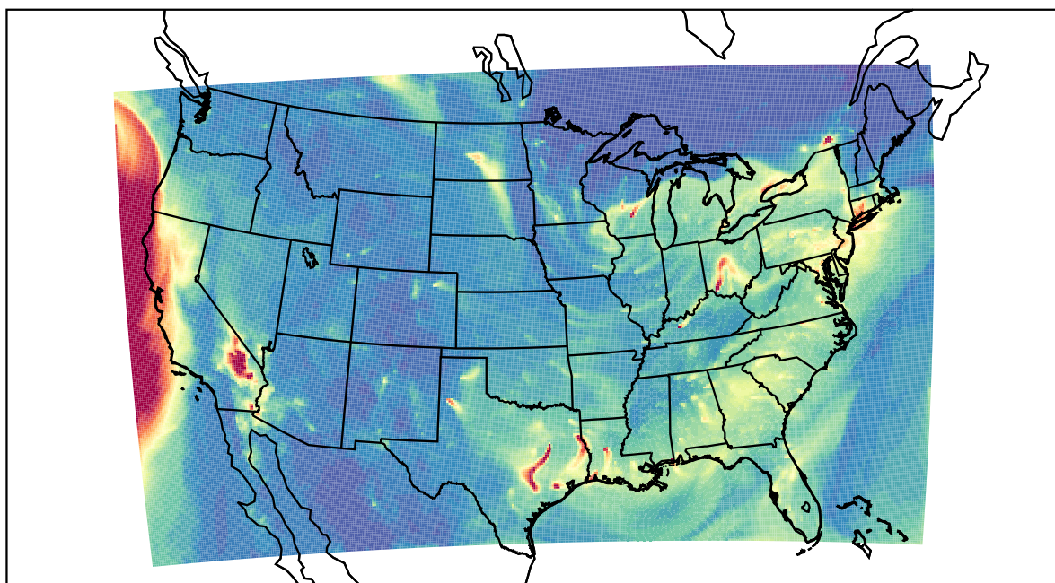
WRF 2023-01-05_15:00:00
