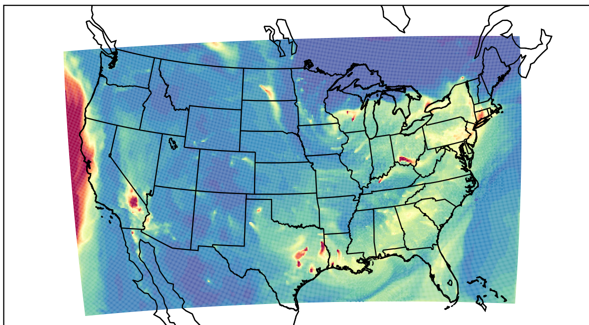
WRF 2023-01-05_11:00:00
