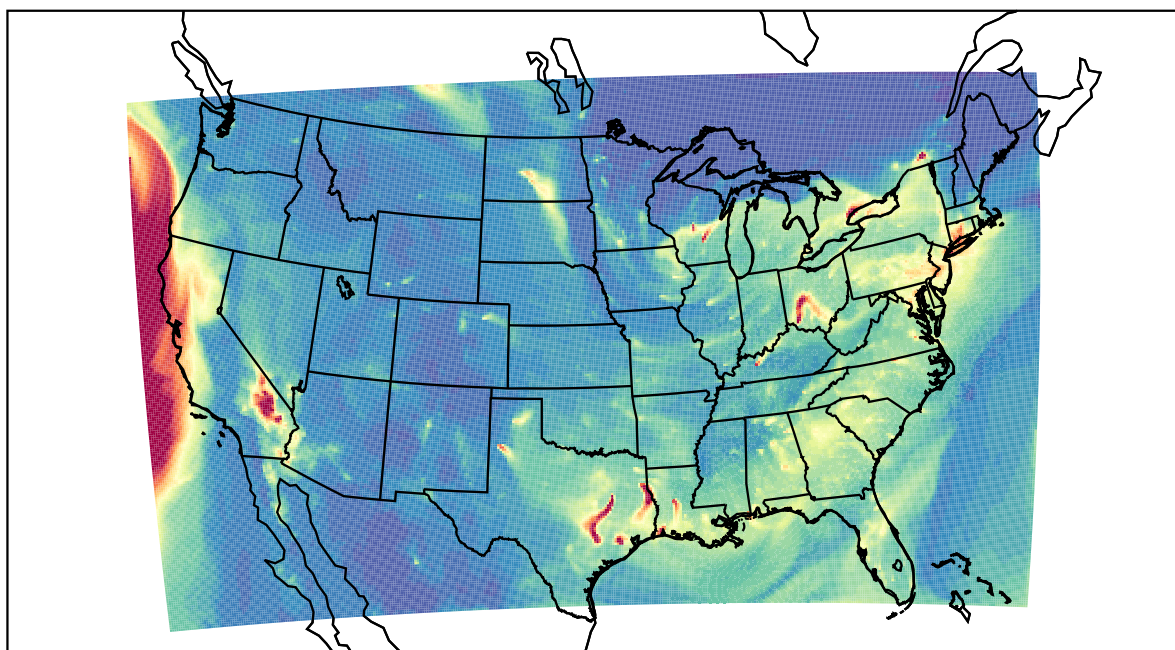
WRF 2023-01-05_14:00:00
