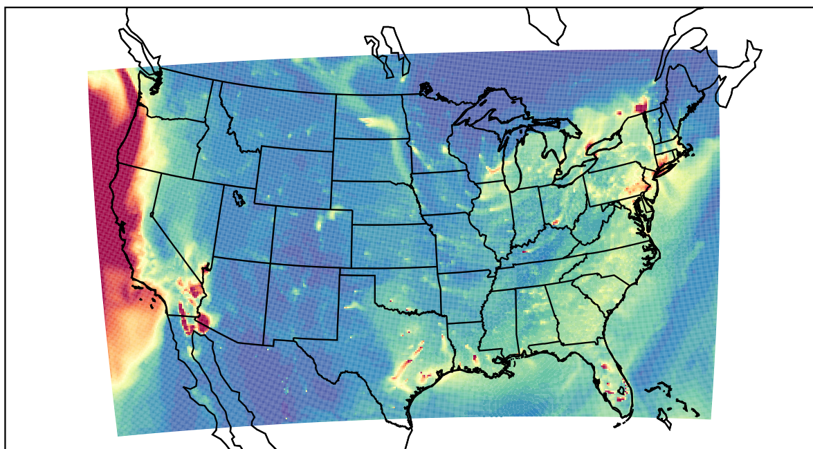
WRF 2023-01-05_23:00:00
