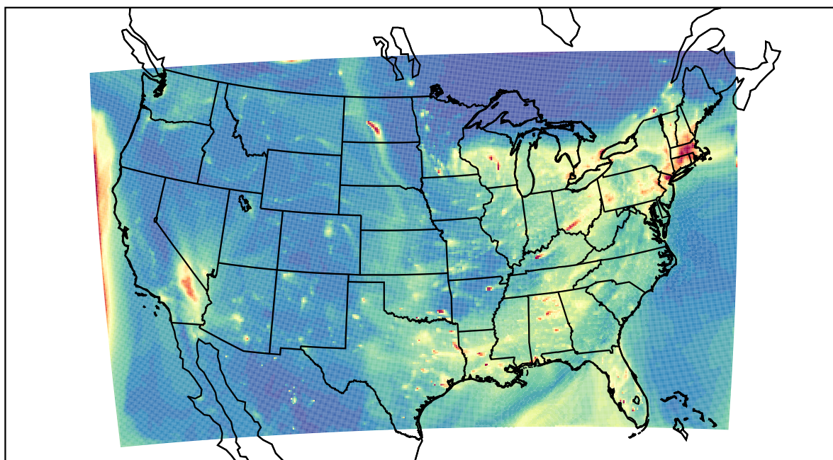
WRF 2023-01-05_01:00:00
