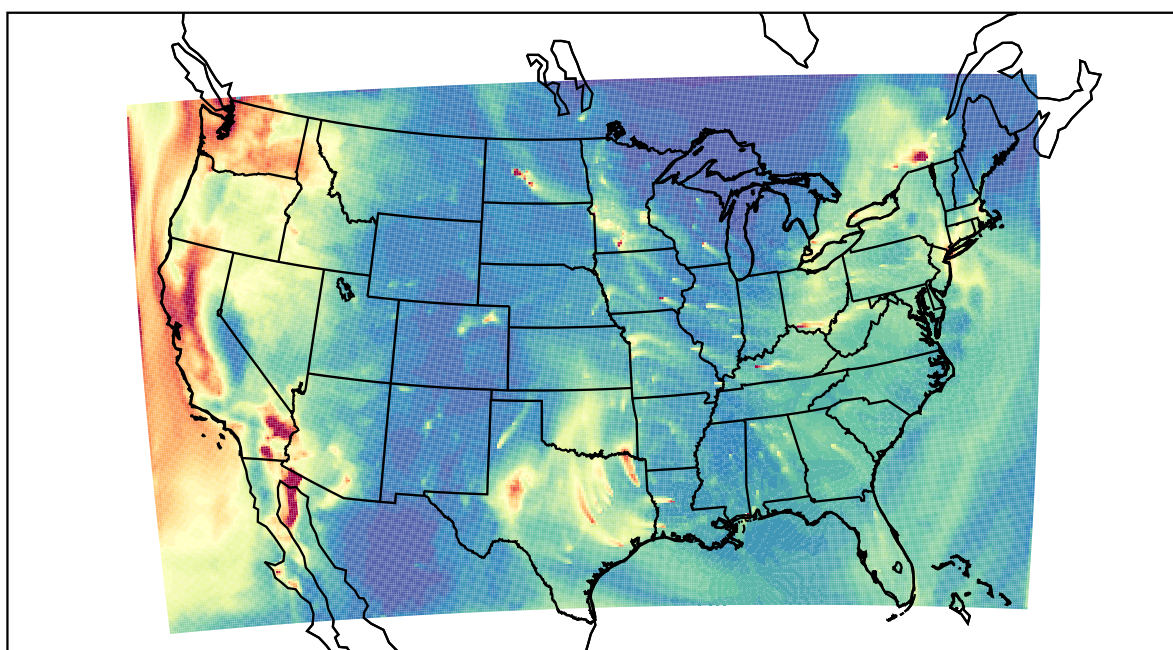
WRF 2023-01-06_16:00:00
