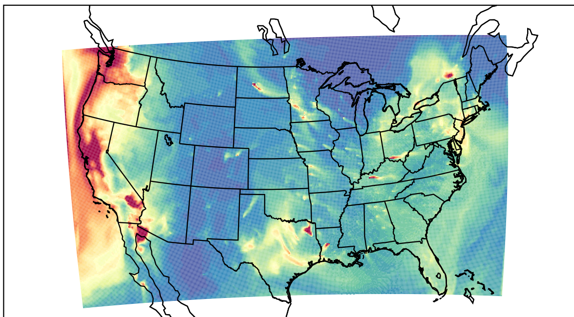
WRF 2023-01-06_11:00:00
