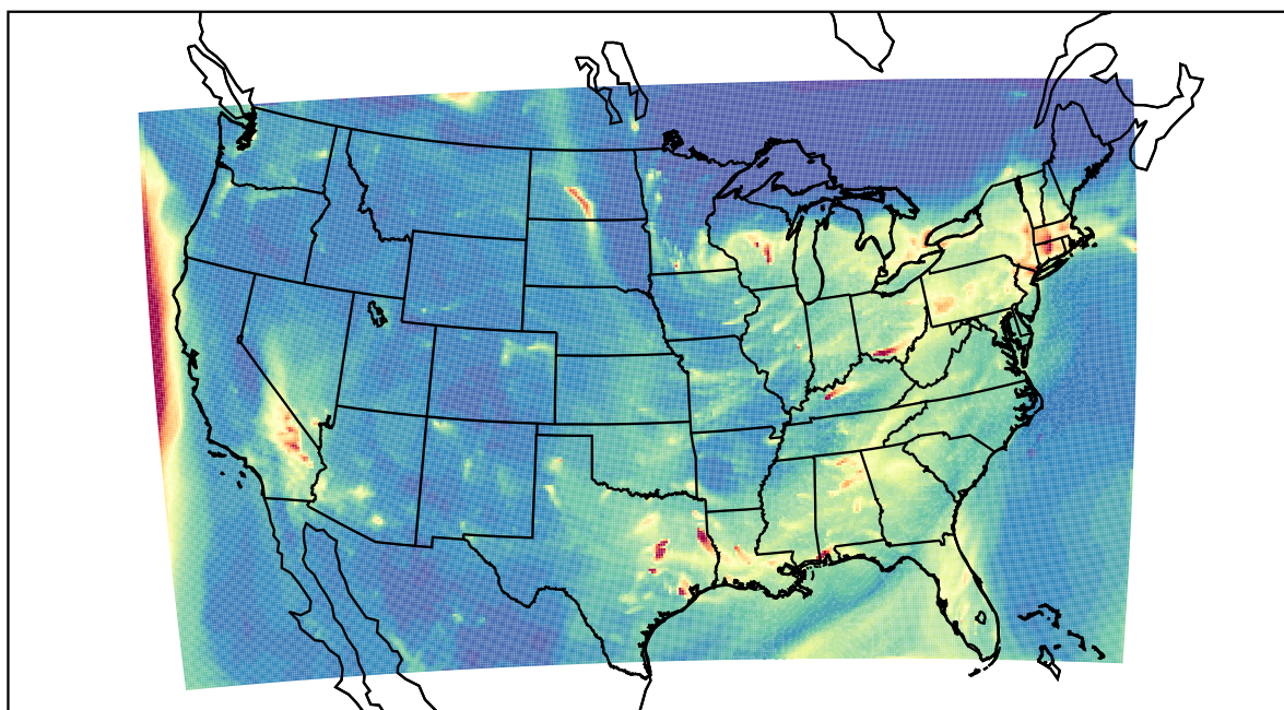
WRF 2023-01-05_05:00:00
