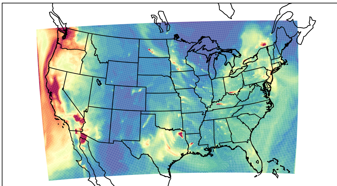
WRF 2023-01-06_12:00:00
