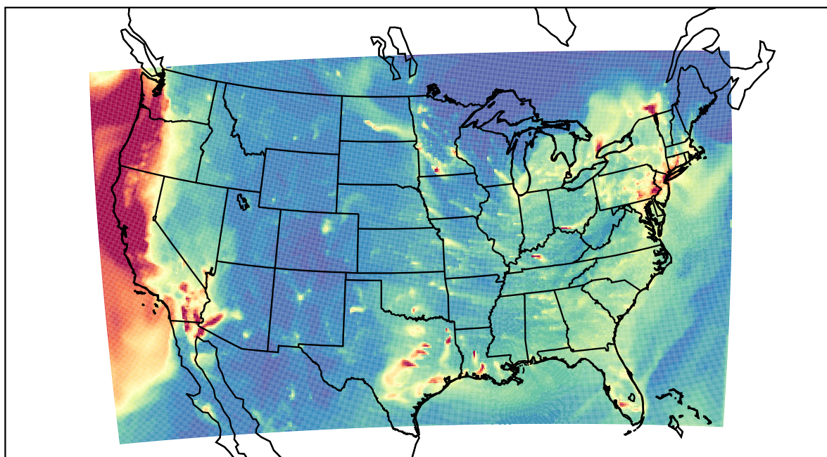
WRF 2023-01-06_04:00:00
