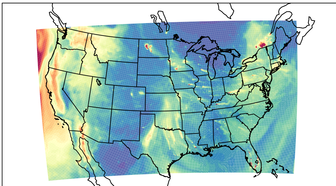
WRF 2023-01-06_22:00:00
