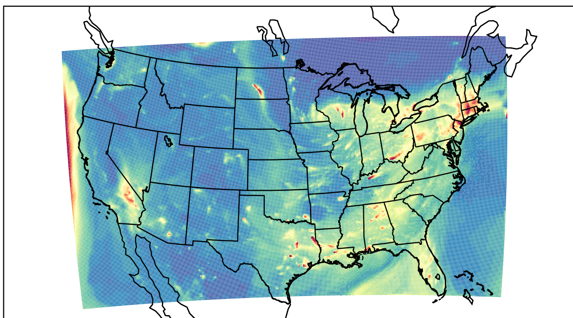
WRF 2023-01-05_03:00:00
