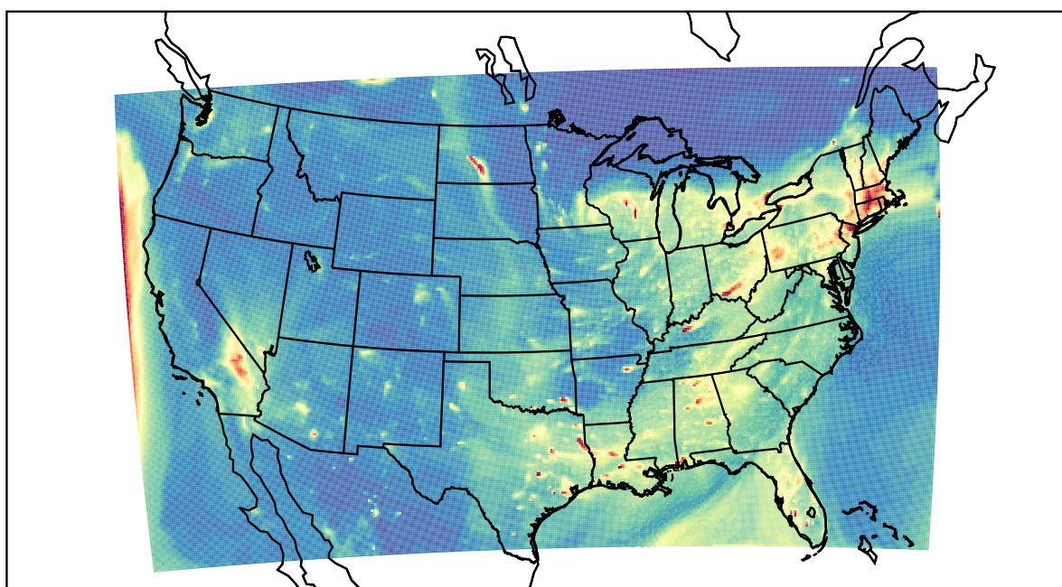
WRF 2023-01-05_02:00:00
