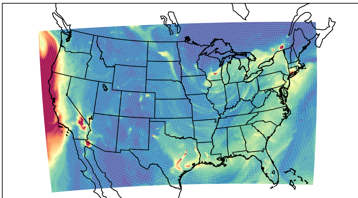
WRF 2023-01-05_19:00:00
