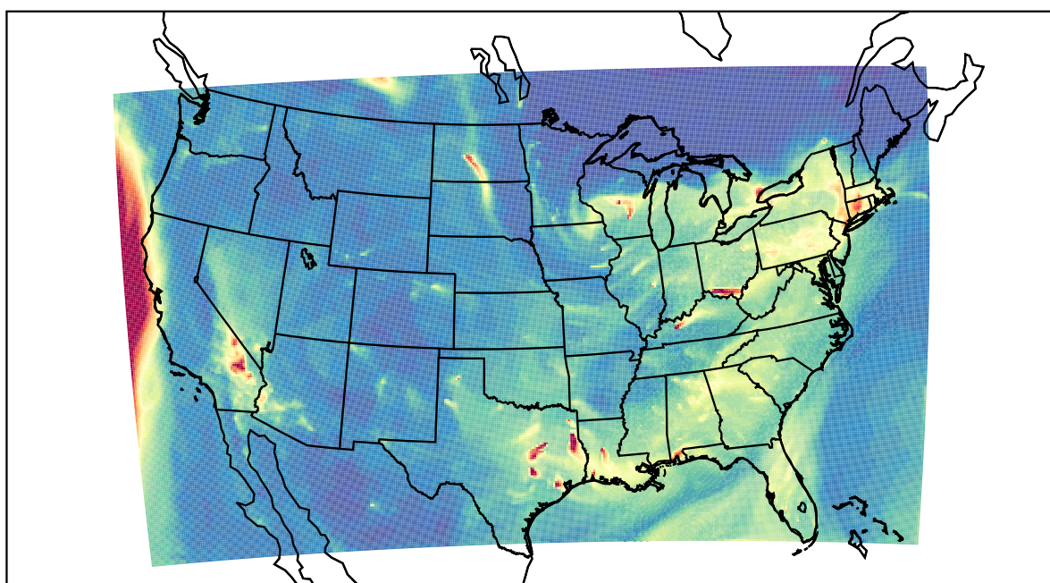
WRF 2023-01-05_08:00:00
