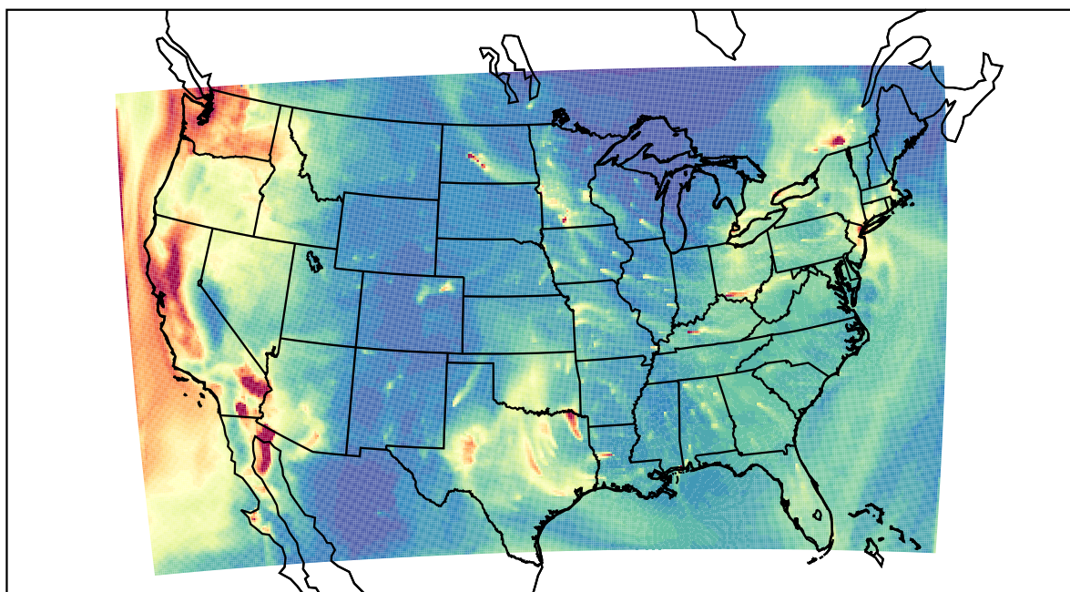
WRF 2023-01-06_15:00:00
