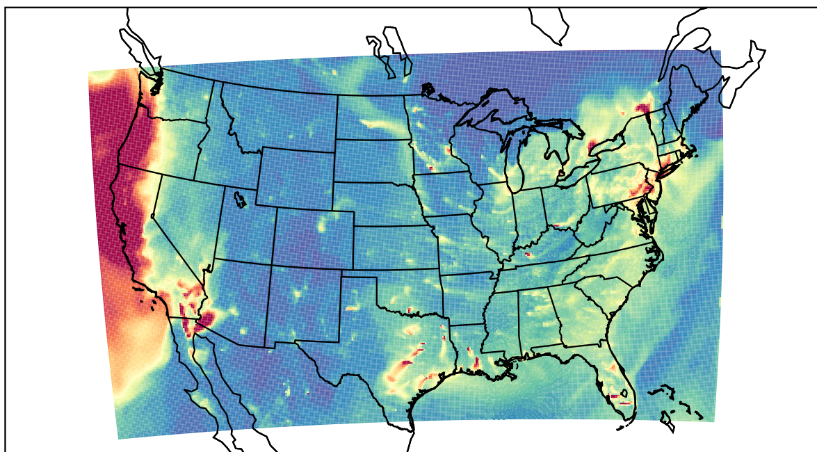
WRF 2023-01-06_02:00:00
