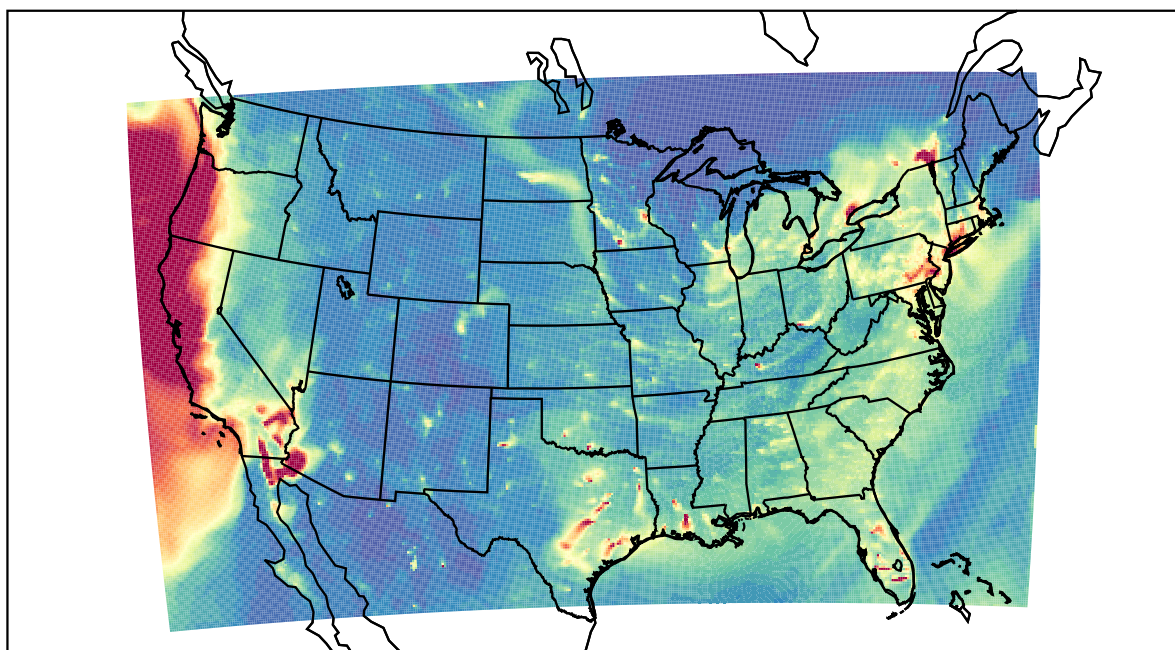
WRF 2023-01-06_01:00:00
