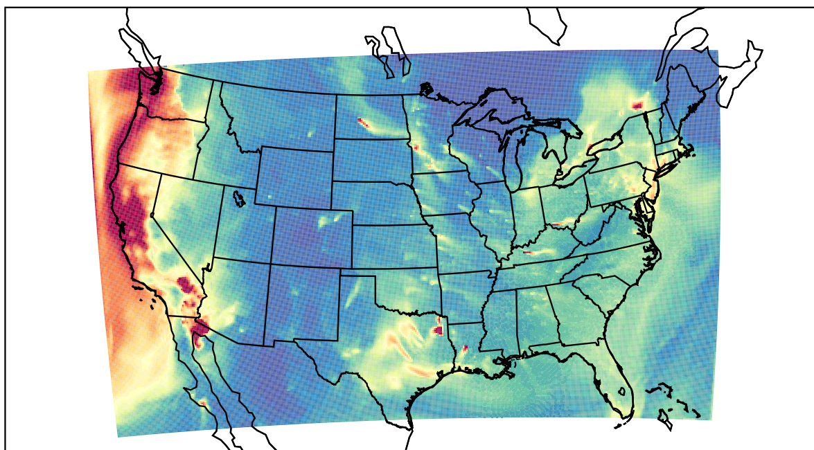
WRF 2023-01-06_09:00:00
