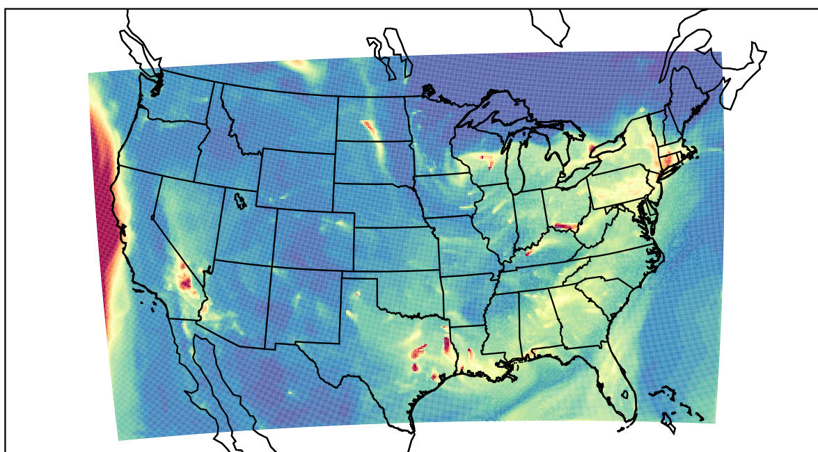
WRF 2023-01-05_09:00:00
