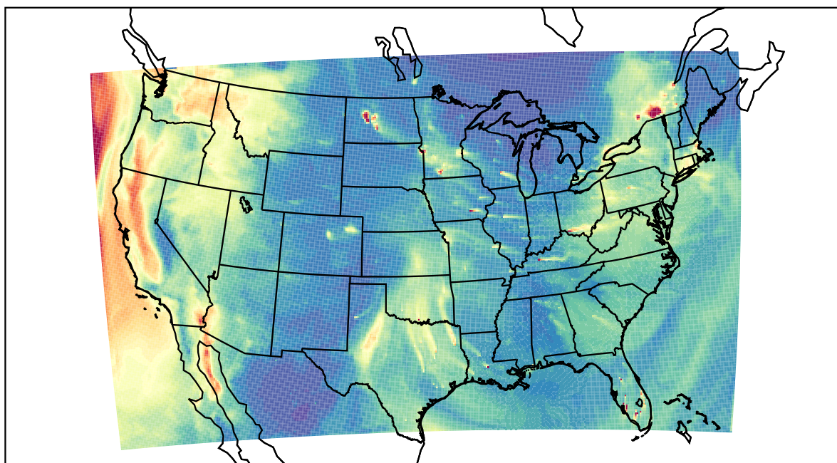
WRF 2023-01-06_21:00:00
