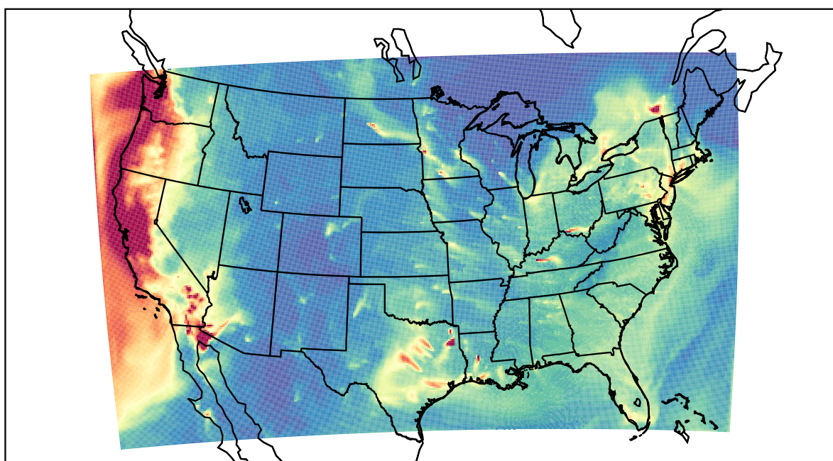
WRF 2023-01-06_07:00:00
