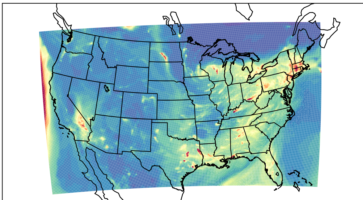
WRF 2023-01-05_04:00:00
