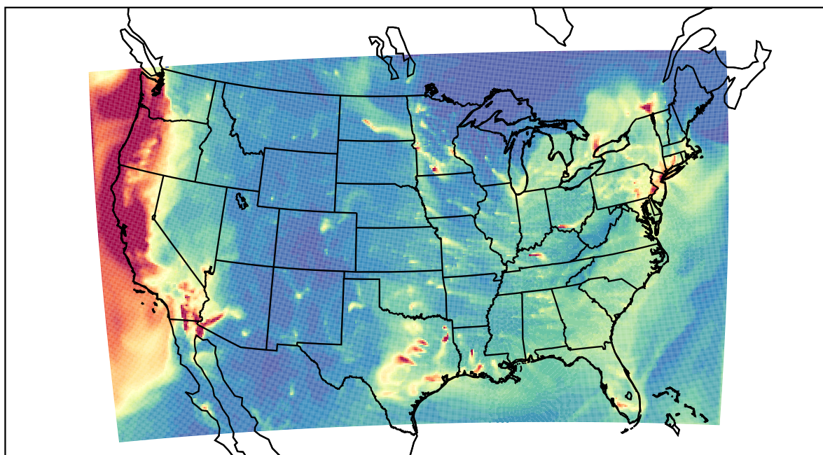
WRF 2023-01-06_05:00:00
