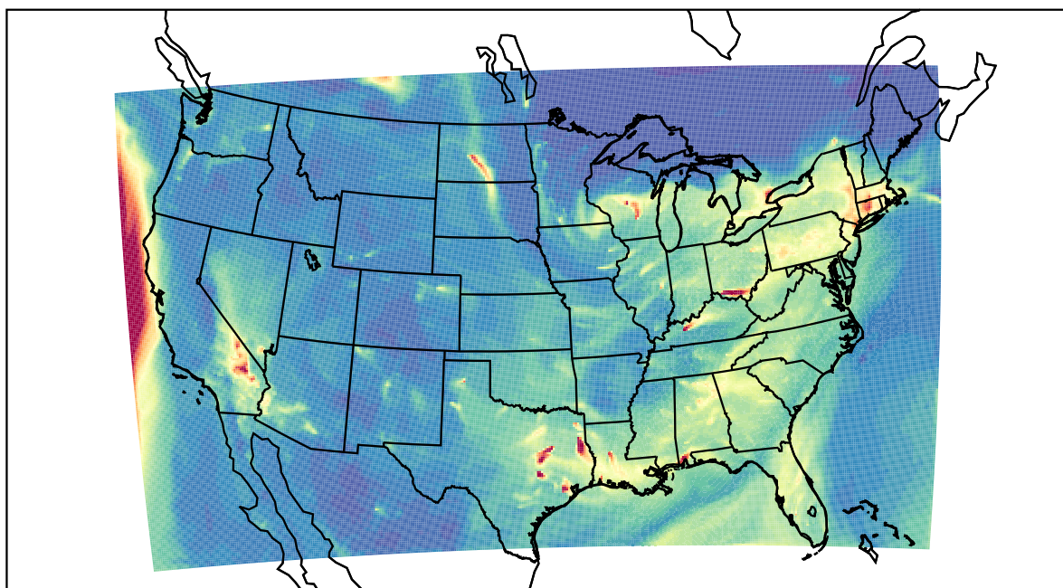
WRF 2023-01-05_07:00:00
