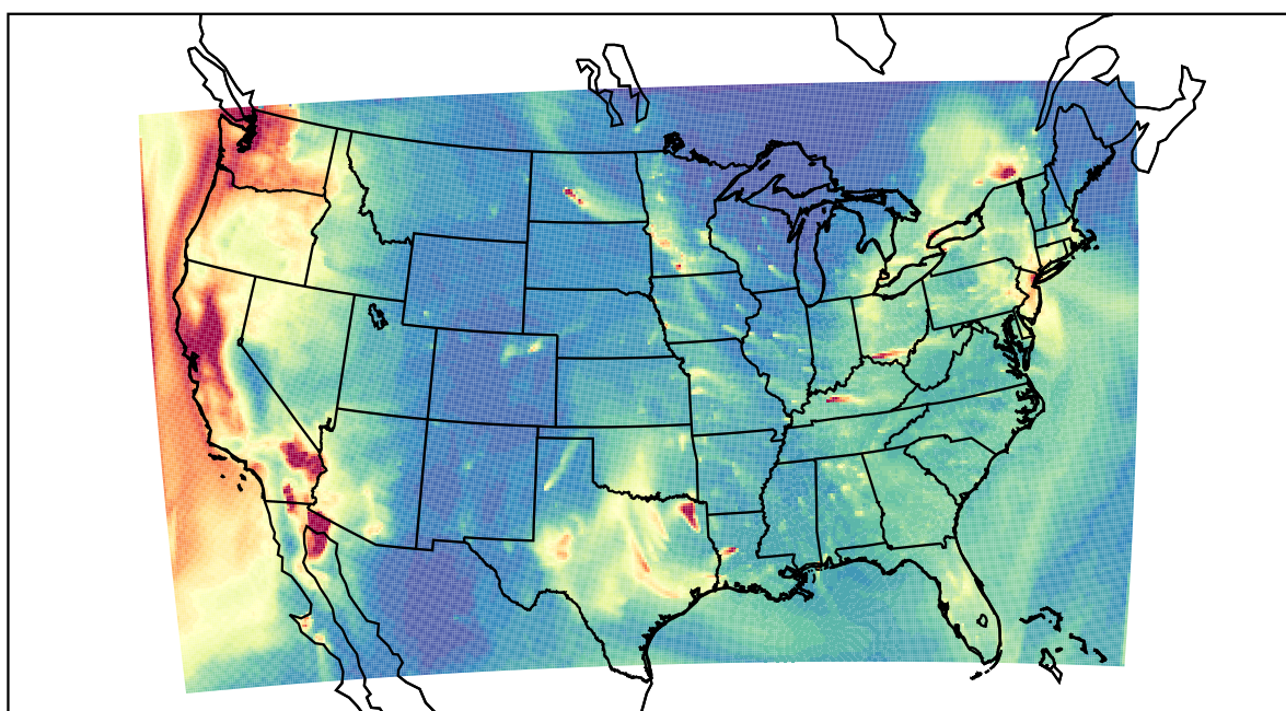
WRF 2023-01-06_13:00:00
