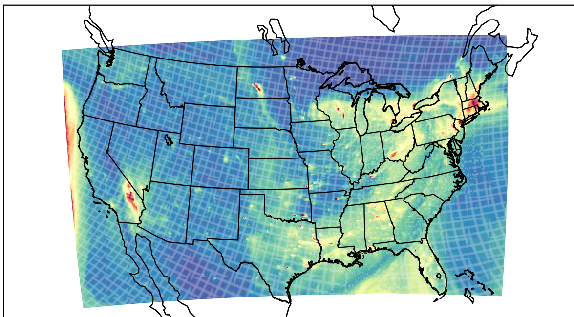
WRF 2023-01-05_00:00:00
