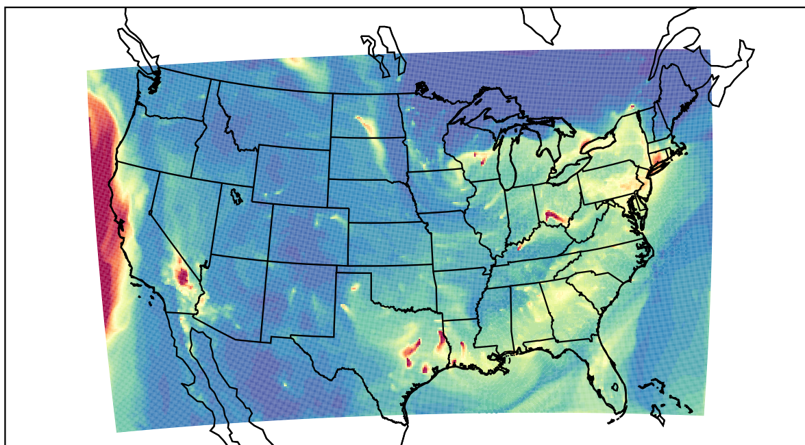
WRF 2023-01-05_12:00:00
