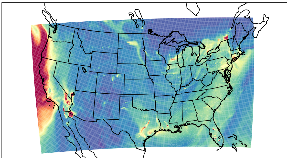
WRF 2023-01-05_21:00:00
