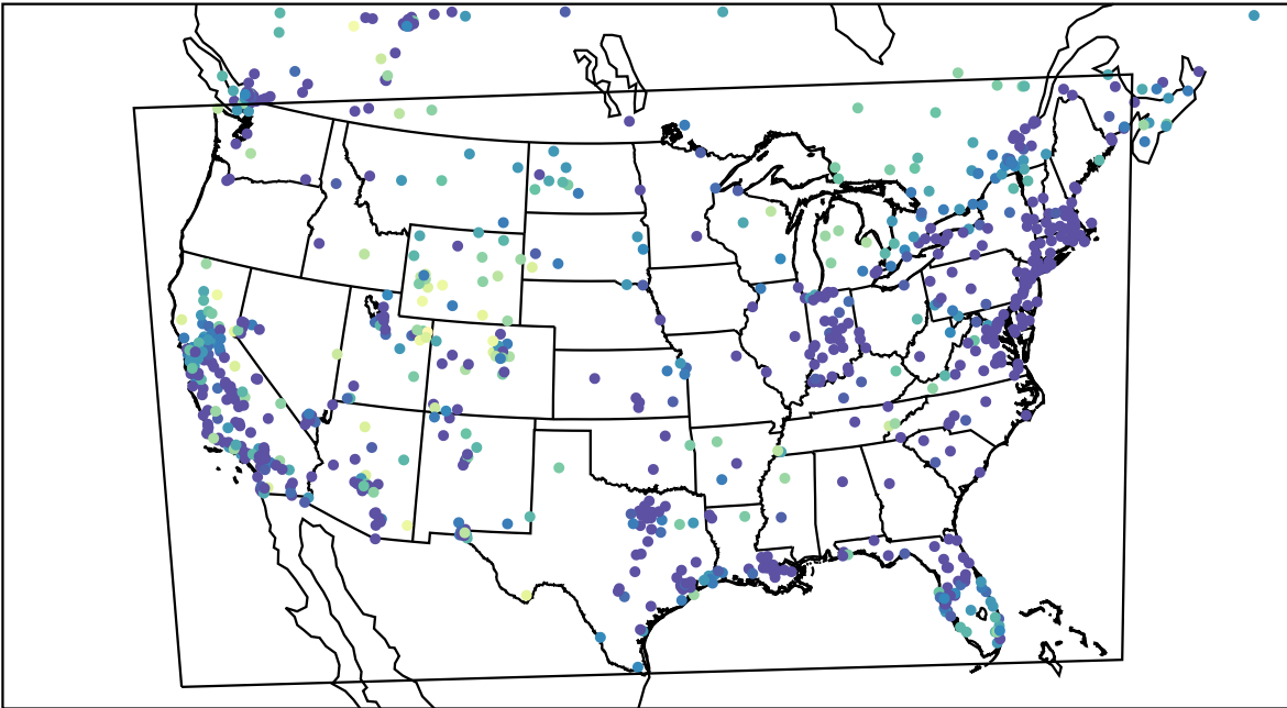
AirNOW (2023-01-07_13:00:00)
