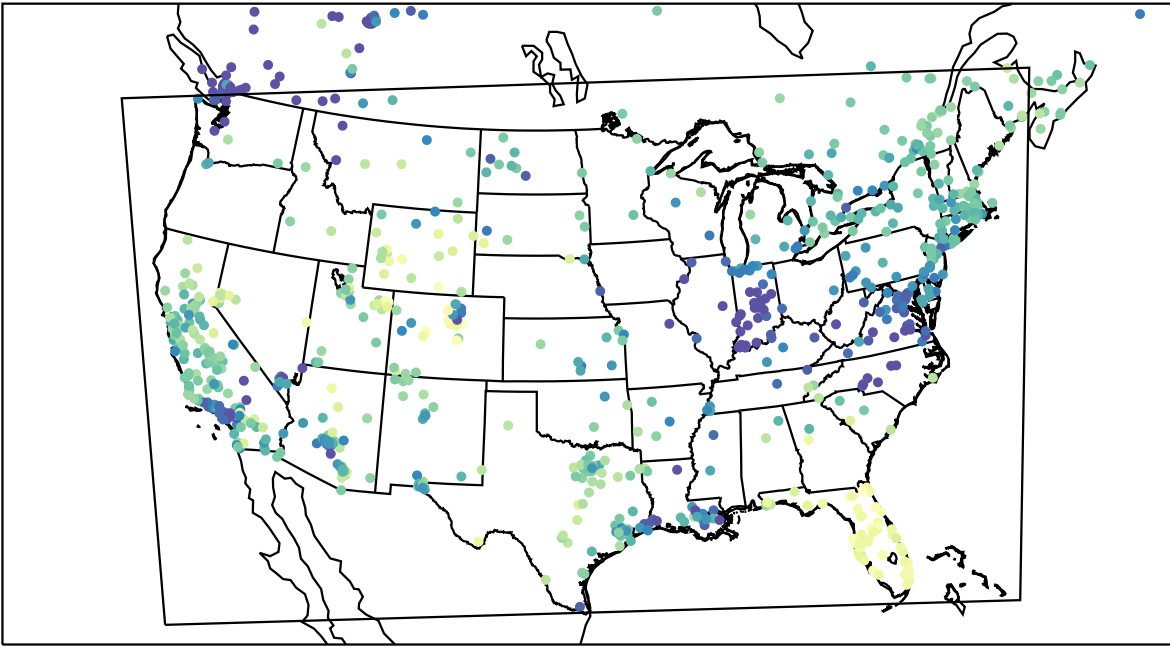
AirNOW (2023-01-08_18:00:00)
