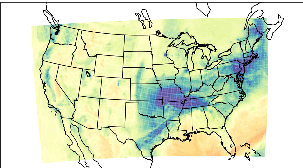
WRF (2023-01-07_21:00:00)
