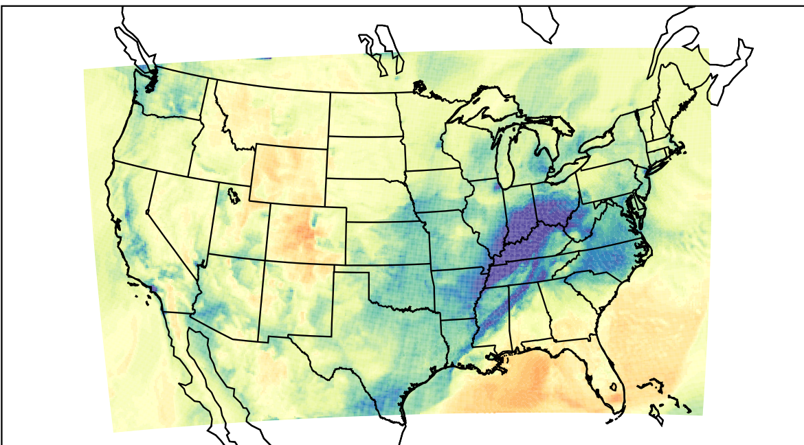
WRF (2023-01-08_19:00:00)
