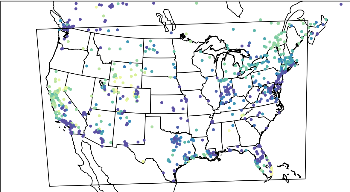
AirNOW (2023-01-08_06:00:00)
