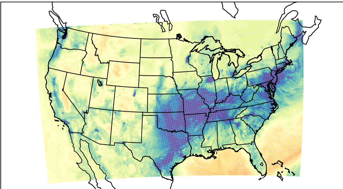
WRF (2023-01-08_01:00:00)
