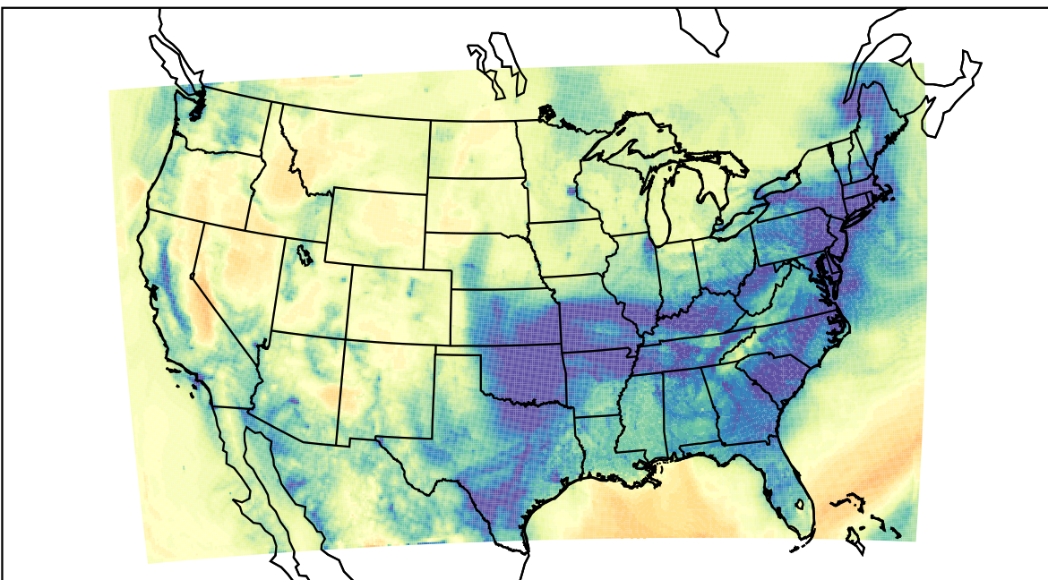
WRF (2023-01-07_15:00:00)
