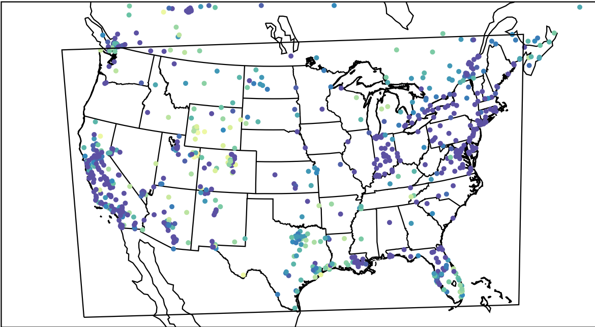
AirNOW (2023-01-07_08:00:00)
