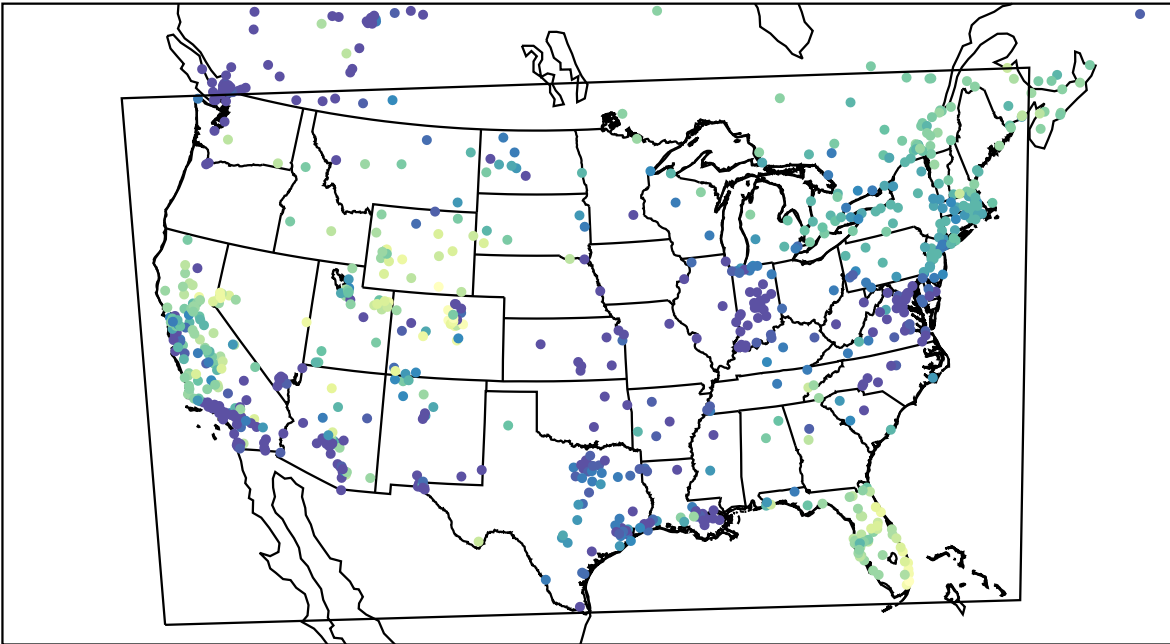
AirNOW (2023-01-08_15:00:00)
