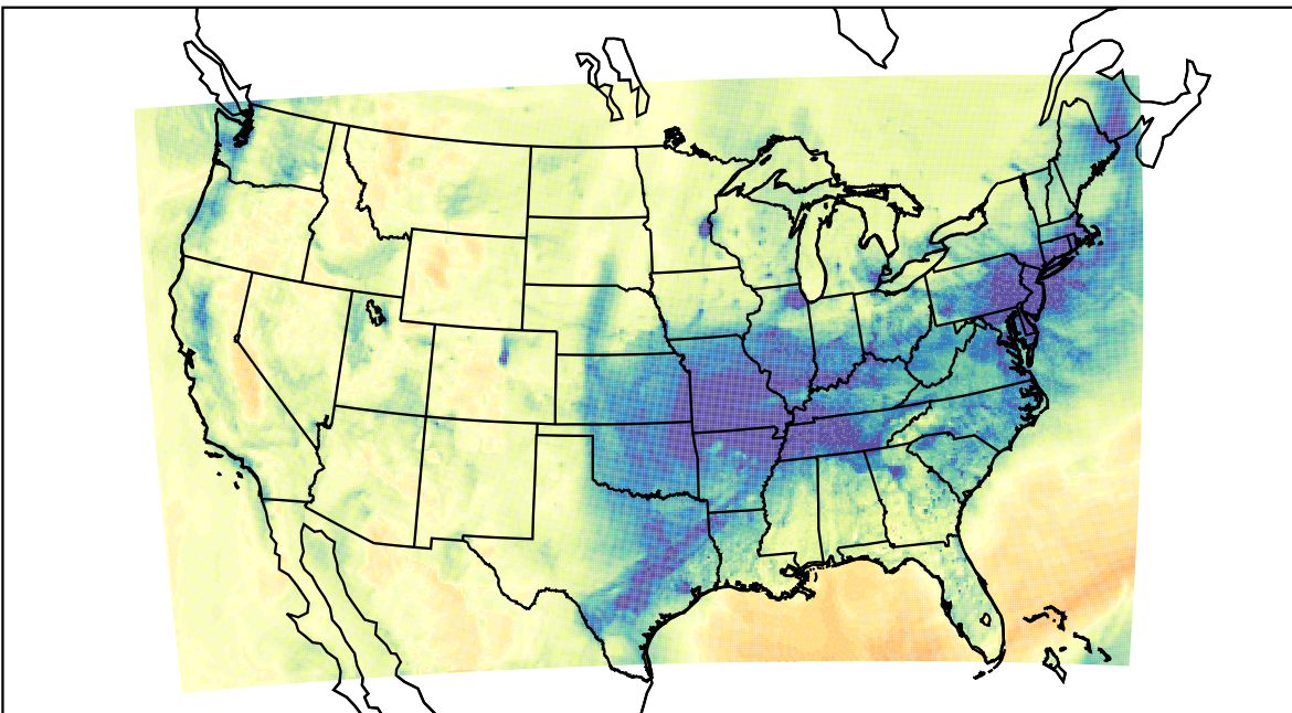
WRF (2023-01-07_23:00:00)
