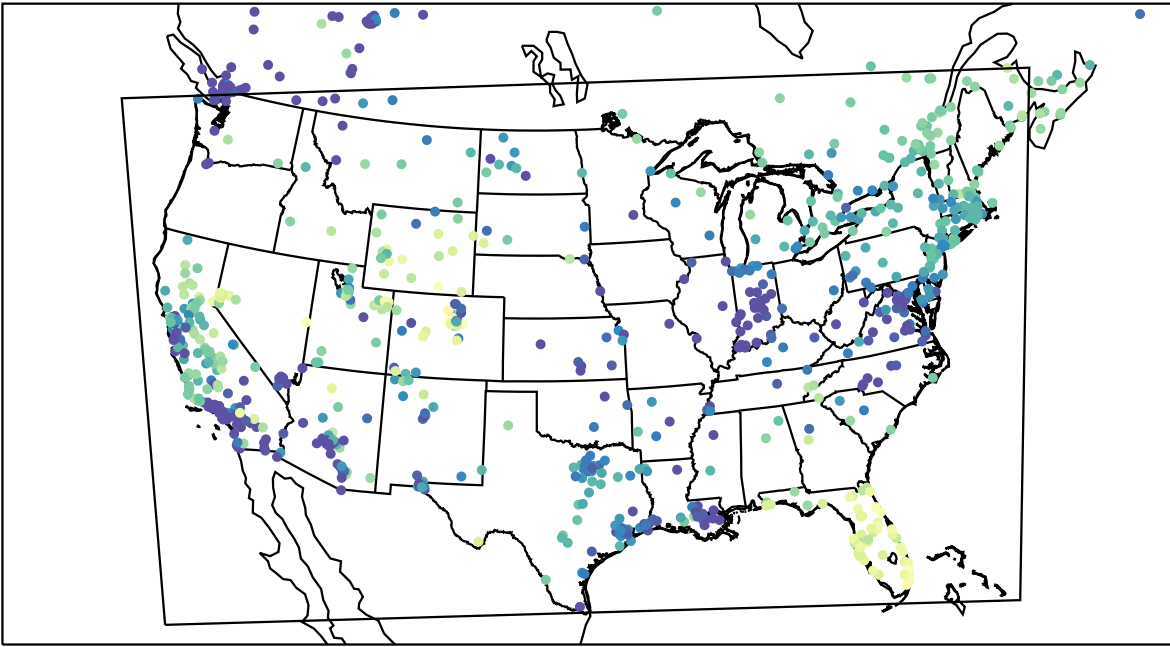
AirNOW (2023-01-08_16:00:00)
