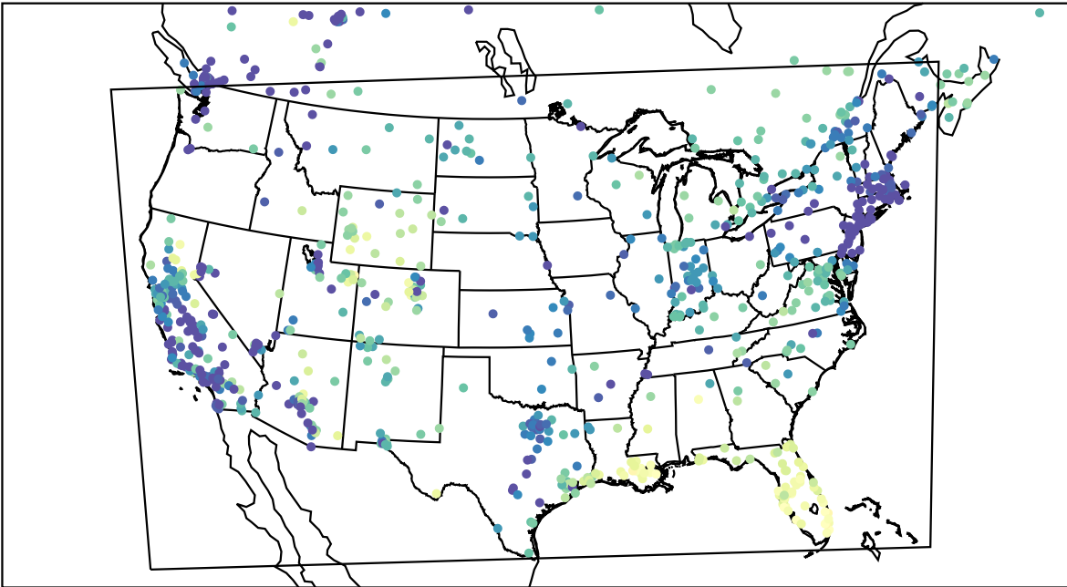
AirNOW (2023-01-07_17:00:00)
