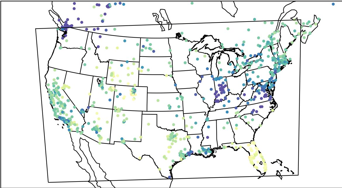
AirNOW (2023-01-08_19:00:00)
