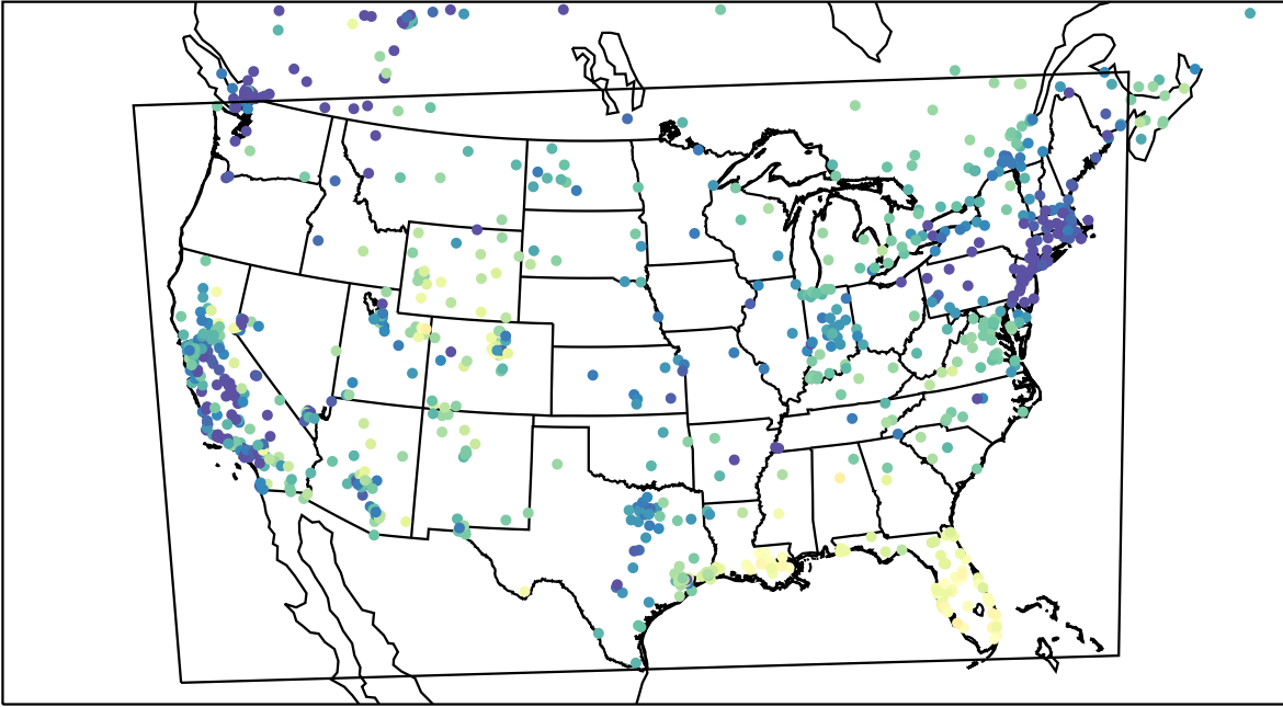
AirNOW (2023-01-07_18:00:00)
