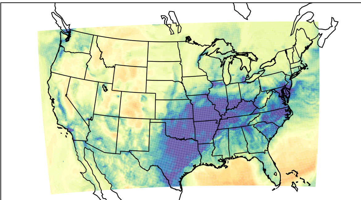
WRF (2023-01-08_06:00:00)
