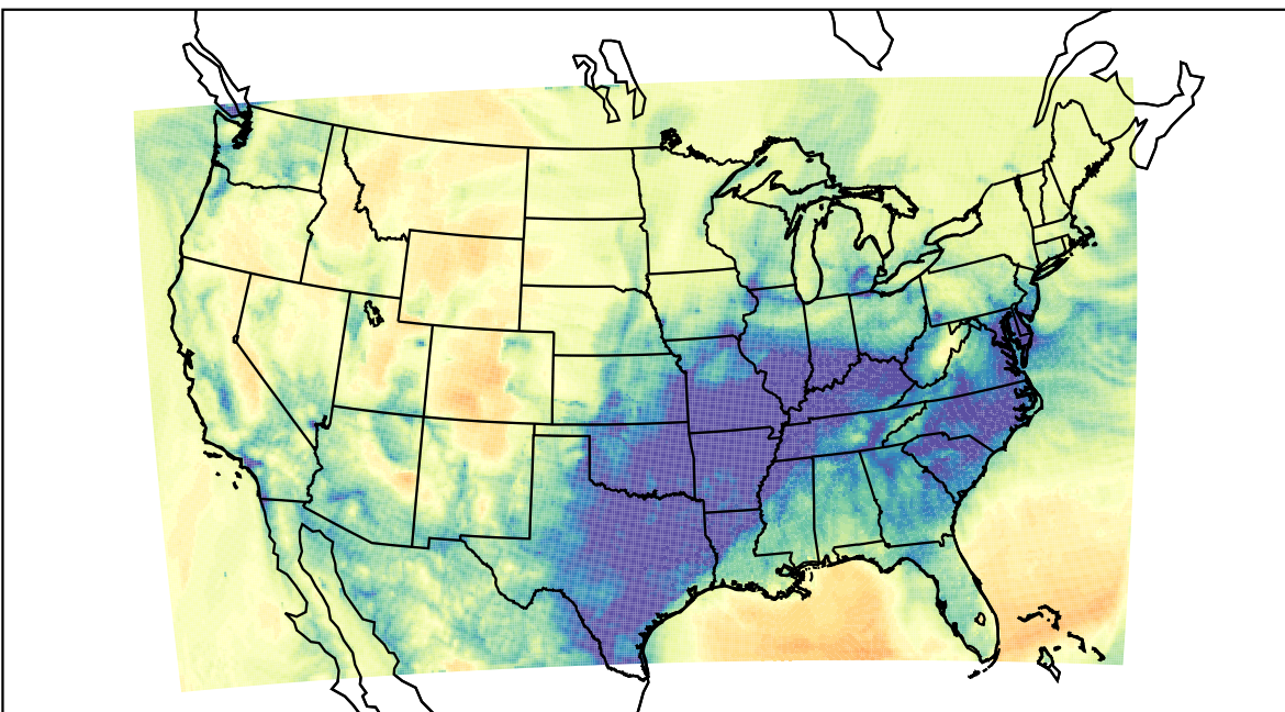
WRF (2023-01-08_09:00:00)
