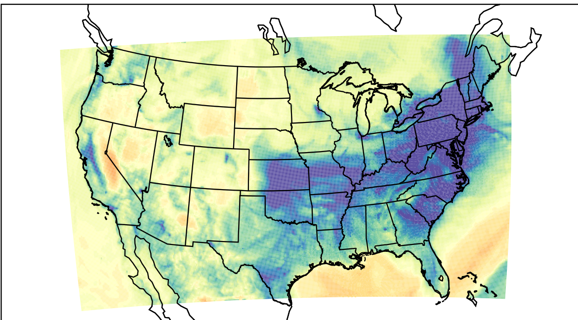
WRF (2023-01-07_07:00:00)
