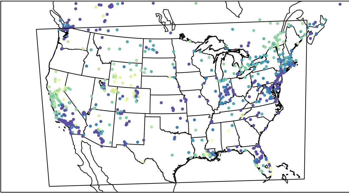
AirNOW (2023-01-08_04:00:00)
