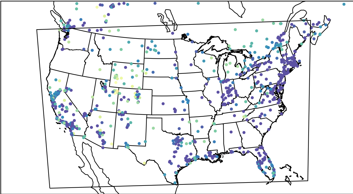
AirNOW (2023-01-07_12:00:00)
