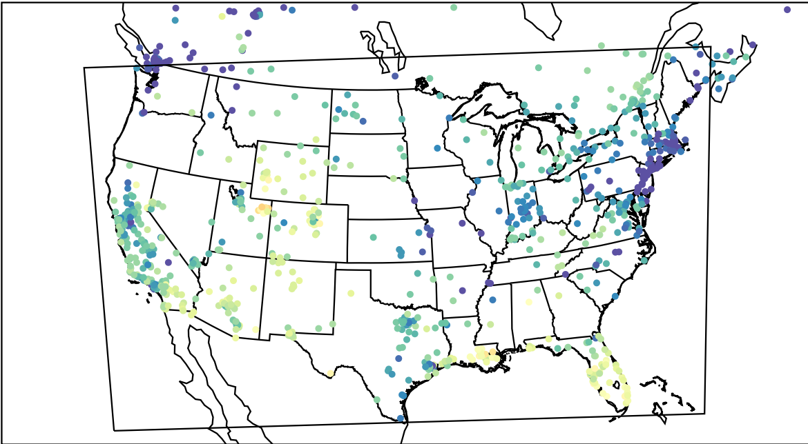
AirNOW (2023-01-07_22:00:00)
