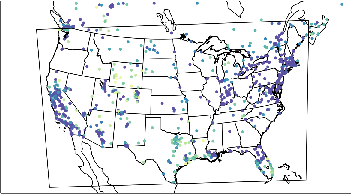
AirNOW (2023-01-07_06:00:00)
