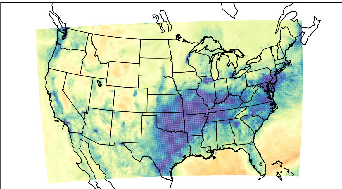
WRF (2023-01-08_03:00:00)
