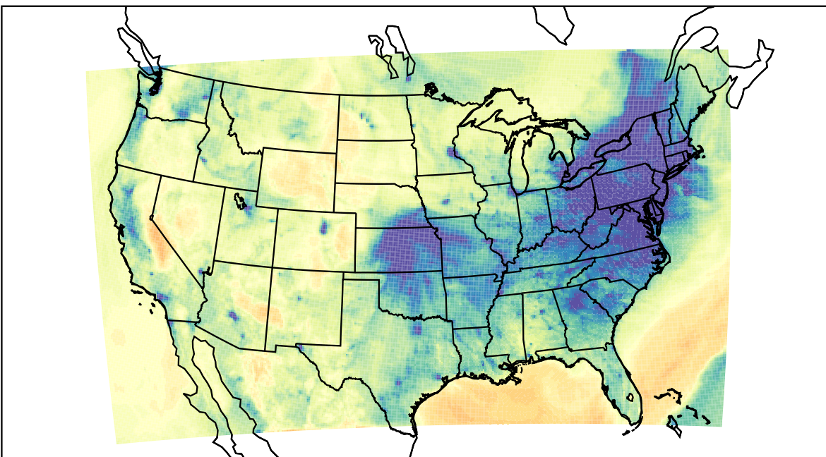
WRF (2023-01-07_01:00:00)
