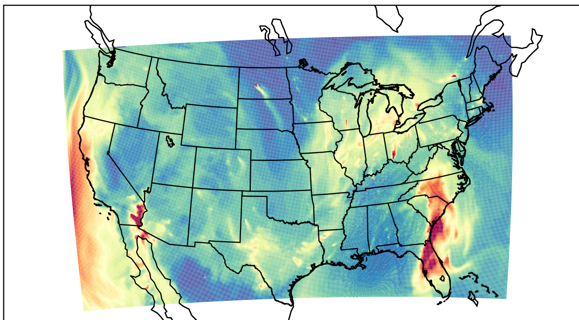
WRF 2023-01-12_11:00:00
