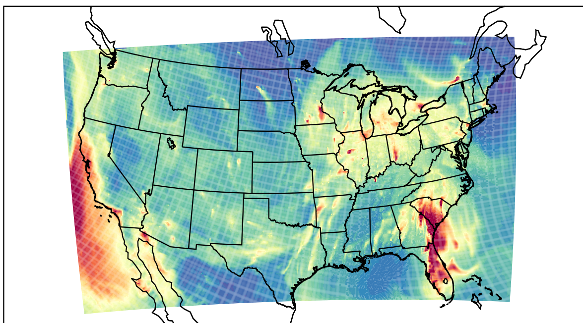
WRF 2023-01-12_04:00:00
