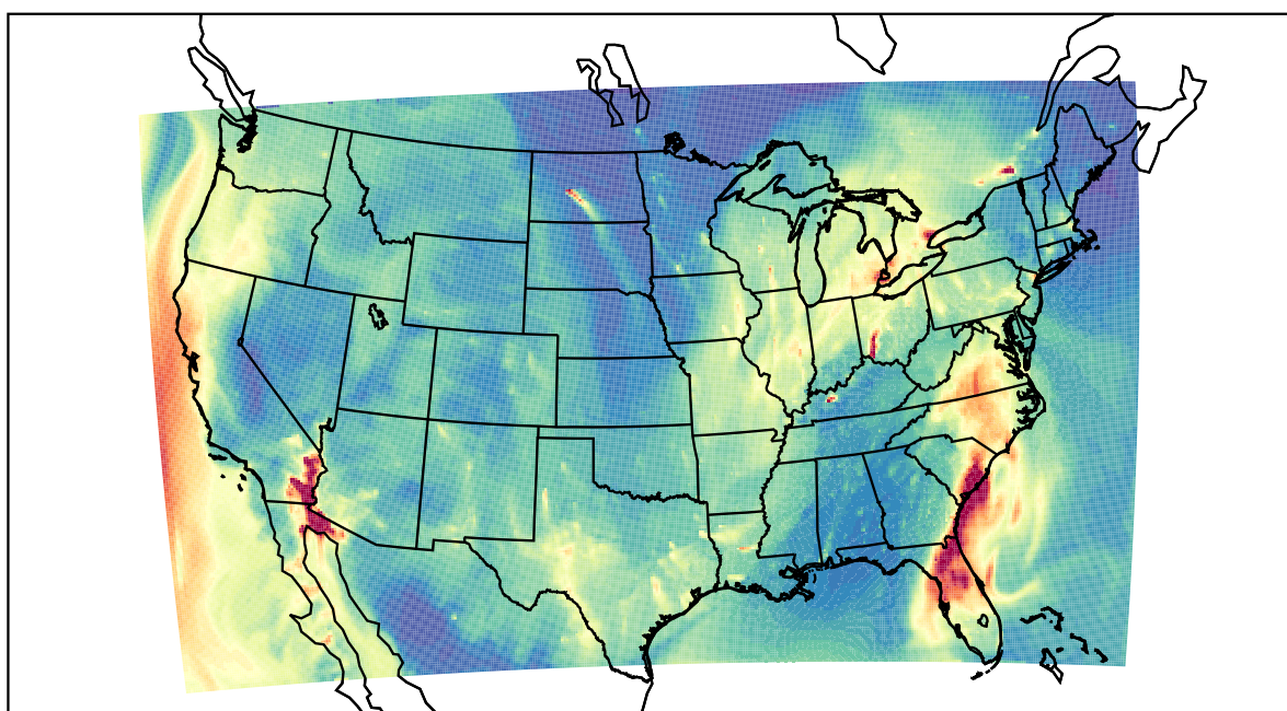
WRF 2023-01-12_14:00:00
