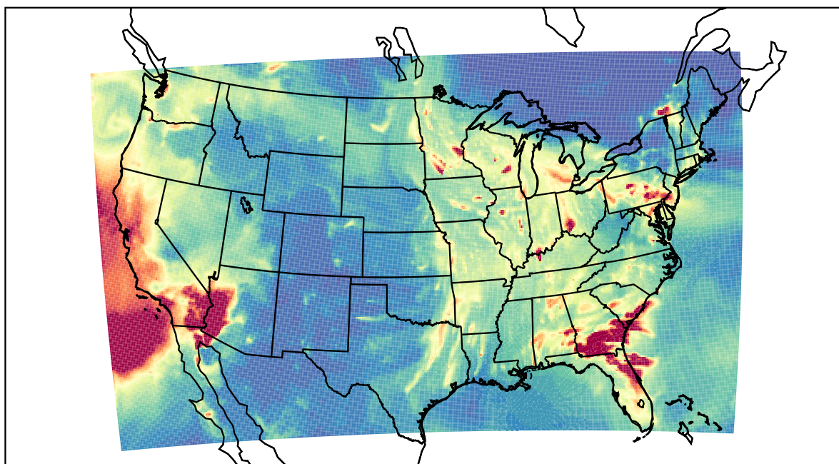
WRF 2023-01-11_05:00:00
