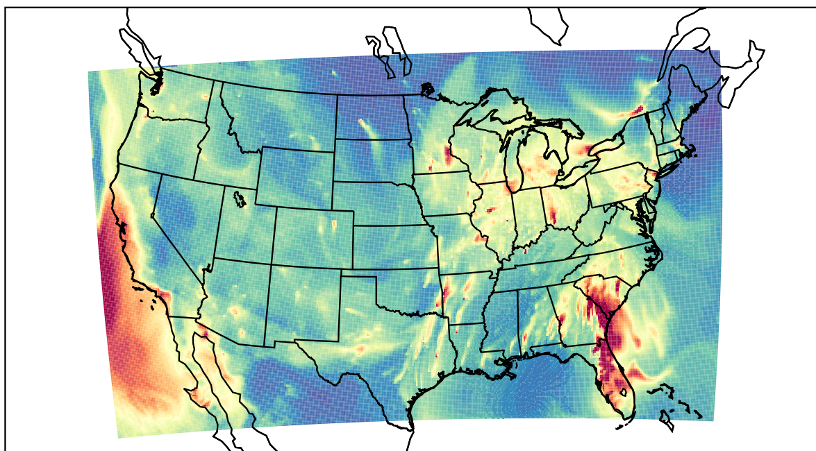
WRF 2023-01-12_03:00:00
