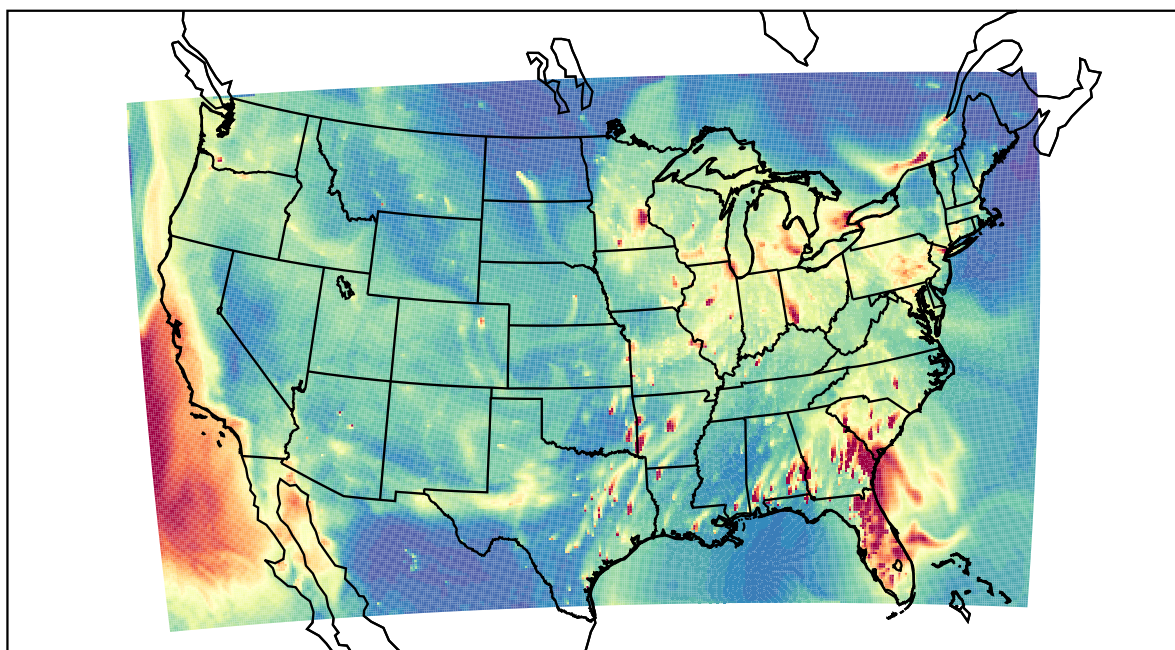
WRF 2023-01-12_00:00:00
