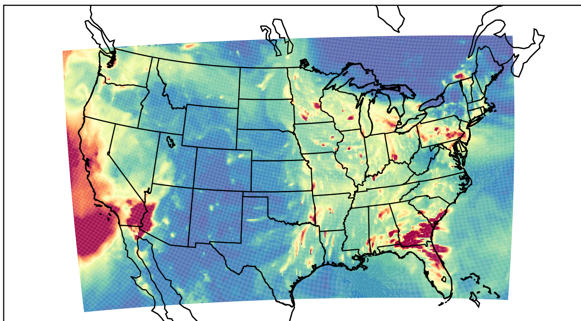
WRF 2023-01-11_03:00:00
