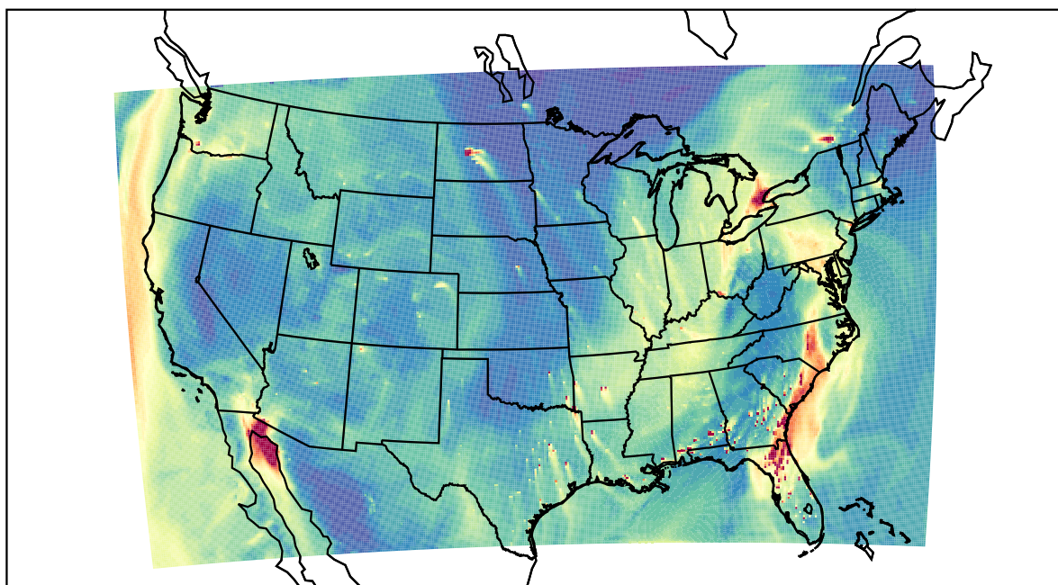
WRF 2023-01-12_22:00:00
