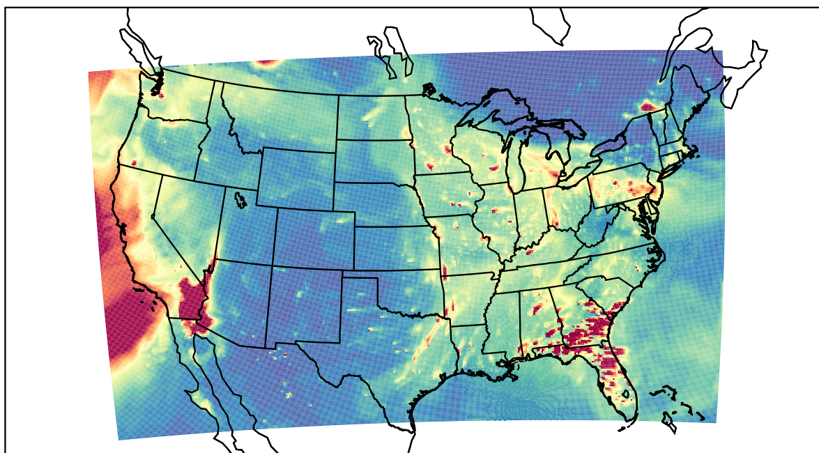
WRF 2023-01-11_00:00:00
