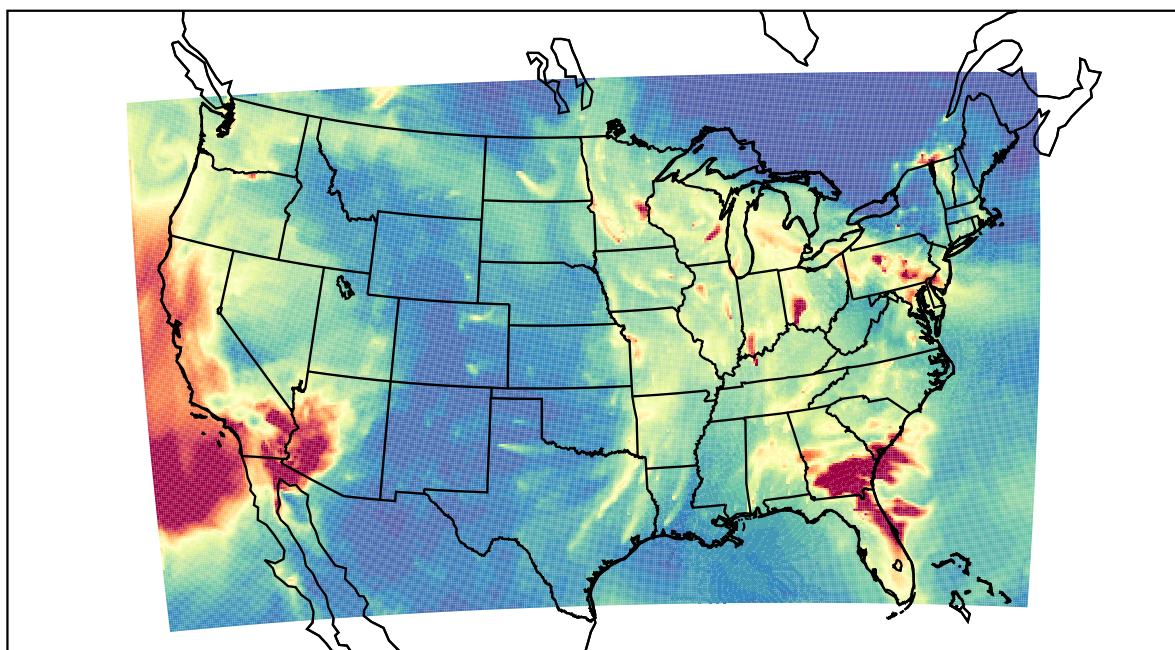
WRF 2023-01-11_08:00:00
