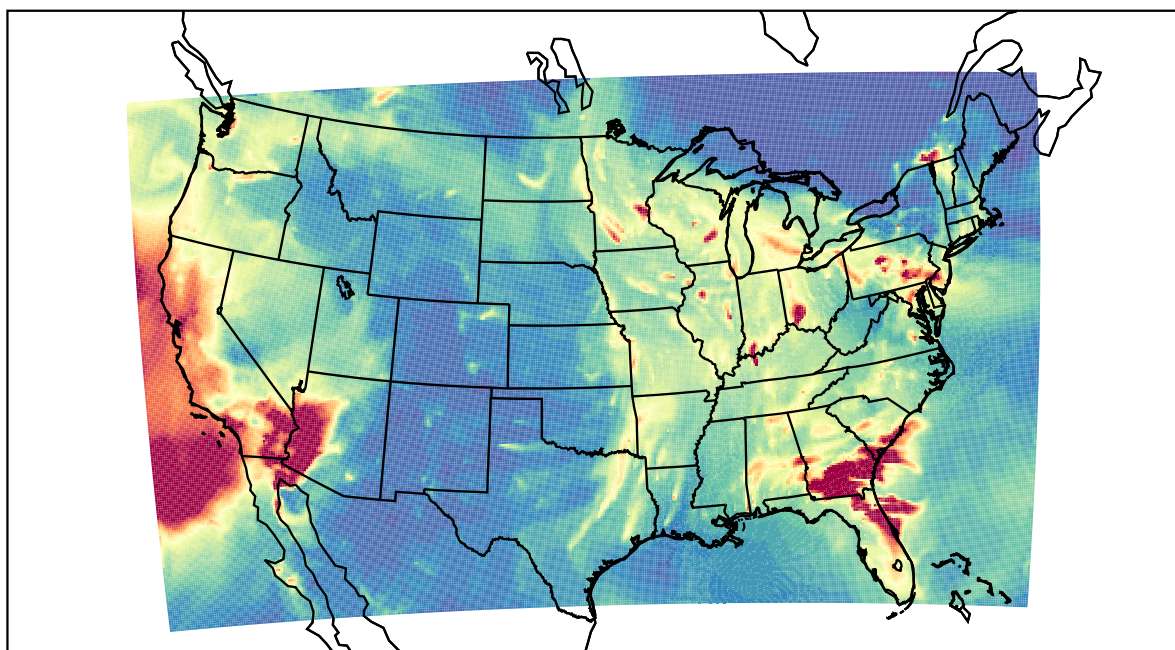
WRF 2023-01-11_06:00:00
