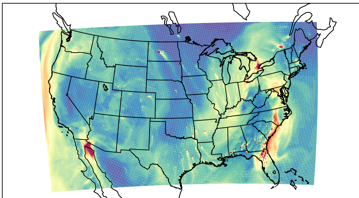
WRF 2023-01-12_21:00:00
