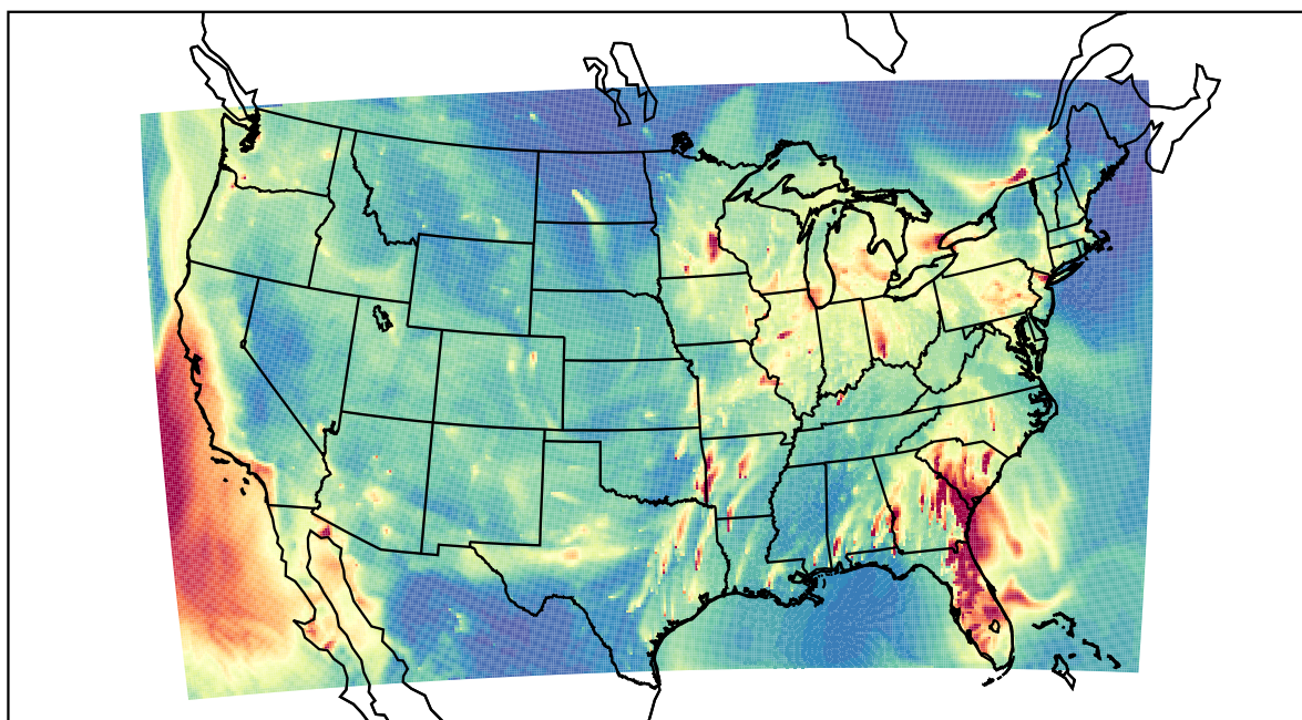
WRF 2023-01-12_02:00:00
