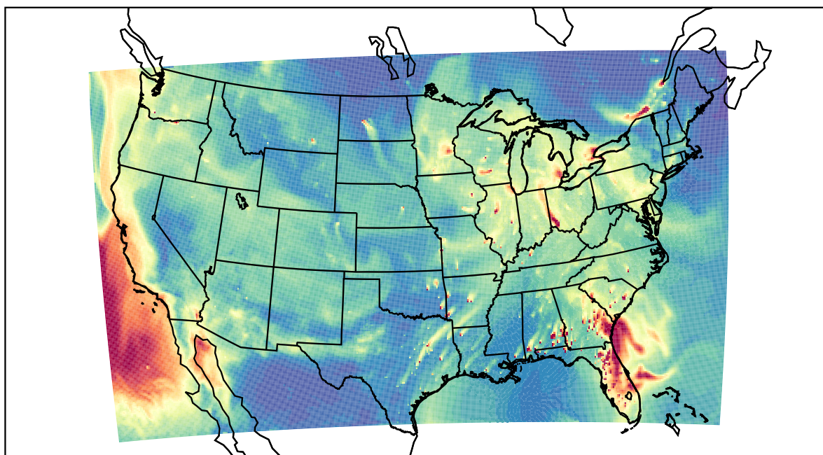
WRF 2023-01-11_21:00:00
