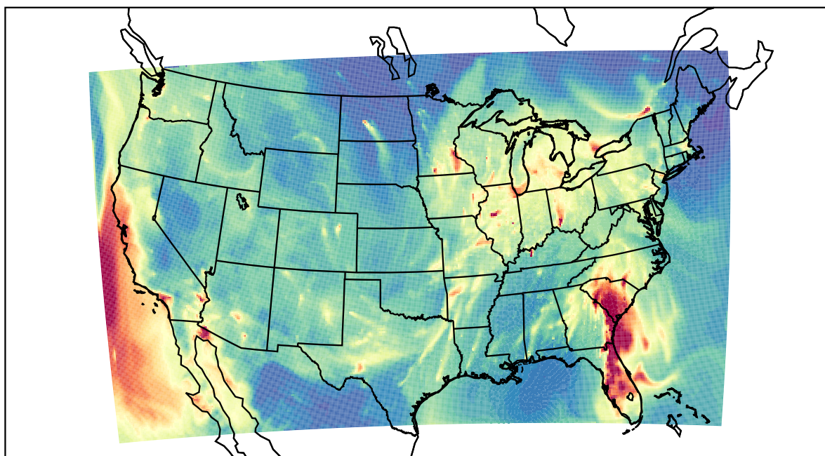
WRF 2023-01-12_05:00:00
