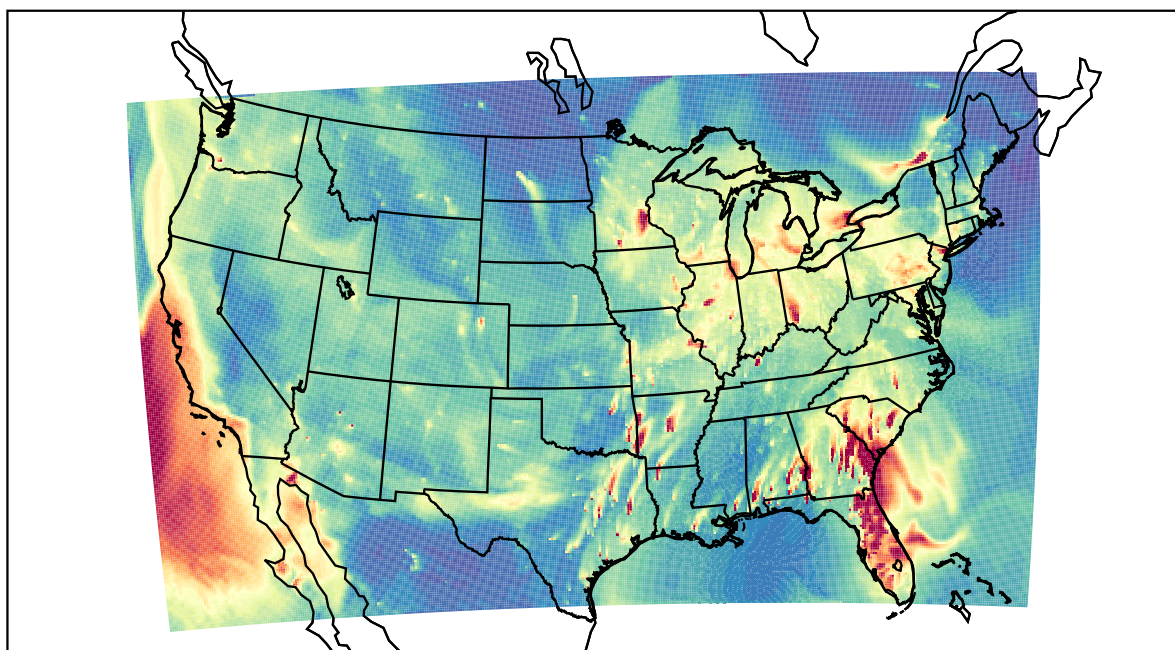
WRF 2023-01-12_01:00:00
