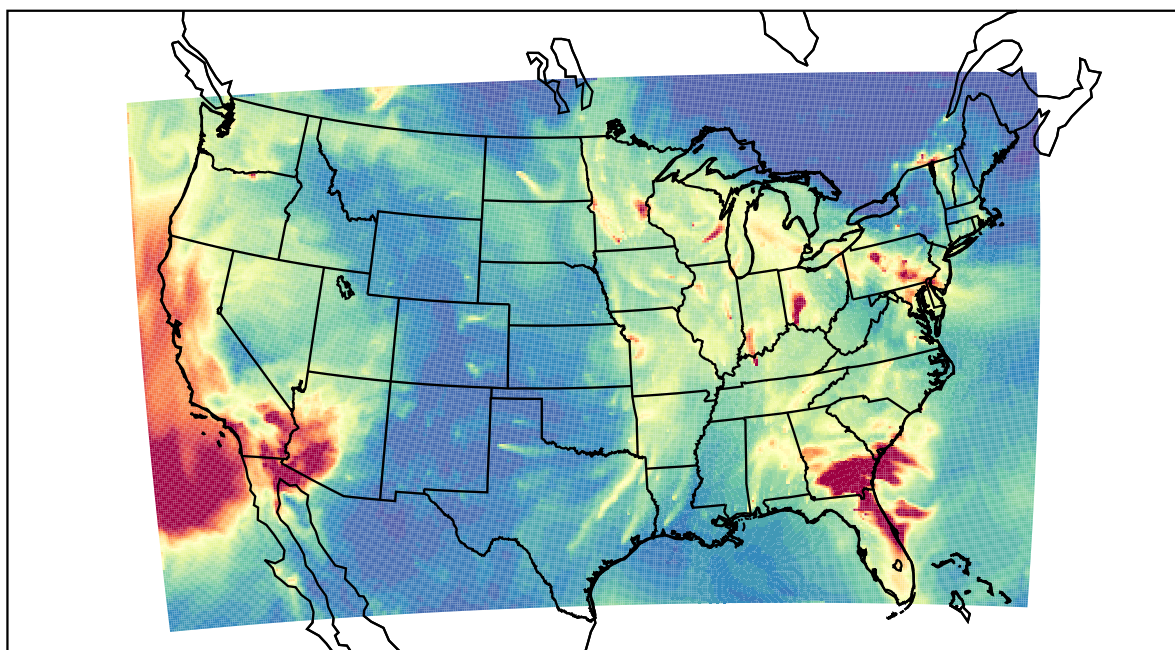
WRF 2023-01-11_09:00:00
