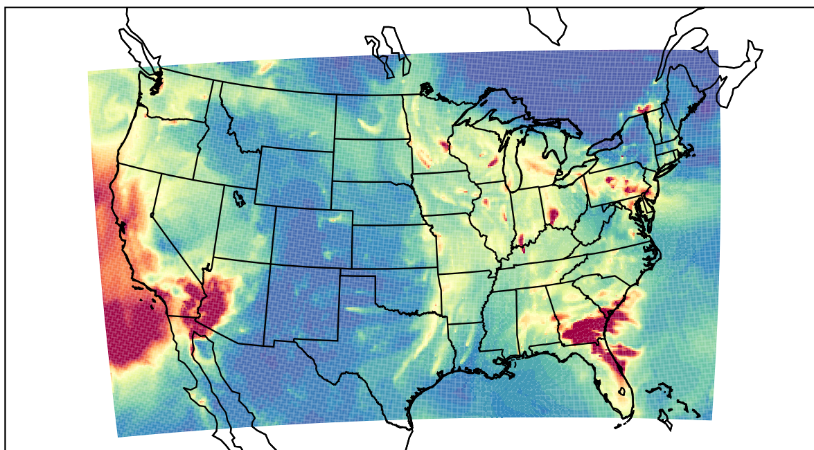
WRF 2023-01-11_07:00:00
