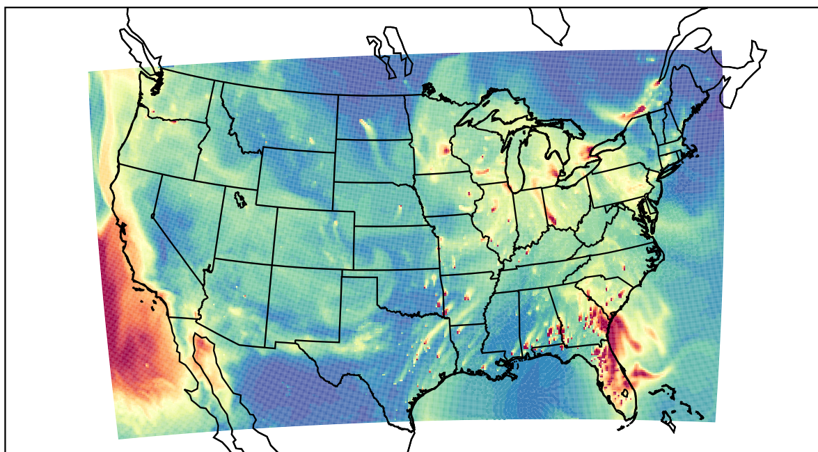
WRF 2023-01-11_22:00:00
