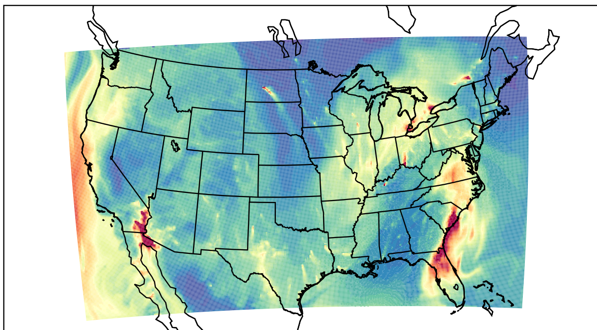
WRF 2023-01-12_15:00:00
