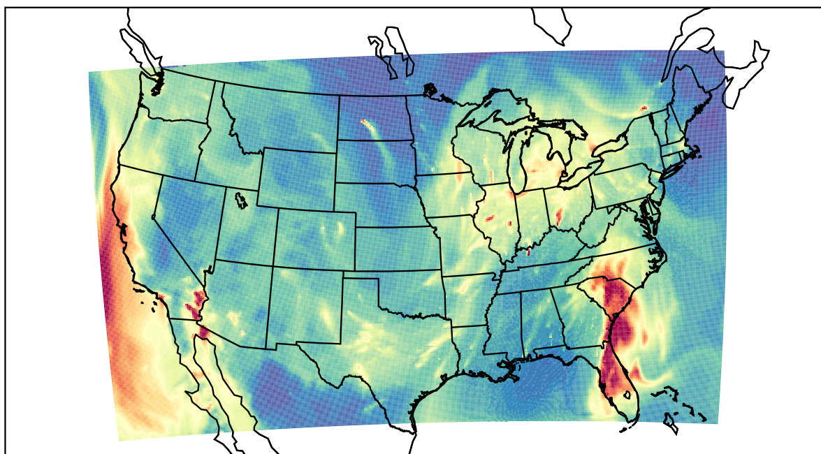
WRF 2023-01-12_08:00:00
