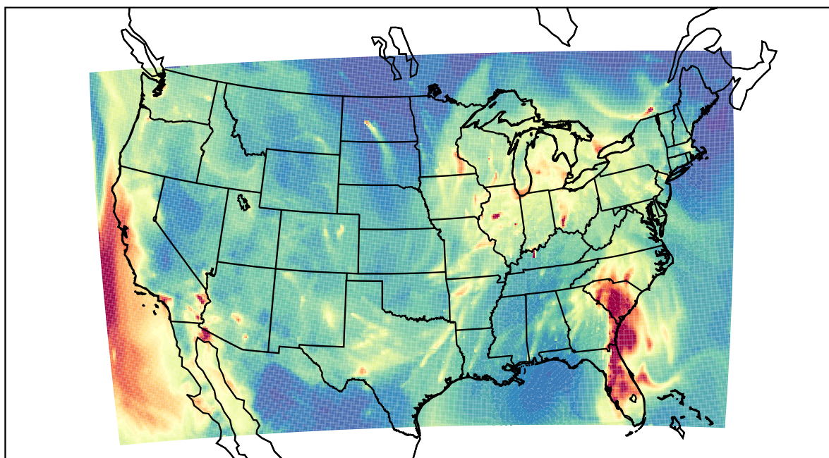
WRF 2023-01-12_06:00:00
