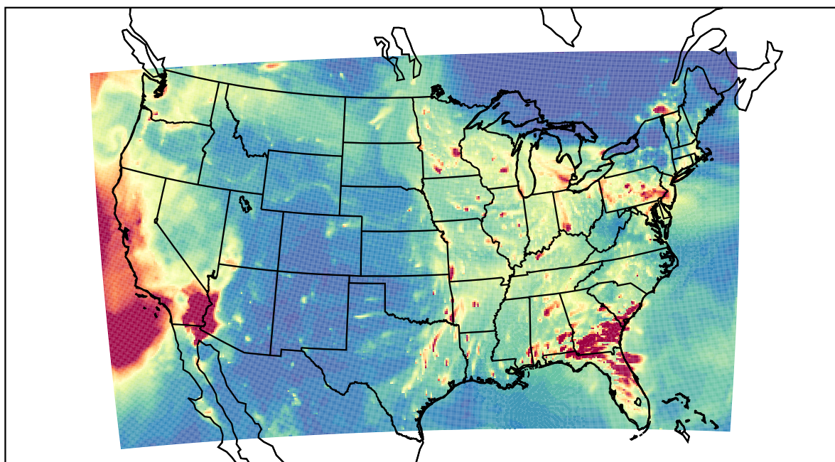
WRF 2023-01-11_02:00:00
