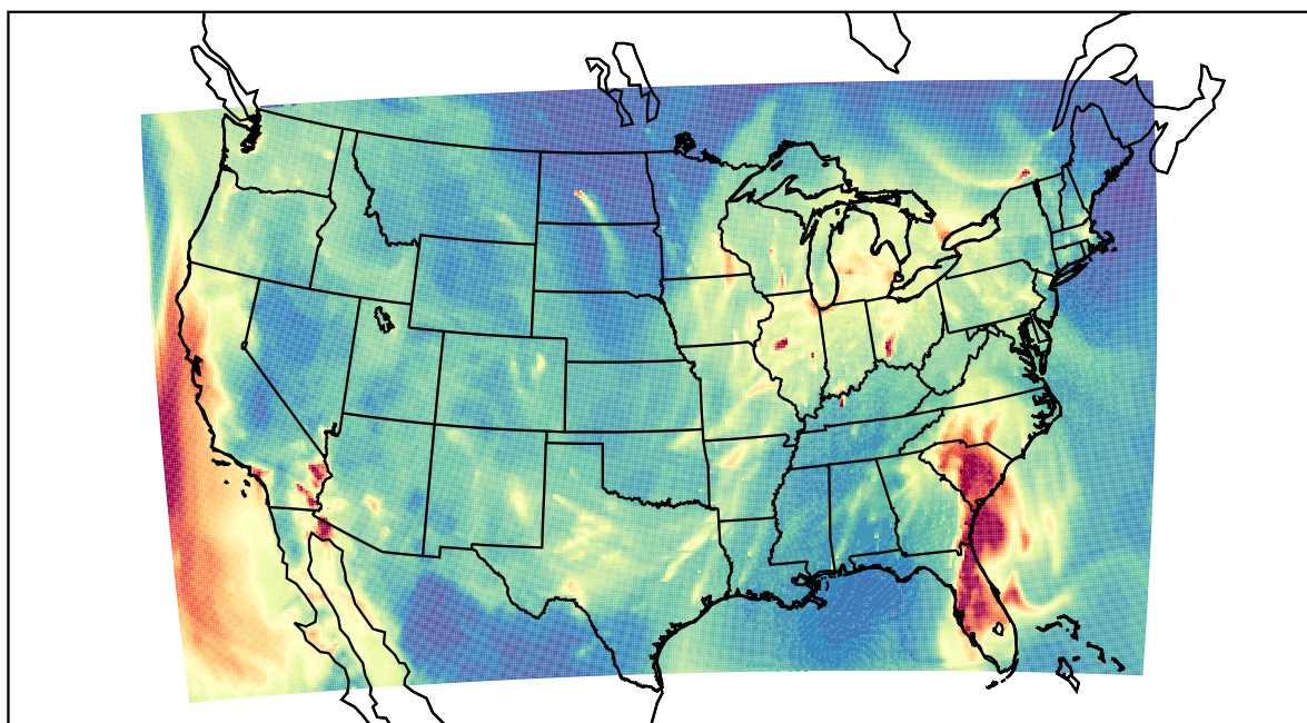
WRF 2023-01-12_07:00:00
