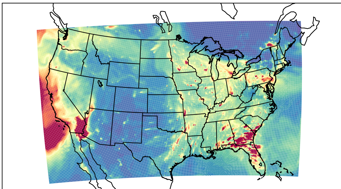
WRF 2023-01-11_01:00:00
