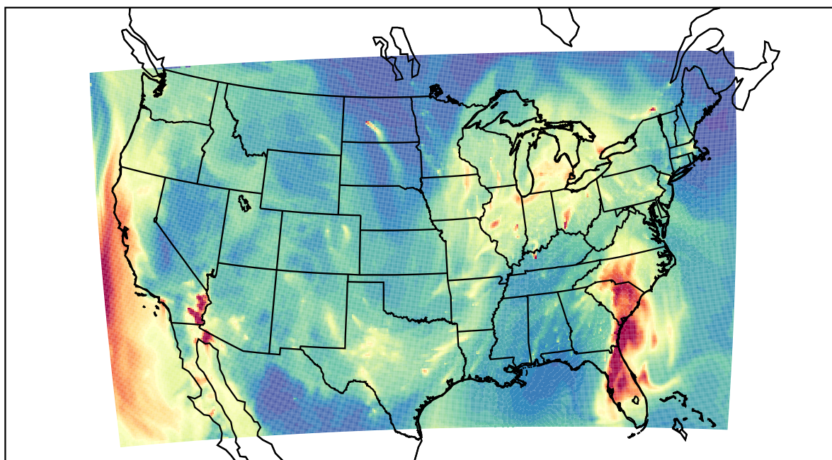
WRF 2023-01-12_09:00:00
