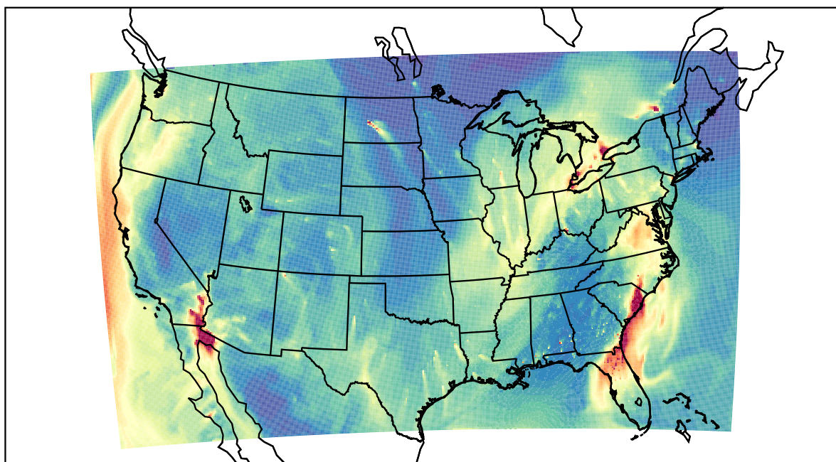
WRF 2023-01-12_17:00:00
