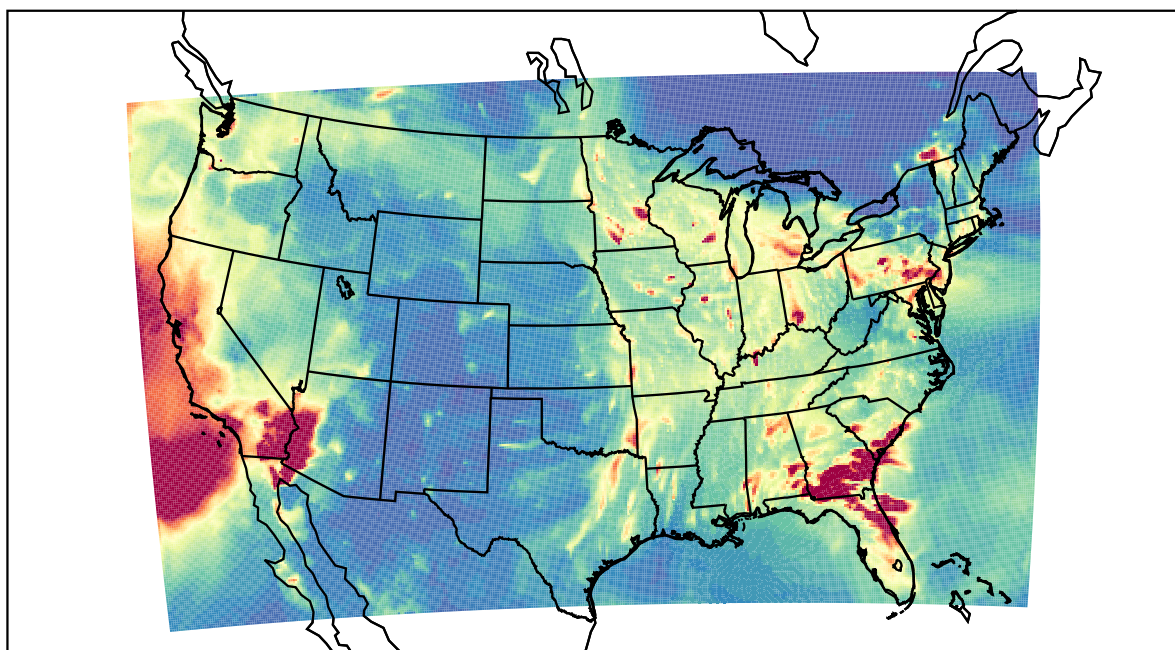
WRF 2023-01-11_04:00:00
