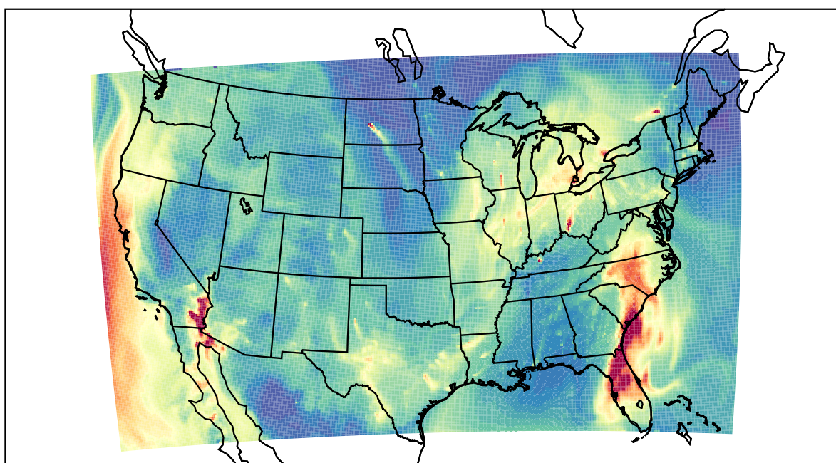
WRF 2023-01-12_12:00:00
