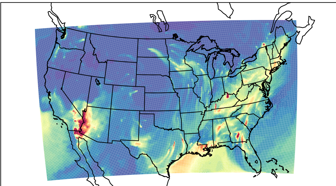
WRF 2023-01-30_07:00:00
