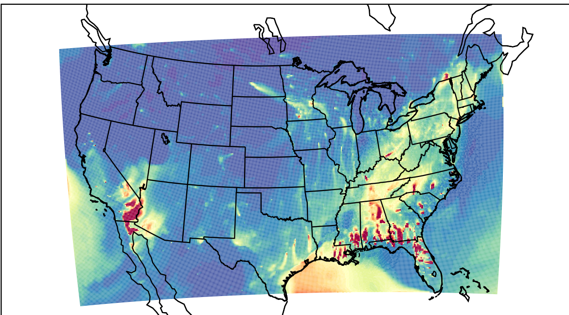
WRF 2023-01-30_00:00:00
