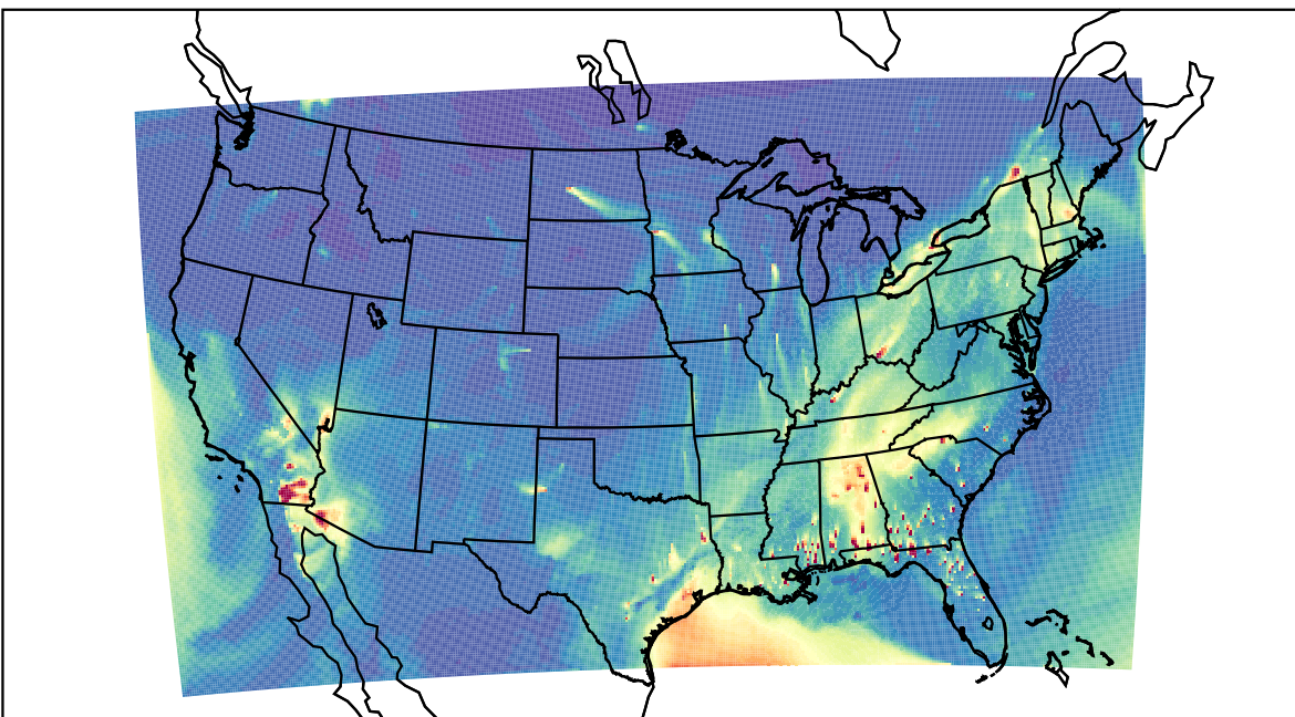
WRF 2023-01-29_19:00:00
