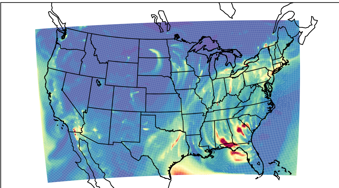
WRF 2023-01-29_07:00:00
