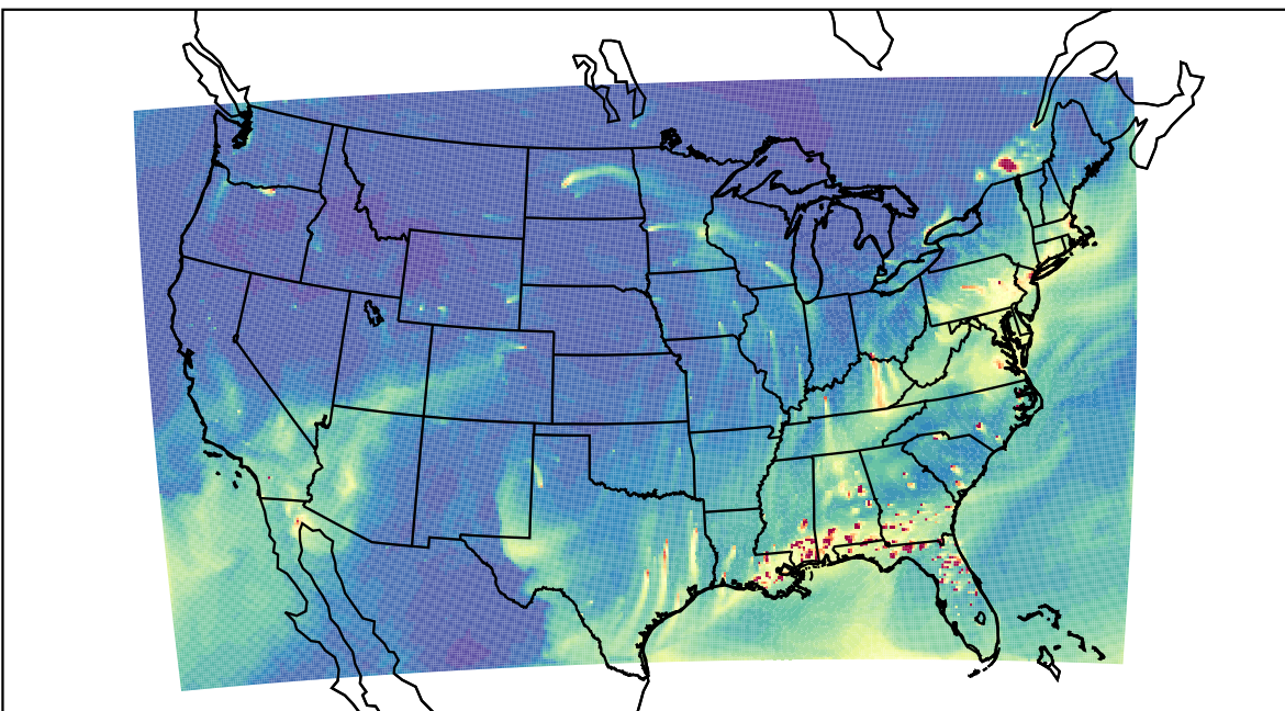
WRF 2023-01-30_21:00:00
