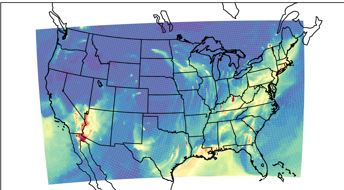
WRF 2023-01-30_09:00:00
