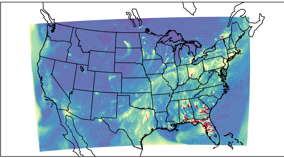
WRF 2023-01-29_00:00:00
