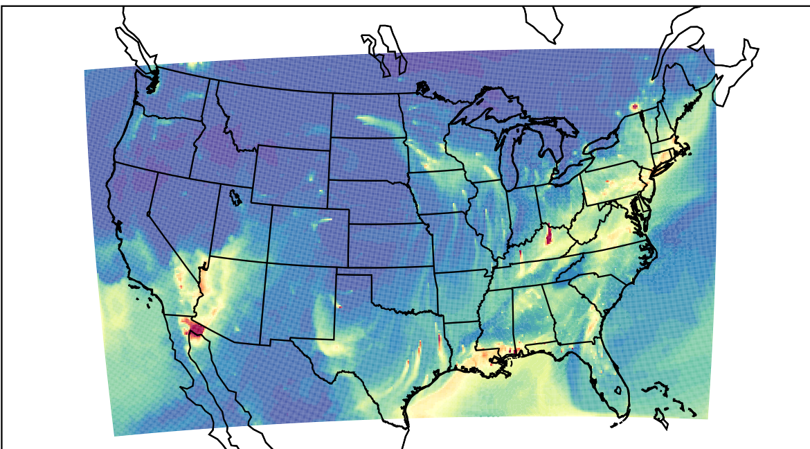
WRF 2023-01-30_11:00:00
