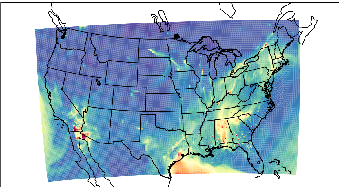
WRF 2023-01-29_17:00:00
