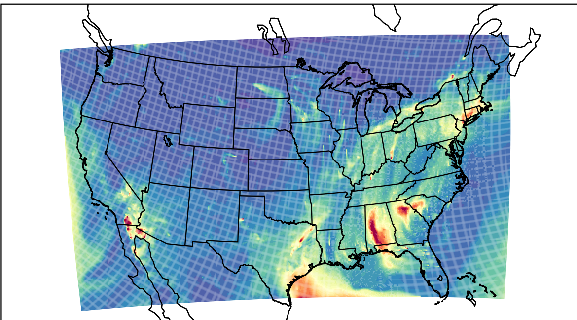
WRF 2023-01-29_12:00:00
