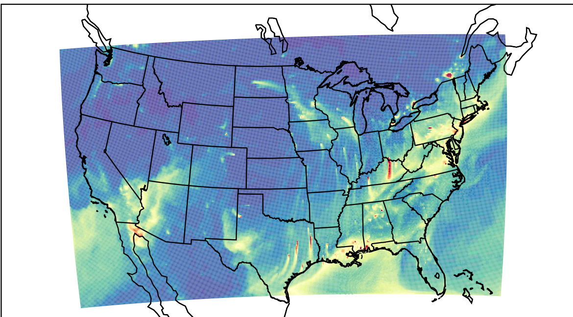
WRF 2023-01-30_15:00:00
