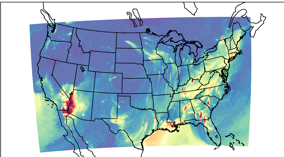
WRF 2023-01-30_06:00:00
