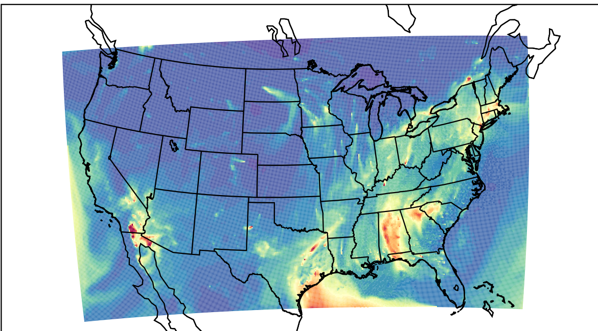
WRF 2023-01-29_14:00:00
