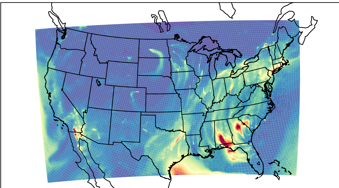
WRF 2023-01-29_09:00:00
