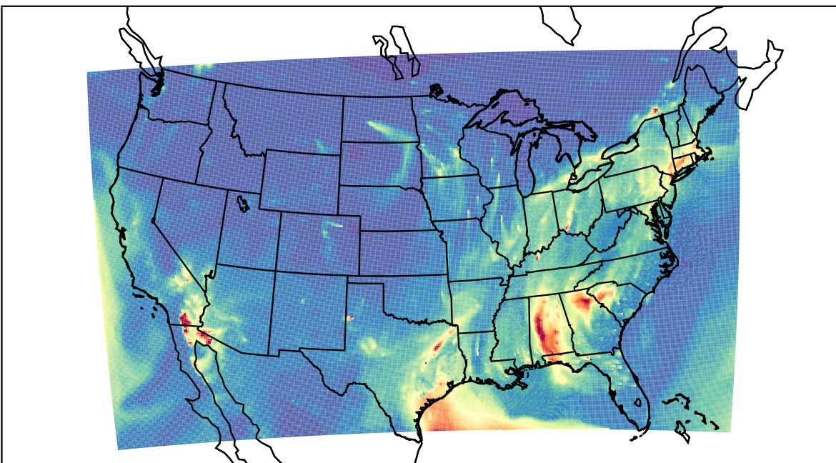
WRF 2023-01-29_13:00:00
