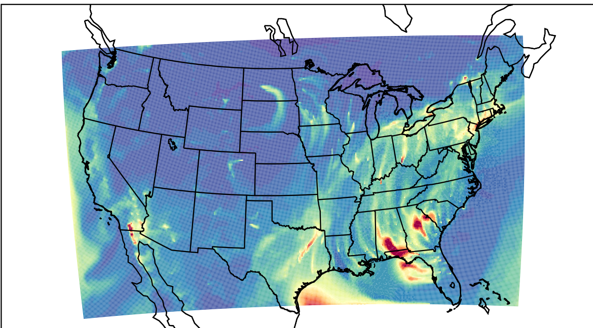
WRF 2023-01-29_08:00:00
