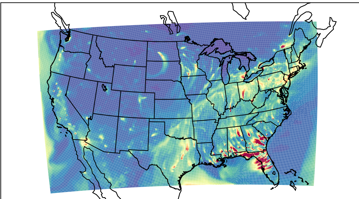
WRF 2023-01-29_02:00:00
