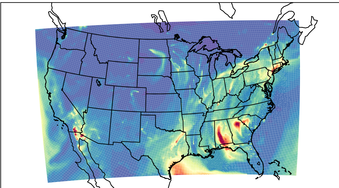
WRF 2023-01-29_11:00:00
