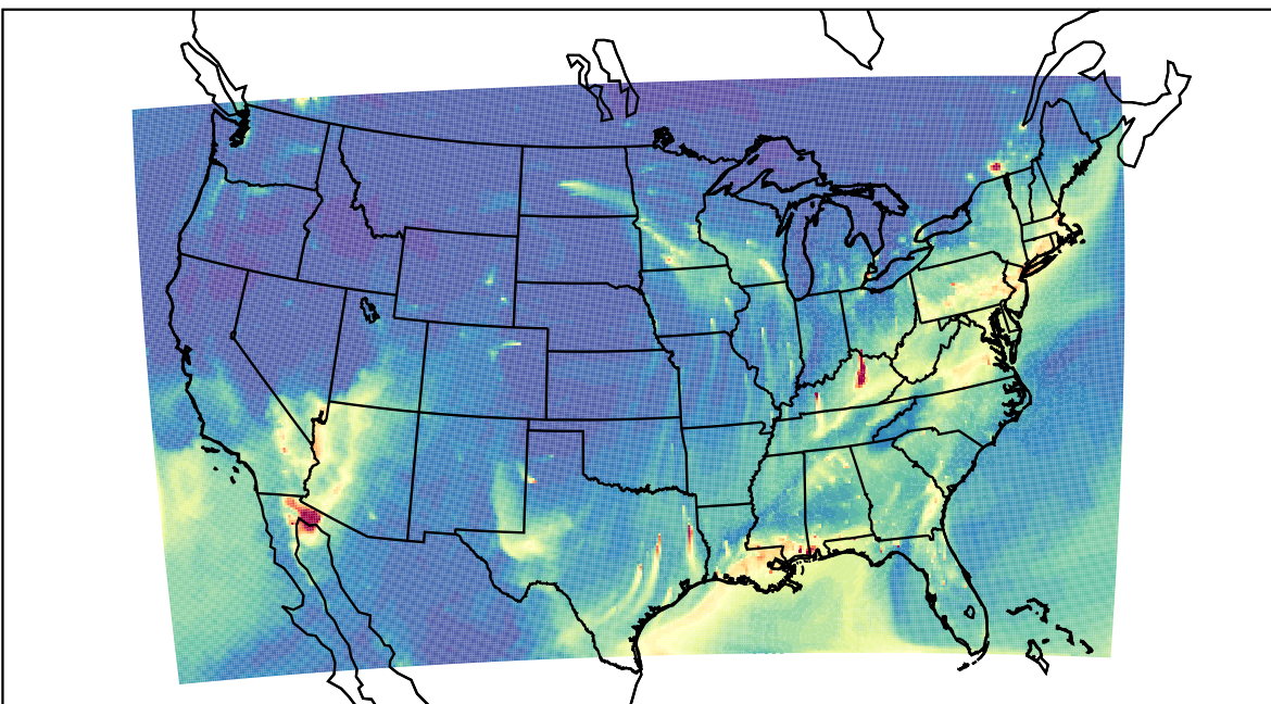
WRF 2023-01-30_12:00:00
