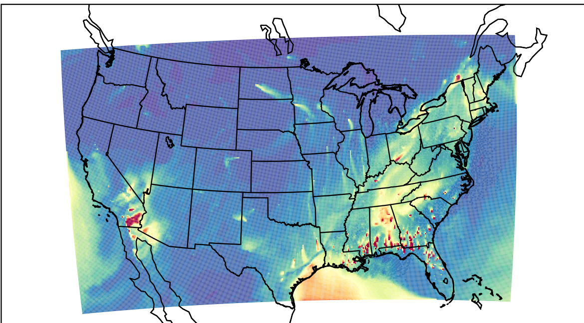
WRF 2023-01-29_21:00:00
