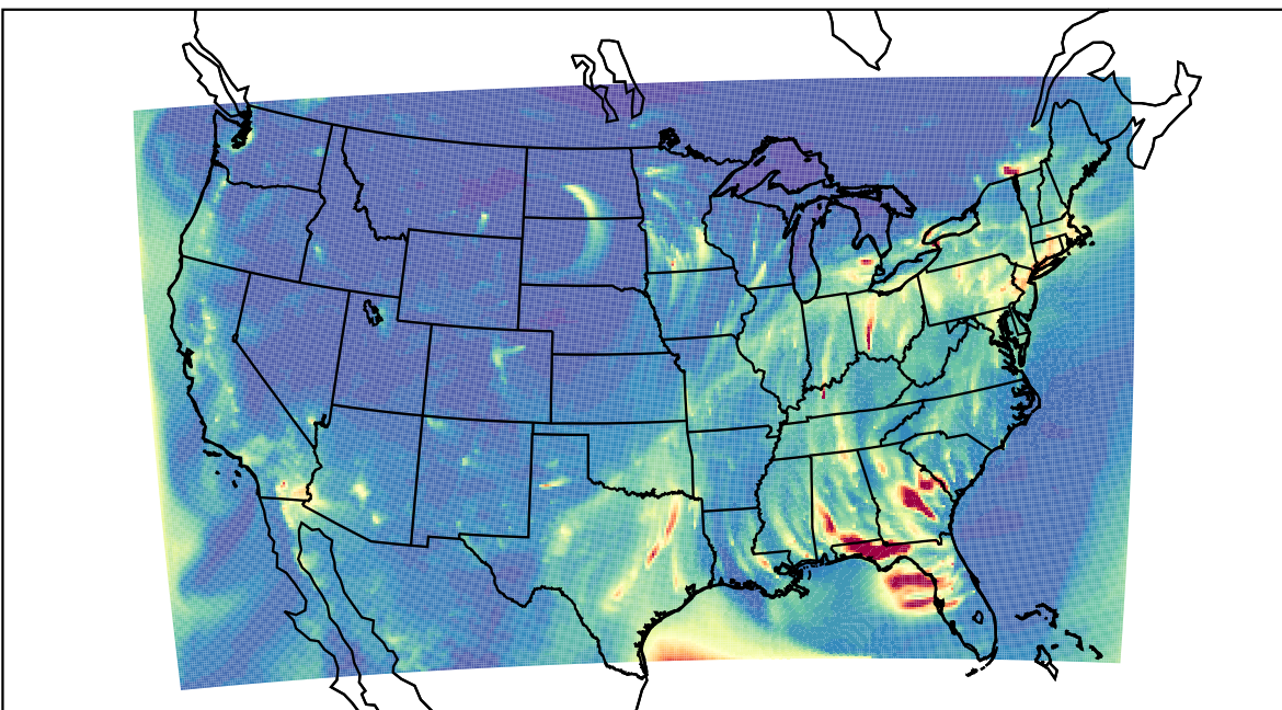
WRF 2023-01-29_05:00:00
