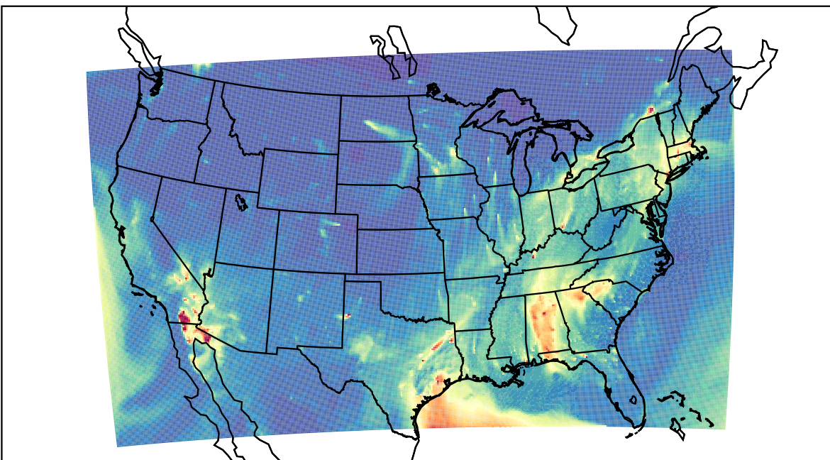
WRF 2023-01-29_15:00:00
