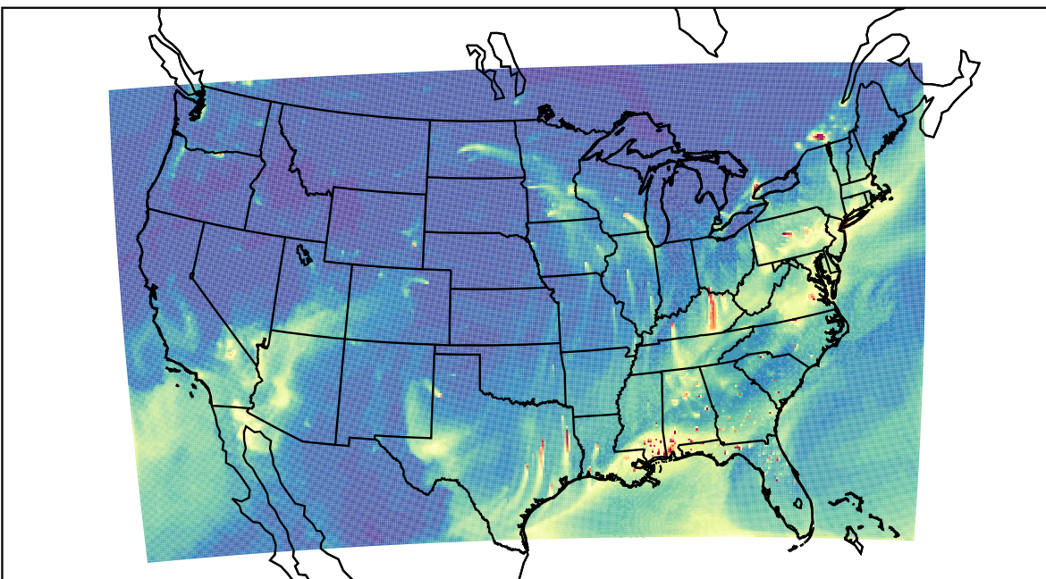
WRF 2023-01-30_17:00:00
