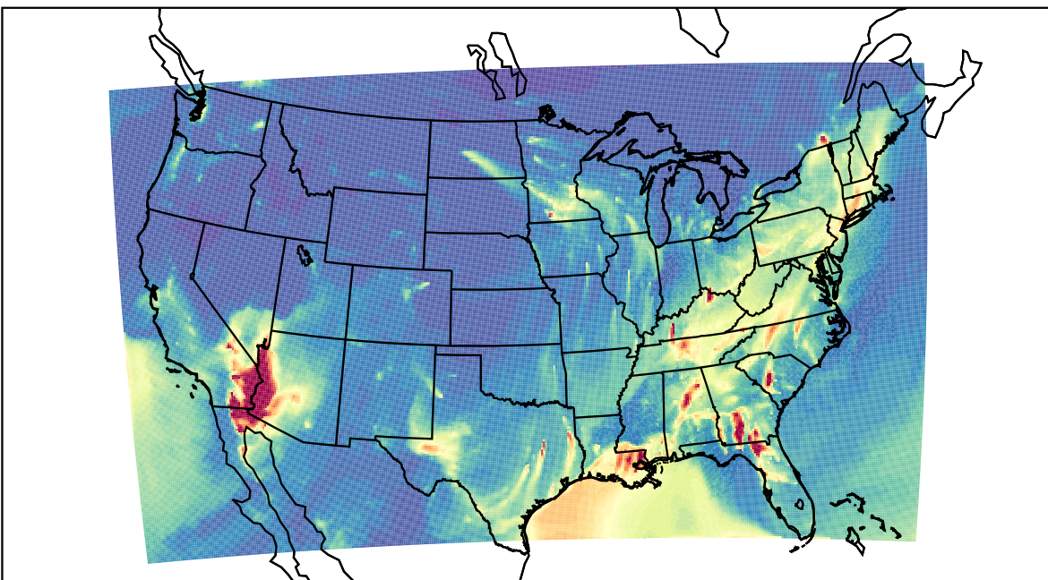
WRF 2023-01-30_05:00:00
