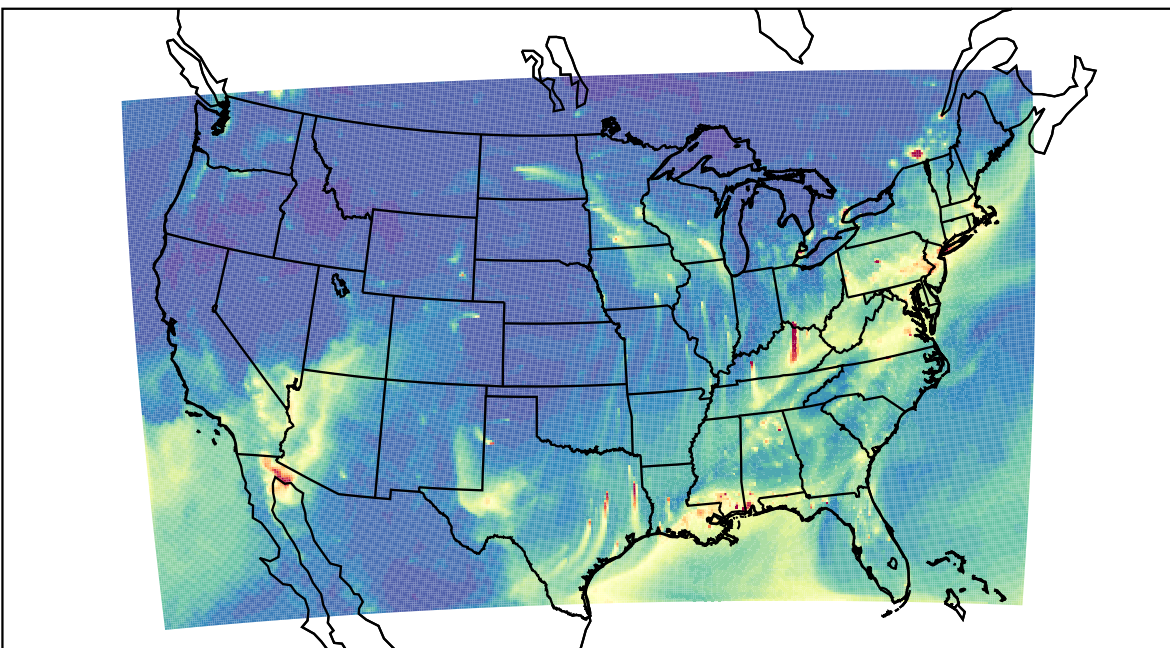
WRF 2023-01-30_14:00:00
