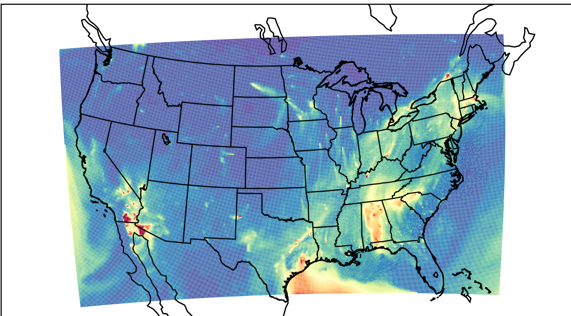
WRF 2023-01-29_16:00:00
