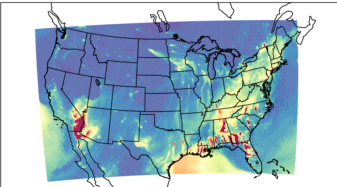
WRF 2023-01-30_02:00:00
