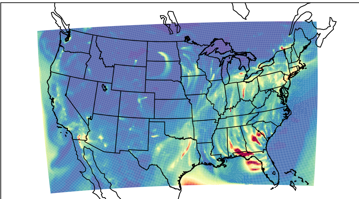
WRF 2023-01-29_06:00:00
