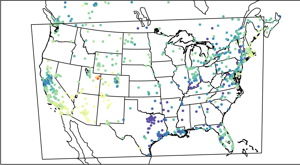
AirNOW (2023-01-29_23:00:00)
