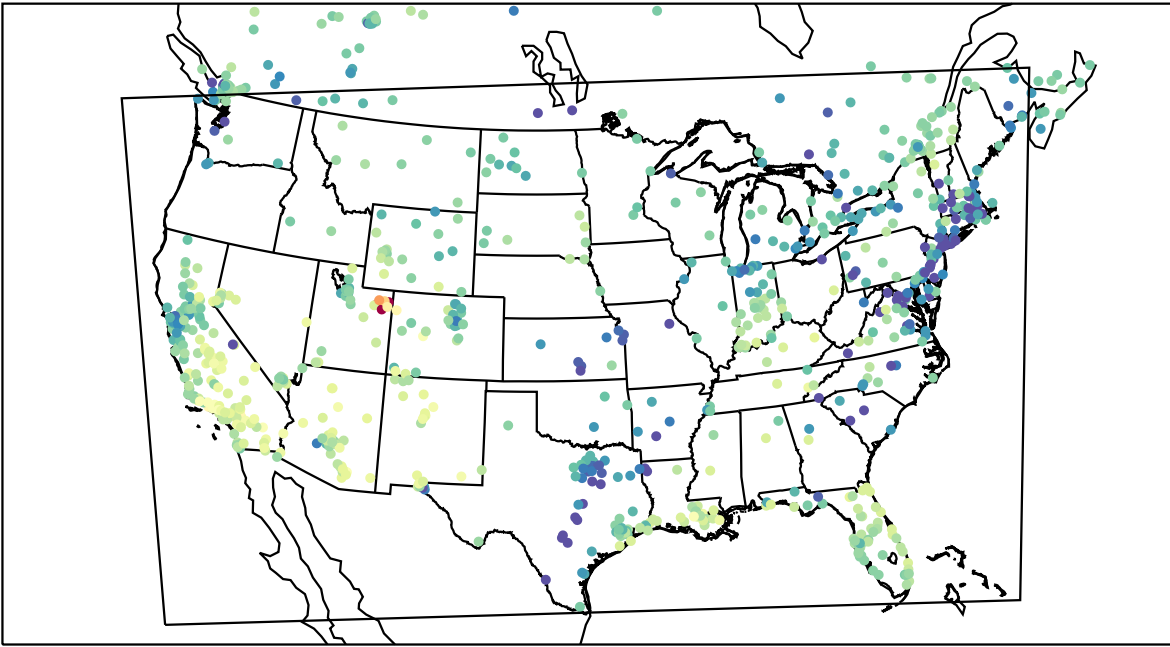
AirNOW (2023-01-29_00:00:00)
