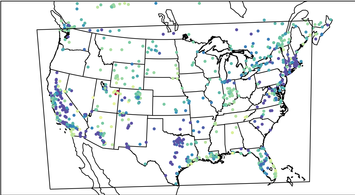
AirNOW (2023-01-29_07:00:00)
