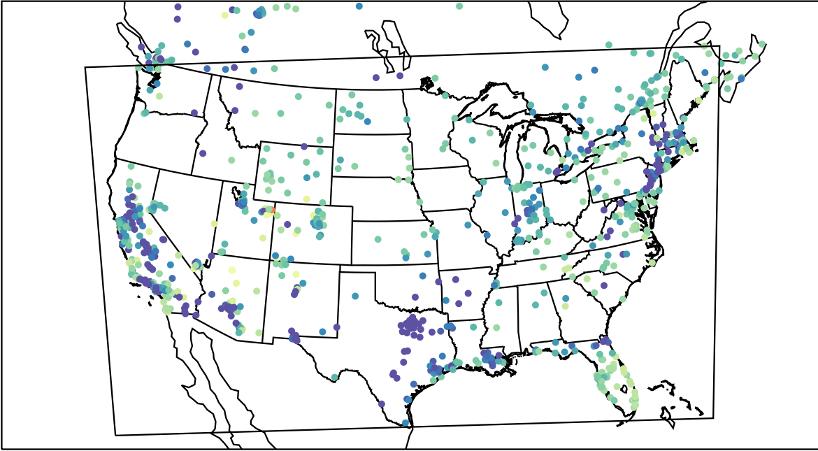
AirNOW (2023-01-29_15:00:00)
