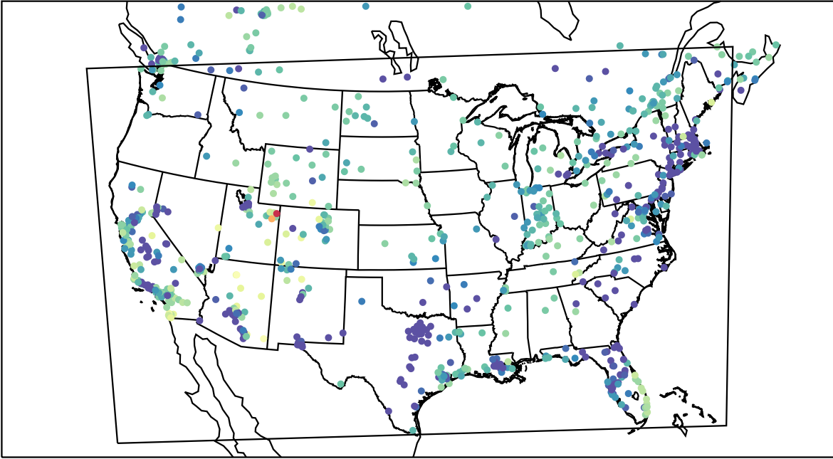
AirNOW (2023-01-29_12:00:00)
