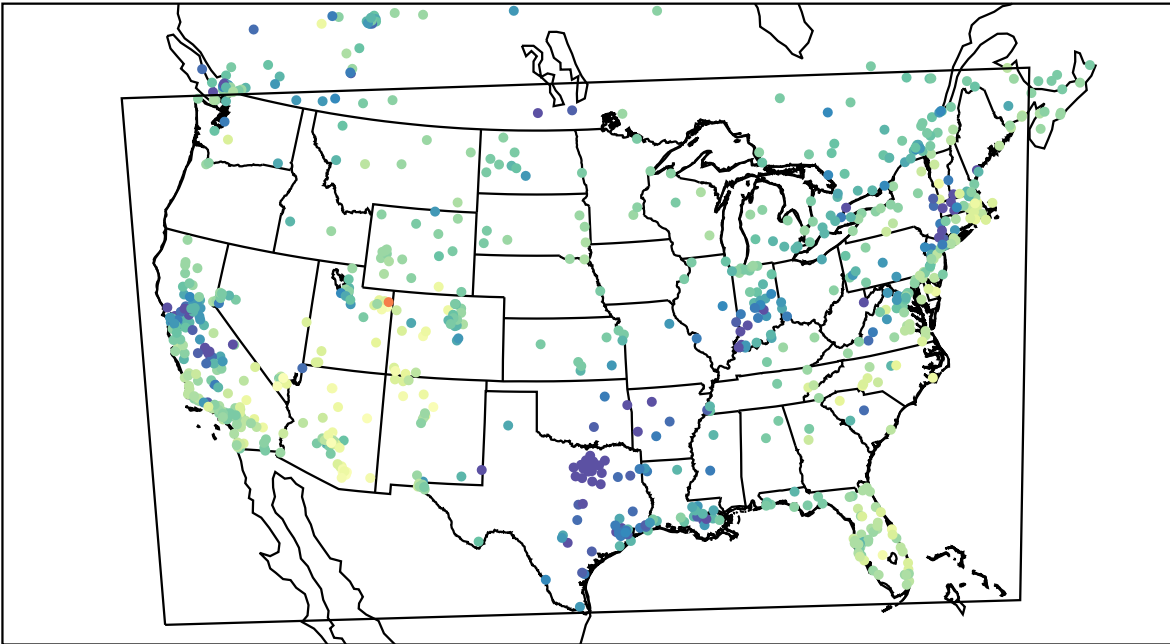
AirNOW (2023-01-29_18:00:00)
