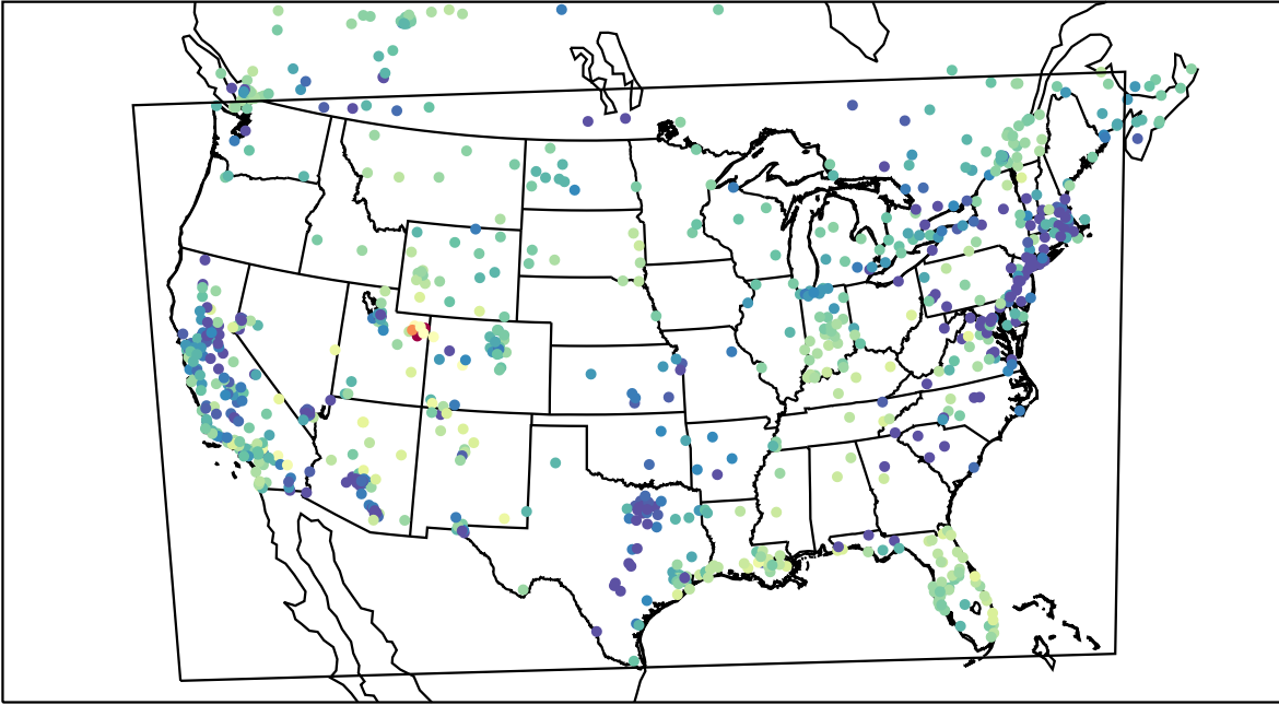
AirNOW (2023-01-29_02:00:00)
