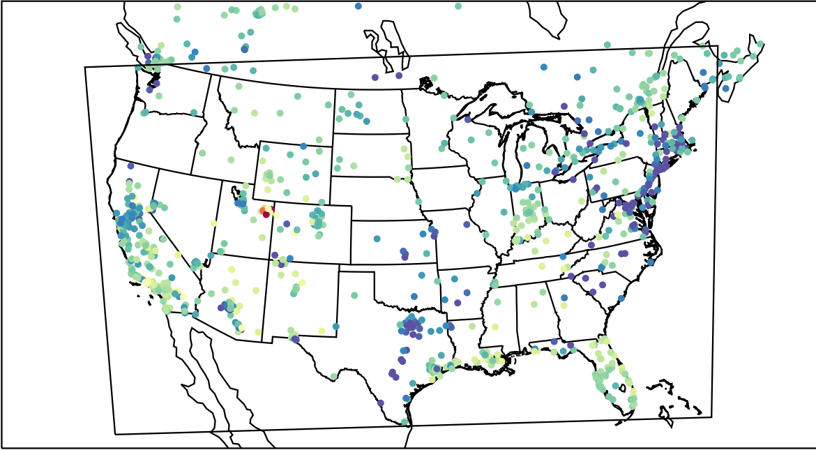
AirNOW (2023-01-29_01:00:00)
