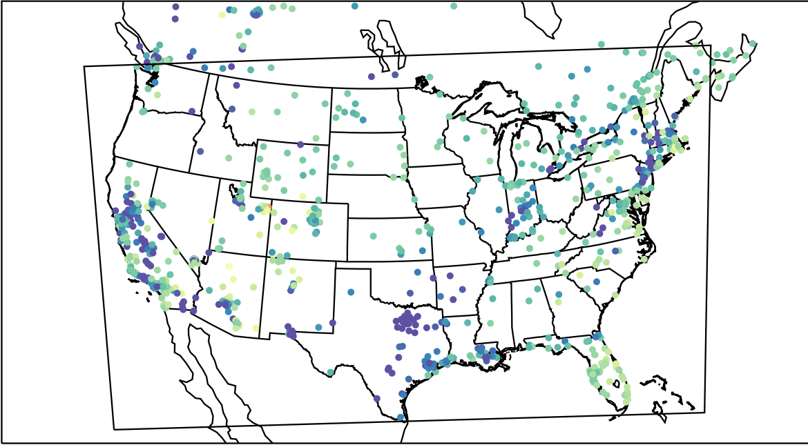
AirNOW (2023-01-29_16:00:00)
