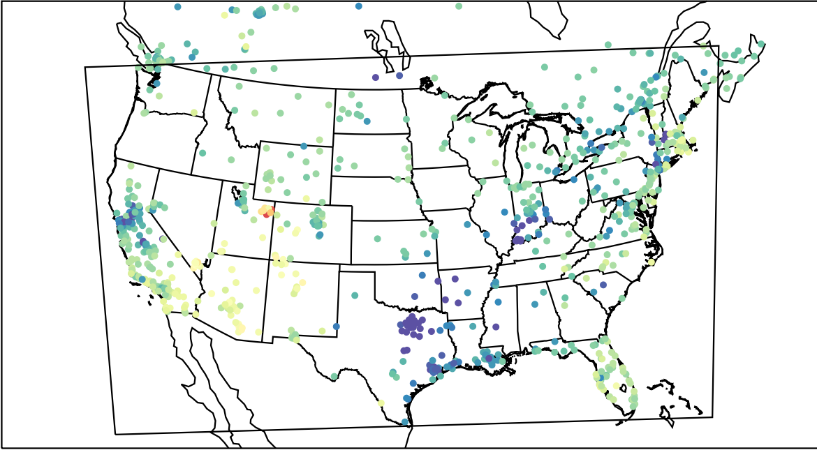
AirNOW (2023-01-29_20:00:00)
