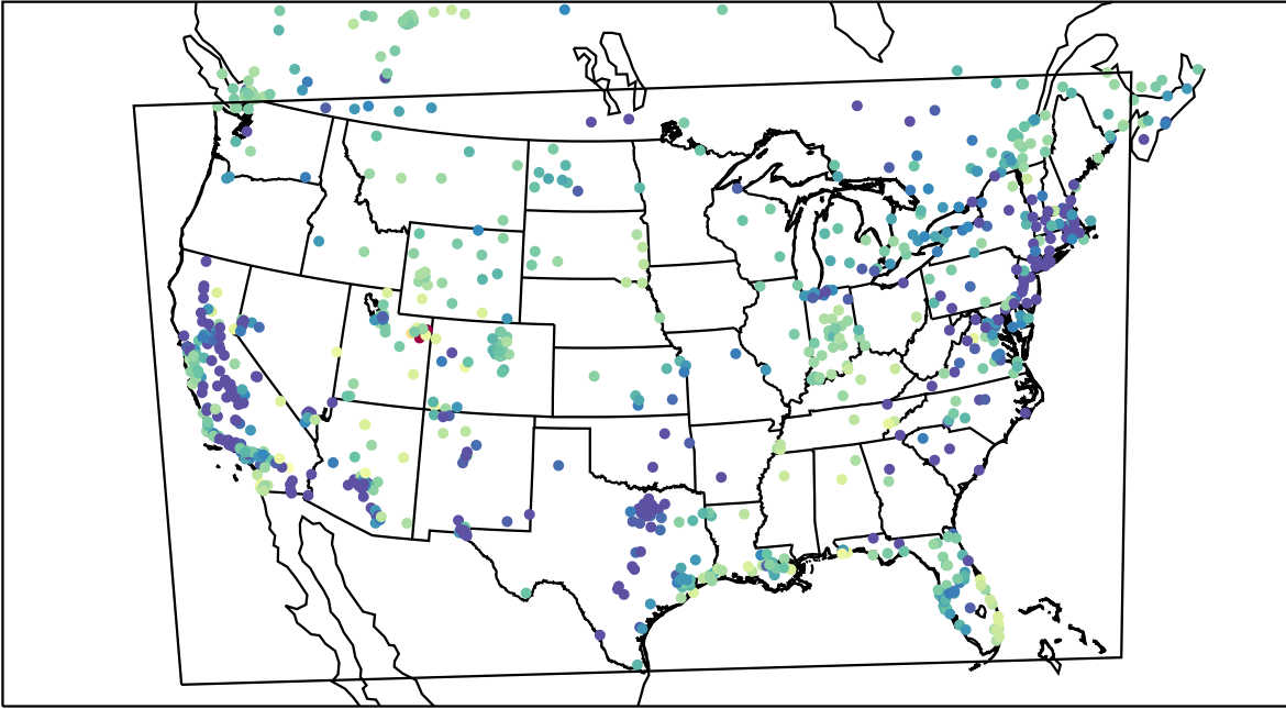
AirNOW (2023-01-29_06:00:00)
