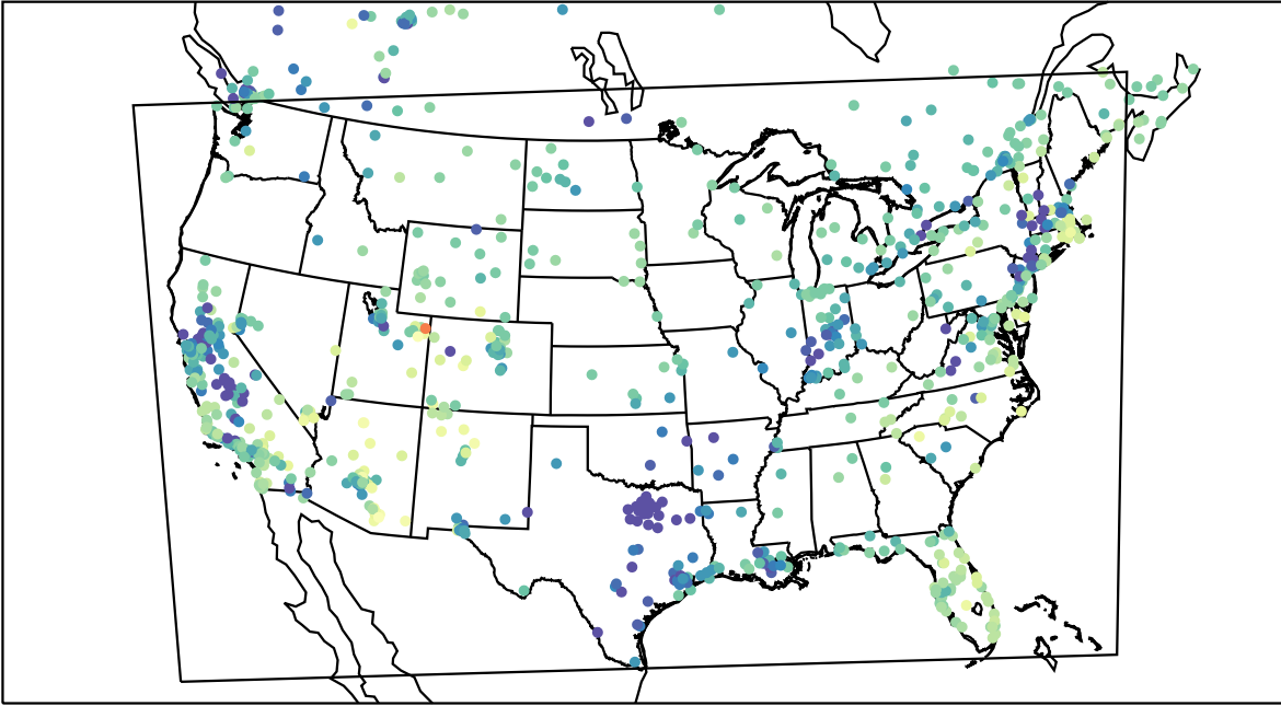
AirNOW (2023-01-29_17:00:00)
