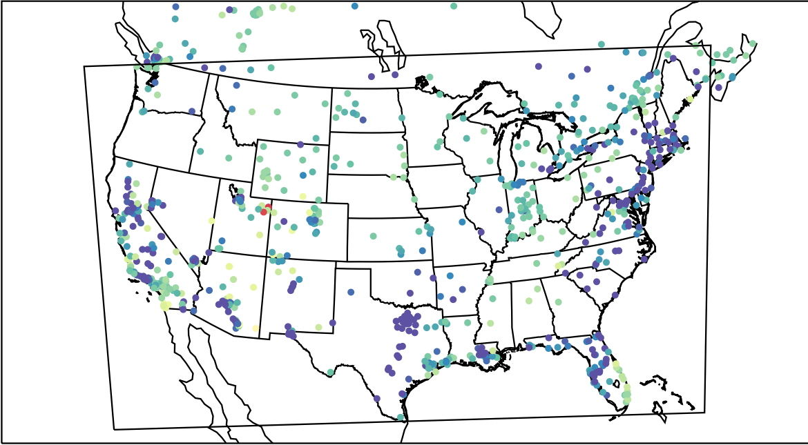
AirNOW (2023-01-29_11:00:00)
