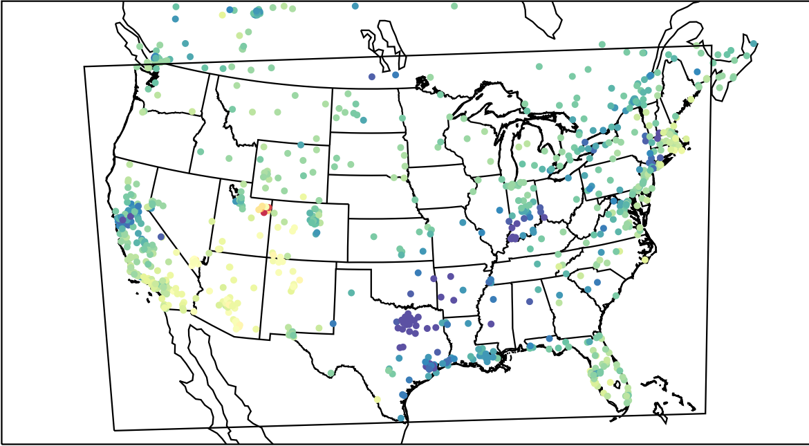
AirNOW (2023-01-29_21:00:00)
