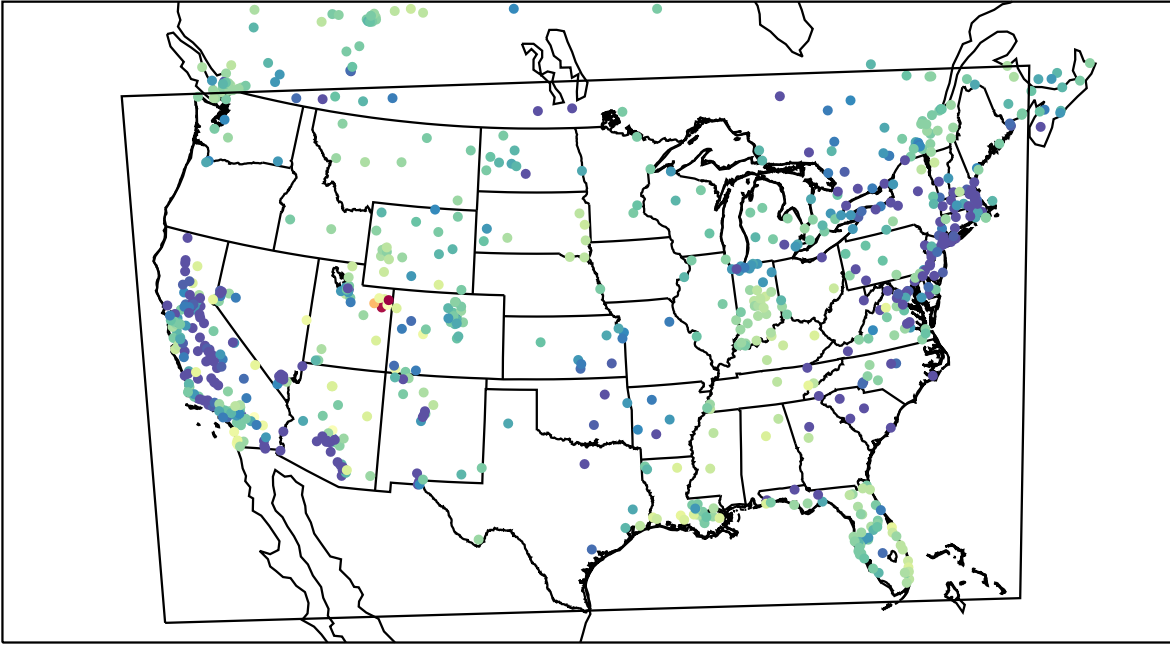
AirNOW (2023-01-29_04:00:00)
