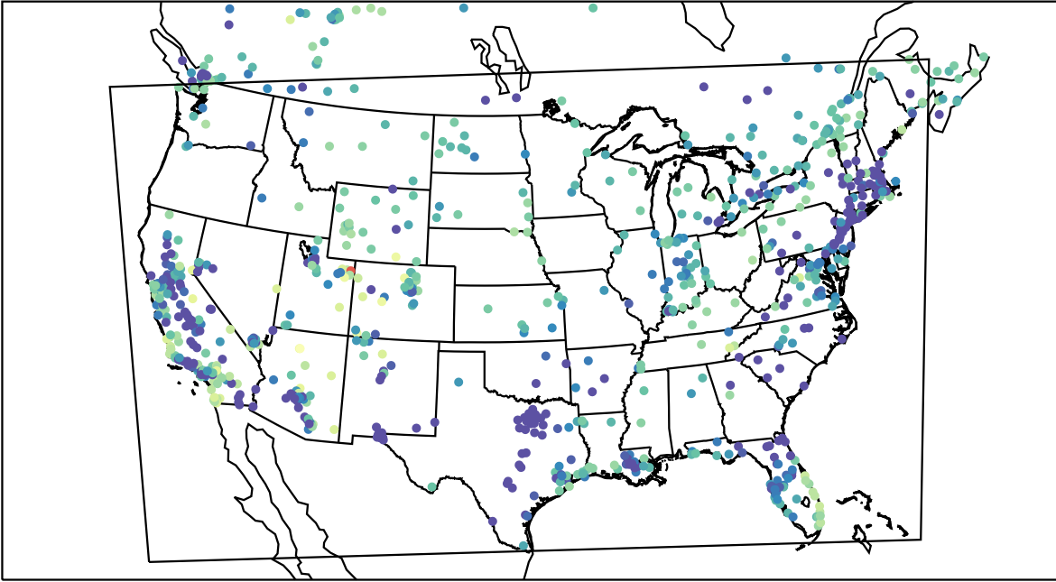
AirNOW (2023-01-29_13:00:00)
