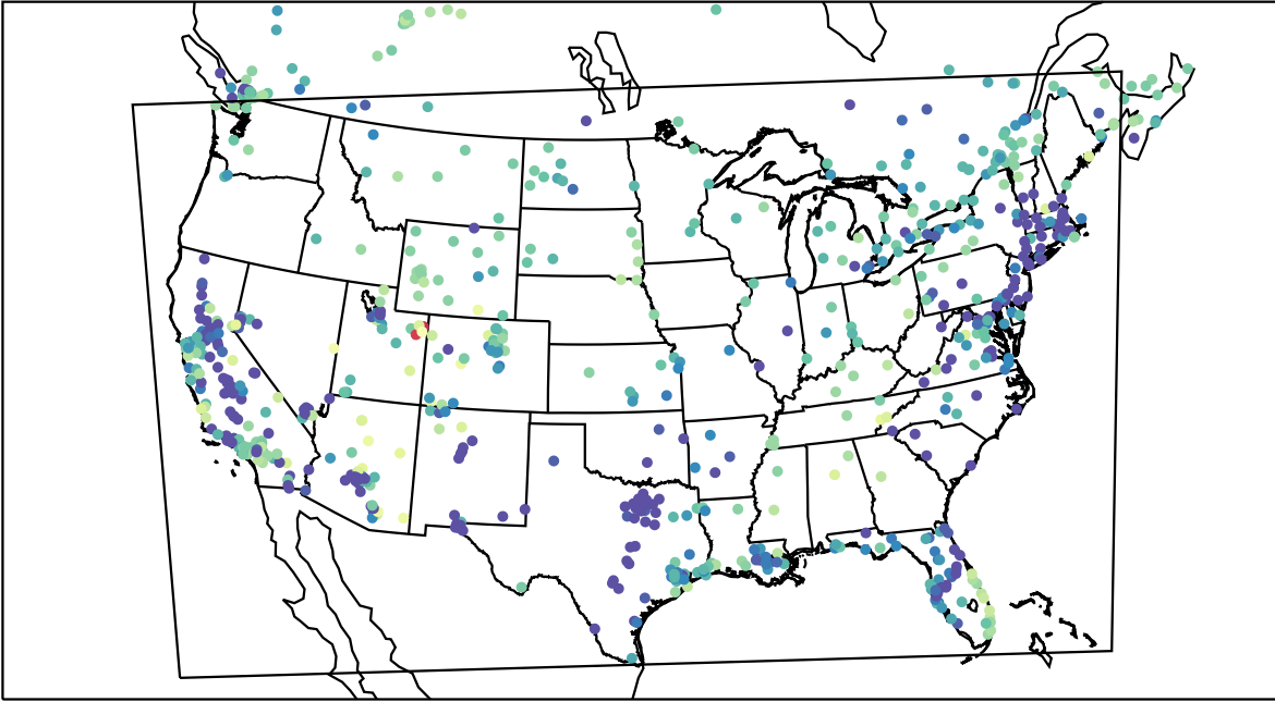
AirNOW (2023-01-29_10:00:00)
