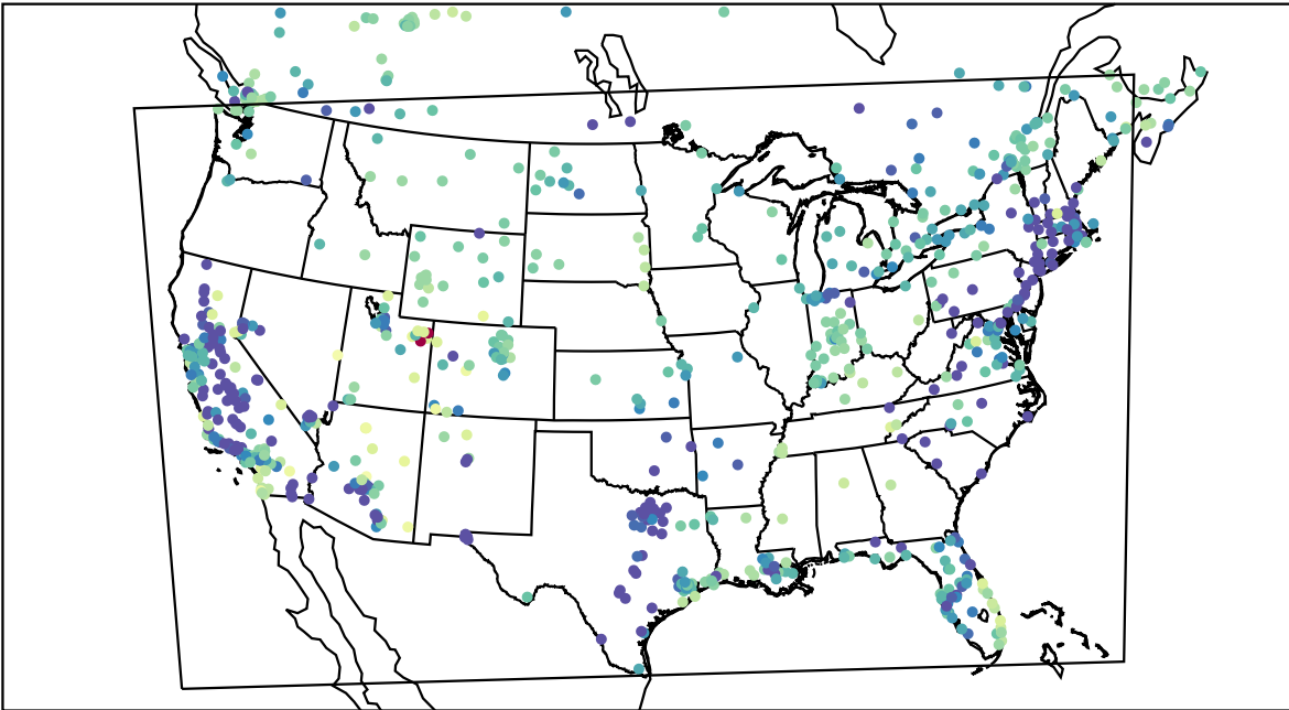
AirNOW (2023-01-29_08:00:00)
