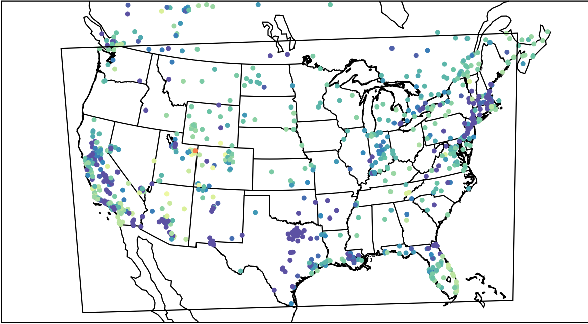
AirNOW (2023-01-29_14:00:00)
