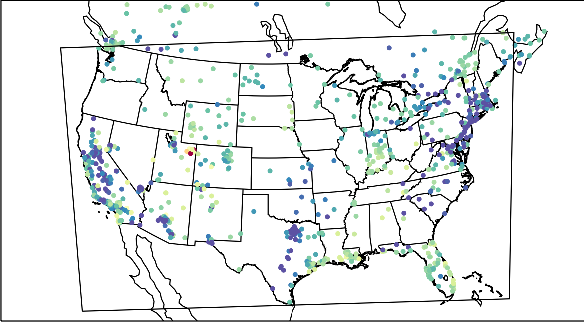
AirNOW (2023-01-29_03:00:00)
