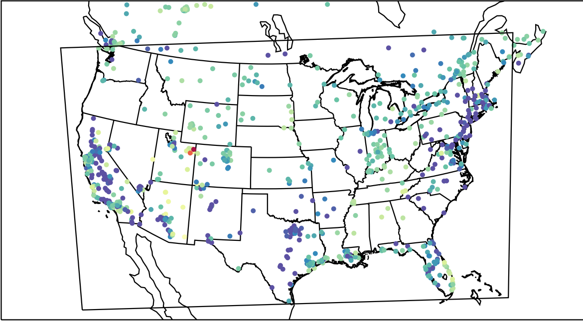
AirNOW (2023-01-29_09:00:00)
