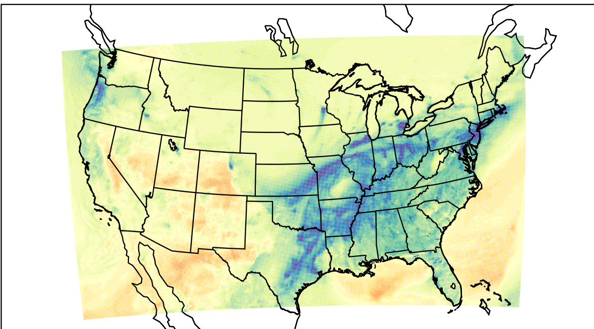
WRF (2023-01-29_00:00:00)
