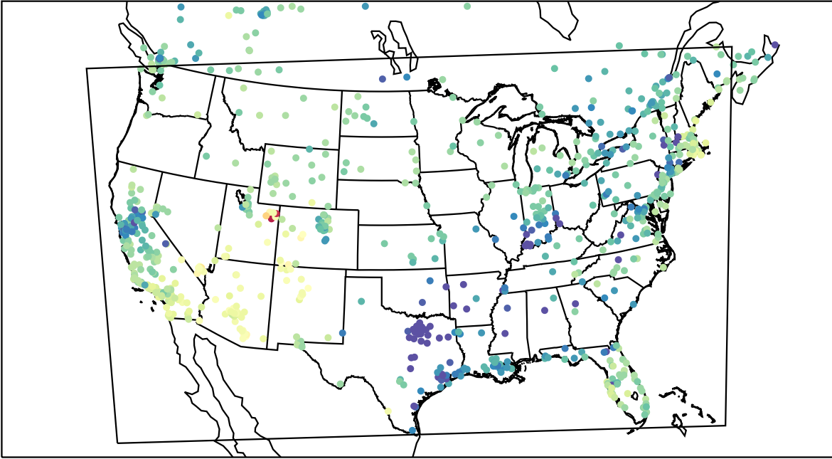
AirNOW (2023-01-29_22:00:00)
