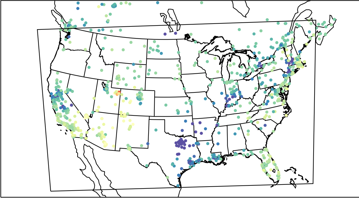
AirNOW (2023-01-29_19:00:00)
