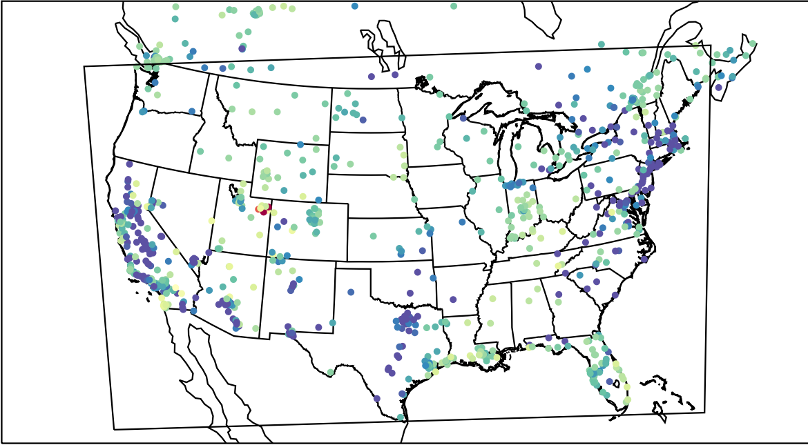
AirNOW (2023-01-29_05:00:00)
