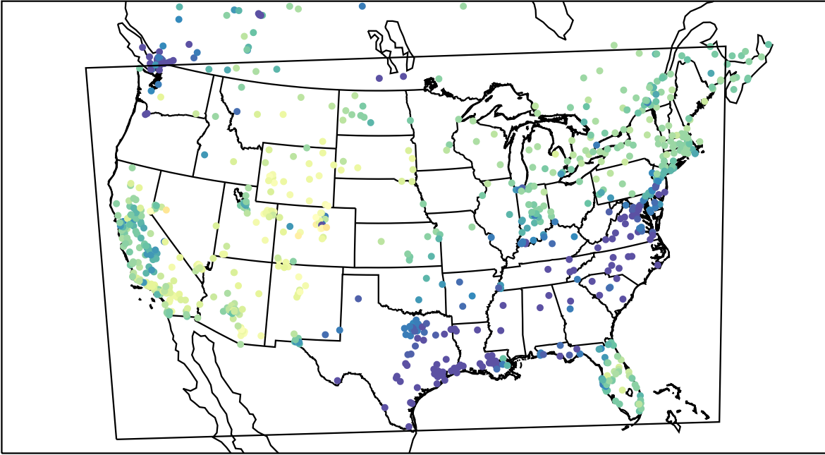
AirNOW (2023-01-31_21:00:00)
