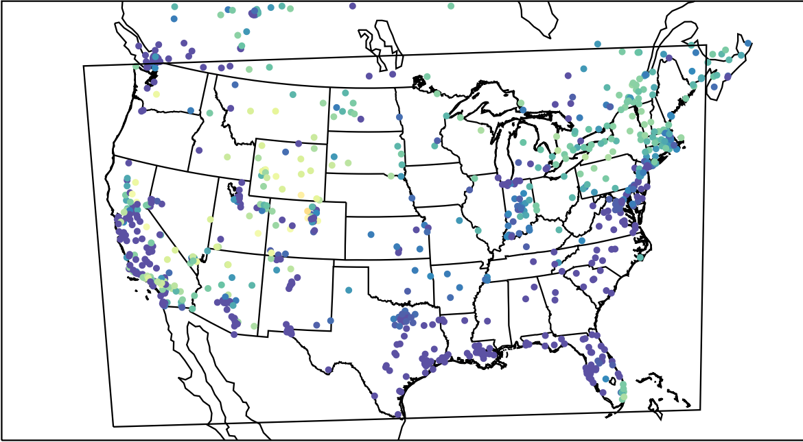
AirNOW (2023-01-31_14:00:00)
