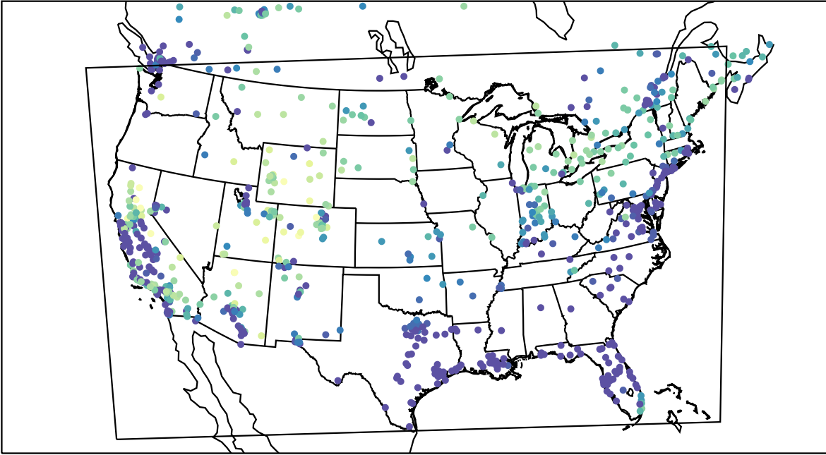
AirNOW (2023-01-31_08:00:00)
