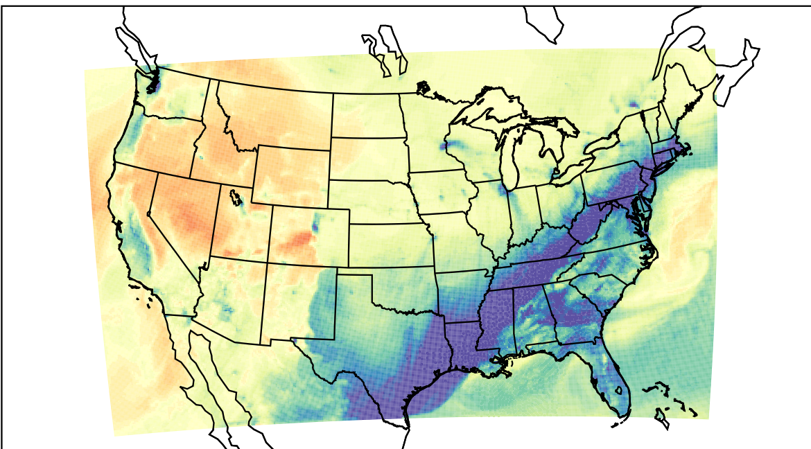
WRF (2023-01-31_01:00:00)
