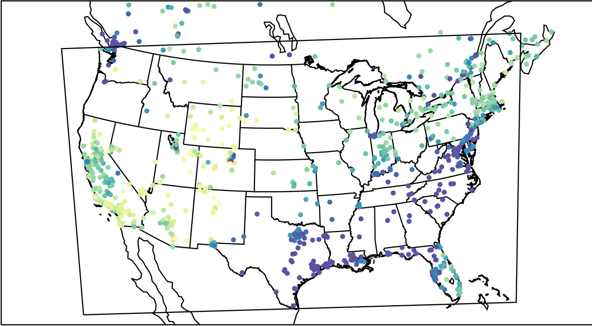
AirNOW (2023-01-31_23:00:00)
