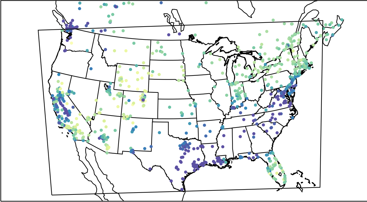
AirNOW (2023-01-31_18:00:00)
