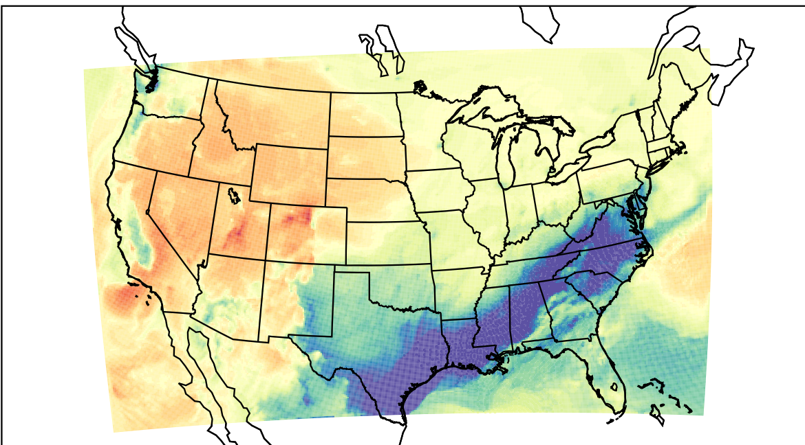
WRF (2023-01-31_19:00:00)
