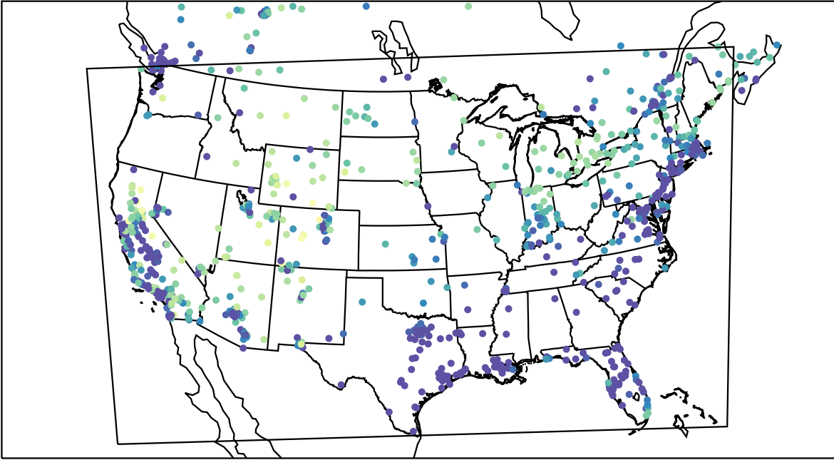
AirNOW (2023-01-31_04:00:00)
