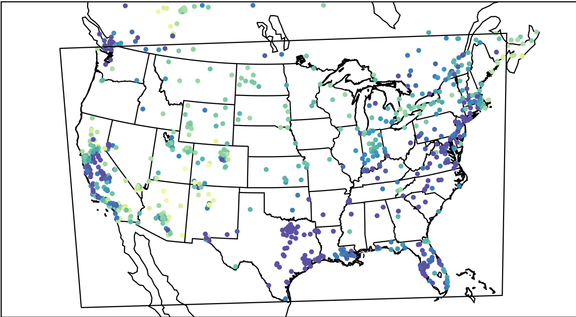
AirNOW (2023-01-30_06:00:00)
