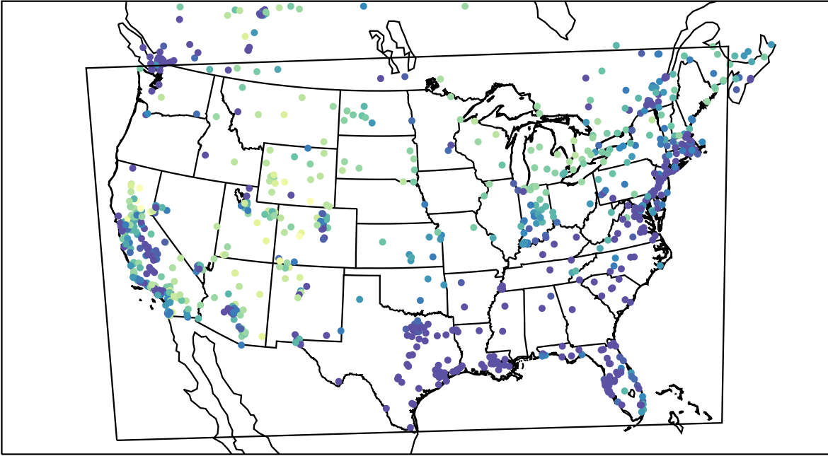
AirNOW (2023-01-31_02:00:00)
