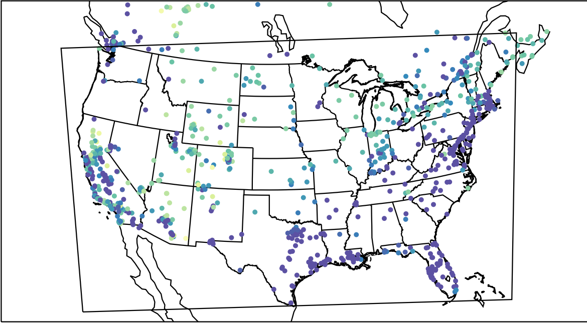
AirNOW (2023-01-30_13:00:00)
