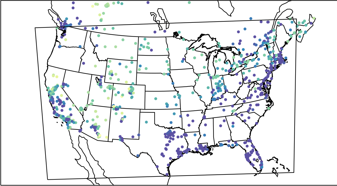
AirNOW (2023-01-30_12:00:00)
