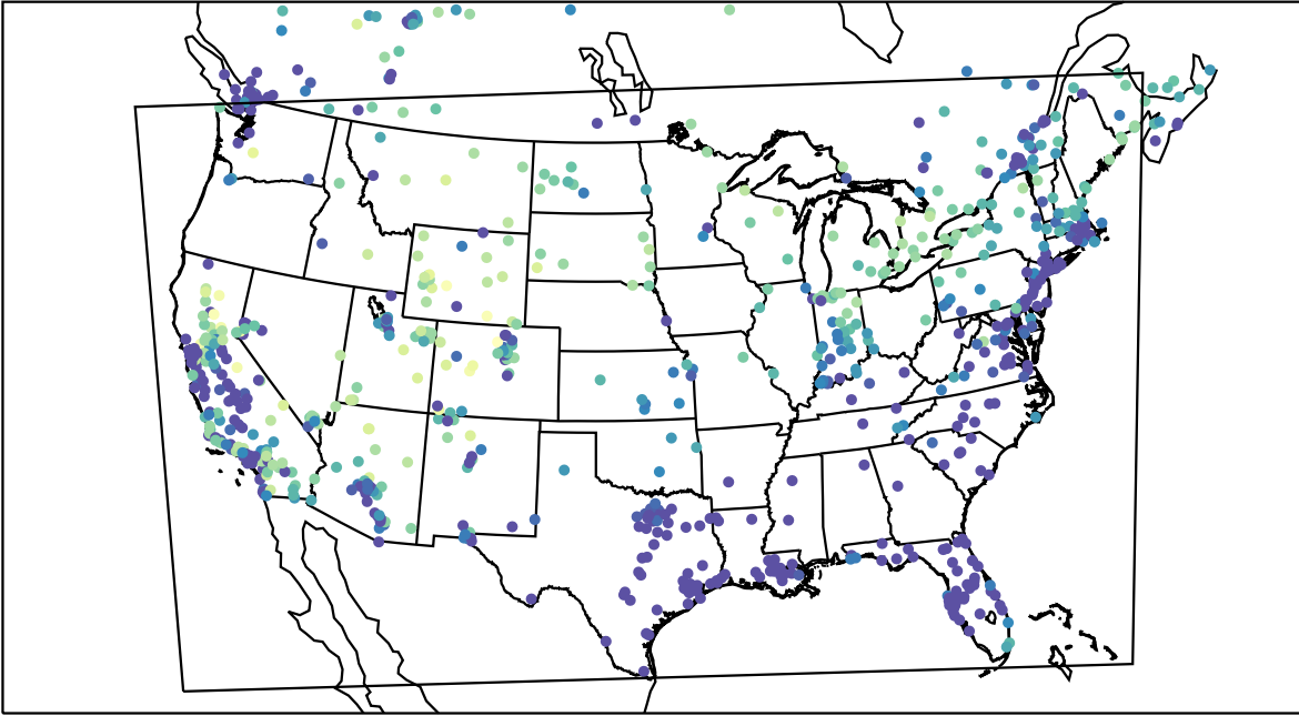
AirNOW (2023-01-31_05:00:00)
