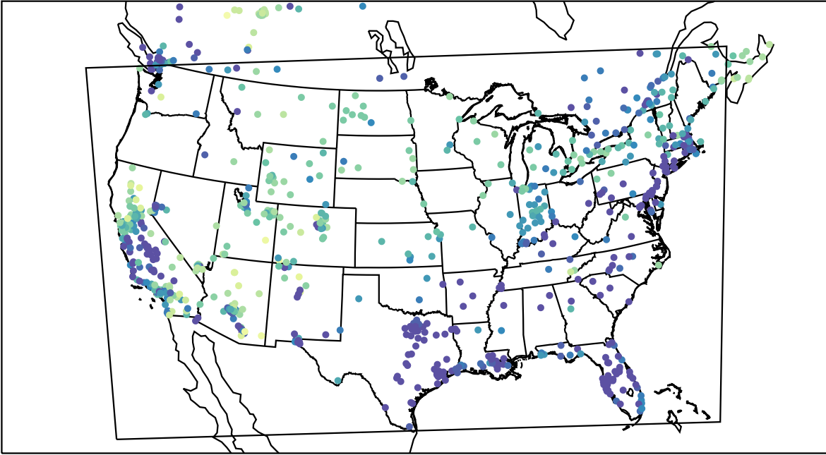
AirNOW (2023-01-30_09:00:00)
