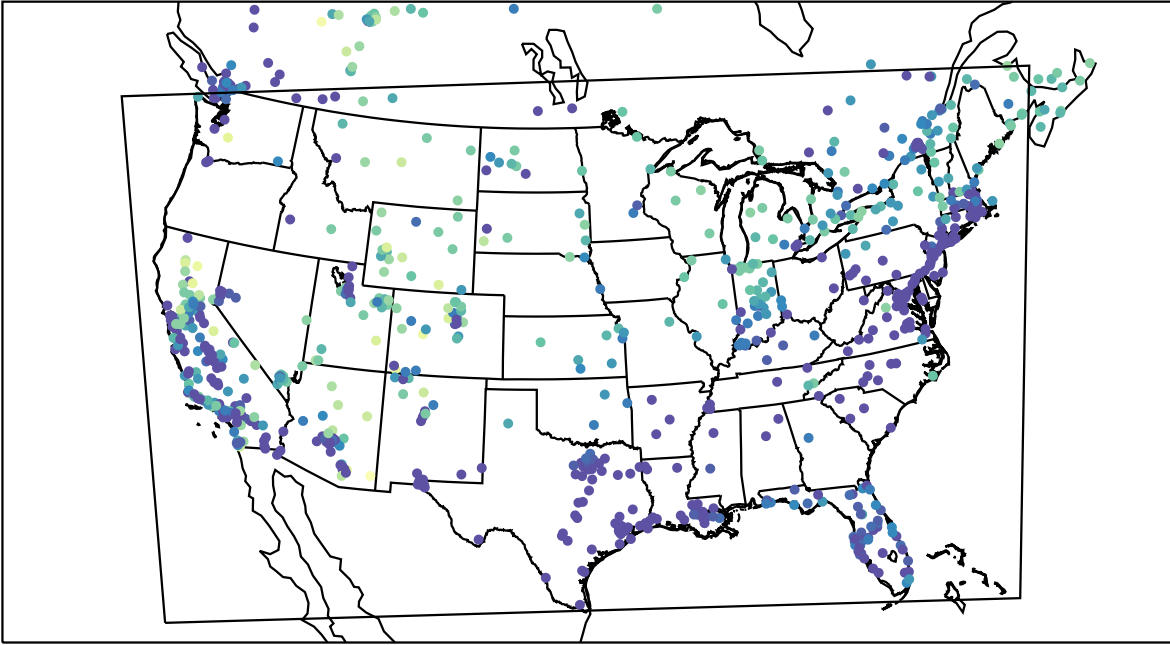
AirNOW (2023-01-30_14:00:00)
