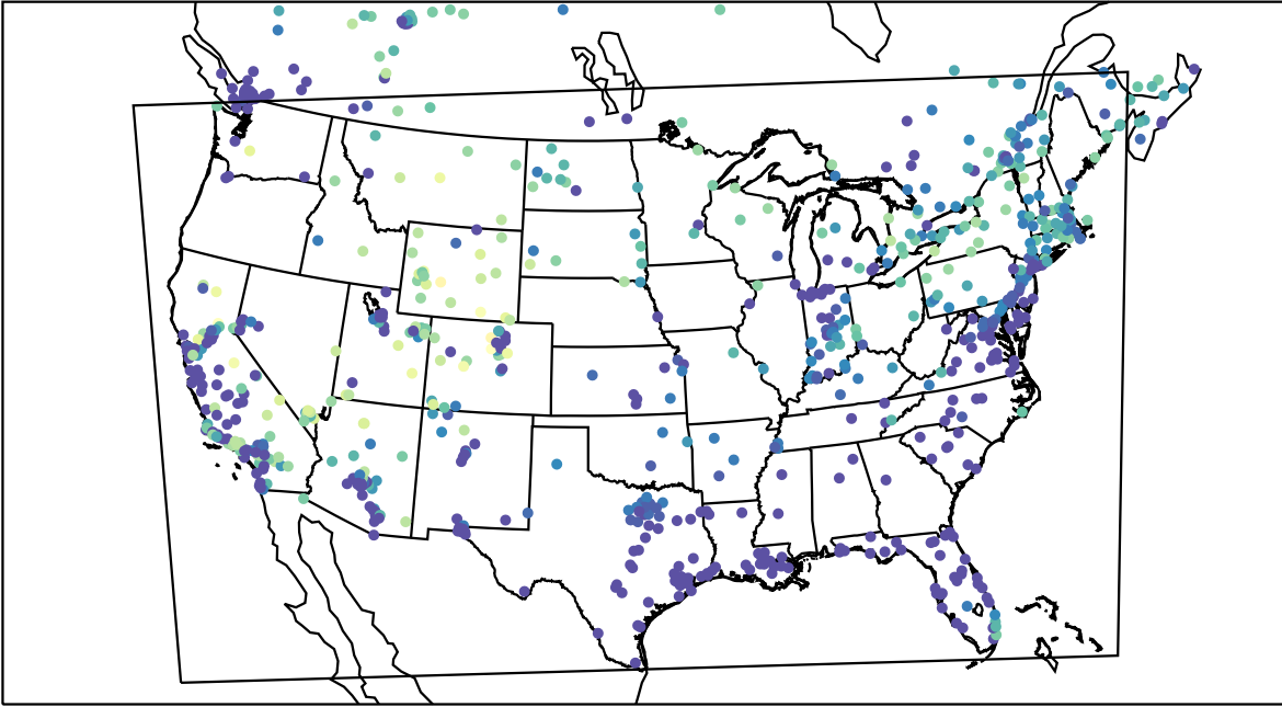
AirNOW (2023-01-31_12:00:00)
