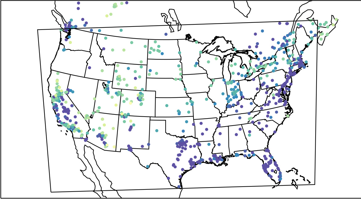
AirNOW (2023-01-30_10:00:00)
