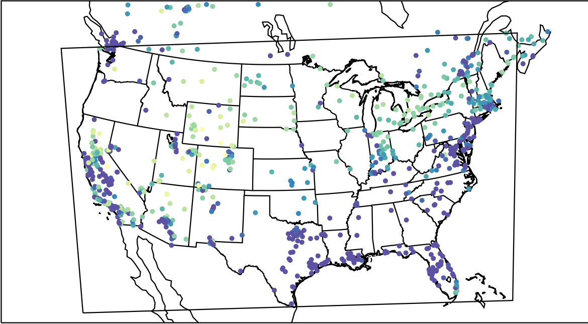
AirNOW (2023-01-31_06:00:00)
