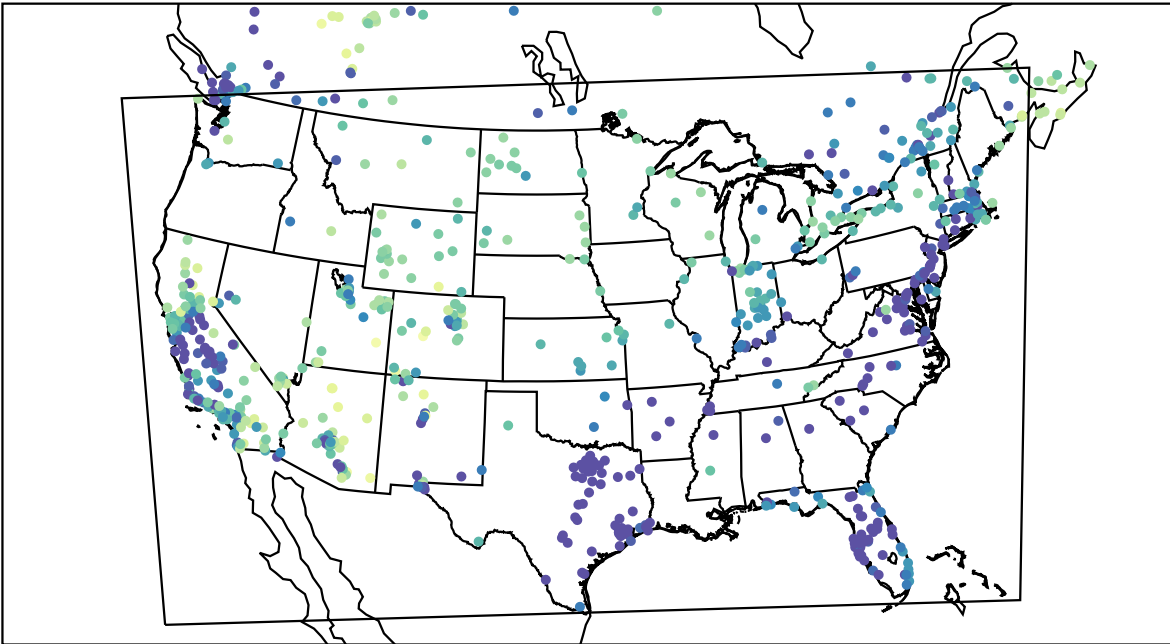
AirNOW (2023-01-30_07:00:00)
