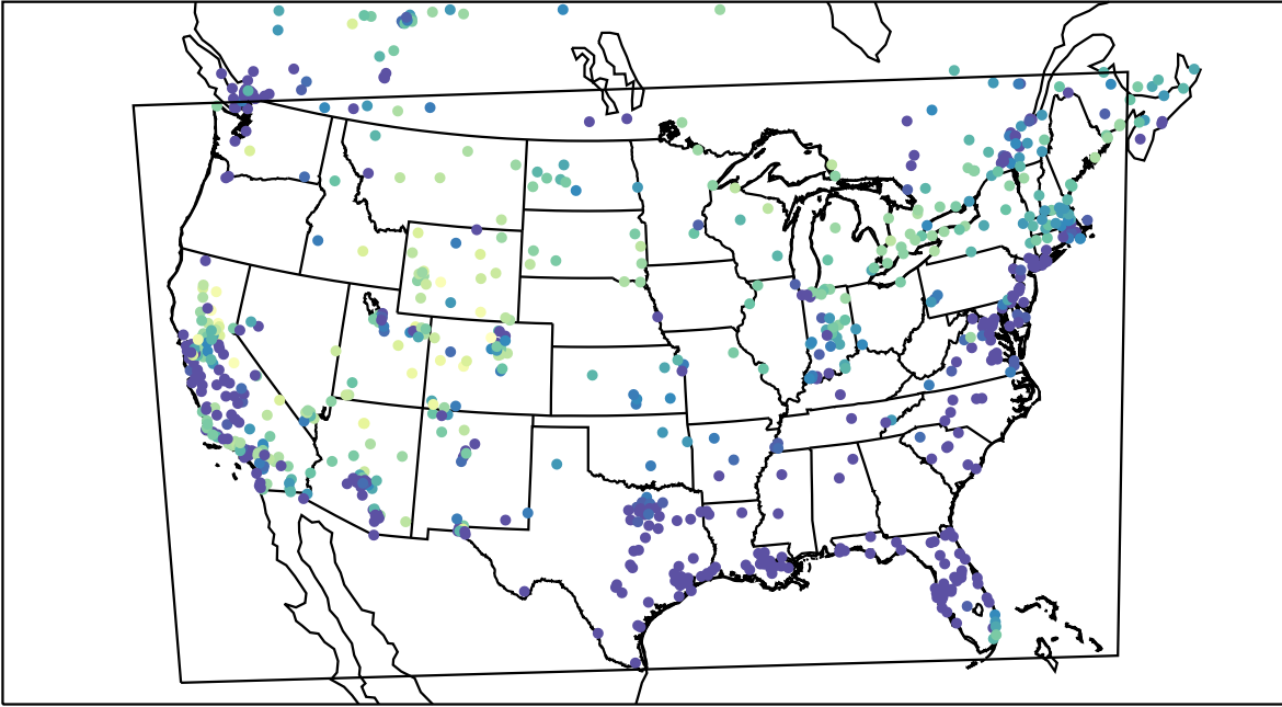
AirNOW (2023-01-31_07:00:00)
