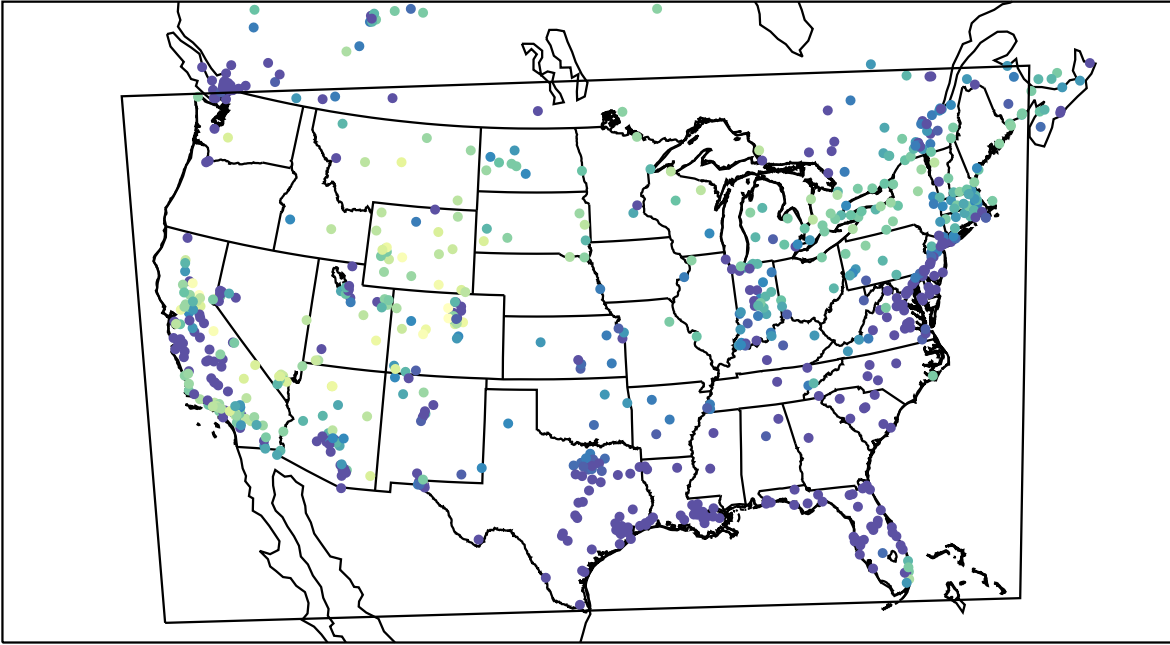
AirNOW (2023-01-31_10:00:00)
