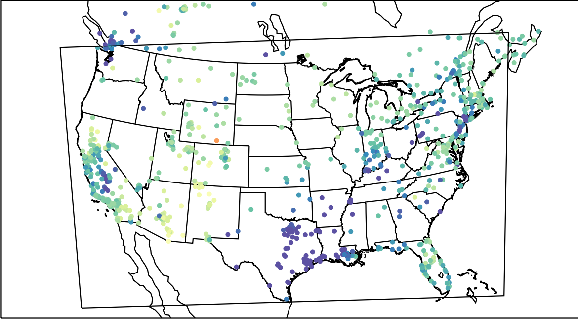
AirNOW (2023-01-30_19:00:00)
