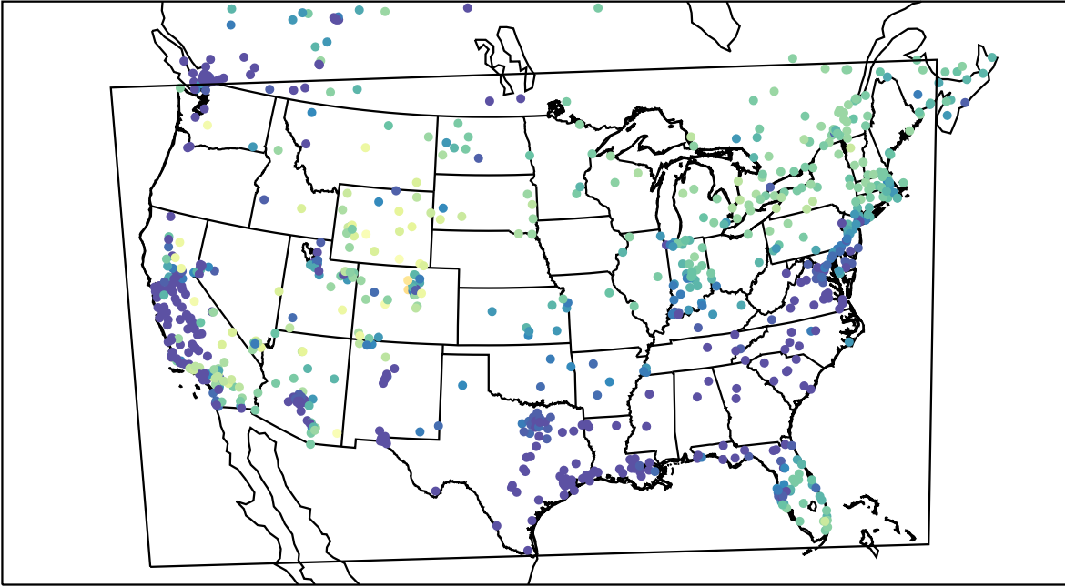
AirNOW (2023-01-31_16:00:00)
