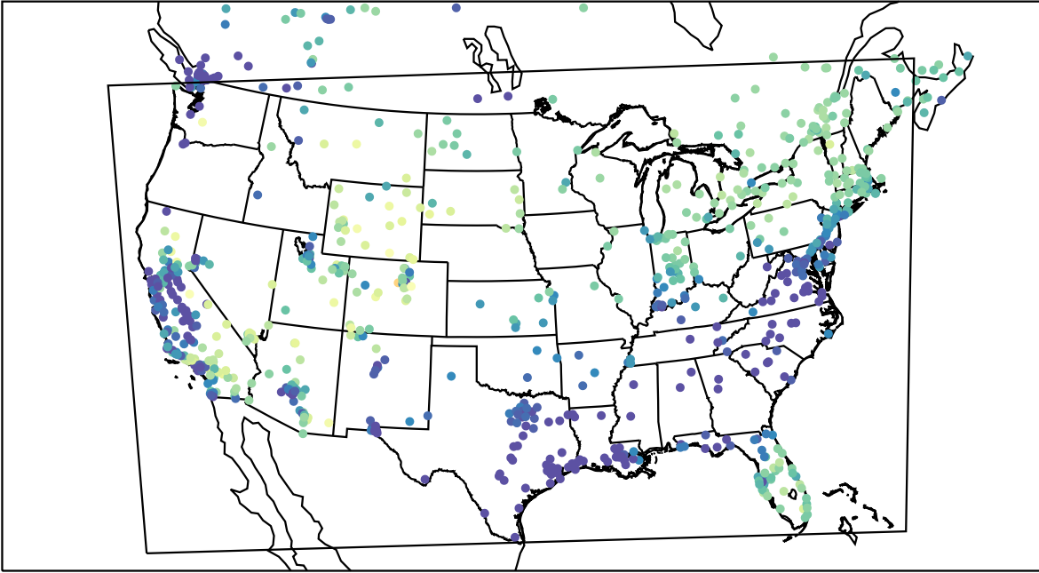
AirNOW (2023-01-31_17:00:00)
