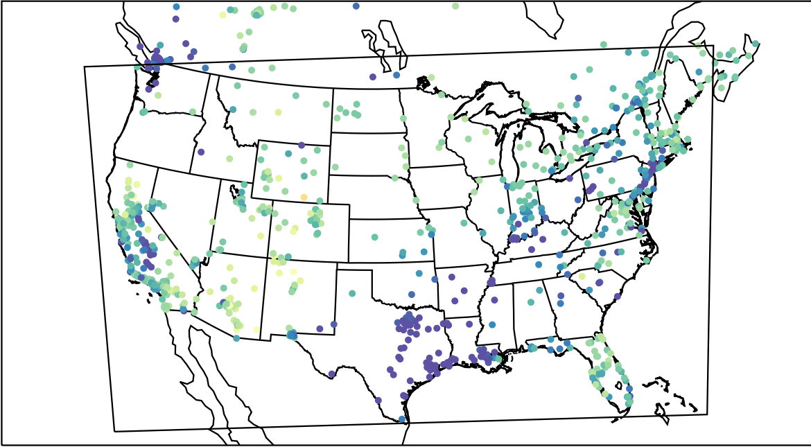
AirNOW (2023-01-30_18:00:00)
