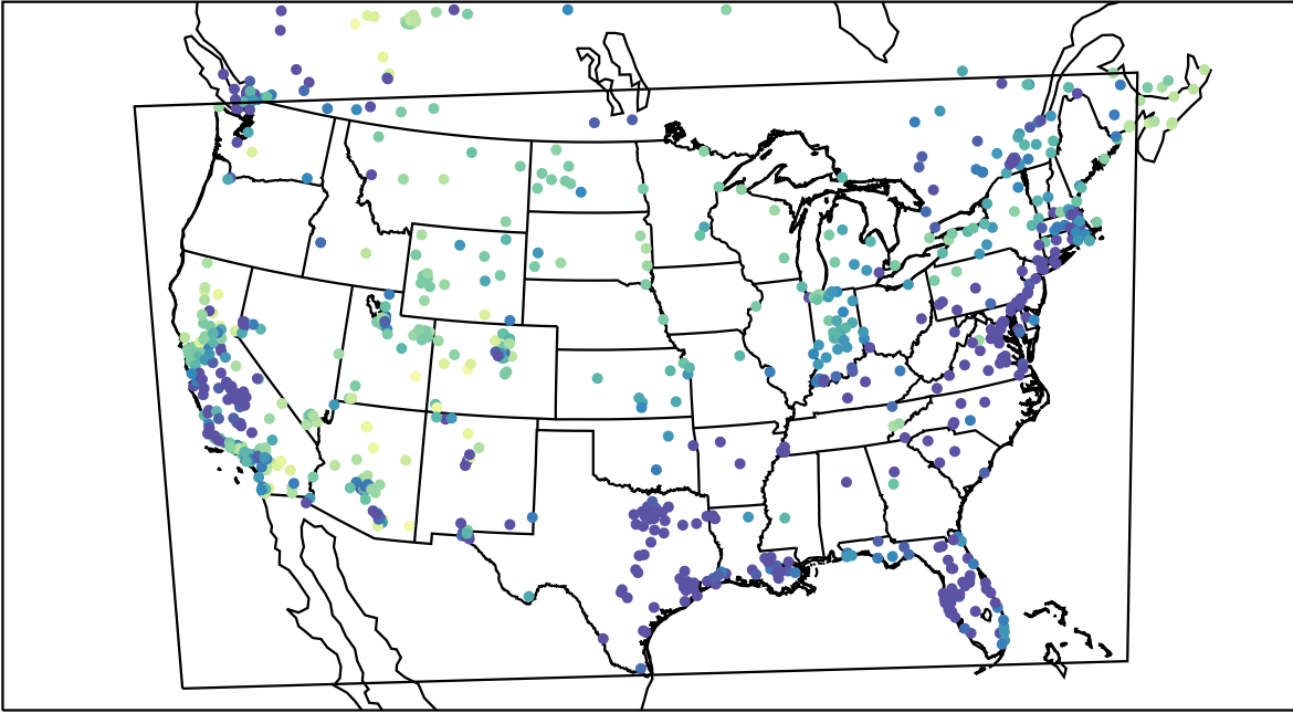
AirNOW (2023-01-30_08:00:00)
