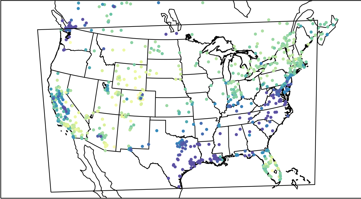
AirNOW (2023-01-31_19:00:00)
