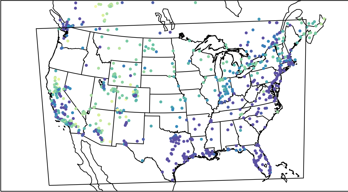
AirNOW (2023-01-30_11:00:00)
