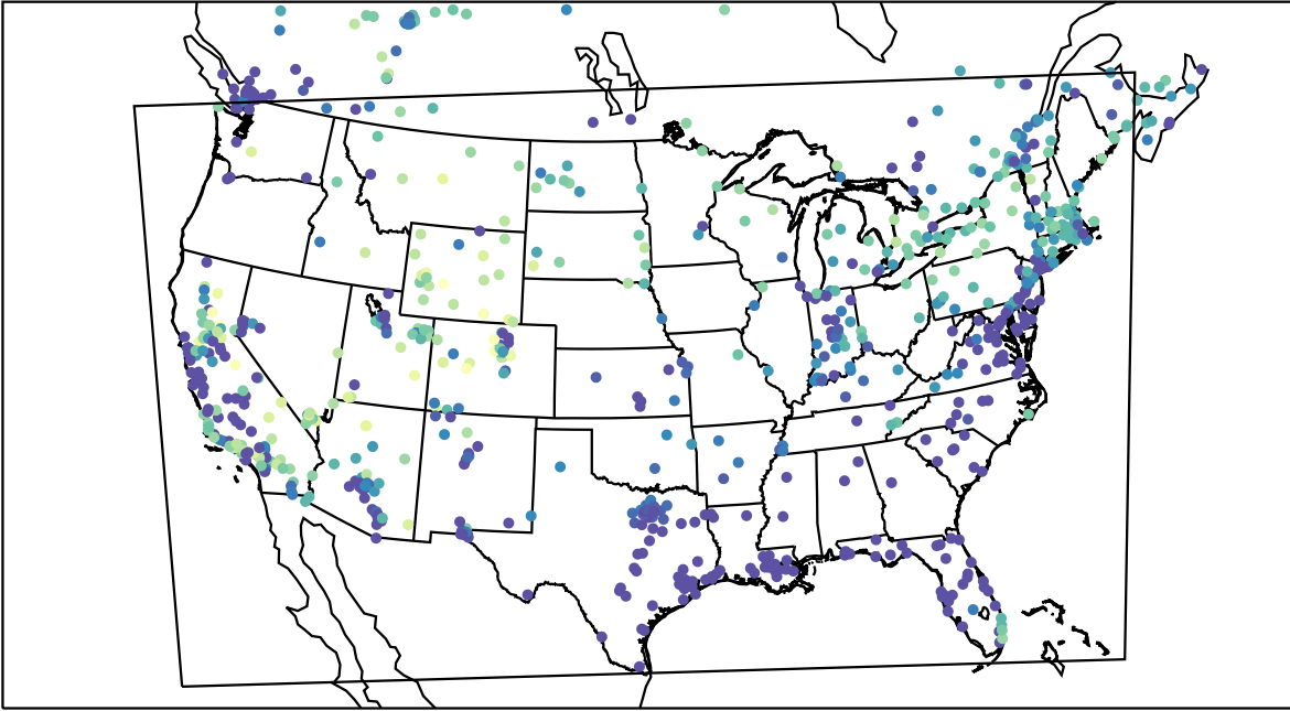
AirNOW (2023-01-31_11:00:00)
