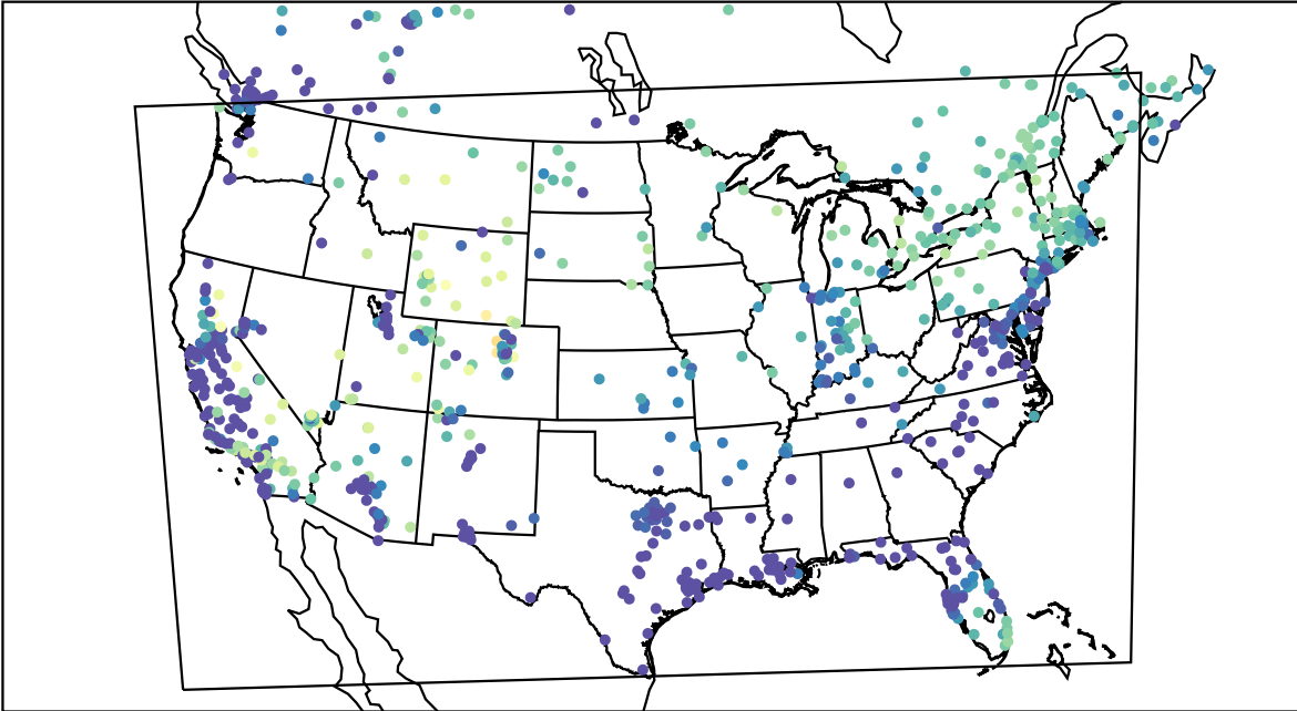
AirNOW (2023-01-31_15:00:00)
