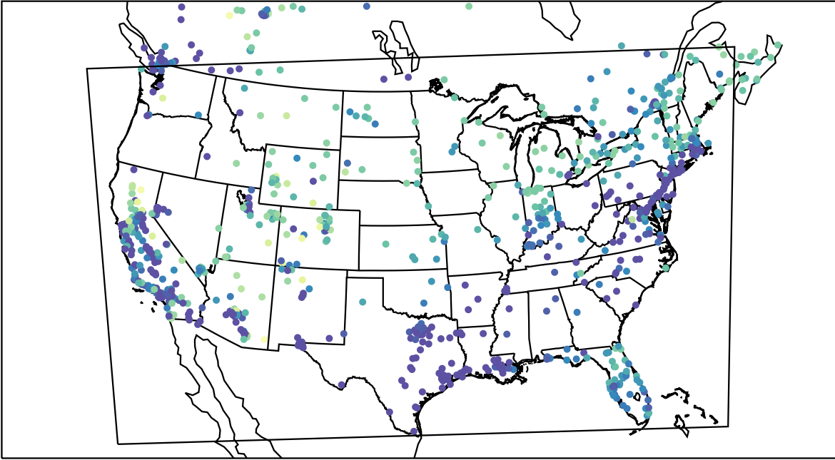
AirNOW (2023-01-30_15:00:00)
