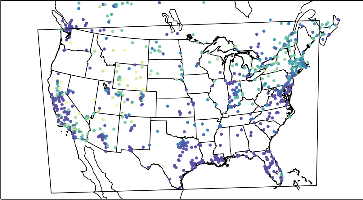
AirNOW (2023-01-31_13:00:00)
