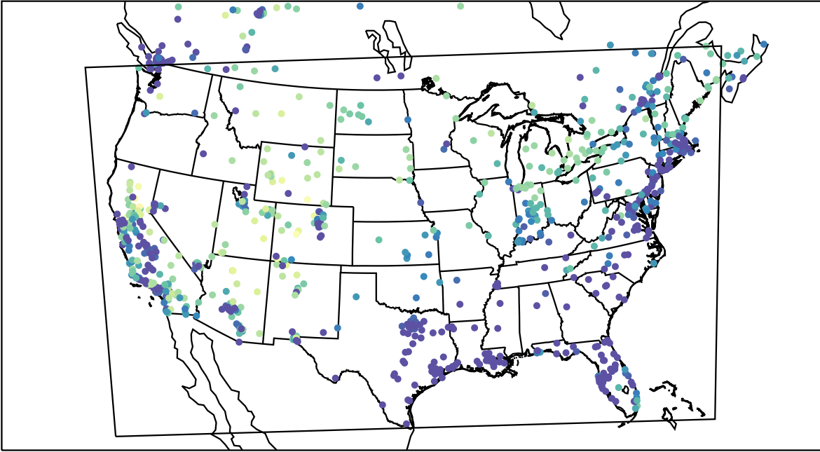
AirNOW (2023-01-31_03:00:00)
