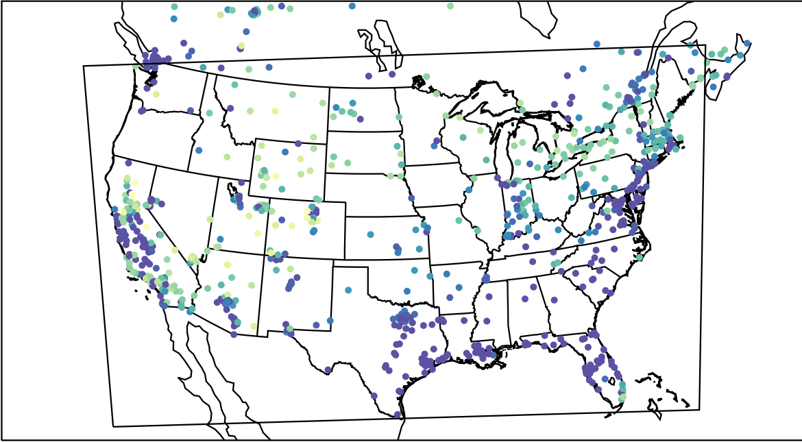
AirNOW (2023-01-31_09:00:00)
