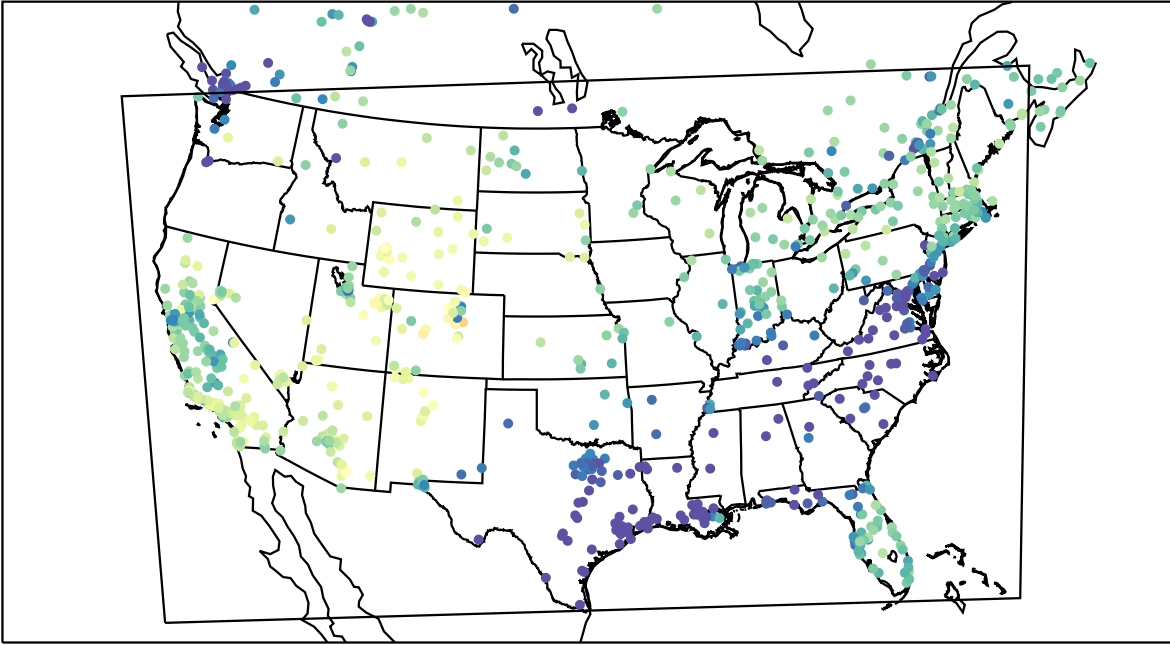
AirNOW (2023-01-31_22:00:00)
