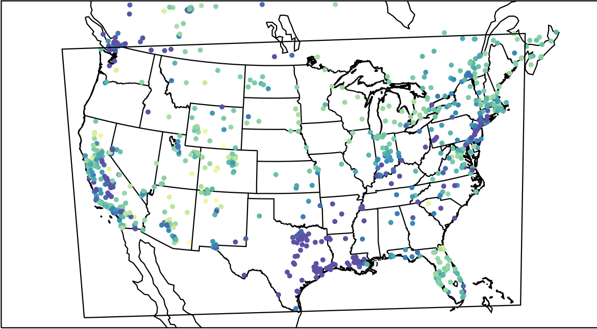
AirNOW (2023-01-30_17:00:00)
