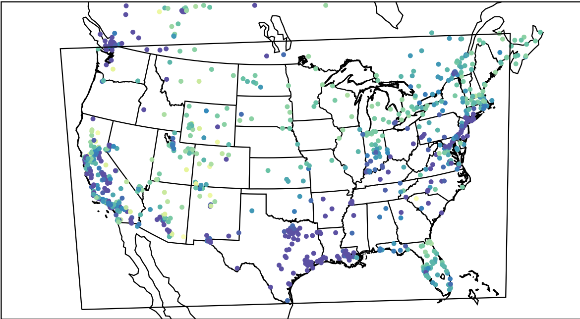
AirNOW (2023-01-30_16:00:00)
