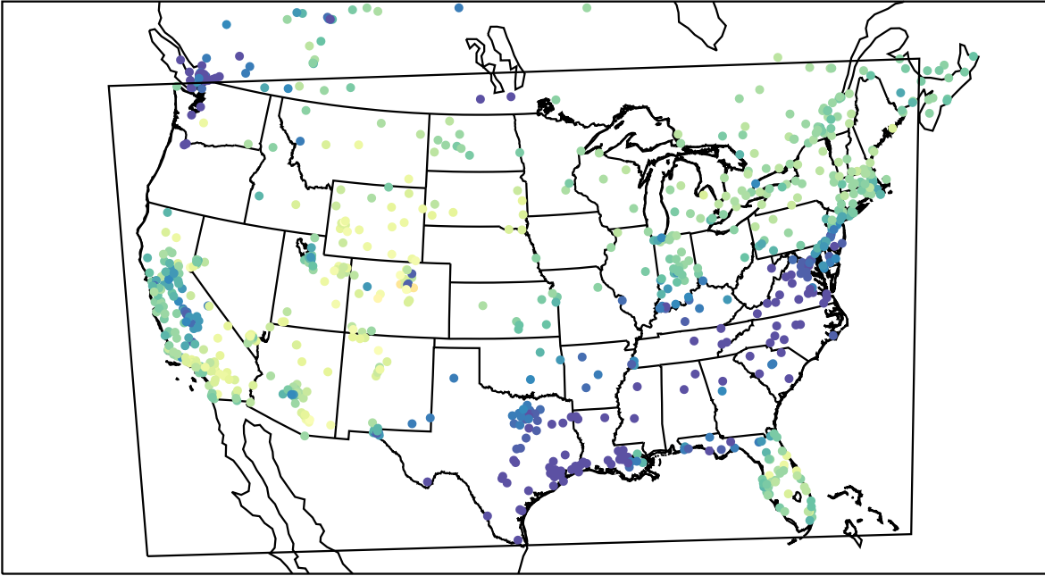
AirNOW (2023-01-31_20:00:00)
