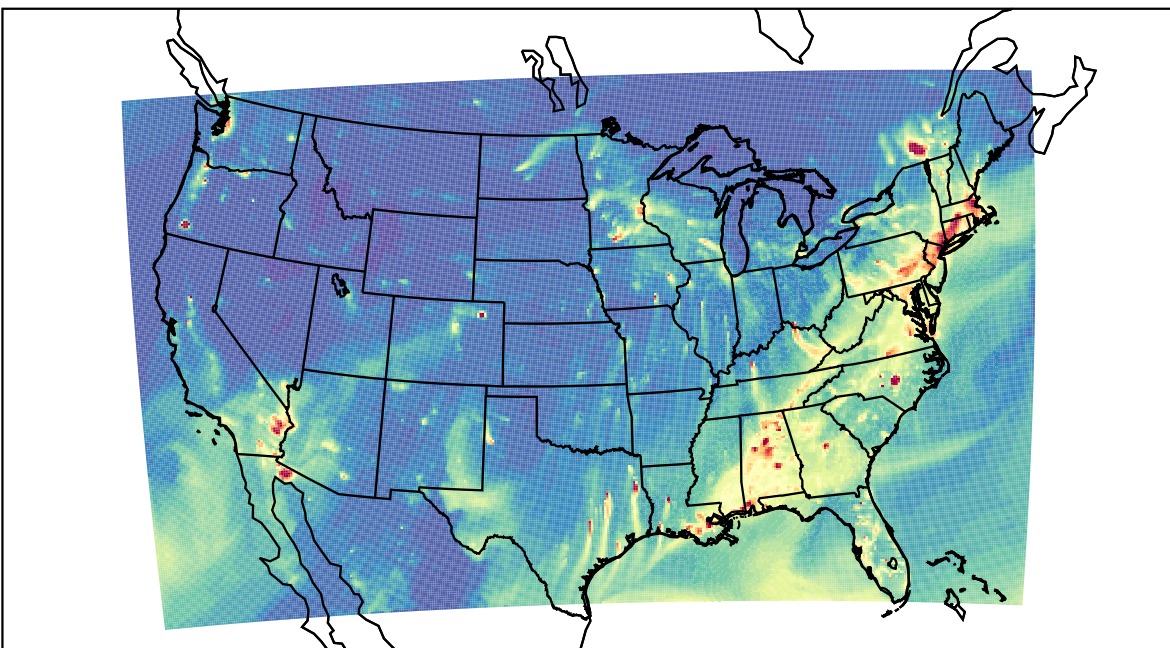
WRF 2023-01-31_02:00:00
