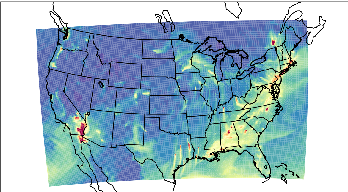
WRF 2023-01-31_06:00:00
