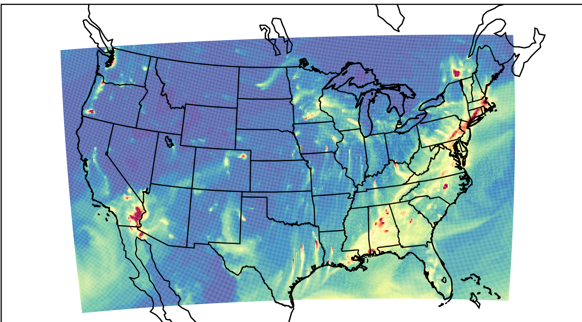
WRF 2023-01-31_04:00:00
