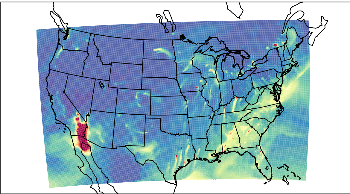
WRF 2023-01-31_15:00:00
