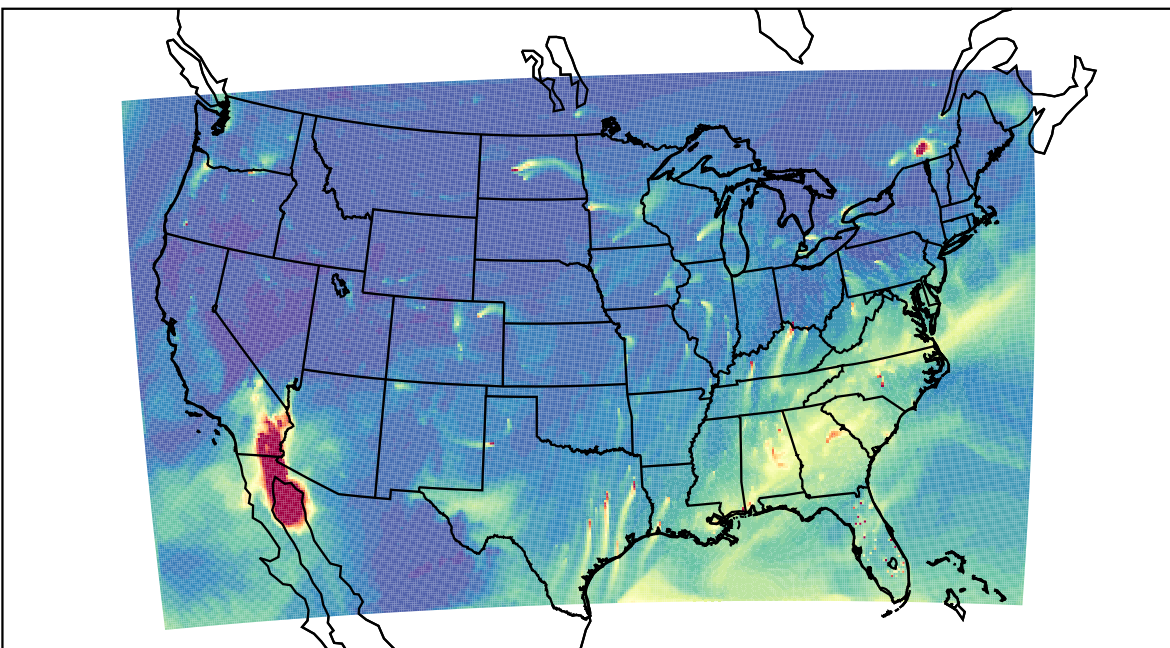
WRF 2023-01-31_20:00:00
