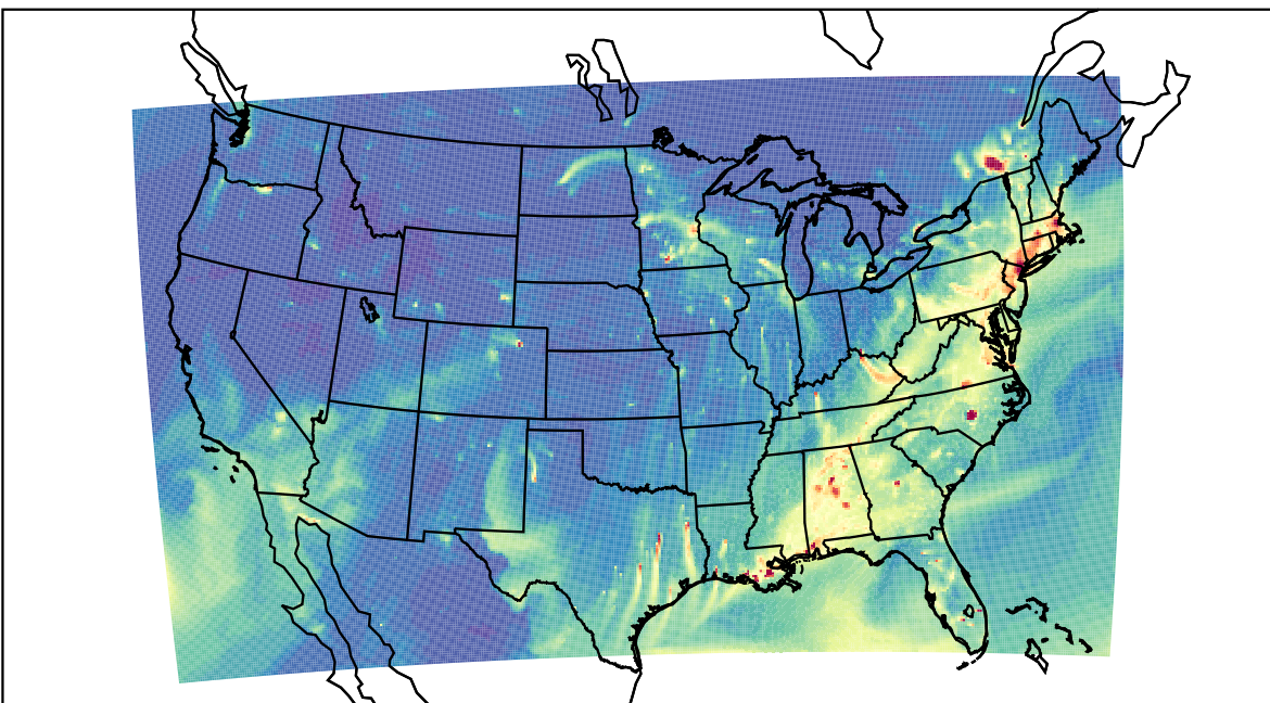
WRF 2023-01-31_00:00:00
