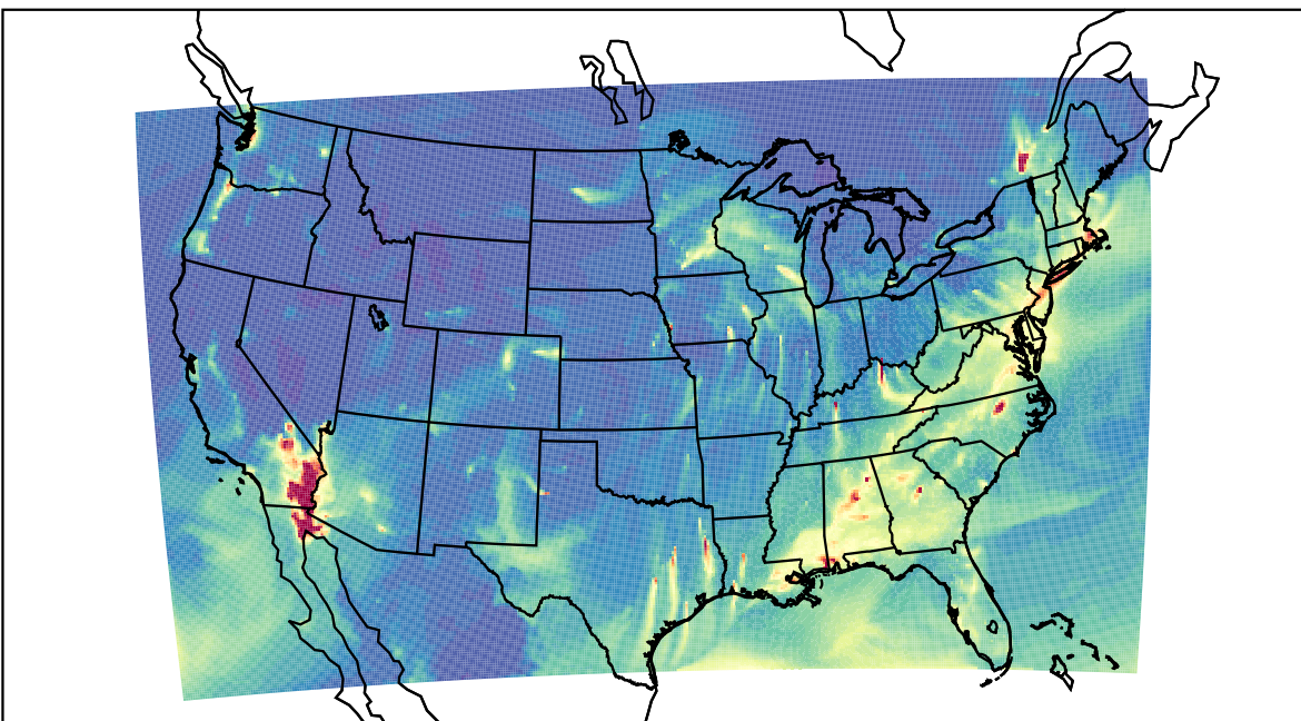
WRF 2023-01-31_07:00:00
