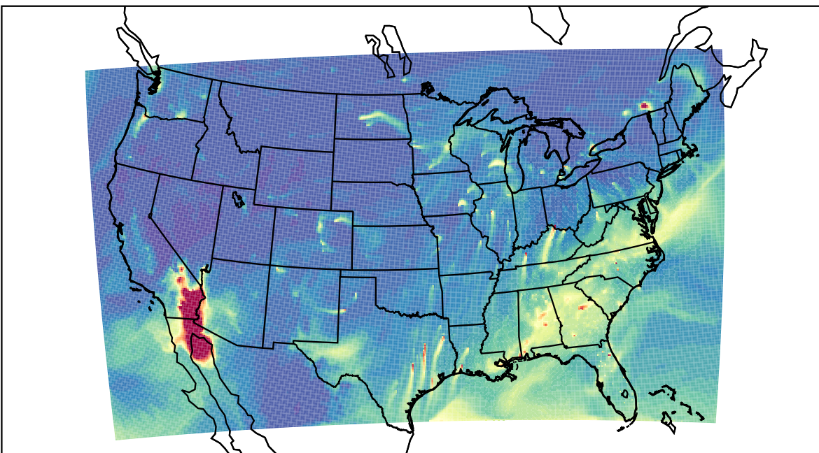
WRF 2023-01-31_17:00:00
