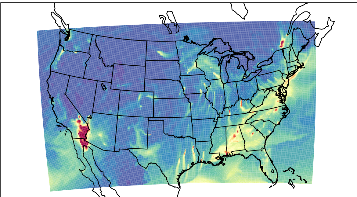
WRF 2023-01-31_09:00:00
