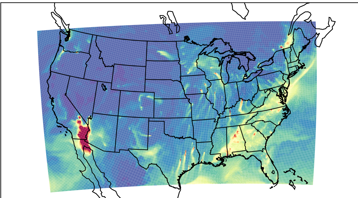
WRF 2023-01-31_12:00:00
