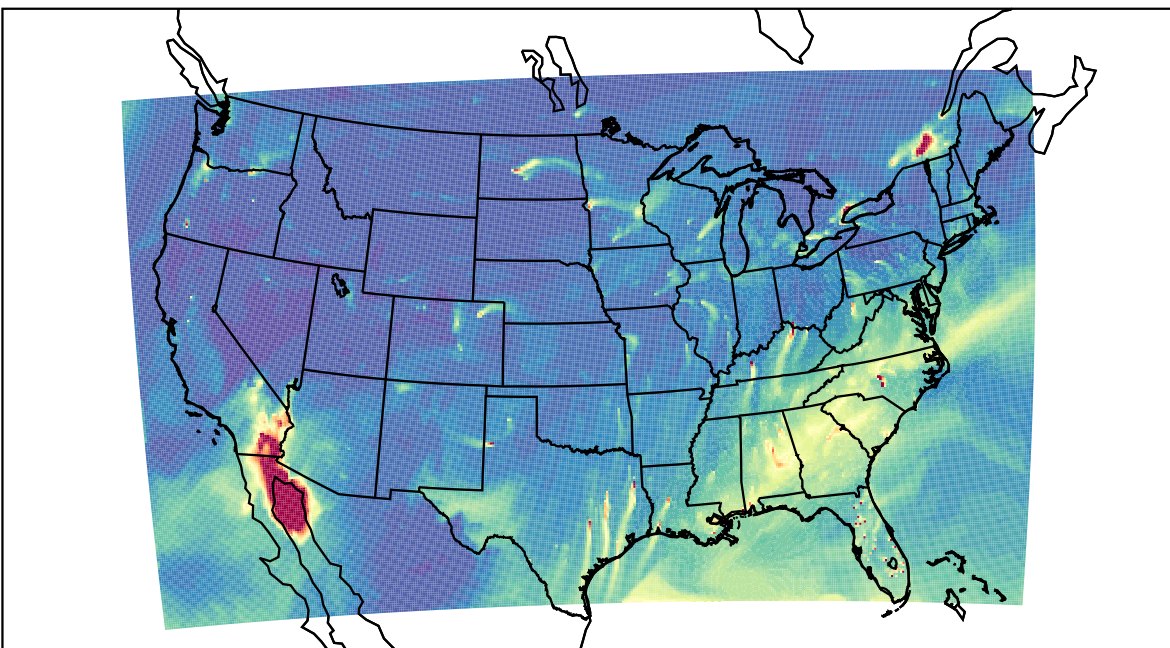
WRF 2023-01-31_22:00:00
