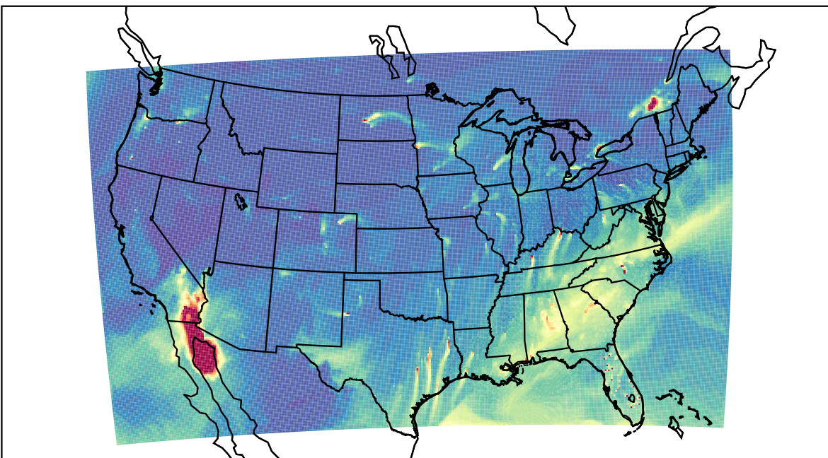
WRF 2023-01-31_21:00:00
