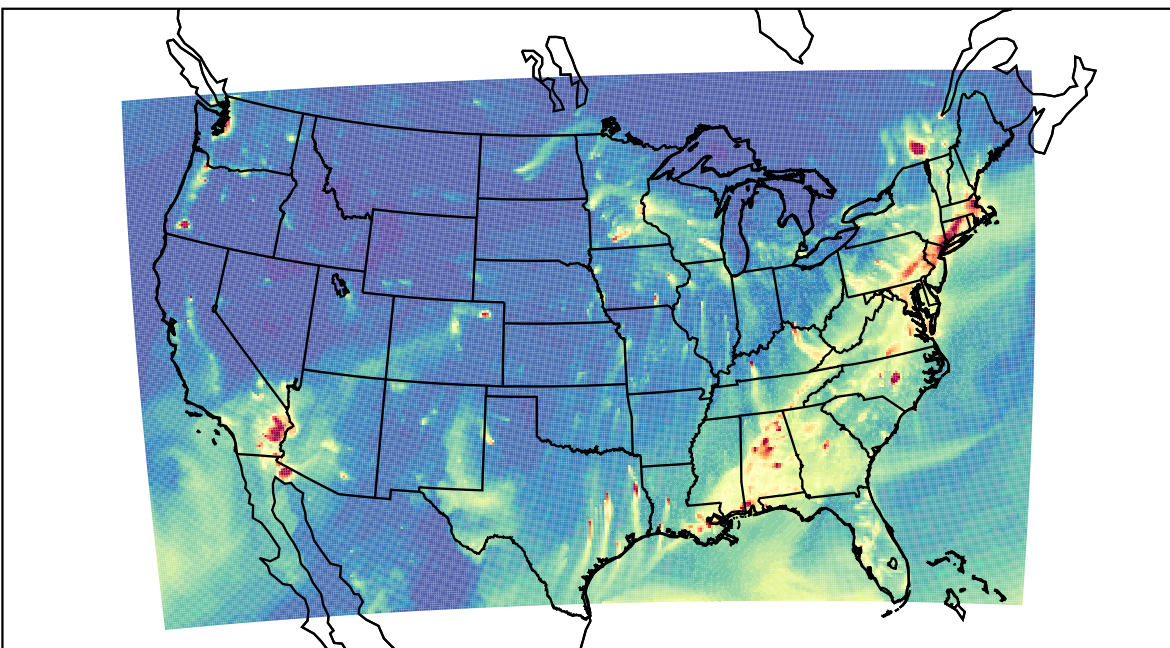
WRF 2023-01-31_03:00:00
