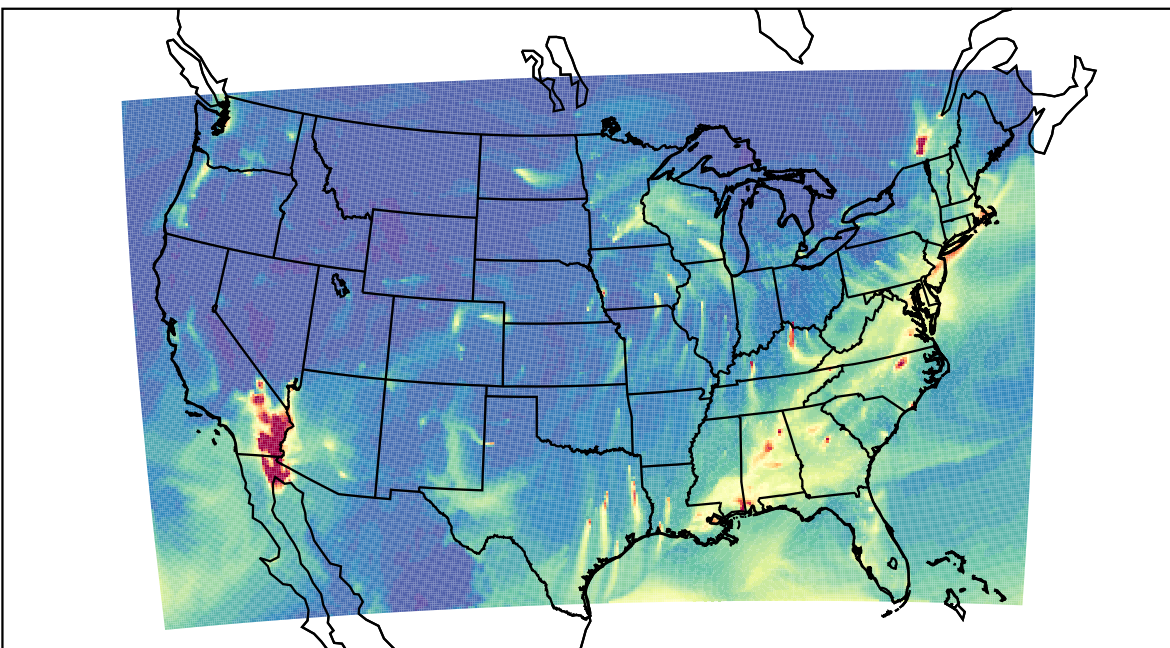
WRF 2023-01-31_08:00:00
