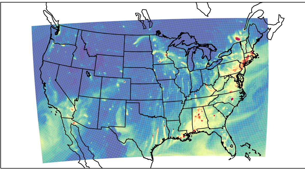
WRF 2023-01-31_01:00:00
