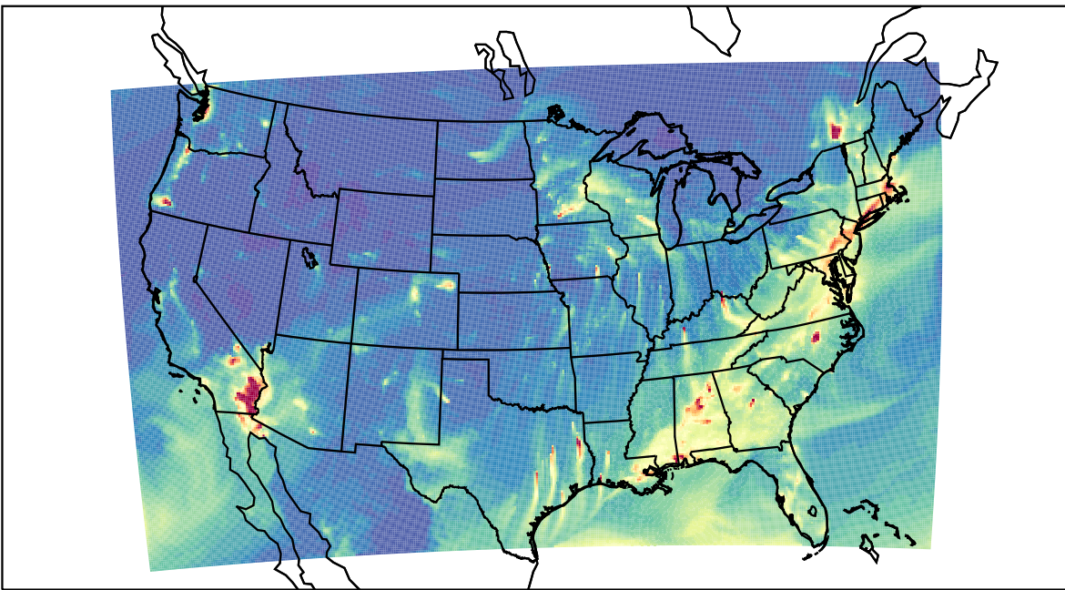
WRF 2023-01-31_05:00:00
