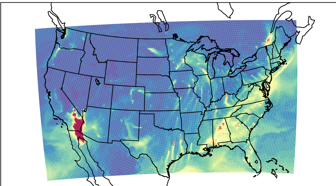
WRF 2023-01-31_11:00:00
