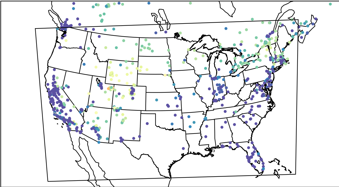
AirNOW (2023-02-02_07:00:00)
