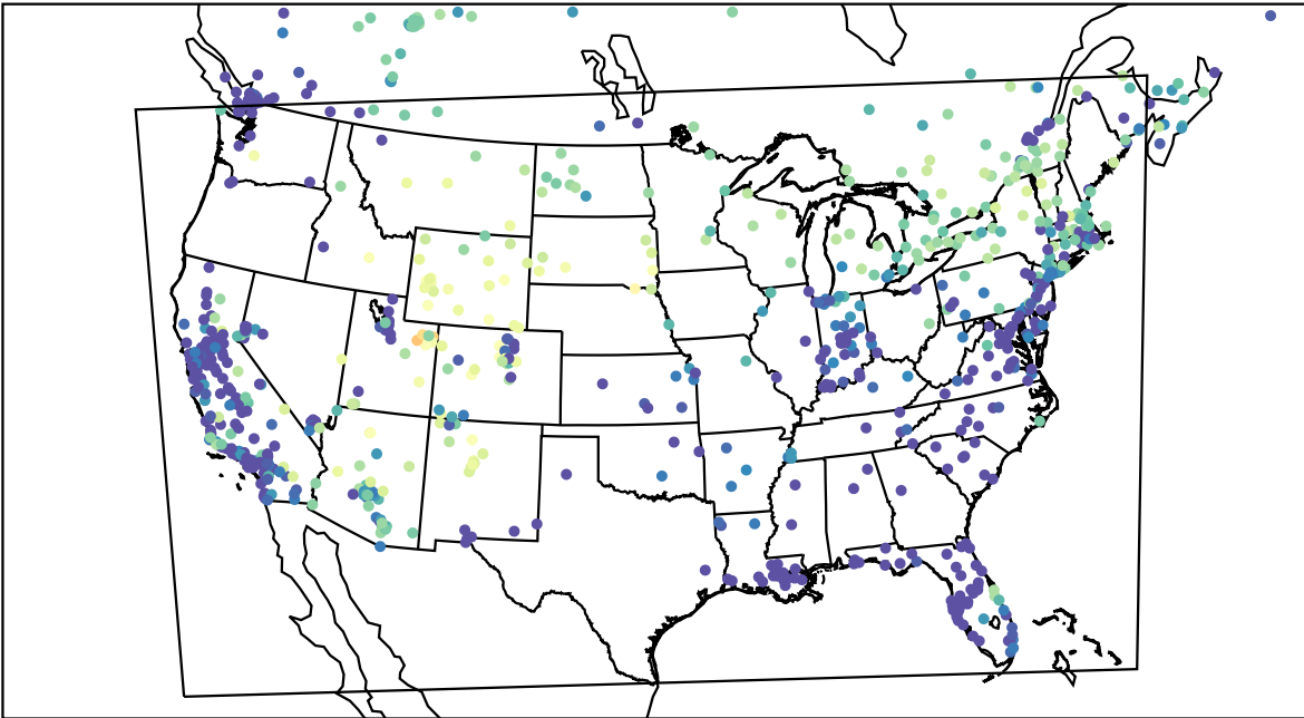
AirNOW (2023-02-02_03:00:00)
