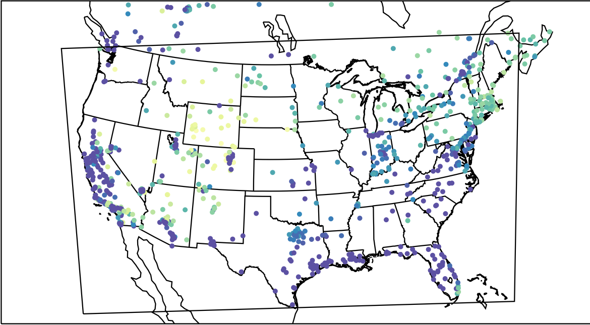
AirNOW (2023-02-01_06:00:00)
