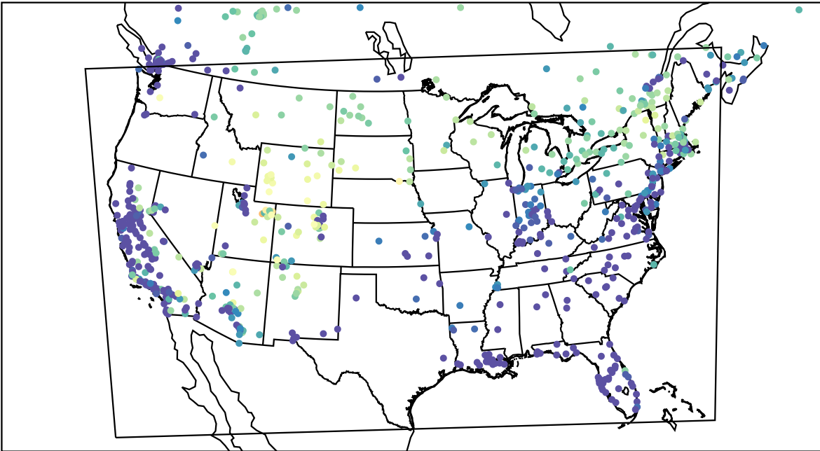
AirNOW (2023-02-02_06:00:00)
