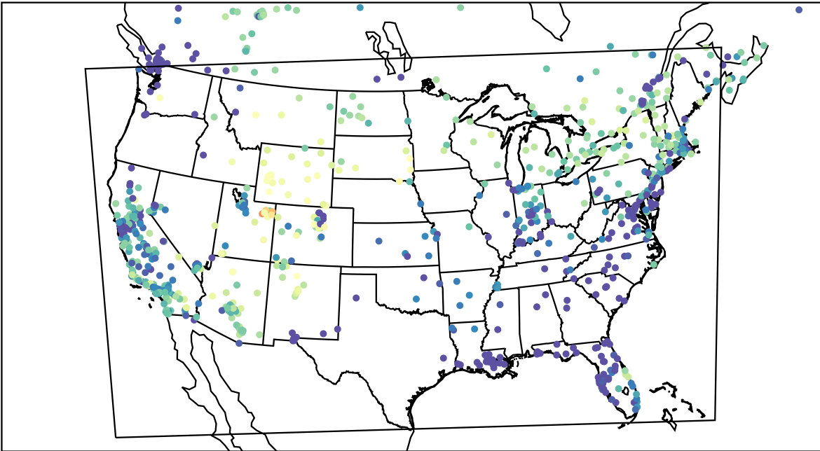
AirNOW (2023-02-02_01:00:00)
