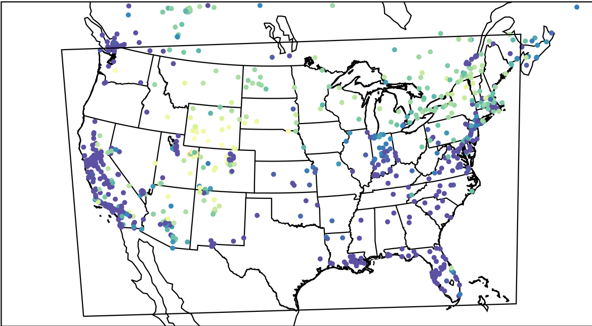
AirNOW (2023-02-02_05:00:00)
