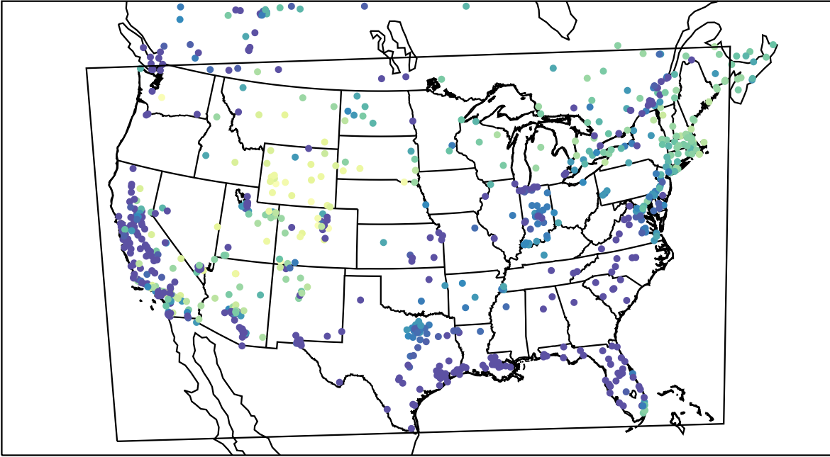
AirNOW (2023-02-01_07:00:00)
