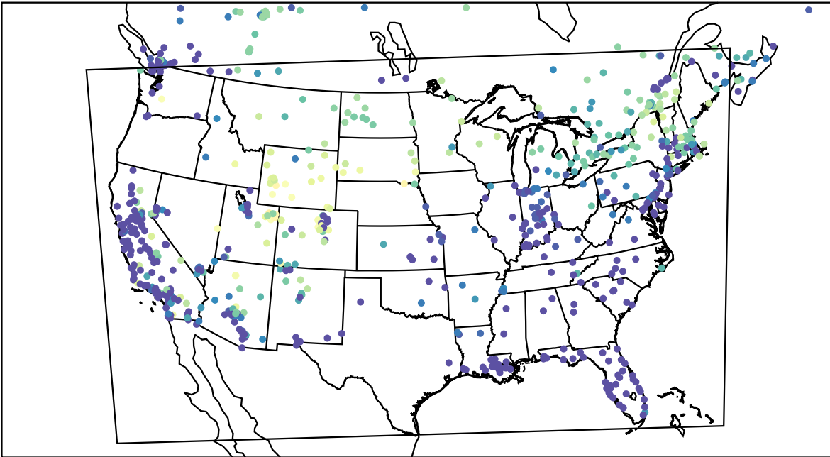
AirNOW (2023-02-02_09:00:00)
