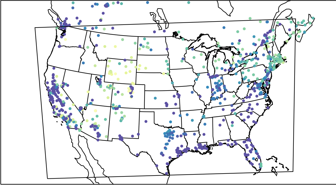
AirNOW (2023-02-01_09:00:00)
