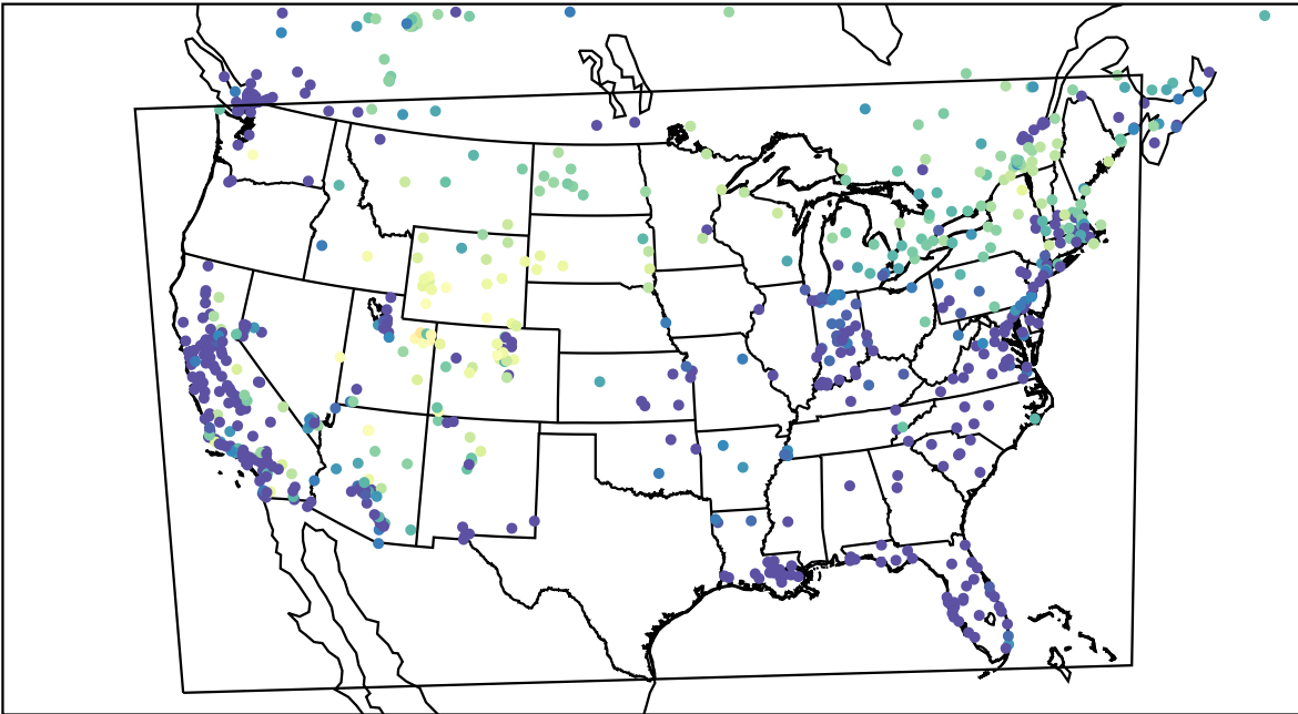
AirNOW (2023-02-02_08:00:00)
