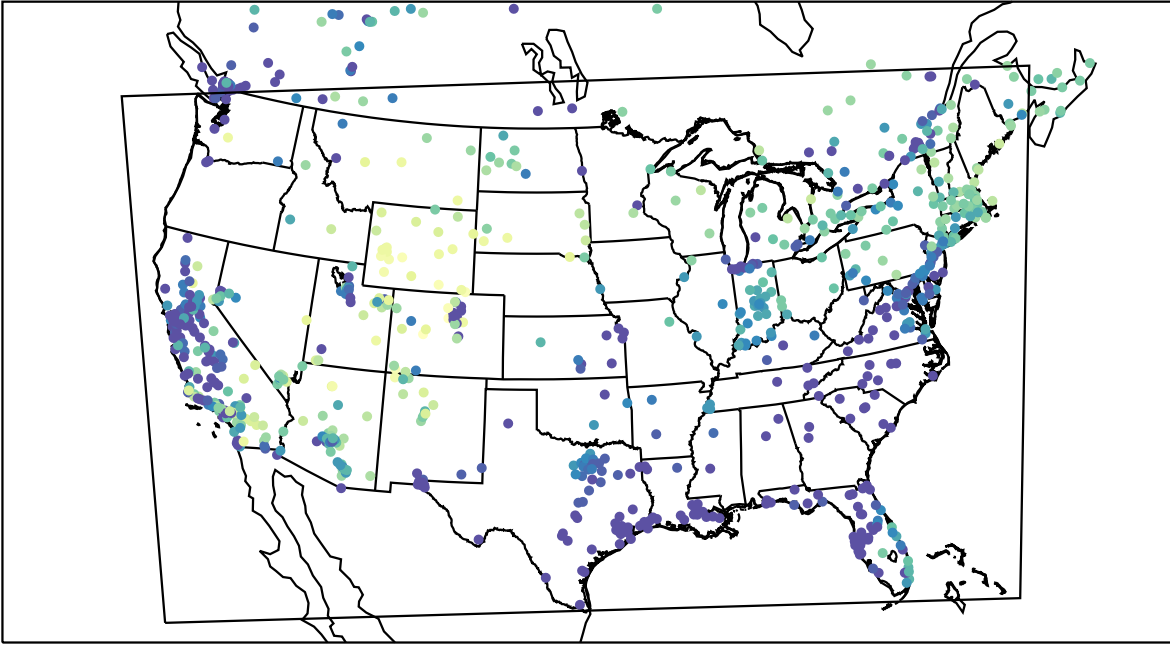
AirNOW (2023-02-01_02:00:00)
