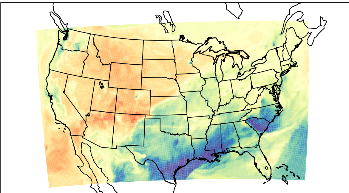
WRF (2023-02-01_21:00:00)
