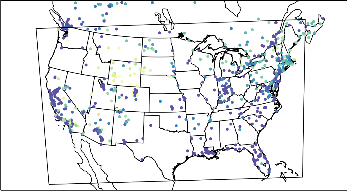
AirNOW (2023-02-01_12:00:00)
