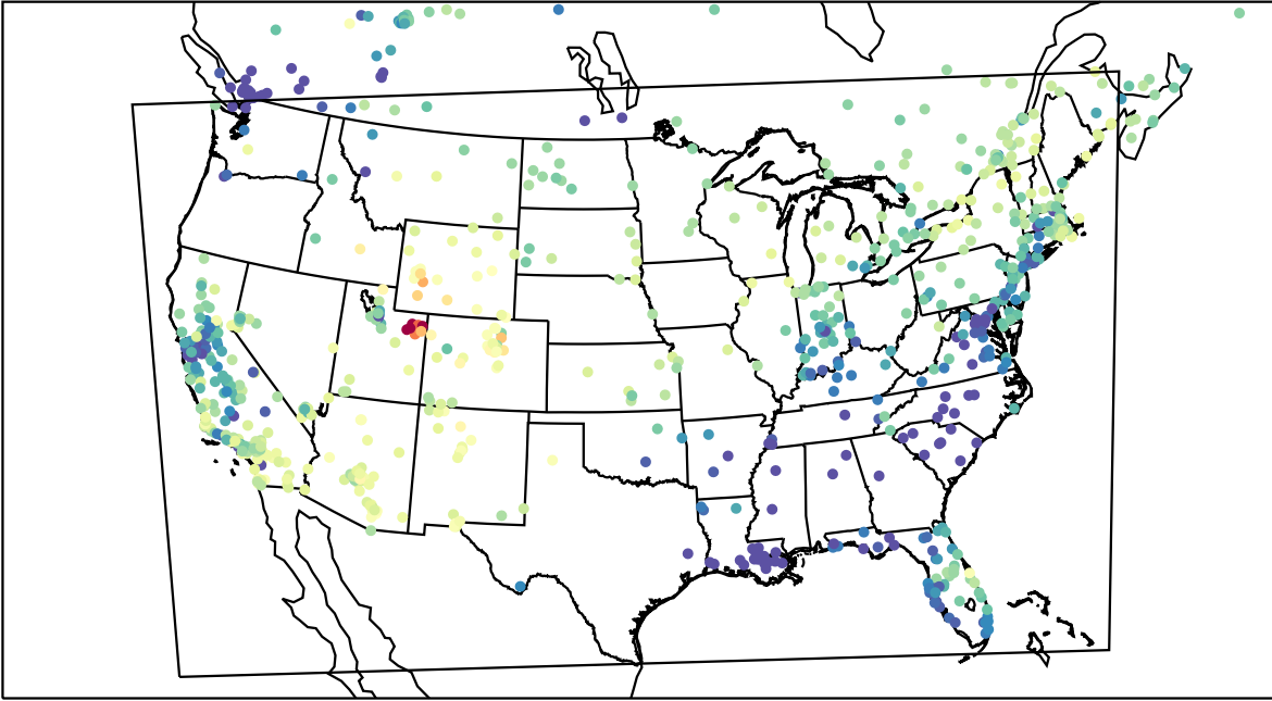
AirNOW (2023-02-02_22:00:00)
