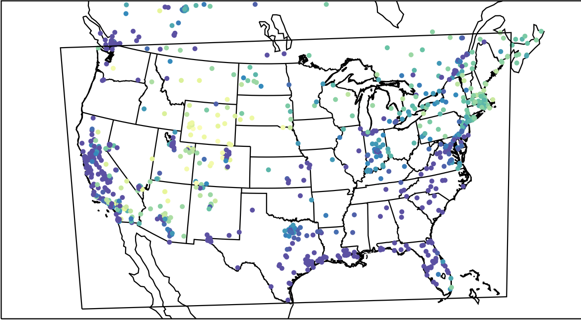
AirNOW (2023-02-01_05:00:00)
