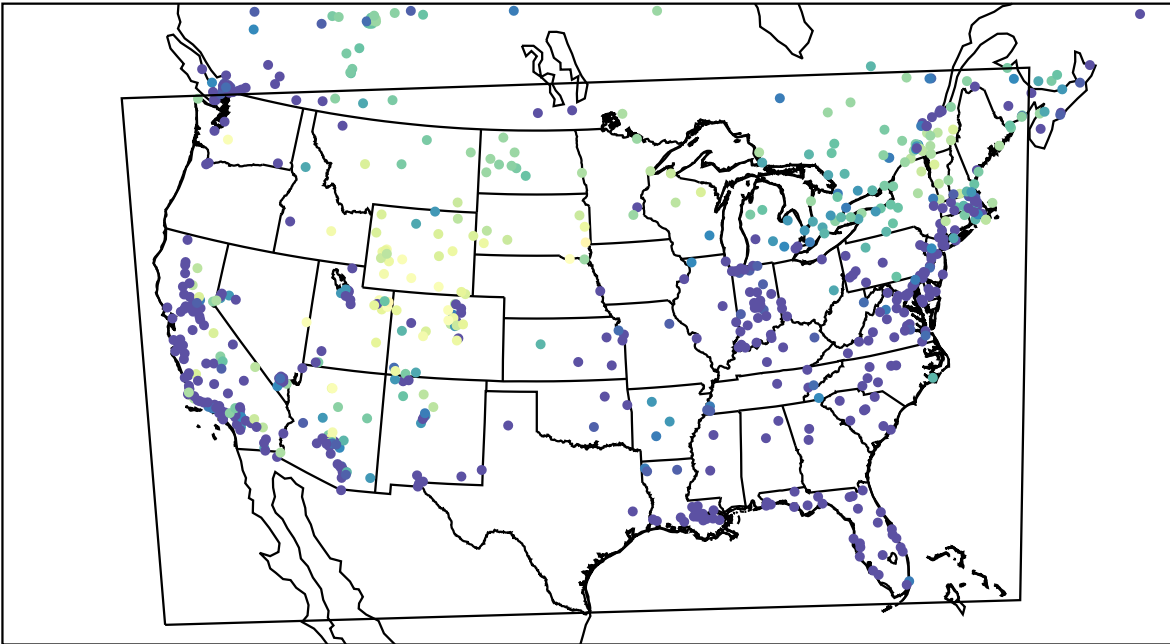
AirNOW (2023-02-02_11:00:00)
