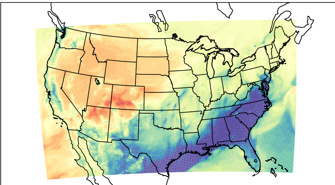
WRF (2023-02-01_09:00:00)
