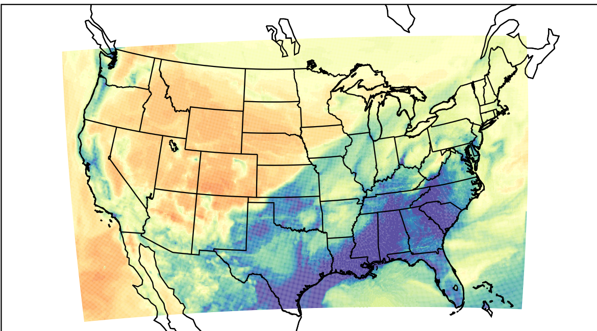
WRF (2023-02-02_08:00:00)
