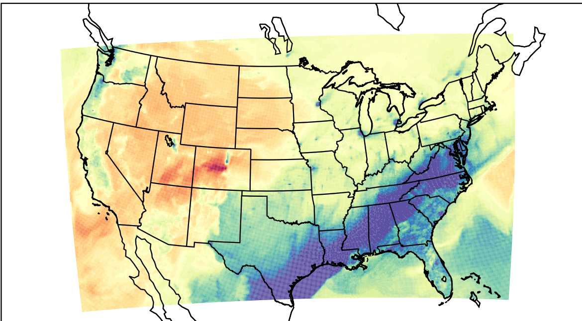
WRF (2023-02-01_00:00:00)
