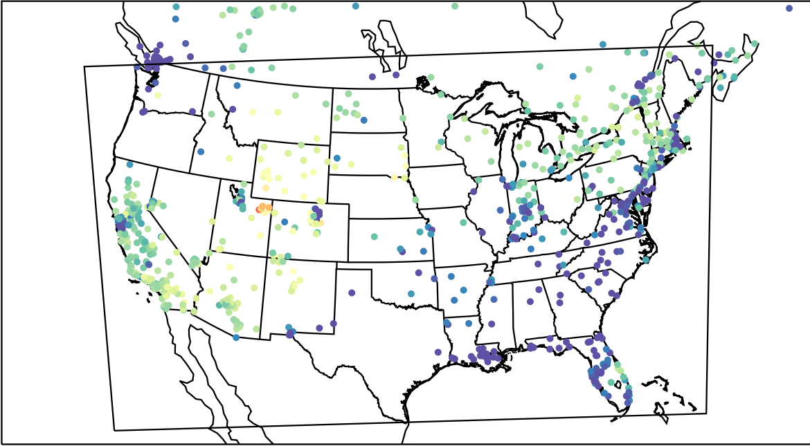
AirNOW (2023-02-02_00:00:00)
