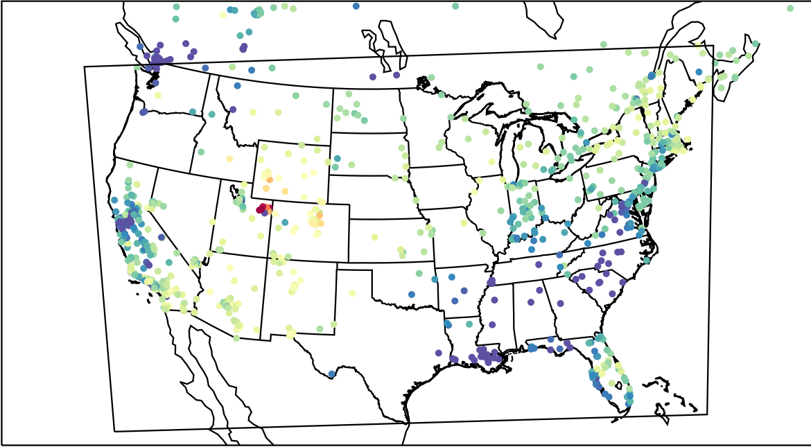
AirNOW (2023-02-02_21:00:00)
