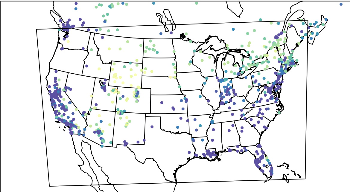
AirNOW (2023-02-02_04:00:00)
