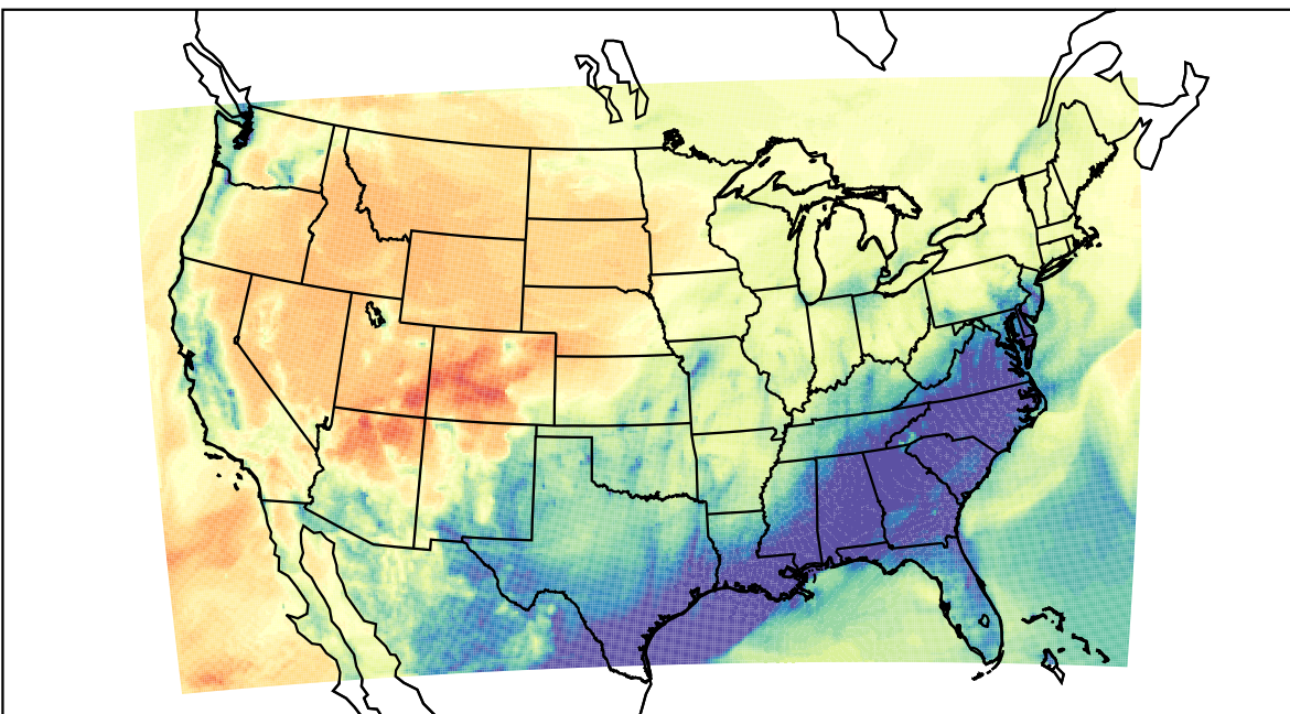
WRF (2023-02-01_07:00:00)
