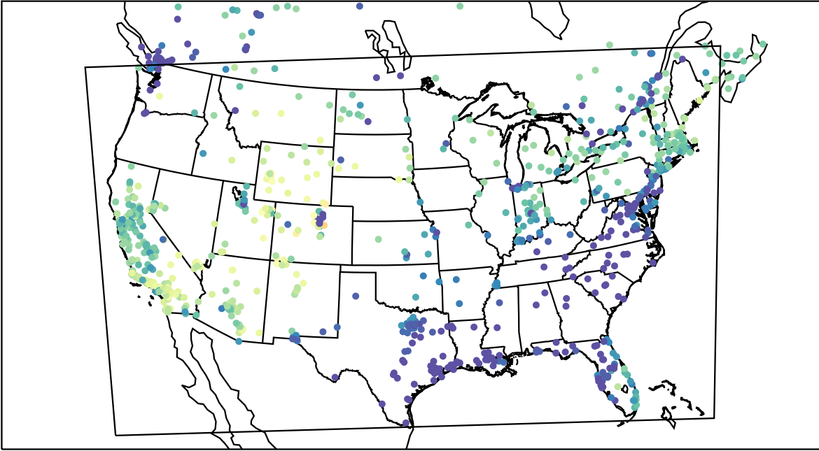
AirNOW (2023-02-01_00:00:00)
