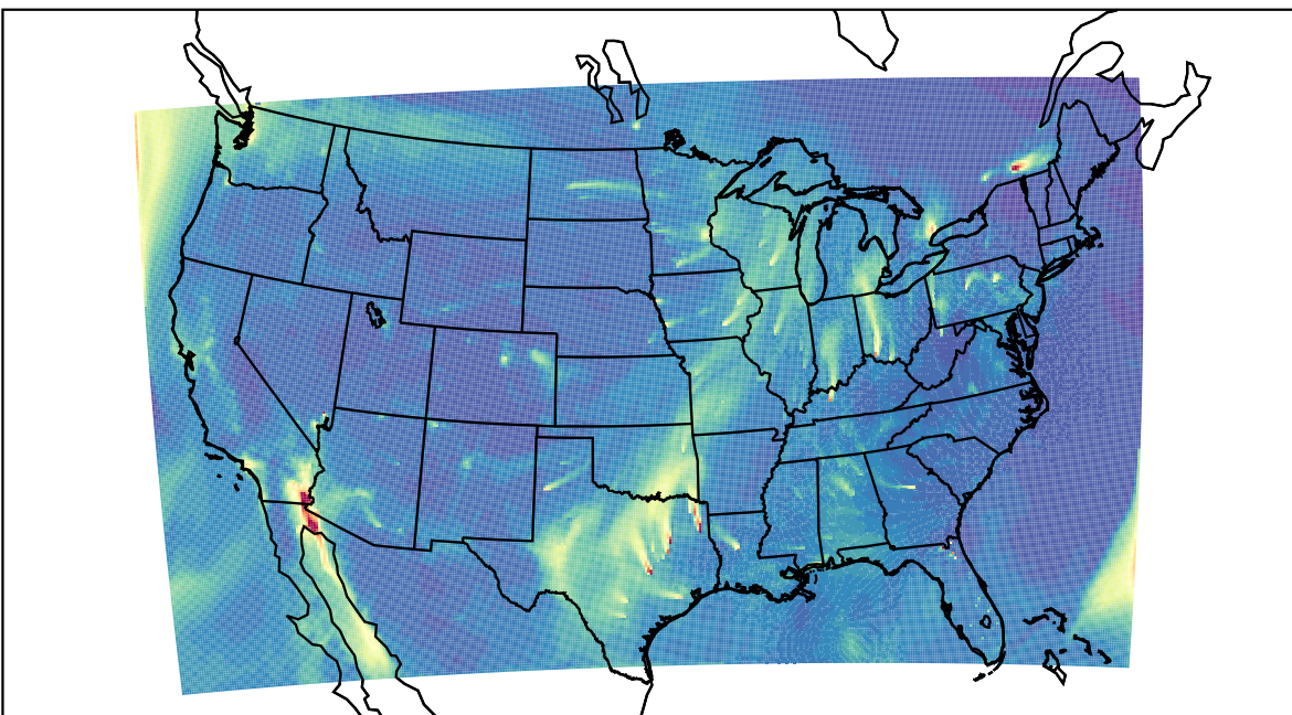
WRF 2023-02-04_17:00:00
