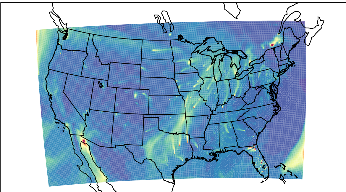
WRF 2023-02-04_21:00:00
