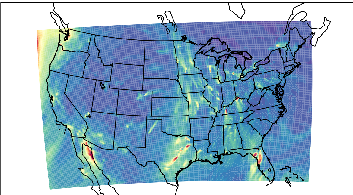
WRF 2023-02-04_05:00:00
