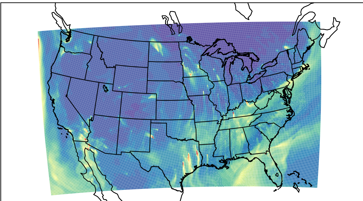
WRF 2023-02-03_09:00:00
