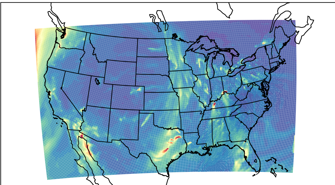
WRF 2023-02-04_07:00:00
