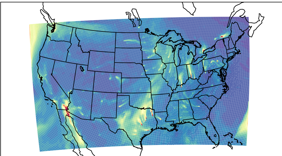
WRF 2023-02-04_16:00:00
