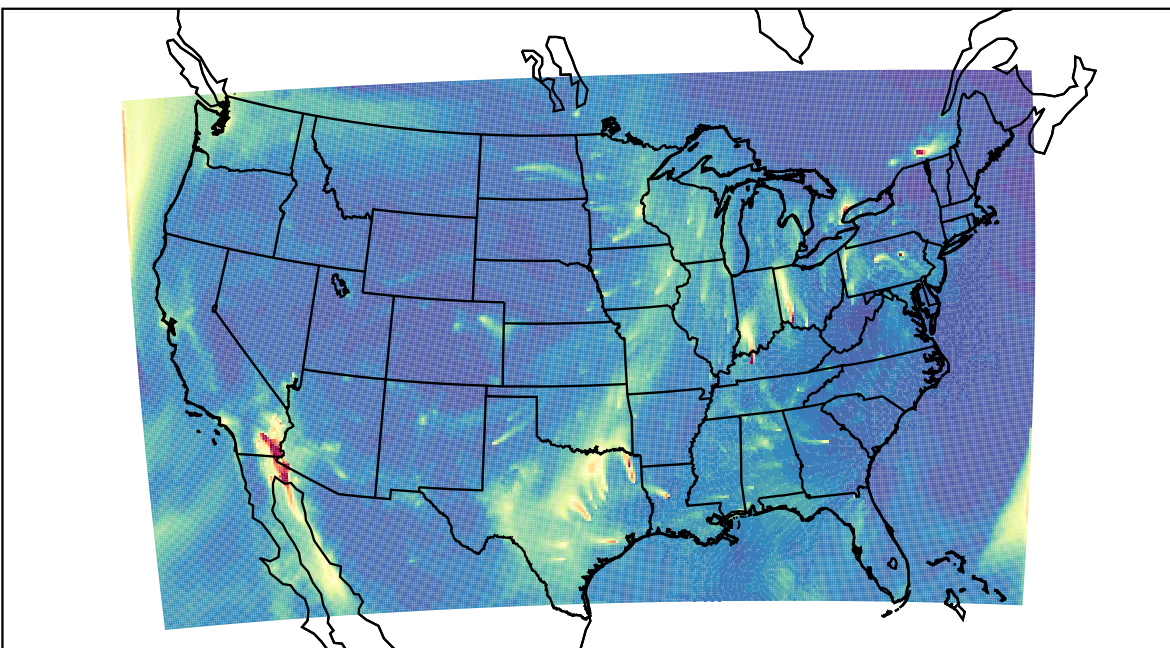
WRF 2023-02-04_15:00:00
