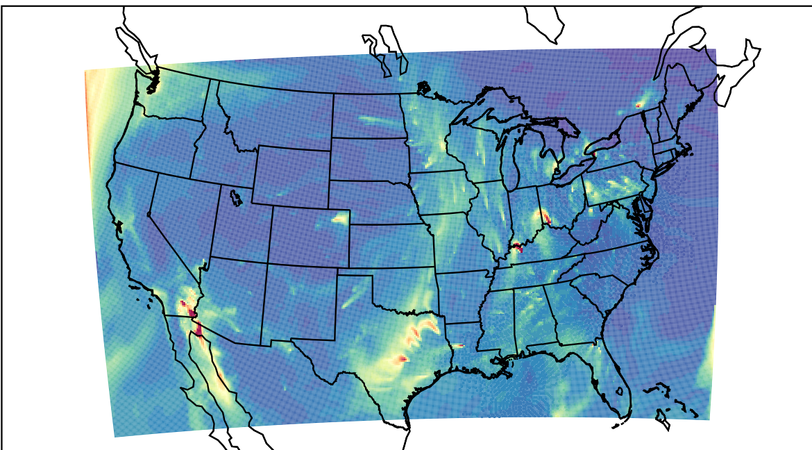
WRF 2023-02-04_11:00:00
