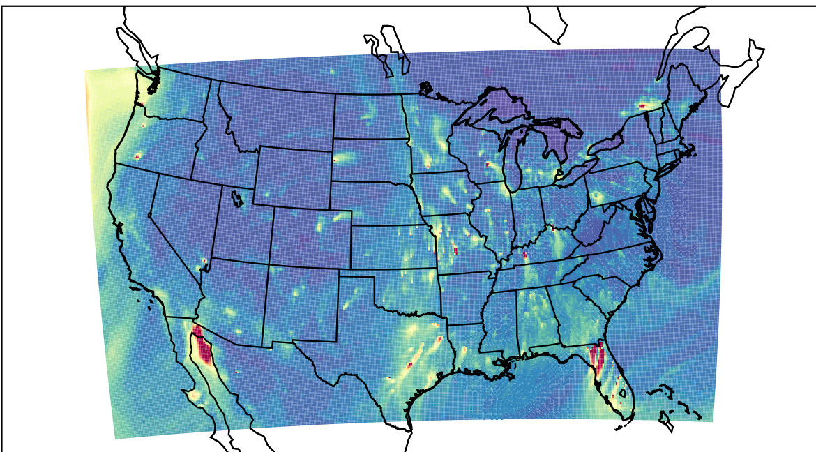
WRF 2023-02-04_01:00:00
