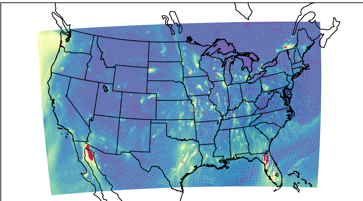
WRF 2023-02-04_00:00:00
