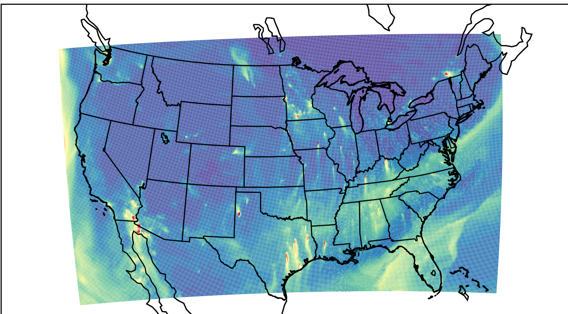
WRF 2023-02-03_12:00:00
