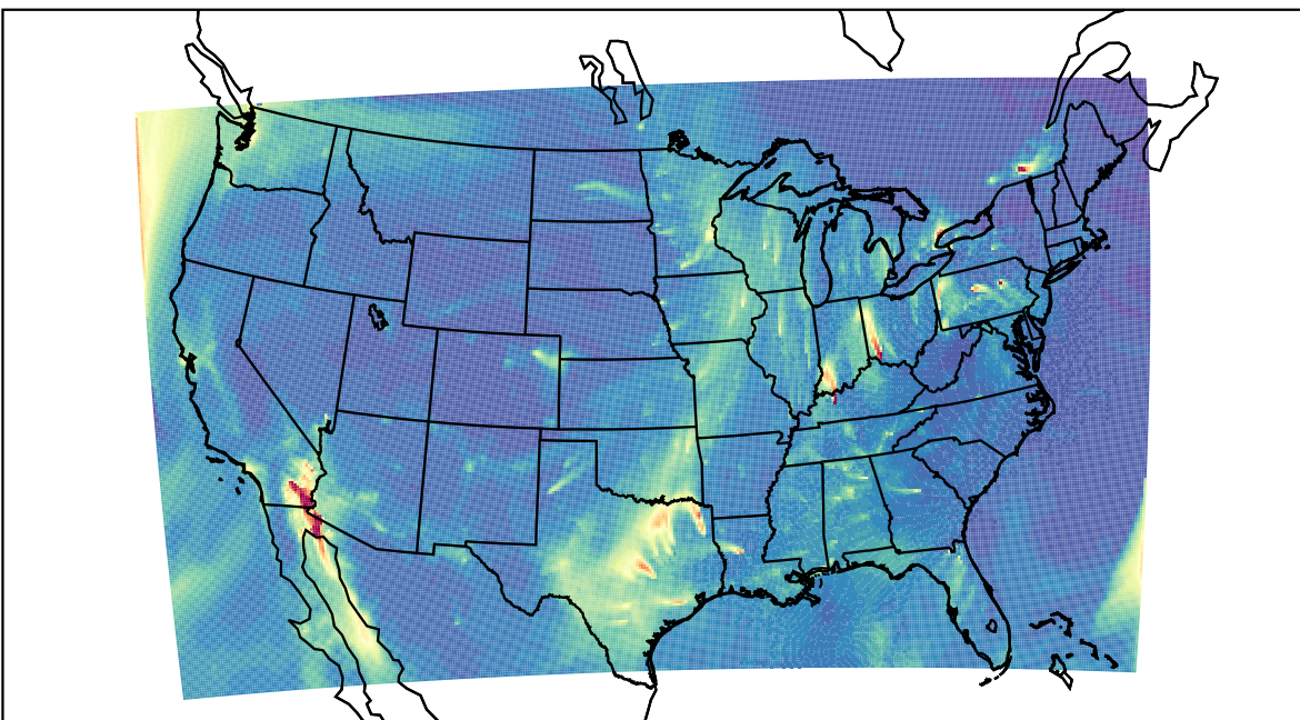
WRF 2023-02-04_14:00:00
