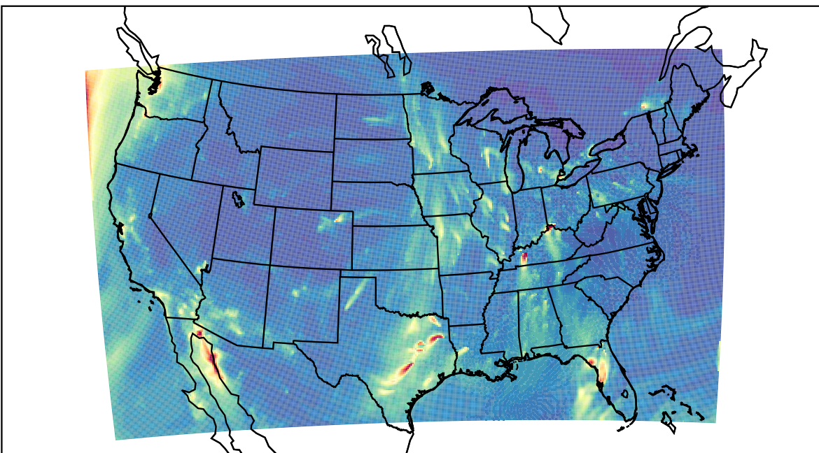
WRF 2023-02-04_06:00:00
