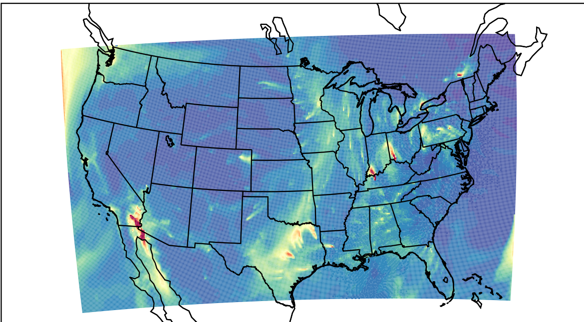
WRF 2023-02-04_13:00:00
