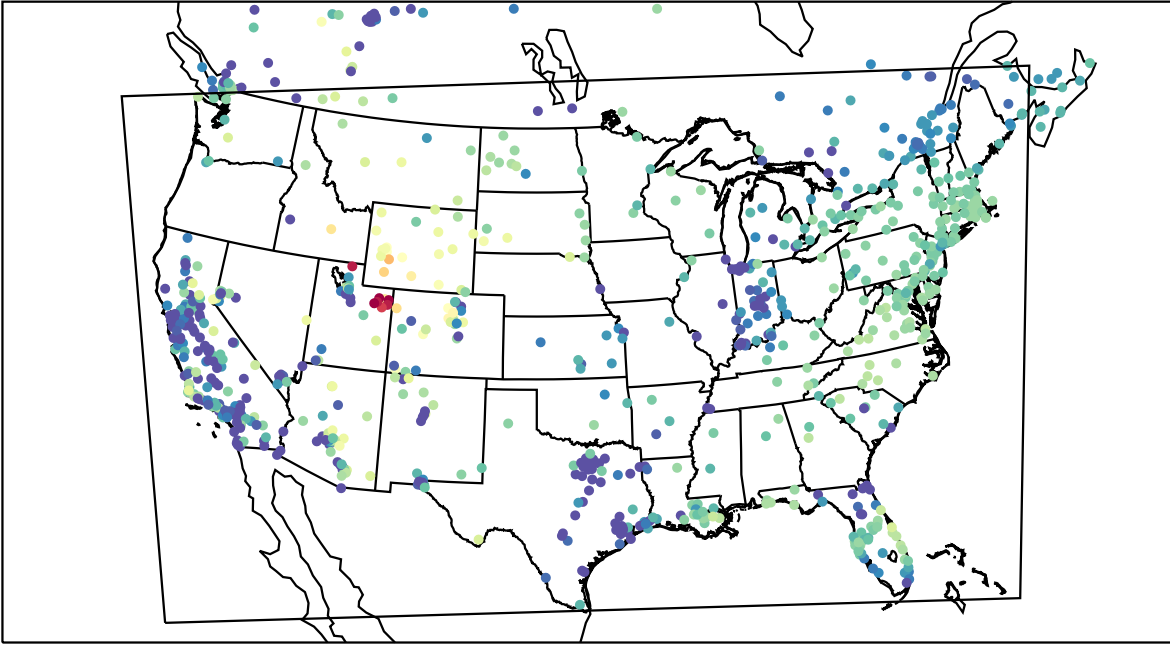
AirNOW (2023-02-04_02:00:00)
