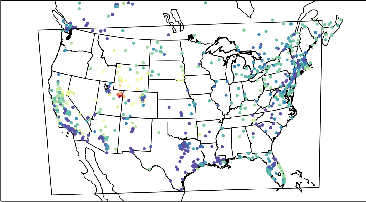
AirNOW (2023-02-05_10:00:00)
