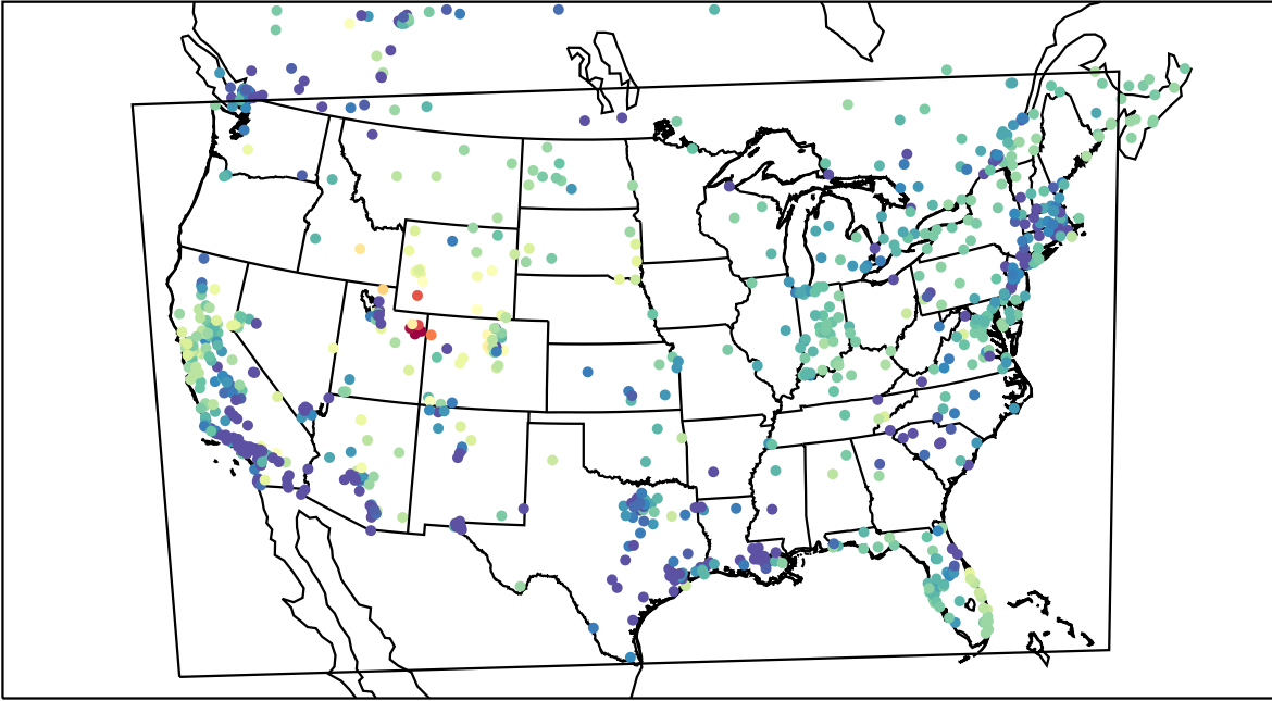
AirNOW (2023-02-05_06:00:00)
