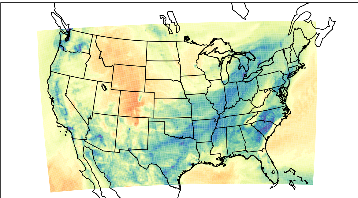
WRF (2023-02-05_16:00:00)
