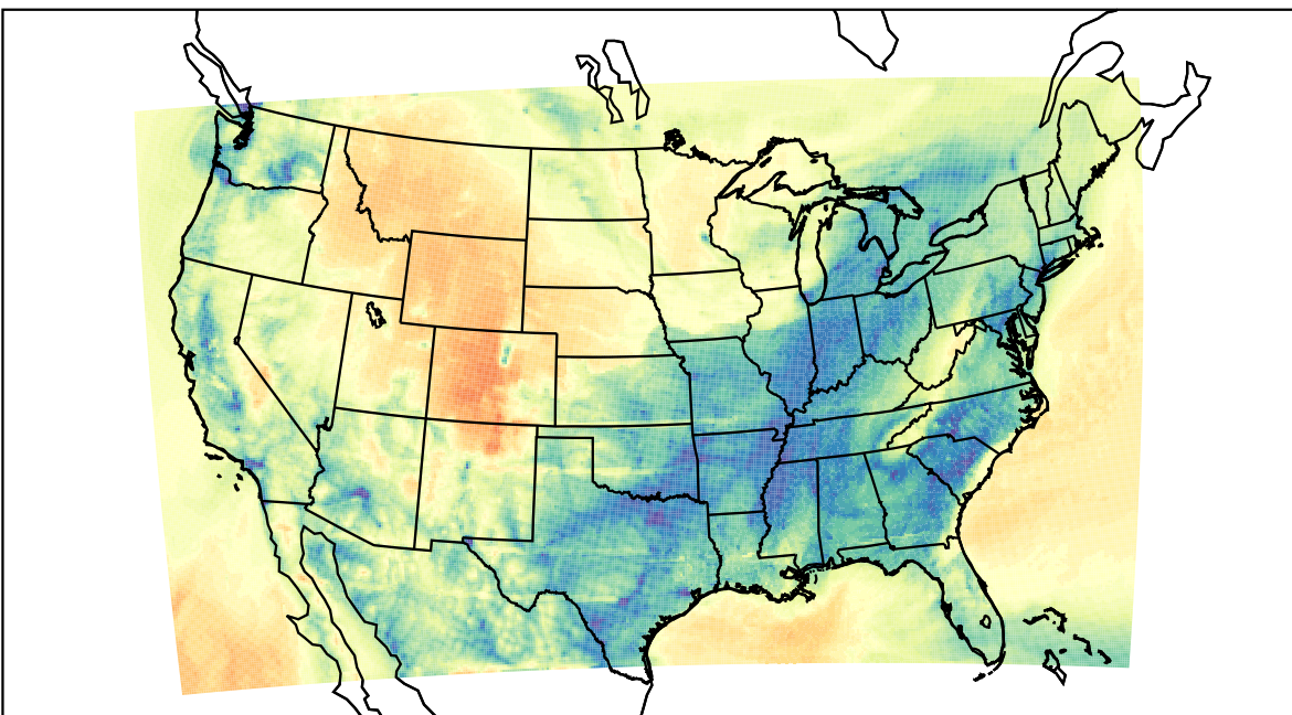
WRF (2023-02-05_15:00:00)
