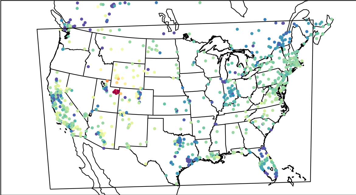
AirNOW (2023-02-04_00:00:00)
