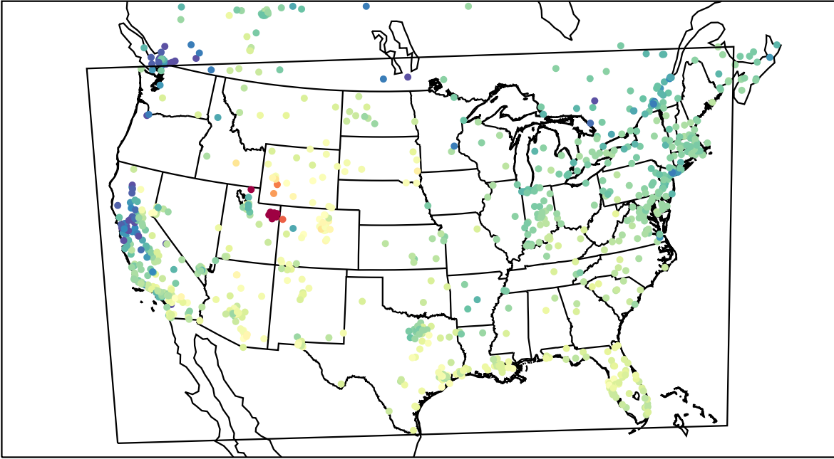
AirNOW (2023-02-04_20:00:00)
