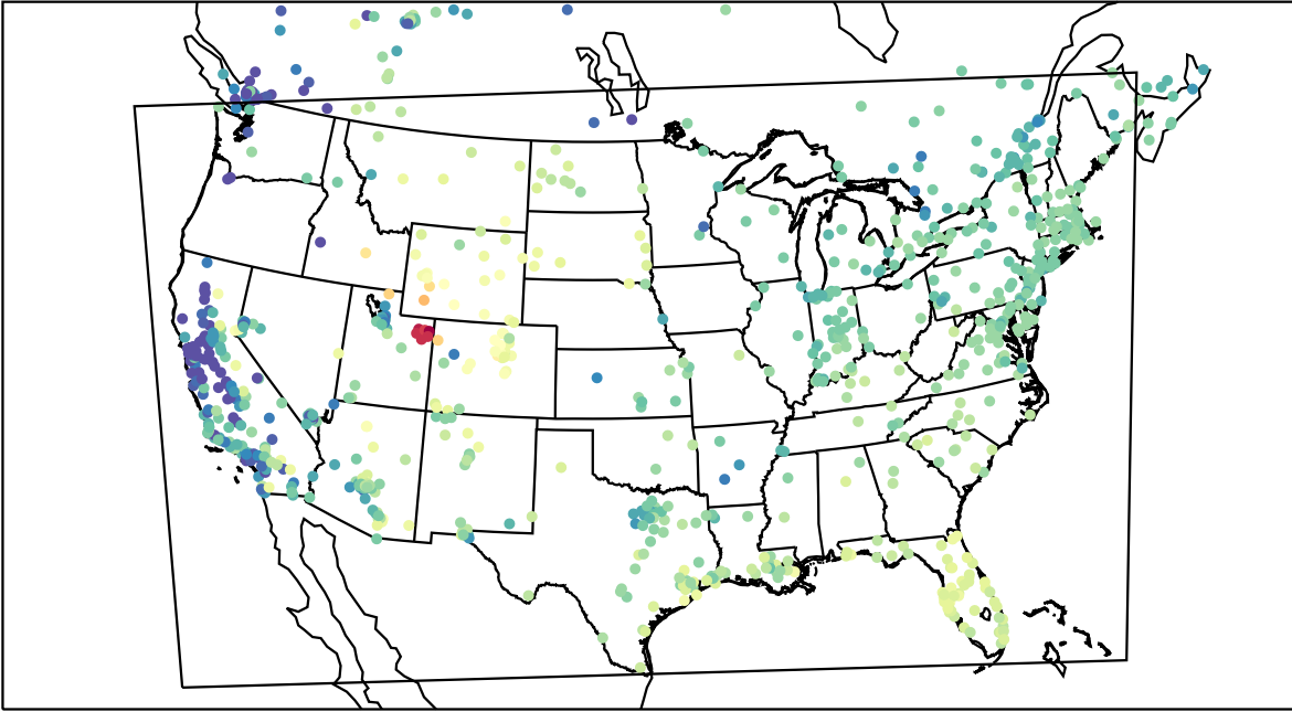
AirNOW (2023-02-04_18:00:00)
