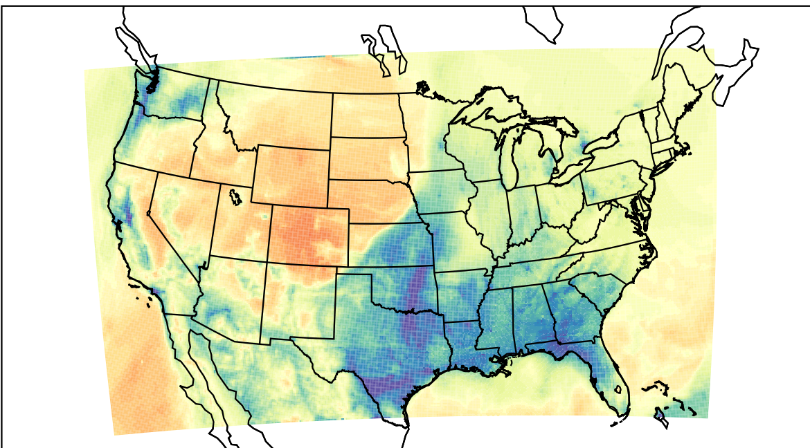
WRF (2023-02-04_12:00:00)
