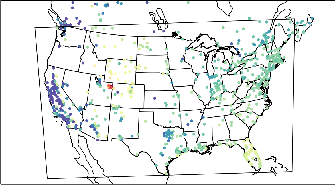
AirNOW (2023-02-04_17:00:00)
