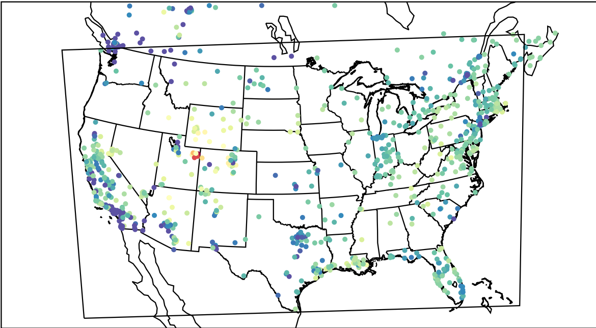
AirNOW (2023-02-05_16:00:00)
