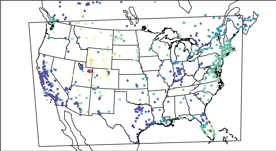
AirNOW (2023-02-04_07:00:00)
