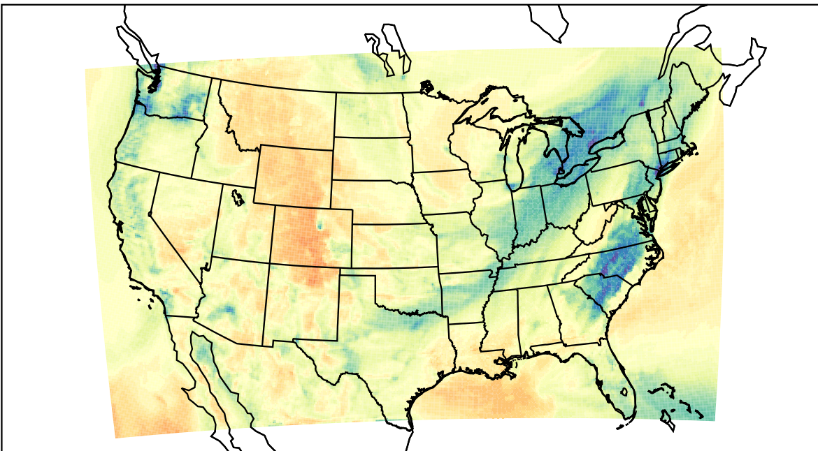
WRF (2023-02-05_19:00:00)
