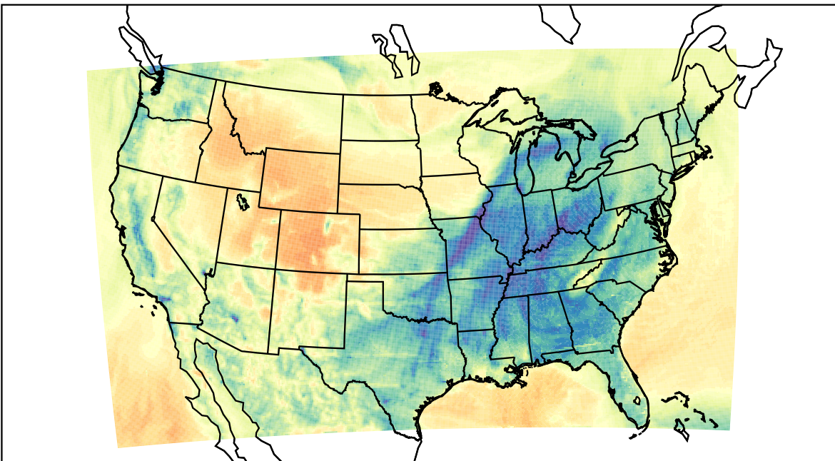
WRF (2023-02-05_07:00:00)
