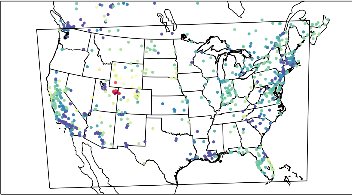
AirNOW (2023-02-05_05:00:00)
