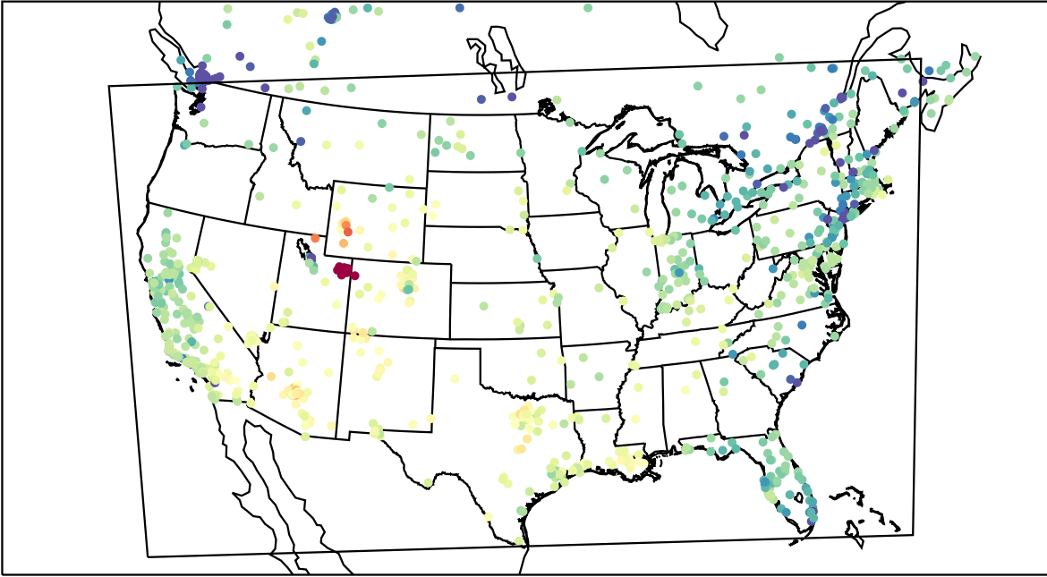
AirNOW (2023-02-05_22:00:00)
