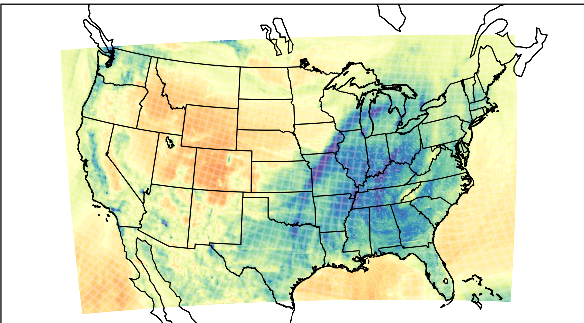
WRF (2023-02-05_05:00:00)
