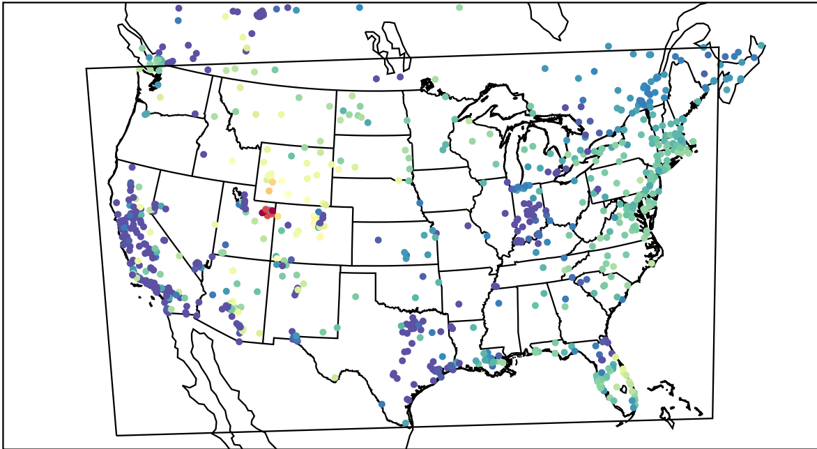
AirNOW (2023-02-04_06:00:00)
