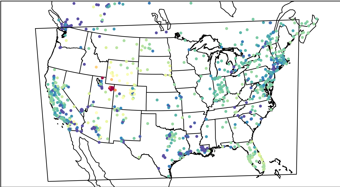
AirNOW (2023-02-05_02:00:00)
