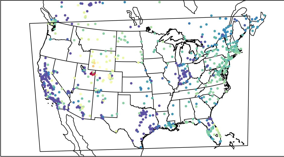
AirNOW (2023-02-04_05:00:00)
