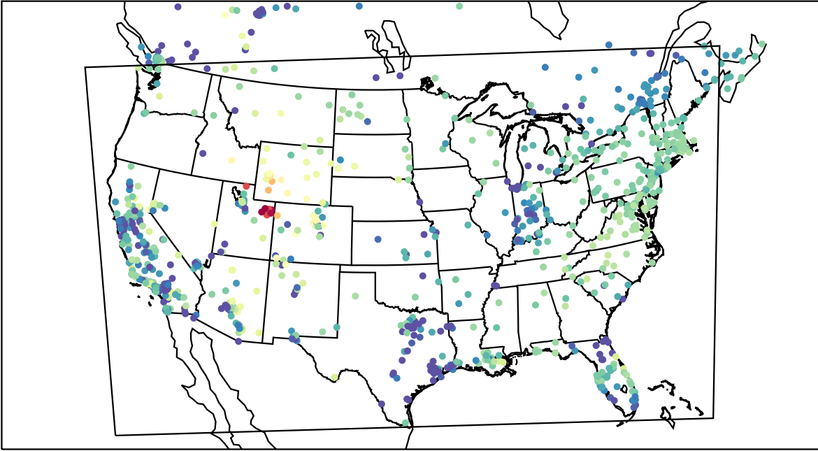
AirNOW (2023-02-04_01:00:00)
