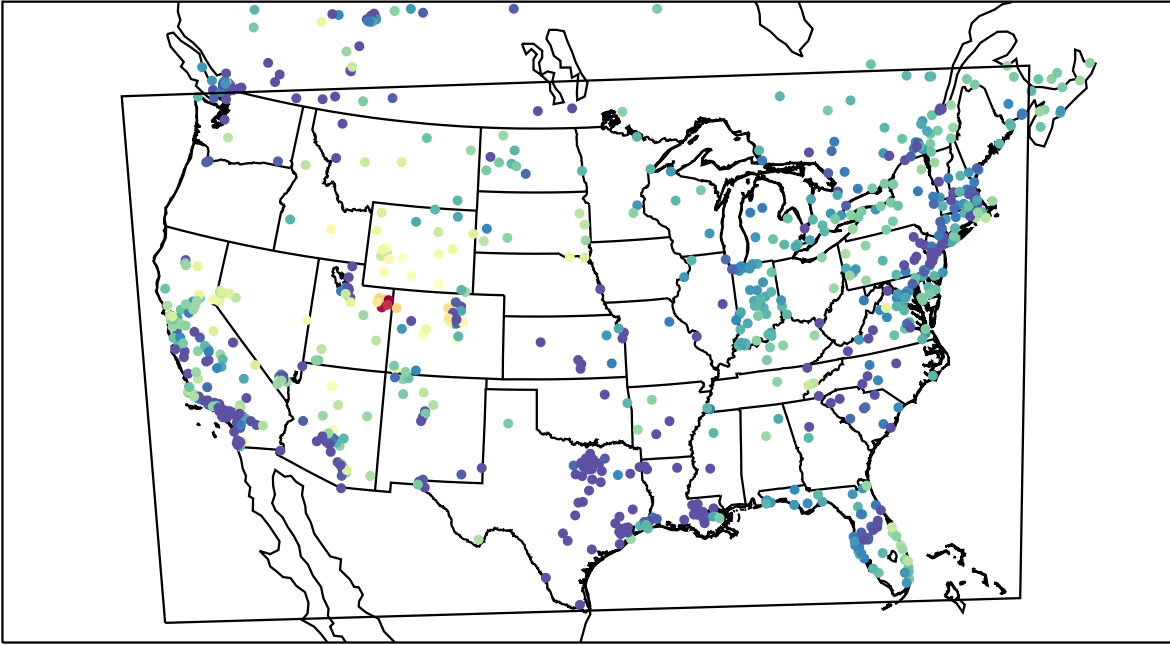
AirNOW (2023-02-05_12:00:00)
