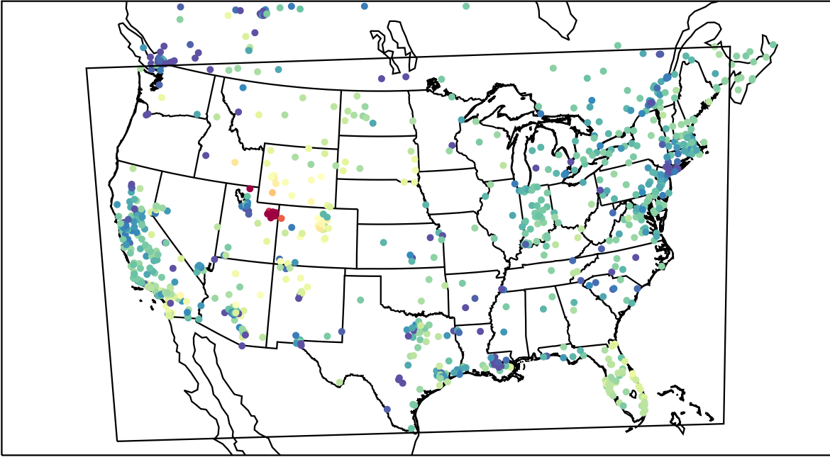
AirNOW (2023-02-05_01:00:00)
