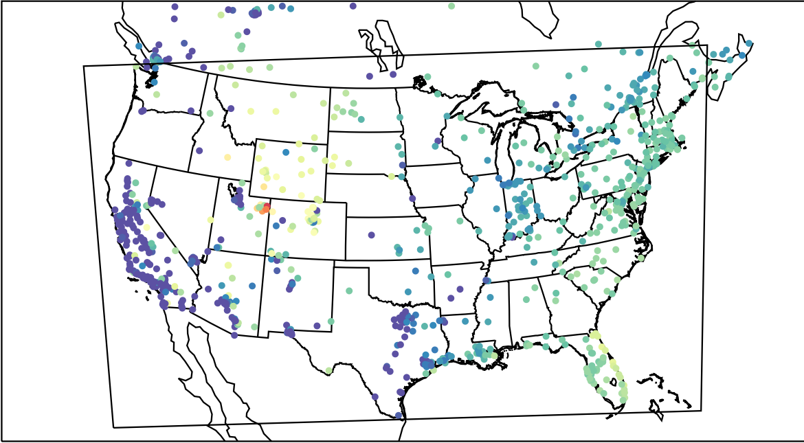
AirNOW (2023-02-04_15:00:00)
