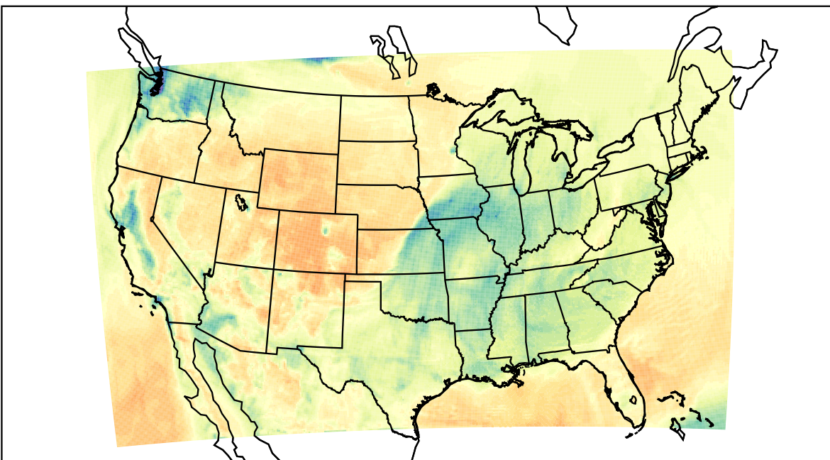
WRF (2023-02-04_19:00:00)
