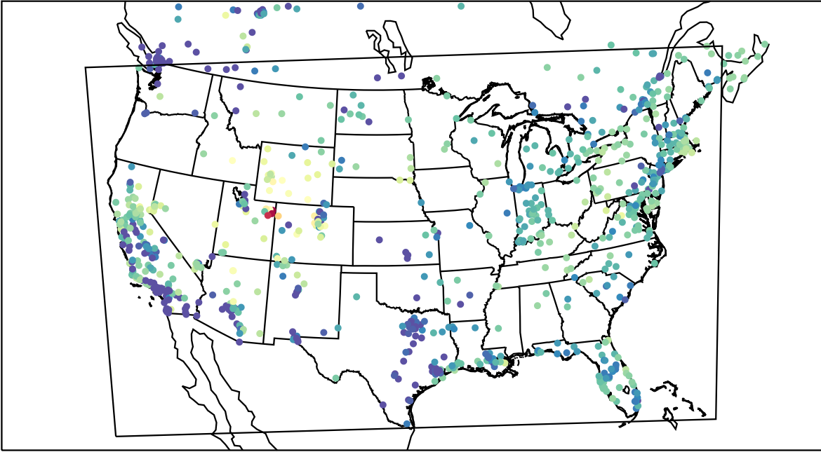
AirNOW (2023-02-05_15:00:00)
