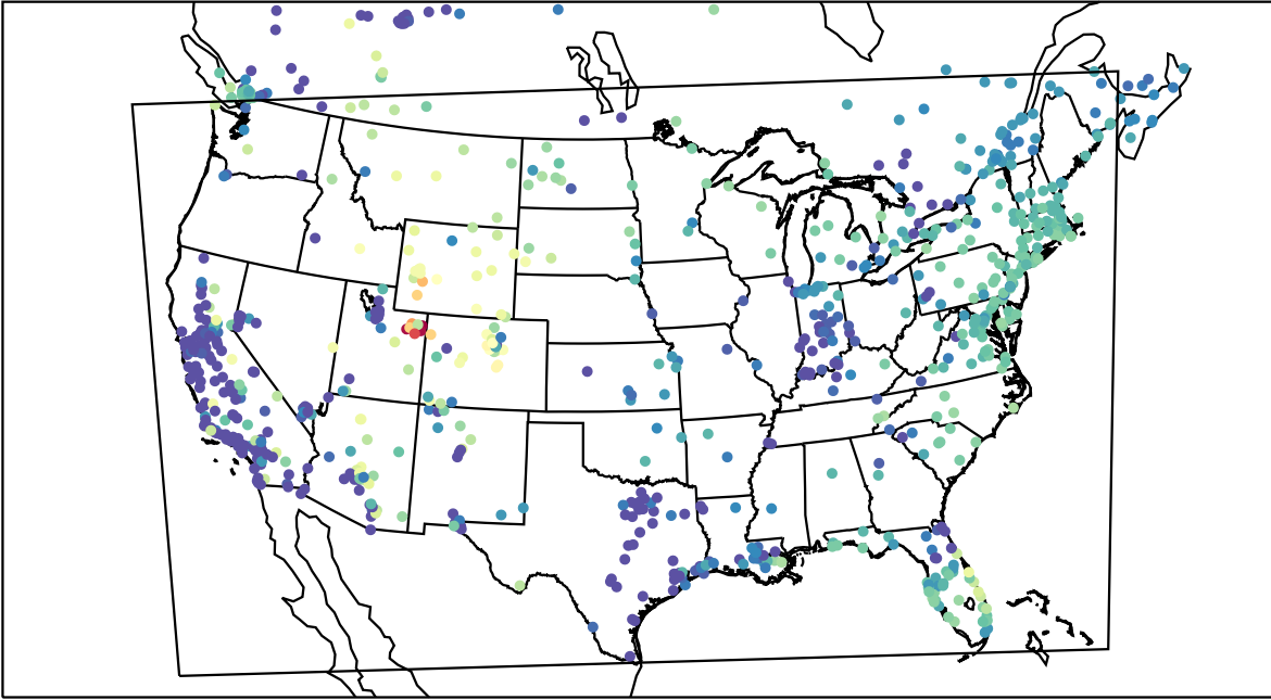
AirNOW (2023-02-04_08:00:00)
