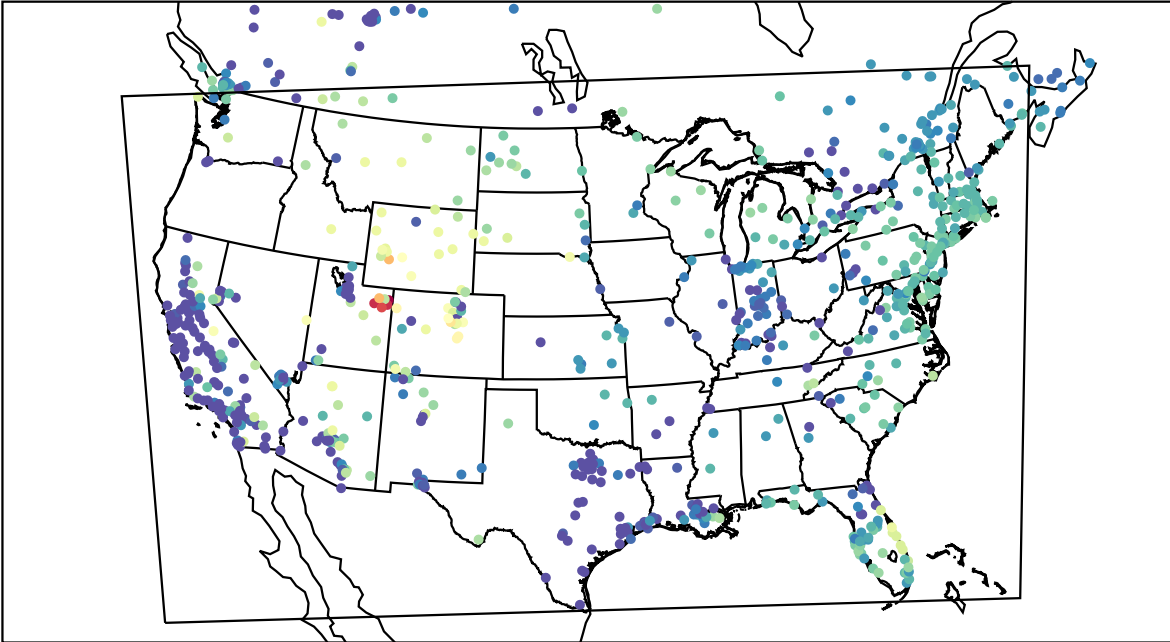
AirNOW (2023-02-04_09:00:00)
