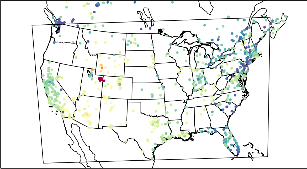
AirNOW (2023-02-05_23:00:00)
