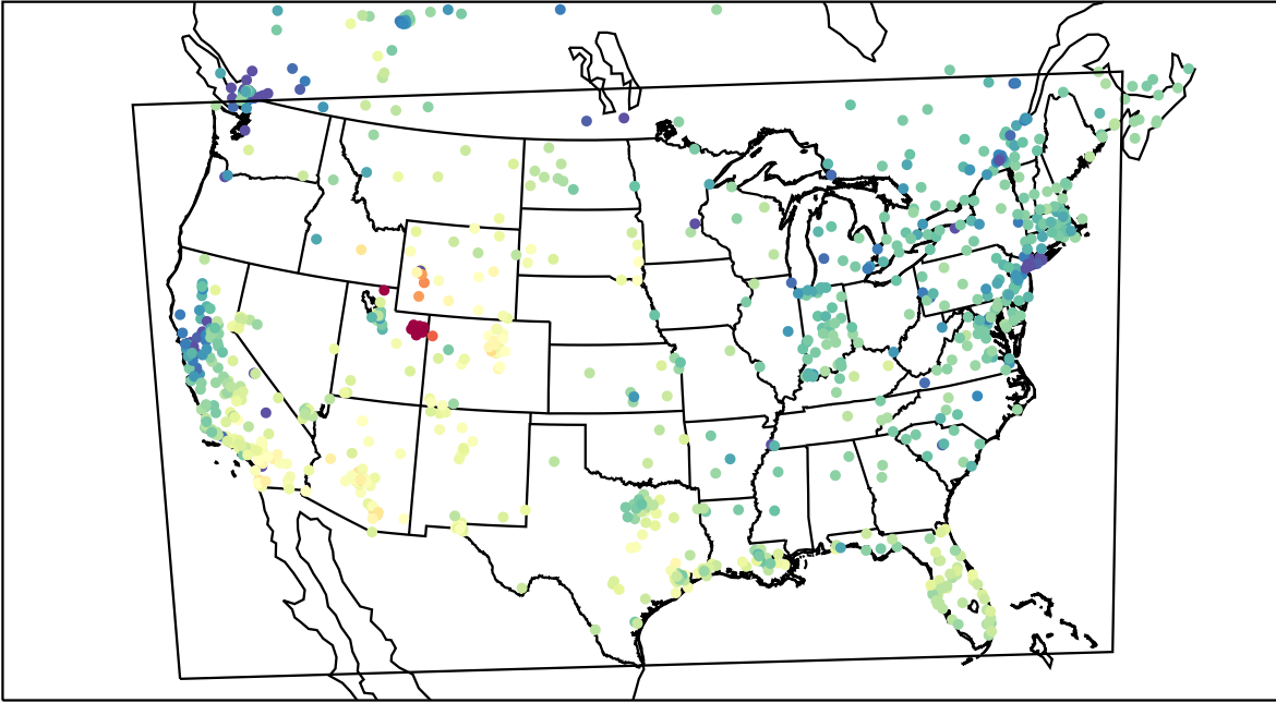
AirNOW (2023-02-04_23:00:00)
