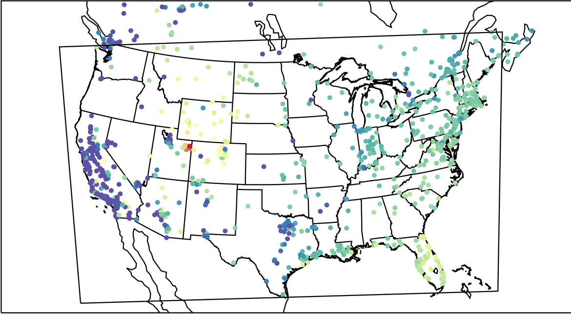
AirNOW (2023-02-04_16:00:00)
