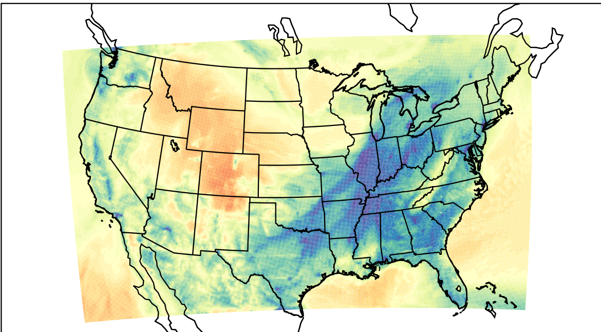
WRF (2023-02-05_12:00:00)
