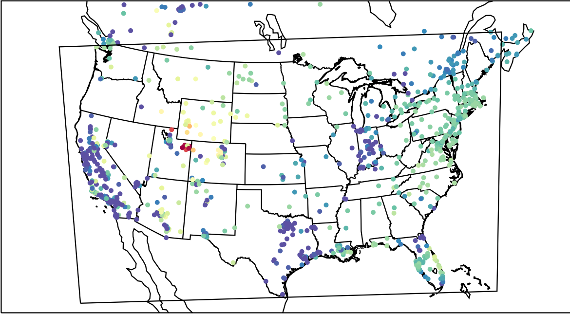
AirNOW (2023-02-04_03:00:00)
