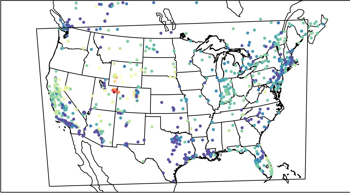
AirNOW (2023-02-05_09:00:00)
