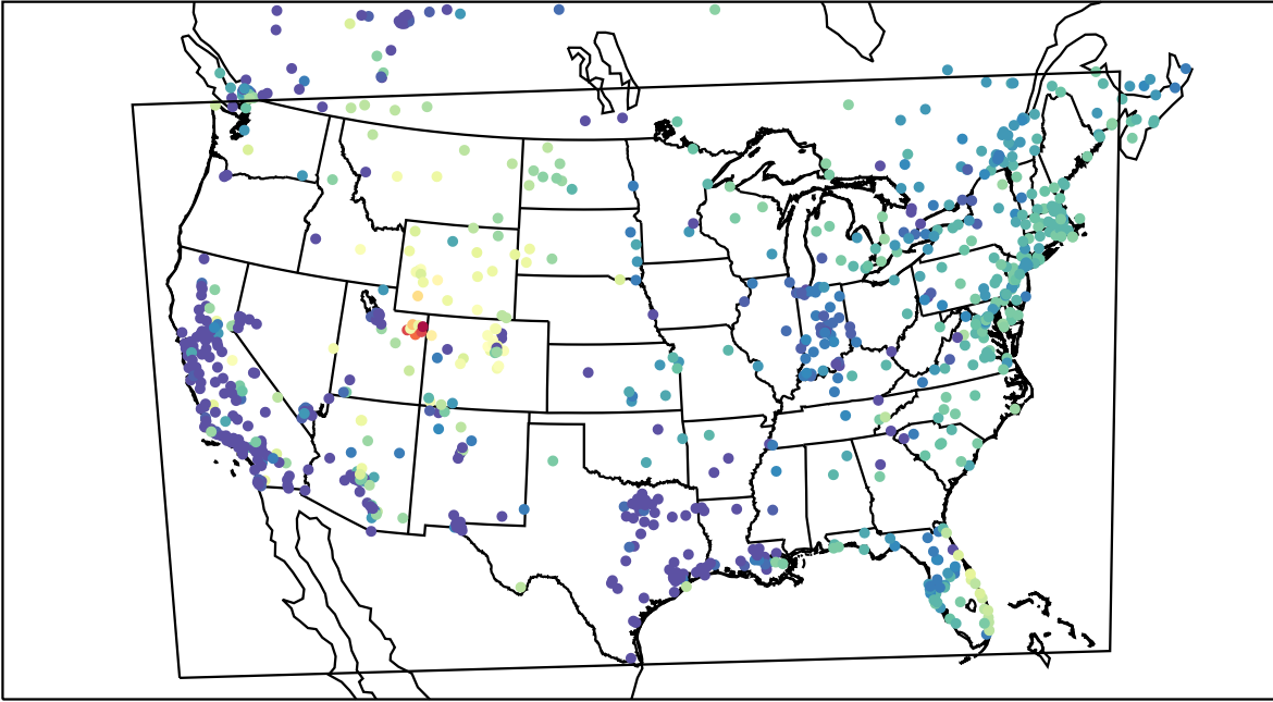
AirNOW (2023-02-04_13:00:00)
