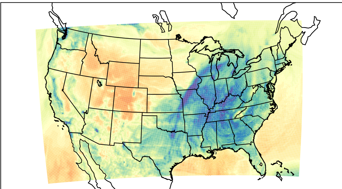
WRF (2023-02-05_04:00:00)
