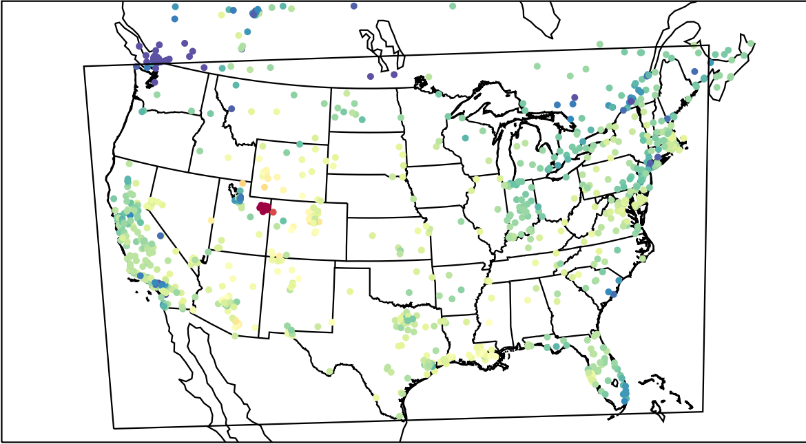
AirNOW (2023-02-05_19:00:00)
