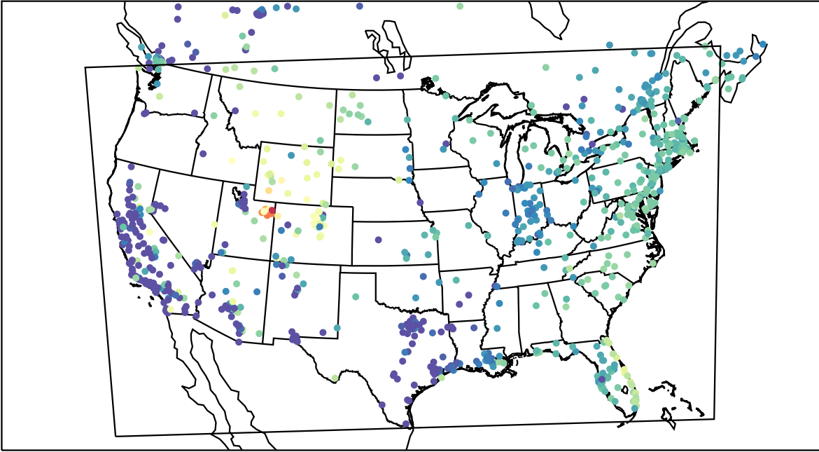
AirNOW (2023-02-04_14:00:00)
