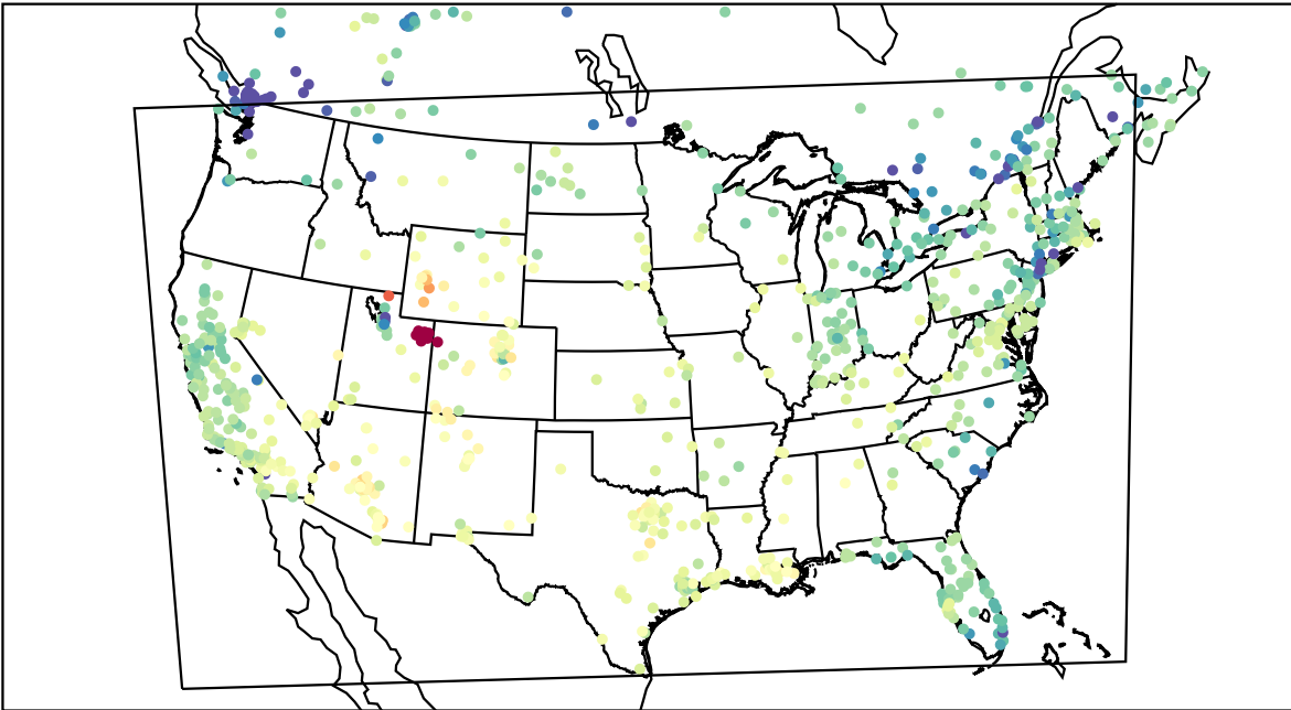
AirNOW (2023-02-05_21:00:00)
