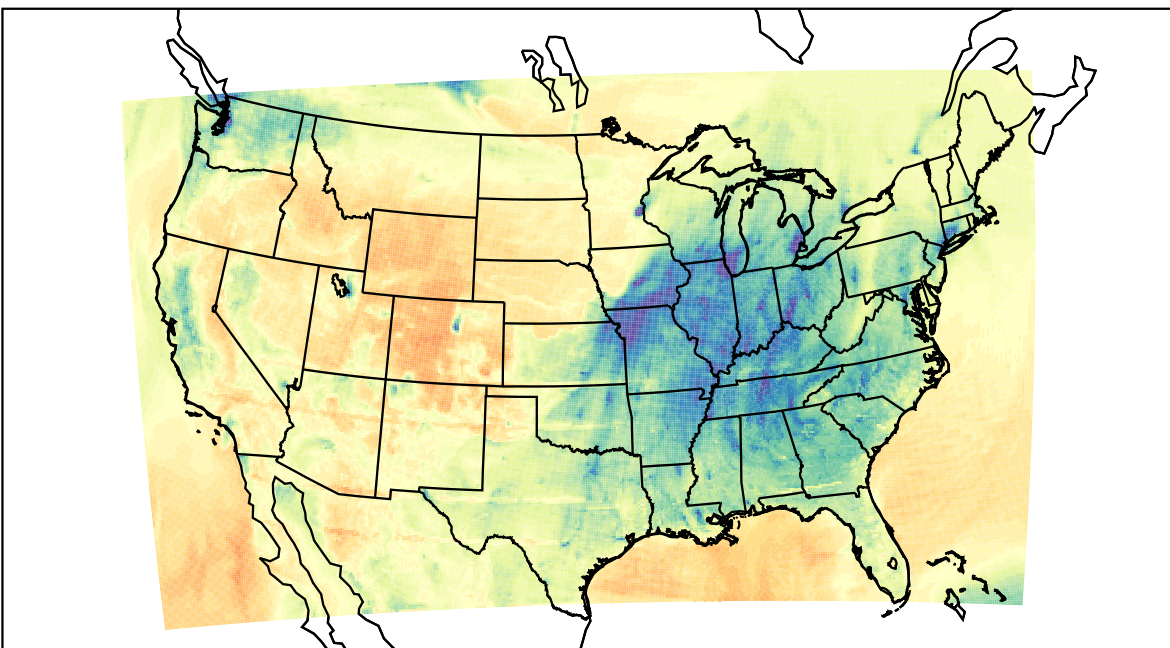
WRF (2023-02-05_00:00:00)
