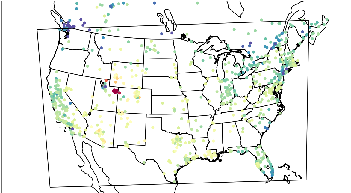
AirNOW (2023-02-05_20:00:00)
