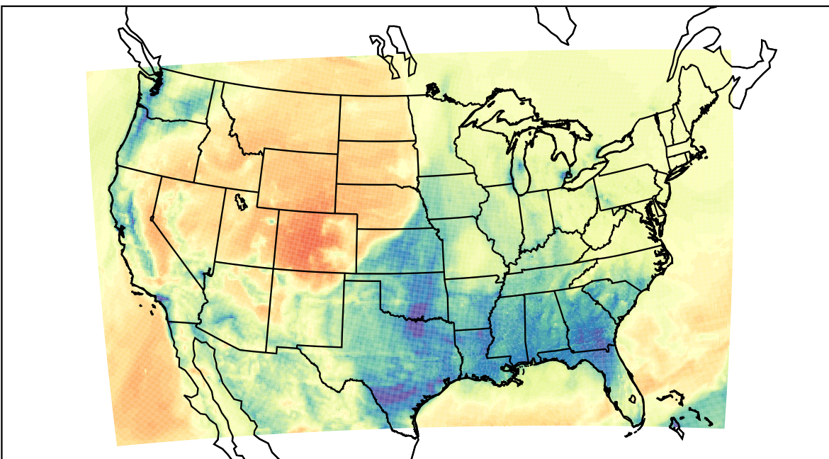
WRF (2023-02-04_08:00:00)
