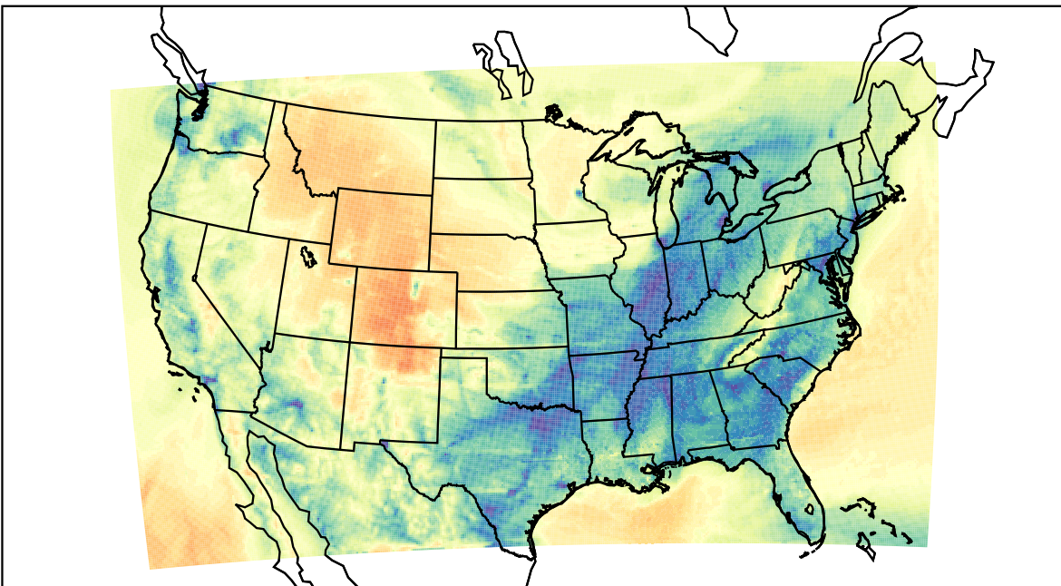
WRF (2023-02-05_14:00:00)
