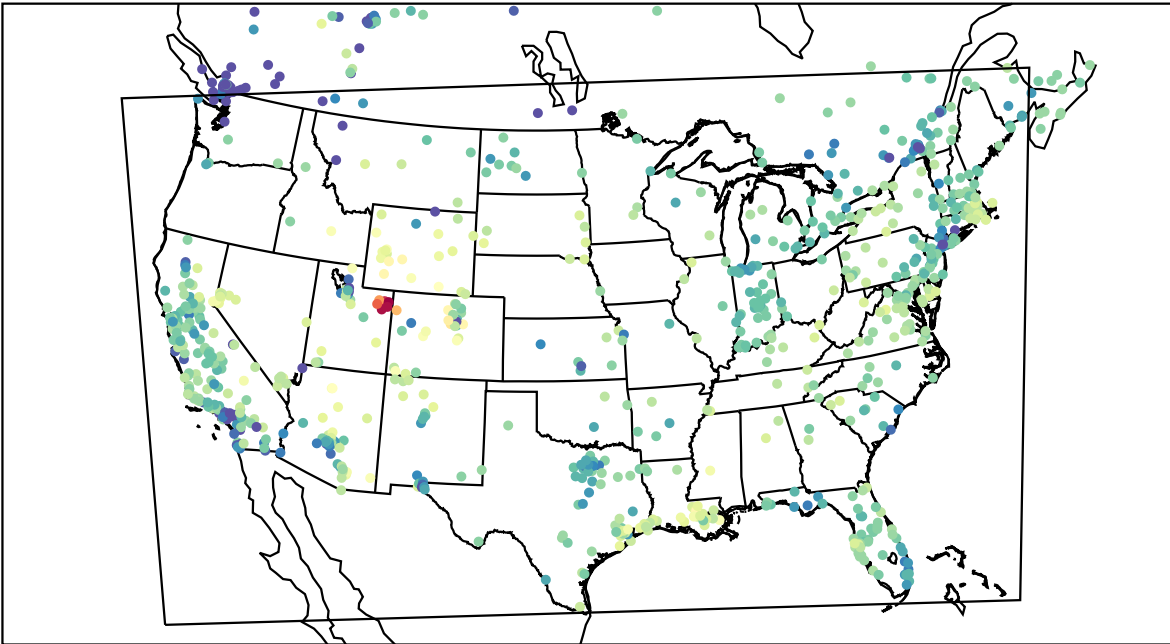
AirNOW (2023-02-05_17:00:00)
