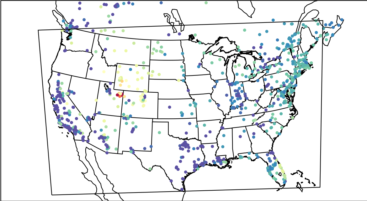
AirNOW (2023-02-04_11:00:00)
