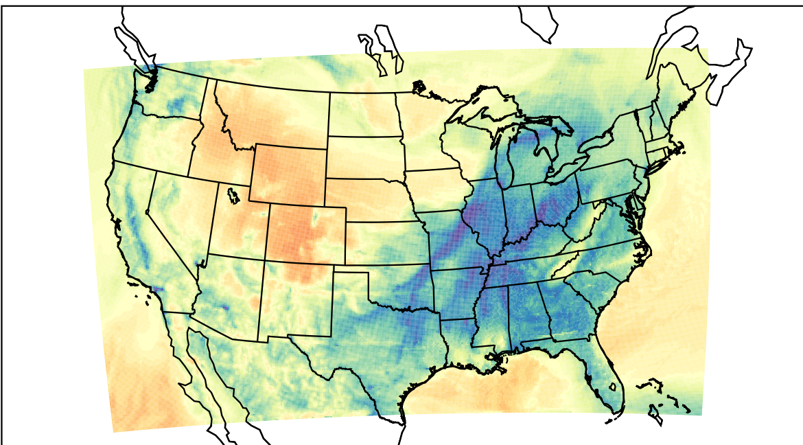
WRF (2023-02-05_09:00:00)
