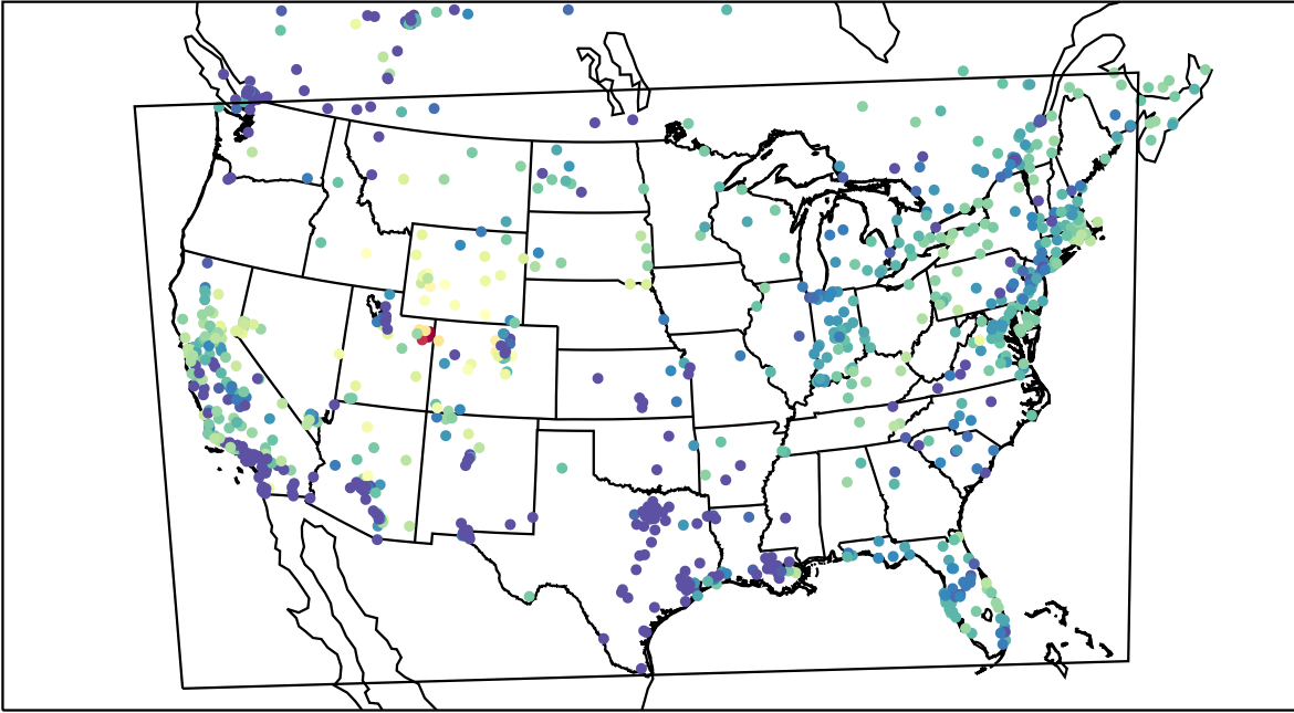
AirNOW (2023-02-05_14:00:00)
