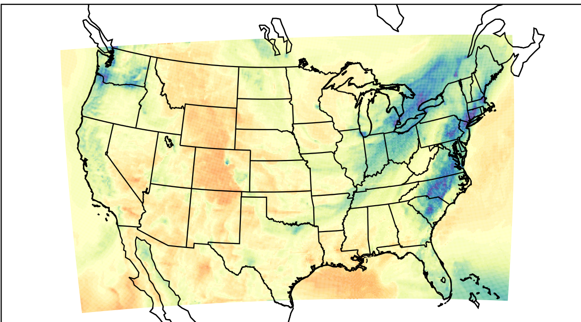
WRF (2023-02-05_21:00:00)
