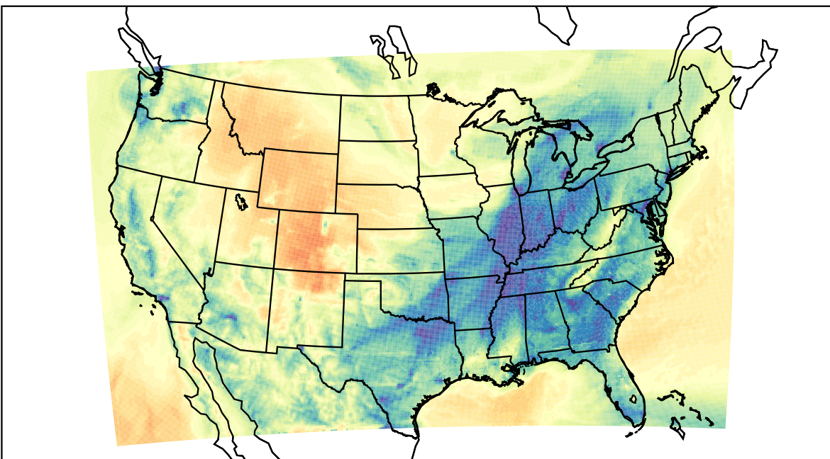
WRF (2023-02-05_13:00:00)
