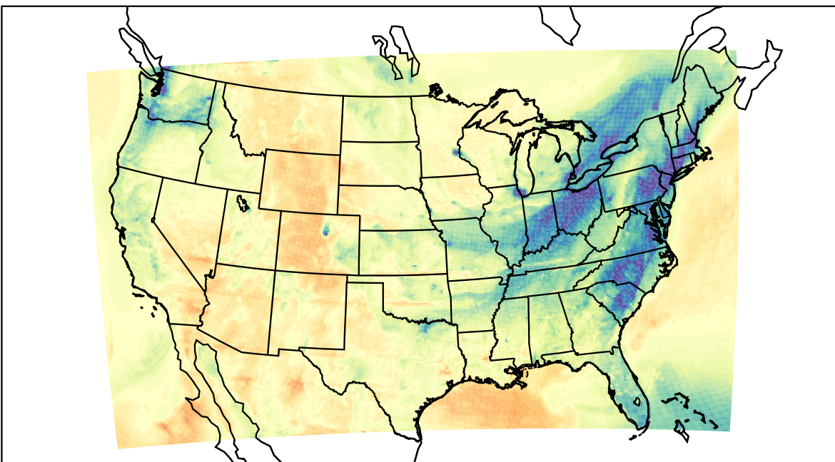
WRF (2023-02-05_23:00:00)
