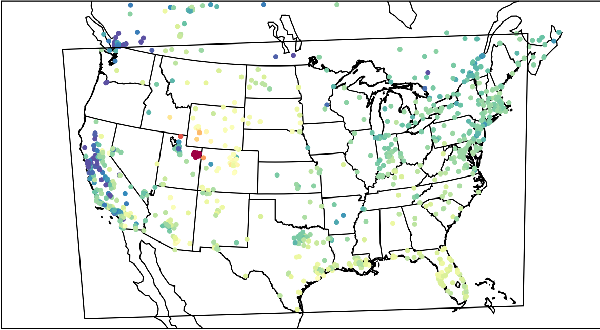
AirNOW (2023-02-04_19:00:00)
