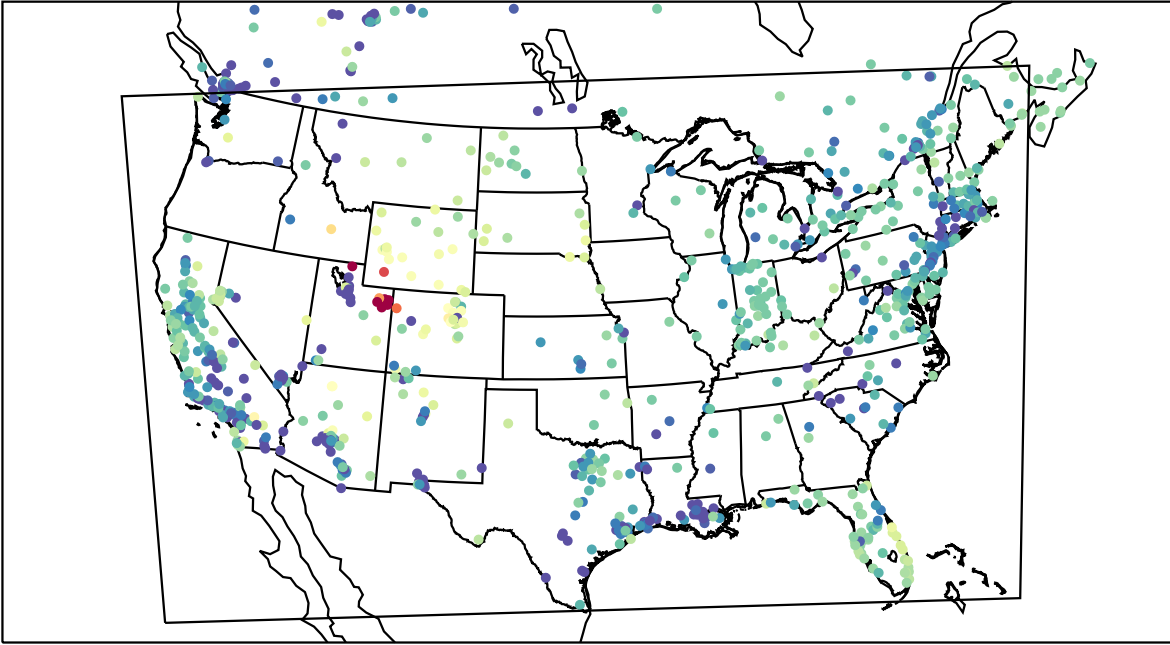
AirNOW (2023-02-05_03:00:00)
