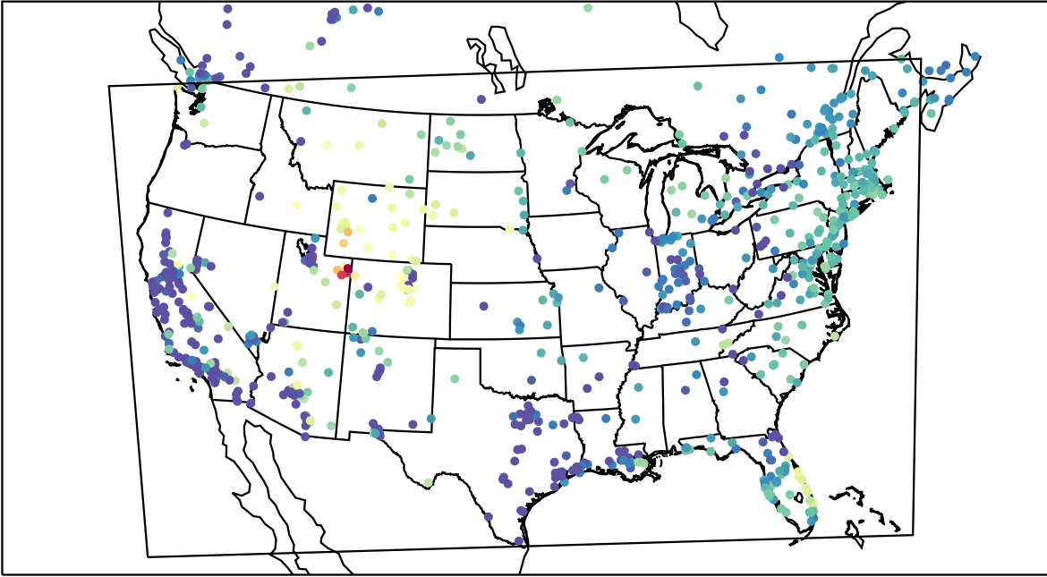
AirNOW (2023-02-04_10:00:00)
