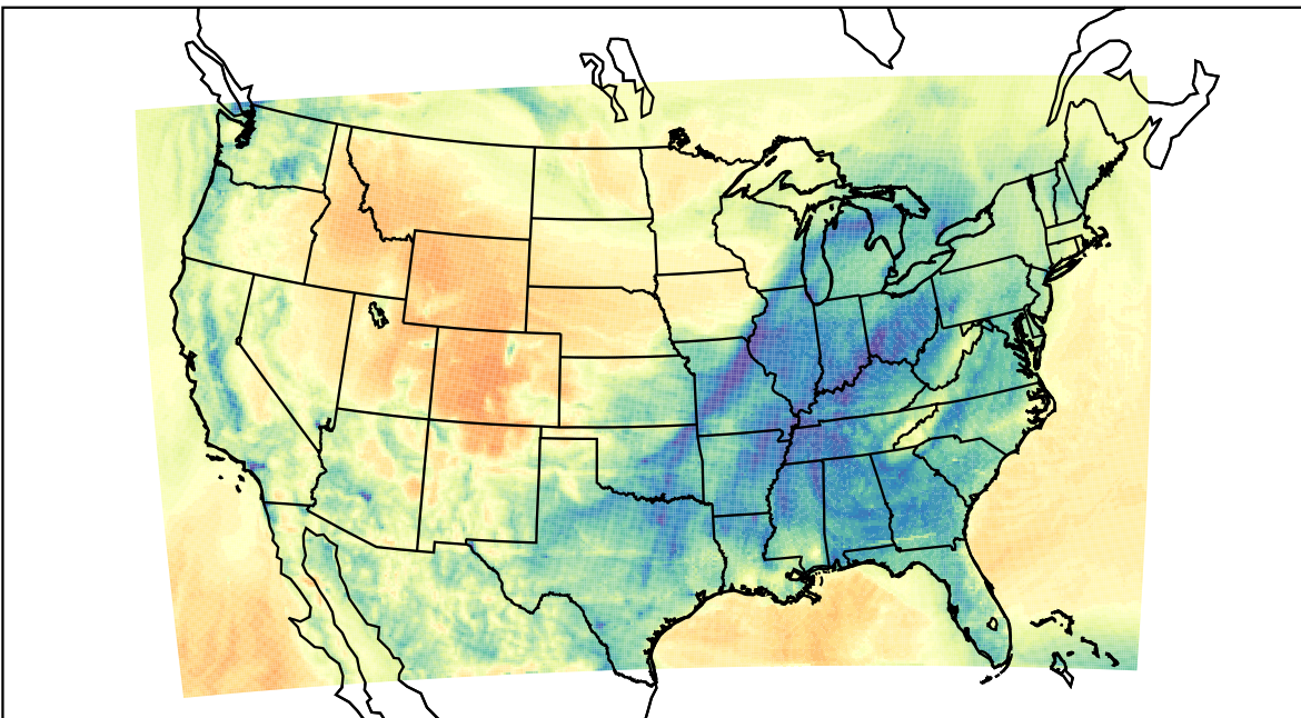
WRF (2023-02-05_08:00:00)
