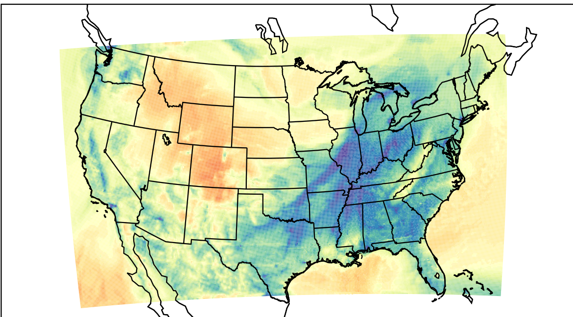
WRF (2023-02-05_11:00:00)
