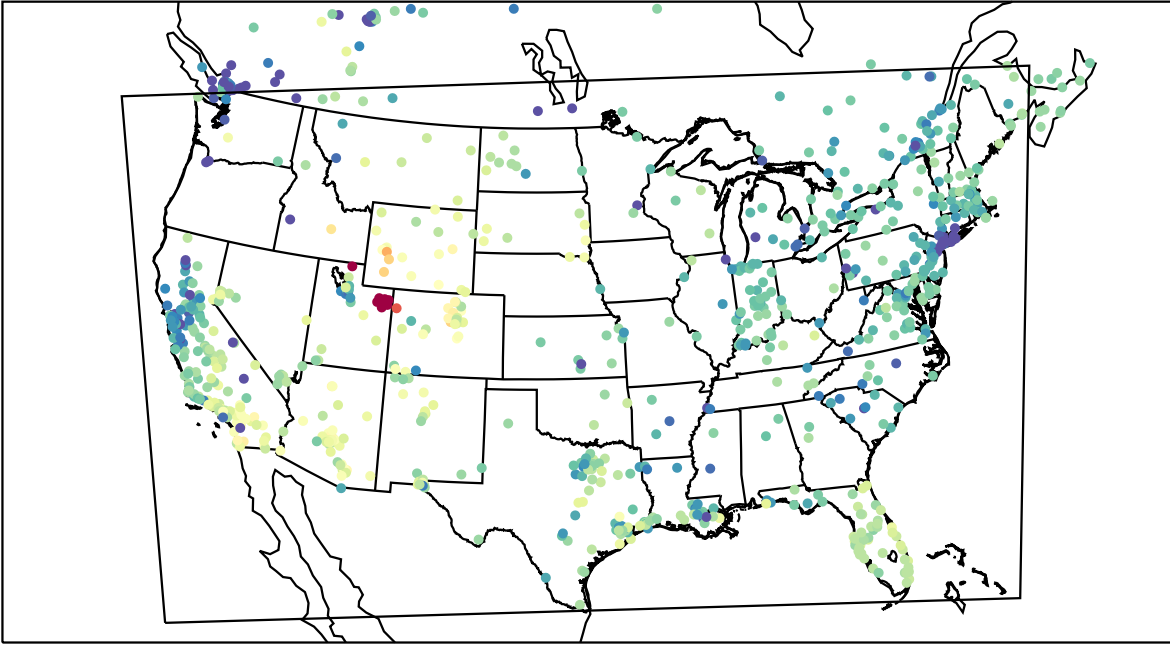
AirNOW (2023-02-05_00:00:00)
