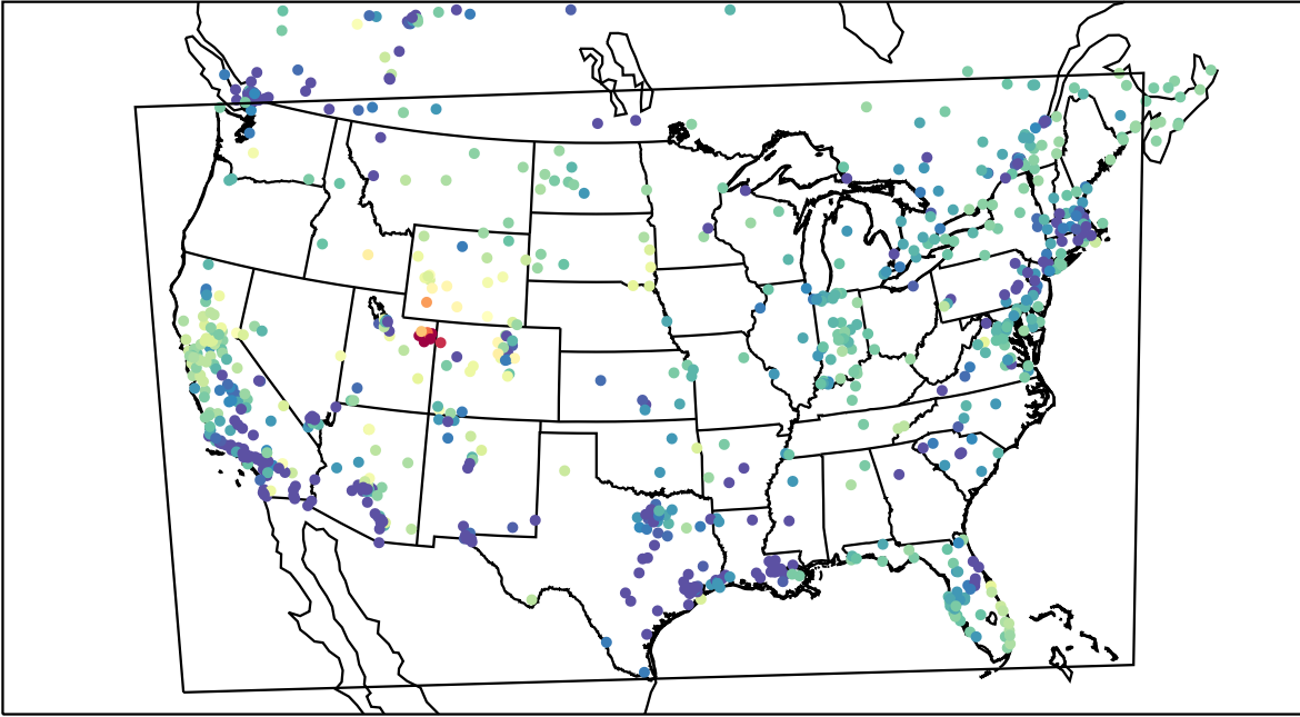
AirNOW (2023-02-05_07:00:00)
