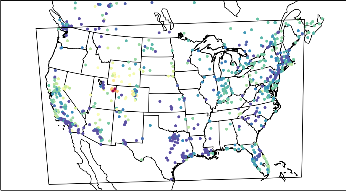
AirNOW (2023-02-05_11:00:00)
