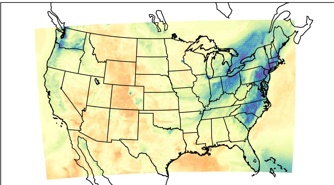
WRF (2023-02-05_22:00:00)
