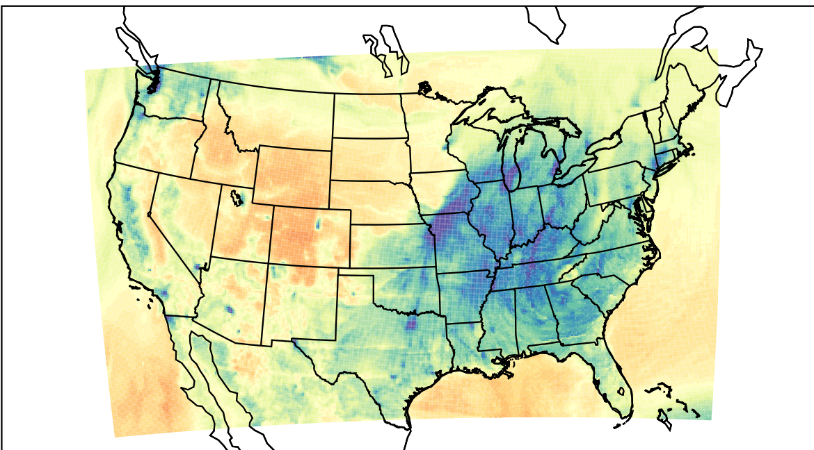
WRF (2023-02-05_02:00:00)
