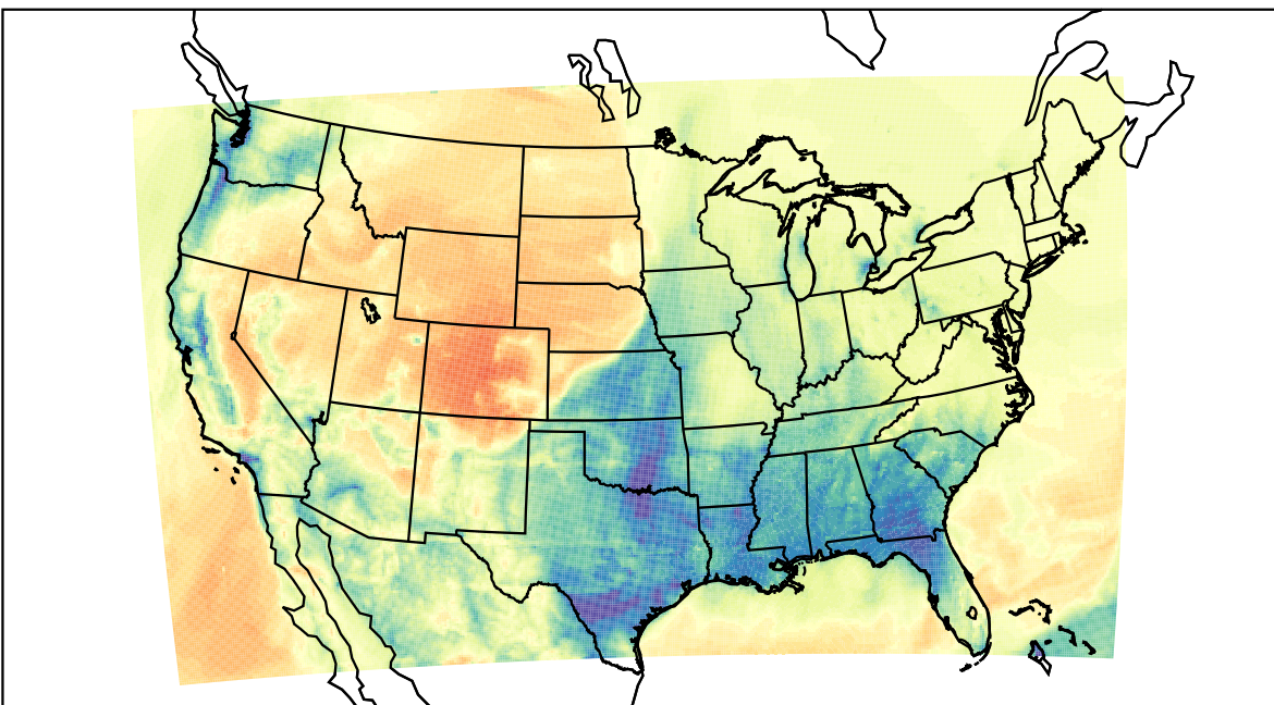
WRF (2023-02-04_09:00:00)
