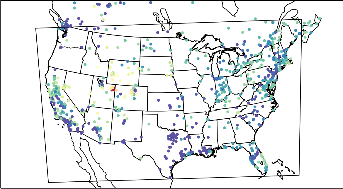
AirNOW (2023-02-05_13:00:00)
