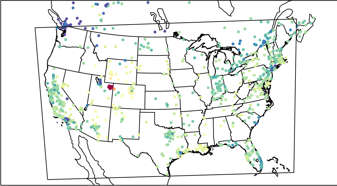
AirNOW (2023-02-05_18:00:00)
