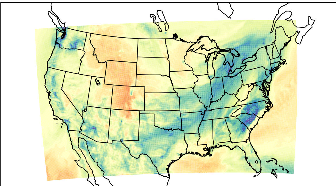
WRF (2023-02-05_17:00:00)
