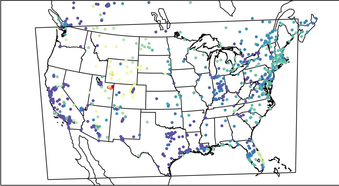
AirNOW (2023-02-04_12:00:00)
