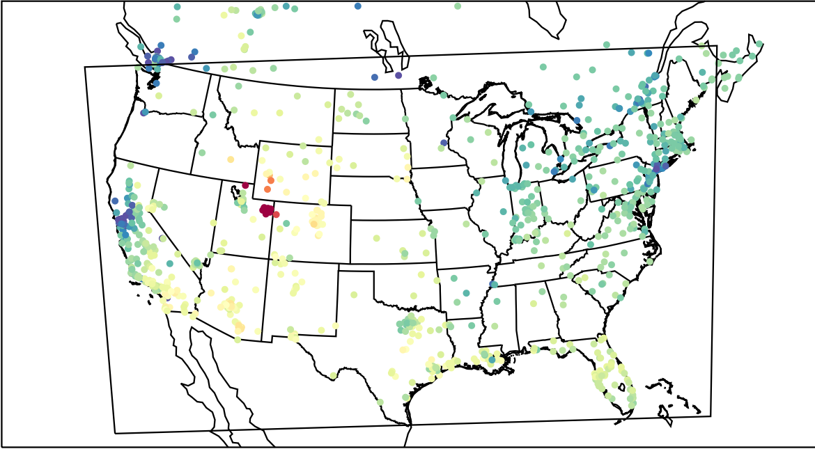
AirNOW (2023-02-04_22:00:00)
