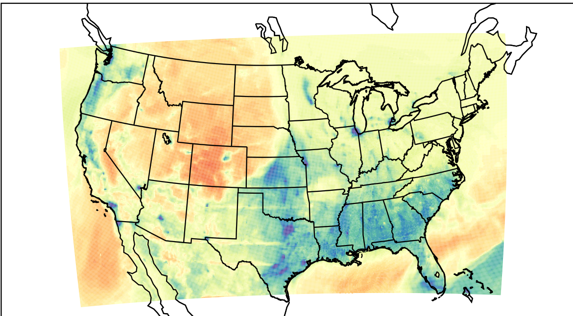
WRF (2023-02-04_02:00:00)
