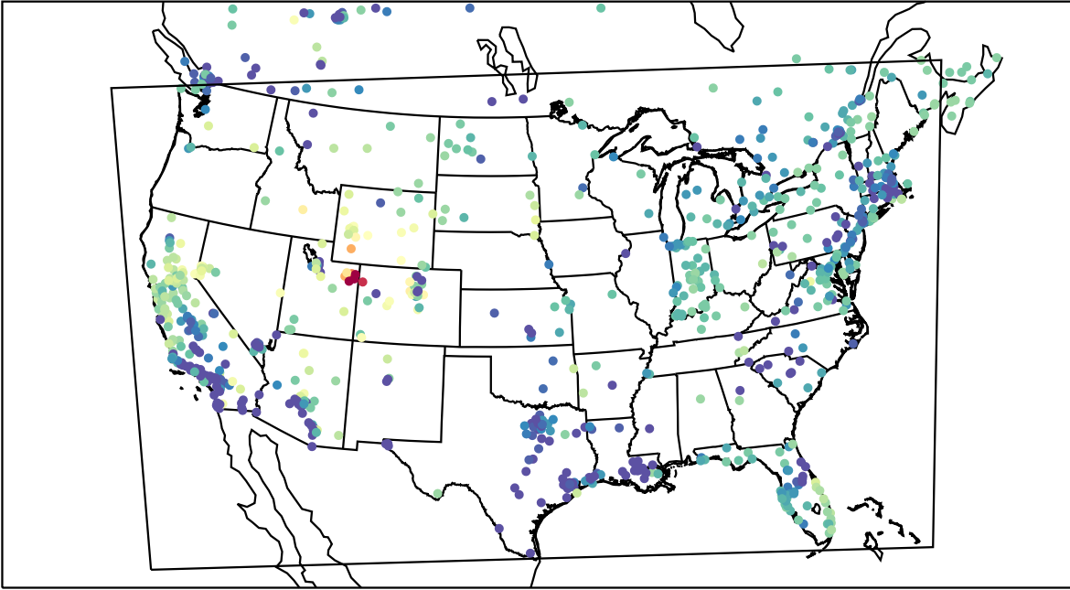
AirNOW (2023-02-05_08:00:00)
