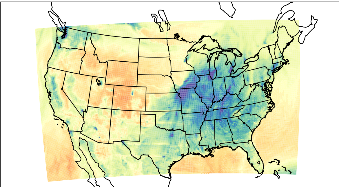
WRF (2023-02-05_01:00:00)
