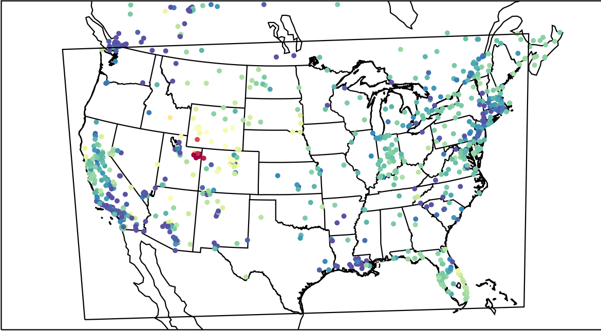
AirNOW (2023-02-05_04:00:00)
