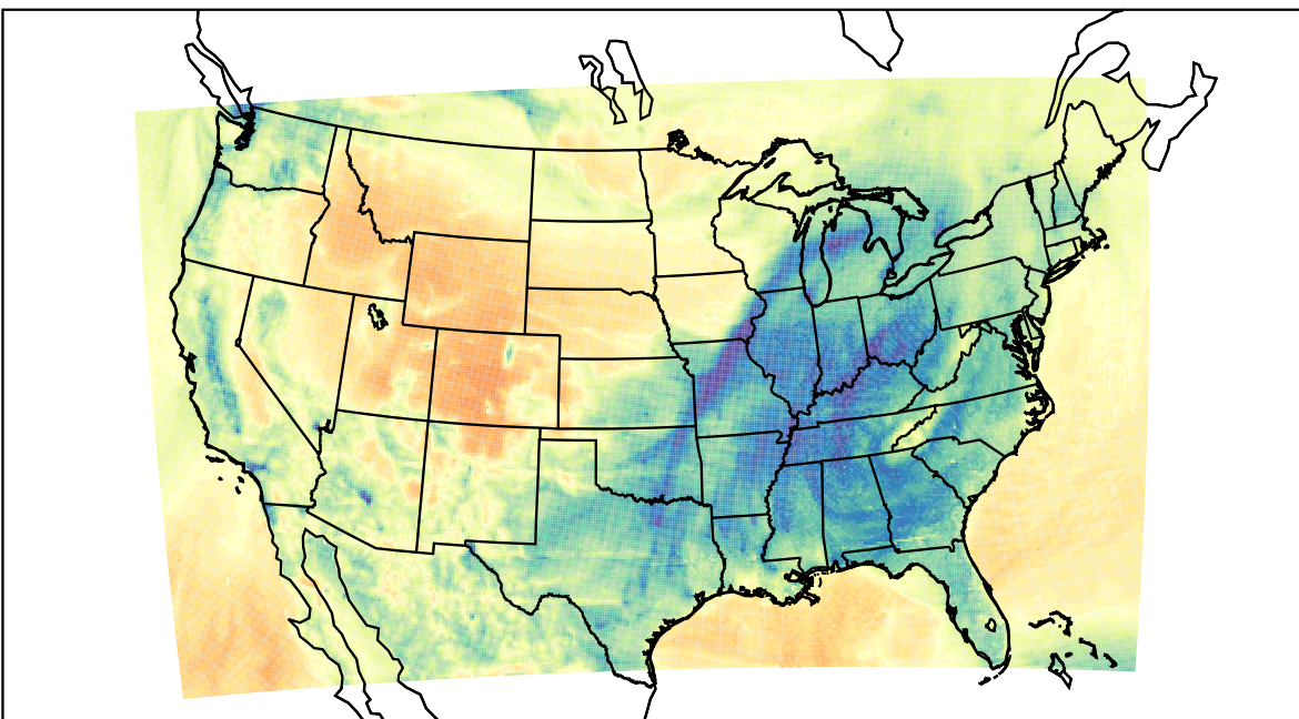
WRF (2023-02-05_06:00:00)
