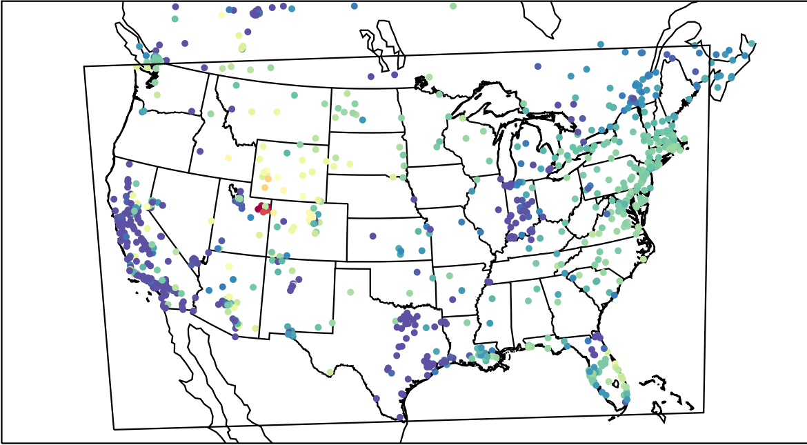
AirNOW (2023-02-04_04:00:00)
