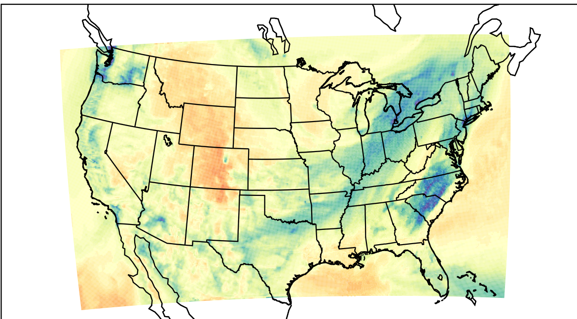
WRF (2023-02-05_18:00:00)
