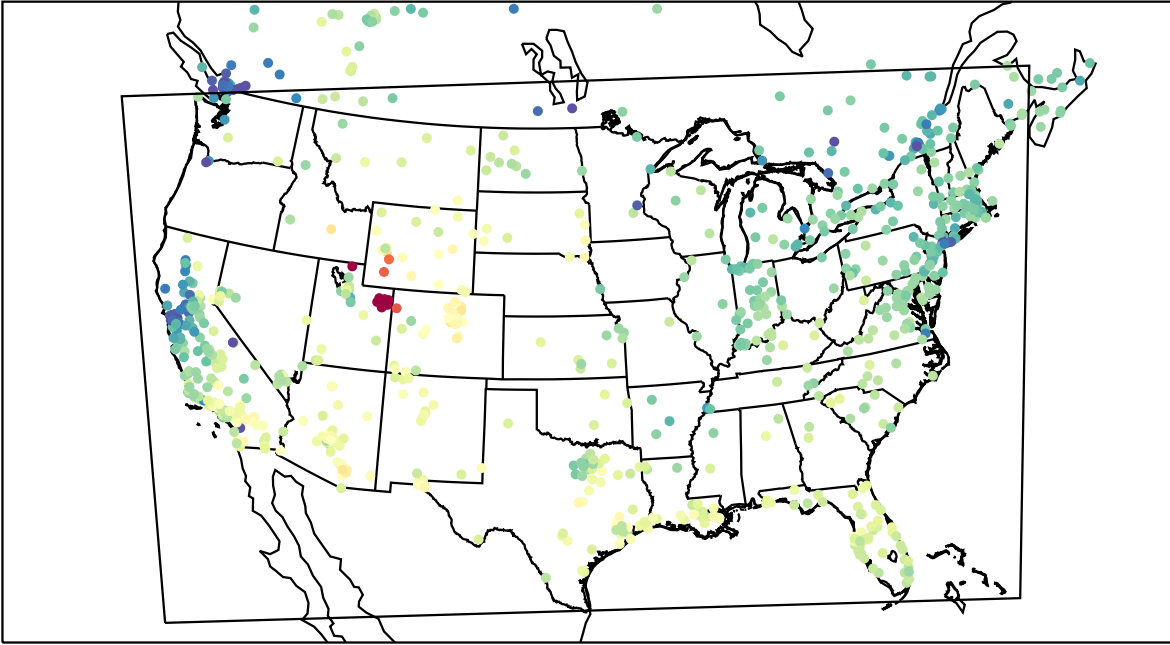
AirNOW (2023-02-04_21:00:00)
