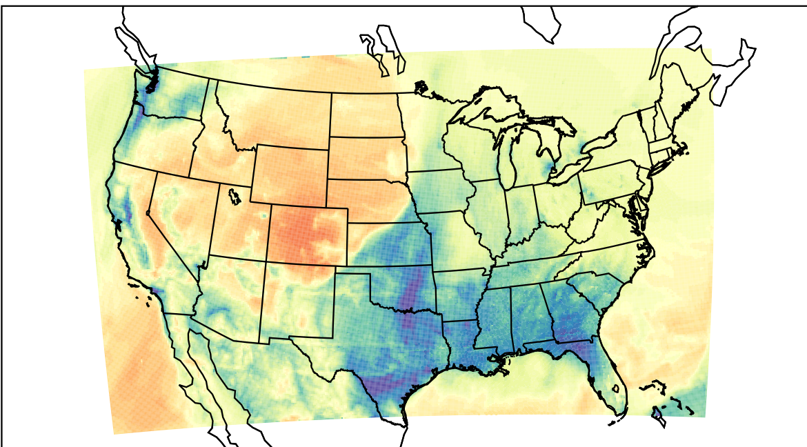
WRF (2023-02-04_10:00:00)
