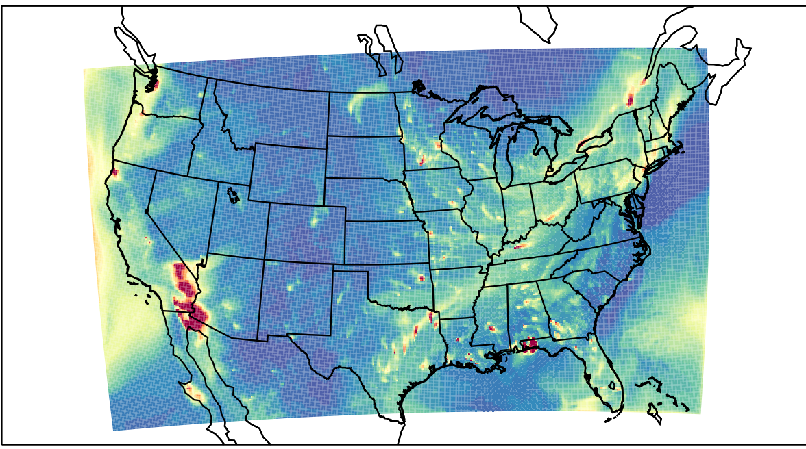
WRF 2023-02-06_02:00:00
