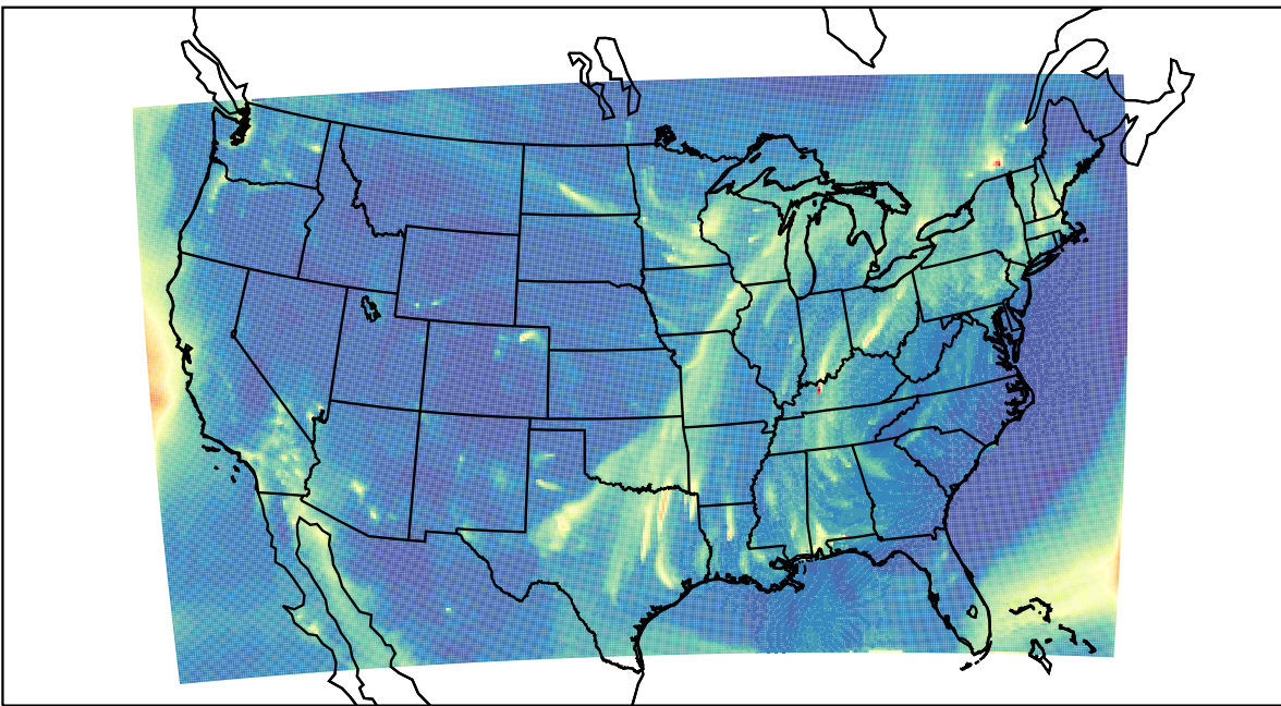
WRF 2023-02-05_07:00:00
