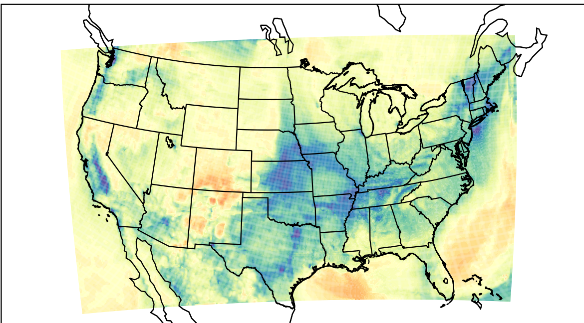
WRF (2023-02-06_16:00:00)
