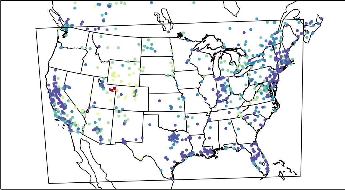
AirNOW (2023-02-06_13:00:00)
