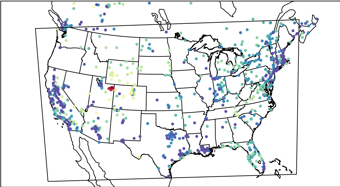
AirNOW (2023-02-06_14:00:00)
