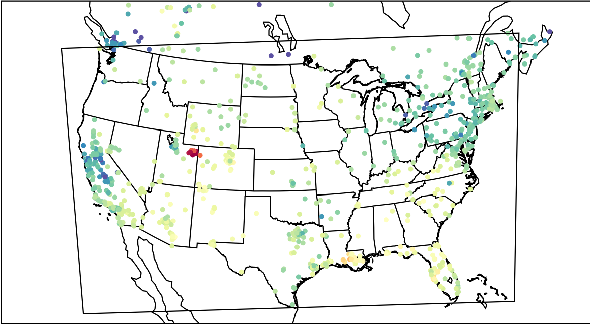
AirNOW (2023-02-06_20:00:00)
