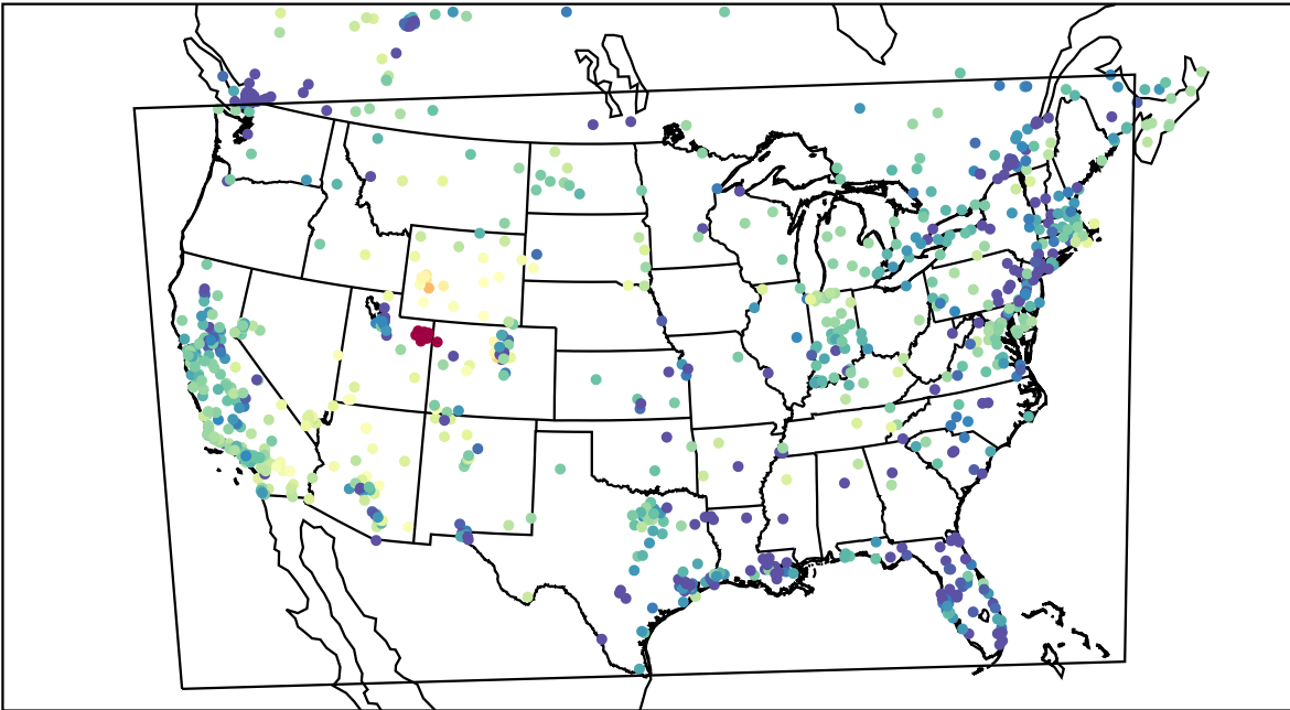
AirNOW (2023-02-06_02:00:00)
