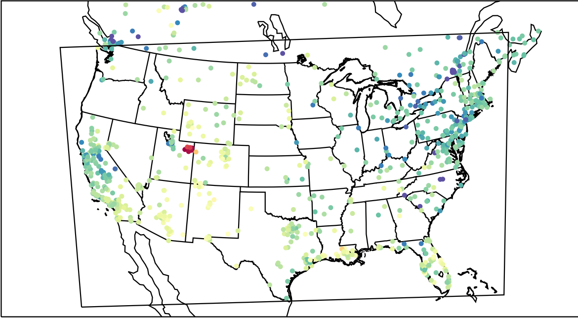
AirNOW (2023-02-06_23:00:00)
