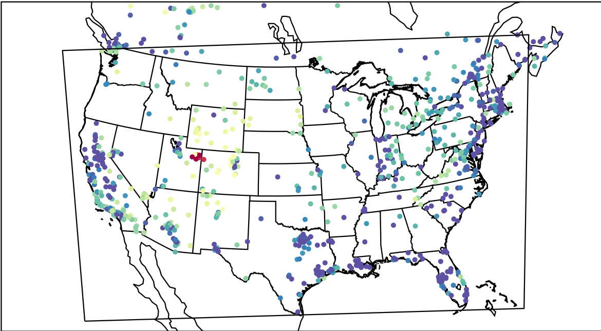
AirNOW (2023-02-06_11:00:00)
