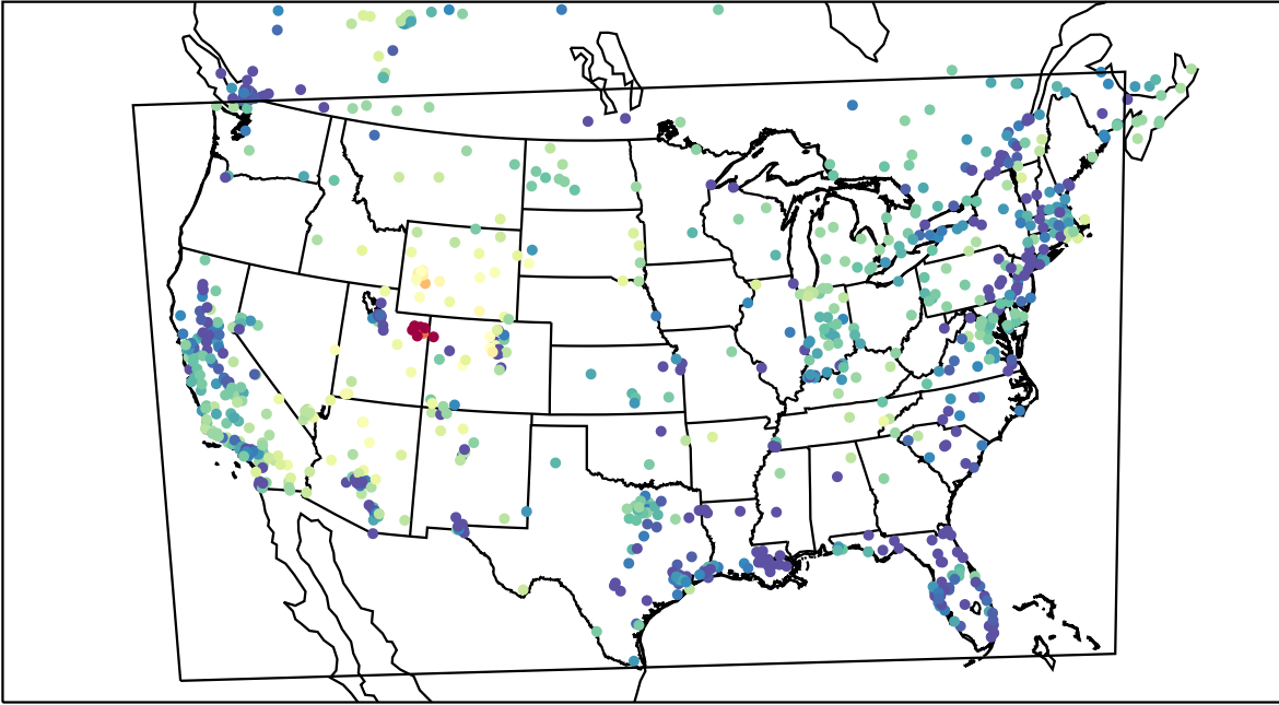
AirNOW (2023-02-06_04:00:00)
