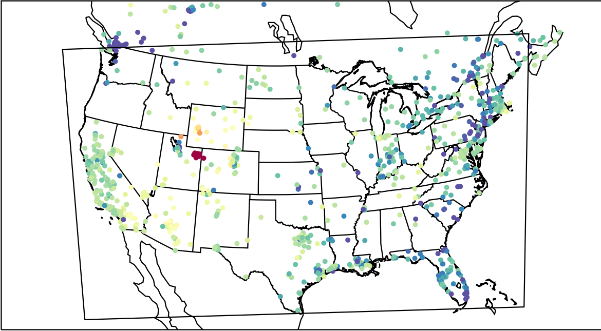
AirNOW (2023-02-06_00:00:00)
