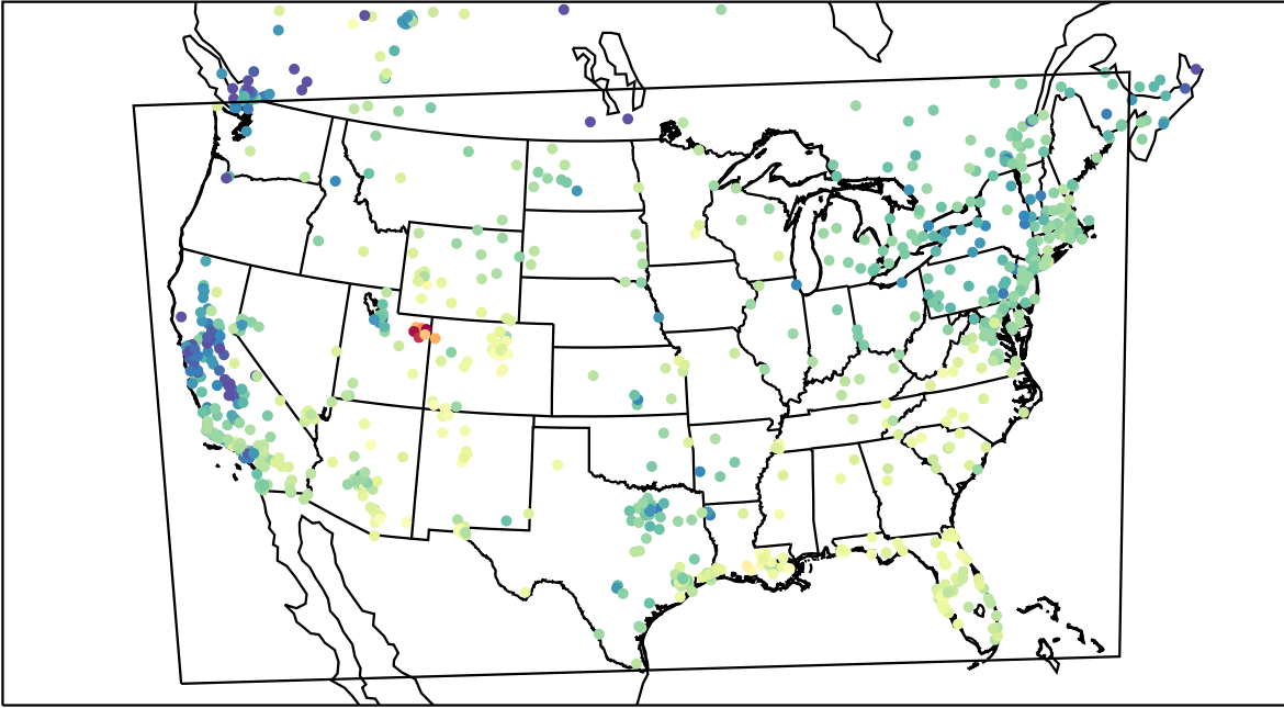
AirNOW (2023-02-06_18:00:00)
