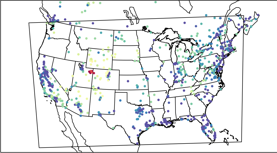
AirNOW (2023-02-06_10:00:00)
