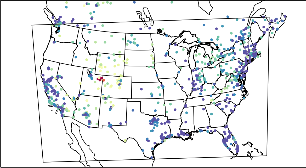
AirNOW (2023-02-06_12:00:00)
