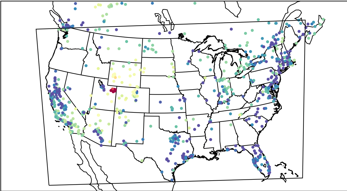
AirNOW (2023-02-06_07:00:00)
