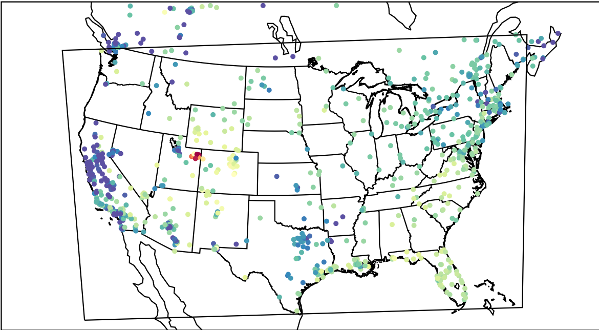
AirNOW (2023-02-06_16:00:00)
