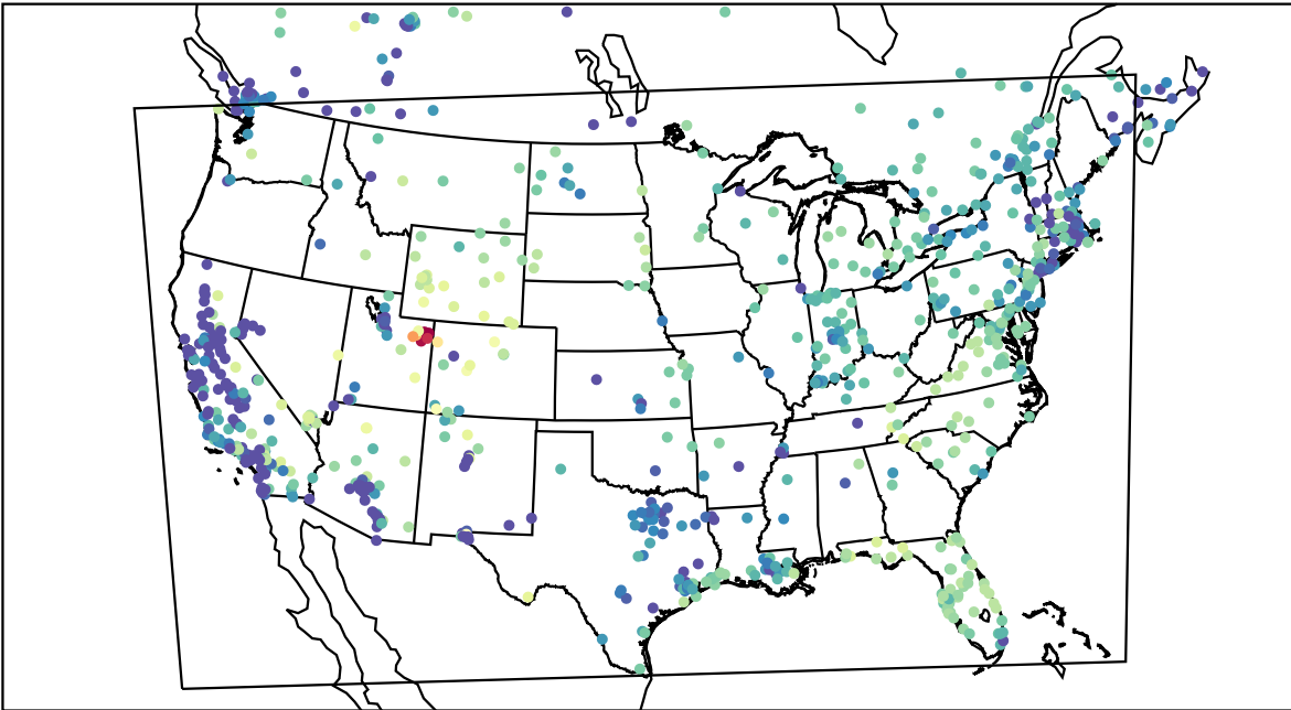
AirNOW (2023-02-06_15:00:00)
