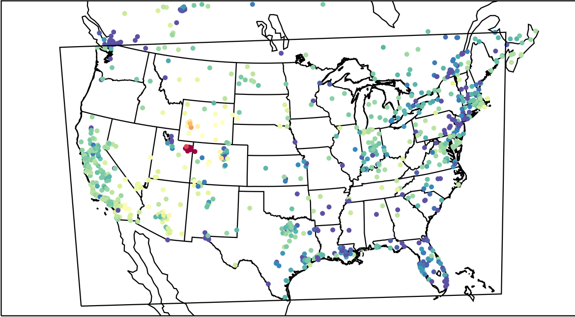
AirNOW (2023-02-06_01:00:00)
