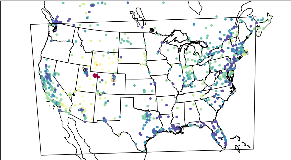
AirNOW (2023-02-06_03:00:00)
