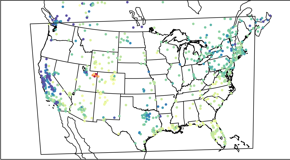
AirNOW (2023-02-06_17:00:00)
