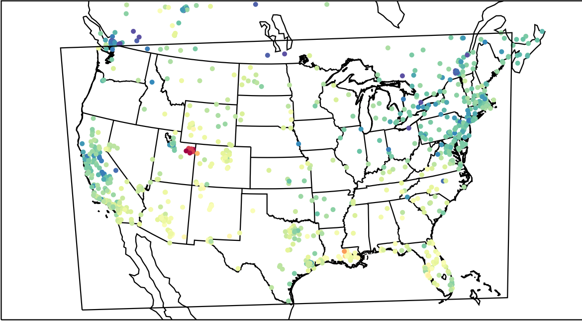
AirNOW (2023-02-06_22:00:00)
