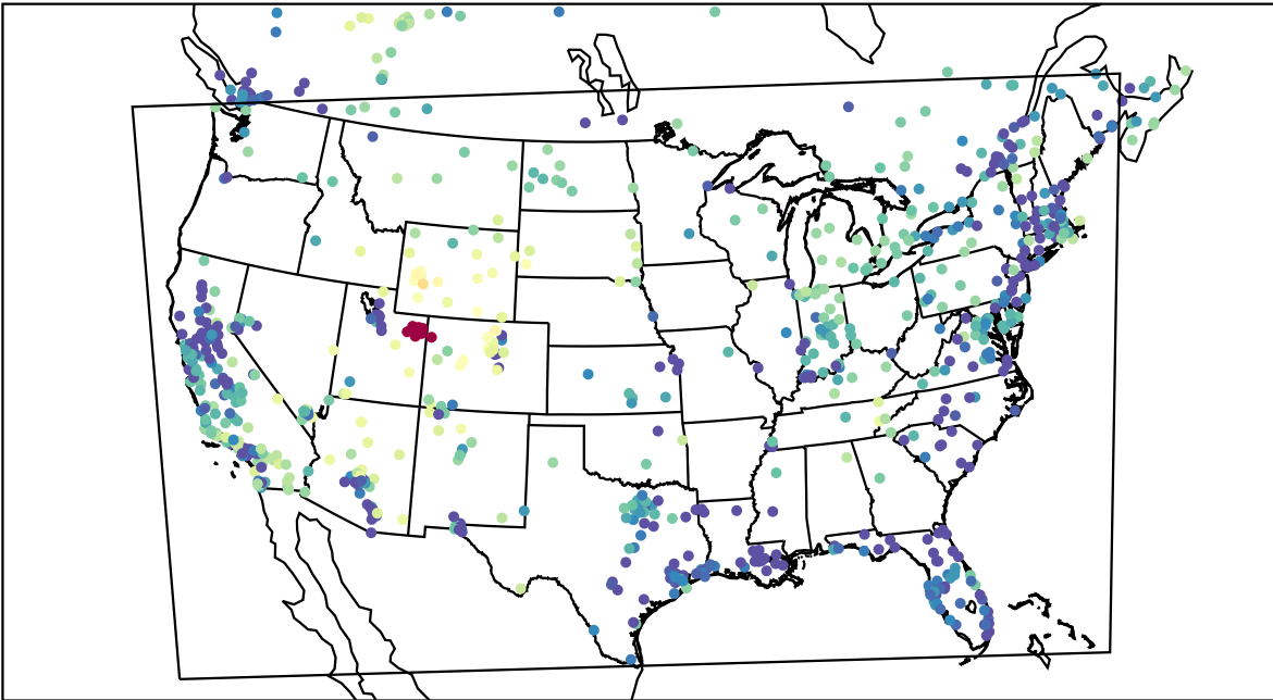
AirNOW (2023-02-06_06:00:00)
