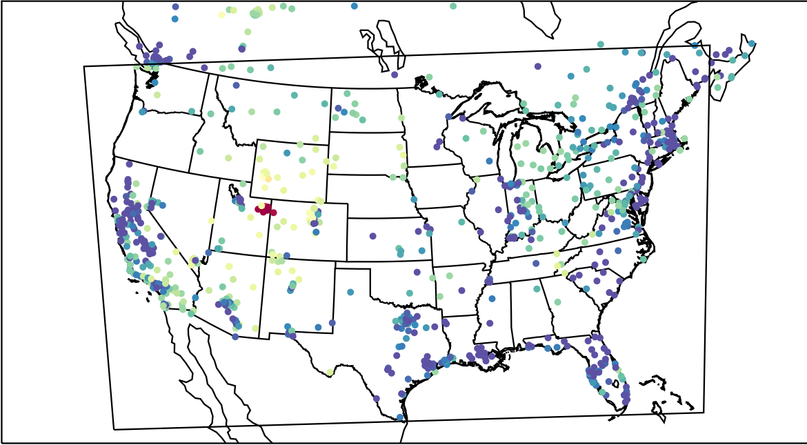
AirNOW (2023-02-06_09:00:00)
