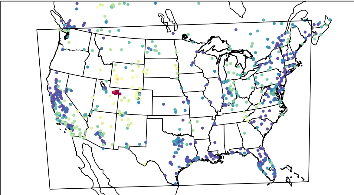
AirNOW (2023-02-06_08:00:00)
