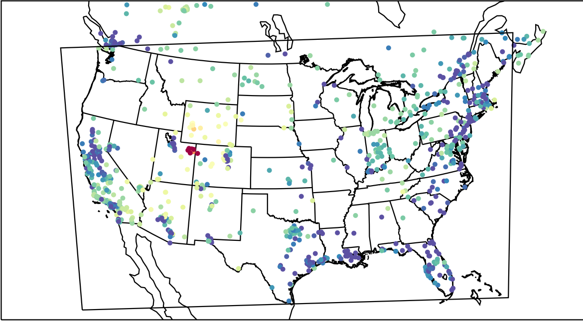
AirNOW (2023-02-06_05:00:00)
