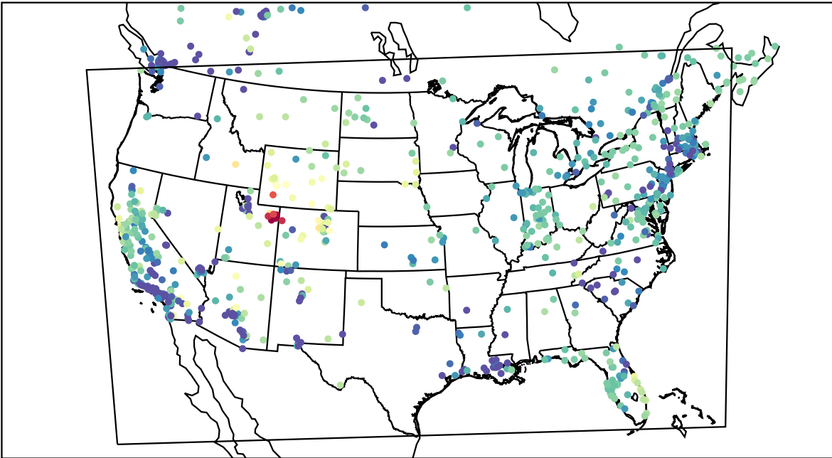
AirNOW (2023-02-05_05:00:00)
