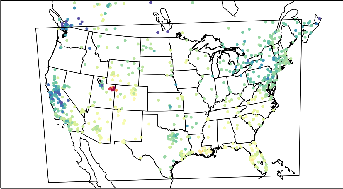
AirNOW (2023-02-06_19:00:00)
