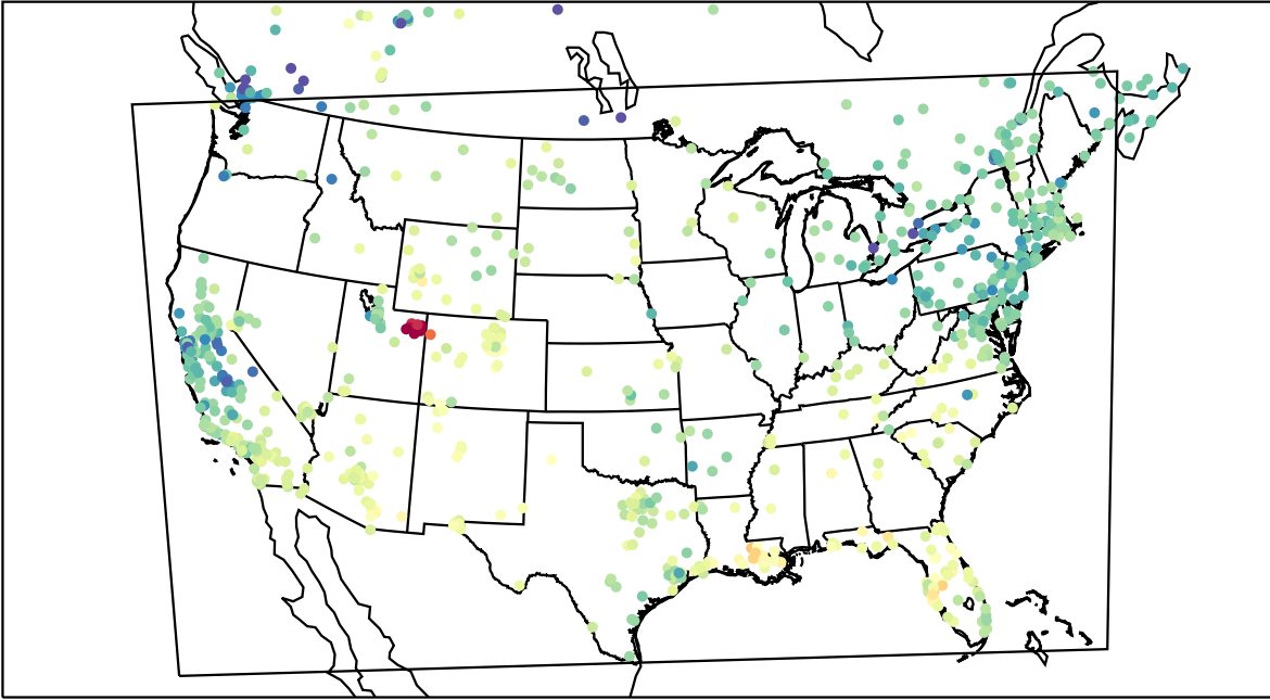
AirNOW (2023-02-06_21:00:00)
