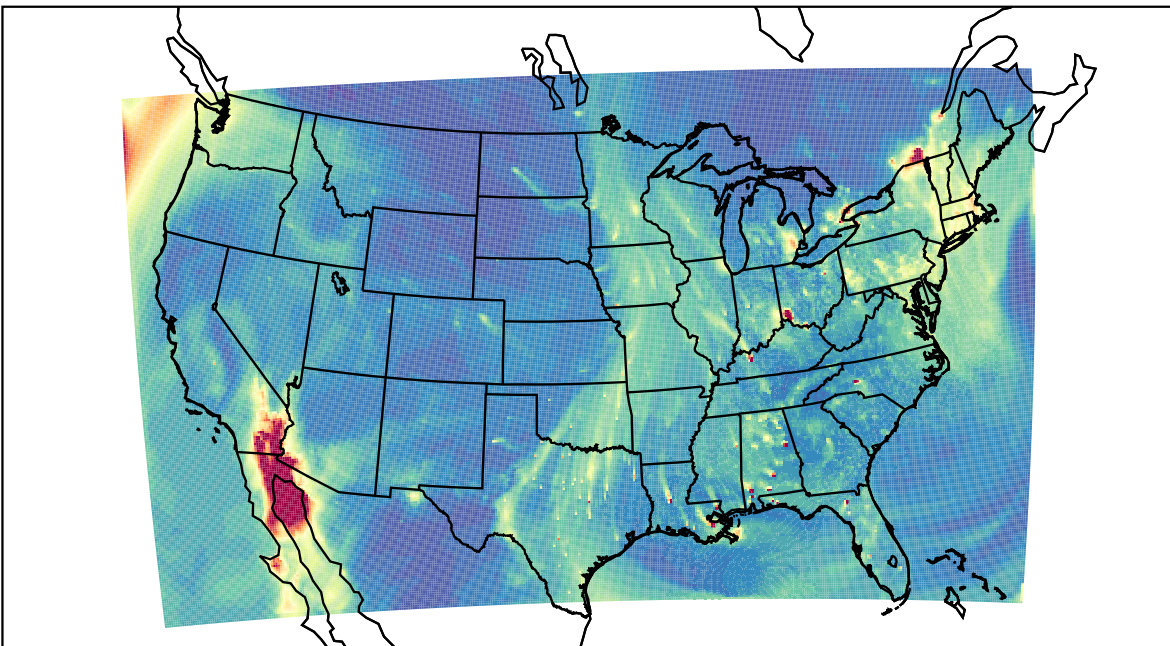
WRF 2023-02-06_23:00:00
