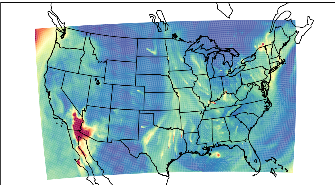
WRF 2023-02-06_17:00:00
