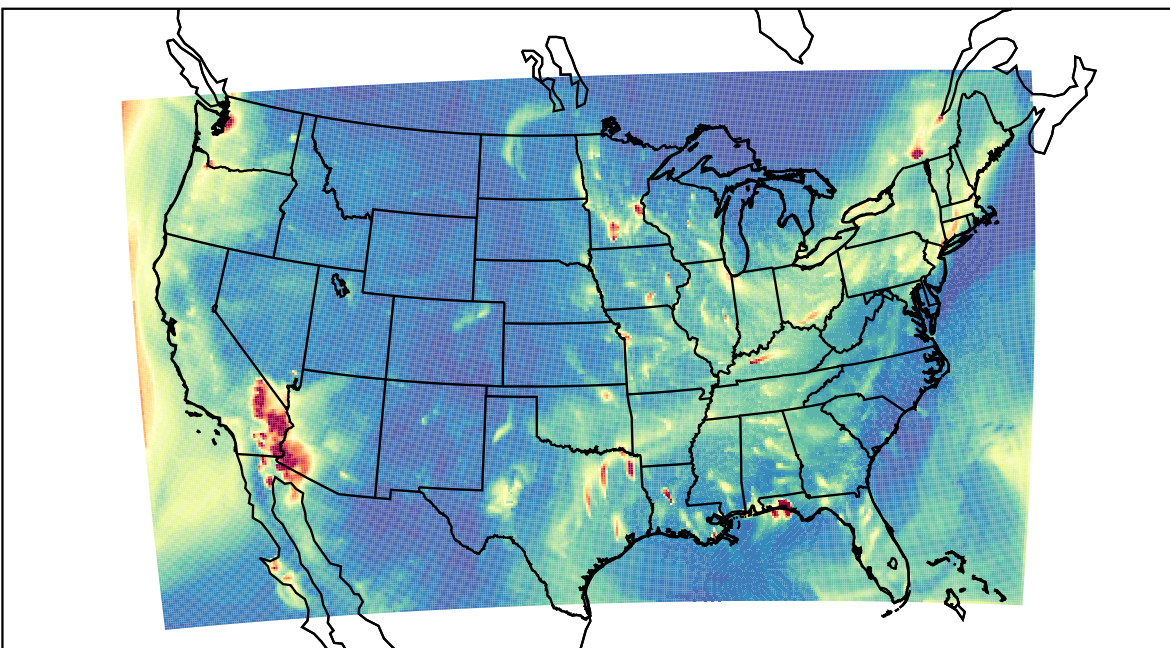
WRF 2023-02-06_05:00:00
