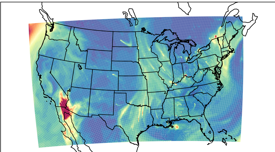
WRF 2023-02-06_19:00:00
