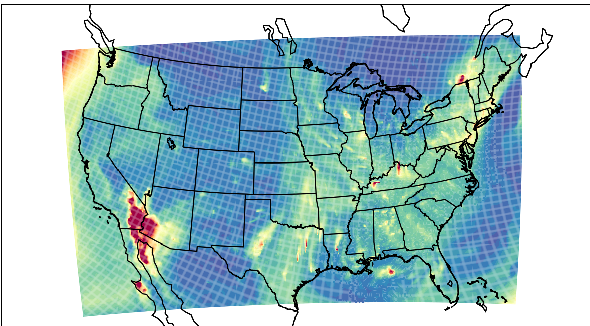
WRF 2023-02-06_14:00:00
