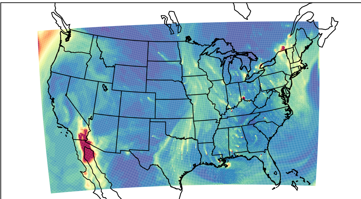
WRF 2023-02-06_22:00:00
