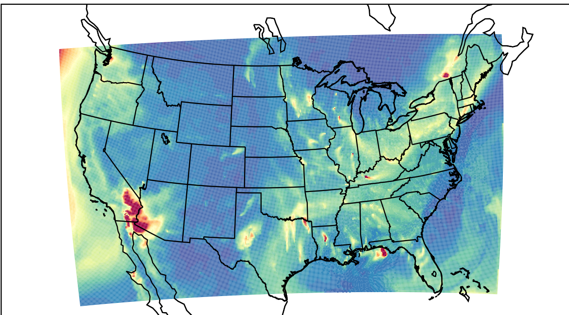
WRF 2023-02-06_08:00:00
