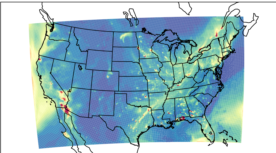
WRF 2023-02-06_00:00:00
