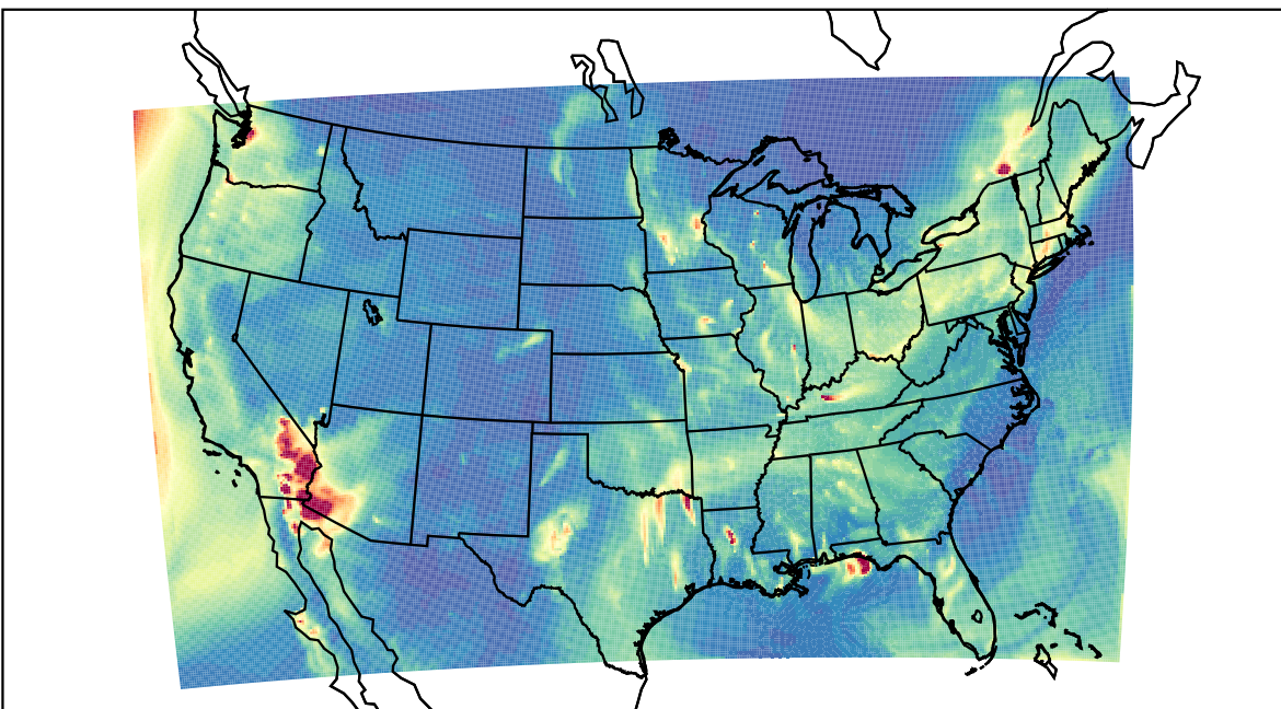
WRF 2023-02-06_07:00:00
