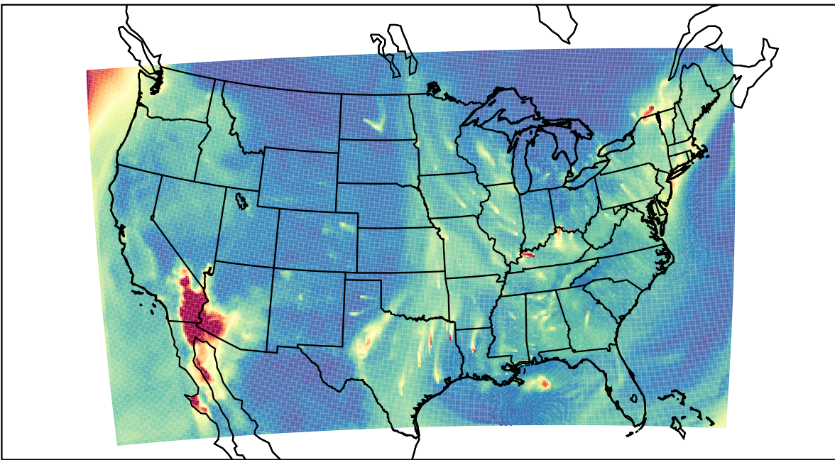
WRF 2023-02-06_16:00:00
