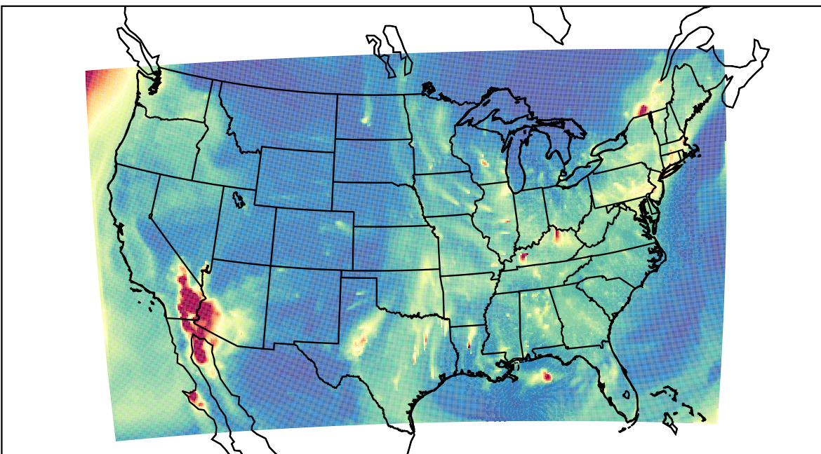
WRF 2023-02-06_13:00:00
