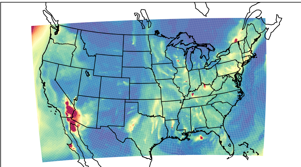
WRF 2023-02-06_12:00:00
