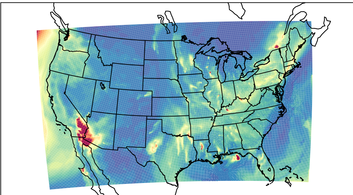
WRF 2023-02-06_09:00:00
