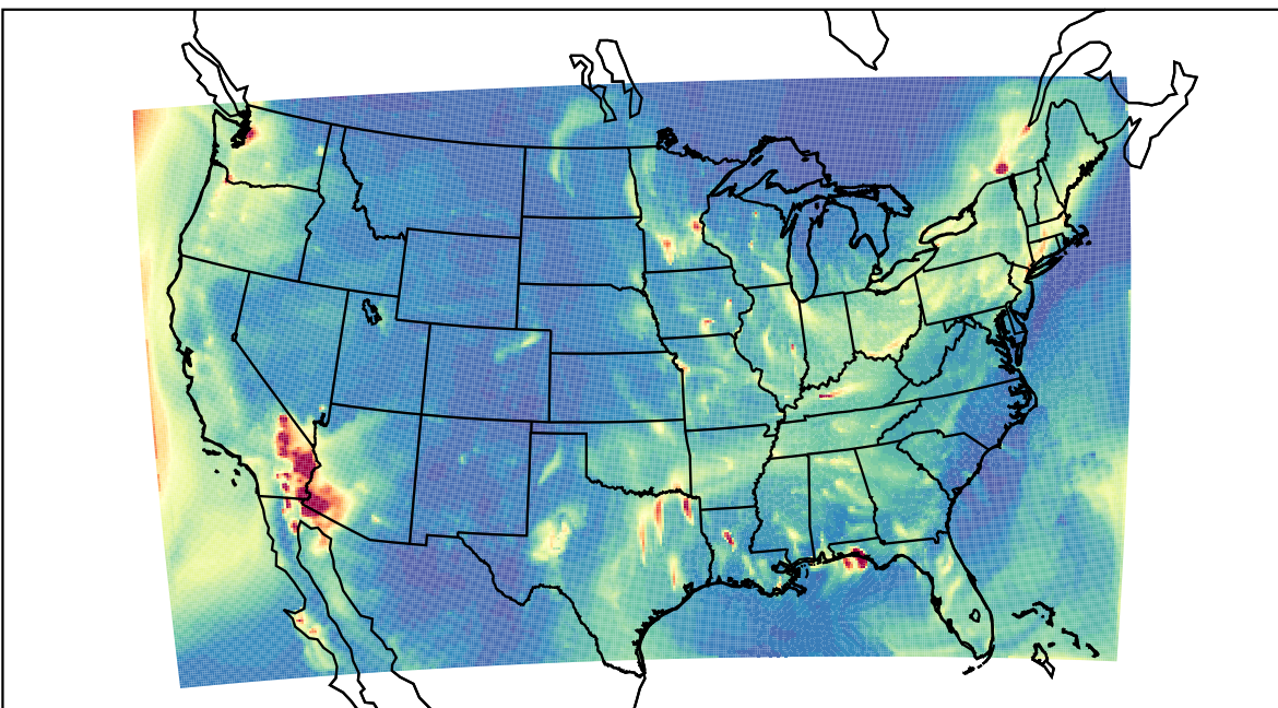
WRF 2023-02-06_06:00:00
