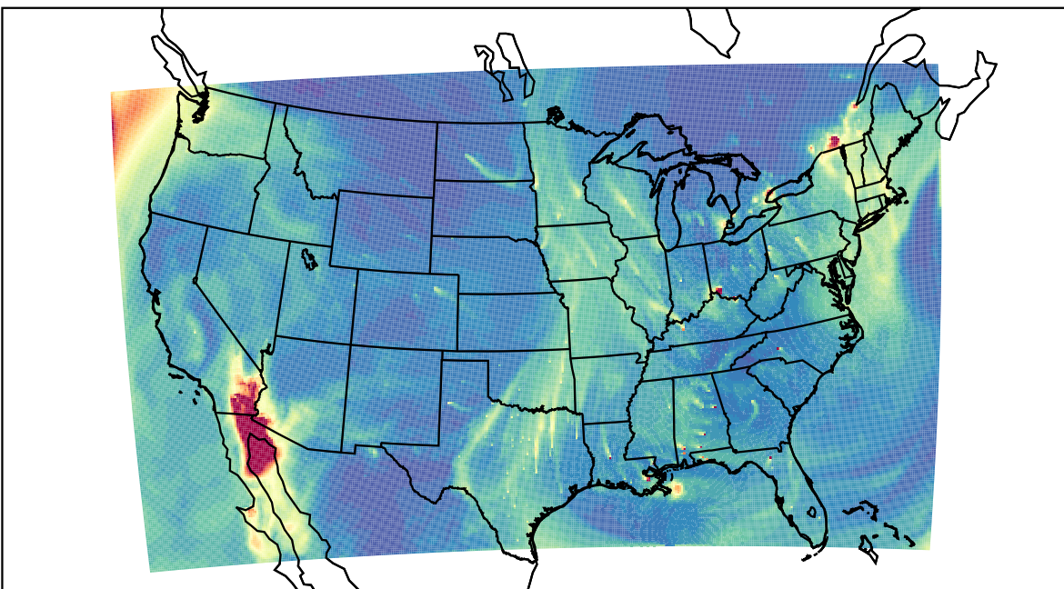
WRF 2023-02-06_21:00:00
