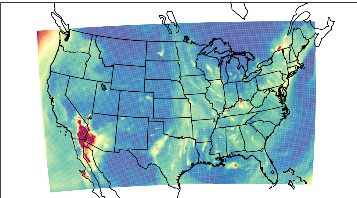
WRF 2023-02-06_15:00:00
