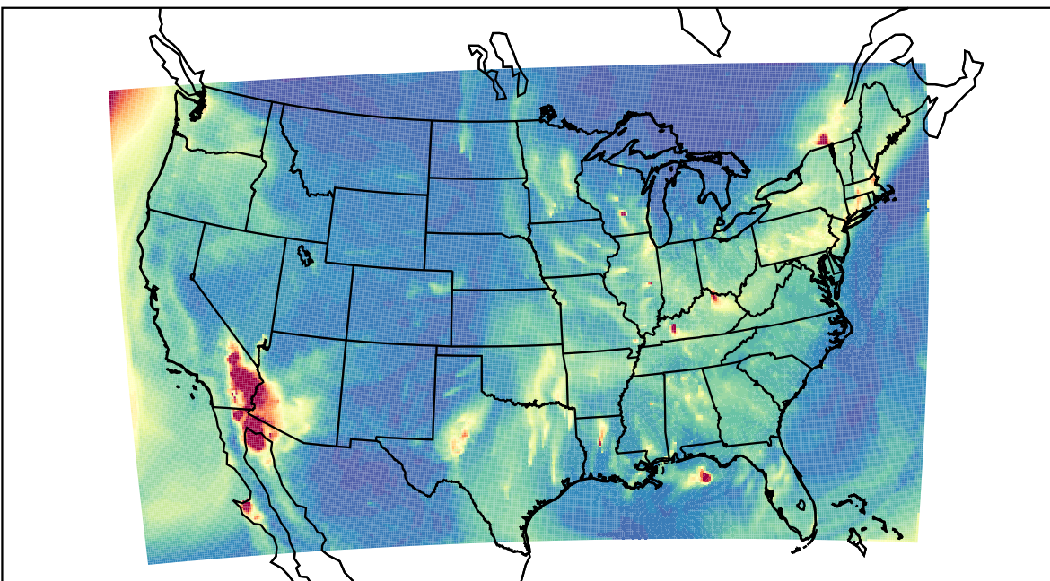
WRF 2023-02-06_11:00:00
