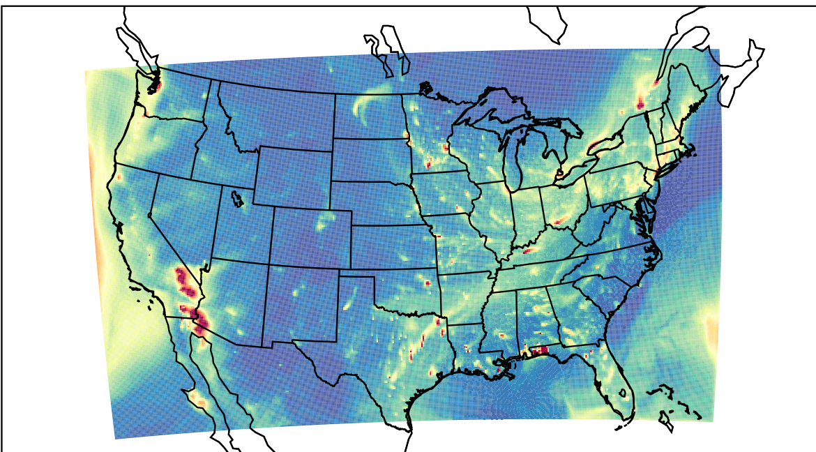
WRF 2023-02-06_02:00:00
