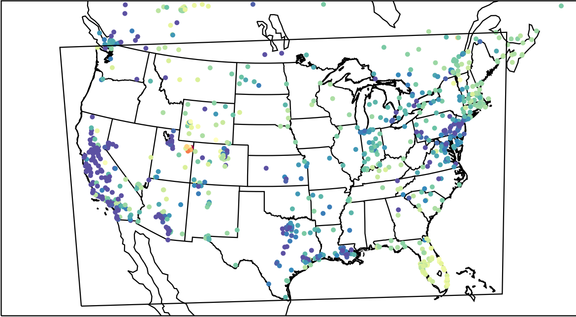
AirNOW (2023-02-07_15:00:00)
