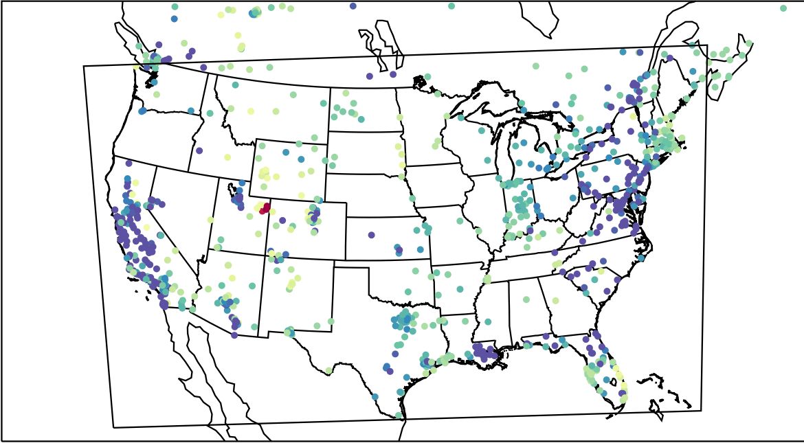
AirNOW (2023-02-07_08:00:00)
