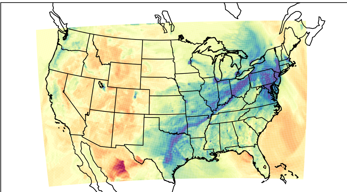
WRF (2023-02-08_00:00:00)
