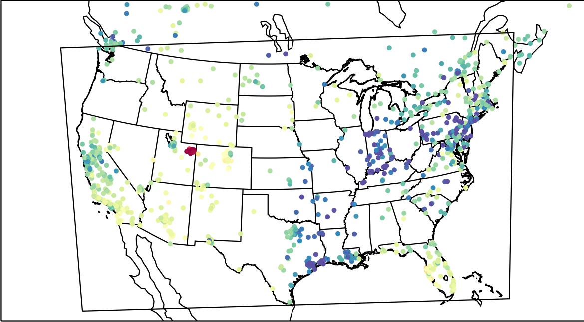
AirNOW (2023-02-08_23:00:00)
