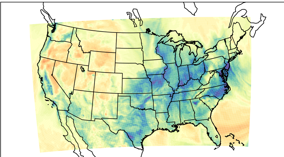
WRF (2023-02-07_07:00:00)
