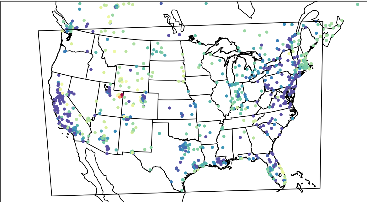
AirNOW (2023-02-07_11:00:00)
