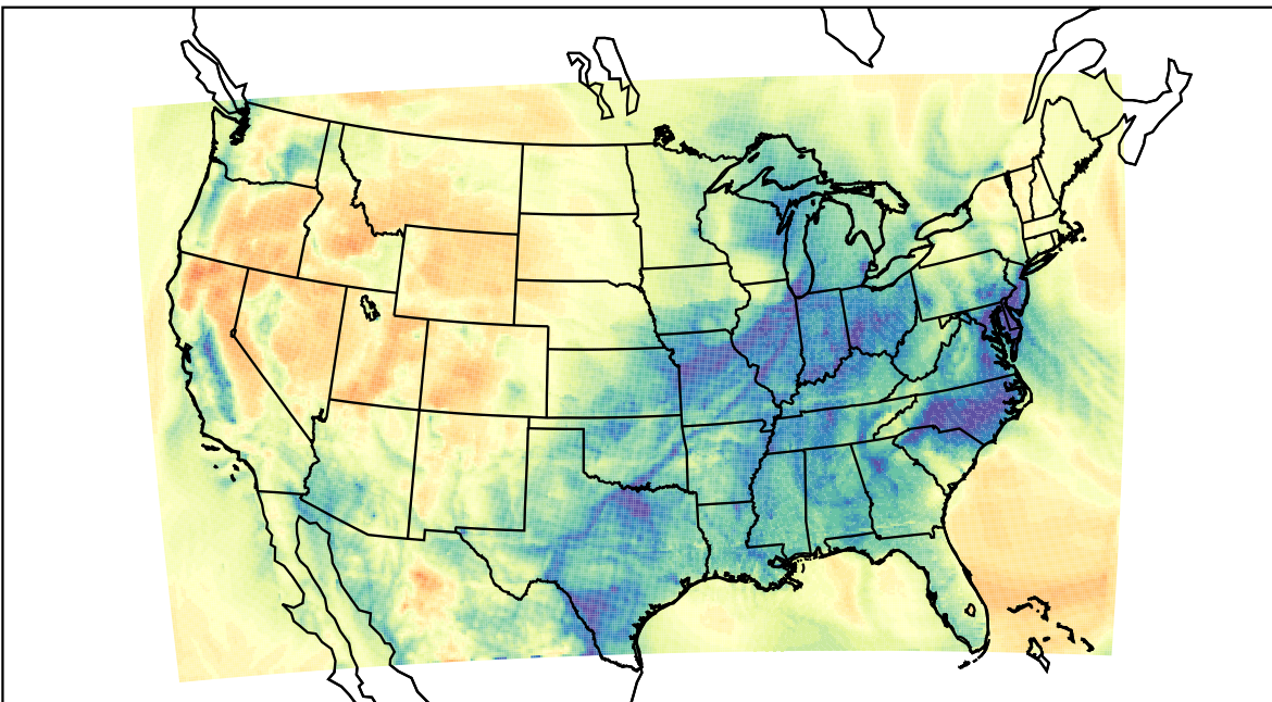
WRF (2023-02-07_12:00:00)
