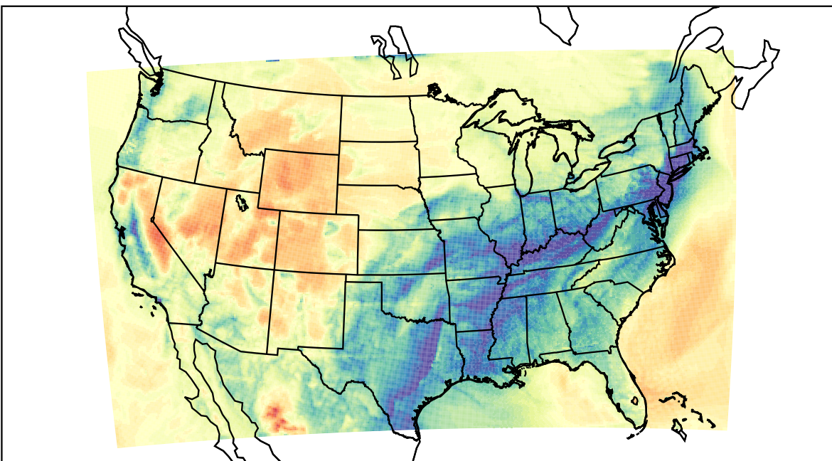
WRF (2023-02-08_09:00:00)
