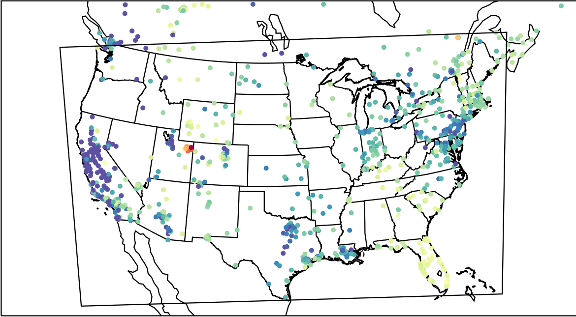
AirNOW (2023-02-07_16:00:00)
