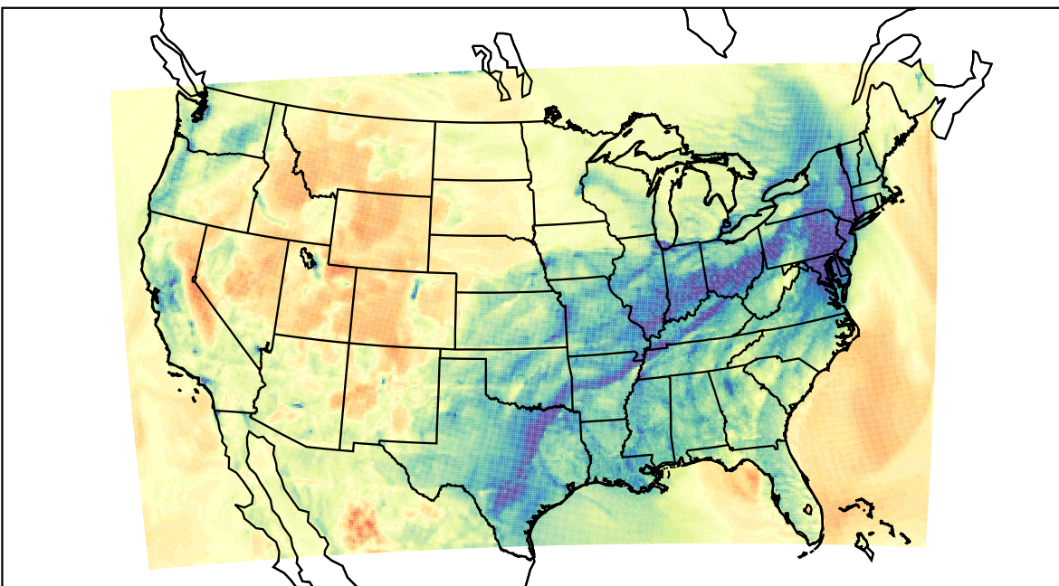
WRF (2023-02-08_03:00:00)
