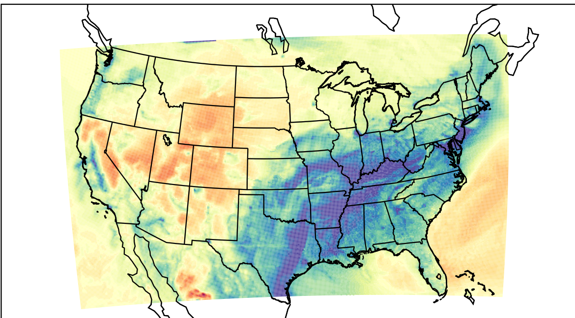
WRF (2023-02-08_13:00:00)
