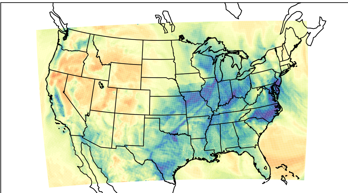
WRF (2023-02-07_10:00:00)
