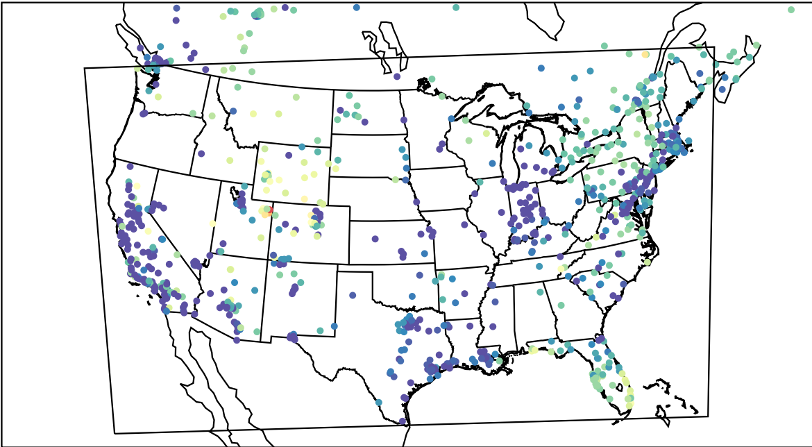
AirNOW (2023-02-08_14:00:00)
