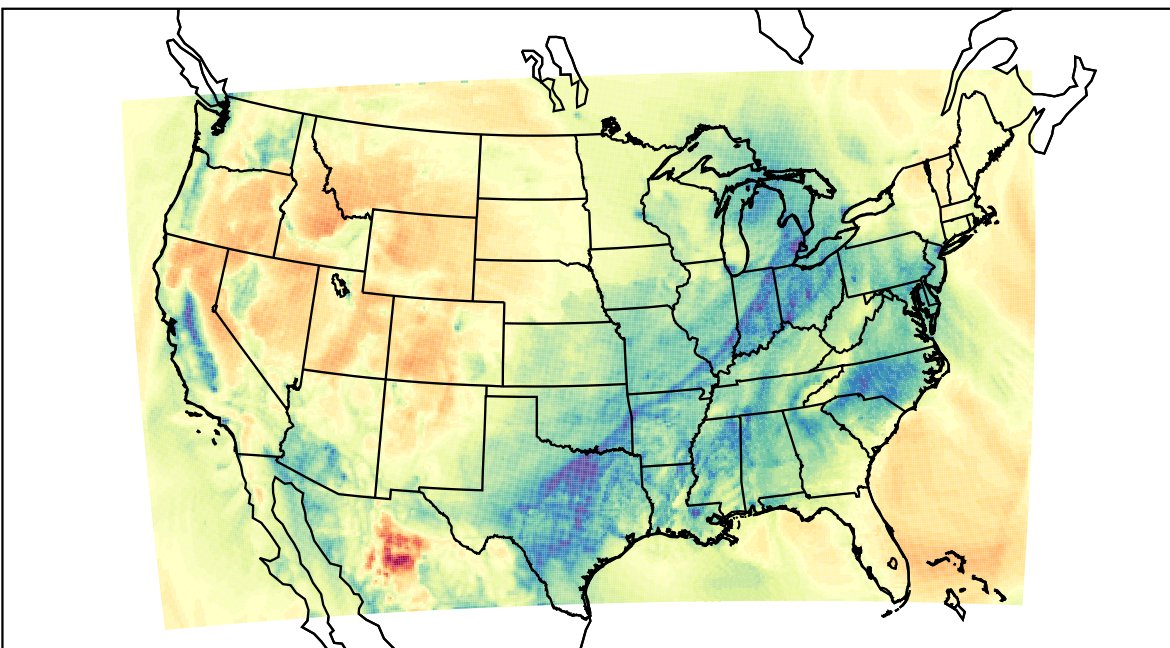
WRF (2023-02-07_16:00:00)
