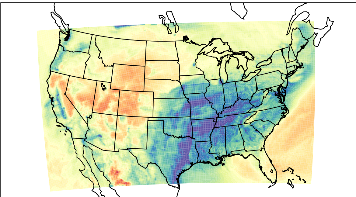
WRF (2023-02-08_15:00:00)
