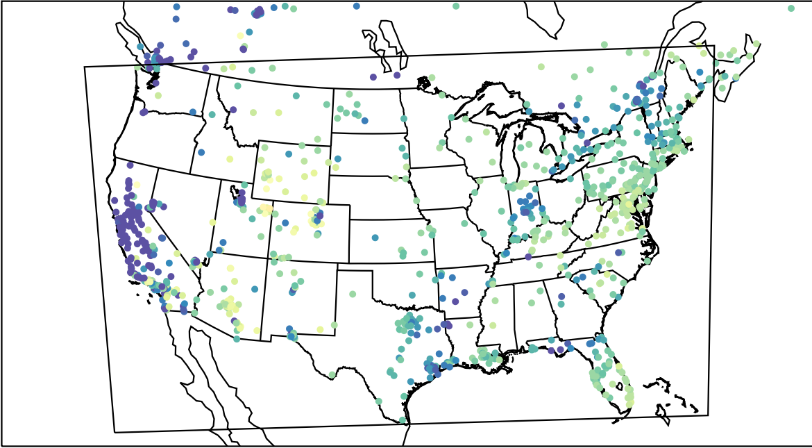
AirNOW (2023-02-10_16:00:00)
