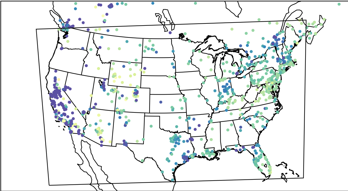
AirNOW (2023-02-10_15:00:00)
