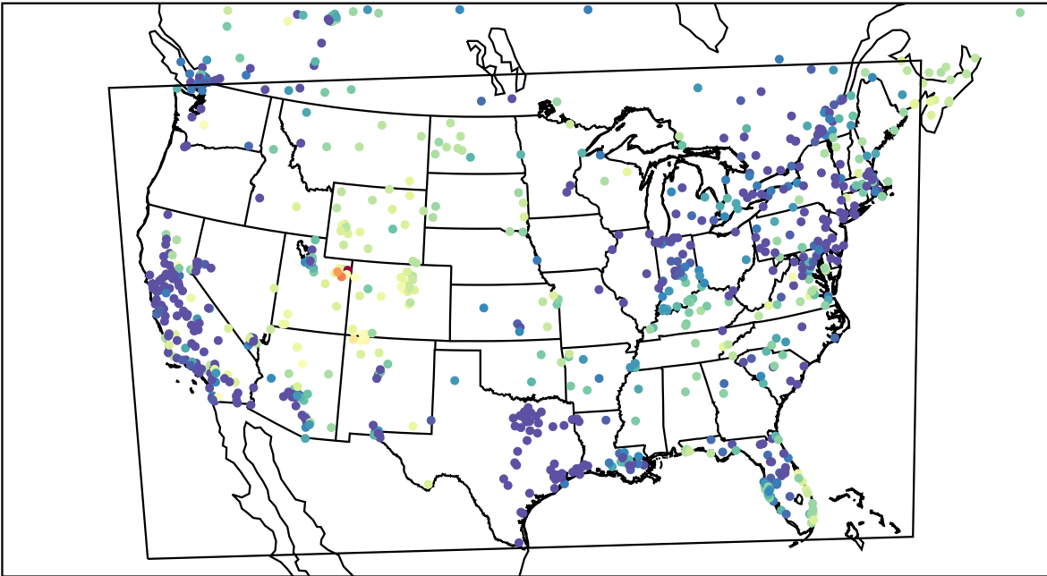
AirNOW (2023-02-09_09:00:00)
