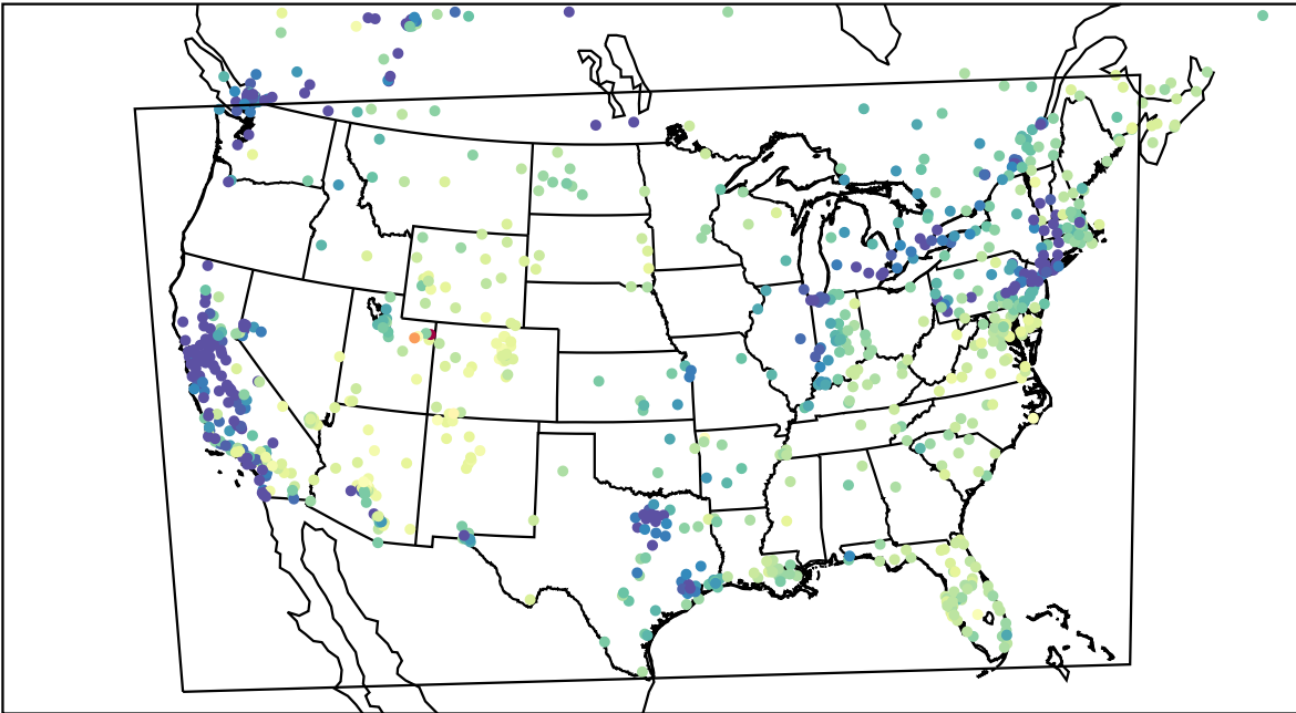
AirNOW (2023-02-09_17:00:00)
