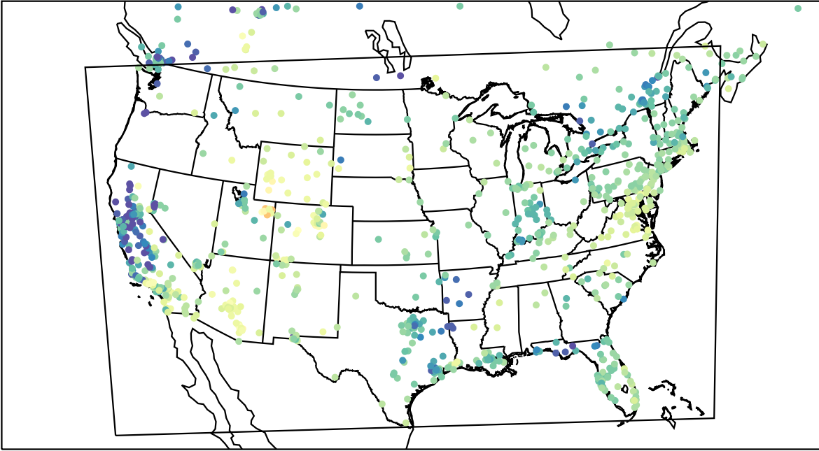
AirNOW (2023-02-10_18:00:00)
