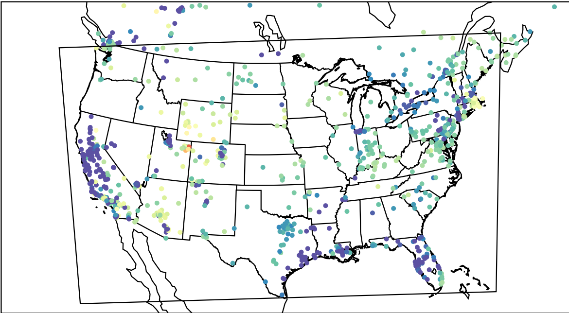
AirNOW (2023-02-10_07:00:00)
