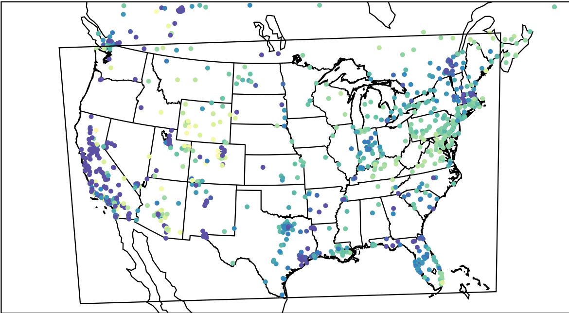
AirNOW (2023-02-10_14:00:00)
