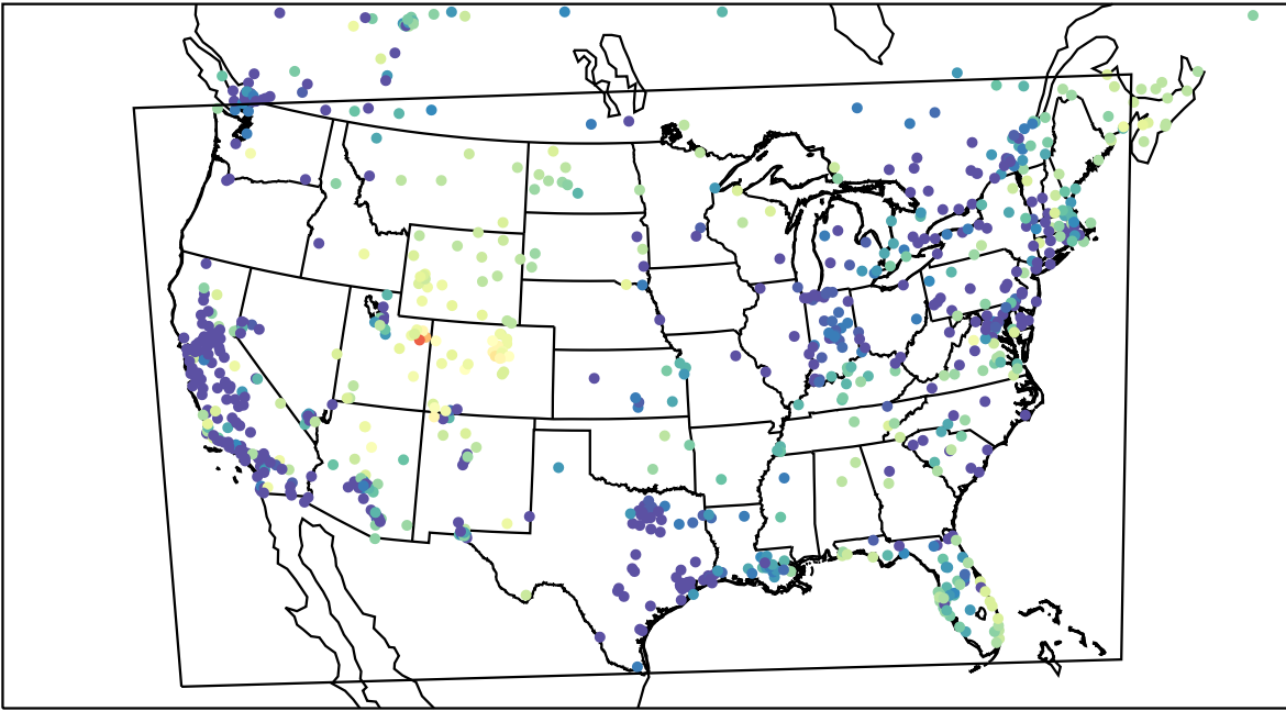
AirNOW (2023-02-09_06:00:00)
