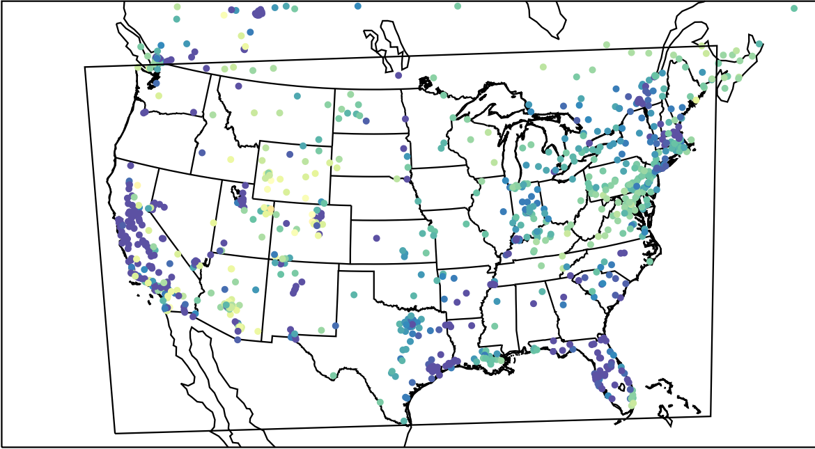
AirNOW (2023-02-10_13:00:00)
