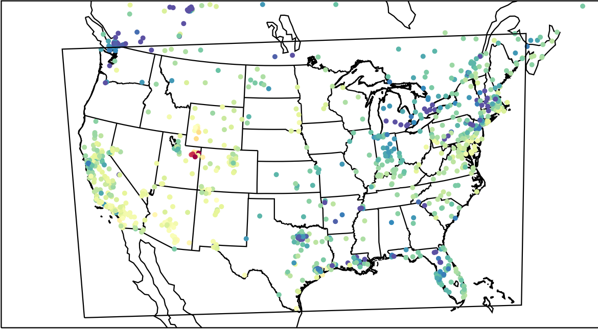
AirNOW (2023-02-10_00:00:00)
