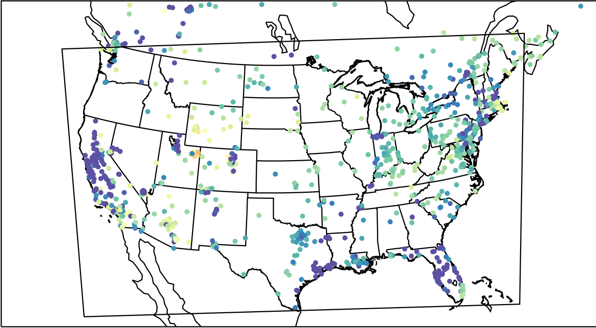
AirNOW (2023-02-10_09:00:00)
