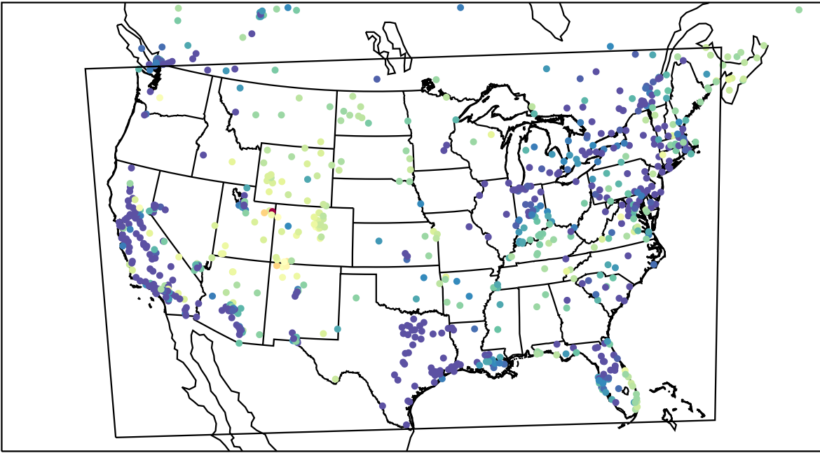
AirNOW (2023-02-09_10:00:00)
