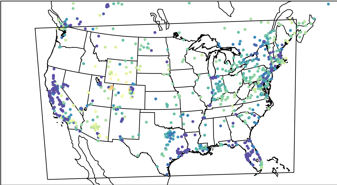
AirNOW (2023-02-10_10:00:00)
