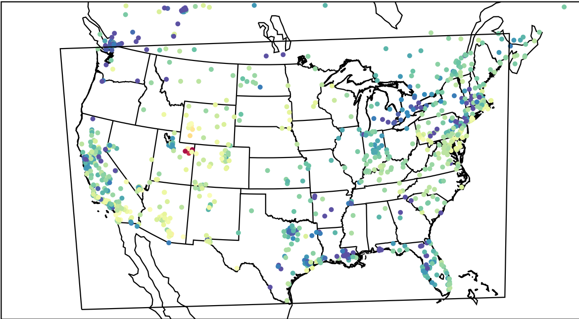
AirNOW (2023-02-10_01:00:00)
