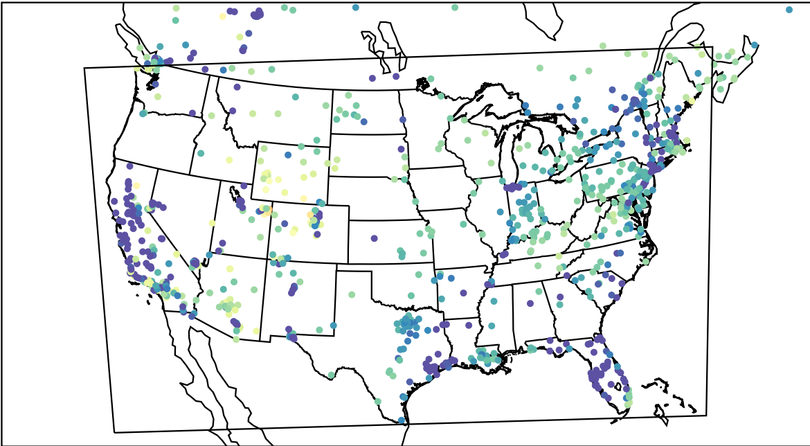
AirNOW (2023-02-10_11:00:00)
