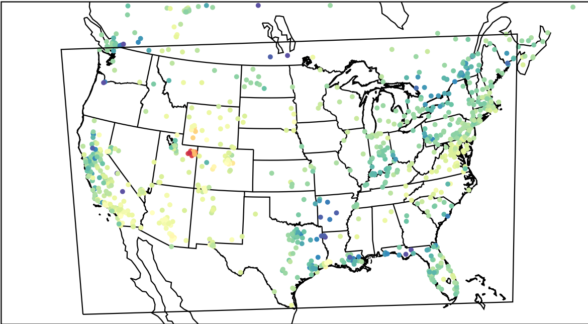
AirNOW (2023-02-10_20:00:00)
