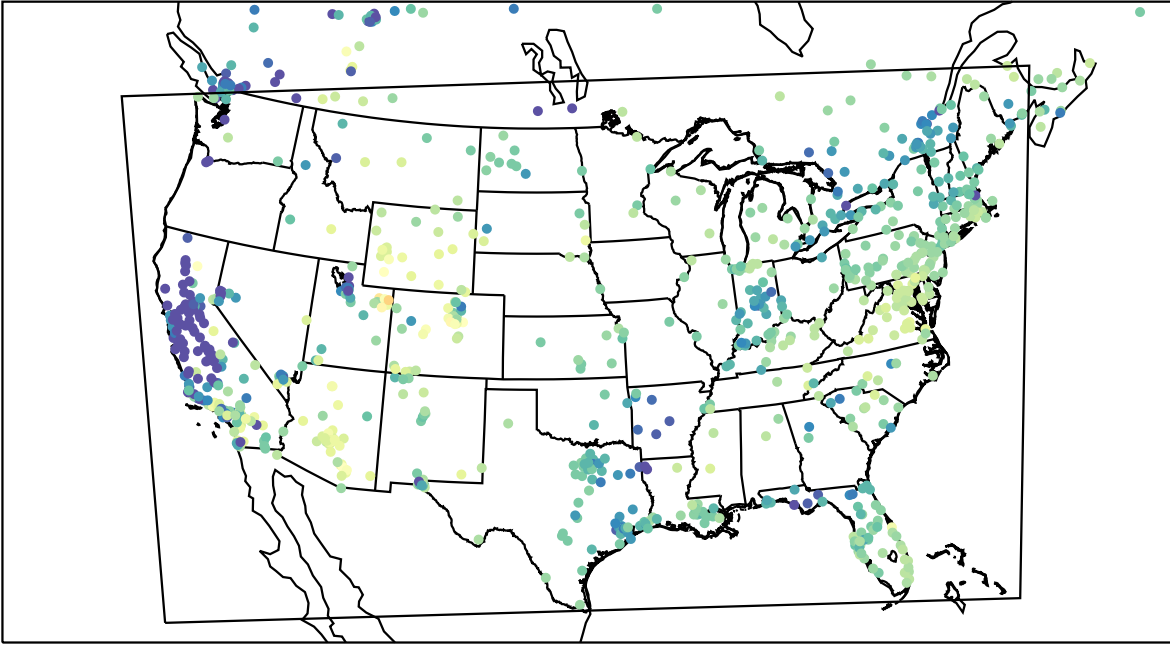
AirNOW (2023-02-10_17:00:00)
