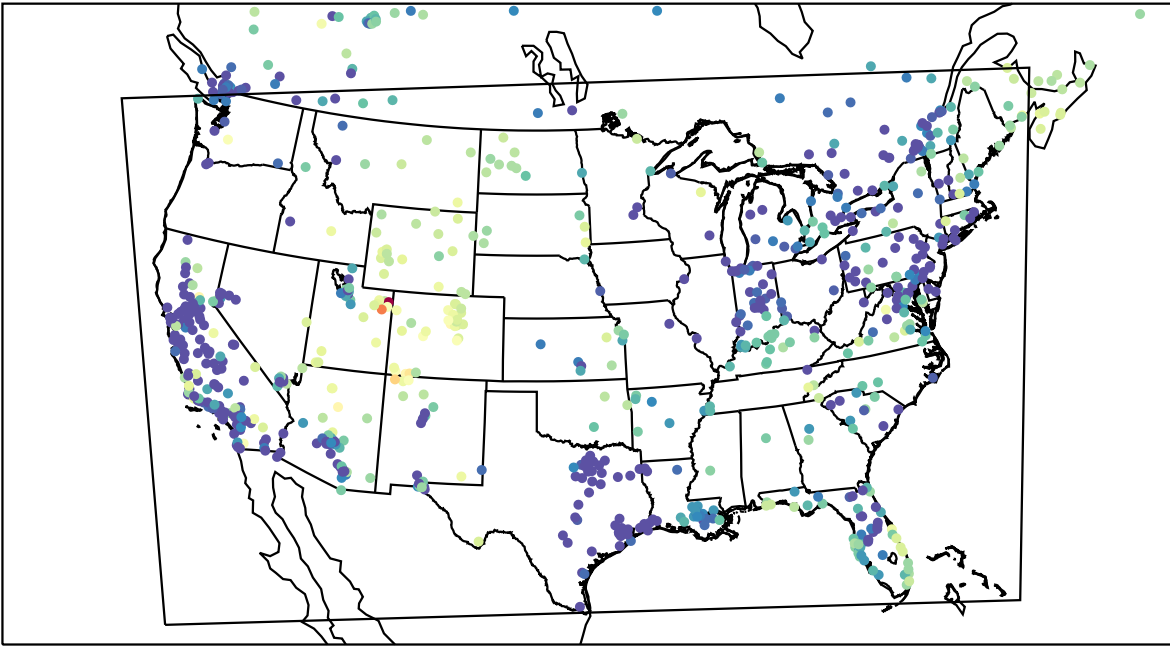
AirNOW (2023-02-09_08:00:00)
