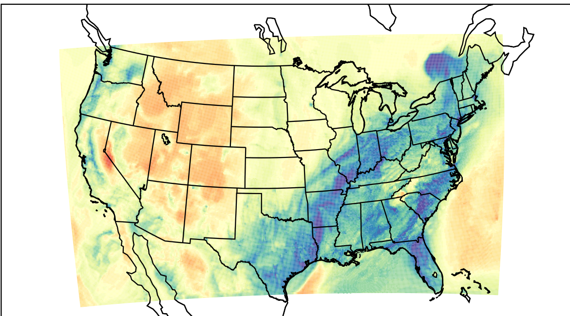
WRF (2023-02-10_13:00:00)
