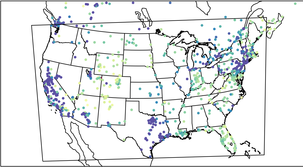
AirNOW (2023-02-09_15:00:00)
