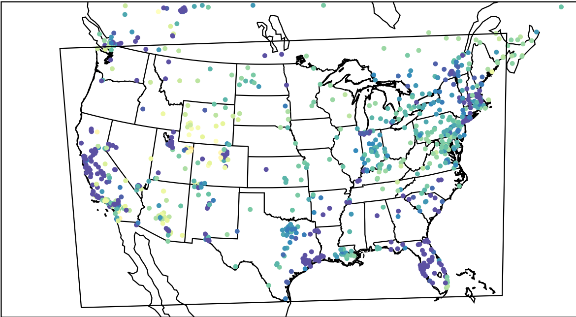
AirNOW (2023-02-10_12:00:00)
