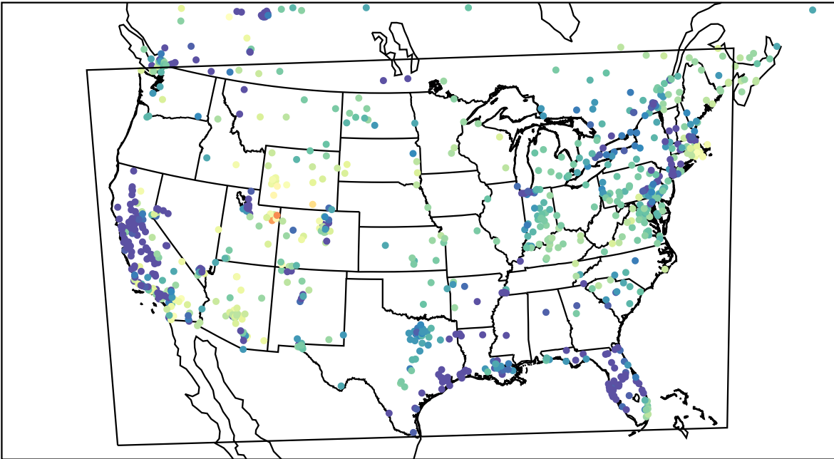
AirNOW (2023-02-10_08:00:00)
