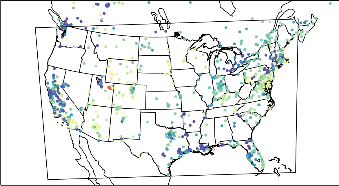
AirNOW (2023-02-10_02:00:00)
