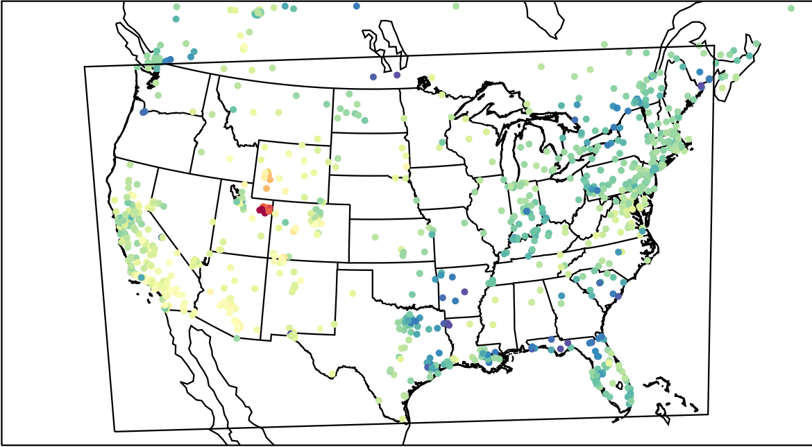
AirNOW (2023-02-10_22:00:00)
