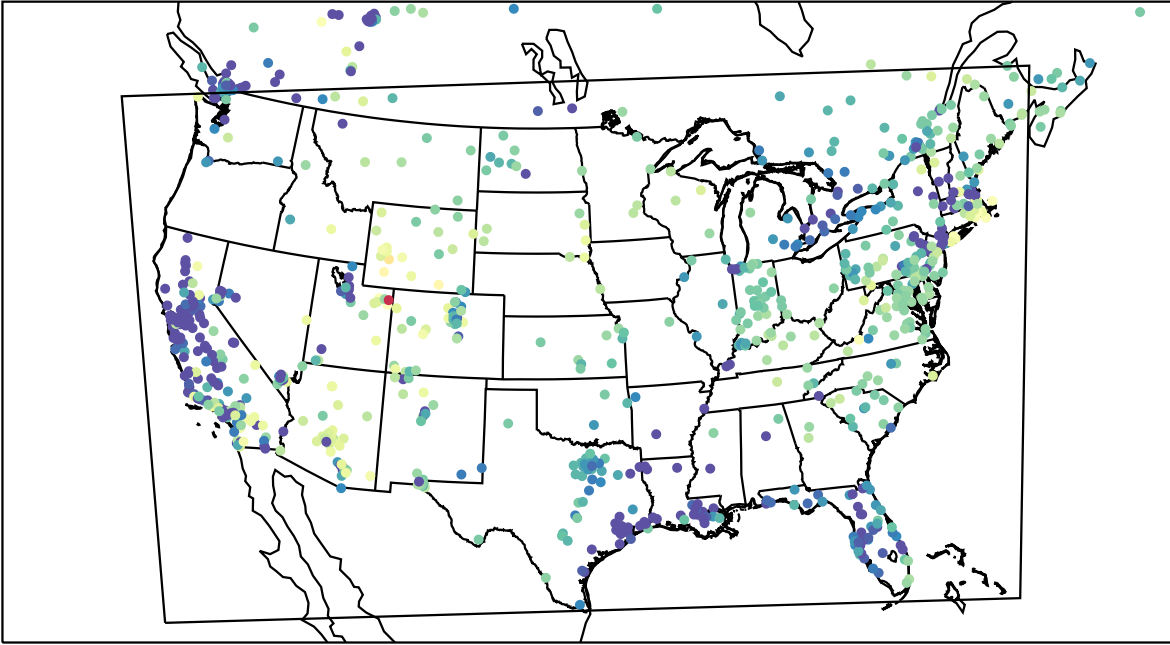
AirNOW (2023-02-10_05:00:00)
