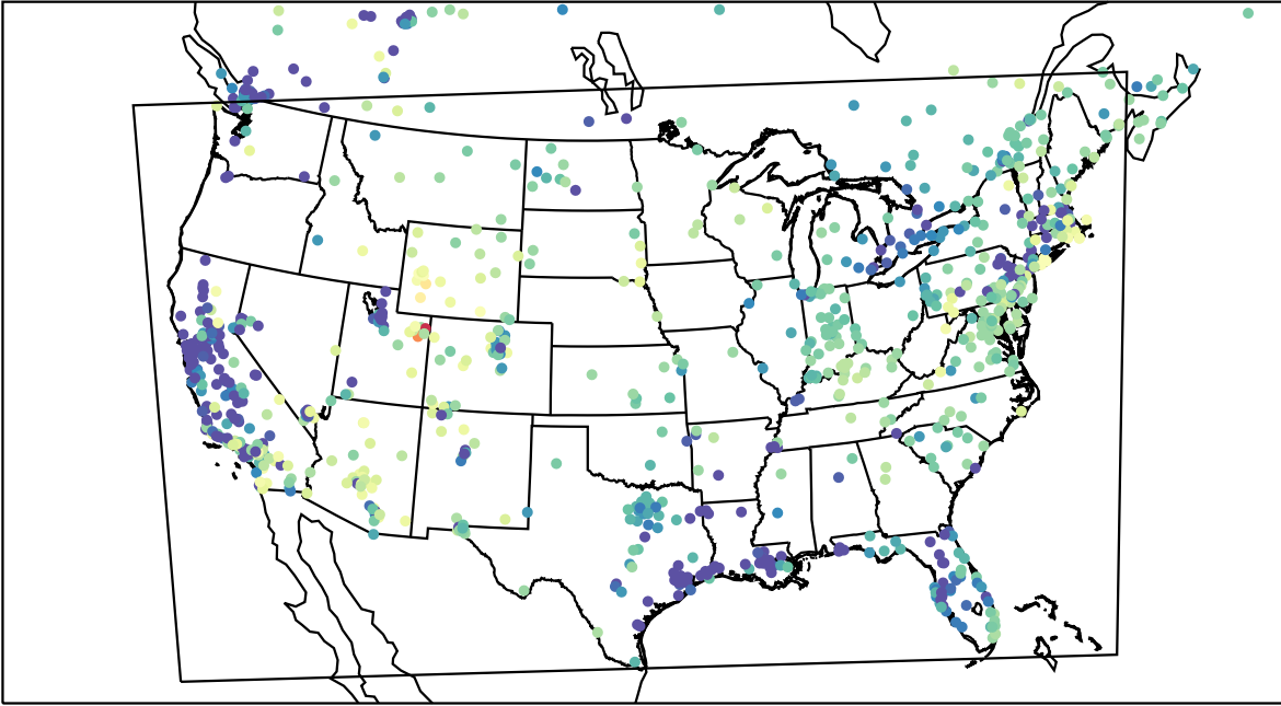
AirNOW (2023-02-10_04:00:00)
