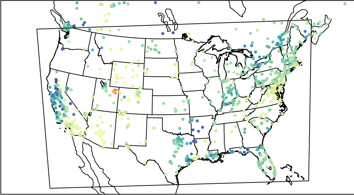
AirNOW (2023-02-10_19:00:00)
