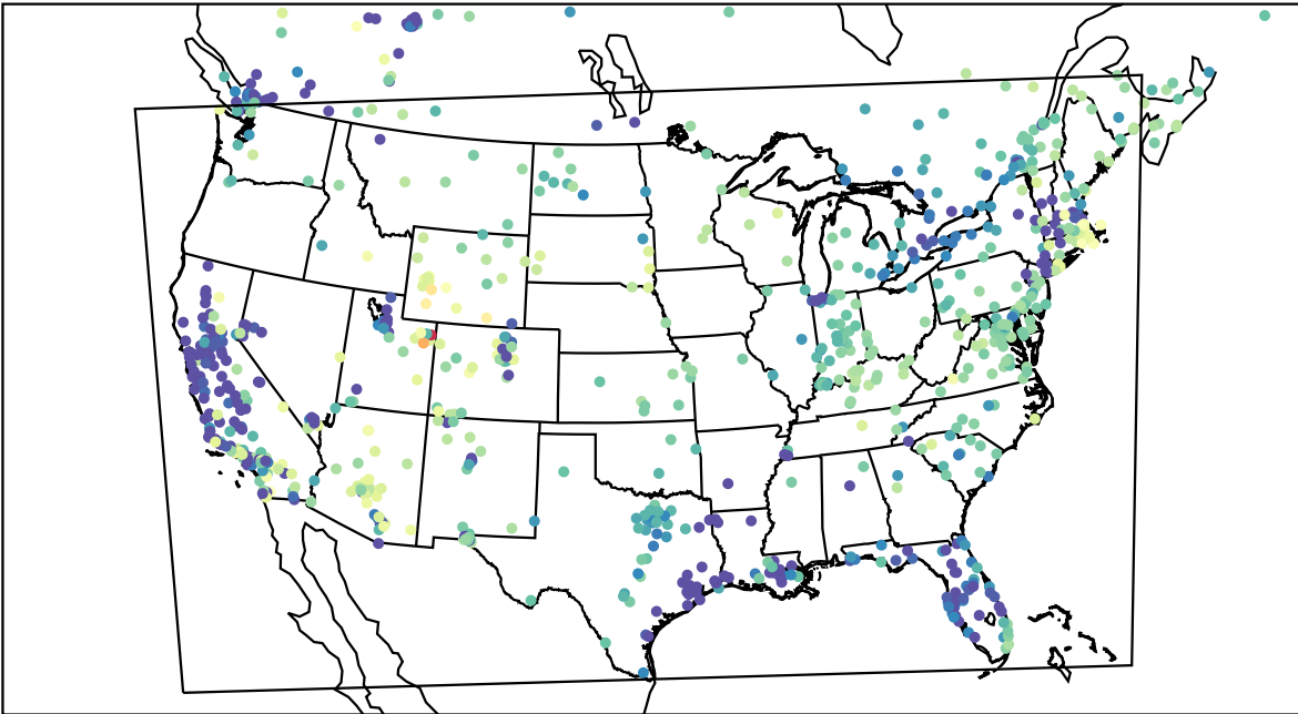
AirNOW (2023-02-10_06:00:00)
