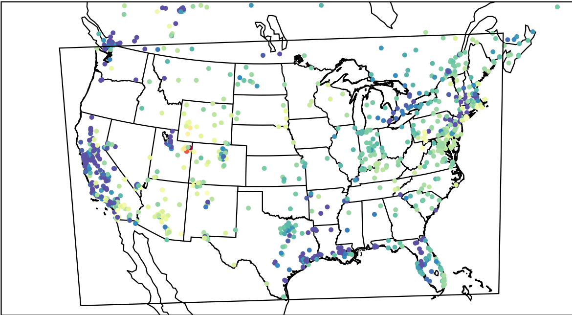
AirNOW (2023-02-10_03:00:00)
