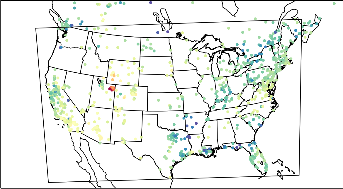
AirNOW (2023-02-10_21:00:00)
