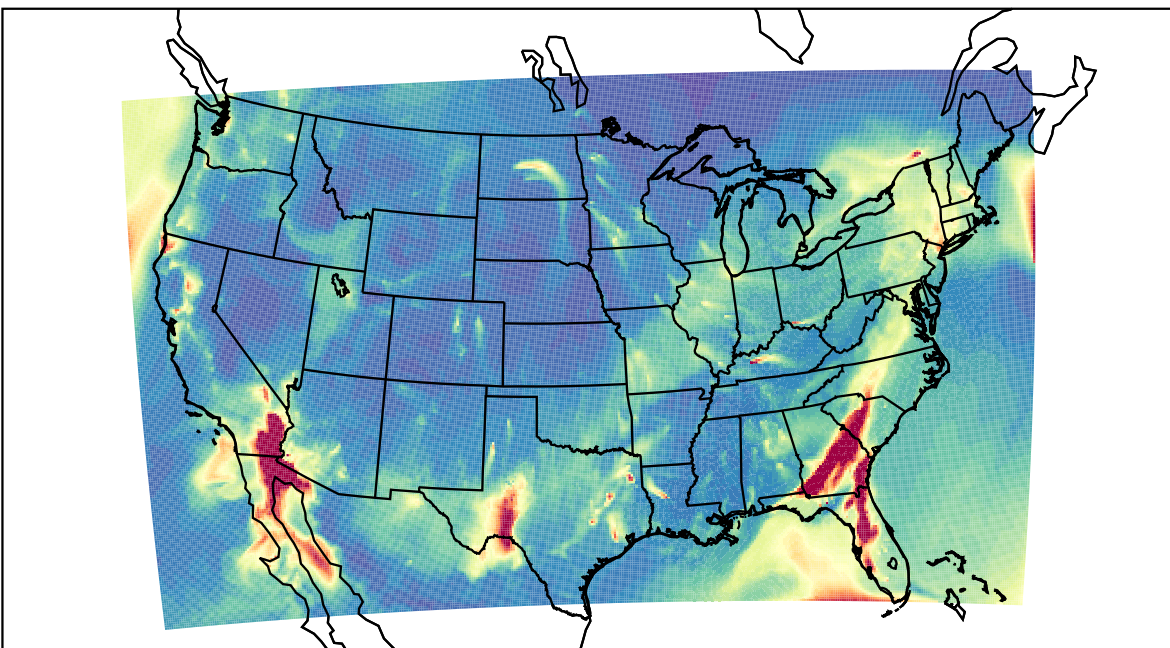
WRF 2023-02-10_06:00:00
