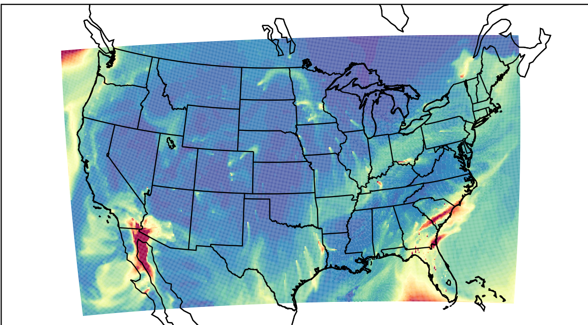
WRF 2023-02-10_17:00:00
