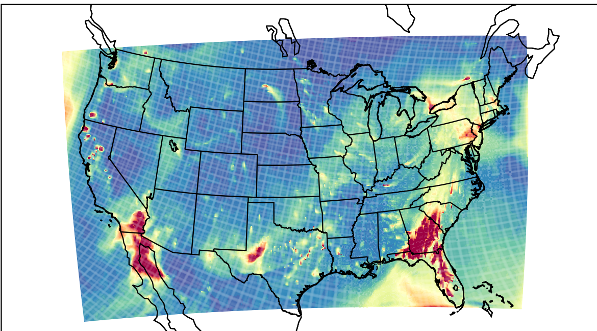
WRF 2023-02-10_02:00:00
