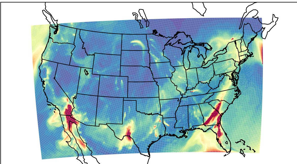
WRF 2023-02-10_07:00:00
