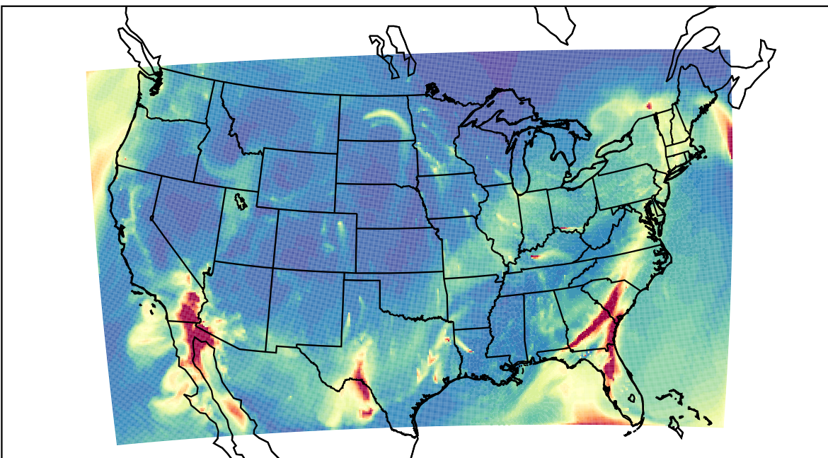
WRF 2023-02-10_09:00:00
