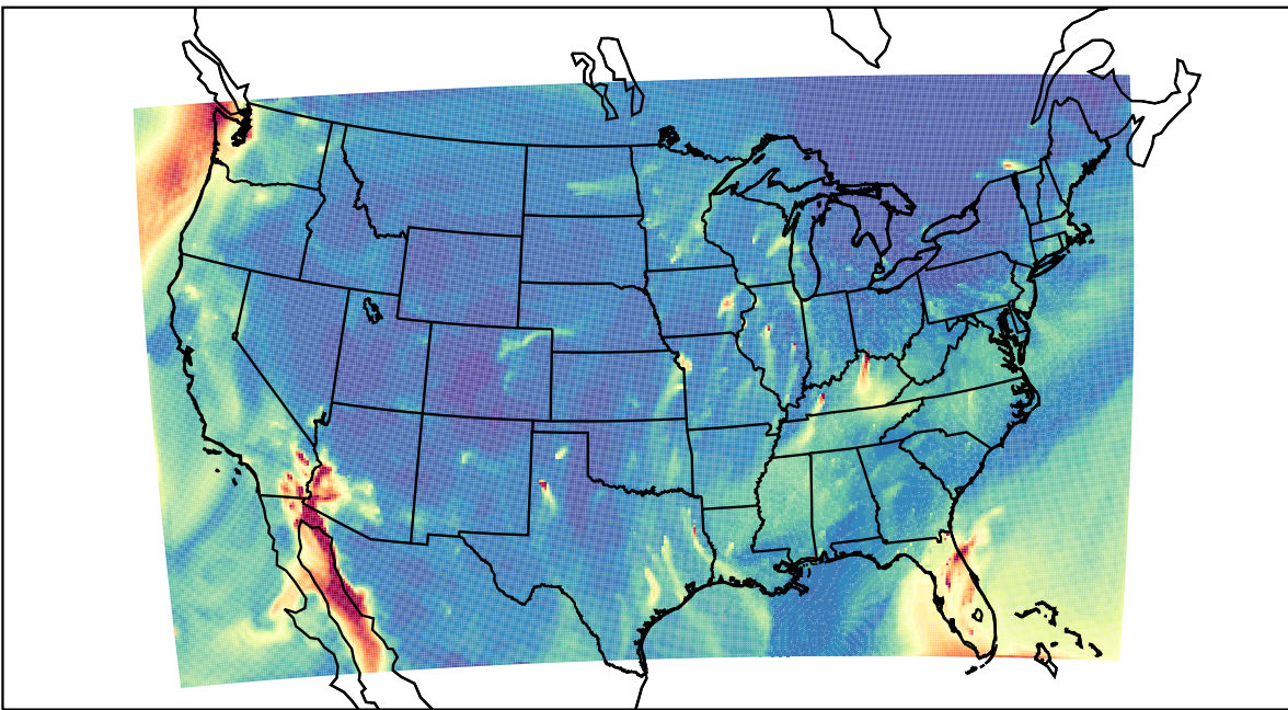
WRF 2023-02-11_09:00:00
