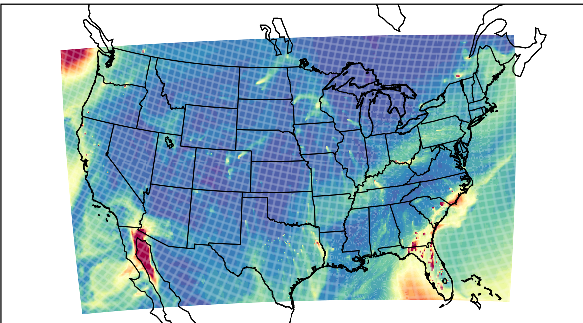
WRF 2023-02-10_21:00:00
