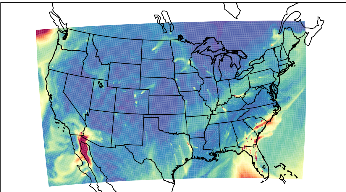
WRF 2023-02-10_19:00:00
