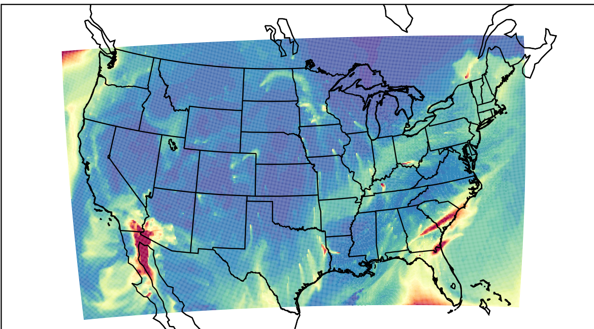
WRF 2023-02-10_16:00:00
