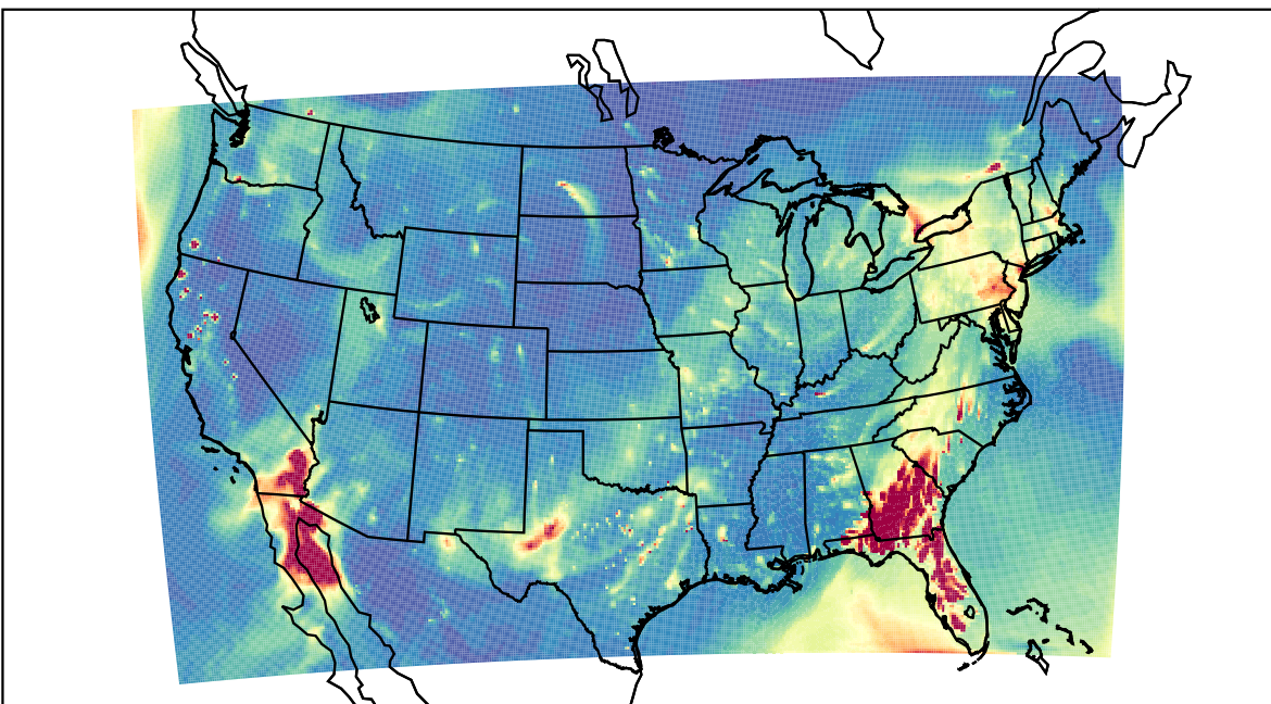
WRF 2023-02-10_01:00:00
