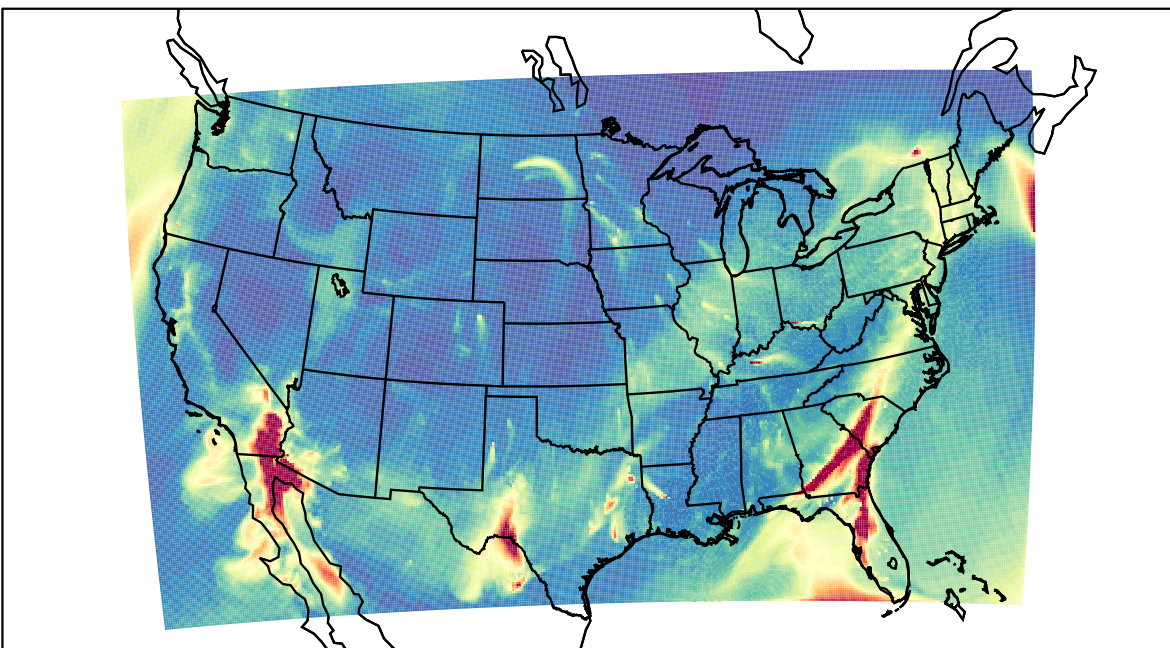
WRF 2023-02-10_08:00:00
