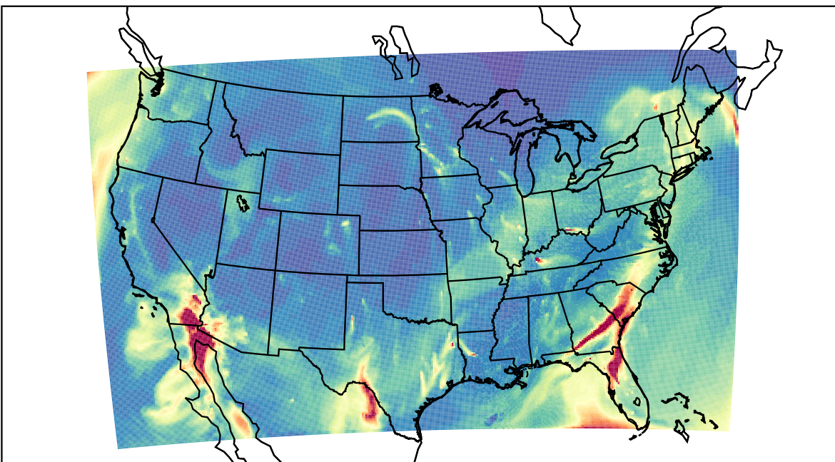
WRF 2023-02-10_11:00:00
