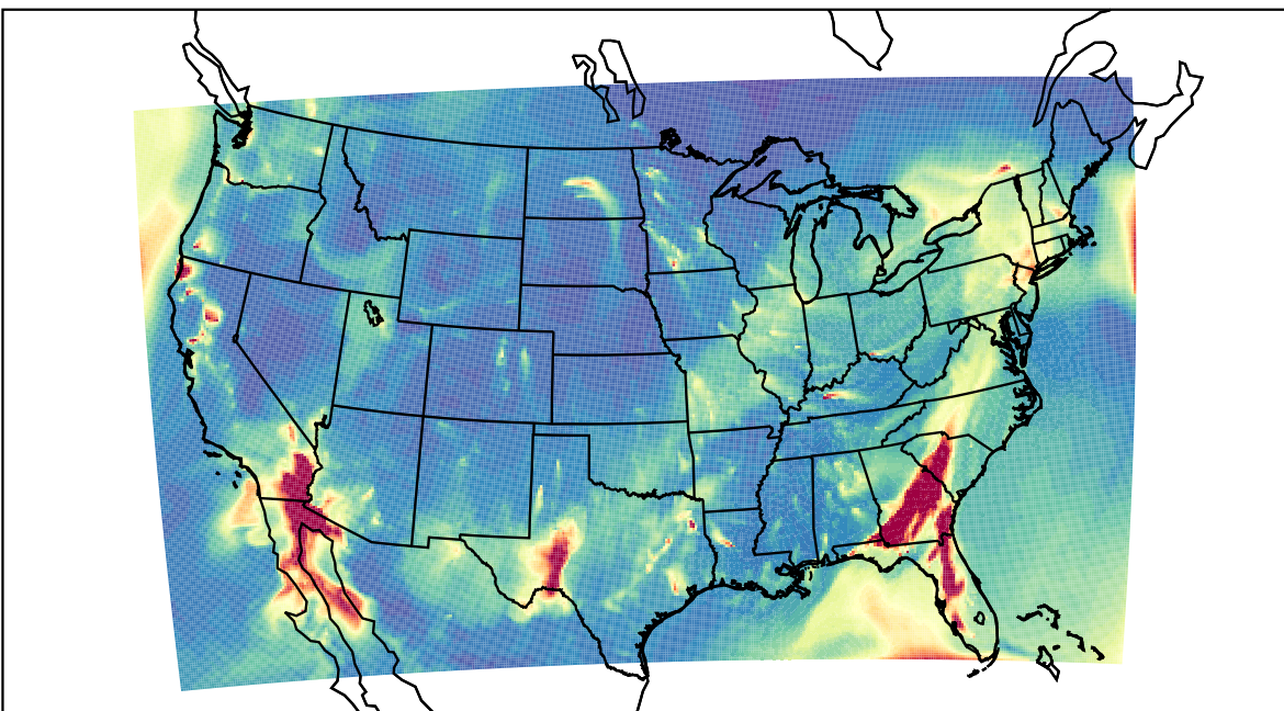
WRF 2023-02-10_05:00:00
