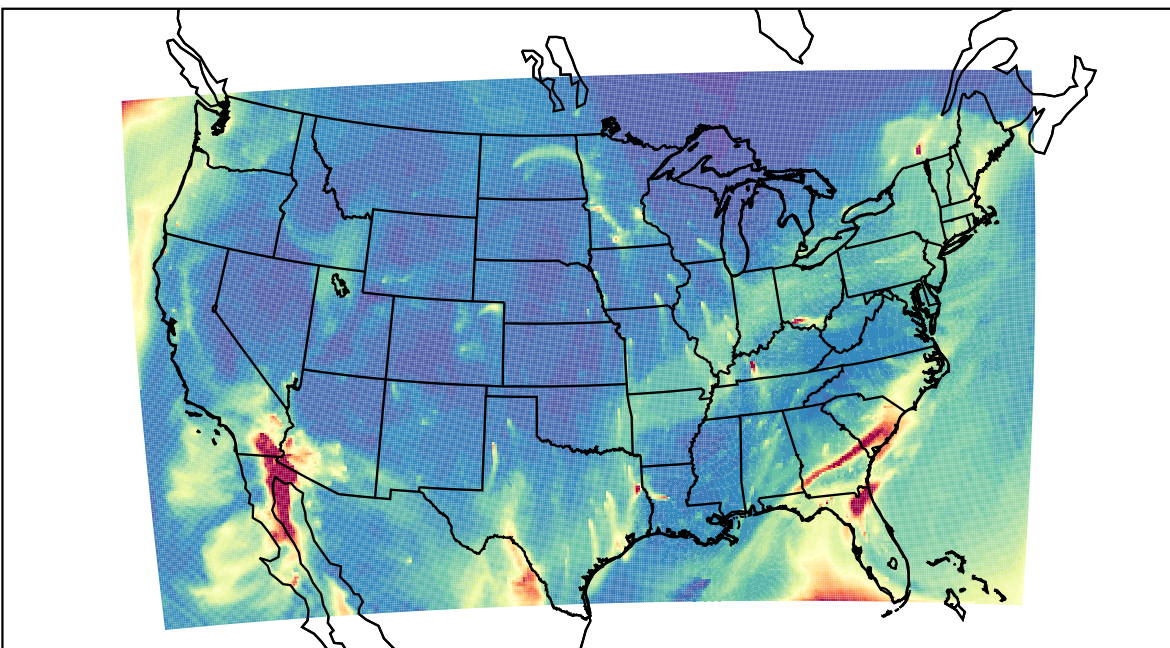
WRF 2023-02-10_14:00:00
