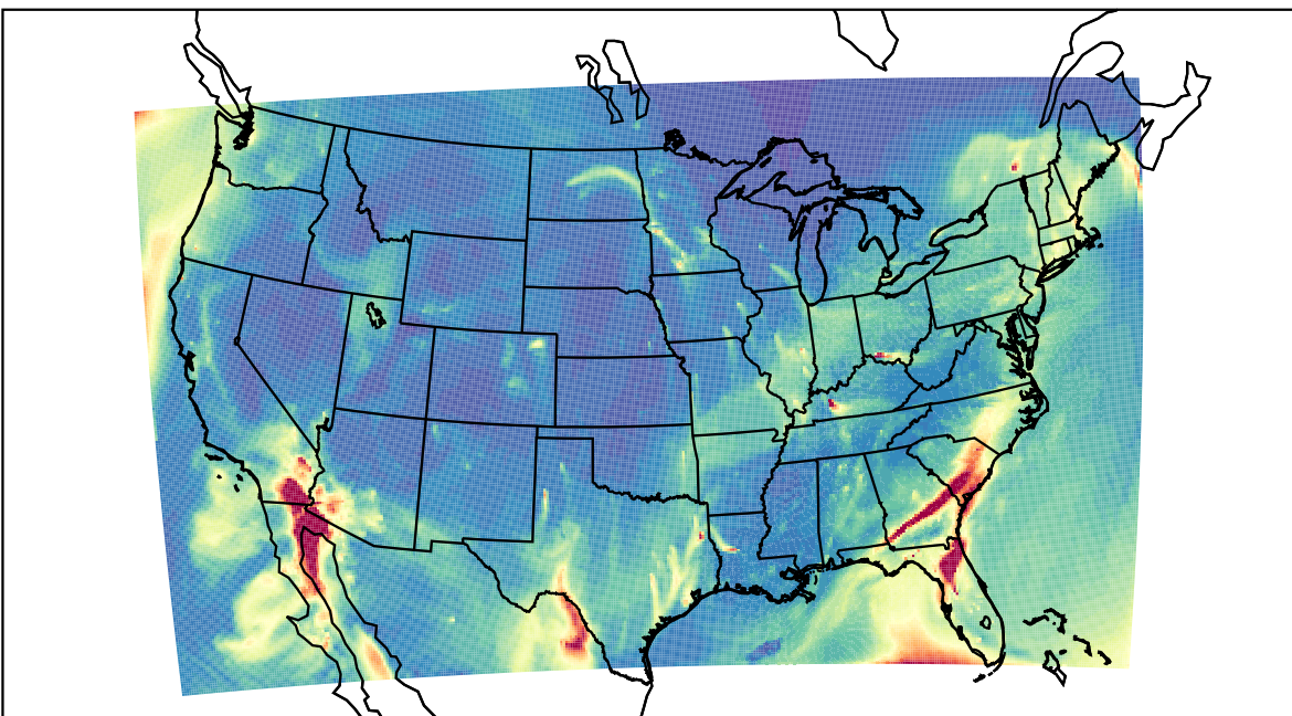
WRF 2023-02-10_12:00:00
