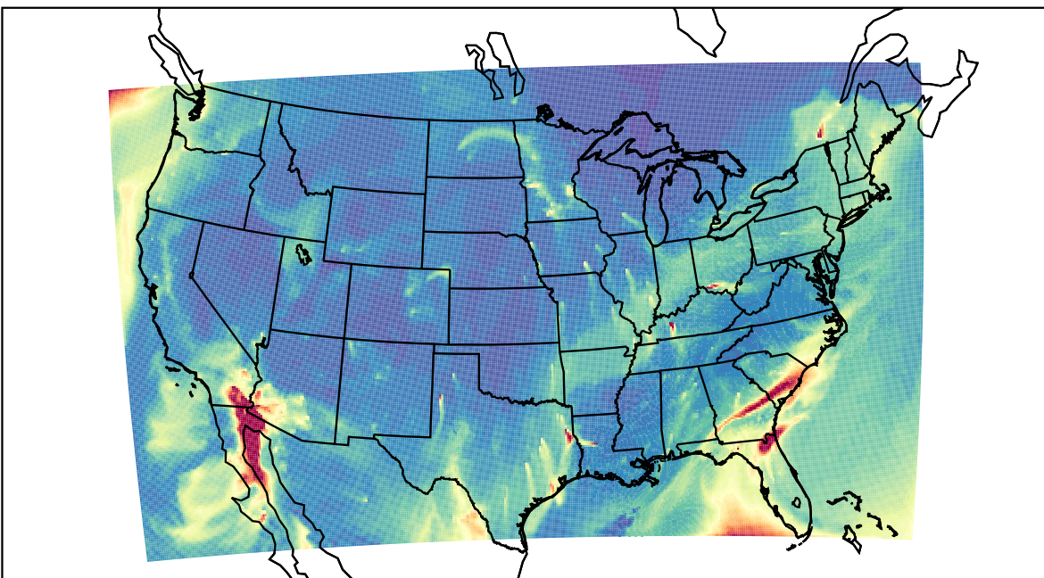
WRF 2023-02-10_15:00:00
