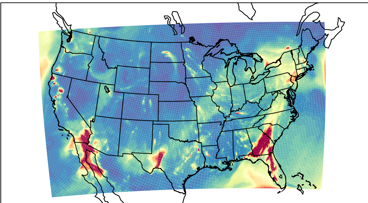
WRF 2023-02-10_04:00:00
