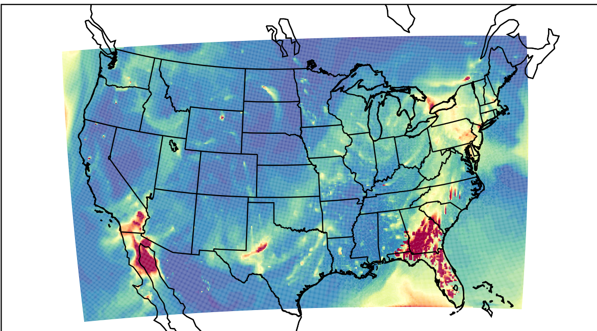
WRF 2023-02-10_00:00:00
