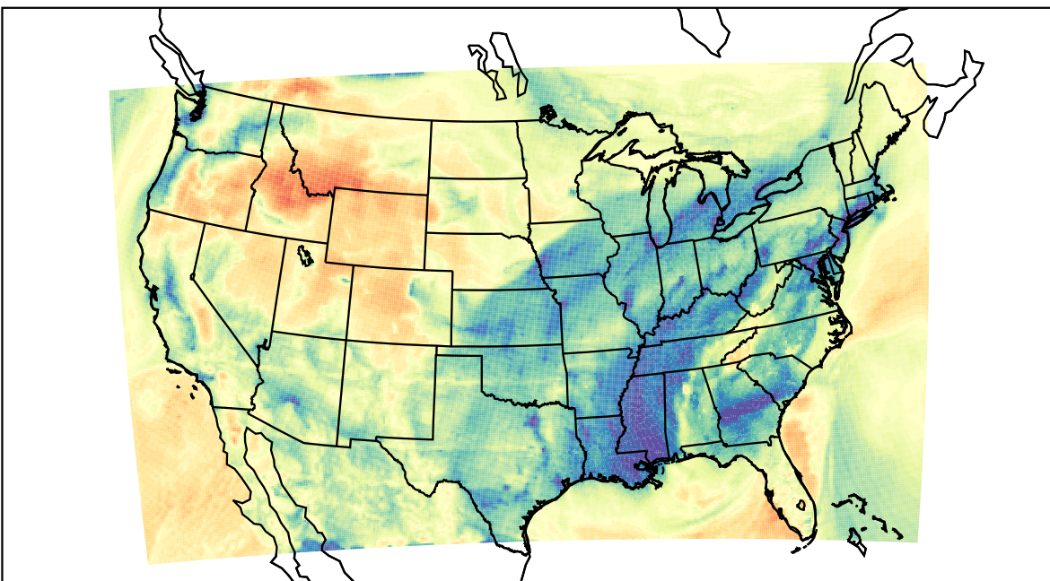
WRF (2023-02-12_12:00:00)
