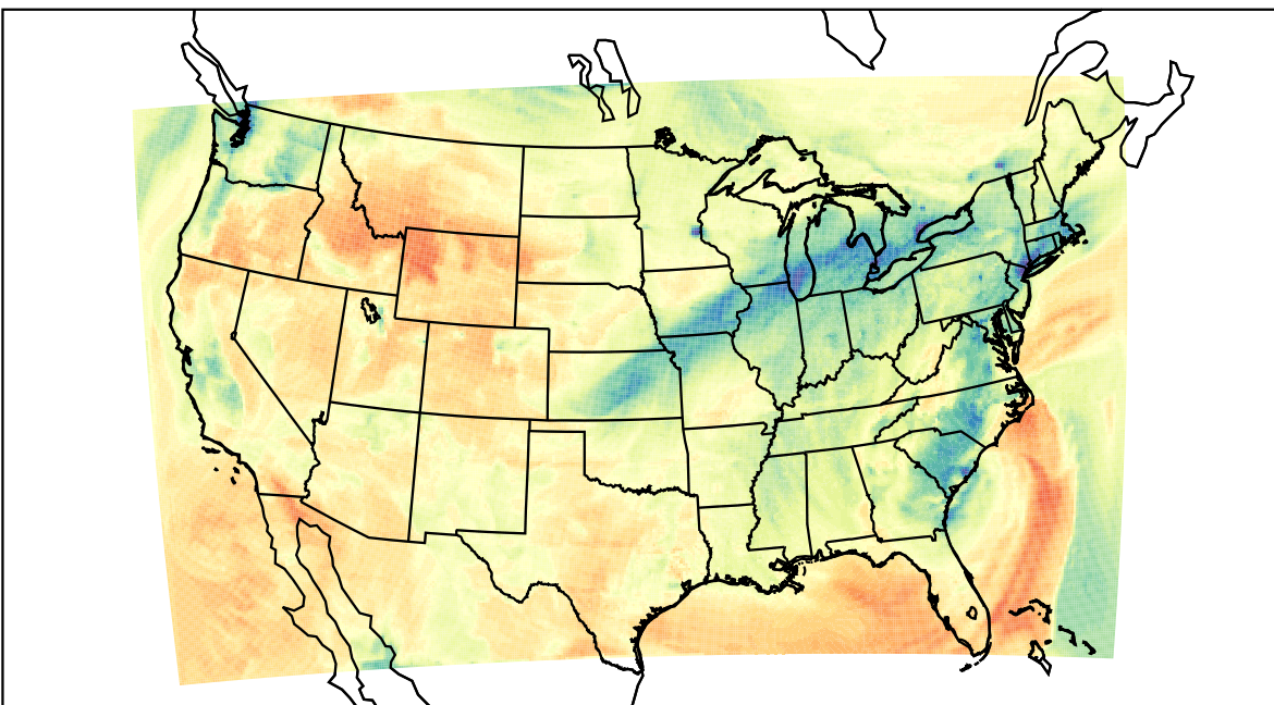
WRF (2023-02-12_21:00:00)
