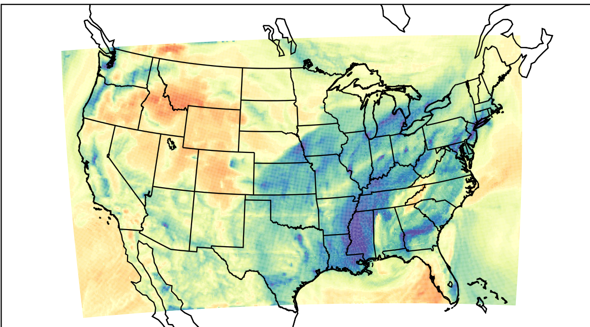
WRF (2023-02-12_09:00:00)
