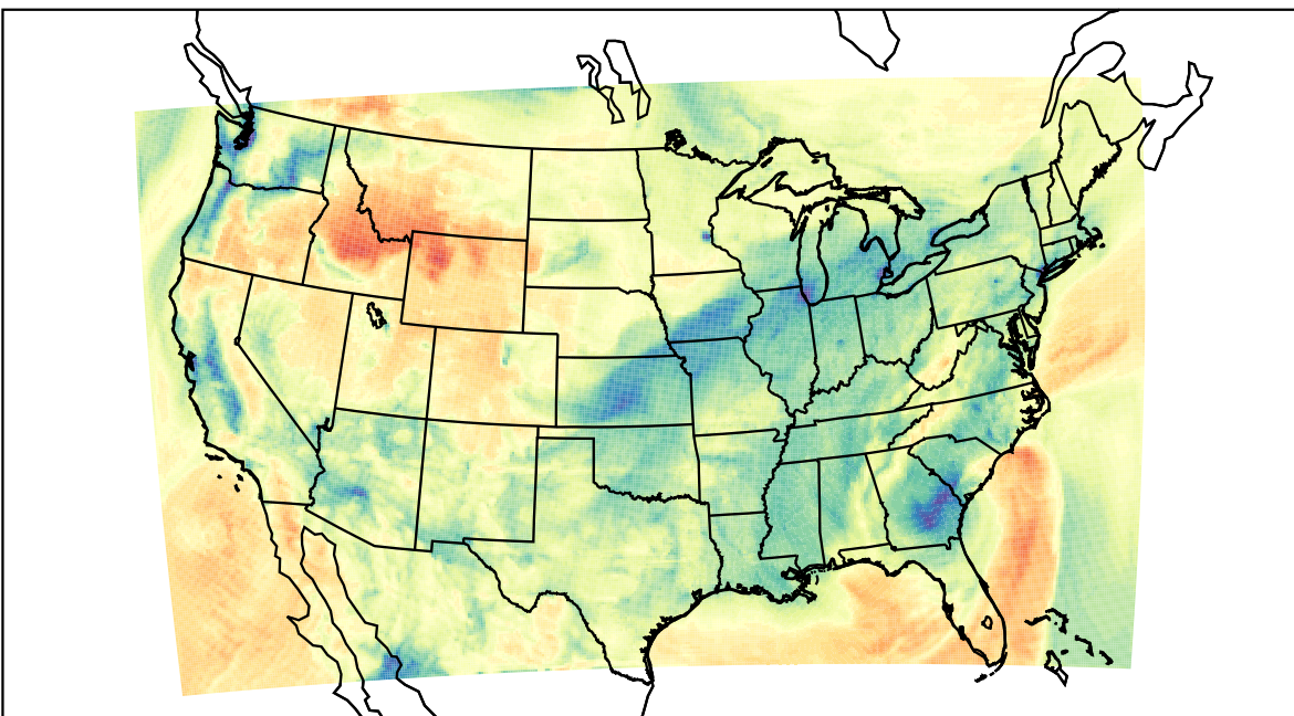
WRF (2023-02-12_17:00:00)
