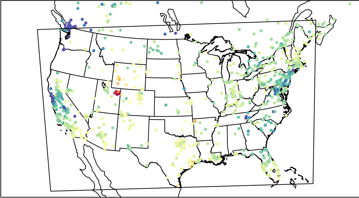
AirNOW (2023-02-12_19:00:00)
