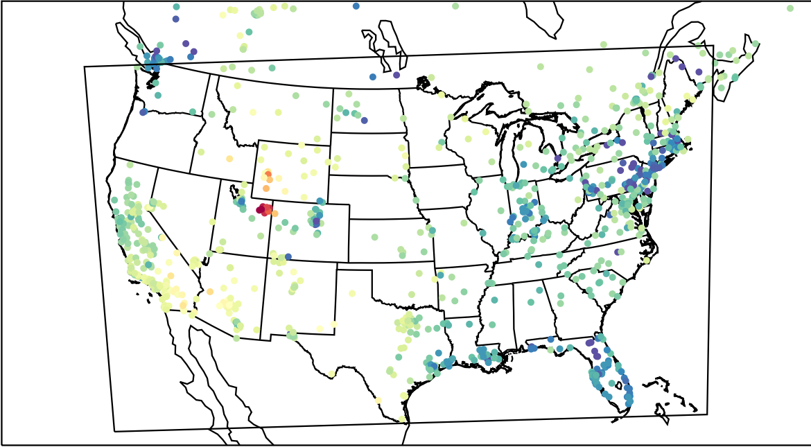
AirNOW (2023-02-11_23:00:00)
