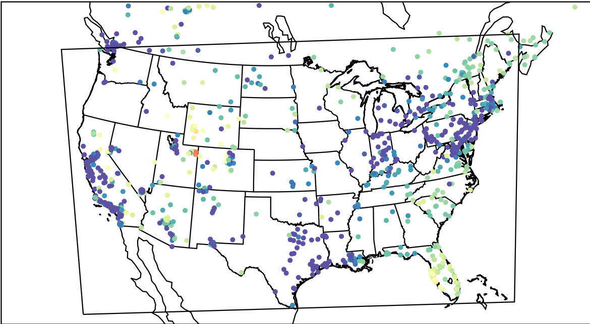
AirNOW (2023-02-12_12:00:00)
