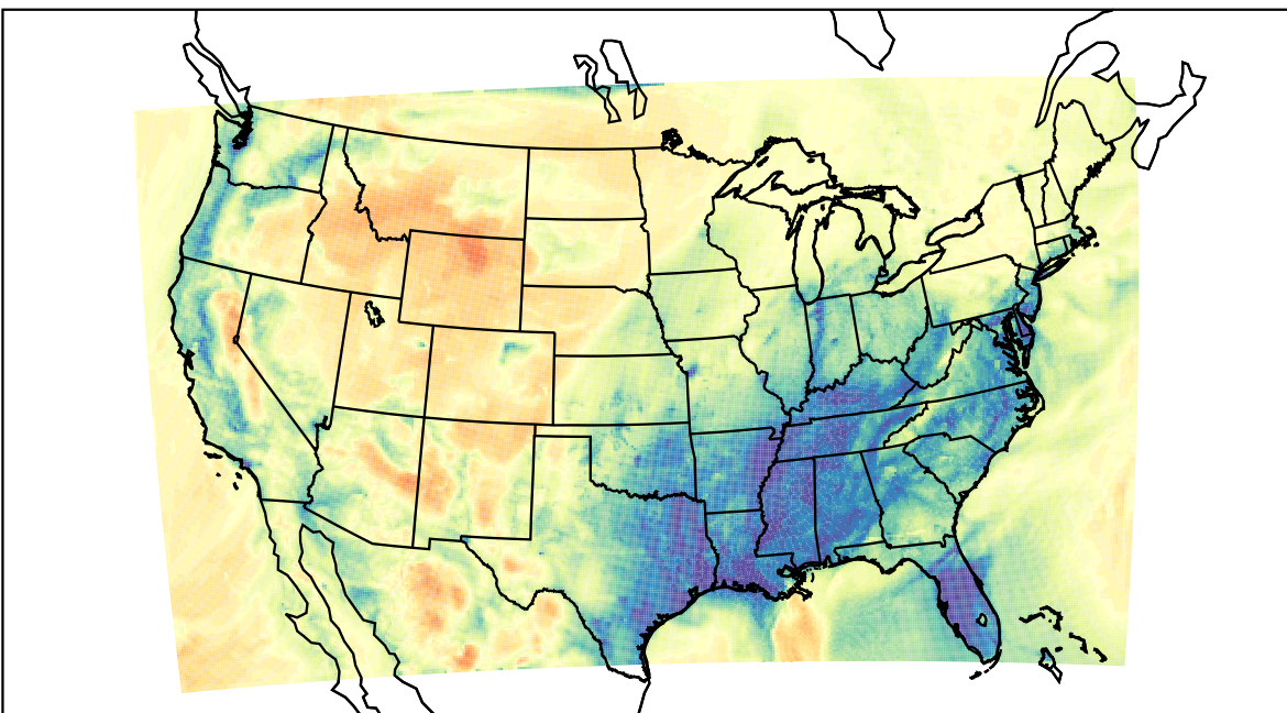
WRF (2023-02-11_12:00:00)
