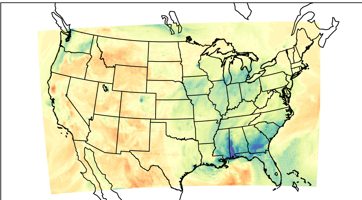
WRF (2023-02-11_21:00:00)
