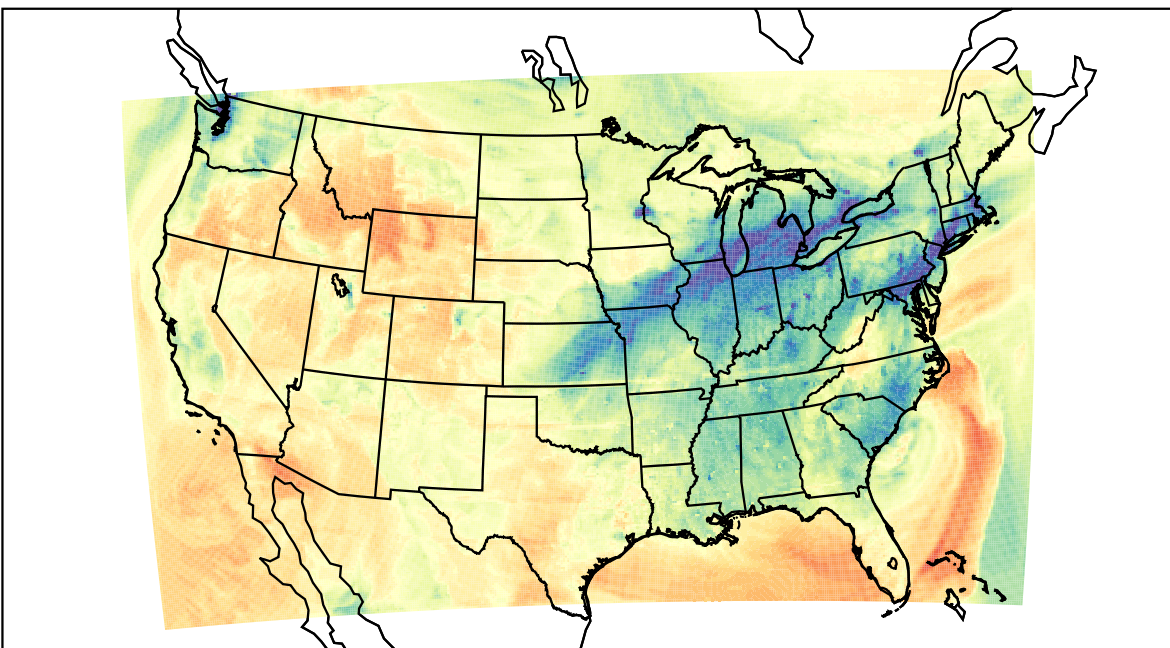
WRF (2023-02-12_23:00:00)
