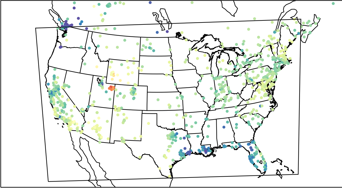
AirNOW (2023-02-11_19:00:00)
