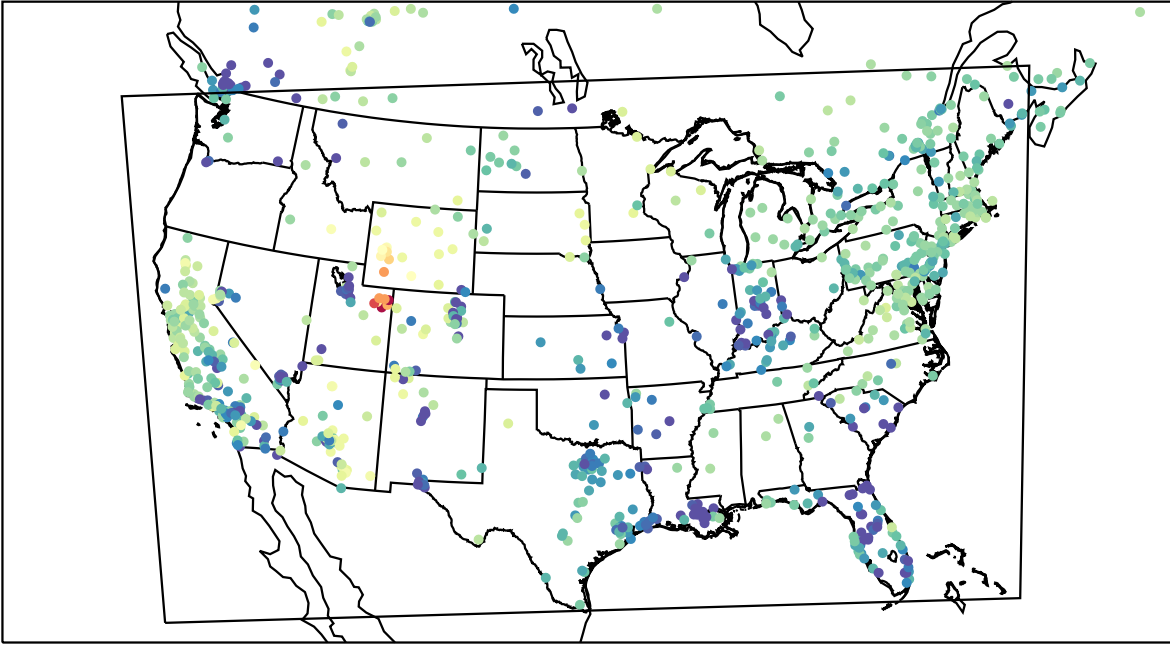
AirNOW (2023-02-11_02:00:00)
