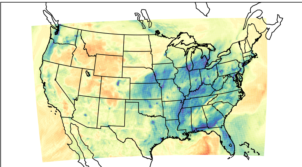
WRF (2023-02-12_02:00:00)
