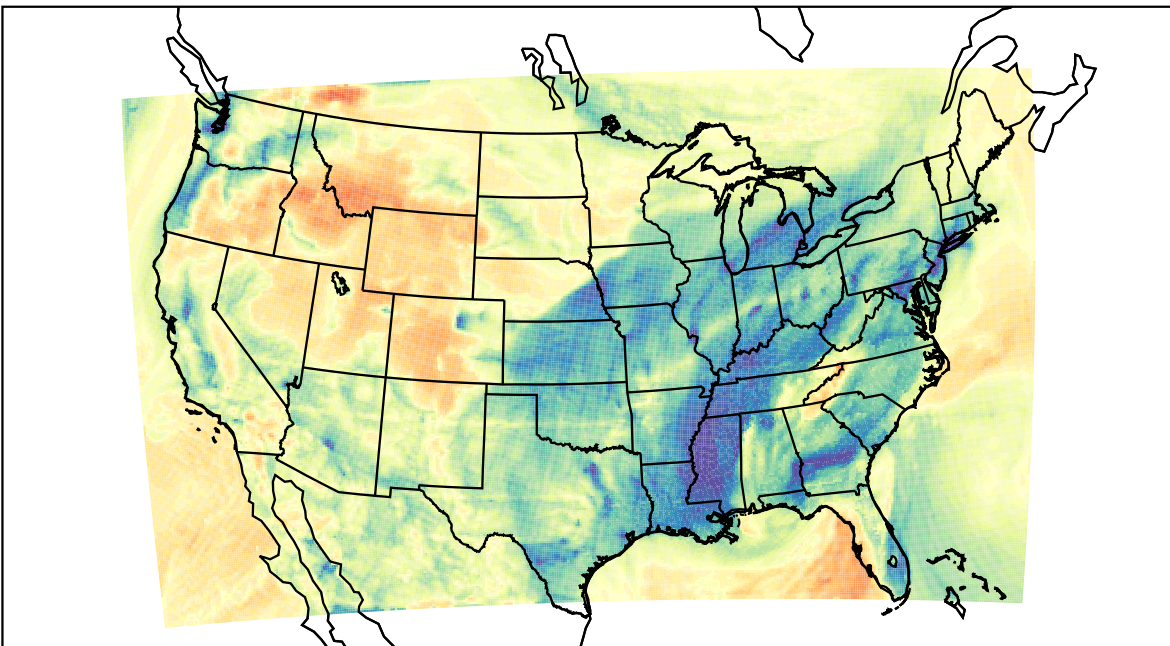
WRF (2023-02-12_08:00:00)
