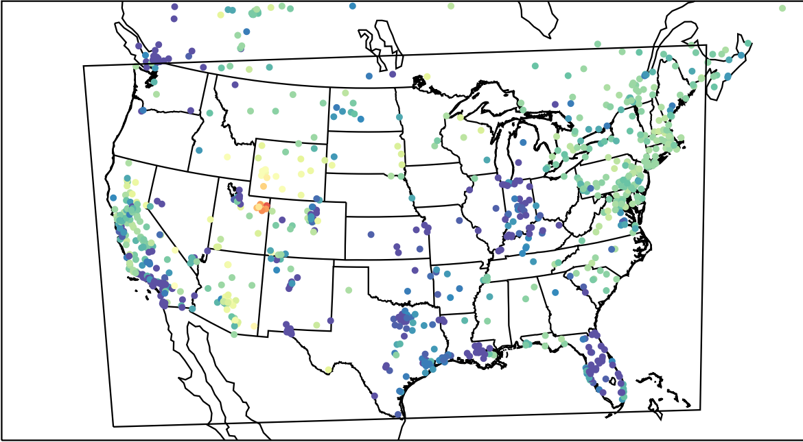
AirNOW (2023-02-11_07:00:00)
