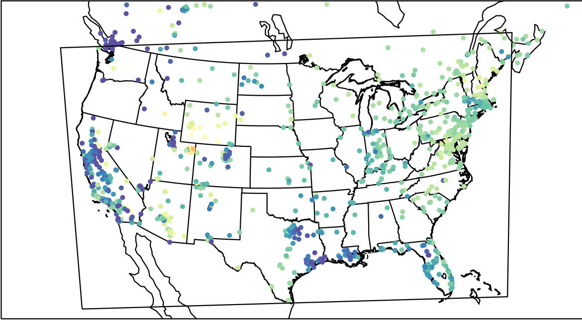
AirNOW (2023-02-11_16:00:00)
