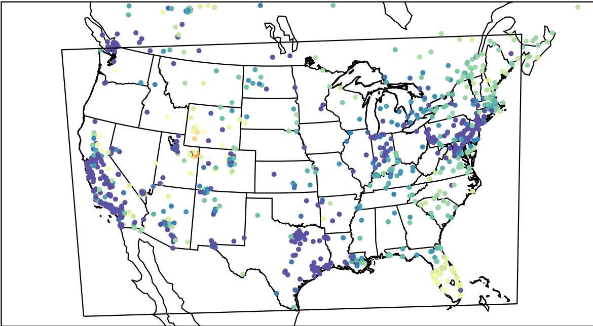
AirNOW (2023-02-12_14:00:00)
