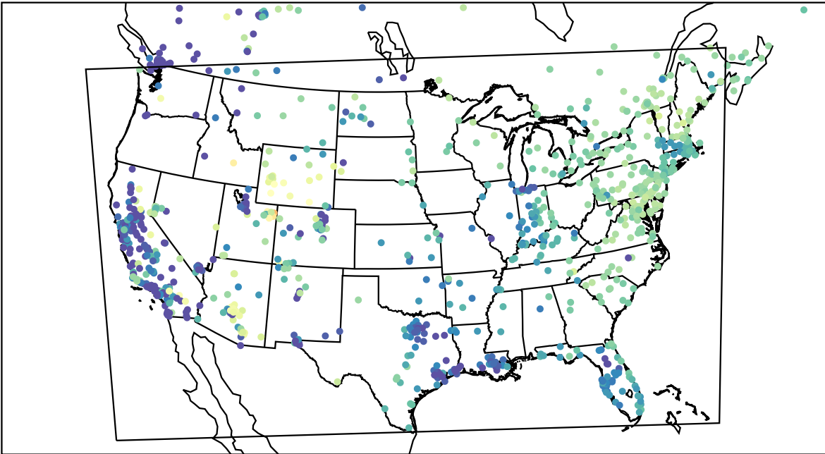
AirNOW (2023-02-11_15:00:00)
