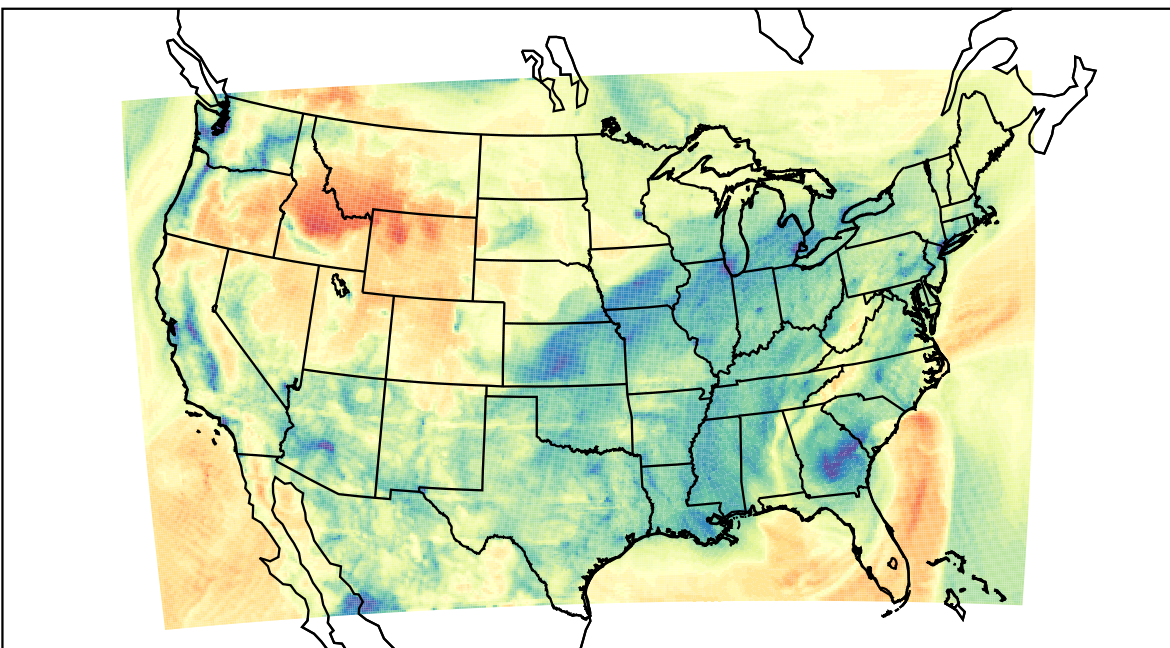
WRF (2023-02-12_16:00:00)
