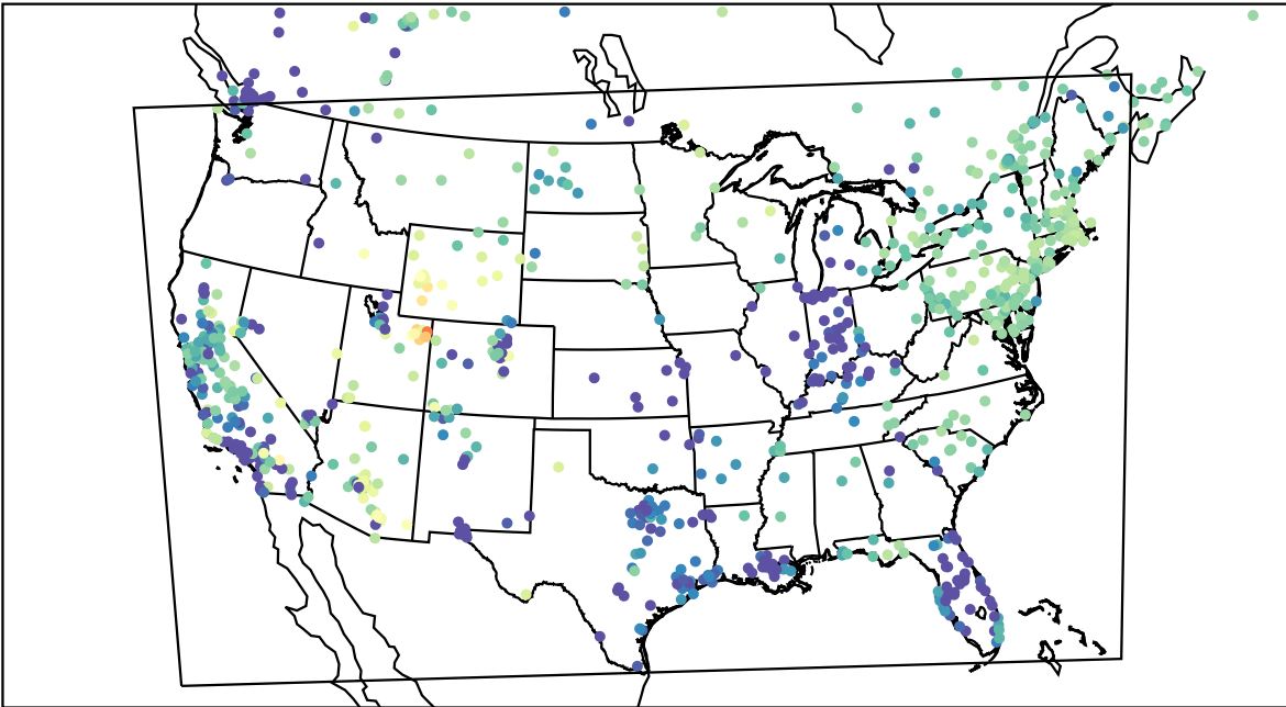
AirNOW (2023-02-11_09:00:00)
