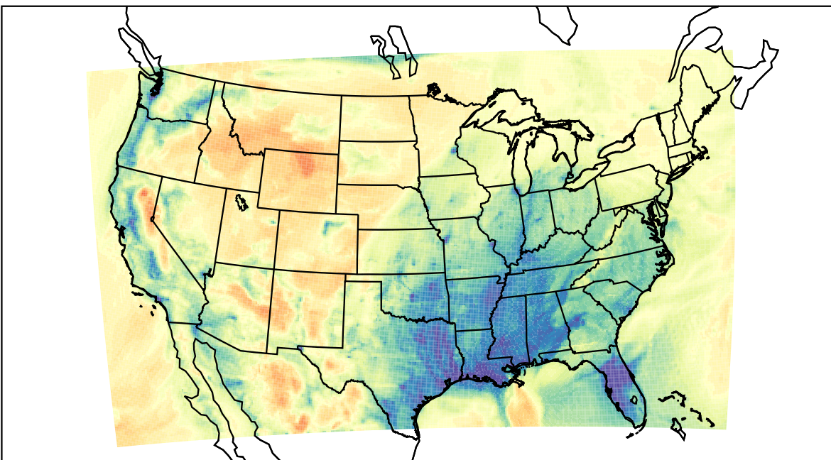
WRF (2023-02-11_14:00:00)
