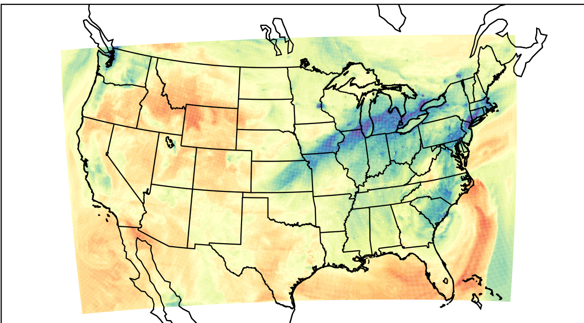
WRF (2023-02-12_22:00:00)
