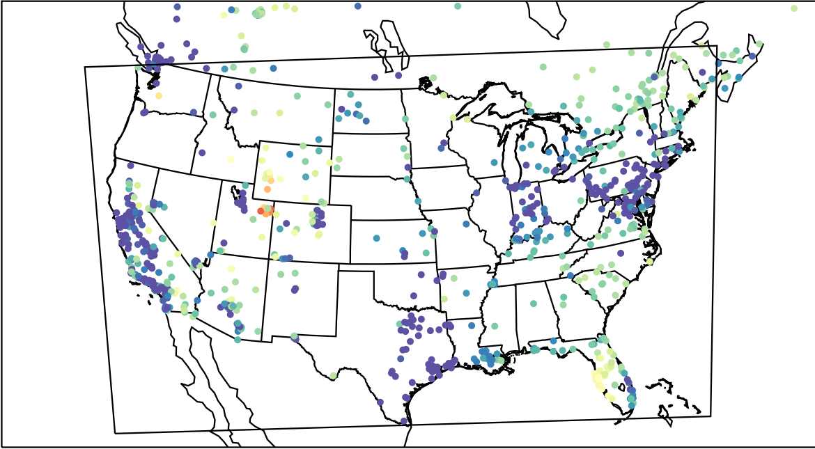
AirNOW (2023-02-12_08:00:00)
