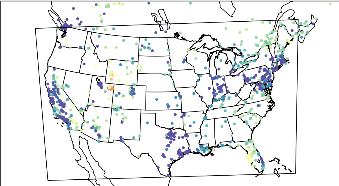
AirNOW (2023-02-12_07:00:00)
