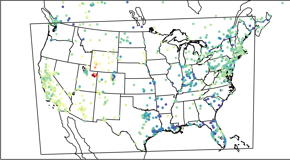
AirNOW (2023-02-11_00:00:00)
