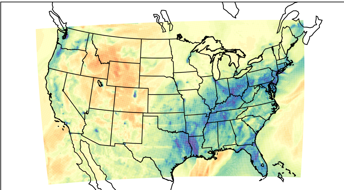
WRF (2023-02-11_02:00:00)
