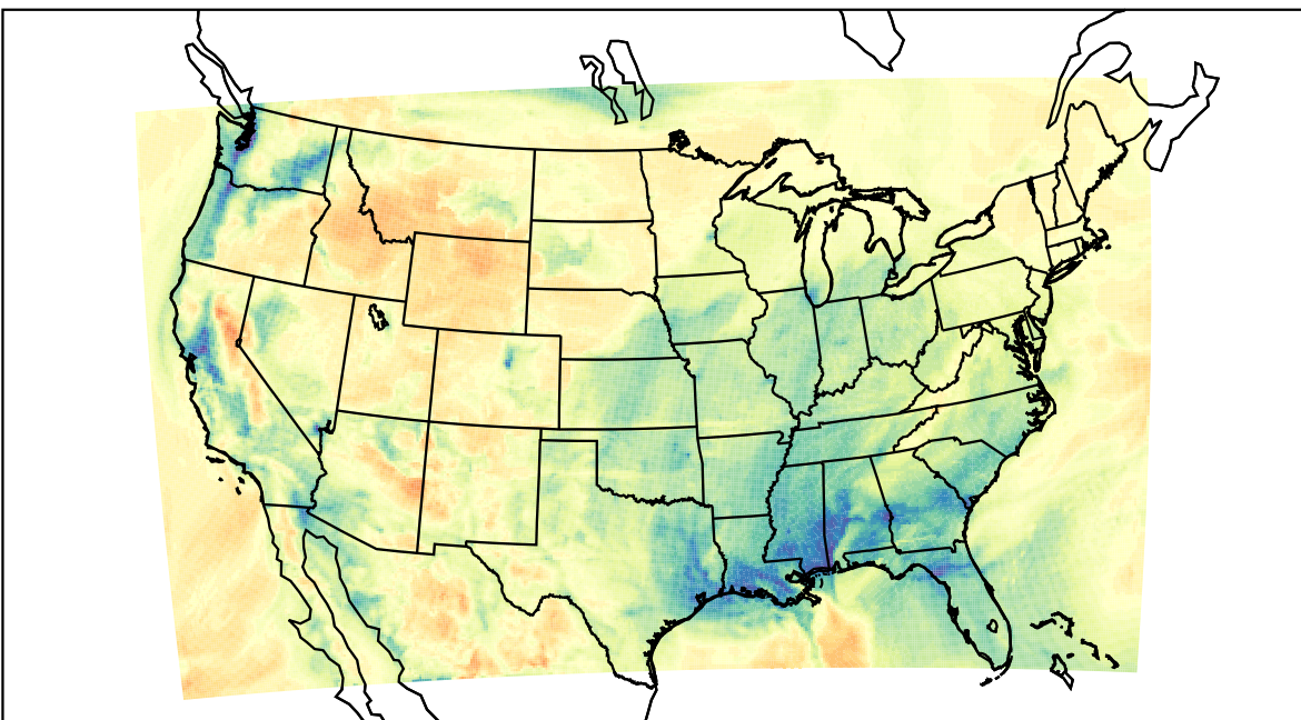
WRF (2023-02-11_17:00:00)
