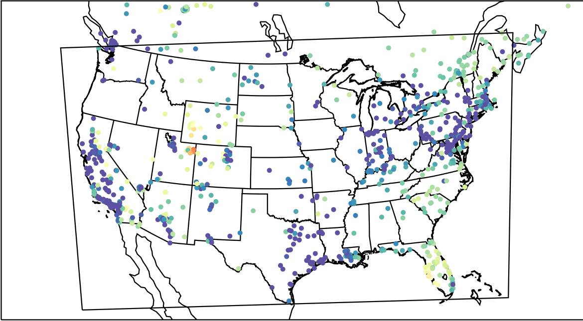
AirNOW (2023-02-12_11:00:00)
