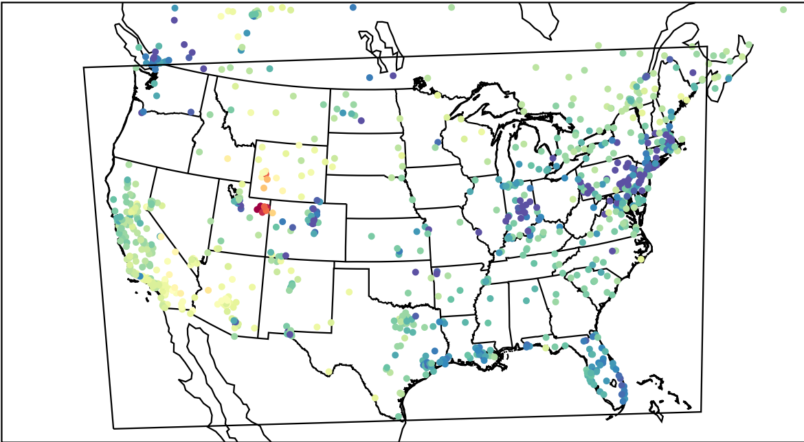
AirNOW (2023-02-12_00:00:00)
