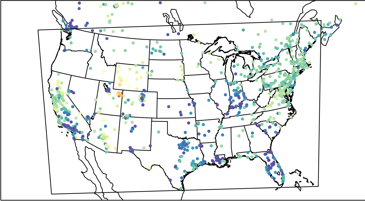
AirNOW (2023-02-11_04:00:00)
