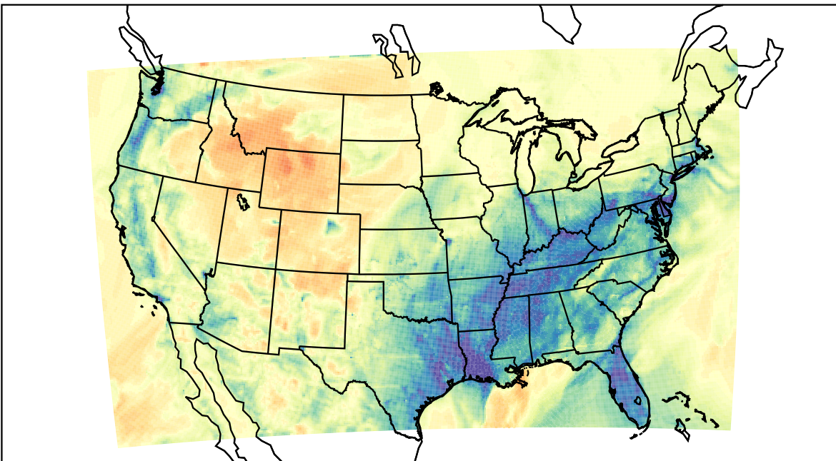
WRF (2023-02-11_07:00:00)
