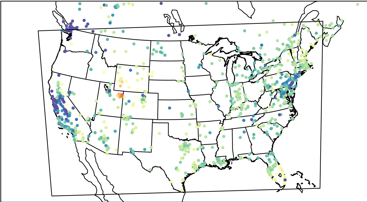
AirNOW (2023-02-12_17:00:00)
