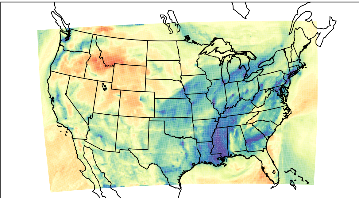
WRF (2023-02-12_11:00:00)
