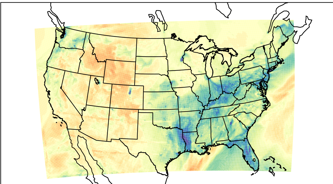
WRF (2023-02-11_00:00:00)
