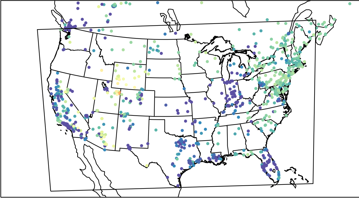
AirNOW (2023-02-11_11:00:00)
