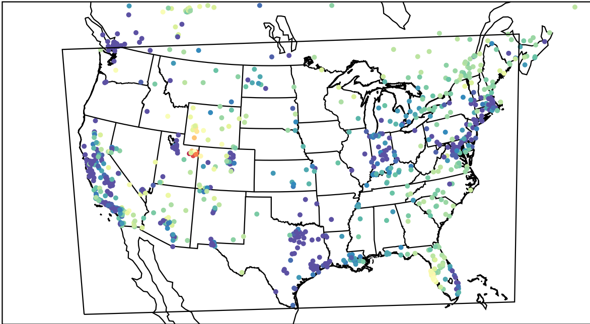
AirNOW (2023-02-12_06:00:00)
