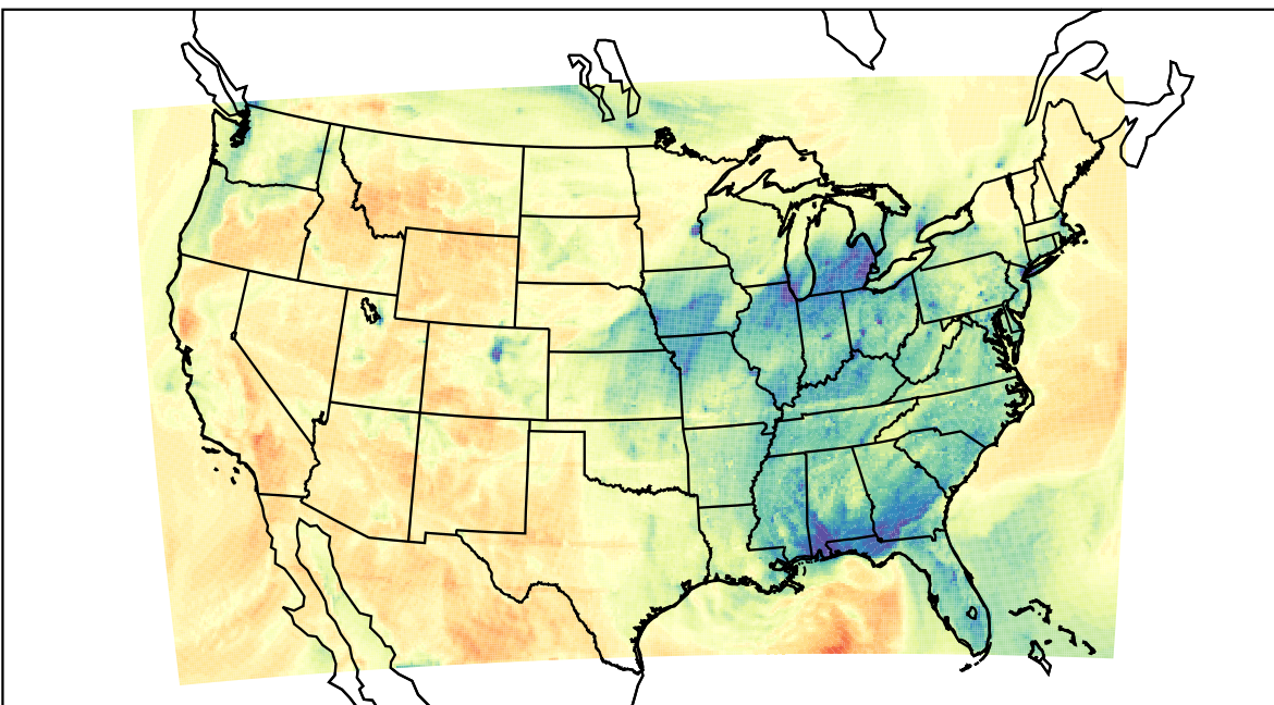
WRF (2023-02-11_23:00:00)
