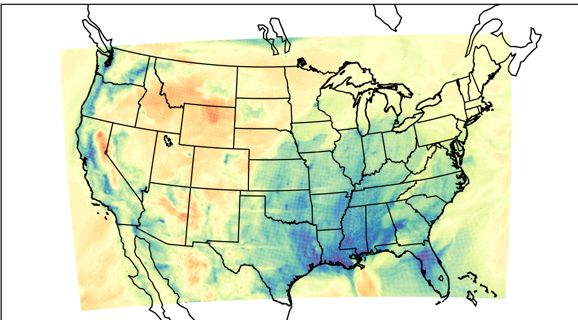
WRF (2023-02-11_15:00:00)
