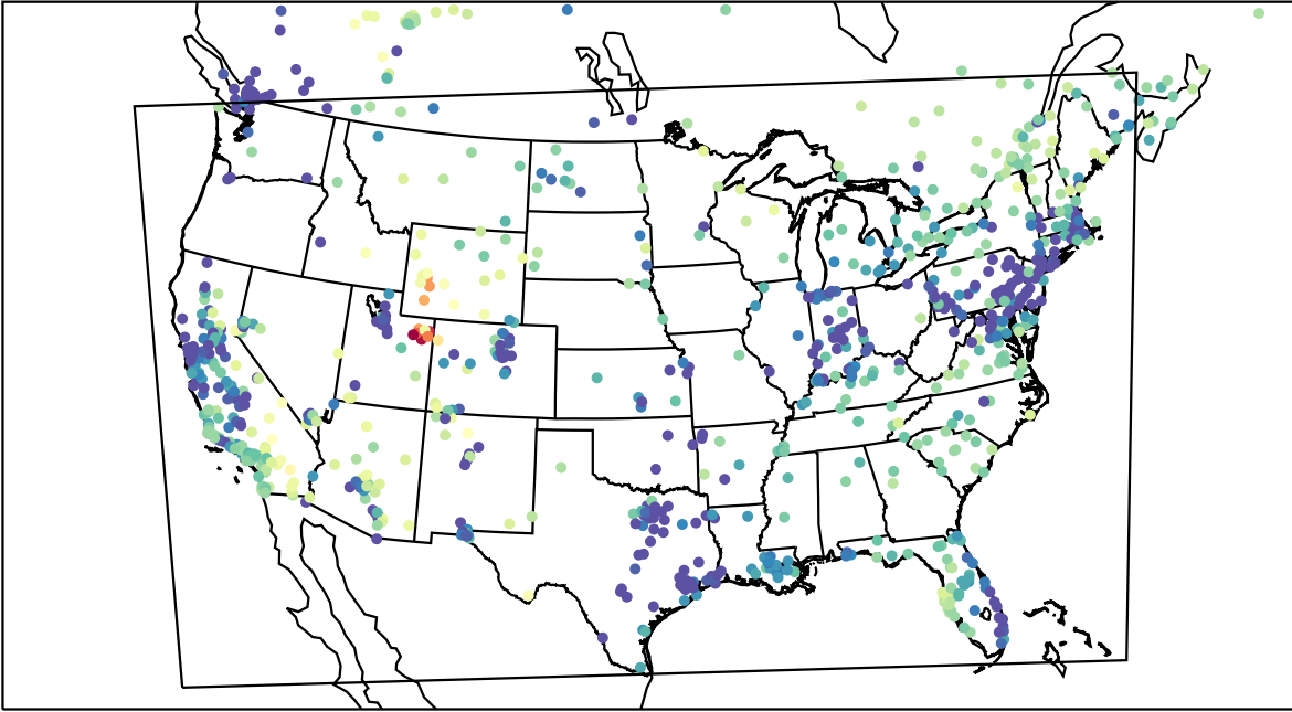
AirNOW (2023-02-12_03:00:00)
