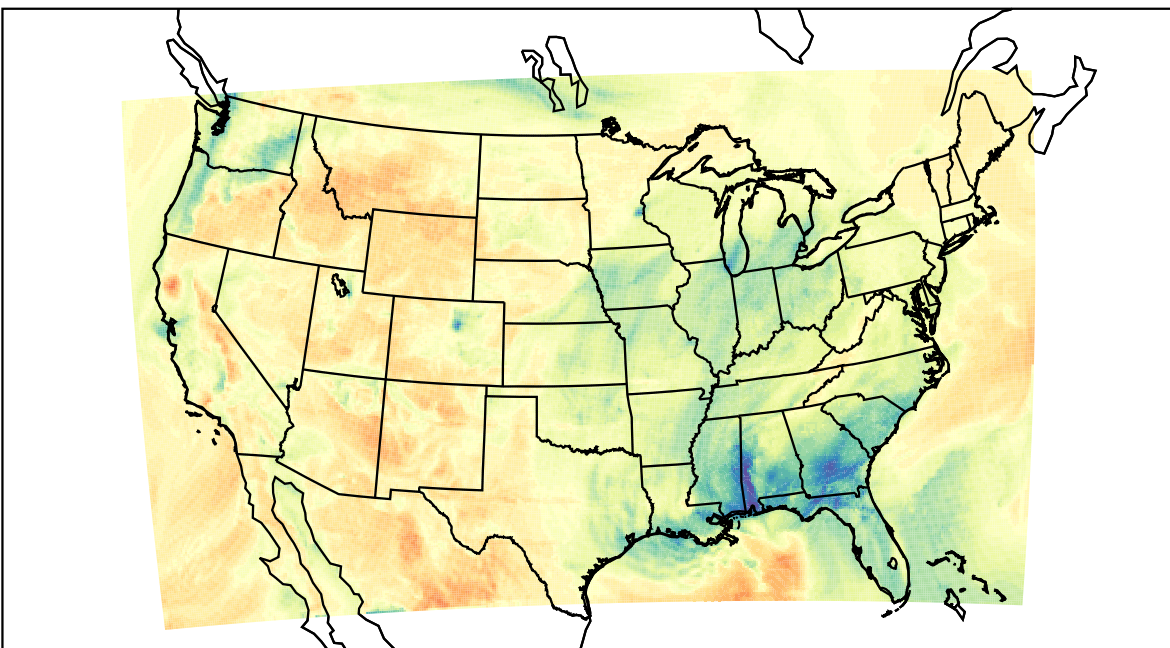
WRF (2023-02-11_20:00:00)
