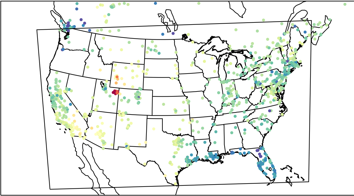
AirNOW (2023-02-11_22:00:00)
