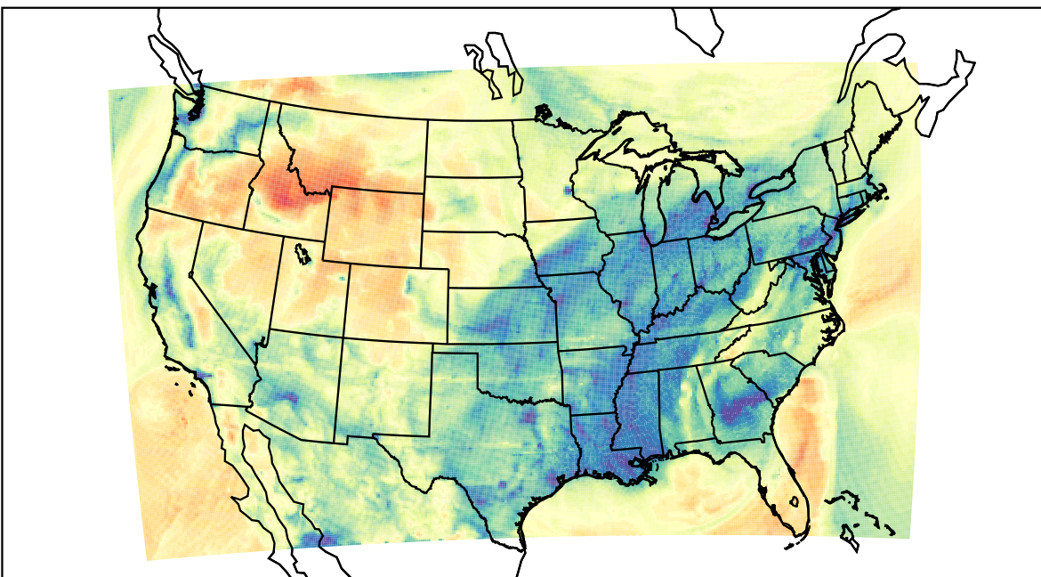
WRF (2023-02-12_14:00:00)
