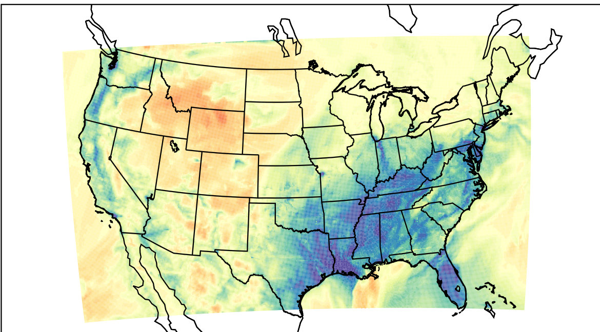
WRF (2023-02-11_09:00:00)
