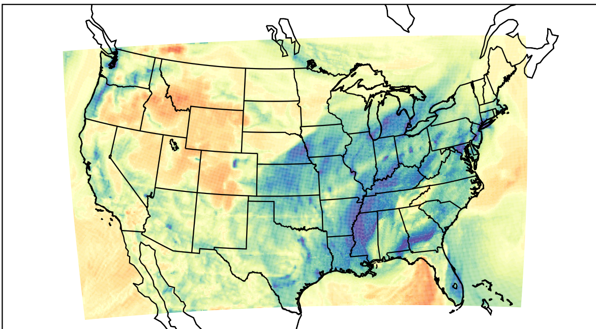
WRF (2023-02-12_06:00:00)
