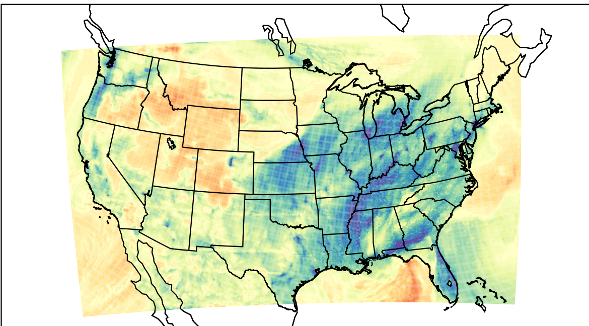
WRF (2023-02-12_04:00:00)
