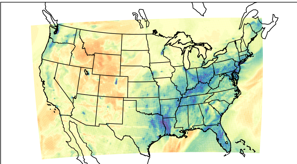
WRF (2023-02-11_01:00:00)
