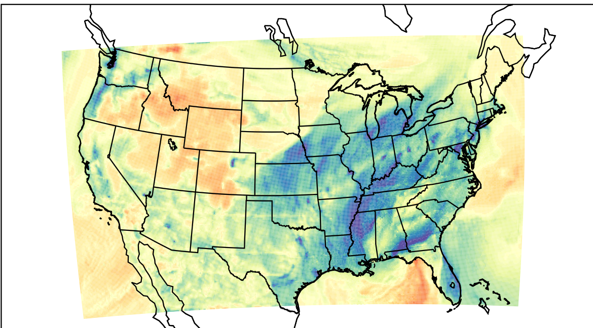
WRF (2023-02-12_05:00:00)
