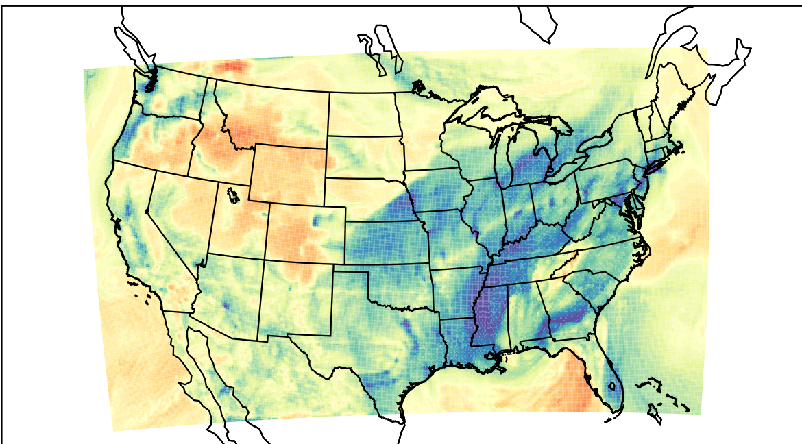
WRF (2023-02-12_07:00:00)
