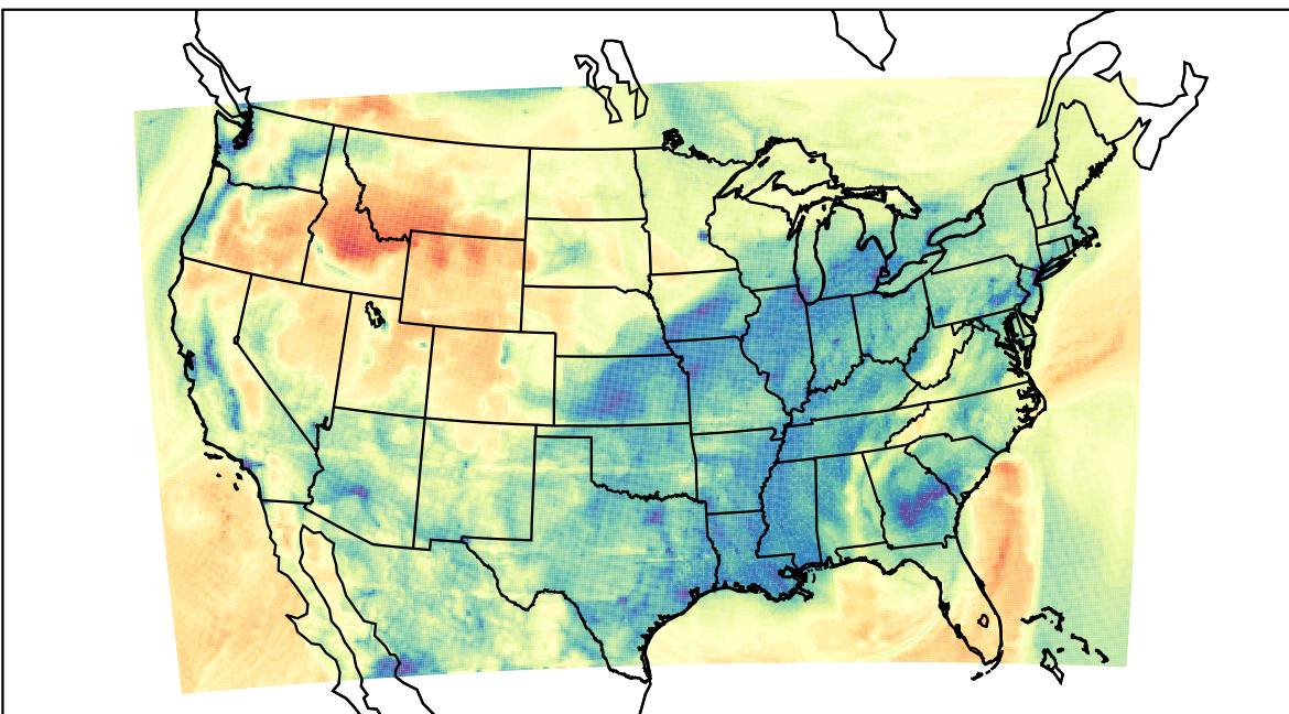
WRF (2023-02-12_15:00:00)
