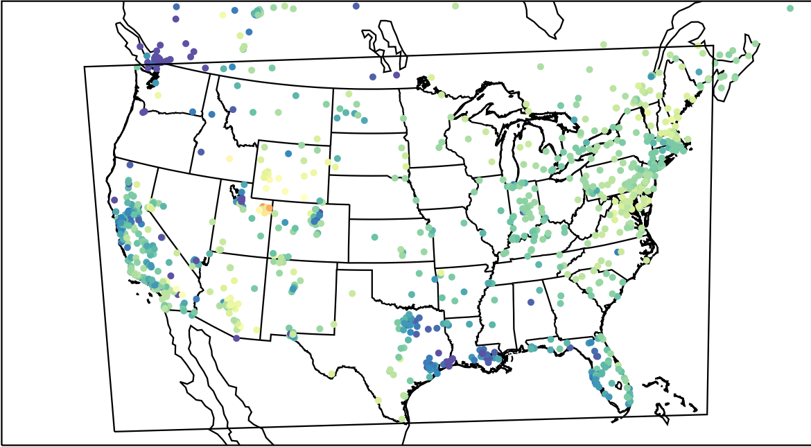
AirNOW (2023-02-11_17:00:00)
