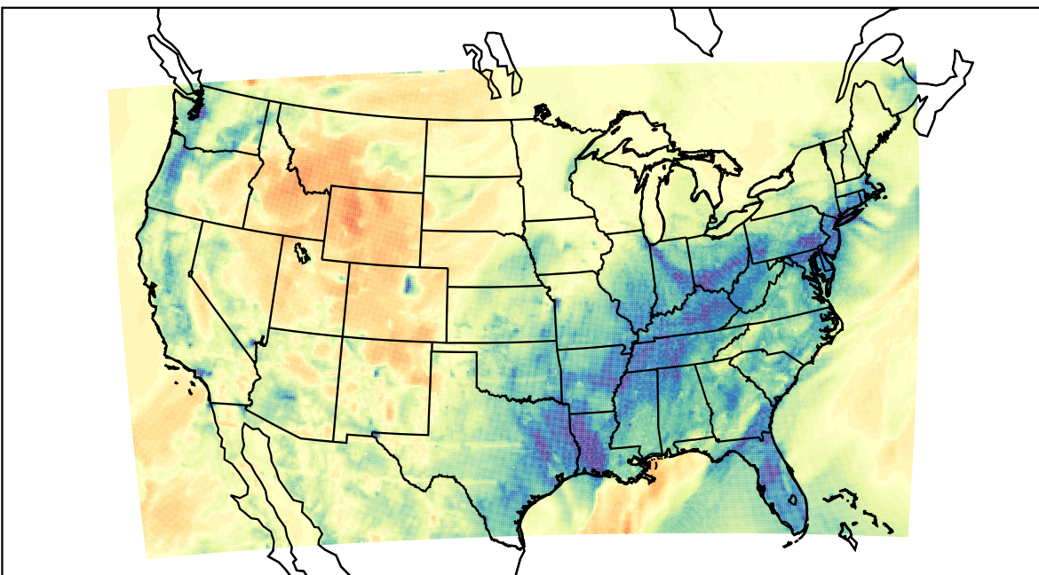
WRF (2023-02-11_04:00:00)
