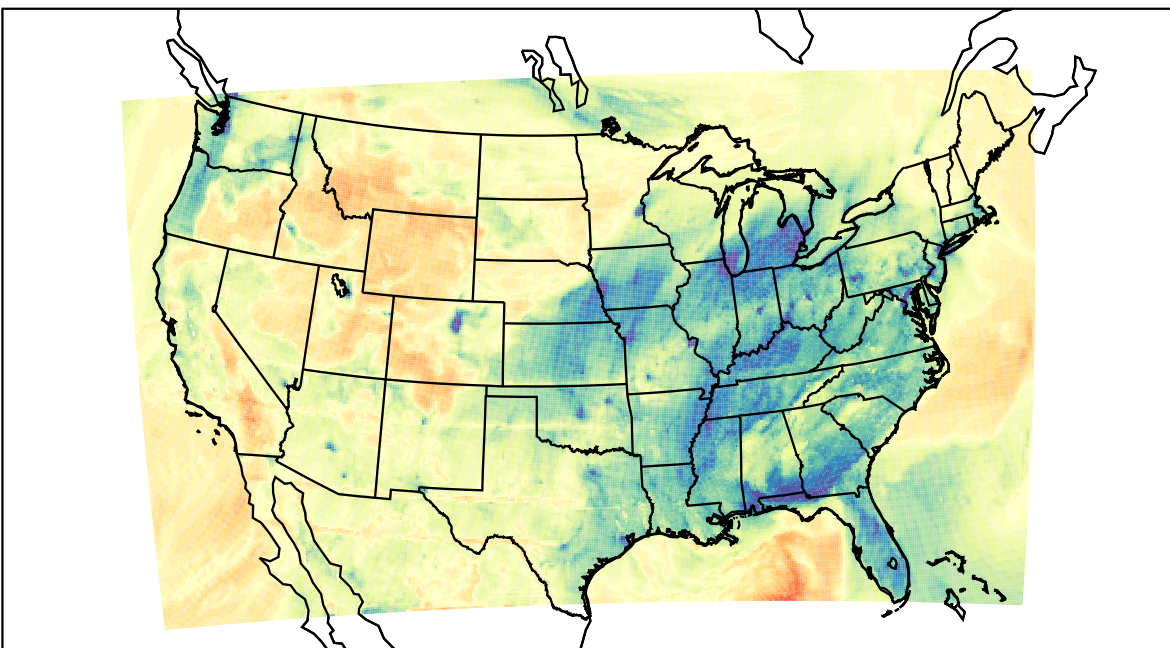
WRF (2023-02-12_01:00:00)
