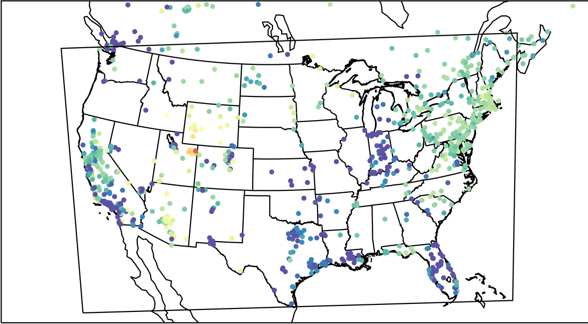
AirNOW (2023-02-11_08:00:00)
