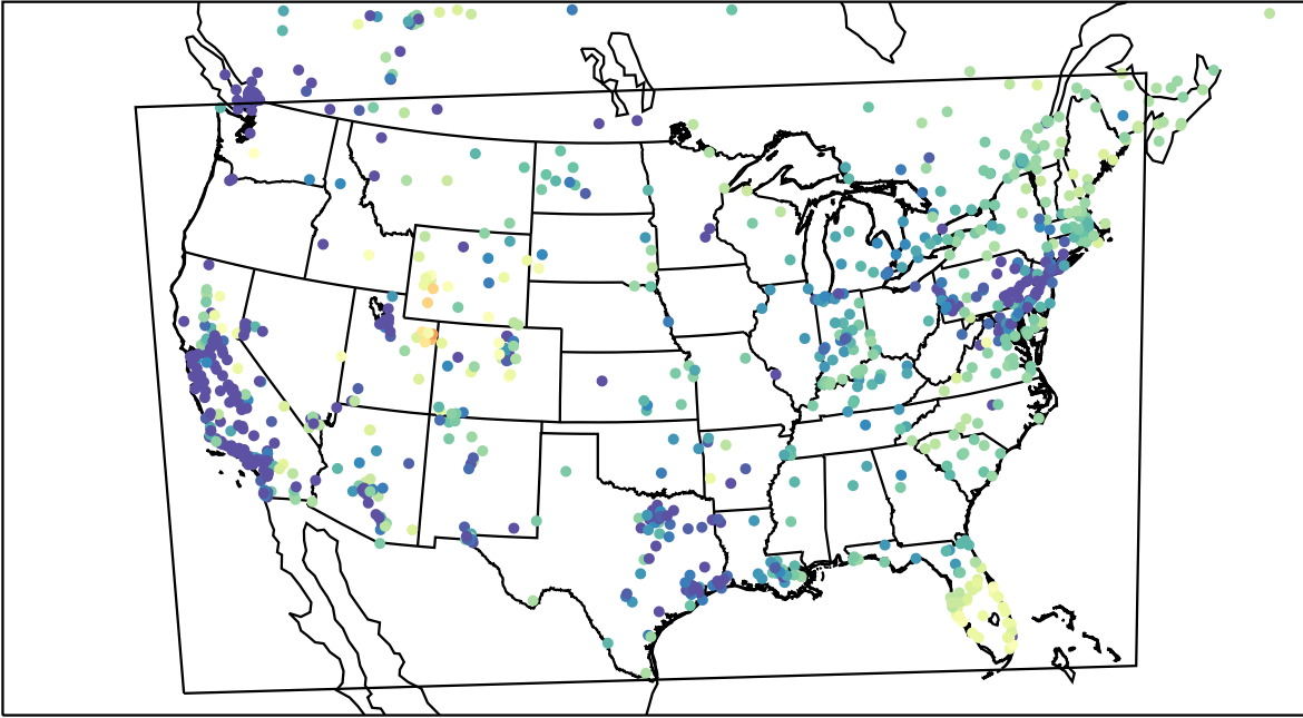
AirNOW (2023-02-12_15:00:00)
