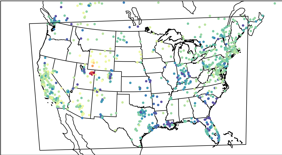
AirNOW (2023-02-11_01:00:00)
