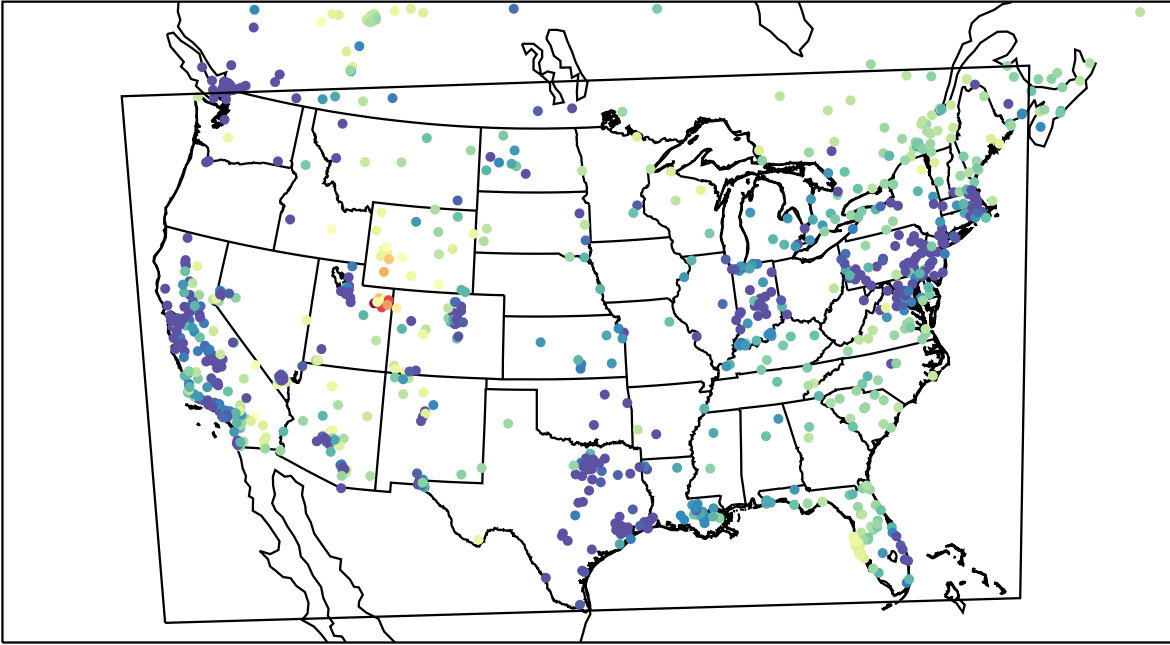
AirNOW (2023-02-12_05:00:00)
