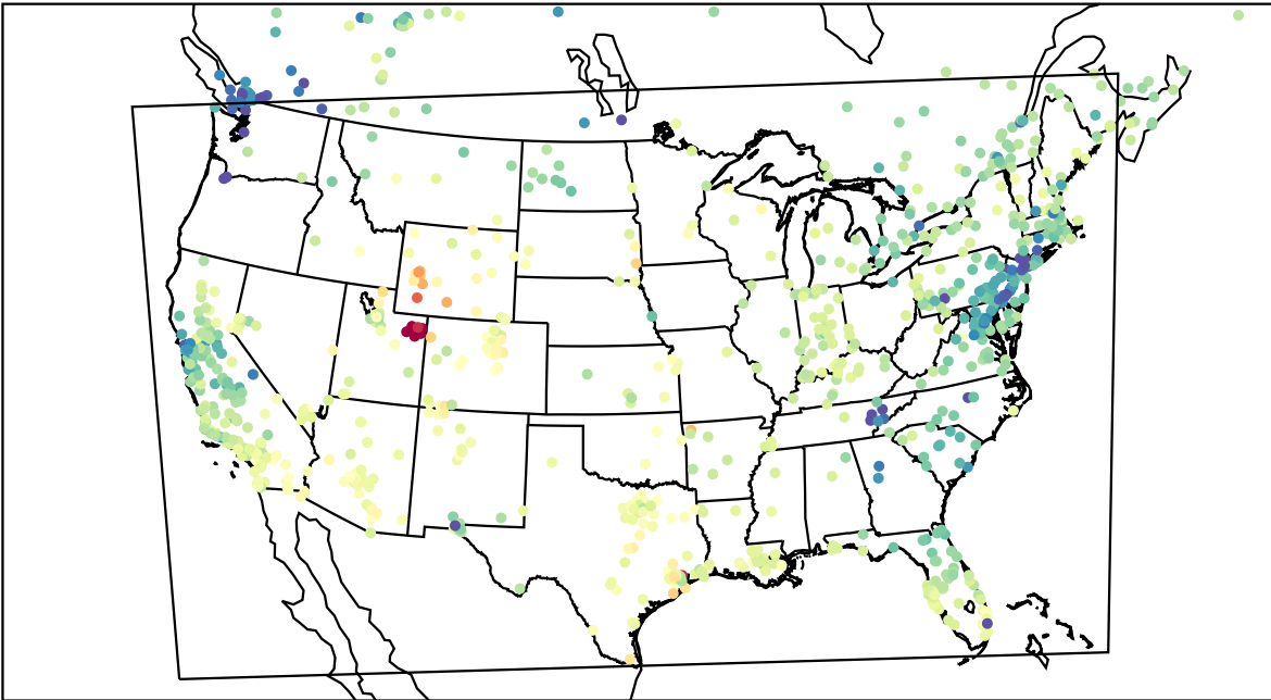
AirNOW (2023-02-12_21:00:00)
