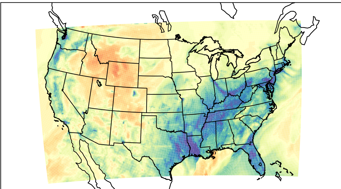
WRF (2023-02-11_05:00:00)
