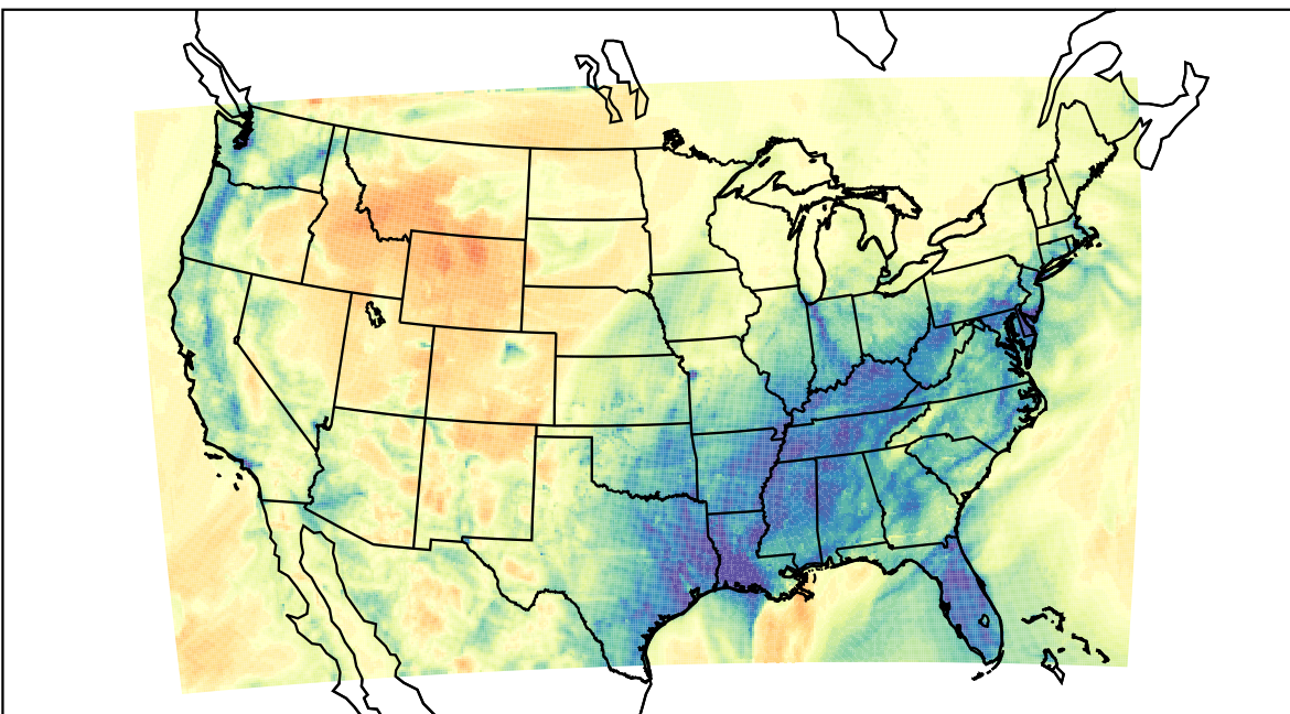
WRF (2023-02-11_08:00:00)
