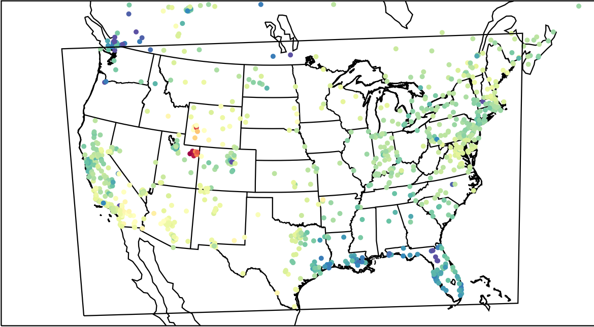
AirNOW (2023-02-11_21:00:00)
