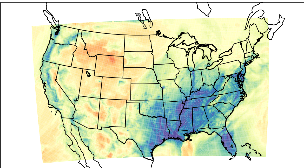
WRF (2023-02-11_11:00:00)
