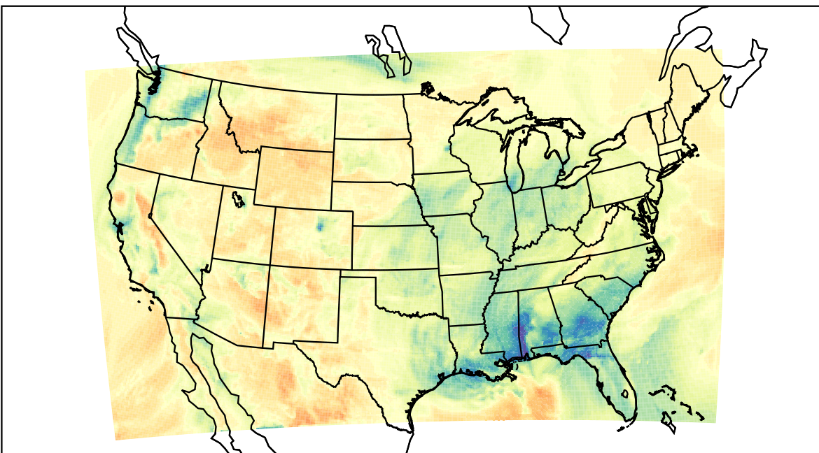
WRF (2023-02-11_19:00:00)
