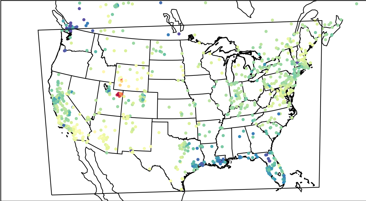
AirNOW (2023-02-11_20:00:00)
