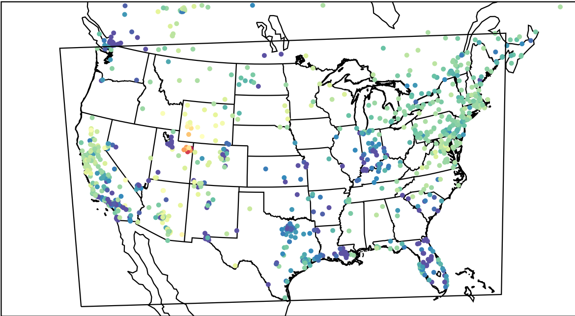
AirNOW (2023-02-11_03:00:00)
