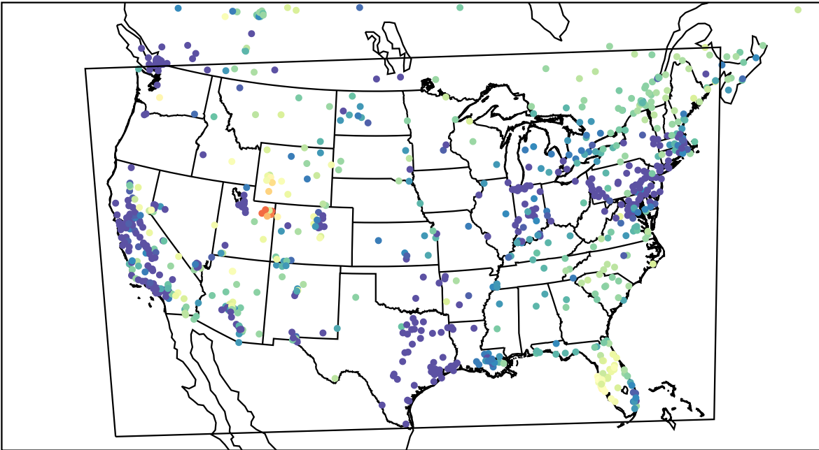
AirNOW (2023-02-12_09:00:00)
