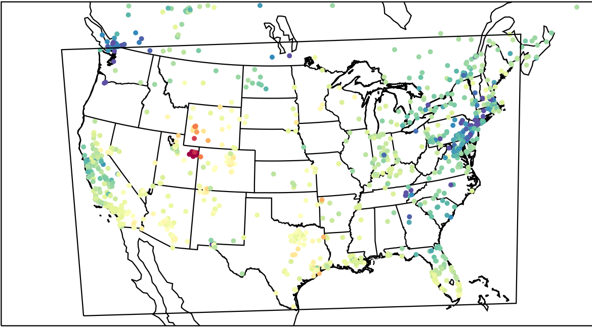
AirNOW (2023-02-12_22:00:00)
