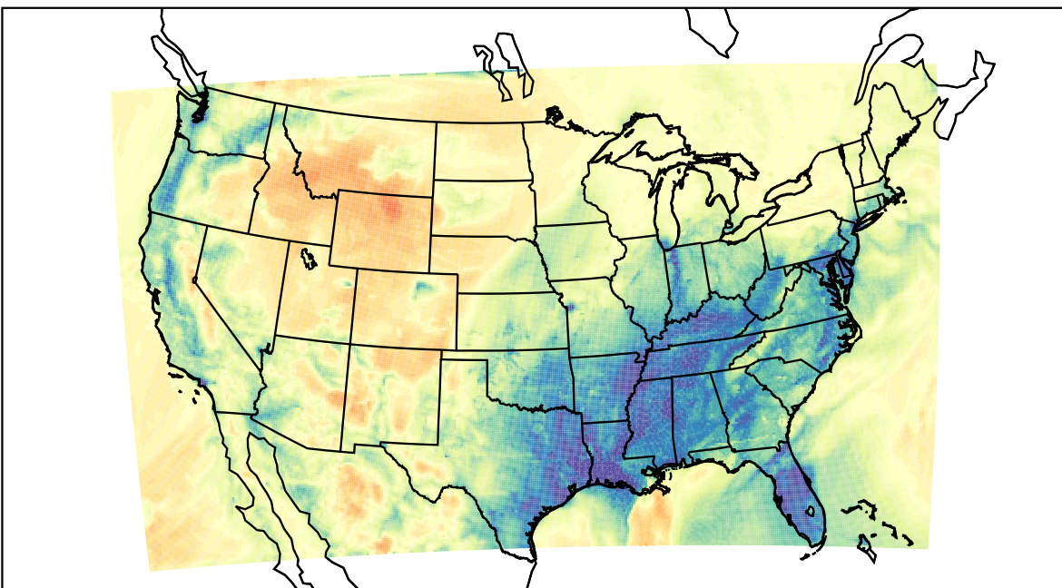
WRF (2023-02-11_10:00:00)
