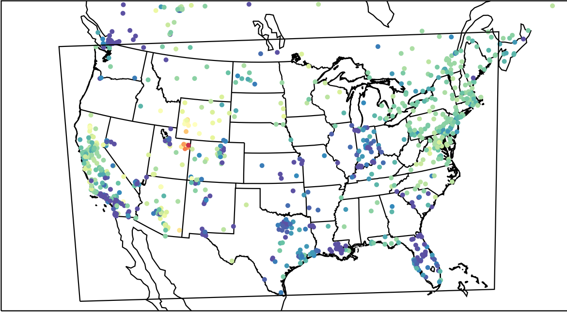
AirNOW (2023-02-11_05:00:00)
