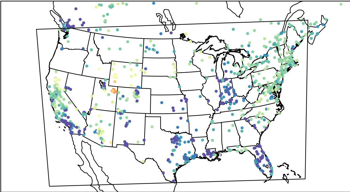
AirNOW (2023-02-11_06:00:00)
