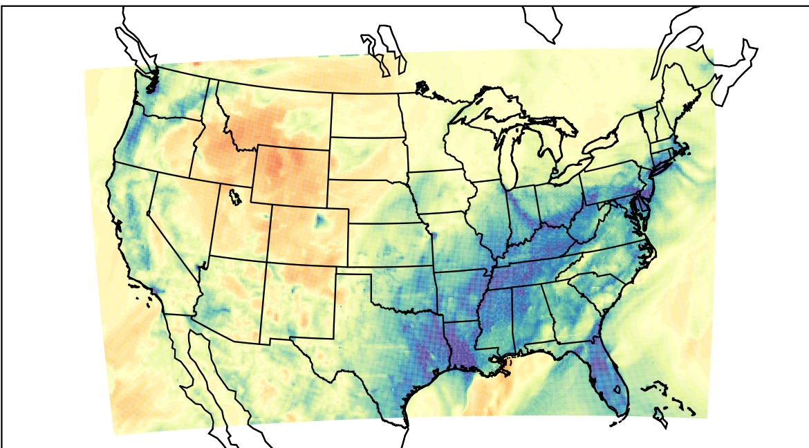
WRF (2023-02-11_06:00:00)
