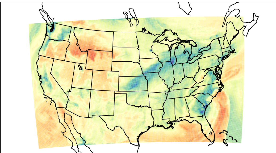
WRF (2023-02-12_19:00:00)
