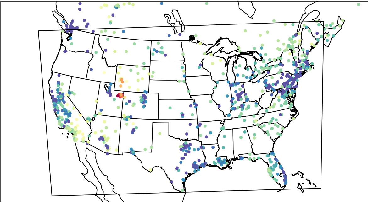
AirNOW (2023-02-12_02:00:00)
