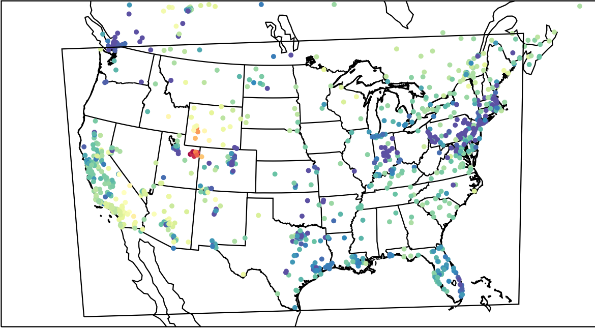
AirNOW (2023-02-12_01:00:00)
