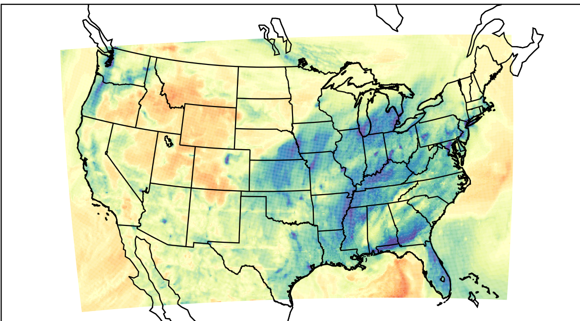
WRF (2023-02-12_03:00:00)
