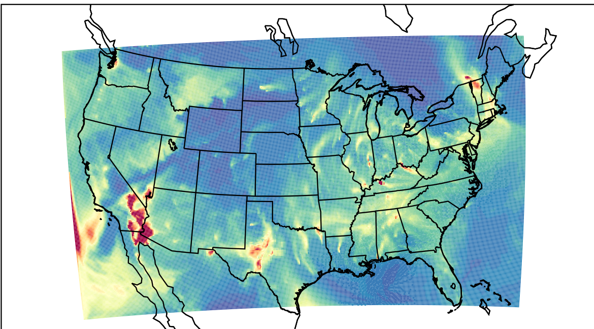
WRF 2023-02-14_07:00:00
