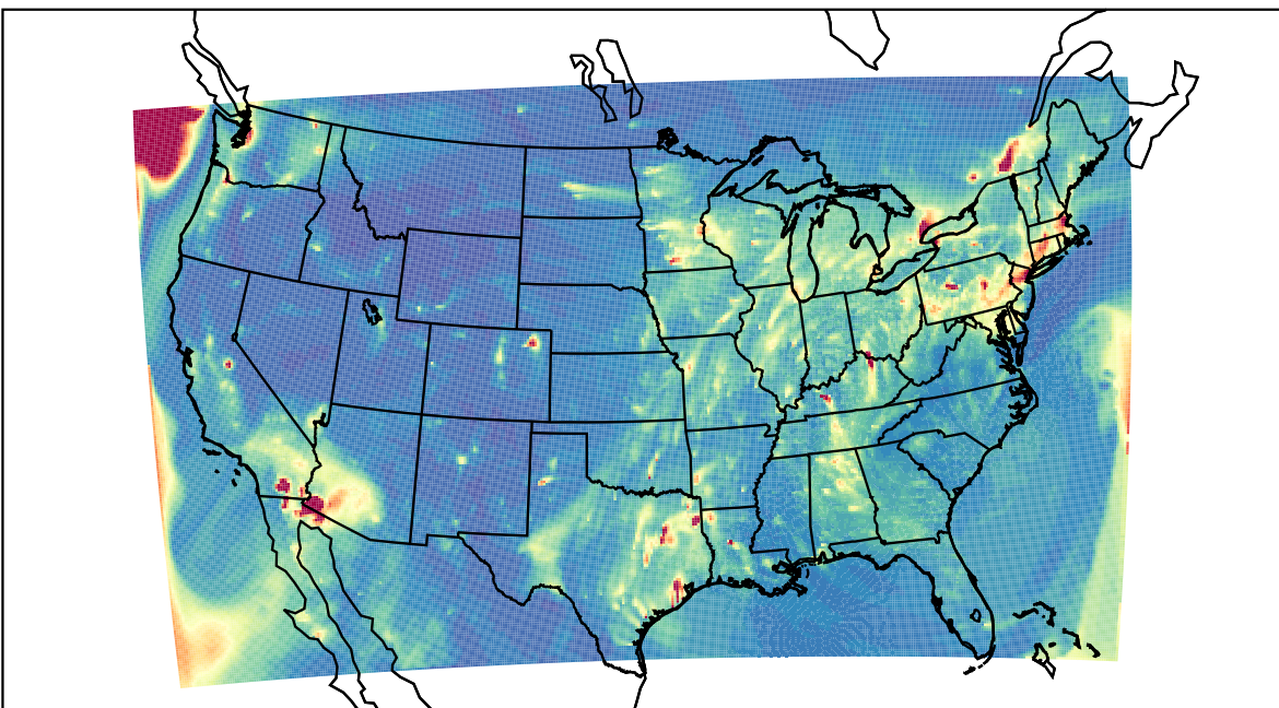
WRF 2023-02-13_02:00:00
