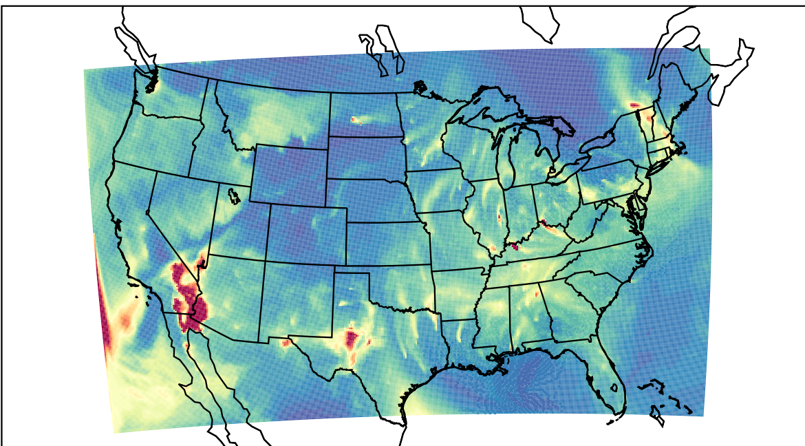
WRF 2023-02-14_08:00:00
