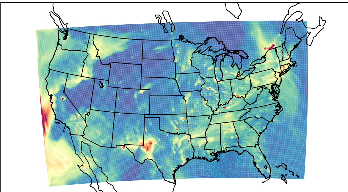
WRF 2023-02-14_01:00:00
