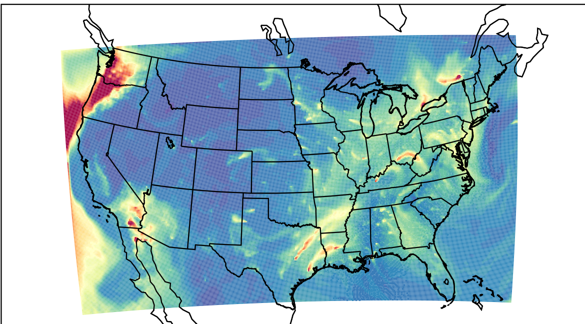
WRF 2023-02-13_14:00:00
