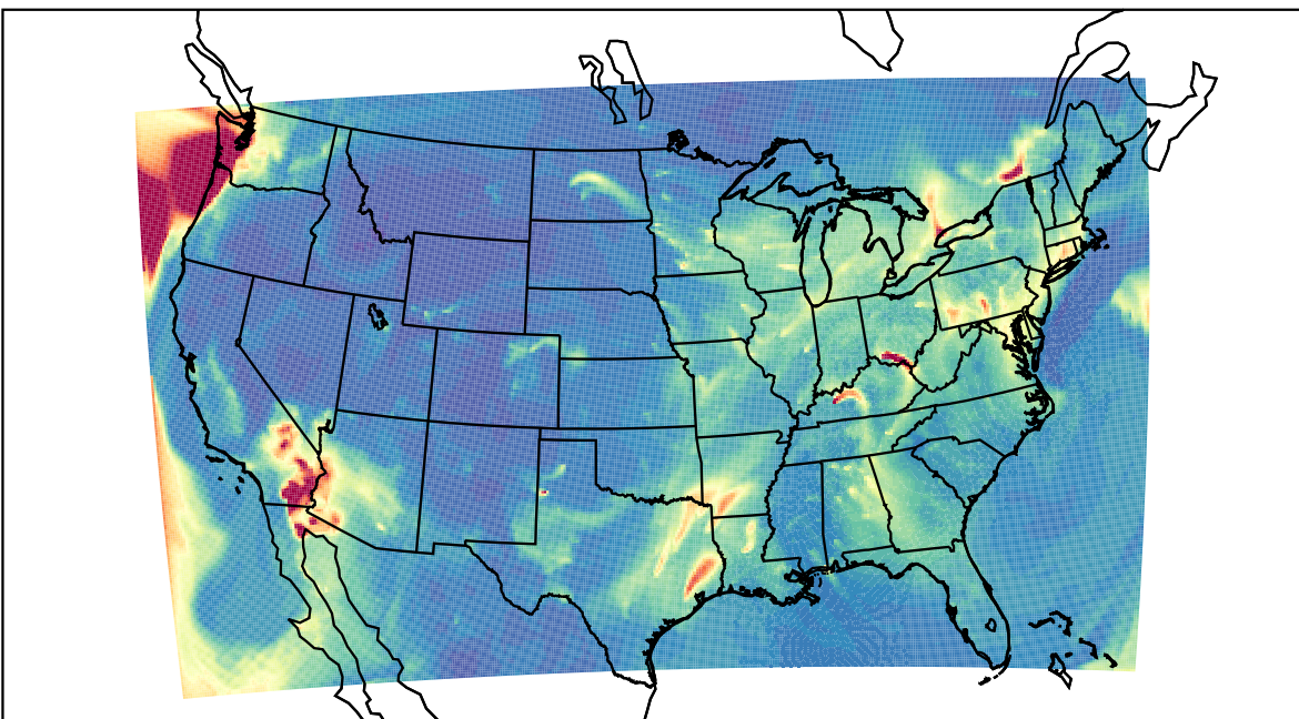
WRF 2023-02-13_09:00:00
