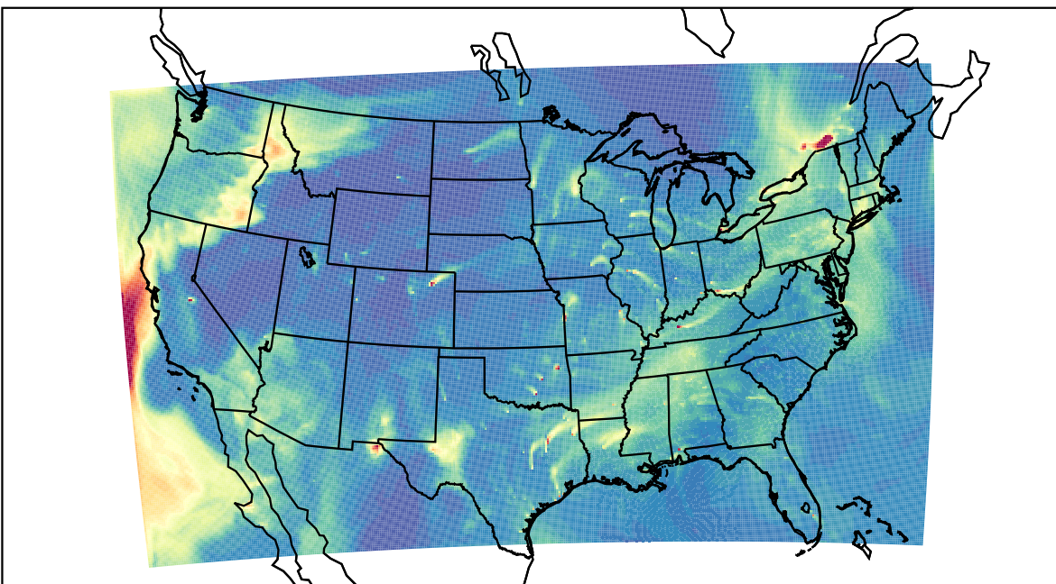
WRF 2023-02-13_22:00:00
