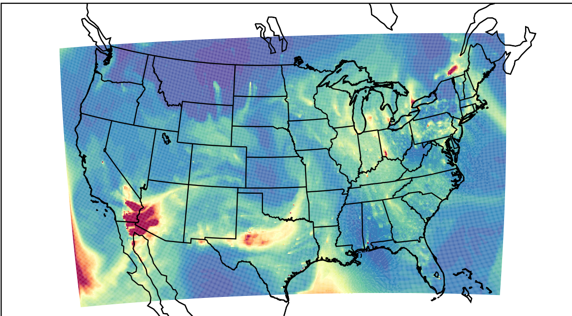
WRF 2023-02-14_23:00:00
