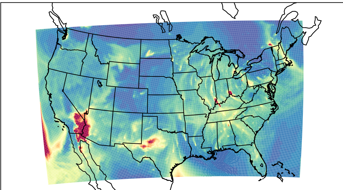
WRF 2023-02-14_12:00:00
