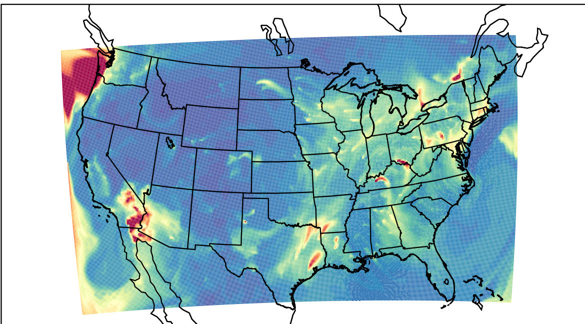
WRF 2023-02-13_08:00:00
