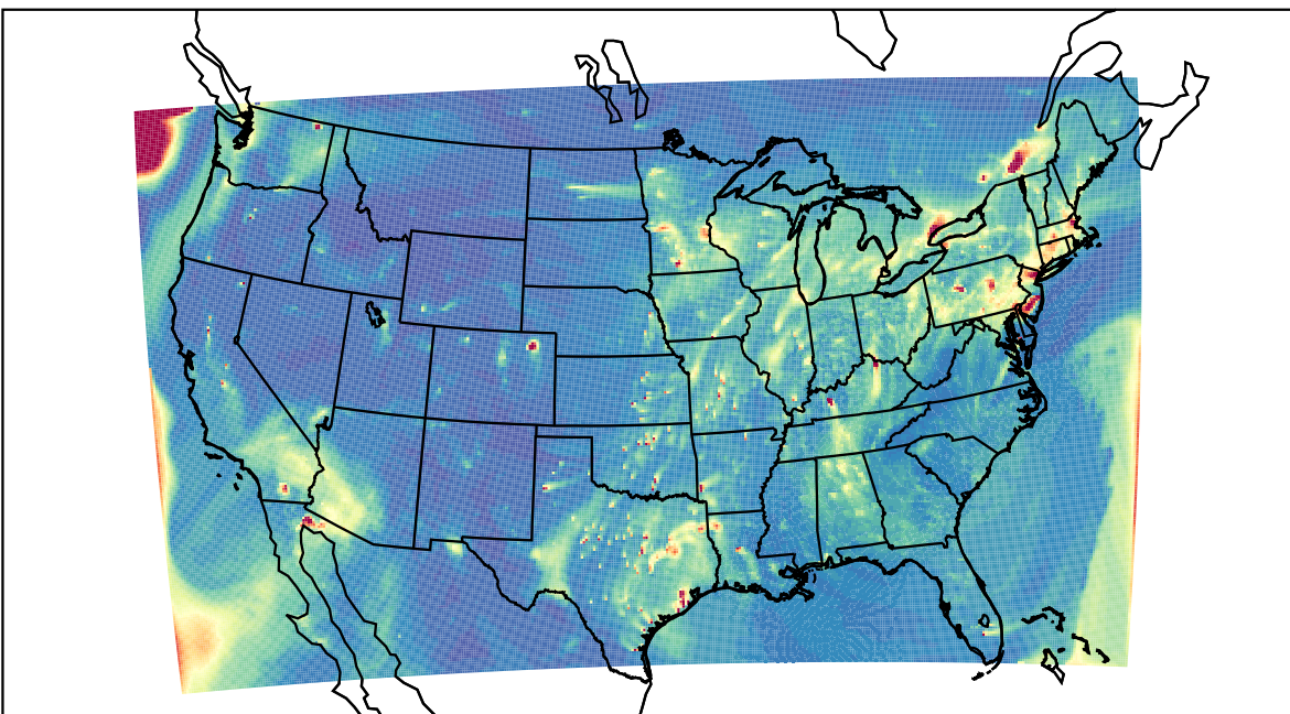
WRF 2023-02-13_00:00:00
