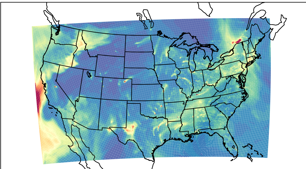
WRF 2023-02-13_23:00:00
