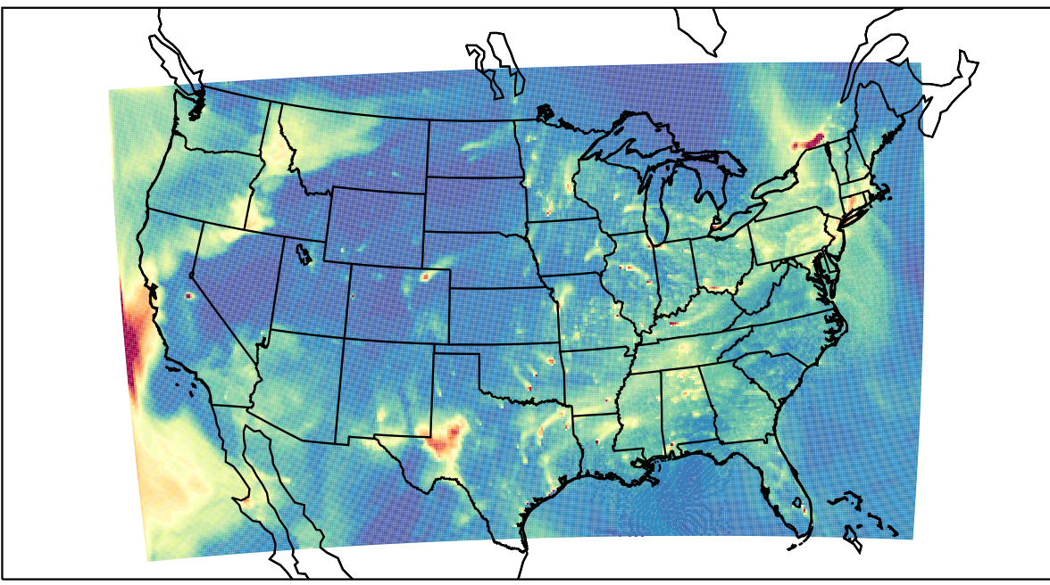
WRF 2023-02-14_00:00:00
