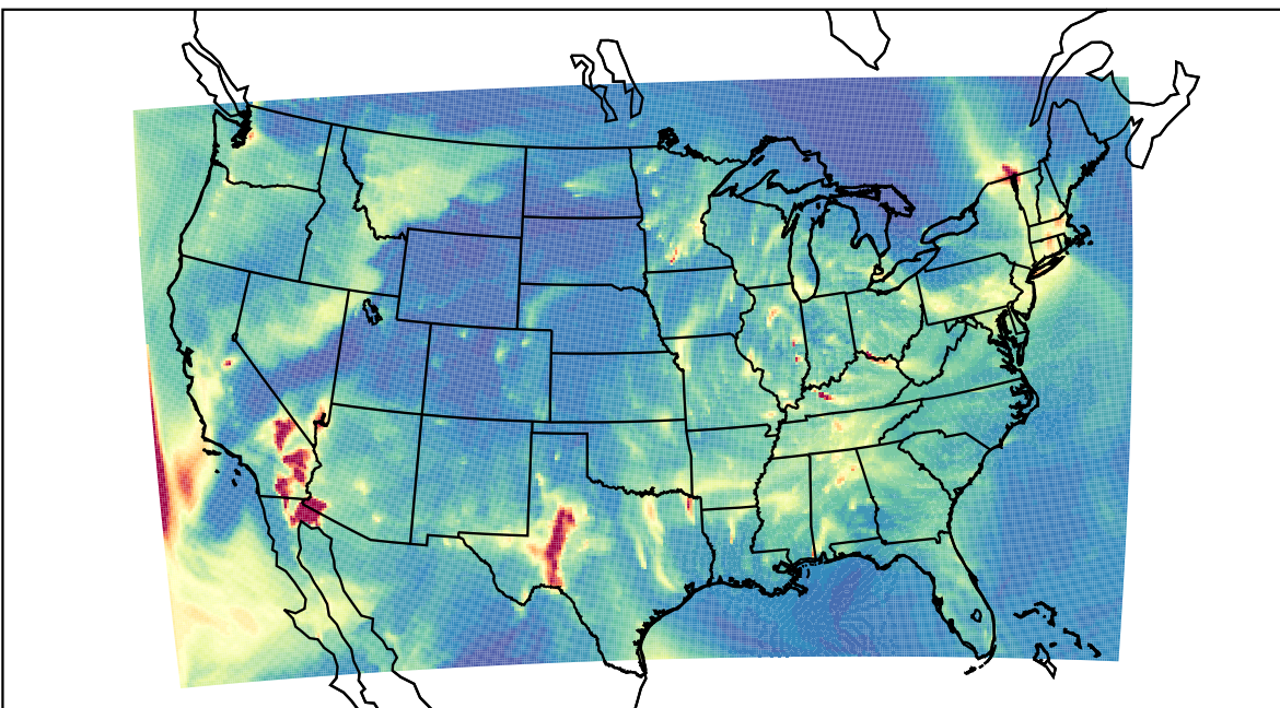
WRF 2023-02-14_05:00:00
