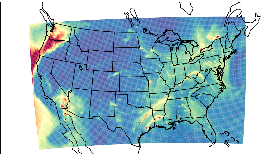
WRF 2023-02-13_15:00:00
