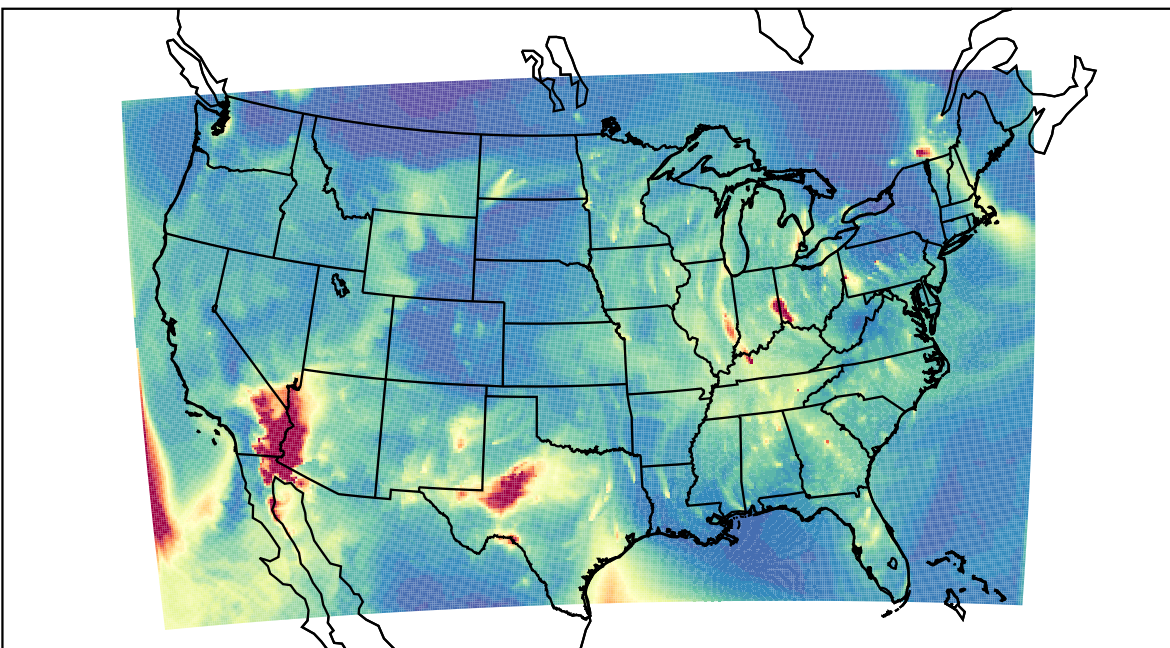
WRF 2023-02-14_14:00:00
