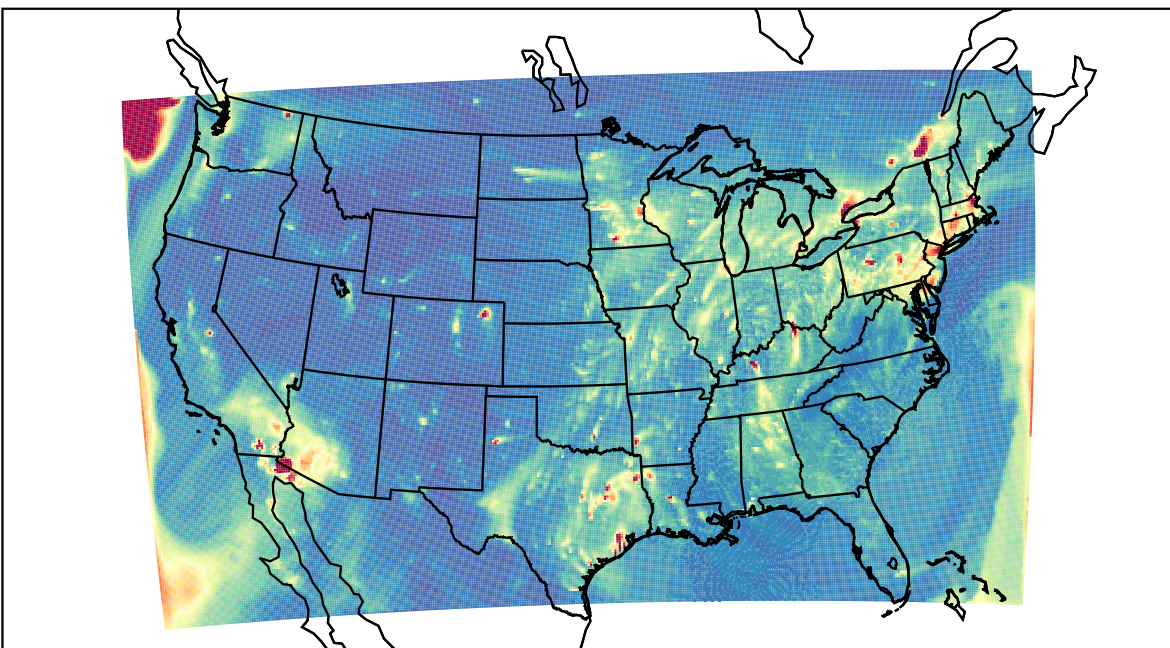
WRF 2023-02-13_01:00:00
