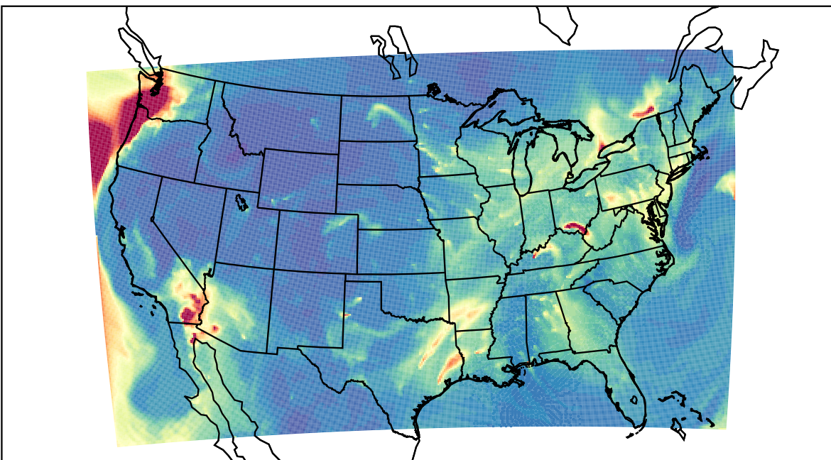
WRF 2023-02-13_11:00:00
