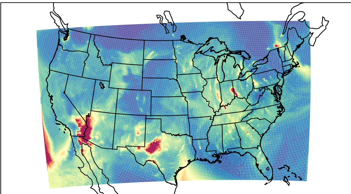
WRF 2023-02-14_15:00:00
