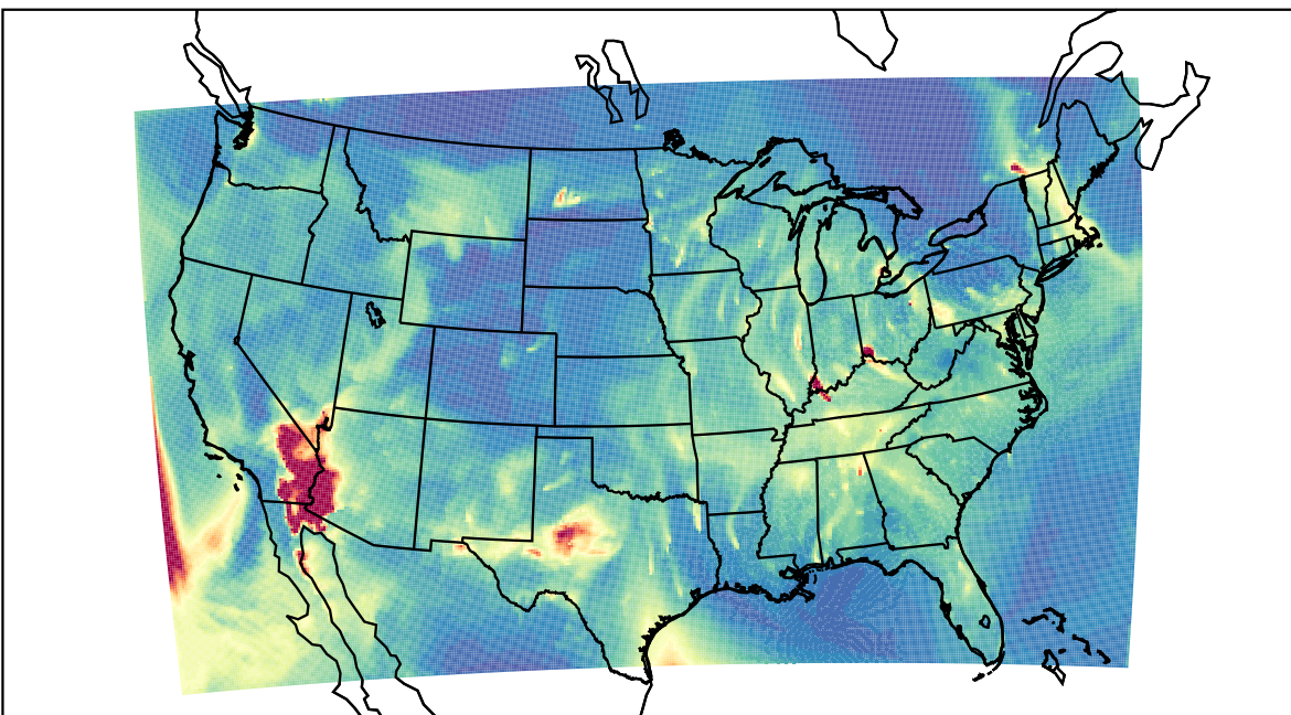
WRF 2023-02-14_11:00:00
