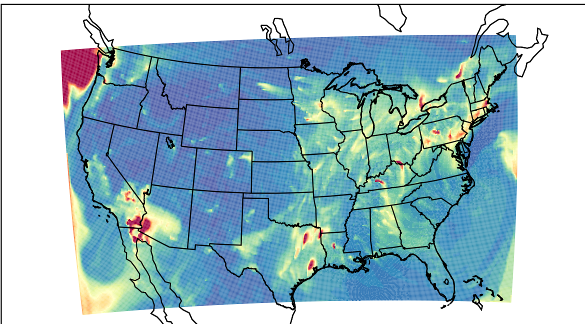
WRF 2023-02-13_05:00:00
