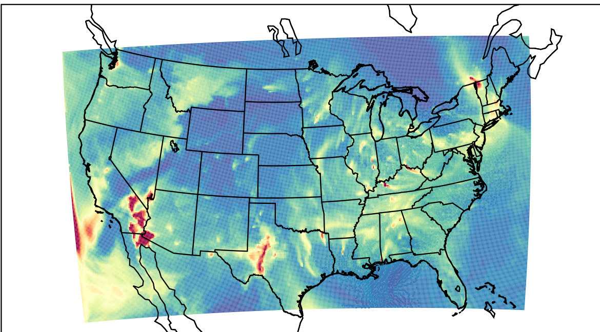
WRF 2023-02-14_06:00:00
