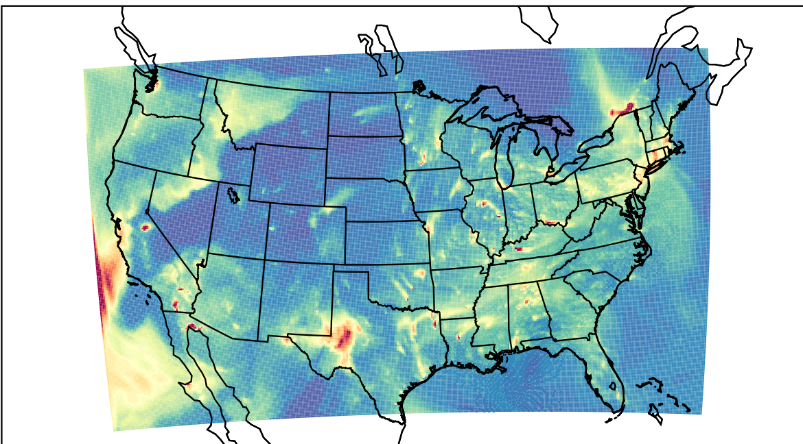
WRF 2023-02-14_02:00:00
