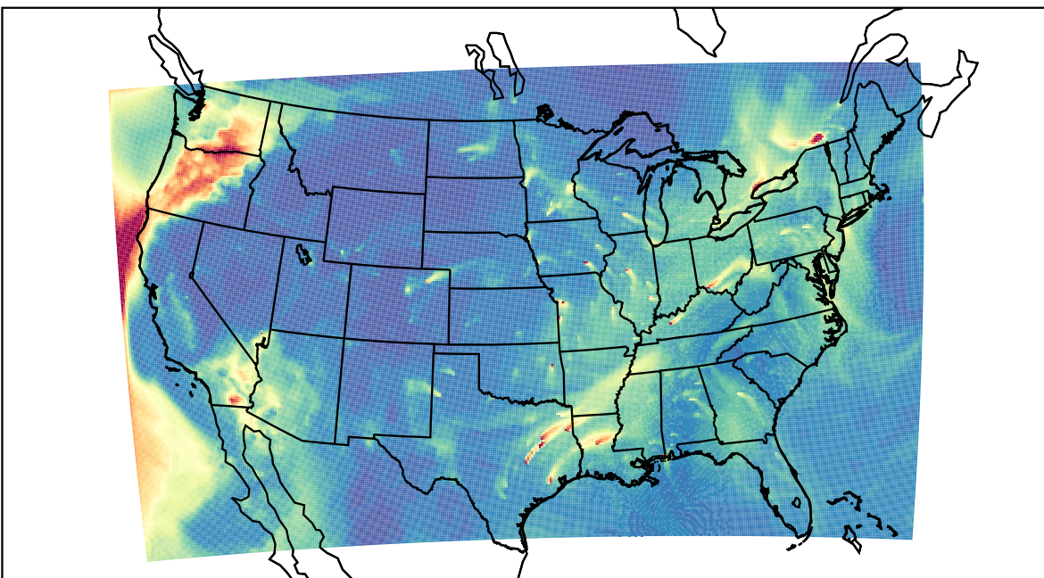
WRF 2023-02-13_17:00:00
