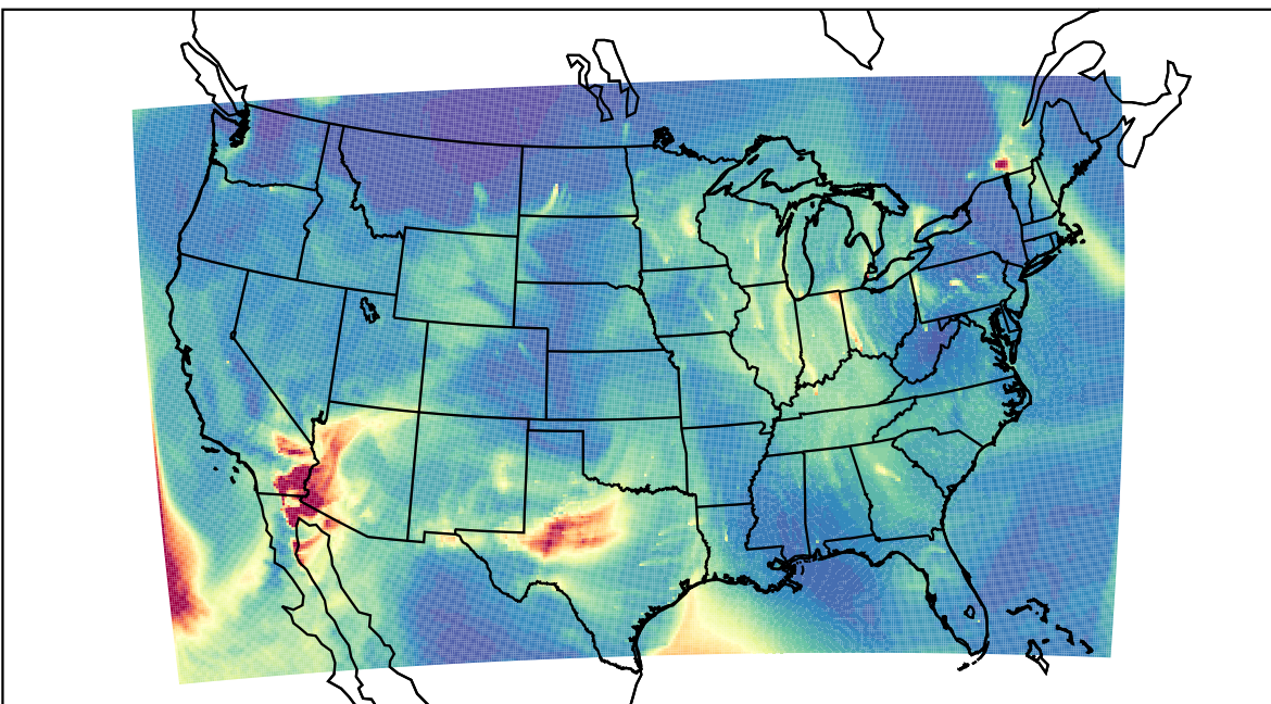
WRF 2023-02-14_19:00:00
