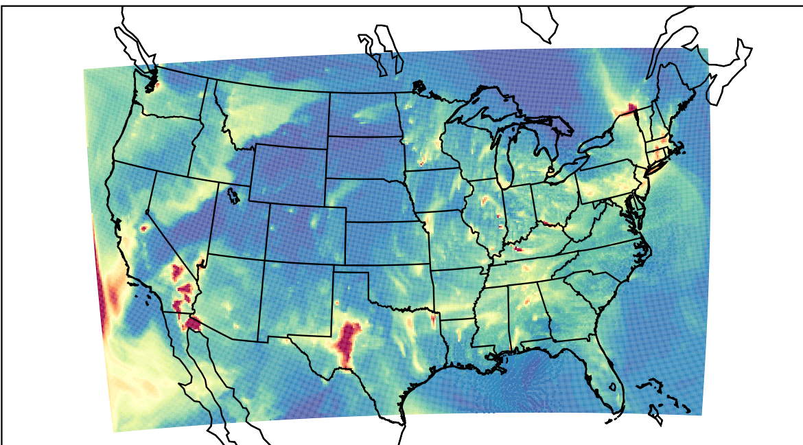
WRF 2023-02-14_04:00:00
