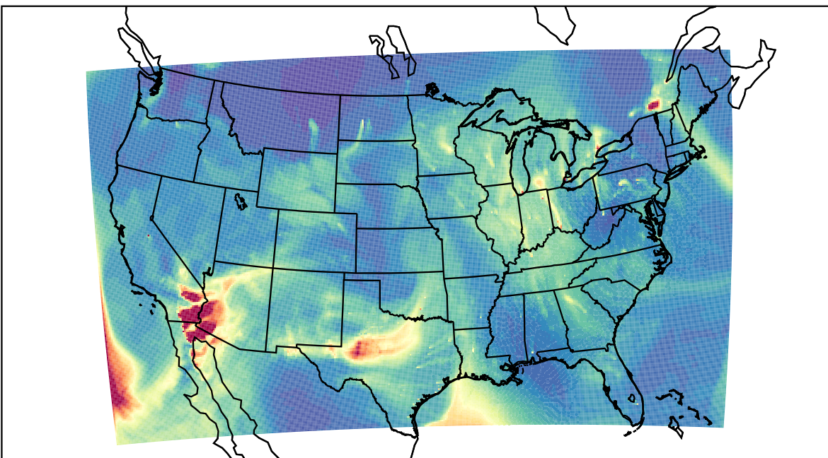
WRF 2023-02-14_21:00:00
