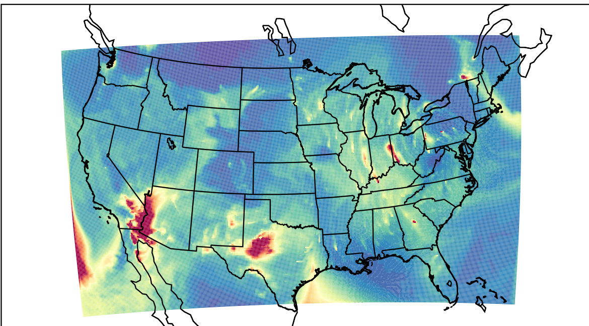
WRF 2023-02-14_16:00:00
