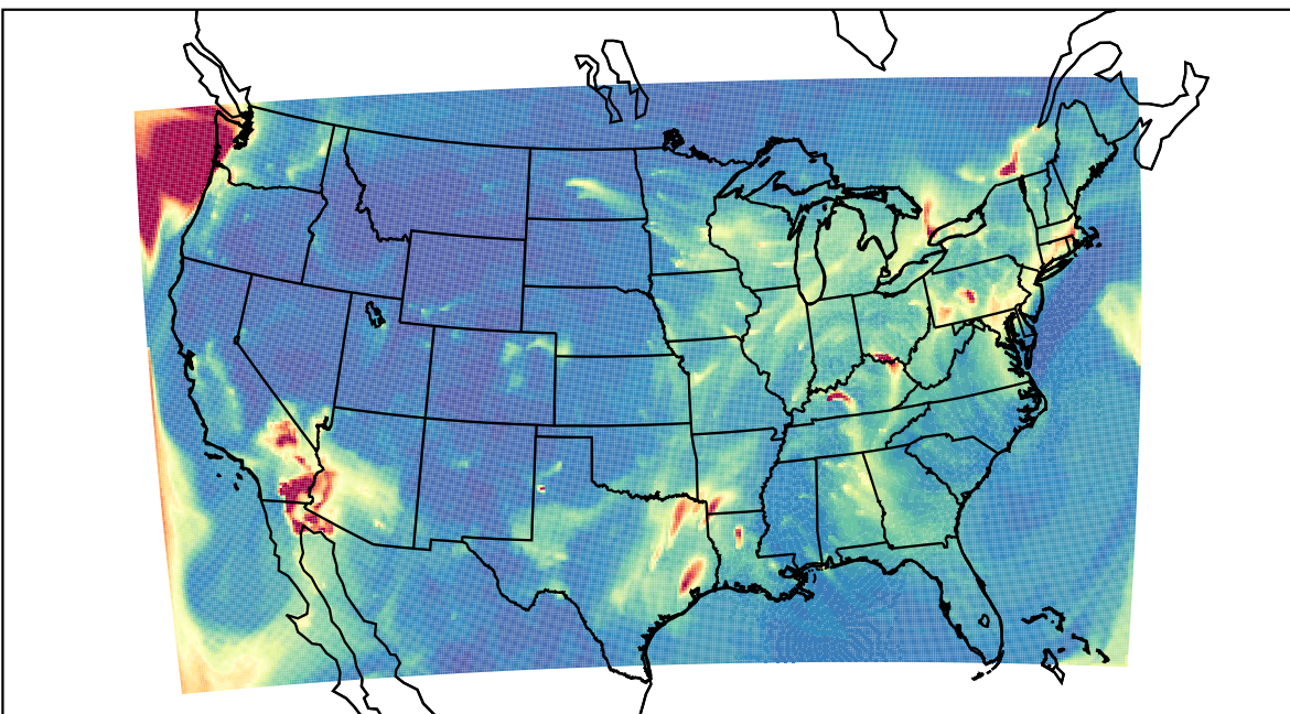
WRF 2023-02-13_07:00:00
