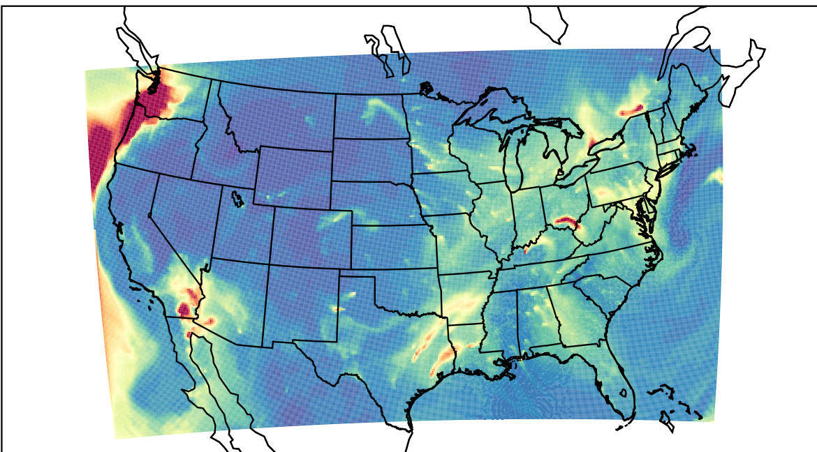
WRF 2023-02-13_12:00:00
