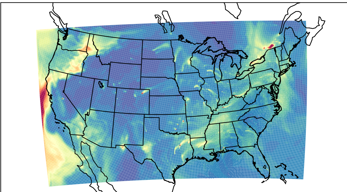
WRF 2023-02-13_21:00:00
