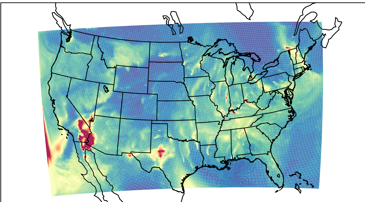
WRF 2023-02-14_09:00:00
