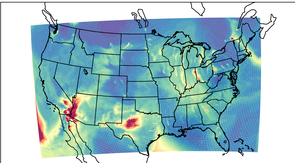
WRF 2023-02-14_17:00:00
