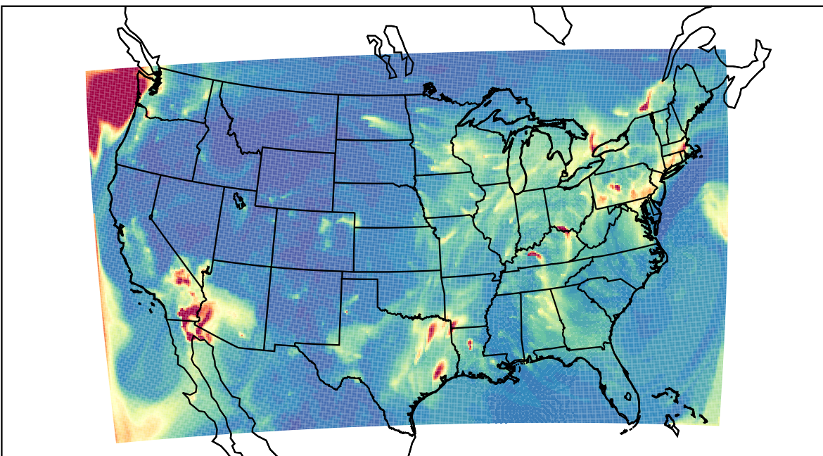
WRF 2023-02-13_06:00:00
