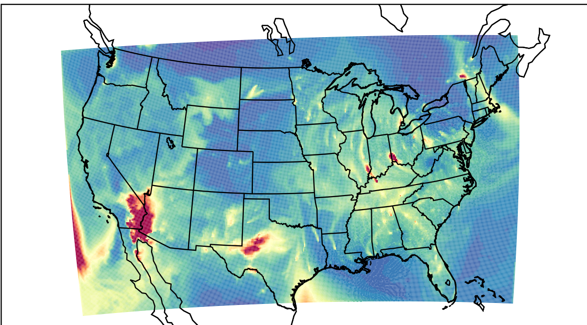
WRF 2023-02-14_13:00:00
