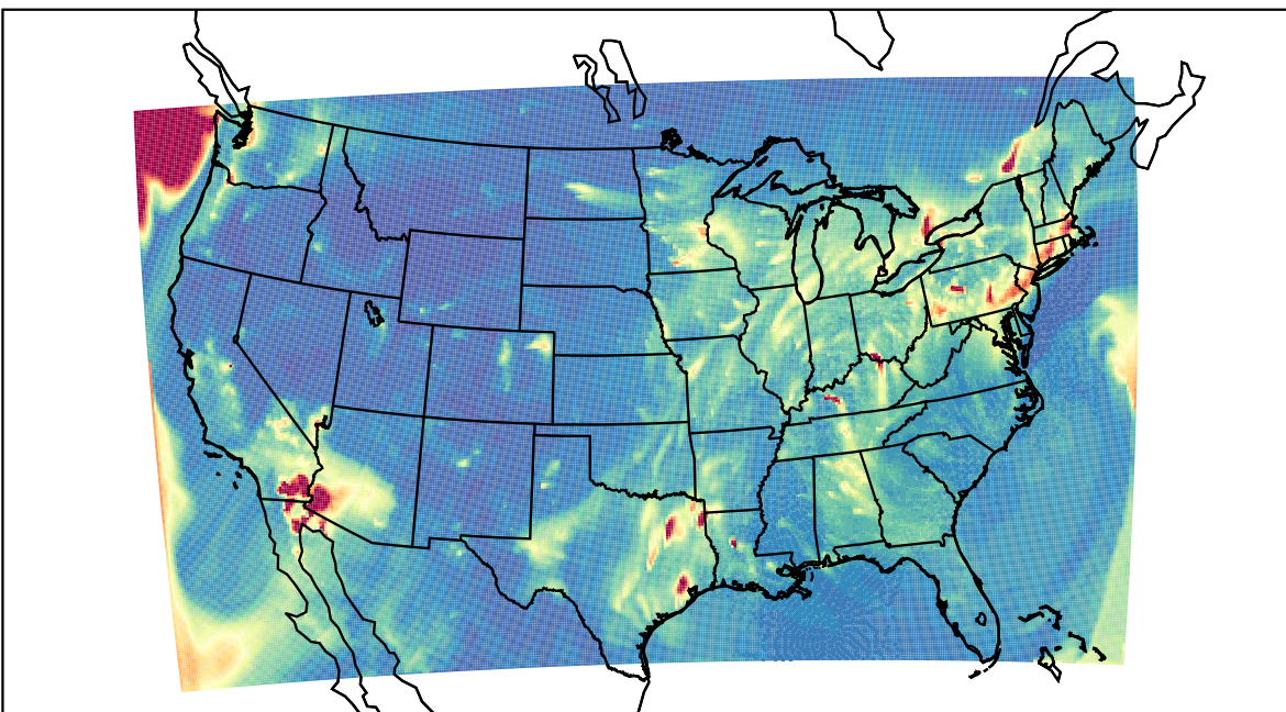
WRF 2023-02-13_04:00:00
