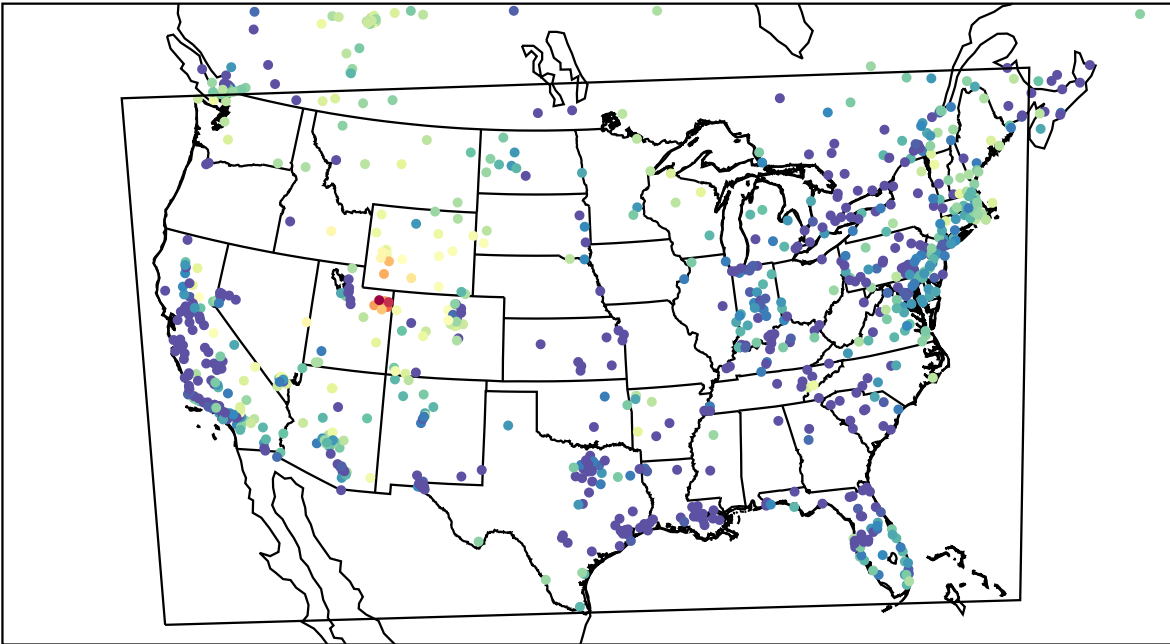
AirNOW (2023-02-13_11:00:00)
