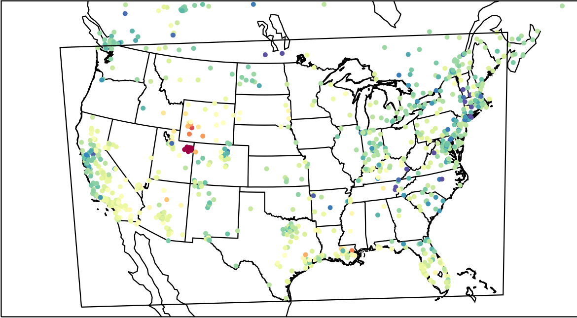
AirNOW (2023-02-13_23:00:00)
