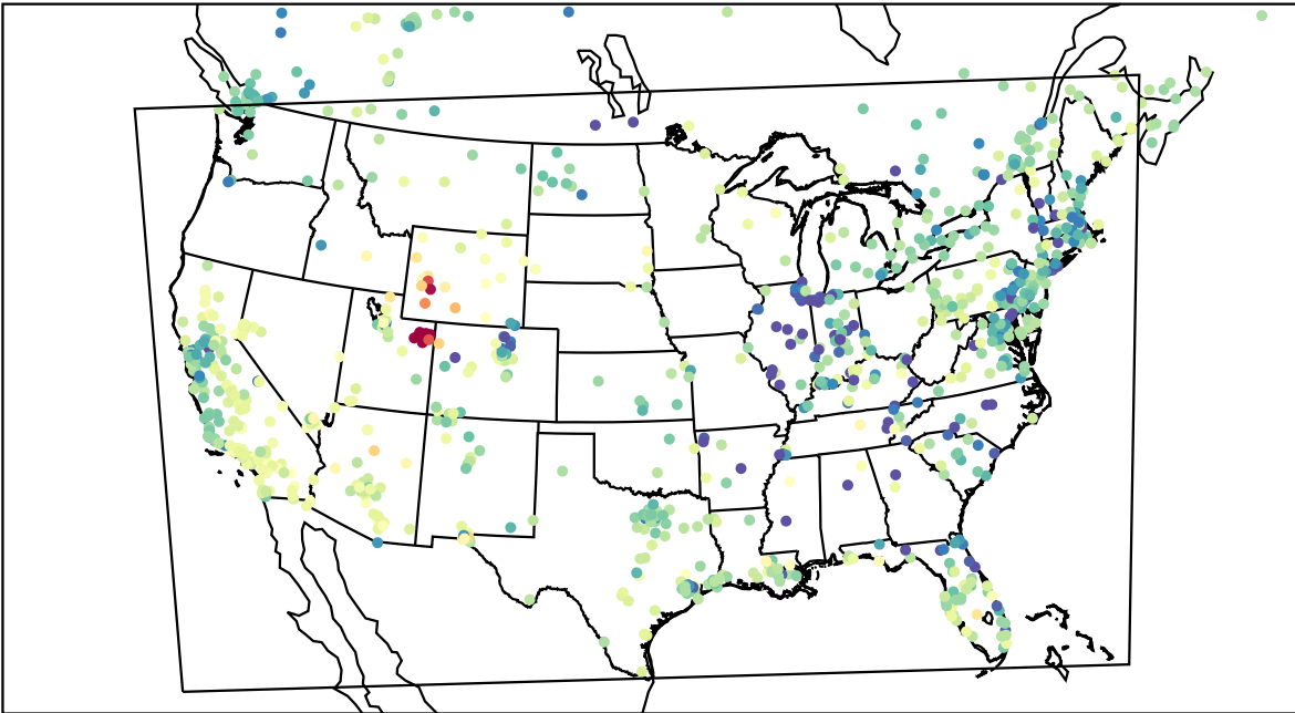
AirNOW (2023-02-14_00:00:00)
