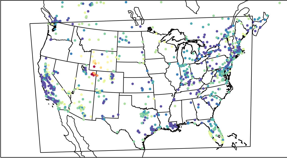
AirNOW (2023-02-13_06:00:00)
