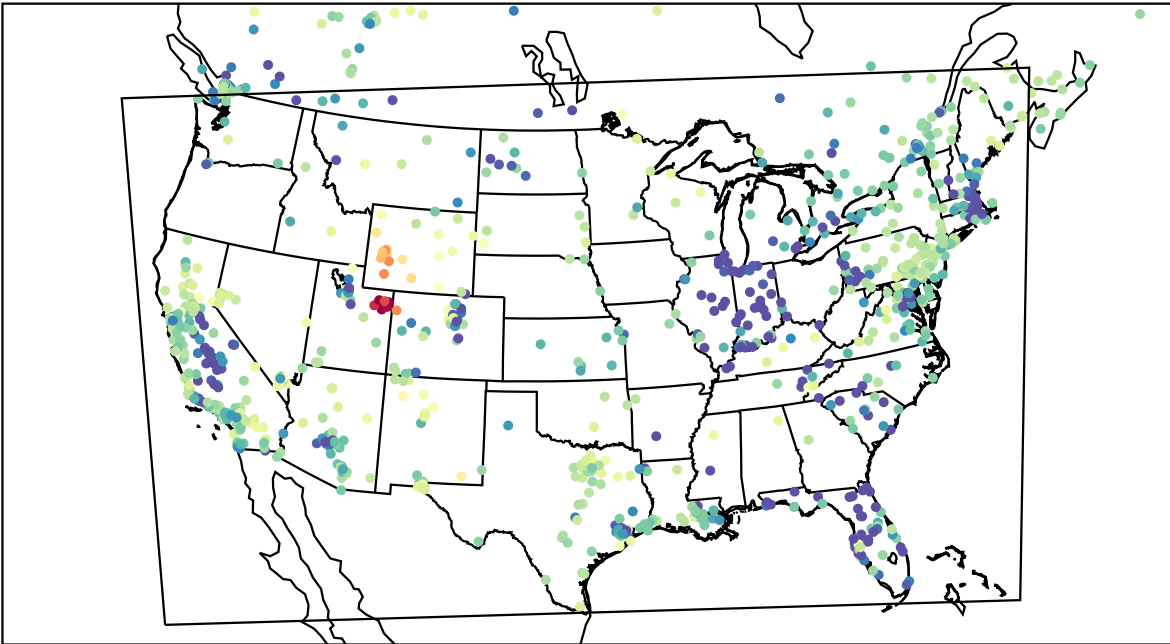
AirNOW (2023-02-14_05:00:00)
