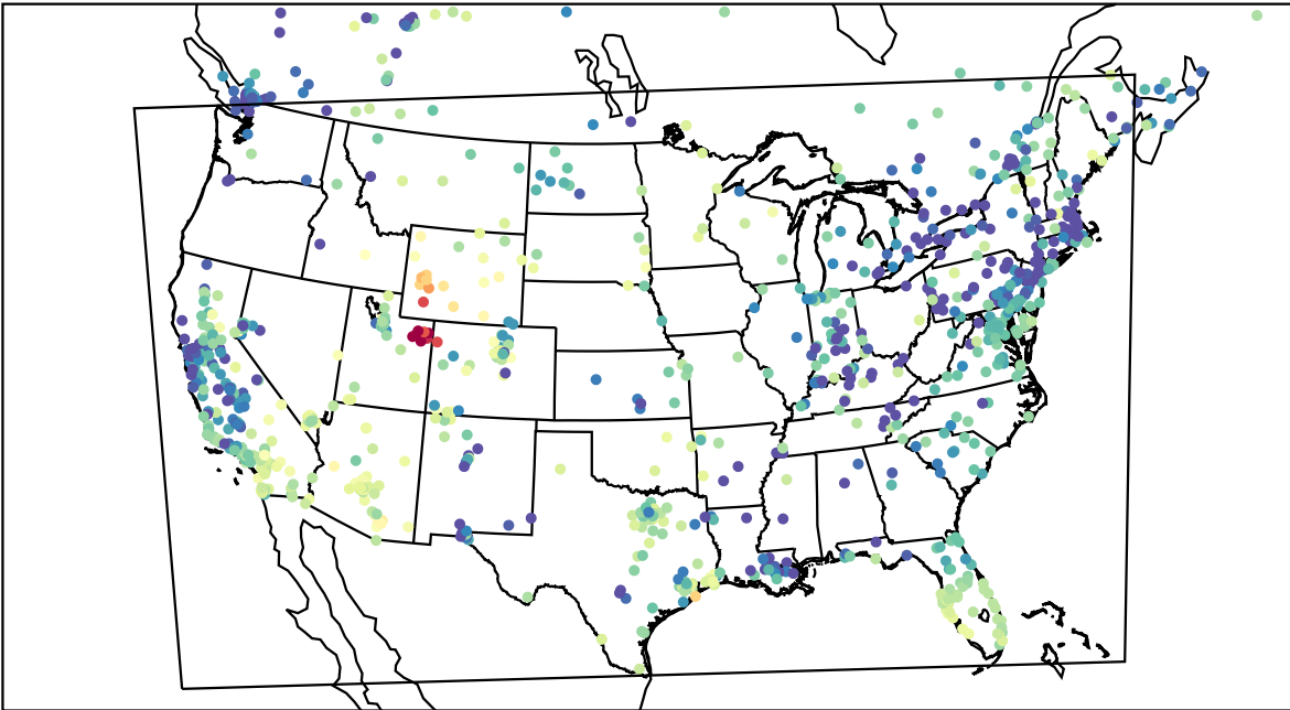
AirNOW (2023-02-13_02:00:00)
