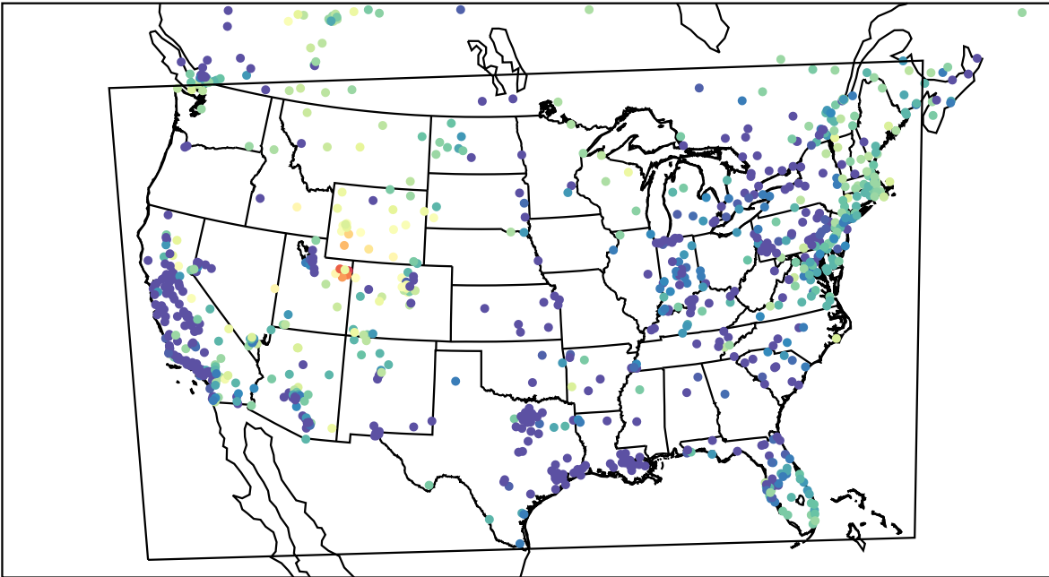
AirNOW (2023-02-13_13:00:00)
