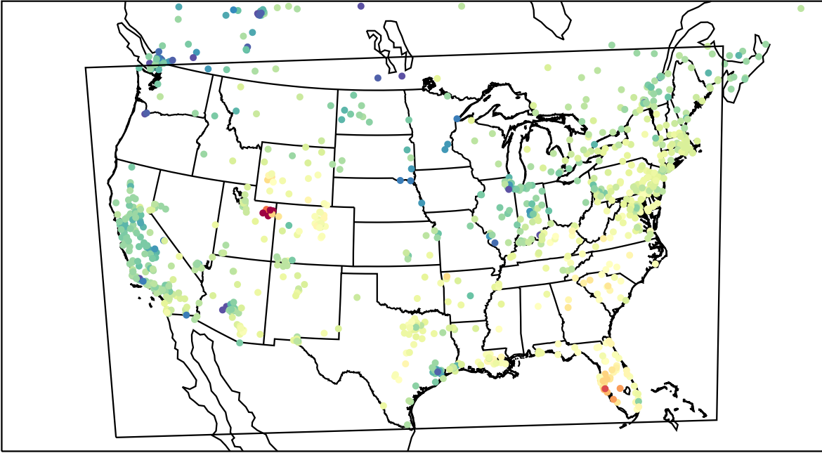
AirNOW (2023-02-14_18:00:00)
