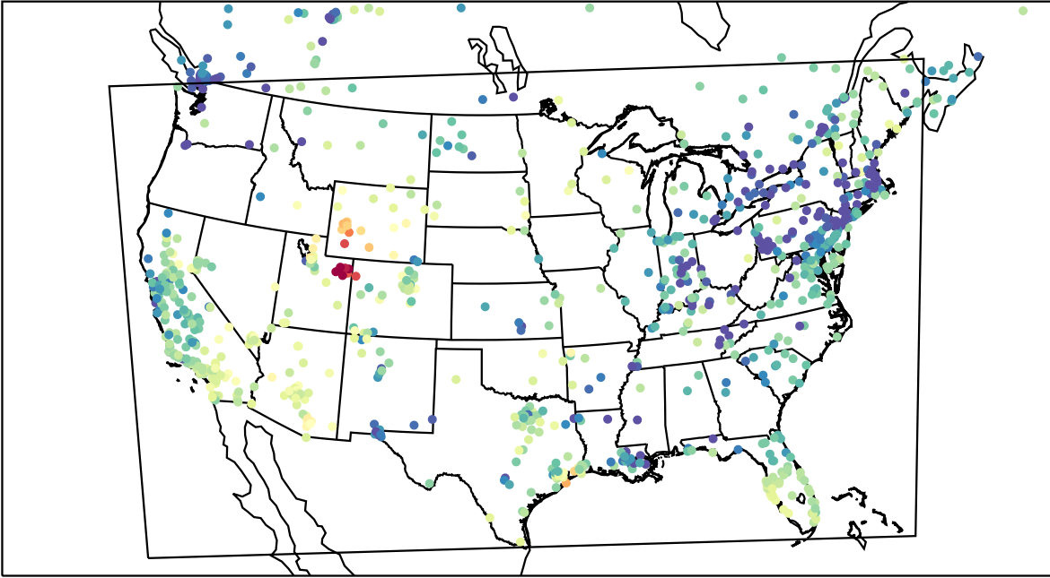
AirNOW (2023-02-13_01:00:00)
