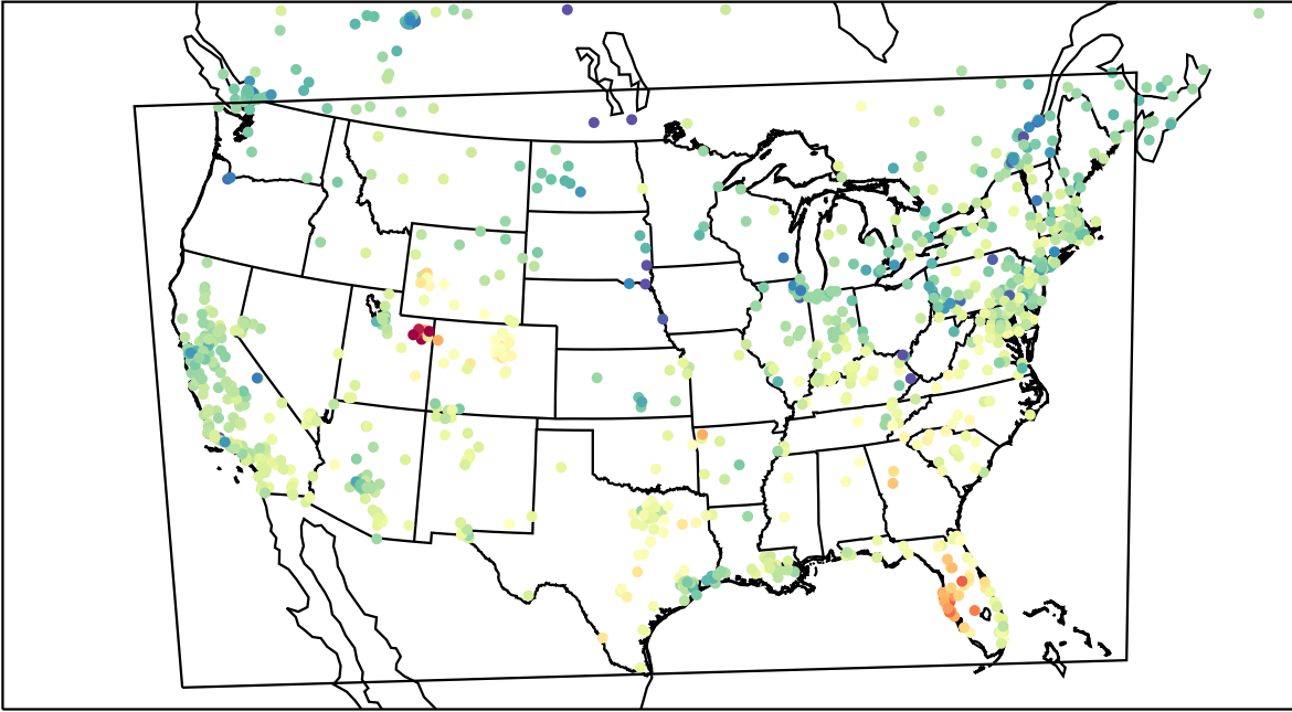
AirNOW (2023-02-14_22:00:00)
