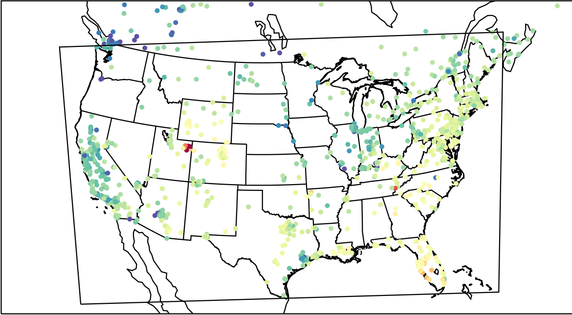
AirNOW (2023-02-14_17:00:00)
