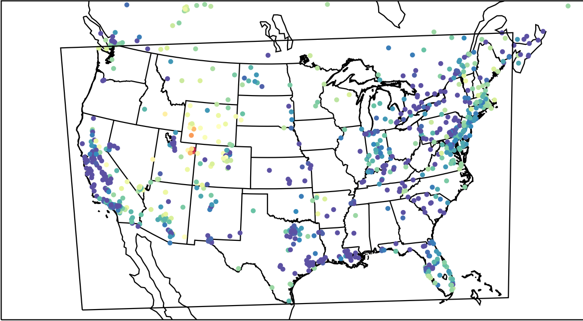
AirNOW (2023-02-13_10:00:00)
