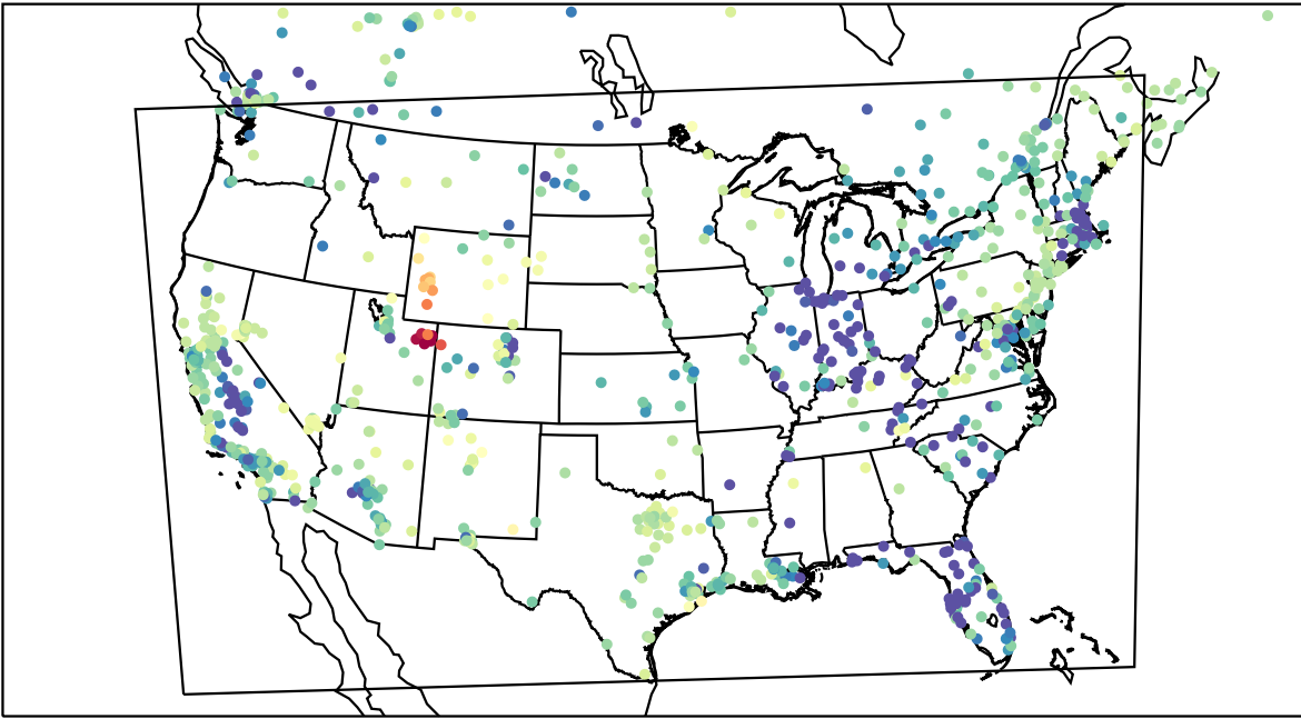
AirNOW (2023-02-14_06:00:00)
