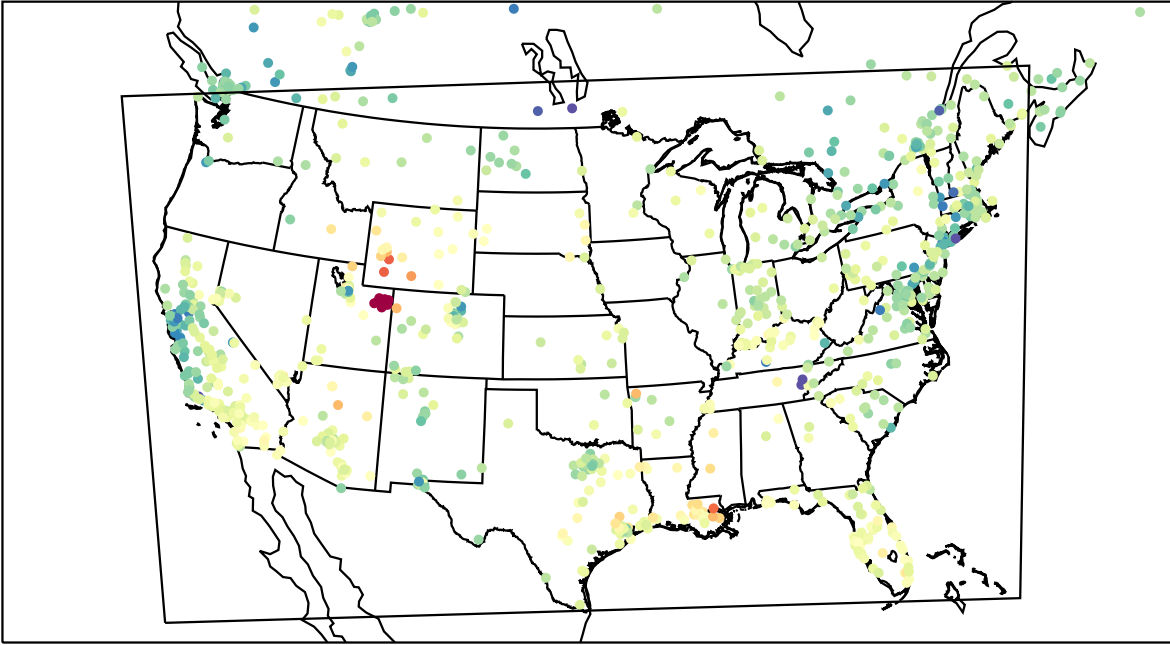
AirNOW (2023-02-13_22:00:00)
