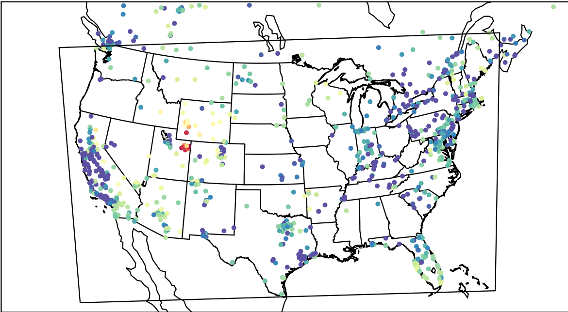
AirNOW (2023-02-13_07:00:00)
