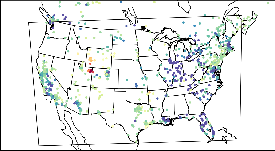
AirNOW (2023-02-14_08:00:00)
