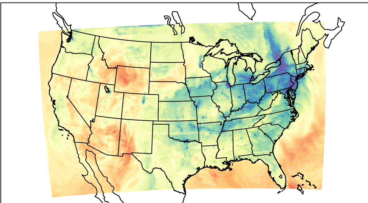
WRF (2023-02-14_00:00:00)
