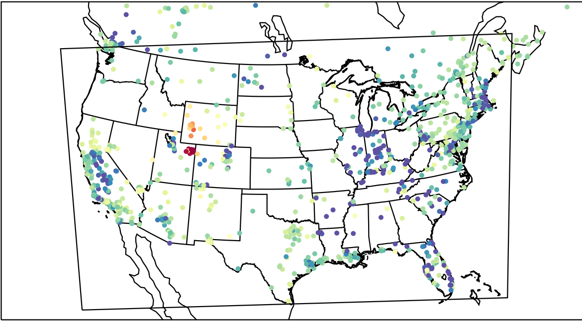
AirNOW (2023-02-14_03:00:00)
