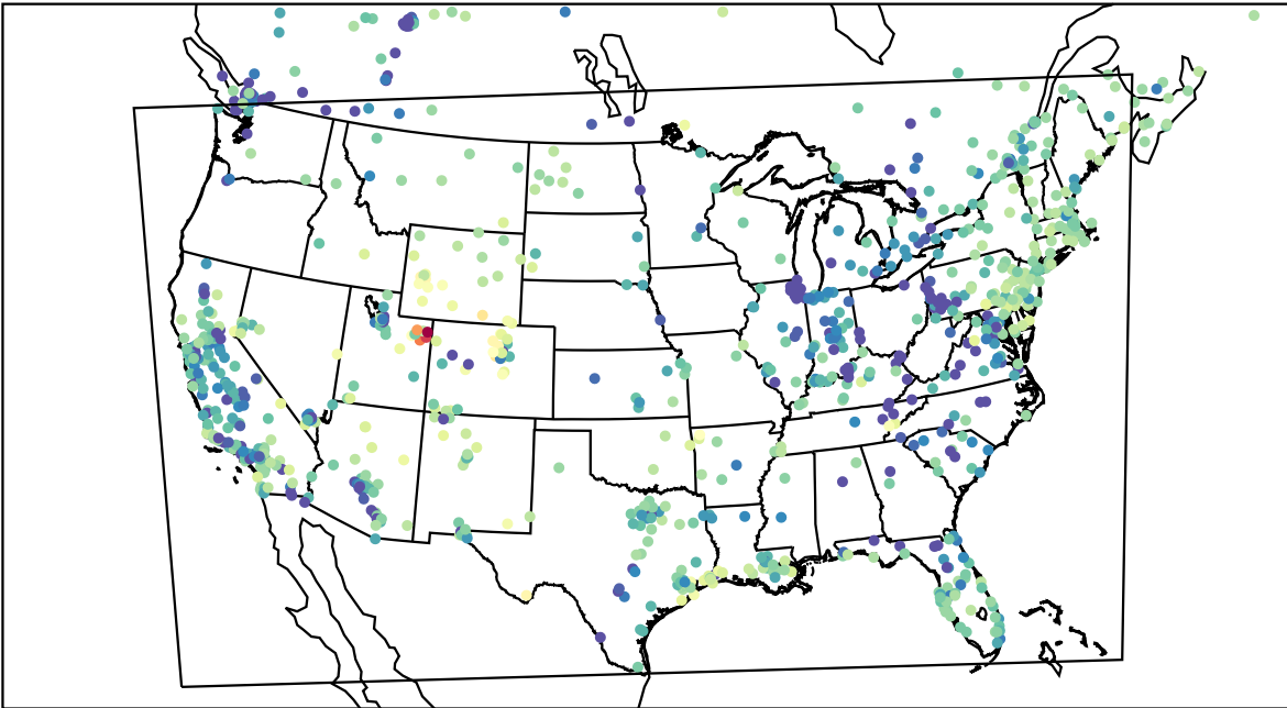
AirNOW (2023-02-14_14:00:00)
