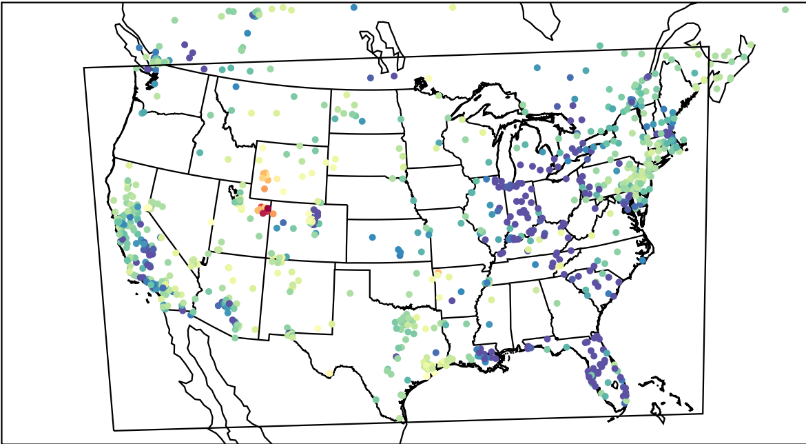
AirNOW (2023-02-14_09:00:00)
