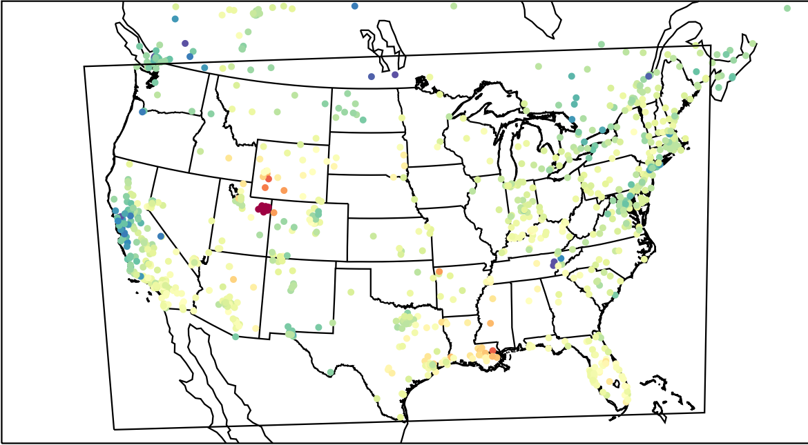
AirNOW (2023-02-13_21:00:00)
