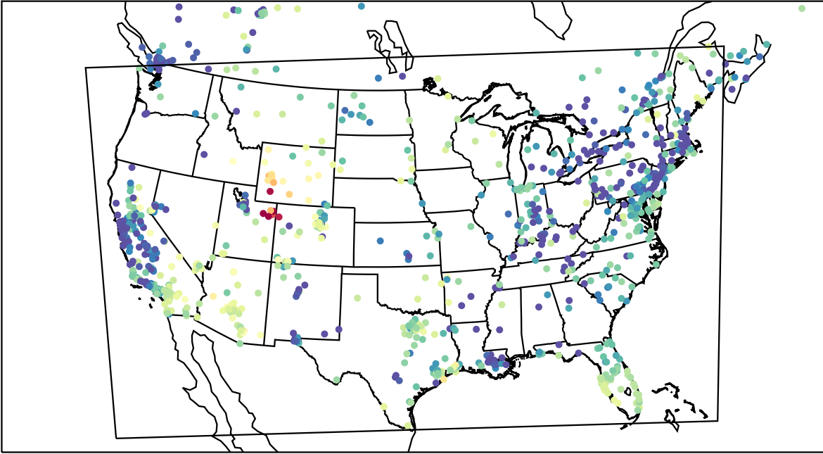
AirNOW (2023-02-13_03:00:00)
