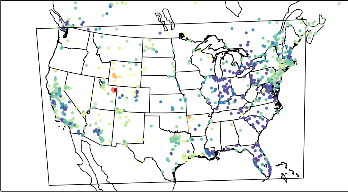
AirNOW (2023-02-14_10:00:00)
