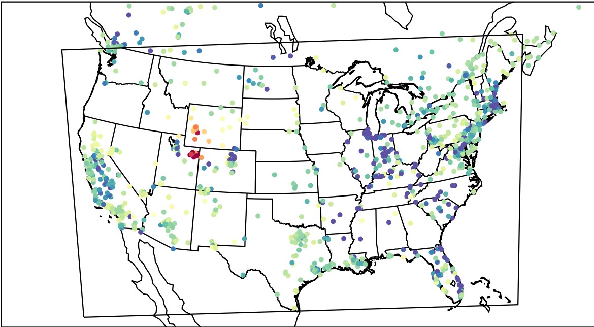
AirNOW (2023-02-14_02:00:00)
