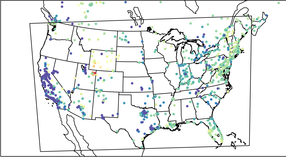
AirNOW (2023-02-13_15:00:00)
