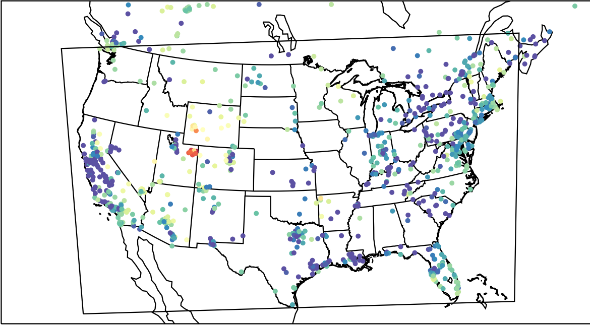
AirNOW (2023-02-13_09:00:00)
