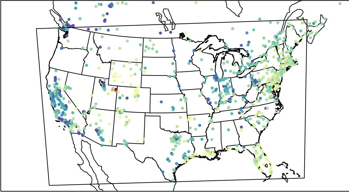
AirNOW (2023-02-14_15:00:00)
