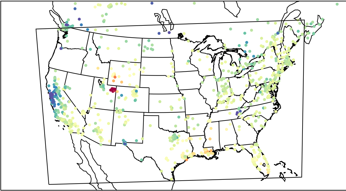
AirNOW (2023-02-13_19:00:00)
