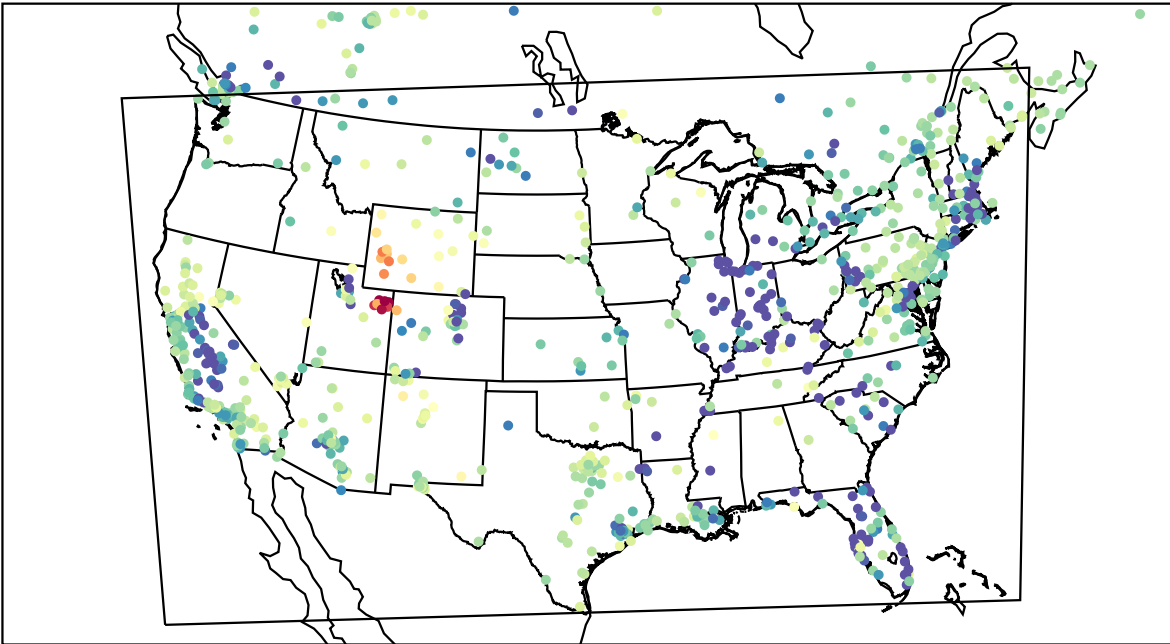
AirNOW (2023-02-14_04:00:00)
