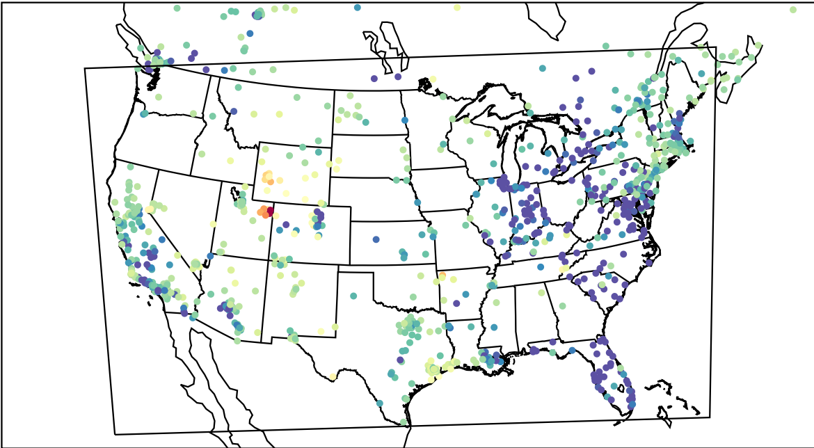
AirNOW (2023-02-14_11:00:00)
