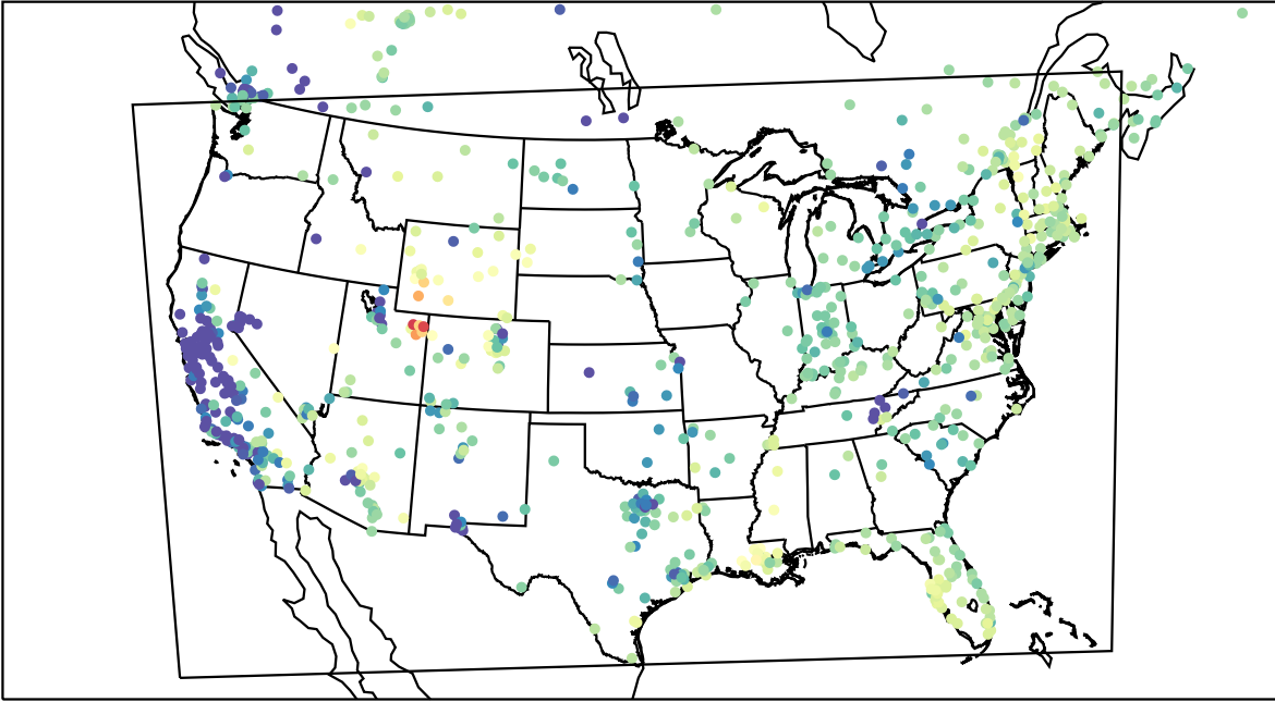
AirNOW (2023-02-13_16:00:00)
