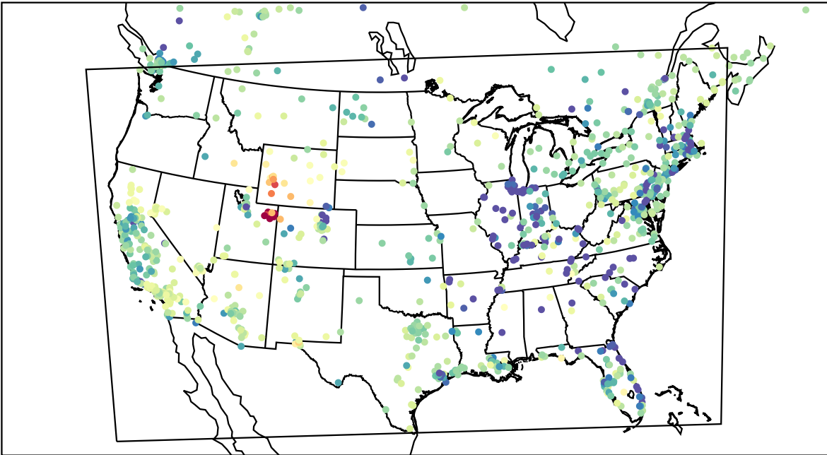
AirNOW (2023-02-14_01:00:00)
