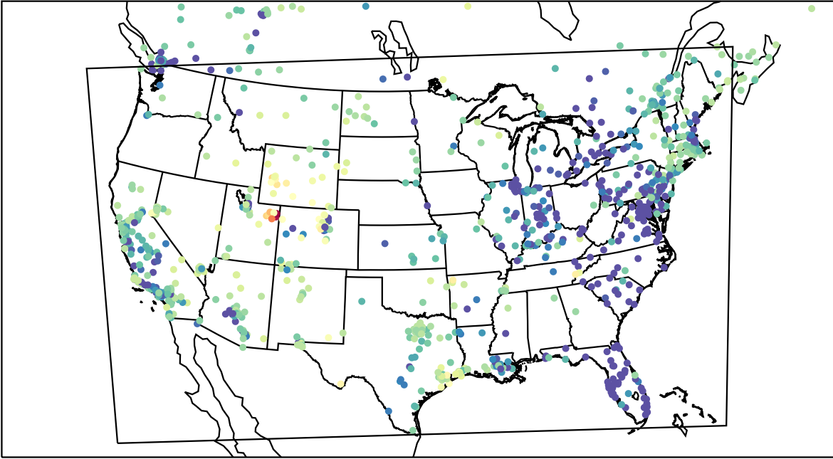
AirNOW (2023-02-14_12:00:00)
