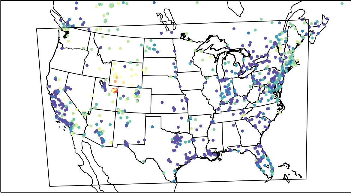
AirNOW (2023-02-13_12:00:00)
