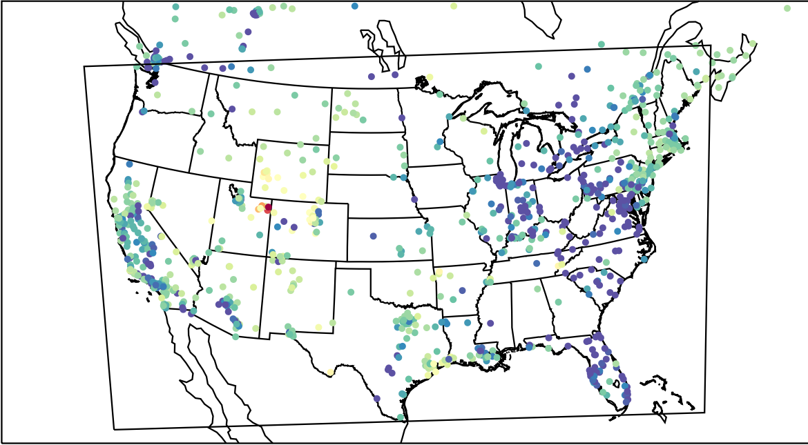
AirNOW (2023-02-14_13:00:00)
