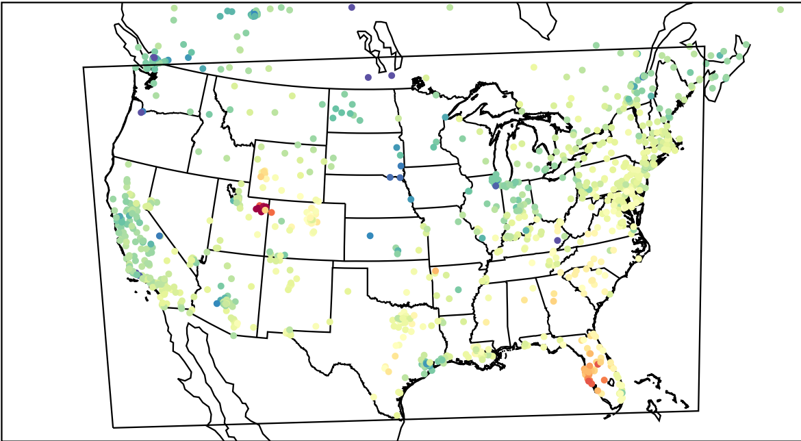
AirNOW (2023-02-14_20:00:00)
