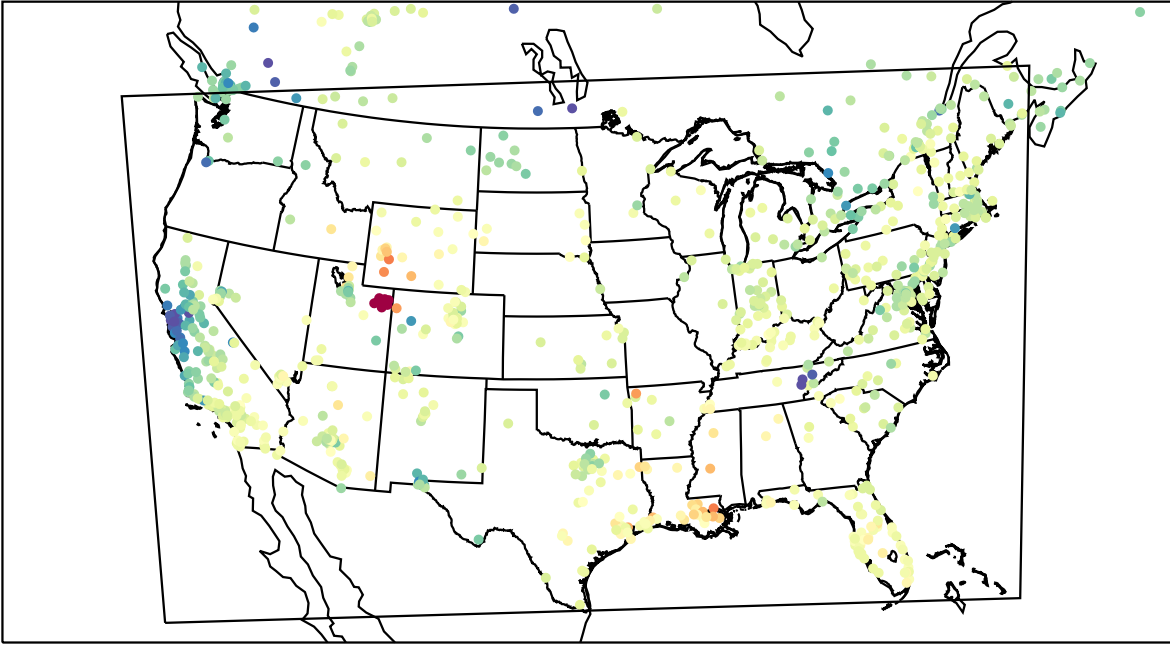
AirNOW (2023-02-13_20:00:00)
