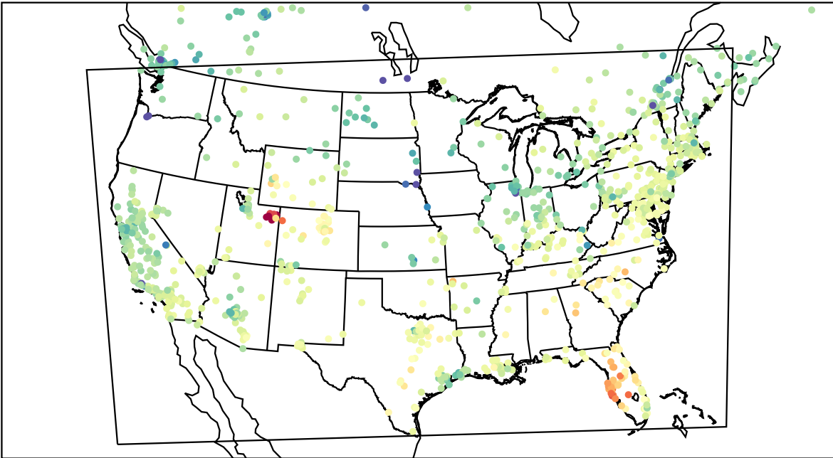
AirNOW (2023-02-14_21:00:00)
