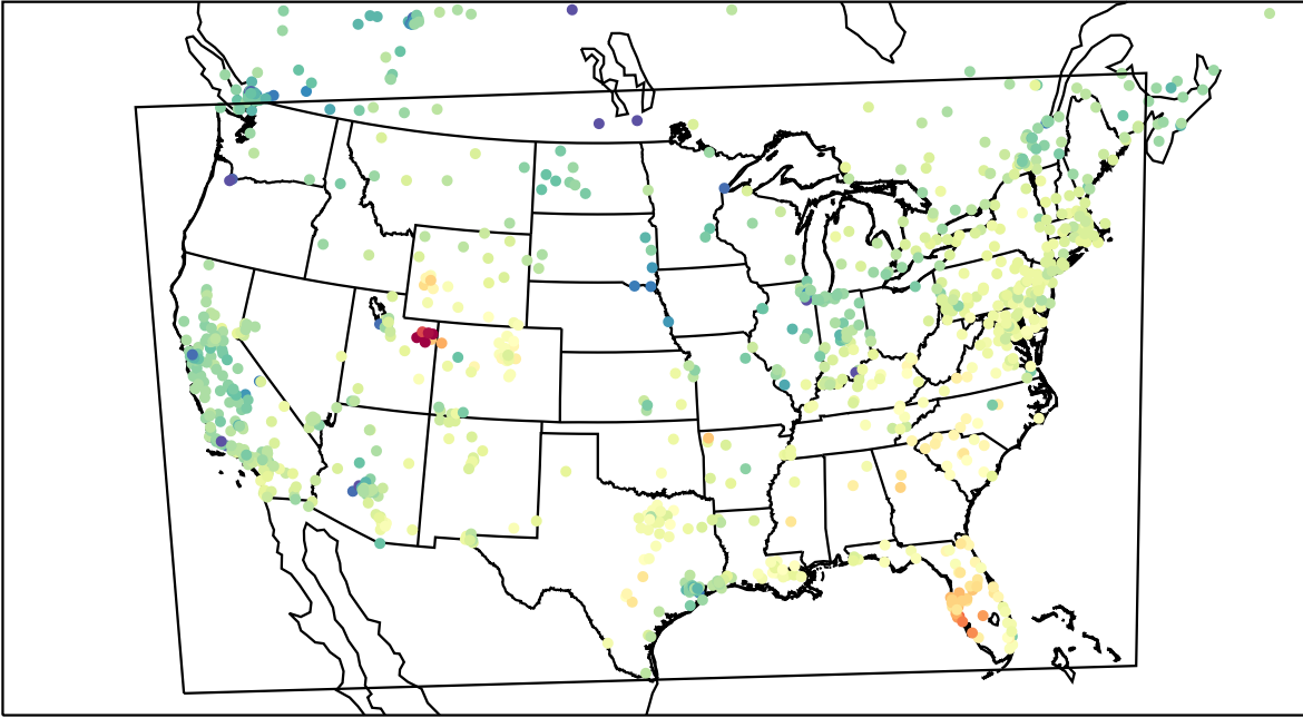
AirNOW (2023-02-14_19:00:00)
