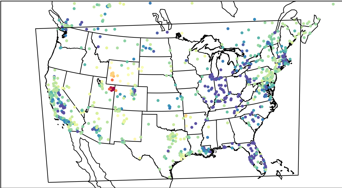
AirNOW (2023-02-14_07:00:00)
