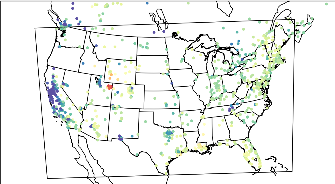
AirNOW (2023-02-13_17:00:00)
