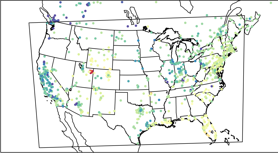
AirNOW (2023-02-14_16:00:00)
