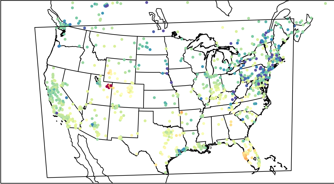
AirNOW (2023-02-14_23:00:00)
