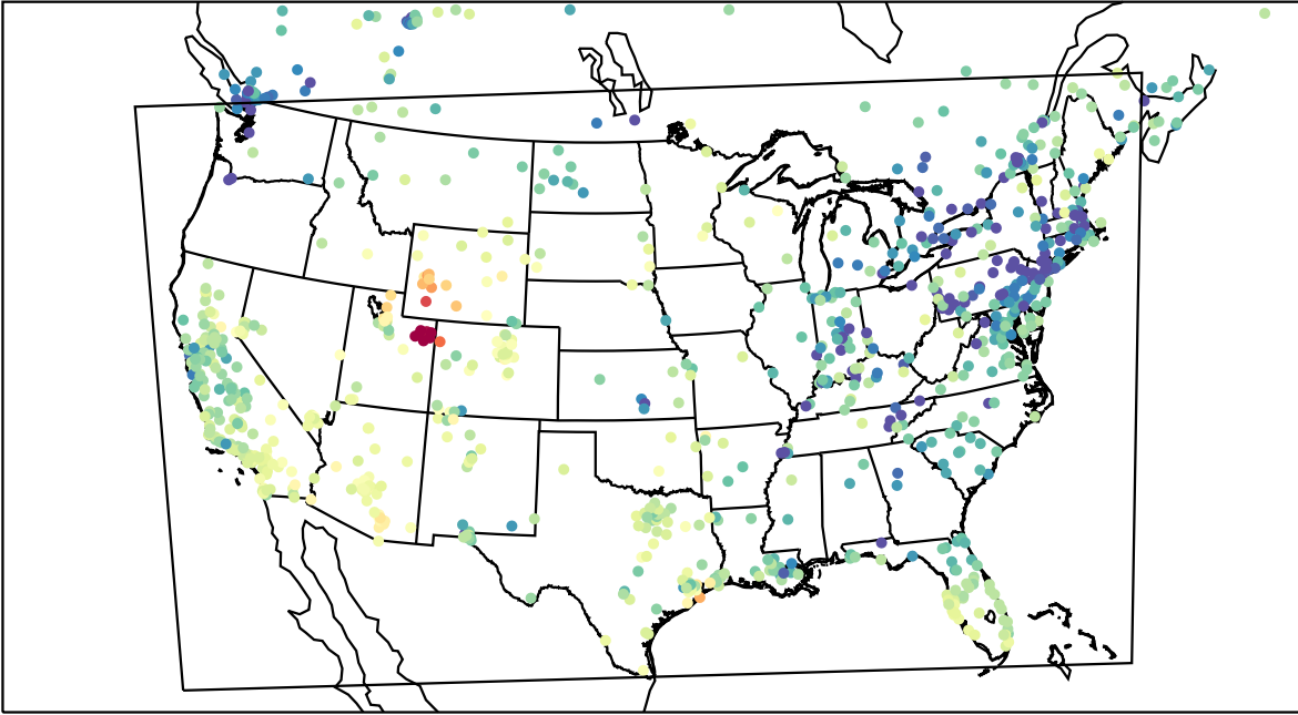
AirNOW (2023-02-13_00:00:00)
