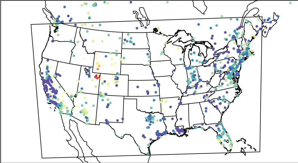
AirNOW (2023-02-13_08:00:00)
