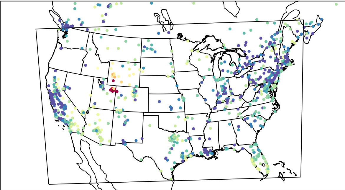
AirNOW (2023-02-13_04:00:00)
