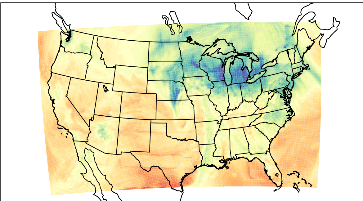
WRF (2023-02-14_22:00:00)
