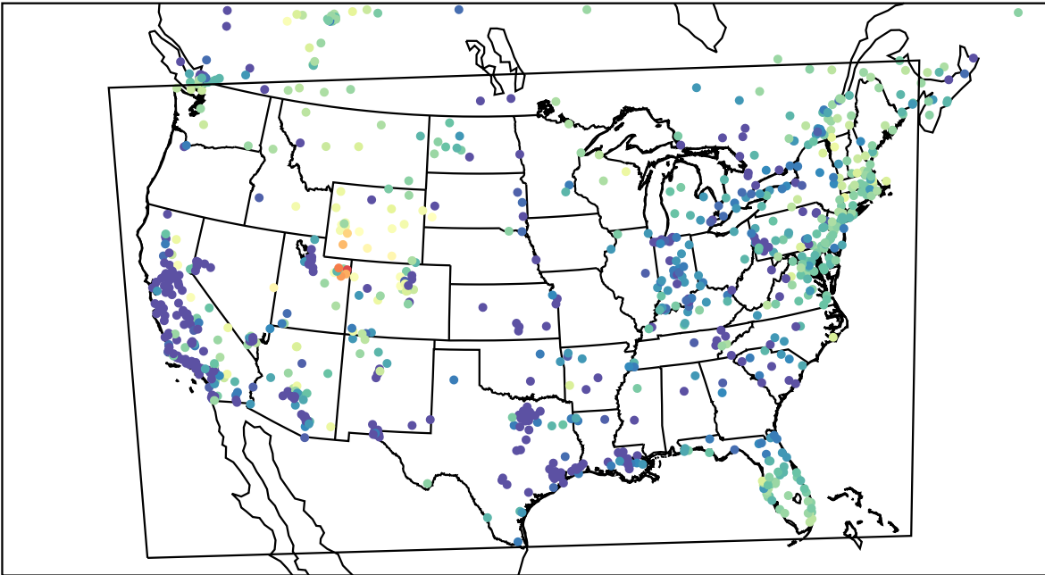
AirNOW (2023-02-13_14:00:00)
