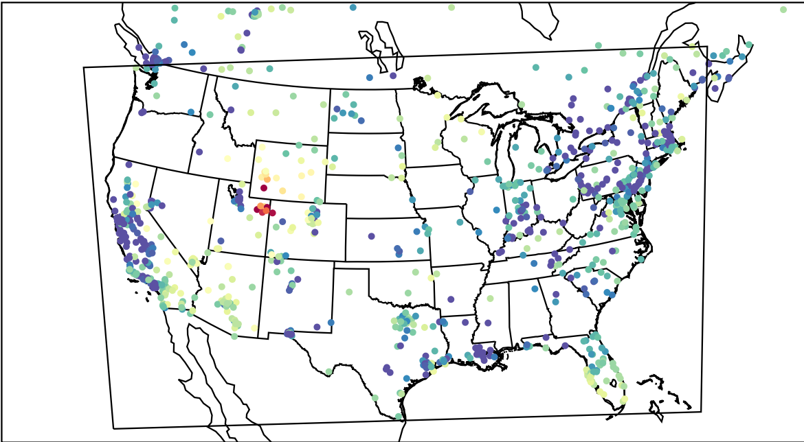
AirNOW (2023-02-13_05:00:00)
