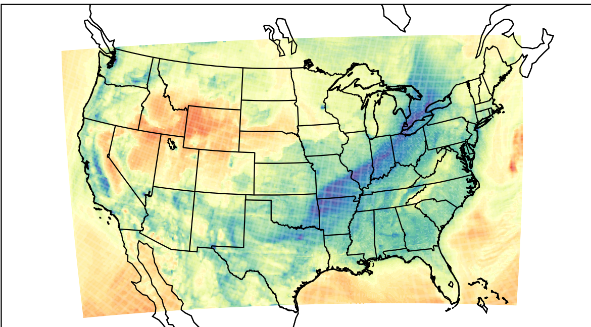
WRF (2023-02-13_16:00:00)
