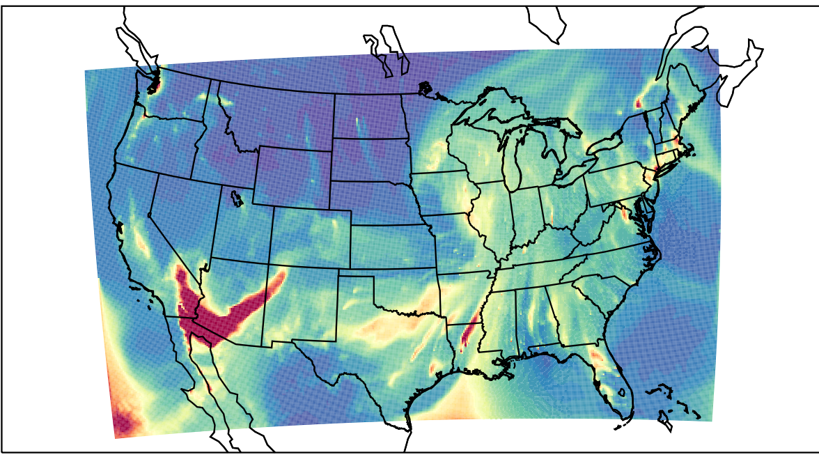
WRF 2023-02-15_06:00:00
