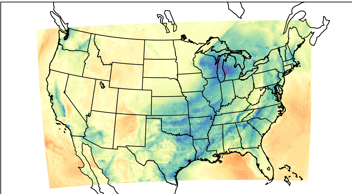
WRF (2023-02-15_15:00:00)
