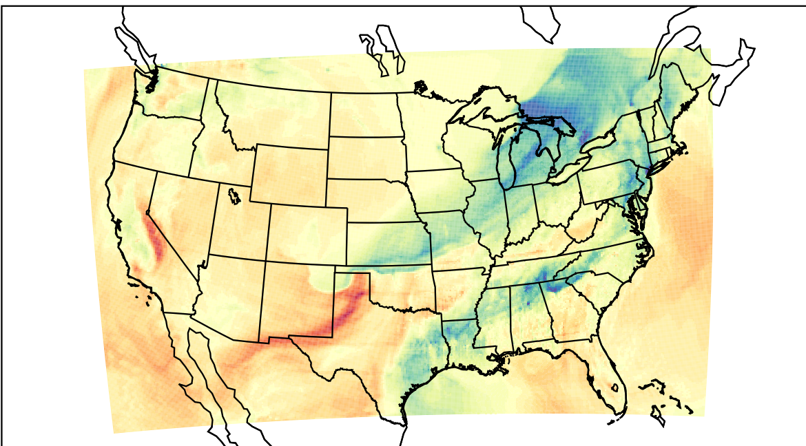
WRF (2023-02-15_22:00:00)
