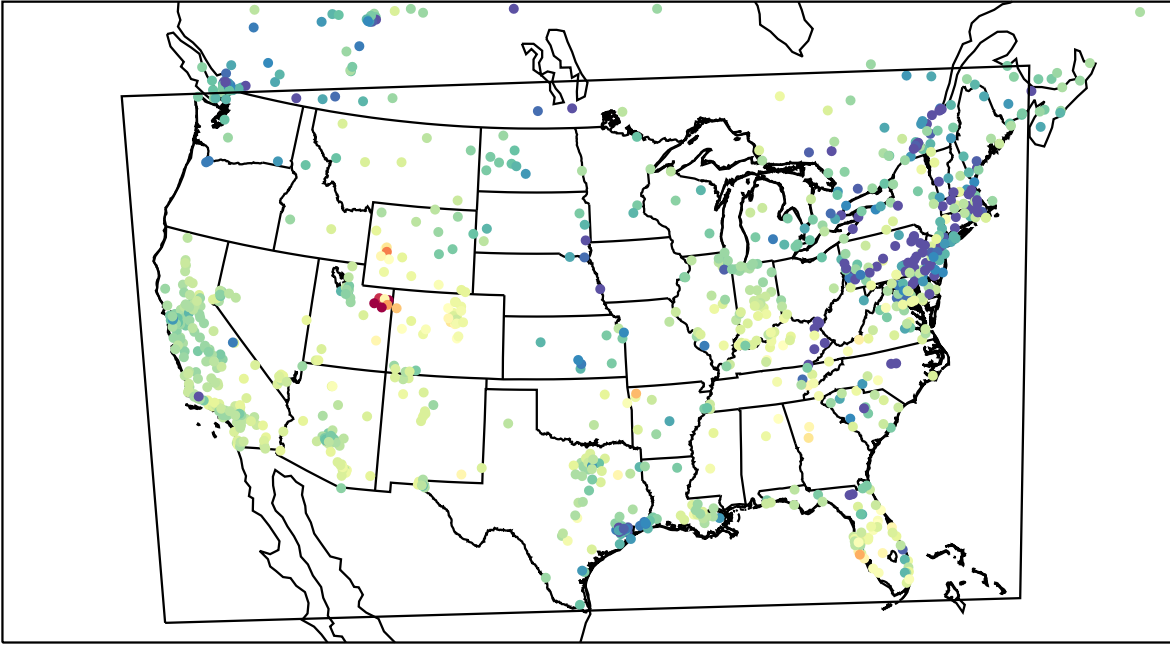
AirNOW (2023-02-15_00:00:00)
