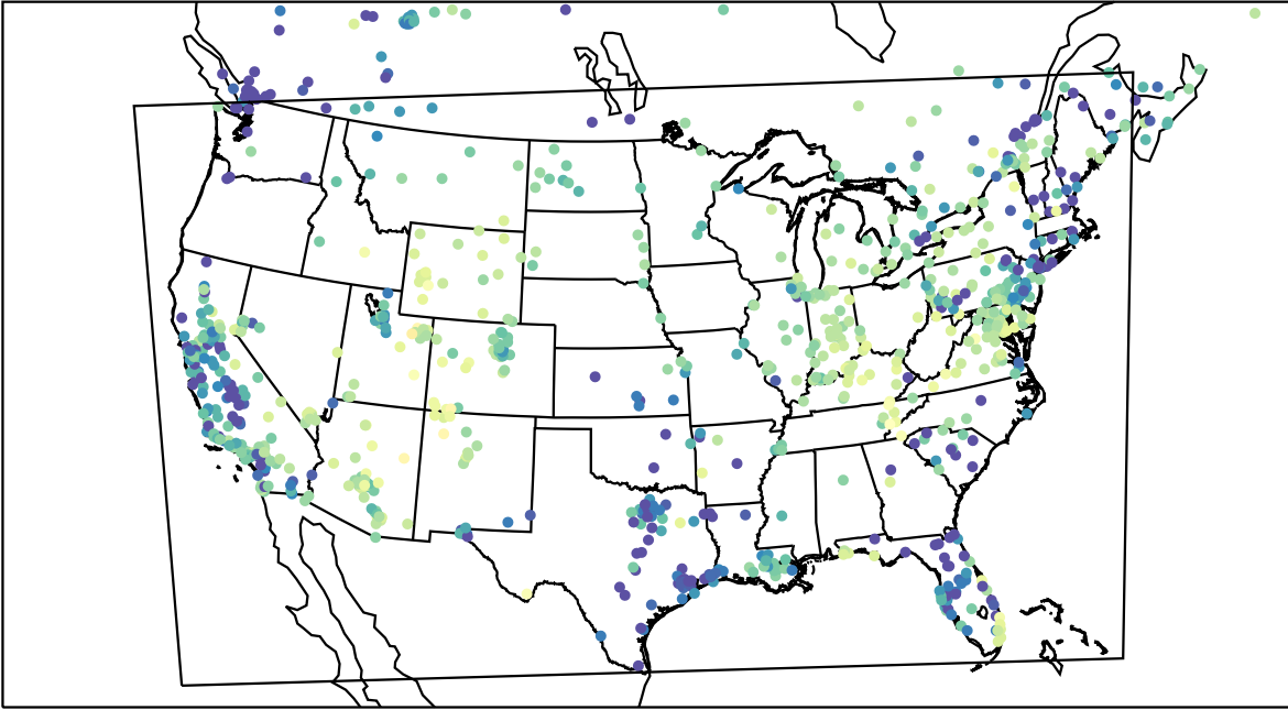
AirNOW (2023-02-15_08:00:00)
