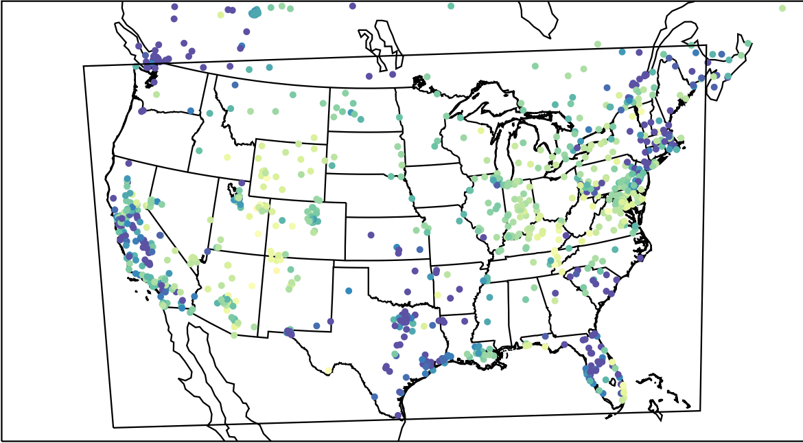
AirNOW (2023-02-15_09:00:00)
