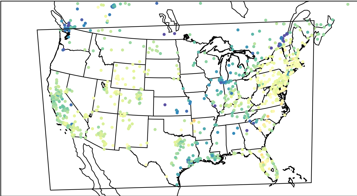
AirNOW (2023-02-15_22:00:00)
