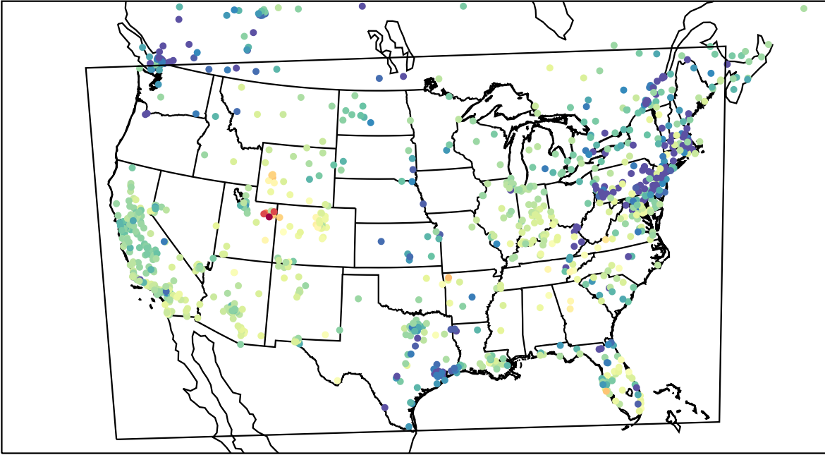
AirNOW (2023-02-15_01:00:00)
