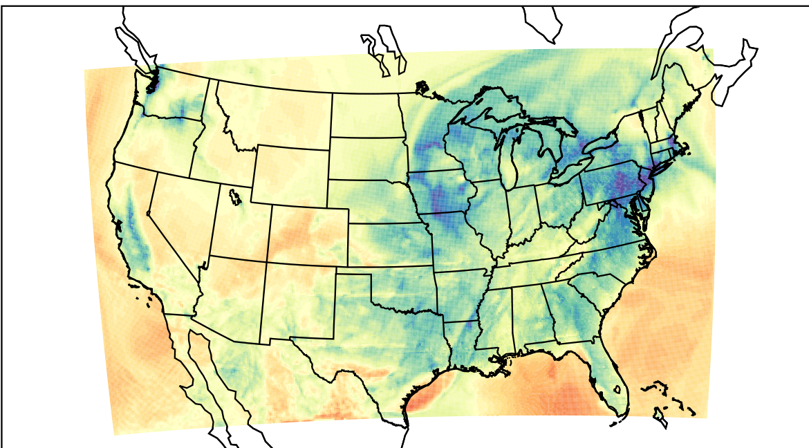
WRF (2023-02-15_05:00:00)
