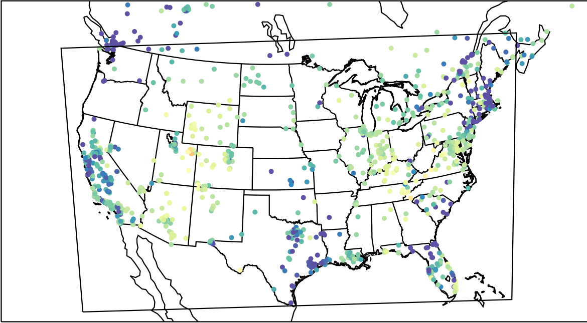
AirNOW (2023-02-15_06:00:00)
