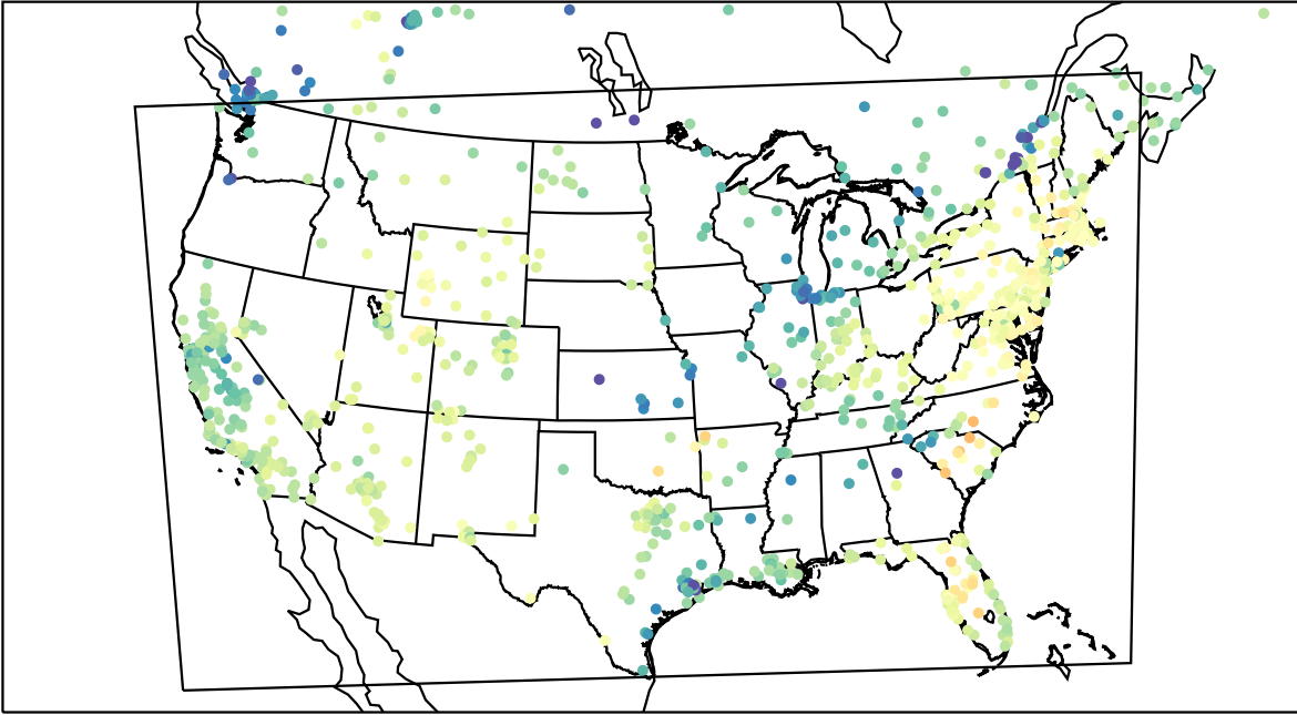
AirNOW (2023-02-15_21:00:00)
