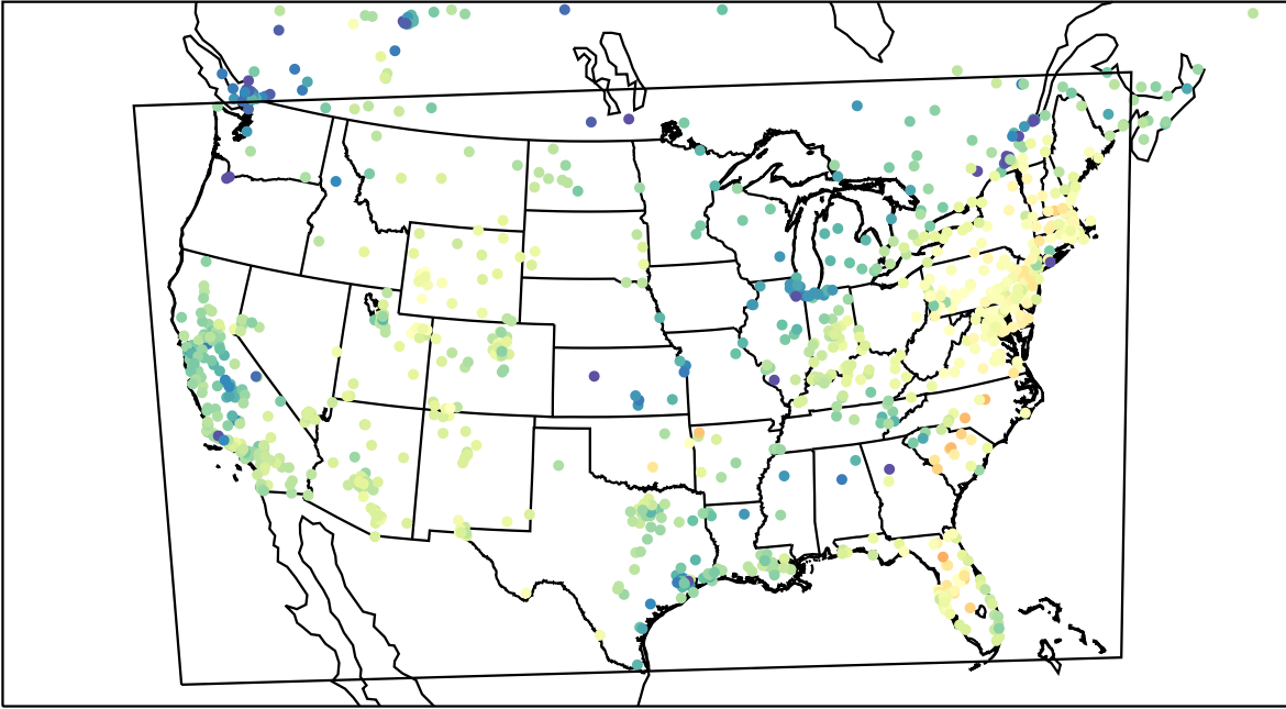
AirNOW (2023-02-15_20:00:00)
