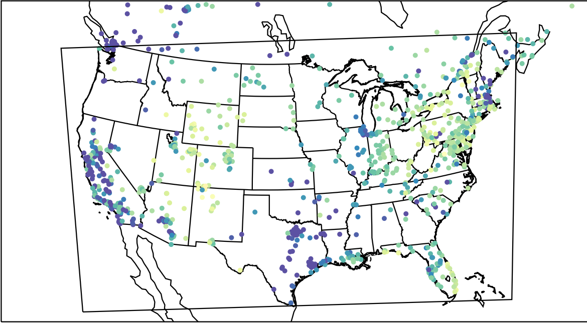
AirNOW (2023-02-15_14:00:00)
