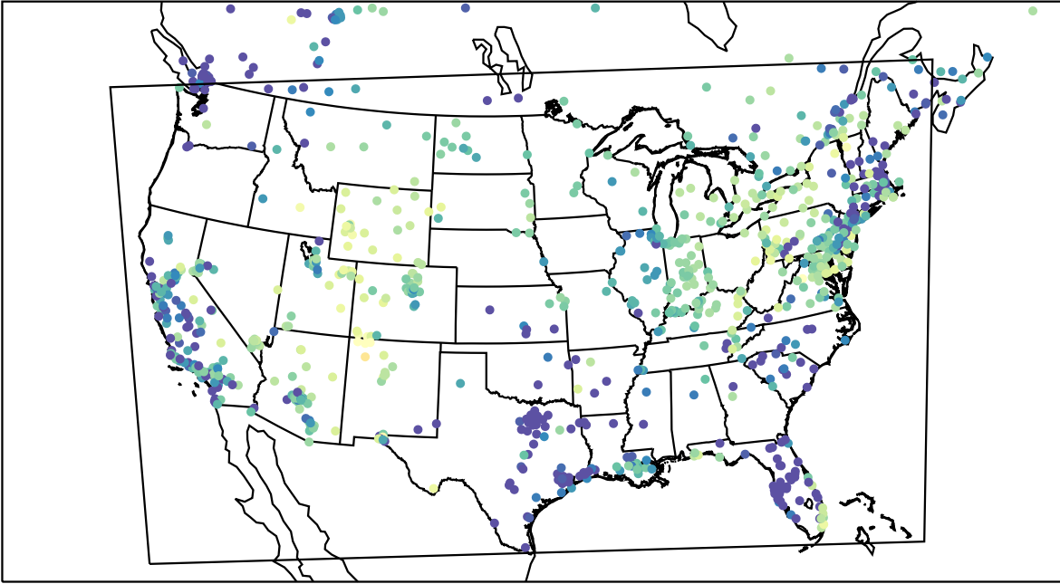
AirNOW (2023-02-15_12:00:00)
