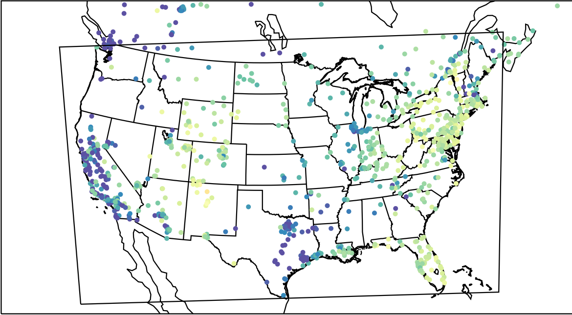
AirNOW (2023-02-15_15:00:00)
