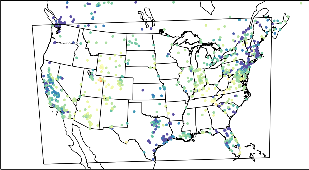
AirNOW (2023-02-15_05:00:00)
