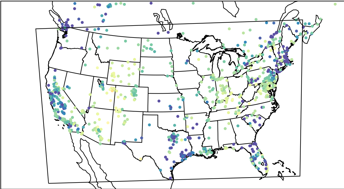
AirNOW (2023-02-15_07:00:00)
