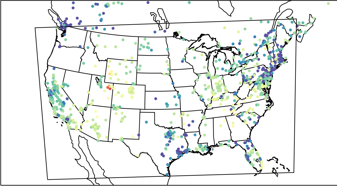
AirNOW (2023-02-15_03:00:00)
