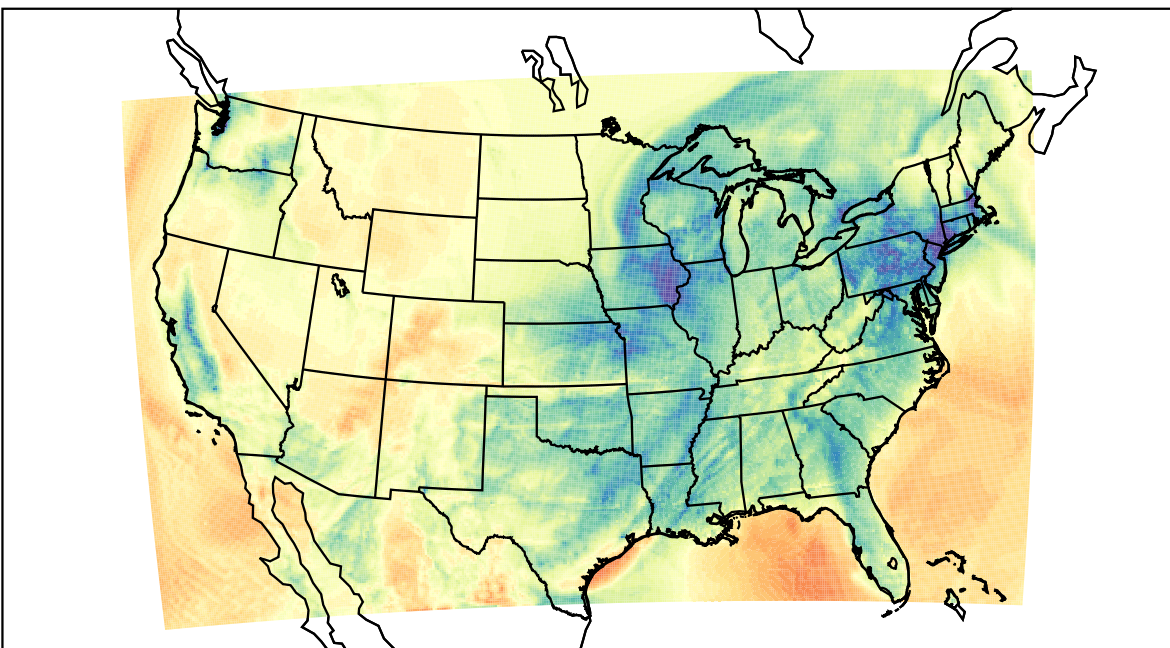
WRF (2023-02-15_08:00:00)
