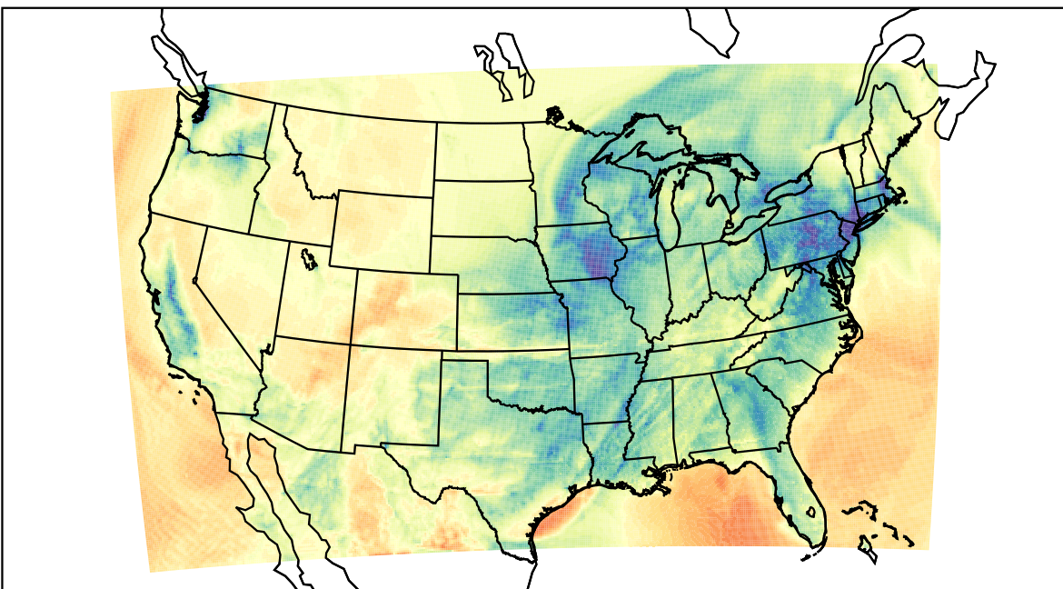
WRF (2023-02-15_07:00:00)
