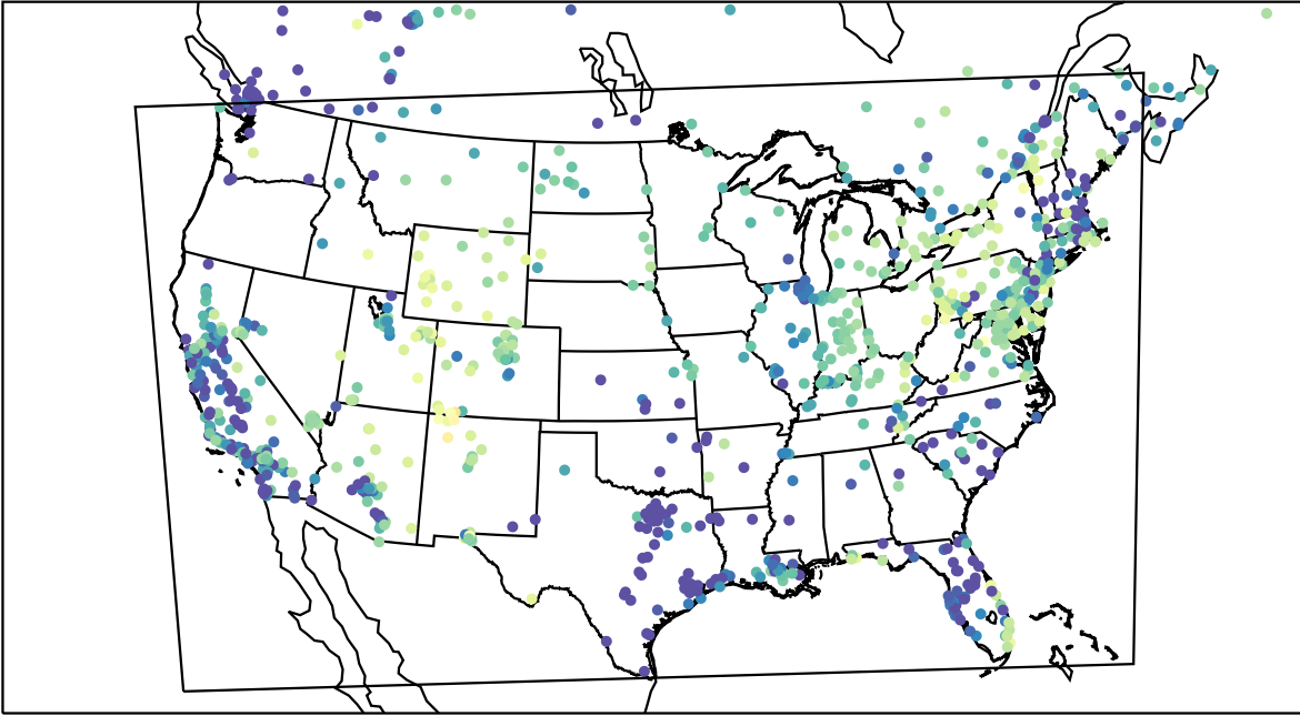
AirNOW (2023-02-15_13:00:00)
