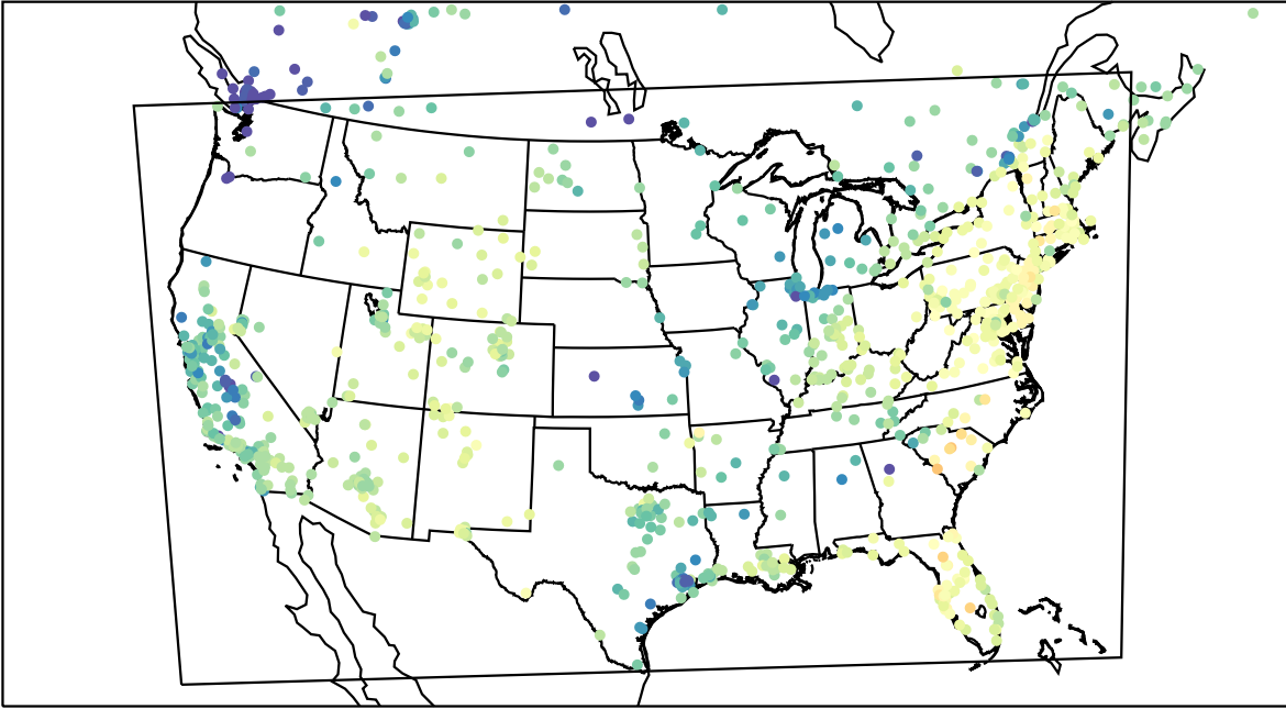
AirNOW (2023-02-15_18:00:00)
