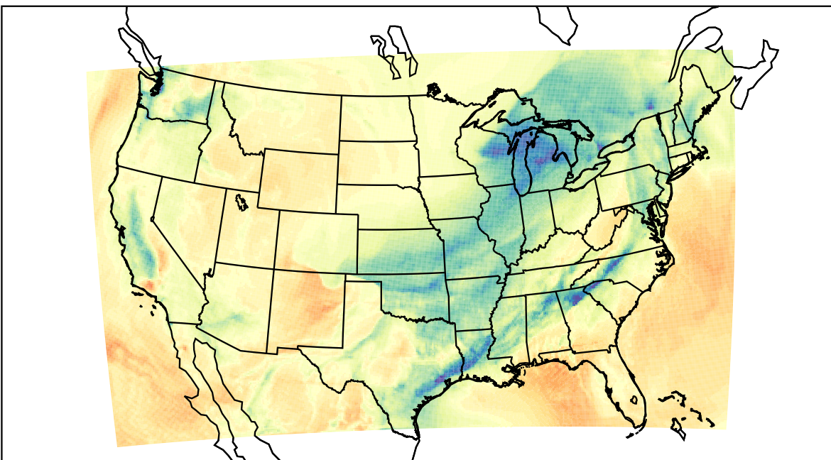
WRF (2023-02-15_17:00:00)
