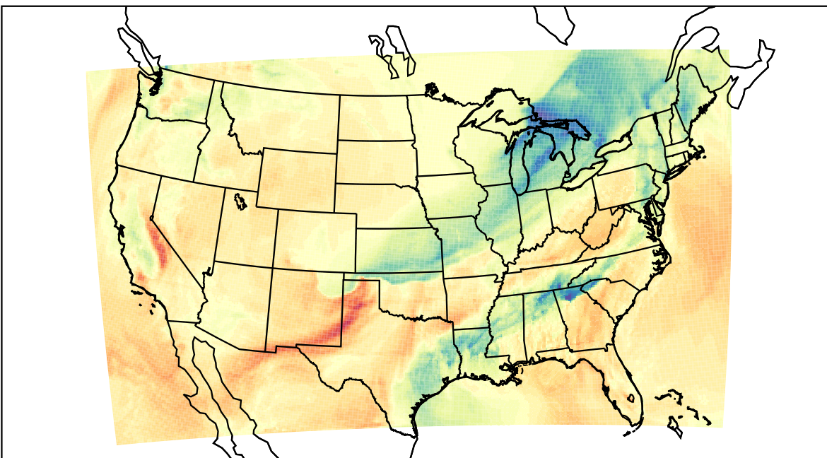
WRF (2023-02-15_21:00:00)
