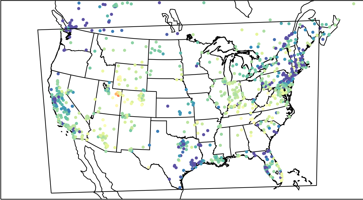
AirNOW (2023-02-15_04:00:00)
