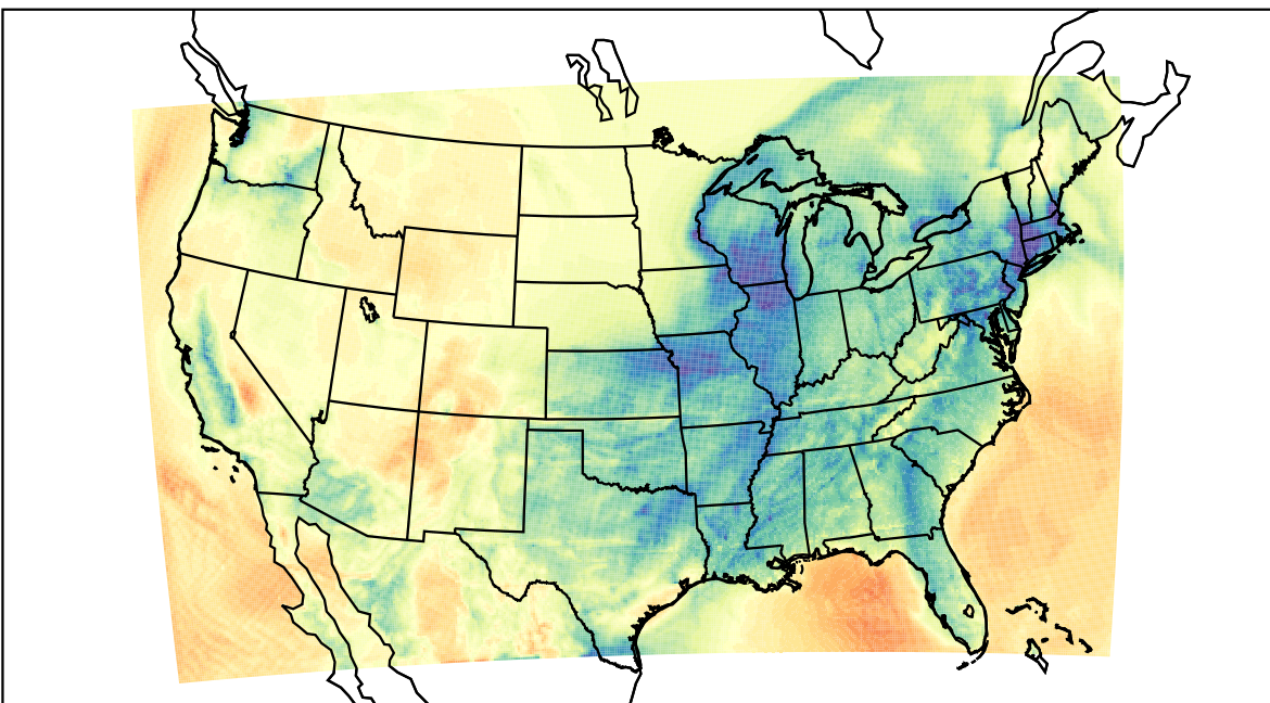
WRF (2023-02-15_11:00:00)
