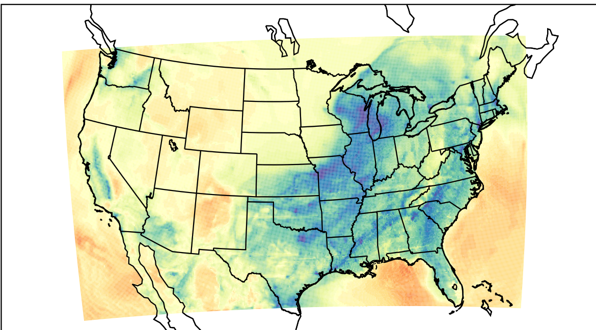
WRF (2023-02-15_14:00:00)
