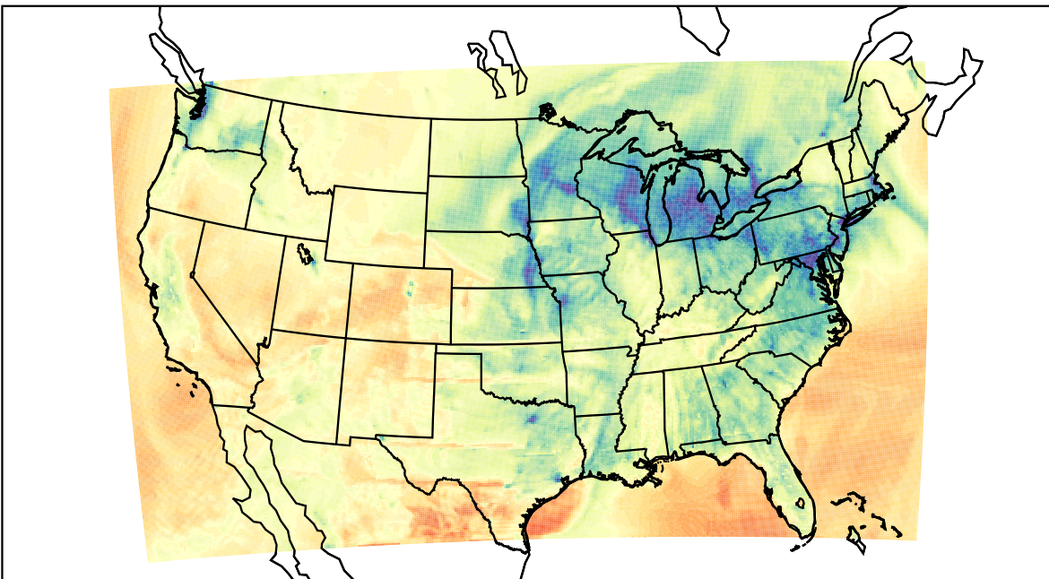
WRF (2023-02-15_01:00:00)
