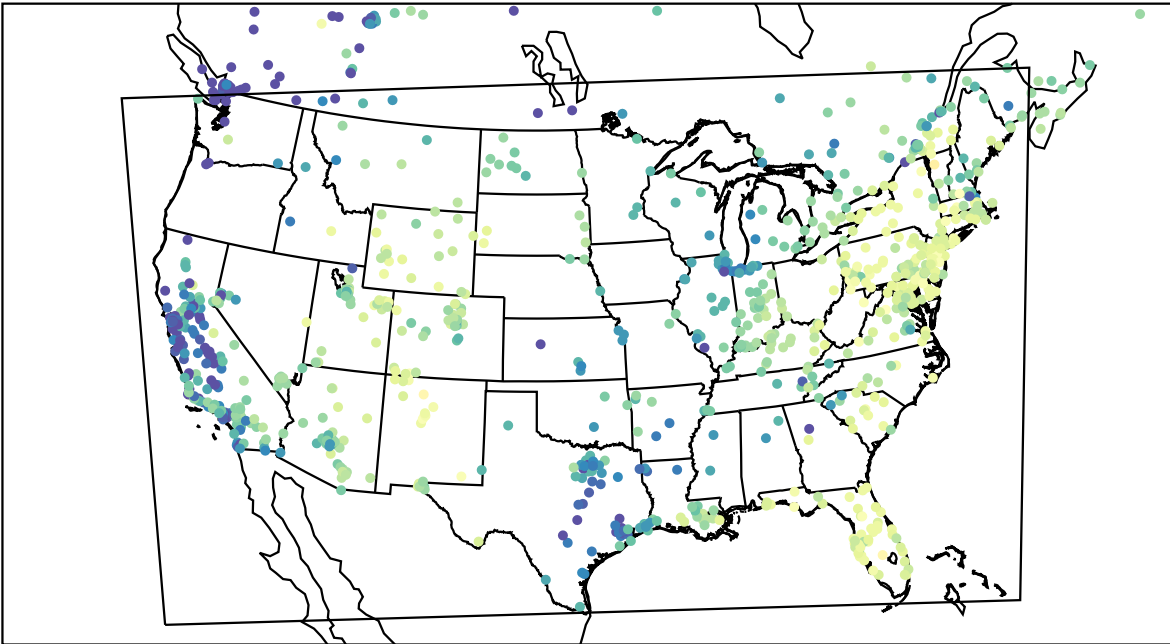
AirNOW (2023-02-15_16:00:00)
