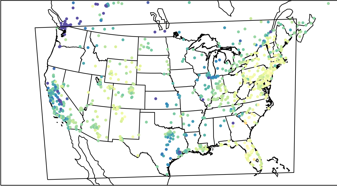
AirNOW (2023-02-15_17:00:00)
