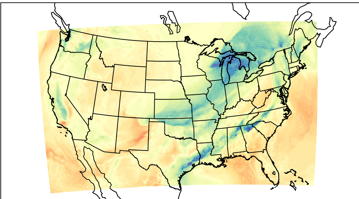
WRF (2023-02-15_18:00:00)
