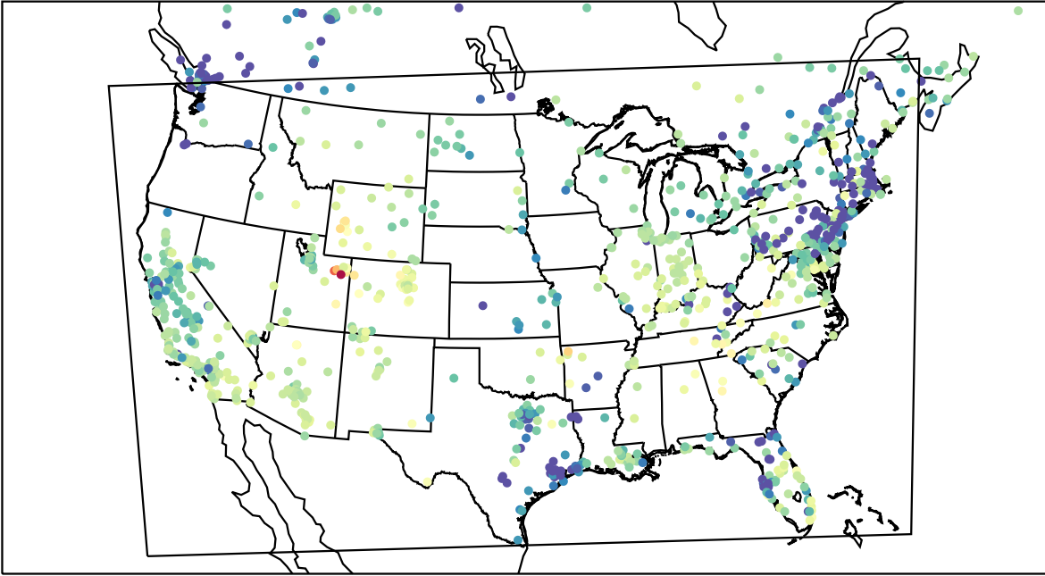
AirNOW (2023-02-15_02:00:00)
