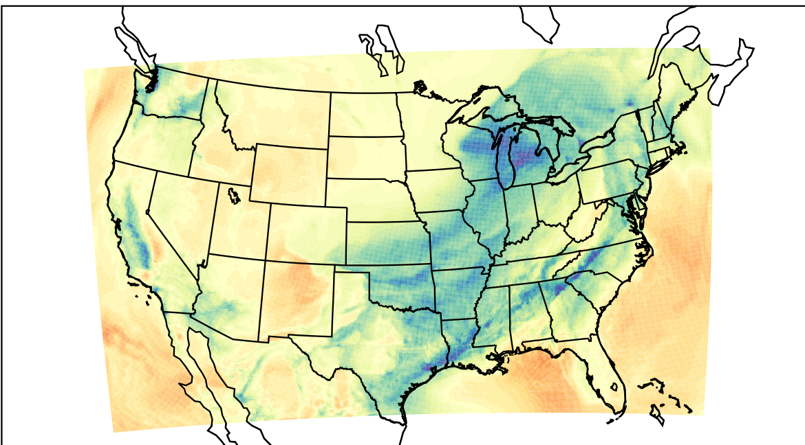
WRF (2023-02-15_16:00:00)
