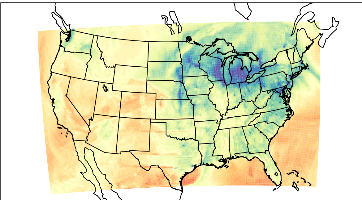
WRF (2023-02-15_00:00:00)
