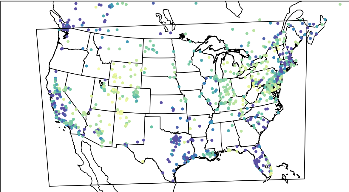
AirNOW (2023-02-15_11:00:00)
