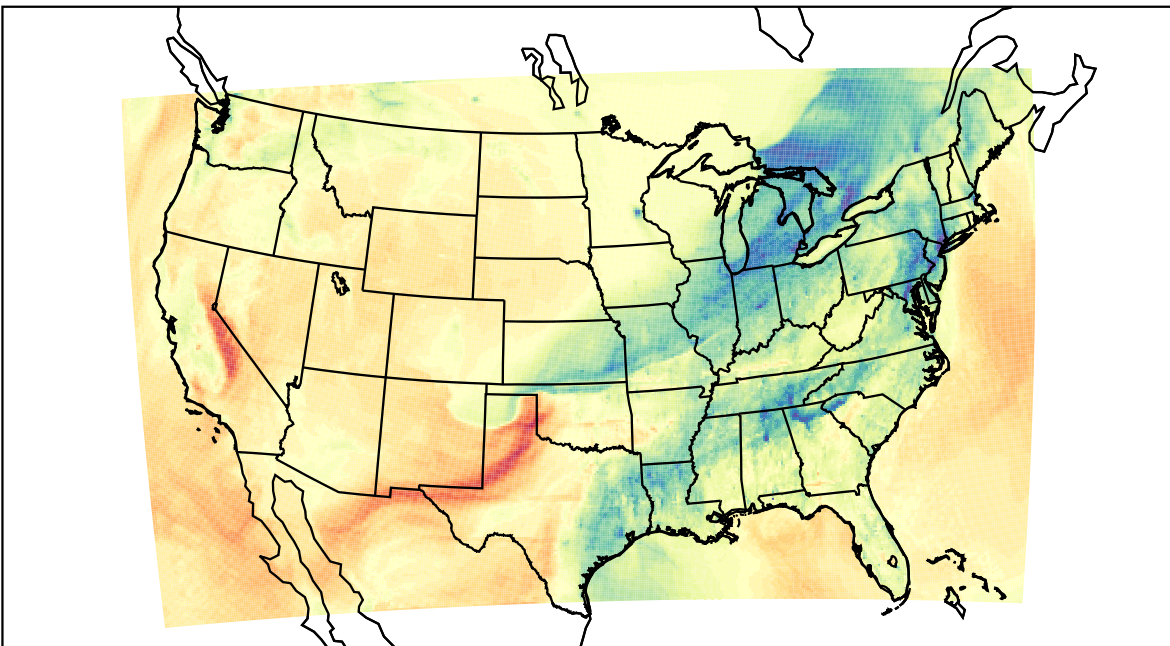
WRF (2023-02-15_23:00:00)
