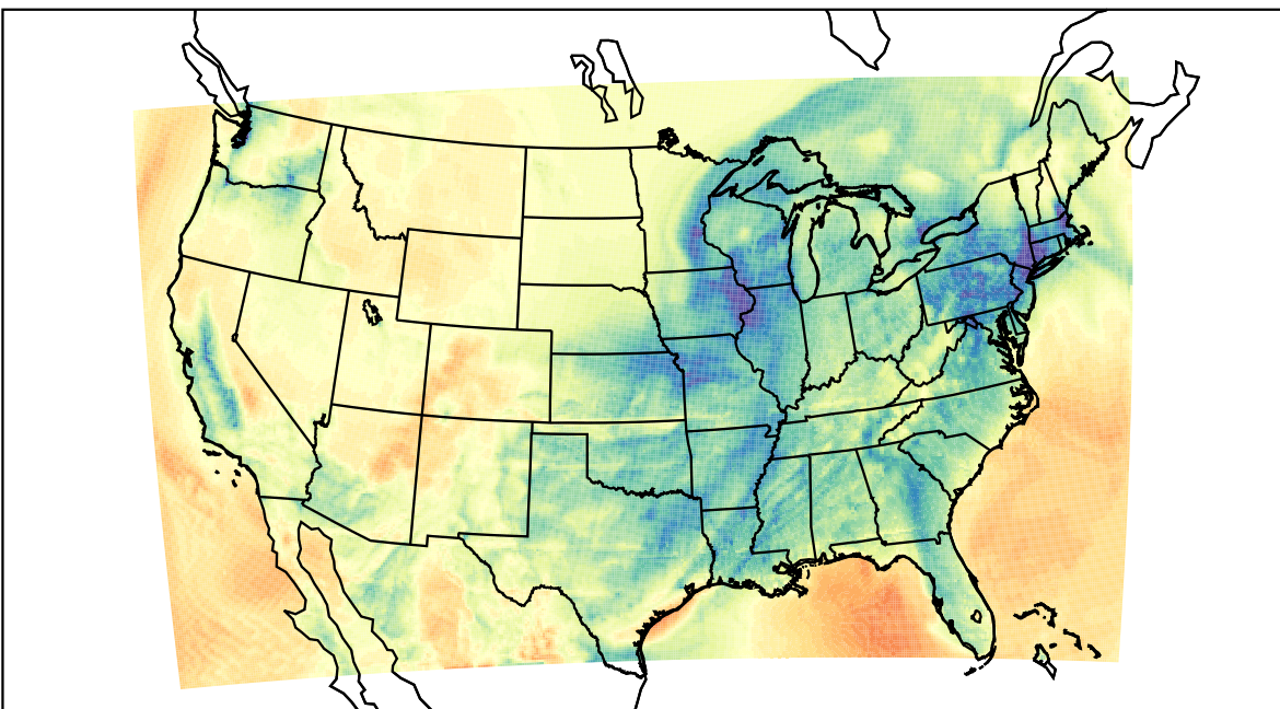
WRF (2023-02-15_09:00:00)
