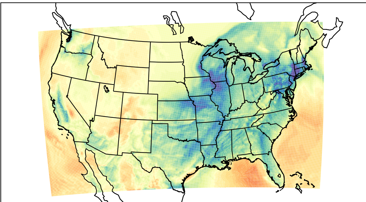
WRF (2023-02-15_10:00:00)
