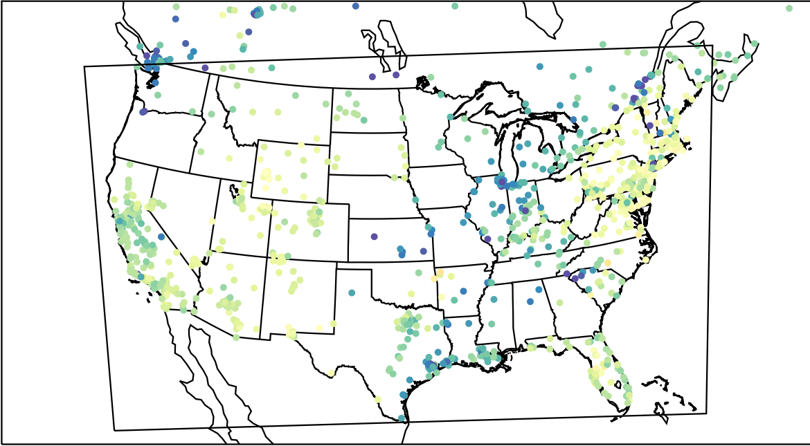
AirNOW (2023-02-15_23:00:00)
