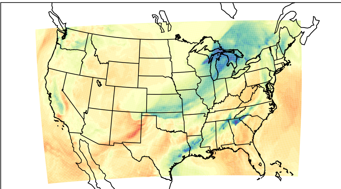
WRF (2023-02-15_19:00:00)
