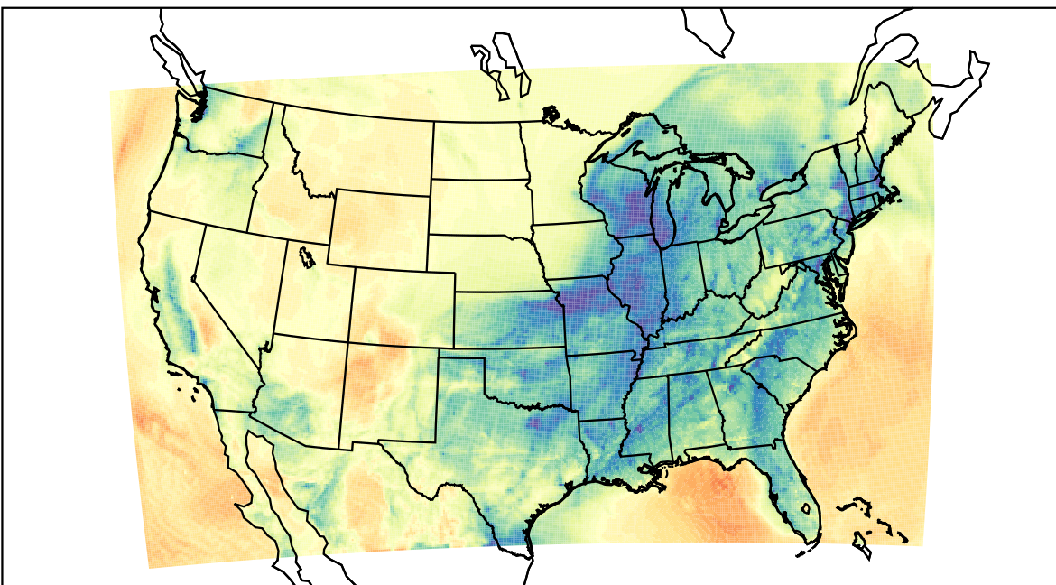
WRF (2023-02-15_13:00:00)
