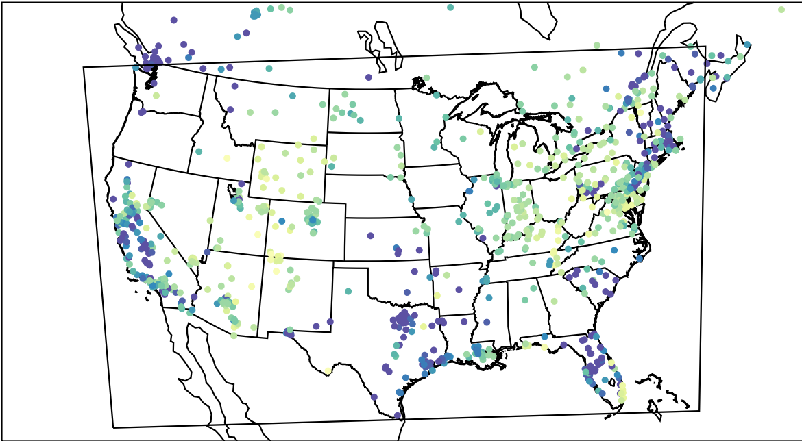
AirNOW (2023-02-15_10:00:00)
