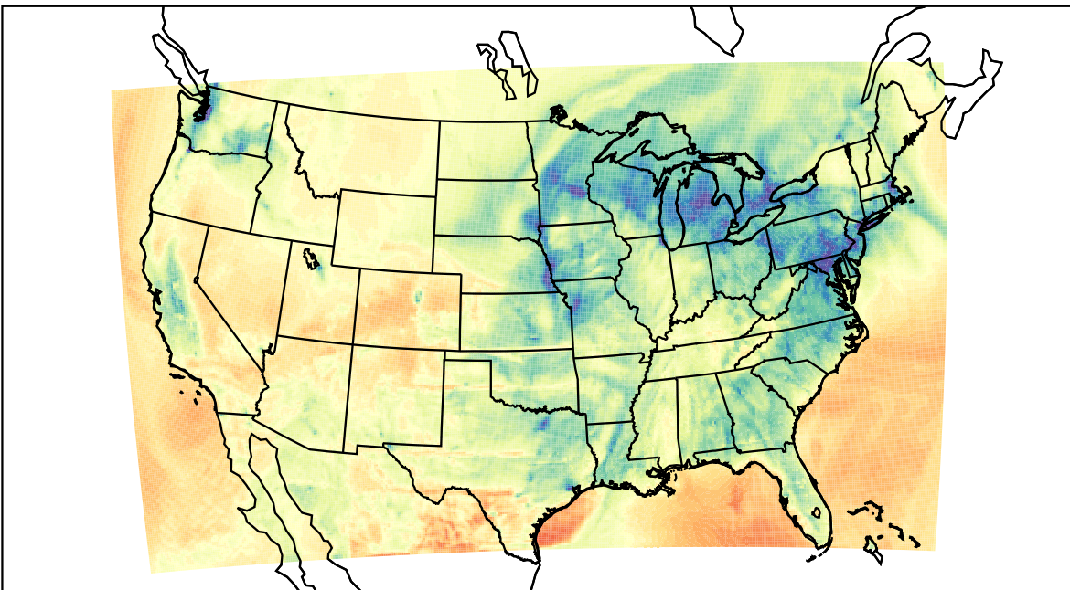
WRF (2023-02-15_02:00:00)
