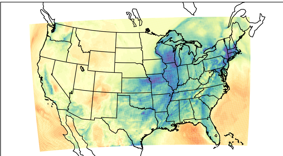
WRF (2023-02-15_12:00:00)
