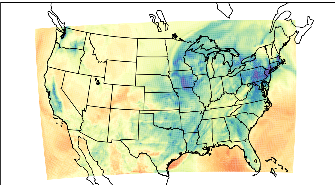
WRF (2023-02-15_06:00:00)
