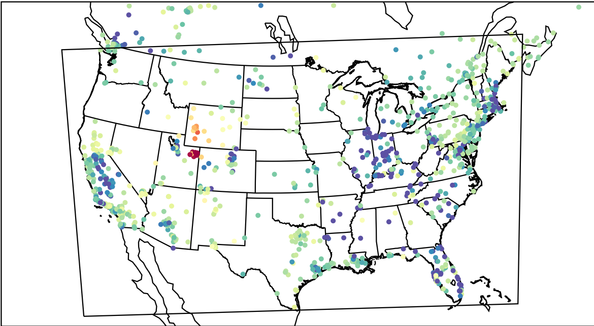
AirNOW (2023-02-14_03:00:00)
