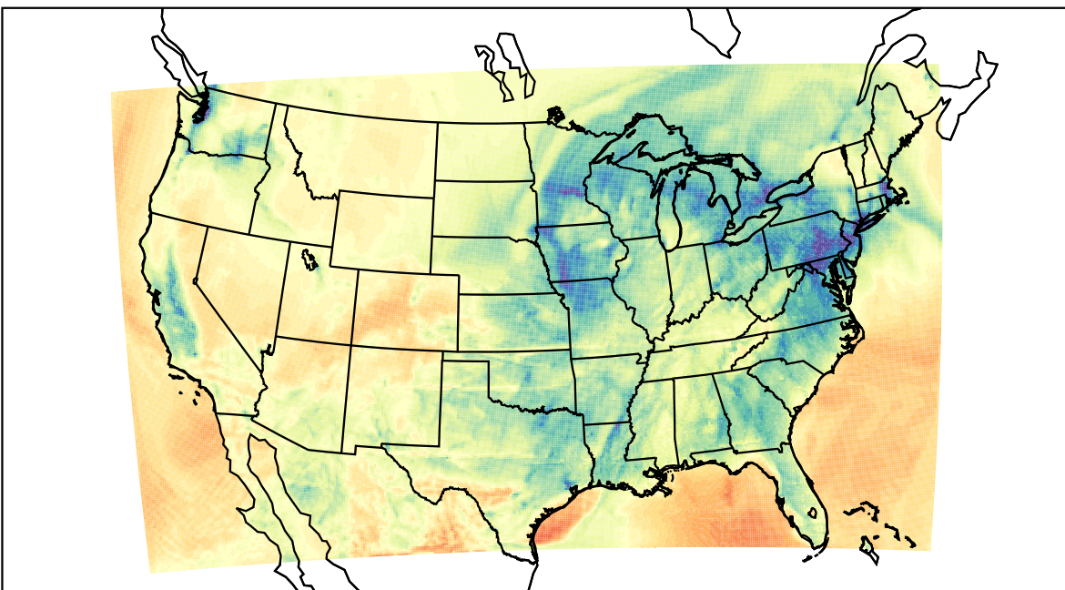
WRF (2023-02-15_04:00:00)
