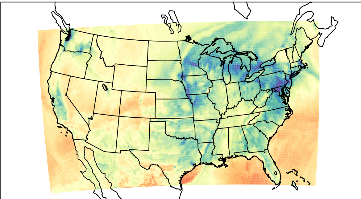
WRF (2023-02-15_03:00:00)
