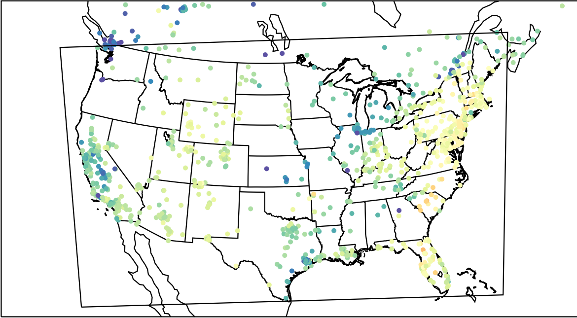
AirNOW (2023-02-15_19:00:00)
