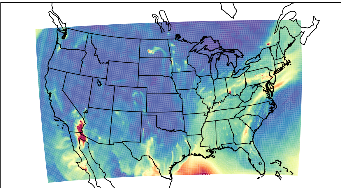
WRF 2023-02-16_14:00:00
