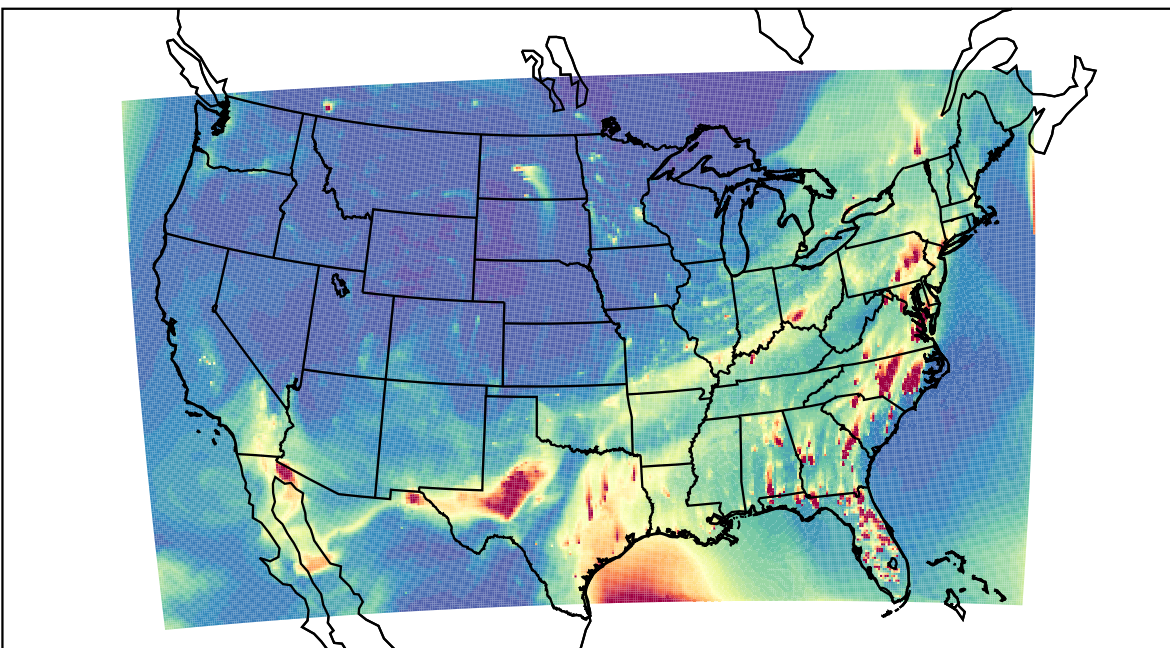
WRF 2023-02-16_00:00:00
