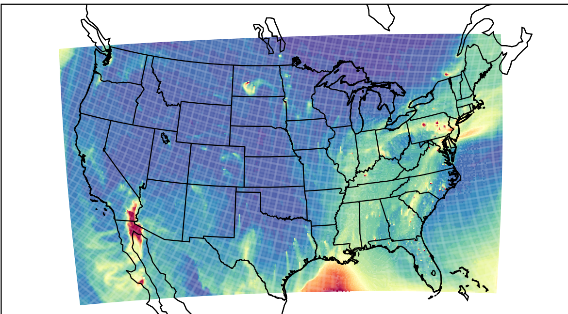
WRF 2023-02-16_17:00:00
