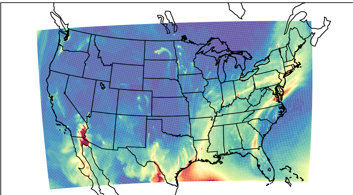
WRF 2023-02-16_11:00:00
