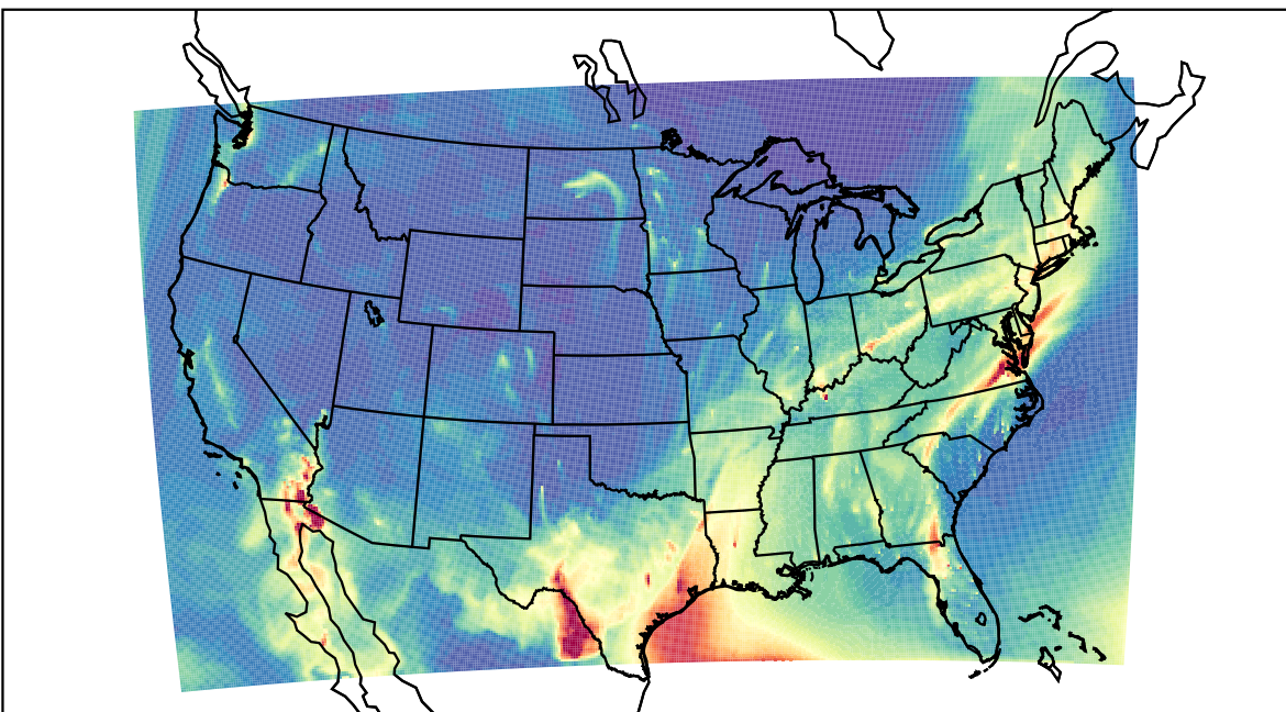
WRF 2023-02-16_08:00:00
