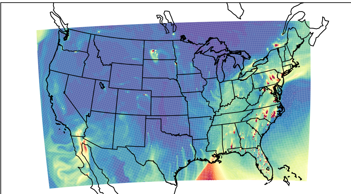
WRF 2023-02-16_21:00:00
