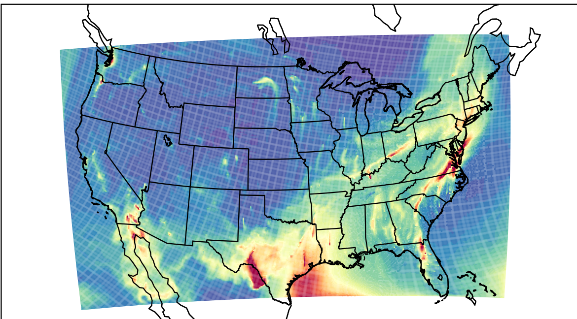
WRF 2023-02-16_06:00:00
