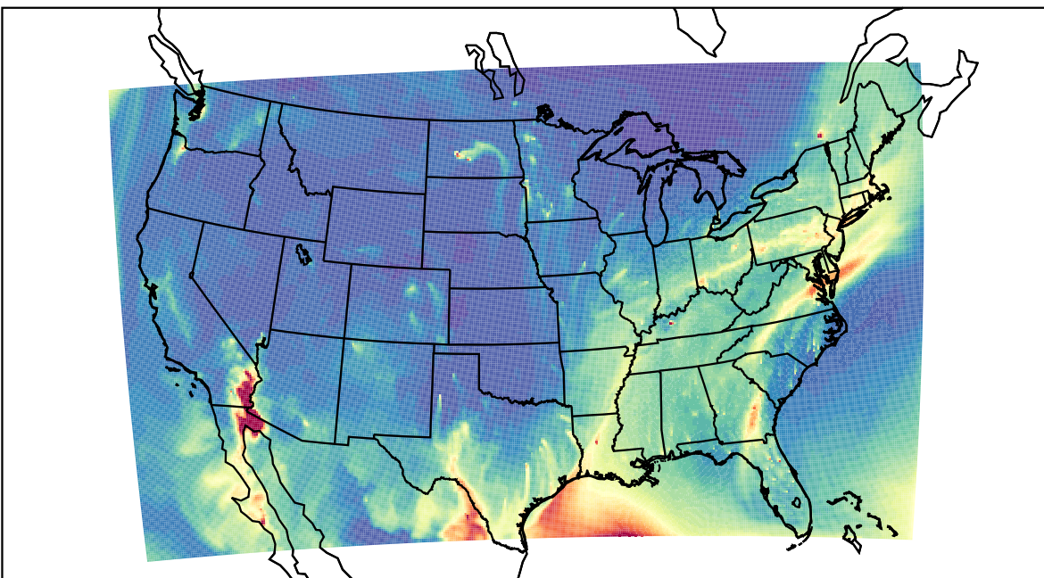
WRF 2023-02-16_12:00:00
