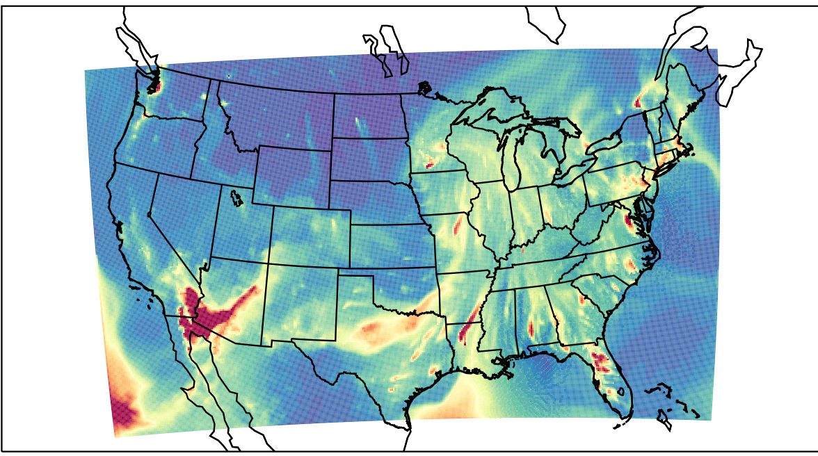
WRF 2023-02-15_04:00:00
