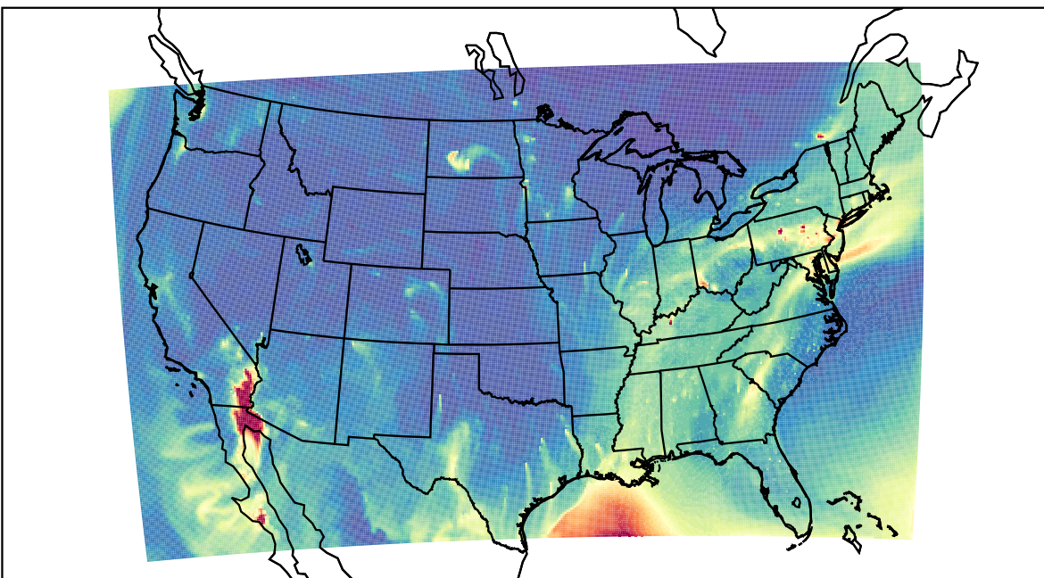
WRF 2023-02-16_16:00:00
