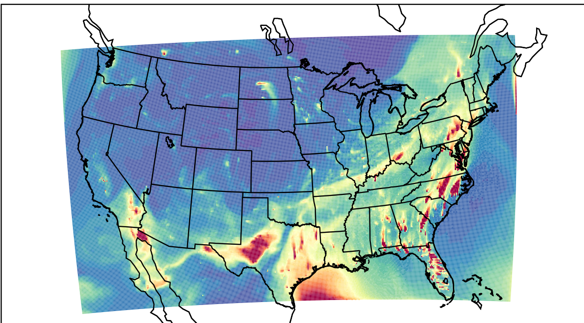
WRF 2023-02-16_01:00:00
