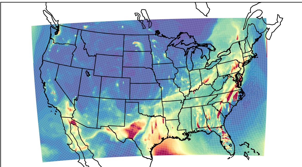
WRF 2023-02-16_02:00:00
