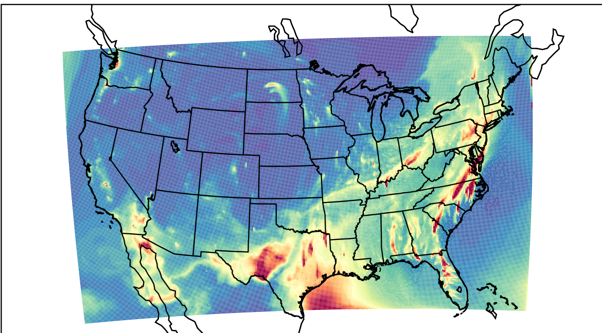
WRF 2023-02-16_03:00:00
