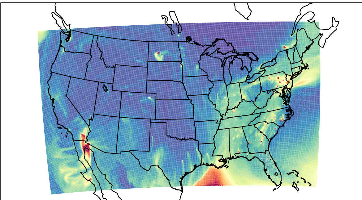
WRF 2023-02-16_18:00:00
