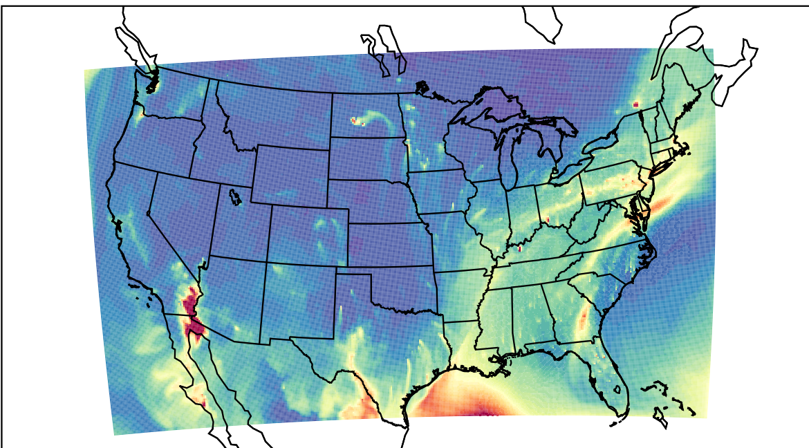
WRF 2023-02-16_13:00:00
