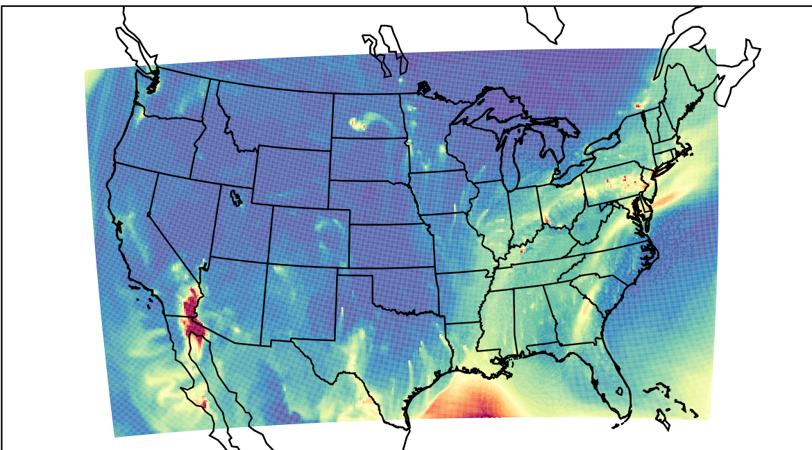
WRF 2023-02-16_15:00:00
