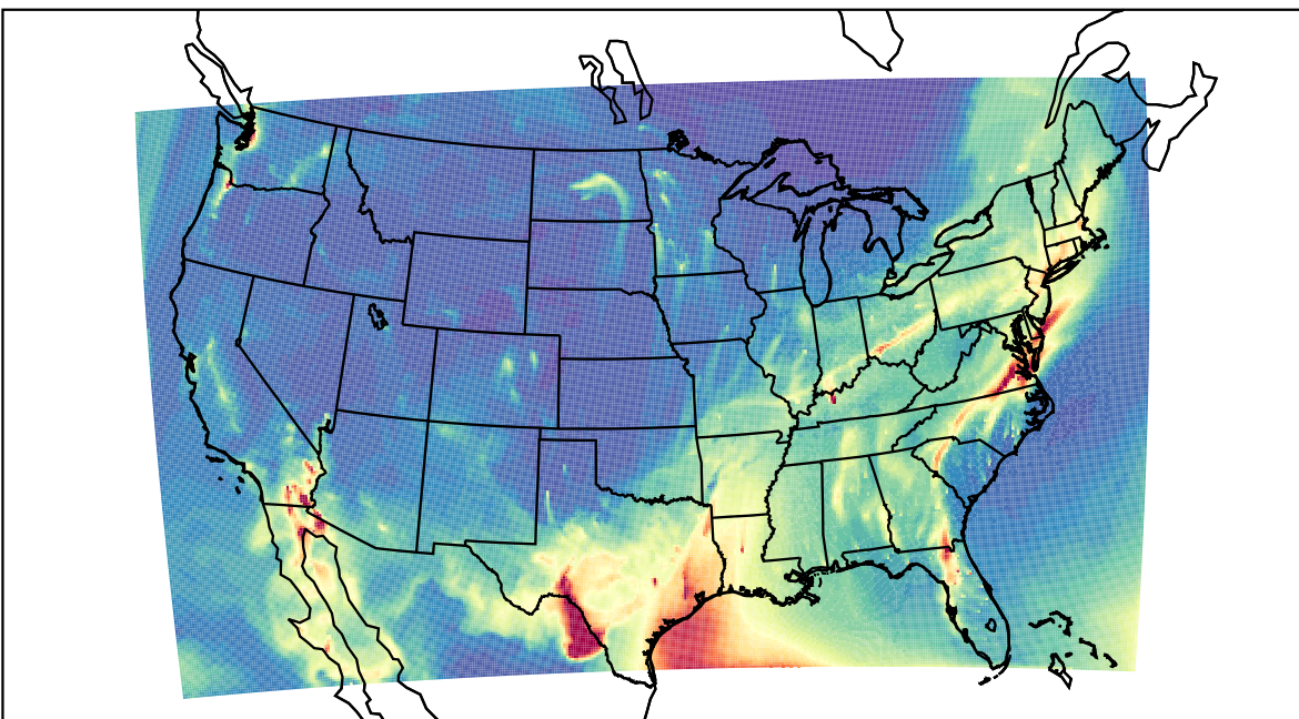
WRF 2023-02-16_07:00:00
