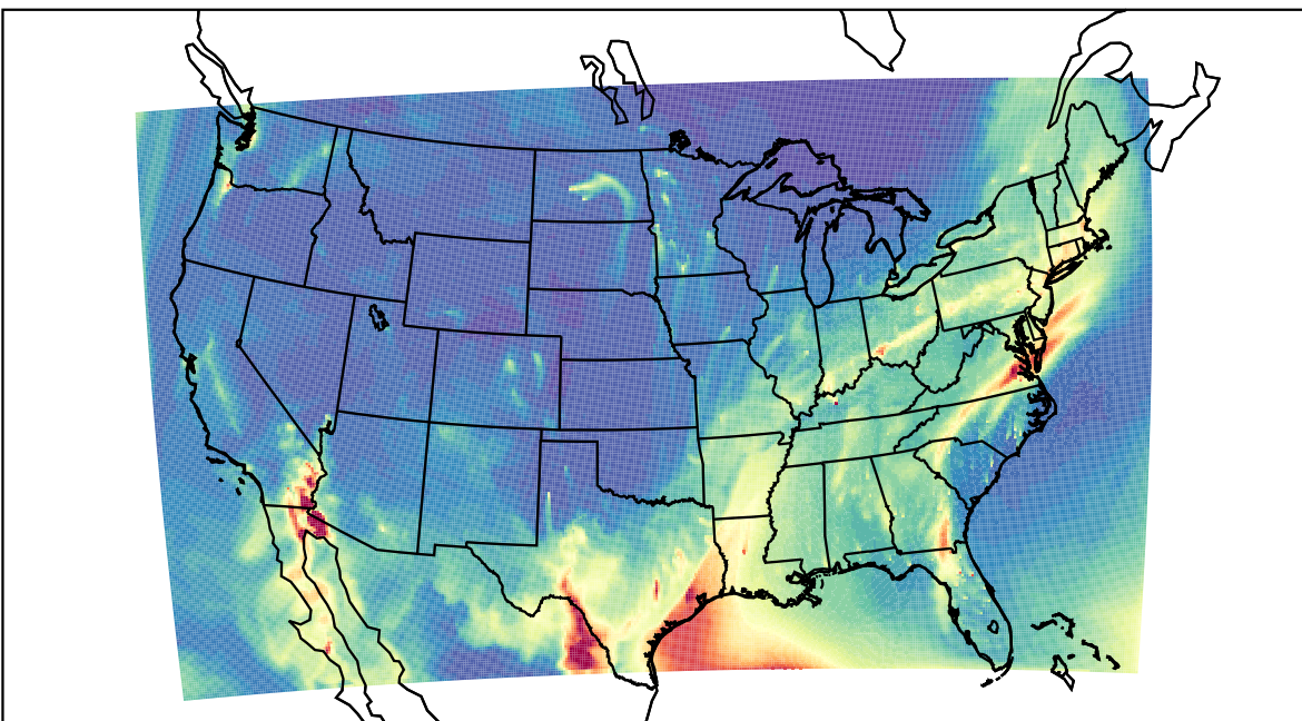
WRF 2023-02-16_09:00:00
