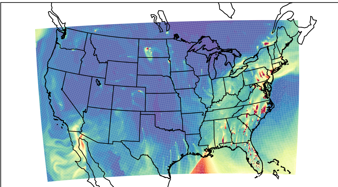
WRF 2023-02-16_22:00:00
