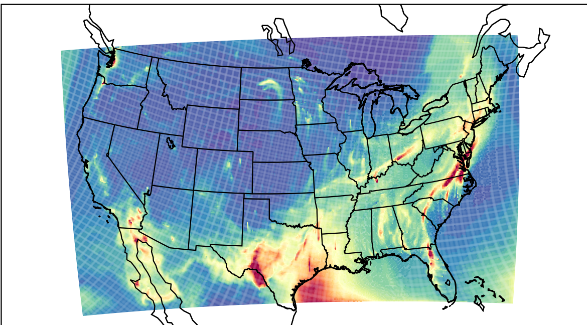
WRF 2023-02-16_05:00:00
