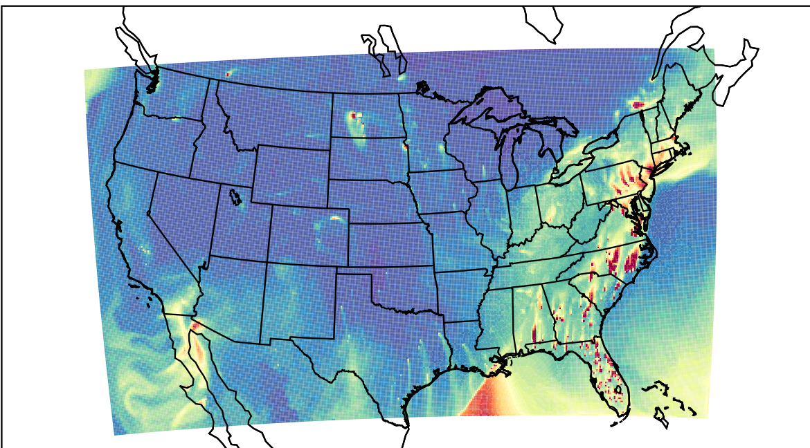
WRF 2023-02-16_23:00:00
