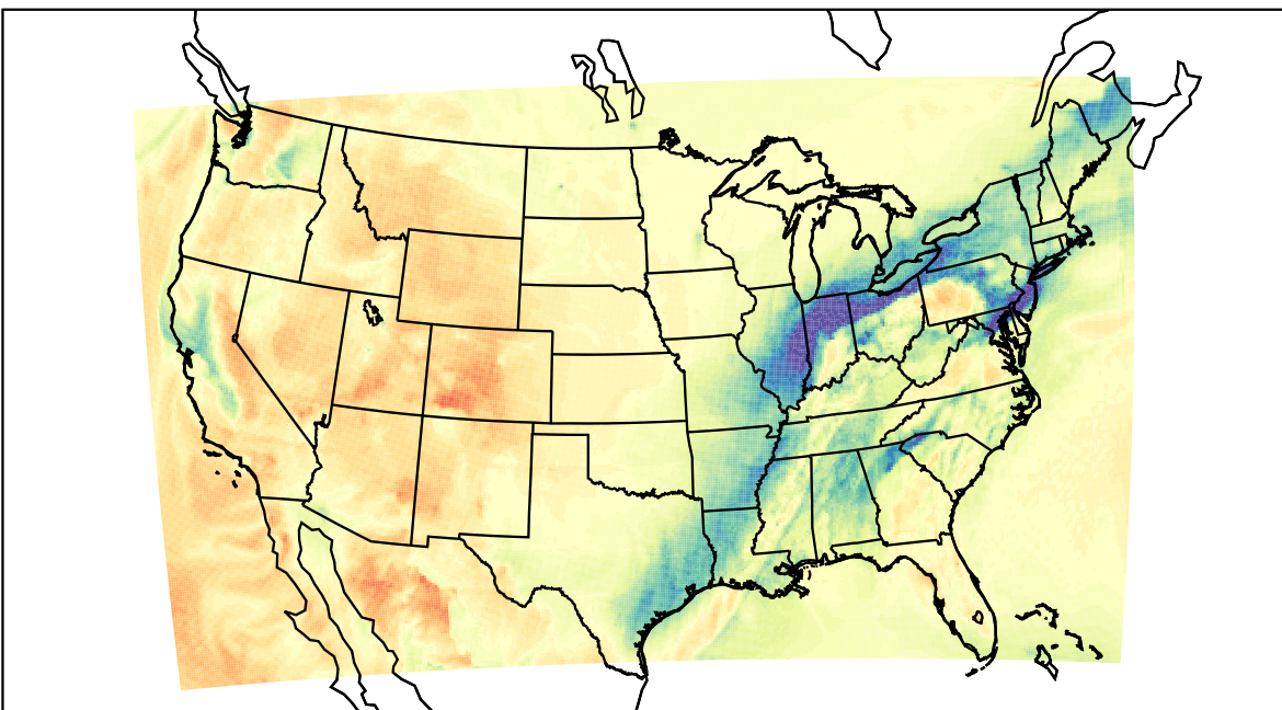
WRF (2023-02-16_19:00:00)
