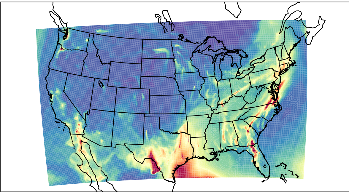
WRF 2023-02-16_06:00:00
