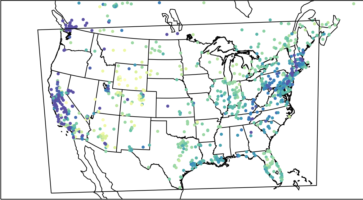
AirNOW (2023-02-17_16:00:00)
