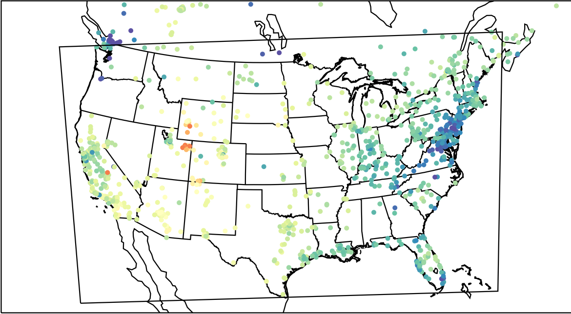
AirNOW (2023-02-17_21:00:00)
