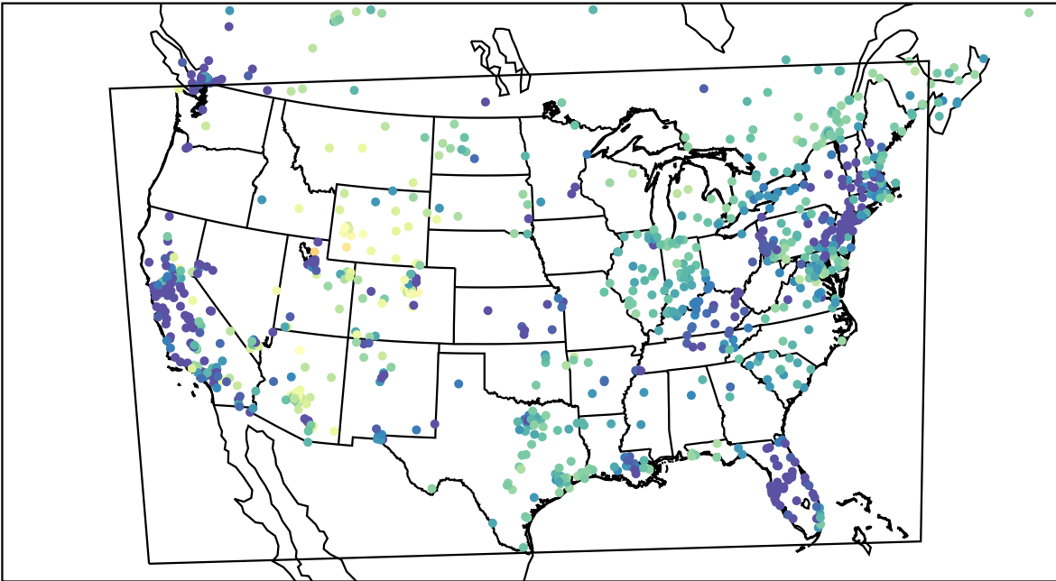
AirNOW (2023-02-17_10:00:00)
