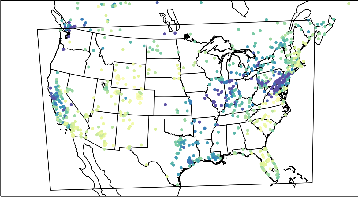
AirNOW (2023-02-16_19:00:00)
