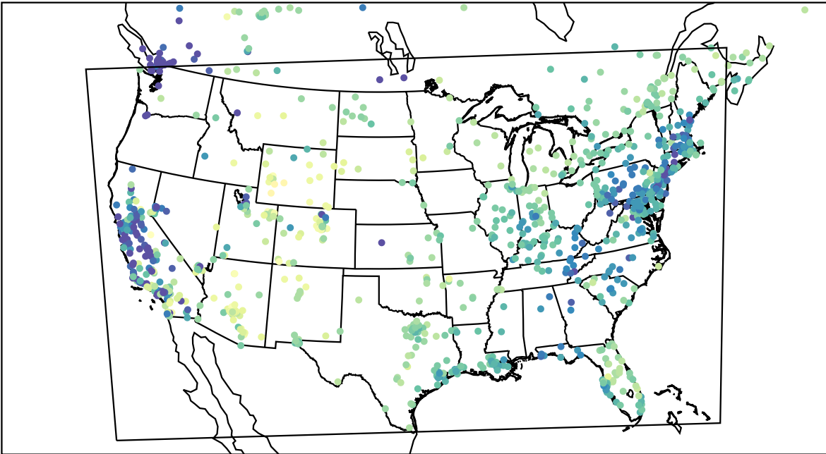
AirNOW (2023-02-17_17:00:00)
