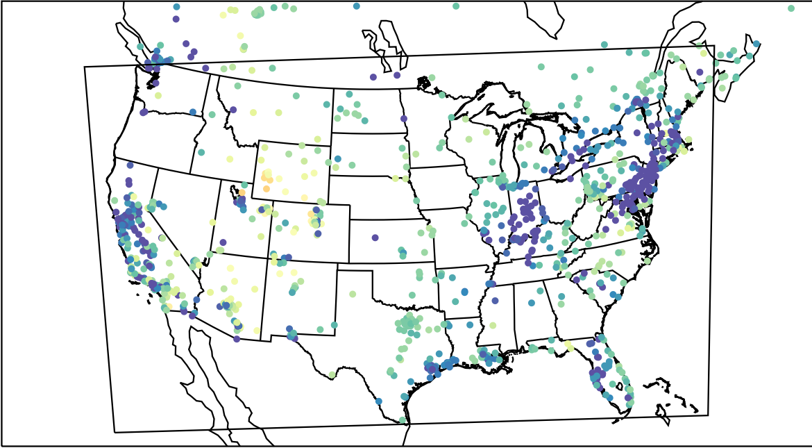
AirNOW (2023-02-17_02:00:00)
