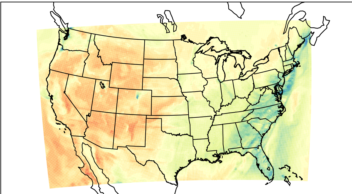
WRF (2023-02-17_22:00:00)
