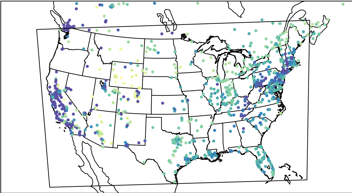
AirNOW (2023-02-17_15:00:00)
