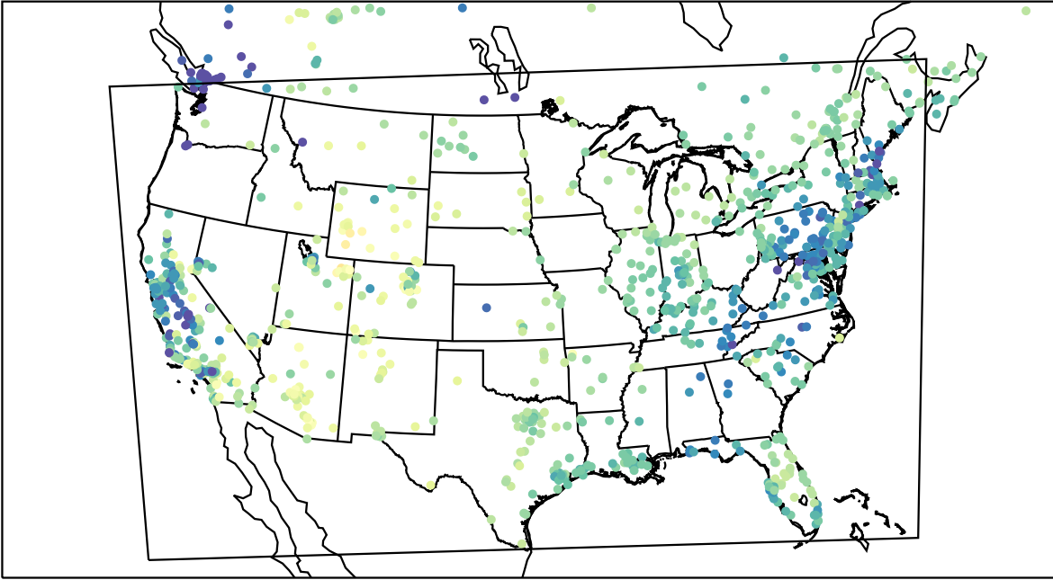
AirNOW (2023-02-17_18:00:00)
