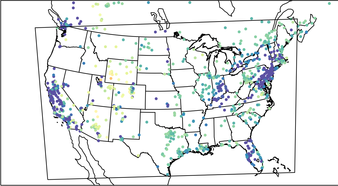
AirNOW (2023-02-17_05:00:00)
