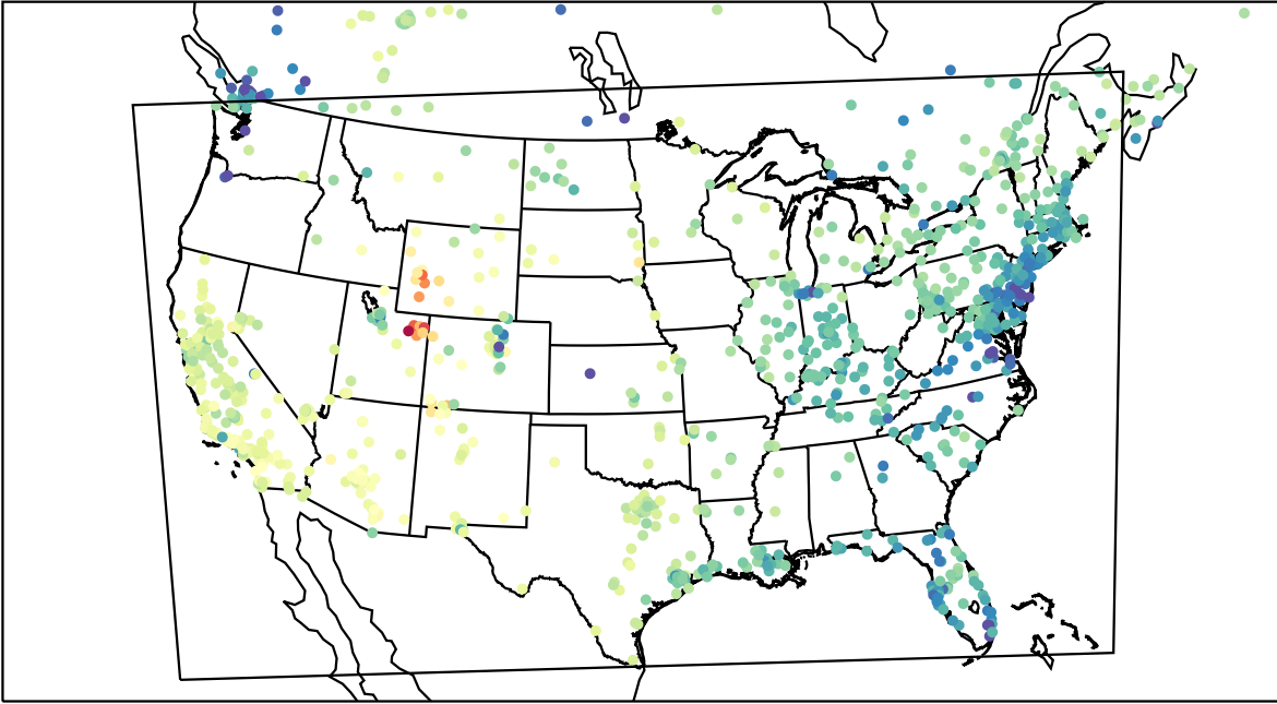
AirNOW (2023-02-17_23:00:00)
