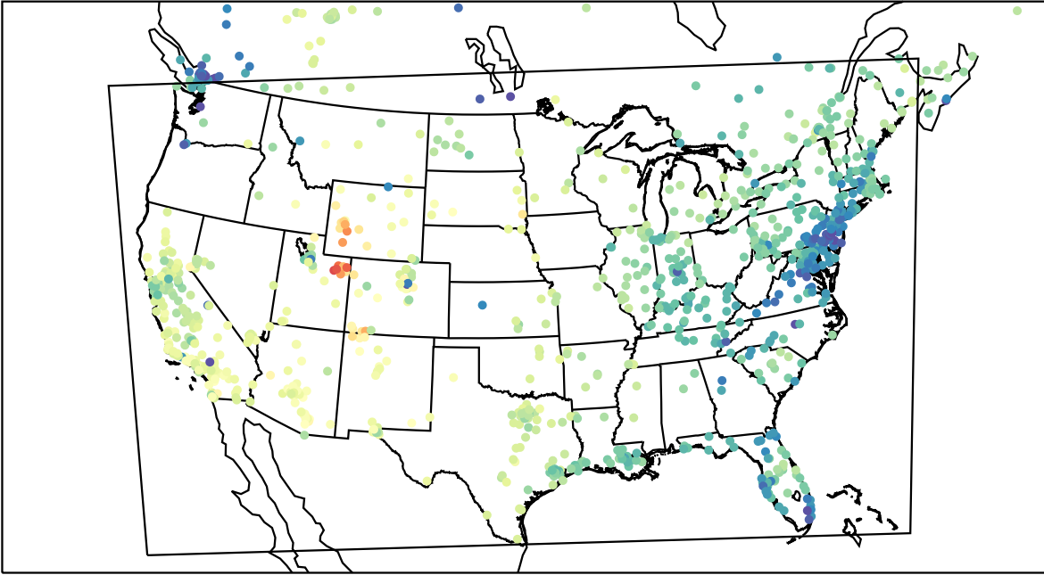
AirNOW (2023-02-17_22:00:00)
