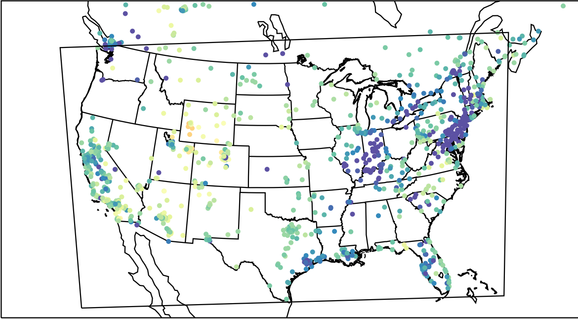
AirNOW (2023-02-17_01:00:00)
