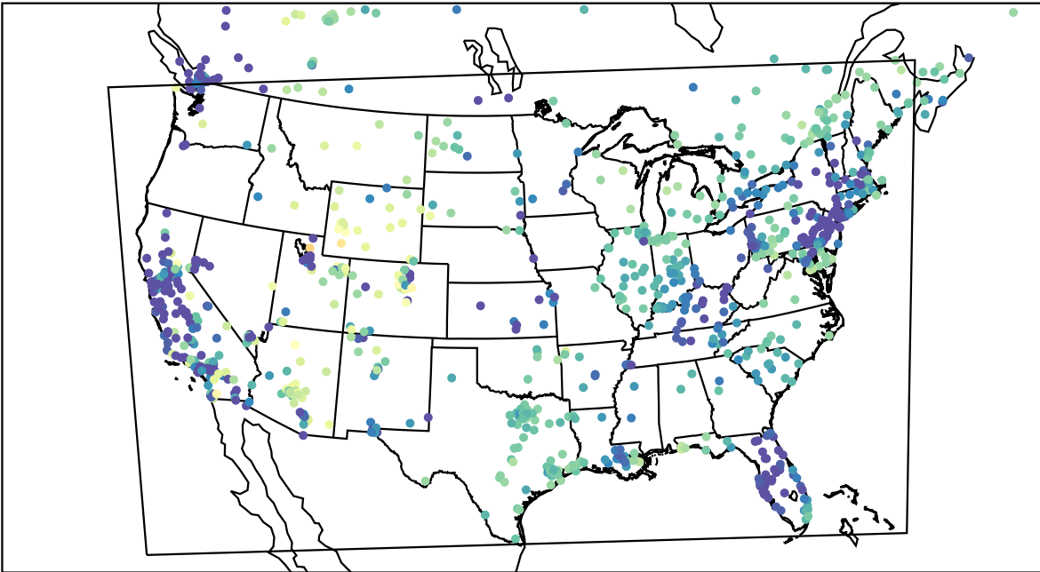
AirNOW (2023-02-17_09:00:00)
