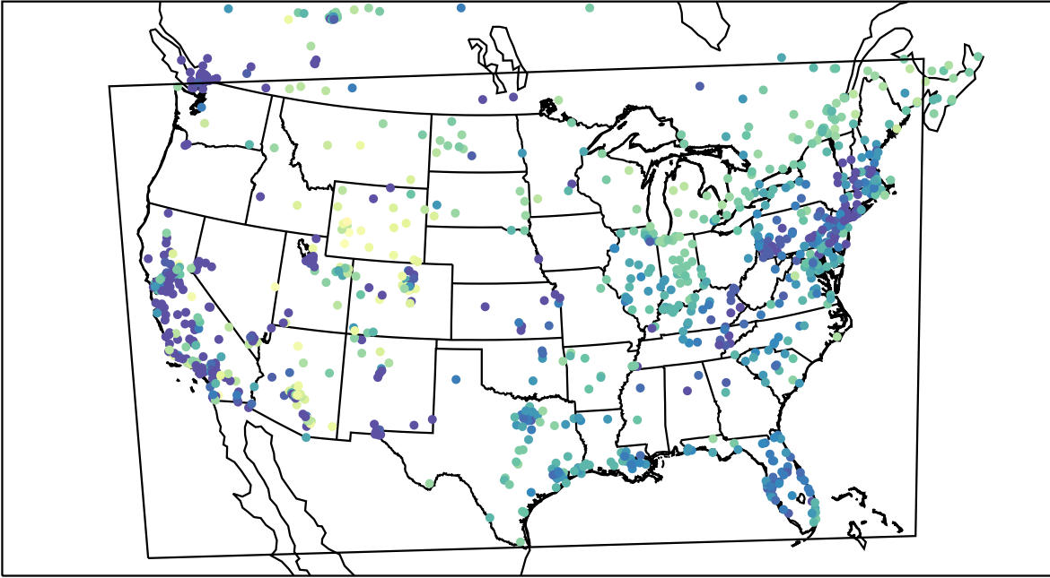
AirNOW (2023-02-17_14:00:00)
