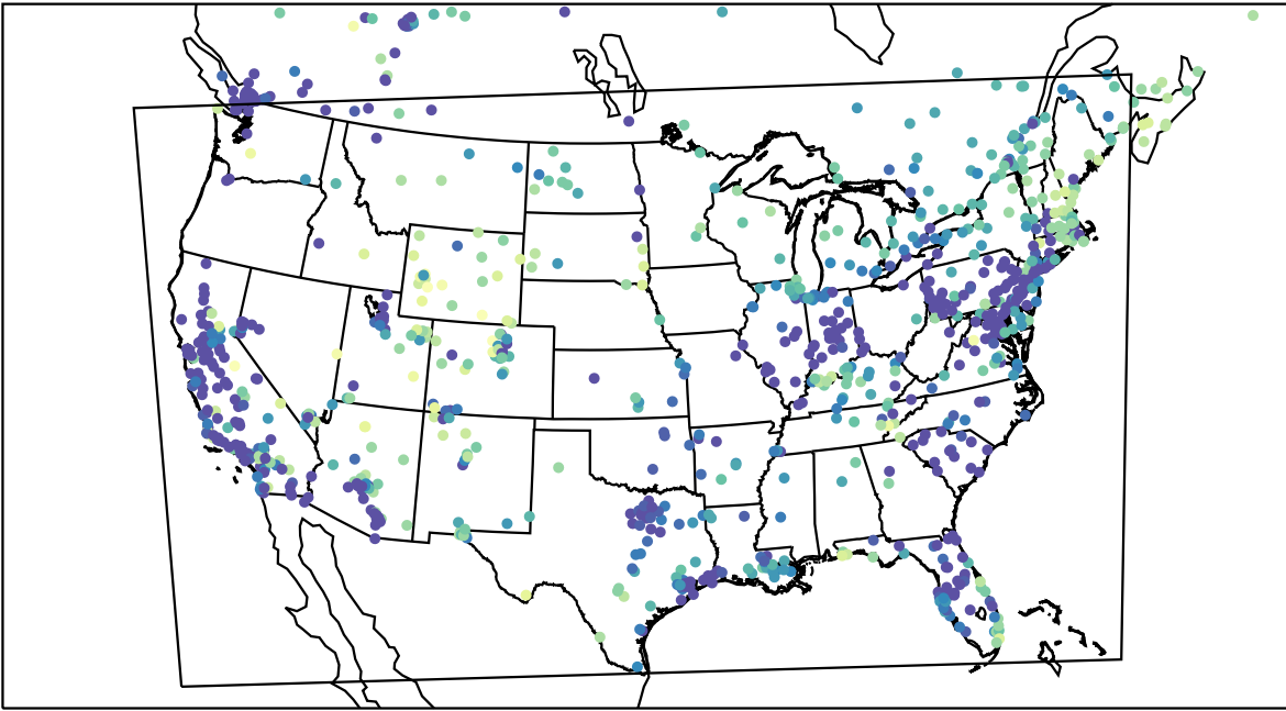
AirNOW (2023-02-16_13:00:00)
