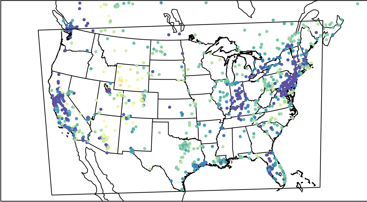
AirNOW (2023-02-17_03:00:00)
