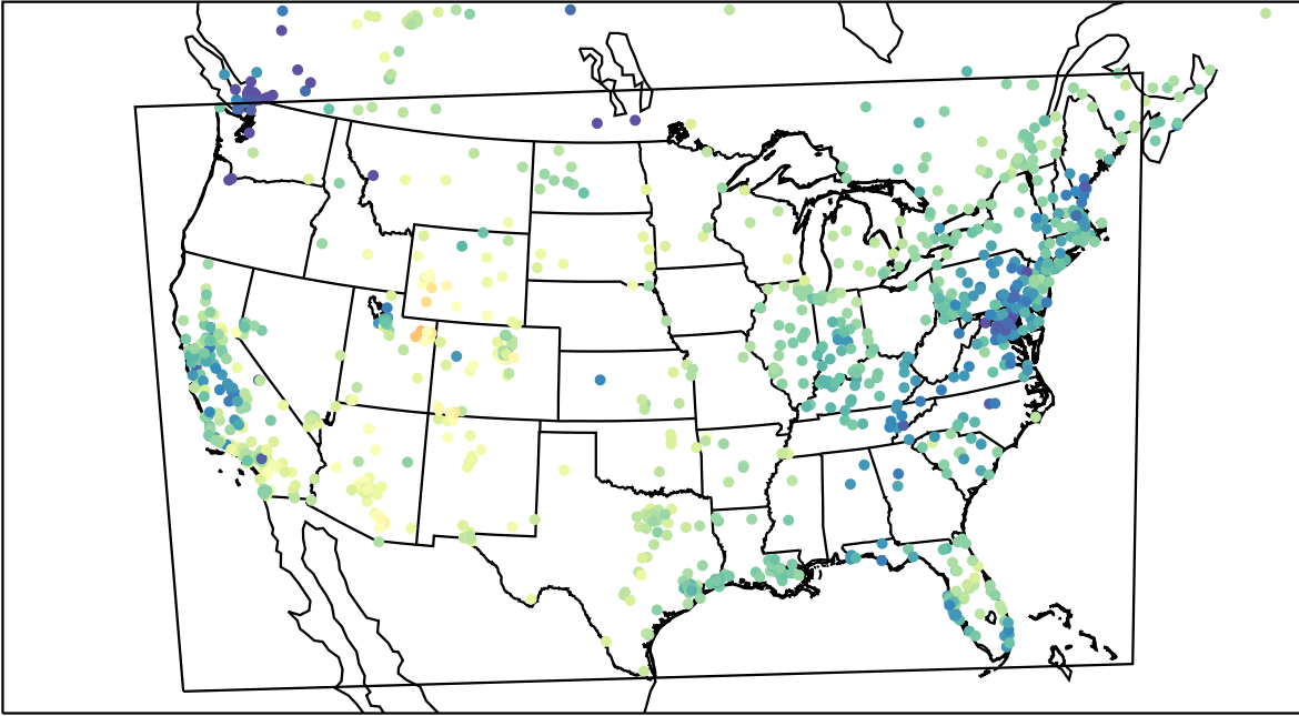
AirNOW (2023-02-17_19:00:00)
