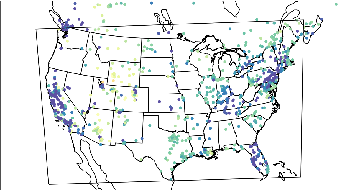
AirNOW (2023-02-17_07:00:00)
