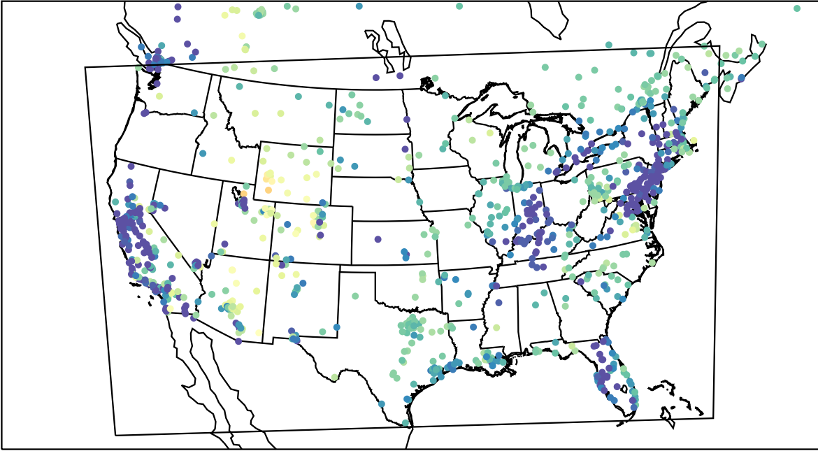
AirNOW (2023-02-17_04:00:00)
