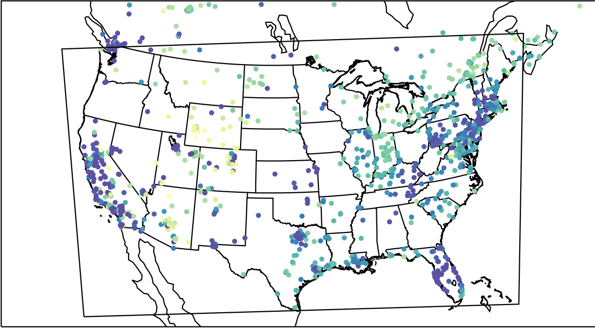
AirNOW (2023-02-17_13:00:00)
