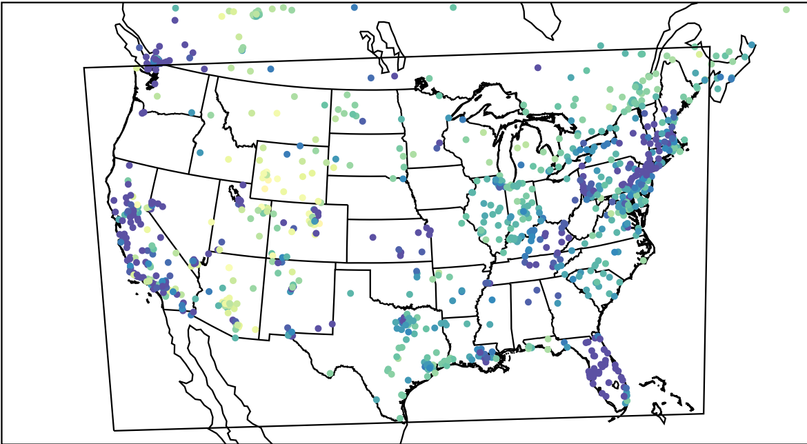
AirNOW (2023-02-17_11:00:00)
