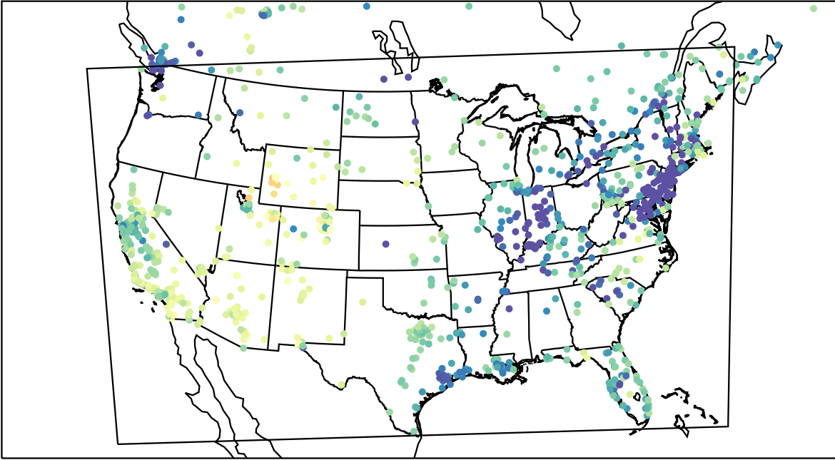
AirNOW (2023-02-17_00:00:00)
