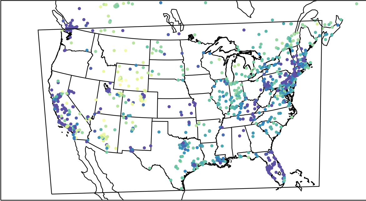
AirNOW (2023-02-17_12:00:00)
