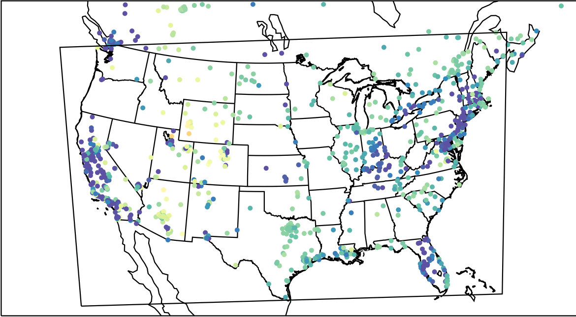
AirNOW (2023-02-17_06:00:00)
