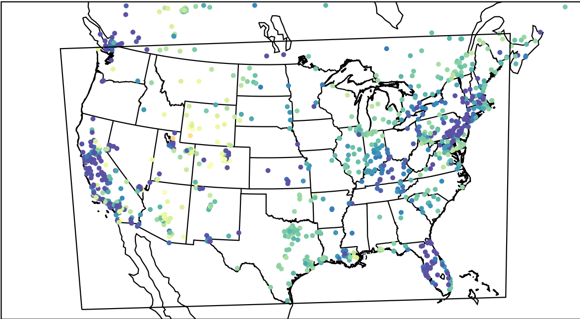
AirNOW (2023-02-17_08:00:00)
