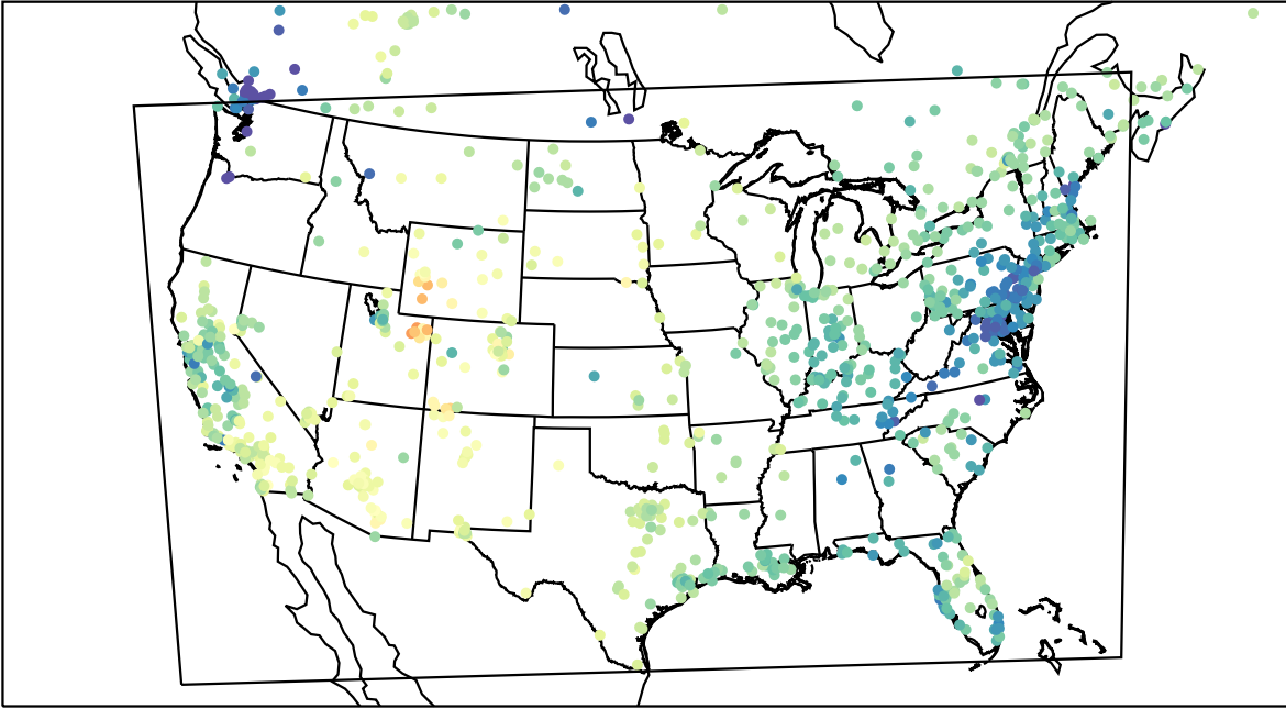
AirNOW (2023-02-17_20:00:00)
