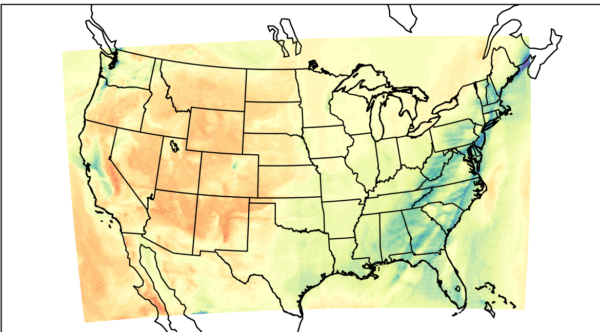
WRF (2023-02-17_19:00:00)
