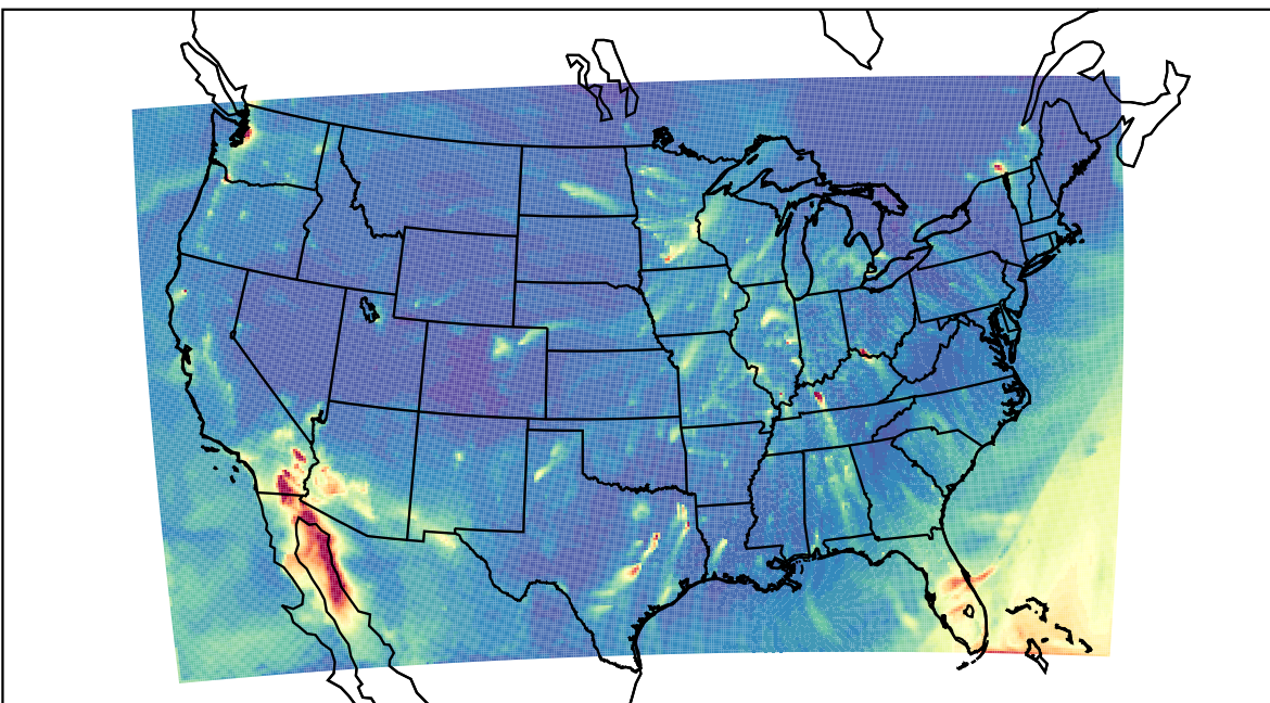
WRF 2023-02-18_05:00:00
