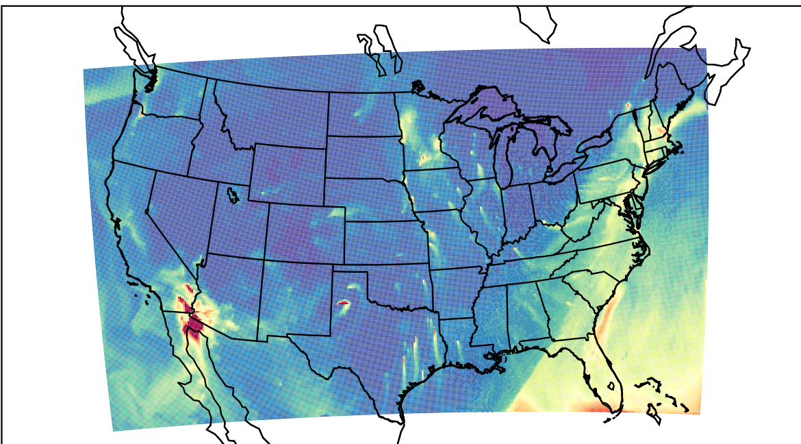
WRF 2023-02-17_14:00:00
