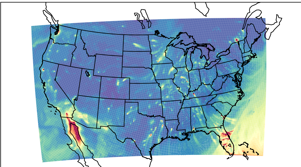
WRF 2023-02-18_02:00:00
