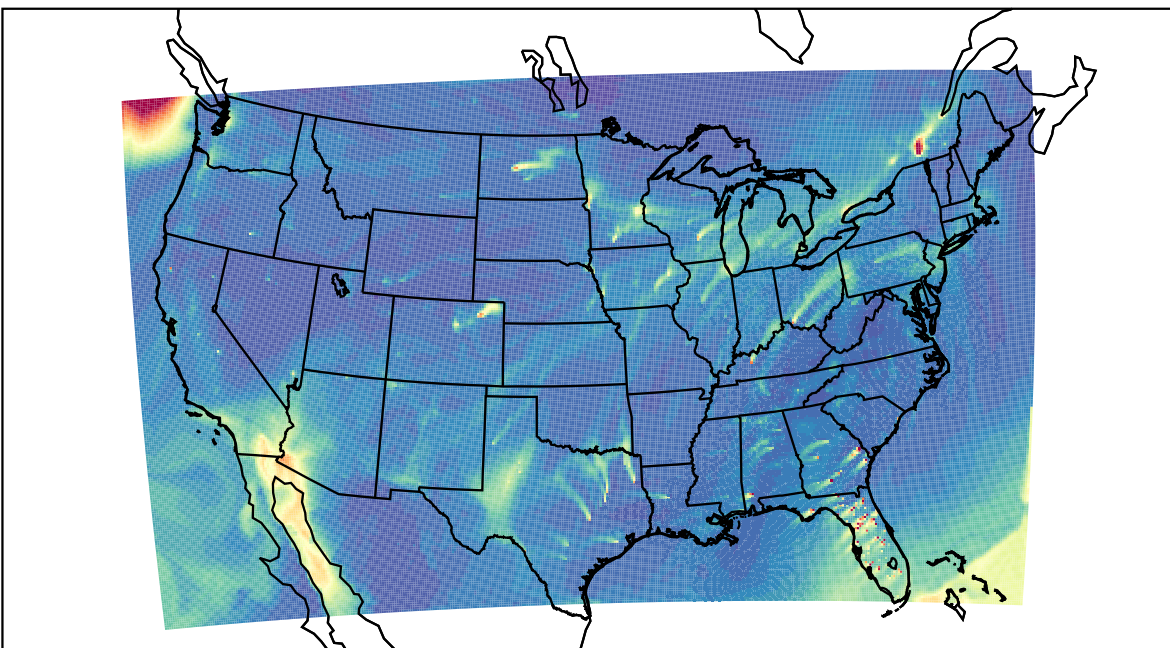
WRF 2023-02-18_21:00:00
