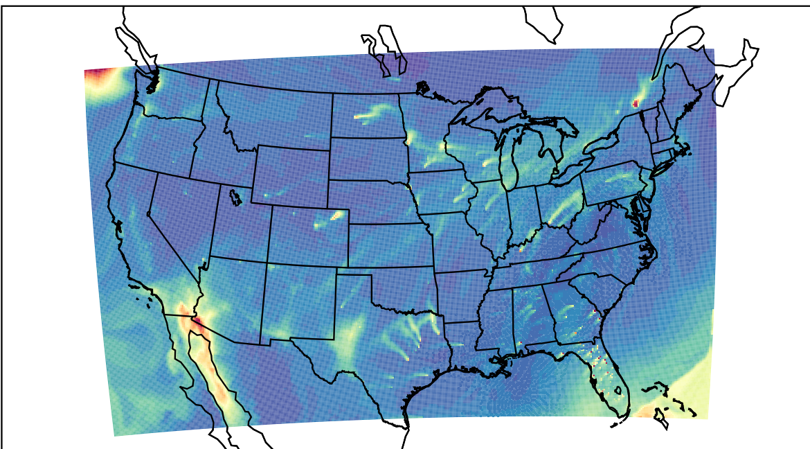
WRF 2023-02-18_19:00:00
