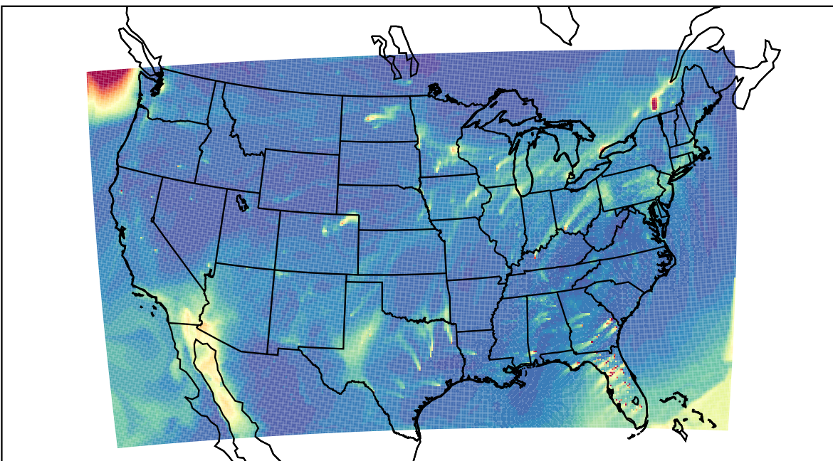
WRF 2023-02-18_22:00:00
