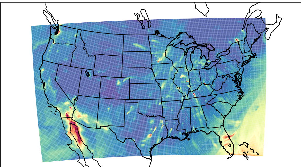
WRF 2023-02-18_04:00:00
