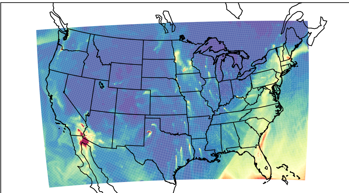
WRF 2023-02-17_13:00:00
