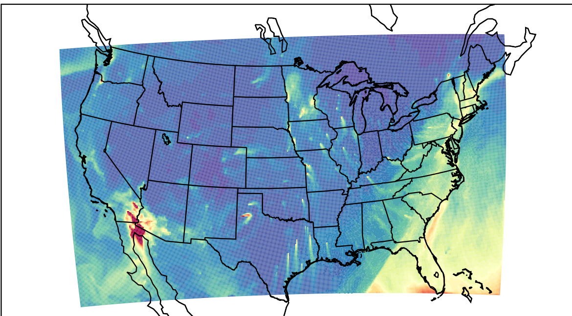
WRF 2023-02-17_15:00:00
