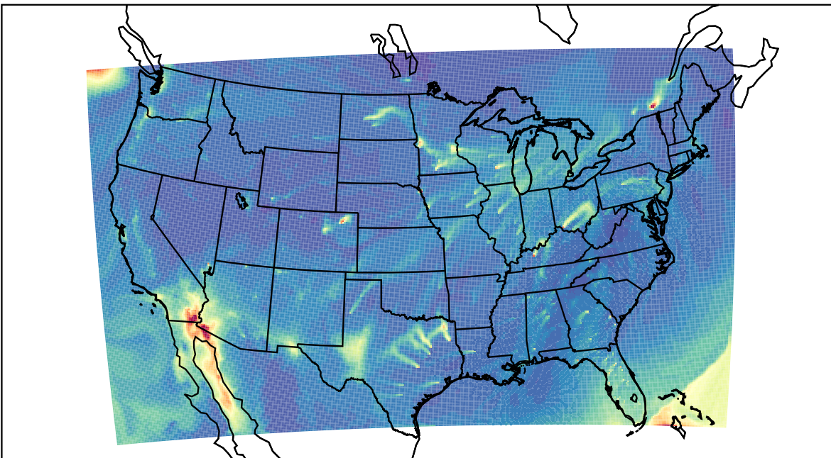
WRF 2023-02-18_17:00:00
