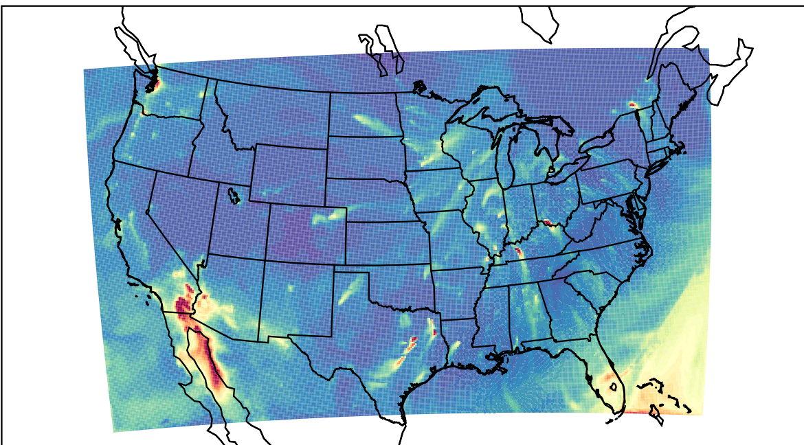
WRF 2023-02-18_07:00:00
