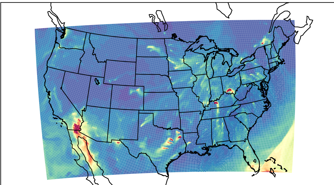
WRF 2023-02-18_12:00:00
