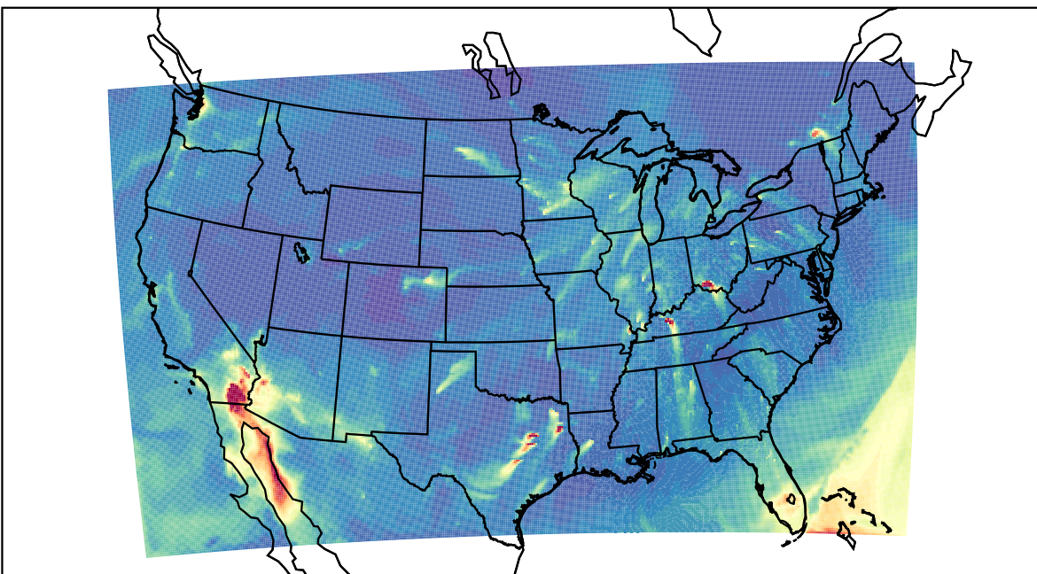
WRF 2023-02-18_09:00:00
