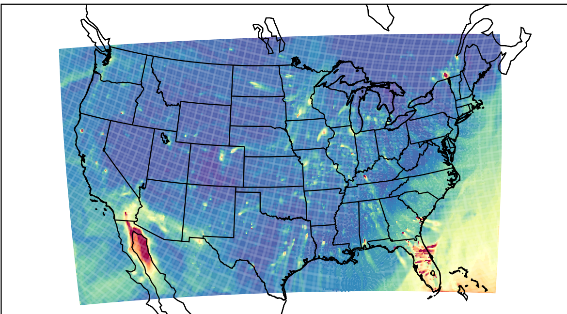
WRF 2023-02-18_01:00:00
