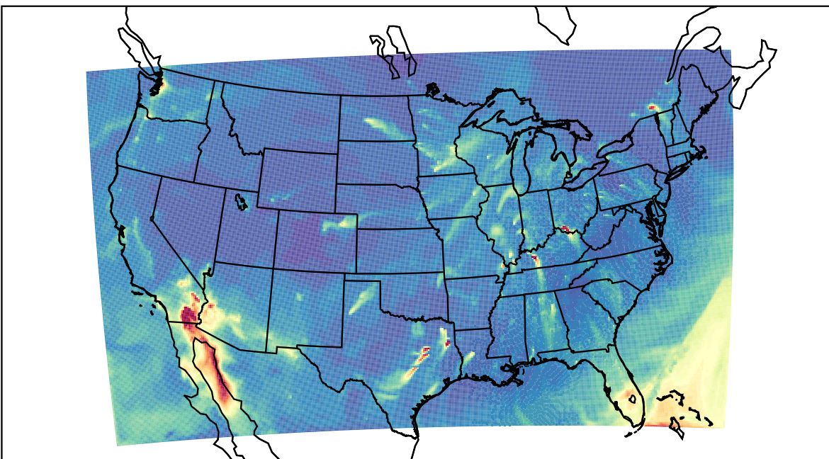
WRF 2023-02-18_08:00:00
