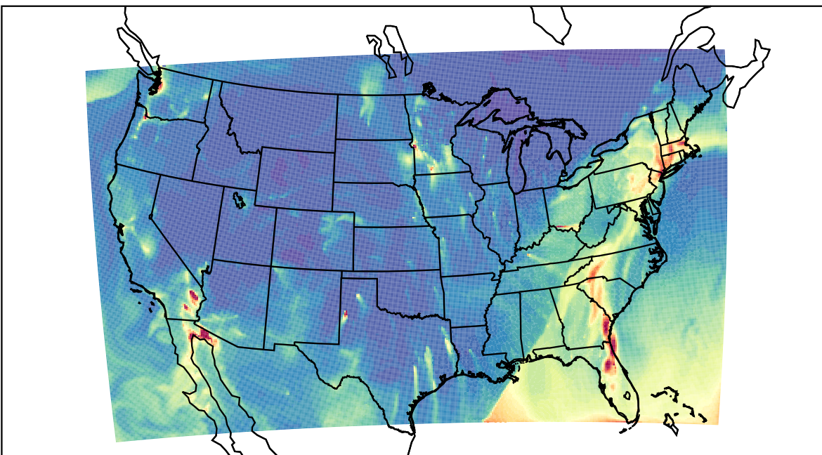
WRF 2023-02-17_07:00:00
