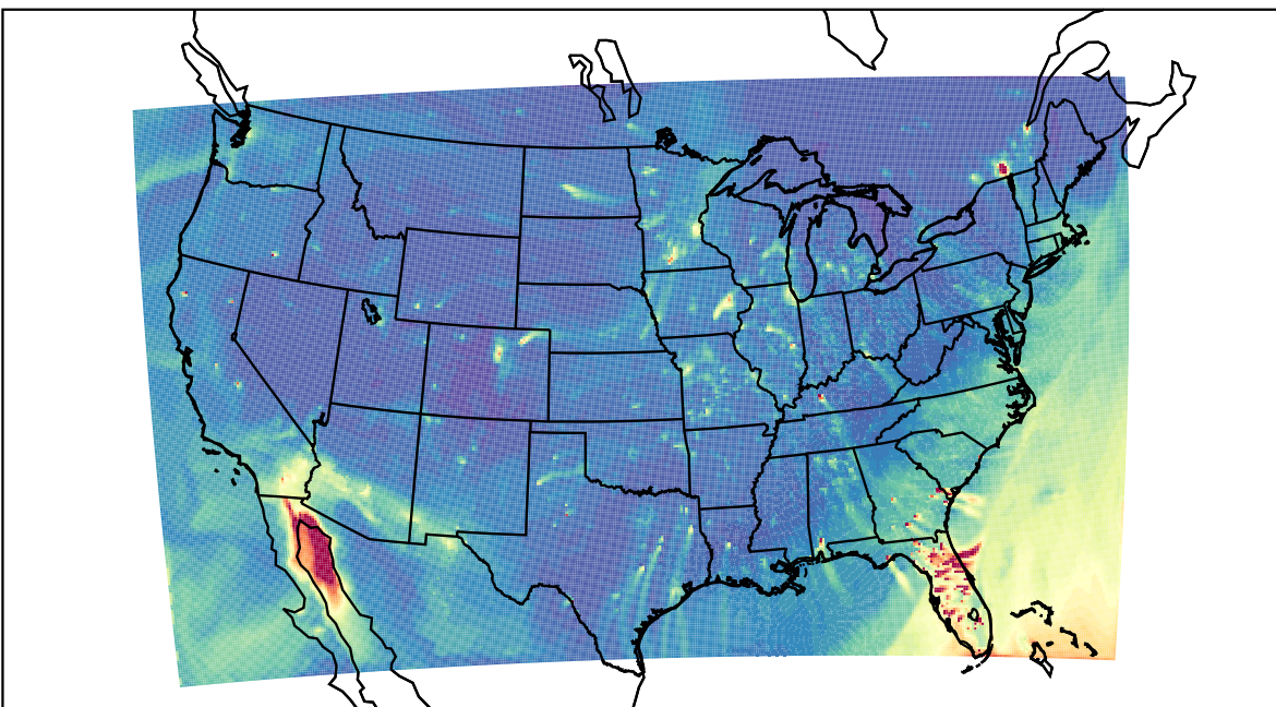
WRF 2023-02-18_00:00:00
