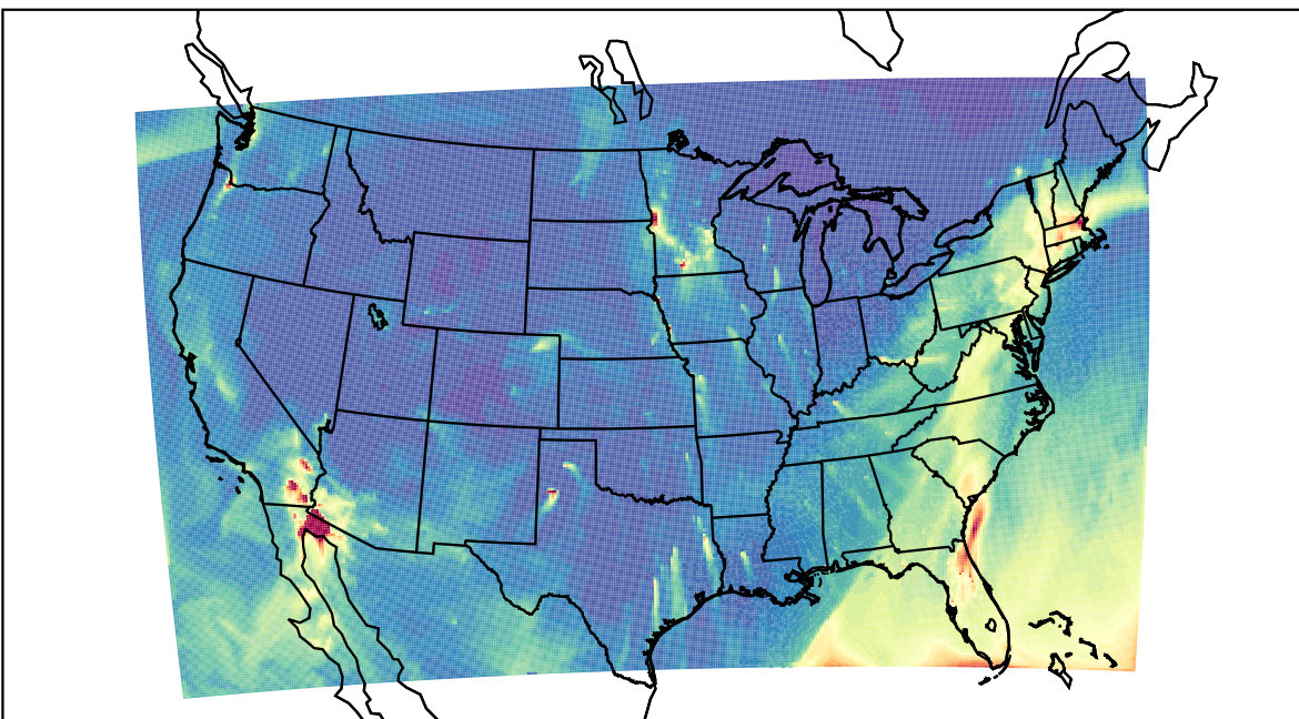
WRF 2023-02-17_11:00:00
