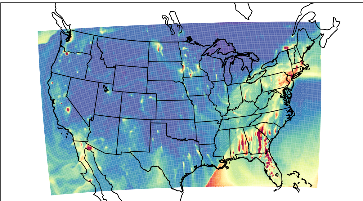
WRF 2023-02-17_02:00:00
