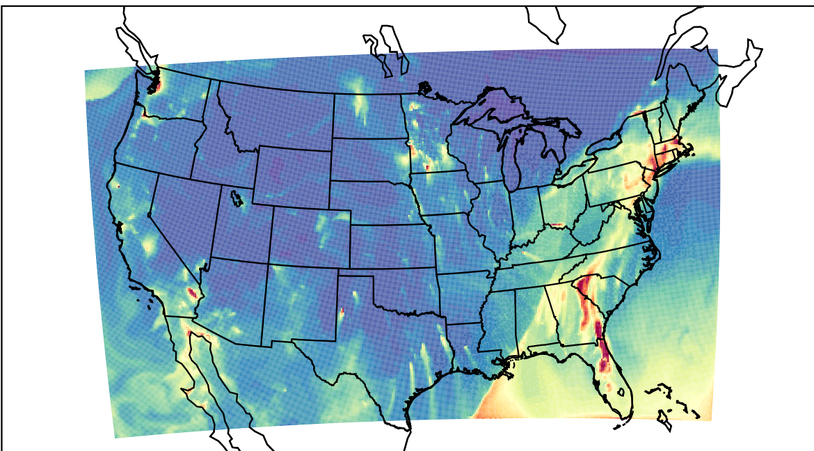
WRF 2023-02-17_05:00:00
