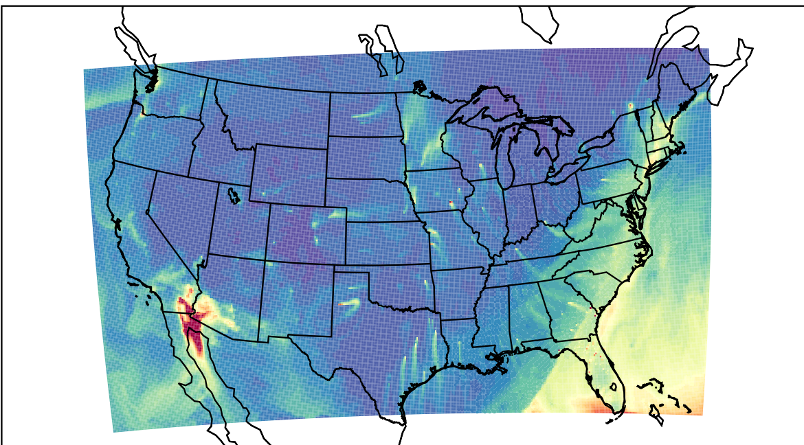
WRF 2023-02-17_17:00:00
