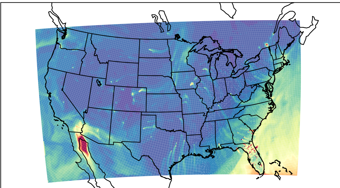
WRF 2023-02-17_21:00:00
