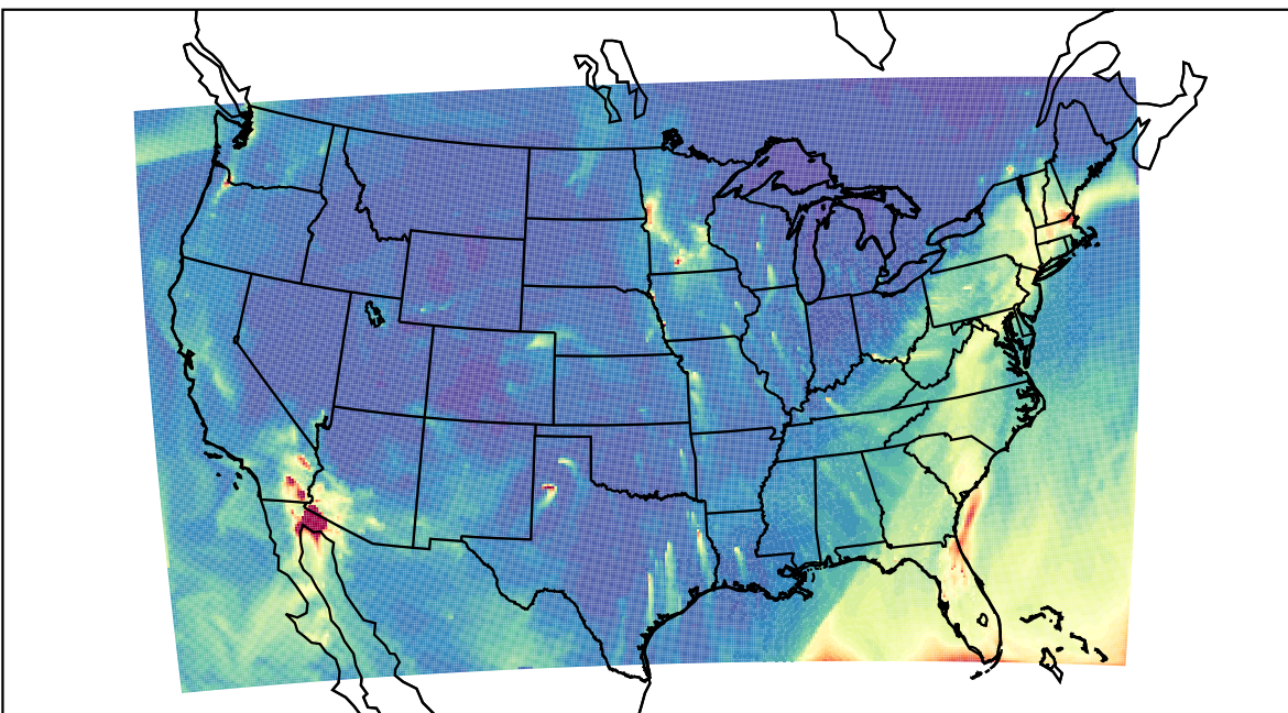
WRF 2023-02-17_12:00:00
