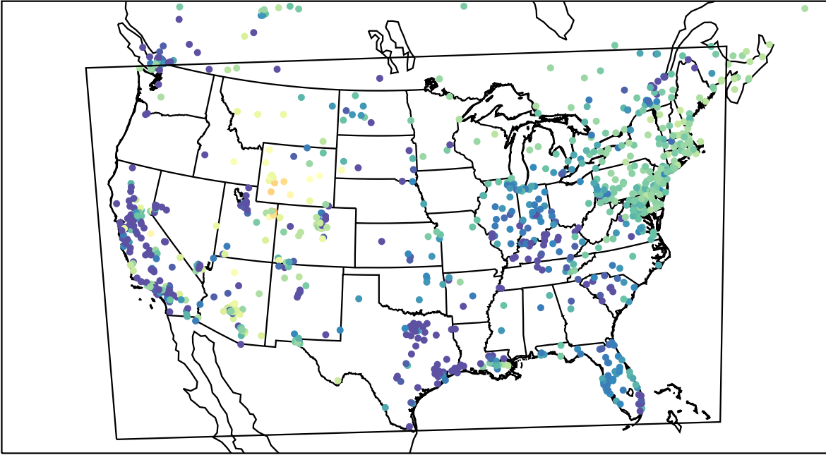
AirNOW (2023-02-18_10:00:00)
