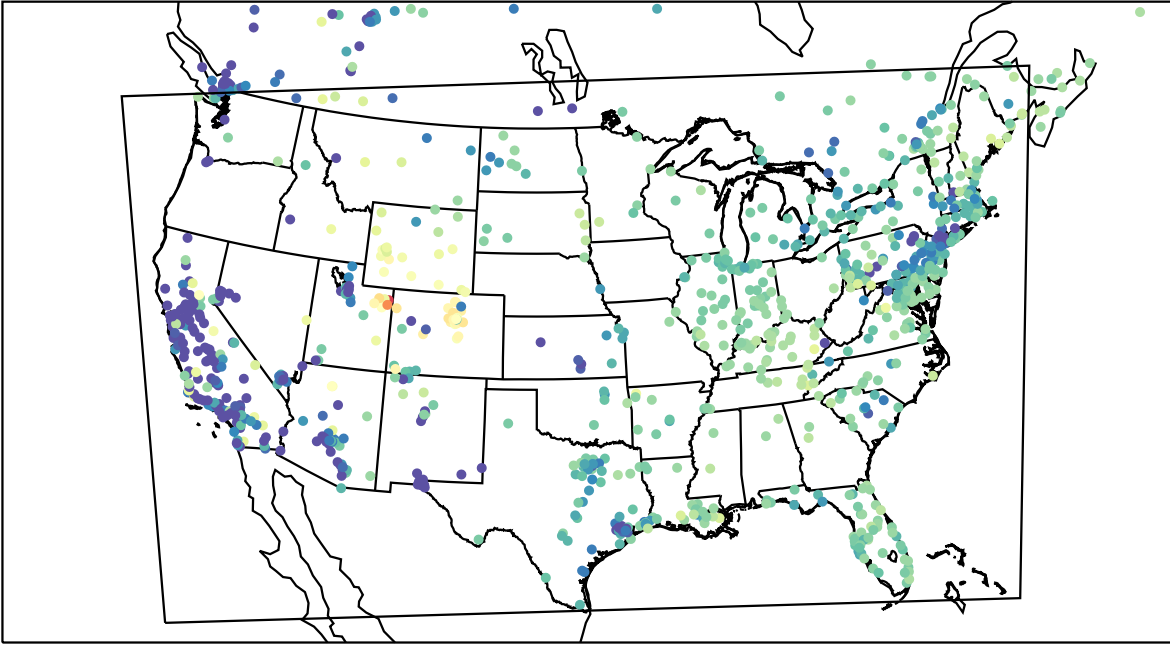
AirNOW (2023-02-19_15:00:00)
