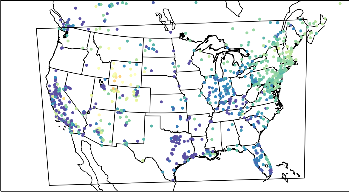
AirNOW (2023-02-18_13:00:00)
