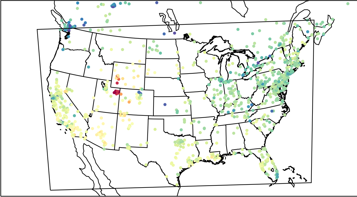
AirNOW (2023-02-18_22:00:00)
