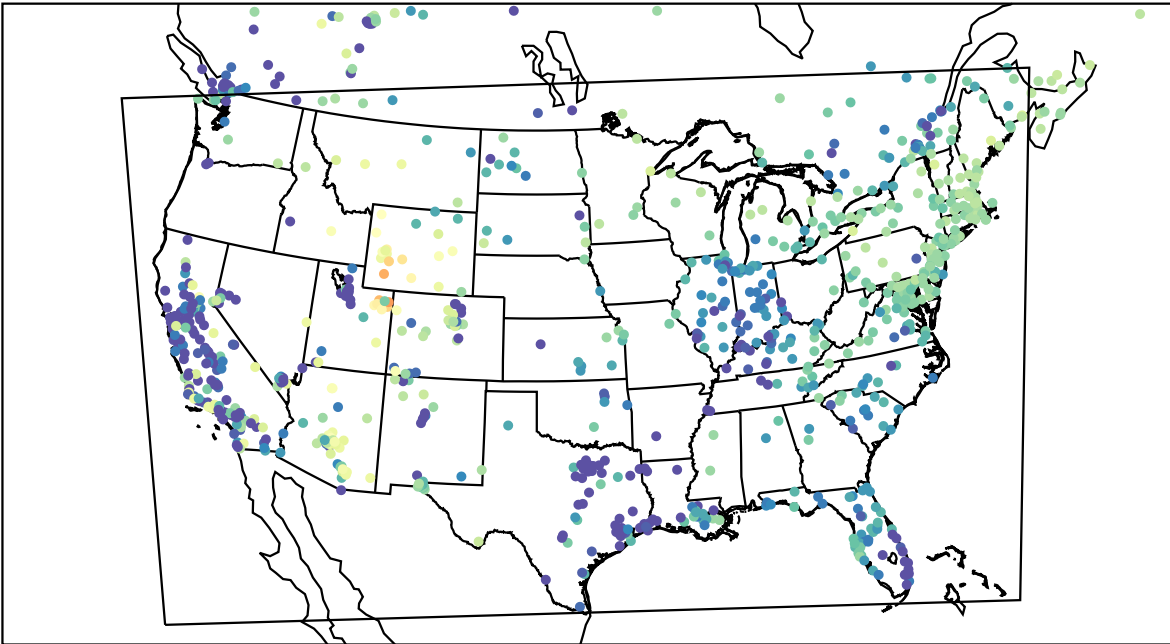
AirNOW (2023-02-18_06:00:00)
