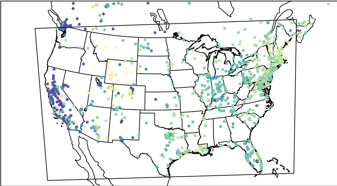
AirNOW (2023-02-18_16:00:00)
