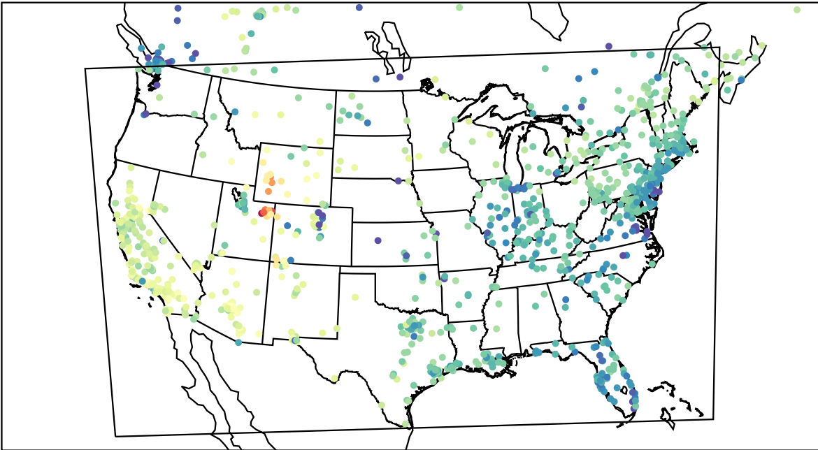
AirNOW (2023-02-18_00:00:00)
