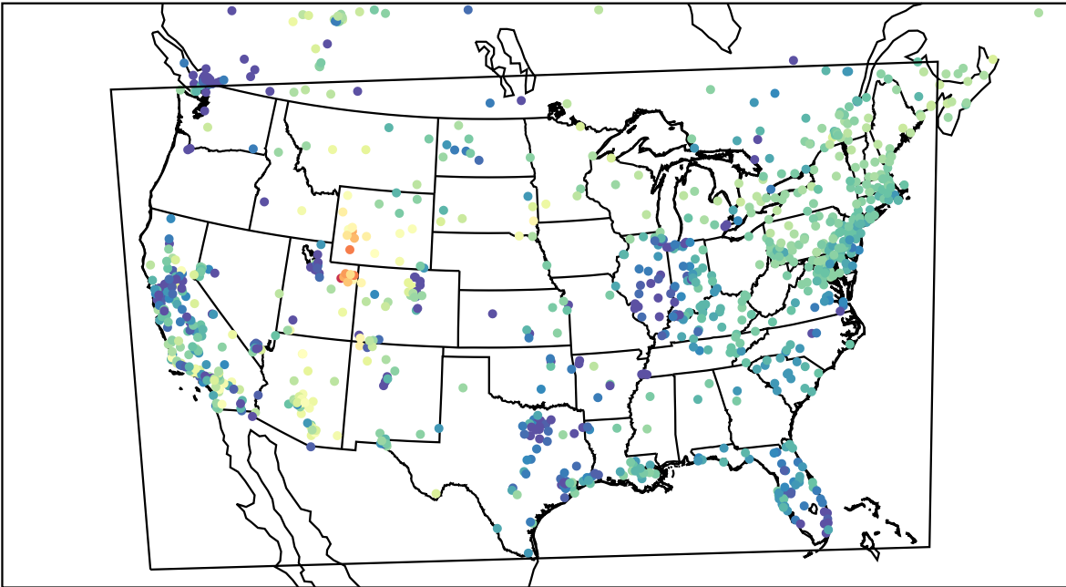
AirNOW (2023-02-18_02:00:00)
