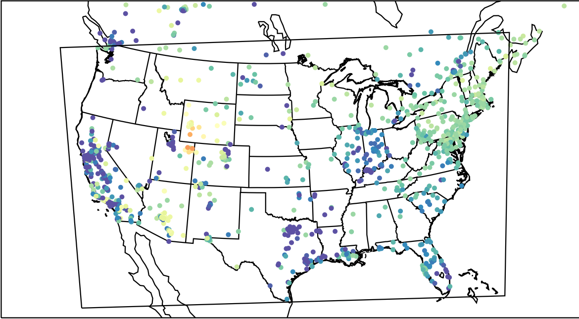
AirNOW (2023-02-18_05:00:00)
