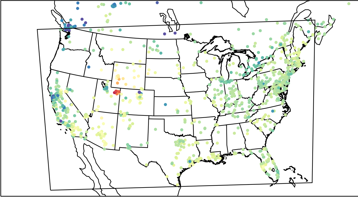
AirNOW (2023-02-18_19:00:00)
