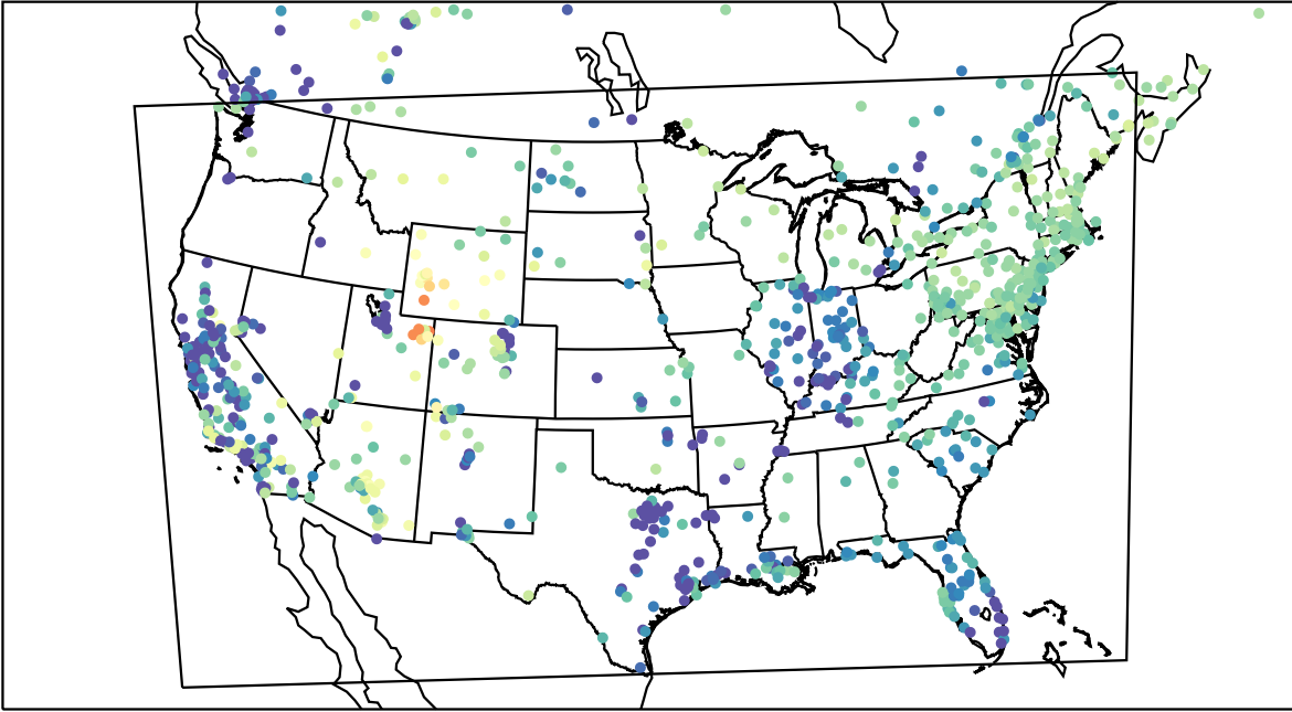
AirNOW (2023-02-18_04:00:00)
