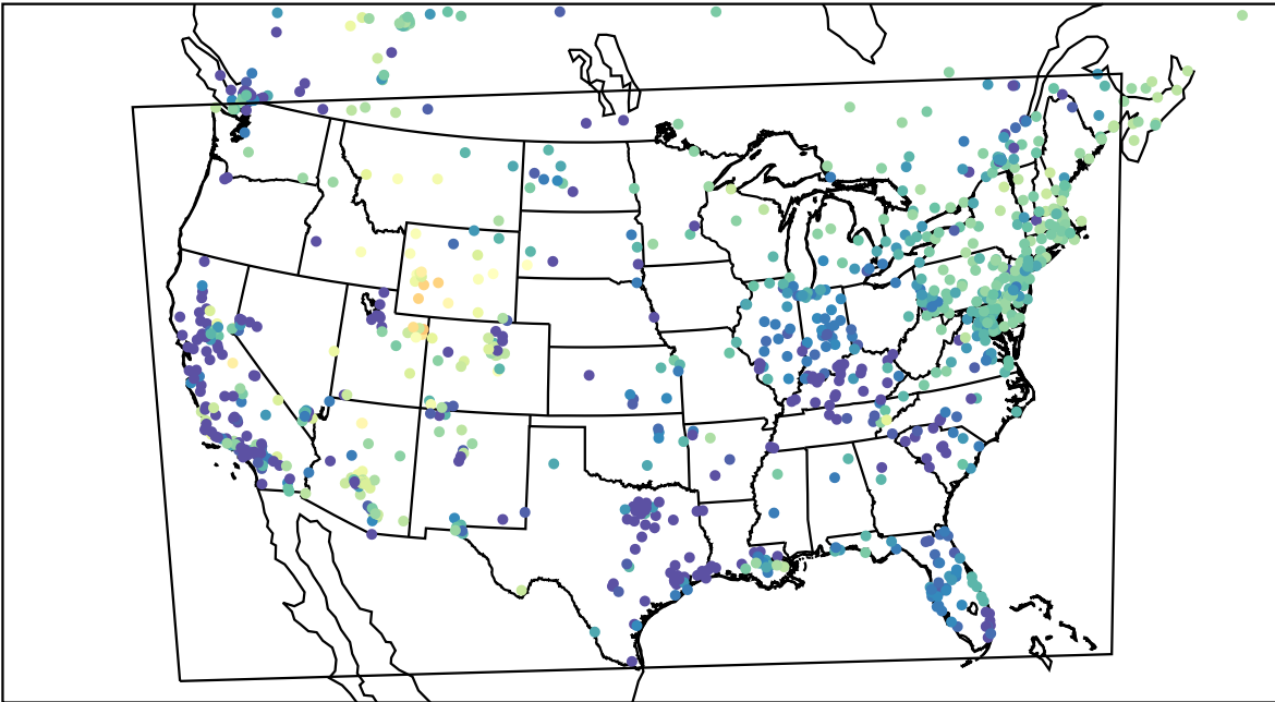
AirNOW (2023-02-18_11:00:00)
