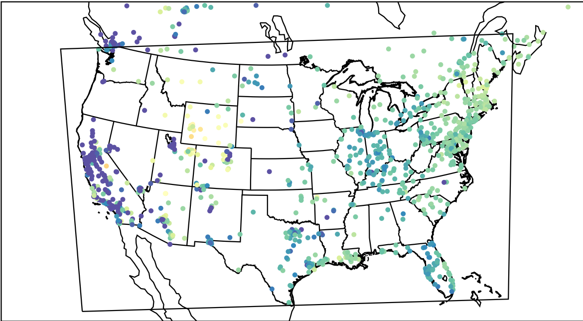
AirNOW (2023-02-18_15:00:00)
