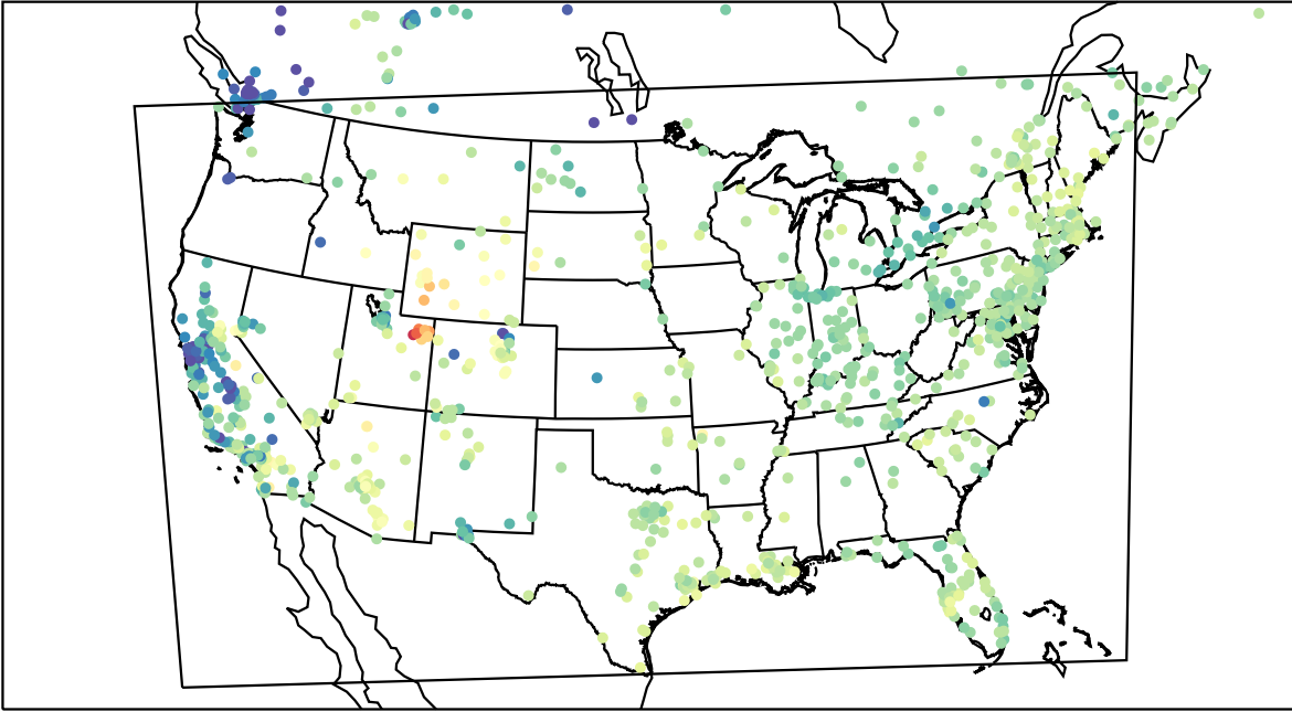
AirNOW (2023-02-18_18:00:00)
