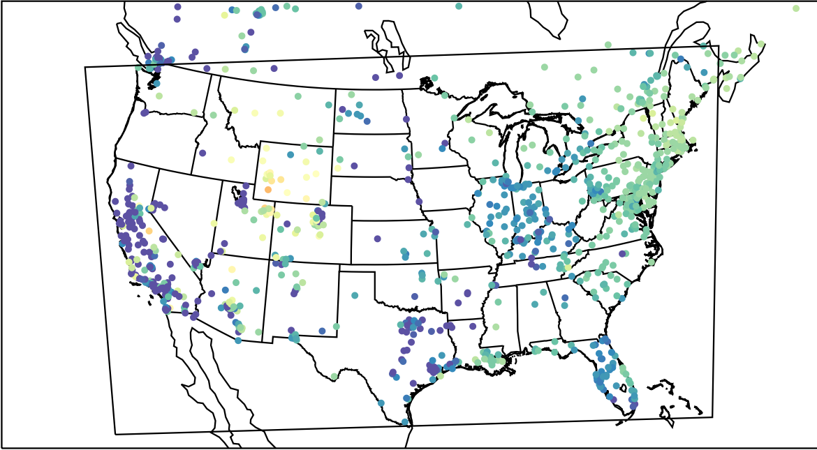
AirNOW (2023-02-18_14:00:00)
