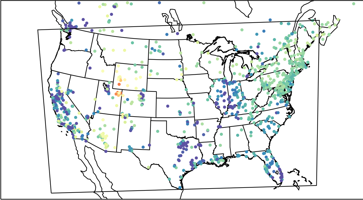
AirNOW (2023-02-18_03:00:00)
