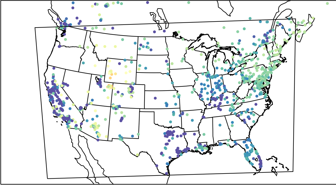
AirNOW (2023-02-18_08:00:00)
