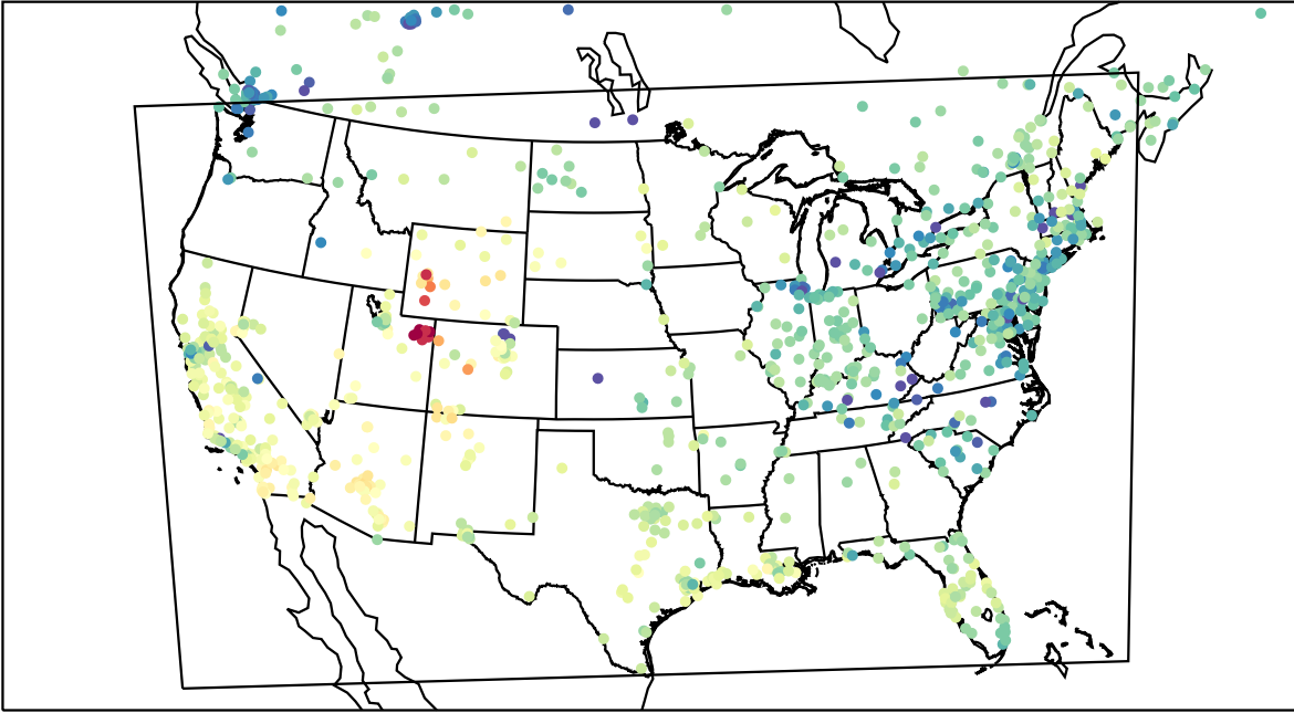
AirNOW (2023-02-18_23:00:00)
