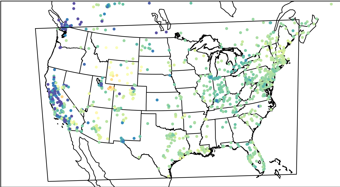
AirNOW (2023-02-18_17:00:00)
