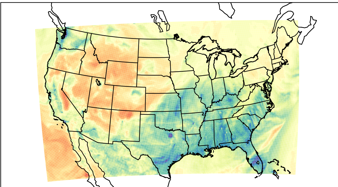
WRF (2023-02-18_06:00:00)
