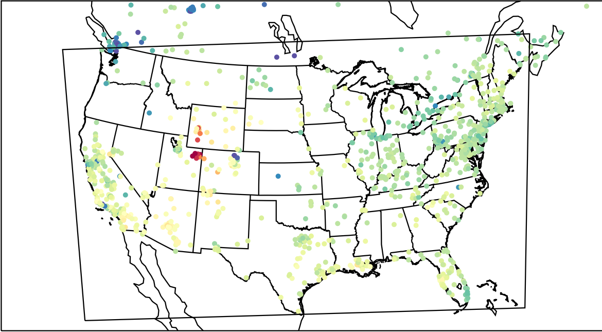
AirNOW (2023-02-18_21:00:00)
