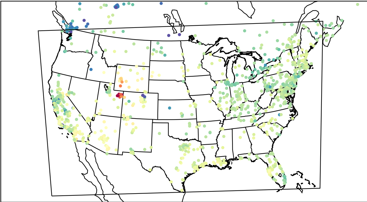
AirNOW (2023-02-18_20:00:00)
