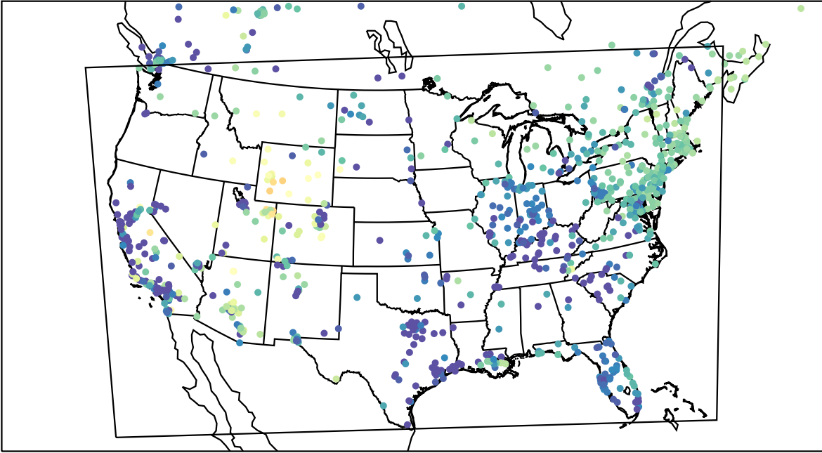
AirNOW (2023-02-18_12:00:00)
