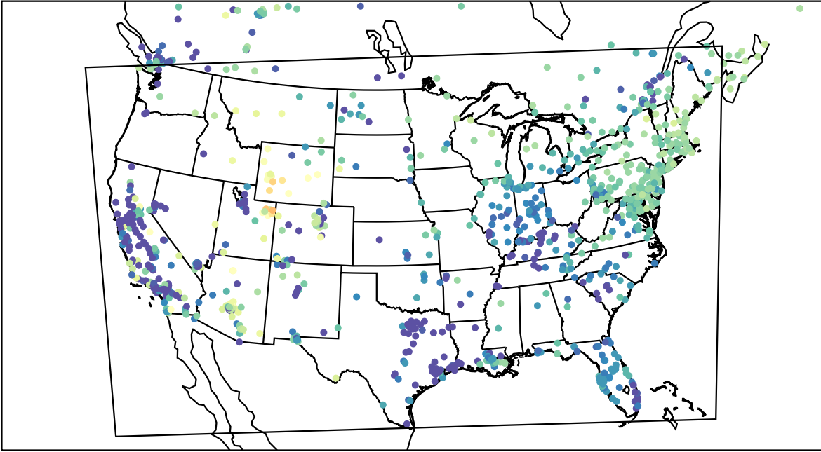
AirNOW (2023-02-18_09:00:00)
