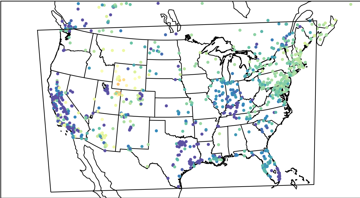
AirNOW (2023-02-18_07:00:00)
