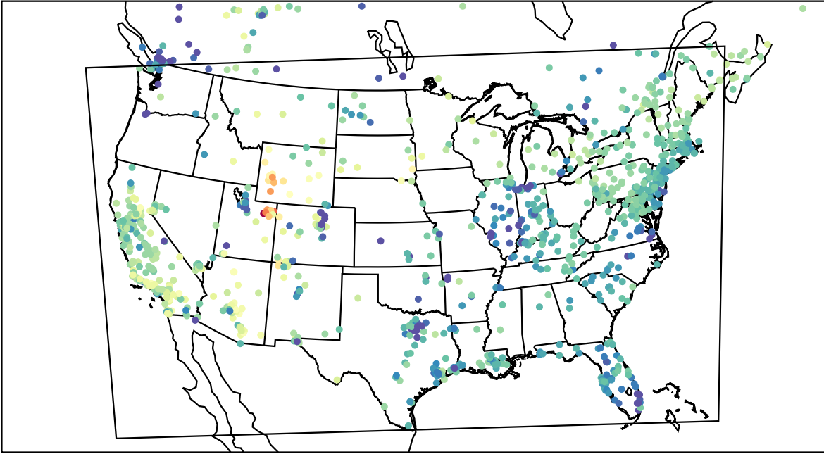
AirNOW (2023-02-18_01:00:00)
