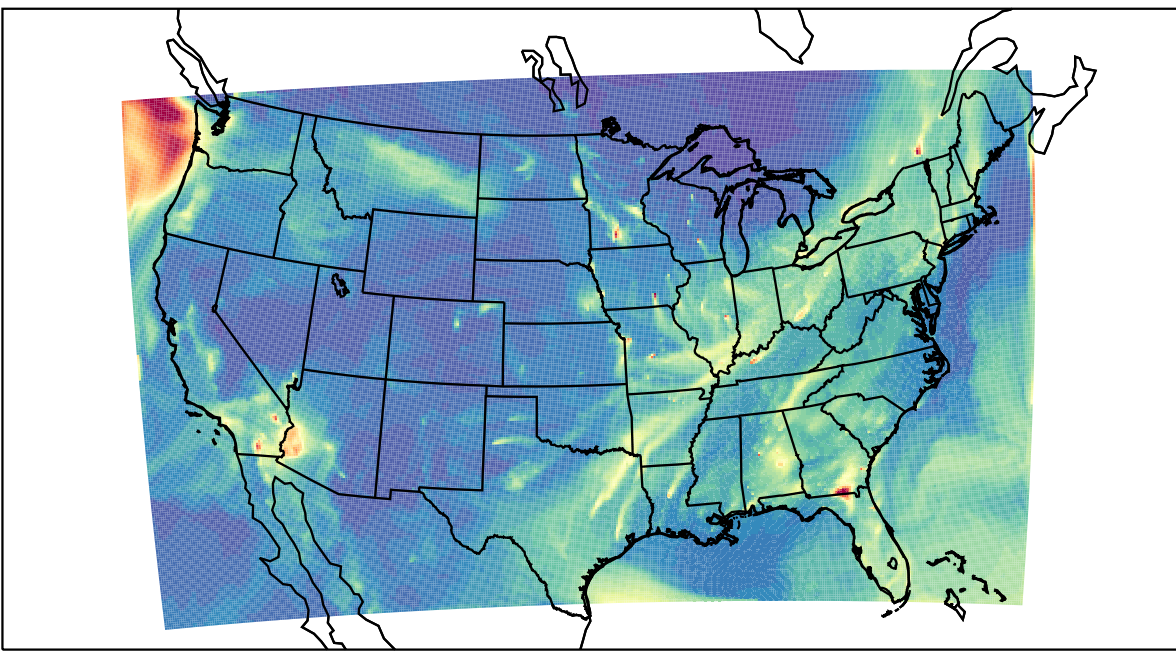
WRF 2023-02-20_09:00:00
