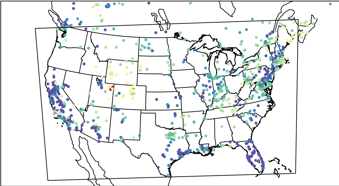
AirNOW (2023-02-20_08:00:00)
