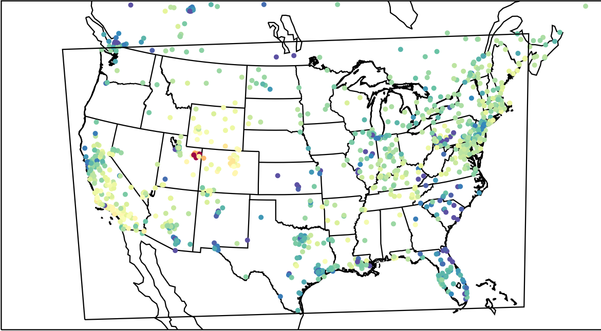
AirNOW (2023-02-20_01:00:00)
