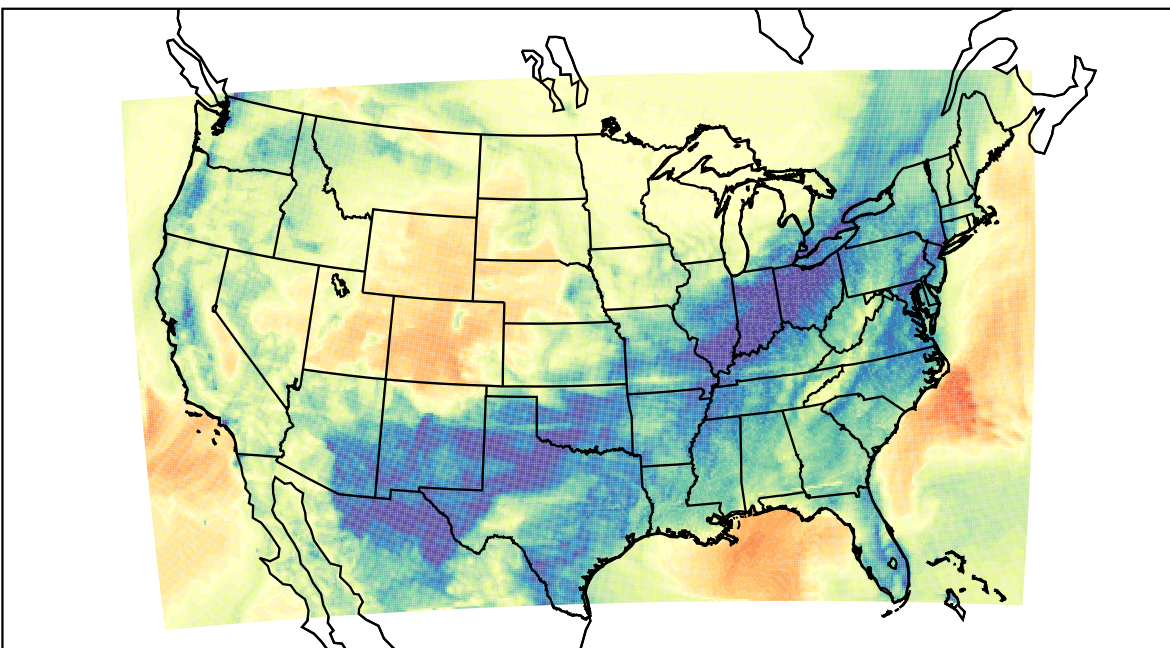
WRF (2023-02-20_08:00:00)
