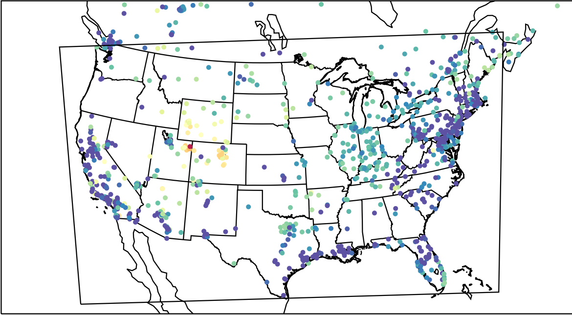
AirNOW (2023-02-19_11:00:00)
