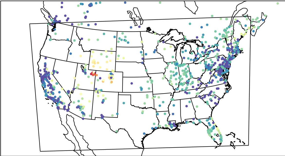
AirNOW (2023-02-19_04:00:00)
