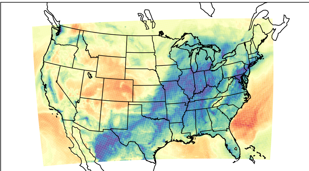
WRF (2023-02-19_13:00:00)
