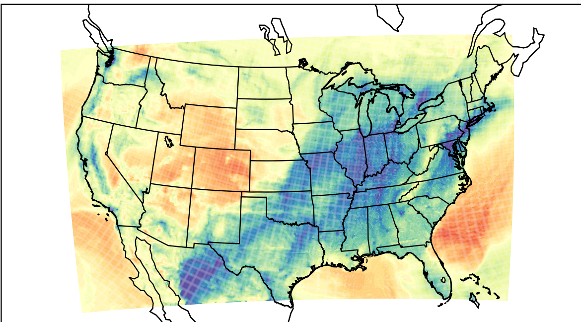
WRF (2023-02-19_11:00:00)
