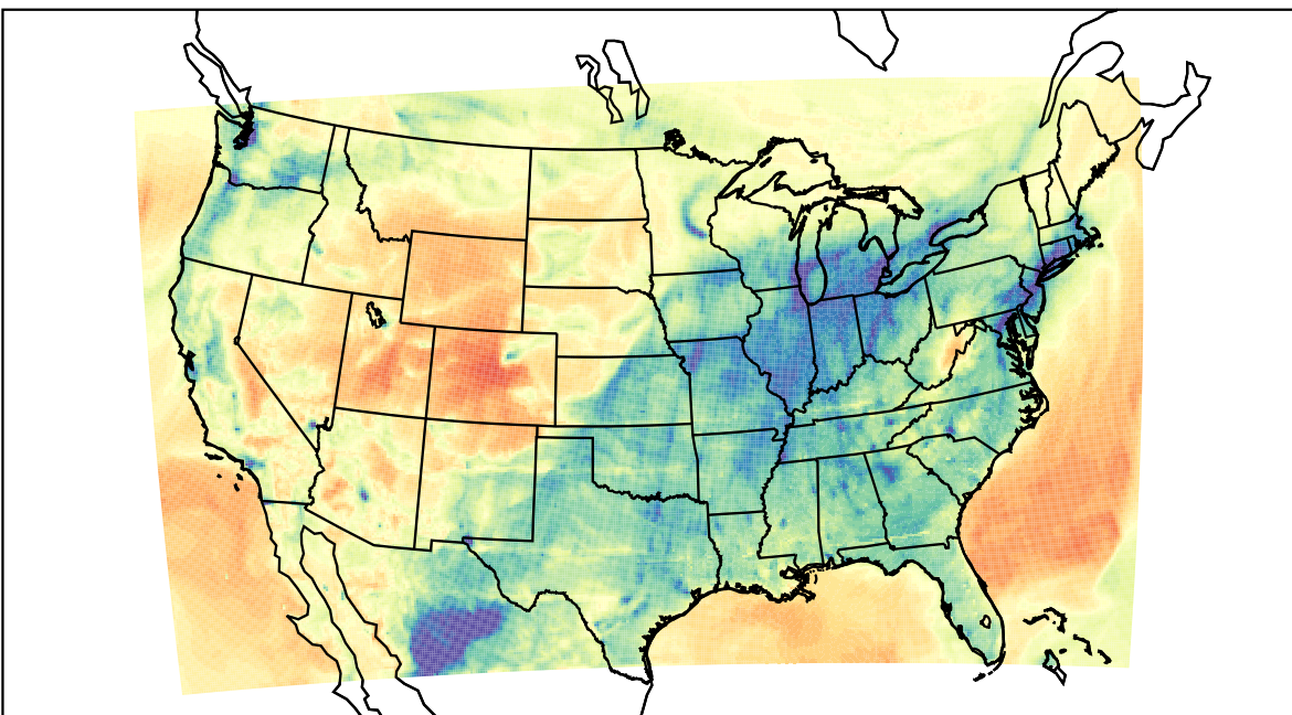
WRF (2023-02-19_03:00:00)
