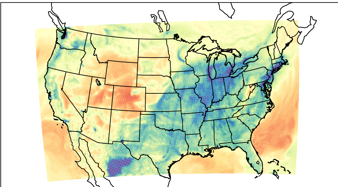
WRF (2023-02-19_04:00:00)
