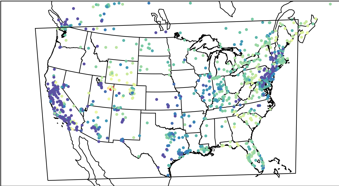
AirNOW (2023-02-20_15:00:00)
