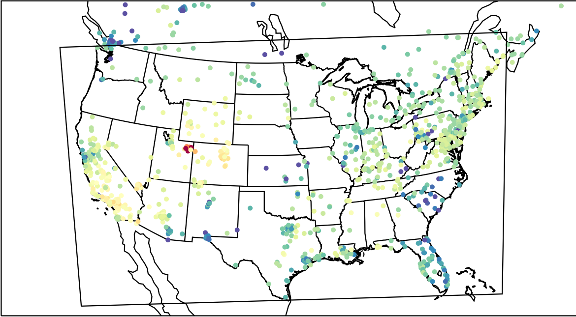
AirNOW (2023-02-20_00:00:00)
