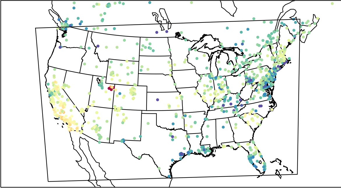
AirNOW (2023-02-20_23:00:00)
