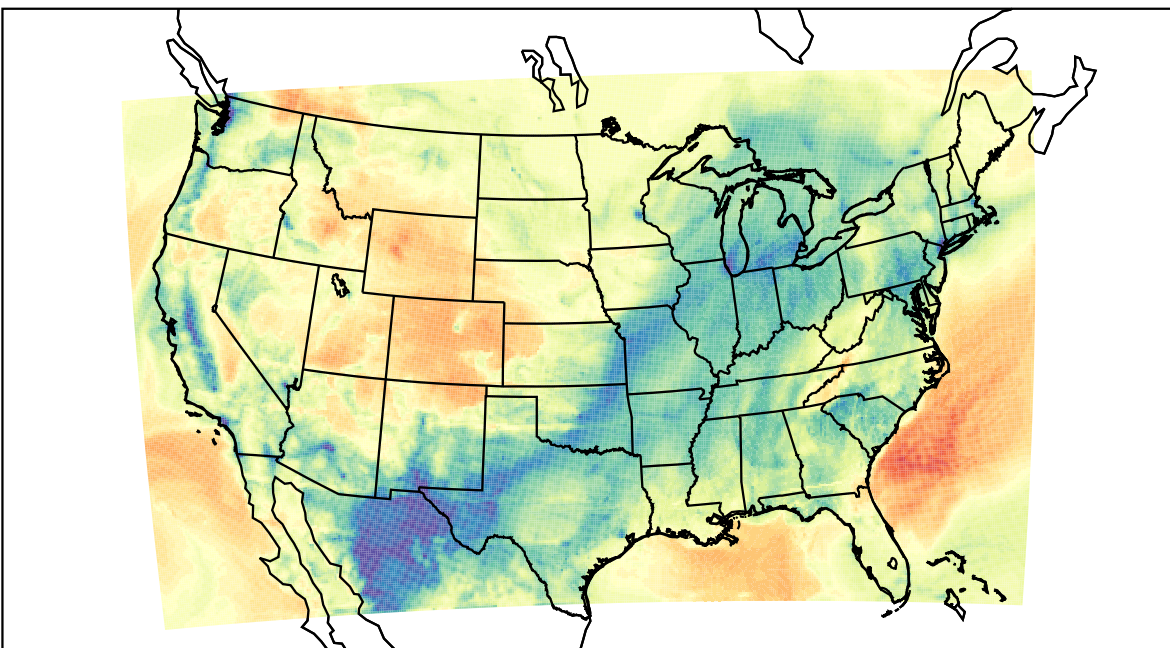
WRF (2023-02-19_16:00:00)
