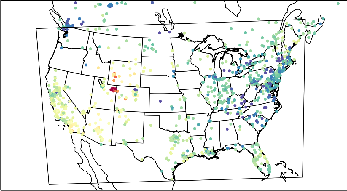
AirNOW (2023-02-19_00:00:00)
