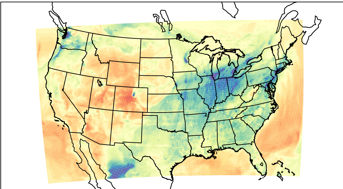
WRF (2023-02-19_00:00:00)
