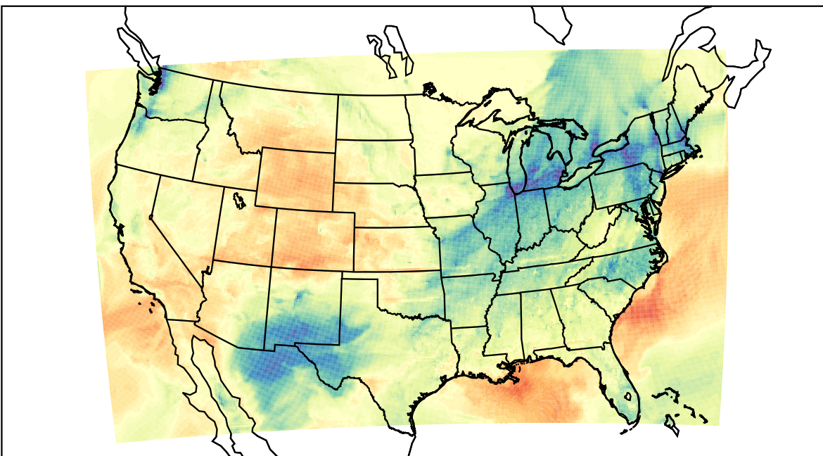
WRF (2023-02-19_23:00:00)
