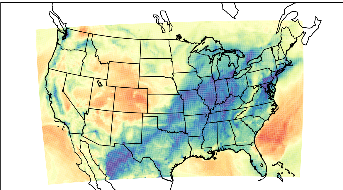
WRF (2023-02-19_12:00:00)
