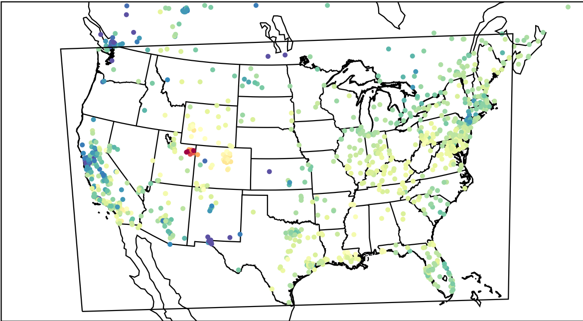
AirNOW (2023-02-19_18:00:00)
