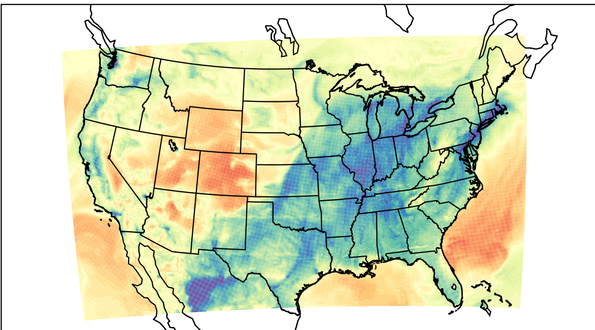
WRF (2023-02-19_07:00:00)
