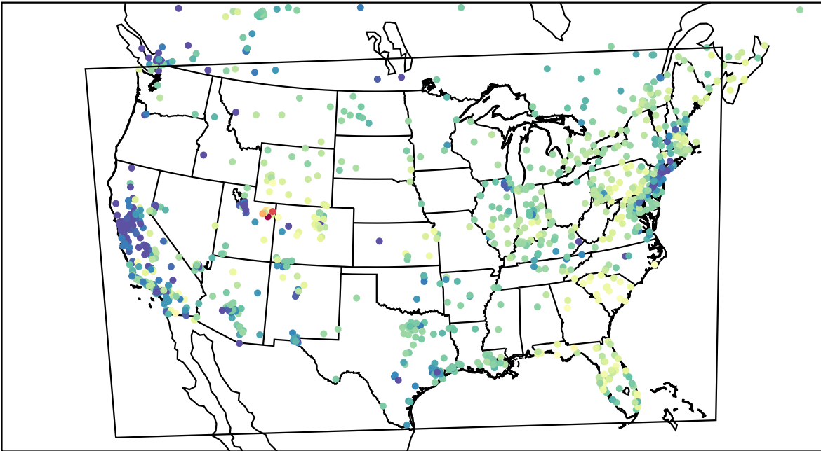
AirNOW (2023-02-20_17:00:00)
