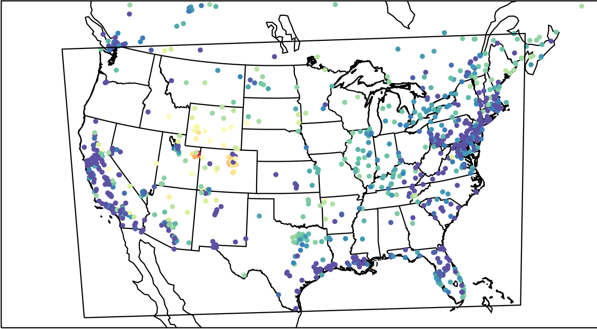
AirNOW (2023-02-19_10:00:00)
