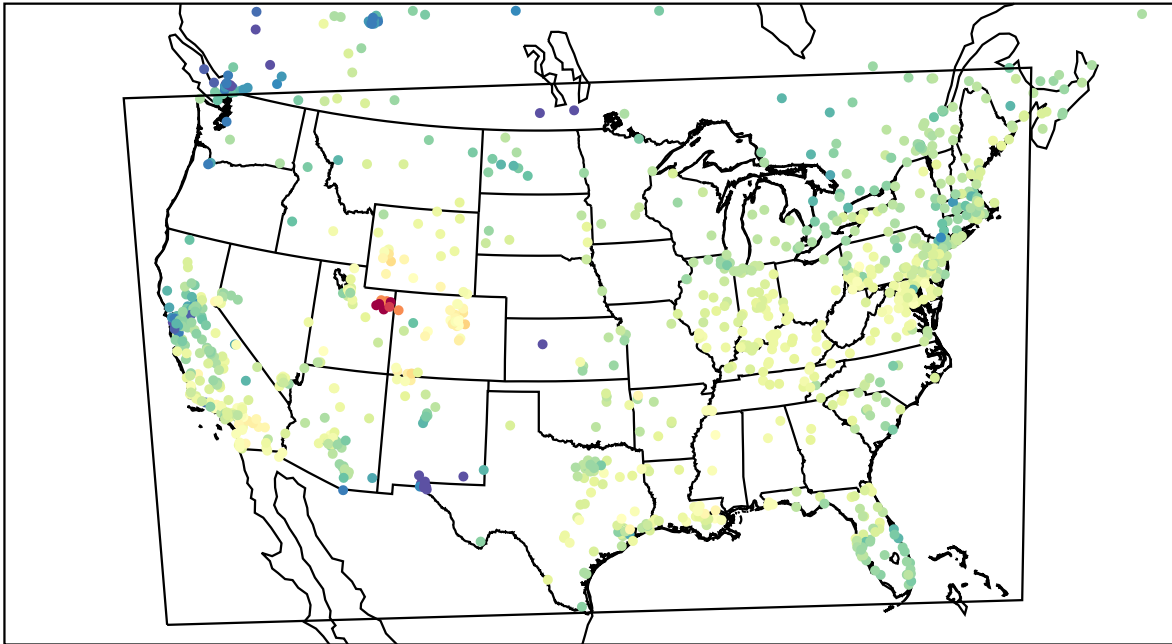
AirNOW (2023-02-19_19:00:00)
