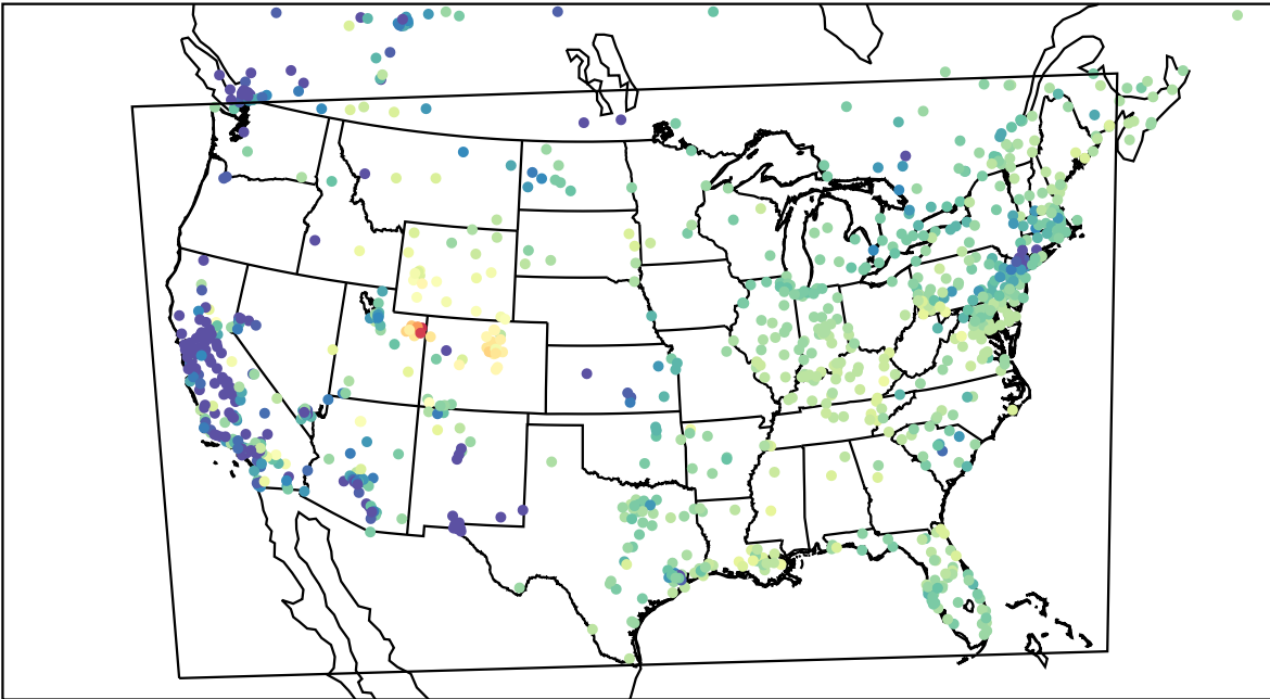
AirNOW (2023-02-19_16:00:00)
