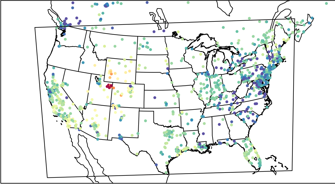
AirNOW (2023-02-19_01:00:00)
