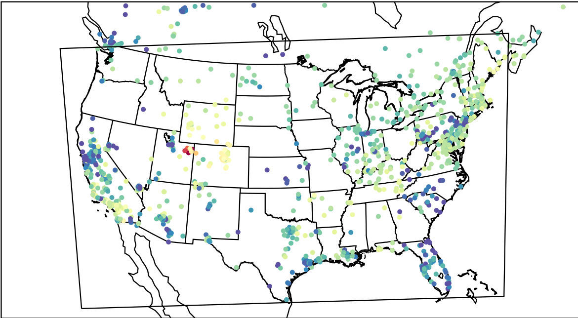
AirNOW (2023-02-20_02:00:00)
