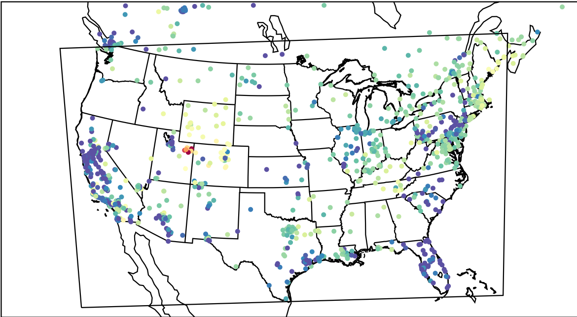
AirNOW (2023-02-20_05:00:00)
