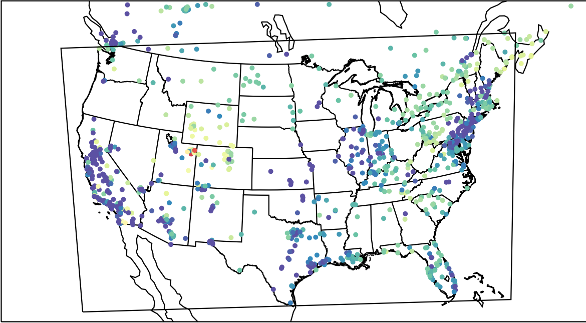
AirNOW (2023-02-20_14:00:00)
