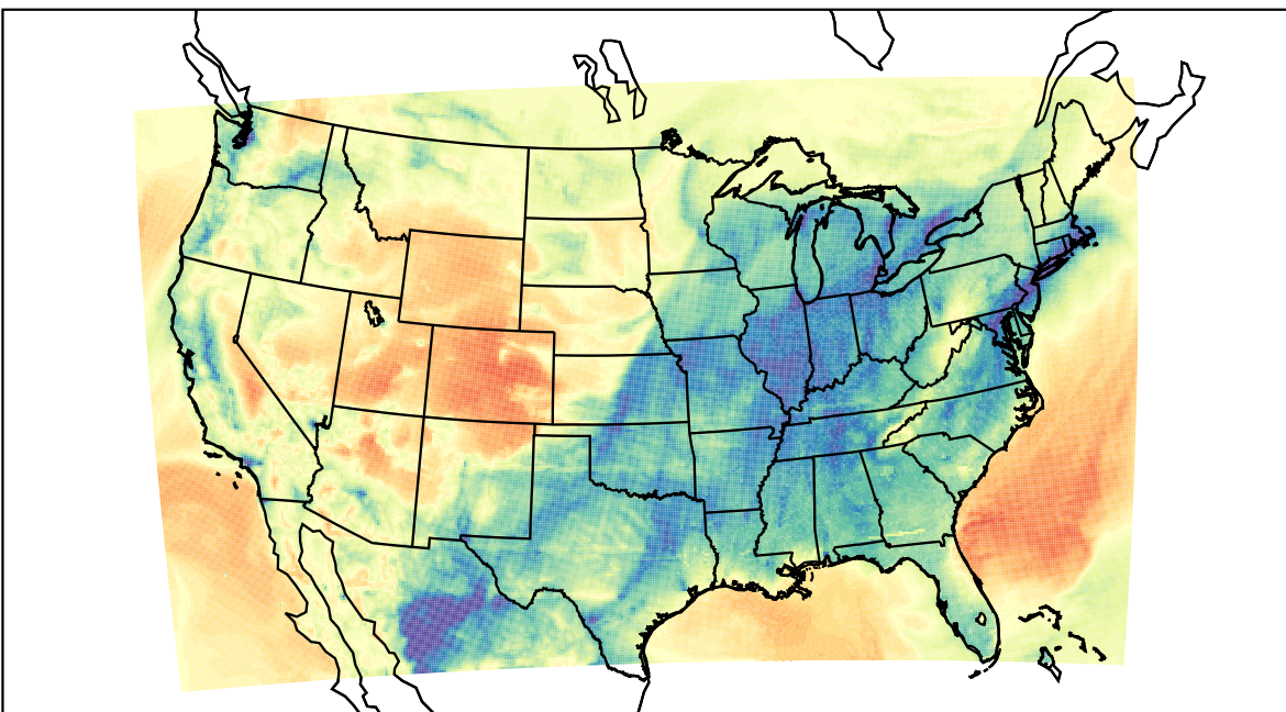
WRF (2023-02-19_08:00:00)
