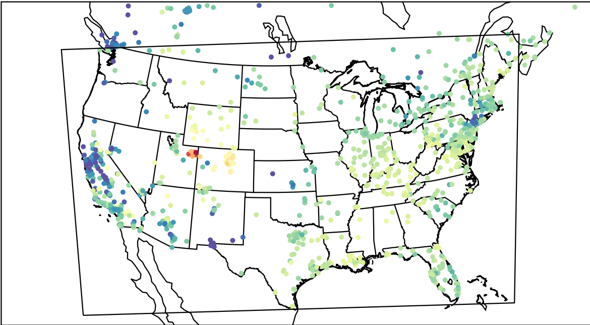
AirNOW (2023-02-19_17:00:00)
