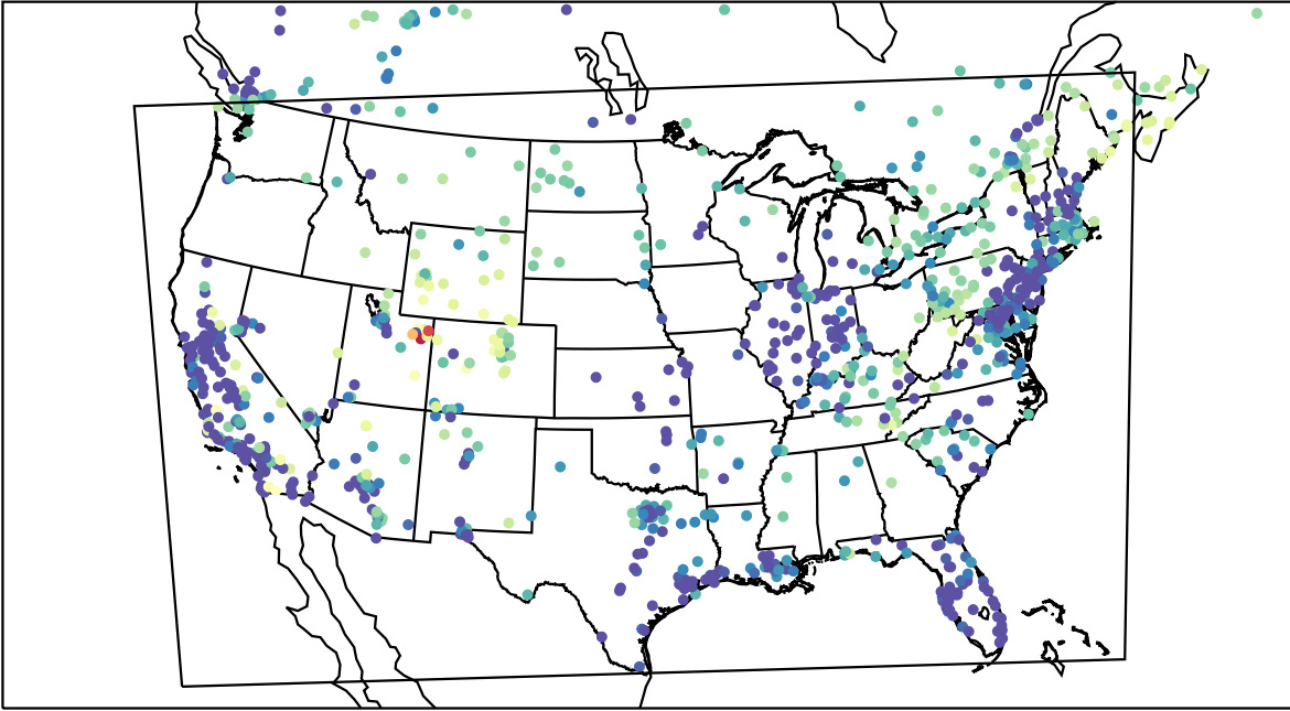
AirNOW (2023-02-20_13:00:00)
