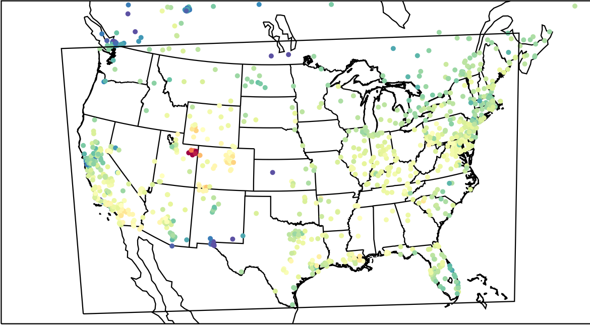
AirNOW (2023-02-19_20:00:00)
