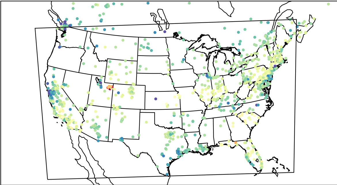
AirNOW (2023-02-20_19:00:00)
