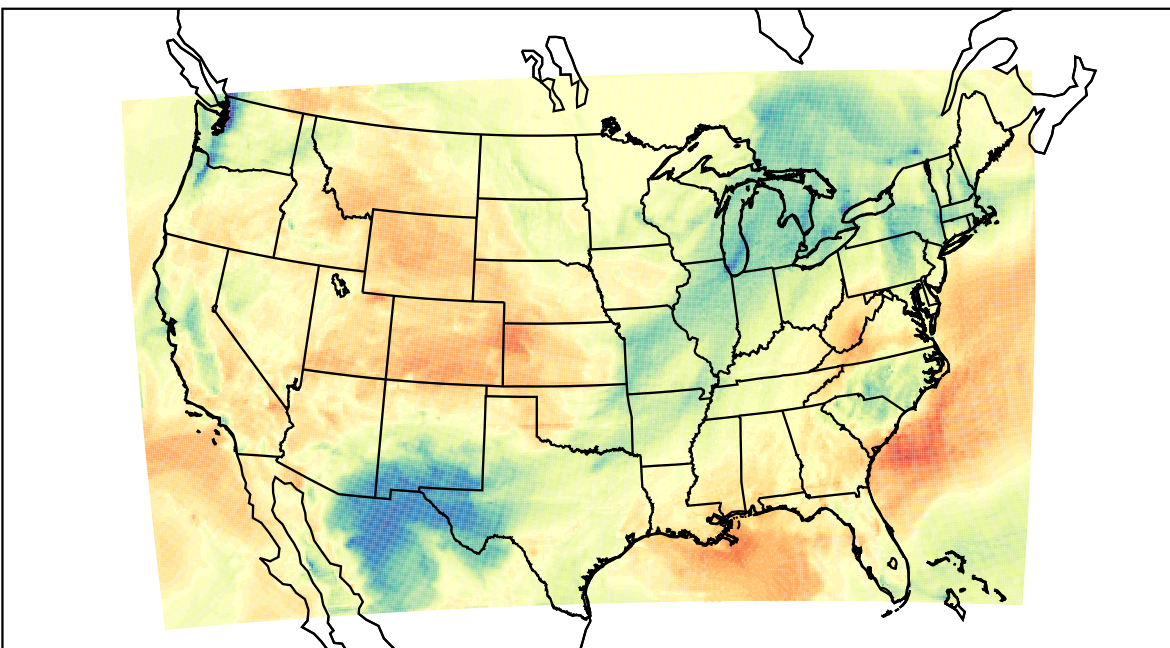
WRF (2023-02-19_20:00:00)
