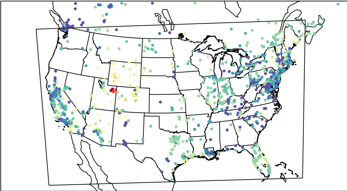
AirNOW (2023-02-19_02:00:00)
