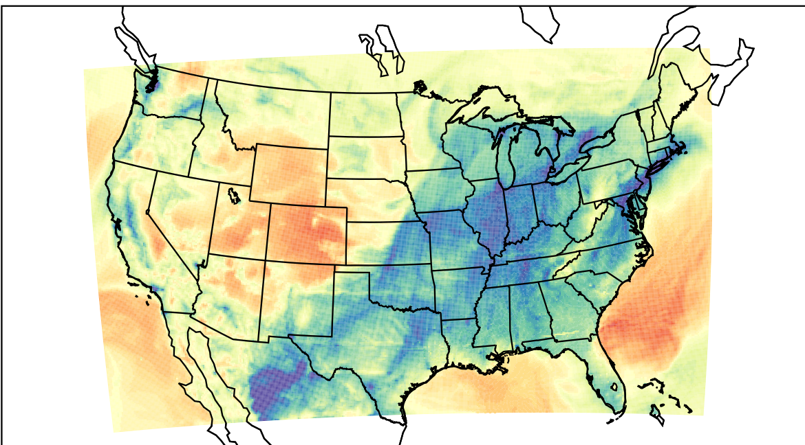
WRF (2023-02-19_09:00:00)
