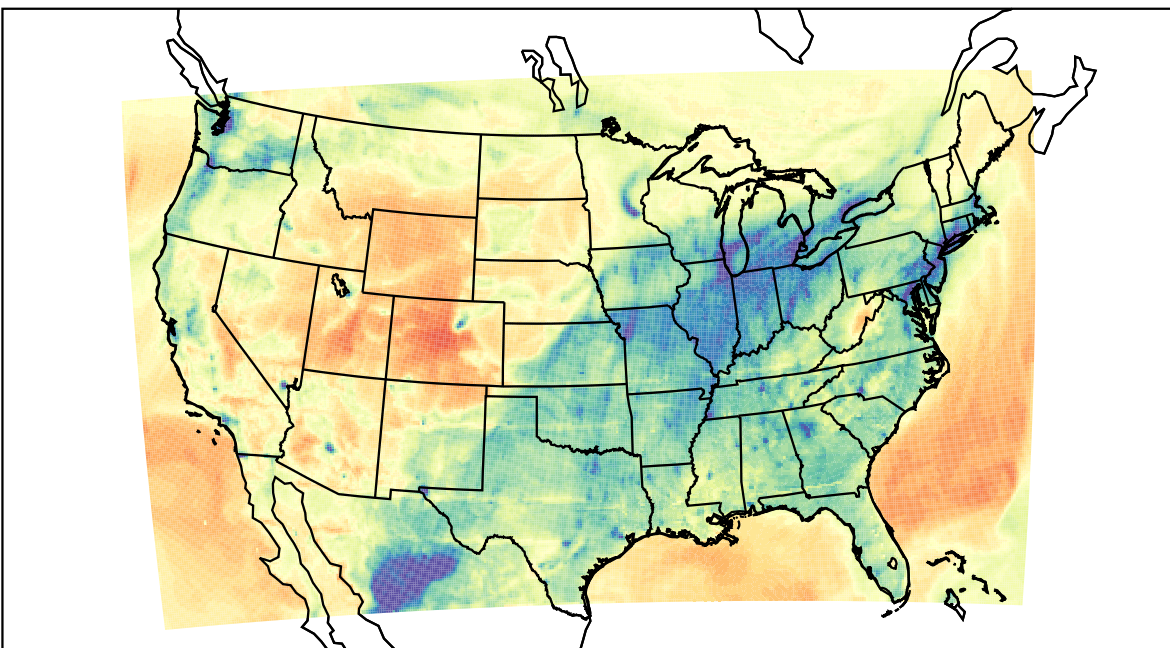
WRF (2023-02-19_02:00:00)
