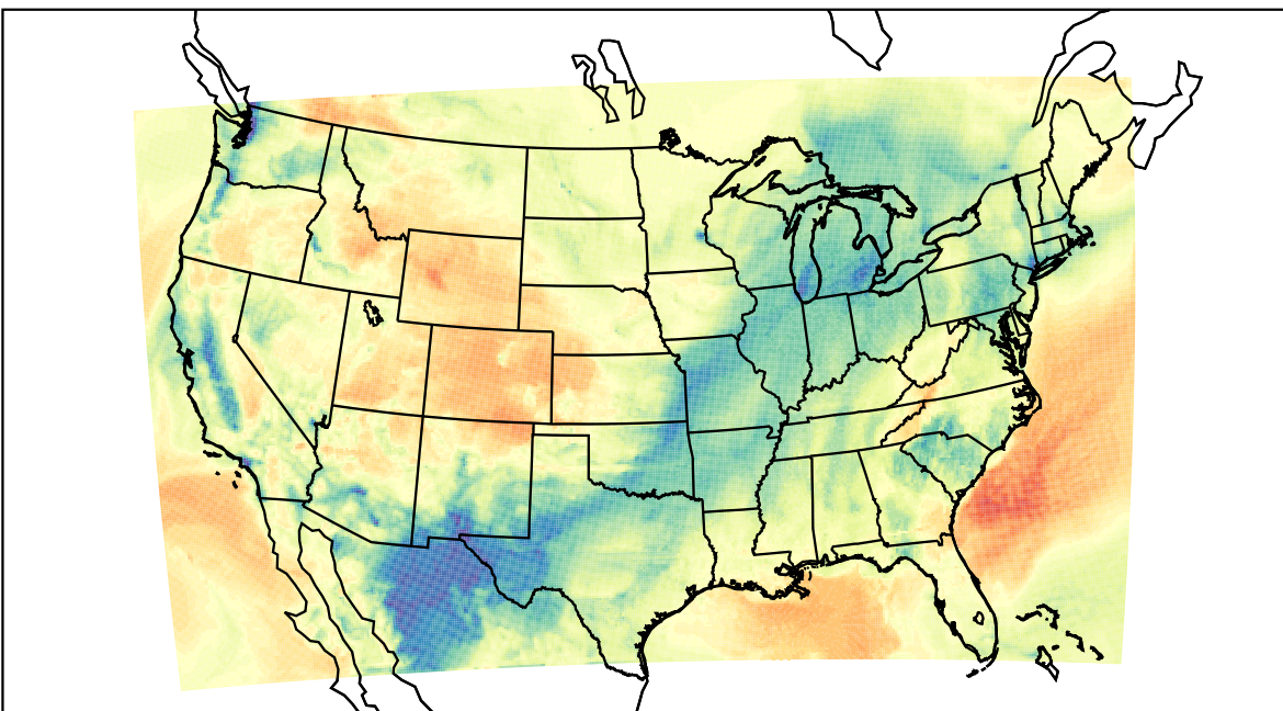
WRF (2023-02-19_17:00:00)
