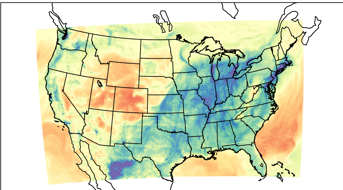
WRF (2023-02-19_05:00:00)
