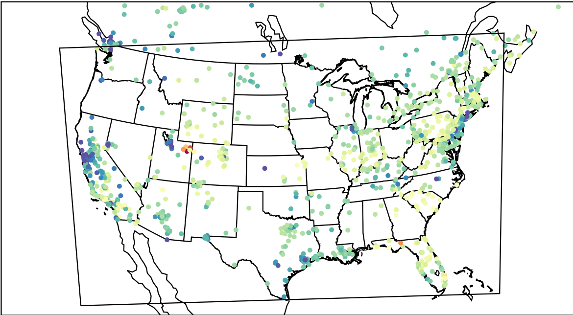
AirNOW (2023-02-20_18:00:00)
