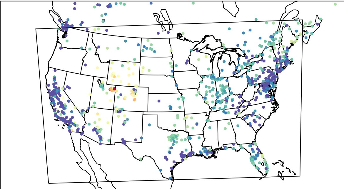
AirNOW (2023-02-19_07:00:00)
