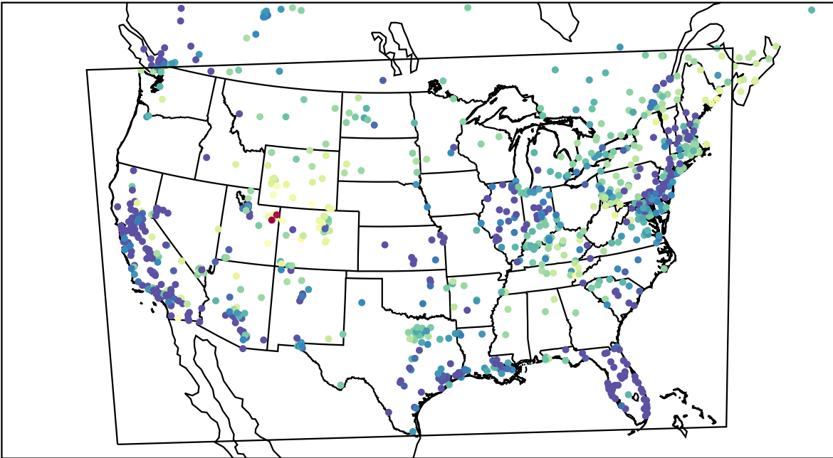
AirNOW (2023-02-20_10:00:00)
