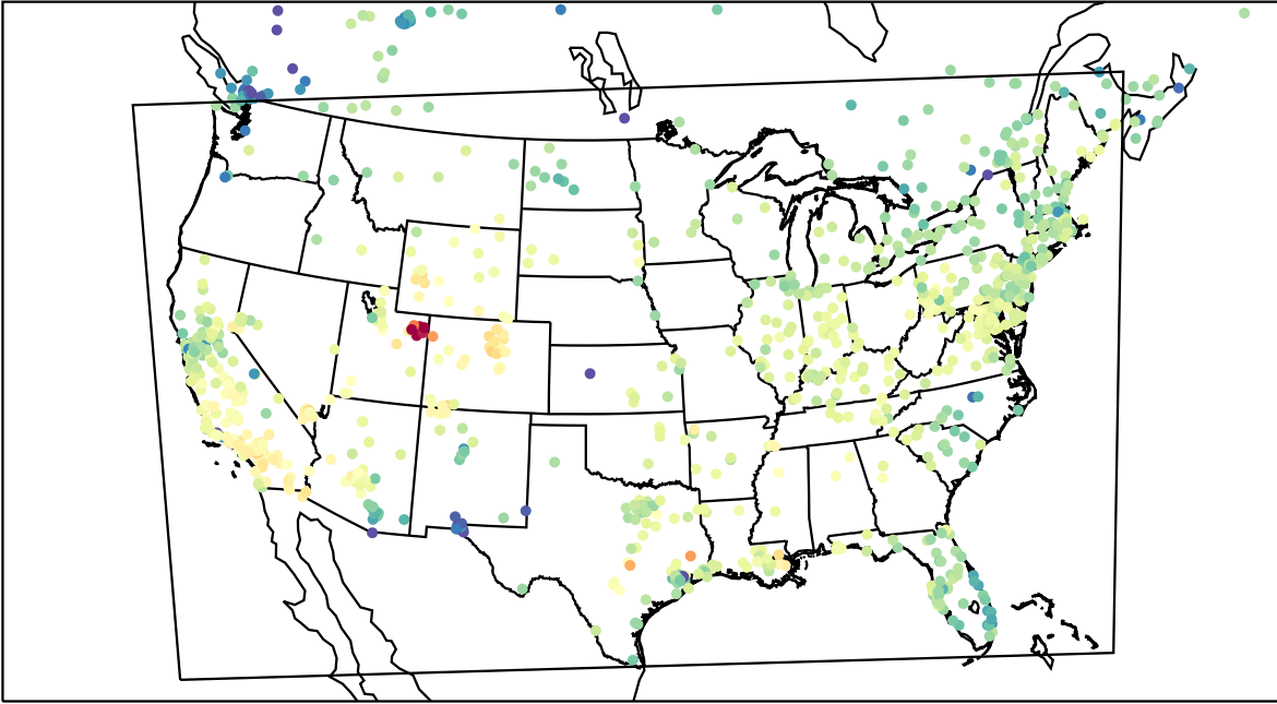
AirNOW (2023-02-19_22:00:00)
