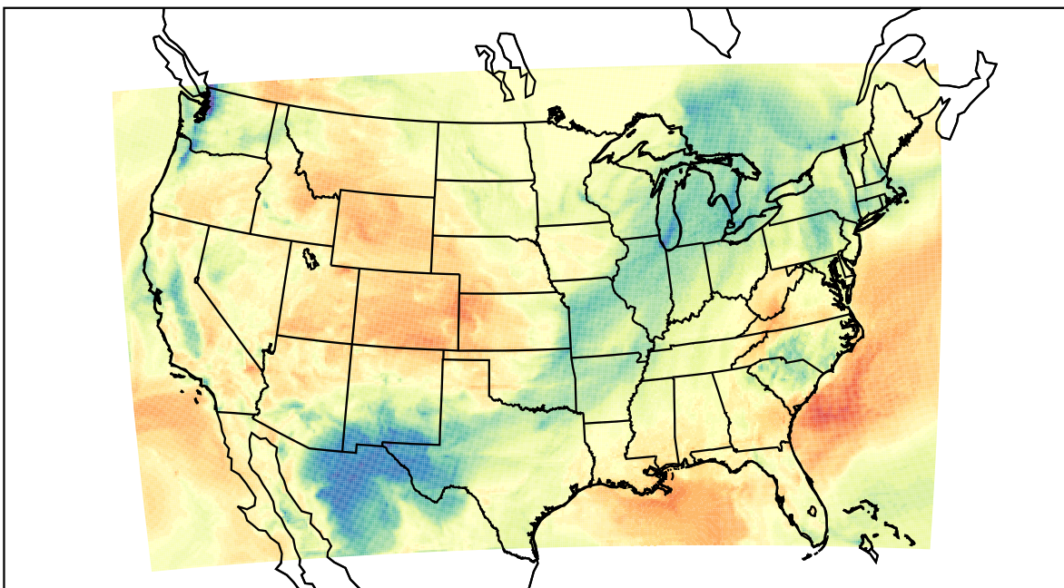
WRF (2023-02-19_19:00:00)
