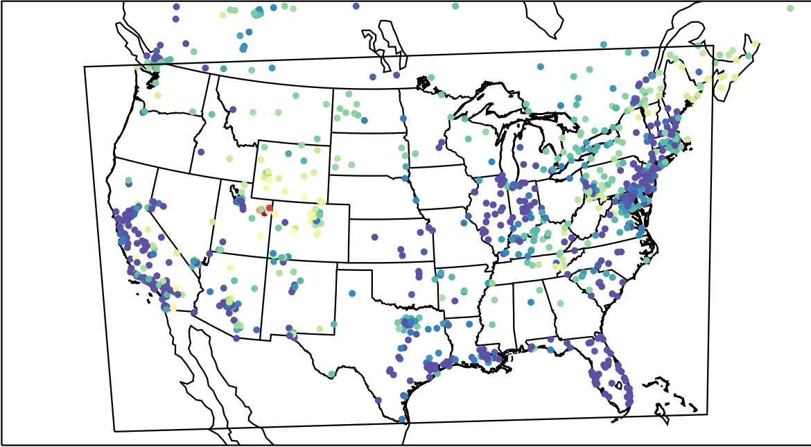
AirNOW (2023-02-20_12:00:00)
