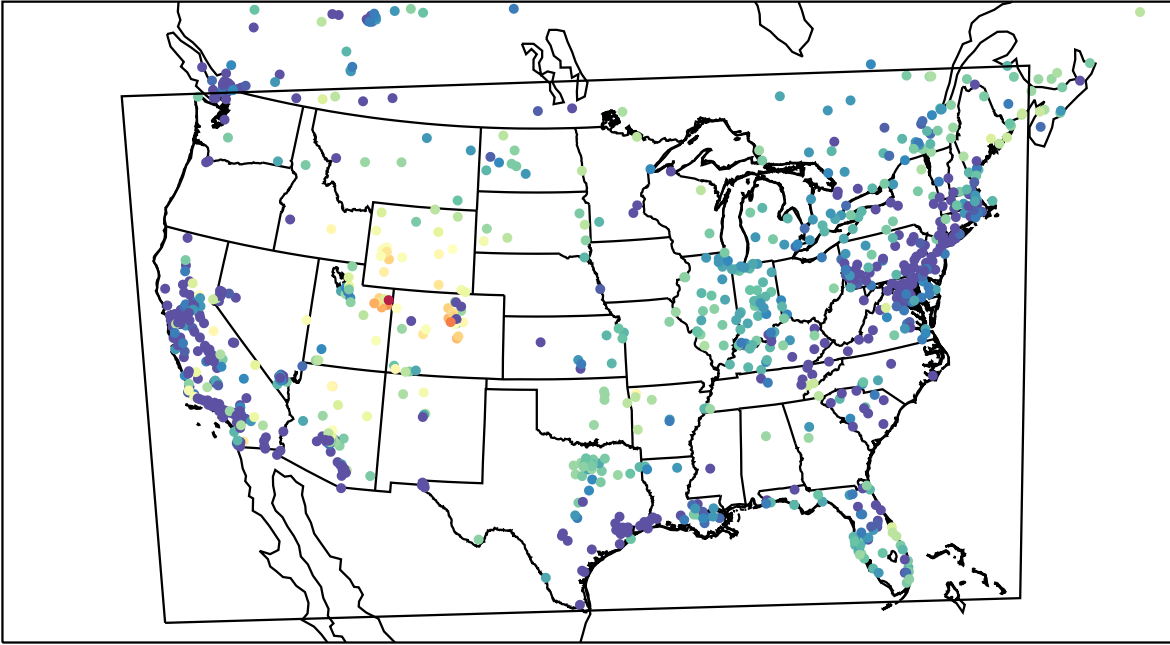
AirNOW (2023-02-19_08:00:00)
