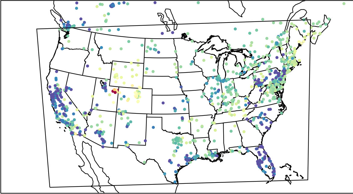
AirNOW (2023-02-20_04:00:00)
