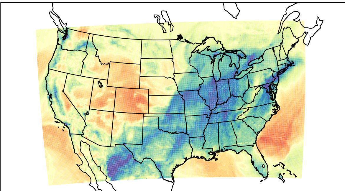
WRF (2023-02-19_10:00:00)
