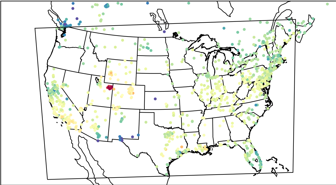
AirNOW (2023-02-19_21:00:00)
