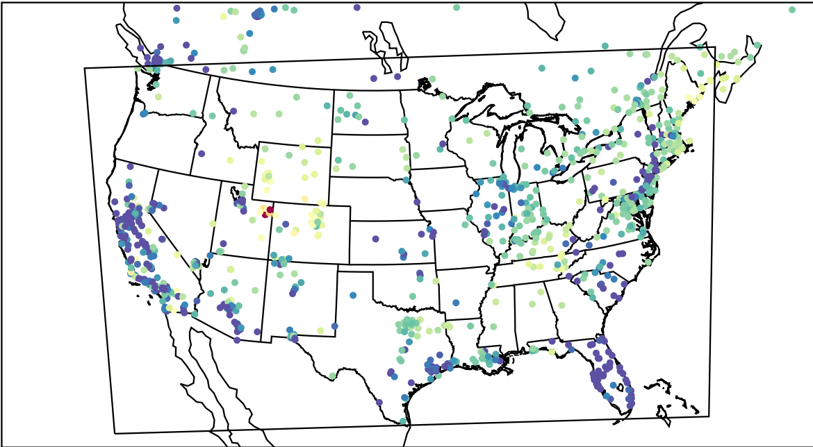
AirNOW (2023-02-20_06:00:00)
