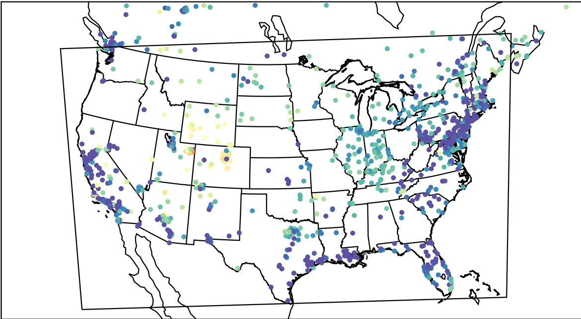
AirNOW (2023-02-19_12:00:00)
