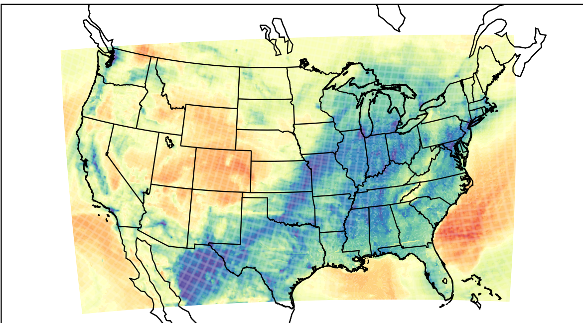
WRF (2023-02-19_14:00:00)
