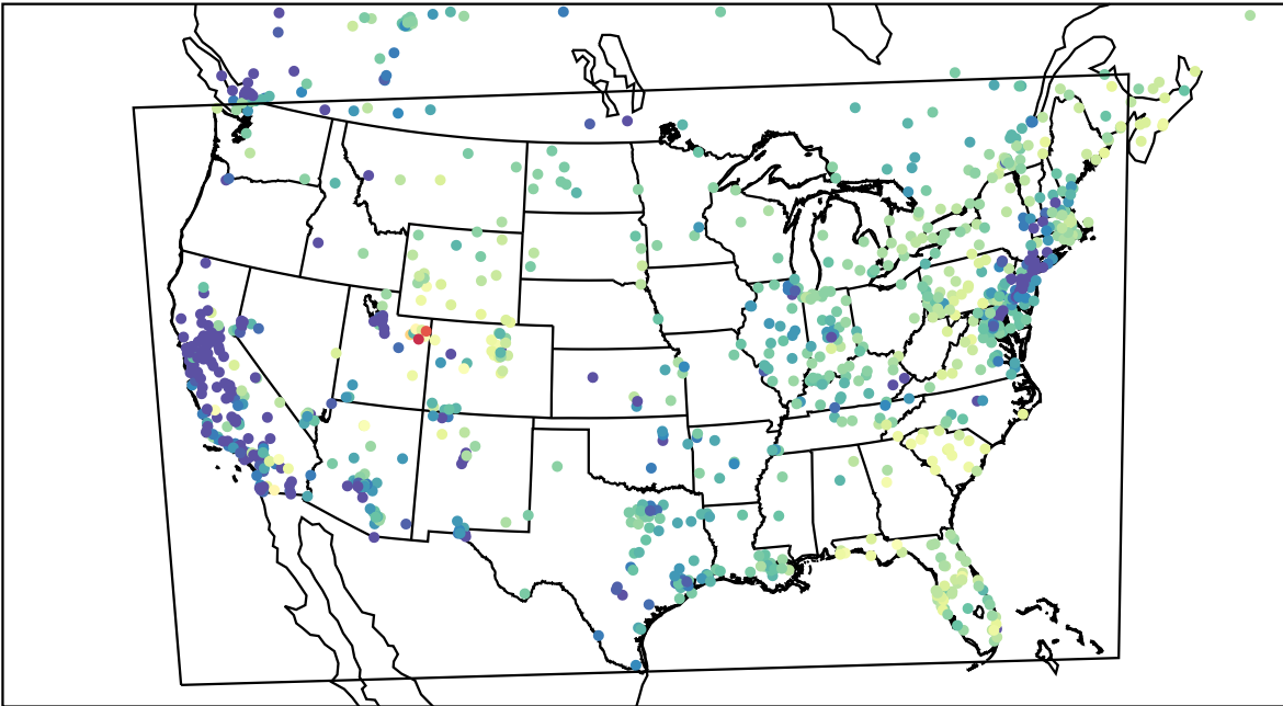
AirNOW (2023-02-20_16:00:00)
