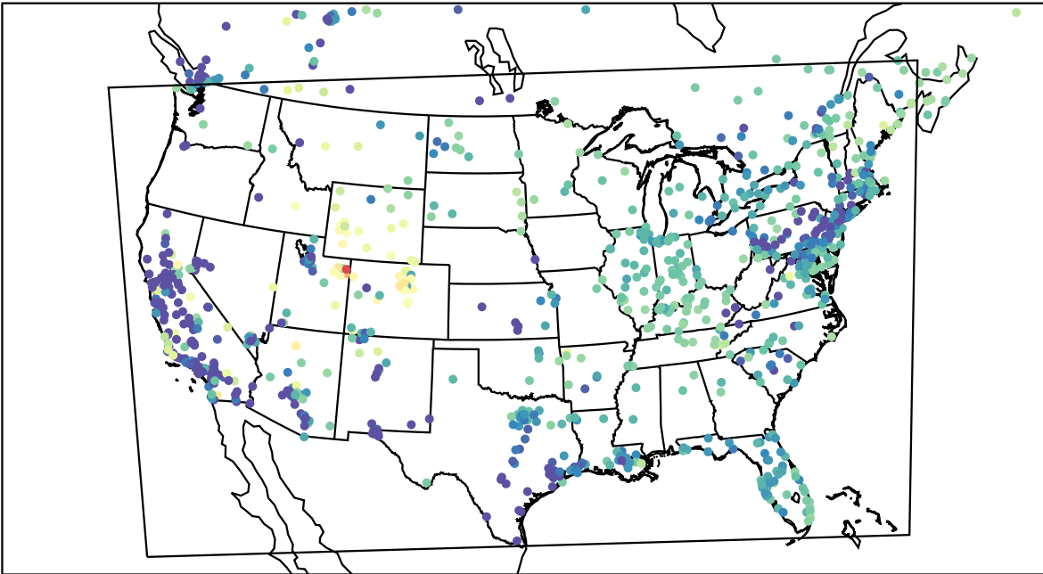
AirNOW (2023-02-19_14:00:00)
