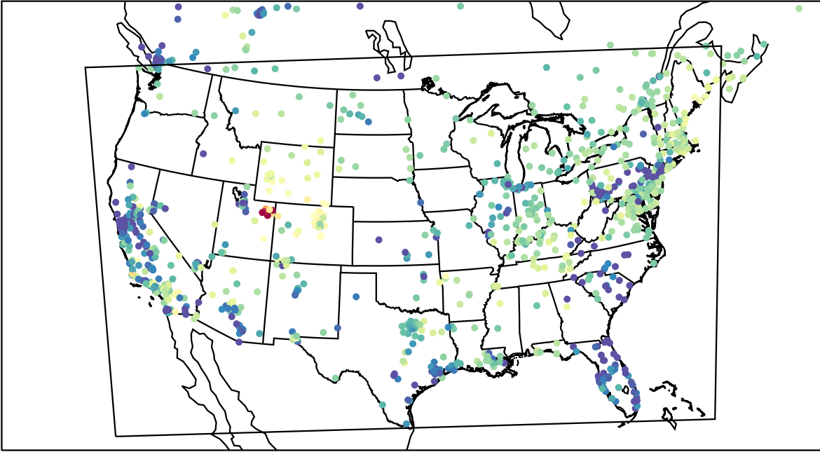
AirNOW (2023-02-20_03:00:00)
