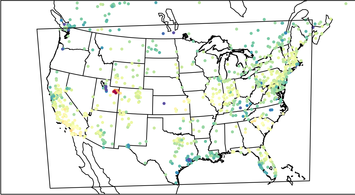
AirNOW (2023-02-20_21:00:00)
