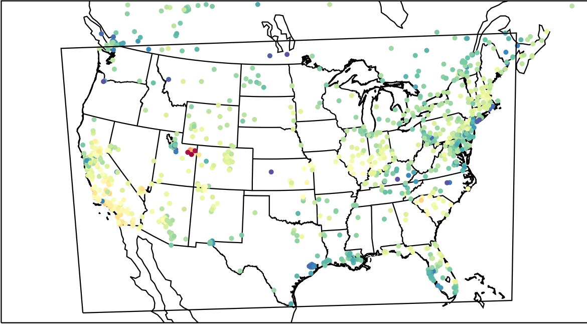
AirNOW (2023-02-20_22:00:00)
