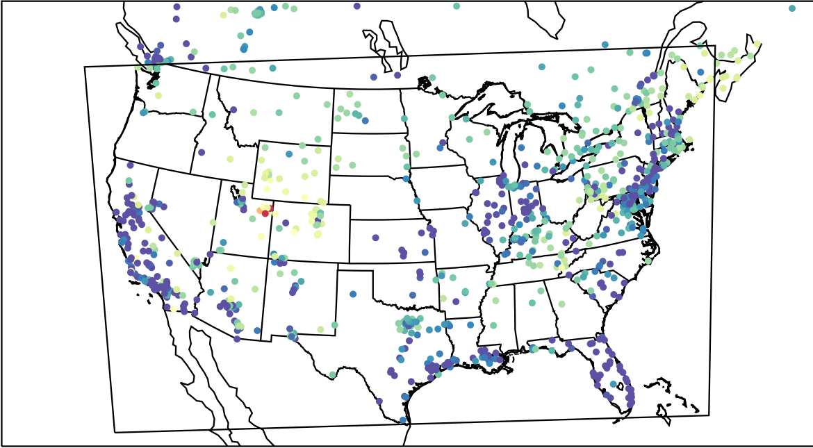
AirNOW (2023-02-20_11:00:00)
