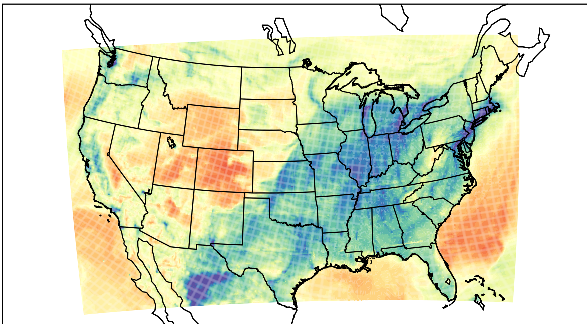
WRF (2023-02-19_06:00:00)
