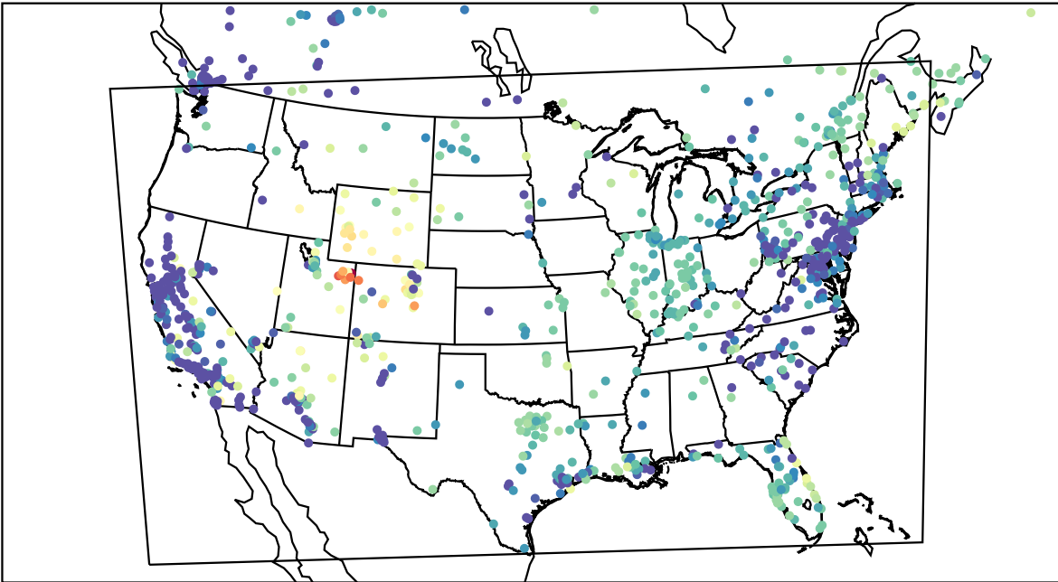
AirNOW (2023-02-19_05:00:00)
