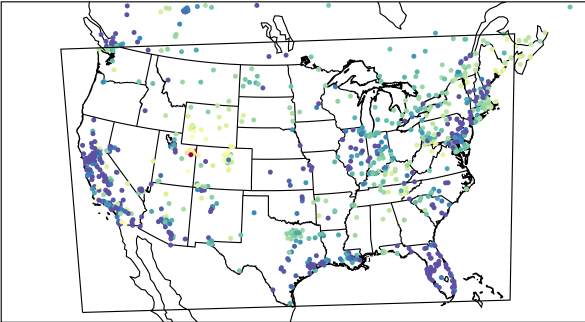
AirNOW (2023-02-20_09:00:00)
