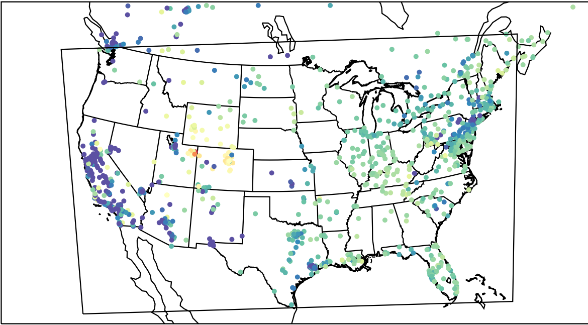
AirNOW (2023-02-19_15:00:00)
