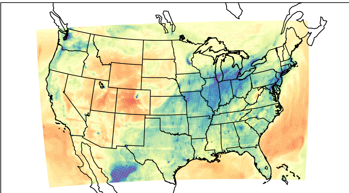
WRF (2023-02-19_01:00:00)
