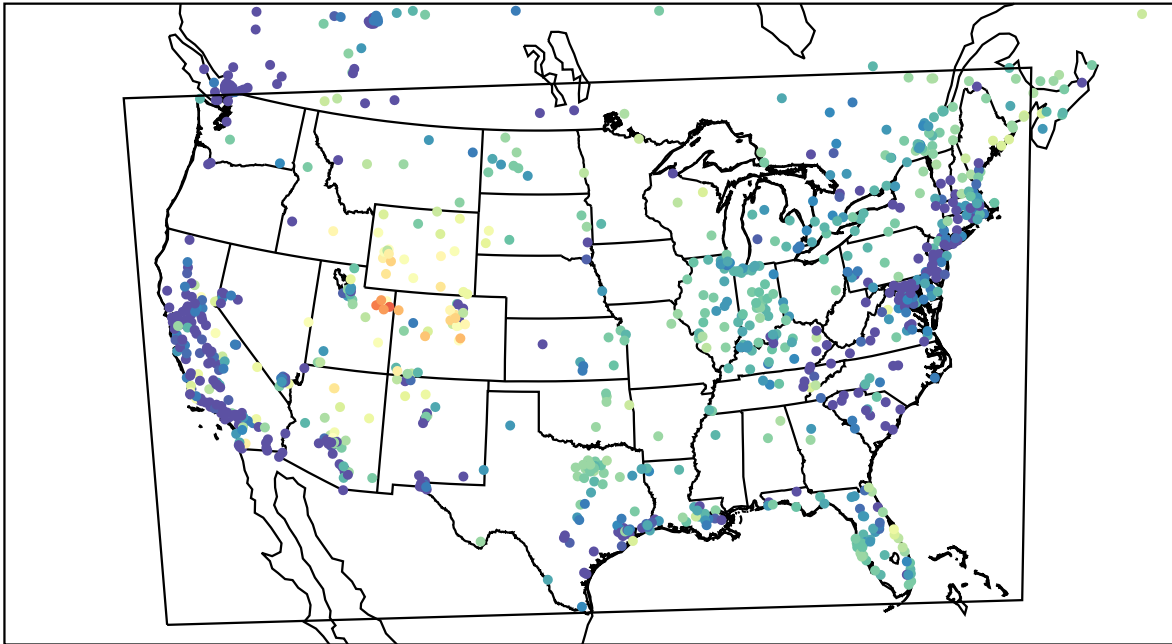
AirNOW (2023-02-19_06:00:00)
