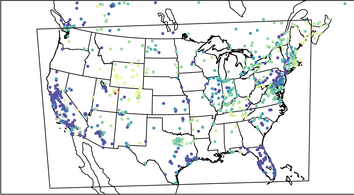
AirNOW (2023-02-20_07:00:00)
