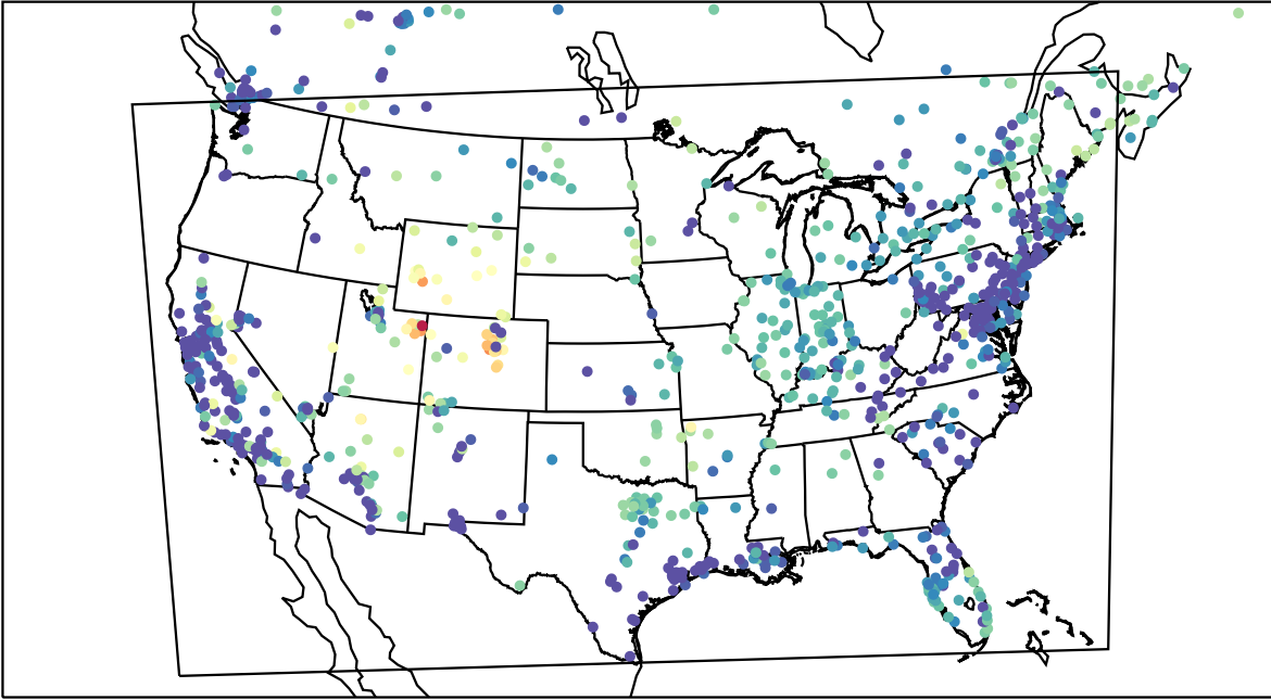
AirNOW (2023-02-19_09:00:00)
