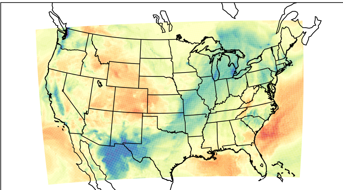
WRF (2023-02-19_18:00:00)
