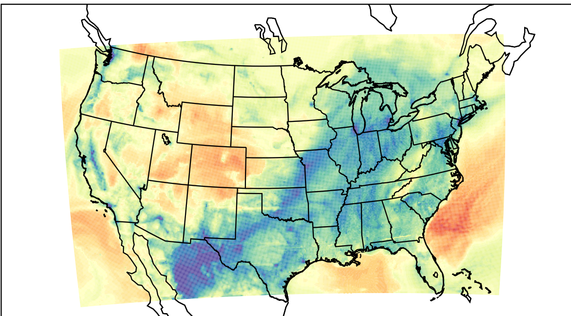
WRF (2023-02-19_15:00:00)
