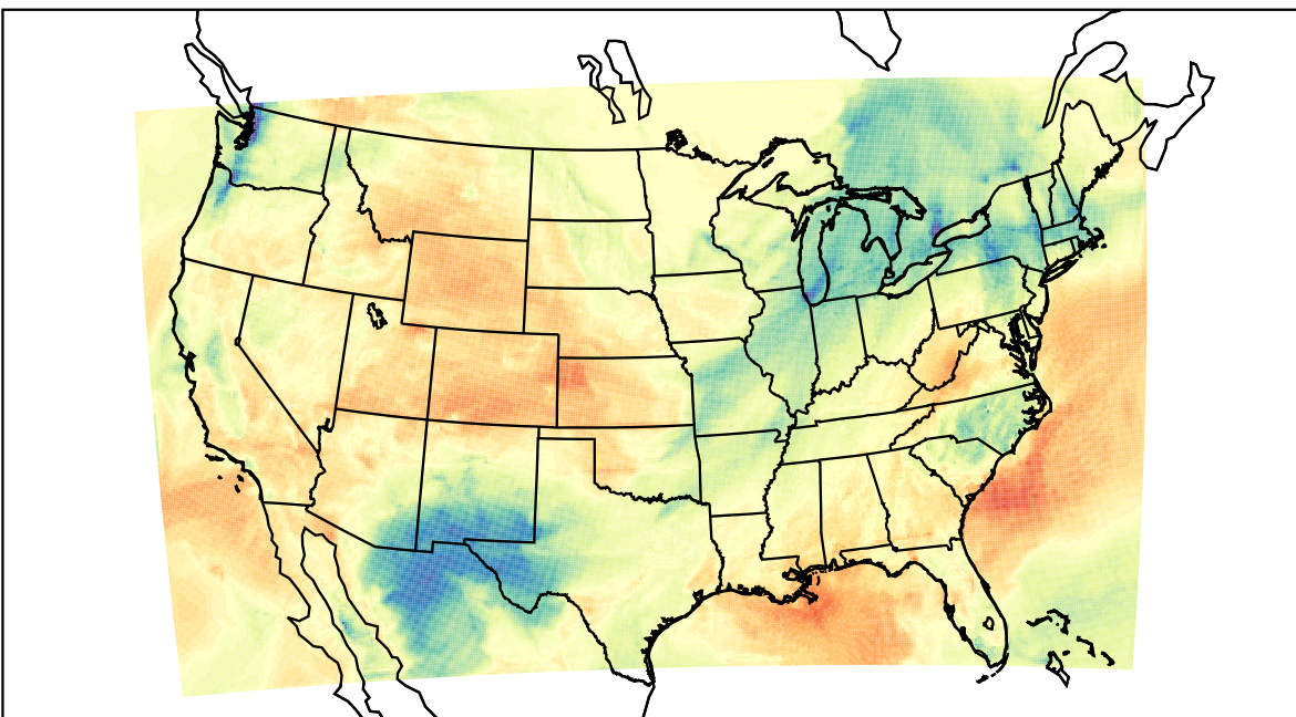
WRF (2023-02-19_21:00:00)
