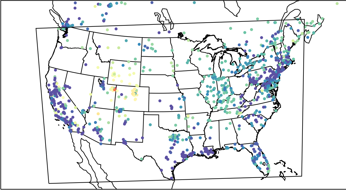
AirNOW (2023-02-19_13:00:00)
