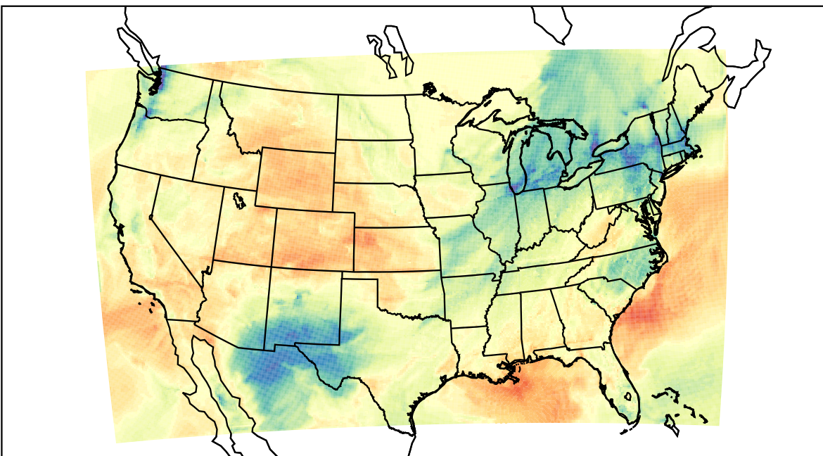
WRF (2023-02-19_22:00:00)
