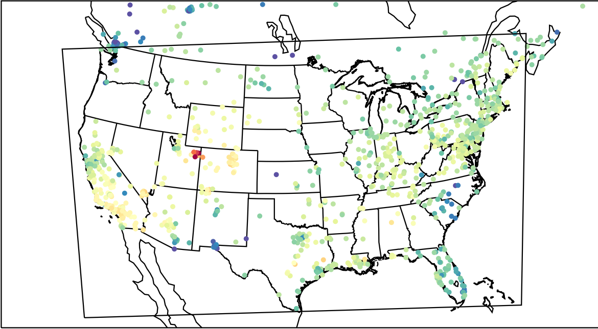
AirNOW (2023-02-19_23:00:00)
