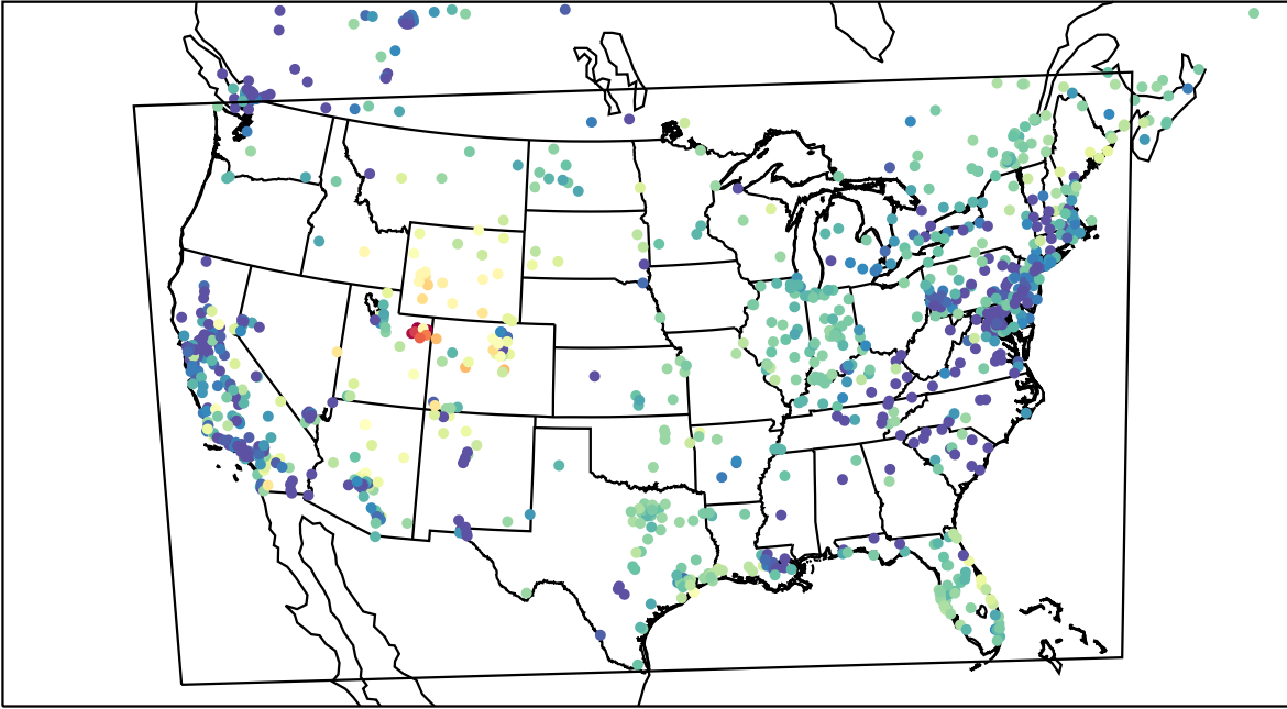
AirNOW (2023-02-19_03:00:00)
