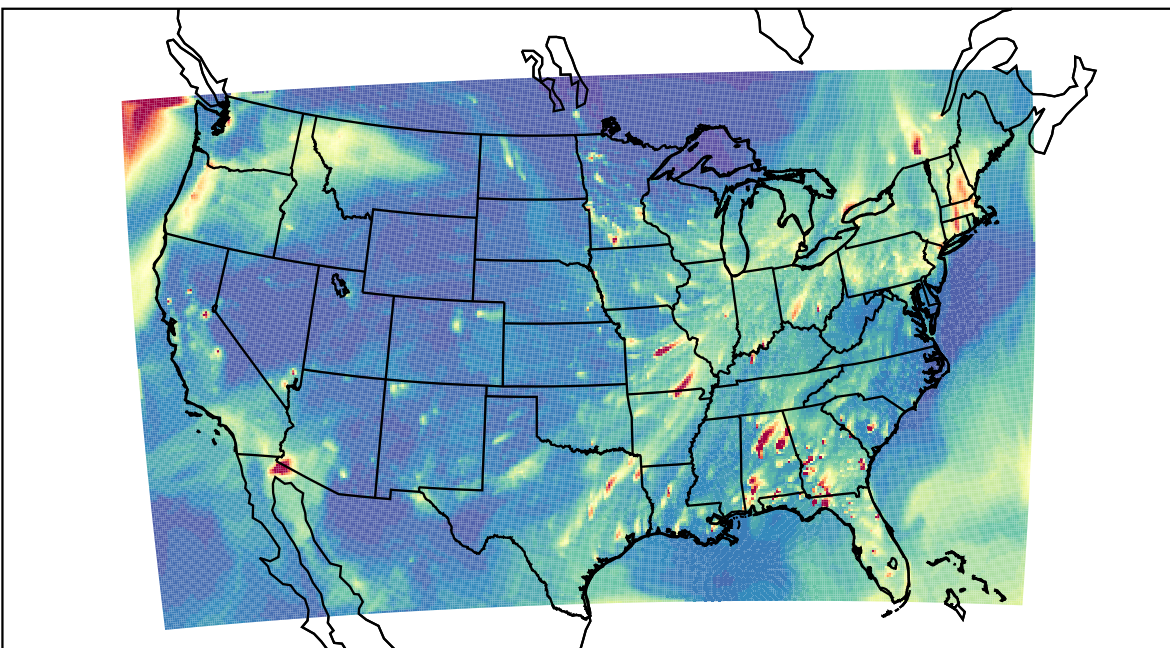
WRF 2023-02-20_02:00:00
