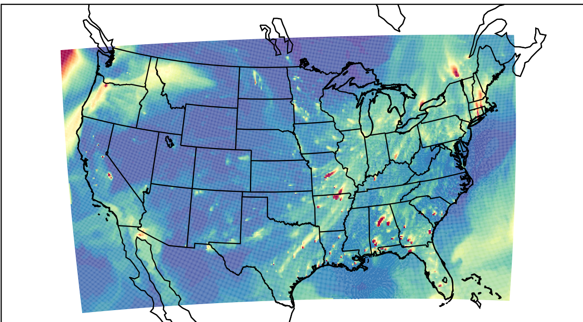
WRF 2023-02-20_00:00:00
