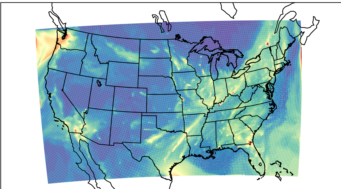
WRF 2023-02-20_12:00:00
