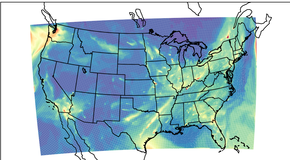
WRF 2023-02-20_13:00:00
