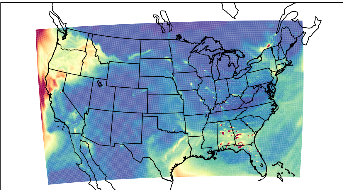
WRF 2023-02-21_21:00:00
