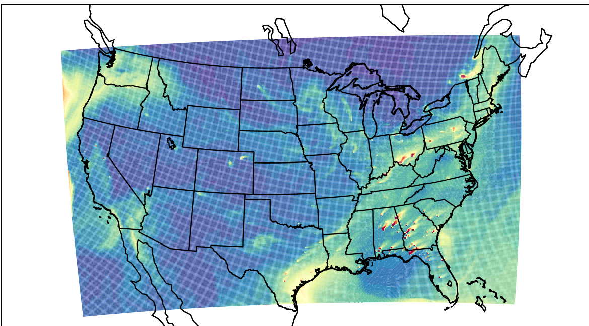
WRF 2023-02-20_21:00:00
