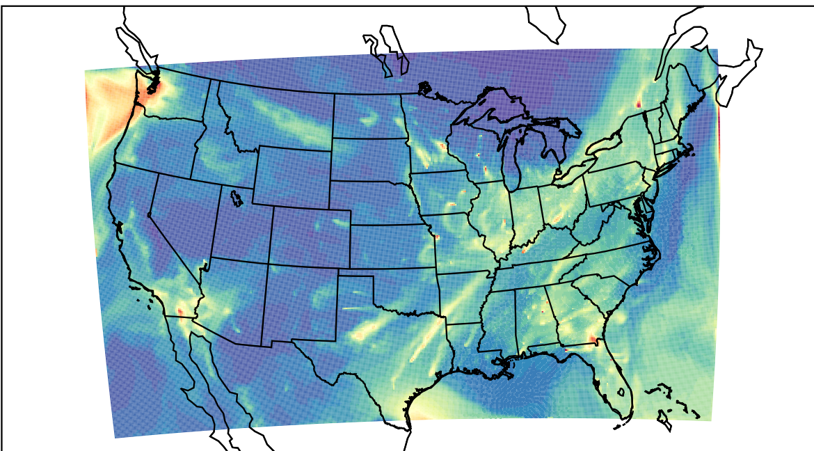
WRF 2023-02-20_11:00:00
