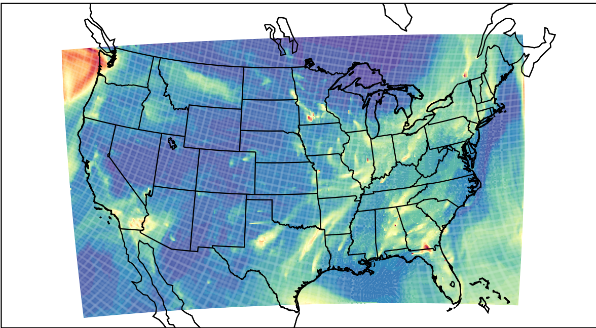
WRF 2023-02-20_08:00:00
