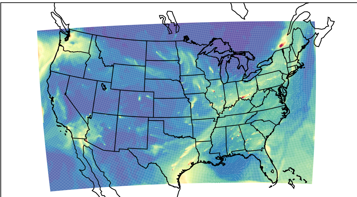
WRF 2023-02-20_17:00:00
