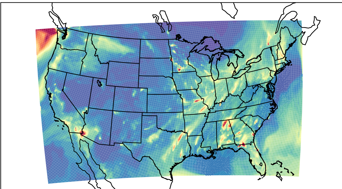
WRF 2023-02-20_05:00:00
