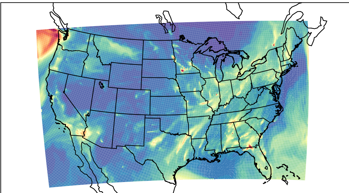
WRF 2023-02-20_07:00:00
