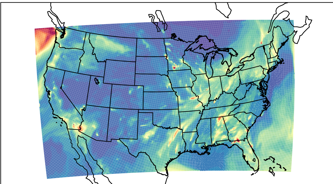
WRF 2023-02-20_06:00:00
