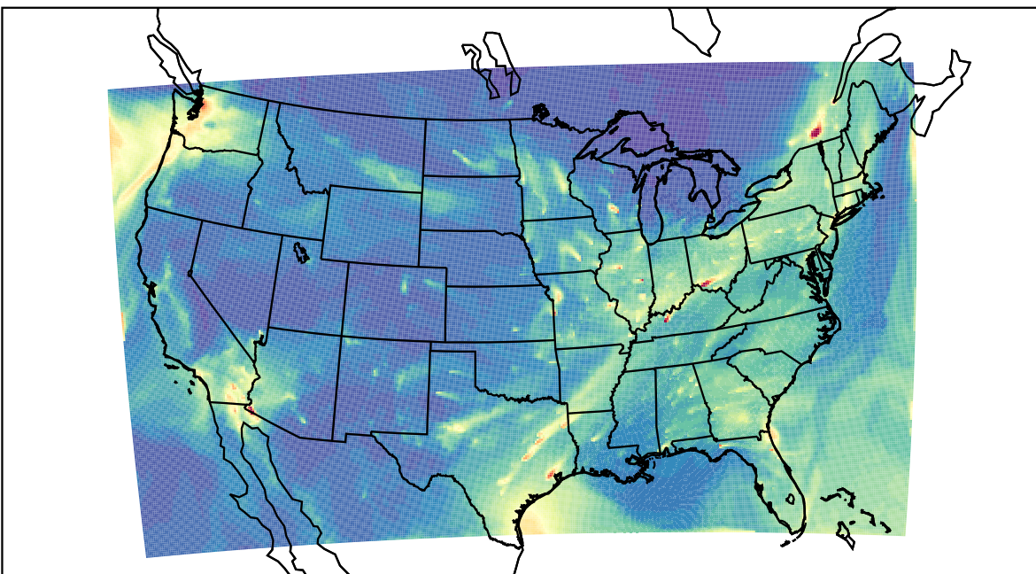
WRF 2023-02-20_15:00:00
