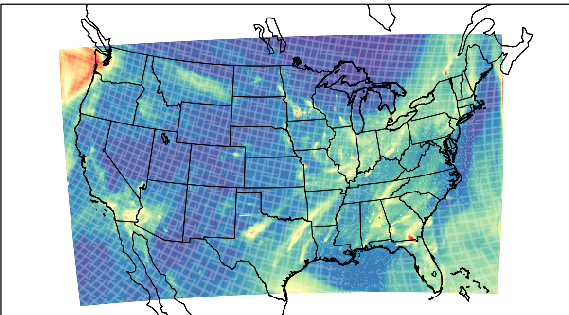
WRF 2023-02-20_09:00:00
