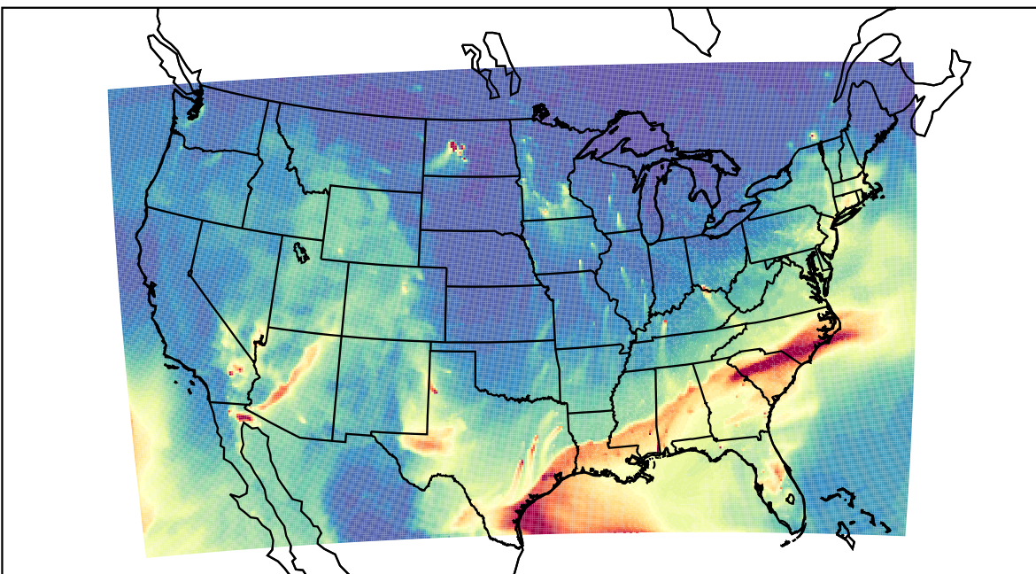
WRF 2023-02-24_10:00:00
