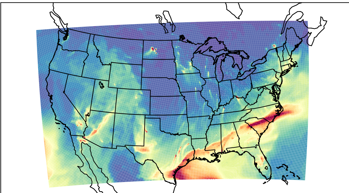
WRF 2023-02-24_11:00:00
