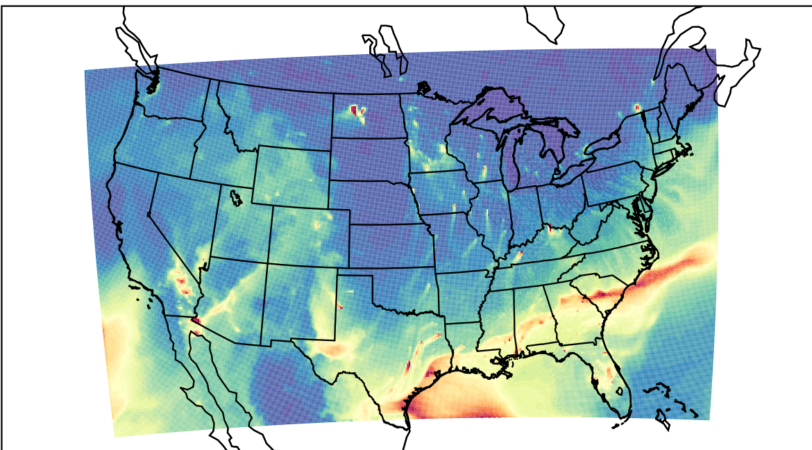
WRF 2023-02-24_14:00:00
