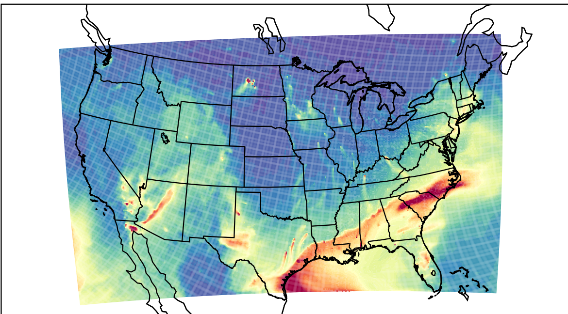
WRF 2023-02-24_09:00:00
