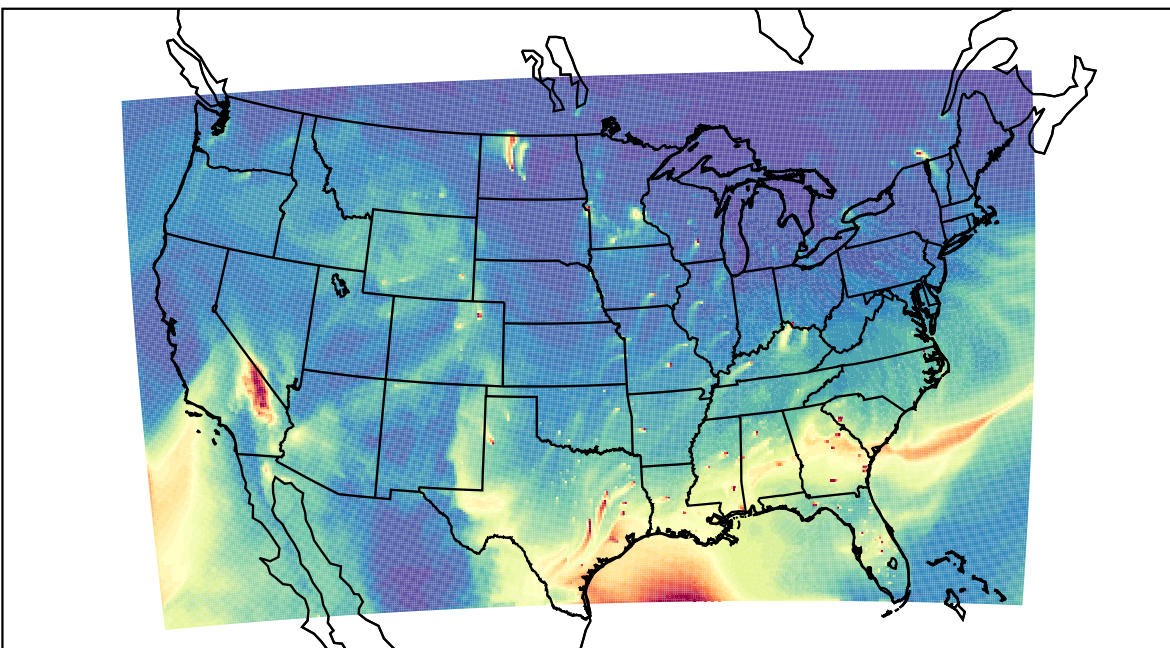
WRF 2023-02-24_19:00:00
