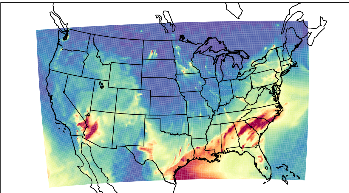
WRF 2023-02-24_05:00:00
