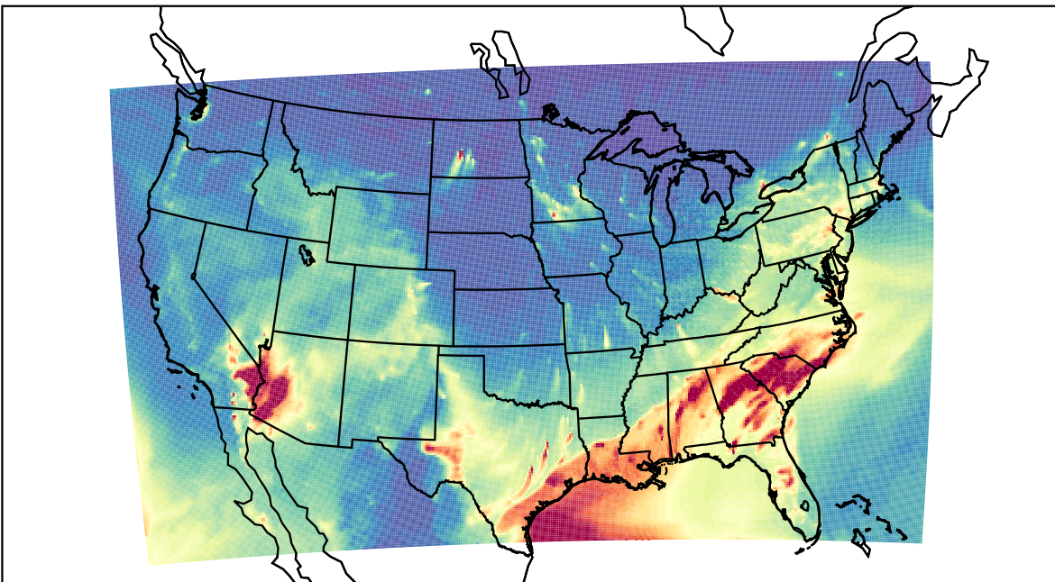
WRF 2023-02-24_04:00:00
