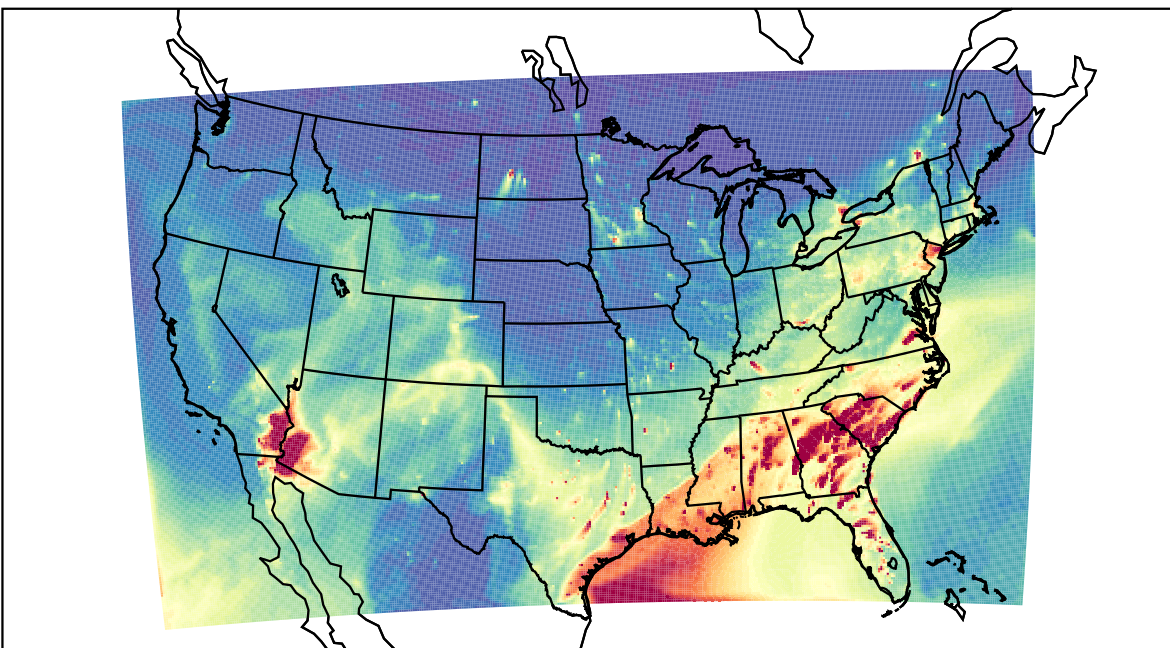
WRF 2023-02-24_01:00:00
