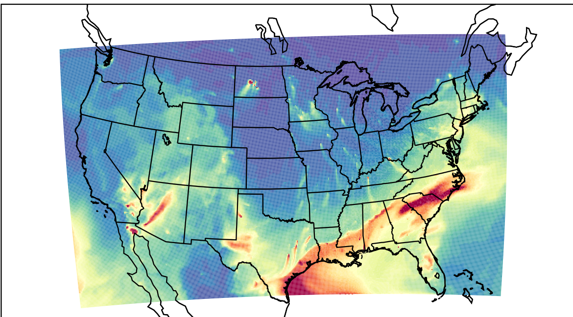
WRF 2023-02-24_08:00:00
