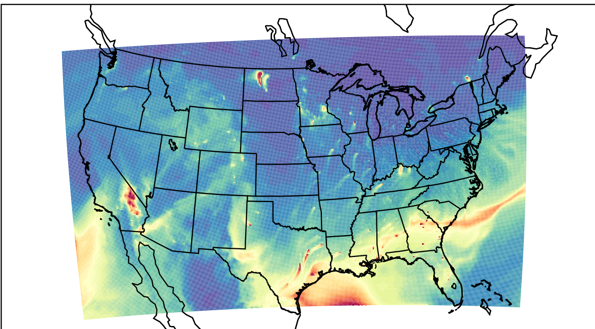
WRF 2023-02-24_17:00:00
