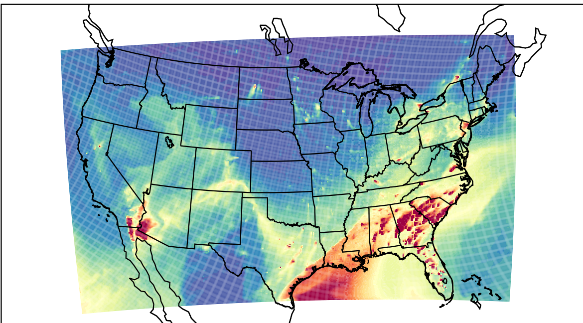
WRF 2023-02-24_00:00:00
