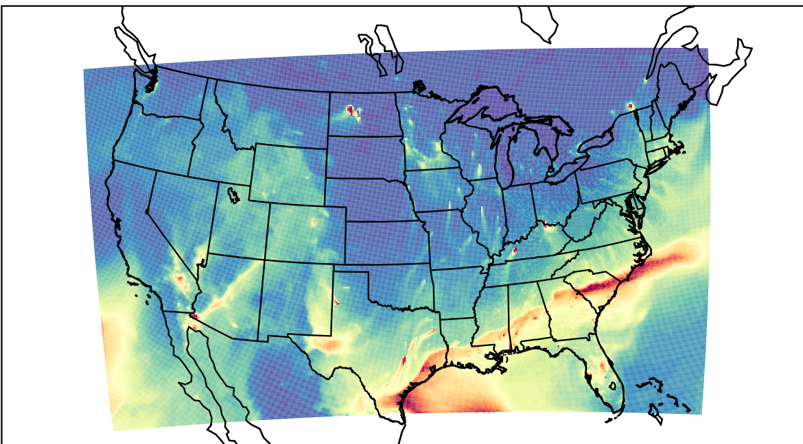
WRF 2023-02-24_13:00:00
