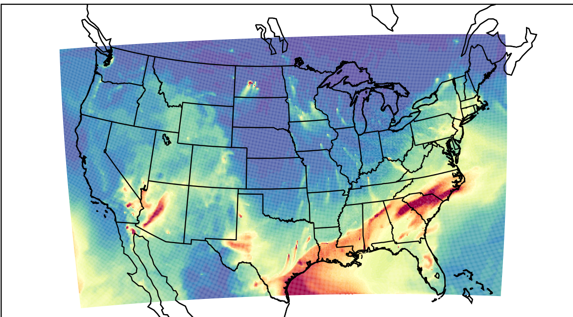
WRF 2023-02-24_07:00:00
