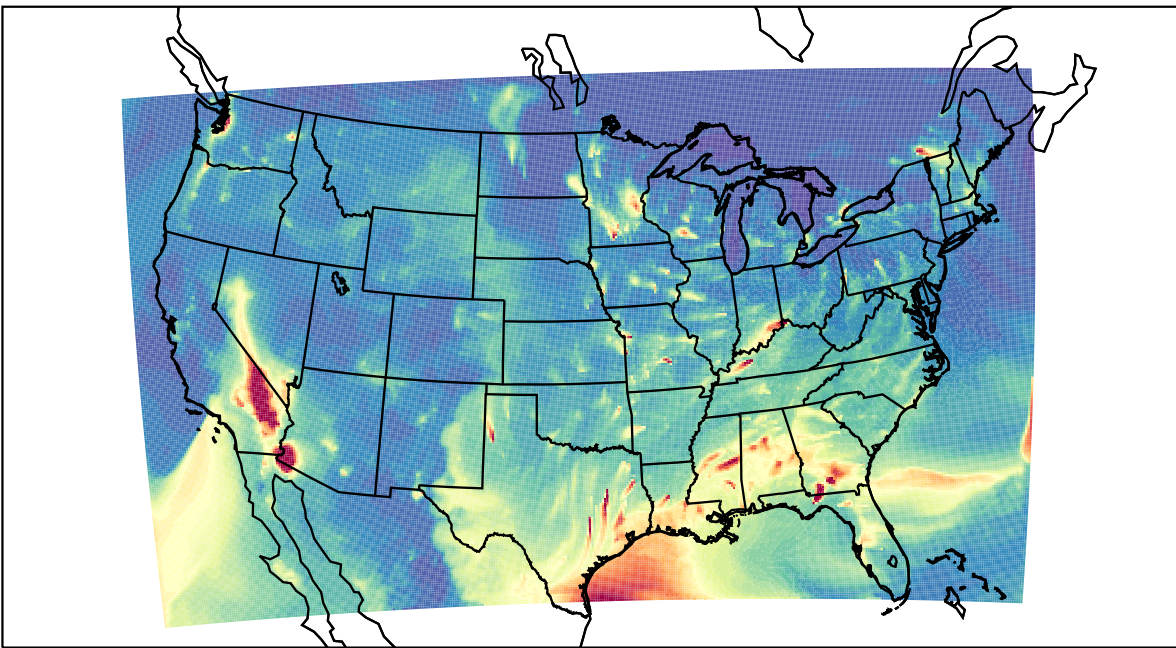
WRF 2023-02-25_04:00:00
