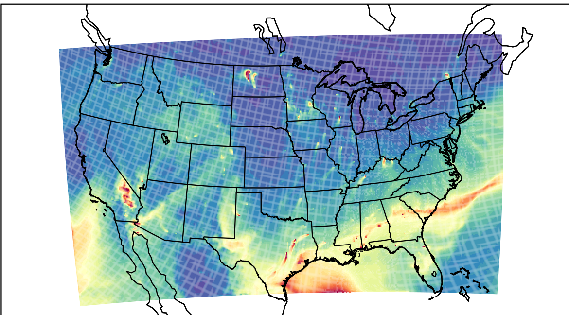
WRF 2023-02-24_16:00:00
