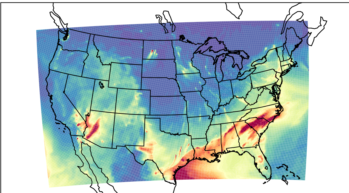
WRF 2023-02-24_06:00:00
