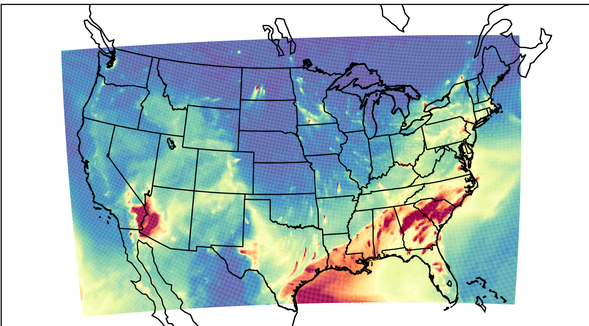
WRF 2023-02-24_03:00:00
