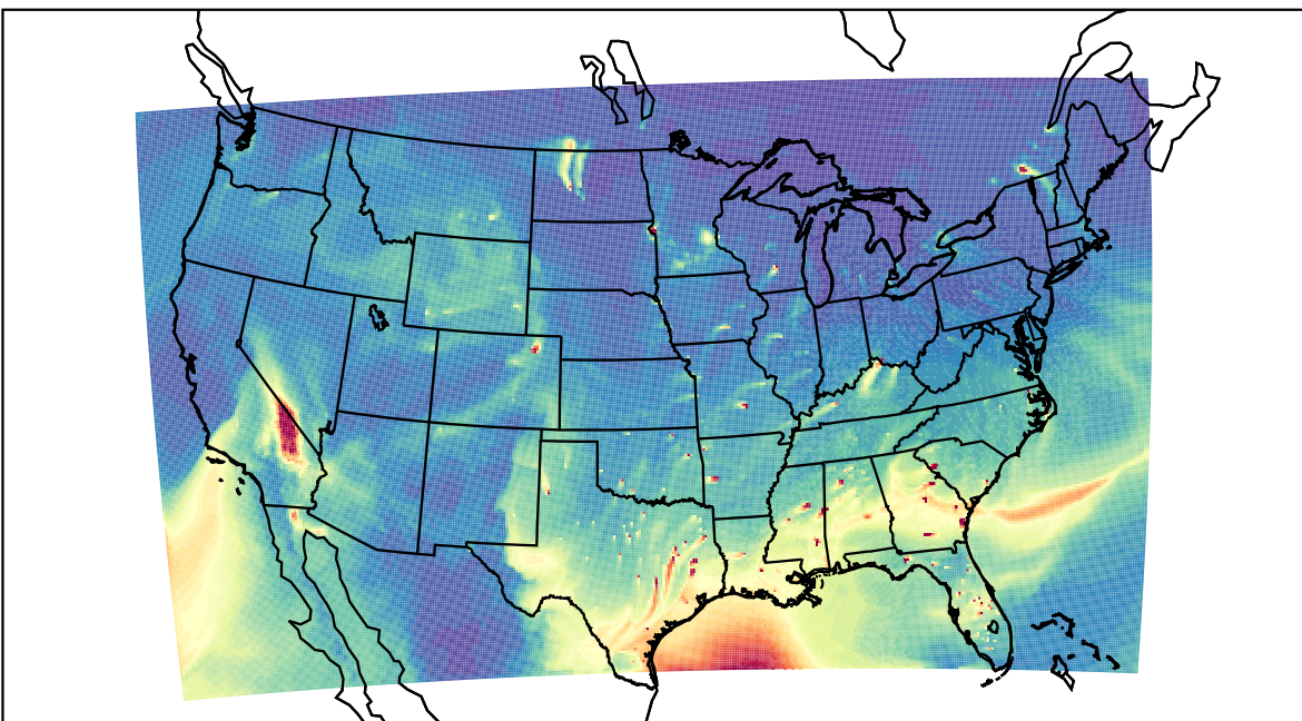
WRF 2023-02-24_21:00:00
