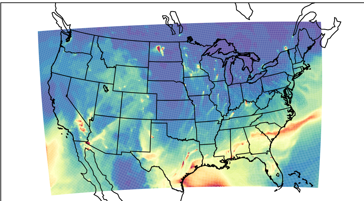
WRF 2023-02-24_15:00:00
