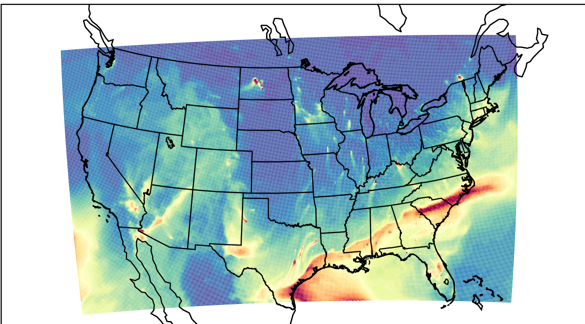
WRF 2023-02-24_12:00:00
